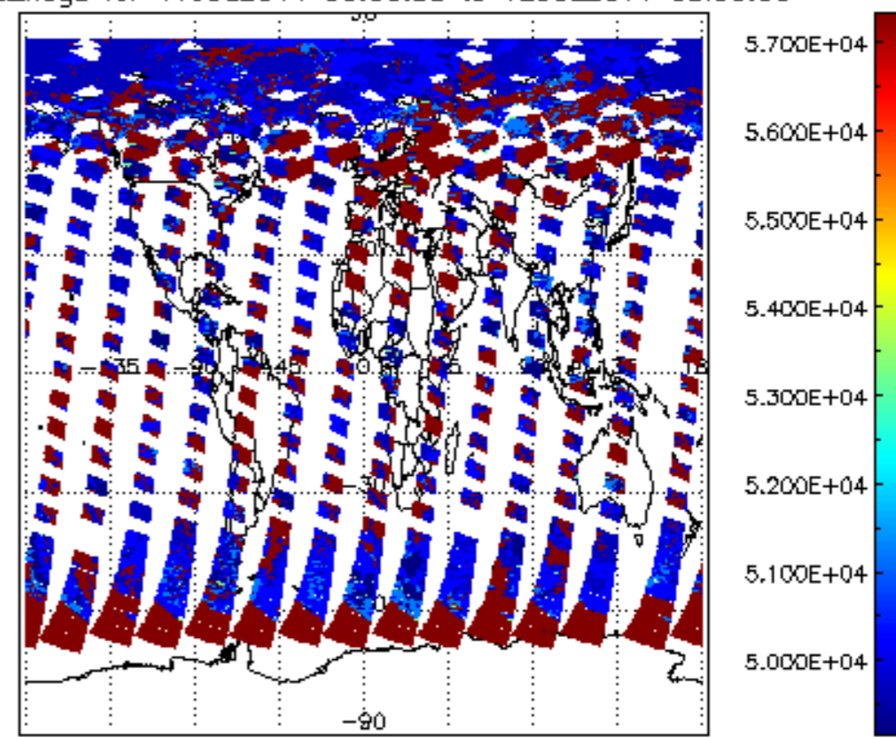
cloud_flags for 11JUL2011 00:00:00 to 12JUL2011 00:00:00
