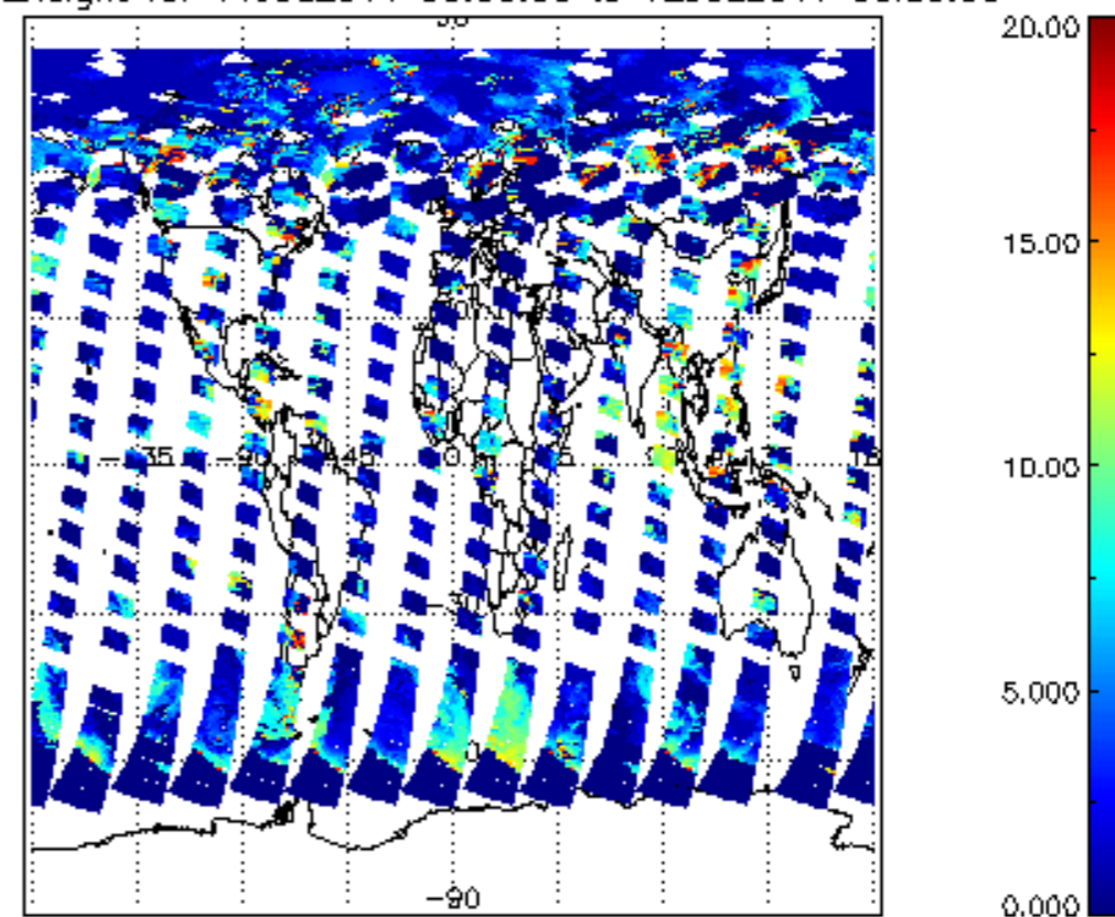
cl_top_height for 11JUL2011 00:00:00 to 12JUL2011 00:00:00
