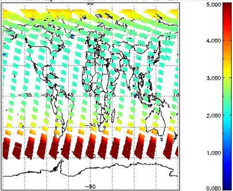
SCIOL2P_NADUV1NO2_amf_gr for 11JUL2011 00:00:00 to 12JUL2011 00:00:00
