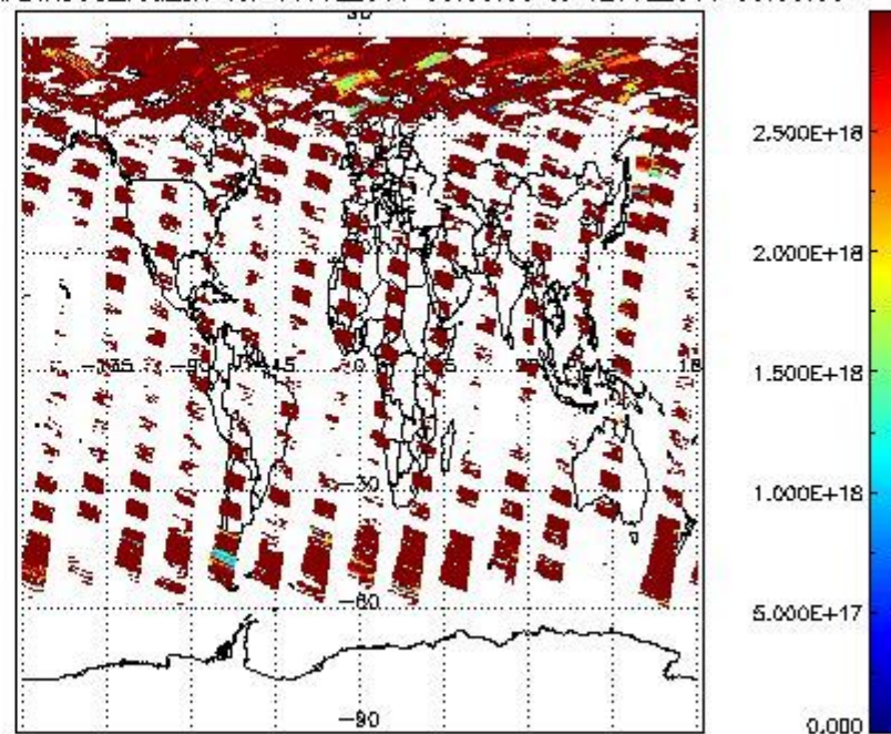
SCIDL2P_NADIR3CO_vcd_err for 11JUL2011 00:00:00 to 12JUL2011 00:00:00
