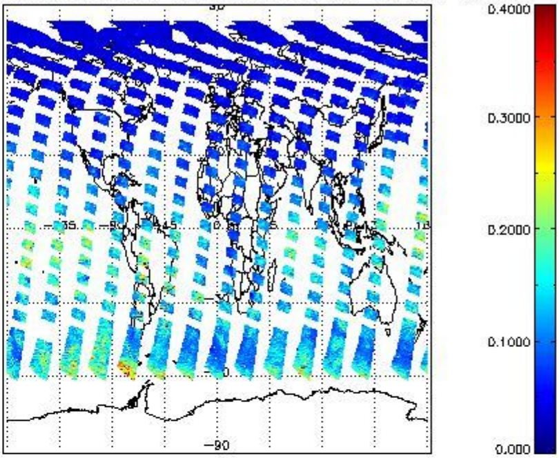
SCIOL2P_NADUV1NO2_vcd_err for 11JUL2011 00:00:00 to 12JUL2011 00:00:00
