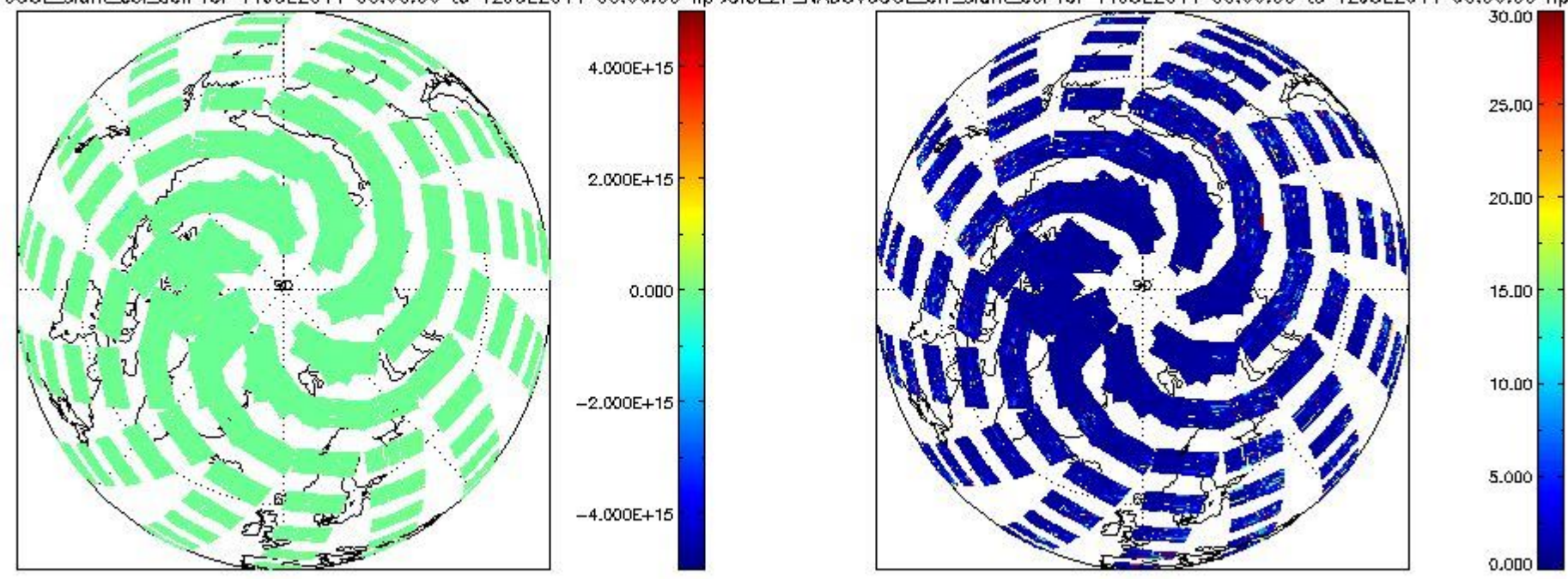
SCIO2P_NADUV6OCLslant_col_den for 11JUL2011 00:00:00 to 12JUL2011 00:00:00 np SCIO2P_NADUV6OCLarr_slant_col for 11JUL2011 00:00:00 to 12JUL2011 00:00:00 np
