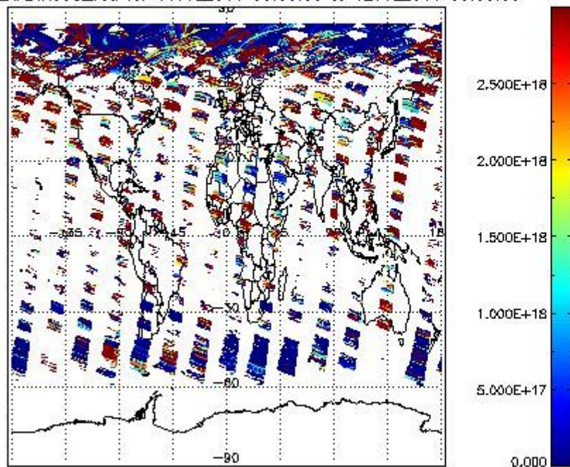
SCIDL2P_NADIR3CO_vcd for 11JUL2011 00:00:00 to 12JUL2011 00:00:00
