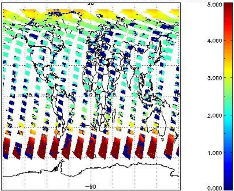
SCIOL2P_NADUV1NO2_amf_cl for 11JUL2011 00:00:00 to 12JUL2011 00:00:00
