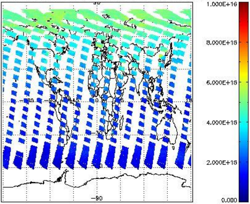
SCIOL2P_NADUV1NO2_vcd for 11JUL2011 00:00:00 to 12JUL2011 00:00:00
