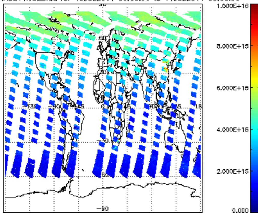
SCIOL2P_NADUV1NO2_vcd for 10JUL2011 00:00:00 to 11JUL2011 00:00:00
