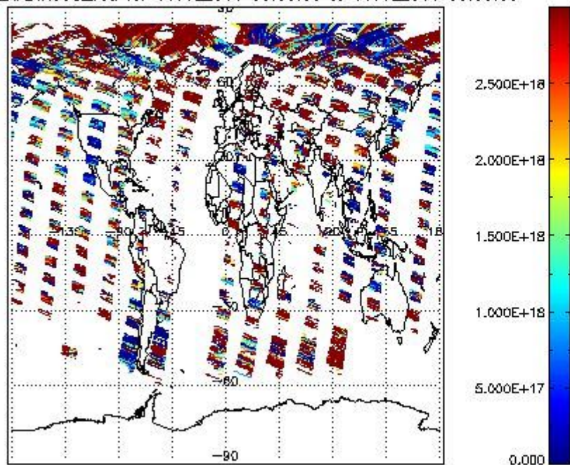
SCIDL2P_NADIR3CO_vcd for 10JUL2011 00:00:00 to 11JUL2011 00:00:00
