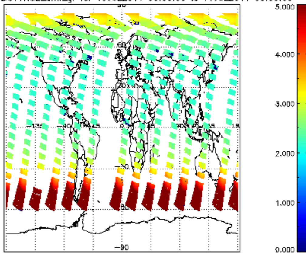
SCIOL2P_NADUV1NO2_amf_gr for 10JUL2011 00:00:00 to 11JUL2011 00:00:00
