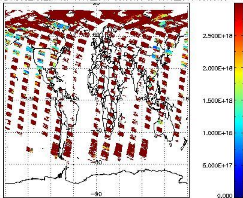
SCIDL2P_NADIR3CO_vcd_err for 10JUL2011 00:00:00 to 11JUL2011 00:00:00
