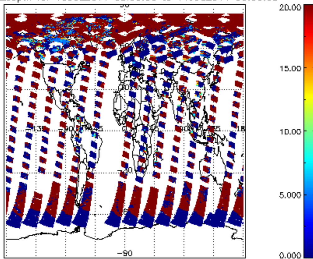
cl_lopt_depth for 10JUL2011 00:00:00 to 11JUL2011 00:00:00
