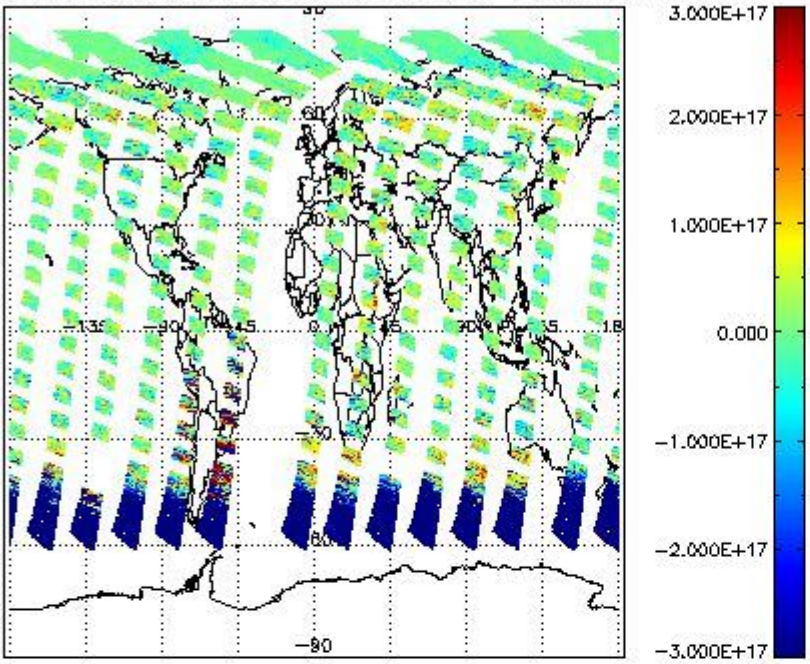
SCIOL2P_NADUV5S02_vcd for 10JUL2011 00:00:00 to 11JUL2011 00:00:00
