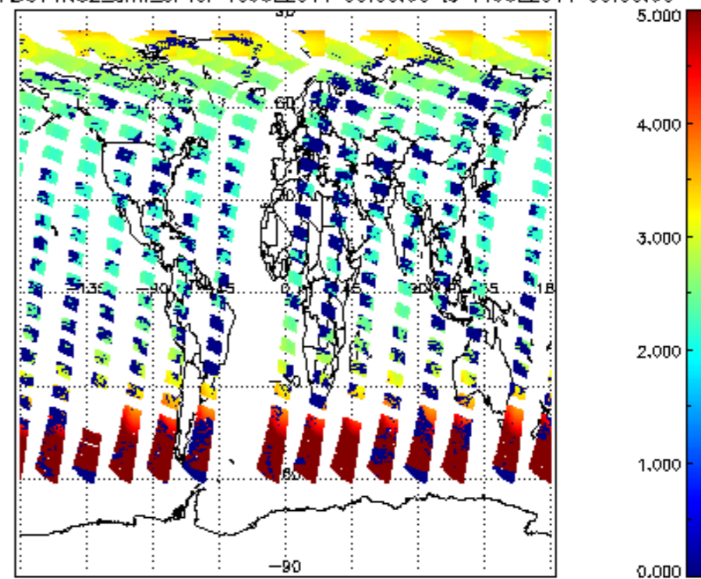
SCIOL2P_NADUV1NO2_amf_cl for 10JUL2011 00:00:00 to 11JUL2011 00:00:00
