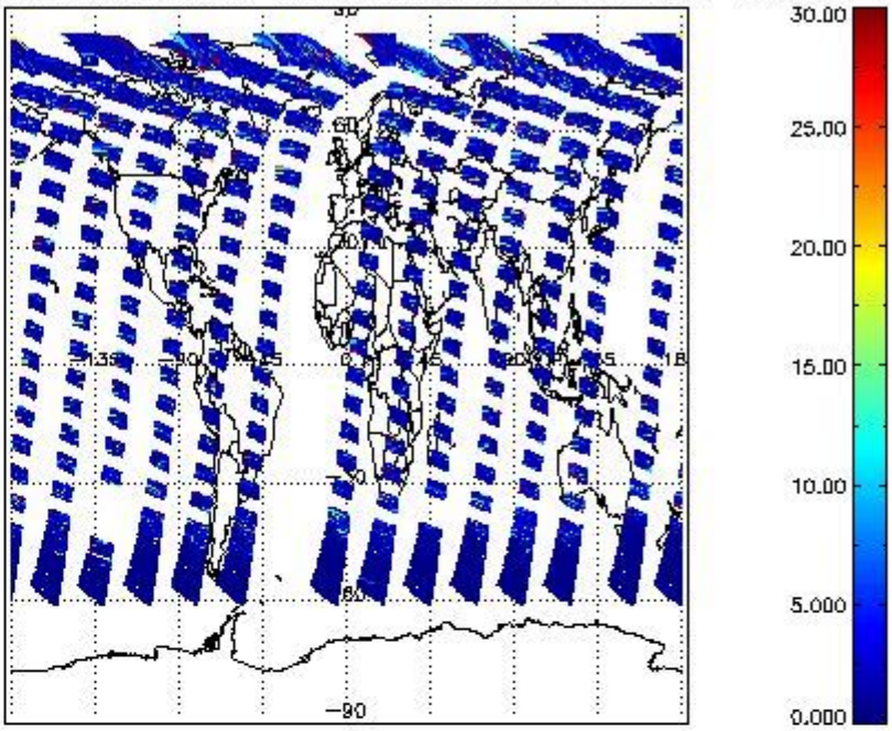
SCIOL2P_NADUV5S02_vcd_err for 10JUL2011 00:00:00 to 11JUL2011 00:00:00
