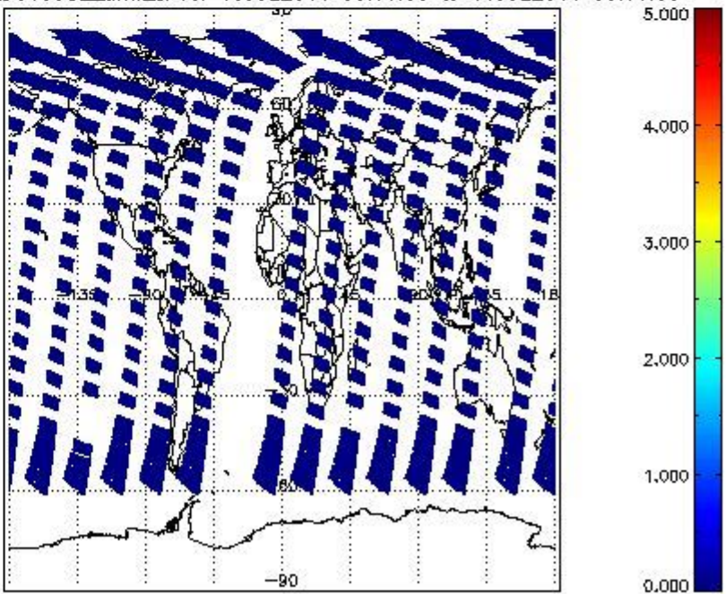
SCIOL2P_NADUV5S02_amf_cl for 10JUL2011 00:00:00 to 11JUL2011 00:00:00
