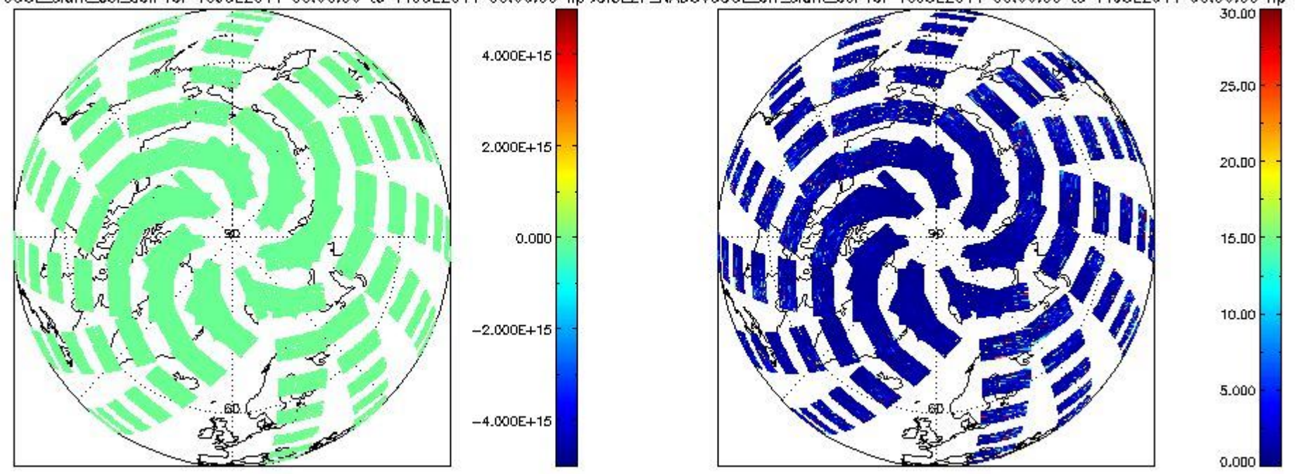
SCIOI2P_NADUV6OCLslant_col_den for 10JUL2011 00:00:00 to 11JUL2011 00:00:00 np SCIOI2P_NADUV6OCLarr_slant_col for 10JUL2011 00:00:00 to 11JUL2011 00:00:00 np
