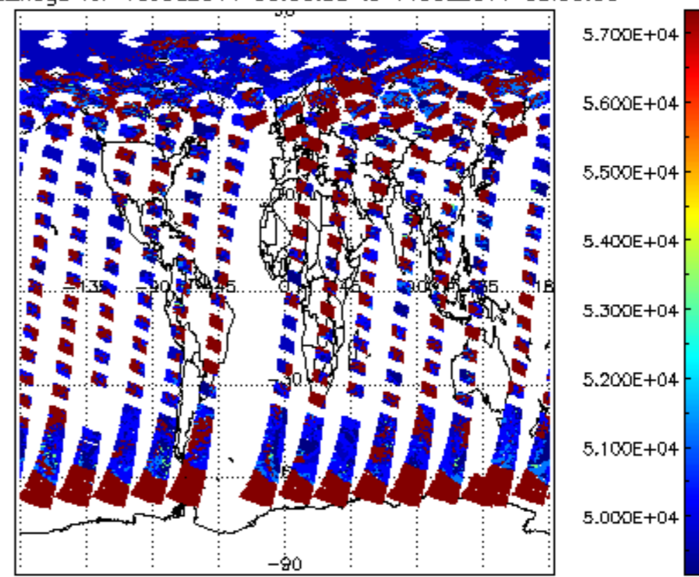
cloud_flags for 10JUL2011 00:00:00 to 11JUL2011 00:00:00
