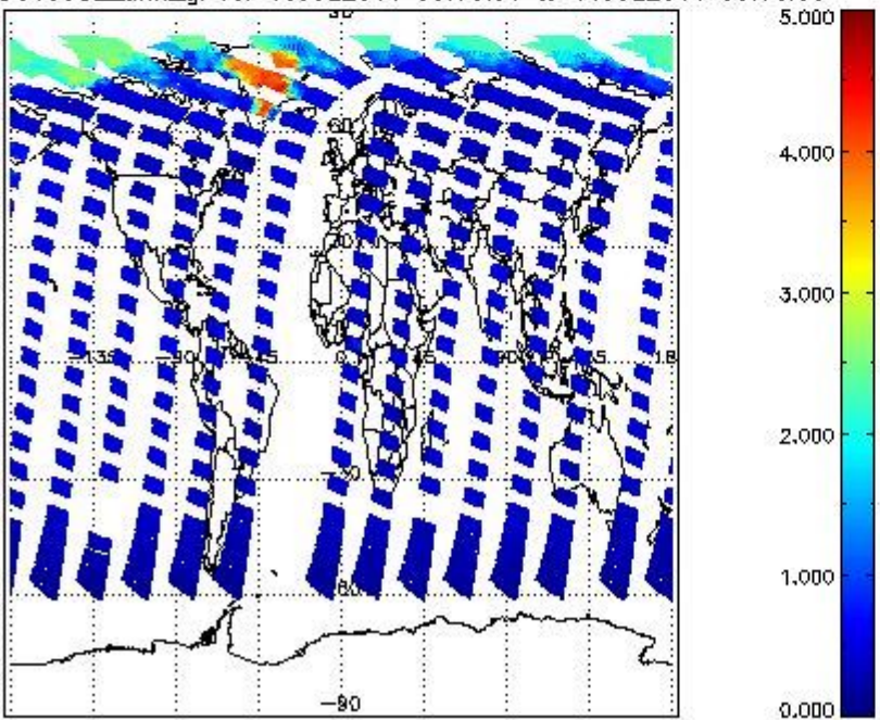
SCIOL2P_NADUV5S02_amf_gr for 10JUL2011 00:00:00 to 11JUL2011 00:00:00
