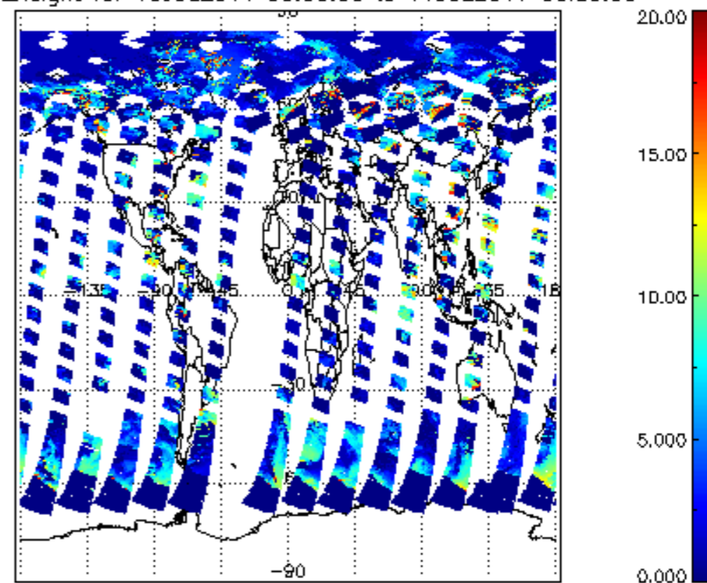
cl_top_height for 10JUL2011 00:00:00 to 11JUL2011 00:00:00
