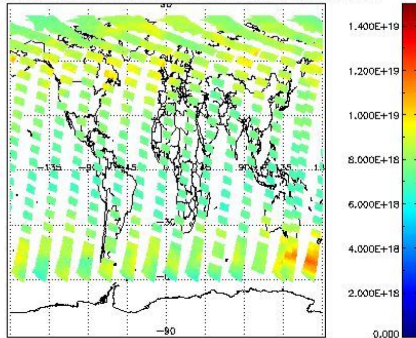
SCIOL2P_NADUV003_vcd for 09JUL2011 00:00:00 to 10JUL2011 00:00:00
