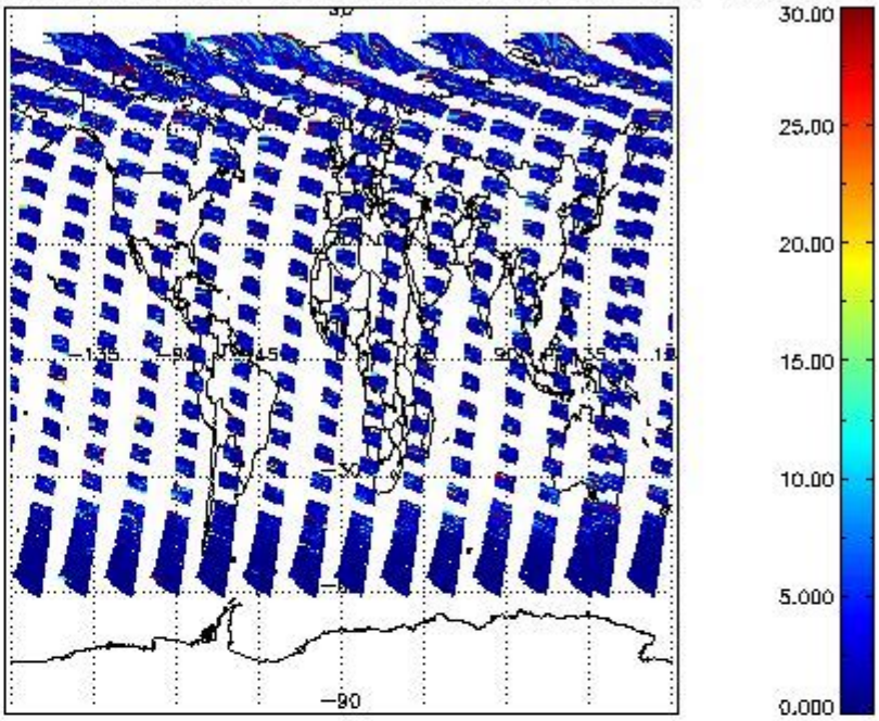
SCIOL2P_NADUV5S02_vcd_err for 09JUL2011 00:00:00 to 10JUL2011 00:00:00
