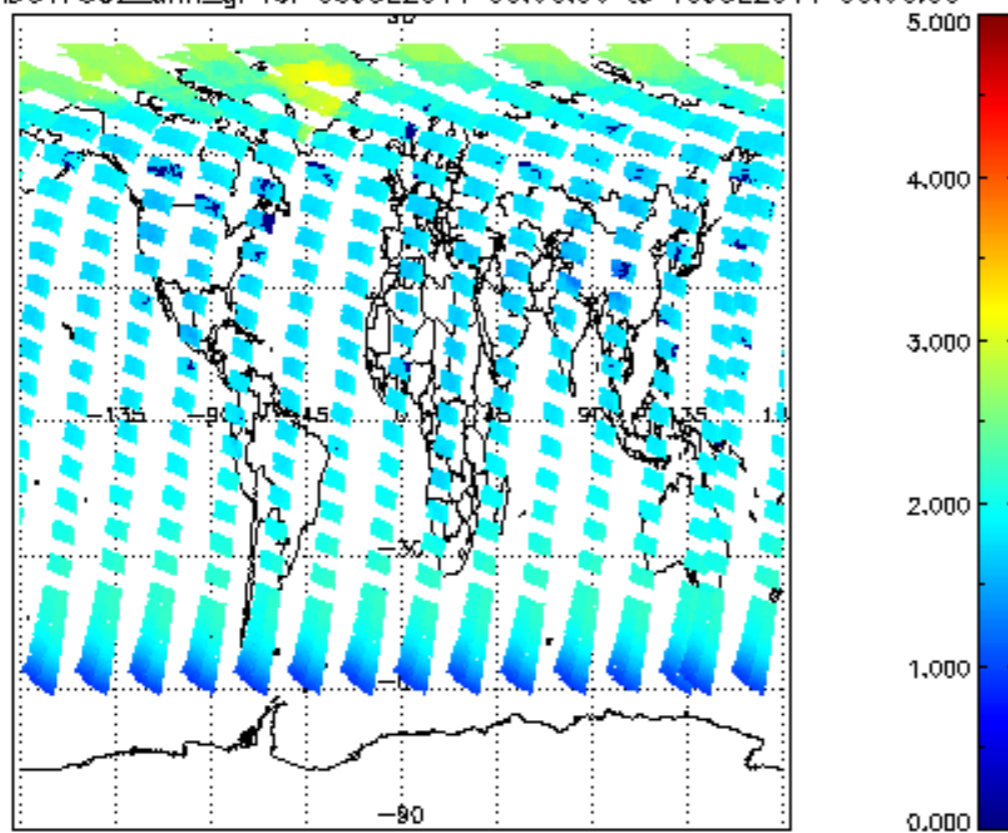
SCIOL2P_NADUV7S02_amf_gr for 09JUL2011 00:00:00 to 10JUL2011 00:00:00
