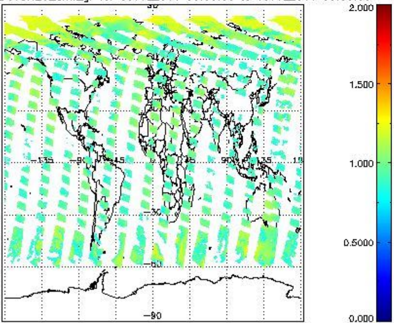
SCIOL2P_NADUV8H2O_amf_gr for 09JUL2011 00:00:00 to 10JUL2011 00:00:00
