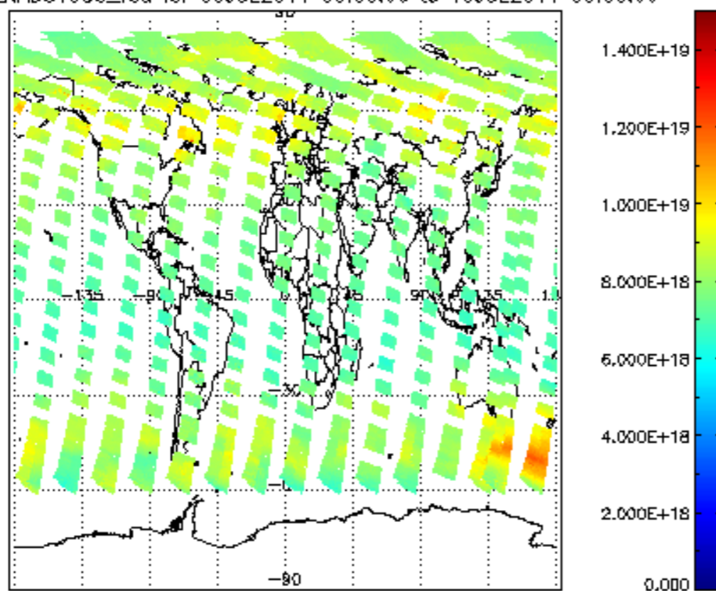
SCIOL2P_NADUV003_vcd for 09JUL2011 00:00:00 to 10JUL2011 00:00:00
