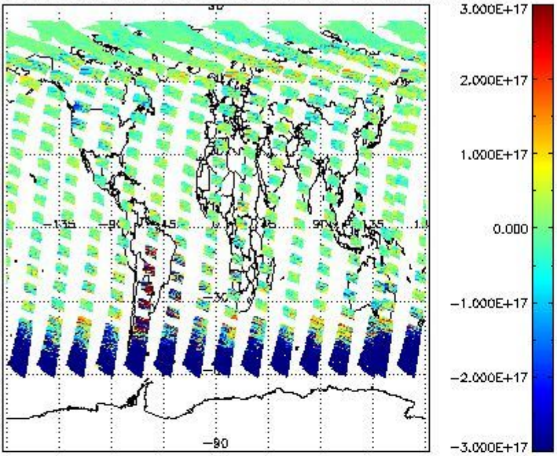
SCIOL2P_NADUV5S02_vcd for 09JUL2011 00:00:00 to 10JUL2011 00:00:00
