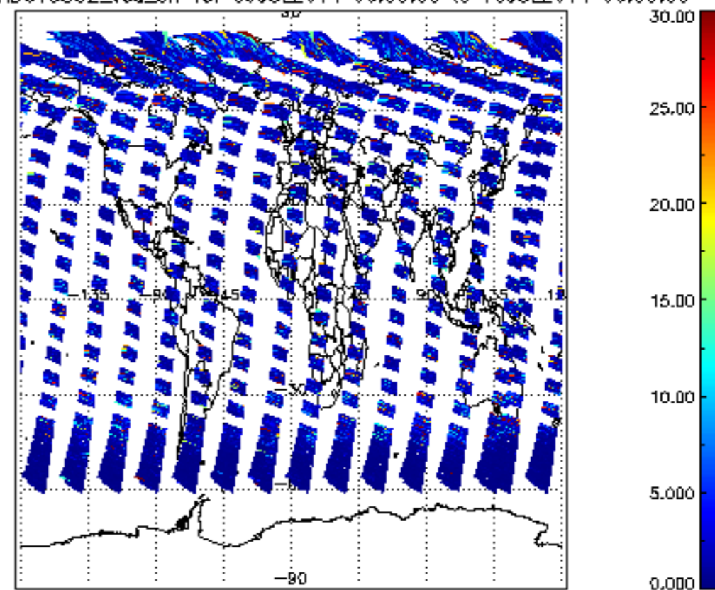
SCIOL2P_NADUV5S02_vcd_err for 09JUL2011 00:00:00 to 10JUL2011 00:00:00
