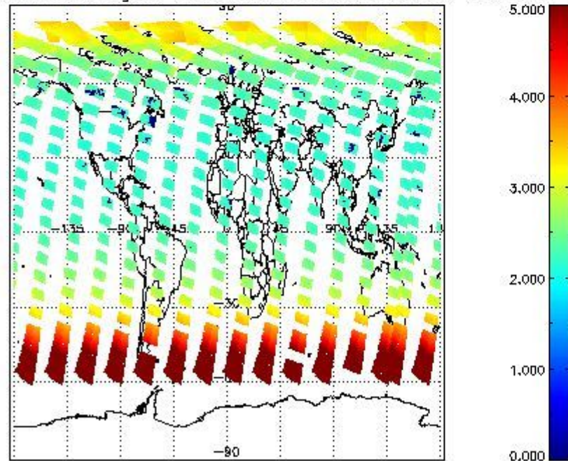
SCIOL2P_NADUV003_amf_gr for 09JUL2011 00:00:00 to 10JUL2011 00:00:00
