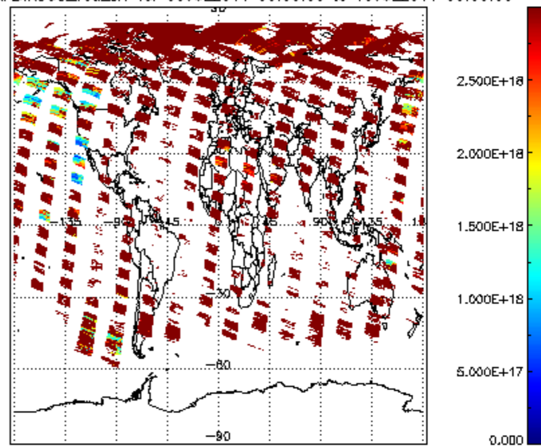
SCIOL2P_NADIR3CO_vcd_err for 09JUL2011 00:00:00 to 10JUL2011 00:00:00
