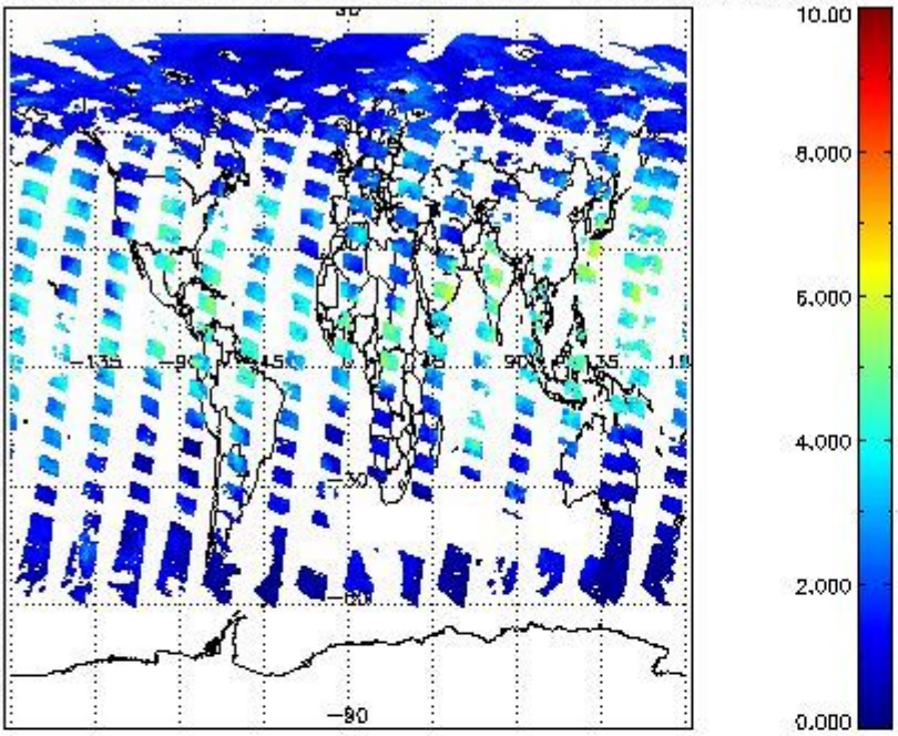
SCIOL2P_NADUV8H2O_vcd for 09JUL2011 00:00:00 to 10JUL2011 00:00:00
