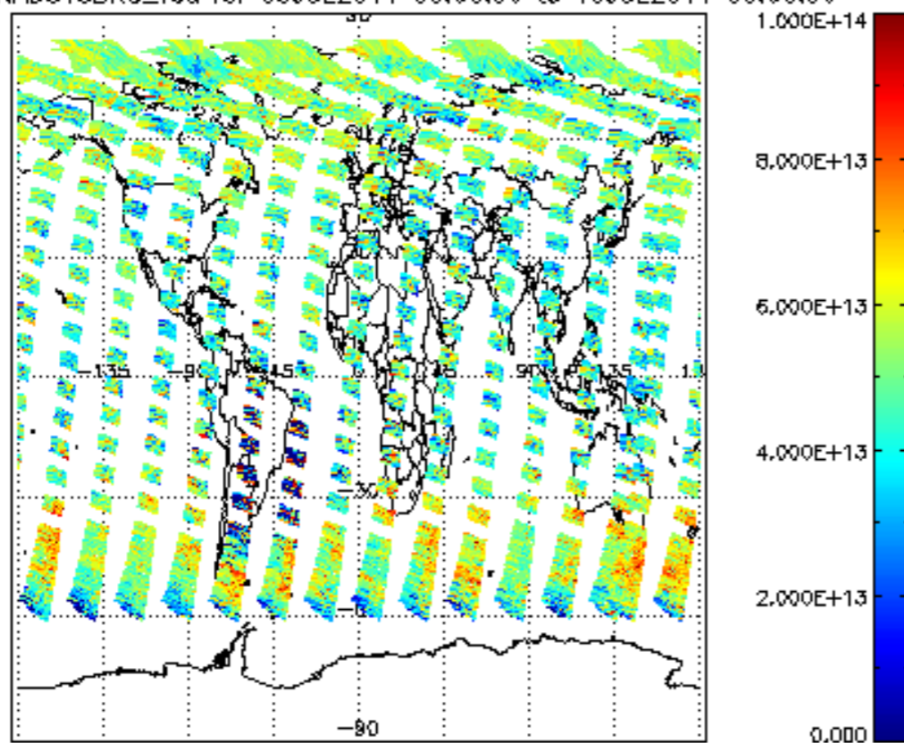
SCIOL2P_NADUV3BRO_vcd for 09JUL2011 00:00:00 to 10JUL2011 00:00:00
