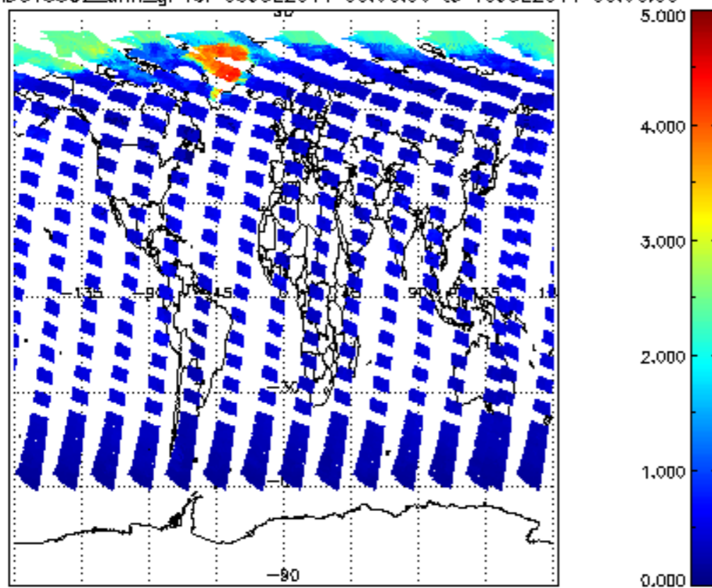
SCIOL2P_NADUV5S02_amf_gr for 09JUL2011 00:00:00 to 10JUL2011 00:00:00
