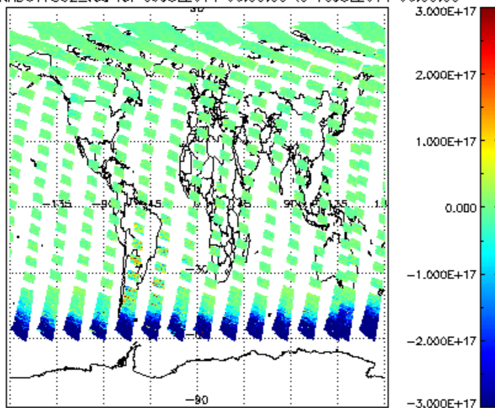
SCIOL2P_NADUV7S02_vcd for 09JUL2011 00:00:00 to 10JUL2011 00:00:00
