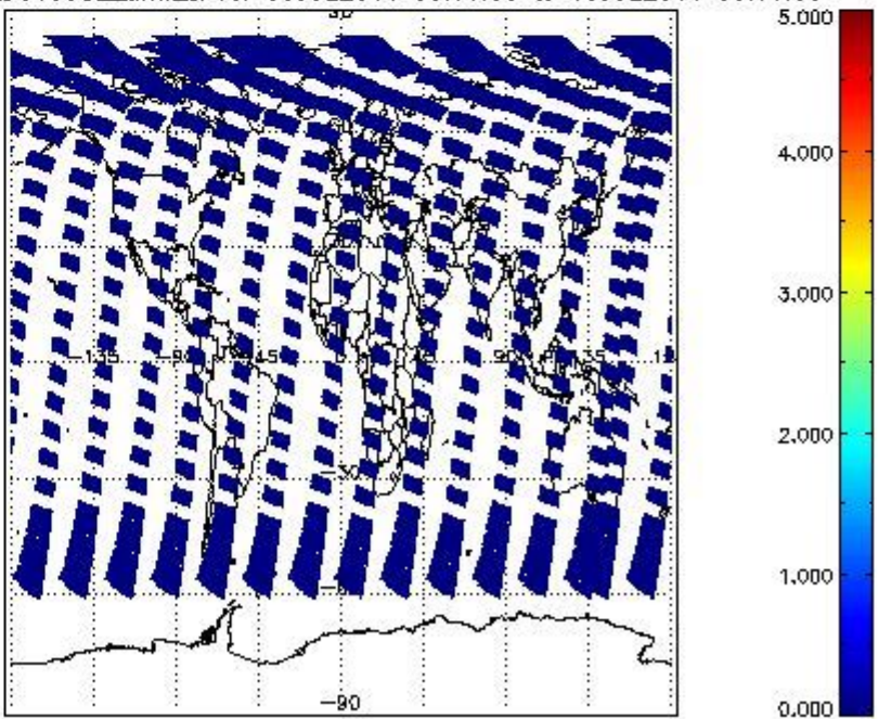
SCIOL2P_NADUV5S02_amf_cl for 09JUL2011 00:00:00 to 10JUL2011 00:00:00
