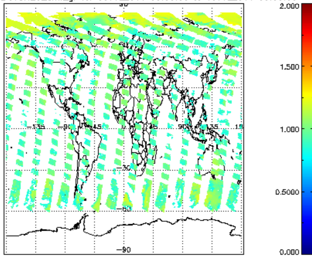
SCIOL2P_NADUV8H2O_amf_gr for 09JUL2011 00:00:00 to 10JUL2011 00:00:00
