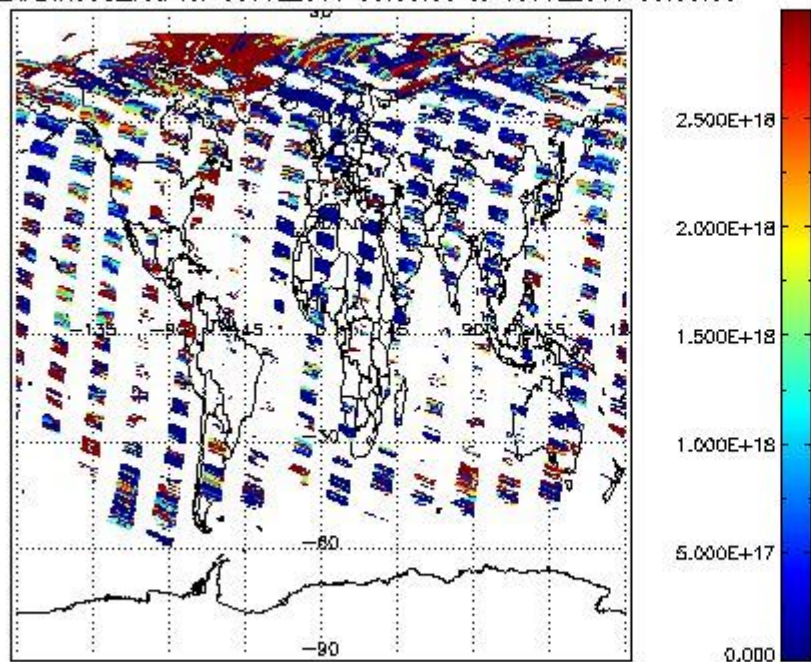
SCIOI2P_NADIR3CO_vcd for 09JUL2011 00:00:00 to 10JUL2011 00:00:00
