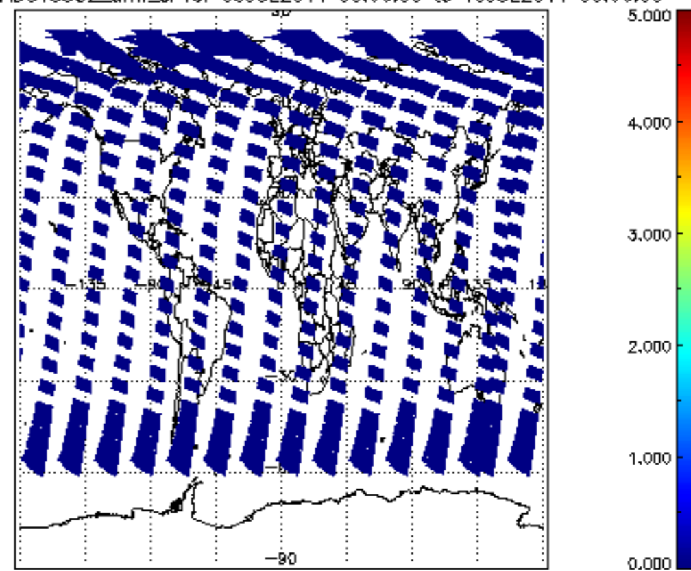
SCIOL2P_NADUV5S02_amf_cl for 09JUL2011 00:00:00 to 10JUL2011 00:00:00
