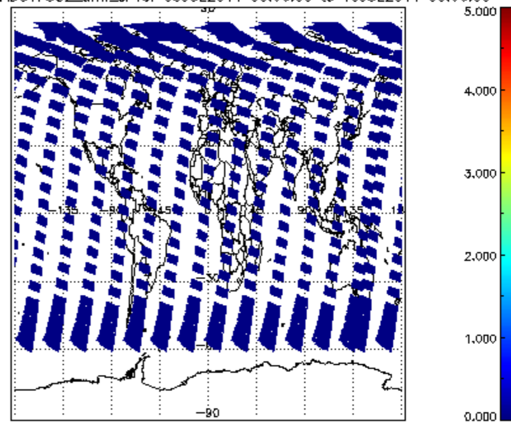
SCIOL2P_NADUV7S02_amf_cl for 09JUL2011 00:00:00 to 10JUL2011 00:00:00
