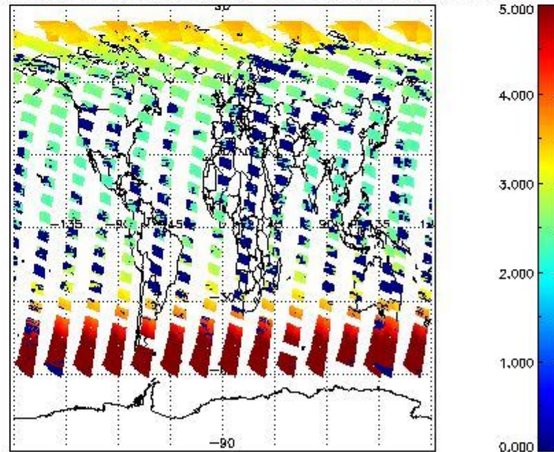
SCIOL2P_NADUV003_amf_cl for 09JUL2011 00:00:00 to 10JUL2011 00:00:00
