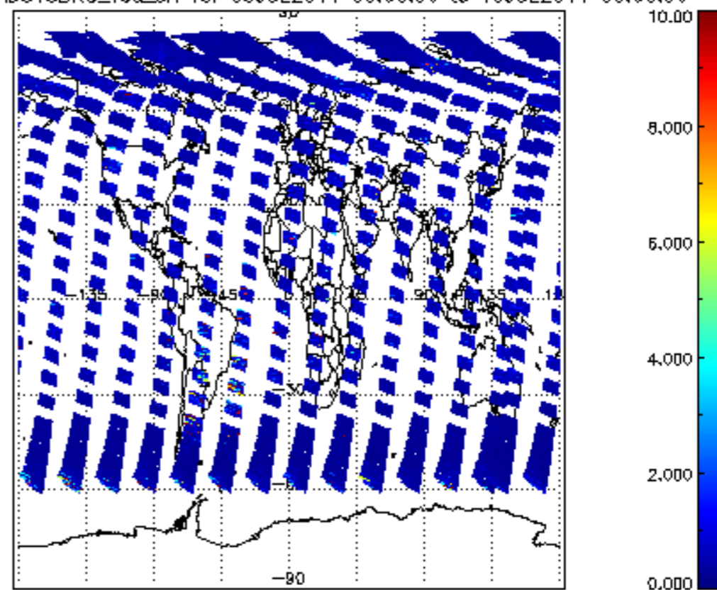
SCIOL2P_NADUV3BRO_vcd_err for 09JUL2011 00:00:00 to 10JUL2011 00:00:00
