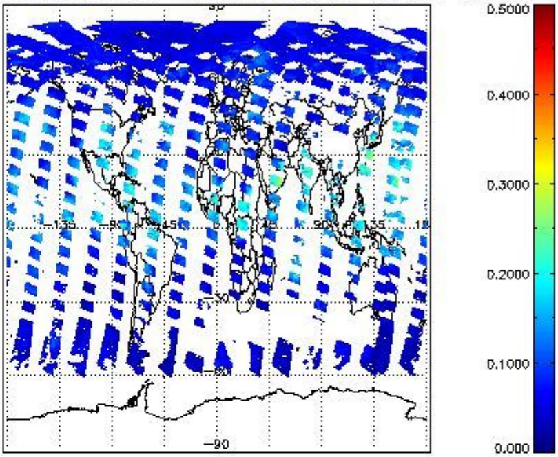
SCIOL2P_NADUV8H2O_vcd_err for 09JUL2011 00:00:00 to 10JUL2011 00:00:00
