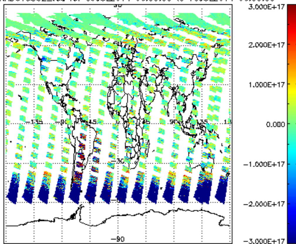
SCIOL2P_NADUV5S02_vcd for 09JUL2011 00:00:00 to 10JUL2011 00:00:00
