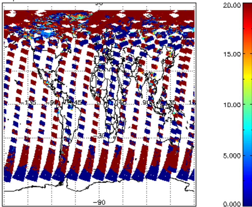
cl_opt_depth for 09JUL2011 00:00:00 to 10JUL2011 00:00:00
