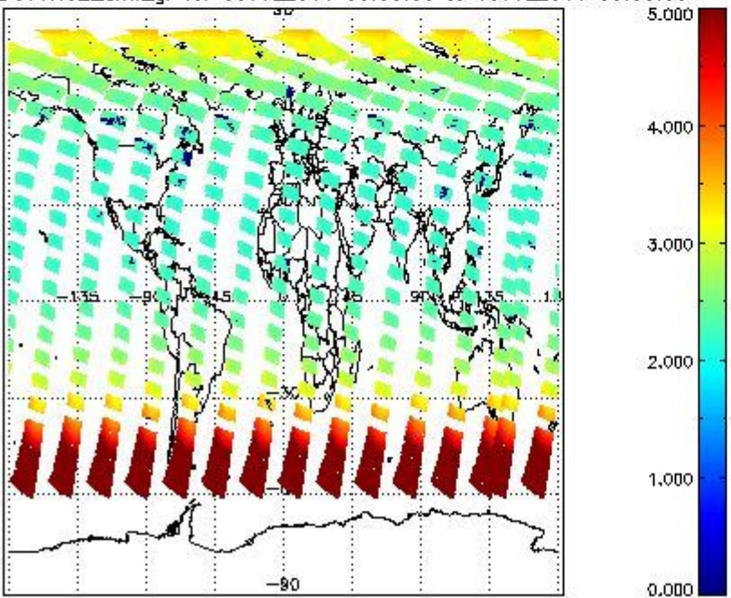
SCIOL2P_NADUV1NO2_amf_gr for 09JUL2011 00:00:00 to 10JUL2011 00:00:00
