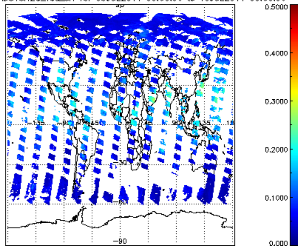
SCIOL2P_NADUV8H2O_vcd_err for 09JUL2011 00:00:00 to 10JUL2011 00:00:00
