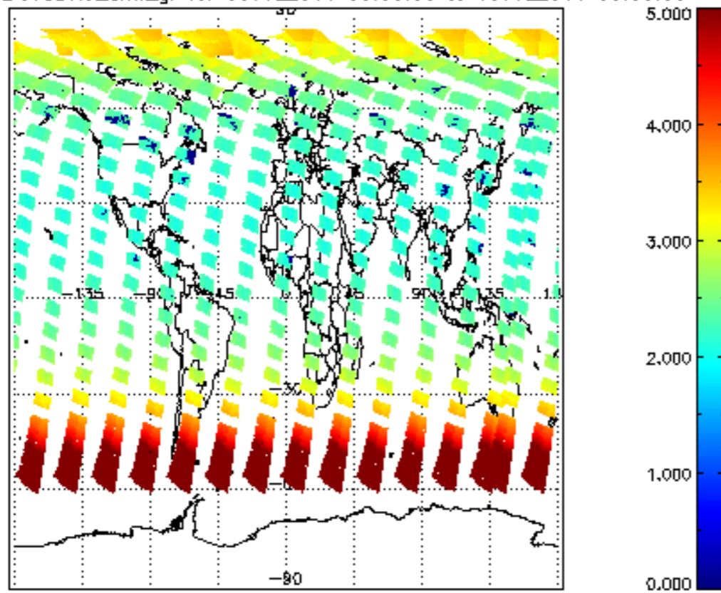
SCIOL2P_NADUV3BRO_arnf_gr for 09JUL2011 00:00:00 to 10JUL2011 00:00:00
