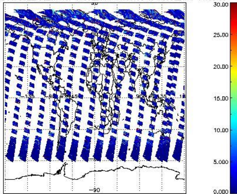
SCIOL2P_NADUV7S02_vcd_err for 09JUL2011 00:00:00 to 10JUL2011 00:00:00
