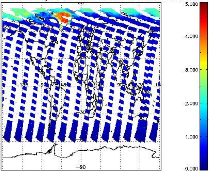
SCIOL2P_NADUV5S02_amf_gr for 09JUL2011 00:00:00 to 10JUL2011 00:00:00
