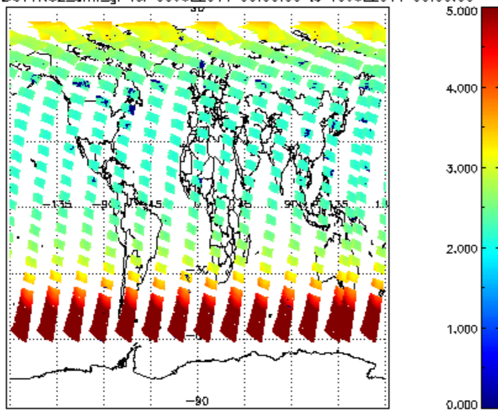
SCIOL2P_NADUV1NO2_amf_gr for 09JUL2011 00:00:00 to 10JUL2011 00:00:00
