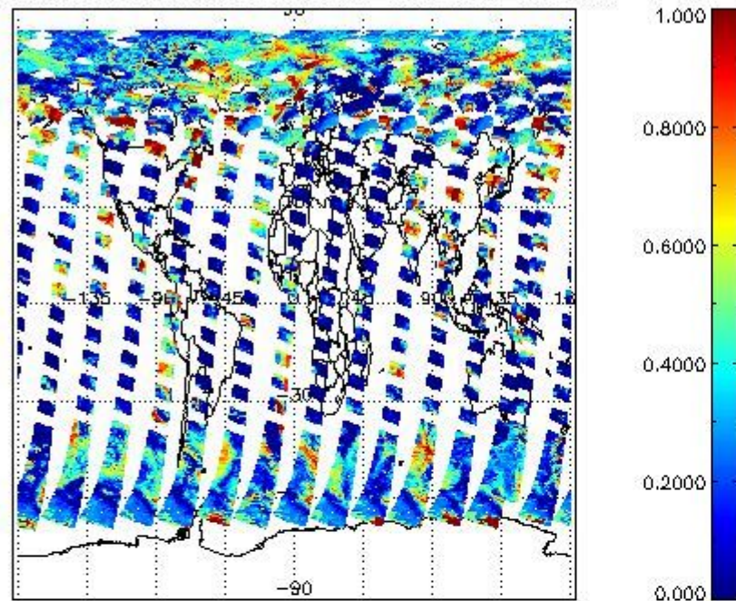
cL_frac for 09JUL2011 00:00:00 to 10JUL2011 00:00:00
