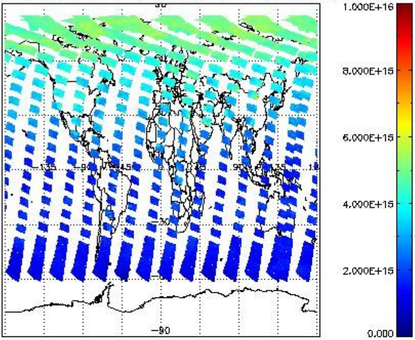
SCIOL2P_NADUV1NO2_vcd for 09JUL2011 00:00:00 to 10JUL2011 00:00:00
