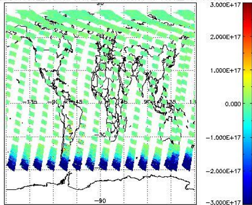
SCIOL2P_NADUV7S02_vcd for 09JUL2011 00:00:00 to 10JUL2011 00:00:00
