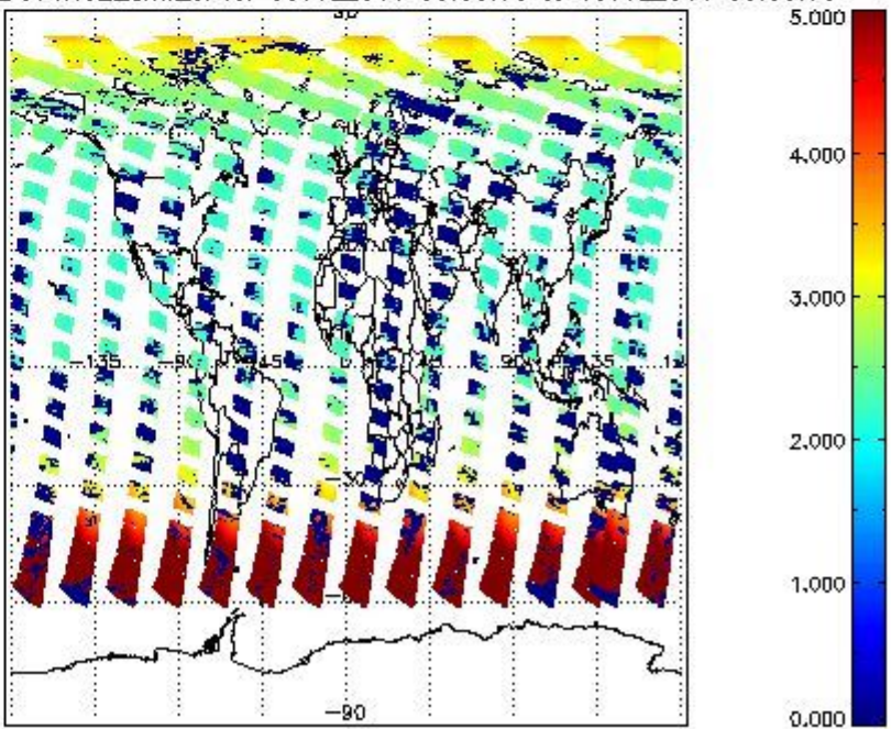
SCIOL2P_NADUV1NO2_amf_cl for 09JUL2011 00:00:00 to 10JUL2011 00:00:00
