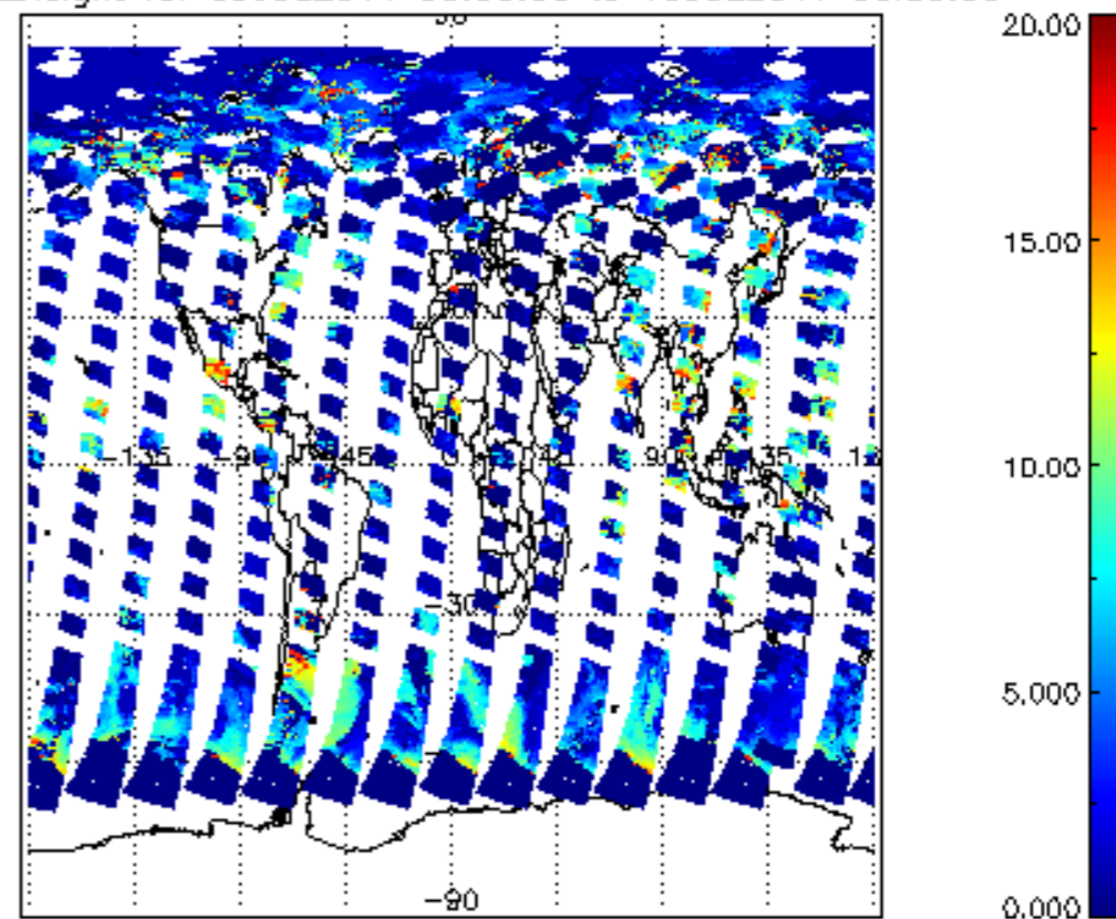
cl_top_height for 09JUL2011 00:00:00 to 10JUL2011 00:00:00
