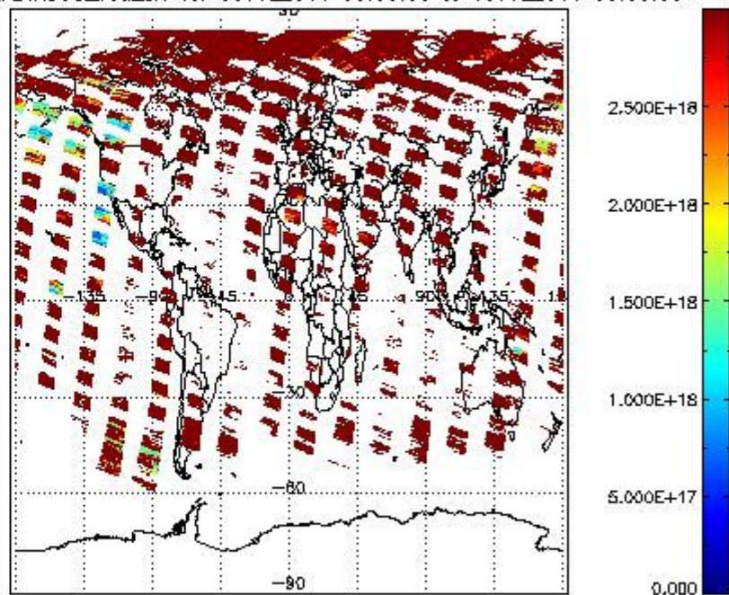
SCIOI2P_NADIR3CO_vcd_err for 09JUL2011 00:00:00 to 10JUL2011 00:00:00
