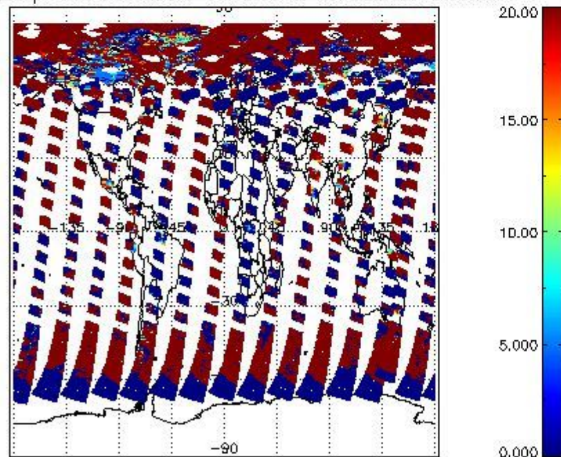
cL_opt_depth for 09JUL2011 00:00:00 to 10JUL2011 00:00:00
