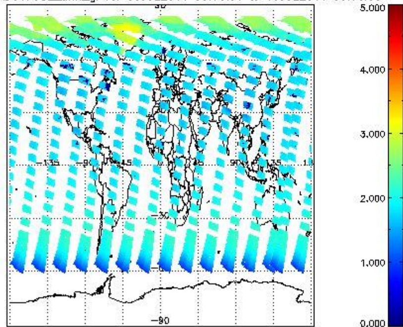
SCIOL2P_NADUV7S02_amf_gr for 09JUL2011 00:00:00 to 10JUL2011 00:00:00
