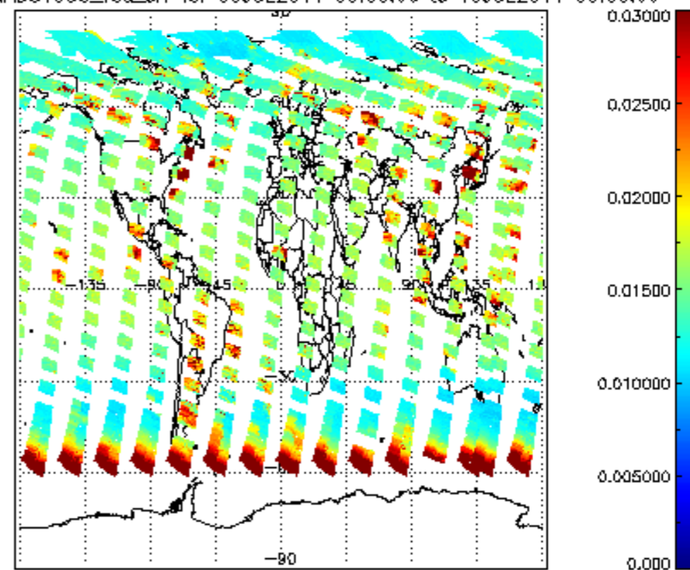
SCIOL2P_NADUV003_vcd_err for 09JUL2011 00:00:00 to 10JUL2011 00:00:00
