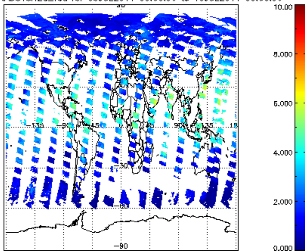
SCIOL2P_NADUV8H2O_vcd for 09JUL2011 00:00:00 to 10JUL2011 00:00:00
