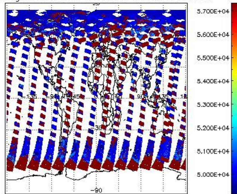
cloud_flags for 09JUL2011 00:00:00 to 10JUL2011 00:00:00
