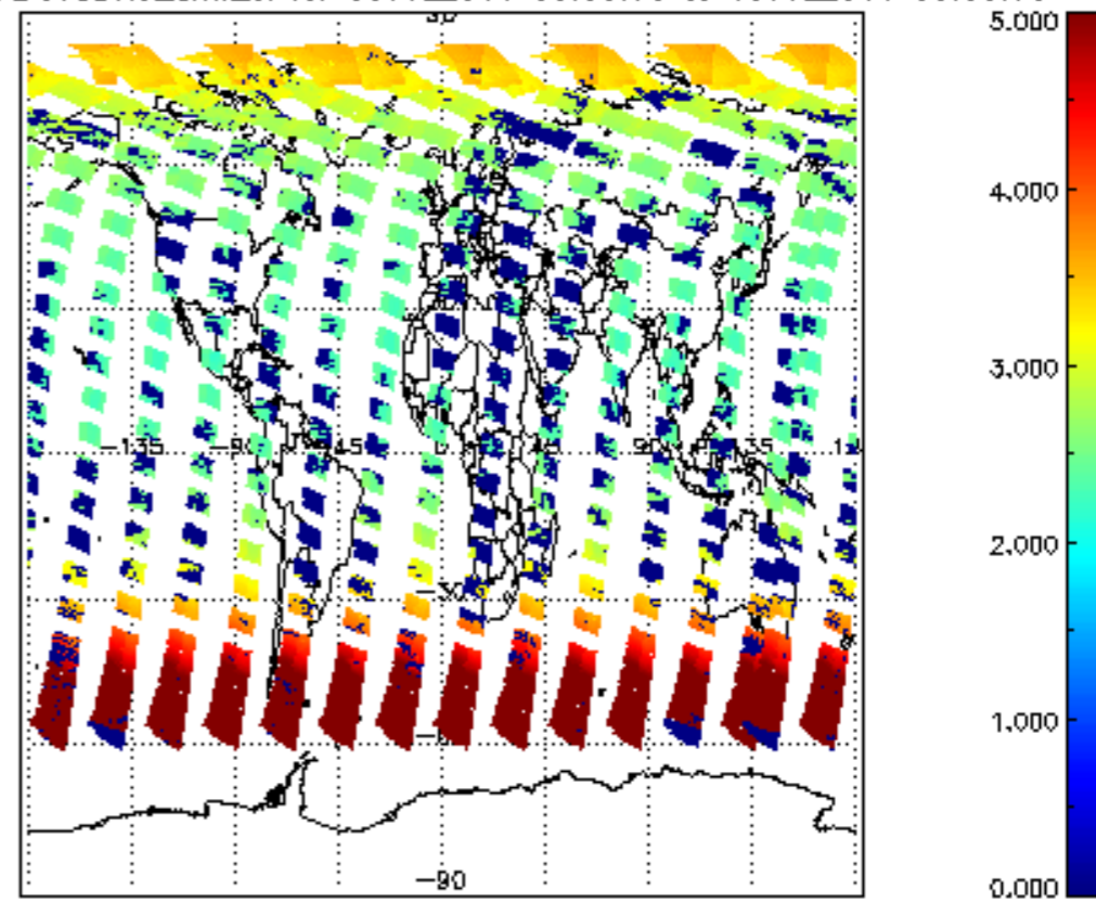
SCIOL2P_NADUV3BRO_arnf_cl for 09JUL2011 00:00:00 to 10JUL2011 00:00:00
