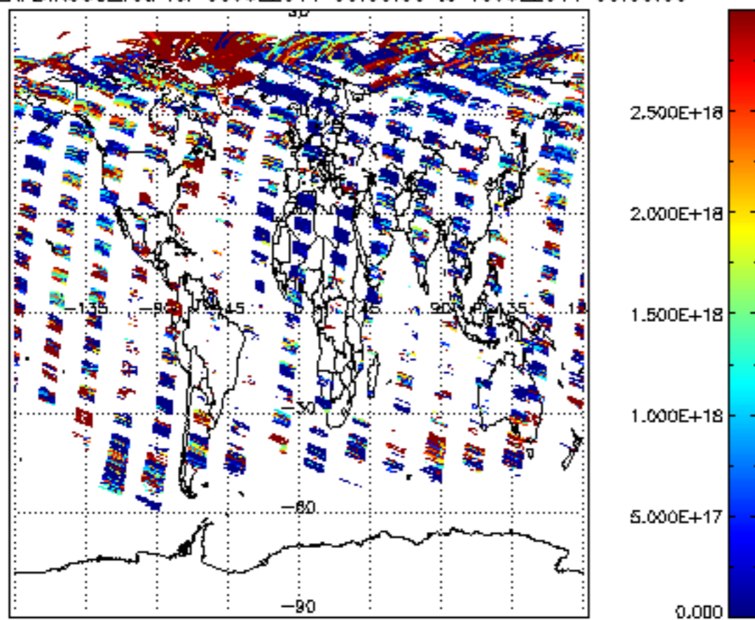
SCIOL2P_NADIR3CO_vcd for 09JUL2011 00:00:00 to 10JUL2011 00:00:00
