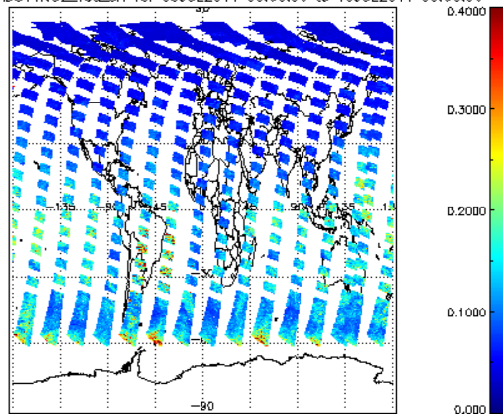
SCIOL2P_NADUV1NO2_vcd_err for 09JUL2011 00:00:00 to 10JUL2011 00:00:00
