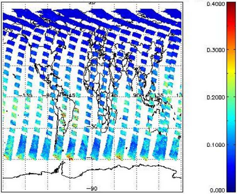
SCIOL2P_NADUV1NO2_vcd_err for 09JUL2011 00:00:00 to 10JUL2011 00:00:00
