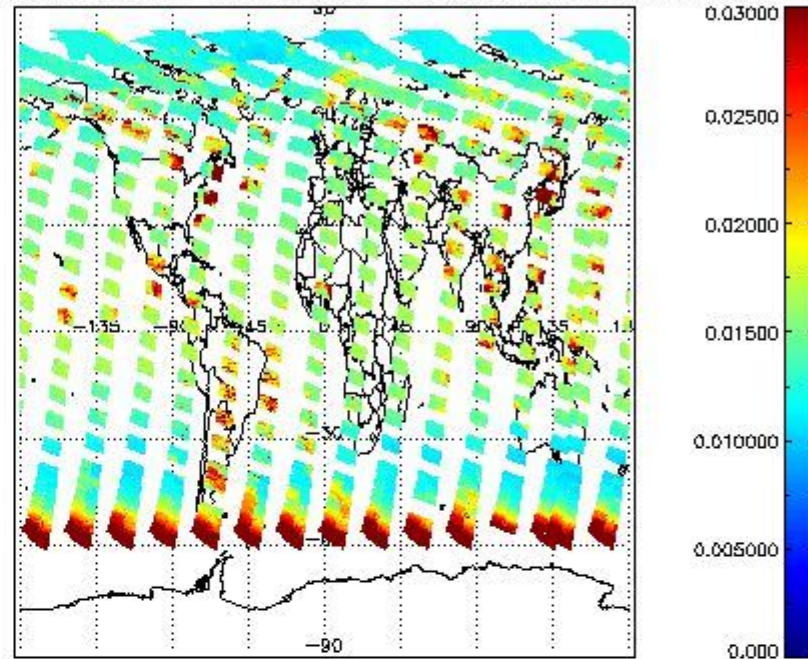
SCIOL2P_NADUV003_vcd_err for 09JUL2011 00:00:00 to 10JUL2011 00:00:00
