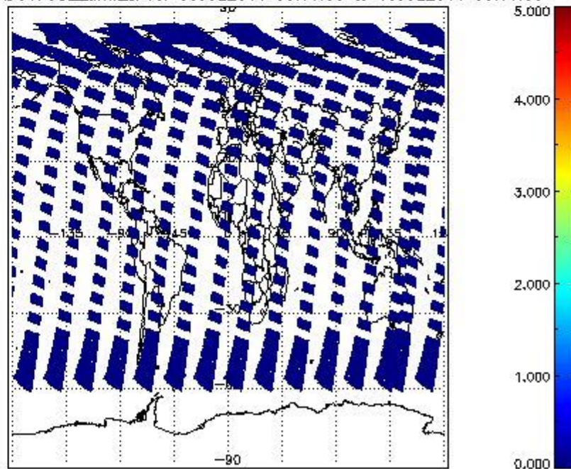
SCIOL2P_NADUV7S02_amf_cl for 09JUL2011 00:00:00 to 10JUL2011 00:00:00
