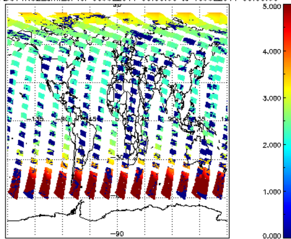
SCIOL2P_NADUV1NO2_amf_cl for 09JUL2011 00:00:00 to 10JUL2011 00:00:00
