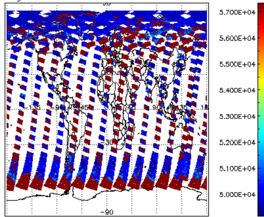
cloud_flags for 09JUL2011 00:00:00 to 10JUL2011 00:00:00
