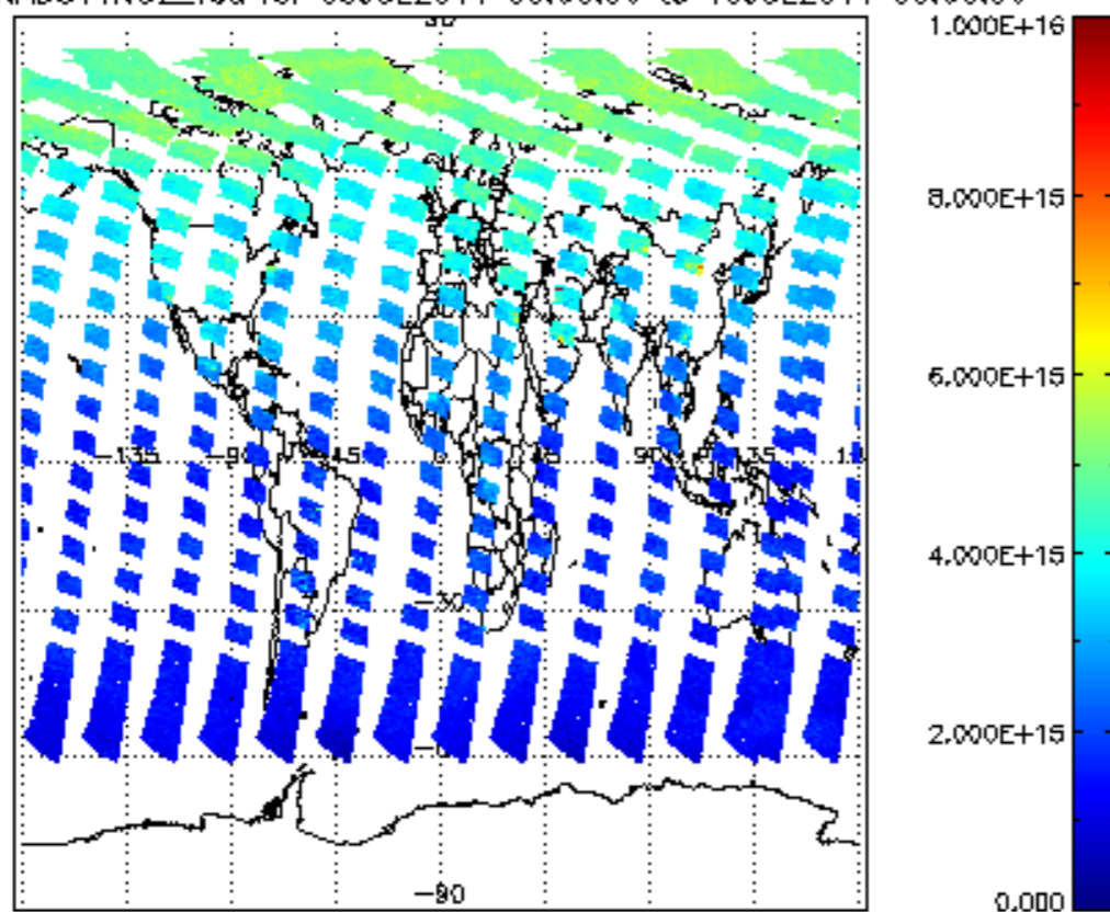
SCIOL2P_NADUV1NO2_vcd for 09JUL2011 00:00:00 to 10JUL2011 00:00:00
