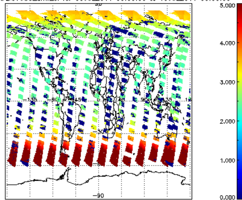
SCIOL2P_NADUV003_amf_cl for 09JUL2011 00:00:00 to 10JUL2011 00:00:00
