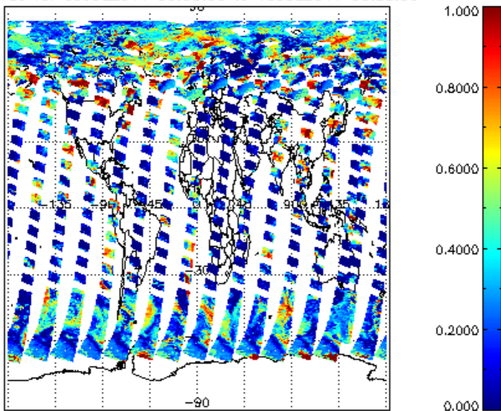
cl_frac for 09JUL2011 00:00:00 to 10JUL2011 00:00:00
