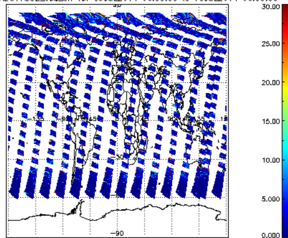
SCIOL2P_NADUV7S02_vcd_err for 09JUL2011 00:00:00 to 10JUL2011 00:00:00
