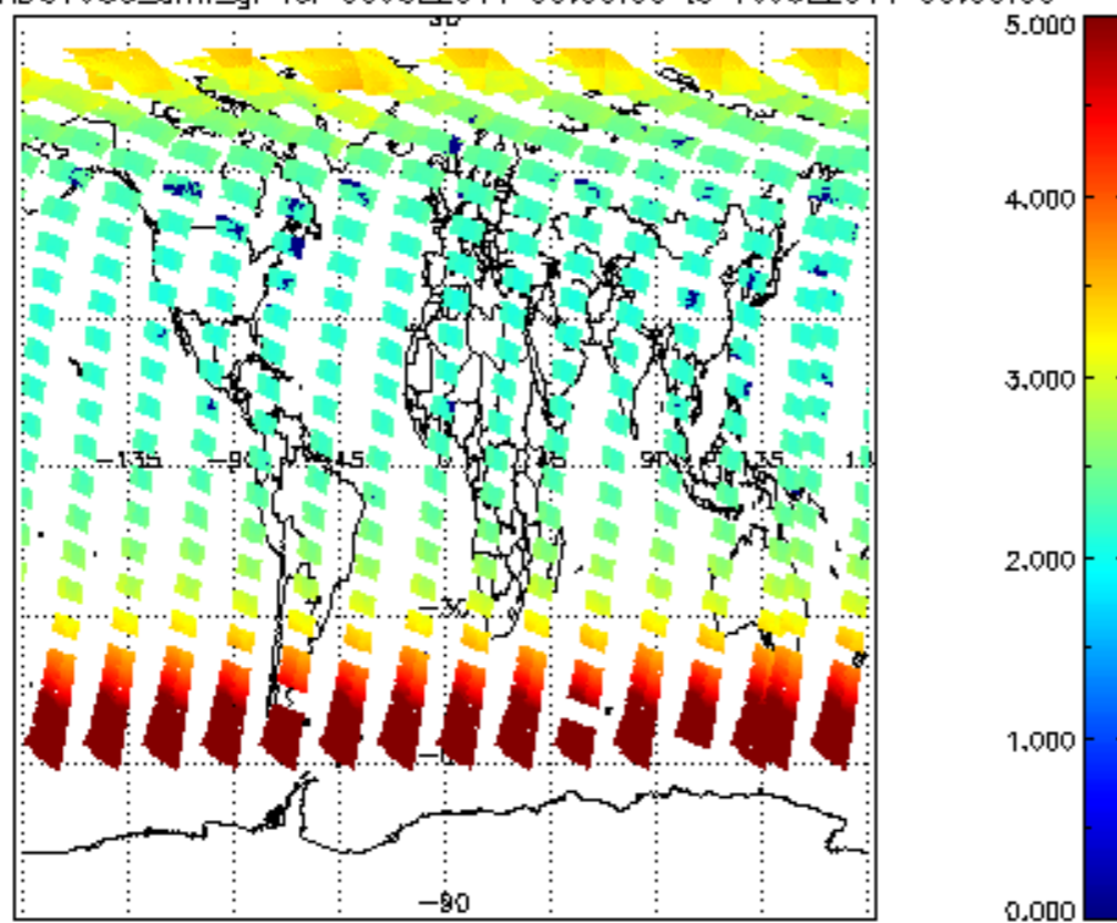
SCIOL2P_NADUV003_amf_gr for 09JUL2011 00:00:00 to 10JUL2011 00:00:00
