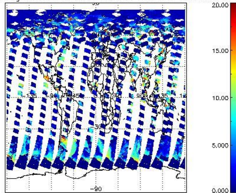
cL_top_height for 09JUL2011 00:00:00 to 10JUL2011 00:00:00
