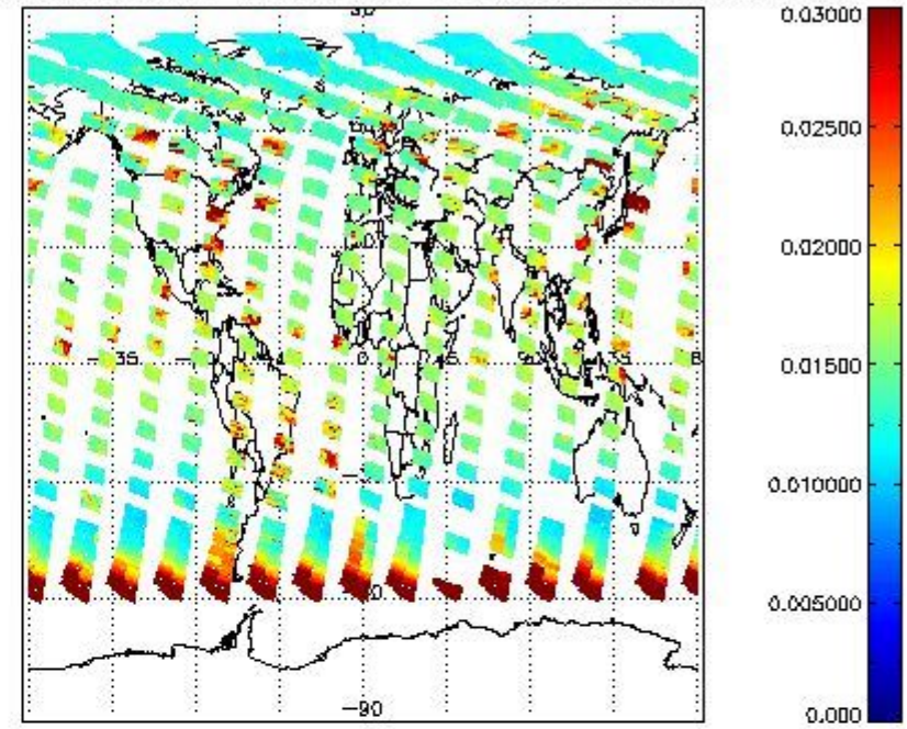
SCIOL2P_NADUV003_vcd_Lerr for 08JUL2011 00:00:00 to 09JUL2011 00:00:00
