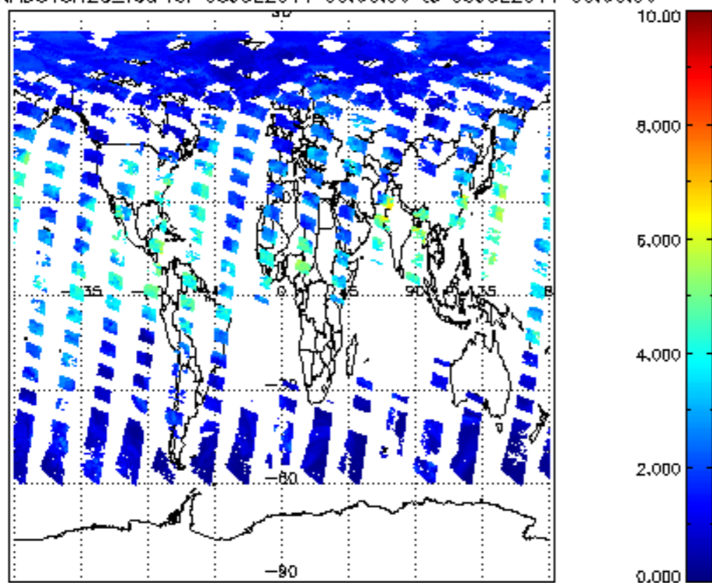
SCIOL2P_NADUV8H20_vcd for 08JUL2011 00:00:00 to 09JUL2011 00:00:00
