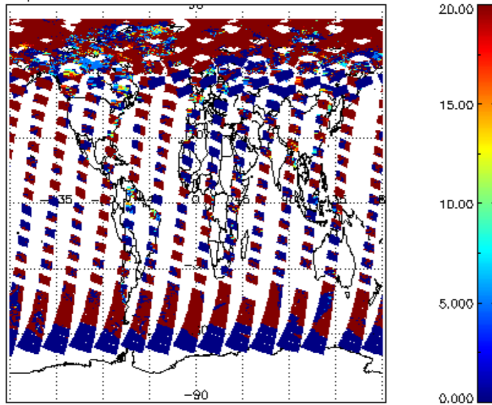
cl_opt_depth for 08JUL2011 00:00:00 to 09JUL2011 00:00:00
