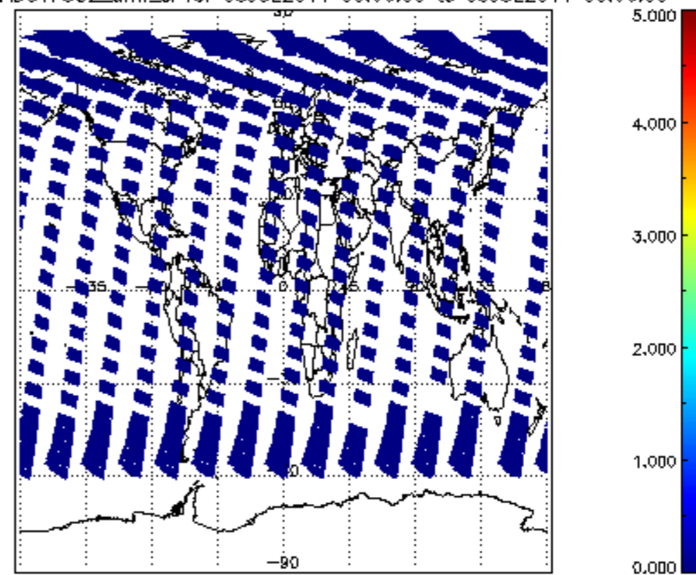
SCIOL2P_NADUV7S02_amf_cl for 08JUL2011 00:00:00 to 09JUL2011 00:00:00
