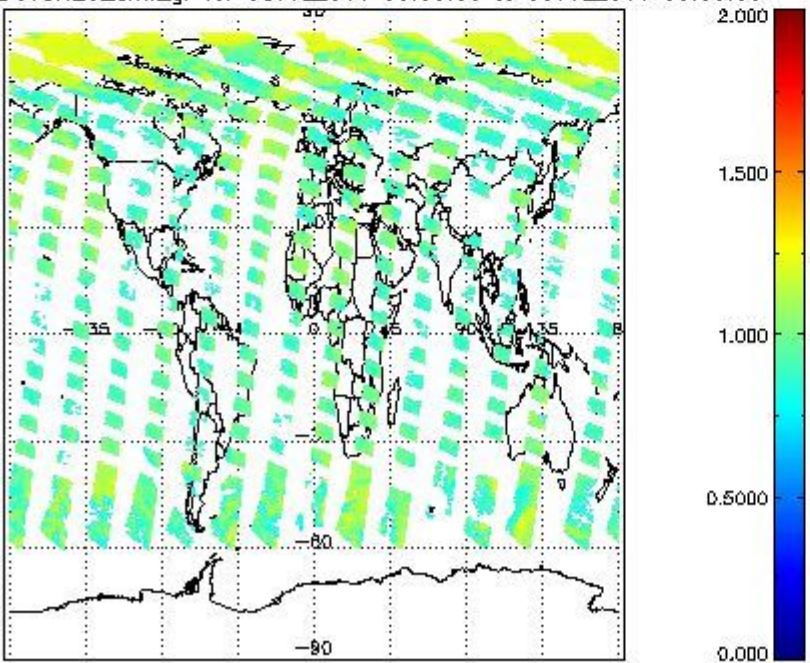
SCIOL2P_NADUV8H2O_amf_gr for 08JUL2011 00:00:00 to 09JUL2011 00:00:00
