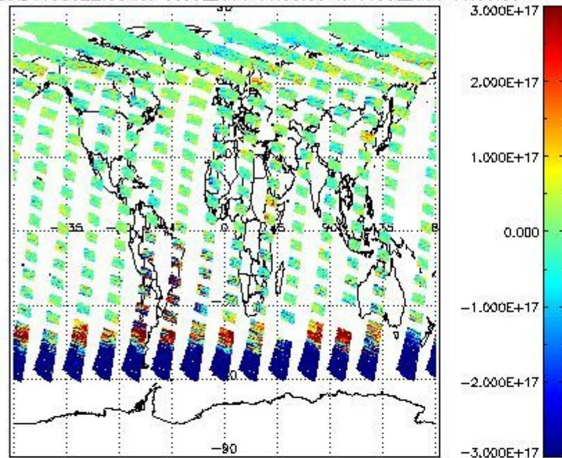
SCIOL2P_NADUV5S02_vcd for 08JUL2011 00:00:00 to 09JUL2011 00:00:00
