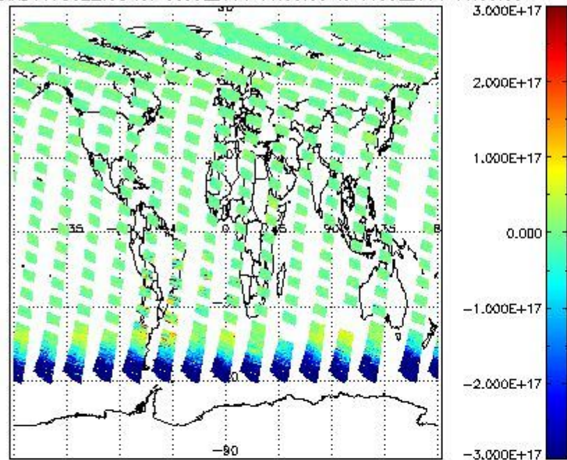
SCIOL2P_NADUV7S02_vcd for 08JUL2011 00:00:00 to 09JUL2011 00:00:00
