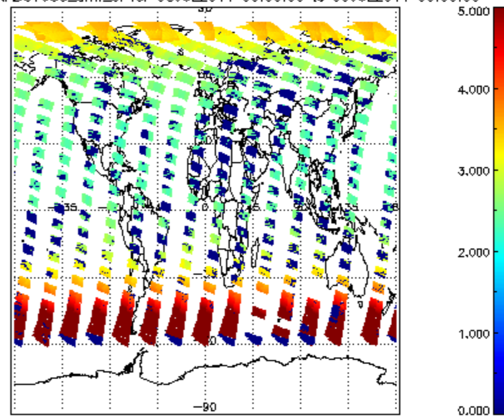
SCIOL2P_NADUV003_amf_cl for 08JUL2011 00:00:00 to 09JUL2011 00:00:00
