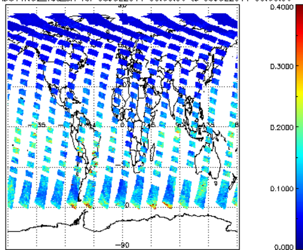
SCIOL2P_NADUV1NO2_vcd_err for 08JUL2011 00:00:00 to 09JUL2011 00:00:00
