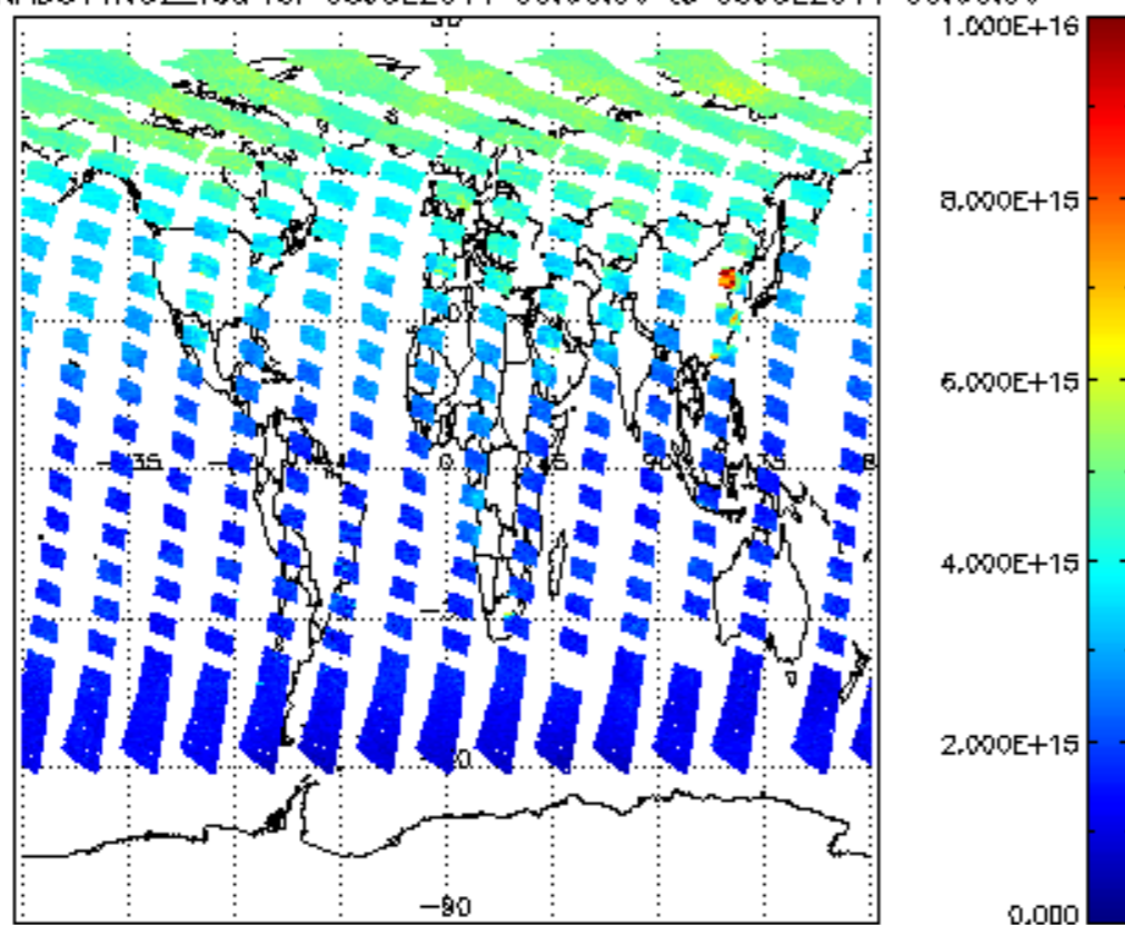
SCIOL2P_NADUV1NO2_vcd for 08JUL2011 00:00:00 to 09JUL2011 00:00:00
