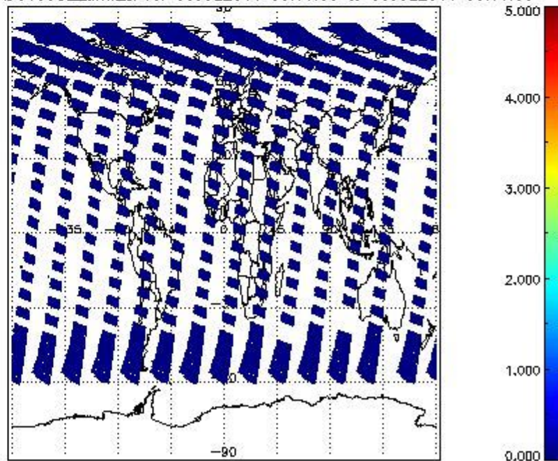
SCIOL2P_NADUV5S02_amf_cl for 08JUL2011 00:00:00 to 09JUL2011 00:00:00
