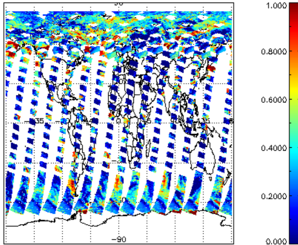
cl_frac for 08JUL2011 00:00:00 to 09JUL2011 00:00:00
