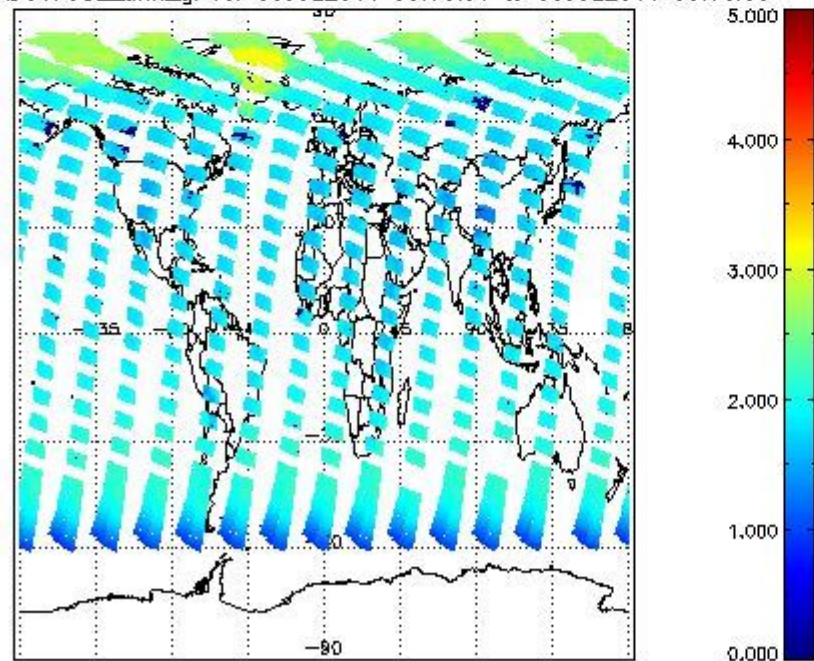
SCIOL2P_NADUV7S02_amf_gr for 08JUL2011 00:00:00 to 09JUL2011 00:00:00
