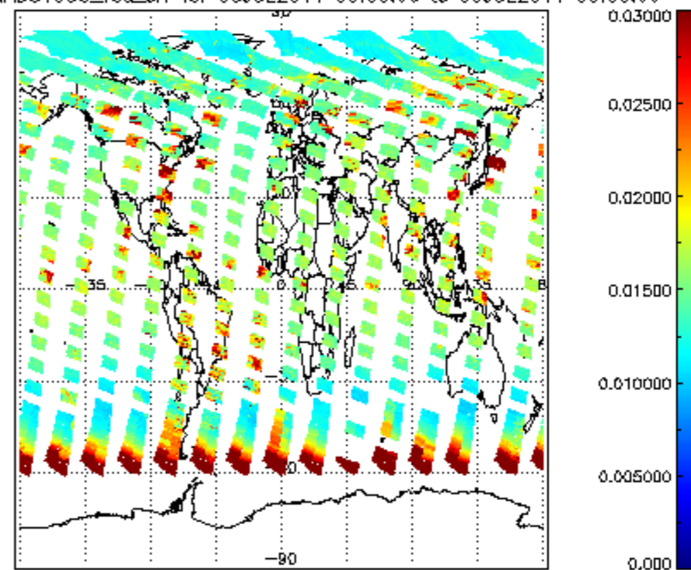
SCIOL2P_NADUV003_vcd_err for 08JUL2011 00:00:00 to 09JUL2011 00:00:00
