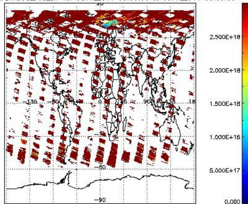
SCIO2P_NADIR3CO_vcd_err for 08JUL2011 00:00:00 to 09JUL2011 00:00:00
