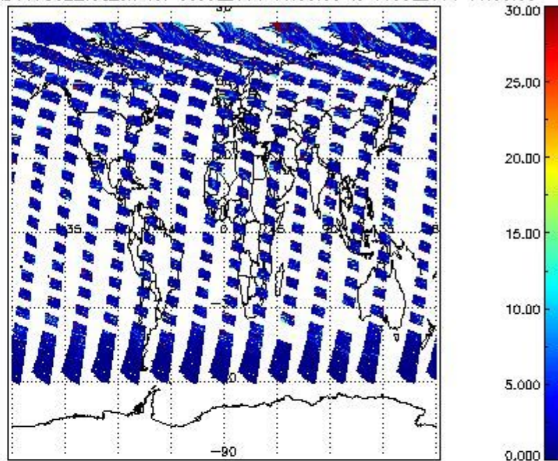
SCIOL2P_NADUV7S02_vcd_err for 08JUL2011 00:00:00 to 09JUL2011 00:00:00
