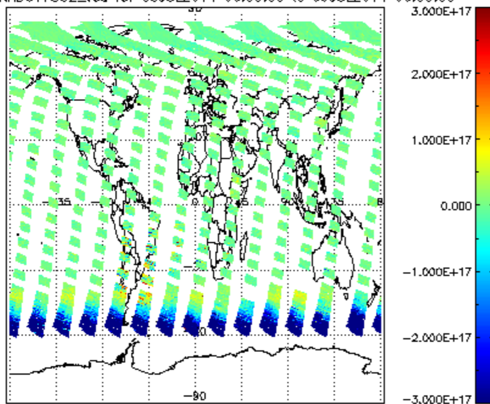
SCIOL2P_NADUV7S02_vcd for 08JUL2011 00:00:00 to 09JUL2011 00:00:00
