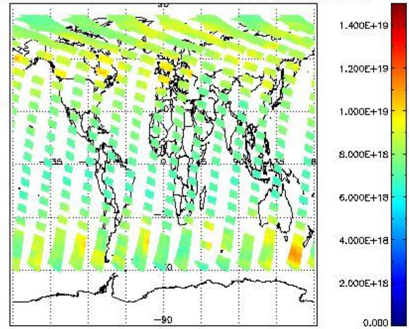
SCIOL2P_NADUV003_vcd for 08JUL2011 00:00:00 to 09JUL2011 00:00:00
