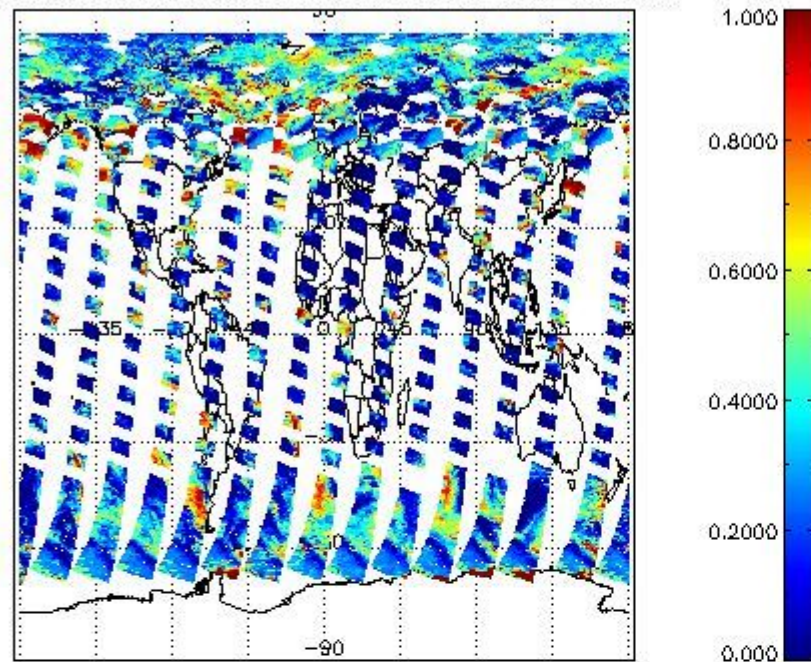
cL_frac for 08JUL2011 00:00:00 to 09JUL2011 00:00:00
