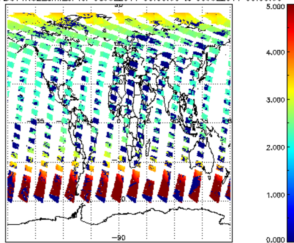
SCIOL2P_NADUV1NO2_amf_cl for 08JUL2011 00:00:00 to 09JUL2011 00:00:00
