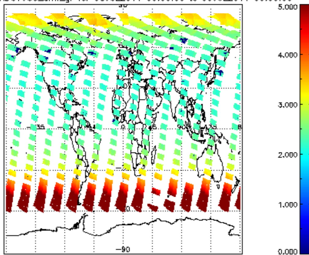
SCIOL2P_NADUV003_amf_gr for 08JUL2011 00:00:00 to 09JUL2011 00:00:00
