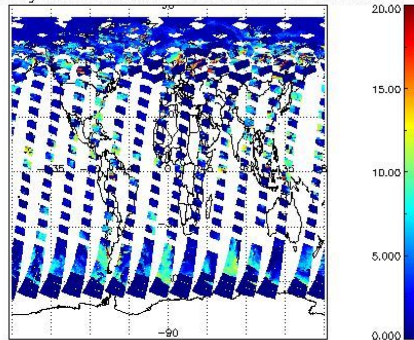
cL_top_height for 08JUL2011 00:00:00 to 09JUL2011 00:00:00
