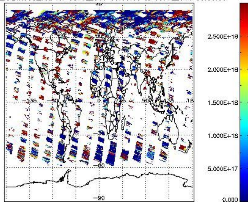
SCIO2P_NADIR3CO_vcd for 08JUL2011 00:00:00 to 09JUL2011 00:00:00
