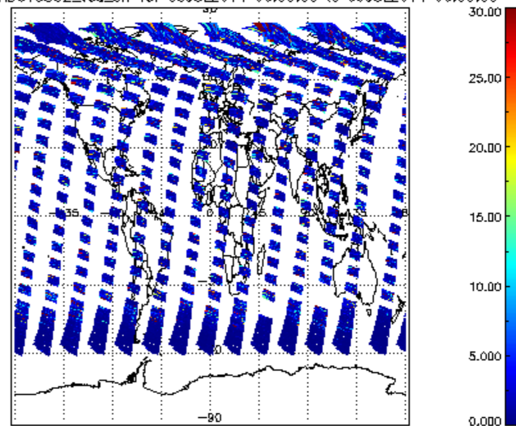
SCIOL2P_NADUV5S02_vcd_err for 08JUL2011 00:00:00 to 09JUL2011 00:00:00
