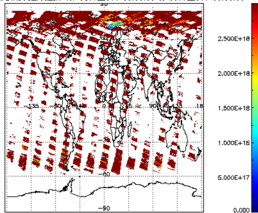
SCIOL2P_NADIR3CO_vcd_err for 08JUL2011 00:00:00 to 09JUL2011 00:00:00
