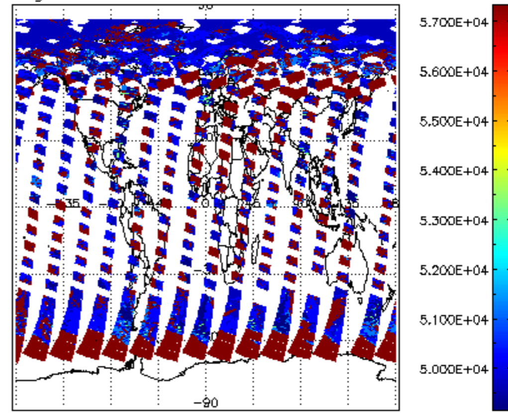
cloud_flags for 08JUL2011 00:00:00 to 09JUL2011 00:00:00
