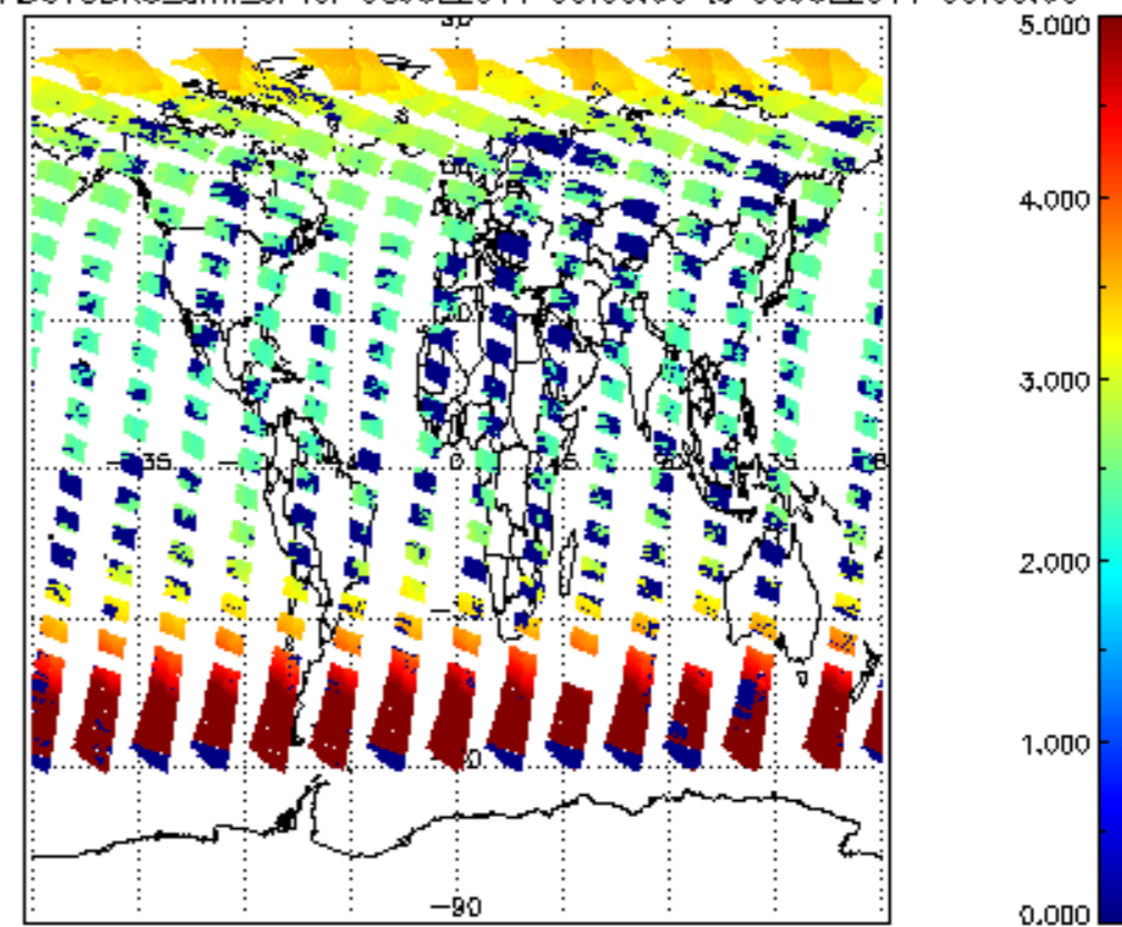
SCIOL2P_NADUV3BRO_arnf_cl for 08JUL2011 00:00:00 to 09JUL2011 00:00:00
