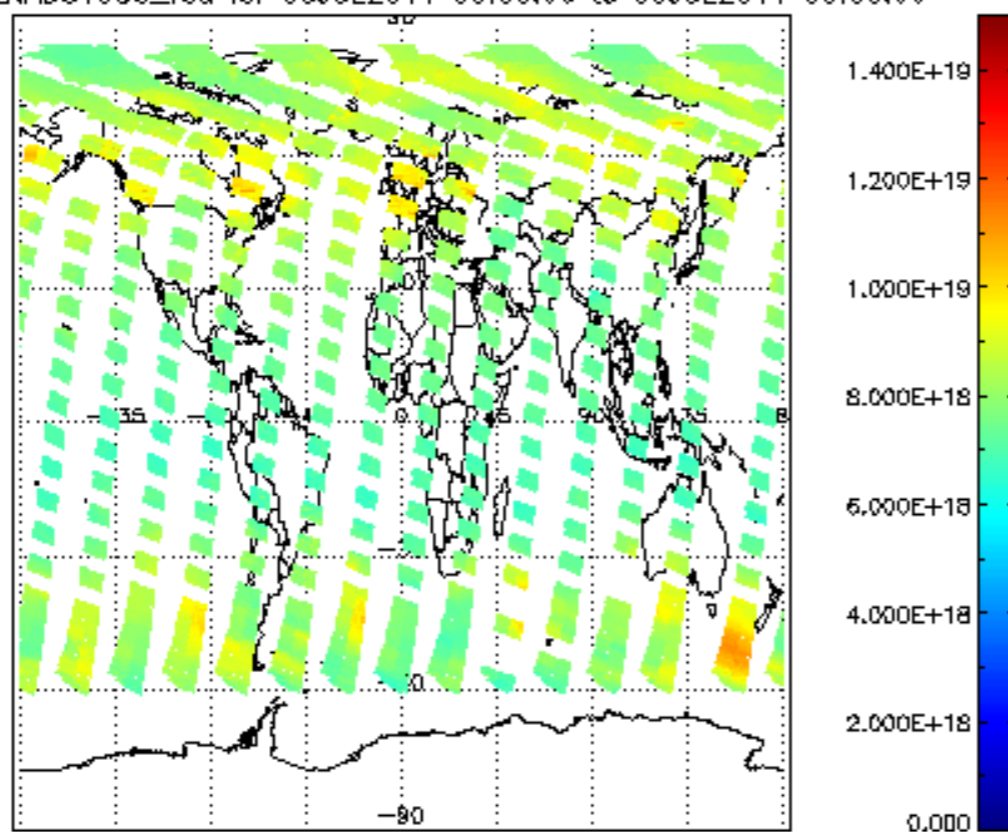
SCIOL2P_NADUV003_vcd for 08JUL2011 00:00:00 to 09JUL2011 00:00:00
