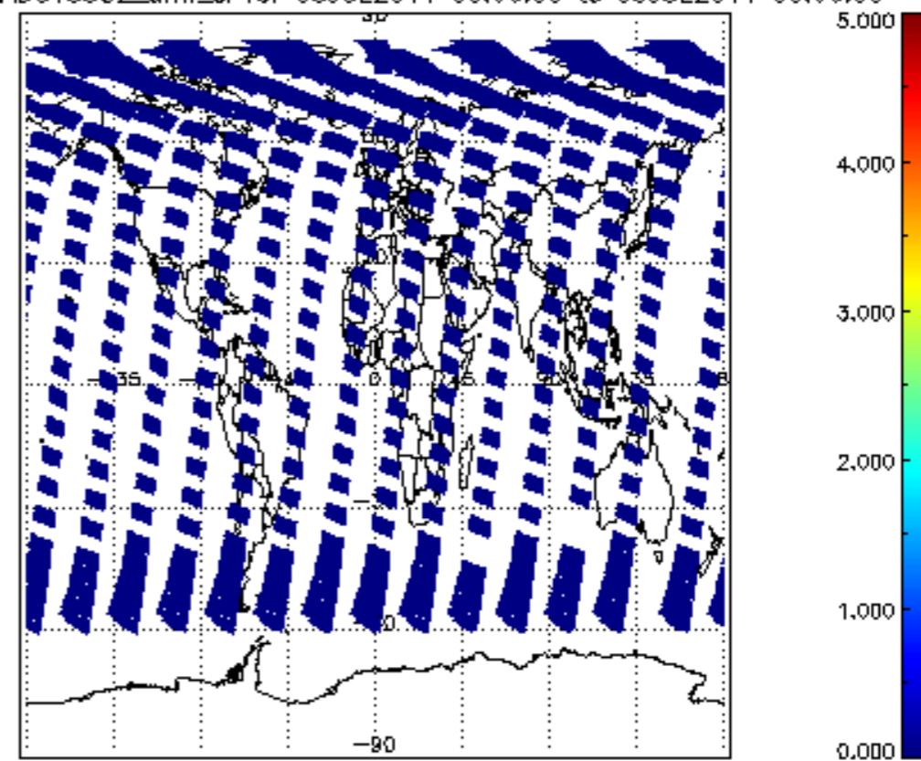
SCIOL2P_NADUV5S02_amf_cl for 08JUL2011 00:00:00 to 09JUL2011 00:00:00
