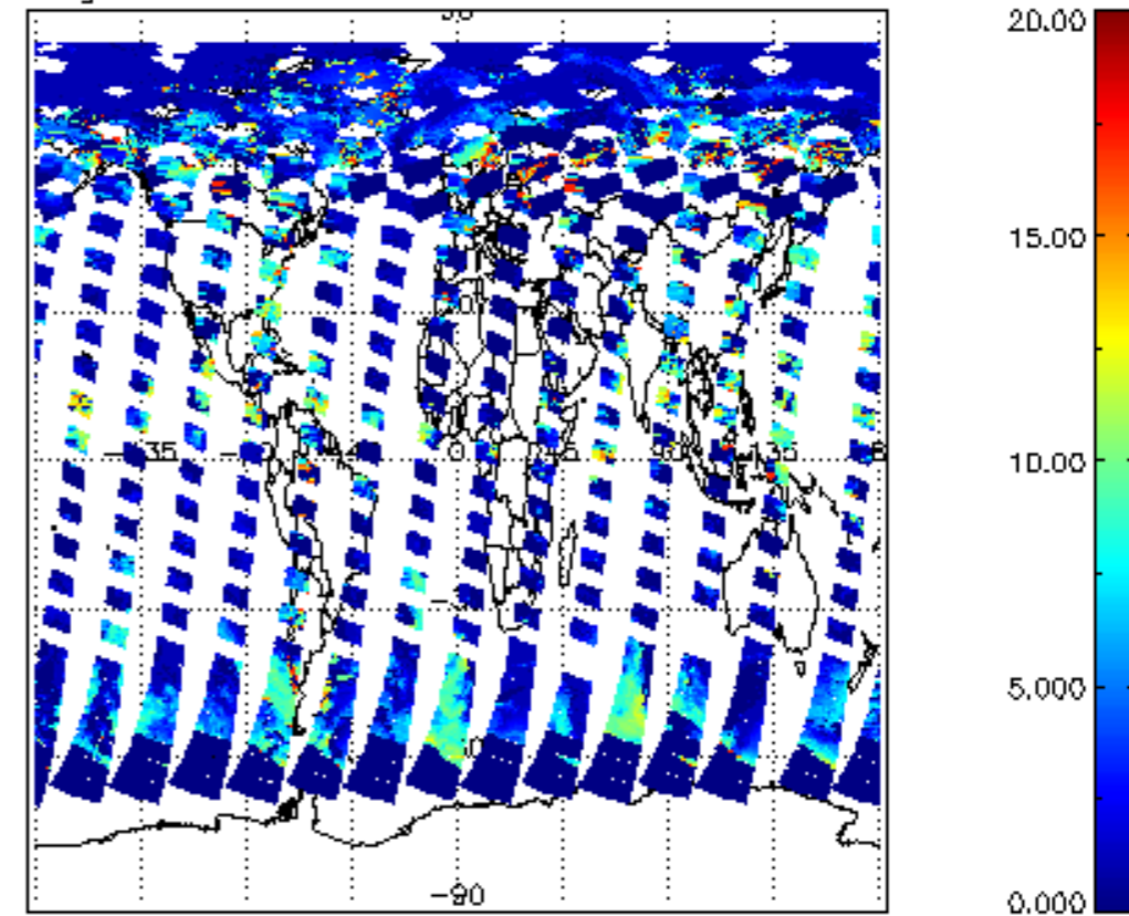
cl_top_height for 08JUL2011 00:00:00 to 09JUL2011 00:00:00
