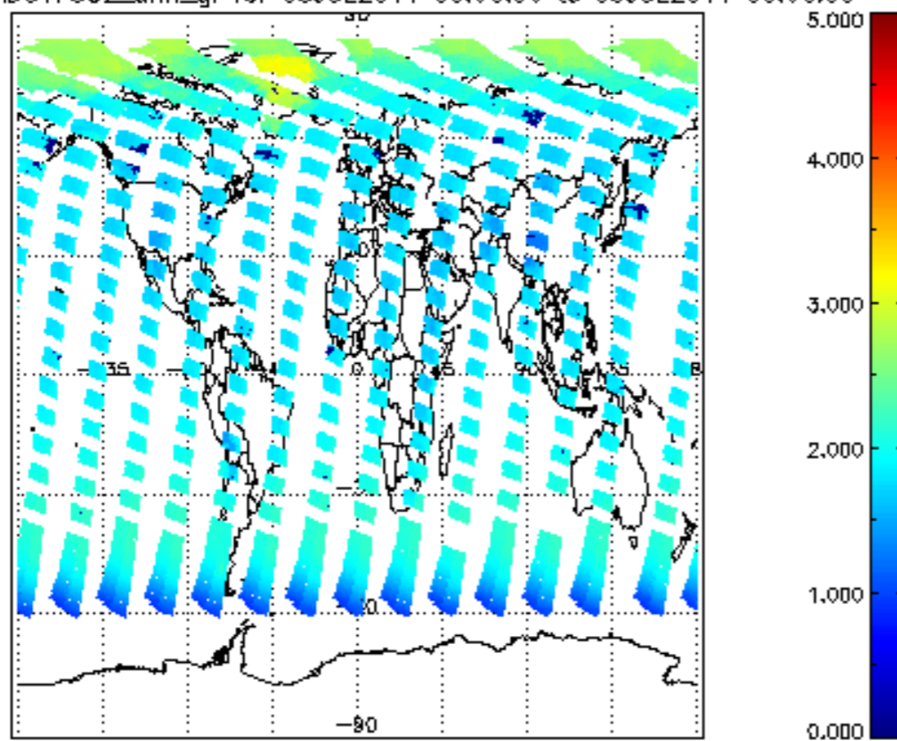
SCIOL2P_NADUV7S02_amf_gr for 08JUL2011 00:00:00 to 09JUL2011 00:00:00
