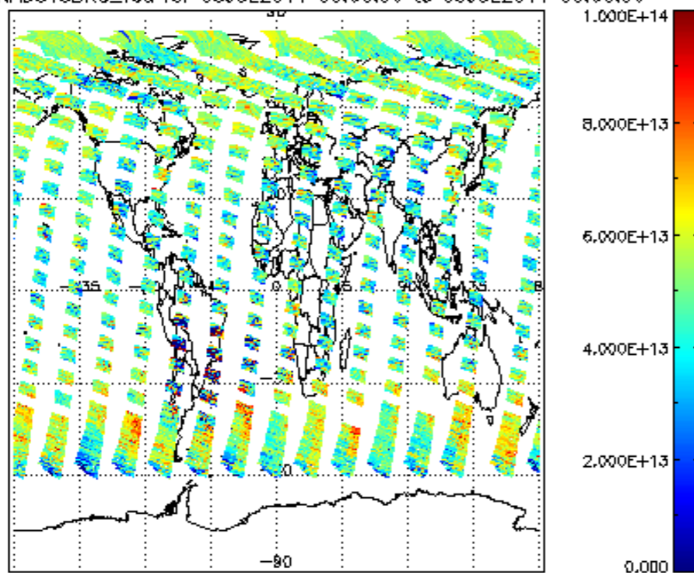
SCIOL2P_NADUV3BRO_vcd for 08JUL2011 00:00:00 to 09JUL2011 00:00:00
