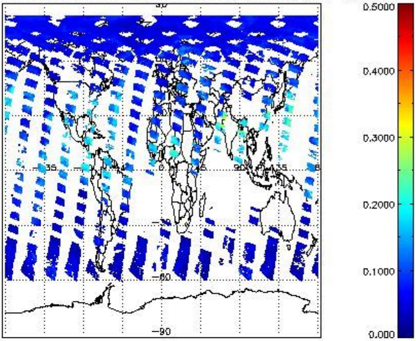
SCIOL2P_NADUV8H2O_vcd_err for 08JUL2011 00:00:00 to 09JUL2011 00:00:00
