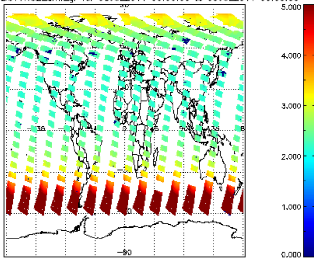
SCIOL2P_NADUV1NO2_amf_gr for 08JUL2011 00:00:00 to 09JUL2011 00:00:00
