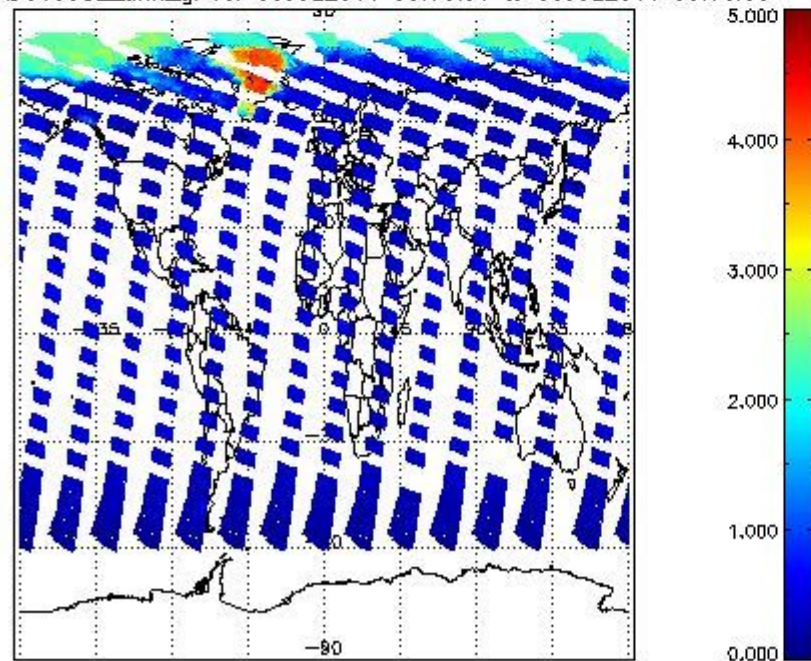
SCIOL2P_NADUV5S02_amf_gr for 08JUL2011 00:00:00 to 09JUL2011 00:00:00
