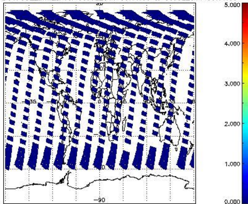
SCIOL2P_NADUV7S02_amf_cl for 08JUL2011 00:00:00 to 09JUL2011 00:00:00
