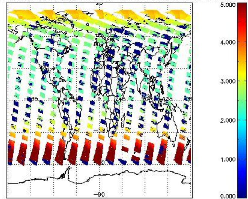
SCIOL2P_NADUV003_amf_cl for 08JUL2011 00:00:00 to 09JUL2011 00:00:00
