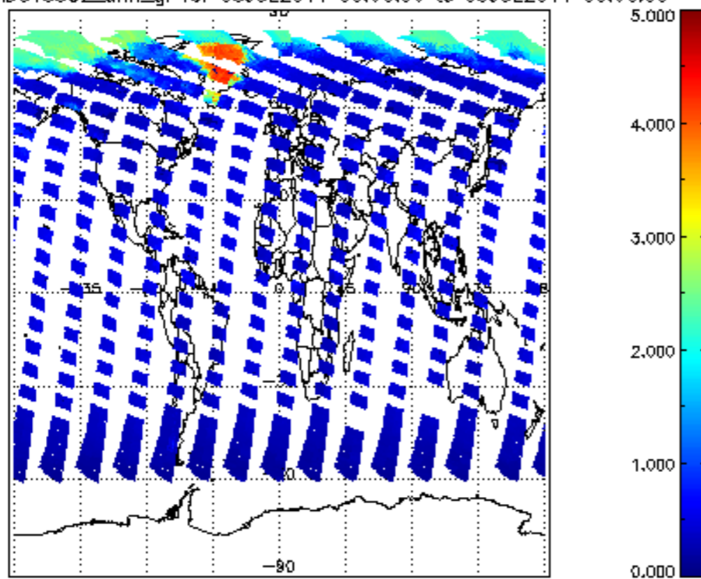
SCIOL2P_NADUV5S02_amf_gr for 08JUL2011 00:00:00 to 09JUL2011 00:00:00
