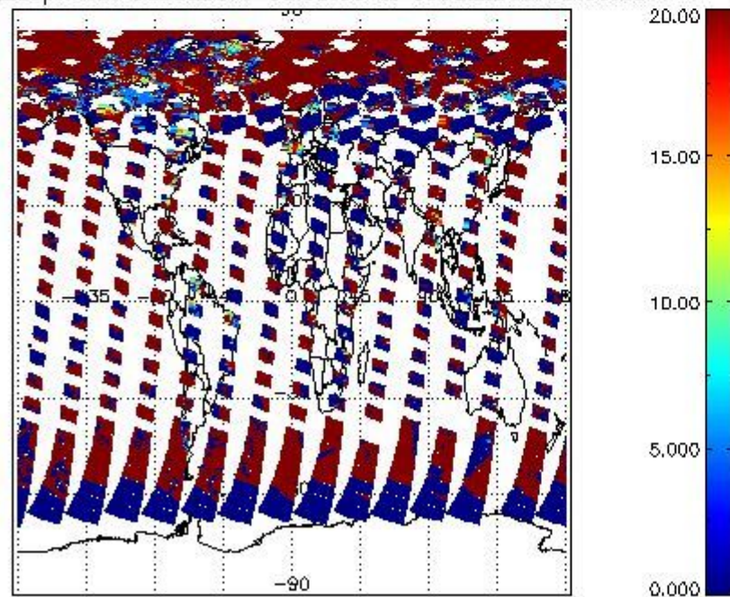
cL_opt_depth for 08JUL2011 00:00:00 to 09JUL2011 00:00:00
