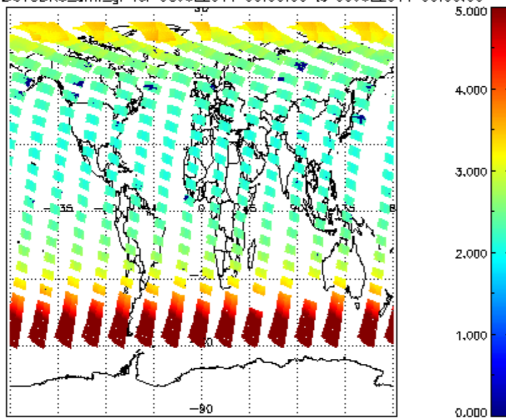
SCIOL2P_NADUV3BRO_arnf_gr for 08JUL2011 00:00:00 to 09JUL2011 00:00:00
