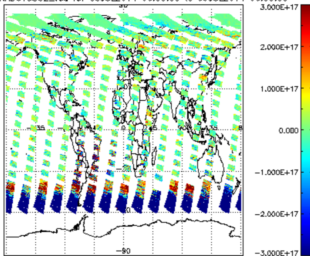
SCIOL2P_NADUV5S02_vcd for 08JUL2011 00:00:00 to 09JUL2011 00:00:00
