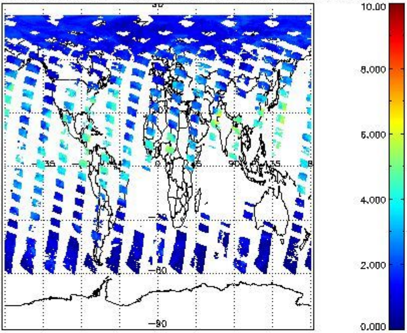
SCIOL2P_NADUV8H2O_vcd for 08JUL2011 00:00:00 to 09JUL2011 00:00:00
