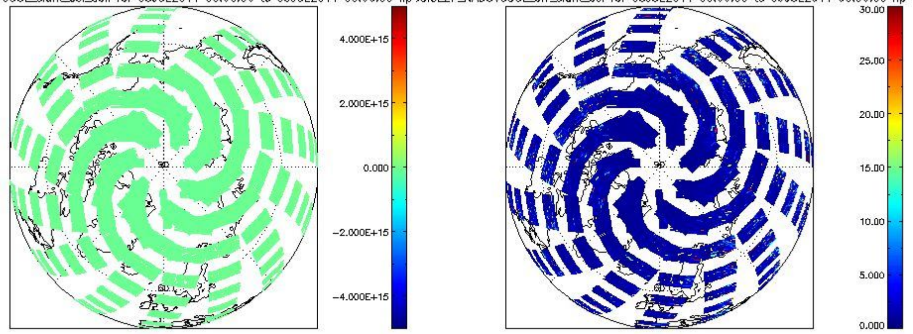
SCIOI2P_NADUV6OCLslant_col_den for 08JUL2011 00:00:00 to 09JUL2011 00:00:00 np SCIOI2P_NADUV6OCLarr_slant_col for 08JUL2011 00:00:00 to 09JUL2011 00:00:00 np
