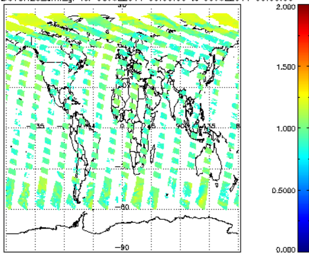
SCIOL2P_NADUV8H20_amf_gr for 08JUL2011 00:00:00 to 09JUL2011 00:00:00
