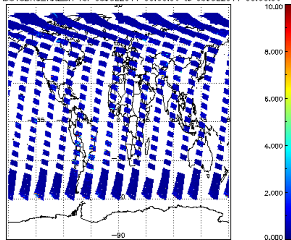
SCIOL2P_NADUV3BRO_vcd_err for 08JUL2011 00:00:00 to 09JUL2011 00:00:00
