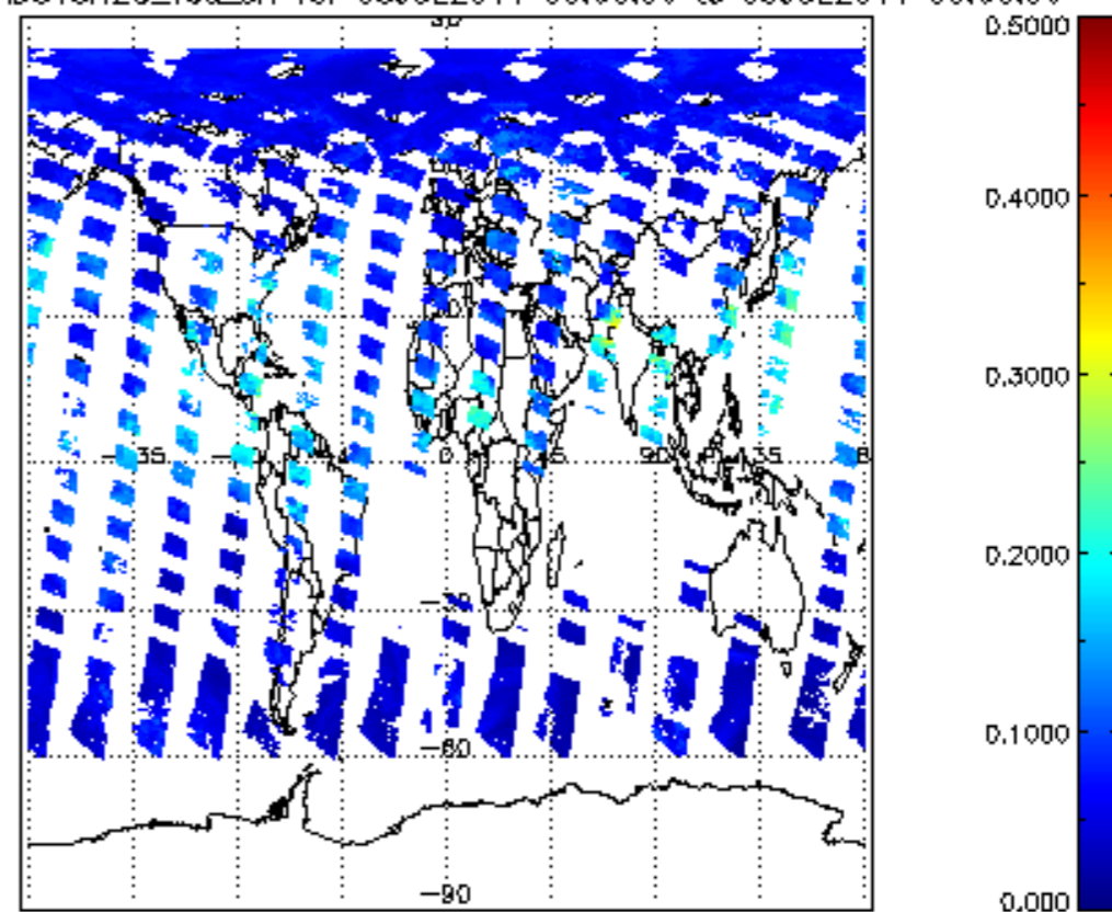
SCIOL2P_NADUV8H20_vcd_err for 08JUL2011 00:00:00 to 09JUL2011 00:00:00
