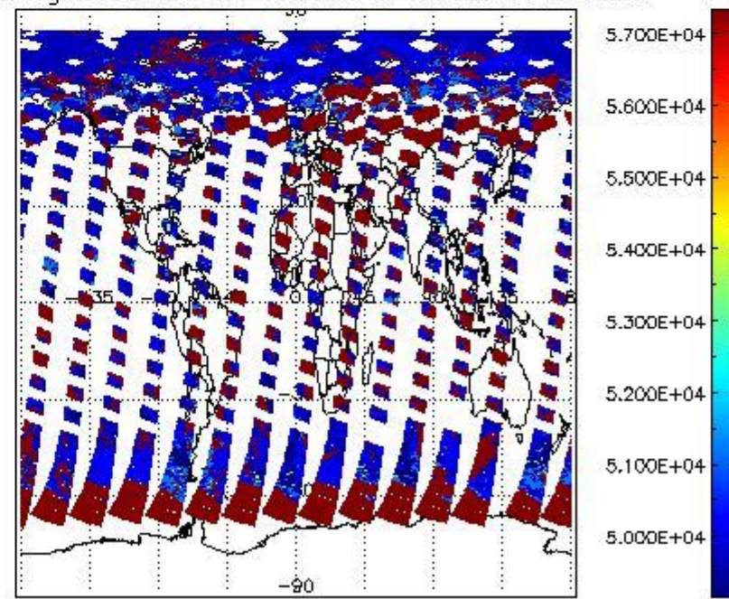
cloud_flags for 08JUL2011 00:00:00 to 09JUL2011 00:00:00
