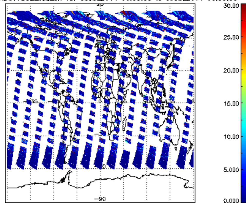
SCIOL2P_NADUV7S02_vcd_err for 08JUL2011 00:00:00 to 09JUL2011 00:00:00
