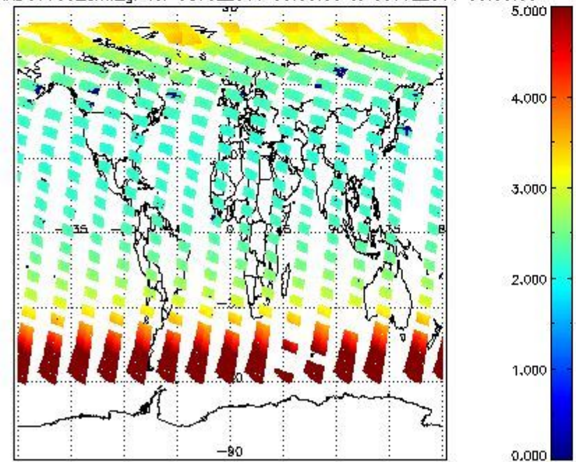
SCIOL2P_NADUV003_amf_gr for 08JUL2011 00:00:00 to 09JUL2011 00:00:00
