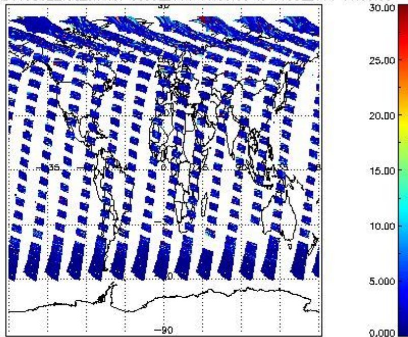
SCIOL2P_NADUV5S02_vcd_err for 08JUL2011 00:00:00 to 09JUL2011 00:00:00
