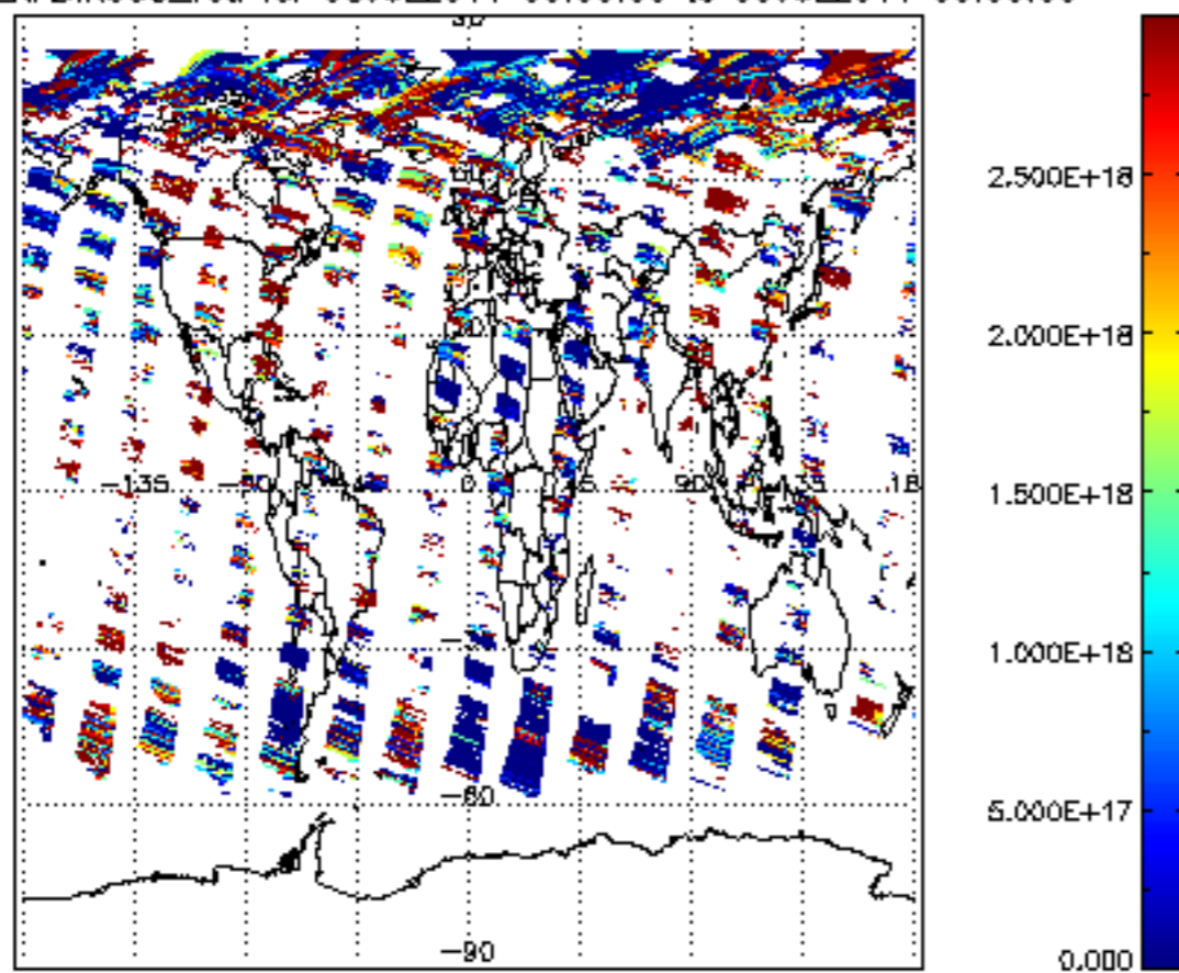
SCIOL2P_NADIR3CO_vcd for 08JUL2011 00:00:00 to 09JUL2011 00:00:00
