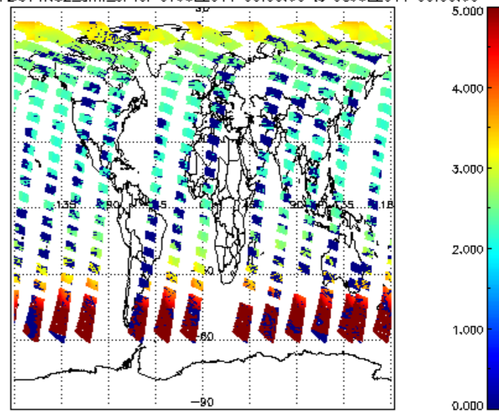
SCIOL2P_NADUV1NO2_amf_cl for 07JUL2011 00:00:00 to 08JUL2011 00:00:00
