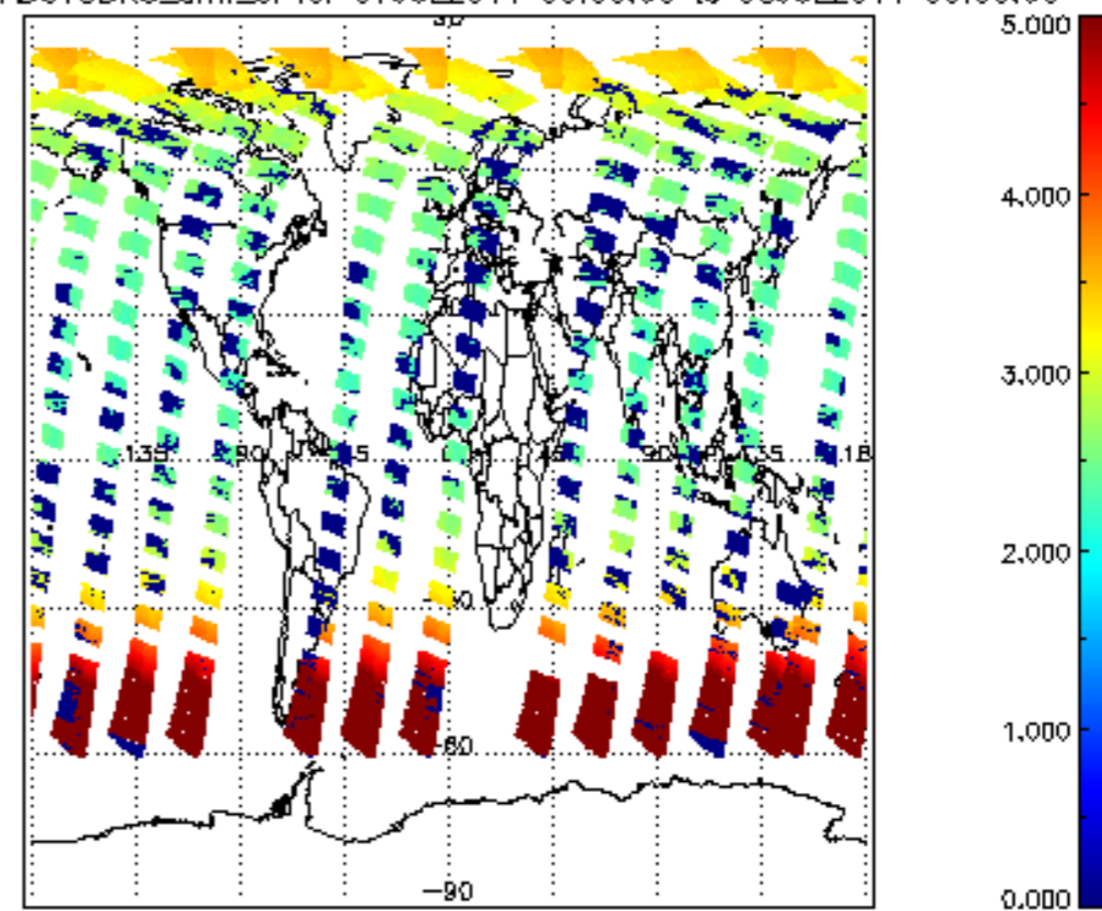
SCIOL2P_NADUV3BRO_amf_cl for 07JUL2011 00:00:00 to 08JUL2011 00:00:00
