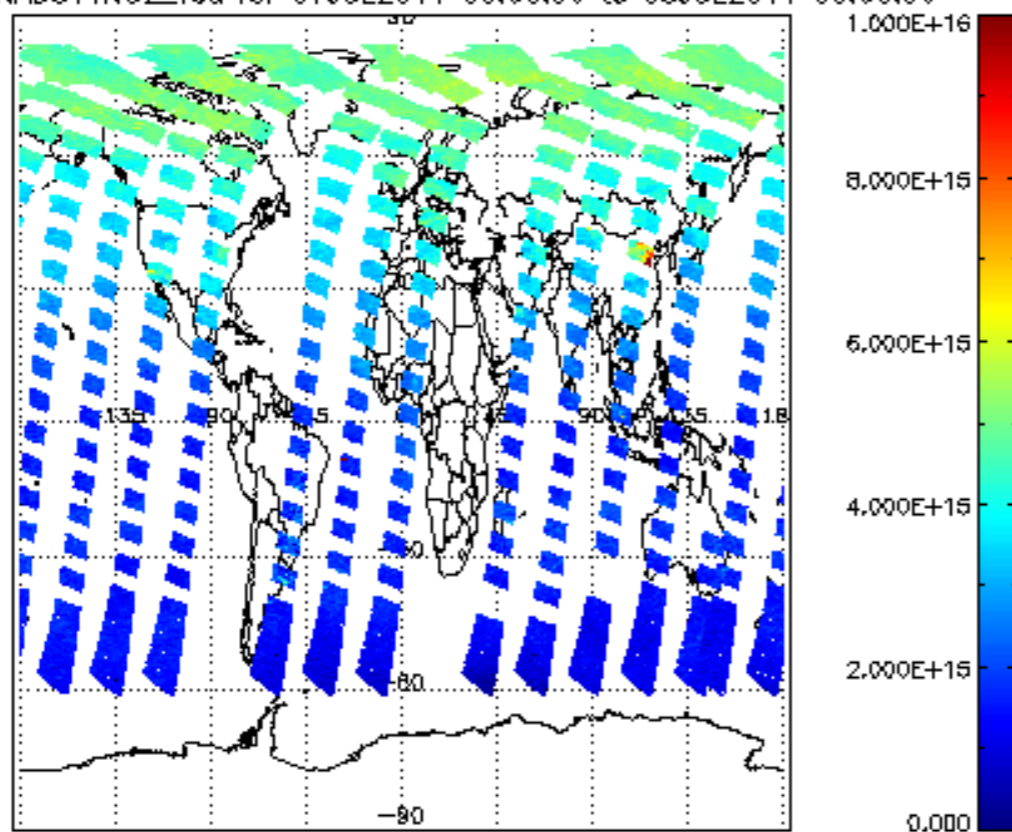
SCIOL2P_NADUV1NO2_vcd for 07JUL2011 00:00:00 to 08JUL2011 00:00:00
