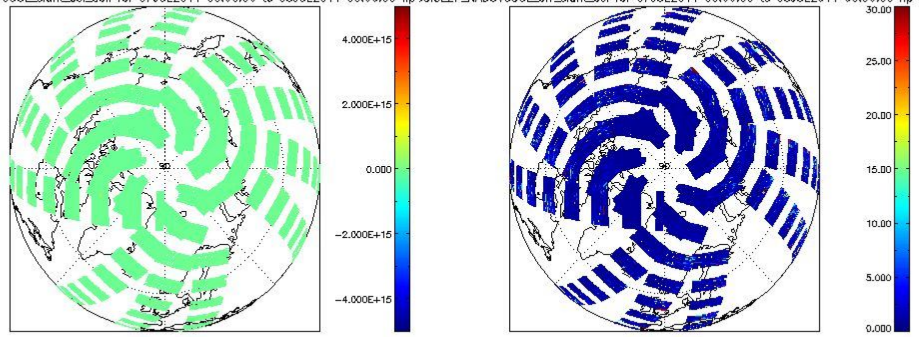
SCIOI2P_NADUV6OCLslant_col_den for 07JUL2011 00:00:00 to 08JUL2011 00:00:00 np SCIOI2P_NADUV6OCLarr_slant_col for 07JUL2011 00:00:00 to 08JUL2011 00:00:00 np
