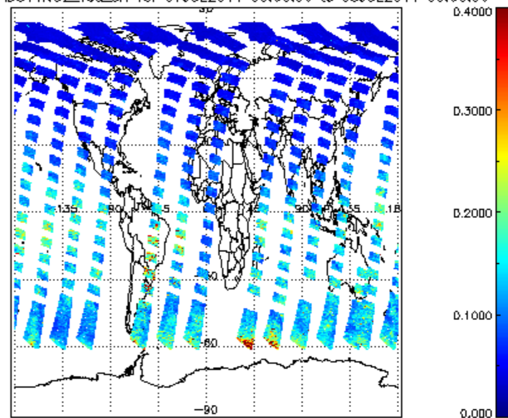
SCIOL2P_NADUV1NO2_vcd_err for 07JUL2011 00:00:00 to 08JUL2011 00:00:00
