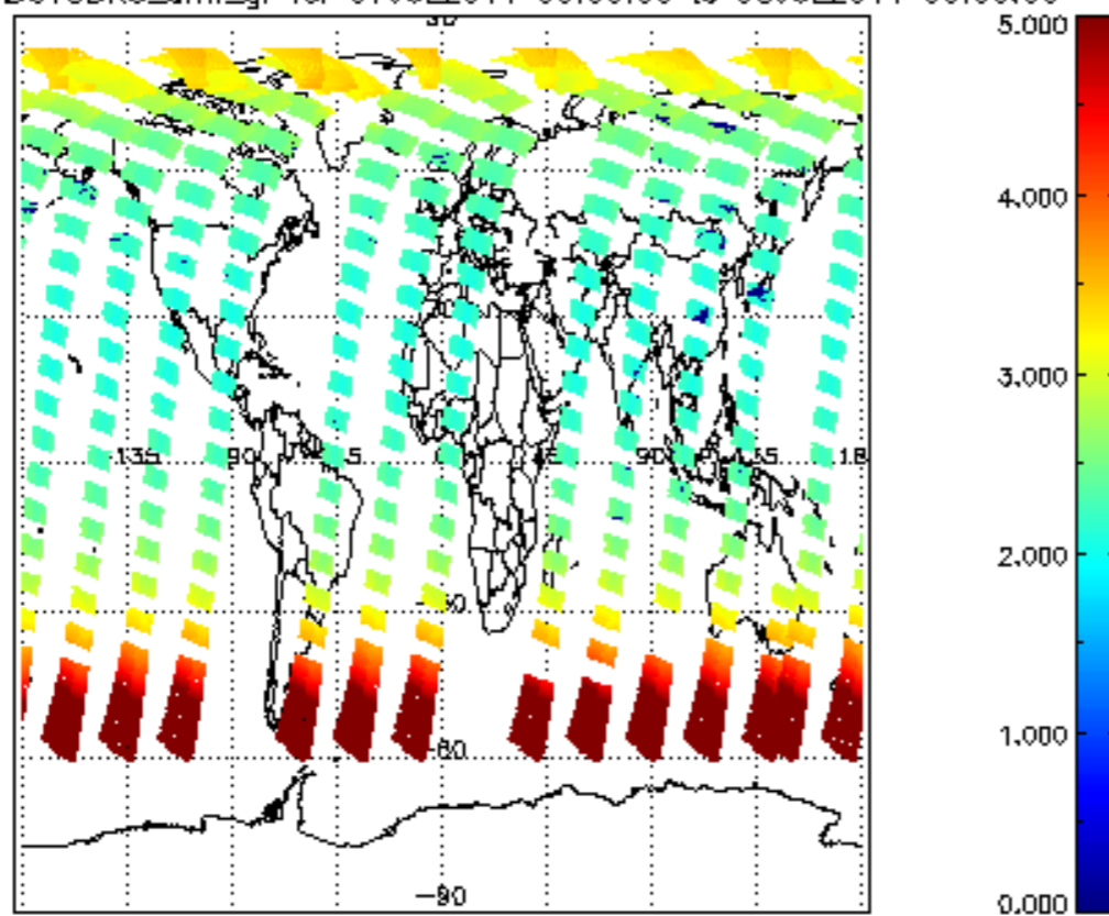
SCIOL2P_NADUV3BRO_amf_gr for 07JUL2011 00:00:00 to 08JUL2011 00:00:00
