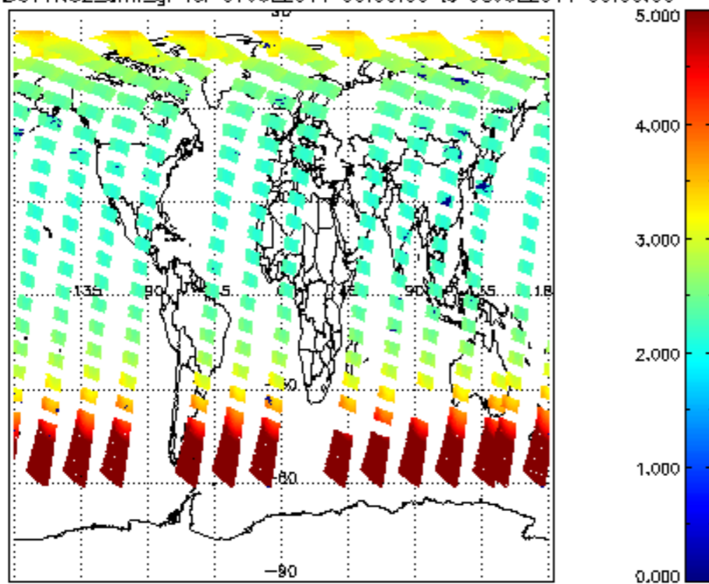
SCIOL2P_NADUV1NO2_amf_gr for 07JUL2011 00:00:00 to 08JUL2011 00:00:00
