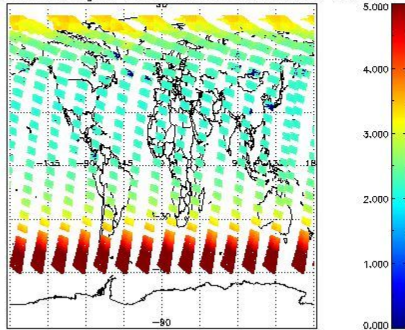
SCIOL2P_NADUV003_amf_gr for 06JUL2011 00:00:00 to 07JUL2011 00:00:00
