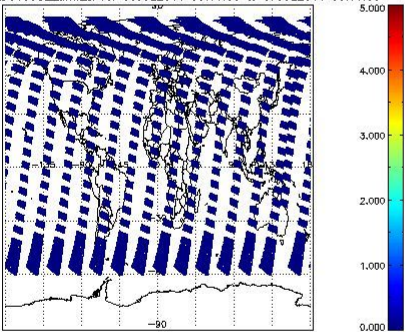
SCIOL2P_NADUV5S02_amf_cl for 06JUL2011 00:00:00 to 07JUL2011 00:00:00
