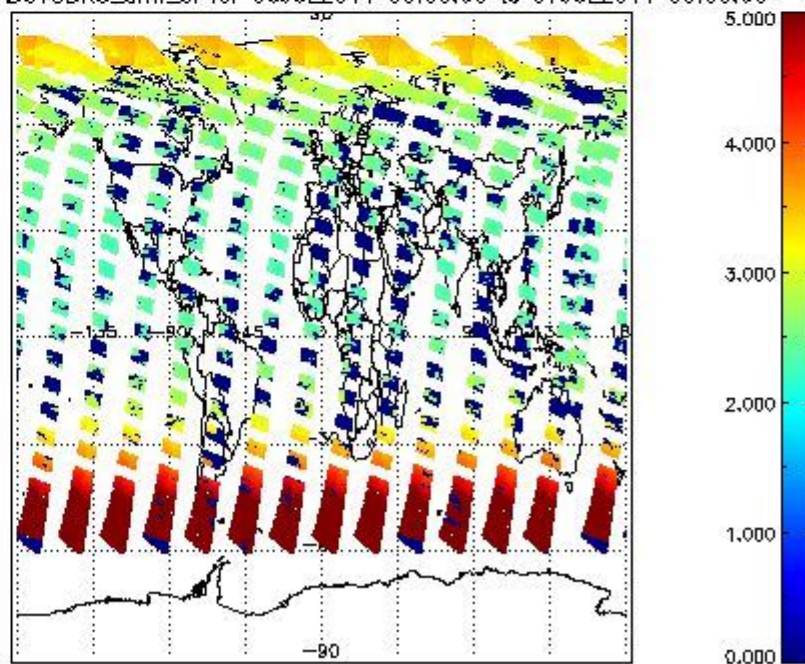
SCIOL2P_NADUV3BRO_amf_cl for 06JUL2011 00:00:00 to 07JUL2011 00:00:00
