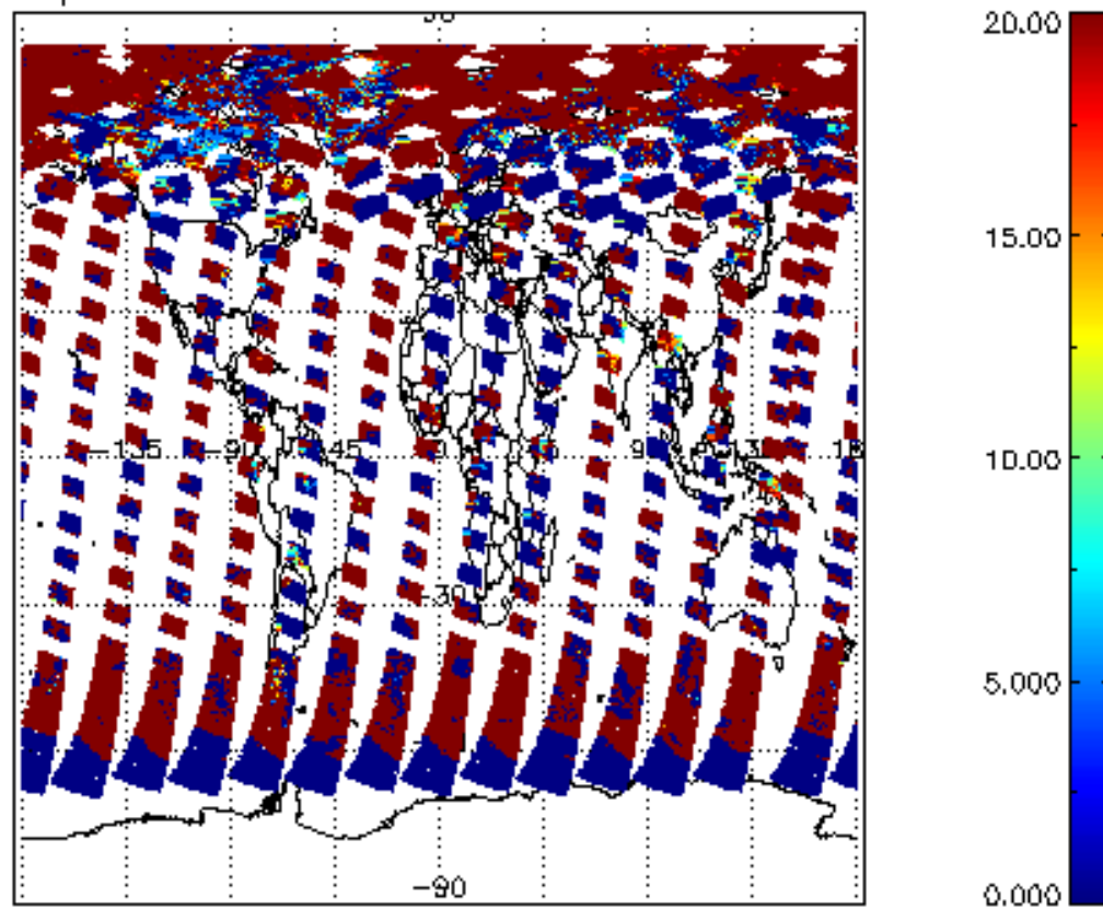
cl_lopt_depth for 06JUL2011 00:00:00 to 07JUL2011 00:00:00
