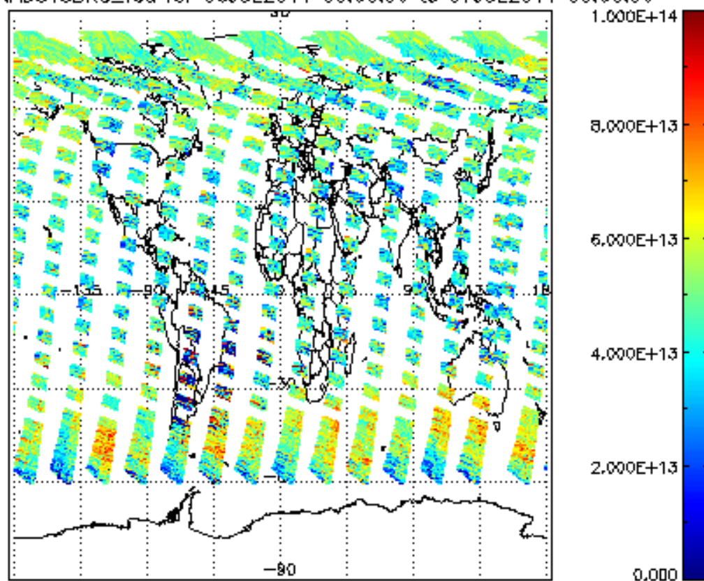
SCIOL2P_NADUV3BRO_vcd for 06JUL2011 00:00:00 to 07JUL2011 00:00:00
