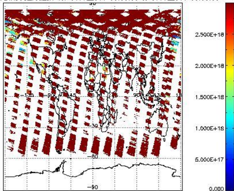
SCIDL2P_NADIR3CO_vcd_err for 06JUL2011 00:00:00 to 07JUL2011 00:00:00
