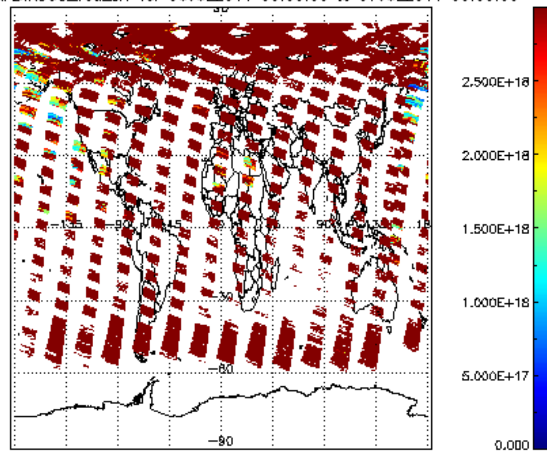
SCIOL2P_NADIR3CO_vcd_err for 06JUL2011 00:00:00 to 07JUL2011 00:00:00
