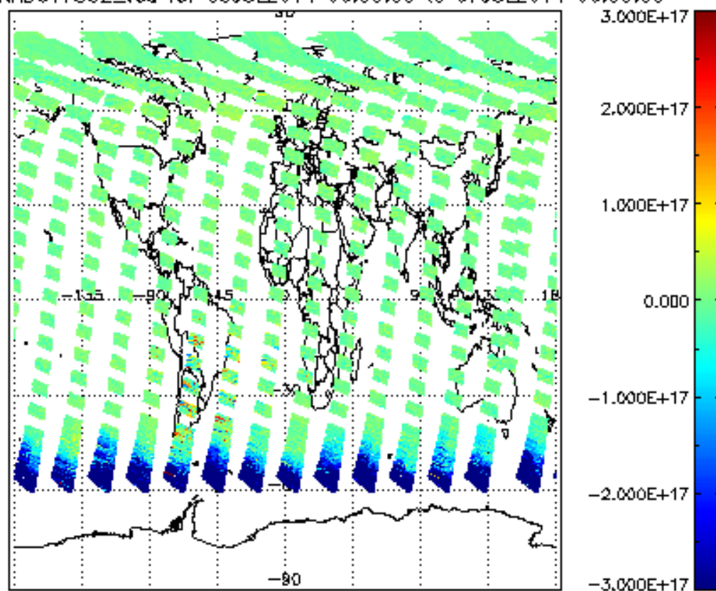
SCIOL2P_NADUV7S02_vcd for 06JUL2011 00:00:00 to 07JUL2011 00:00:00
