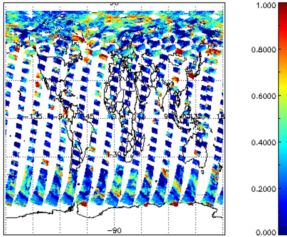
cl_frac for 06JUL2011 00:00:00 to 07JUL2011 00:00:00
