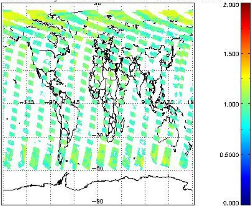
SCIOL2P_NADUV8H20_amf_gr for 06JUL2011 00:00:00 to 07JUL2011 00:00:00
