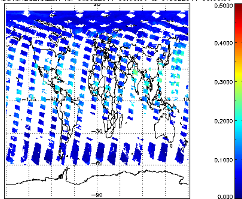
SCIOL2P_NADUV8H2O_vcd_err for 06JUL2011 00:00:00 to 07JUL2011 00:00:00
