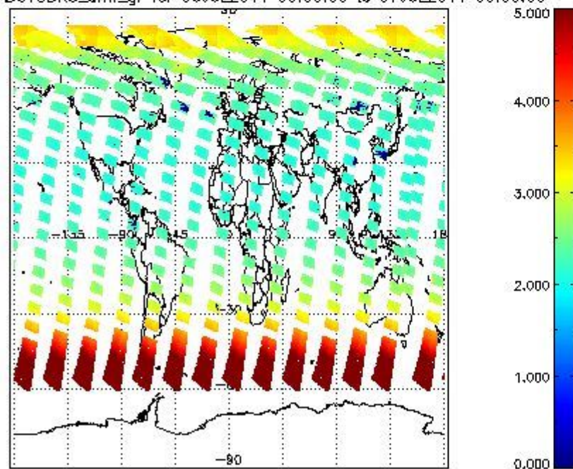
SCIOL2P_NADUV3BRO_amf_gr for 06JUL2011 00:00:00 to 07JUL2011 00:00:00
