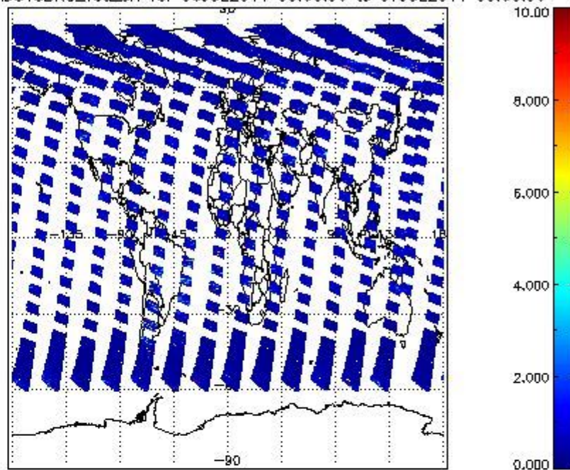
SCIOL2P_NADUV3BRO_vcd_err for 06JUL2011 00:00:00 to 07JUL2011 00:00:00
