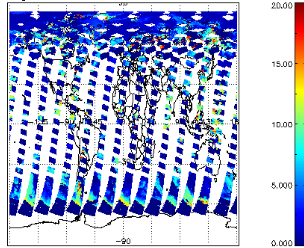
cl_top_height for 06JUL2011 00:00:00 to 07JUL2011 00:00:00
