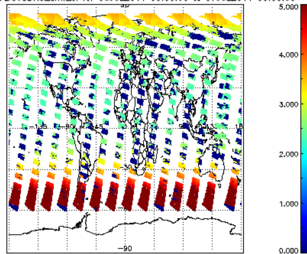
SCIOL2P_NADUV3BRO_amf_cl for 06JUL2011 00:00:00 to 07JUL2011 00:00:00
