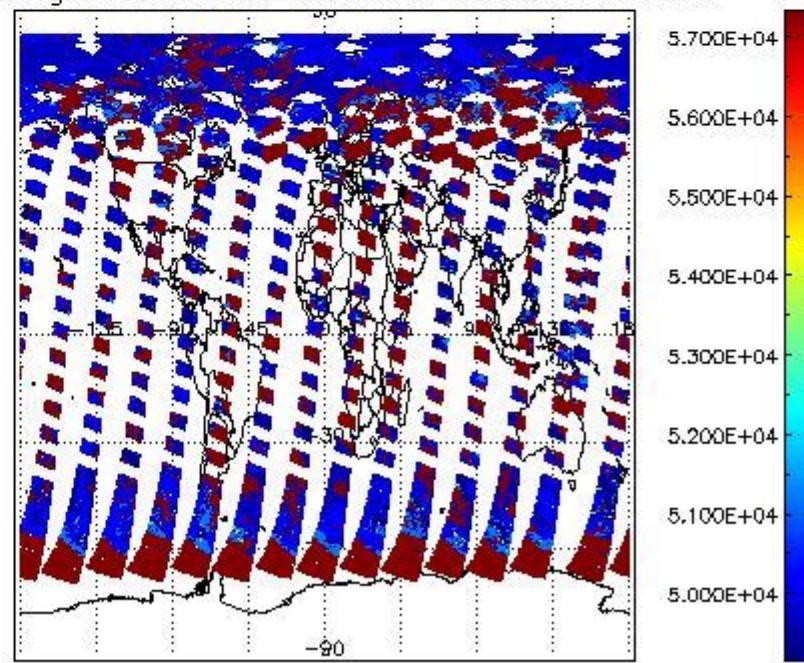
cloud_flags for 06JUL2011 00:00:00 to 07JUL2011 00:00:00
