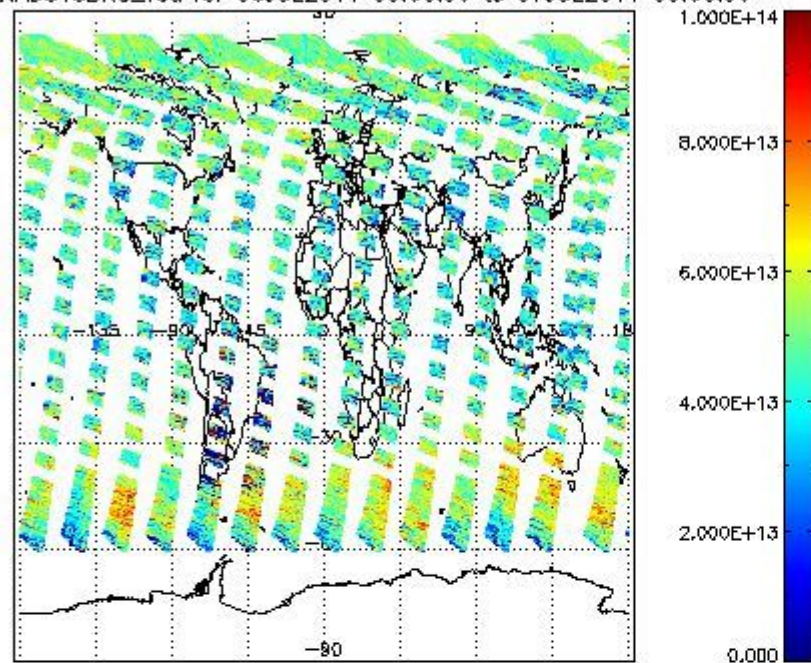
SCIOL2P_NADUV3BRO_vcd for 06JUL2011 00:00:00 to 07JUL2011 00:00:00
