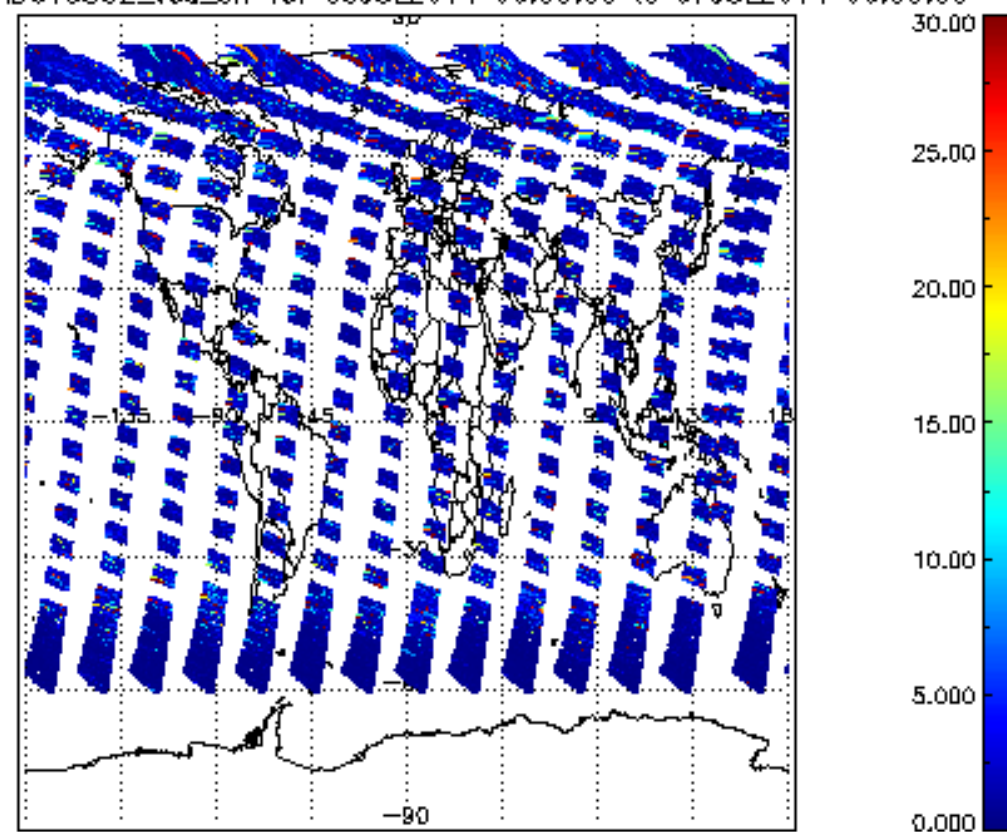
SCIOL2P_NADUV5S02_vcd_err for 06JUL2011 00:00:00 to 07JUL2011 00:00:00
