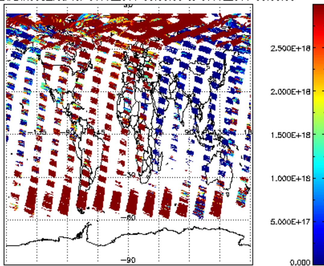
SCIOL2P_NADIR3CO_vcd for 06JUL2011 00:00:00 to 07JUL2011 00:00:00
