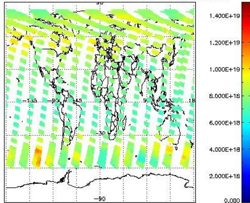
SCIOL2P_NADUV003_vcd for 06JUL2011 00:00:00 to 07JUL2011 00:00:00
