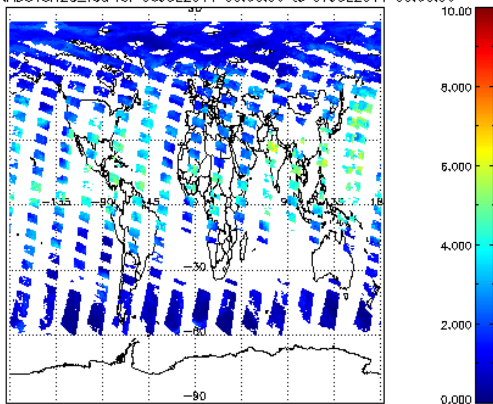
SCIOL2P_NADUV8H2O_vcd for 06JUL2011 00:00:00 to 07JUL2011 00:00:00
