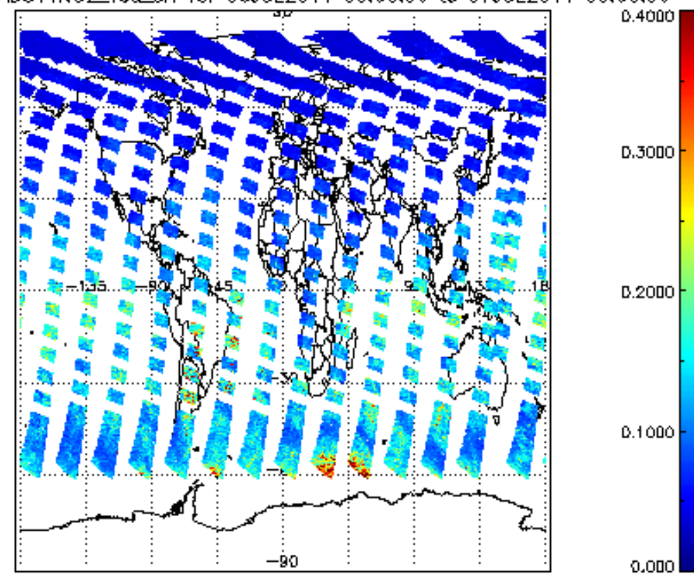
SCIOL2P_NADUV1NO2_vcd_err for 06JUL2011 00:00:00 to 07JUL2011 00:00:00
