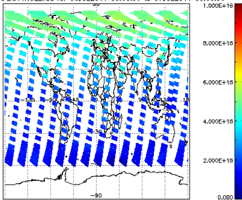
SCIOL2P_NADUV1NO2_vcd for 06JUL2011 00:00:00 to 07JUL2011 00:00:00
