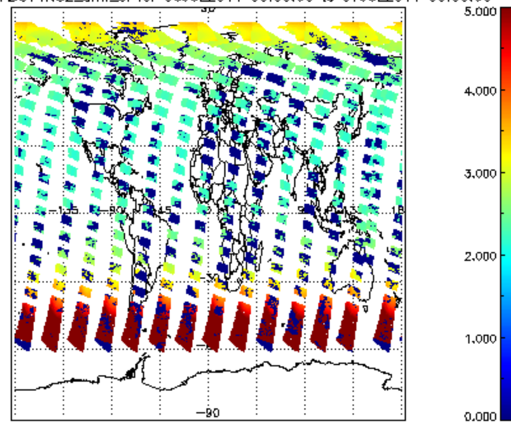
SCIOL2P_NADUV1NO2_amf_cl for 06JUL2011 00:00:00 to 07JUL2011 00:00:00
