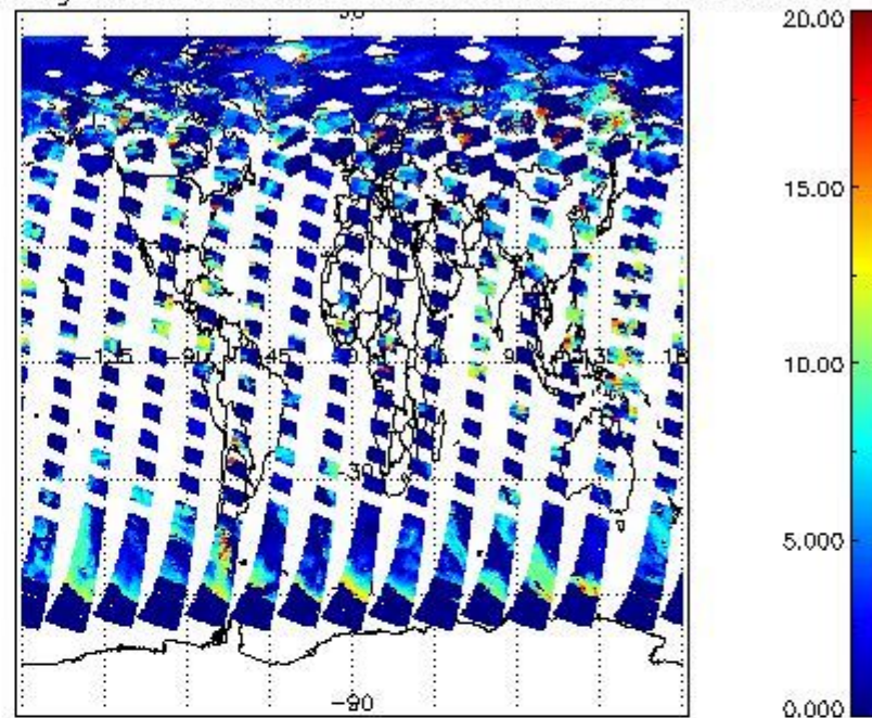
cL_top_height for 06JUL2011 00:00:00 to 07JUL2011 00:00:00
