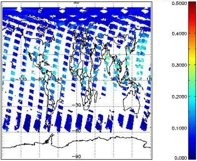
SCIOL2P_NADUV8H20_vcd_err for 06JUL2011 00:00:00 to 07JUL2011 00:00:00
