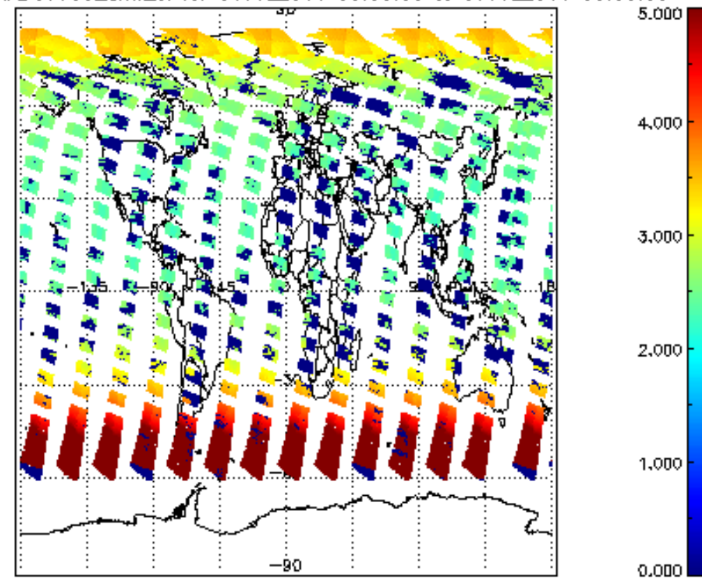
SCIOL2P_NADUV003_amf_cl for 06JUL2011 00:00:00 to 07JUL2011 00:00:00
