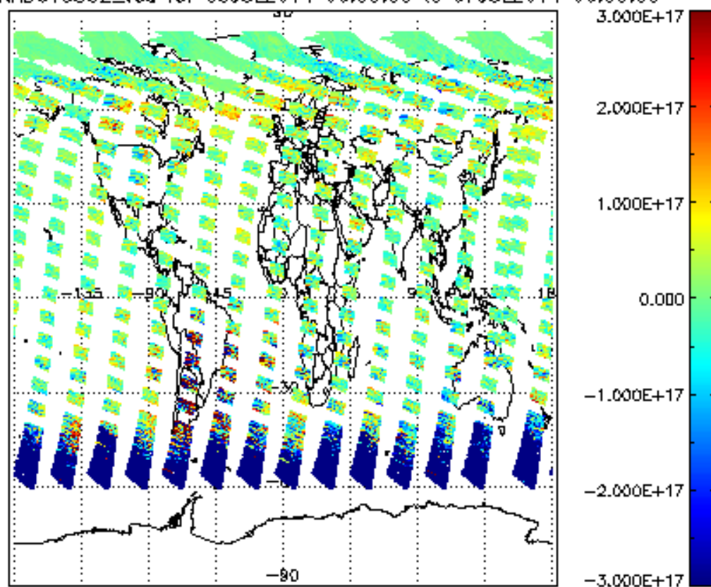
SCIOL2P_NADUV5S02_vcd for 06JUL2011 00:00:00 to 07JUL2011 00:00:00
