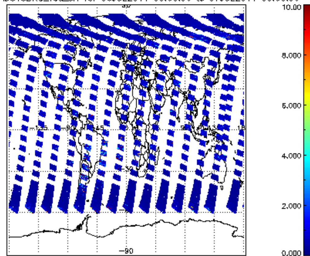
SCIOL2P_NADUV3BRO_vcd_err for 06JUL2011 00:00:00 to 07JUL2011 00:00:00
