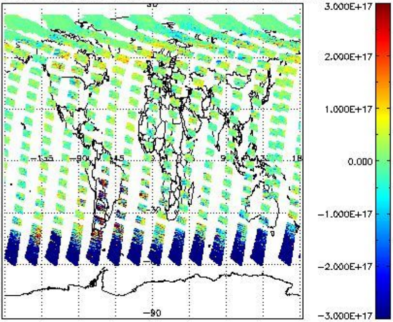
SCIOL2P_NADUV5S02_vcd for 06JUL2011 00:00:00 to 07JUL2011 00:00:00
