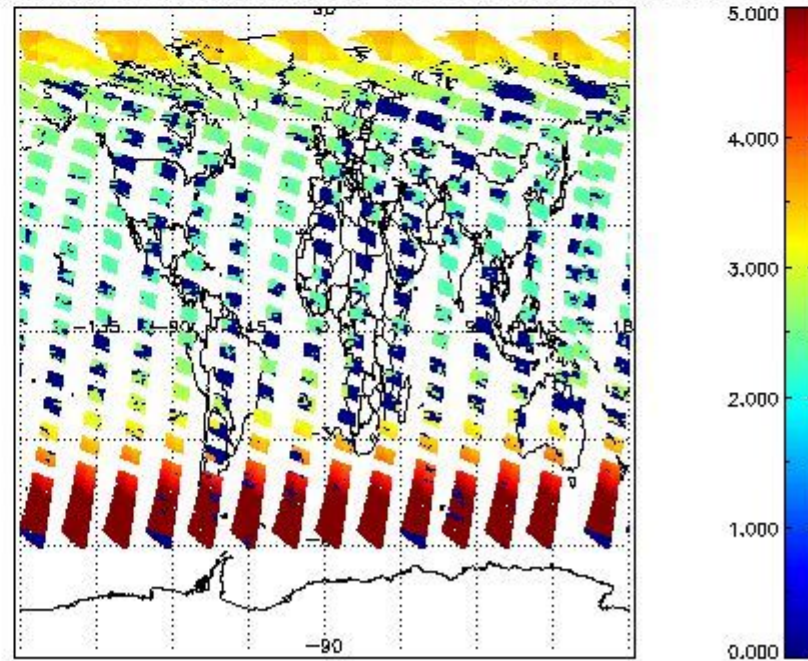
SCIOL2P_NADUV003_amf_cl for 06JUL2011 00:00:00 to 07JUL2011 00:00:00
