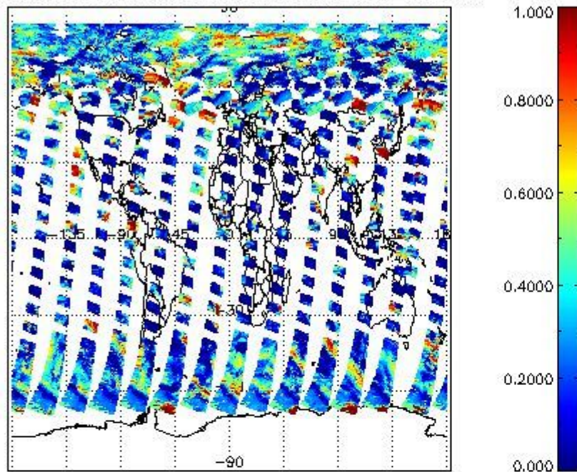
cL_frac for 06JUL2011 00:00:00 to 07JUL2011 00:00:00
