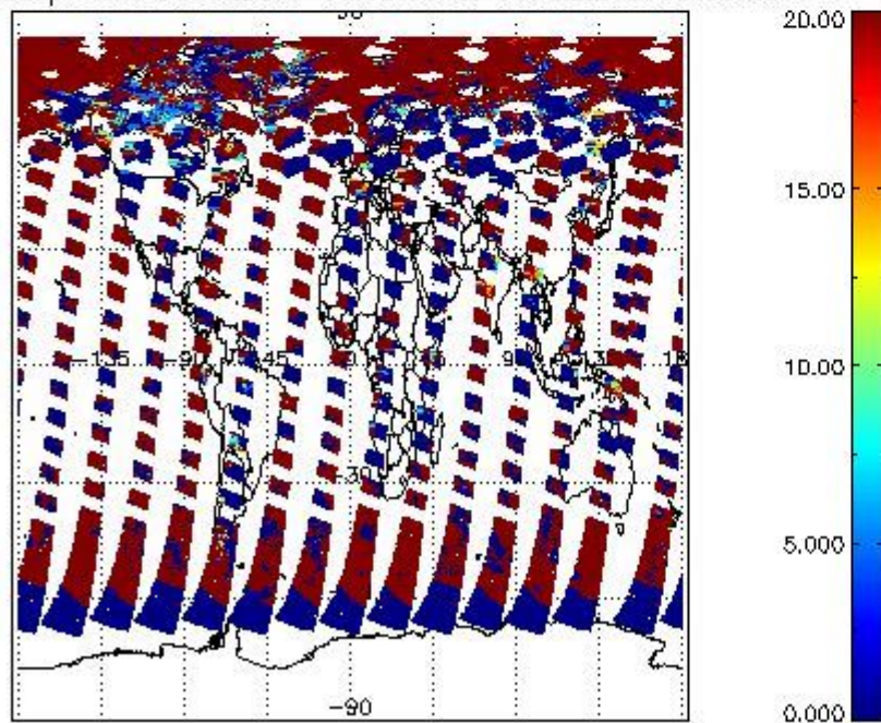
cL_opt_depth for 06JUL2011 00:00:00 to 07JUL2011 00:00:00
