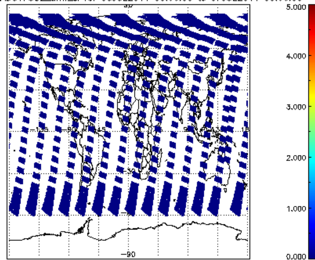
SCIOL2P_NADUV7S02_amf_cl for 06JUL2011 00:00:00 to 07JUL2011 00:00:00
