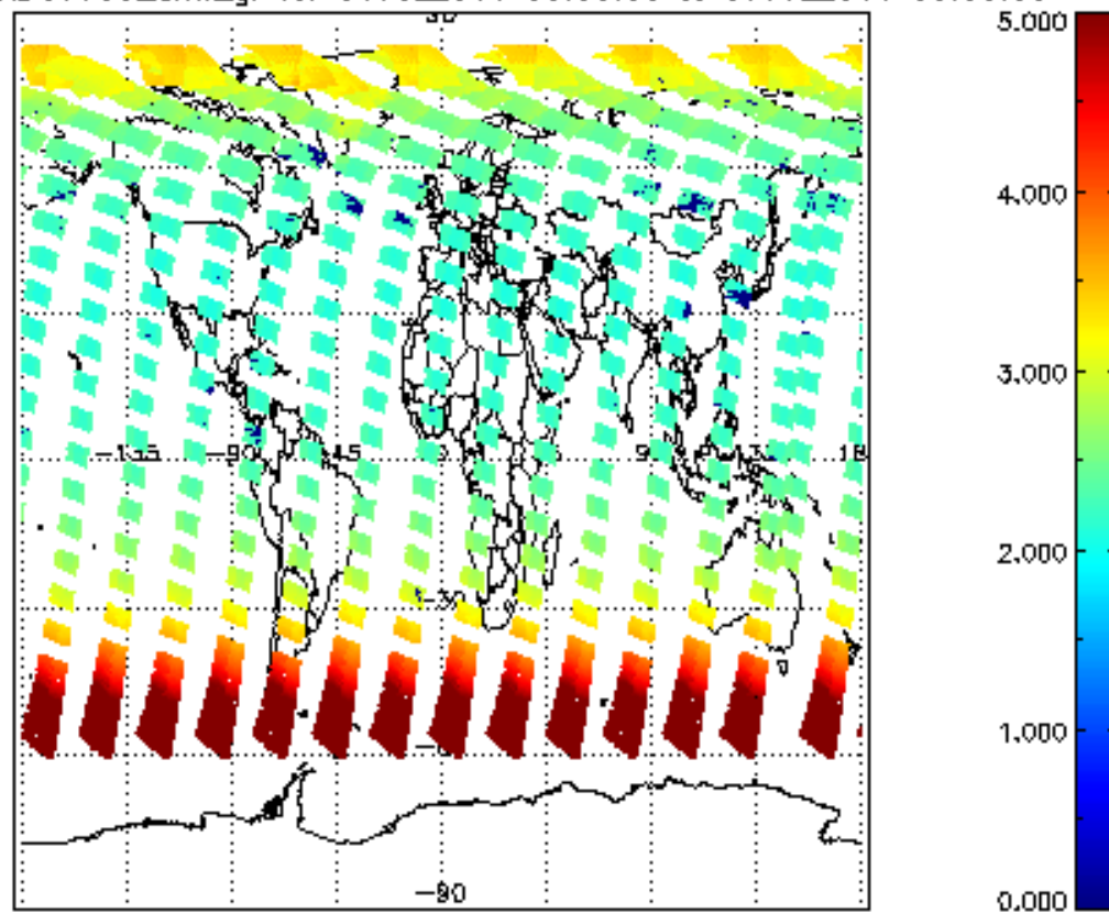
SCIOL2P_NADUV003_amf_gr for 06JUL2011 00:00:00 to 07JUL2011 00:00:00
