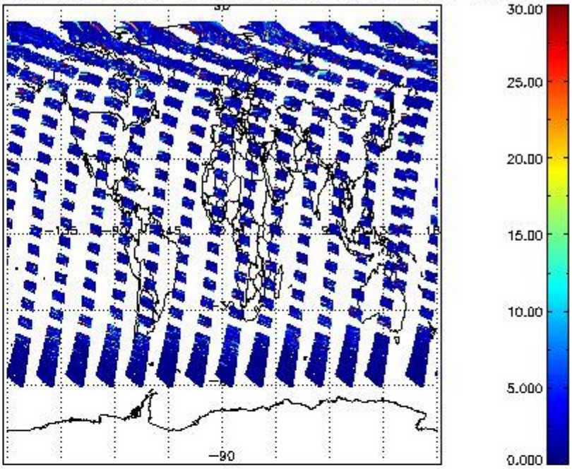
SCIOL2P_NADUV5S02_vcd_err for 06JUL2011 00:00:00 to 07JUL2011 00:00:00
