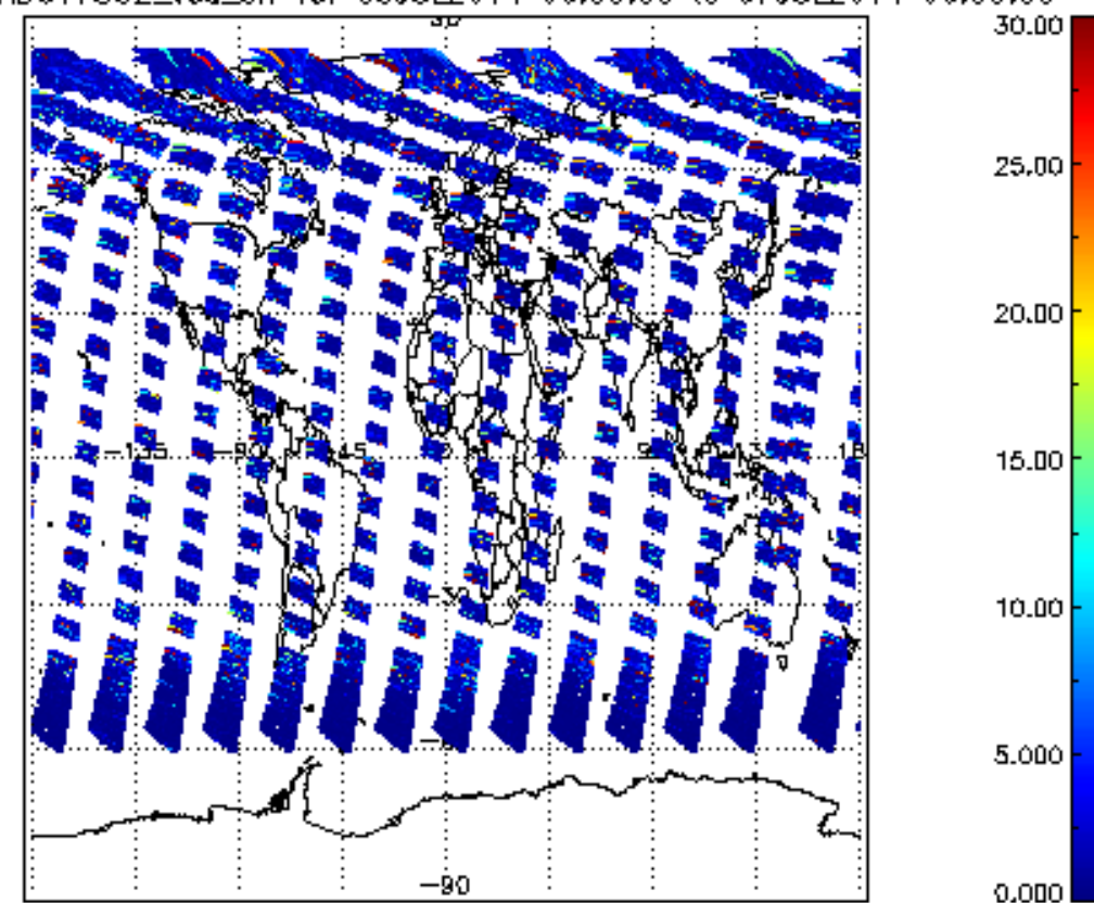
SCIOL2P_NADUV7S02_vcd_err for 06JUL2011 00:00:00 to 07JUL2011 00:00:00
