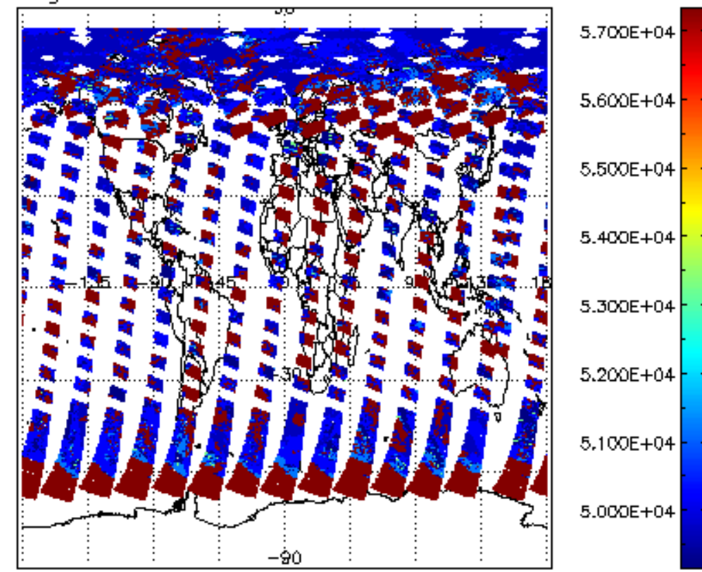
cloud_flags for 06JUL2011 00:00:00 to 07JUL2011 00:00:00
