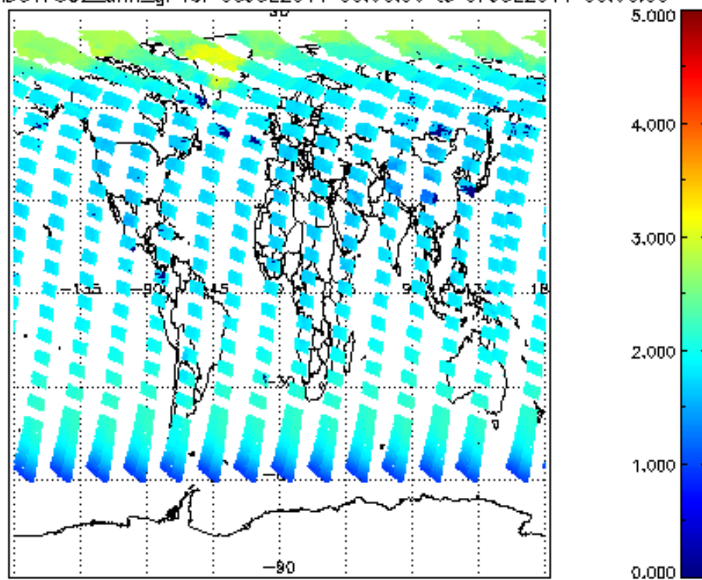
SCIOL2P_NADUV7S02_amf_gr for 06JUL2011 00:00:00 to 07JUL2011 00:00:00
