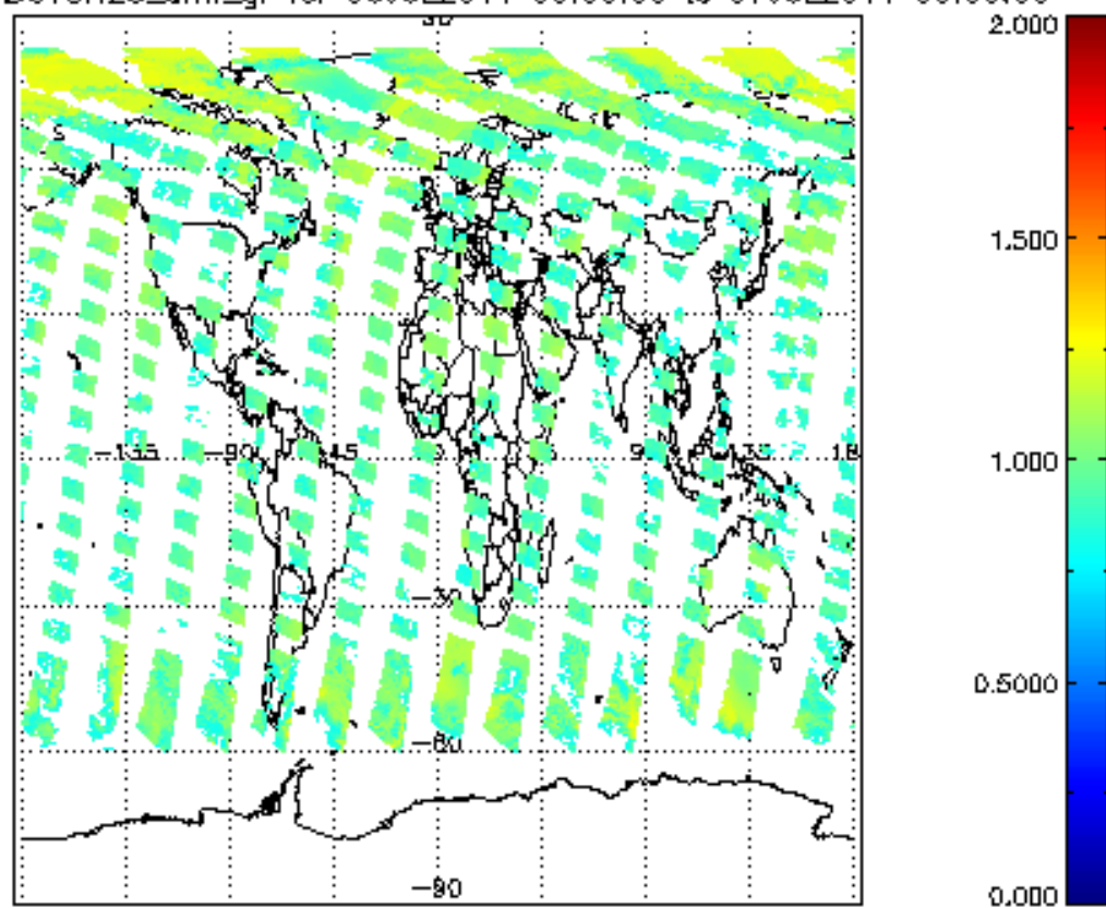
SCIOL2P_NADUV8H2O_amf_gr for 06JUL2011 00:00:00 to 07JUL2011 00:00:00
