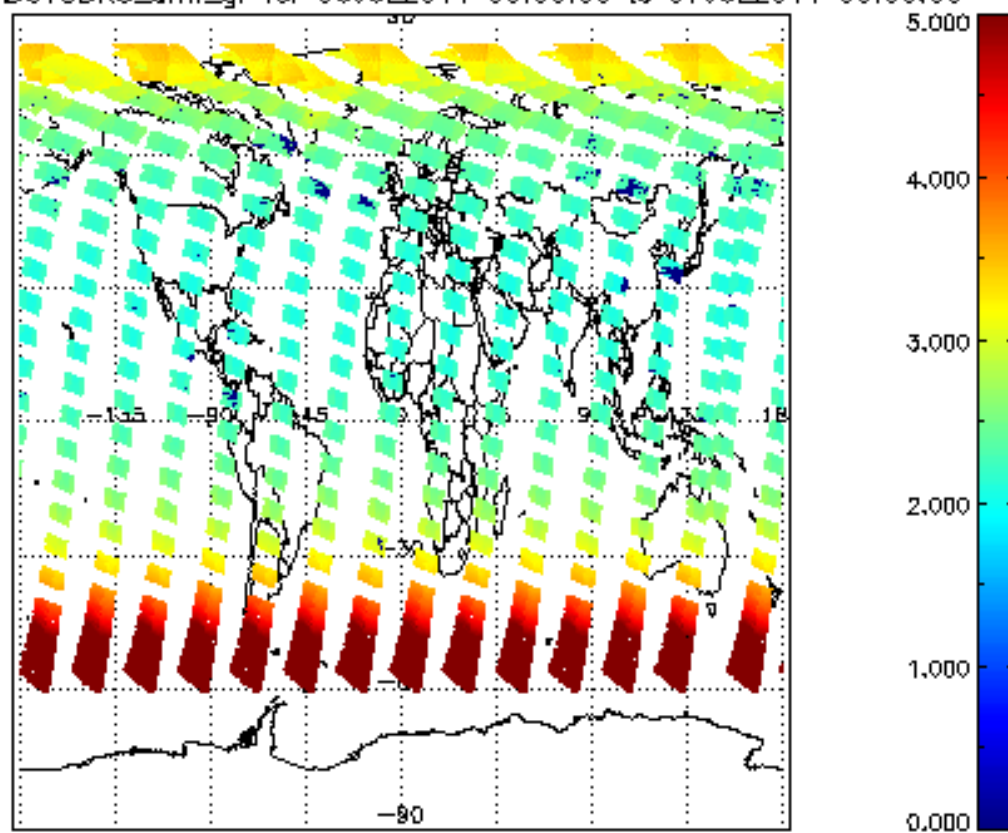
SCIOL2P_NADUV3BRO_amf_gr for 06JUL2011 00:00:00 to 07JUL2011 00:00:00
