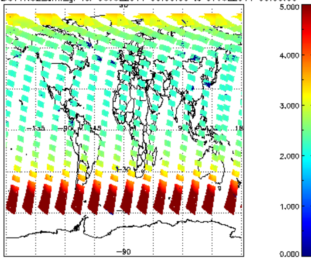
SCIOL2P_NADUV1NO2_amf_gr for 06JUL2011 00:00:00 to 07JUL2011 00:00:00
