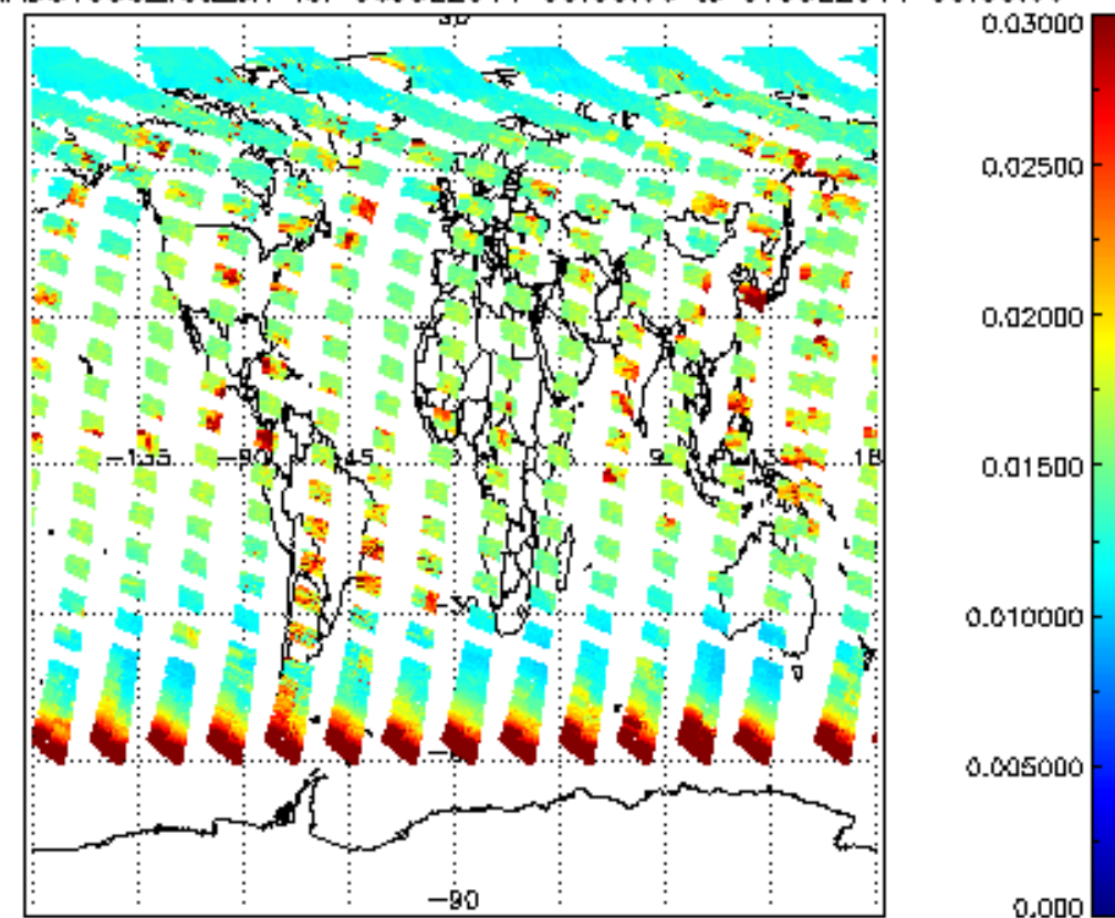
SCIOL2P_NADUV003_vcd_err for 06JUL2011 00:00:00 to 07JUL2011 00:00:00
