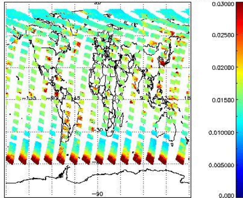
SCIOL2P_NADUV003_vcd_err for 06JUL2011 00:00:00 to 07JUL2011 00:00:00
