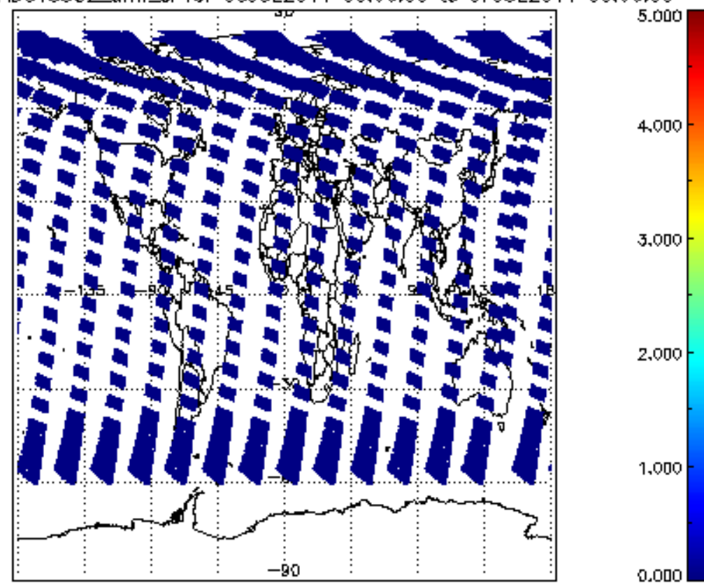
SCIOL2P_NADUV5S02_amf_cl for 06JUL2011 00:00:00 to 07JUL2011 00:00:00
