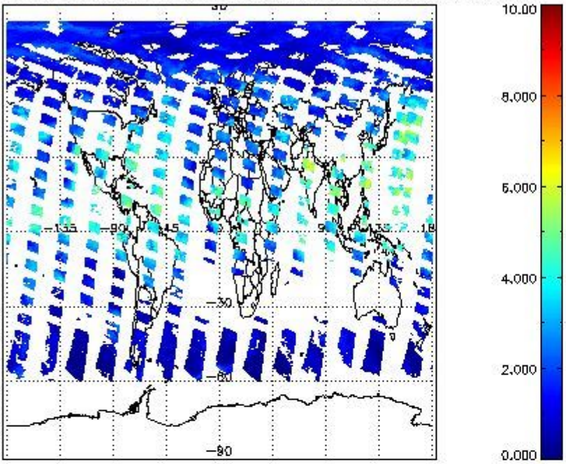
SCIOL2P_NADUV8H20_vcd for 06JUL2011 00:00:00 to 07JUL2011 00:00:00
