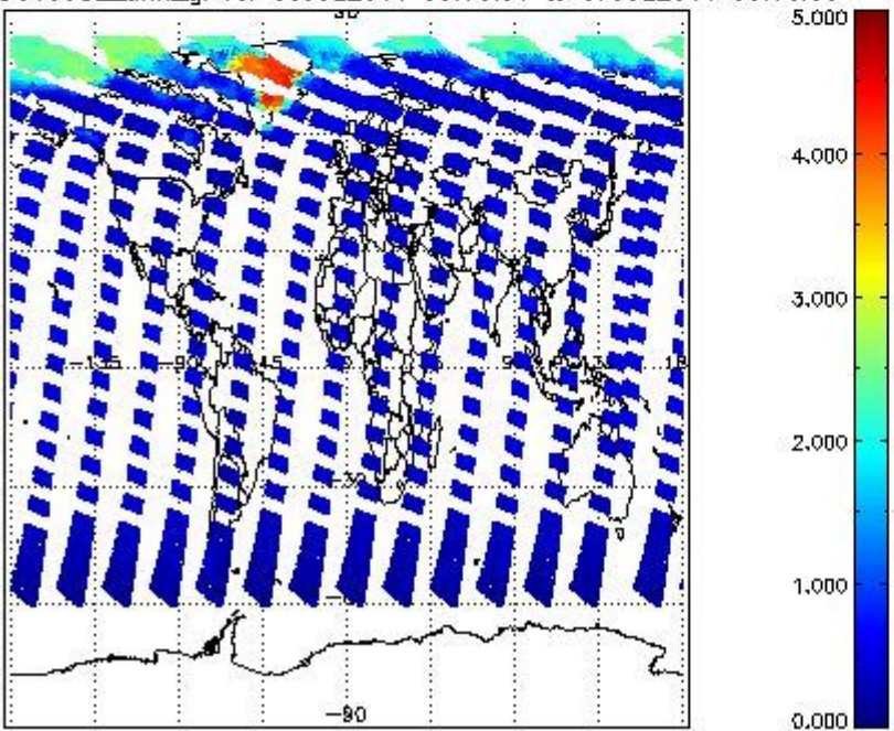
SCIOL2P_NADUV5S02_amf_gr for 06JUL2011 00:00:00 to 07JUL2011 00:00:00
