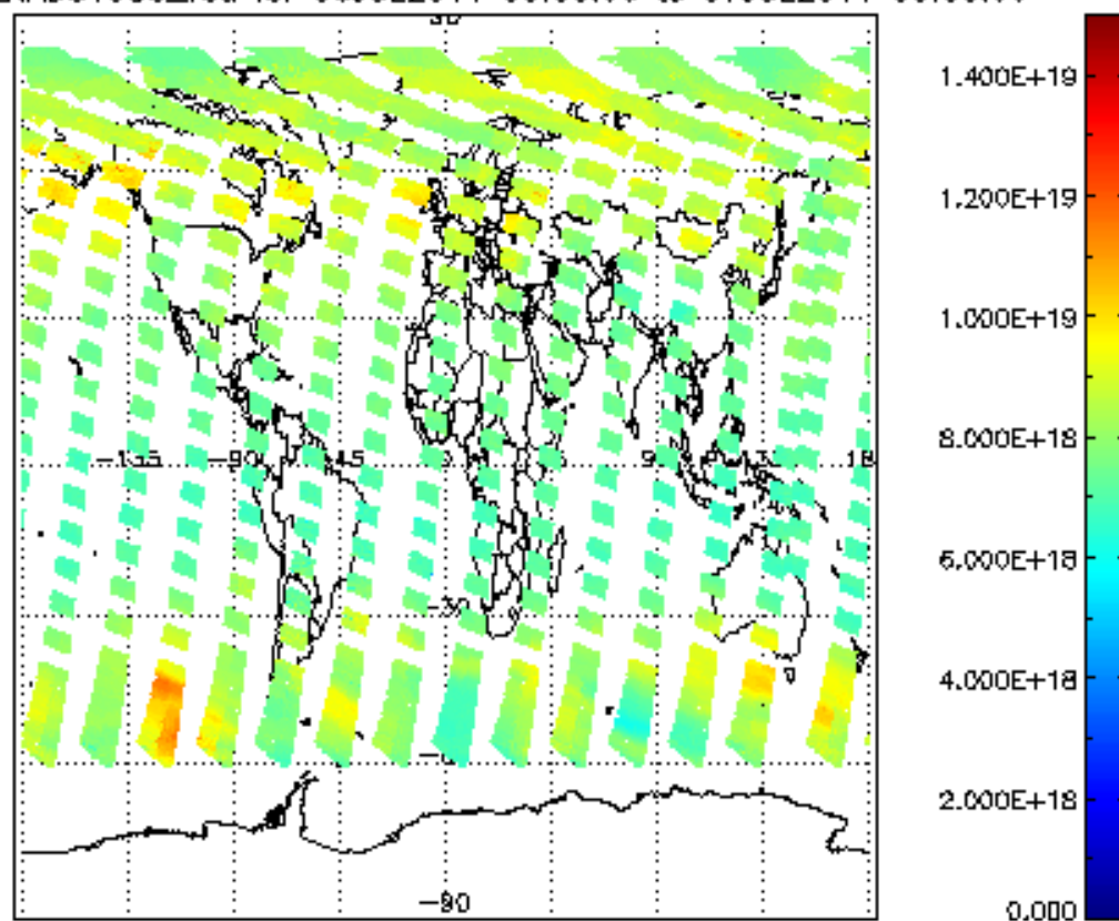
SCIOL2P_NADUV003_vcd for 06JUL2011 00:00:00 to 07JUL2011 00:00:00
