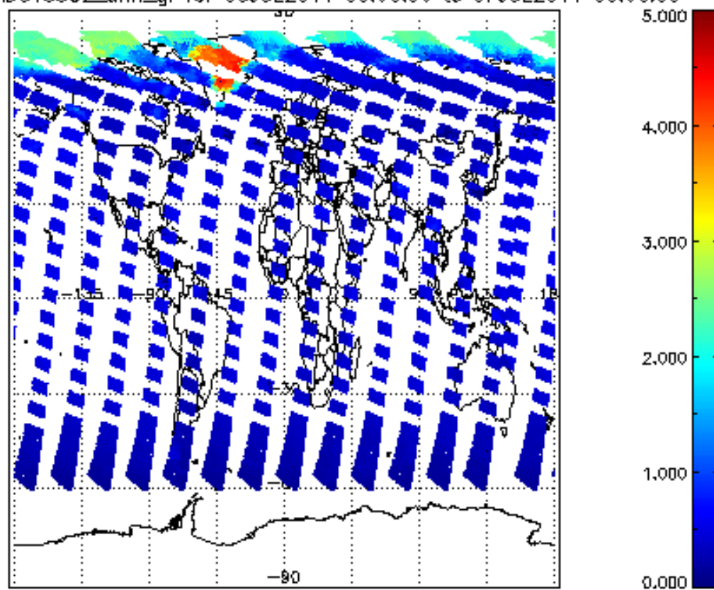
SCIOL2P_NADUV5S02_amf_gr for 06JUL2011 00:00:00 to 07JUL2011 00:00:00
