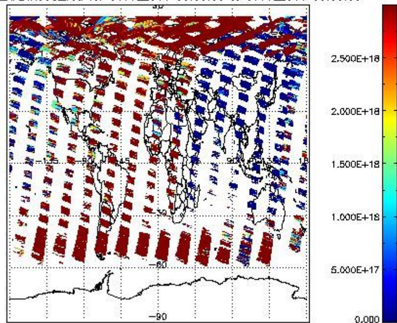
SCIDL2P_NADIR3CO_vcd for 06JUL2011 00:00:00 to 07JUL2011 00:00:00
