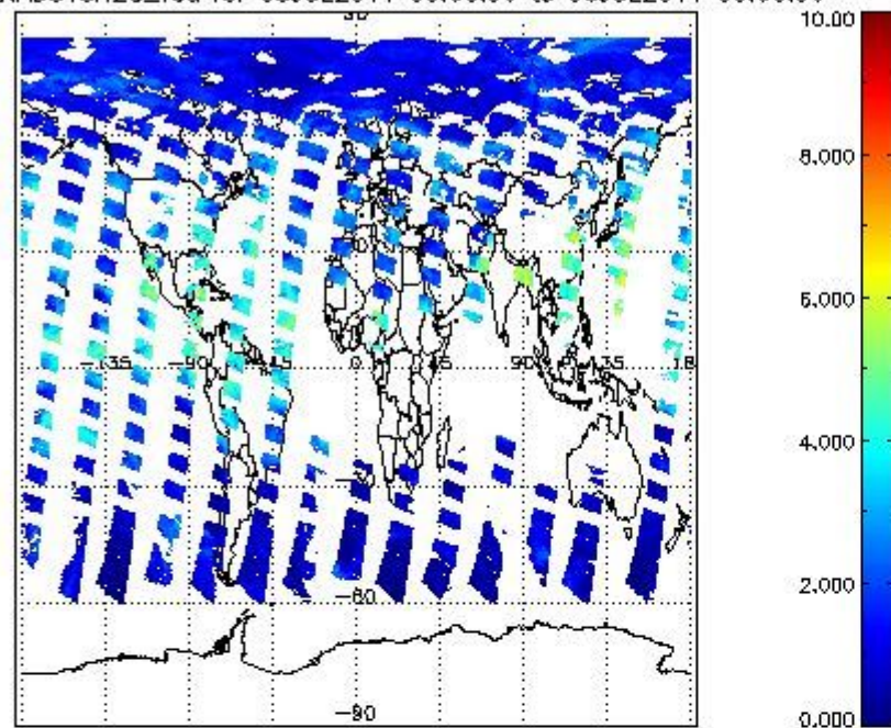
SCIOL2P_NADUV8H2O_vcd for 05JUL2011 00:00:00 to 06JUL2011 00:00:00
