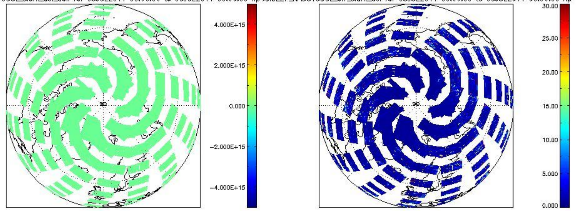
SCIOI2P_NADUV6OCLslant_col_den for 05JUL2011 00:00:00 to 06JUL2011 00:00:00 np SCIOI2P_NADUV6OCLarr_slant_col for 05JUL2011 00:00:00 to 06JUL2011 00:00:00 np
