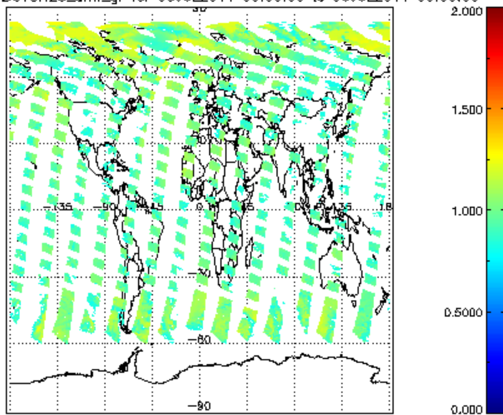
SCIOL2P_NADUV8H20_amf_gr for 05JUL2011 00:00:00 to 06JUL2011 00:00:00
