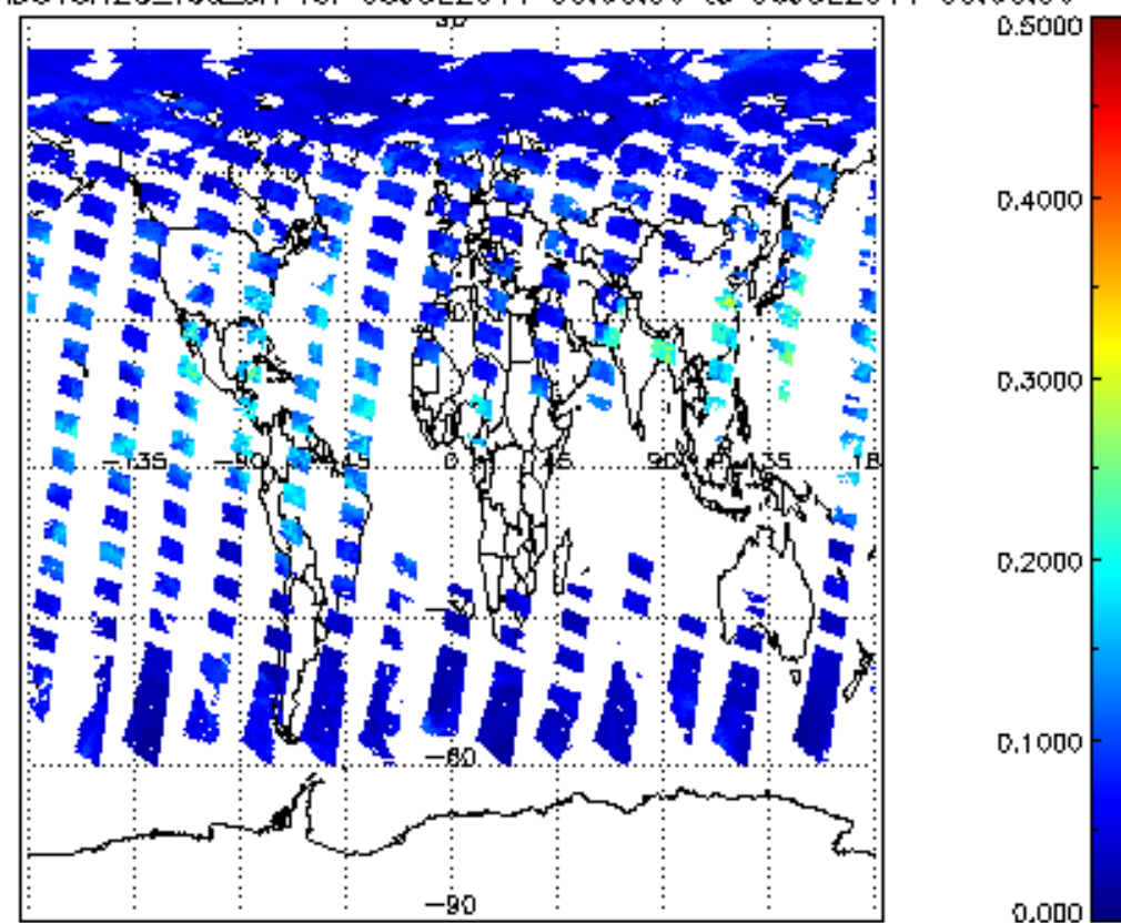
SCIOL2P_NADUV8H20_vcd_err for 05JUL2011 00:00:00 to 06JUL2011 00:00:00
