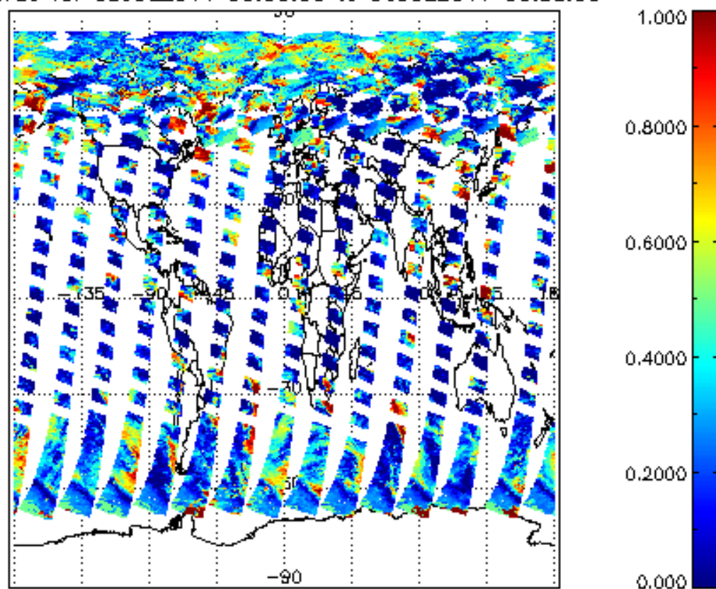
cl_frac for 05JUL2011 00:00:00 to 06JUL2011 00:00:00
