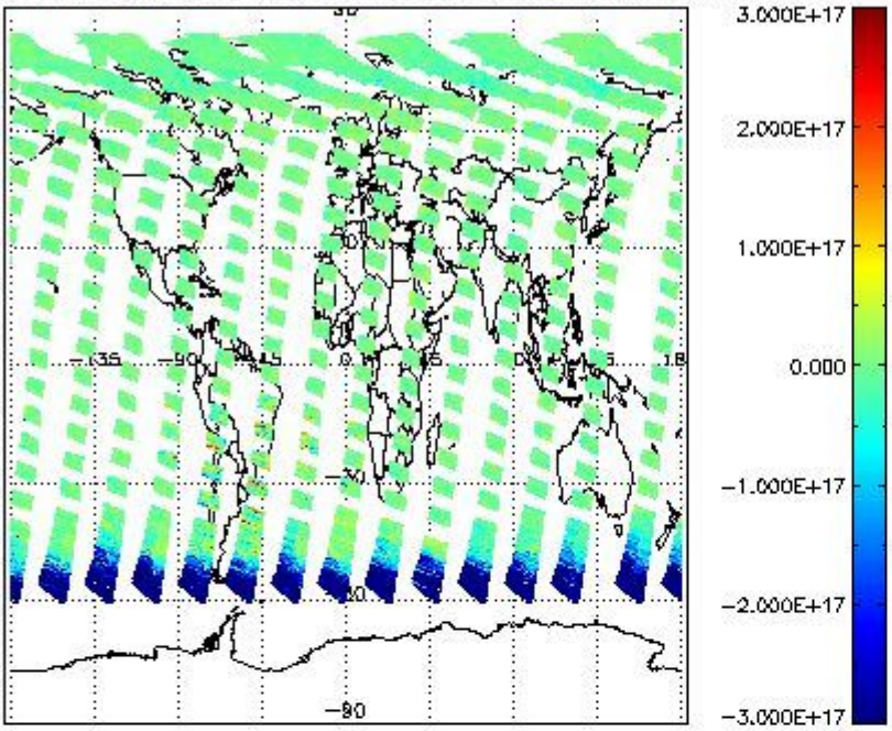
SCIOL2P_NADUV7S02_vcd for 05JUL2011 00:00:00 to 06JUL2011 00:00:00
