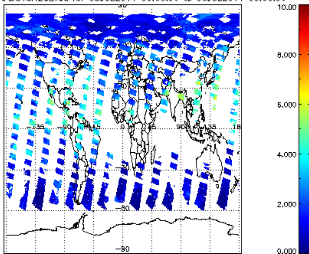
SCIOL2P_NADUV8H20_vcd for 05JUL2011 00:00:00 to 06JUL2011 00:00:00
