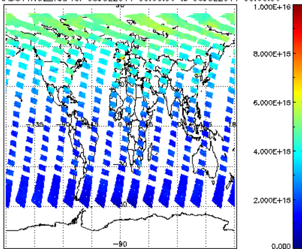
SCIOL2P_NADUV1NO2_vcd for 05JUL2011 00:00:00 to 06JUL2011 00:00:00
