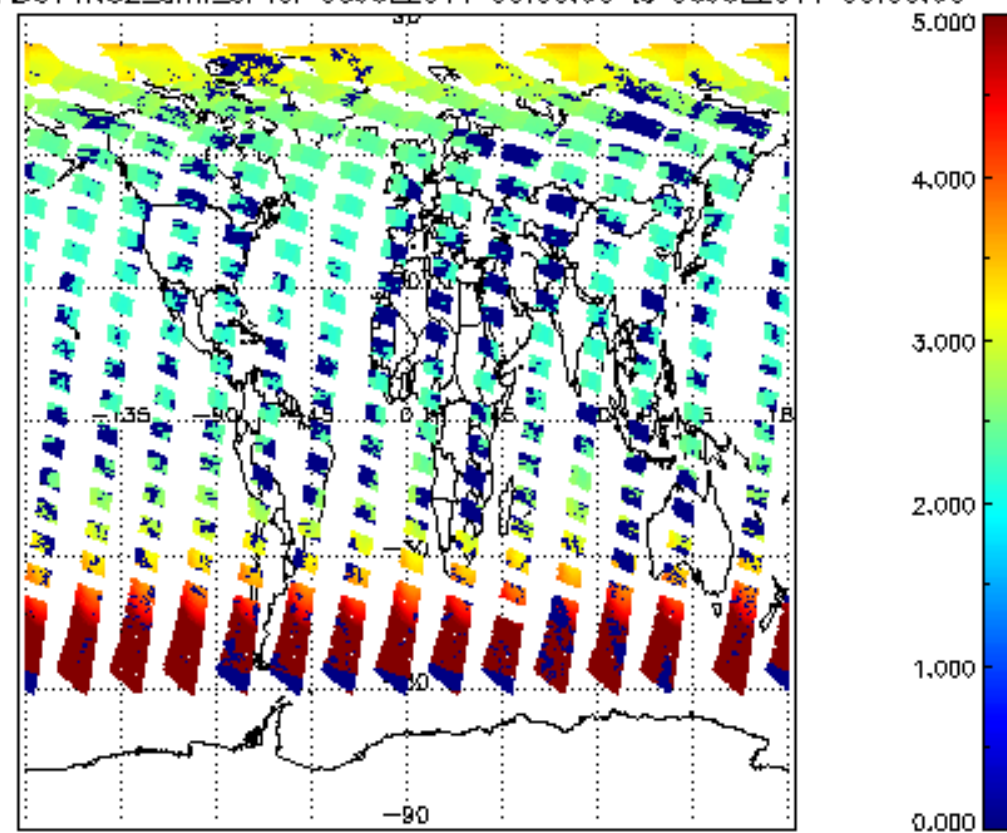
SCIOL2P_NADUV1NO2_amf_cl for 05JUL2011 00:00:00 to 06JUL2011 00:00:00
