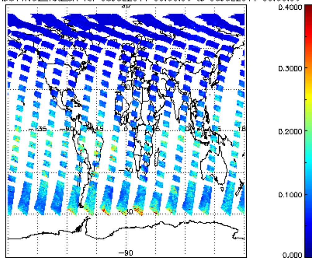
SCIOL2P_NADUV1NO2_vcd_err for 05JUL2011 00:00:00 to 06JUL2011 00:00:00
