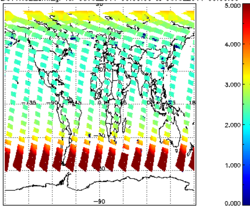
SCIOL2P_NADUV1NO2_amf_gr for 05JUL2011 00:00:00 to 06JUL2011 00:00:00
