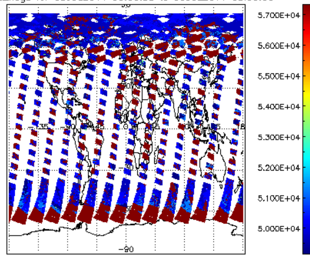
cloud_flags for 05JUL2011 00:00:00 to 06JUL2011 00:00:00
