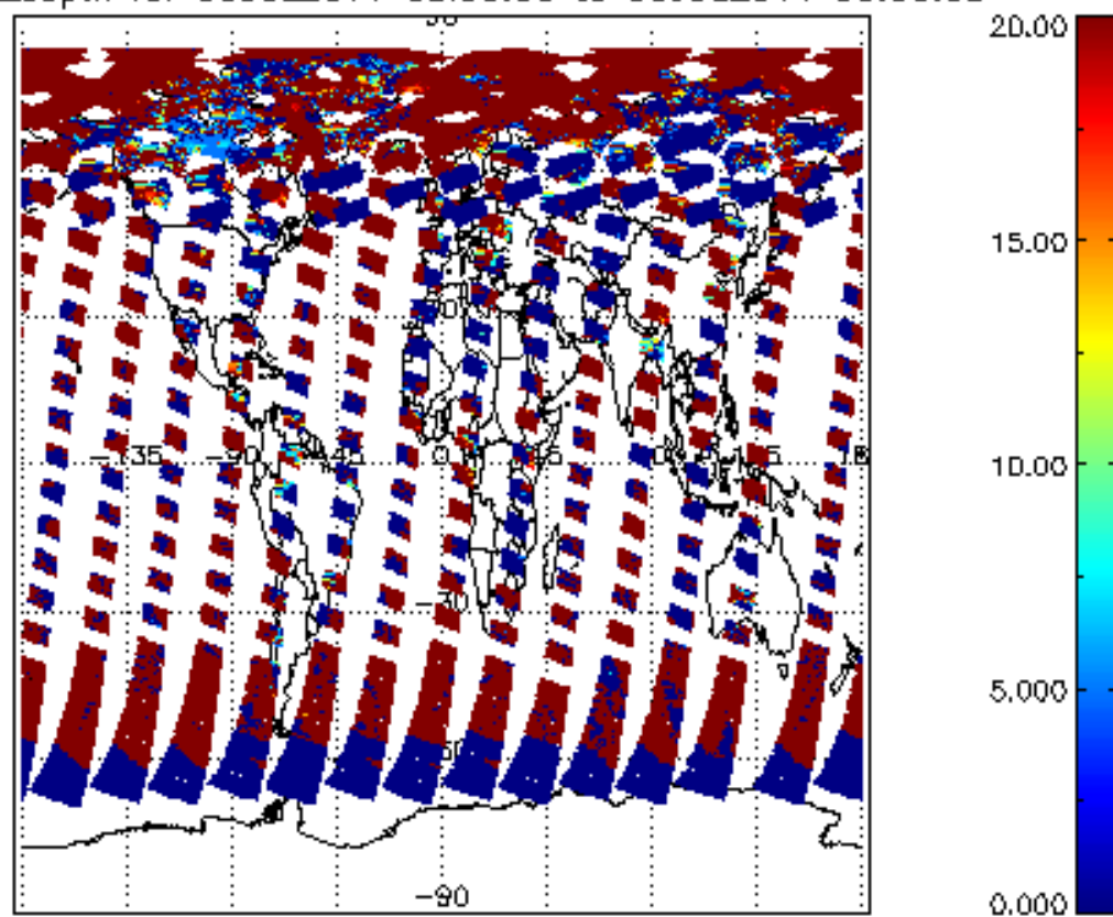
cl_lopt_depth for 05JUL2011 00:00:00 to 06JUL2011 00:00:00
