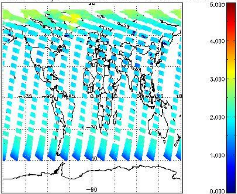
SCIOL2P_NADUV7S02_amf_gr for 05JUL2011 00:00:00 to 06JUL2011 00:00:00
