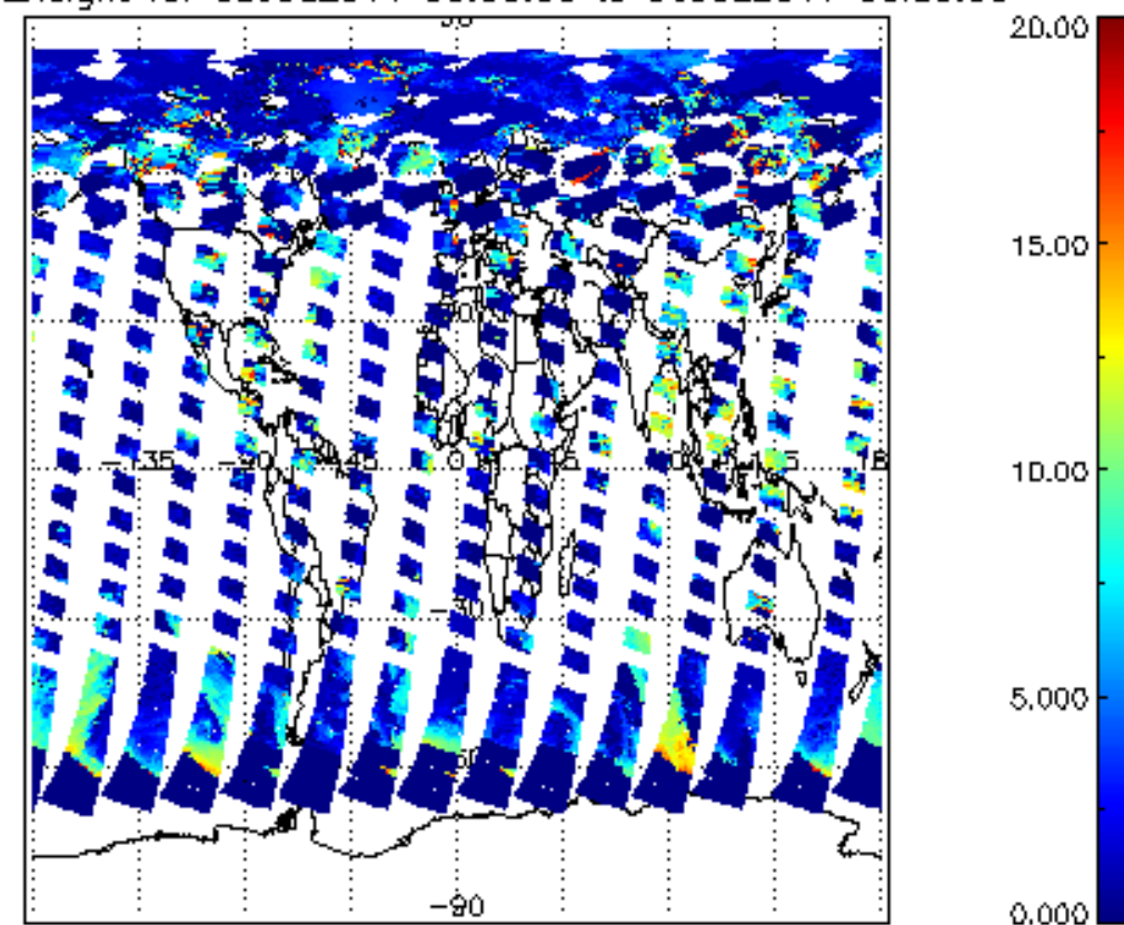
cl_top_height for 05JUL2011 00:00:00 to 06JUL2011 00:00:00
