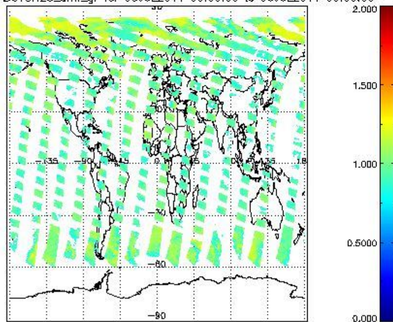
SCIOL2P_NADUV8H2O_amf_gr for 05JUL2011 00:00:00 to 06JUL2011 00:00:00
