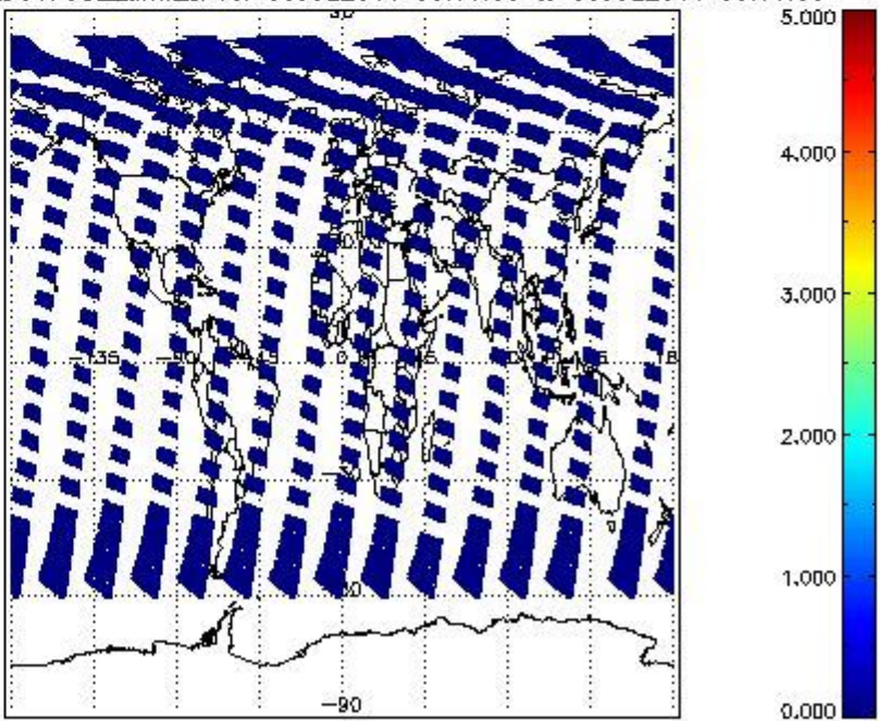
SCIOL2P_NADUV7S02_amf_cl for 05JUL2011 00:00:00 to 06JUL2011 00:00:00
