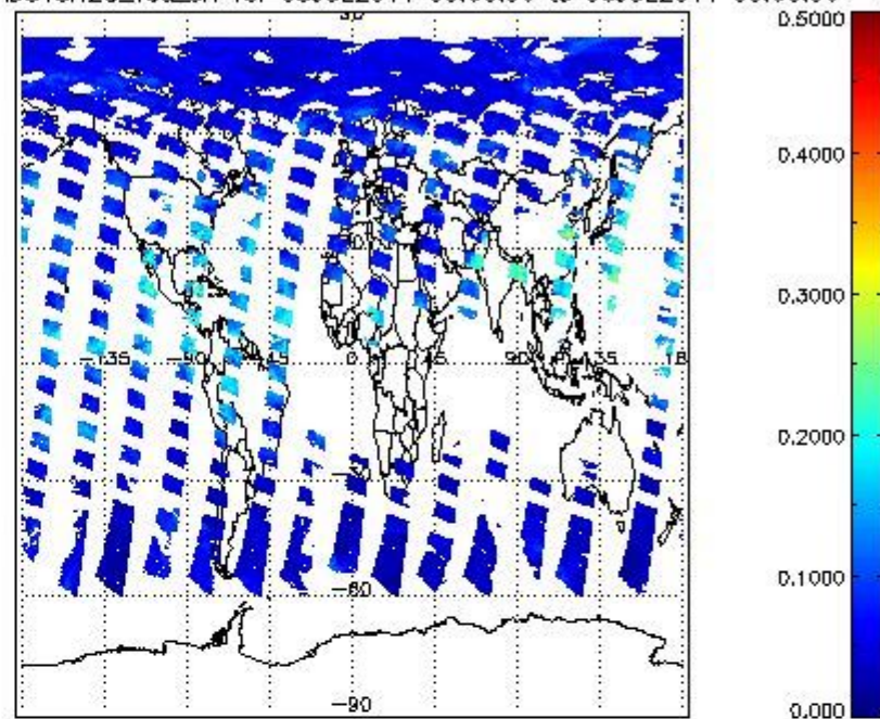
SCIOL2P_NADUV8H2O_vcd_err for 05JUL2011 00:00:00 to 06JUL2011 00:00:00
