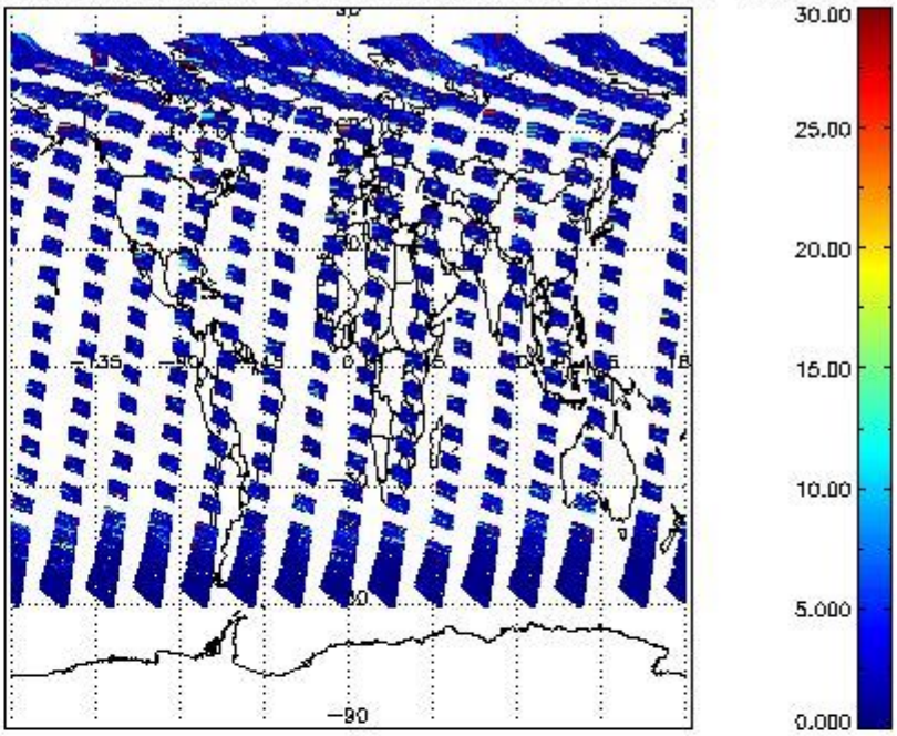
SCIOL2P_NADUV7S02_vcd_err for 05JUL2011 00:00:00 to 06JUL2011 00:00:00
