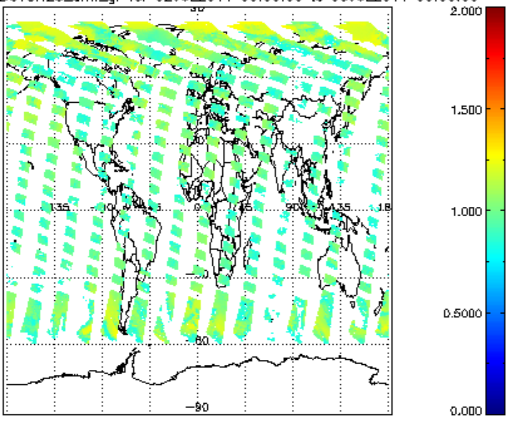
SCIOL2P_NADUV8H20_amf_gr for 02JUL2011 00:00:00 to 03JUL2011 00:00:00
