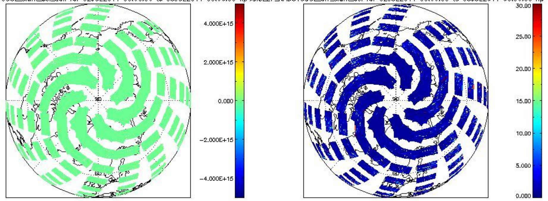
SCIOI2P_NADUV6OCLslant_col_den for 02JUL2011 00:00:00 to 03JUL2011 00:00:00 np SCIOI2P_NADUV6OCLarr_slant_col for 02JUL2011 00:00:00 to 03JUL2011 00:00:00 np
