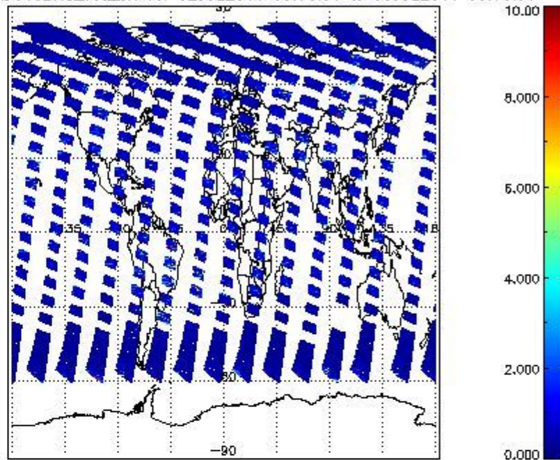
SCIOL2P_NADUV3BRO_vcd_err for 02JUL2011 00:00:00 to 03JUL2011 00:00:00
