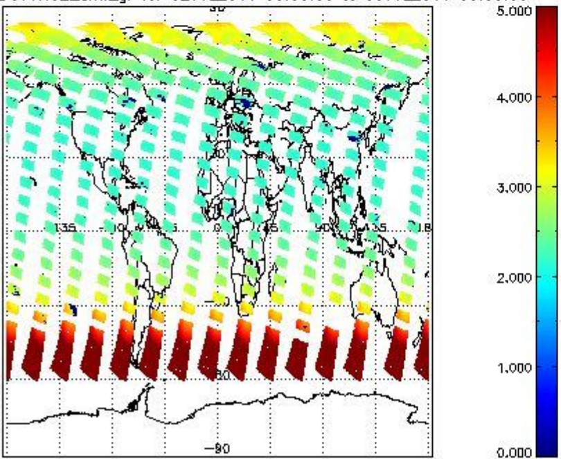
SCIOL2P_NADUV1NO2_amf_gr for 02JUL2011 00:00:00 to 03JUL2011 00:00:00
