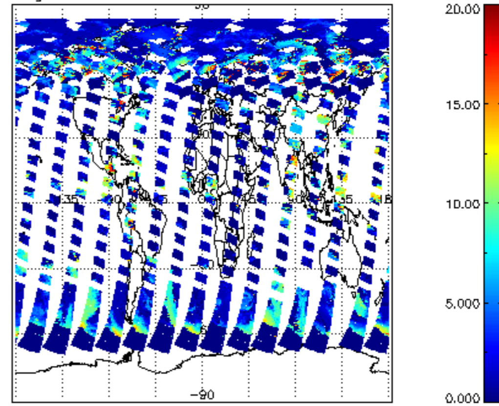
cl_top_height for 02JUL2011 00:00:00 to 03JUL2011 00:00:00
