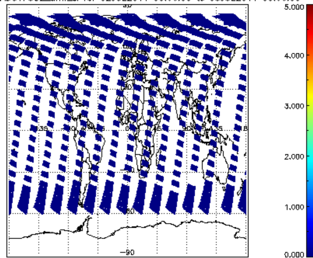
SCIOL2P_NADUV7S02_amf_cl for 02JUL2011 00:00:00 to 03JUL2011 00:00:00
