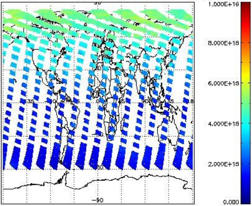
SCIOL2P_NADUV1NO2_vcd for 02JUL2011 00:00:00 to 03JUL2011 00:00:00
