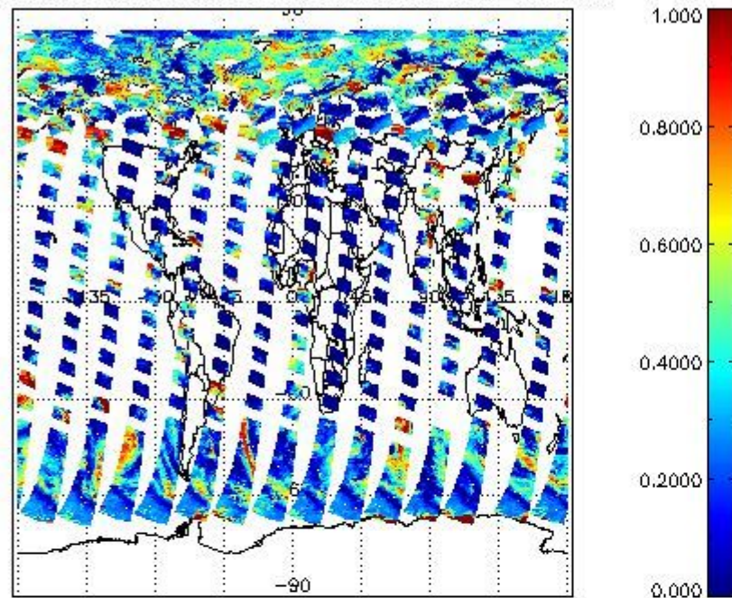
cL_frac for 02JUL2011 00:00:00 to 03JUL2011 00:00:00
