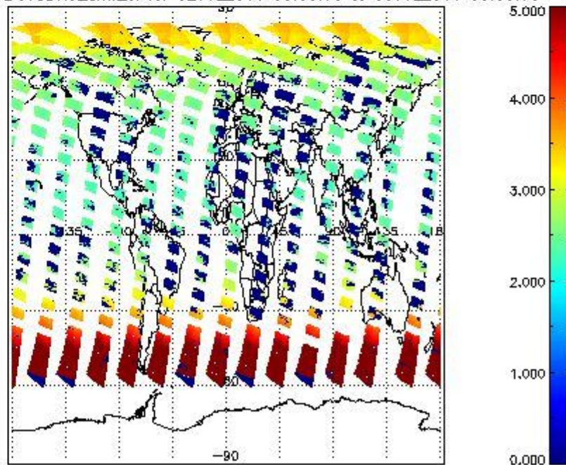
SCIOL2P_NADUV3BRO_amf_cl for 02JUL2011 00:00:00 to 03JUL2011 00:00:00
