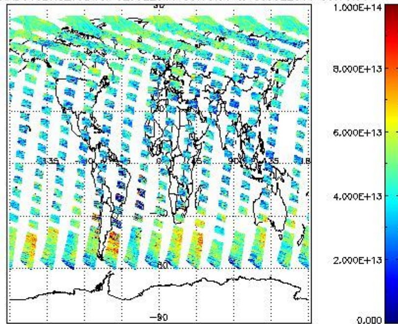
SCIOL2P_NADUV3BRO_vcd for 02JUL2011 00:00:00 to 03JUL2011 00:00:00
