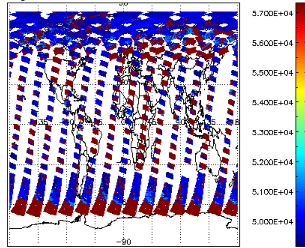
cloud_flags for 02JUL2011 00:00:00 to 03JUL2011 00:00:00
