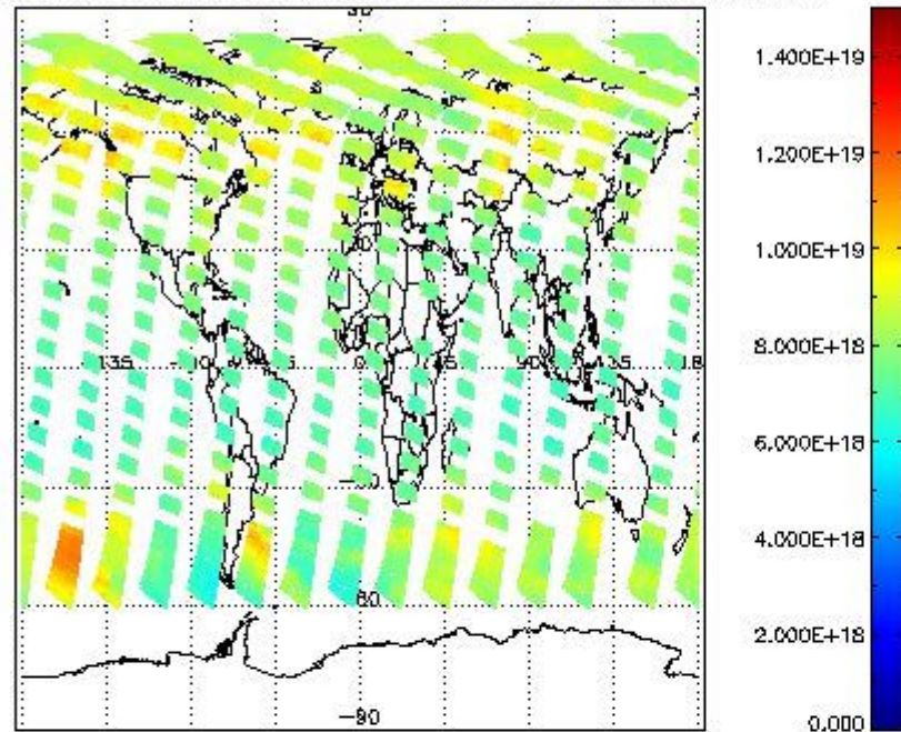
SCIOL2P_NADUV003_vcd for 02JUL2011 00:00:00 to 03JUL2011 00:00:00
