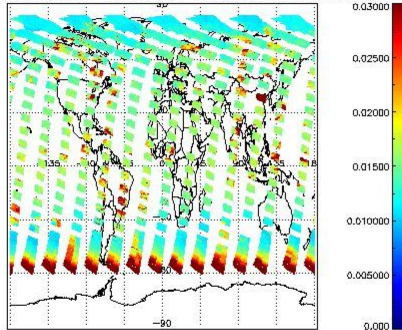
SCIOL2P_NADUV003_vcd_err for 02JUL2011 00:00:00 to 03JUL2011 00:00:00
