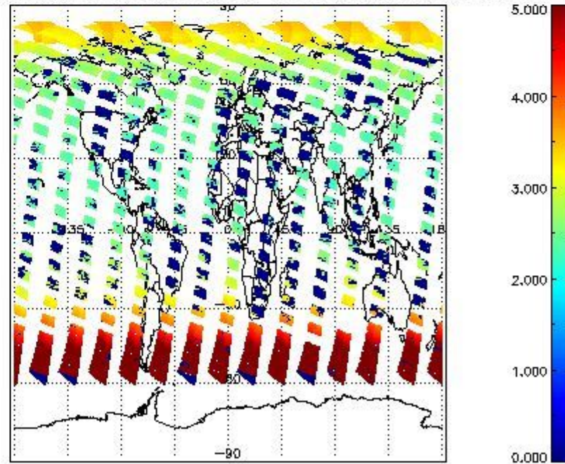
SCIOL2P_NADUV003_amf_cl for 02JUL2011 00:00:00 to 03JUL2011 00:00:00
