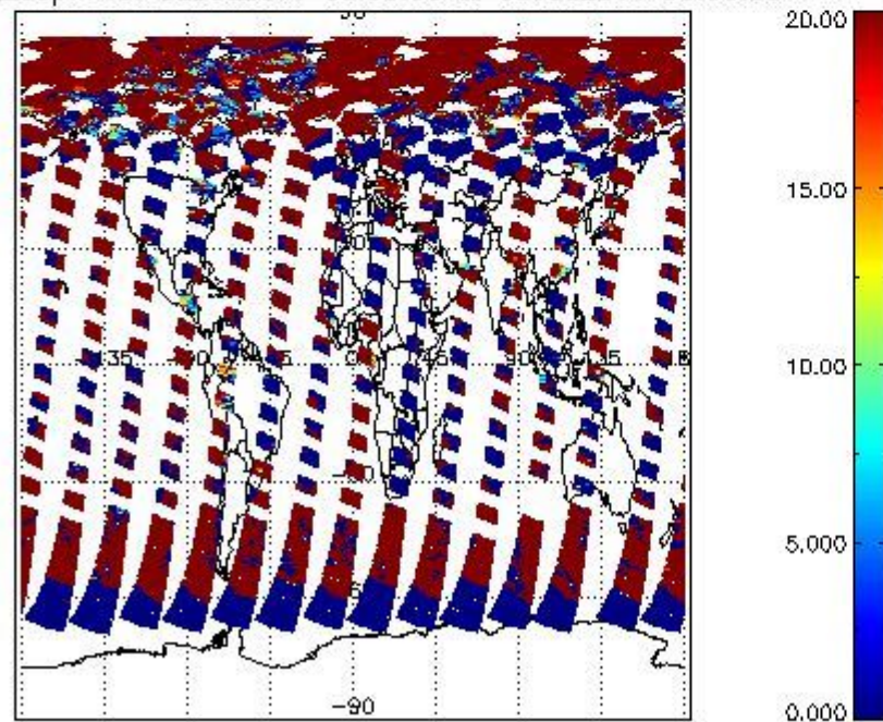
cL_opt_depth for 02JUL2011 00:00:00 to 03JUL2011 00:00:00
