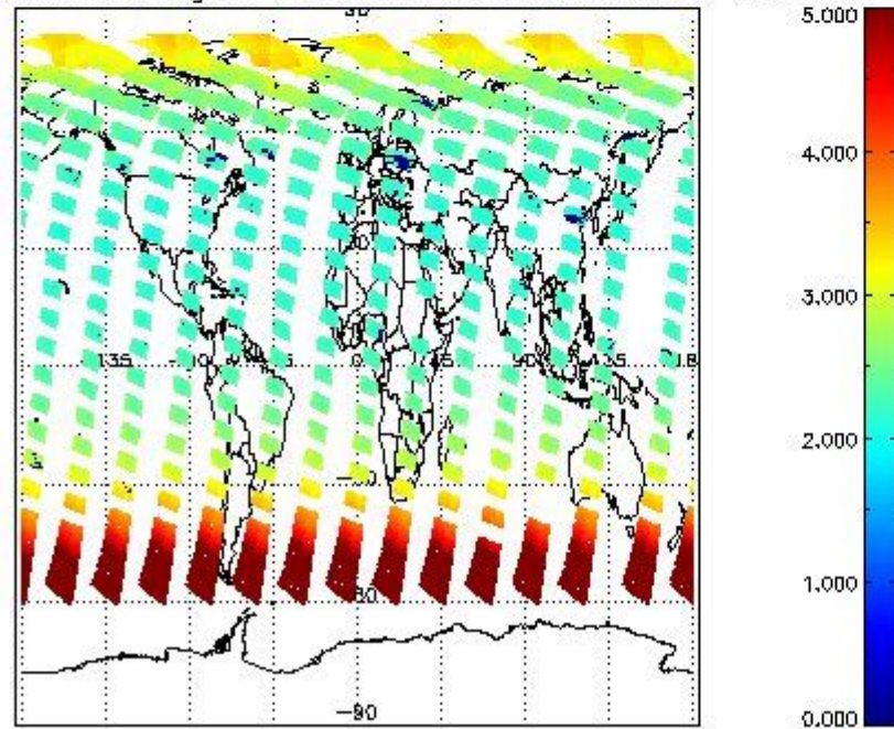
SCIOL2P_NADUV003_amf_gr for 02JUL2011 00:00:00 to 03JUL2011 00:00:00
