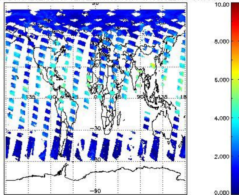
SCIOL2P_NADUV8H20_vcd for 02JUL2011 00:00:00 to 03JUL2011 00:00:00
