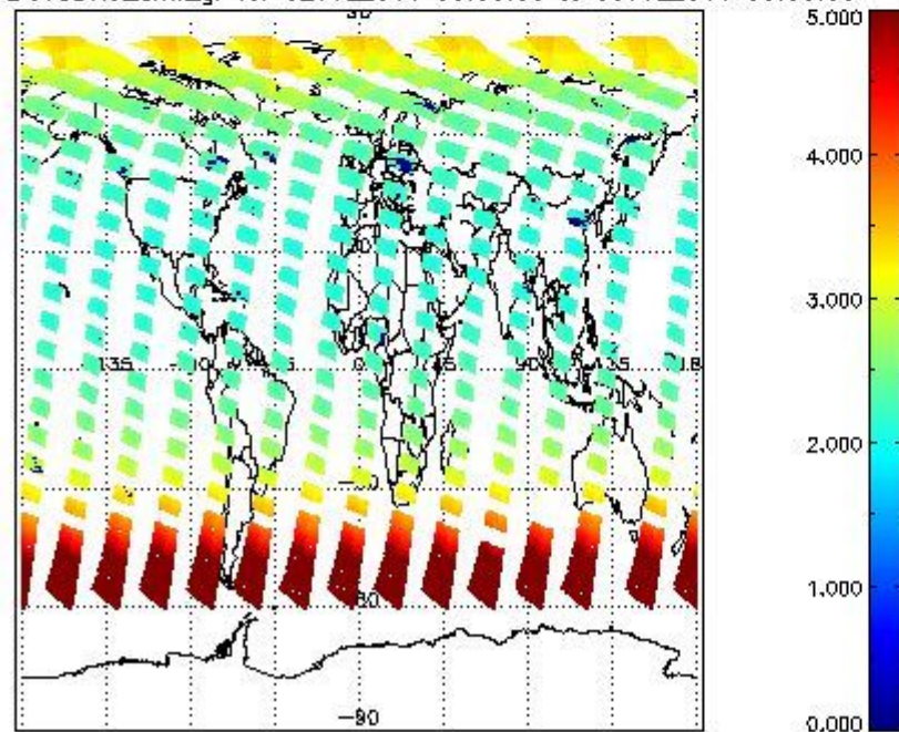
SCIOL2P_NADUV3BRO_amf_gr for 02JUL2011 00:00:00 to 03JUL2011 00:00:00
