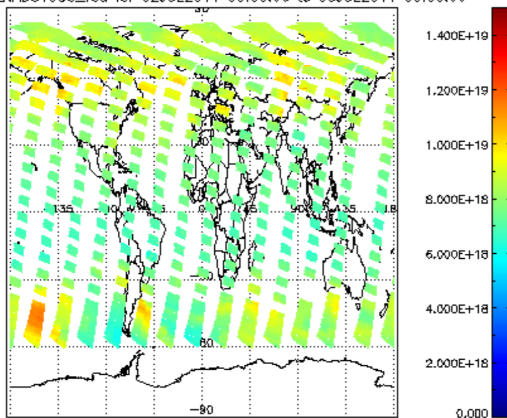
SCIOL2P_NADUV003_vcd for 02JUL2011 00:00:00 to 03JUL2011 00:00:00
