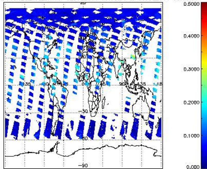
SCIOL2P_NADUV8H20_vcd_err for 02JUL2011 00:00:00 to 03JUL2011 00:00:00
