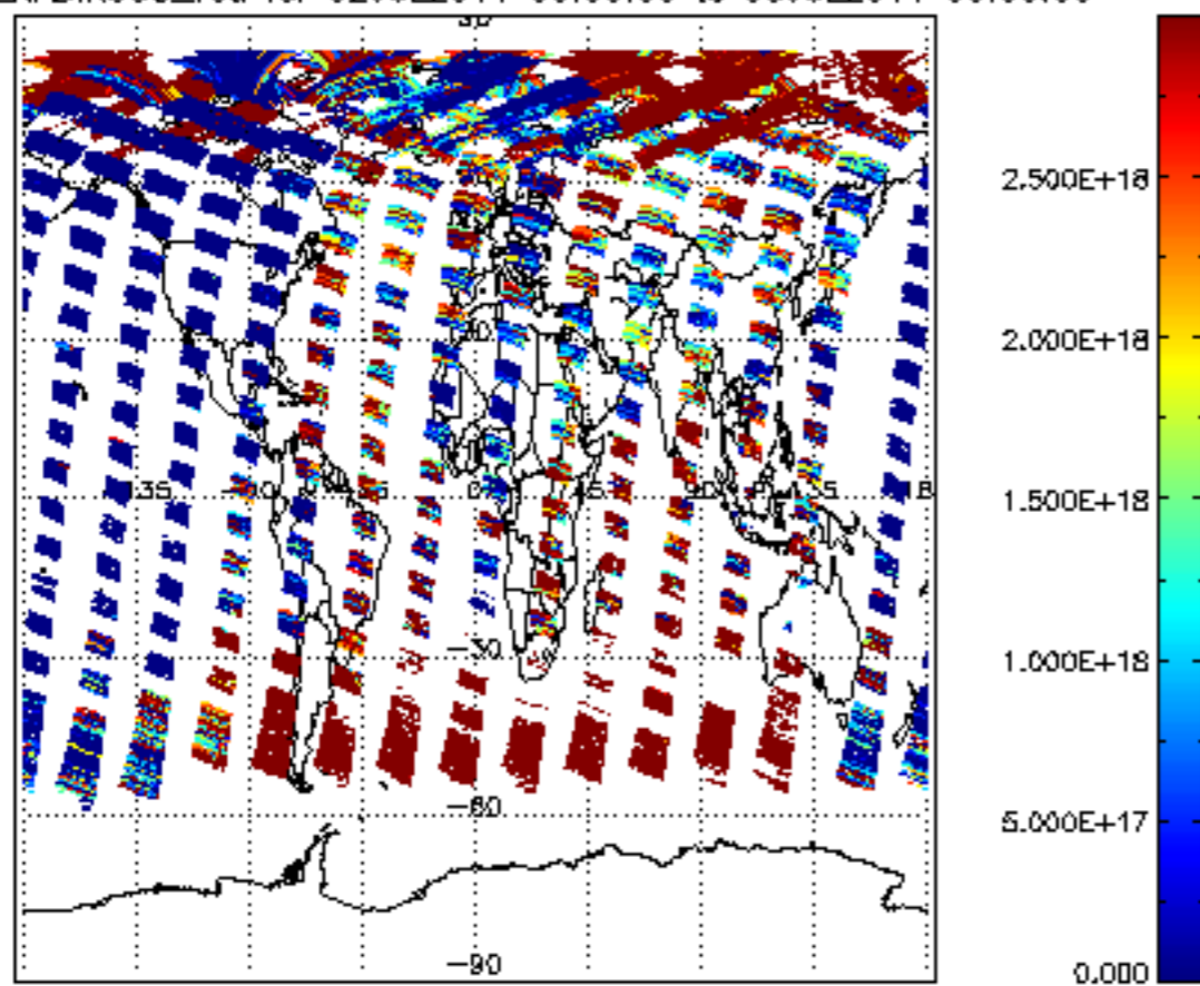
SCIOL2P_NADIR3CO_vcd for 02JUL2011 00:00:00 to 03JUL2011 00:00:00
