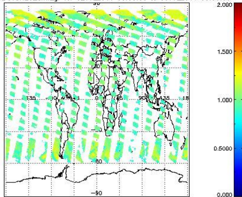
SCIOL2P_NADUV8H20_amf_gr for 02JUL2011 00:00:00 to 03JUL2011 00:00:00
