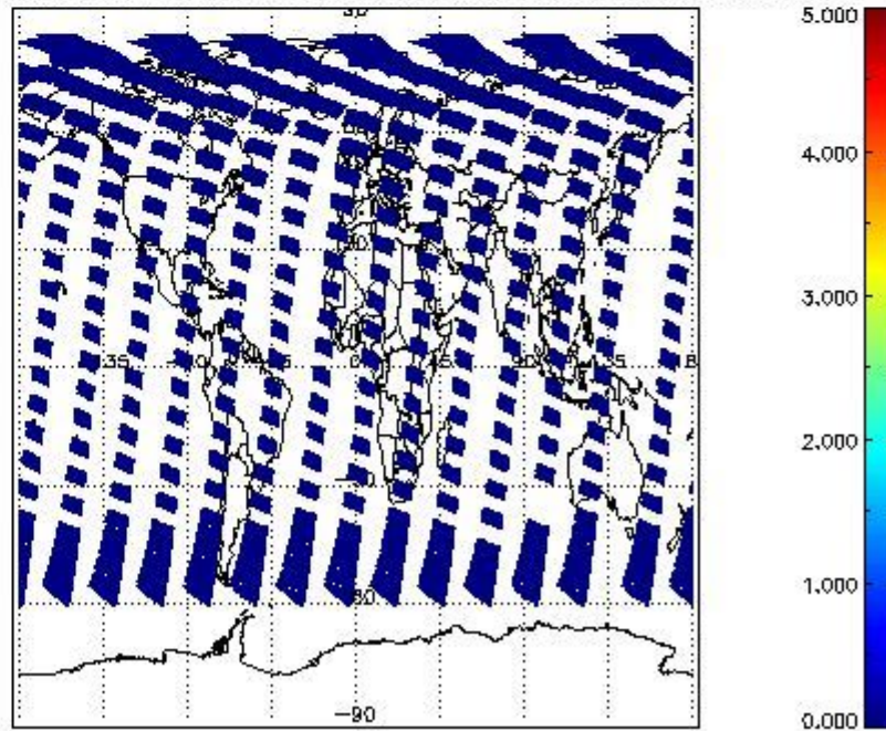
SCIOL2P_NADUV7S02_amf_cl for 02JUL2011 00:00:00 to 03JUL2011 00:00:00
