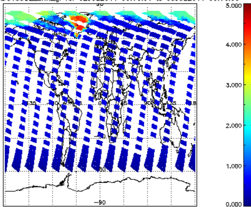
SCIOL2P_NADUV5S02_amf_gr for 02JUL2011 00:00:00 to 03JUL2011 00:00:00
