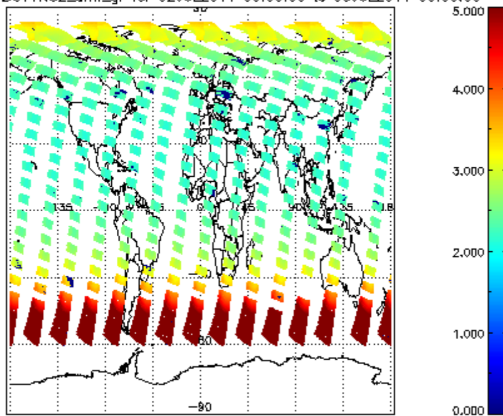
SCIOL2P_NADUV1N02_amf_gr for 02JUL2011 00:00:00 to 03JUL2011 00:00:00
