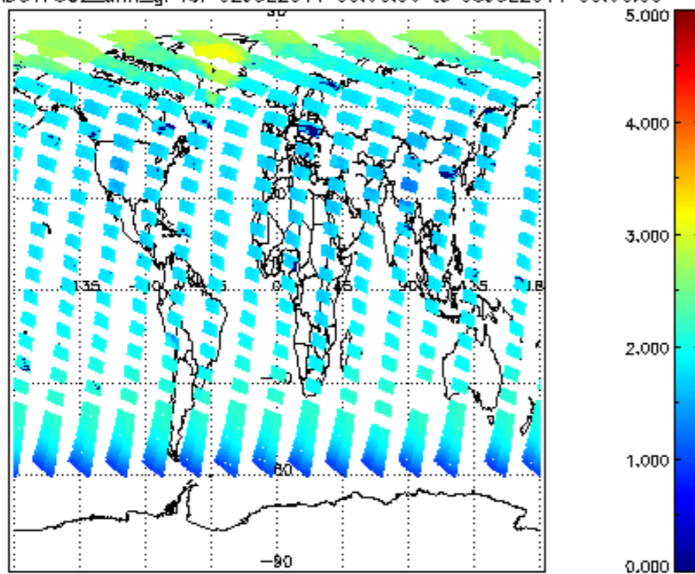
SCIOL2P_NADUV7S02_amf_gr for 02JUL2011 00:00:00 to 03JUL2011 00:00:00
