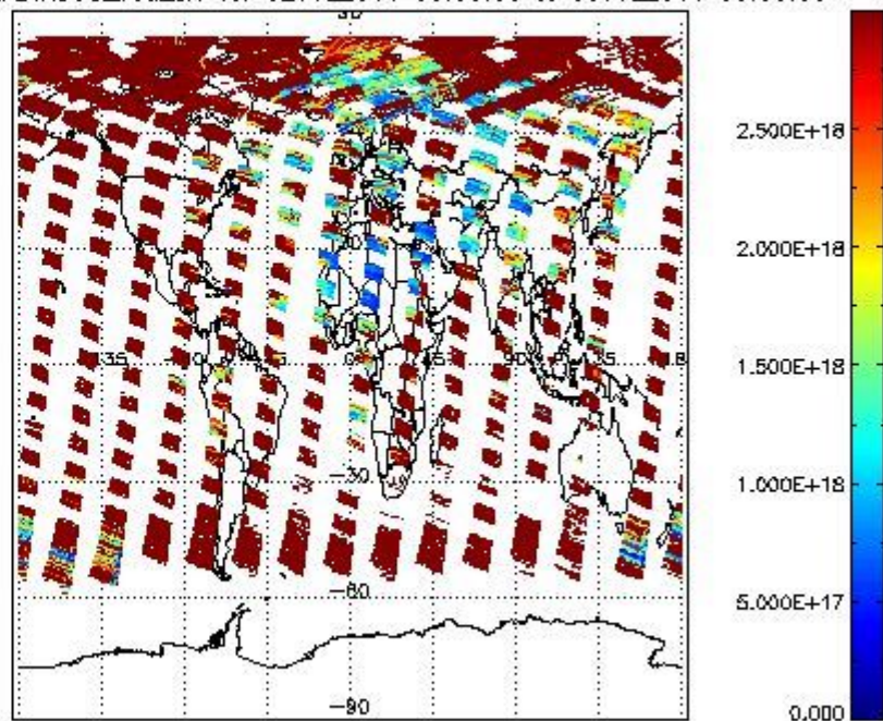
SCIDL2P_NADIR3CO_vcd_err for 02JUL2011 00:00:00 to 03JUL2011 00:00:00
