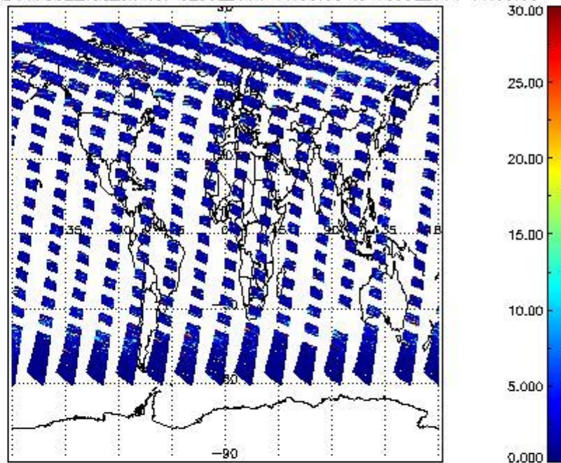
SCIOL2P_NADUV7S02_vcd_err for 02JUL2011 00:00:00 to 03JUL2011 00:00:00
