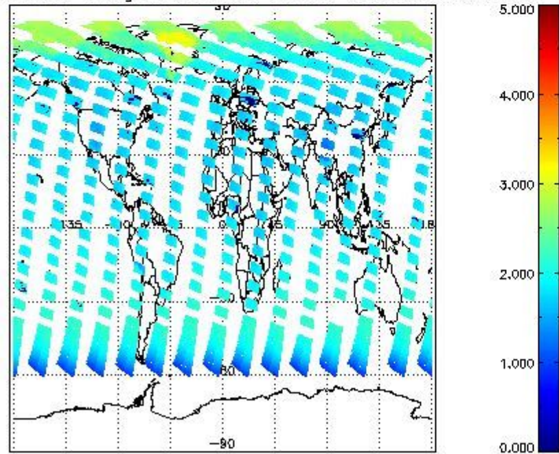
SCIOL2P_NADUV7S02_amf_gr for 02JUL2011 00:00:00 to 03JUL2011 00:00:00
