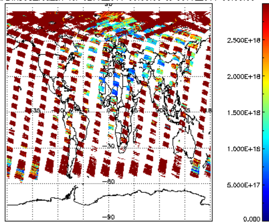
SCIOL2P_NADIR3CO_vcd_err for 02JUL2011 00:00:00 to 03JUL2011 00:00:00
