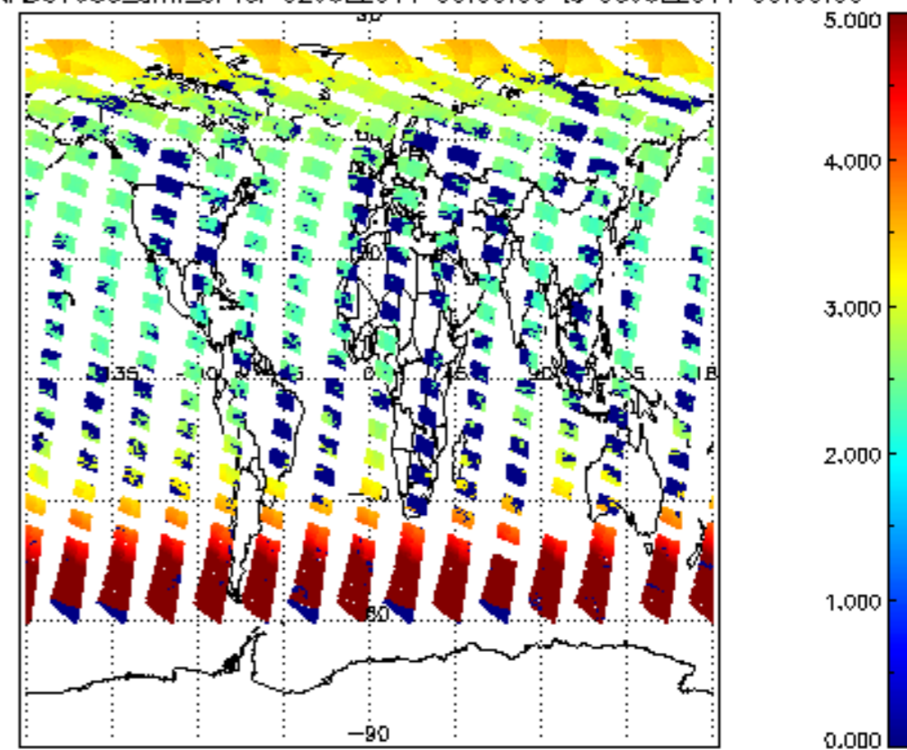
SCIOL2P_NADUV003_amf_cl for 02JUL2011 00:00:00 to 03JUL2011 00:00:00
