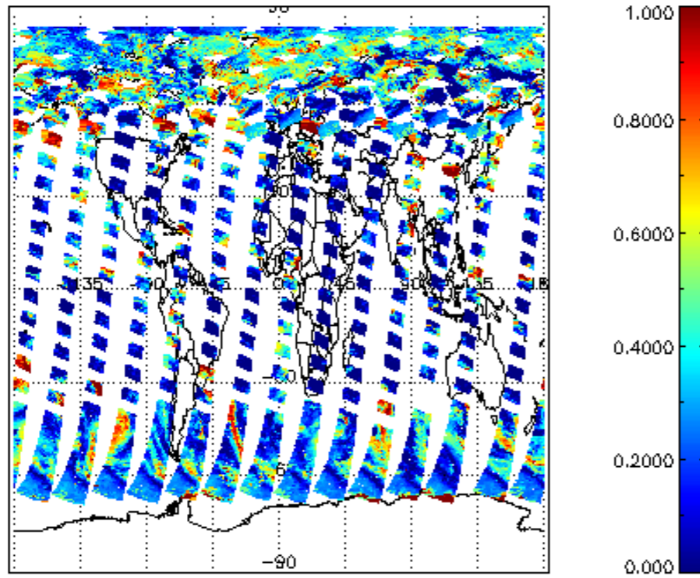
cl_frac for 02JUL2011 00:00:00 to 03JUL2011 00:00:00
