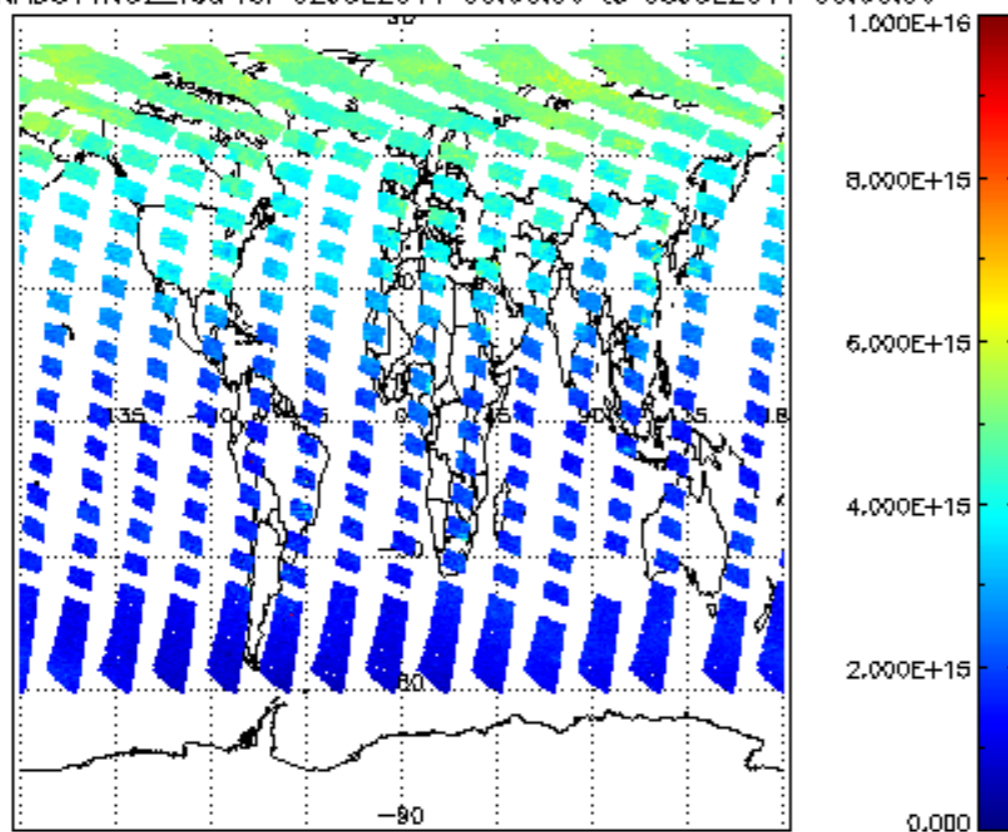
SCIOL2P_NADUV1N02_vcd for 02JUL2011 00:00:00 to 03JUL2011 00:00:00
