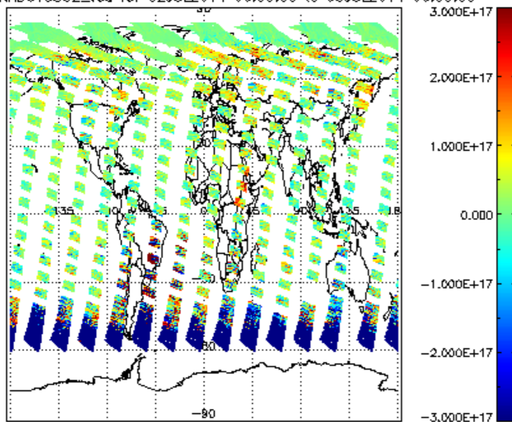
SCIOL2P_NADUV5S02_vcd for 02JUL2011 00:00:00 to 03JUL2011 00:00:00
