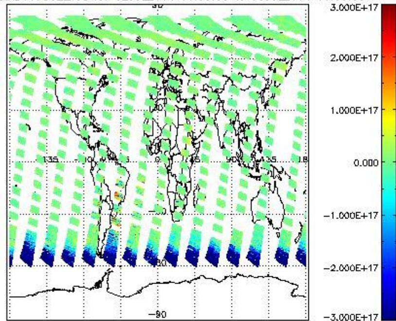
SCIOL2P_NADUV7S02_vcd for 02JUL2011 00:00:00 to 03JUL2011 00:00:00
