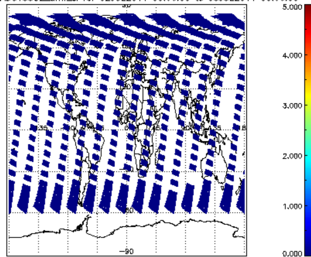
SCIOL2P_NADUV5S02_amf_cl for 02JUL2011 00:00:00 to 03JUL2011 00:00:00
