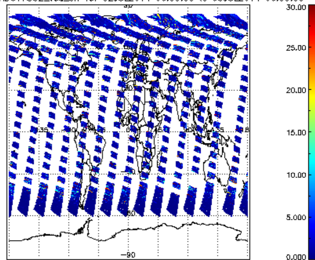
SCIOL2P_NADUV7S02_vcd_err for 02JUL2011 00:00:00 to 03JUL2011 00:00:00
