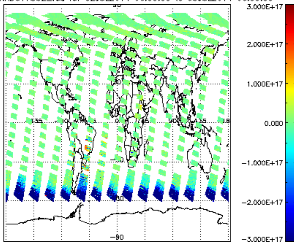
SCIOL2P_NADUV7S02_vcd for 02JUL2011 00:00:00 to 03JUL2011 00:00:00
