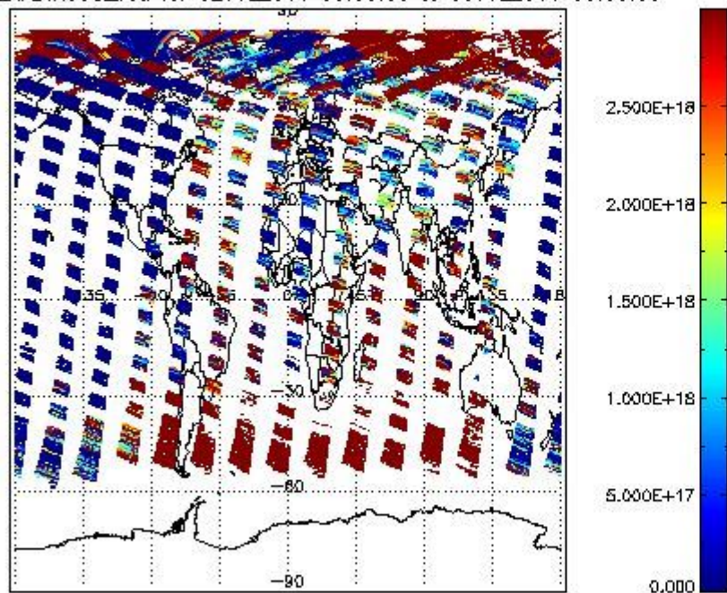
SCIDL2P_NADIR3CO_vcd for 02JUL2011 00:00:00 to 03JUL2011 00:00:00
