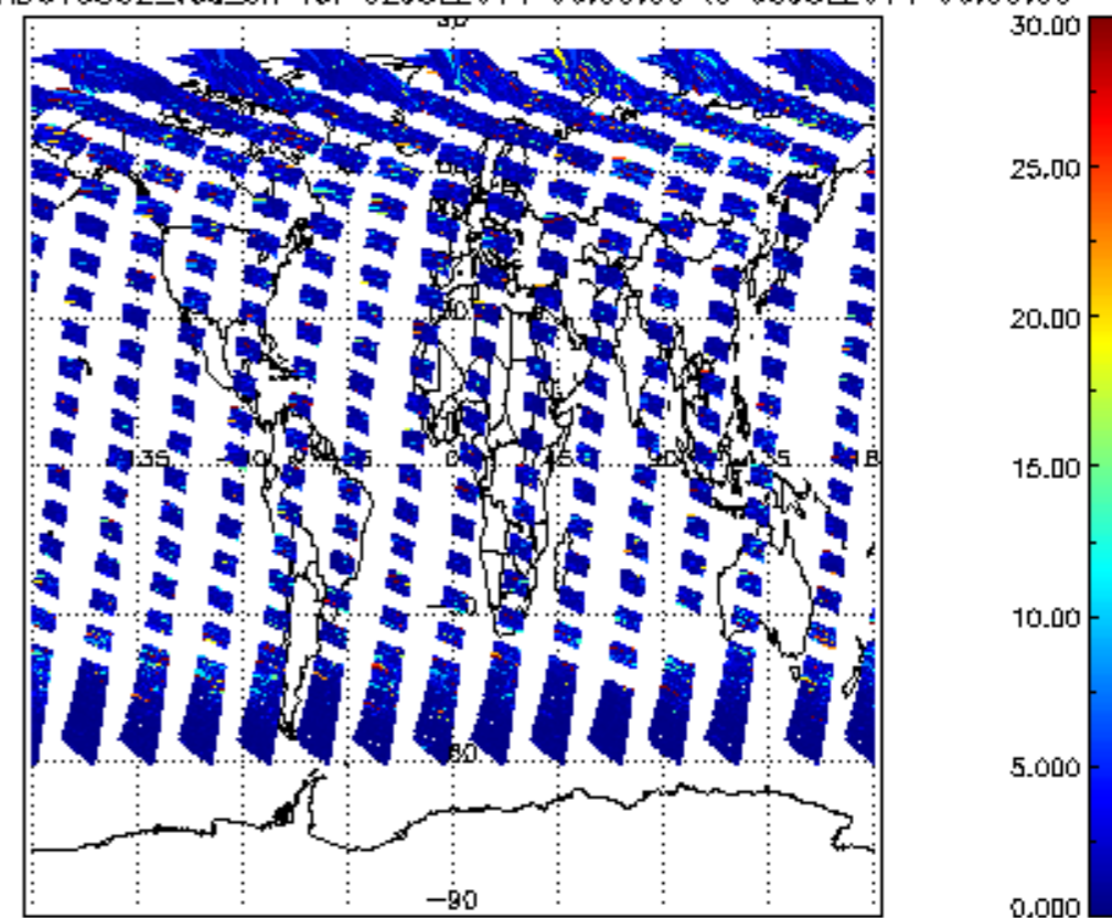
SCIOL2P_NADUV5S02_vcd_err for 02JUL2011 00:00:00 to 03JUL2011 00:00:00
