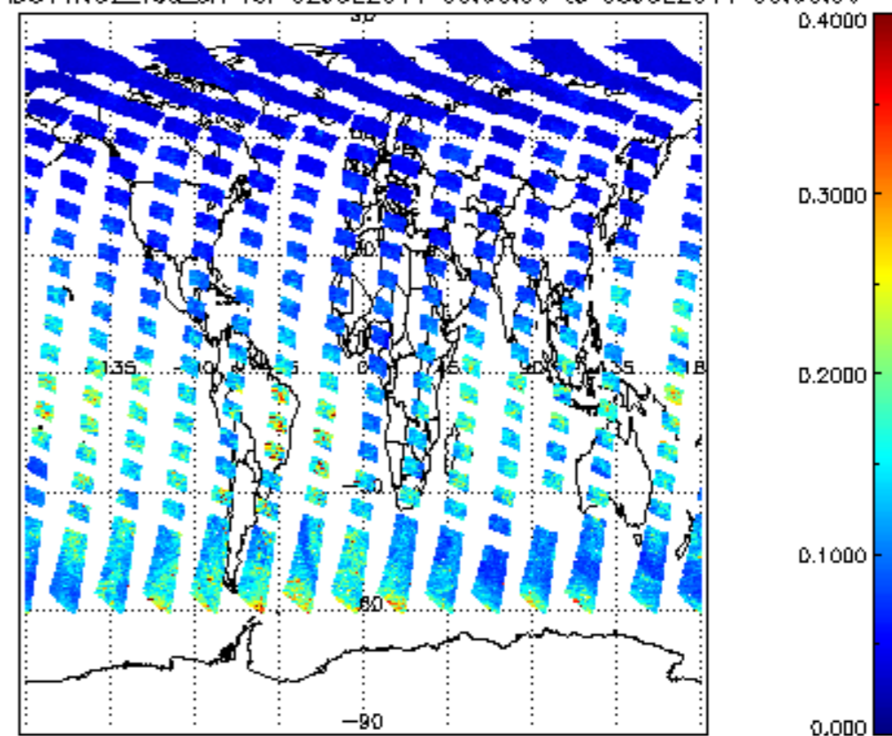
SCIOL2P_NADUV1N02_vcd_err for 02JUL2011 00:00:00 to 03JUL2011 00:00:00
