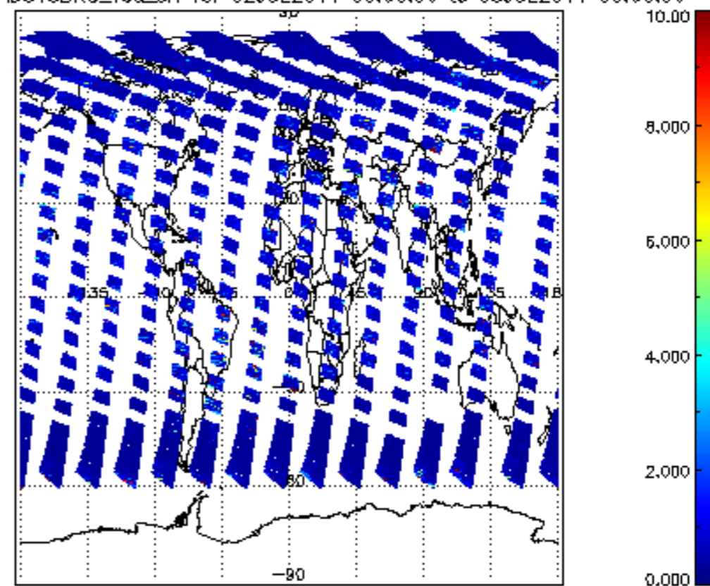
SCIOL2P_NADUV3BRO_vcd_err for 02JUL2011 00:00:00 to 03JUL2011 00:00:00
