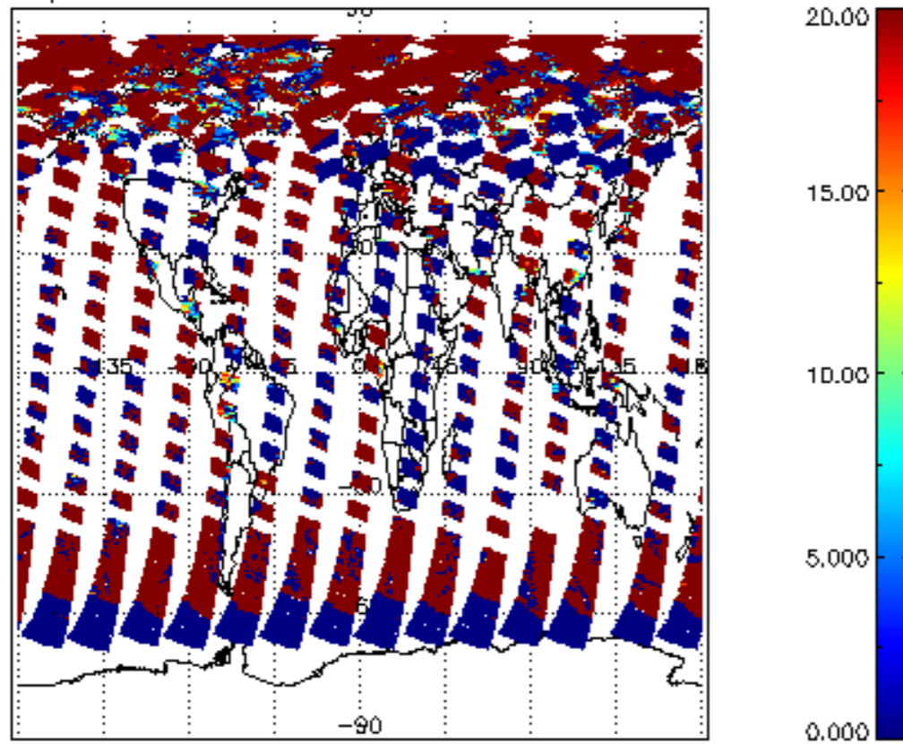
cl_opt_depth for 02JUL2011 00:00:00 to 03JUL2011 00:00:00
