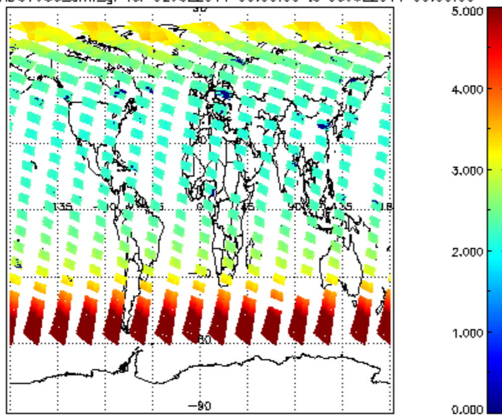
SCIOL2P_NADUV003_amf_gr for 02JUL2011 00:00:00 to 03JUL2011 00:00:00
