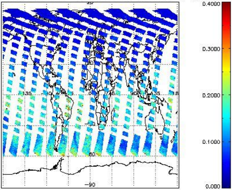
SCIOL2P_NADUV1NO2_vcd_err for 02JUL2011 00:00:00 to 03JUL2011 00:00:00
