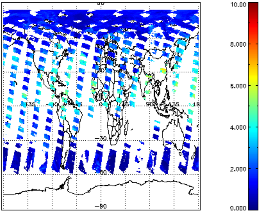
SCIOL2P_NADUV8H20_vcd for 02JUL2011 00:00:00 to 03JUL2011 00:00:00
