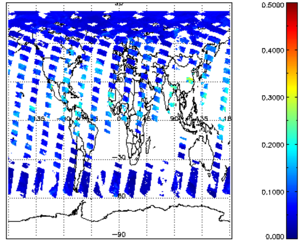
SCIOL2P_NADUV8H20_vcd_err for 02JUL2011 00:00:00 to 03JUL2011 00:00:00
