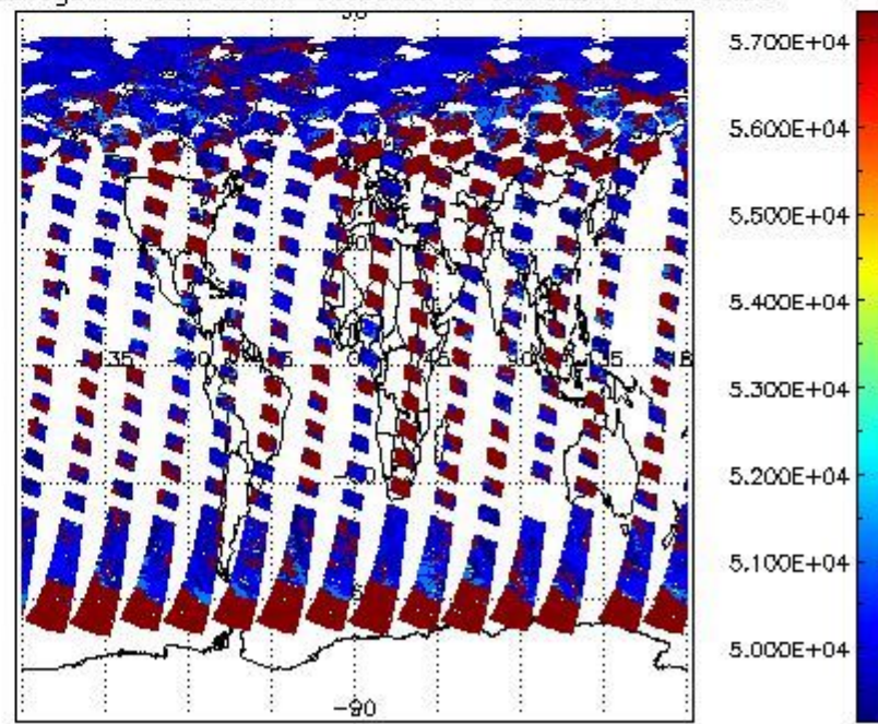
cloud_flags for 02JUL2011 00:00:00 to 03JUL2011 00:00:00
