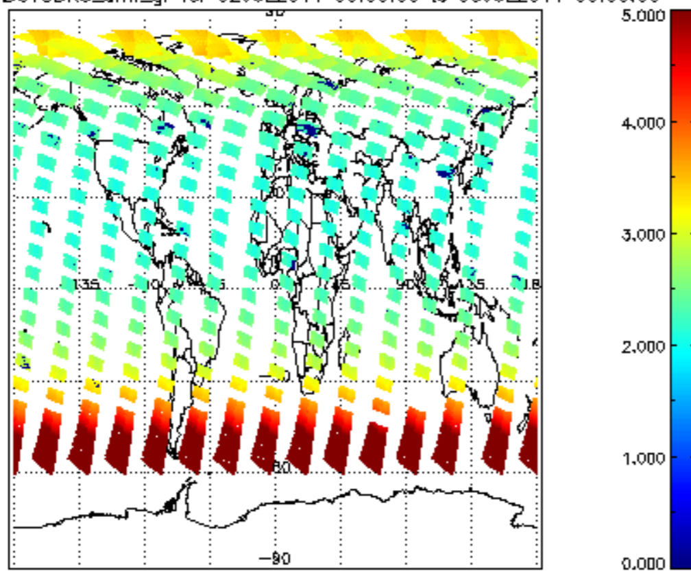
SCIOL2P_NADUV3BRO_arnf_gr for 02JUL2011 00:00:00 to 03JUL2011 00:00:00
