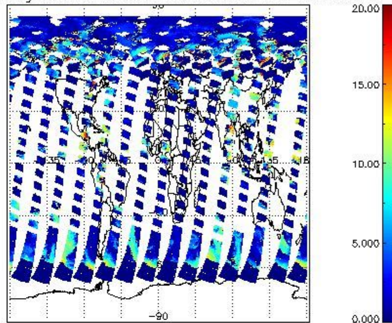
cL_top_height for 02JUL2011 00:00:00 to 03JUL2011 00:00:00
