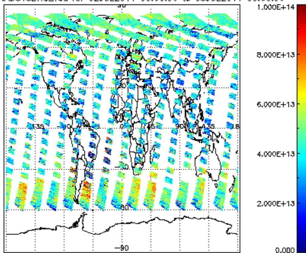
SCIOL2P_NADUV3BRO_vcd for 02JUL2011 00:00:00 to 03JUL2011 00:00:00
