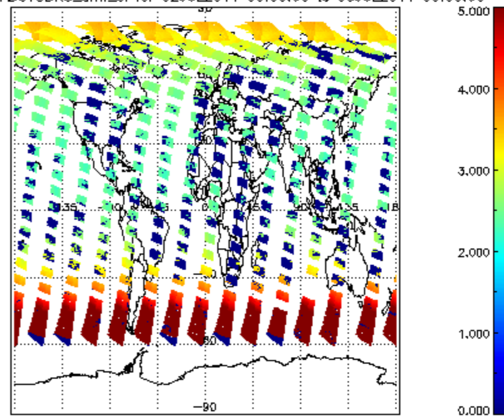
SCIOL2P_NADUV3BRO_arnf_cl for 02JUL2011 00:00:00 to 03JUL2011 00:00:00
