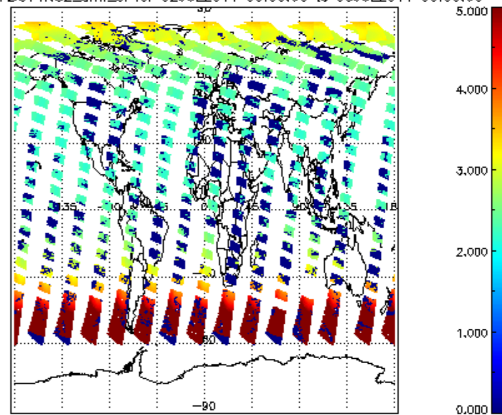
SCIOL2P_NADUV1N02_amf_cl for 02JUL2011 00:00:00 to 03JUL2011 00:00:00
