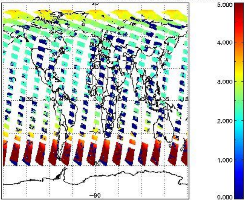
SCIOL2P_NADUV1NO2_amf_cl for 02JUL2011 00:00:00 to 03JUL2011 00:00:00
