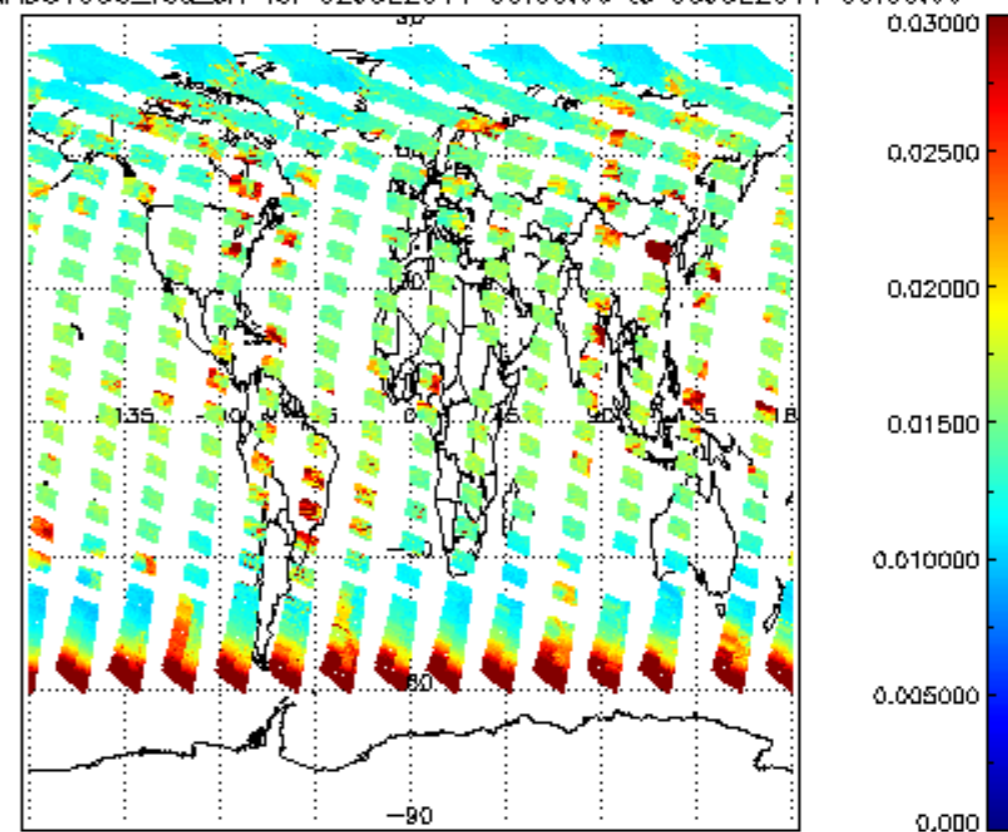
SCIOL2P_NADUV003_vcd_err for 02JUL2011 00:00:00 to 03JUL2011 00:00:00
