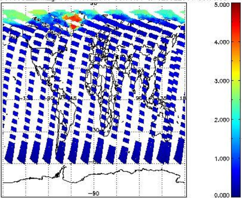
SCIOL2P_NADUV5S02_amf_gr for 01JUL2011 00:00:00 to 02JUL2011 00:00:00
