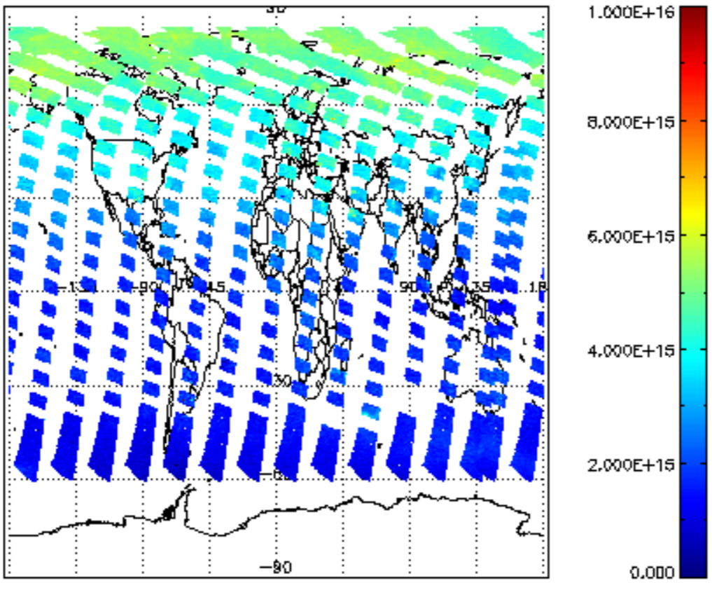
SCIOL2P_NADUV1NO2_vcd for 01JUL2011 00:00:00 to 02JUL2011 00:00:00
