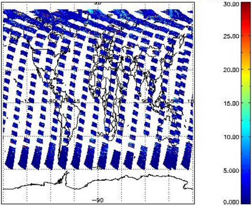
SCIOL2P_NADUV5S02_vcd_err for 01JUL2011 00:00:00 to 02JUL2011 00:00:00
