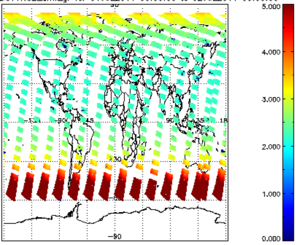
SCIOL2P_NADUV1NO2_amf_gr for 01JUL2011 00:00:00 to 02JUL2011 00:00:00
