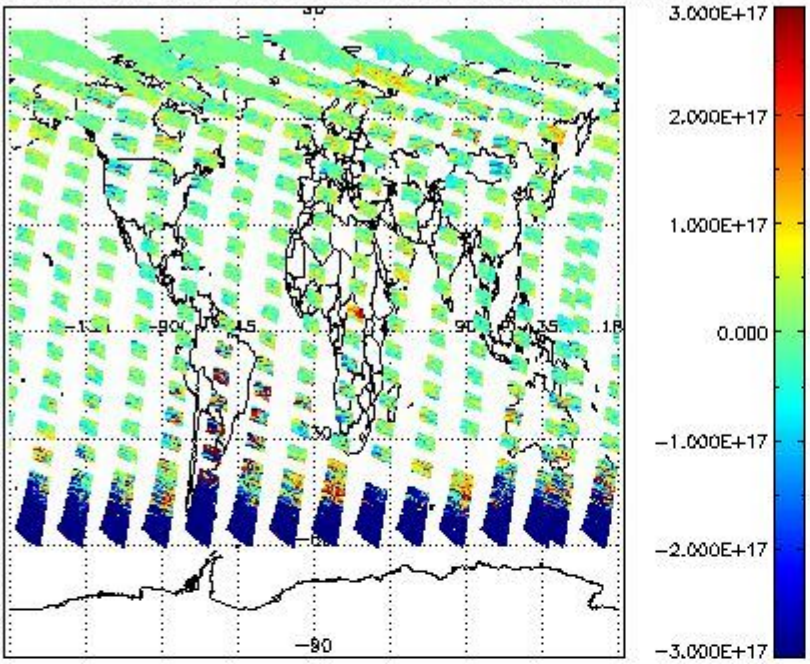
SCIOL2P_NADUV5S02_vcd for 01JUL2011 00:00:00 to 02JUL2011 00:00:00
