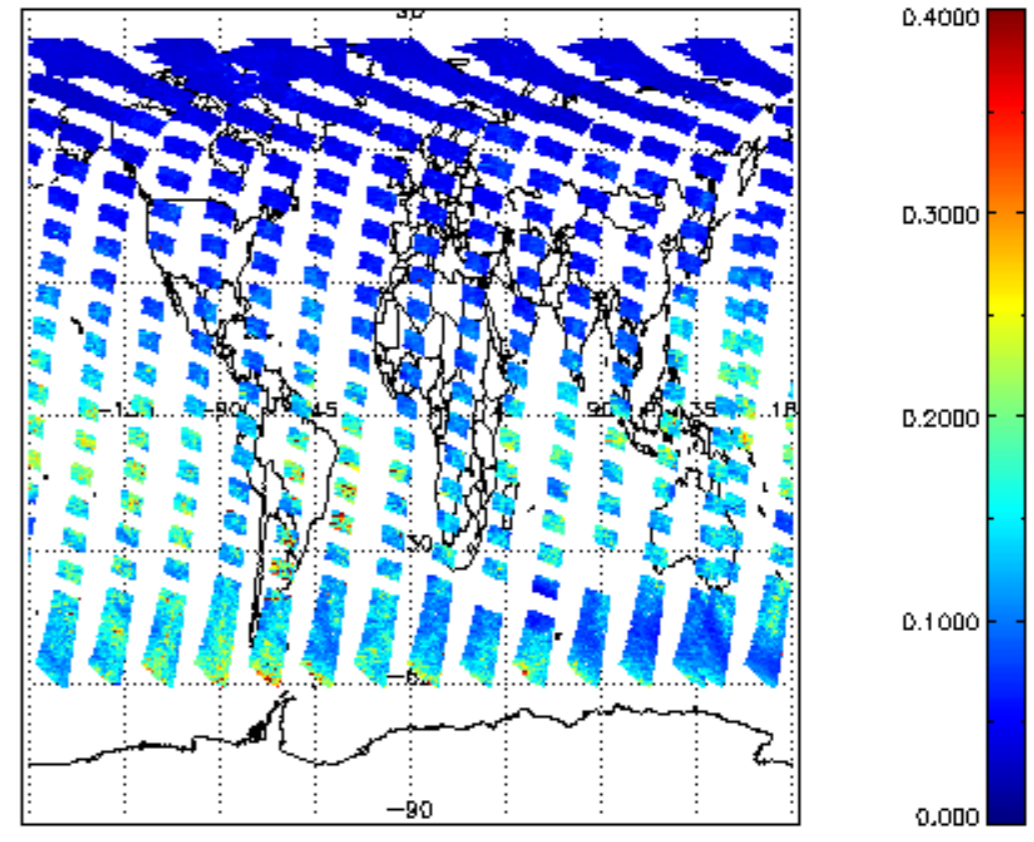
SCIOL2P_NADUV1NO2_vcd_err for 01JUL2011 00:00:00 to 02JUL2011 00:00:00
