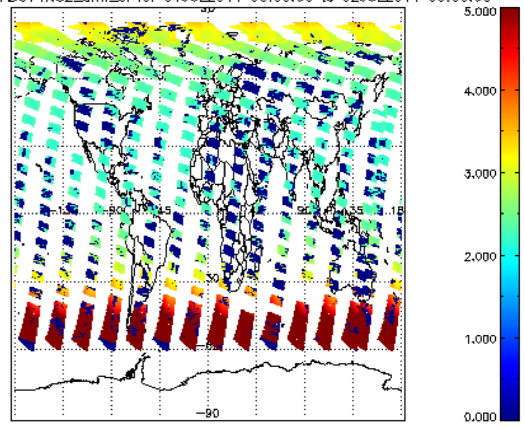
SCIOL2P_NADUV1NO2_amf_cl for 01JUL2011 00:00:00 to 02JUL2011 00:00:00
