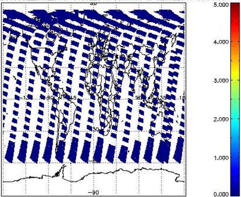
SCIOL2P_NADUV5S02_amf_cl for 01JUL2011 00:00:00 to 02JUL2011 00:00:00
