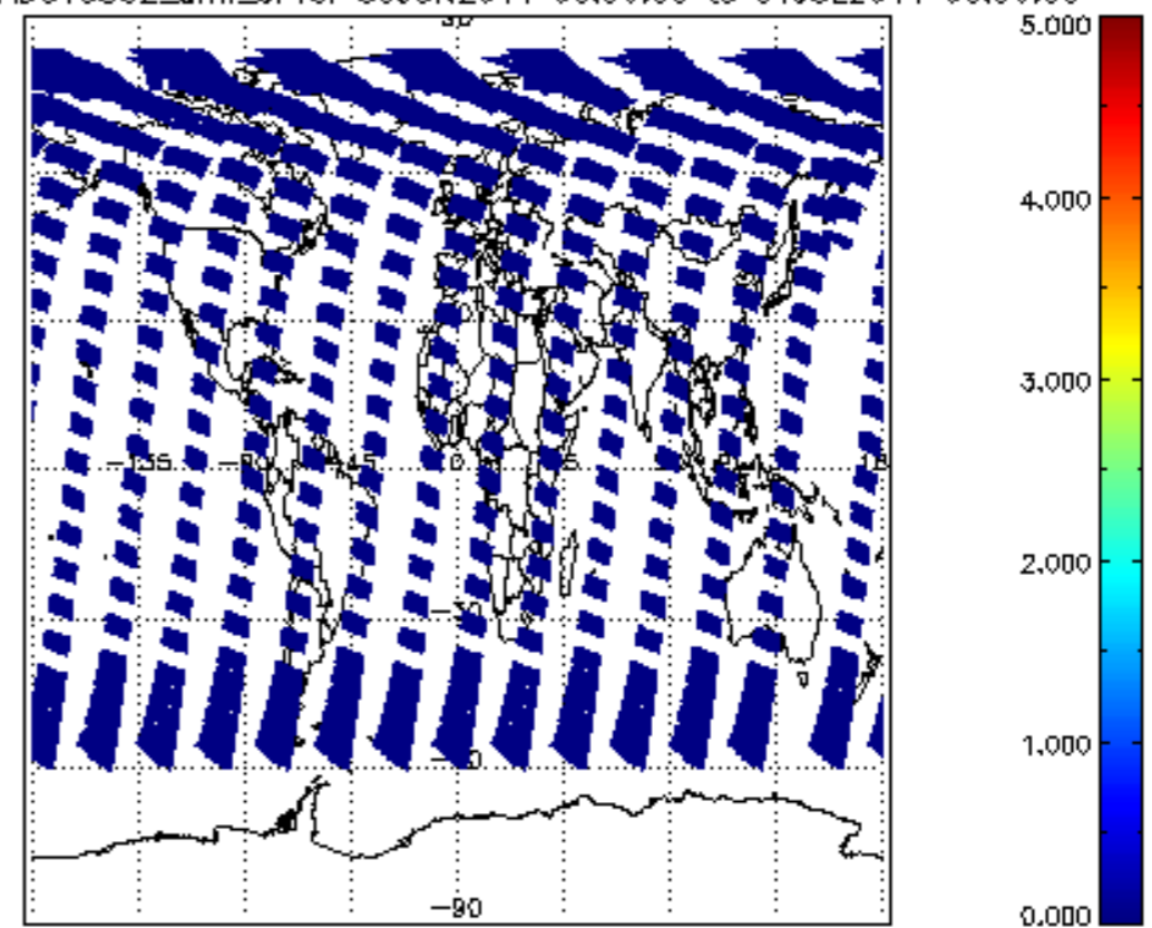
SCIOL2P_NADUV5S02_amf_cl for 30JUN2011 00:00:00 to 01JUL2011 00:00:00
