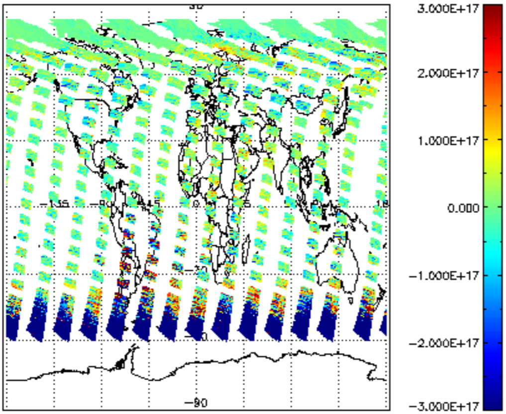
SCIOL2P_NADUV5S02_vcd for 30JUN2011 00:00:00 to 01JUL2011 00:00:00
