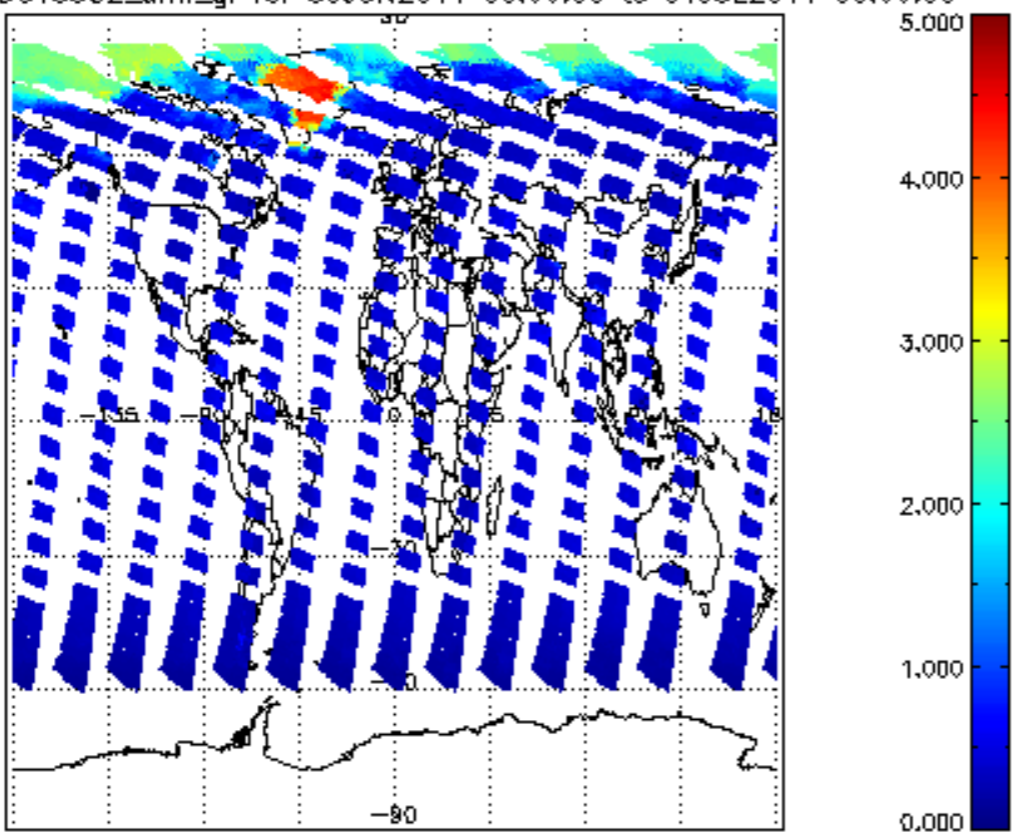
SCIOL2P_NADUV5S02_amf_gr for 30JUN2011 00:00:00 to 01JUL2011 00:00:00
