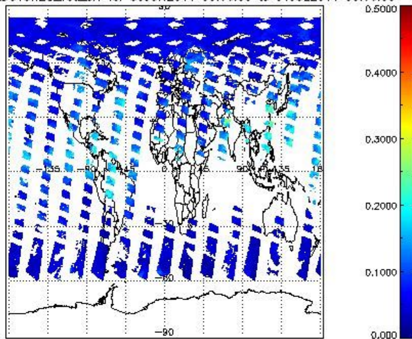
SCIOL2P_NADUV8H20_vcd_err for 30JUN2011 00:00:00 to 01JUL2011 00:00:00
