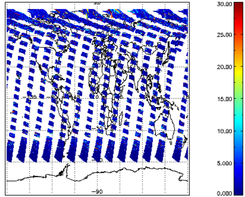
SCIOL2P_NADUV5S02_vcd_err for 30JUN2011 00:00:00 to 01JUL2011 00:00:00
