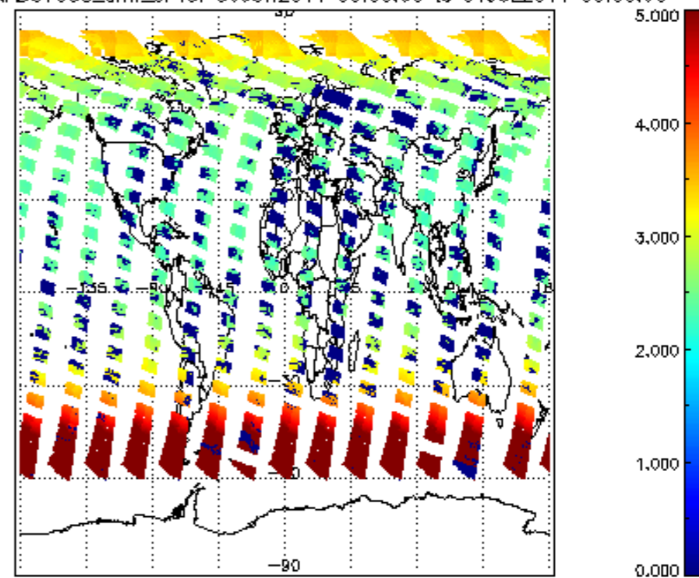
SCIOL2P_NADUV003_amf_sl for 30JUN2011 00:00:00 to 01JUL2011 00:00:00
