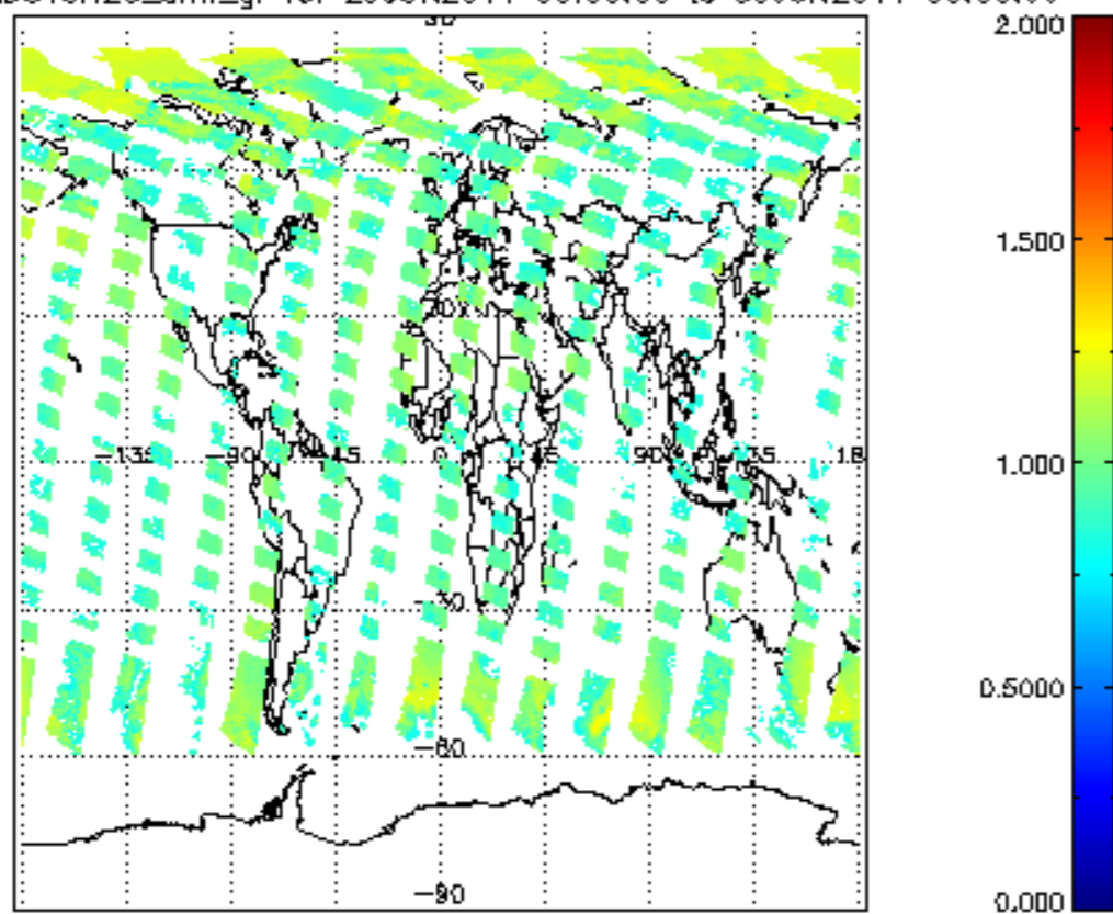
SCIOL2P_NADUV8H2O_amf_gr for 29JUN2011 00:00:00 to 30JUN2011 00:00:00
