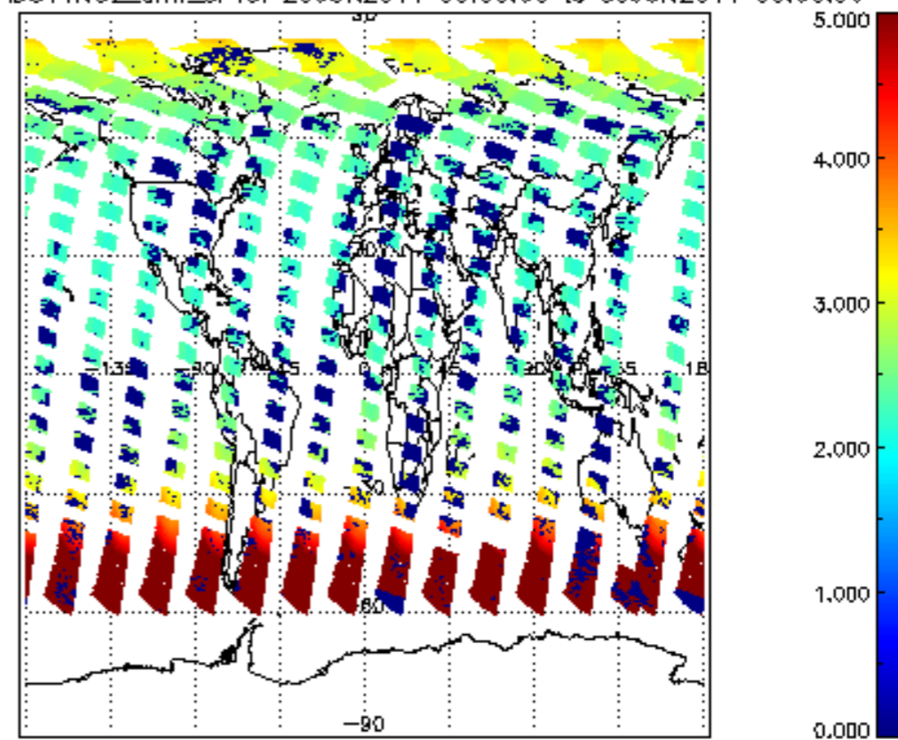
SCIOL2P_NADUV1NO2_amf_sl for 29JUN2011 00:00:00 to 30JUN2011 00:00:00
