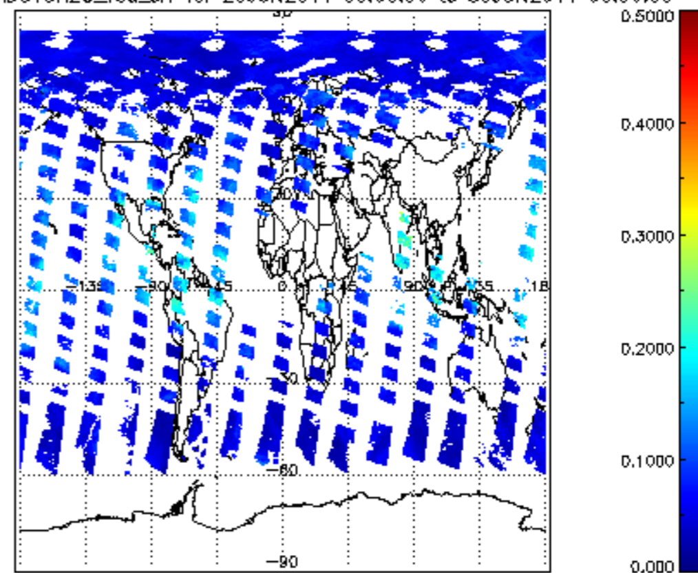
SCIOL2P_NADUV8H2O_vcd_err for 29JUN2011 00:00:00 to 30JUN2011 00:00:00
