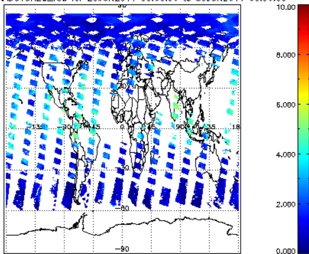
SCIOL2P_NADUV8H2O_vcd for 29JUN2011 00:00:00 to 30JUN2011 00:00:00
