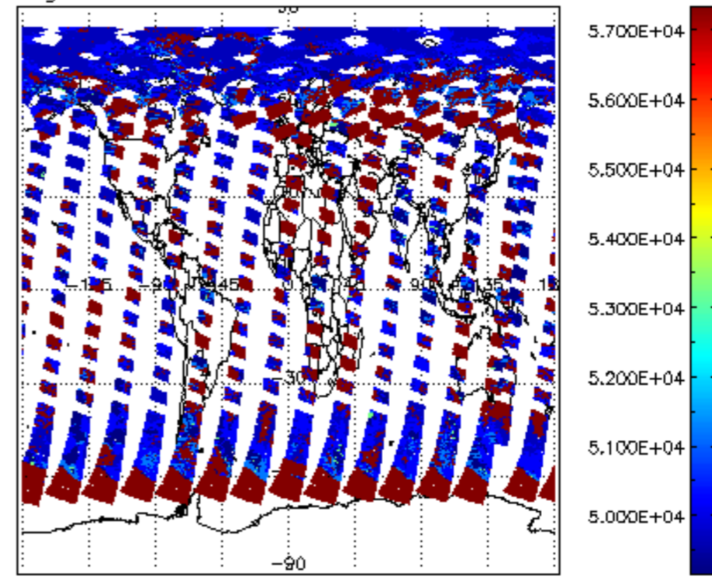
cloud_flags for 28JUN2011 00:00:00 to 29JUN2011 00:00:00
