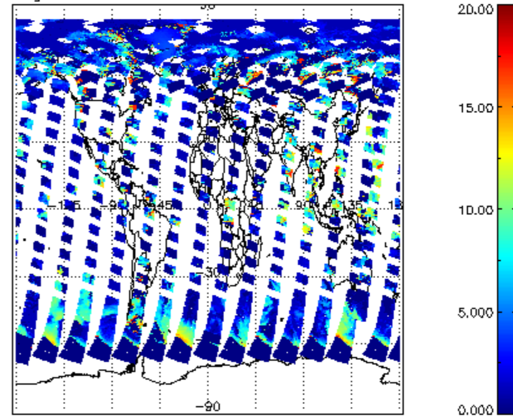
cl_top_height for 28JUN2011 00:00:00 to 29JUN2011 00:00:00
