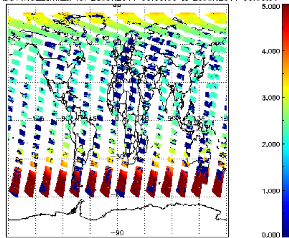
SCIOL2P_NADUV1NO2_amf_sl for 28JUN2011 00:00:00 to 29JUN2011 00:00:00
