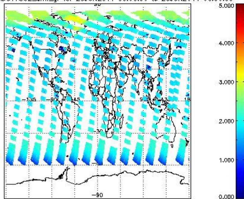
SCIOL2P_NADUV7S02_amf_gr for 25JUN2011 00:00:00 to 26JUN2011 00:00:00
