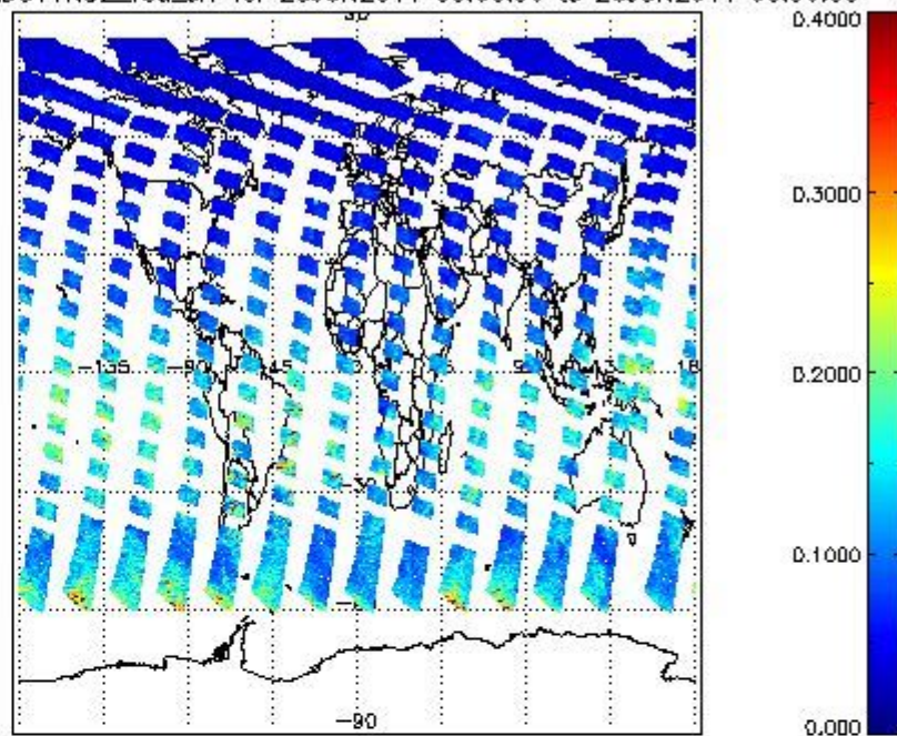
SCIOL2P_NADUV1NO2_vcd_err for 25JUN2011 00:00:00 to 26JUN2011 00:00:00
