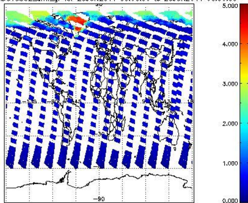
SCIOL2P_NADUV5S02_amf_gr for 25JUN2011 00:00:00 to 26JUN2011 00:00:00
