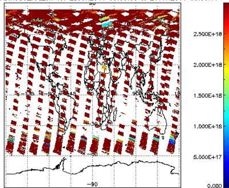
SCIOL2P_NADIR3CO_vcd_err for 25JUN2011 00:00:00 to 26JUN2011 00:00:00
