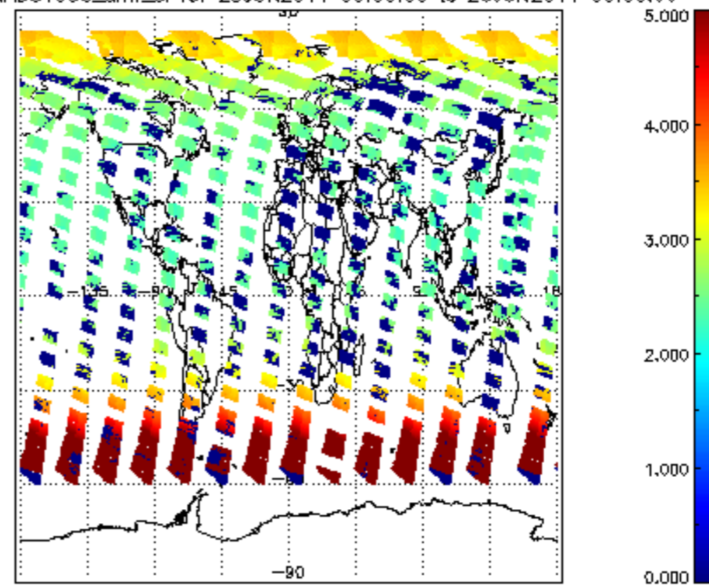
SCIOL2P_NADUV003_amf_cl for 25JUN2011 00:00:00 to 26JUN2011 00:00:00
