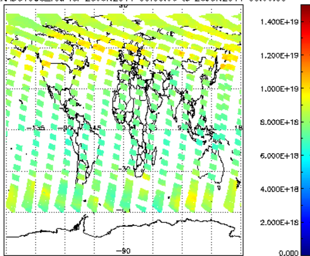
SCIOL2P_NADUV003_vcd for 25JUN2011 00:00:00 to 26JUN2011 00:00:00
