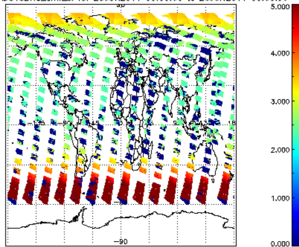
SCIOL2P_NADUV3BRO_amf_sl for 25JUN2011 00:00:00 to 26JUN2011 00:00:00
