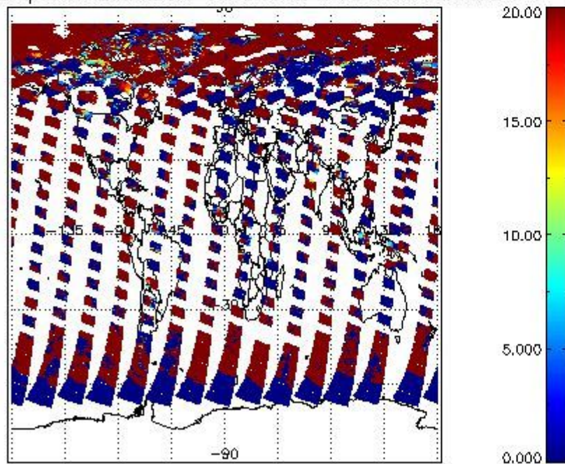
cL_opt_depth for 25JUN2011 00:00:00 to 26JUN2011 00:00:00
