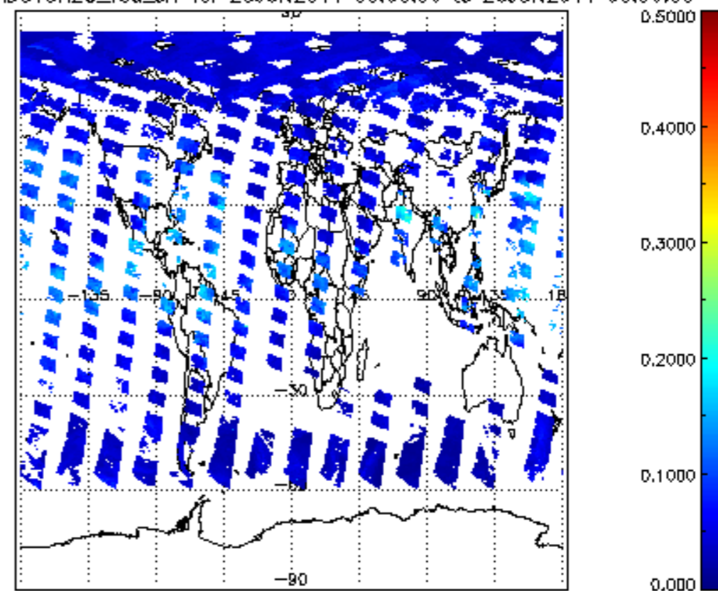
SCIOL2P_NADUV8H2O_vcd_err for 25JUN2011 00:00:00 to 26JUN2011 00:00:00
