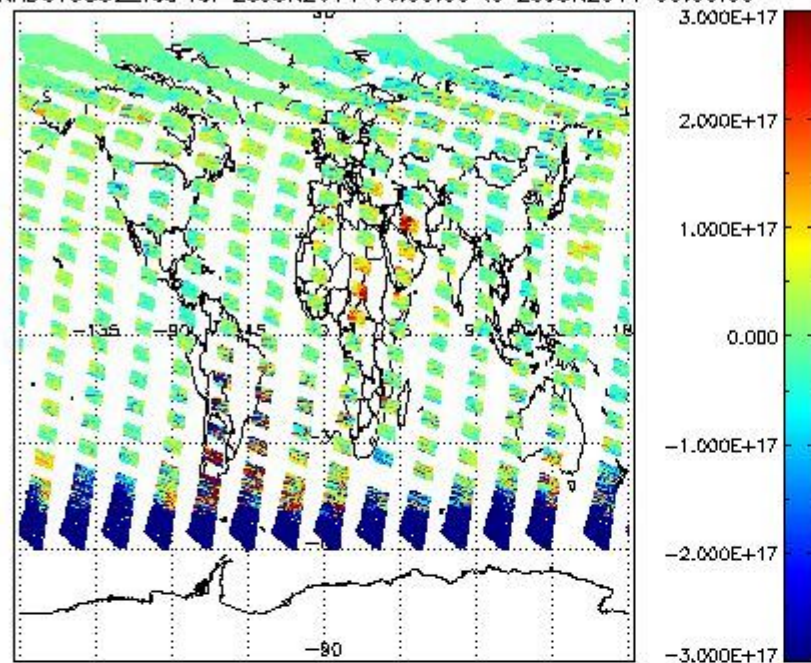
SCIOL2P_NADUV5S02_vcd for 25JUN2011 00:00:00 to 26JUN2011 00:00:00
