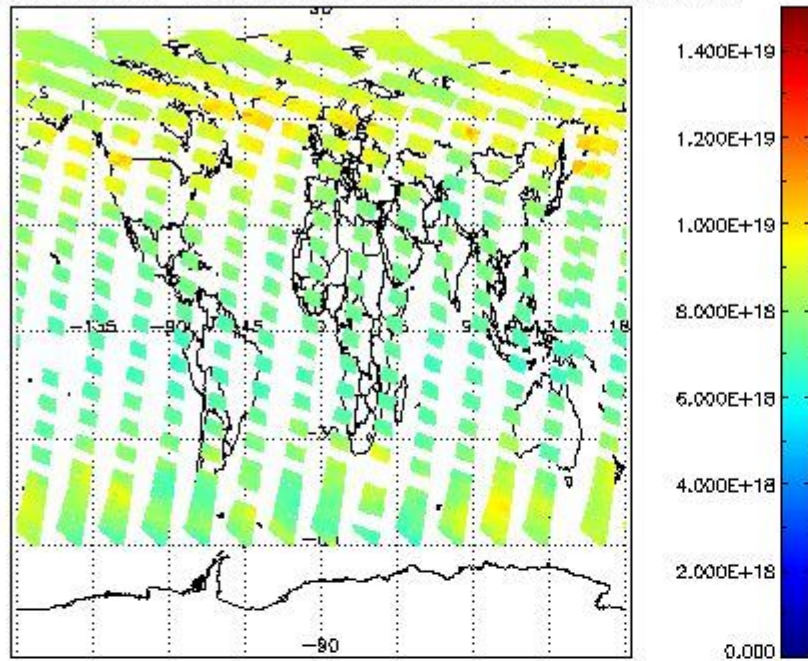
SCIOL2P_NADUV003_vcd for 25JUN2011 00:00:00 to 26JUN2011 00:00:00
