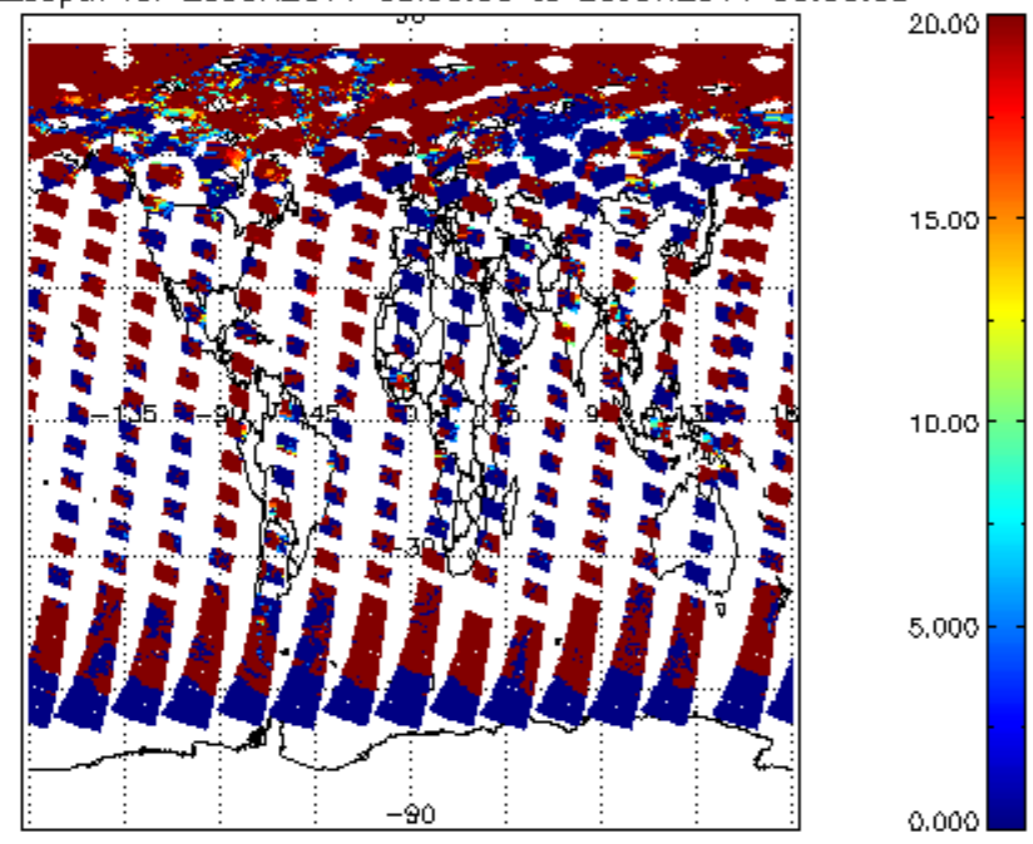
cl_opt_depth for 25JUN2011 00:00:00 to 26JUN2011 00:00:00
