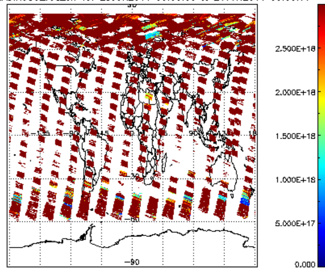
SCIOL2P_NADIR3CO_vcd_err for 25JUN2011 00:00:00 to 26JUN2011 00:00:00
