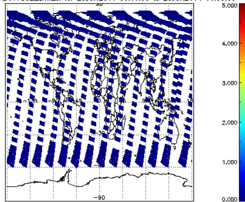
SCIOL2P_NADUV7S02_amf_cl for 25JUN2011 00:00:00 to 26JUN2011 00:00:00
