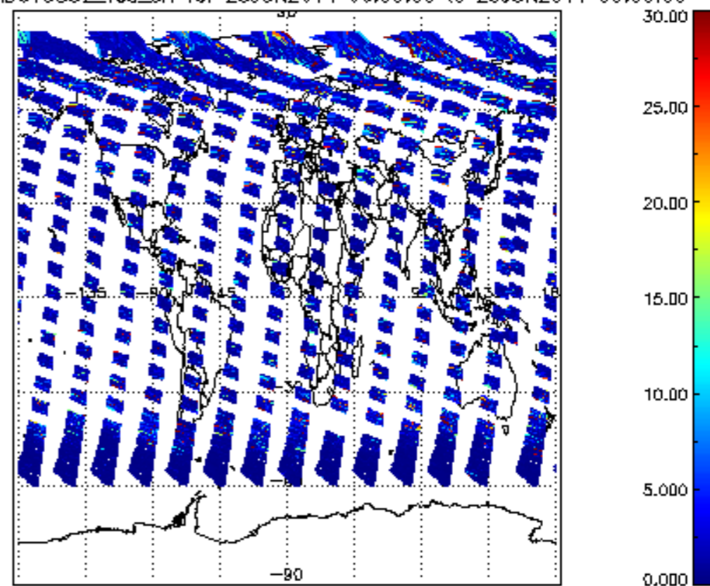
SCIOL2P_NADUV5S02_vcd_err for 25JUN2011 00:00:00 to 26JUN2011 00:00:00
