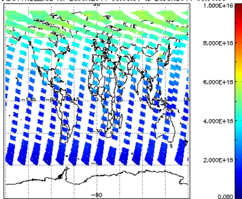
SCIOL2P_NADUV1NO2_vcd for 25JUN2011 00:00:00 to 26JUN2011 00:00:00
