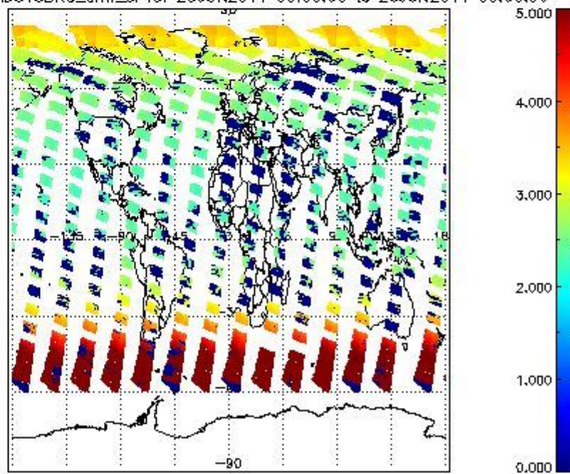
SCIOL2P_NADUV3BRO_amf_cl for 25JUN2011 00:00:00 to 26JUN2011 00:00:00
