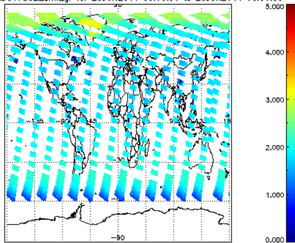
SCIOL2P_NADUV7S02_amf_gr for 25JUN2011 00:00:00 to 26JUN2011 00:00:00
