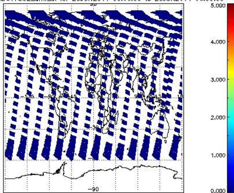
SCIOL2P_NADUV7S02_amf_cl for 25JUN2011 00:00:00 to 26JUN2011 00:00:00
