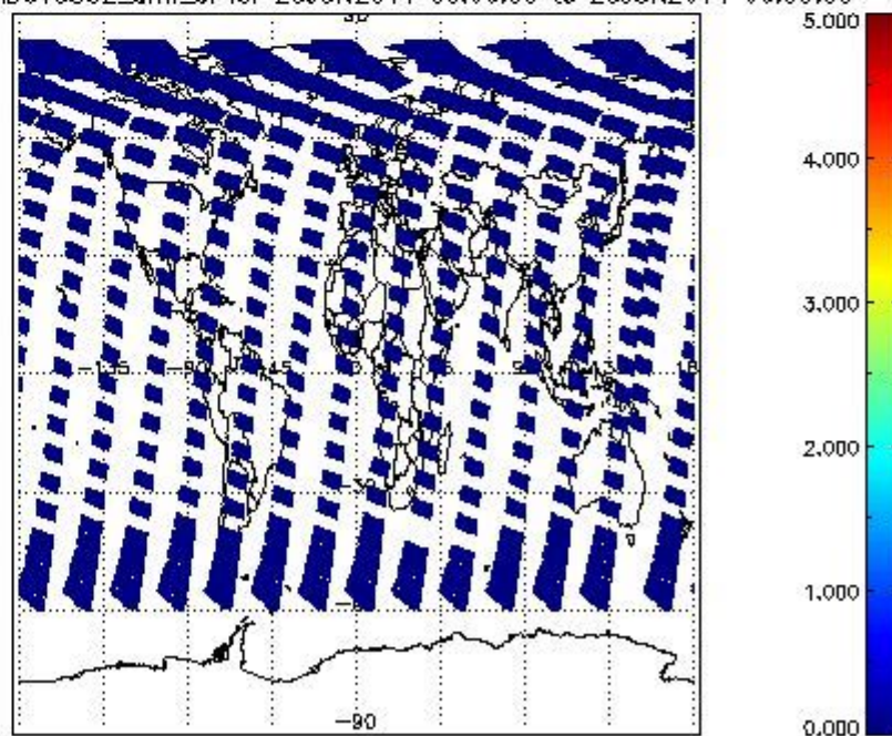
SCIOL2P_NADUV5S02_amf_cl for 25JUN2011 00:00:00 to 26JUN2011 00:00:00
