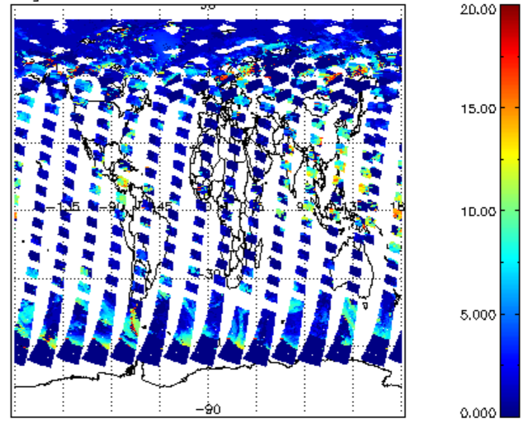
cl_top_height for 25JUN2011 00:00:00 to 26JUN2011 00:00:00
