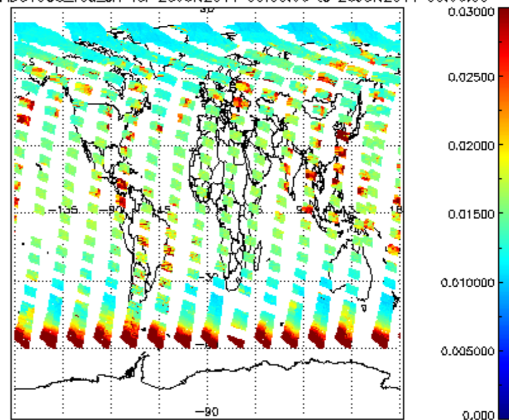
SCIOL2P_NADUV003_vcd_err for 25JUN2011 00:00:00 to 26JUN2011 00:00:00
