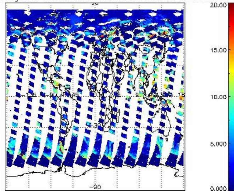
cL_top_height for 25JUN2011 00:00:00 to 26JUN2011 00:00:00
