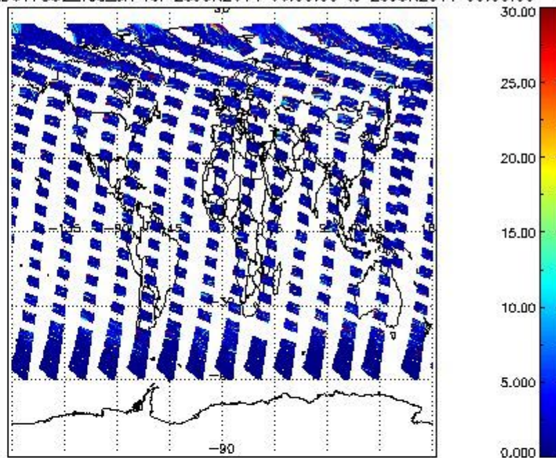
SCIOL2P_NADUV7S02_vcd_err for 25JUN2011 00:00:00 to 26JUN2011 00:00:00
