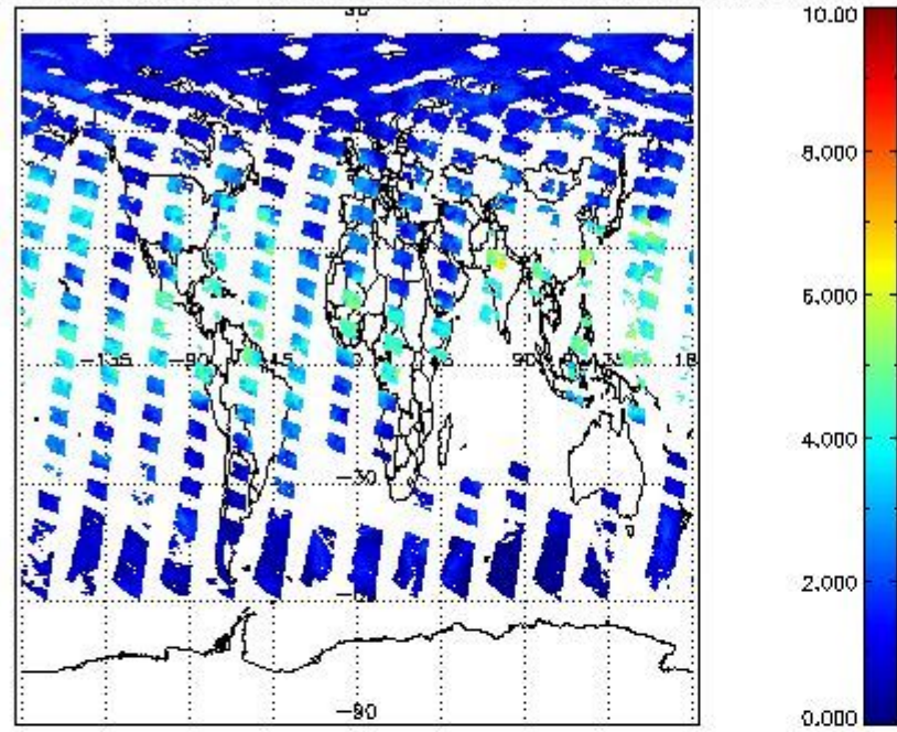
SCIOL2P_NADUV8H2O_vcd for 25JUN2011 00:00:00 to 26JUN2011 00:00:00
