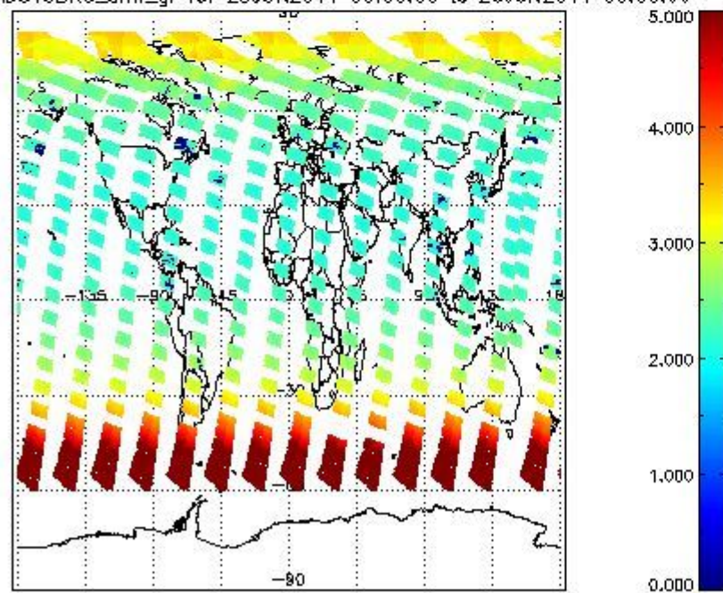
SCIOL2P_NADUV3BRO_amf_gr for 25JUN2011 00:00:00 to 26JUN2011 00:00:00
