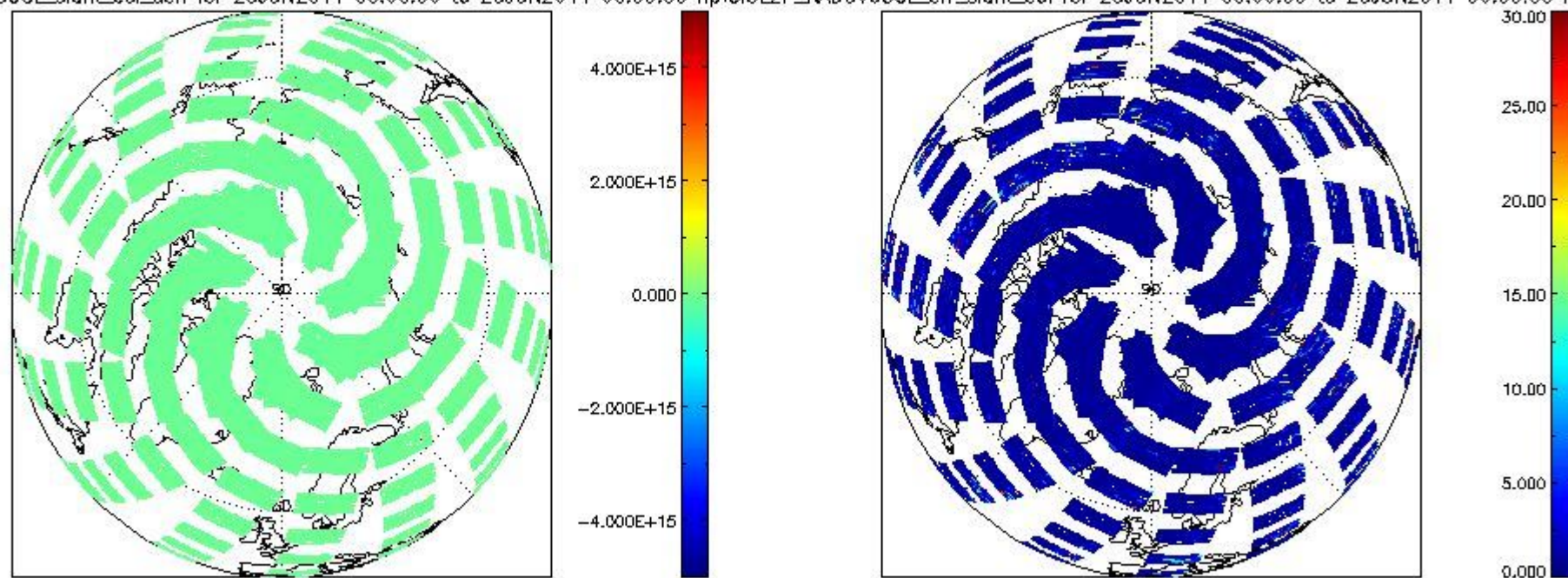
CIOL2P_NADUV6OCLslant_col_den for 25JUN2011 00:00:00 to 26JUN2011 00:00:00 np; CIOL2P_NADUV6OCLarr_slant_col for 25JUN2011 00:00:00 to 26JUN2011 00:00:00 np
