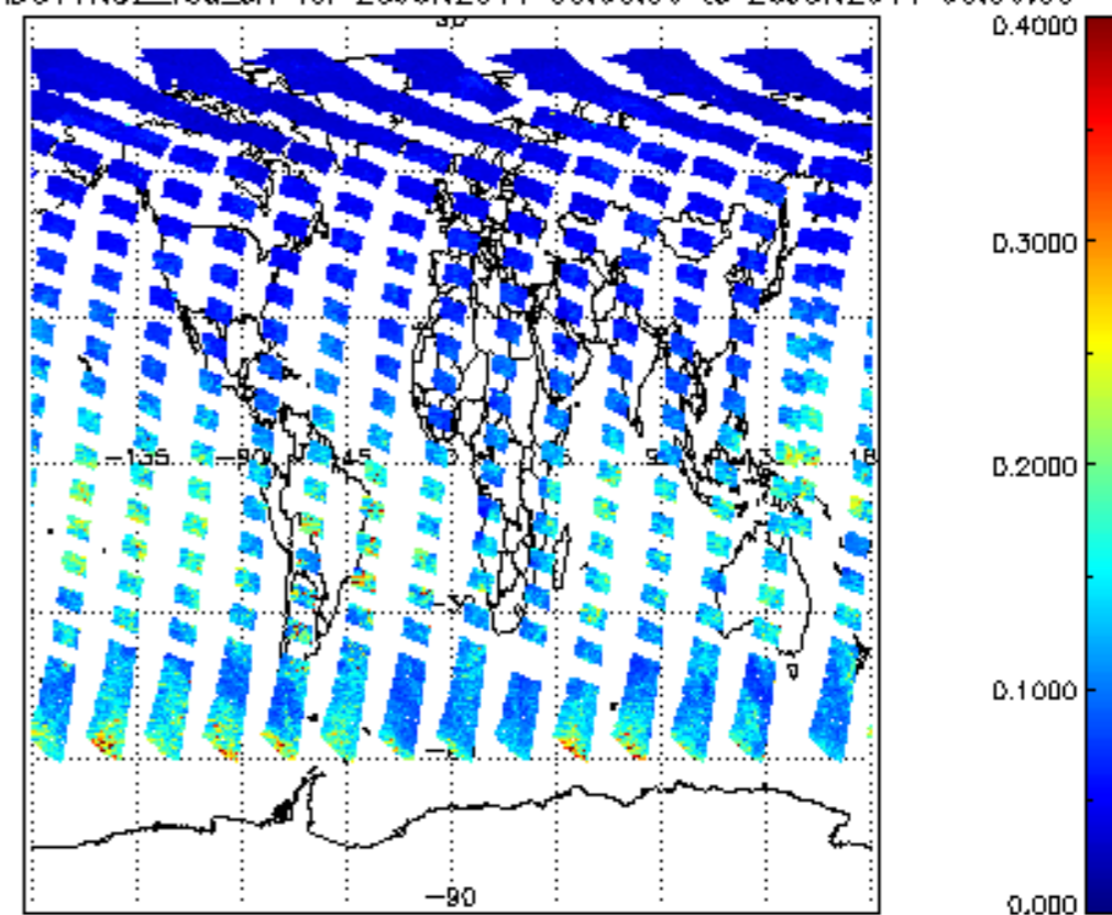
SCIOL2P_NADUV1NO2_vcd_err for 25JUN2011 00:00:00 to 26JUN2011 00:00:00
