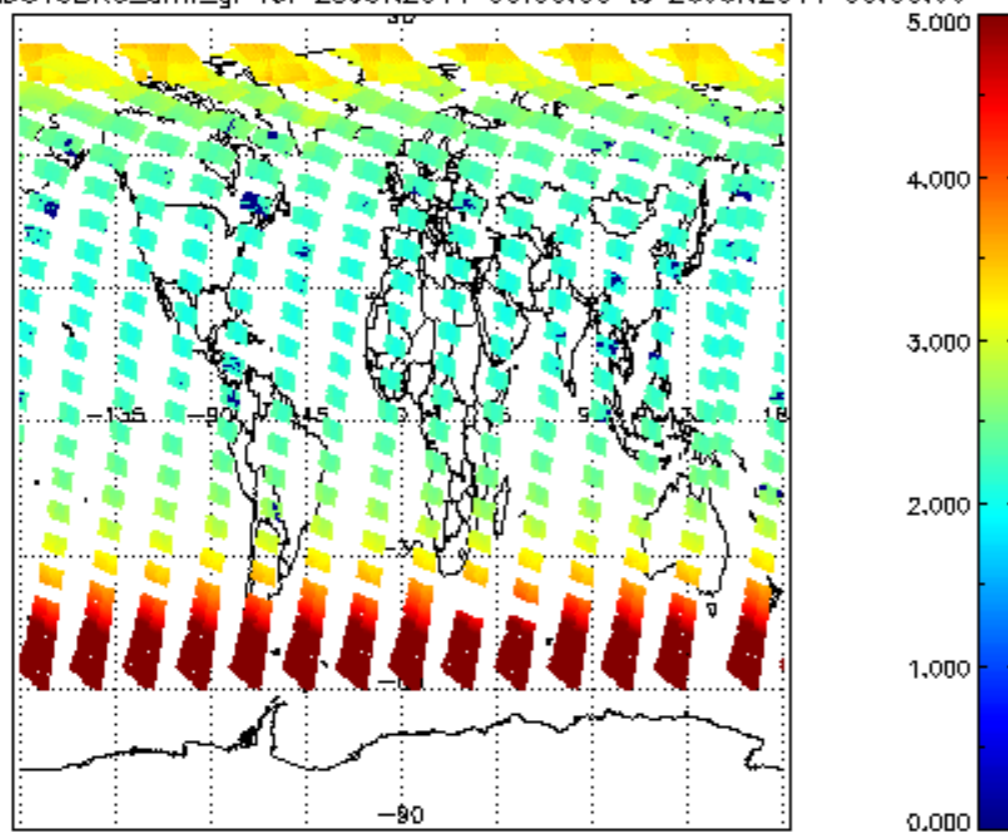
SCIOL2P_NADUV3BRO_amf_gr for 25JUN2011 00:00:00 to 26JUN2011 00:00:00
