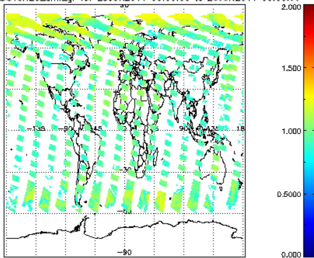
SCIOL2P_NADUV8H2O_amf_gr for 25JUN2011 00:00:00 to 26JUN2011 00:00:00
