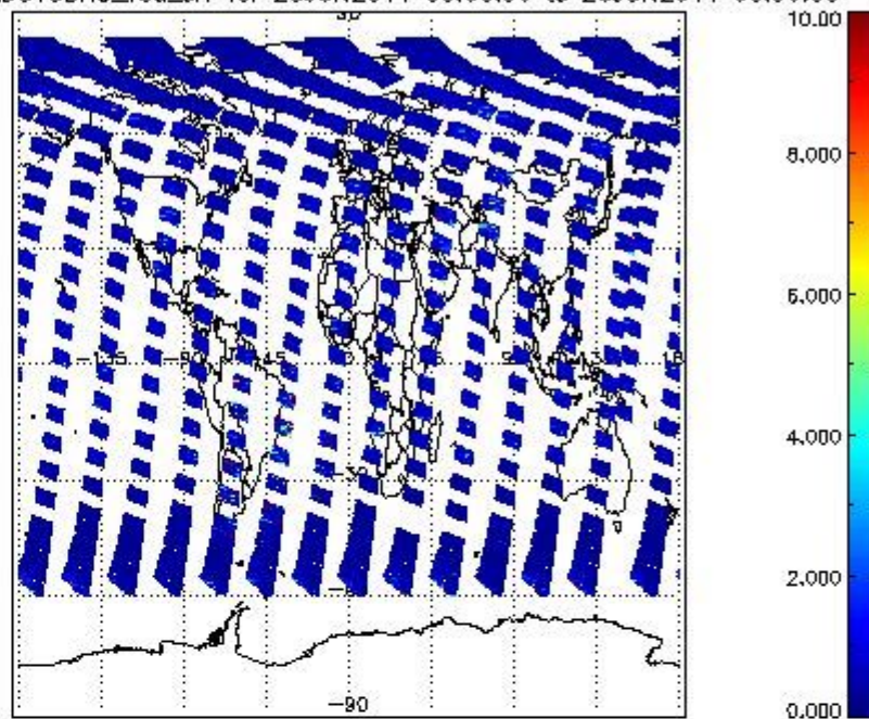
SCIOL2P_NADUV3BRO_vcd_err for 25JUN2011 00:00:00 to 26JUN2011 00:00:00
