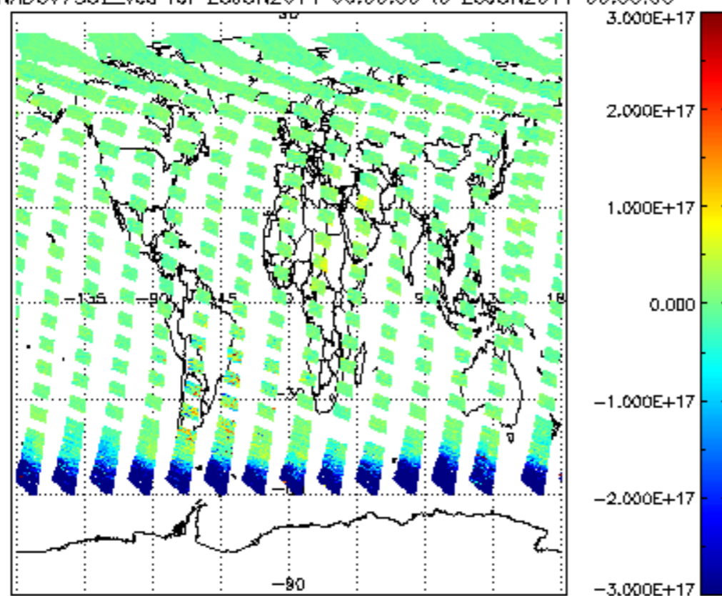
SCIOL2P_NADUV7S02_vcd for 25JUN2011 00:00:00 to 26JUN2011 00:00:00
