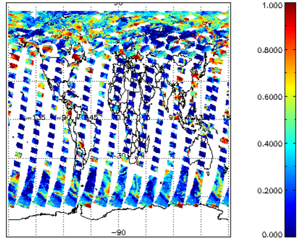
cl_frac for 25JUN2011 00:00:00 to 26JUN2011 00:00:00
