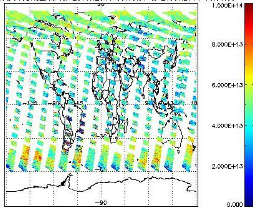
SCIOL2P_NADUV3BRO_vcd for 25JUN2011 00:00:00 to 26JUN2011 00:00:00
