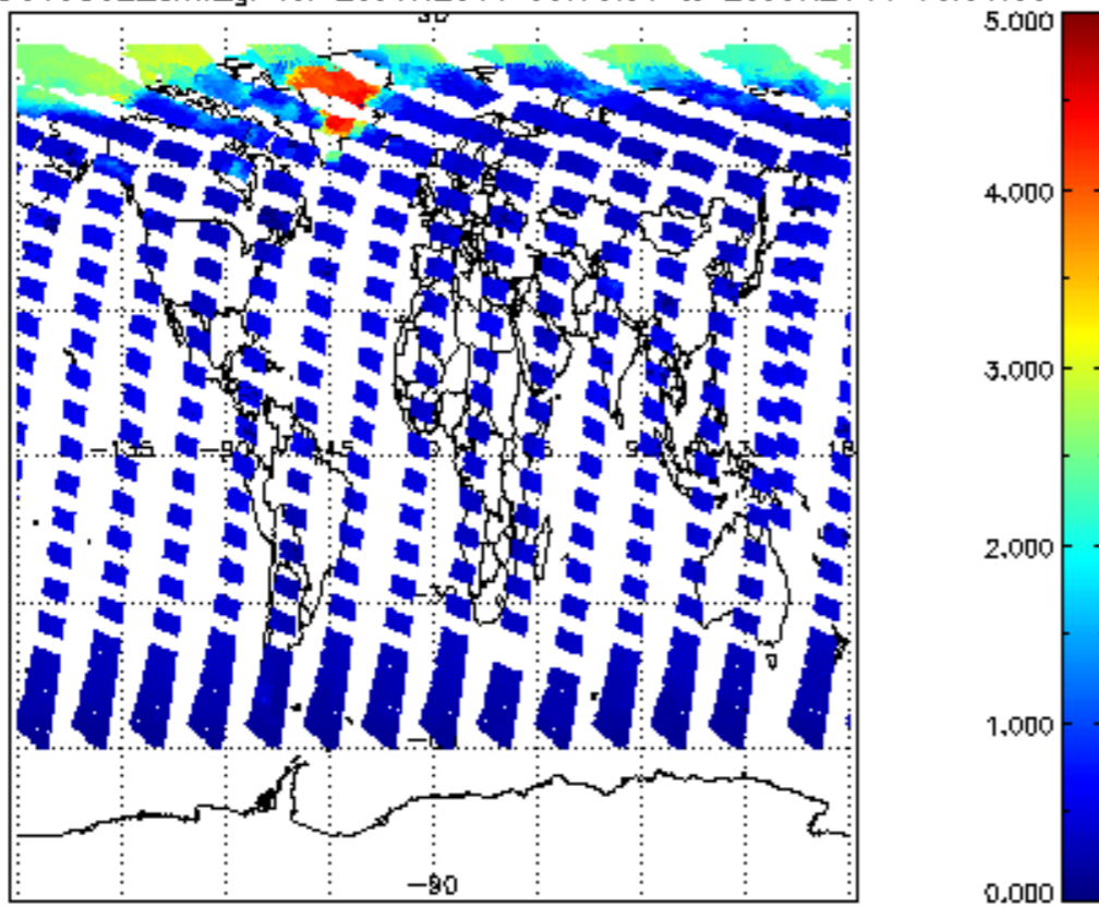
SCIOL2P_NADUV5S02_amf_gr for 25JUN2011 00:00:00 to 26JUN2011 00:00:00
