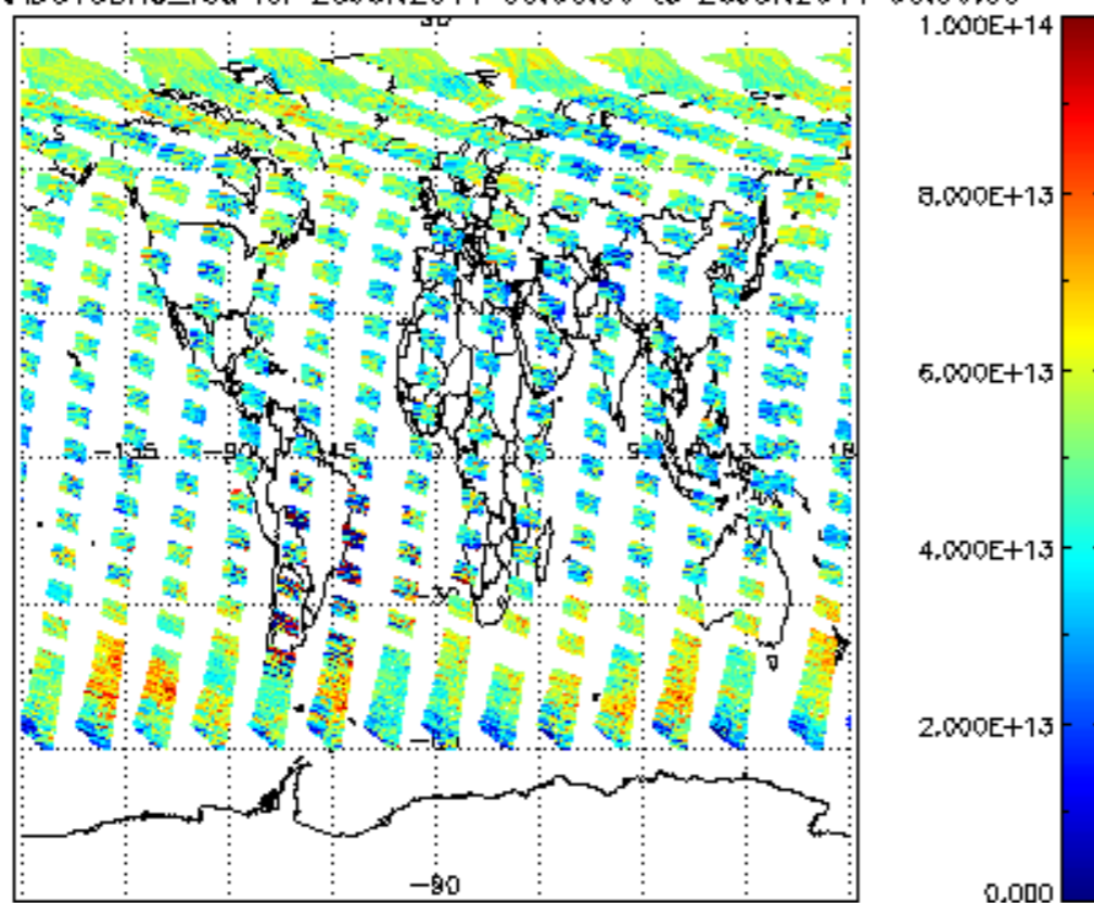
SCIOL2P_NADUV3BRO_vcd for 25JUN2011 00:00:00 to 26JUN2011 00:00:00
