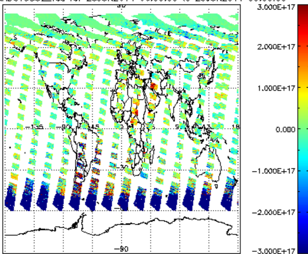
SCIOL2P_NADUV5S02_vcd for 25JUN2011 00:00:00 to 26JUN2011 00:00:00
