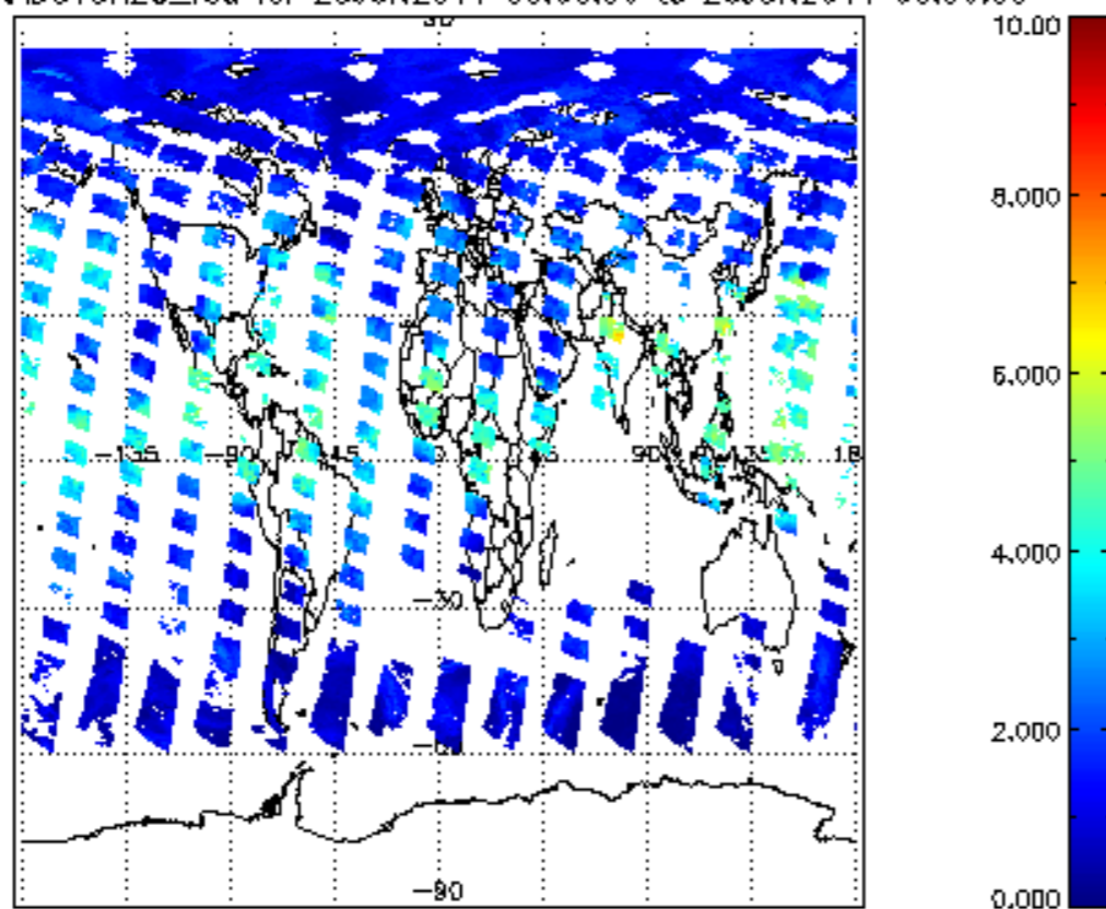
SCIOL2P_NADUV8H2O_vcd for 25JUN2011 00:00:00 to 26JUN2011 00:00:00
