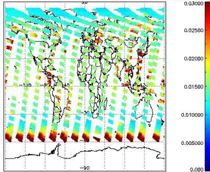
SCIOL2P_NADUV003_vcd_err for 25JUN2011 00:00:00 to 26JUN2011 00:00:00
