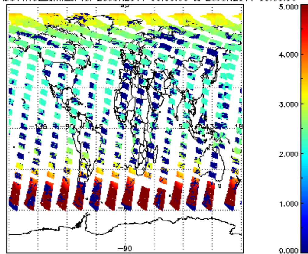
SCIOL2P_NADUV1NO2_amf_sl for 25JUN2011 00:00:00 to 26JUN2011 00:00:00
