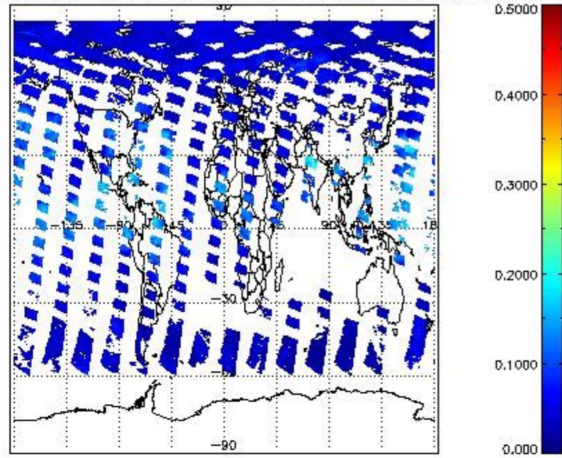
SCIOL2P_NADUV8H2O_vcd_err for 25JUN2011 00:00:00 to 26JUN2011 00:00:00
