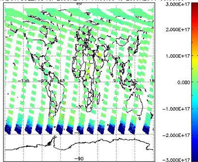
SCIOL2P_NADUV7S02_vcd for 25JUN2011 00:00:00 to 26JUN2011 00:00:00
