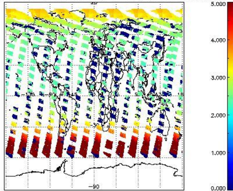
SCIOL2P_NADUV003_amf_cl for 25JUN2011 00:00:00 to 26JUN2011 00:00:00
