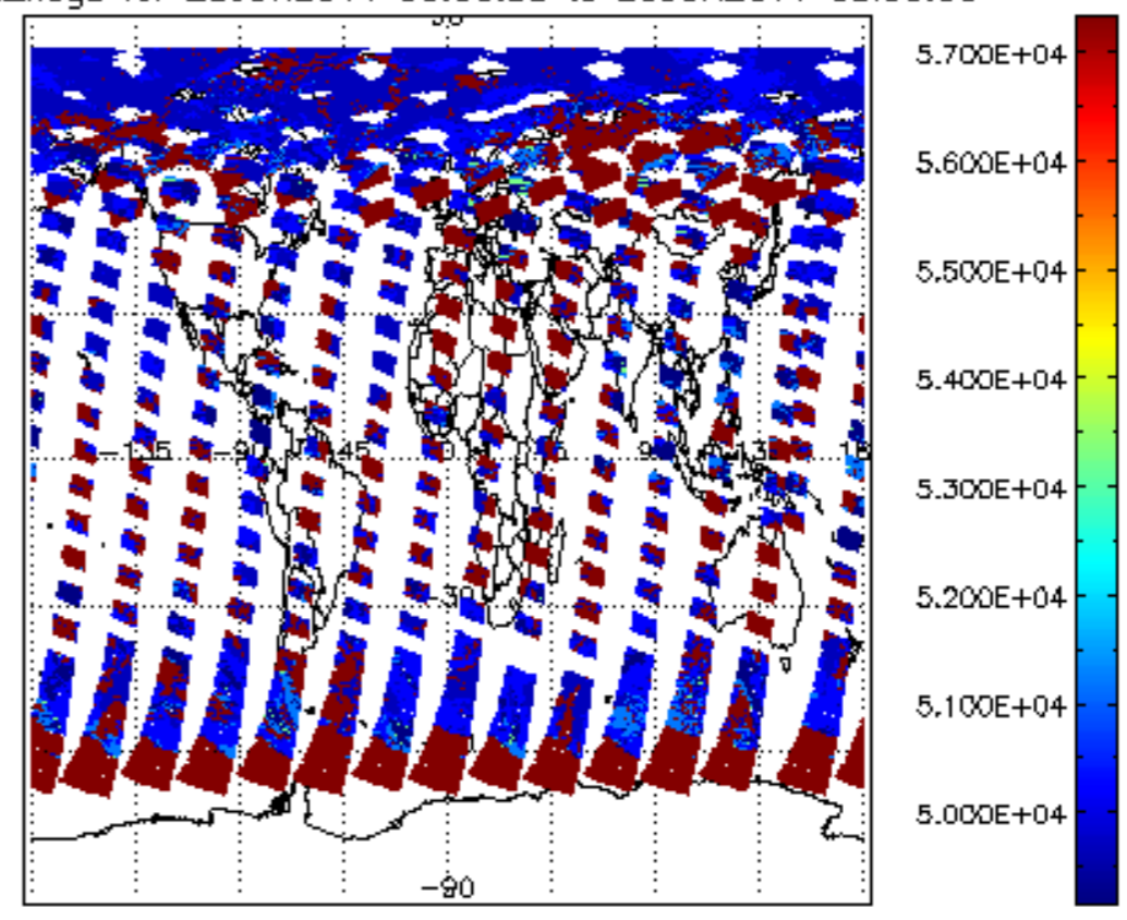
cloud_flags for 25JUN2011 00:00:00 to 26JUN2011 00:00:00
