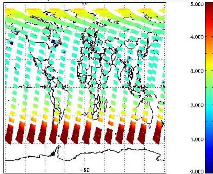
SCIOL2P_NADUV1NO2_amf_gr for 25JUN2011 00:00:00 to 26JUN2011 00:00:00
