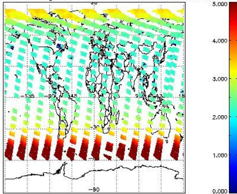
SCIOL2P_NADUV003_amf_gr for 25JUN2011 00:00:00 to 26JUN2011 00:00:00
