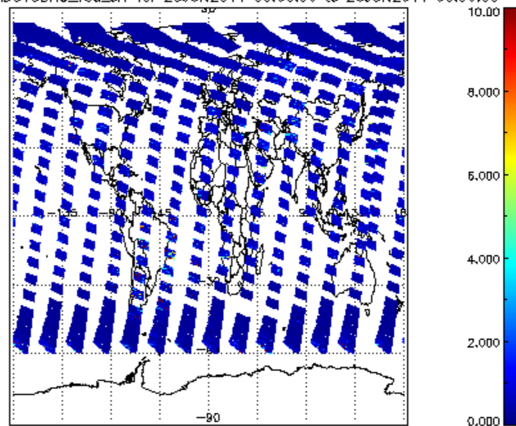
SCIOL2P_NADUV3BRO_vcd_err for 25JUN2011 00:00:00 to 26JUN2011 00:00:00
