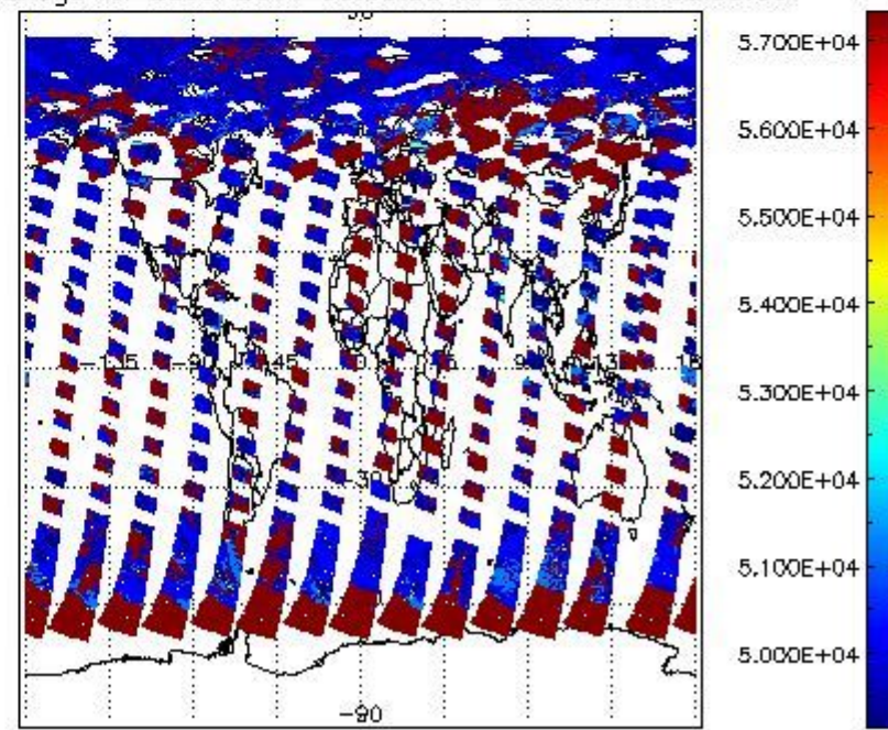
cloud_flags for 25JUN2011 00:00:00 to 26JUN2011 00:00:00
