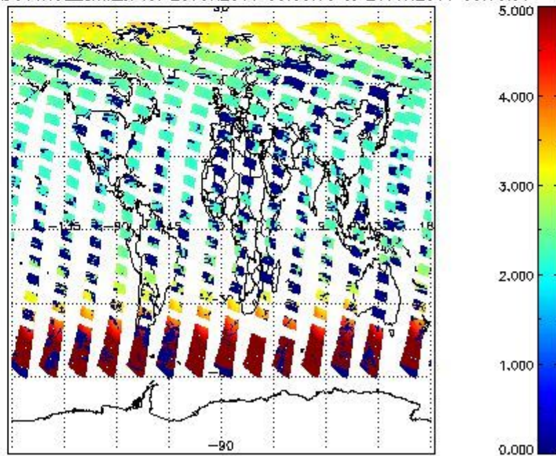
SCIOL2P_NADUV1NO2_amf_cl for 25JUN2011 00:00:00 to 26JUN2011 00:00:00
