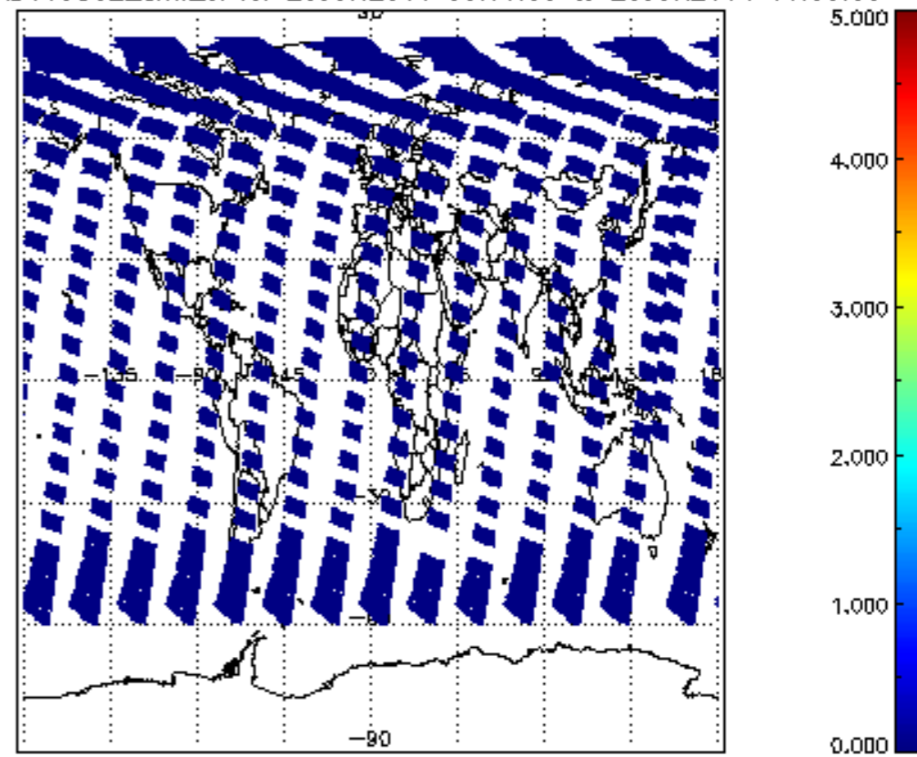
SCIOL2P_NADUV5S02_amf_cl for 25JUN2011 00:00:00 to 26JUN2011 00:00:00
