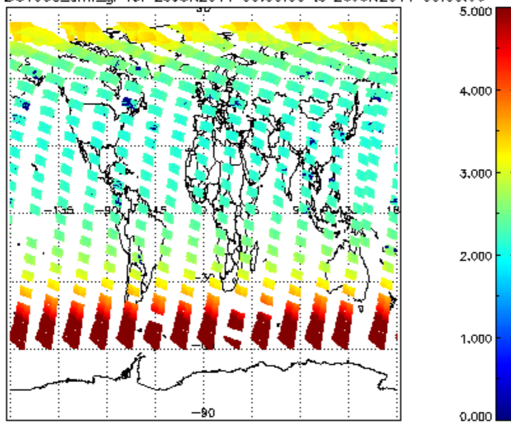
SCIOL2P_NADUV003_amf_gr for 25JUN2011 00:00:00 to 26JUN2011 00:00:00
