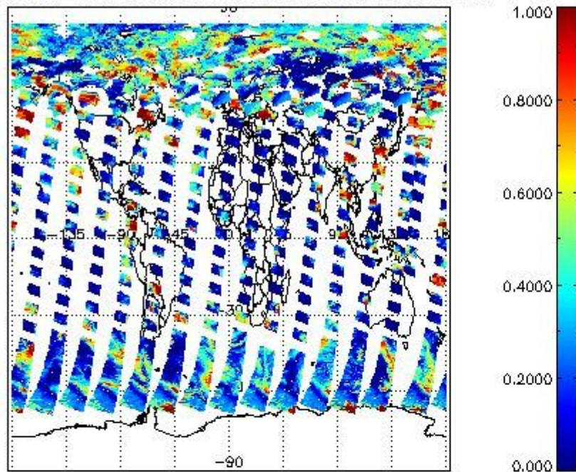
cL_frac for 25JUN2011 00:00:00 to 26JUN2011 00:00:00
