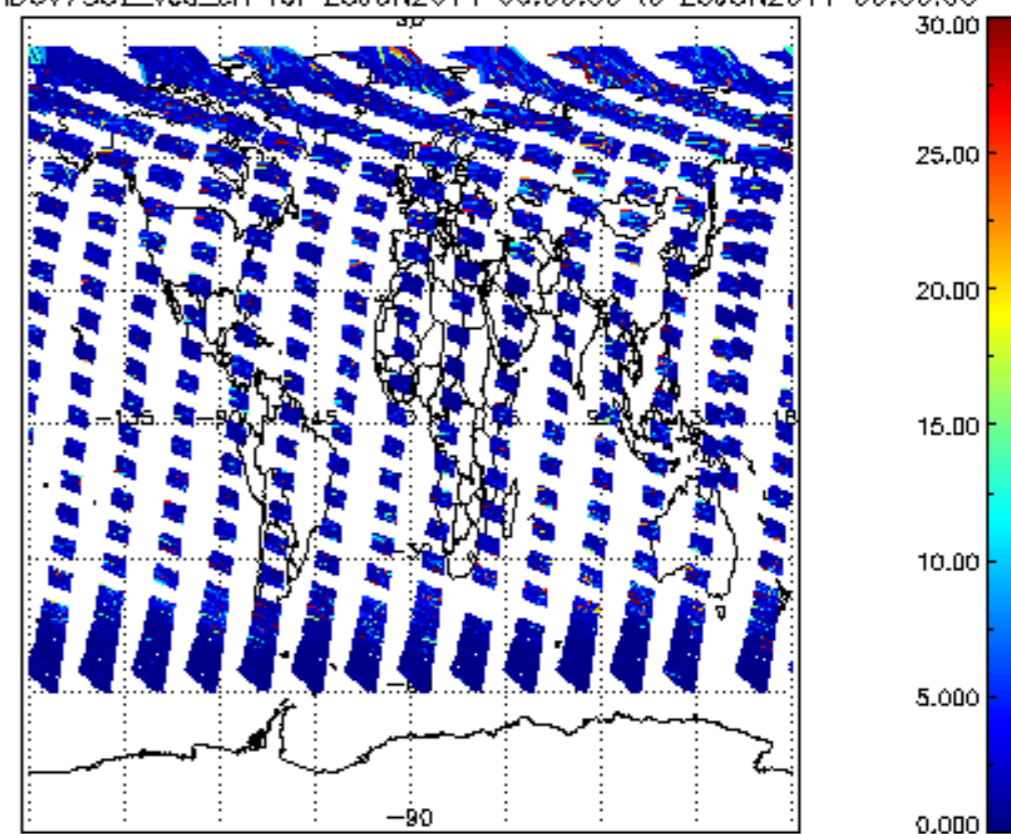
SCIOL2P_NADUV7S02_vcd_err for 25JUN2011 00:00:00 to 26JUN2011 00:00:00
