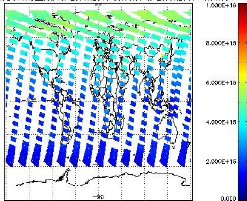
SCIOL2P_NADUV1NO2_vcd for 25JUN2011 00:00:00 to 26JUN2011 00:00:00
