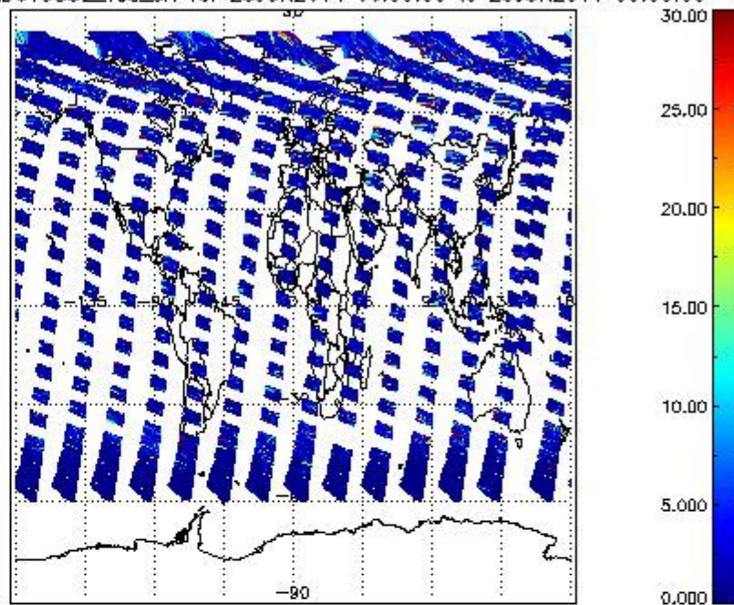
SCIOL2P_NADUV5S02_vcd_err for 25JUN2011 00:00:00 to 26JUN2011 00:00:00
