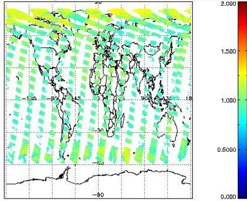
SCIOL2P_NADUV8H2O_arnf_gr for 25JUN2011 00:00:00 to 26JUN2011 00:00:00
