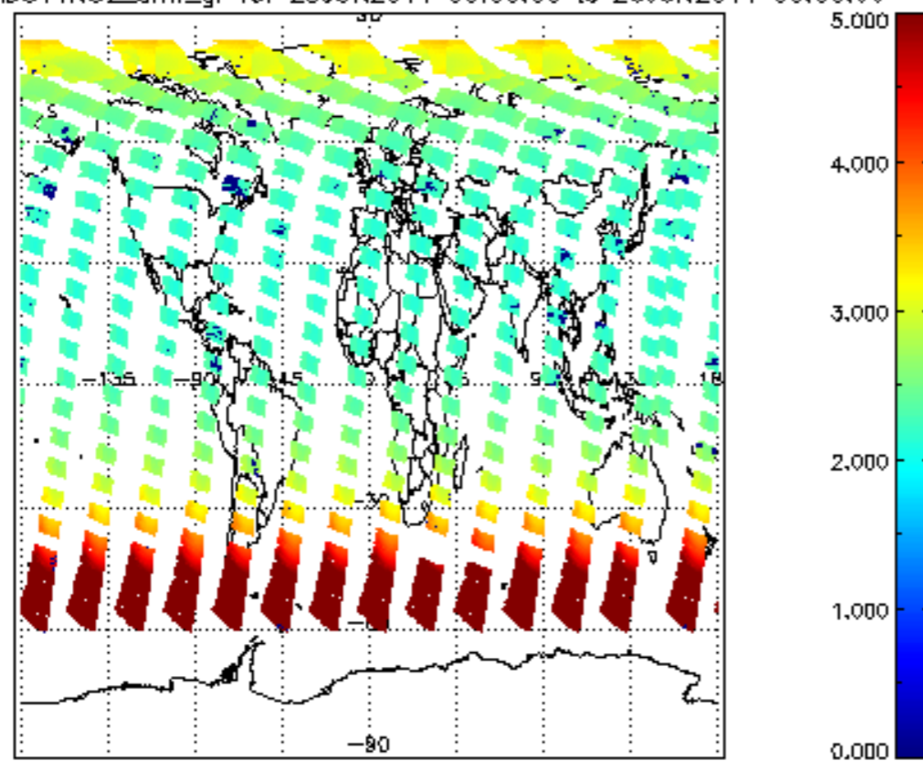
SCIOL2P_NADUV1NO2_amf_gr for 25JUN2011 00:00:00 to 26JUN2011 00:00:00
