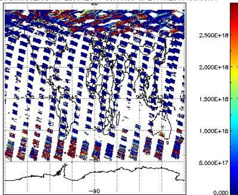
SCIOL2P_NADIR3CO_vcd for 25JUN2011 00:00:00 to 26JUN2011 00:00:00
