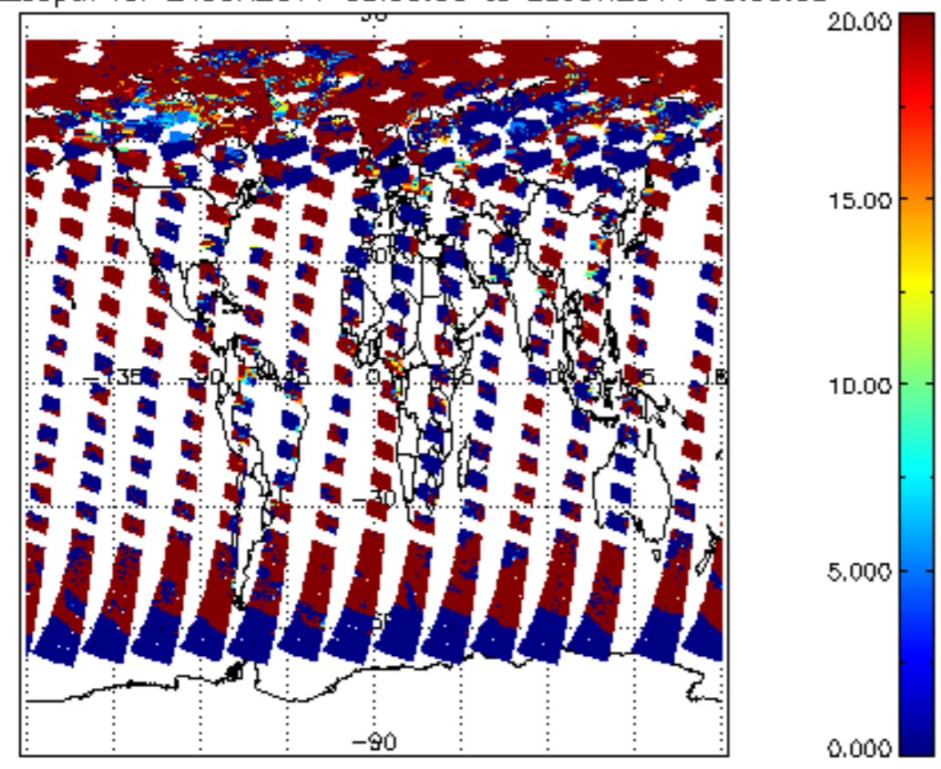
cl_opt_depth for 24JUN2011 00:00:00 to 25JUN2011 00:00:00
