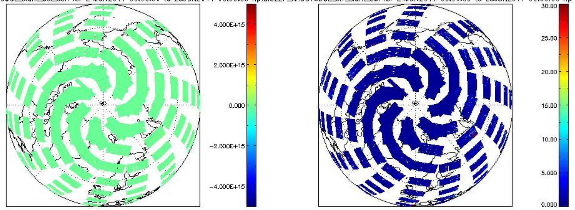
CIOL2P_NADUV60CLslant_col_den for 24JUN2011 00:00:00 to 25JUN2011 00:00:00 np; CIOL2P_NADUV60CLerr_slant_col for 24JUN2011 00:00:00 to 25JUN2011 00:00:00 np
