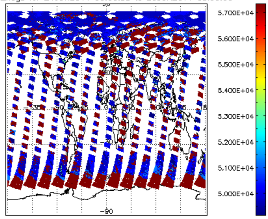
cloud_flags for 24JUN2011 00:00:00 to 25JUN2011 00:00:00
