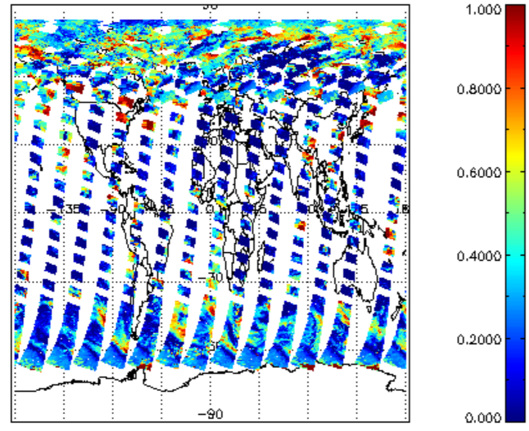
cl_frac for 24JUN2011 00:00:00 to 25JUN2011 00:00:00
