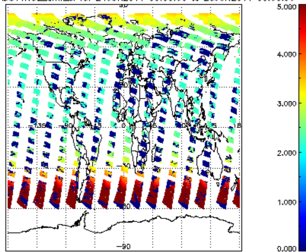
SCIOL2P_NADUV1NO2_amf_cl for 24JUN2011 00:00:00 to 25JUN2011 00:00:00
