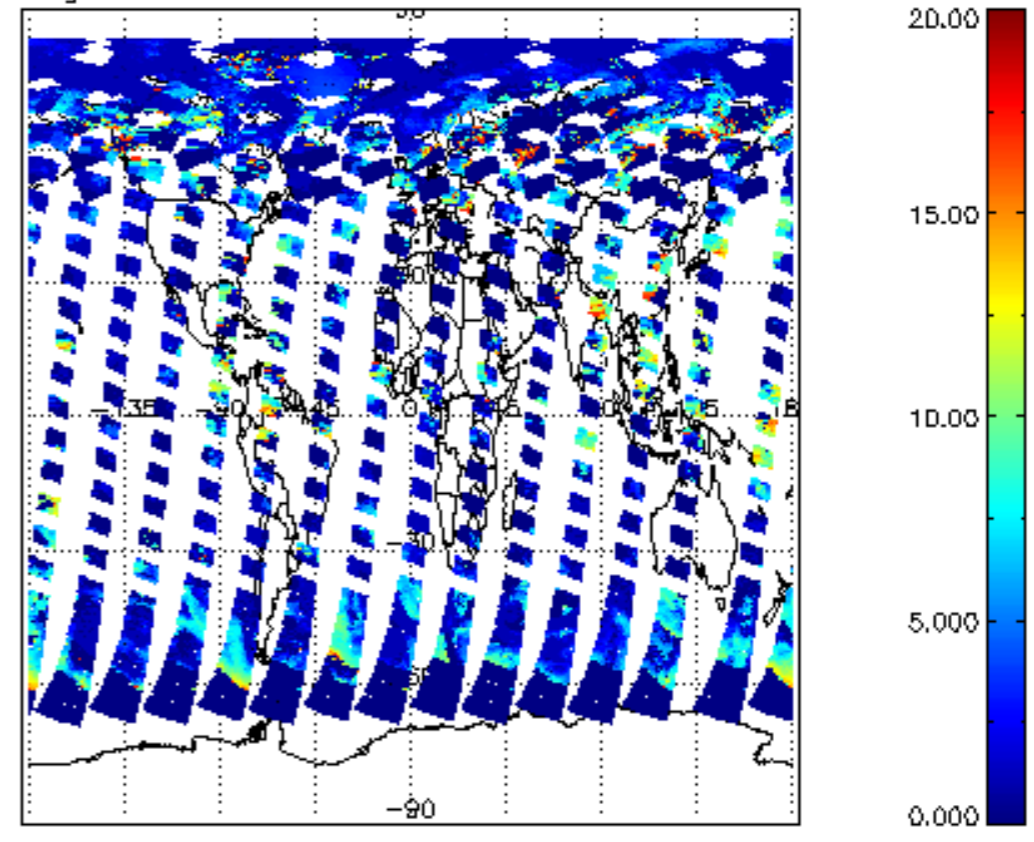
cl_top_height for 24JUN2011 00:00:00 to 25JUN2011 00:00:00
