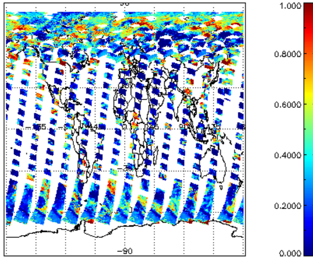
cl_frac for 22JUN2011 00:00:00 to 23JUN2011 00:00:00
