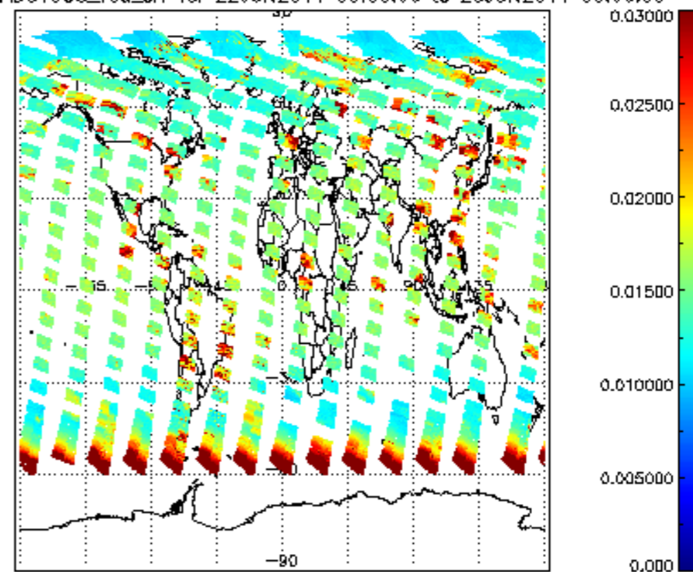
SCIOL2P_NADUV003_vcd_err for 22JUN2011 00:00:00 to 23JUN2011 00:00:00
