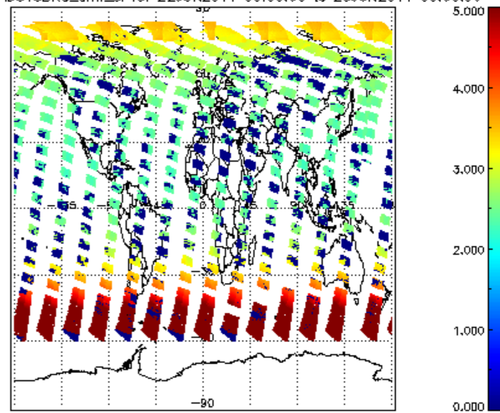
SCIOL2P_NADUV3BRO_amf_sl for 22JUN2011 00:00:00 to 23JUN2011 00:00:00
