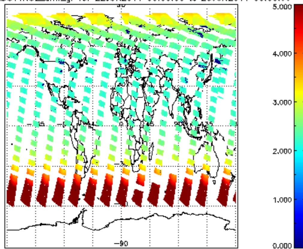
SCIOL2P_NADUV1NO2_amf_gr for 22JUN2011 00:00:00 to 23JUN2011 00:00:00
