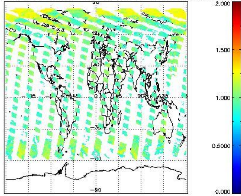
SCIOL2P_NADUV8H2O_arnf_gr for 22JUN2011 00:00:00 to 23JUN2011 00:00:00
