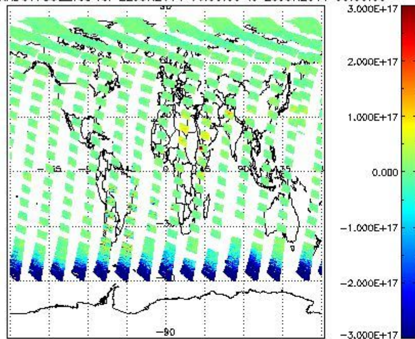
SCIOL2P_NADUV7S02_vcd for 22JUN2011 00:00:00 to 23JUN2011 00:00:00
