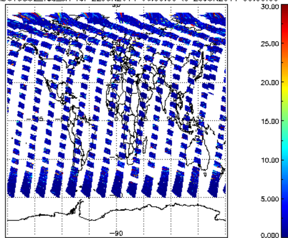
SCIOL2P_NADUV5S02_vcd_err for 22JUN2011 00:00:00 to 23JUN2011 00:00:00
