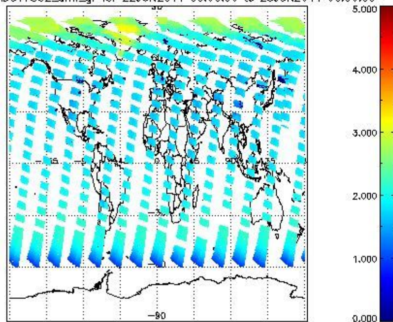
SCIOL2P_NADUV7S02_amf_gr for 22JUN2011 00:00:00 to 23JUN2011 00:00:00
