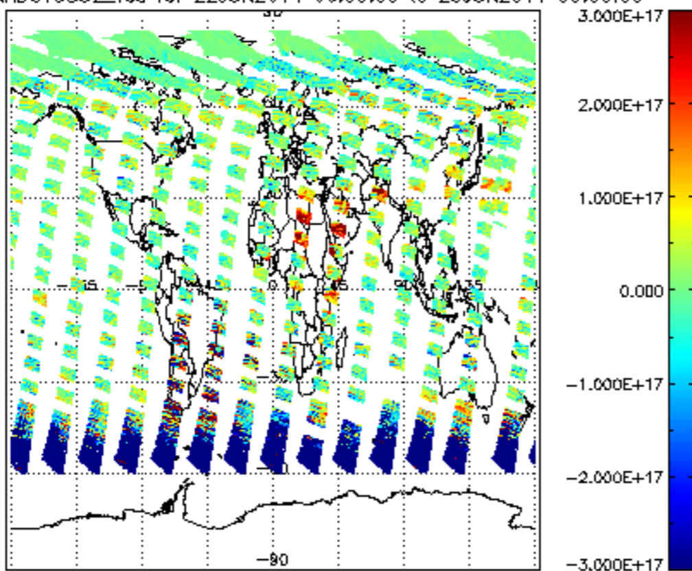
SCIOL2P_NADUV5S02_vcd for 22JUN2011 00:00:00 to 23JUN2011 00:00:00
