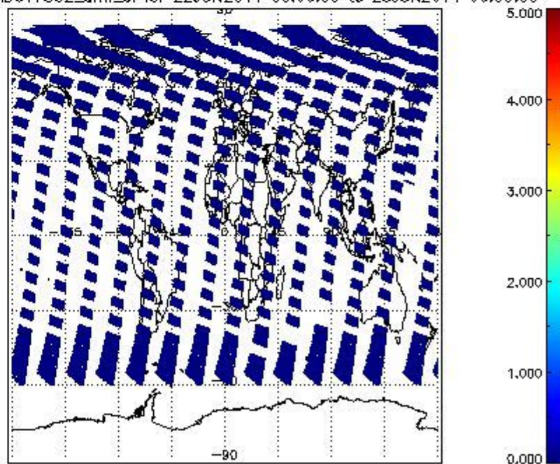
SCIOL2P_NADUV7S02_amf_cl for 22JUN2011 00:00:00 to 23JUN2011 00:00:00
