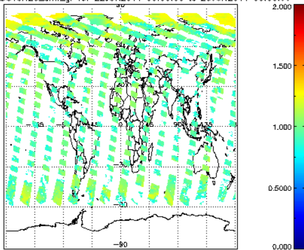
SCIOL2P_NADUV8H2O_amf_gr for 22JUN2011 00:00:00 to 23JUN2011 00:00:00
