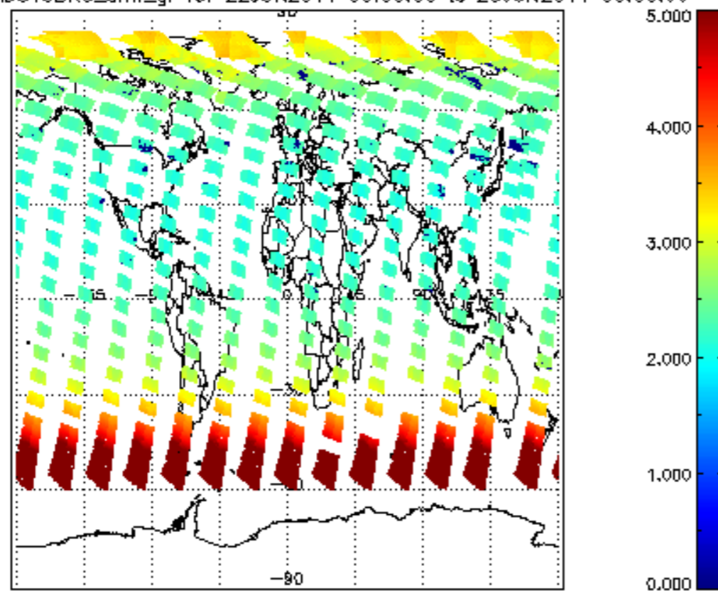
SCIOL2P_NADUV3BRO_amf_gr for 22JUN2011 00:00:00 to 23JUN2011 00:00:00
