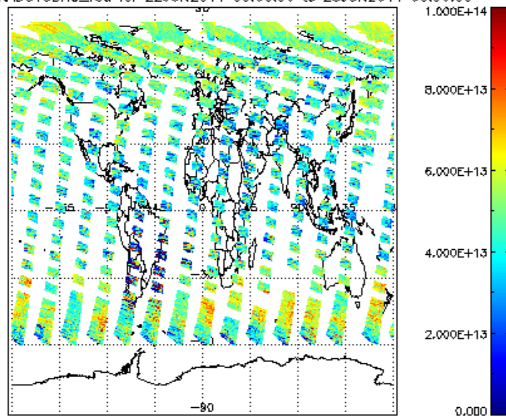
SCIOL2P_NADUV3BRO_vcd for 22JUN2011 00:00:00 to 23JUN2011 00:00:00
