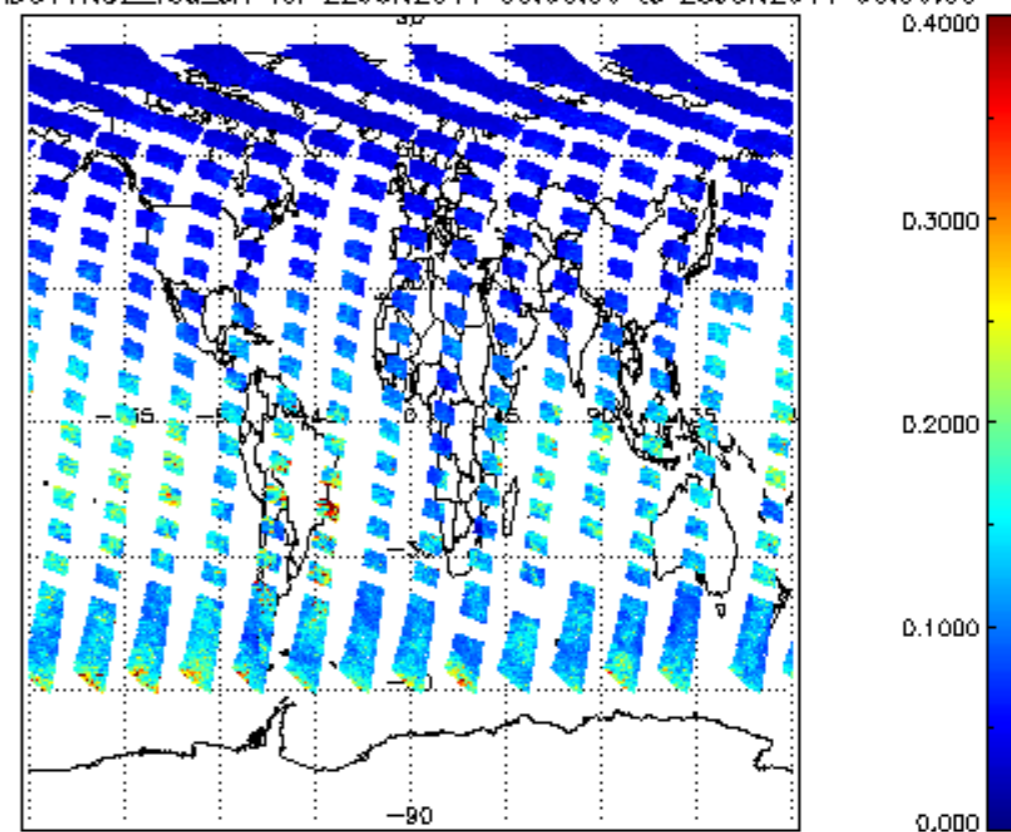
SCIOL2P_NADUV1NO2_vcd_err for 22JUN2011 00:00:00 to 23JUN2011 00:00:00
