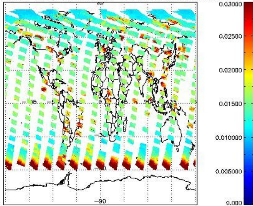
SCIOL2P_NADUV003_vcd_err for 22JUN2011 00:00:00 to 23JUN2011 00:00:00
