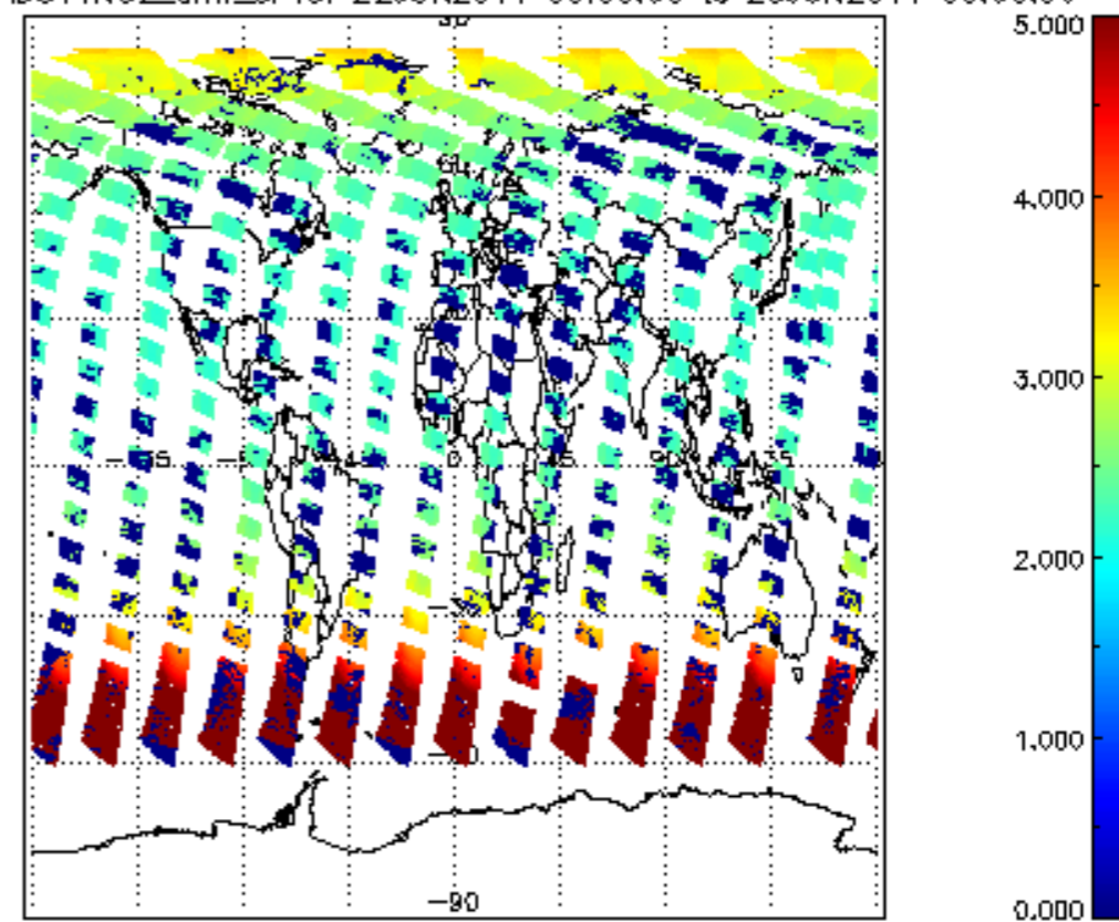
SCIOL2P_NADUV1NO2_amf_sl for 22JUN2011 00:00:00 to 23JUN2011 00:00:00
