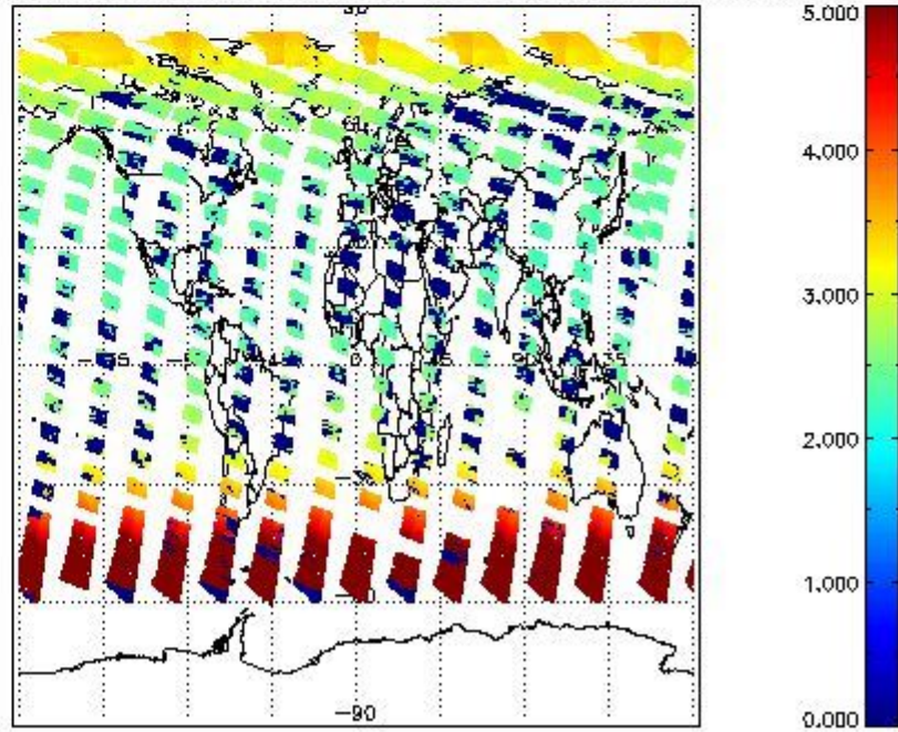
SCIOL2P_NADUV003_amf_cl for 22JUN2011 00:00:00 to 23JUN2011 00:00:00
