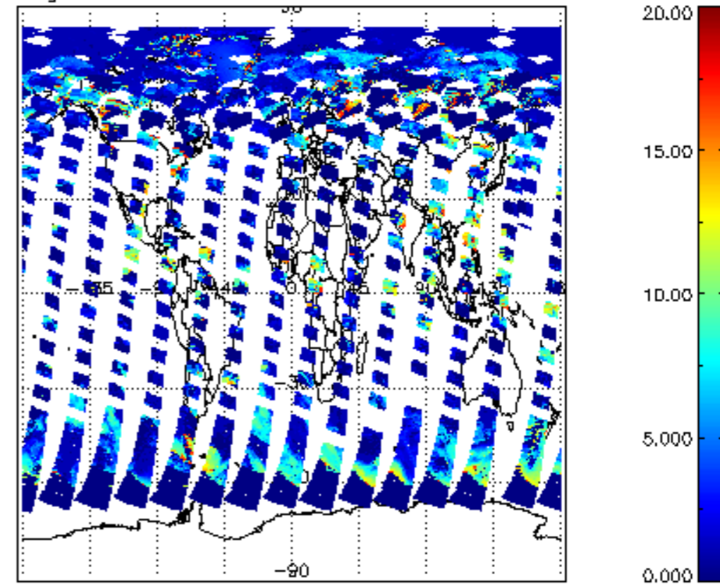
cl_top_height for 22JUN2011 00:00:00 to 23JUN2011 00:00:00
