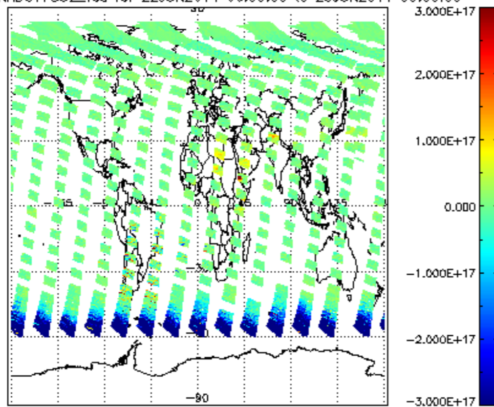
SCIOL2P_NADUV7S02_vcd for 22JUN2011 00:00:00 to 23JUN2011 00:00:00
