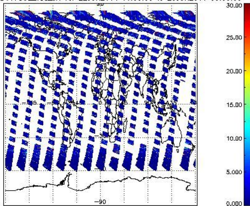
SCIOL2P_NADUV7S02_vcd_err for 22JUN2011 00:00:00 to 23JUN2011 00:00:00
