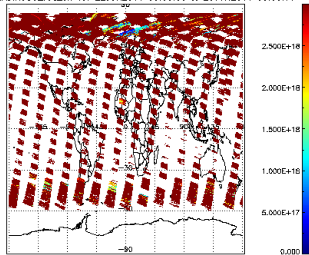
SCIOL2P_NADIR3CO_vcd_err for 22JUN2011 00:00:00 to 23JUN2011 00:00:00
