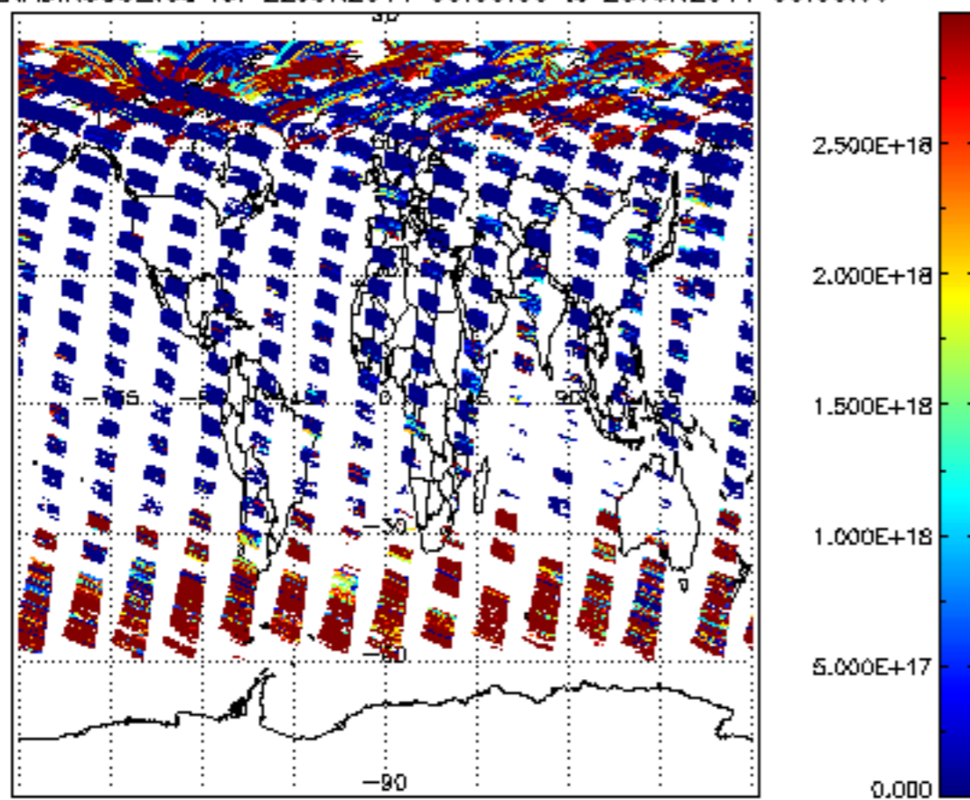
SCIOL2P_NADIR3CO_vcd for 22JUN2011 00:00:00 to 23JUN2011 00:00:00
