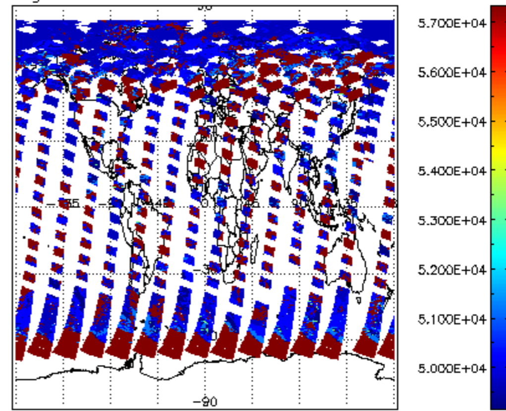
cloud_flags for 22JUN2011 00:00:00 to 23JUN2011 00:00:00
