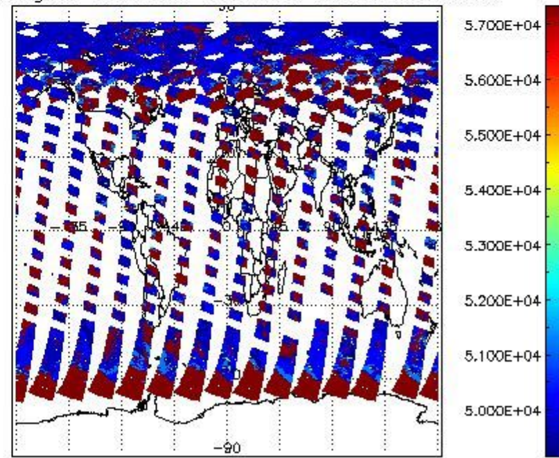
cloud_flags for 22JUN2011 00:00:00 to 23JUN2011 00:00:00
