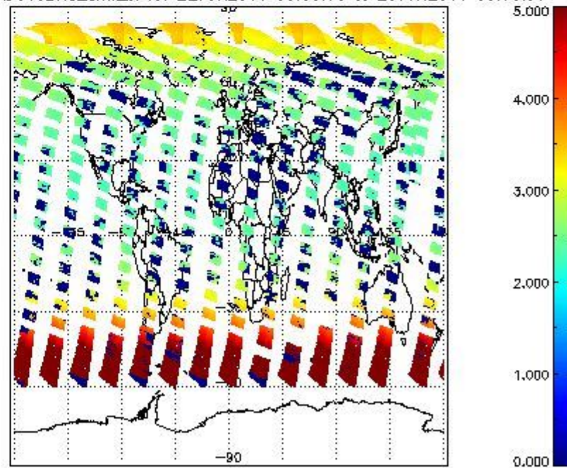
SCIOL2P_NADUV3BRO_amf_cl for 22JUN2011 00:00:00 to 23JUN2011 00:00:00
