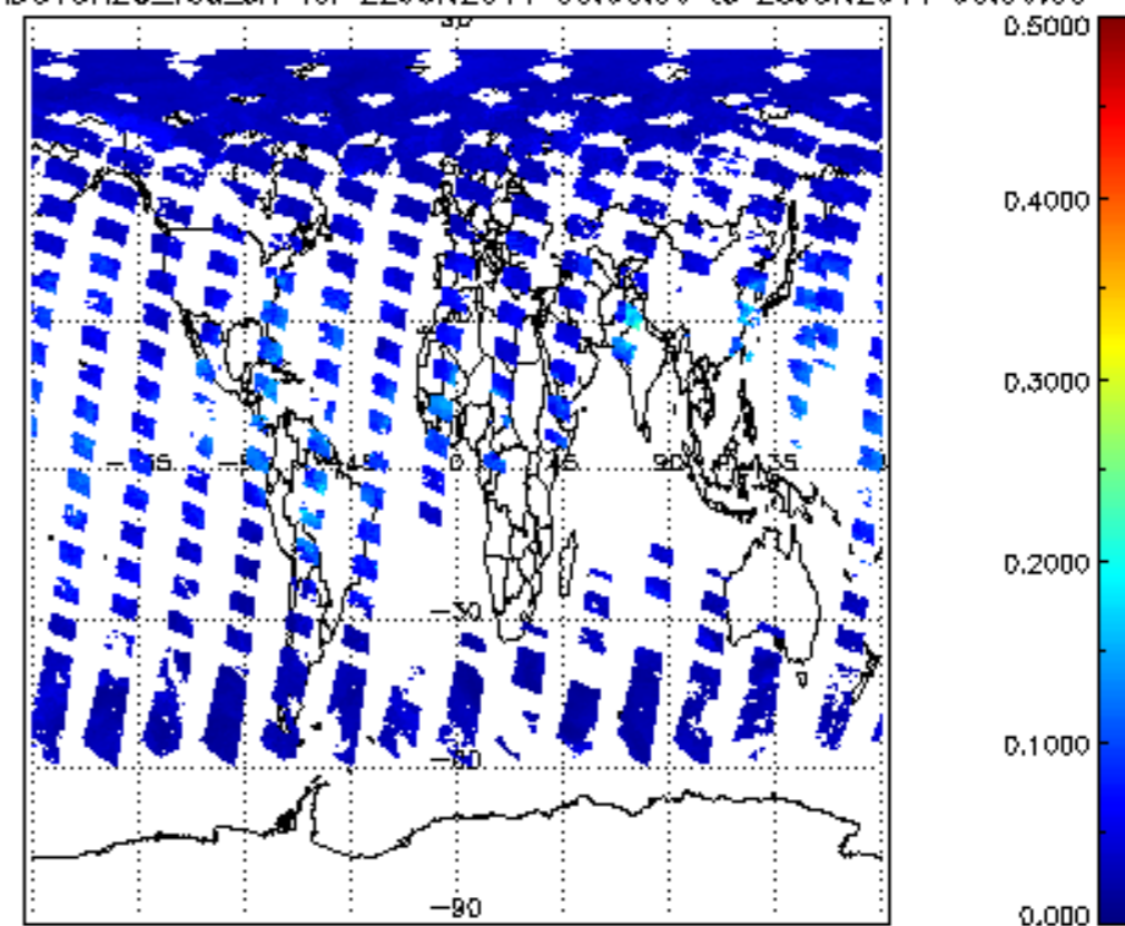
SCIOL2P_NADUV8H2O_vcd_err for 22JUN2011 00:00:00 to 23JUN2011 00:00:00
