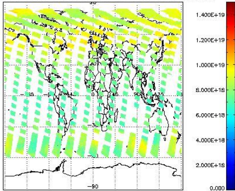
SCIOL2P_NADUV003_vcd for 22JUN2011 00:00:00 to 23JUN2011 00:00:00
