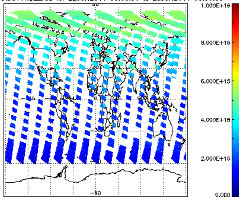
SCIOL2P_NADUV1NO2_vcd for 22JUN2011 00:00:00 to 23JUN2011 00:00:00
