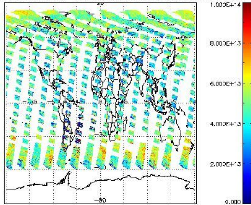
SCIOL2P_NADUV3BRO_vcd for 22JUN2011 00:00:00 to 23JUN2011 00:00:00
