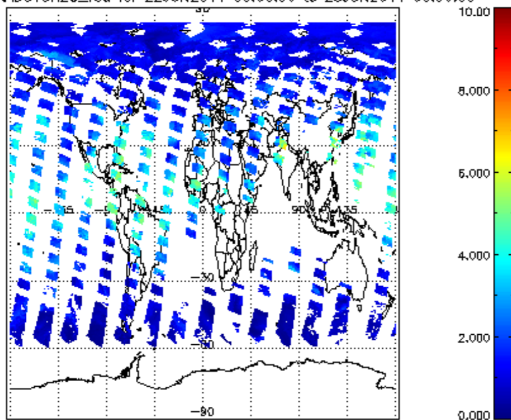
SCIOL2P_NADUV8H2O_vcd for 22JUN2011 00:00:00 to 23JUN2011 00:00:00
