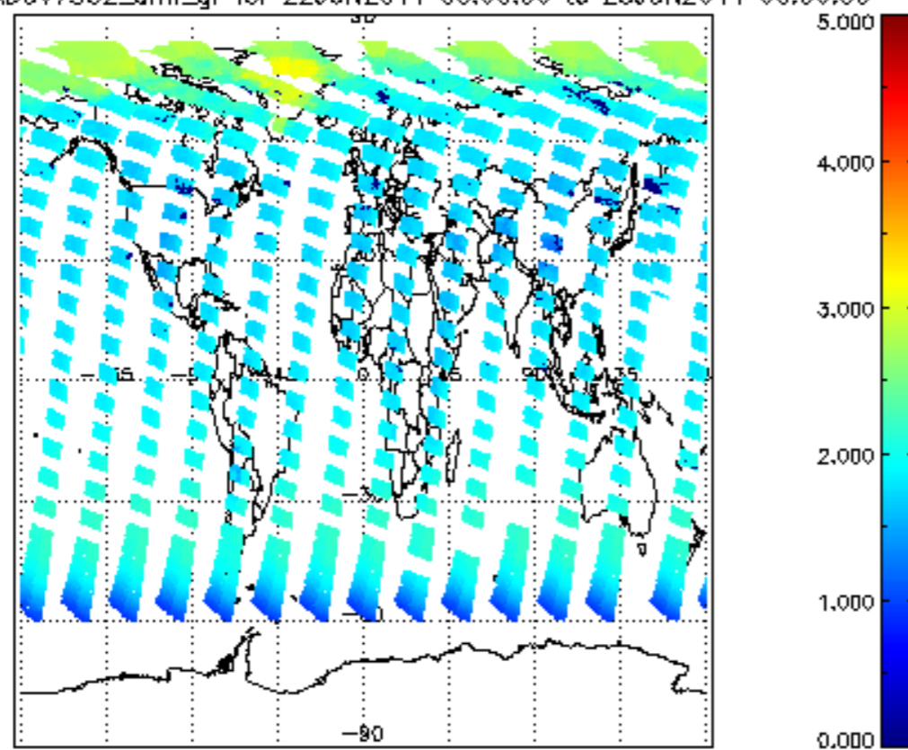
SCIOL2P_NADUV7S02_amf_gr for 22JUN2011 00:00:00 to 23JUN2011 00:00:00
