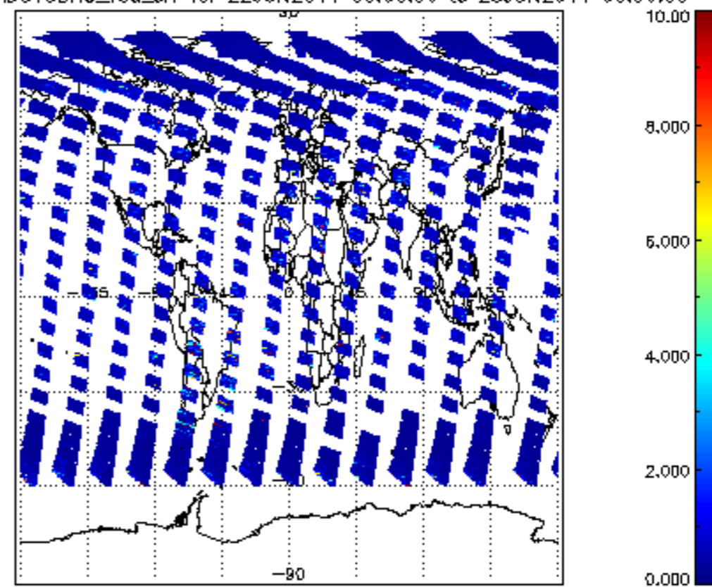
SCIOL2P_NADUV3BRO_vcd_err for 22JUN2011 00:00:00 to 23JUN2011 00:00:00
