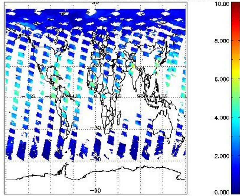
SCIOL2P_NADUV8H2O_vcd for 22JUN2011 00:00:00 to 23JUN2011 00:00:00
