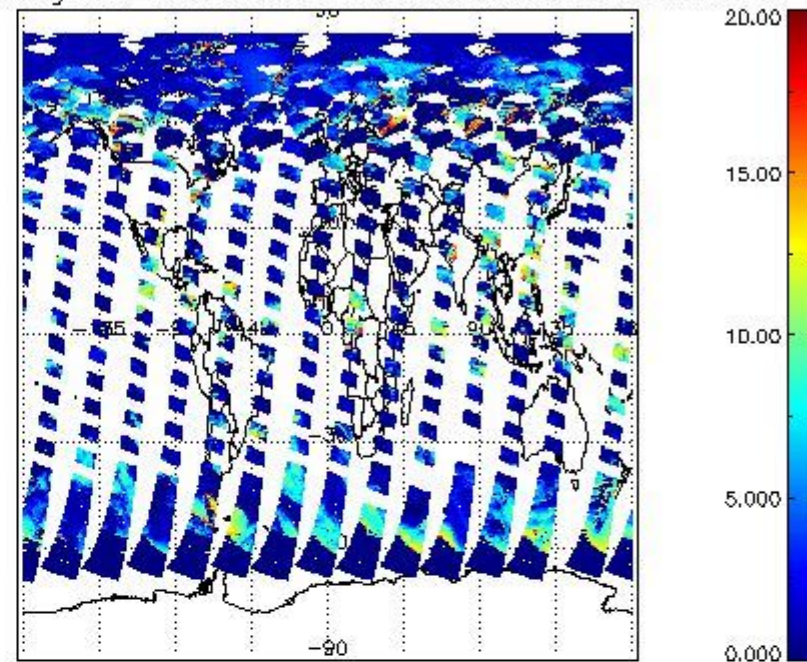
cL_top_height for 22JUN2011 00:00:00 to 23JUN2011 00:00:00
