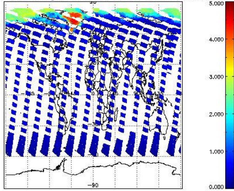
SCIOL2P_NADUV5S02_amf_gr for 22JUN2011 00:00:00 to 23JUN2011 00:00:00
