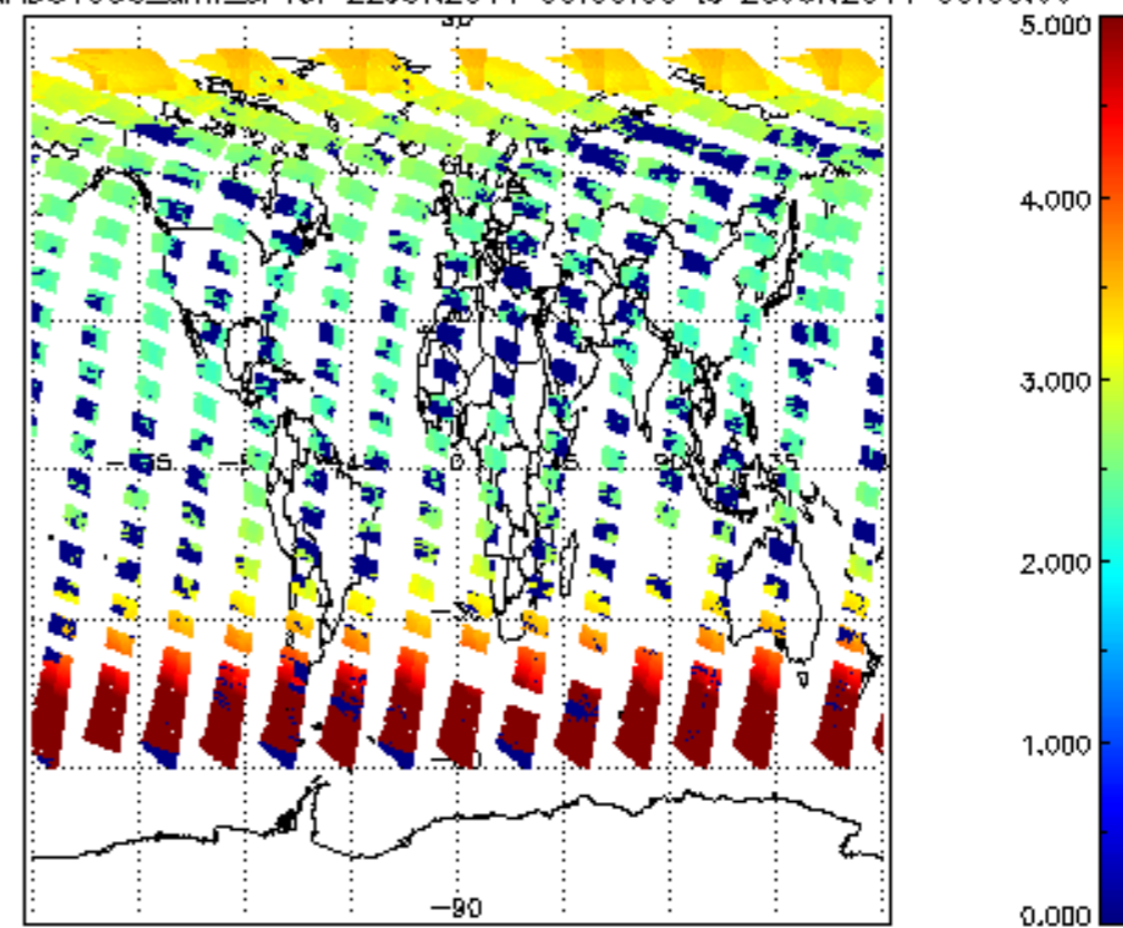
SCIOL2P_NADUV003_amf_cl for 22JUN2011 00:00:00 to 23JUN2011 00:00:00
