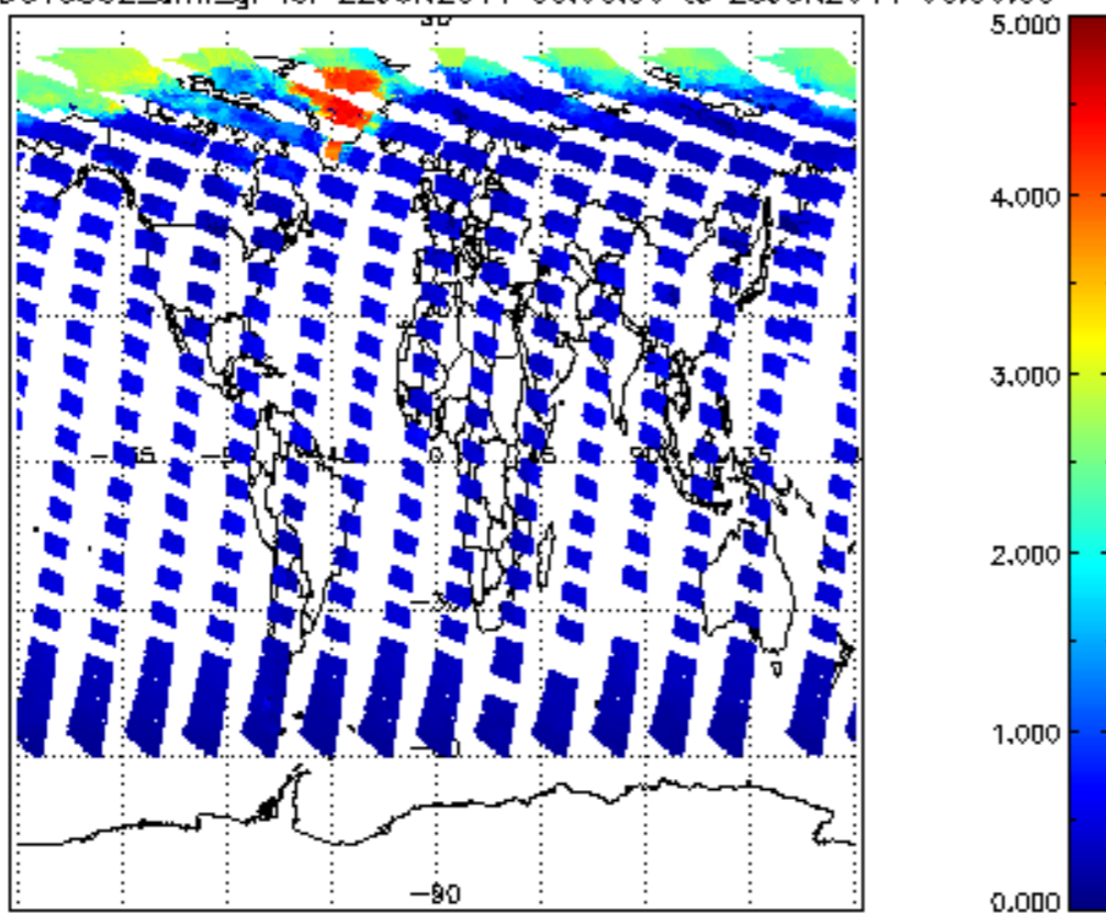
SCIOL2P_NADUV5S02_amf_gr for 22JUN2011 00:00:00 to 23JUN2011 00:00:00
