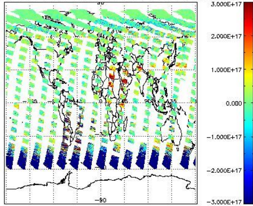
SCIOL2P_NADUV5S02_vcd for 22JUN2011 00:00:00 to 23JUN2011 00:00:00
