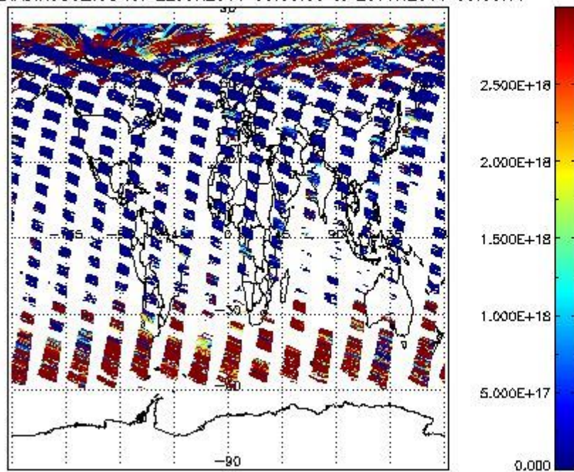
SCIDL2P_NADIR3CO_vcd for 22JUN2011 00:00:00 to 23JUN2011 00:00:00
