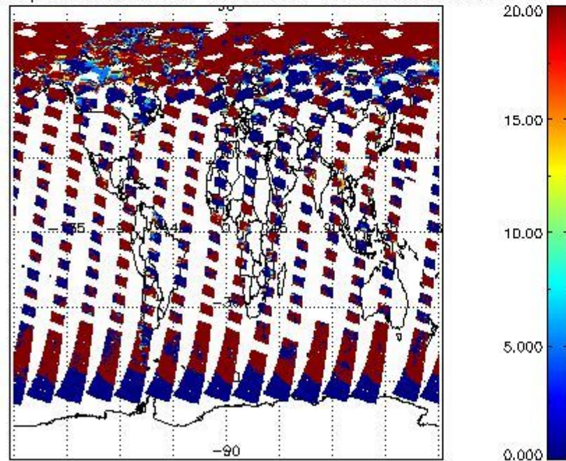
cL_opt_depth for 22JUN2011 00:00:00 to 23JUN2011 00:00:00
