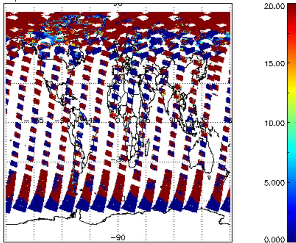
cl_opt_depth for 22JUN2011 00:00:00 to 23JUN2011 00:00:00
