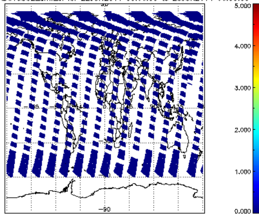
SCIOL2P_NADUV5S02_amf_cl for 22JUN2011 00:00:00 to 23JUN2011 00:00:00
