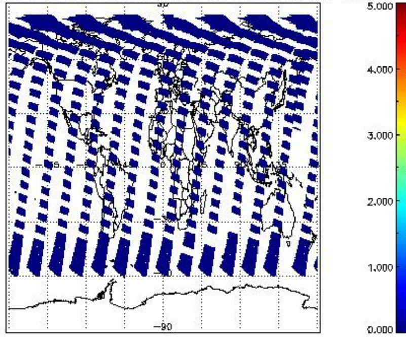
SCIOL2P_NADUV5S02_amf_cl for 22JUN2011 00:00:00 to 23JUN2011 00:00:00
