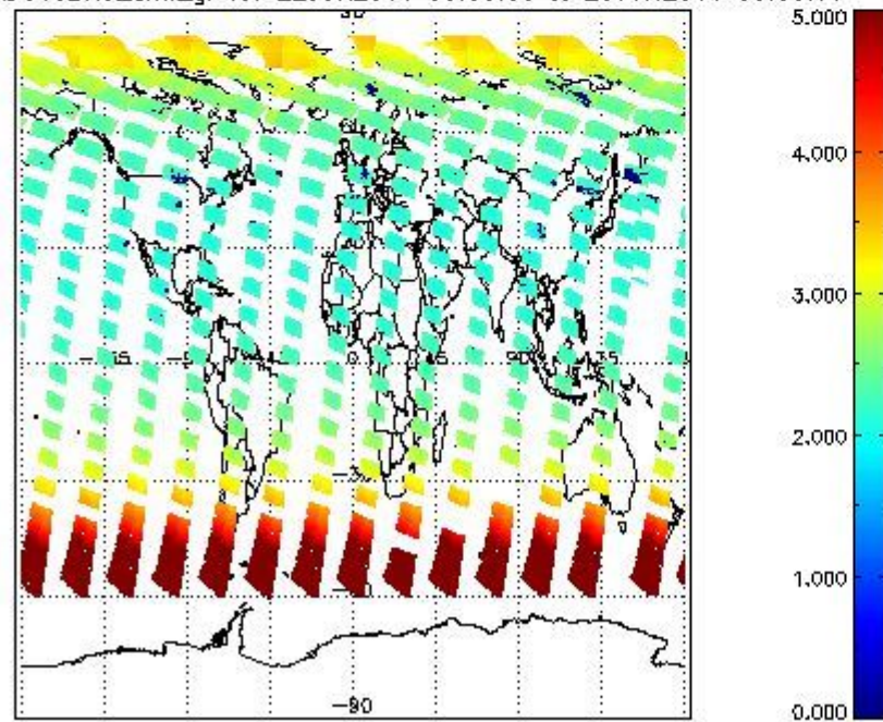
SCIOL2P_NADUV3BRO_amf_gr for 22JUN2011 00:00:00 to 23JUN2011 00:00:00
