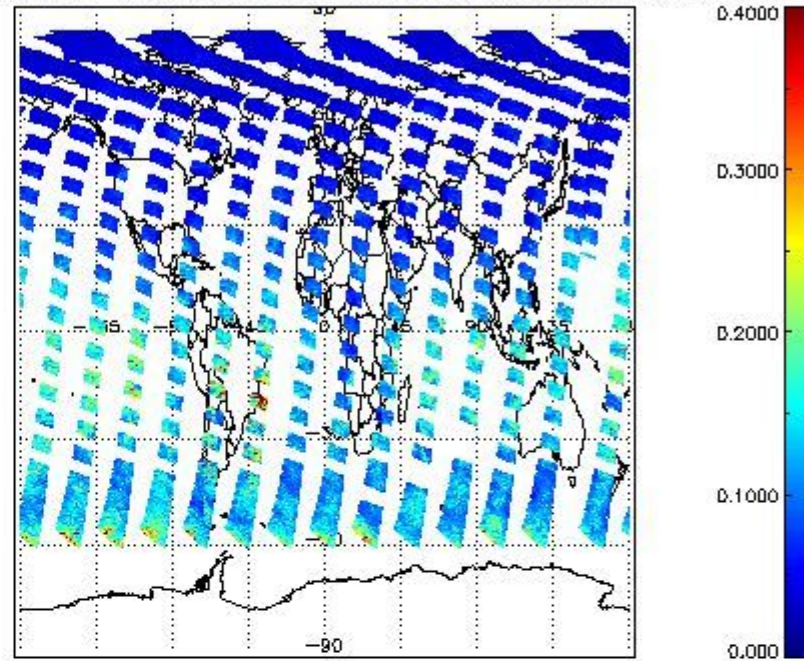
SCIOL2P_NADUV1NO2_vcd_err for 22JUN2011 00:00:00 to 23JUN2011 00:00:00
