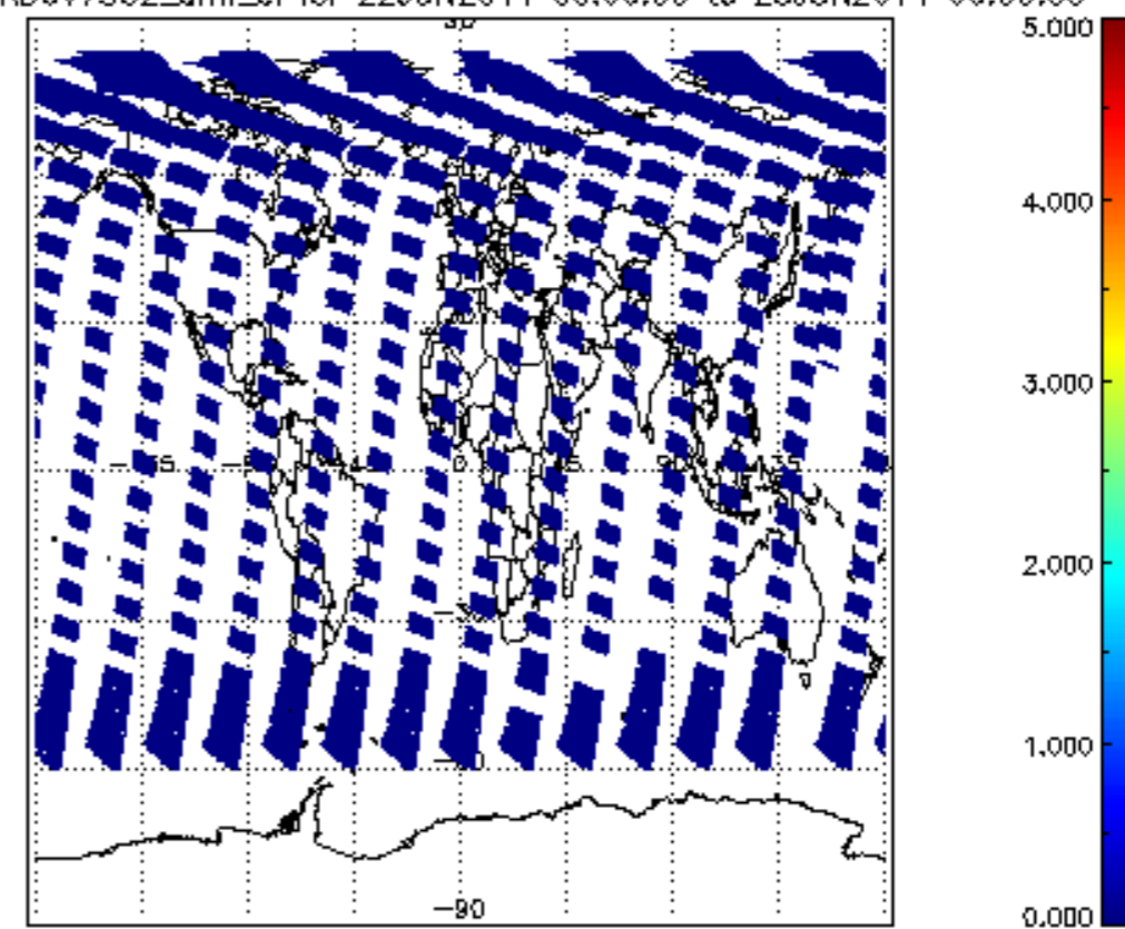
SCIOL2P_NADUV7S02_amf_cl for 22JUN2011 00:00:00 to 23JUN2011 00:00:00
