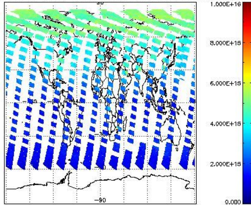
SCIOL2P_NADUV1NO2_vcd for 22JUN2011 00:00:00 to 23JUN2011 00:00:00
