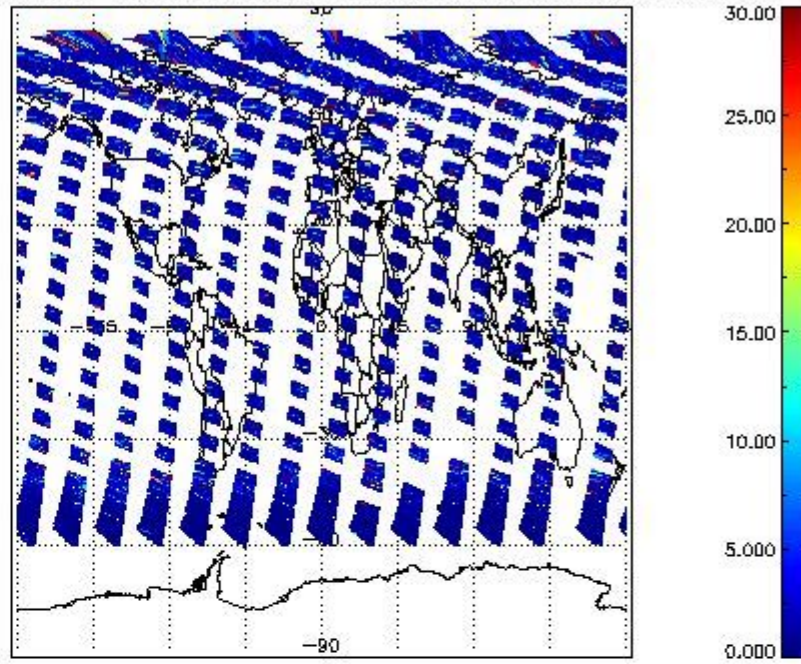
SCIOL2P_NADUV5S02_vcd_err for 22JUN2011 00:00:00 to 23JUN2011 00:00:00
