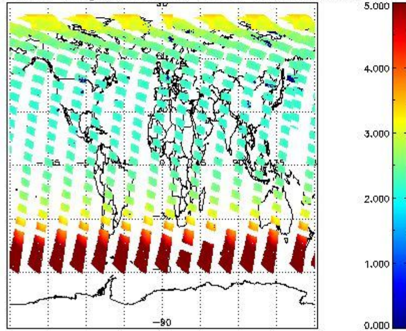
SCIOL2P_NADUV1NO2_amf_gr for 22JUN2011 00:00:00 to 23JUN2011 00:00:00
