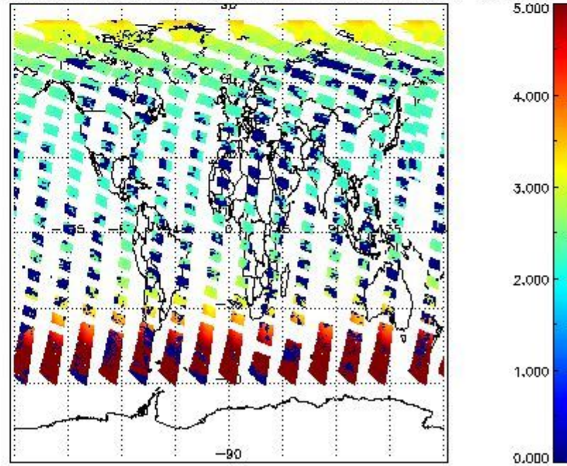
SCIOL2P_NADUV1NO2_amf_cl for 22JUN2011 00:00:00 to 23JUN2011 00:00:00
