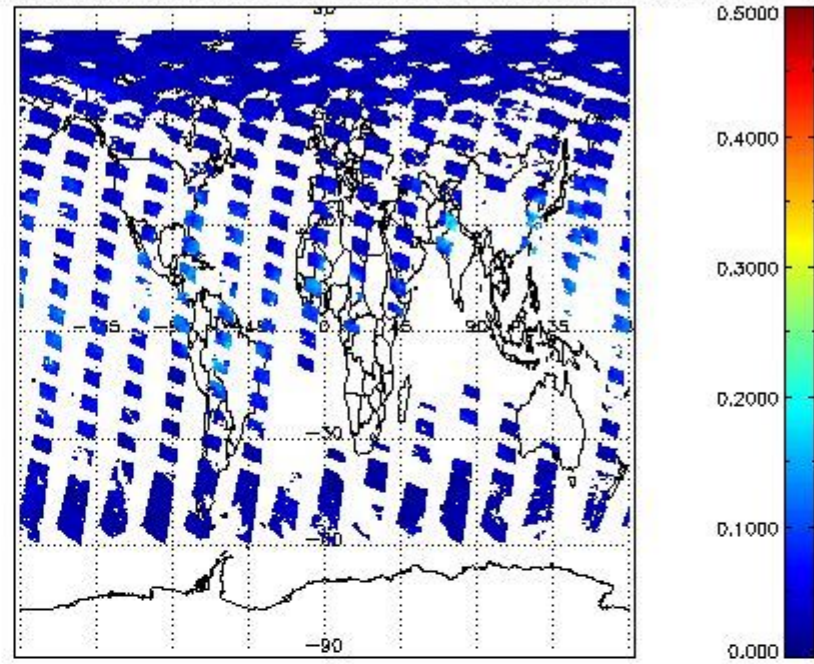
SCIOL2P_NADUV8H2O_vcd_err for 22JUN2011 00:00:00 to 23JUN2011 00:00:00
