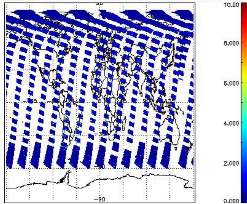
SCIOL2P_NADUV3BRO_vcd_err for 22JUN2011 00:00:00 to 23JUN2011 00:00:00
