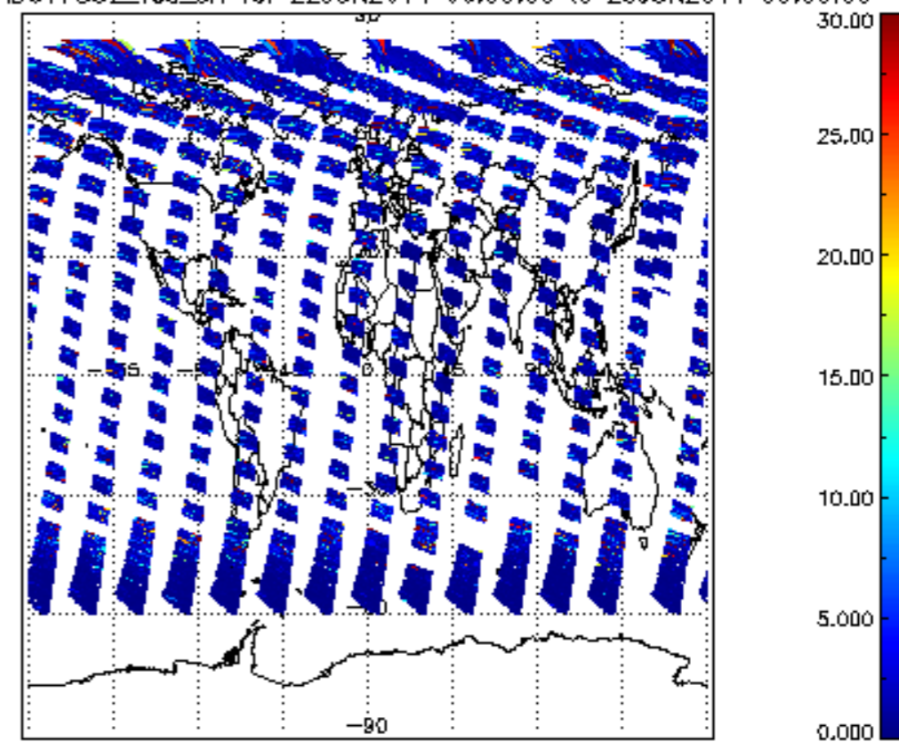
SCIOL2P_NADUV7S02_vcd_err for 22JUN2011 00:00:00 to 23JUN2011 00:00:00
