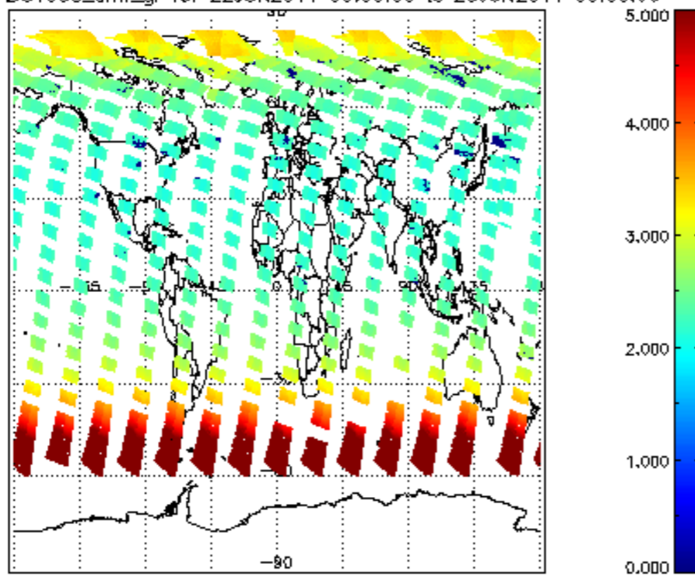
SCIOL2P_NADUV003_amf_gr for 22JUN2011 00:00:00 to 23JUN2011 00:00:00
