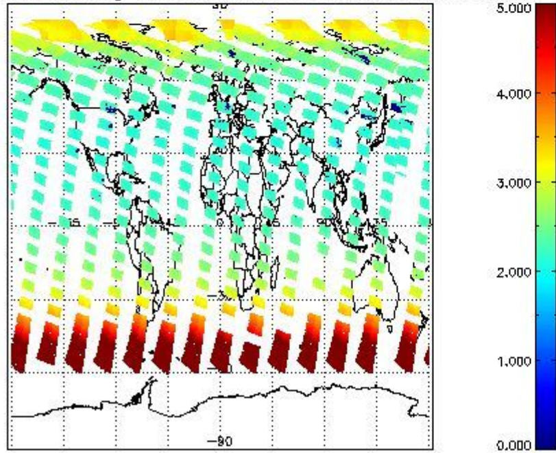
SCIOL2P_NADUV003_amf_gr for 22JUN2011 00:00:00 to 23JUN2011 00:00:00
