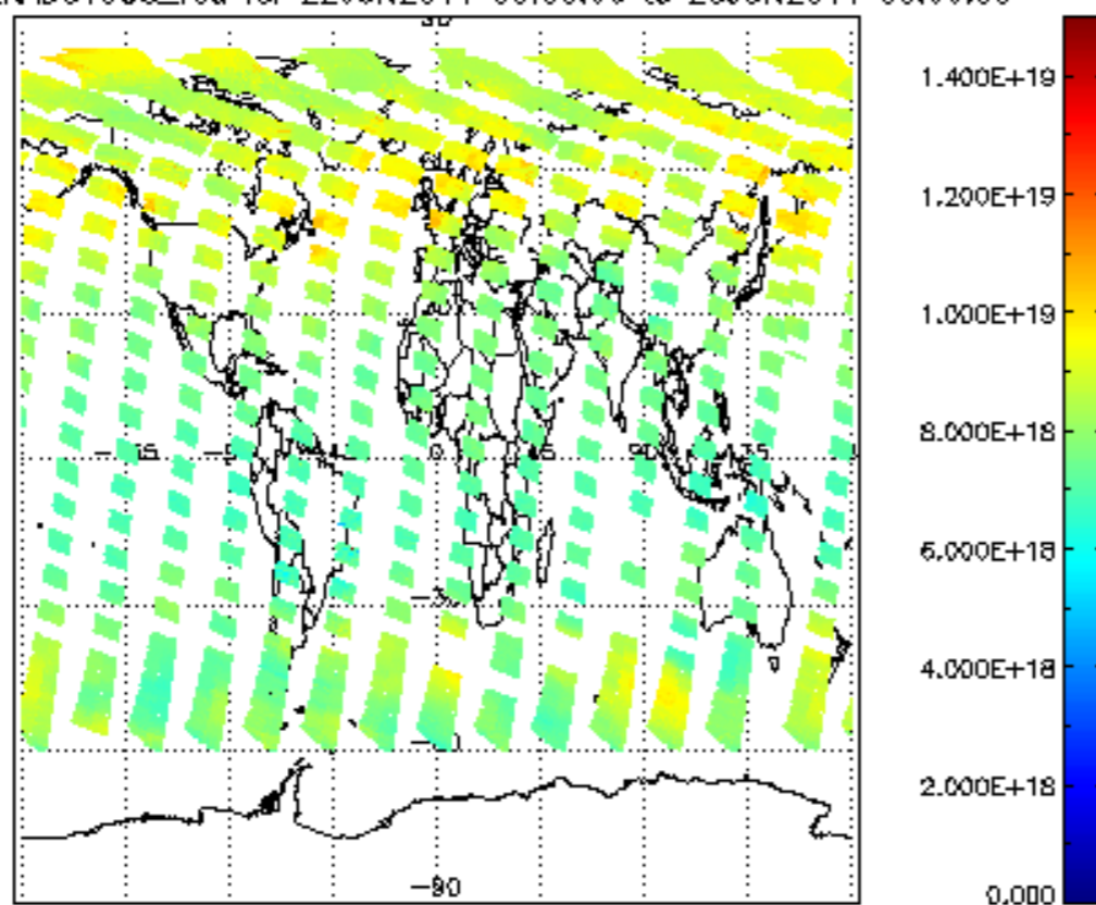
SCIOL2P_NADUV003_vcd for 22JUN2011 00:00:00 to 23JUN2011 00:00:00
