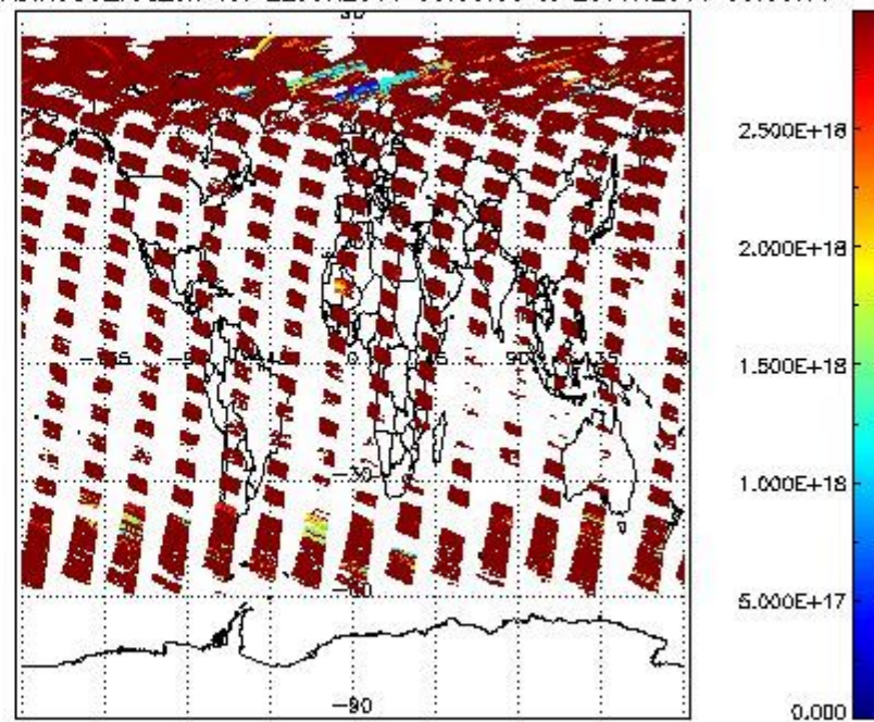
SCIDL2P_NADIR3CO_vcd_err for 22JUN2011 00:00:00 to 23JUN2011 00:00:00
