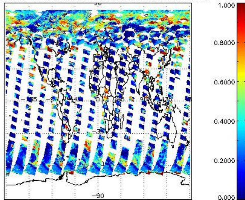
cL_frac for 22JUN2011 00:00:00 to 23JUN2011 00:00:00
