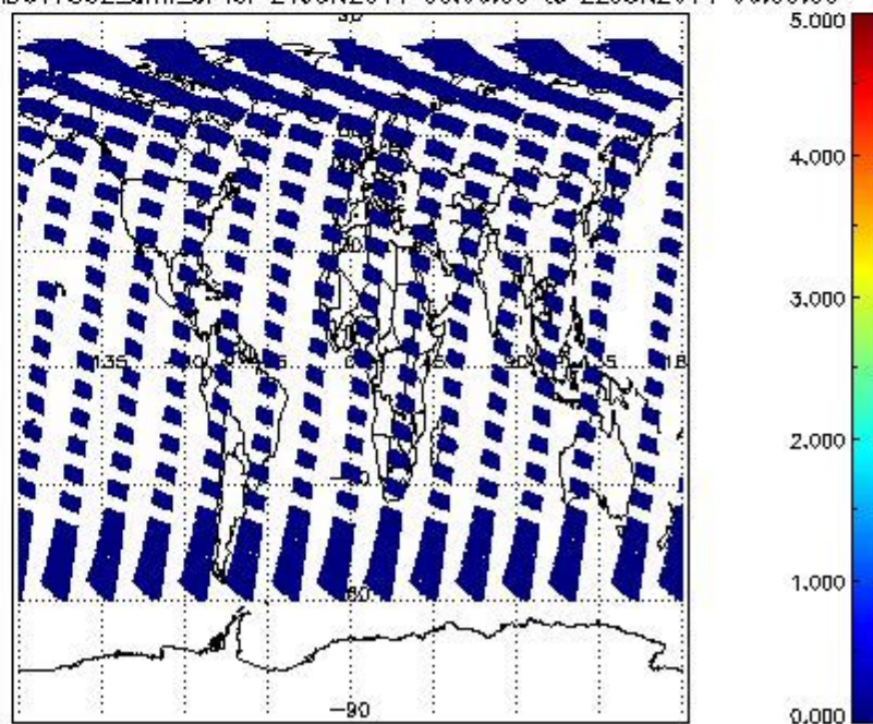
SCIOL2P_NADUV7S02_amf_cl for 21JUN2011 00:00:00 to 22JUN2011 00:00:00
