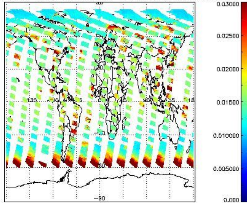
SCIOL2P_NADUV003_vcd_err for 21JUN2011 00:00:00 to 22JUN2011 00:00:00
