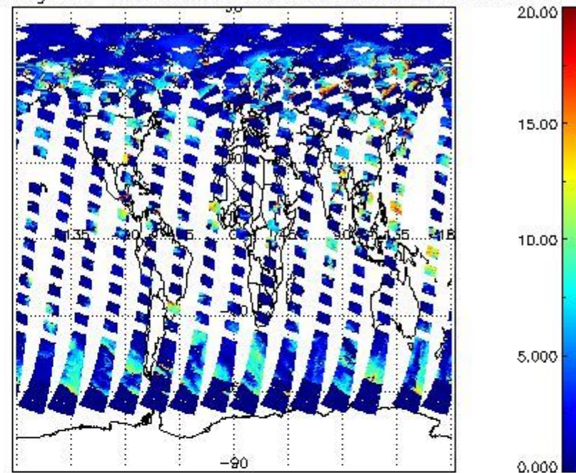
cL_top_height for 21JUN2011 00:00:00 to 22JUN2011 00:00:00
