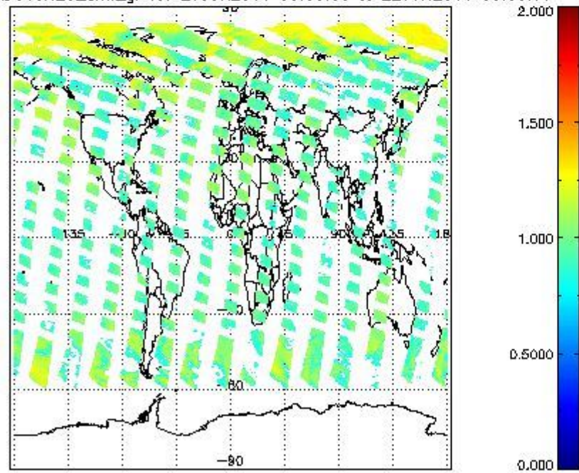
SCIOL2P_NADUV8H2O_amf_gr for 21JUN2011 00:00:00 to 22JUN2011 00:00:00
