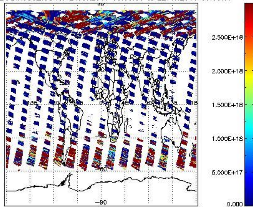
SCIOL2P_NADIR3CO_vcd for 21JUN2011 00:00:00 to 22JUN2011 00:00:00
