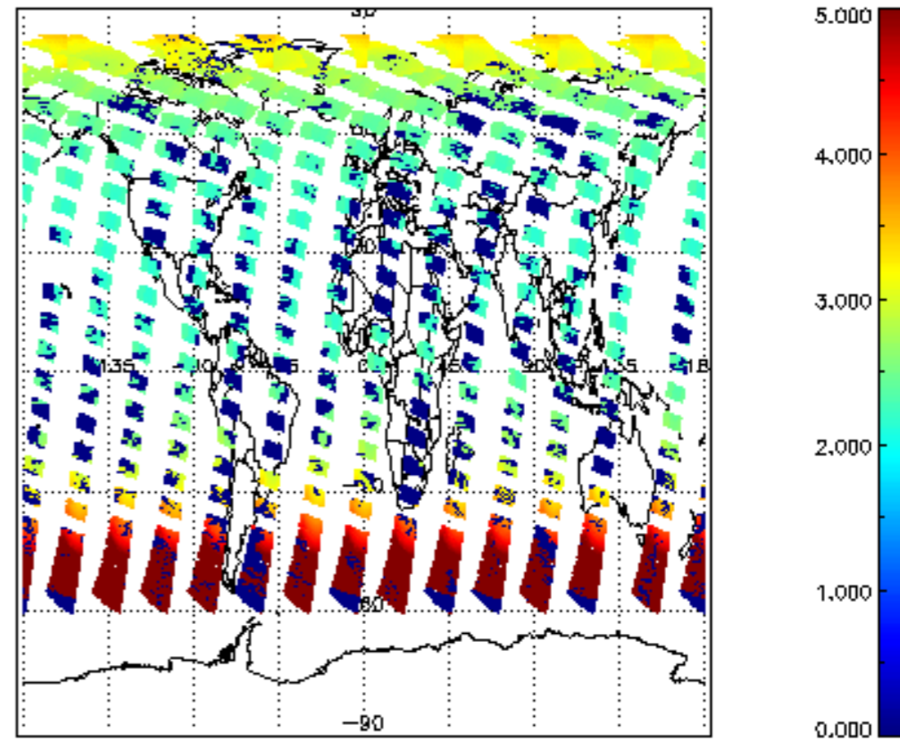
SCIOL2P_NADUV1NO2_amf_sl for 21JUN2011 00:00:00 to 22JUN2011 00:00:00
