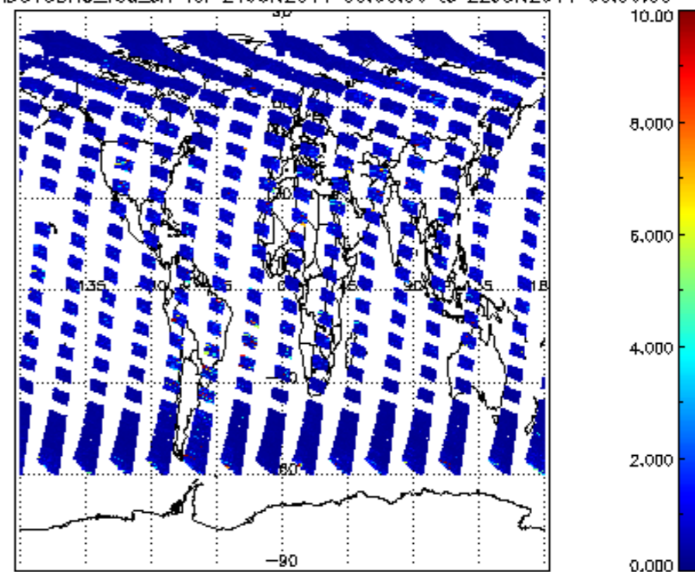
SCIOL2P_NADUV3BRO_vcd_err for 21JUN2011 00:00:00 to 22JUN2011 00:00:00
