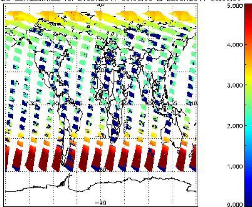
SCIOL2P_NADUV3BRO_amf_cl for 21JUN2011 00:00:00 to 22JUN2011 00:00:00
