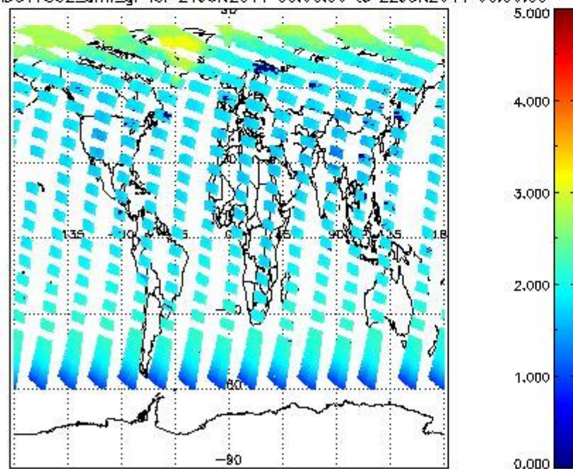
SCIOL2P_NADUV7S02_amf_gr for 21JUN2011 00:00:00 to 22JUN2011 00:00:00
