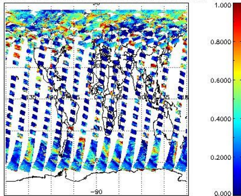
cL_frac for 21JUN2011 00:00:00 to 22JUN2011 00:00:00
