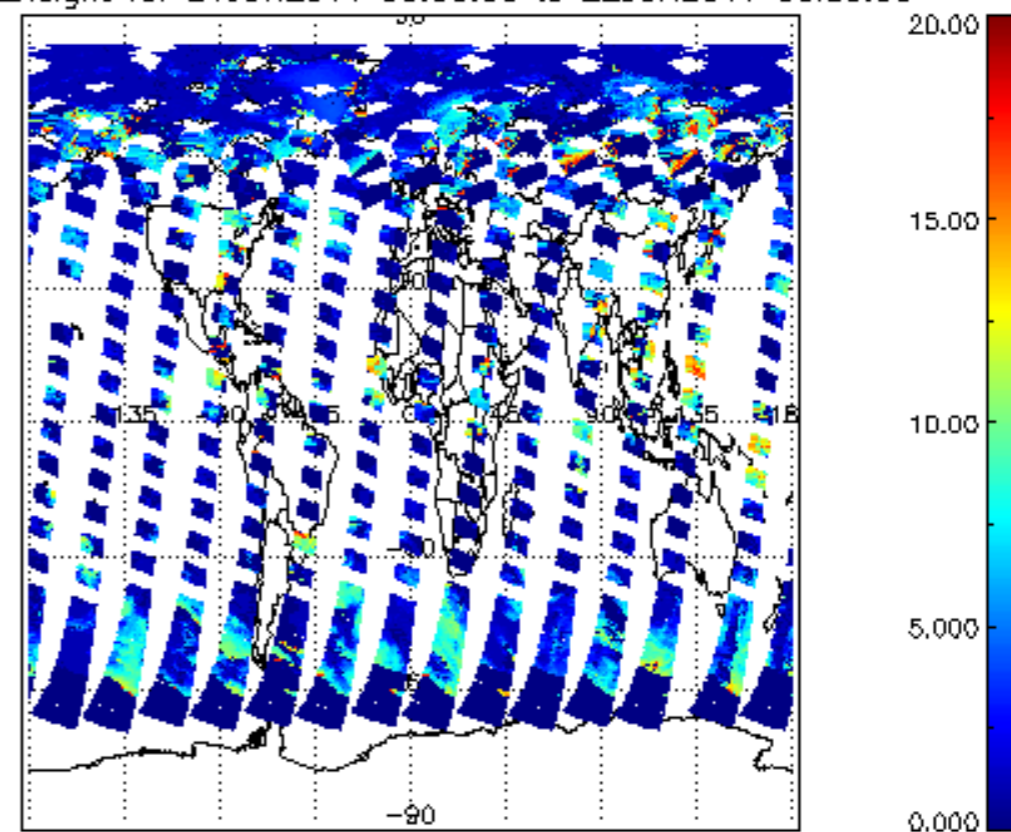
cl_top_height for 21JUN2011 00:00:00 to 22JUN2011 00:00:00
