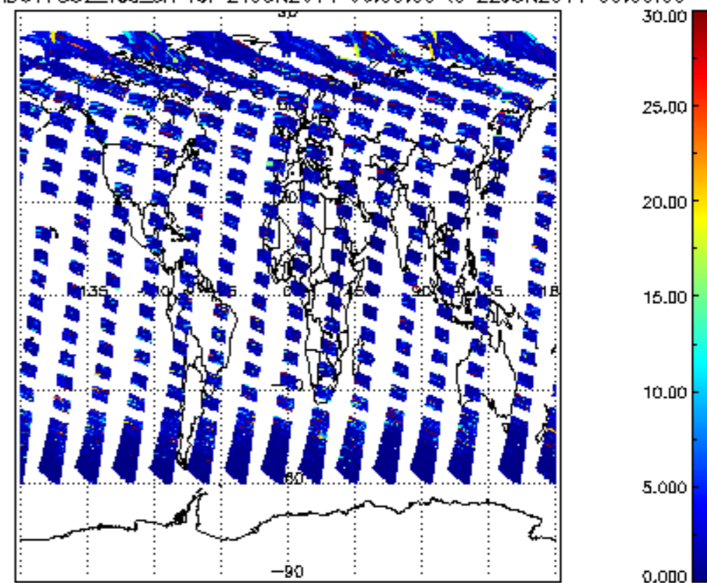
SCIOL2P_NADUV7S02_vcd_err for 21JUN2011 00:00:00 to 22JUN2011 00:00:00
