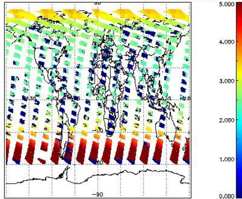
SCIOL2P_NADUV003_amf_cl for 21JUN2011 00:00:00 to 22JUN2011 00:00:00
