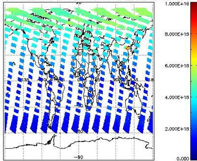
SCIOL2P_NADUV1N02_vcd for 21JUN2011 00:00:00 to 22JUN2011 00:00:00
