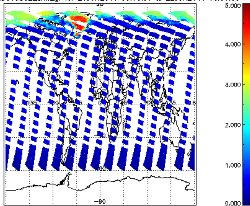
SCIOL2P_NADUV5S02_amf_gr for 21JUN2011 00:00:00 to 22JUN2011 00:00:00
