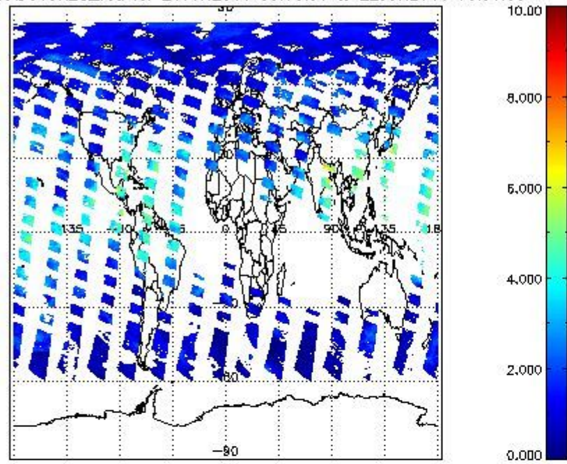
SCIOL2P_NADUV8H2O_vcd for 21JUN2011 00:00:00 to 22JUN2011 00:00:00
