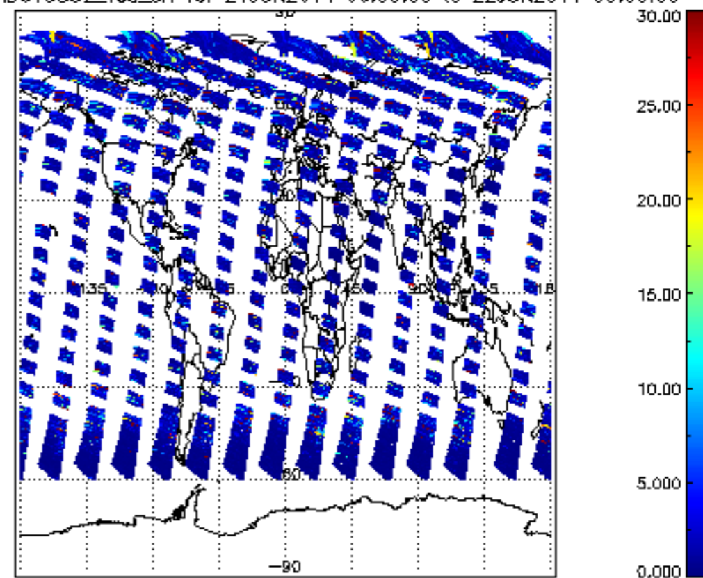
SCIOL2P_NADUV5S02_vcd_err for 21JUN2011 00:00:00 to 22JUN2011 00:00:00
