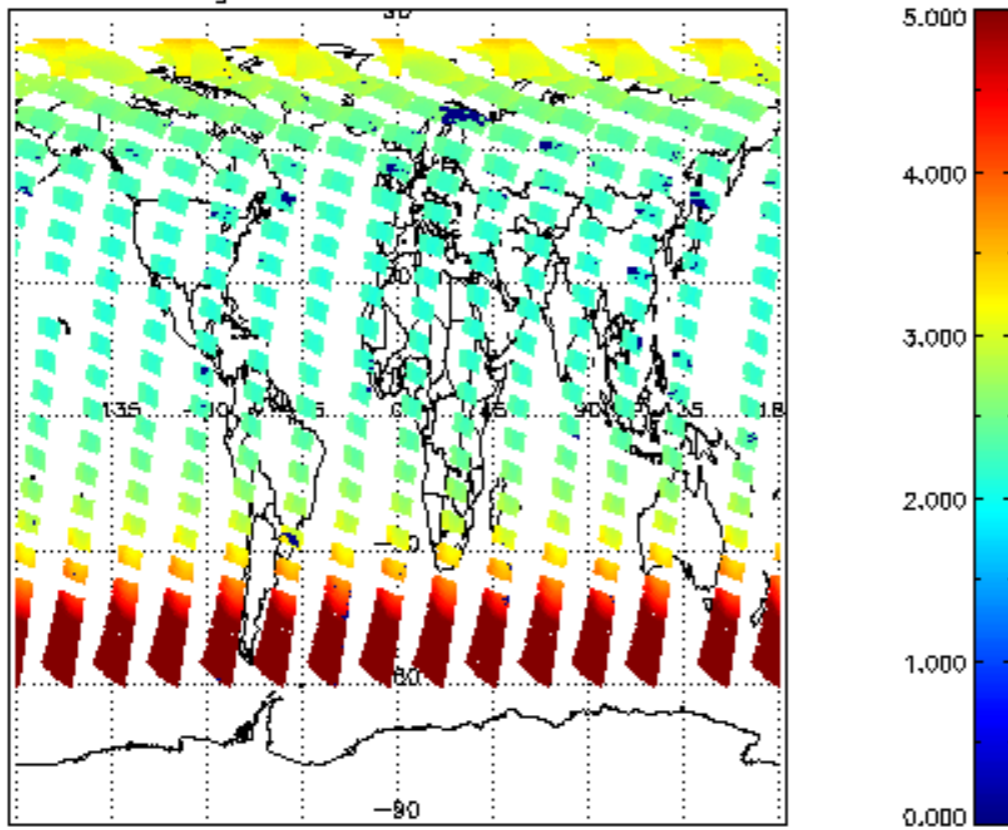
SCIOL2P_NADUV1NO2_amf_gr for 21JUN2011 00:00:00 to 22JUN2011 00:00:00
