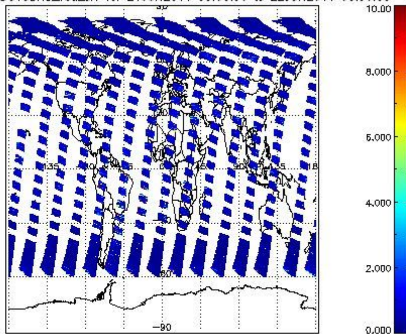
SCIOL2P_NADUV3BRO_vcd_err for 21JUN2011 00:00:00 to 22JUN2011 00:00:00
