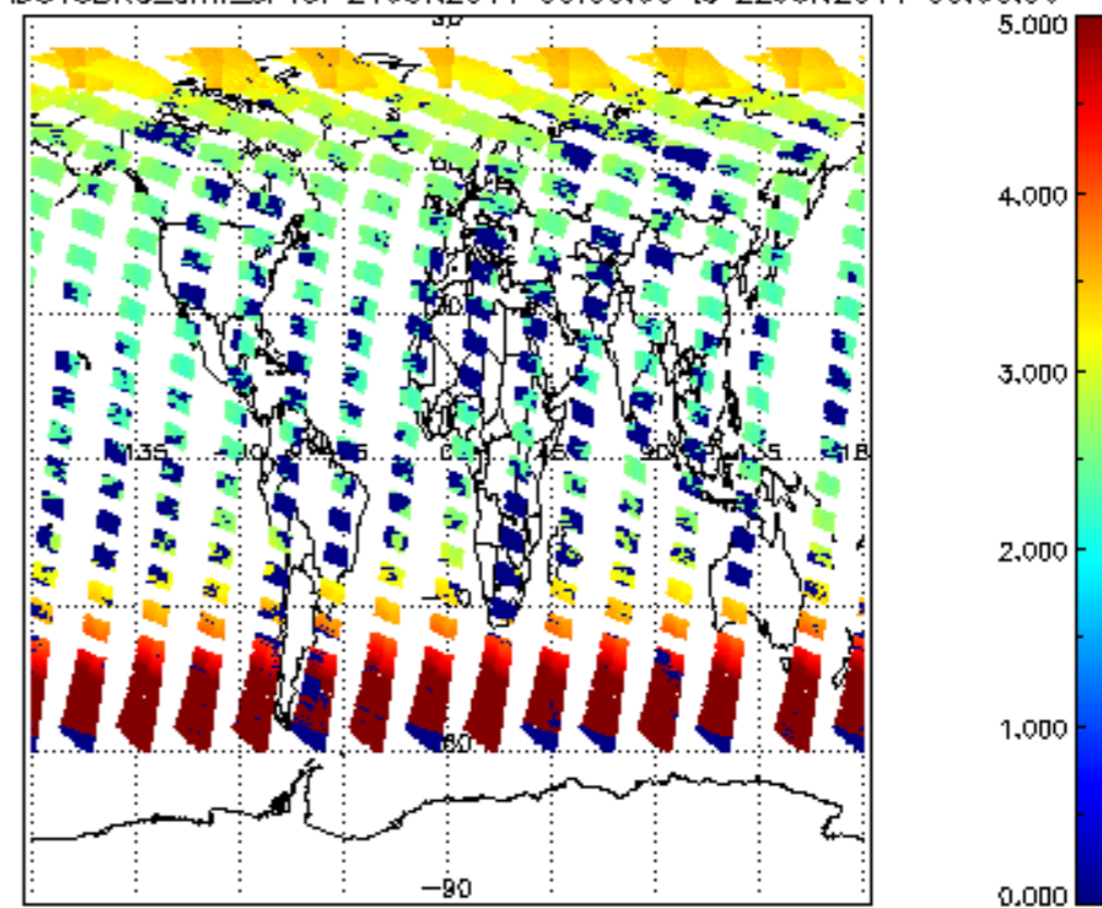
SCIOL2P_NADUV3BRO_amf_sl for 21JUN2011 00:00:00 to 22JUN2011 00:00:00
