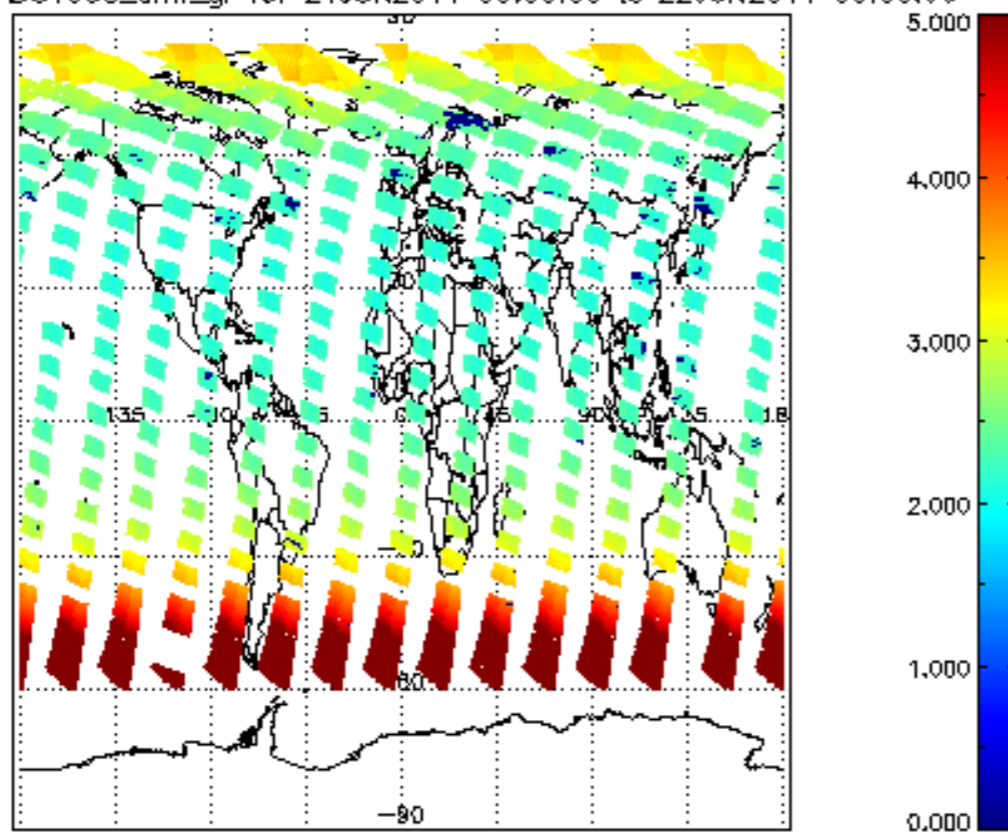
SCIOL2P_NADUV003_amf_gr for 21JUN2011 00:00:00 to 22JUN2011 00:00:00
