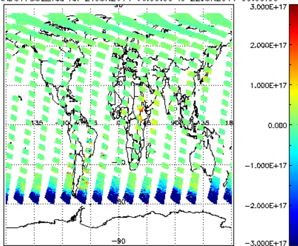
SCIOL2P_NADUV7S02_vcd for 21JUN2011 00:00:00 to 22JUN2011 00:00:00
