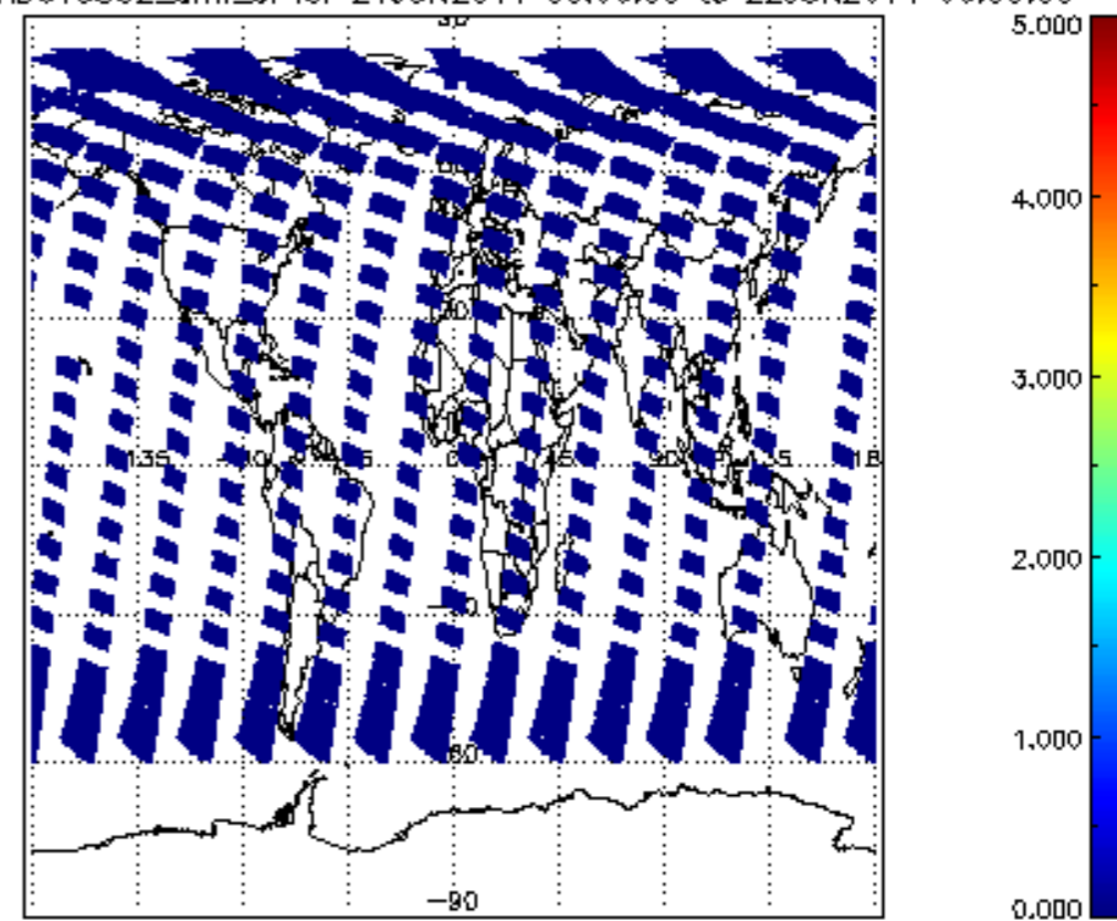
SCIOL2P_NADUV5S02_amf_cl for 21JUN2011 00:00:00 to 22JUN2011 00:00:00
