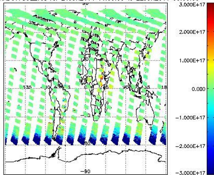
SCIOL2P_NADUV7S02_vcd for 21JUN2011 00:00:00 to 22JUN2011 00:00:00
