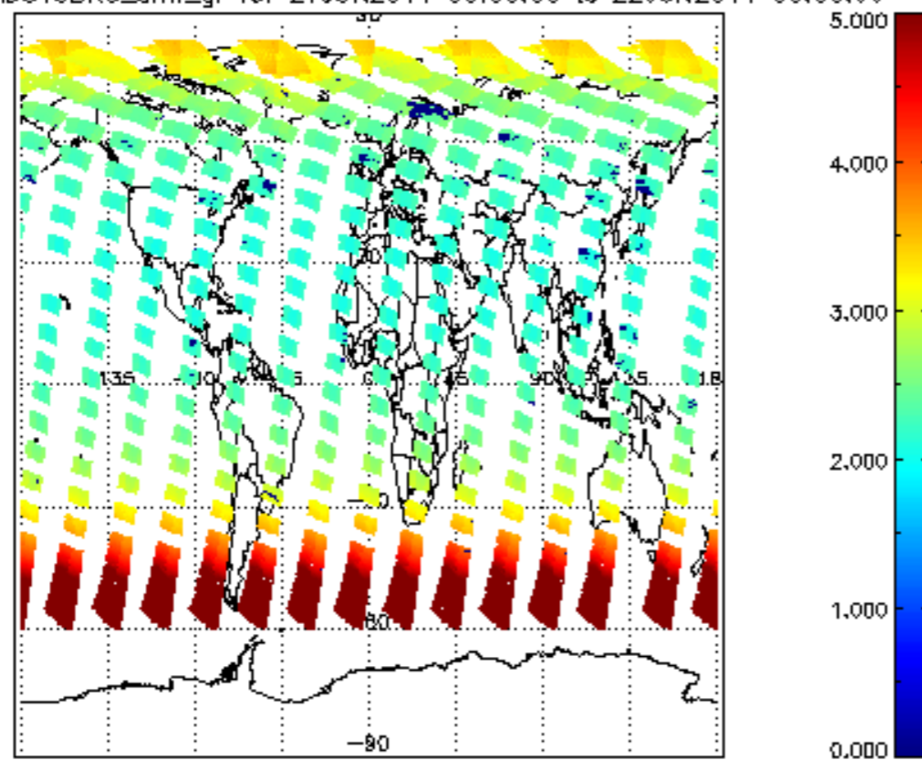
SCIOL2P_NADUV3BRO_amf_gr for 21JUN2011 00:00:00 to 22JUN2011 00:00:00
