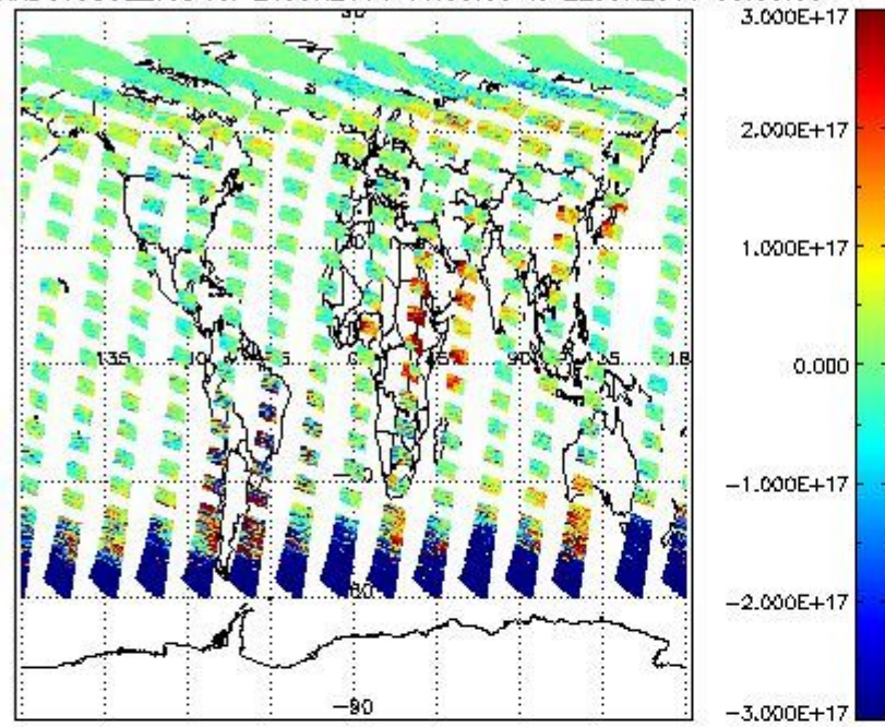
SCIOL2P_NADUV5S02_vcd for 21JUN2011 00:00:00 to 22JUN2011 00:00:00
