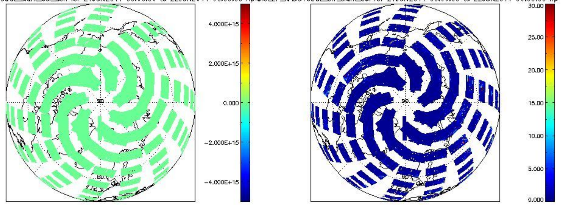
CIOL2P_NADUV60CL_slant_col_den for 21JUN2011 00:00:00 to 22JUN2011 00:00:00 np | CIOL2P_NADUV60CL_err_slant_col for 21JUN2011 00:00:00 to 22JUN2011 00:00:00 np
