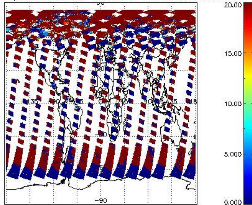
cL_opt_depth for 21JUN2011 00:00:00 to 22JUN2011 00:00:00
