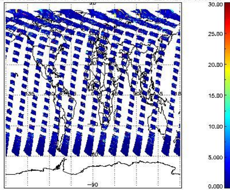
SCIOL2P_NADUV5S02_vcd_err for 21JUN2011 00:00:00 to 22JUN2011 00:00:00
