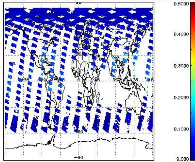
SCIOL2P_NADUV8H2O_vcd_err for 21JUN2011 00:00:00 to 22JUN2011 00:00:00
