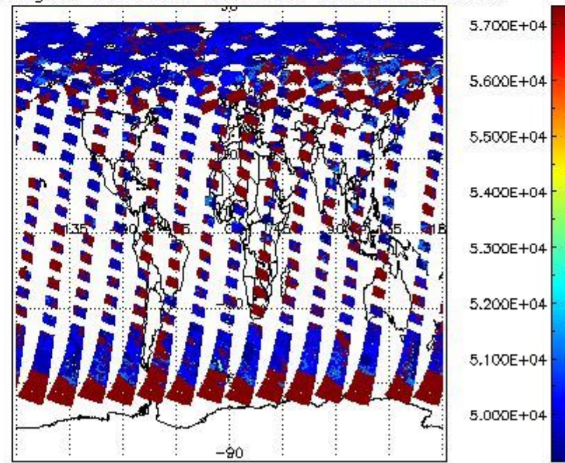
cloud_flags for 21JUN2011 00:00:00 to 22JUN2011 00:00:00
