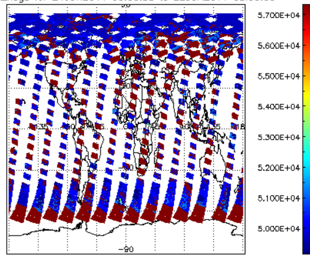
cloud_flags for 21JUN2011 00:00:00 to 22JUN2011 00:00:00
