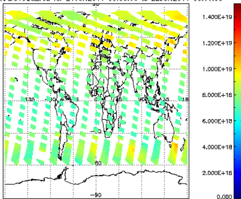
SCIOL2P_NADUV003_vcd for 21JUN2011 00:00:00 to 22JUN2011 00:00:00
