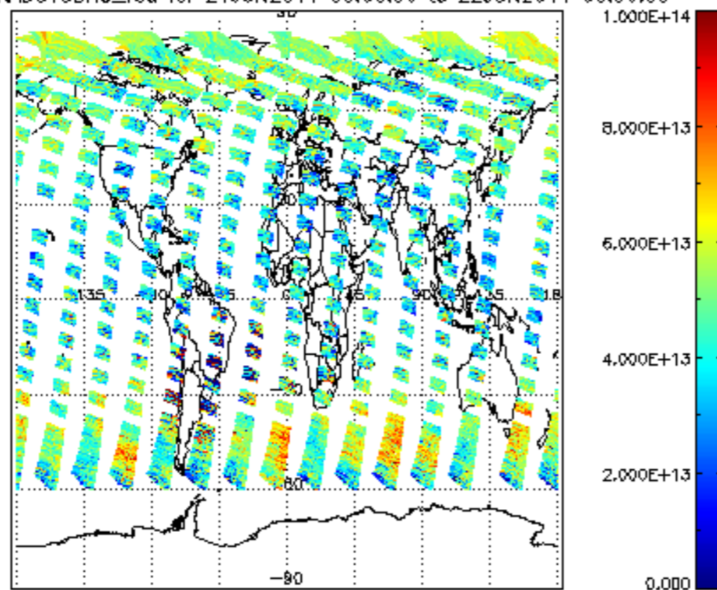
SCIOL2P_NADUV3BRO_vcd for 21JUN2011 00:00:00 to 22JUN2011 00:00:00
