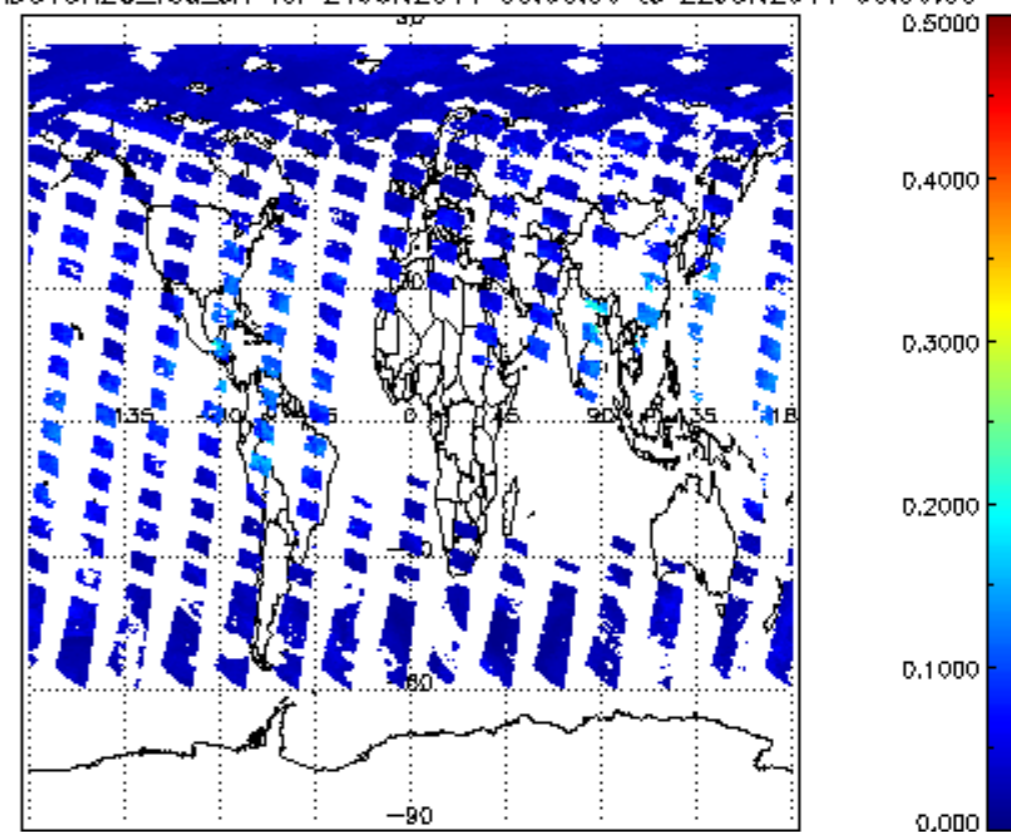
SCIOL2P_NADUV8H2O_vcd_err for 21JUN2011 00:00:00 to 22JUN2011 00:00:00
