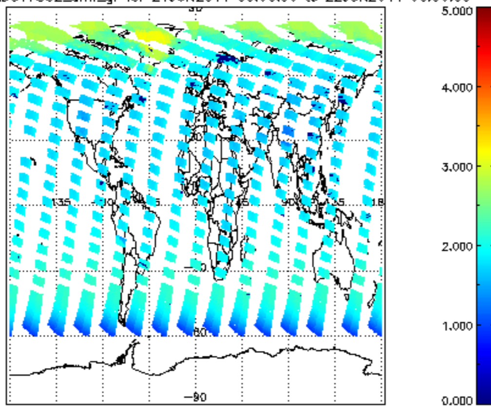
SCIOL2P_NADUV7S02_amf_gr for 21JUN2011 00:00:00 to 22JUN2011 00:00:00
