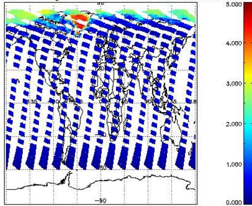
SCIOL2P_NADUV5S02_amf_gr for 21JUN2011 00:00:00 to 22JUN2011 00:00:00
