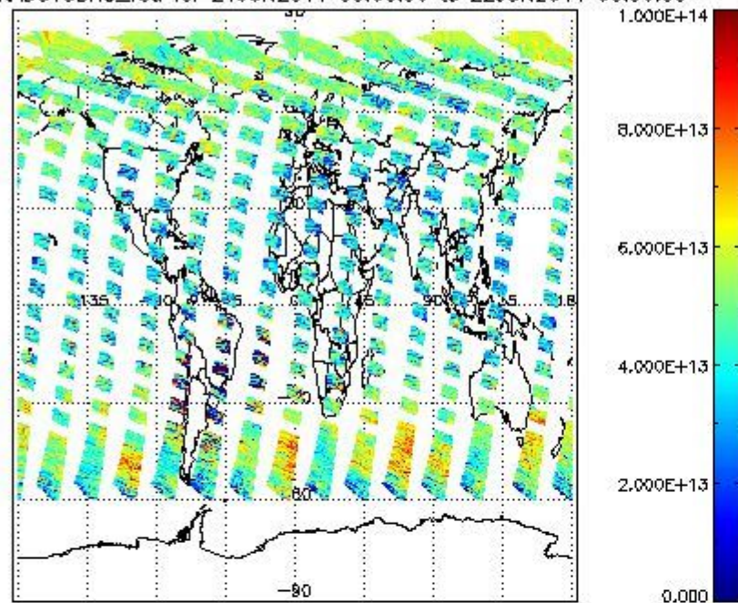
SCIOL2P_NADUV3BRO_vcd for 21JUN2011 00:00:00 to 22JUN2011 00:00:00
