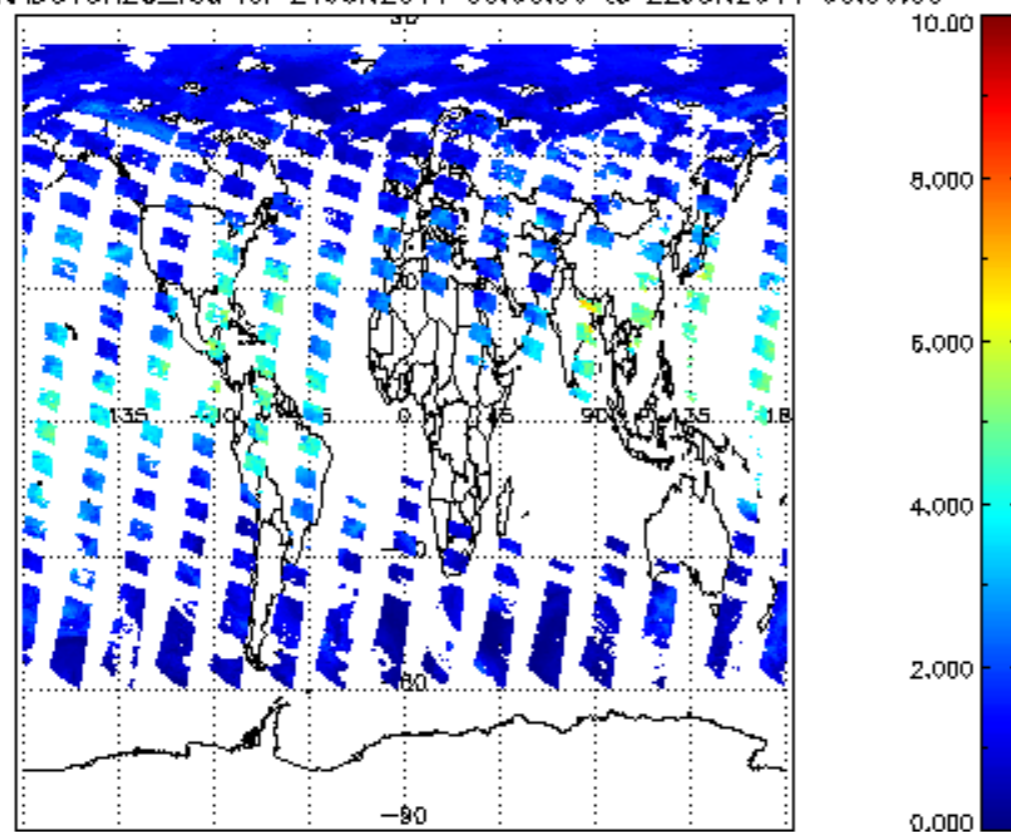
SCIOL2P_NADUV8H2O_vcd for 21JUN2011 00:00:00 to 22JUN2011 00:00:00
