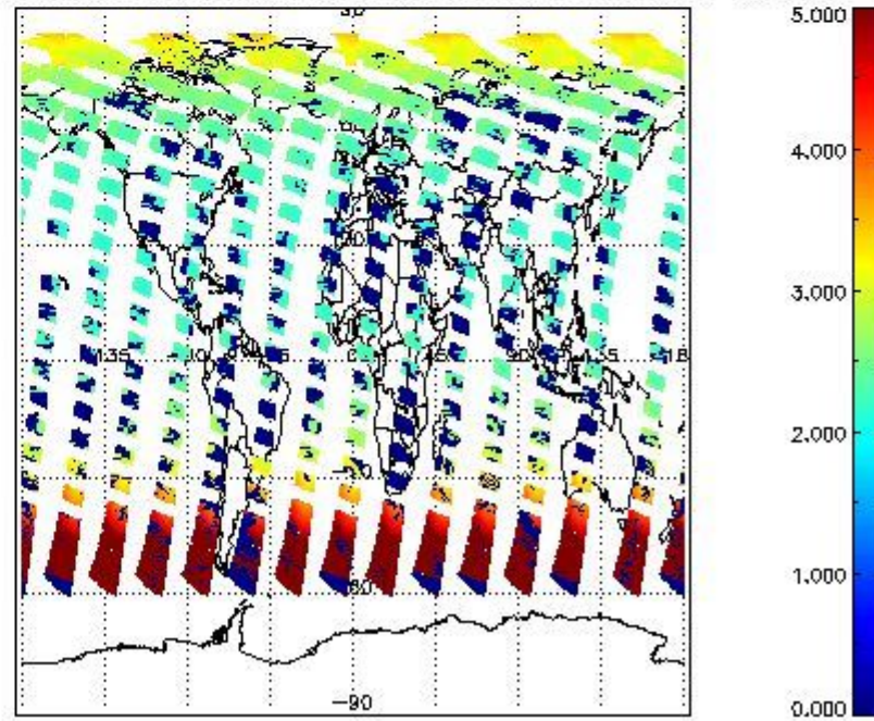
SCIOL2P_NADUV1N02_amf_cl for 21JUN2011 00:00:00 to 22JUN2011 00:00:00
