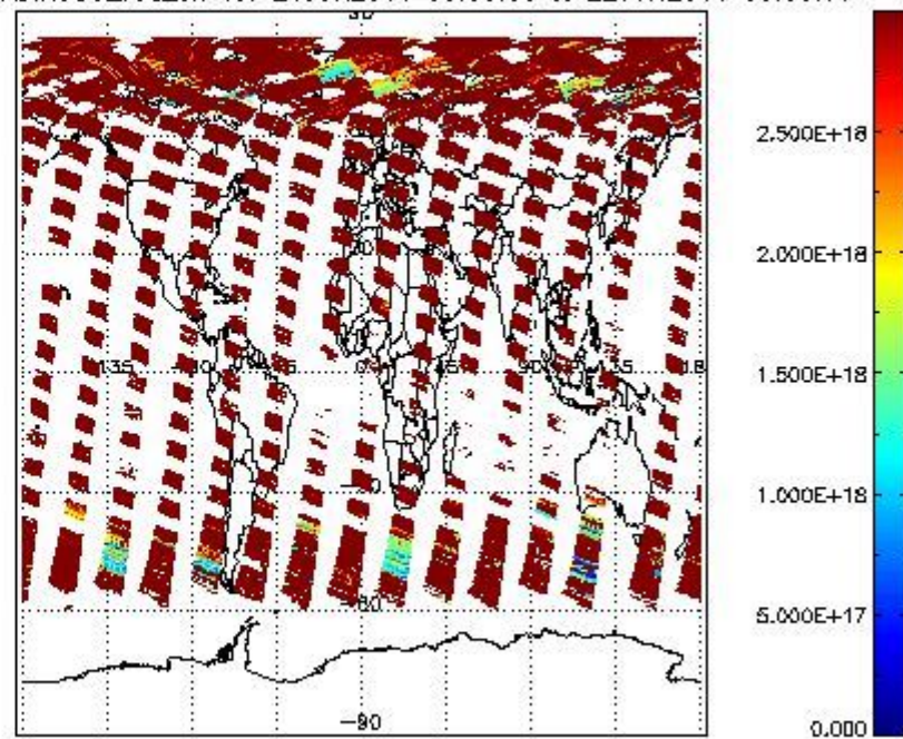
SCIOL2P_NADIR3CO_vcd_err for 21JUN2011 00:00:00 to 22JUN2011 00:00:00
