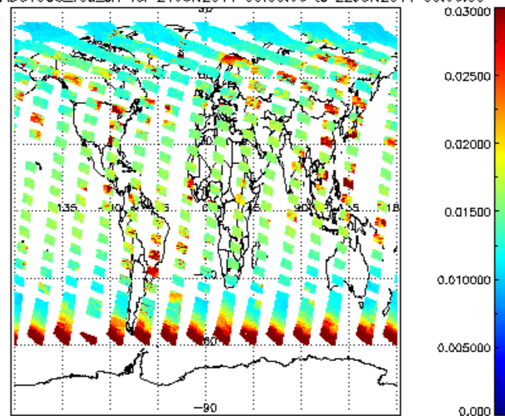
SCIOL2P_NADUV003_vcd_err for 21JUN2011 00:00:00 to 22JUN2011 00:00:00
