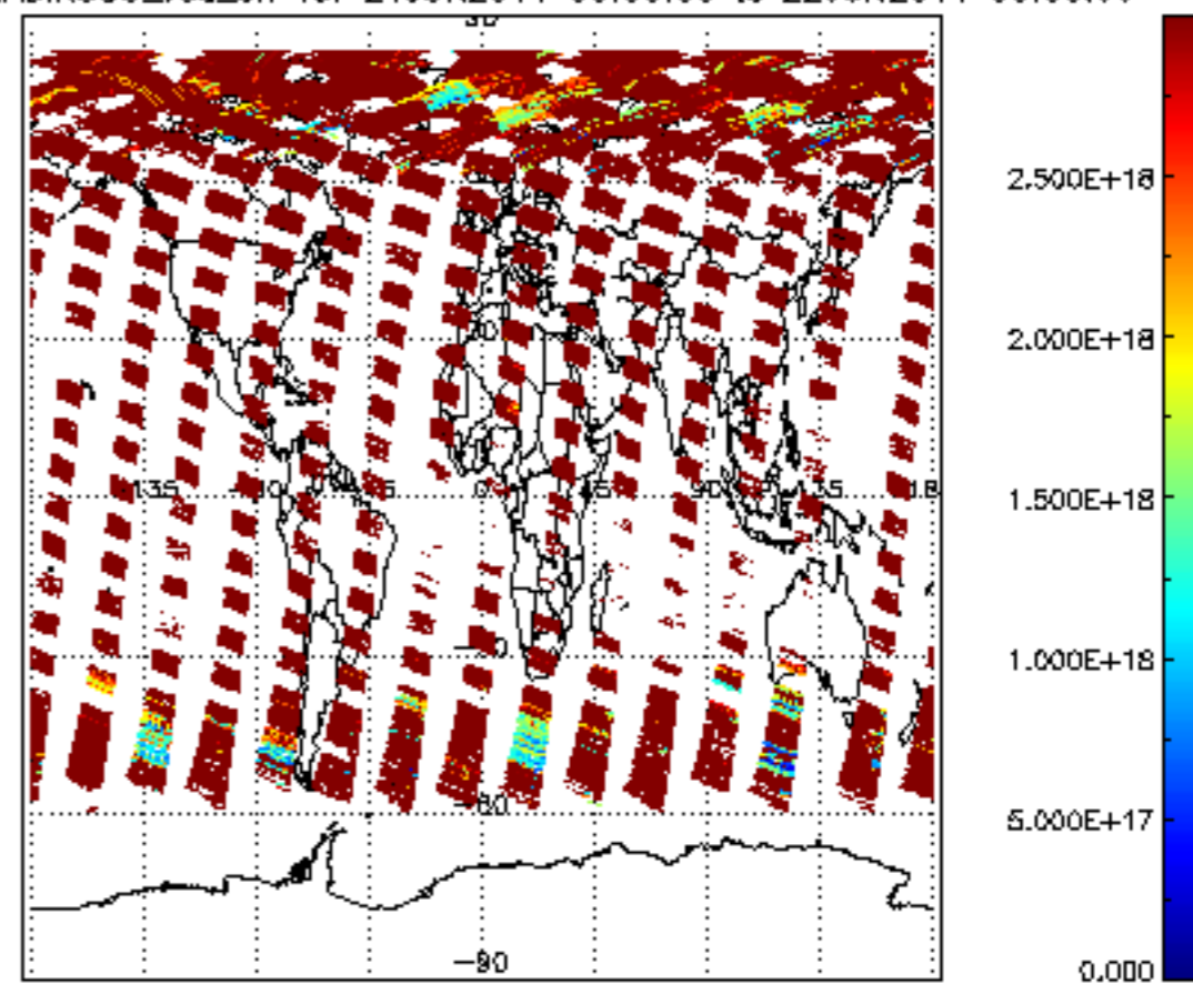
SCIOL2P_NADIR3CO_vcd_err for 21JUN2011 00:00:00 to 22JUN2011 00:00:00
