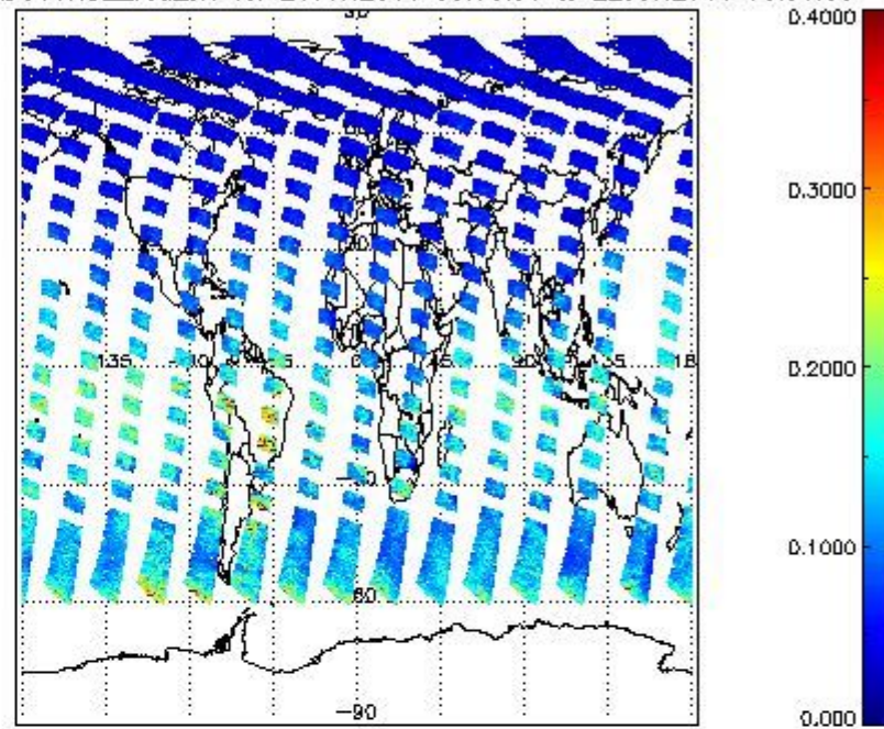
SCIOL2P_NADUV1N02_vcd_err for 21JUN2011 00:00:00 to 22JUN2011 00:00:00
