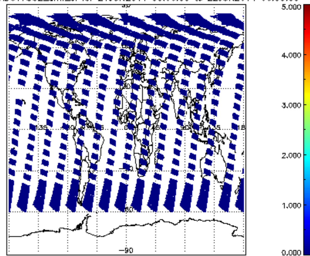
SCIOL2P_NADUV7S02_amf_cl for 21JUN2011 00:00:00 to 22JUN2011 00:00:00
