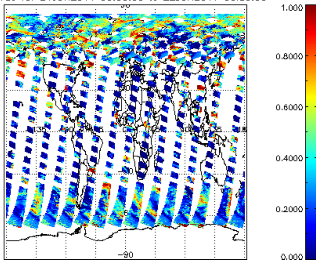
cl_frac for 21JUN2011 00:00:00 to 22JUN2011 00:00:00
