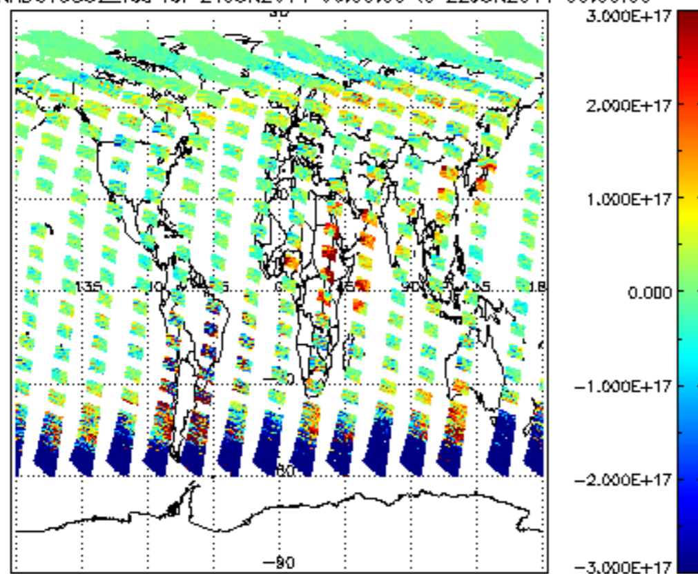
SCIOL2P_NADUV5S02_vcd for 21JUN2011 00:00:00 to 22JUN2011 00:00:00
