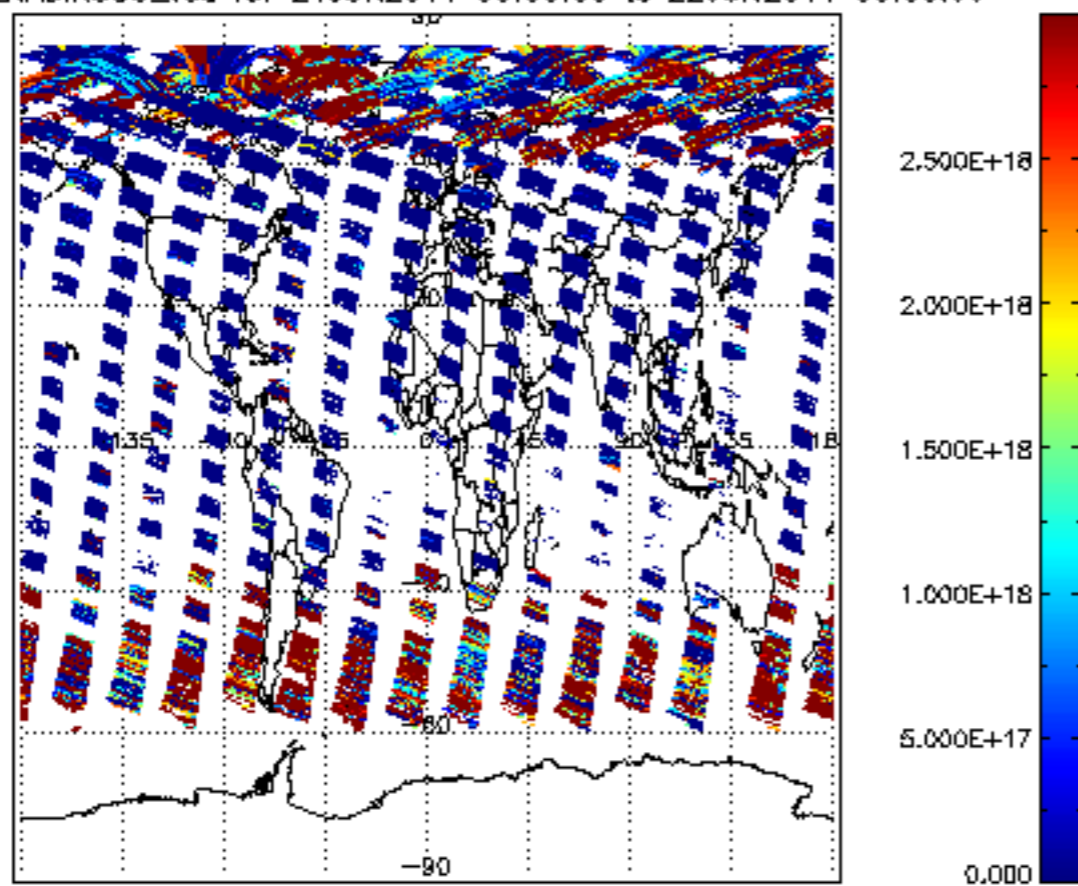
SCIOL2P_NADIR3CO_vcd for 21JUN2011 00:00:00 to 22JUN2011 00:00:00
