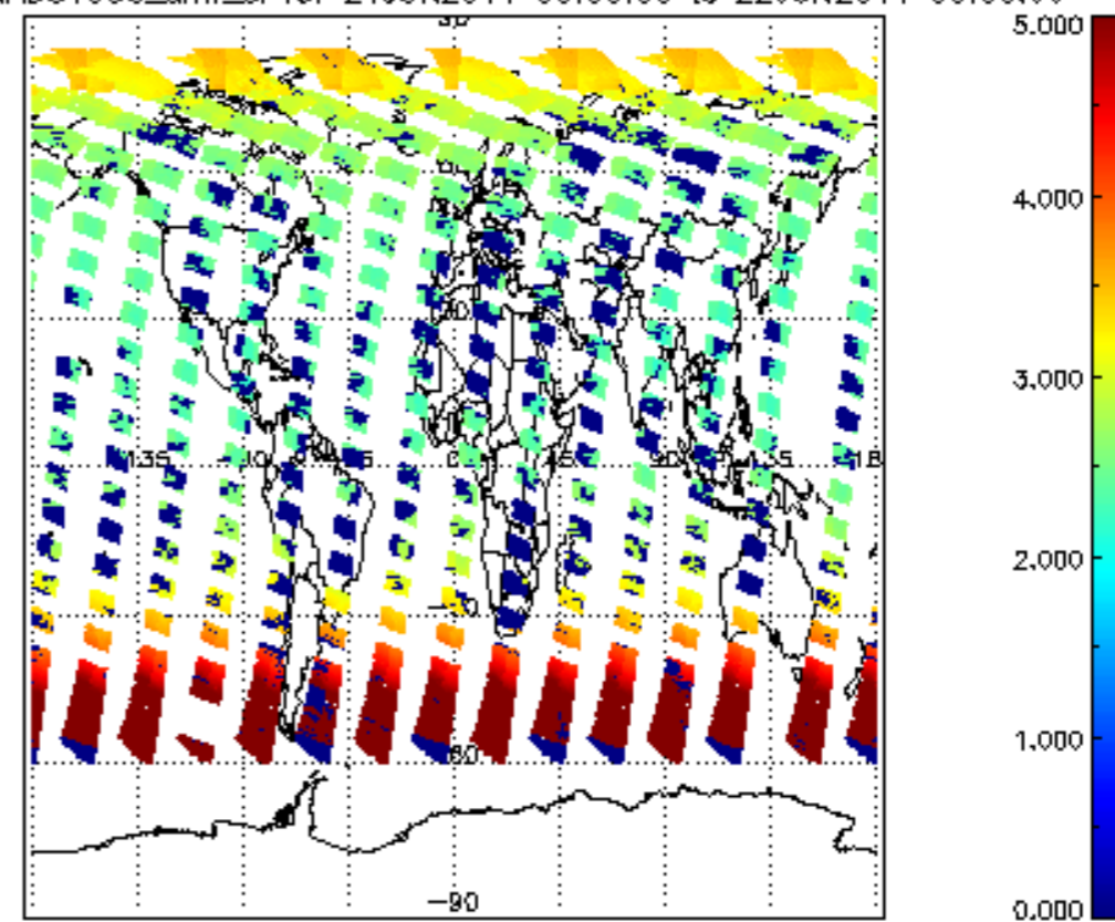
SCIOL2P_NADUV003_amf_cl for 21JUN2011 00:00:00 to 22JUN2011 00:00:00
