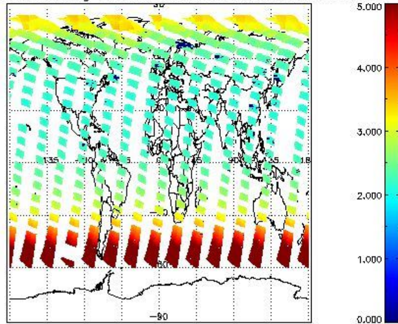
SCIOL2P_NADUV003_amf_gr for 21JUN2011 00:00:00 to 22JUN2011 00:00:00
