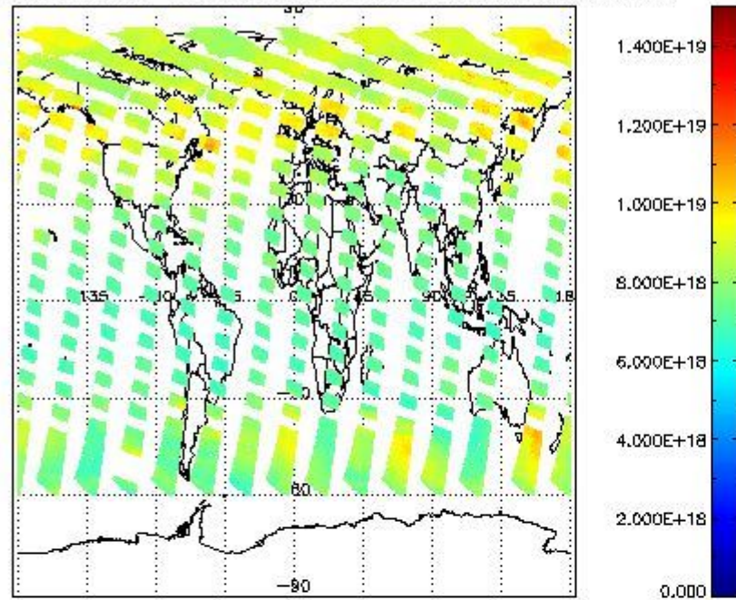
SCIOL2P_NADUV003_vcd for 21JUN2011 00:00:00 to 22JUN2011 00:00:00
