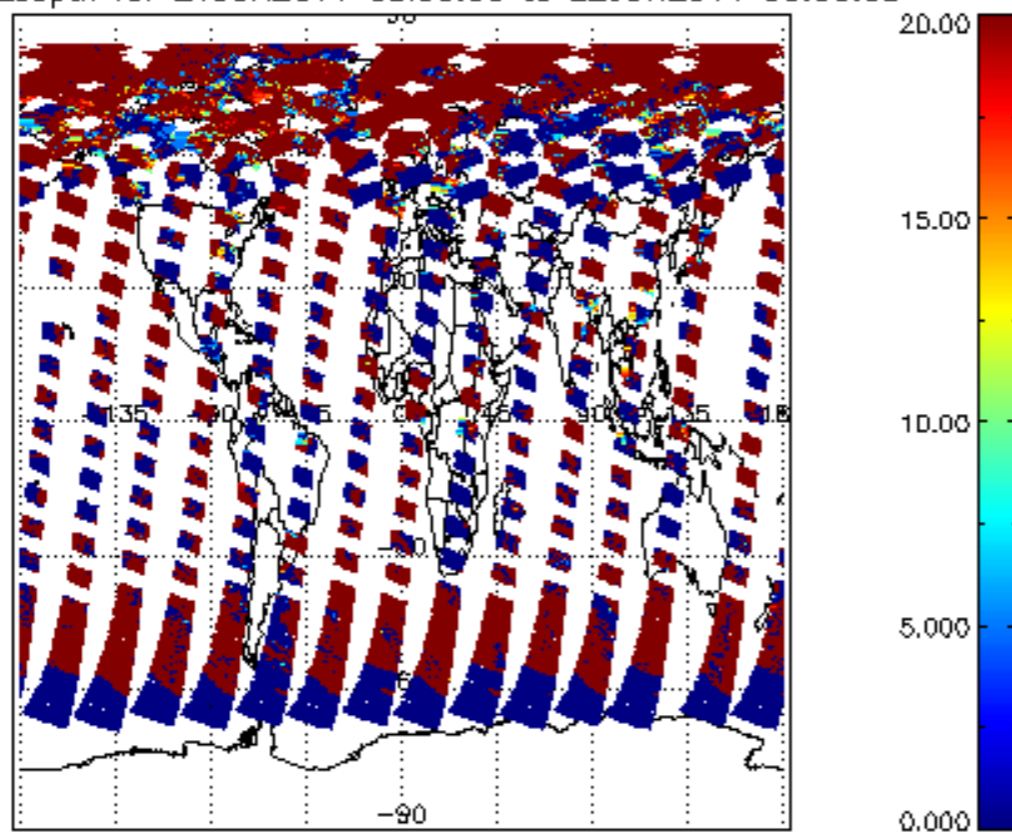
cl_opt_depth for 21JUN2011 00:00:00 to 22JUN2011 00:00:00
