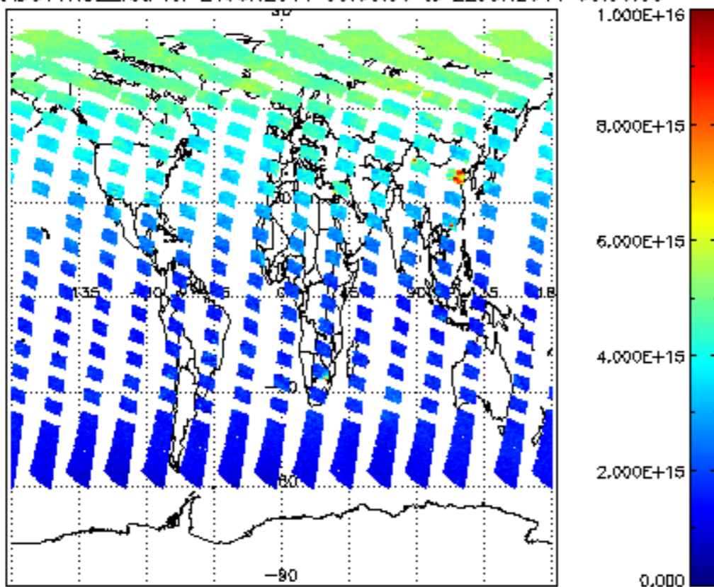
SCIOL2P_NADUV1NO2_vcd for 21JUN2011 00:00:00 to 22JUN2011 00:00:00
