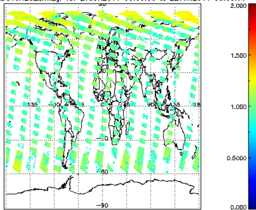
SCIOL2P_NADUV8H2O_amf_gr for 21JUN2011 00:00:00 to 22JUN2011 00:00:00
