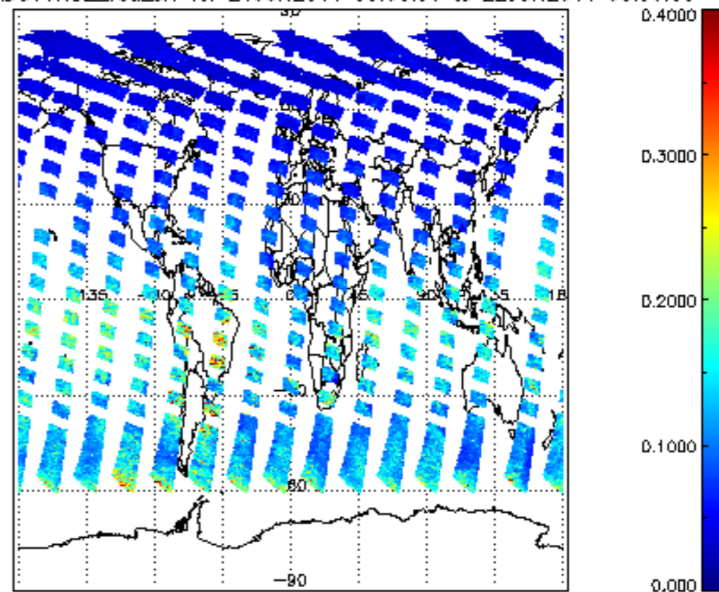
SCIOL2P_NADUV1NO2_vcd_err for 21JUN2011 00:00:00 to 22JUN2011 00:00:00
