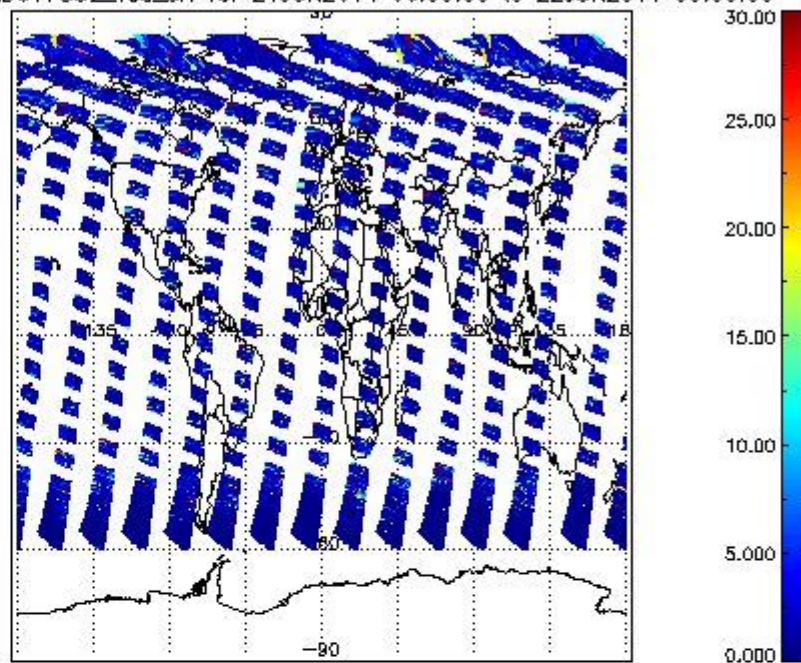
SCIOL2P_NADUV7S02_vcd_err for 21JUN2011 00:00:00 to 22JUN2011 00:00:00
