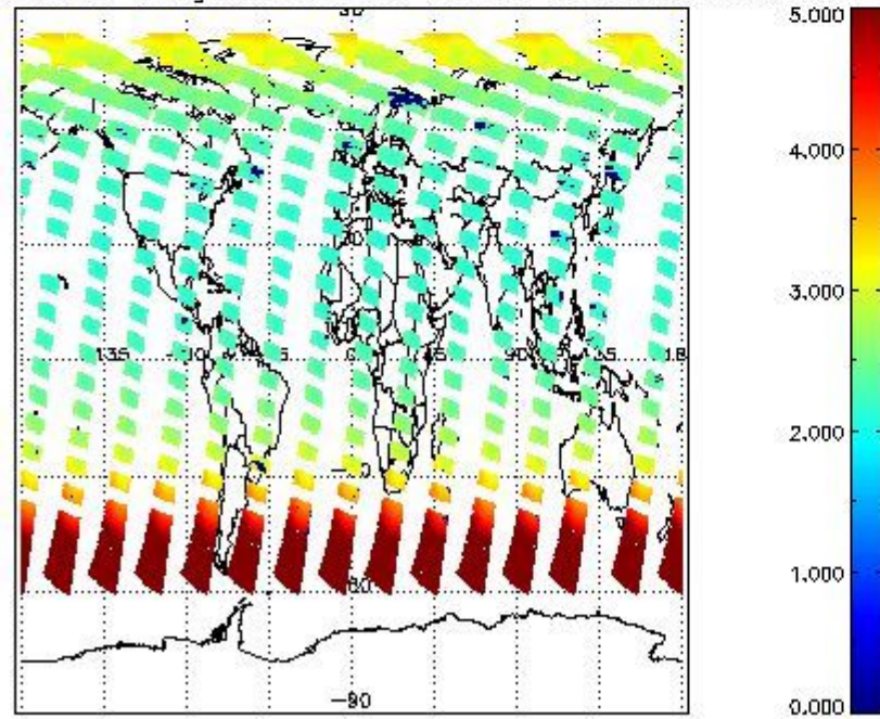
SCIOL2P_NADUV1N02_amf_gr for 21JUN2011 00:00:00 to 22JUN2011 00:00:00
