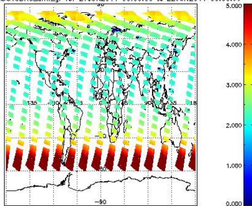
SCIOL2P_NADUV3BRO_amf_gr for 21JUN2011 00:00:00 to 22JUN2011 00:00:00
