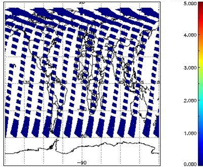
SCIOL2P_NADUV5S02_amf_cl for 21JUN2011 00:00:00 to 22JUN2011 00:00:00
