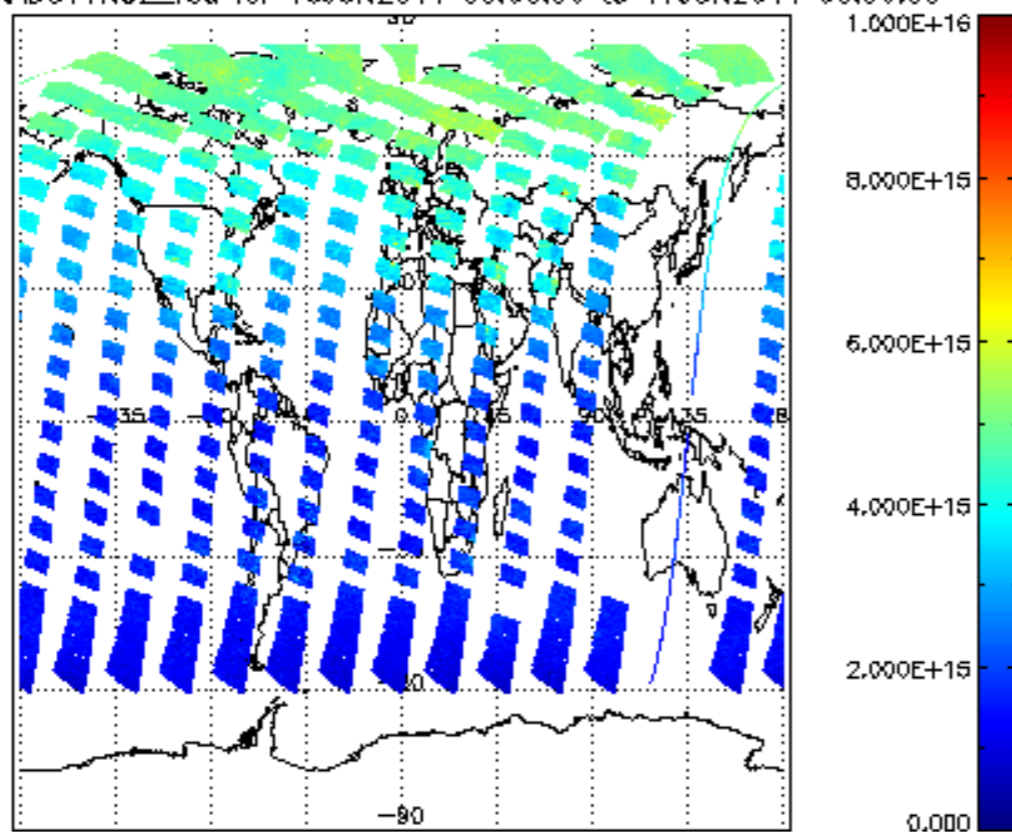
SCIOL2P_NADUV1NO2_vcd for 16JUN2011 00:00:00 to 17JUN2011 00:00:00
