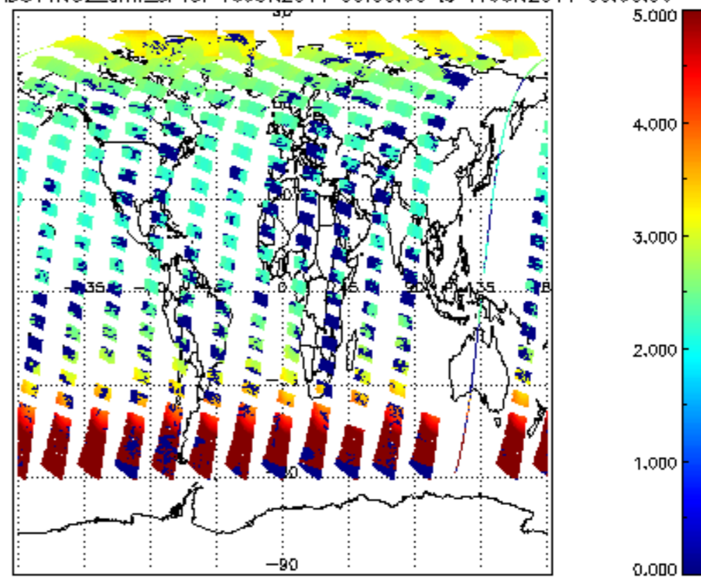
SCIOL2P_NADUV1NO2_amf_cl for 16JUN2011 00:00:00 to 17JUN2011 00:00:00
