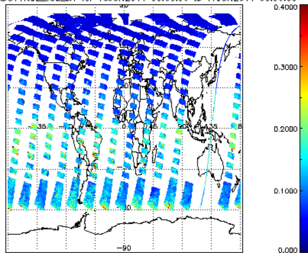
SCIOL2P_NADUV1NO2_vcd_err for 16JUN2011 00:00:00 to 17JUN2011 00:00:00
