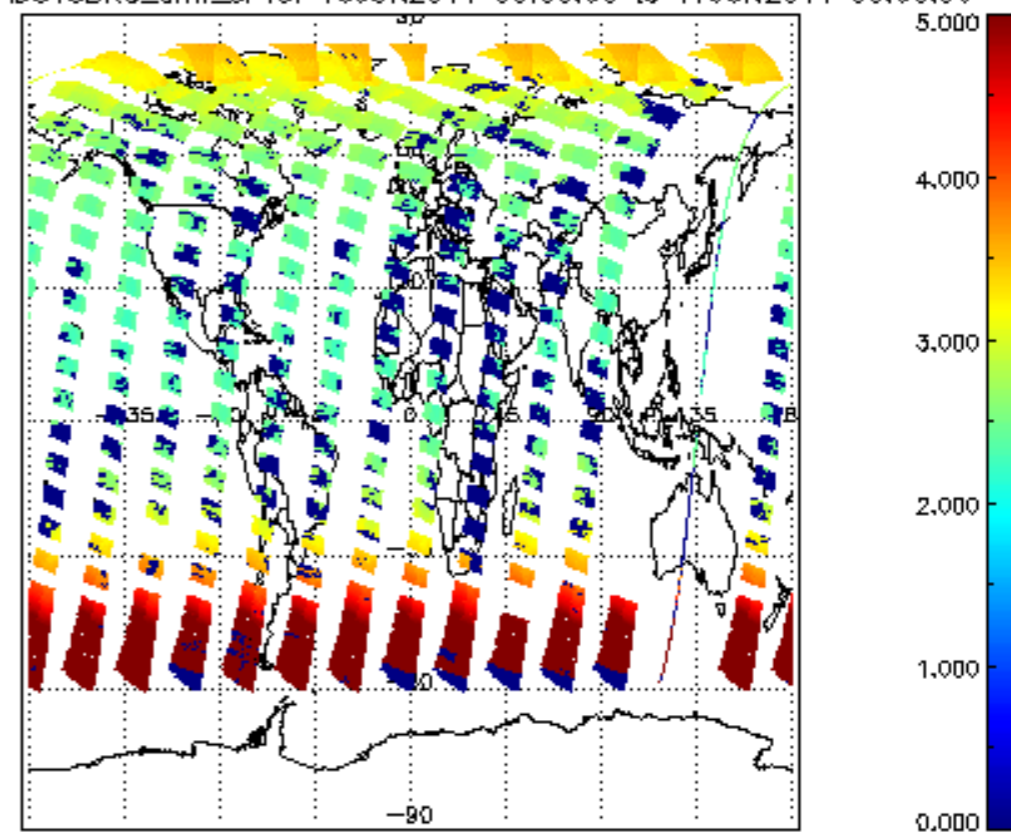
SCIOL2P_NADUV3BRO_amf_cl for 16JUN2011 00:00:00 to 17JUN2011 00:00:00
