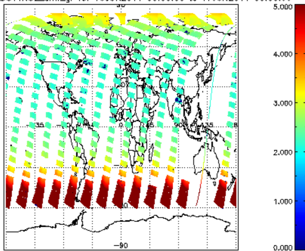
SCIOL2P_NADUV1NO2_amf_gr for 16JUN2011 00:00:00 to 17JUN2011 00:00:00
