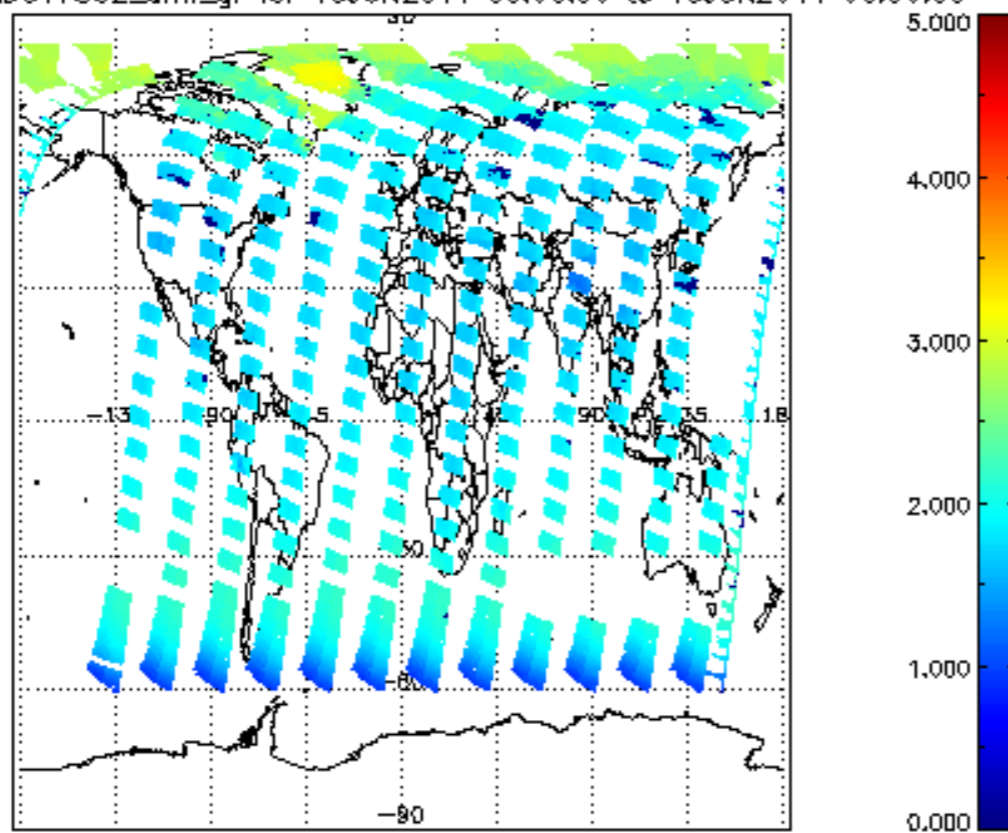
SCIOL2P_NADUV7S02_amf_gr for 15JUN2011 00:00:00 to 16JUN2011 00:00:00
