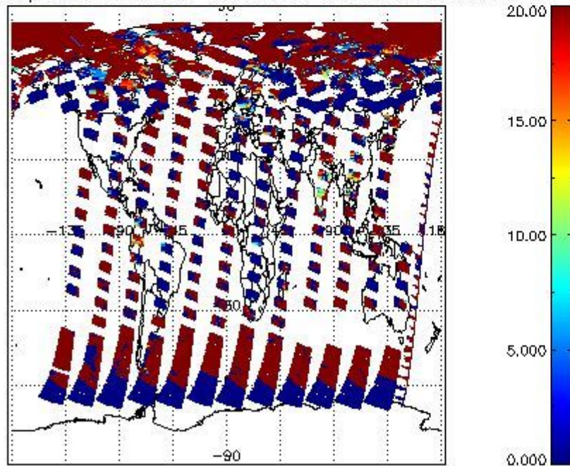
cL_opt_depth for 15JUN2011 00:00:00 to 16JUN2011 00:00:00
