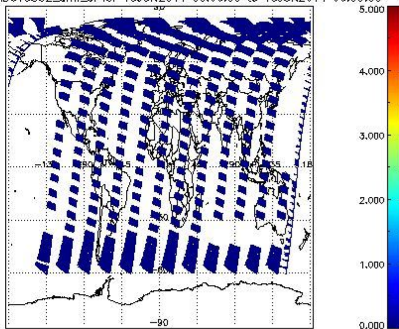
SCIOL2P_NADUV5S02_amf_cl for 15JUN2011 00:00:00 to 16JUN2011 00:00:00
