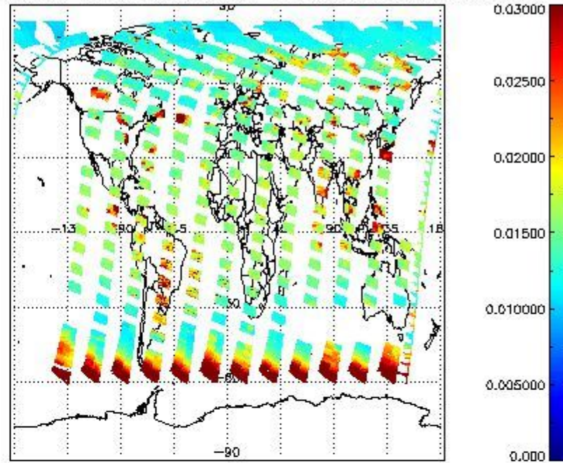
SCIOL2P_NADUV003_vcd_err for 15JUN2011 00:00:00 to 16JUN2011 00:00:00
