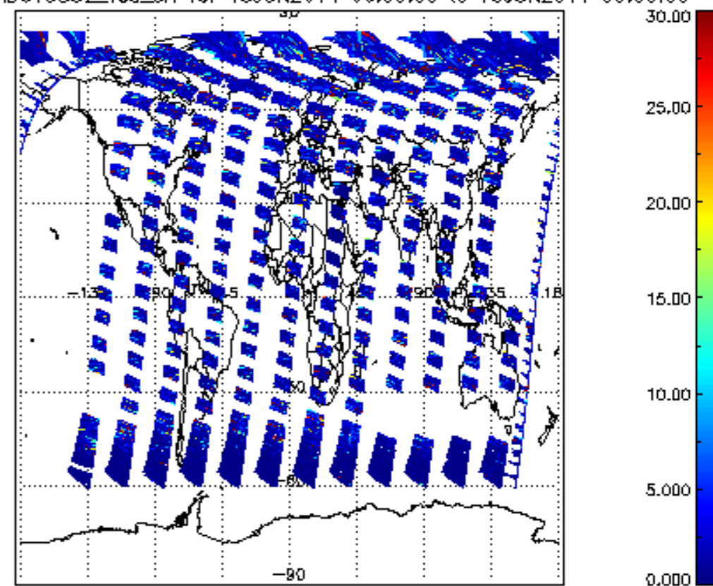
SCIOL2P_NADUV5S02_vcd_err for 15JUN2011 00:00:00 to 16JUN2011 00:00:00
