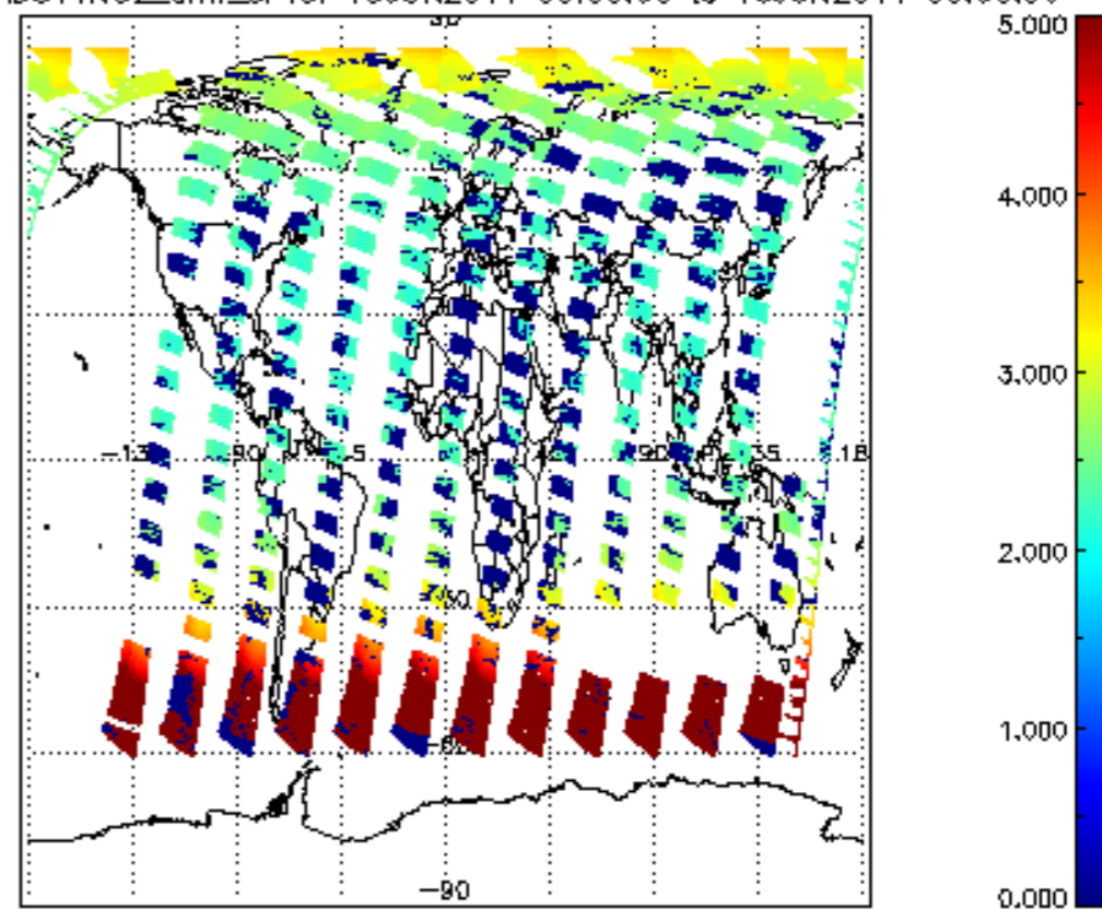
SCIOL2P_NADUV1NO2_amf_sl for 15JUN2011 00:00:00 to 16JUN2011 00:00:00
