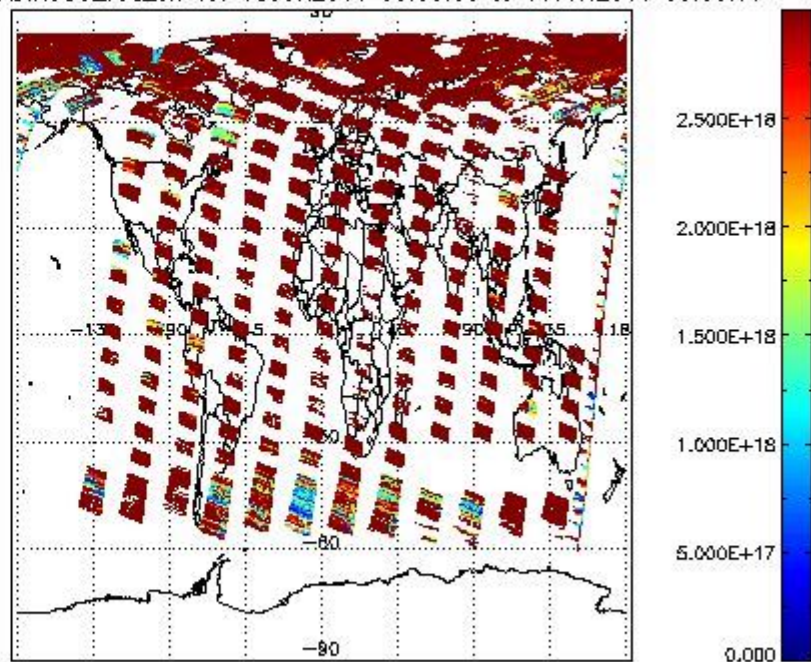
SCIO2P_NADIR3CO_vcd_err for 15JUN2011 00:00:00 to 16JUN2011 00:00:00
