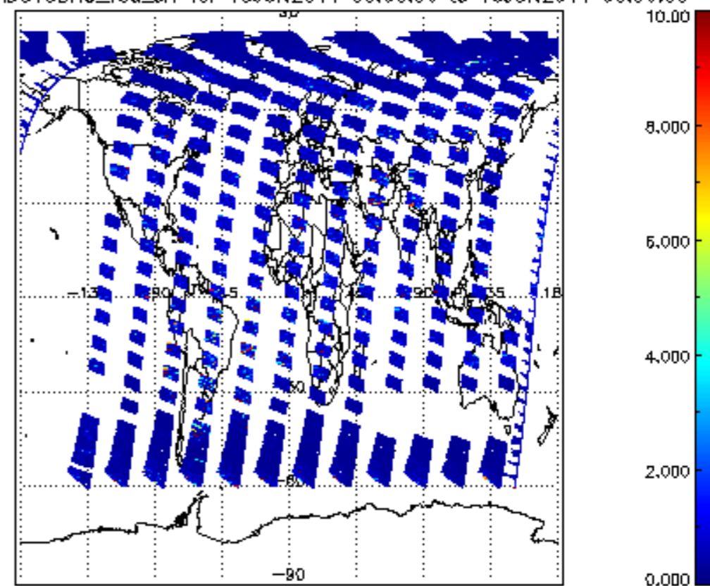
SCIOL2P_NADUV3BRO_vcd_err for 15JUN2011 00:00:00 to 16JUN2011 00:00:00
