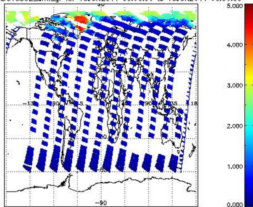
SCIOL2P_NADUV5S02_amf_gr for 15JUN2011 00:00:00 to 16JUN2011 00:00:00
