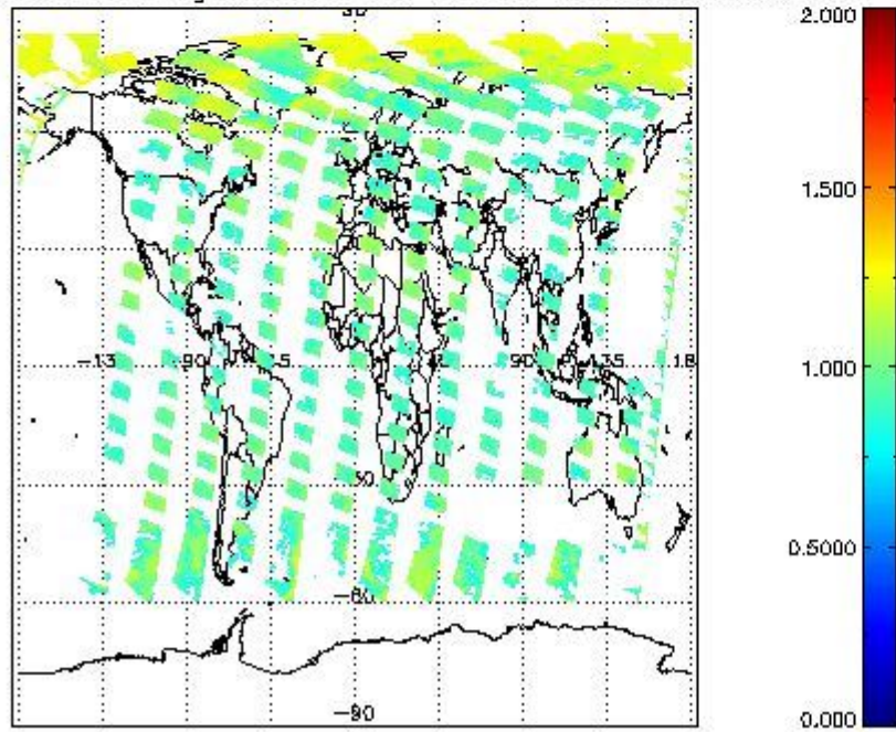
SCIOL2P_NADUV8H2O_arnf_gr for 15JUN2011 00:00:00 to 16JUN2011 00:00:00
