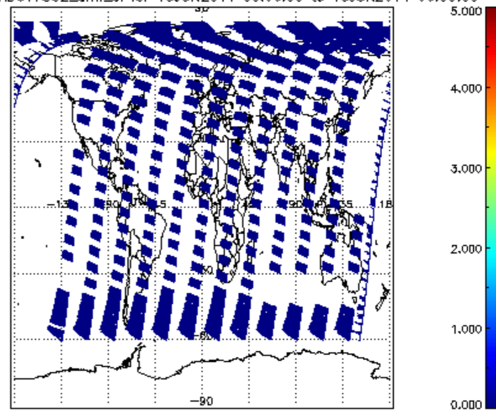
SCIOL2P_NADUV7S02_amf_cl for 15JUN2011 00:00:00 to 16JUN2011 00:00:00
