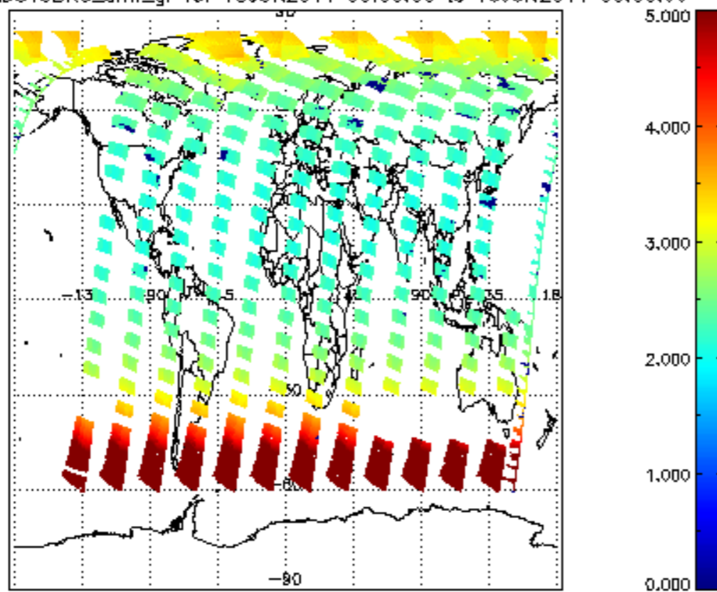
SCIOL2P_NADUV3BRO_amf_gr for 15JUN2011 00:00:00 to 16JUN2011 00:00:00
