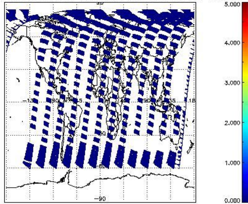
SCIOL2P_NADUV7S02_amf_cl for 15JUN2011 00:00:00 to 16JUN2011 00:00:00
