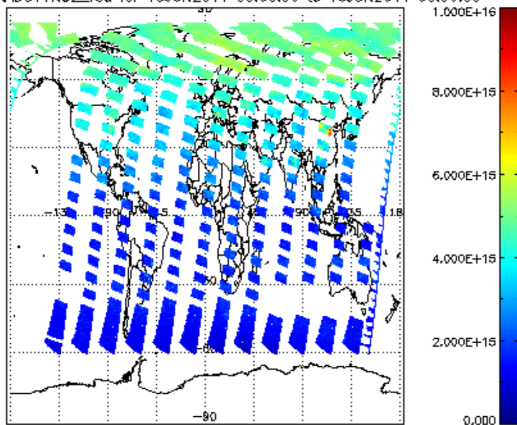
SCIOL2P_NADUV1NO2_vcd for 15JUN2011 00:00:00 to 16JUN2011 00:00:00
