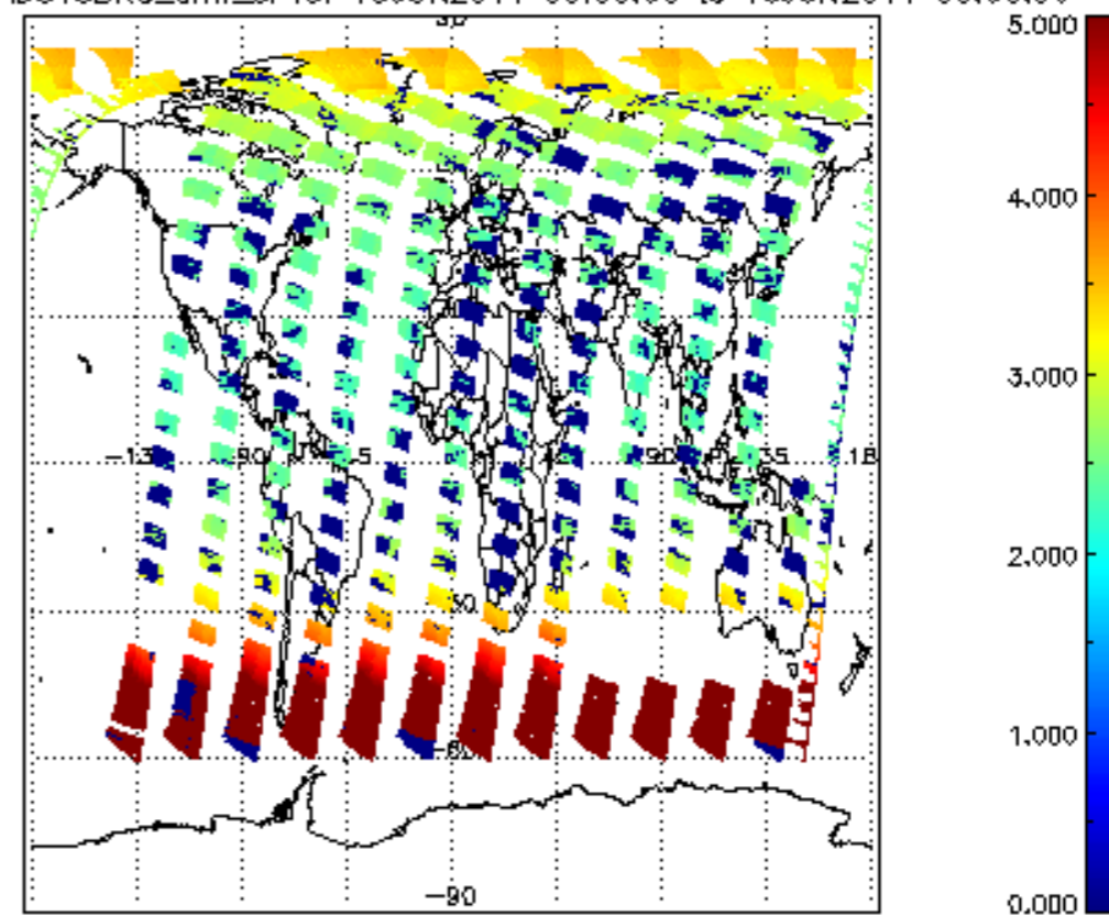
SCIOL2P_NADUV3BRO_amf_sl for 15JUN2011 00:00:00 to 16JUN2011 00:00:00
