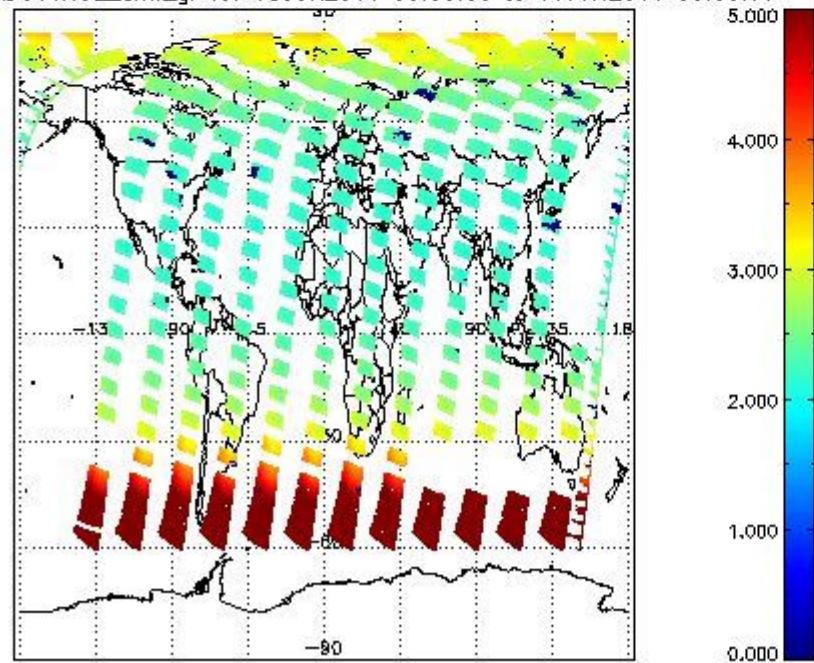
SCIOL2P_NADUV1NO2_amf_gr for 15JUN2011 00:00:00 to 16JUN2011 00:00:00
