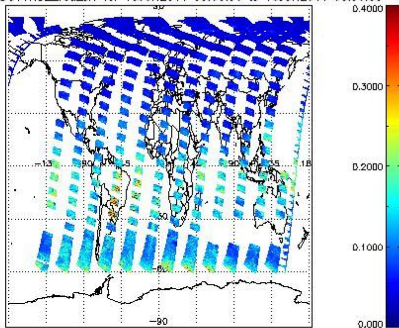
SCIOL2P_NADUV1NO2_vcd_err for 15JUN2011 00:00:00 to 16JUN2011 00:00:00
