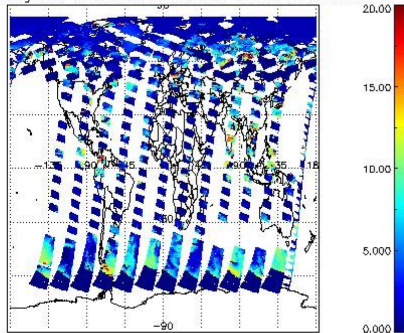
cL_top_height for 15JUN2011 00:00:00 to 16JUN2011 00:00:00
