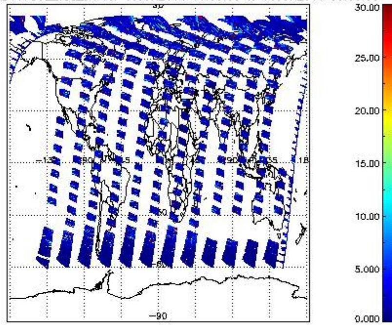
SCIOL2P_NADUV7S02_vcd_err for 15JUN2011 00:00:00 to 16JUN2011 00:00:00
