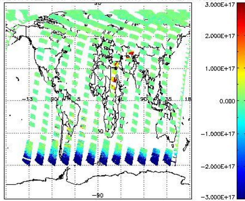
SCIOL2P_NADUV7S02_vcd for 15JUN2011 00:00:00 to 16JUN2011 00:00:00
