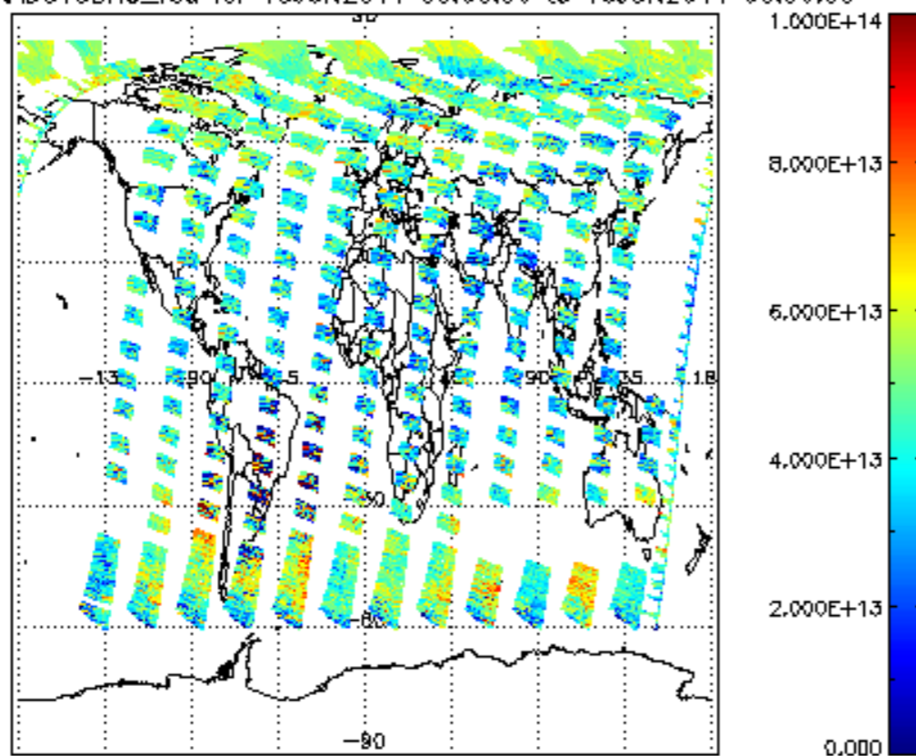
SCIOL2P_NADUV3BRO_vcd for 15JUN2011 00:00:00 to 16JUN2011 00:00:00
