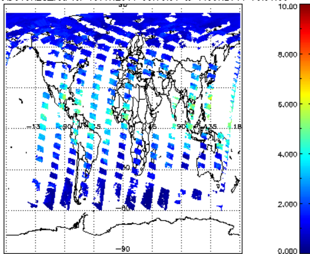
SCIOL2P_NADUV8H2O_vcd for 15JUN2011 00:00:00 to 16JUN2011 00:00:00
