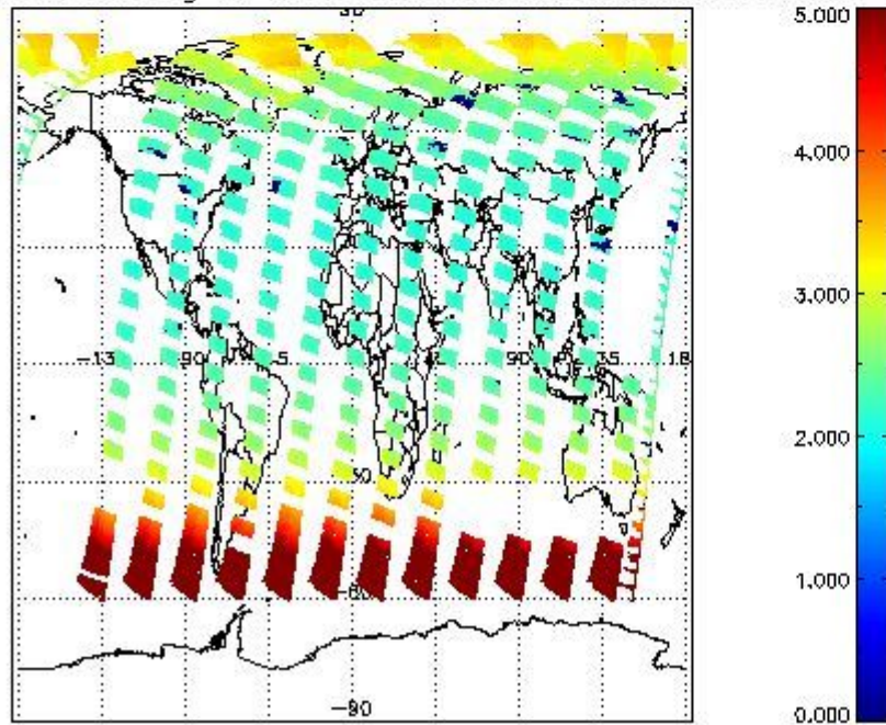
SCIOL2P_NADUV003_amf_gr for 15JUN2011 00:00:00 to 16JUN2011 00:00:00
