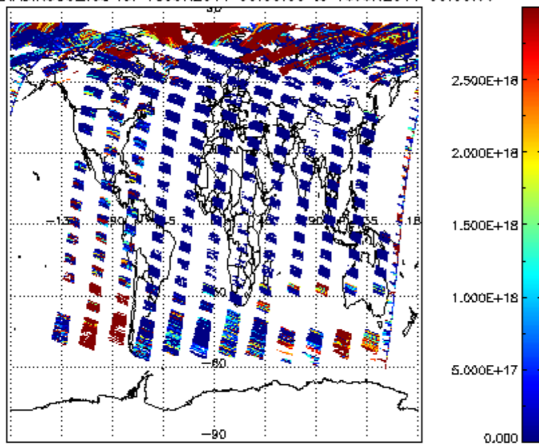
SCIOL2P_NADIR3CO_vcd for 15JUN2011 00:00:00 to 16JUN2011 00:00:00
