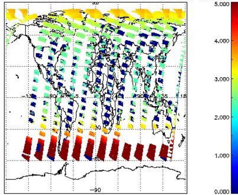
SCIOL2P_NADUV3BRO_amf_cl for 15JUN2011 00:00:00 to 16JUN2011 00:00:00
