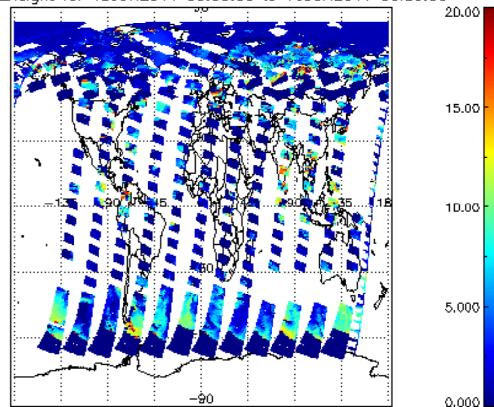
cl_top_height for 15JUN2011 00:00:00 to 16JUN2011 00:00:00
