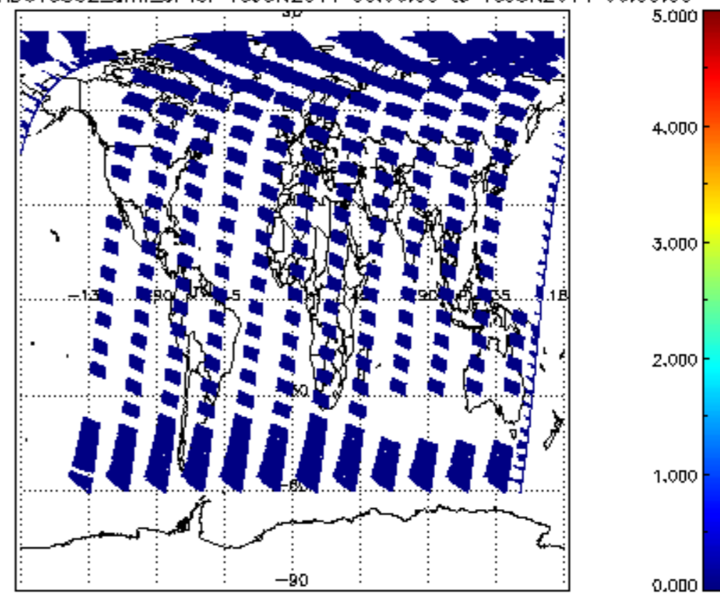
SCIOL2P_NADUV5S02_amf_cl for 15JUN2011 00:00:00 to 16JUN2011 00:00:00
