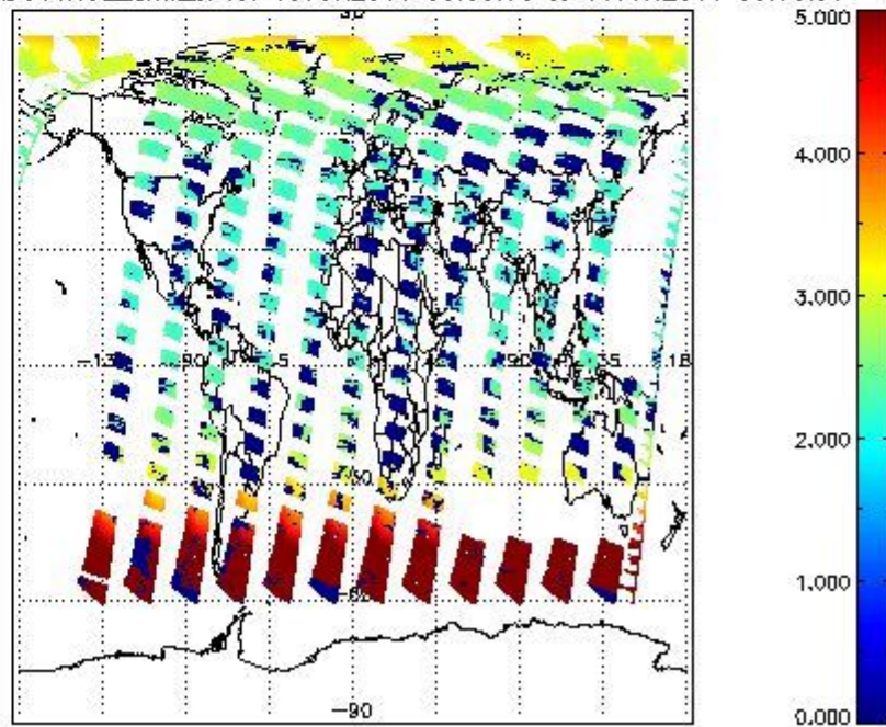
SCIOL2P_NADUV1NO2_amf_cl for 15JUN2011 00:00:00 to 16JUN2011 00:00:00
