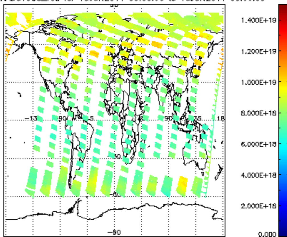
SCIOL2P_NADUV003_vcd for 15JUN2011 00:00:00 to 16JUN2011 00:00:00
