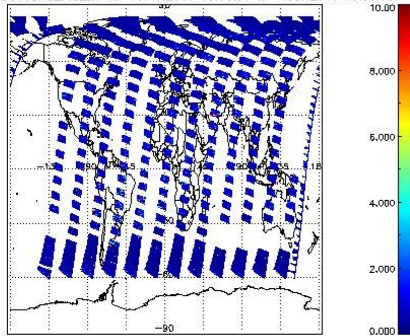
SCIOL2P_NADUV3BRO_vcd_err for 15JUN2011 00:00:00 to 16JUN2011 00:00:00
