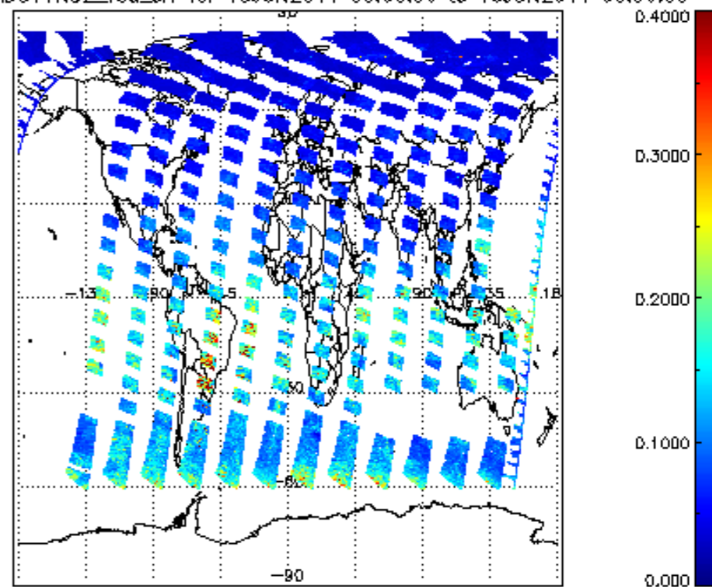
SCIOL2P_NADUV1NO2_vcd_err for 15JUN2011 00:00:00 to 16JUN2011 00:00:00
