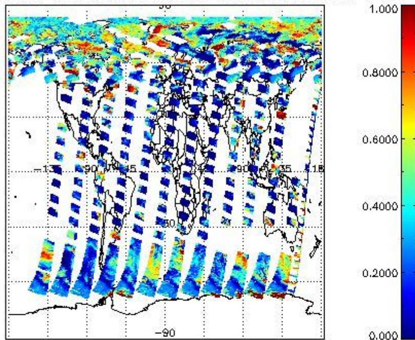
cL_frac for 15JUN2011 00:00:00 to 16JUN2011 00:00:00
