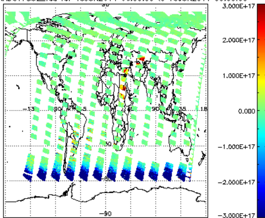
SCIOL2P_NADUV7S02_vcd for 15JUN2011 00:00:00 to 16JUN2011 00:00:00
