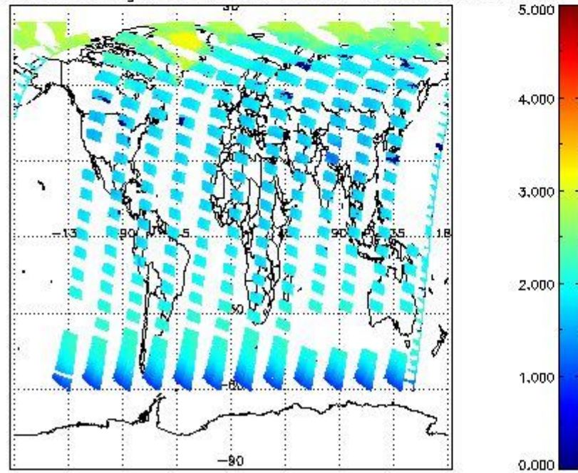
SCIOL2P_NADUV7S02_amf_gr for 15JUN2011 00:00:00 to 16JUN2011 00:00:00
