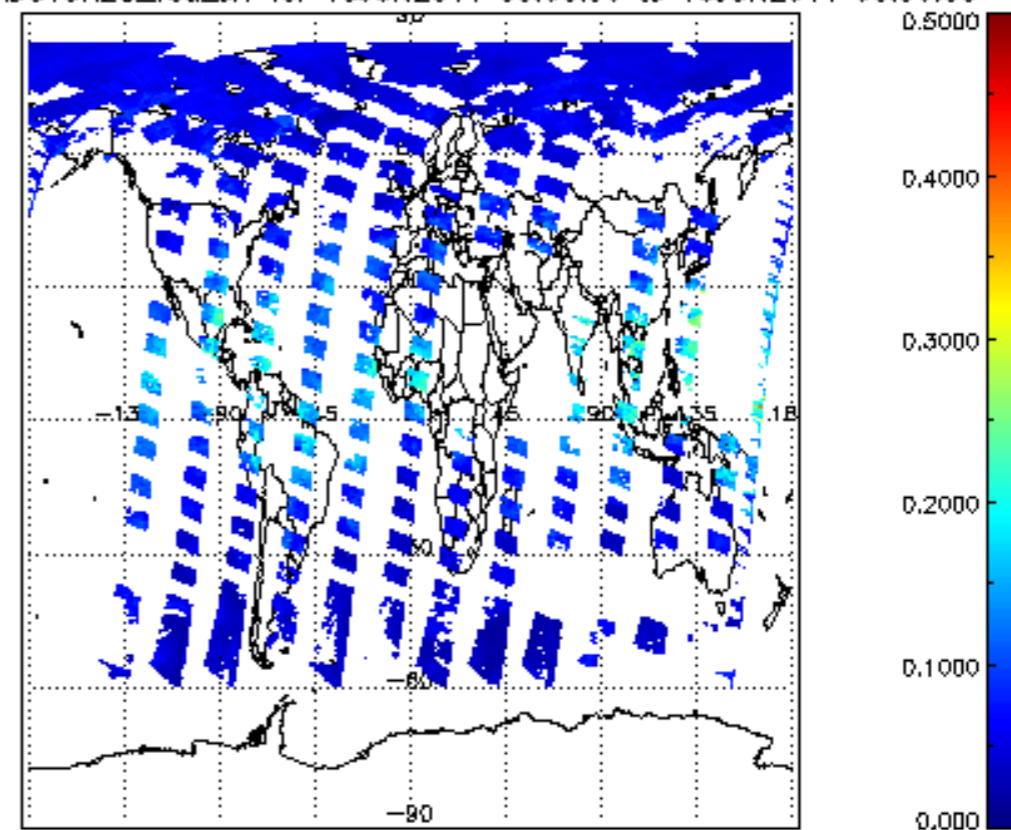
SCIOL2P_NADUV8H2O_vcd_err for 15JUN2011 00:00:00 to 16JUN2011 00:00:00
