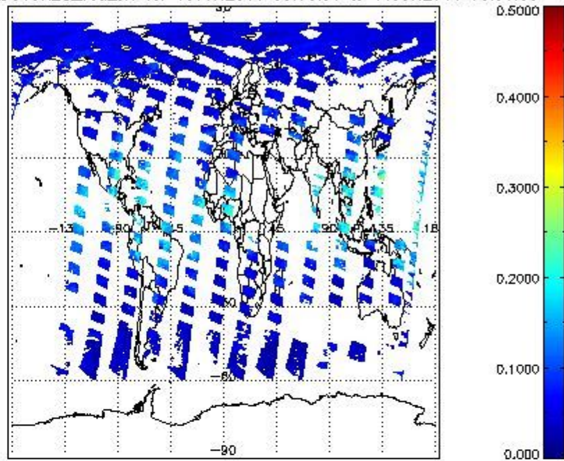
SCIOL2P_NADUV8H2O_vcd_err for 15JUN2011 00:00:00 to 16JUN2011 00:00:00
