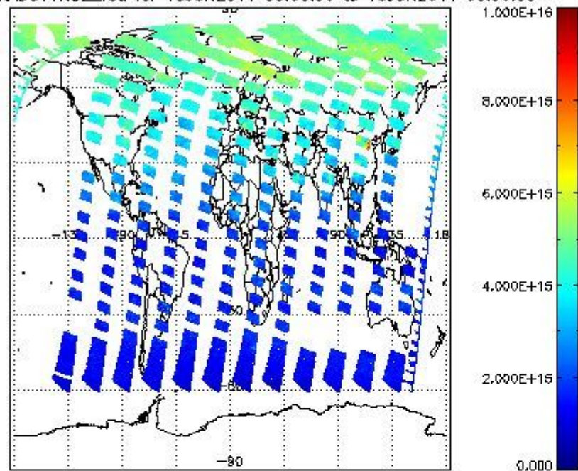
SCIOL2P_NADUV1NO2_vcd for 15JUN2011 00:00:00 to 16JUN2011 00:00:00
