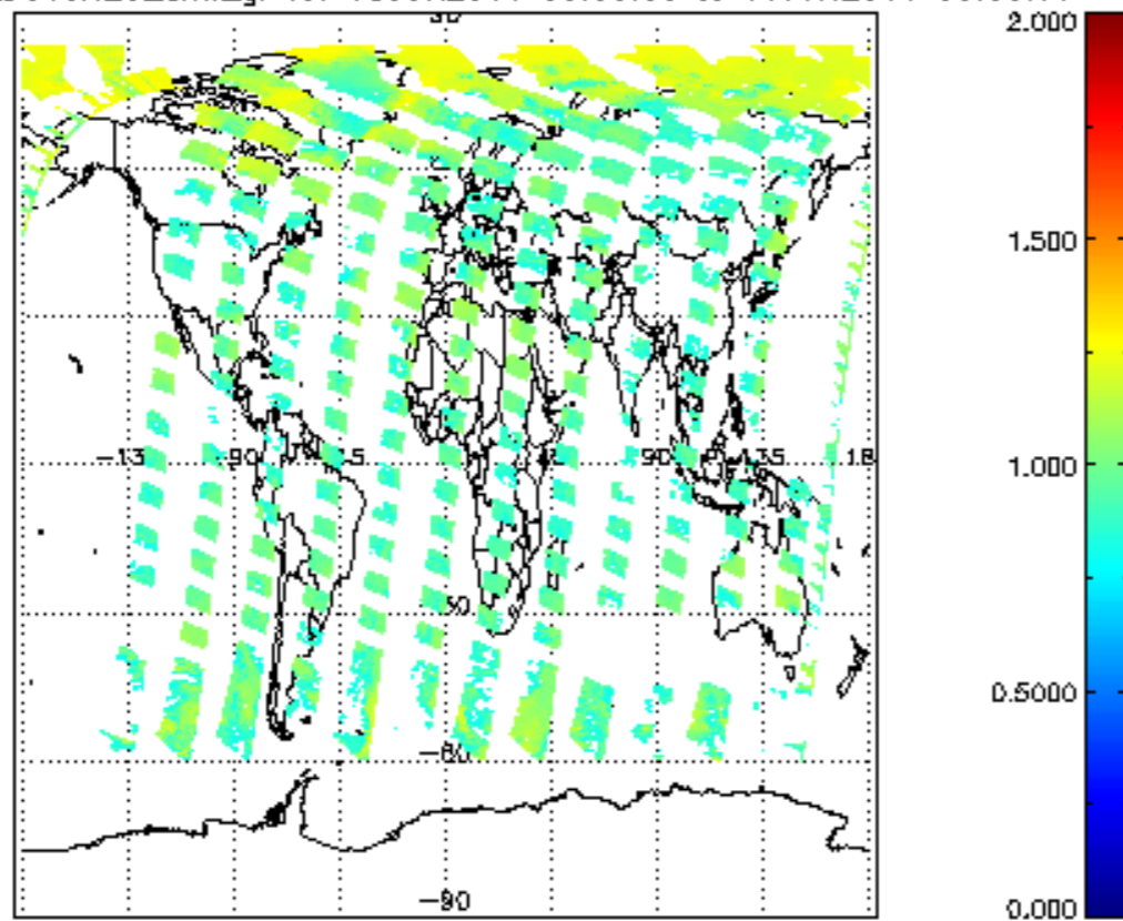
SCIOL2P_NADUV8H2O_amf_gr for 15JUN2011 00:00:00 to 16JUN2011 00:00:00
