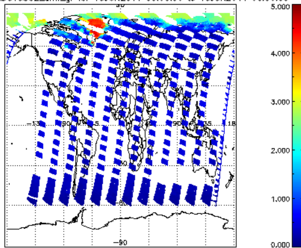
SCIOL2P_NADUV5S02_amf_gr for 15JUN2011 00:00:00 to 16JUN2011 00:00:00
