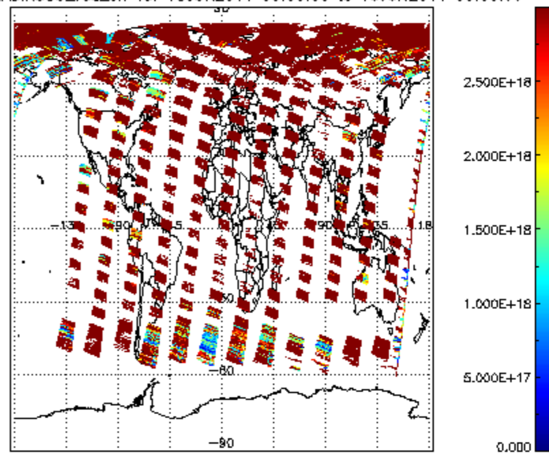
SCIOL2P_NADIR3CO_vcd_err for 15JUN2011 00:00:00 to 16JUN2011 00:00:00
