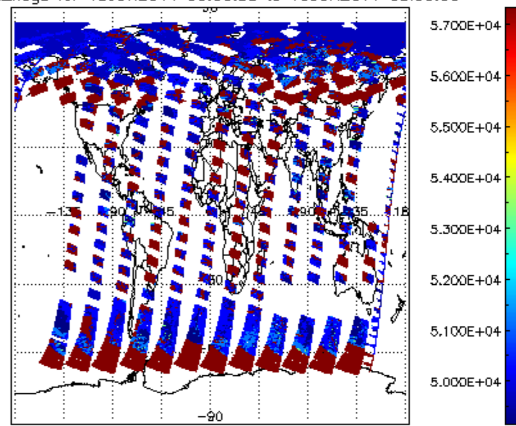
cloud_flags for 15JUN2011 00:00:00 to 16JUN2011 00:00:00
