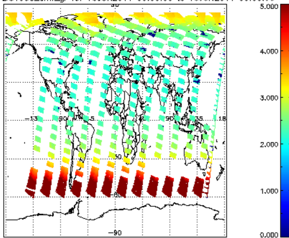
SCIOL2P_NADUV003_amf_gr for 15JUN2011 00:00:00 to 16JUN2011 00:00:00
