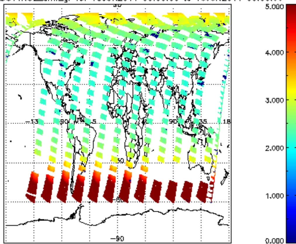
SCIOL2P_NADUV1NO2_amf_gr for 15JUN2011 00:00:00 to 16JUN2011 00:00:00
