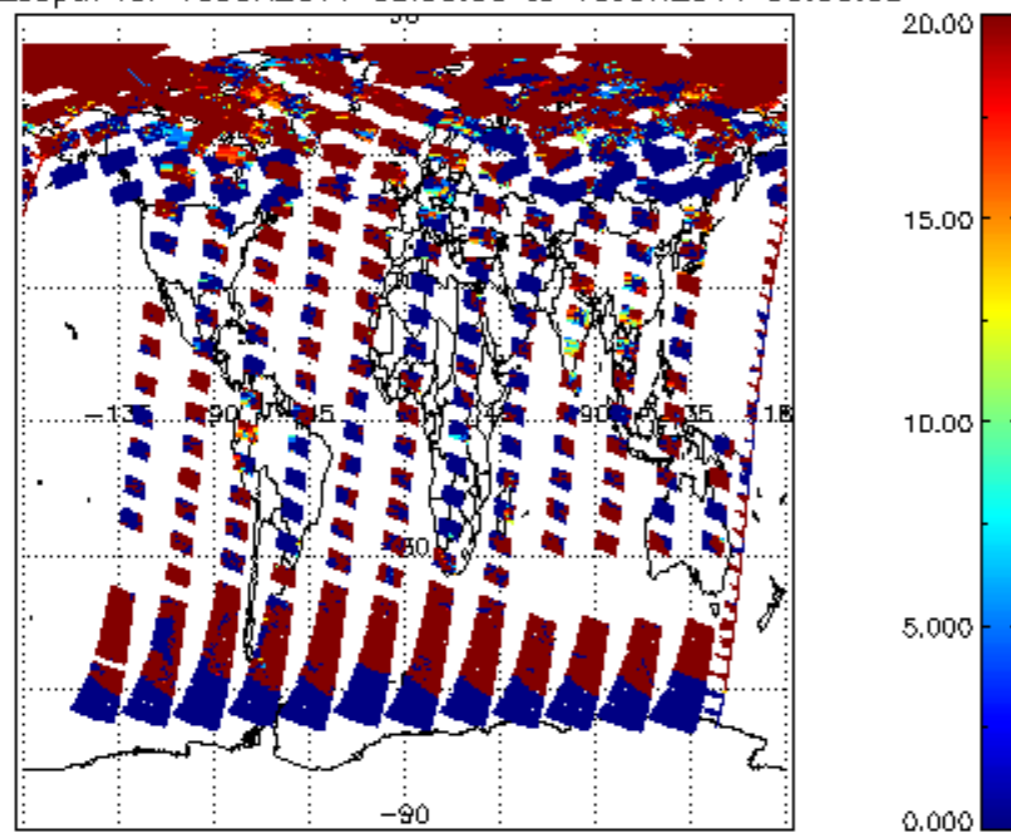
cl_opt_depth for 15JUN2011 00:00:00 to 16JUN2011 00:00:00
