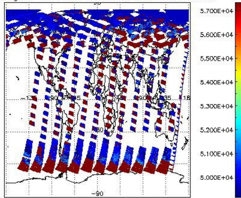
cloud_flags for 15JUN2011 00:00:00 to 16JUN2011 00:00:00
