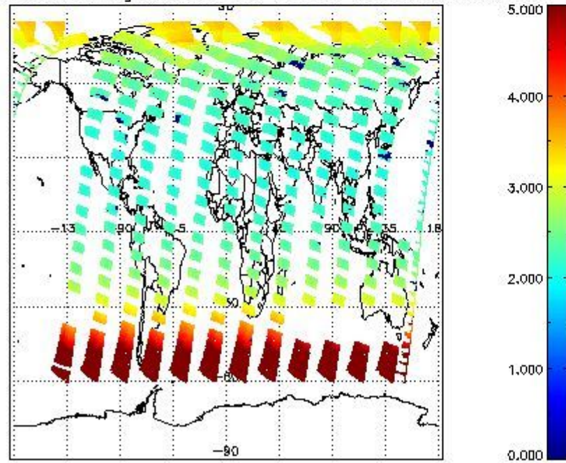
SCIOL2P_NADUV3BRO_amf_gr for 15JUN2011 00:00:00 to 16JUN2011 00:00:00
