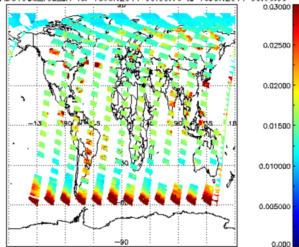
SCIOL2P_NADUV003_vcd_err for 15JUN2011 00:00:00 to 16JUN2011 00:00:00
