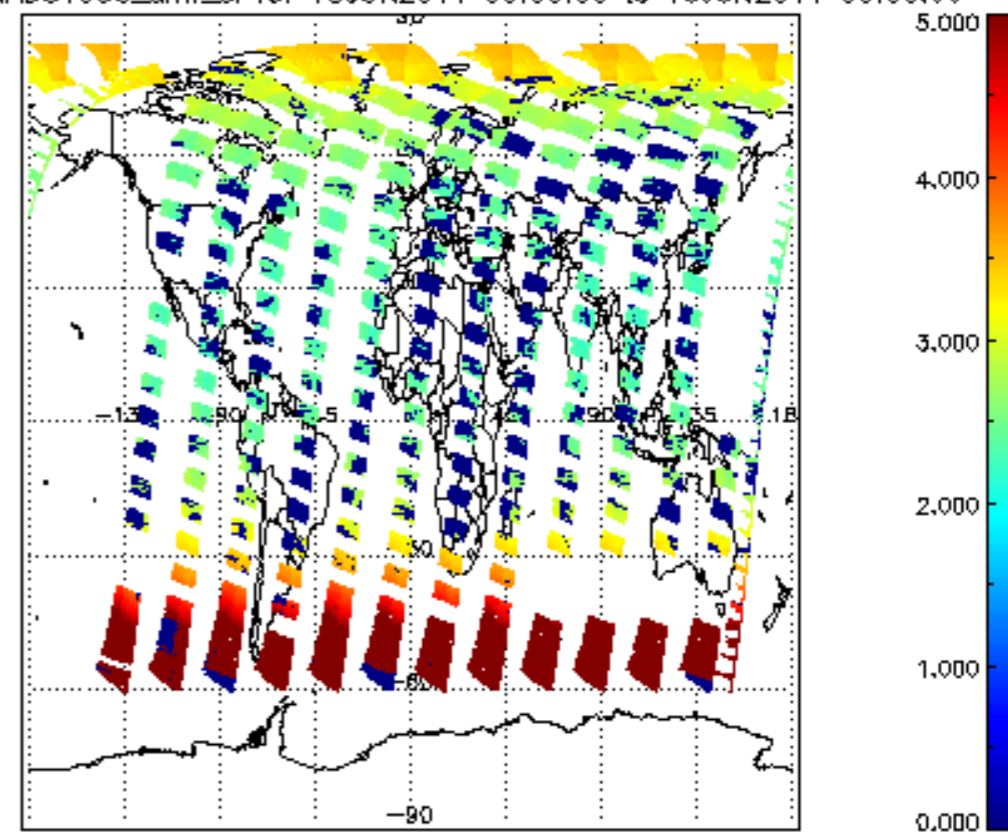
SCIOL2P_NADUV003_amf_cl for 15JUN2011 00:00:00 to 16JUN2011 00:00:00
