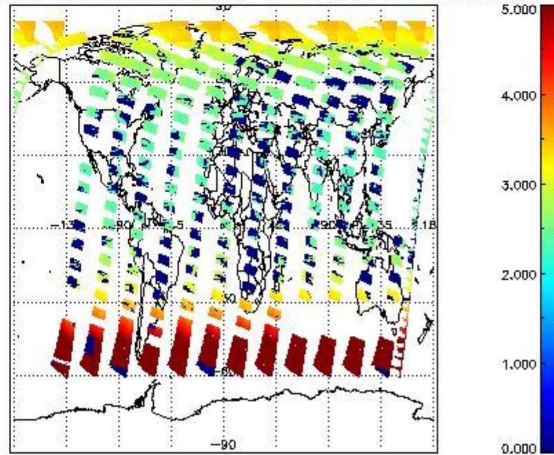
SCIOL2P_NADUV003_amf_cl for 15JUN2011 00:00:00 to 16JUN2011 00:00:00
