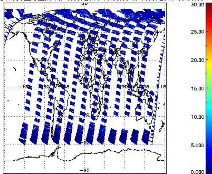
SCIOL2P_NADUV5S02_vcd_err for 15JUN2011 00:00:00 to 16JUN2011 00:00:00
