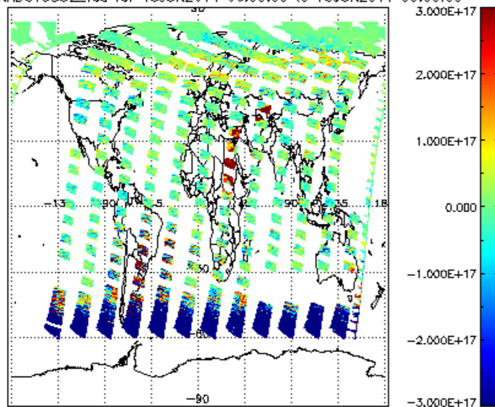
SCIOL2P_NADUV5S02_vcd for 15JUN2011 00:00:00 to 16JUN2011 00:00:00
