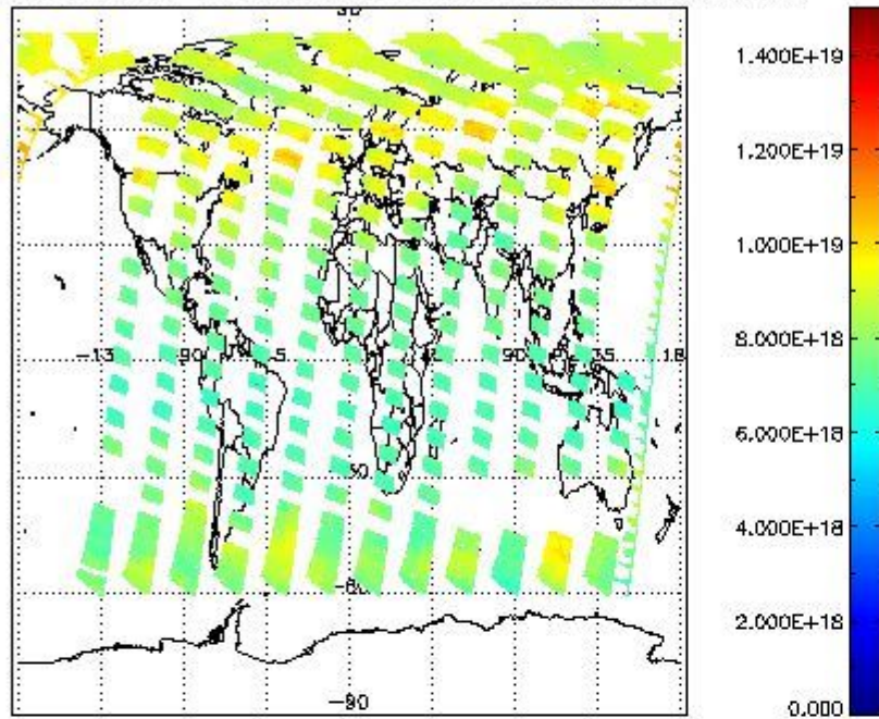
SCIOL2P_NADUV003_vcd for 15JUN2011 00:00:00 to 16JUN2011 00:00:00
