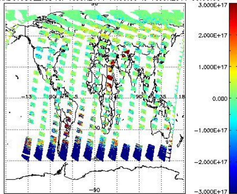
SCIOL2P_NADUV5S02_vcd for 15JUN2011 00:00:00 to 16JUN2011 00:00:00
