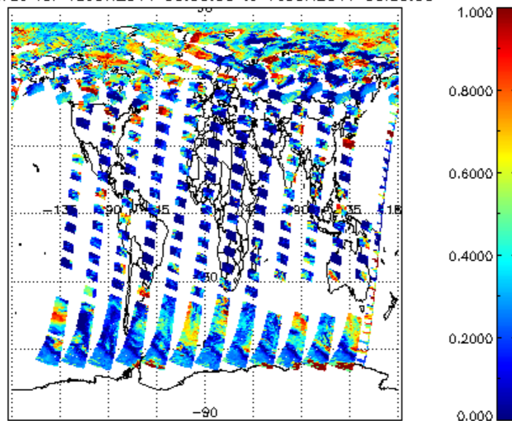
cl_frac for 15JUN2011 00:00:00 to 16JUN2011 00:00:00
