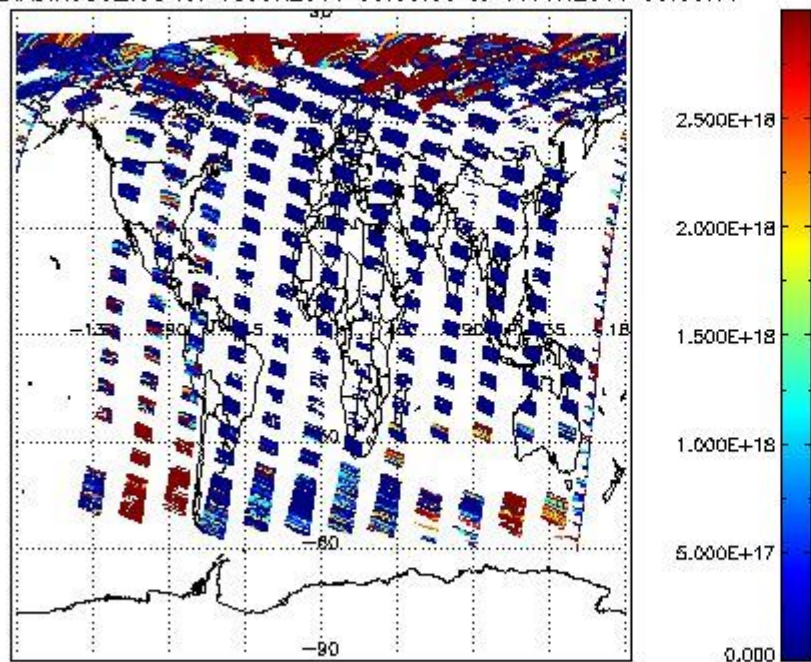
SCIO2P_NADIR3CO_vcd for 15JUN2011 00:00:00 to 16JUN2011 00:00:00
