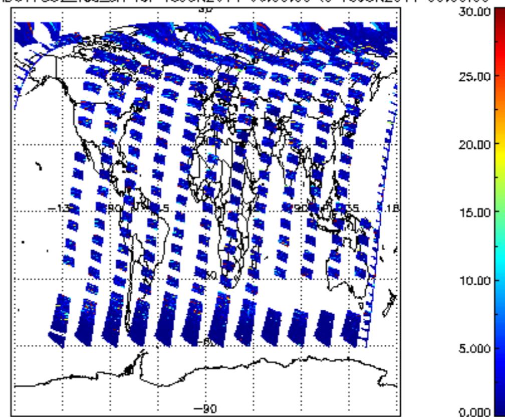
SCIOL2P_NADUV7S02_vcd_err for 15JUN2011 00:00:00 to 16JUN2011 00:00:00
