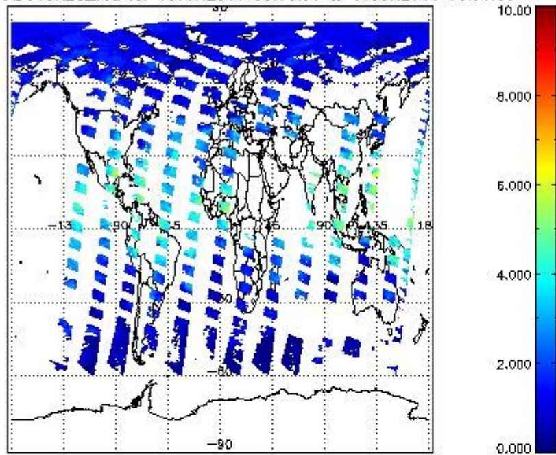
SCIOL2P_NADUV8H2O_vcd for 15JUN2011 00:00:00 to 16JUN2011 00:00:00
