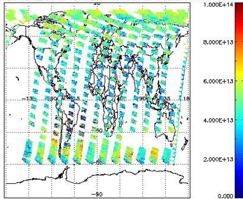
SCIOL2P_NADUV3BRO_vcd for 15JUN2011 00:00:00 to 16JUN2011 00:00:00
