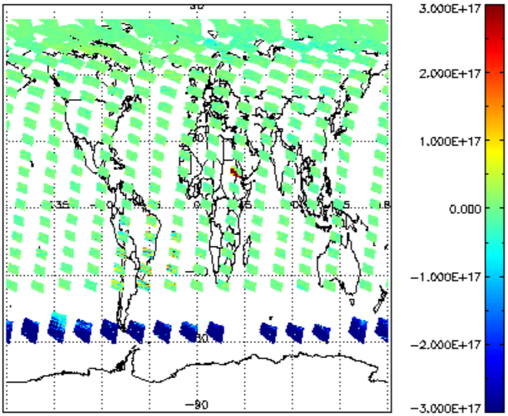
SCIOL2P_NADUV7S02_vcd for 13JUN2011 00:00:00 to 14JUN2011 00:00:00
