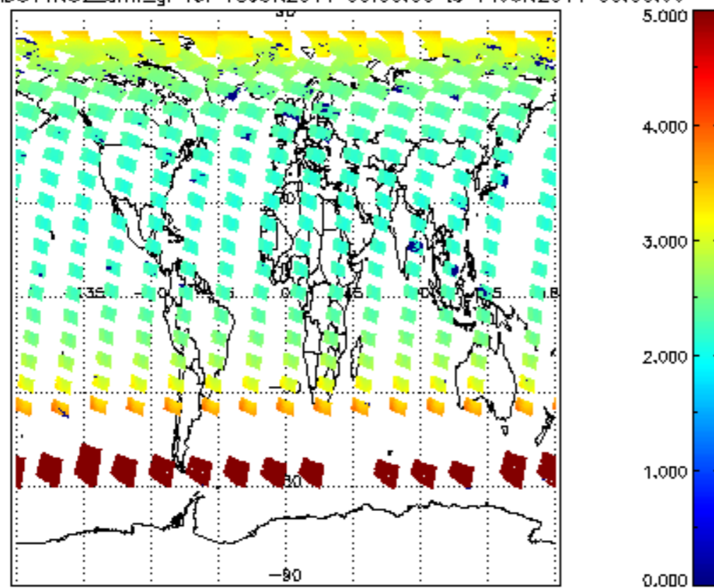
SCIOL2P_NADUV1NO2_amf_gr for 13JUN2011 00:00:00 to 14JUN2011 00:00:00
