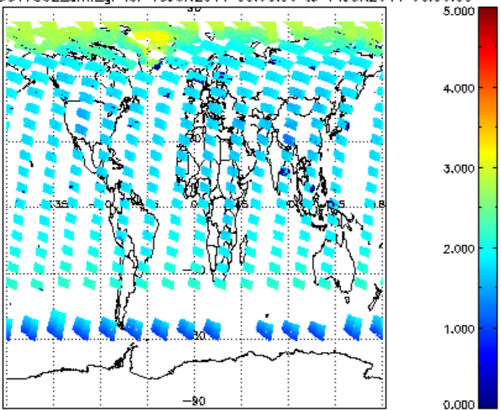
SCIOL2P_NADUV7S02_amf_gr for 13JUN2011 00:00:00 to 14JUN2011 00:00:00
