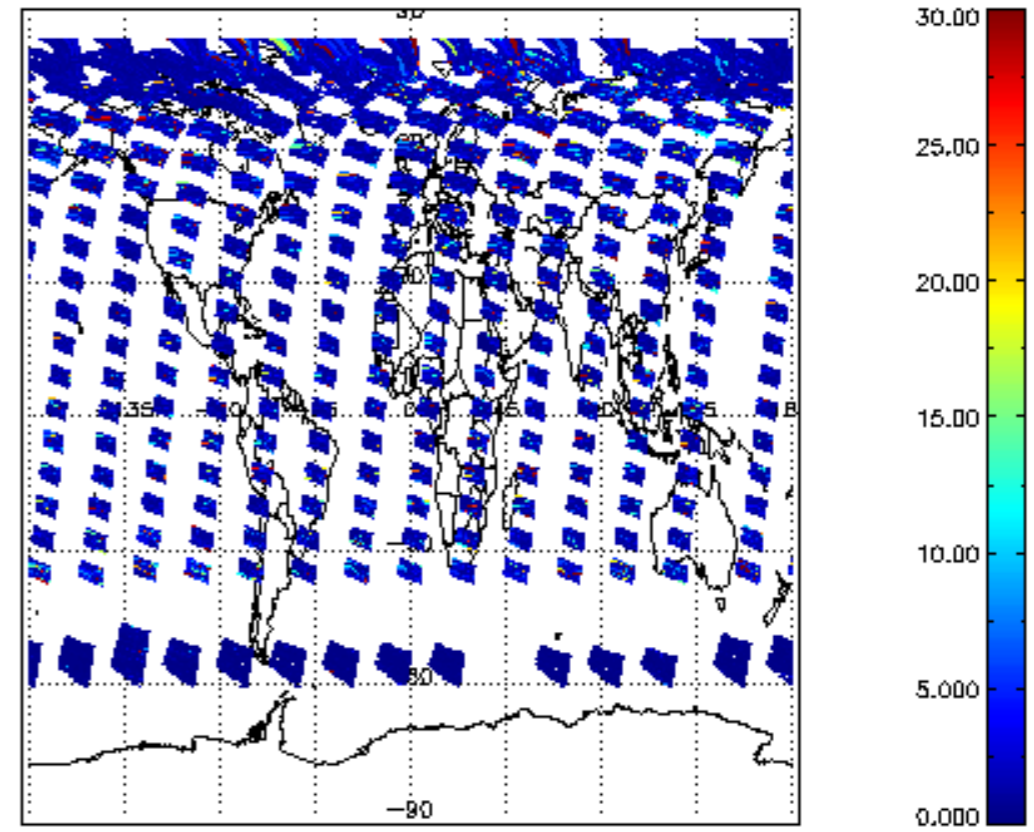
SCIOL2P_NADUV7S02_vcd_err for 13JUN2011 00:00:00 to 14JUN2011 00:00:00
