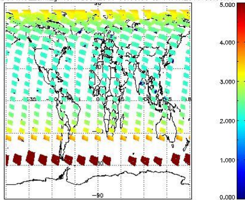
SCIOL2P_NADUV1N02_amf_gr for 13JUN2011 00:00:00 to 14JUN2011 00:00:00
