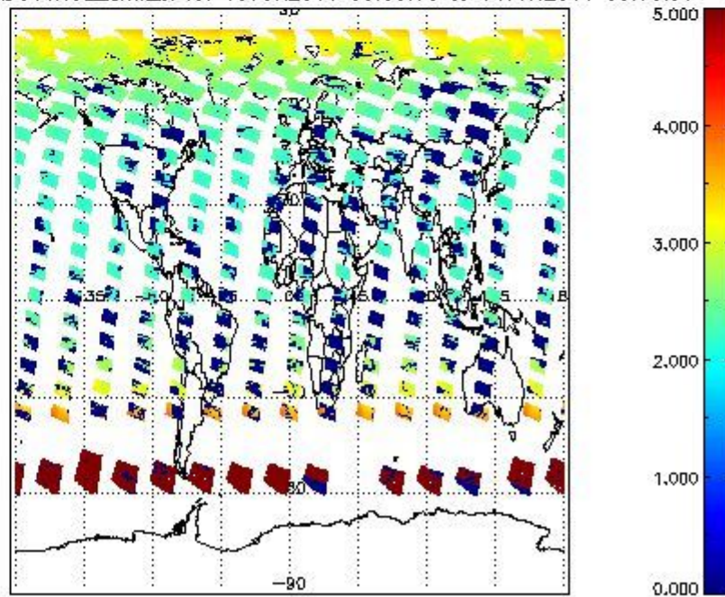
SCIOL2P_NADUV1N02_amf_cl for 13JUN2011 00:00:00 to 14JUN2011 00:00:00
