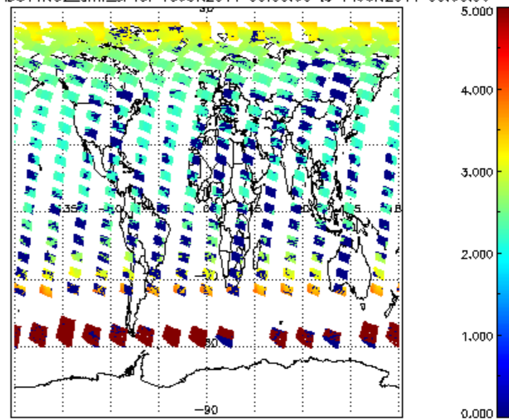
SCIOL2P_NADUV1NO2_amf_sl for 13JUN2011 00:00:00 to 14JUN2011 00:00:00
