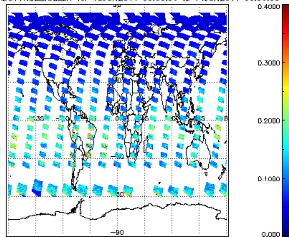
SCIOL2P_NADUV1NO2_vcd_err for 13JUN2011 00:00:00 to 14JUN2011 00:00:00
