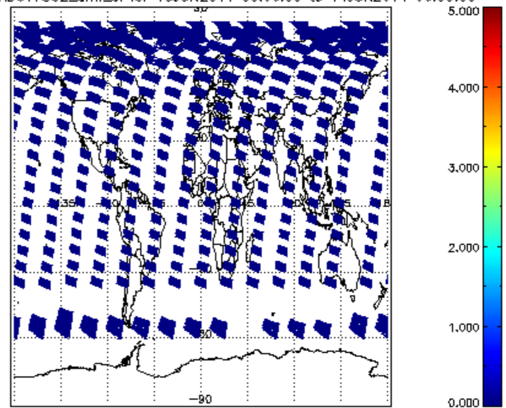
SCIOL2P_NADUV7S02_amf_cl for 13JUN2011 00:00:00 to 14JUN2011 00:00:00
