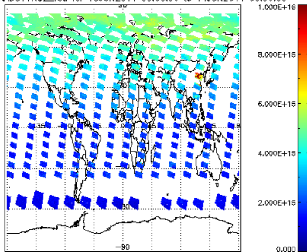
SCIOL2P_NADUV1NO2_vcd for 13JUN2011 00:00:00 to 14JUN2011 00:00:00
