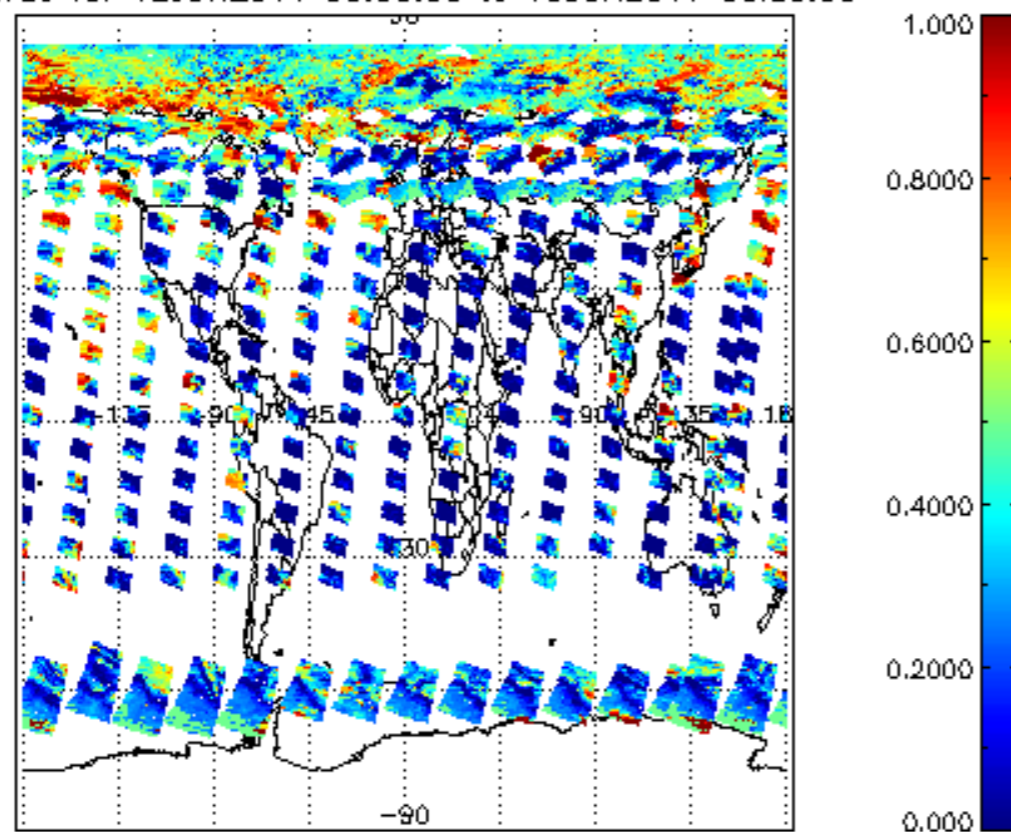
cl_frac for 12JUN2011 00:00:00 to 13JUN2011 00:00:00
