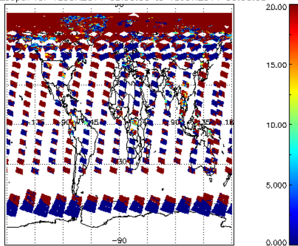
cl_opt_depth for 12JUN2011 00:00:00 to 13JUN2011 00:00:00
