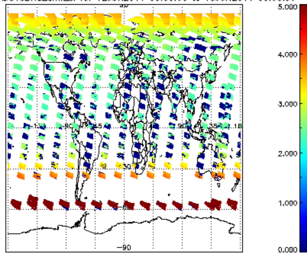
SCIOL2P_NADUV3BRO_amf_sl for 12JUN2011 00:00:00 to 13JUN2011 00:00:00
