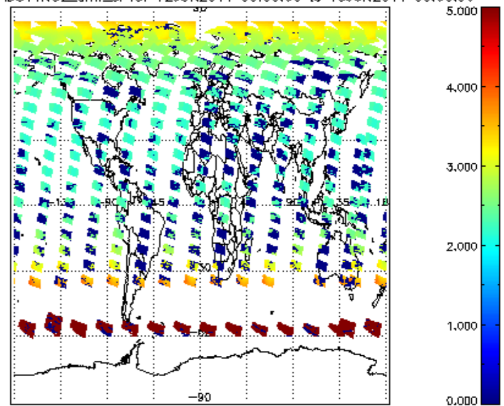
SCIOL2P_NADUV1NO2_amf_sl for 12JUN2011 00:00:00 to 13JUN2011 00:00:00
