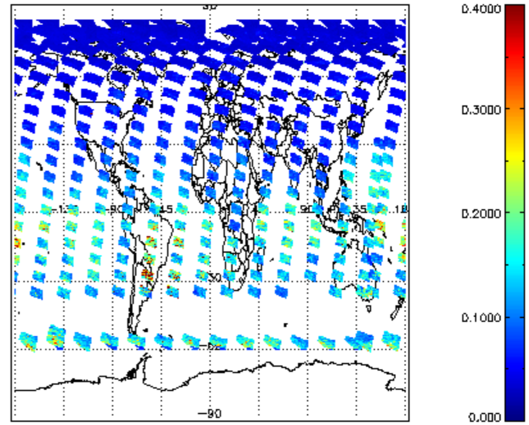
SCIOL2P_NADUV1NO2_vcd_err for 12JUN2011 00:00:00 to 13JUN2011 00:00:00
