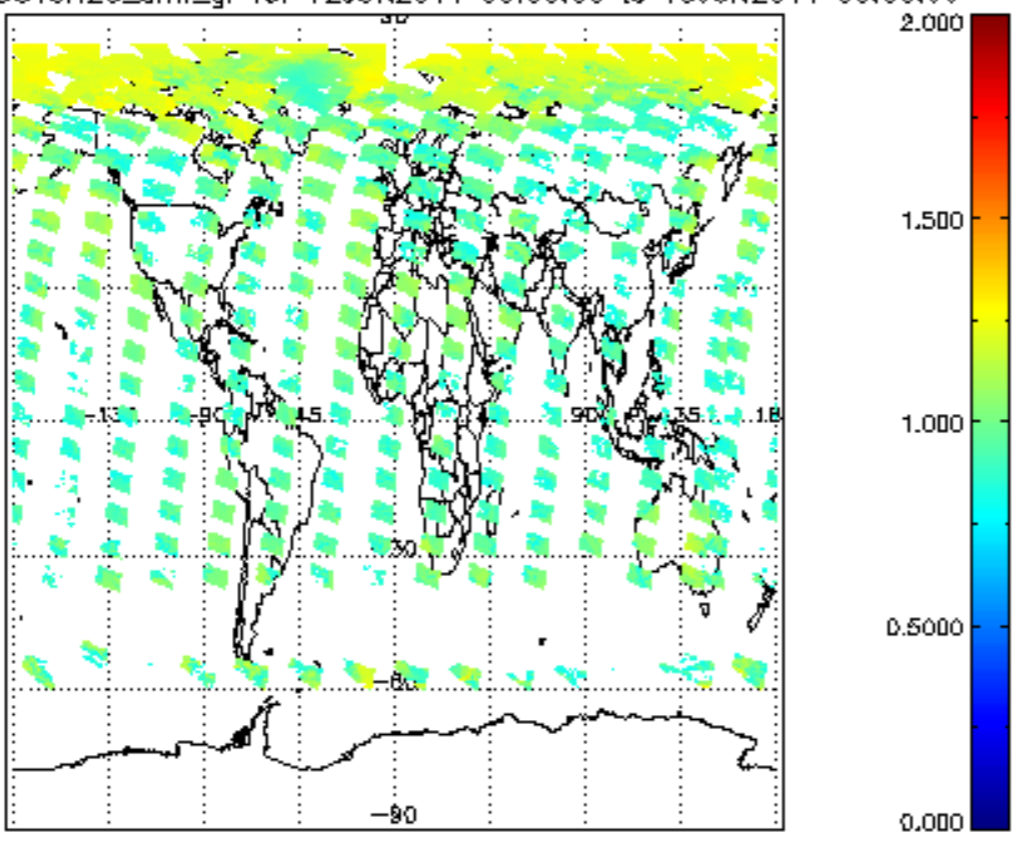
SCIOL2P_NADUV8H2O_amf_gr for 12JUN2011 00:00:00 to 13JUN2011 00:00:00
