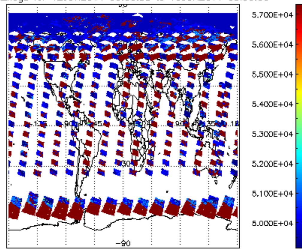
cloud_flags for 12JUN2011 00:00:00 to 13JUN2011 00:00:00
