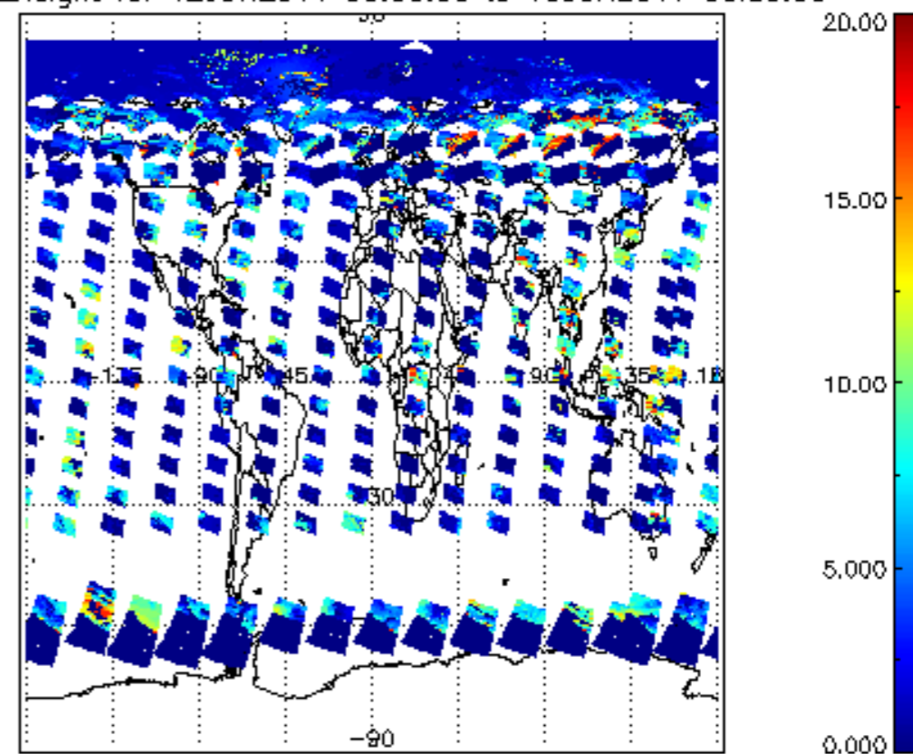
cl_top_height for 12JUN2011 00:00:00 to 13JUN2011 00:00:00
