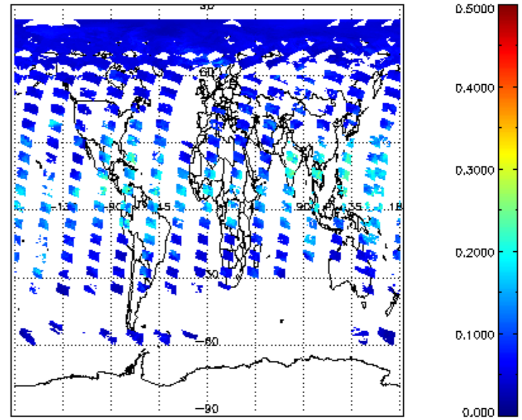
SCIOL2P_NADUV8H2O_vcd_err for 12JUN2011 00:00:00 to 13JUN2011 00:00:00
