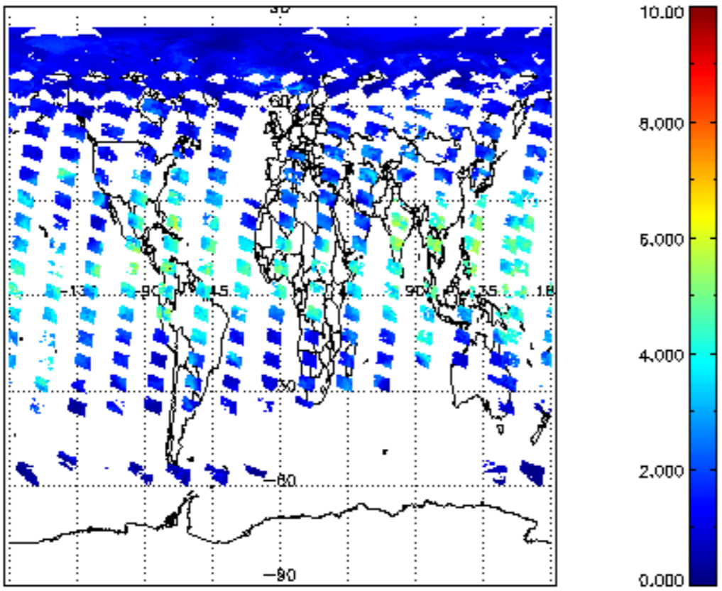
SCIOL2P_NADUV8H2O_vcd for 12JUN2011 00:00:00 to 13JUN2011 00:00:00
