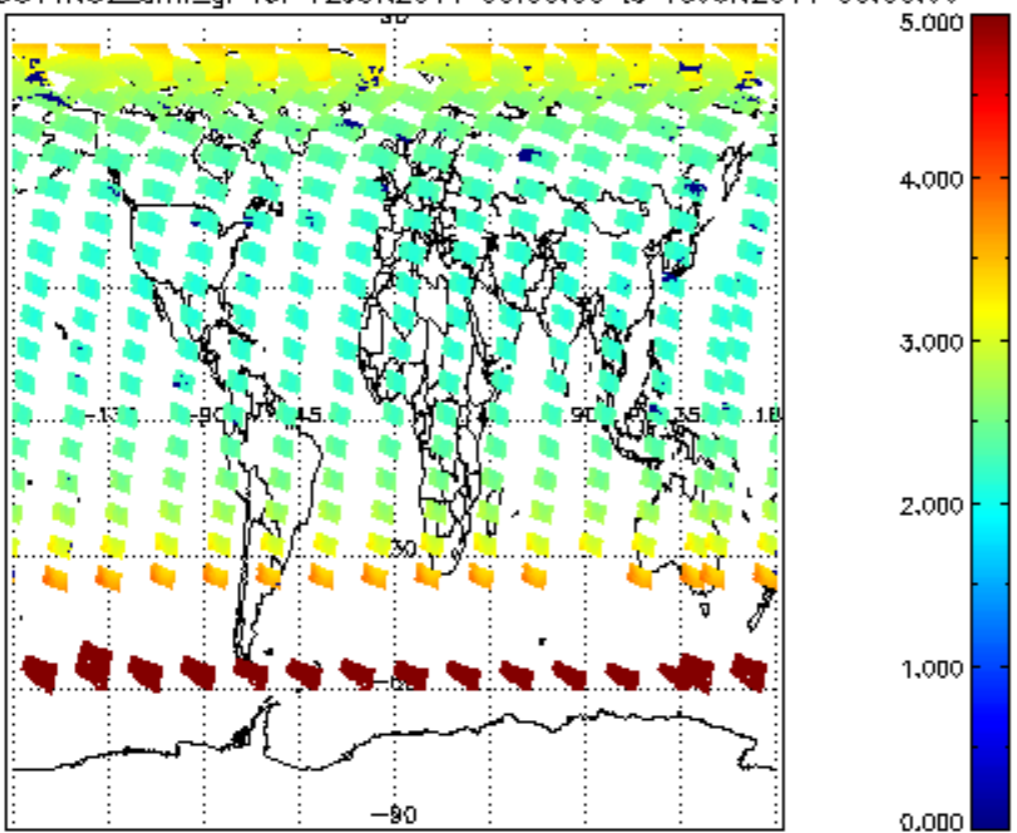
SCIOL2P_NADUV1NO2_amf_gr for 12JUN2011 00:00:00 to 13JUN2011 00:00:00
