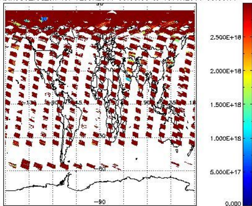
SCIO2P_NADIR3CO_vcd_err for 12JUN2011 00:00:00 to 13JUN2011 00:00:00
