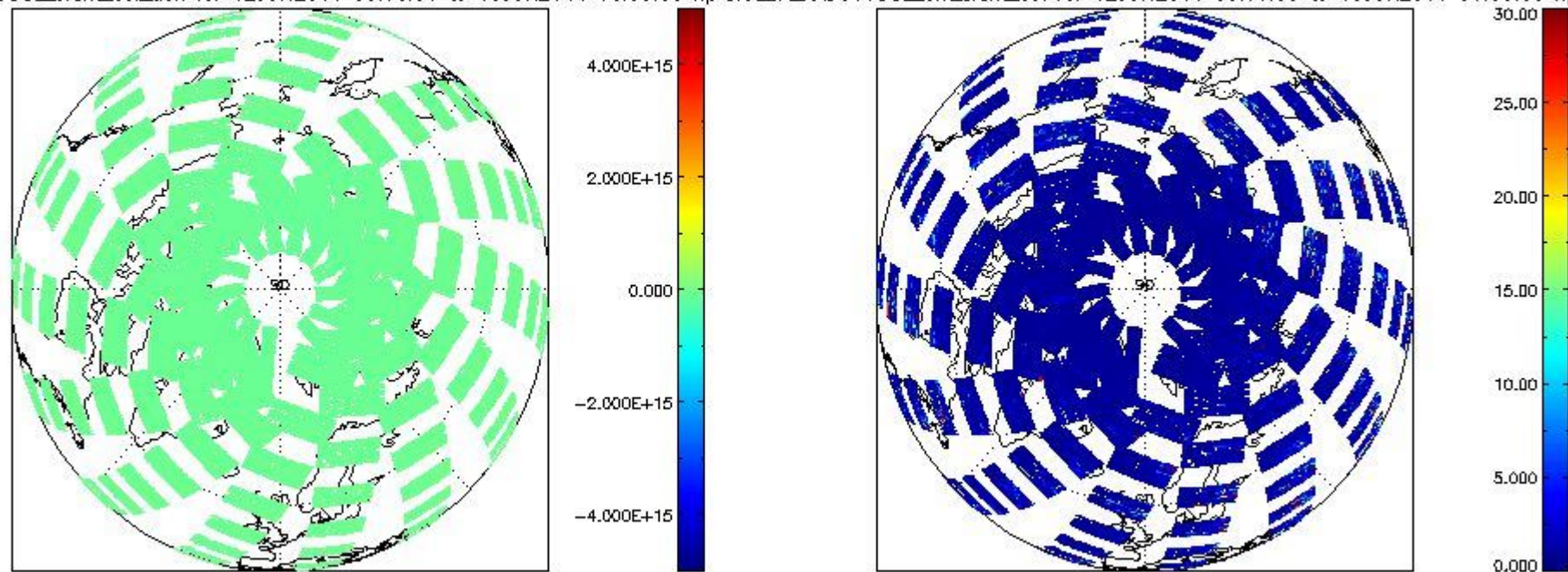
CIOL2P_NADUV6OCL_slant_col_den for 12JUN2011 00:00:00 to 13JUN2011 00:00:00 np; CIOL2P_NADUV6OCL_err_slant_col for 12JUN2011 00:00:00 to 13JUN2011 00:00:00 np
