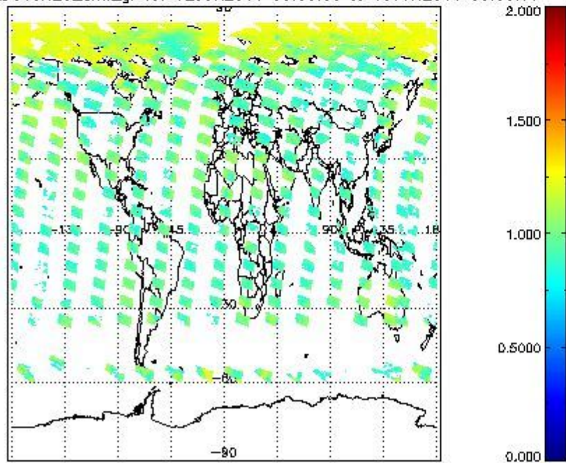
SCIOL2P_NADUV8H2O_amf_gr for 12JUN2011 00:00:00 to 13JUN2011 00:00:00
