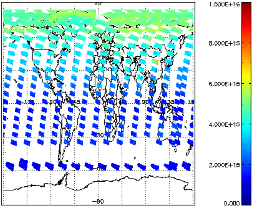
SCIOL2P_NADUV1NO2_vcd for 12JUN2011 00:00:00 to 13JUN2011 00:00:00
