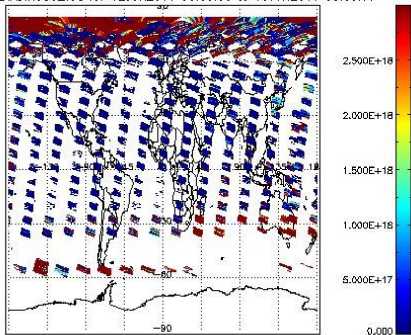
SCIO2P_NADIR3CO_vcd for 12JUN2011 00:00:00 to 13JUN2011 00:00:00
