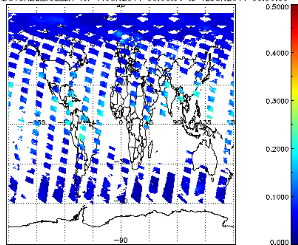
SCIOL2P_NADUV8H2O_vcd_err for 11JUN2011 00:00:00 to 12JUN2011 00:00:00
