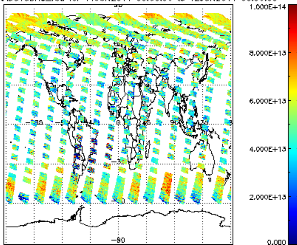
SCIOL2P_NADUV3BRO_vcd for 11JUN2011 00:00:00 to 12JUN2011 00:00:00
