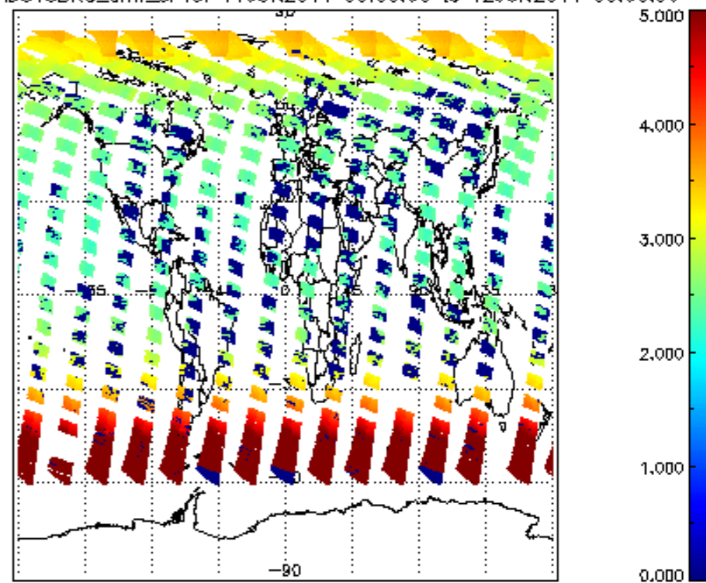
SCIOL2P_NADUV3BRO_amf_cl for 11JUN2011 00:00:00 to 12JUN2011 00:00:00
