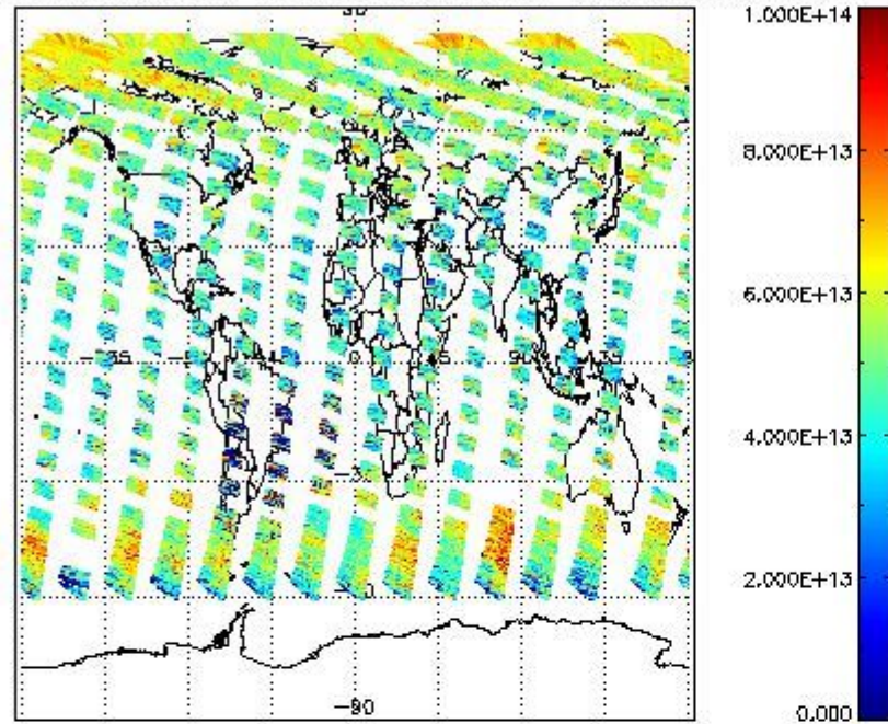
SCIOL2P_NADUV3BRO_vcd for 11JUN2011 00:00:00 to 12JUN2011 00:00:00
