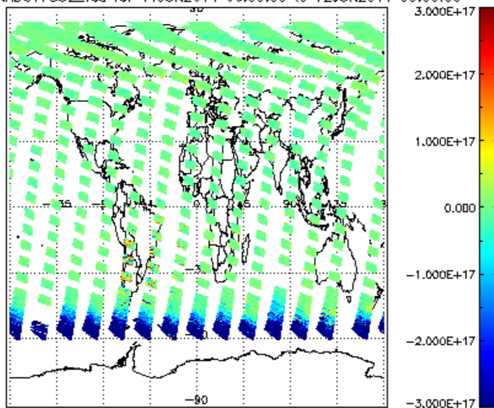
SCIOL2P_NADUV7S02_vcd for 11JUN2011 00:00:00 to 12JUN2011 00:00:00
