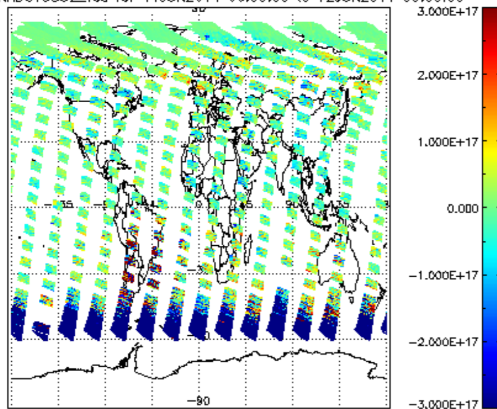
SCIOL2P_NADUV5S02_vcd for 11JUN2011 00:00:00 to 12JUN2011 00:00:00
