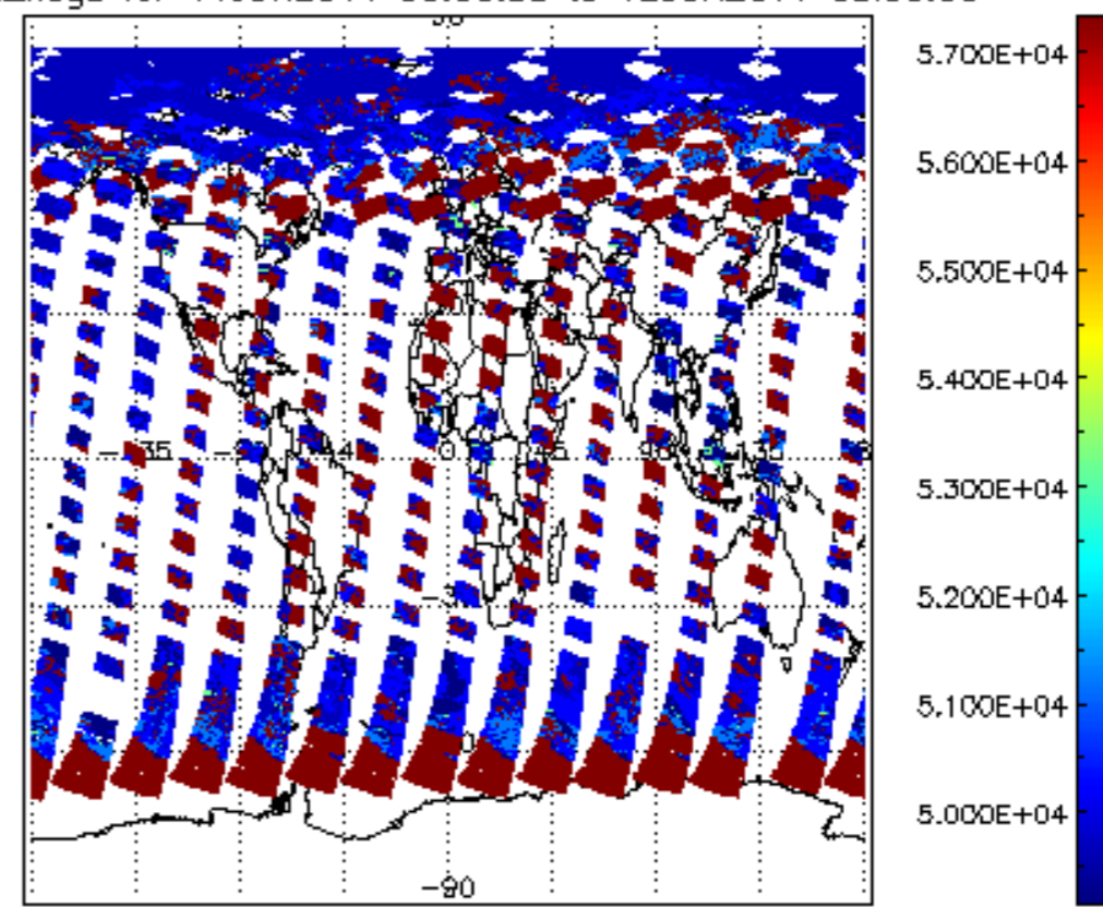
cloud_flags for 11JUN2011 00:00:00 to 12JUN2011 00:00:00
