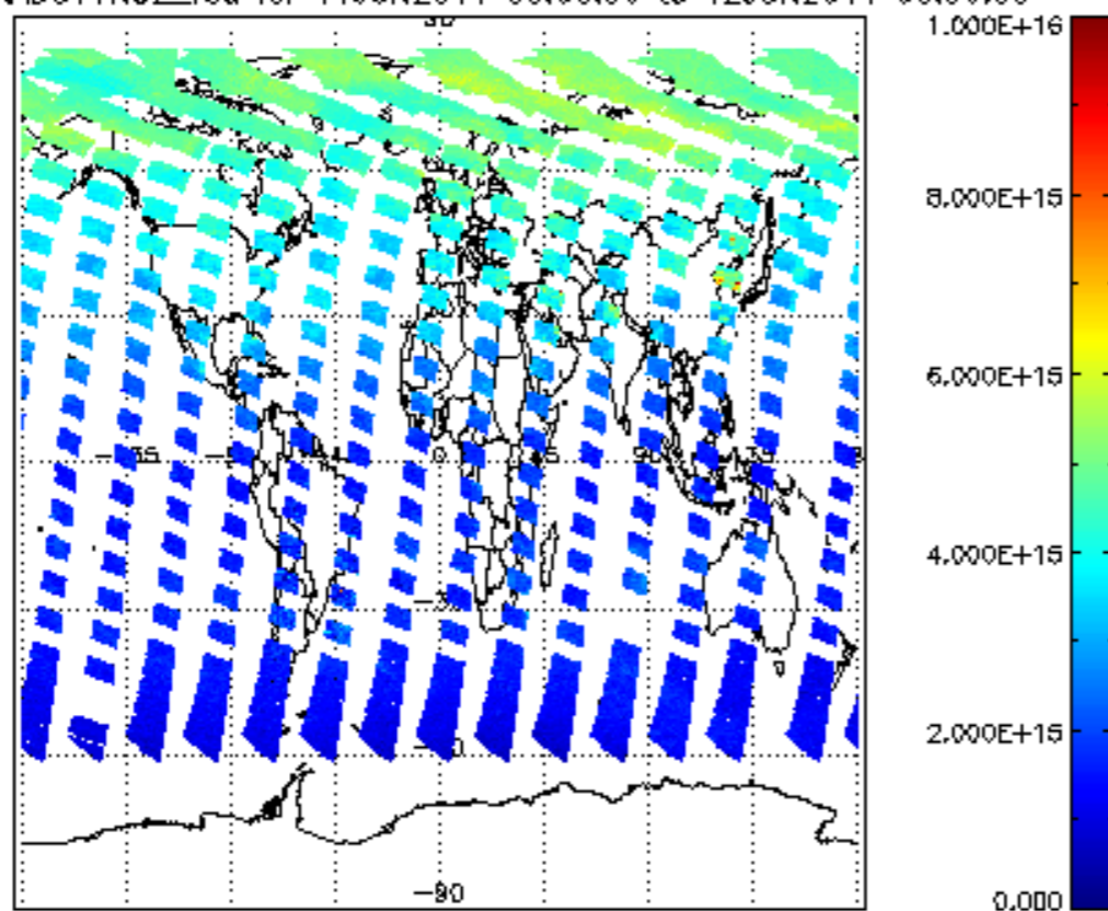
SCIOL2P_NADUV1NO2_vcd for 11JUN2011 00:00:00 to 12JUN2011 00:00:00
