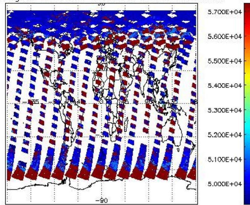
cloud_flags for 11JUN2011 00:00:00 to 12JUN2011 00:00:00
