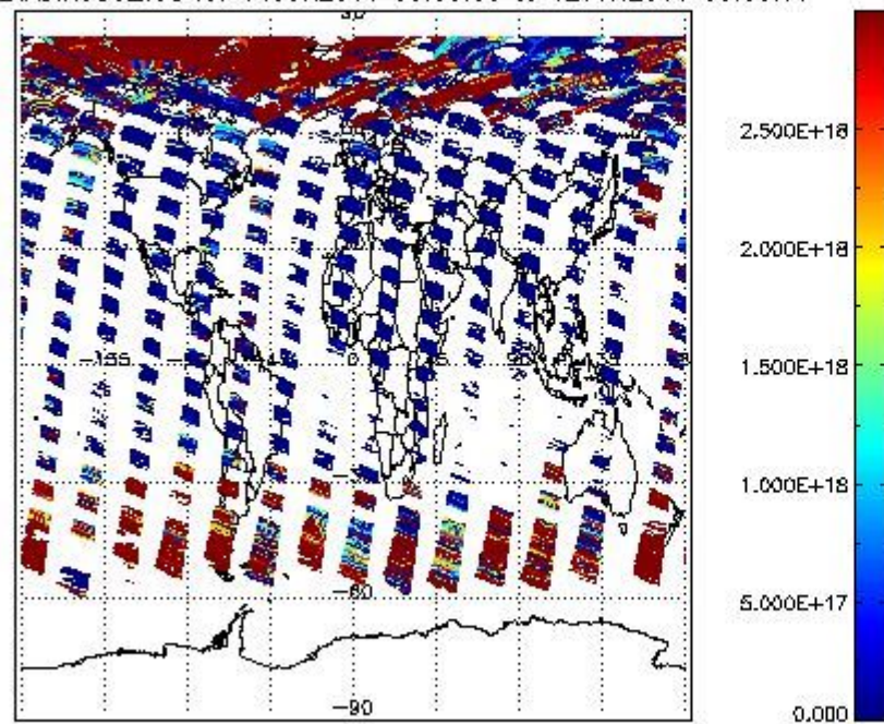
SCIO2P_NADIR3CO_vcd for 11JUN2011 00:00:00 to 12JUN2011 00:00:00
