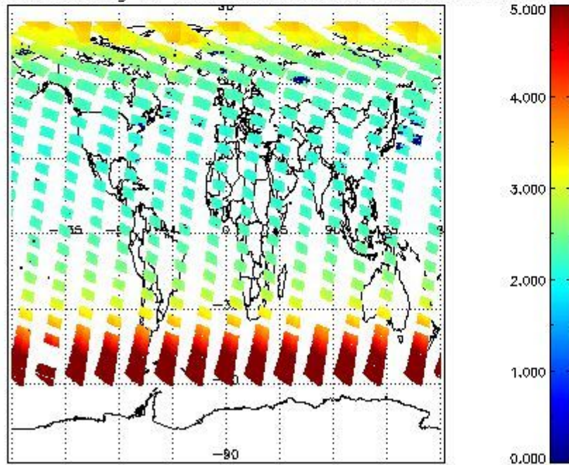
SCIOL2P_NADUV003_amf_gr for 11JUN2011 00:00:00 to 12JUN2011 00:00:00
