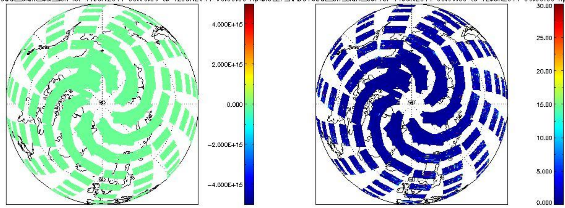
CIOL2P_NADUV60CLslant_col_den for 11JUN2011 00:00:00 to 12JUN2011 00:00:00 np; CIOL2P_NADUV60CLerr_slant_col for 11JUN2011 00:00:00 to 12JUN2011 00:00:00 np
