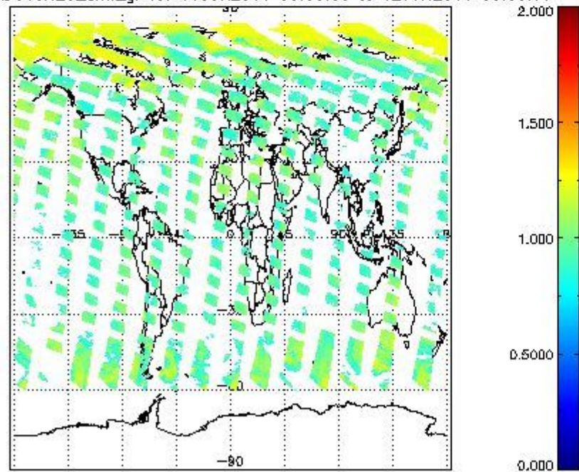
SCIOL2P_NADUV8H2O_arnf_gr for 11JUN2011 00:00:00 to 12JUN2011 00:00:00
