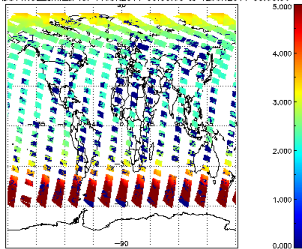
SCIOL2P_NADUV1NO2_amf_sl for 11JUN2011 00:00:00 to 12JUN2011 00:00:00
