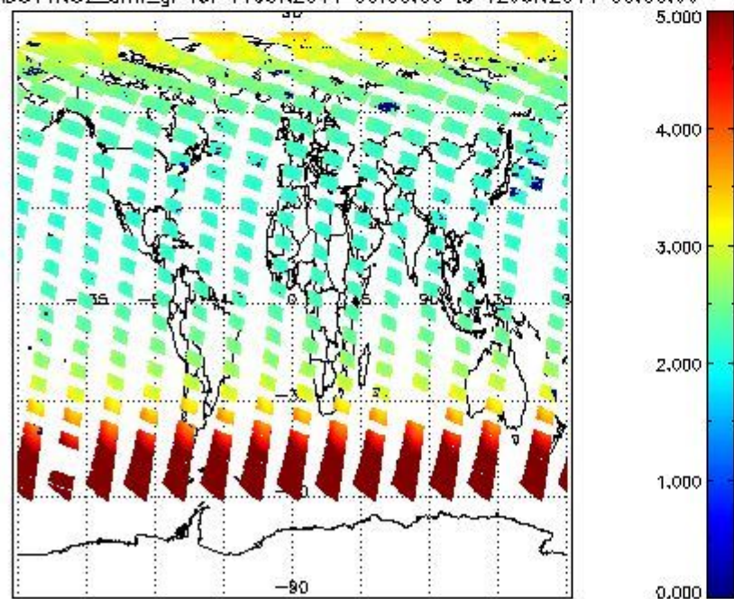
SCIOL2P_NADUV1NO2_amf_gr for 11JUN2011 00:00:00 to 12JUN2011 00:00:00
