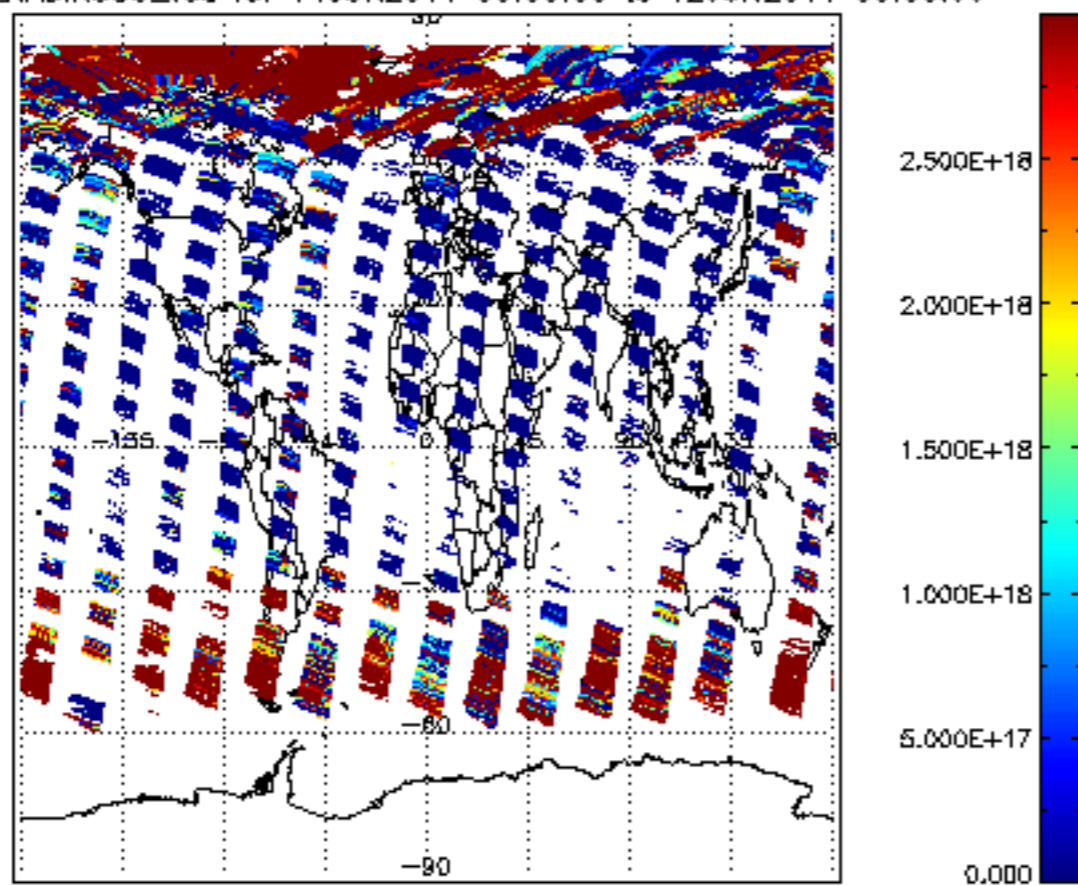
SCIOL2P_NADIR3CO_vcd for 11JUN2011 00:00:00 to 12JUN2011 00:00:00
