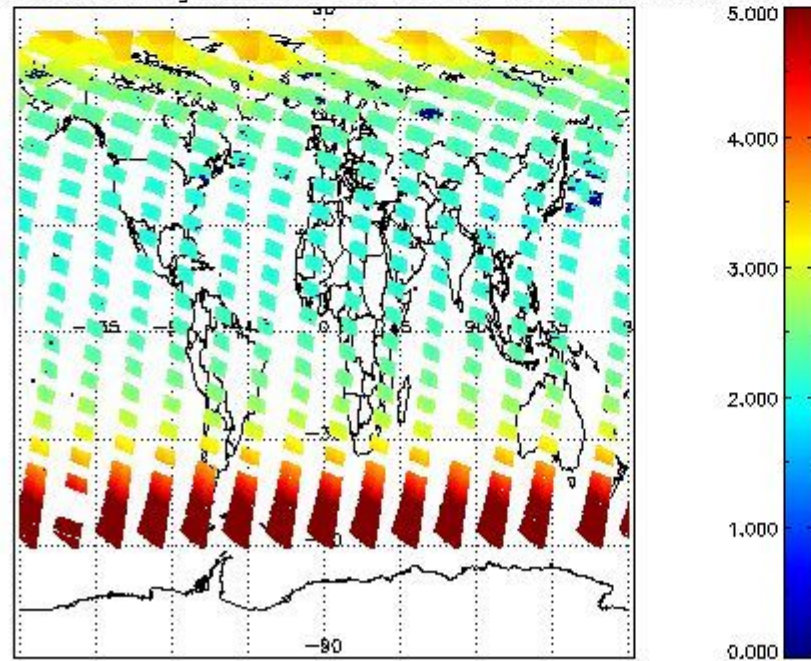
SCIOL2P_NADUV3BRO_amf_gr for 11JUN2011 00:00:00 to 12JUN2011 00:00:00
