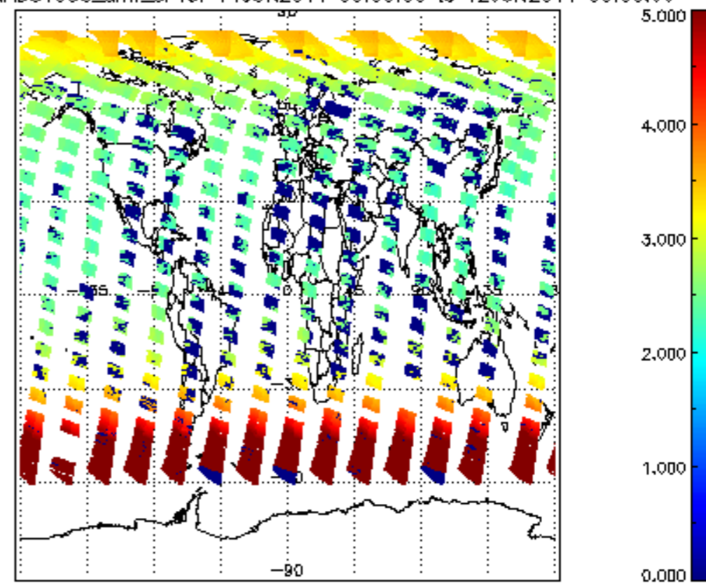
SCIOL2P_NADUV003_amf_cl for 11JUN2011 00:00:00 to 12JUN2011 00:00:00
