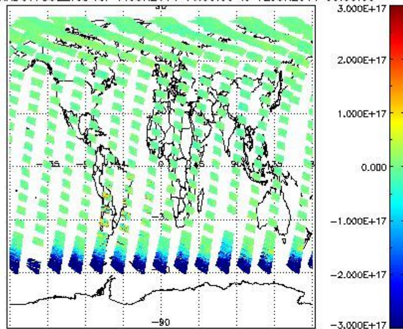
SCIOL2P_NADUV7S02_vcd for 11JUN2011 00:00:00 to 12JUN2011 00:00:00
