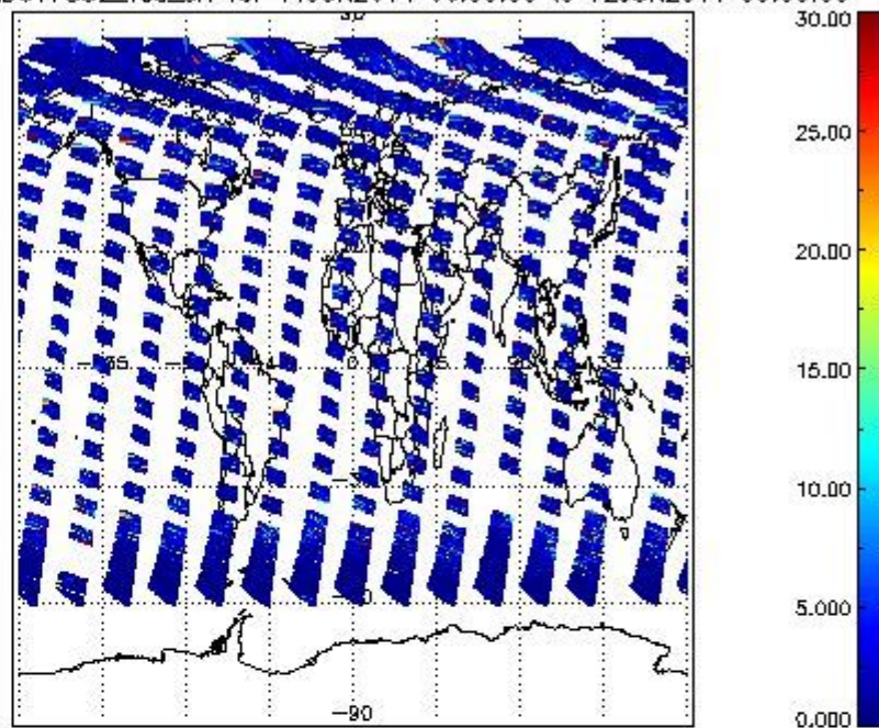
SCIOL2P_NADUV7S02_vcd_err for 11JUN2011 00:00:00 to 12JUN2011 00:00:00
