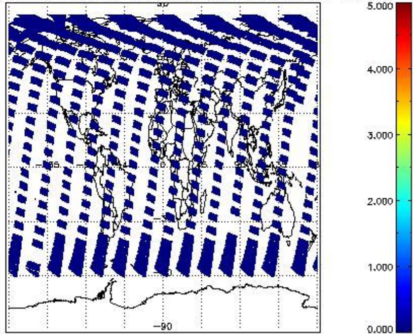
SCIOL2P_NADUV5S02_amf_cl for 11JUN2011 00:00:00 to 12JUN2011 00:00:00
