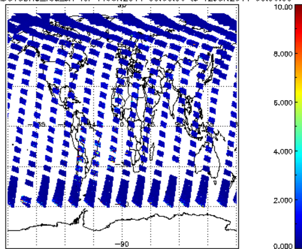
SCIOL2P_NADUV3BRO_vcd_err for 11JUN2011 00:00:00 to 12JUN2011 00:00:00
