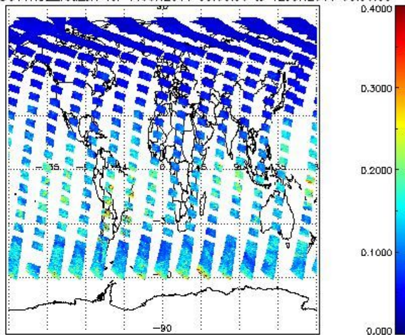
SCIOL2P_NADUV1NO2_vcd_err for 11JUN2011 00:00:00 to 12JUN2011 00:00:00
