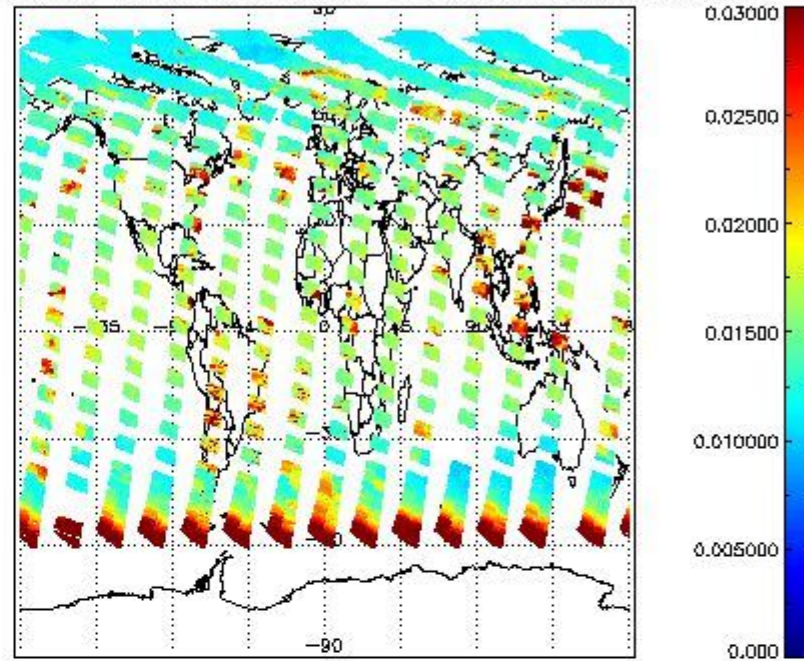
SCIOL2P_NADUV003_vcd_err for 11JUN2011 00:00:00 to 12JUN2011 00:00:00
