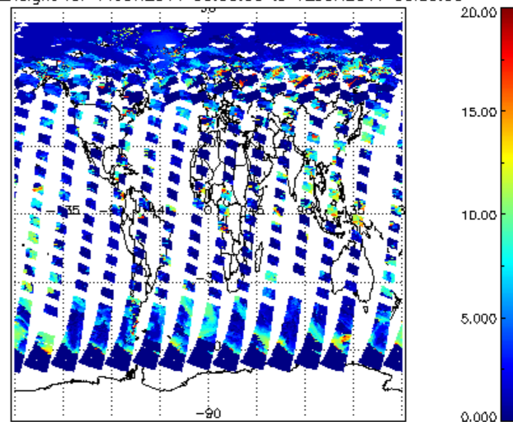
cl_top_height for 11JUN2011 00:00:00 to 12JUN2011 00:00:00
