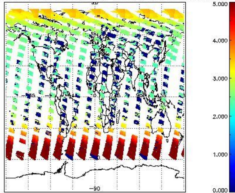
SCIOL2P_NADUV003_amf_cl for 11JUN2011 00:00:00 to 12JUN2011 00:00:00
