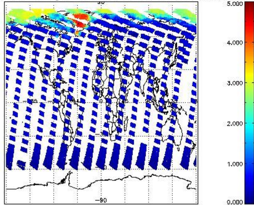
SCIOL2P_NADUV5S02_amf_gr for 11JUN2011 00:00:00 to 12JUN2011 00:00:00
