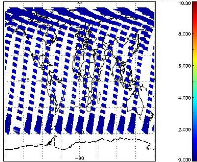
SCIOL2P_NADUV3BRO_vcd_err for 11JUN2011 00:00:00 to 12JUN2011 00:00:00
