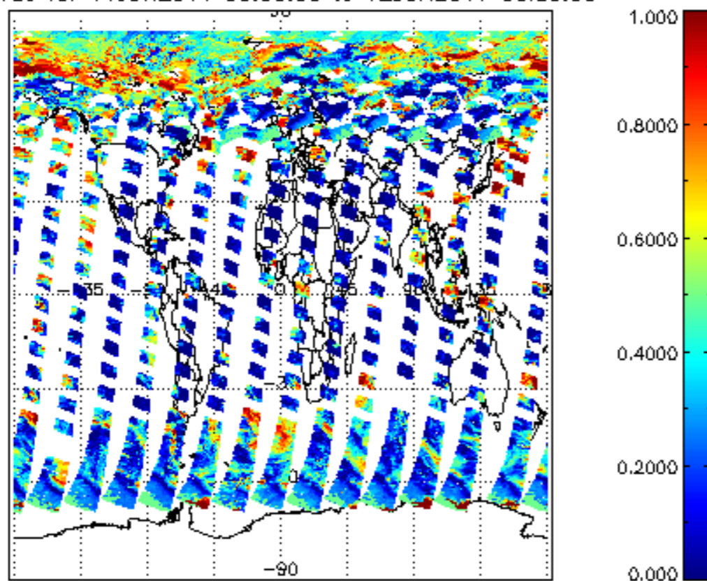
cl_frac for 11JUN2011 00:00:00 to 12JUN2011 00:00:00
