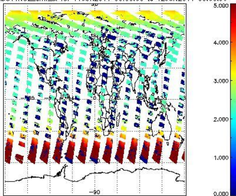
SCIOL2P_NADUV1NO2_amf_cl for 11JUN2011 00:00:00 to 12JUN2011 00:00:00
