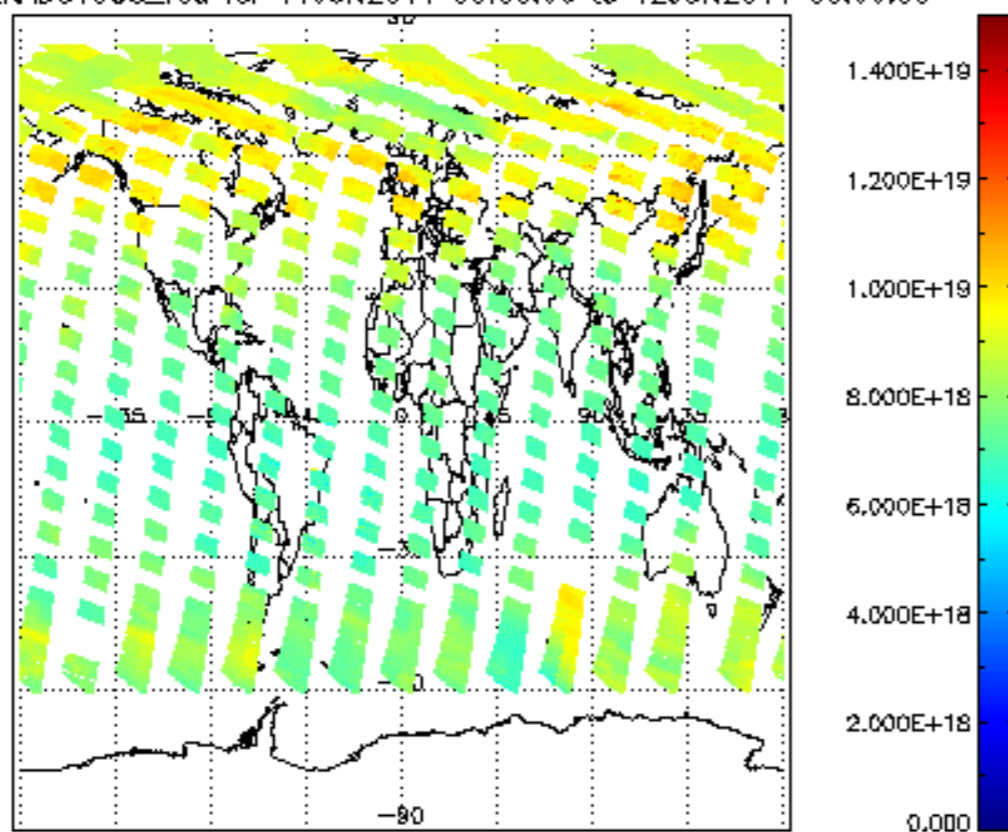
SCIOL2P_NADUV003_vcd for 11JUN2011 00:00:00 to 12JUN2011 00:00:00
