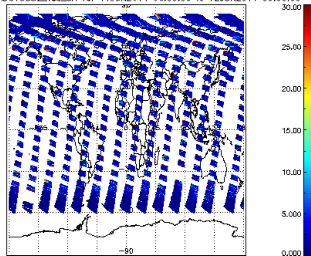
SCIOL2P_NADUV5S02_vcd_err for 11JUN2011 00:00:00 to 12JUN2011 00:00:00
