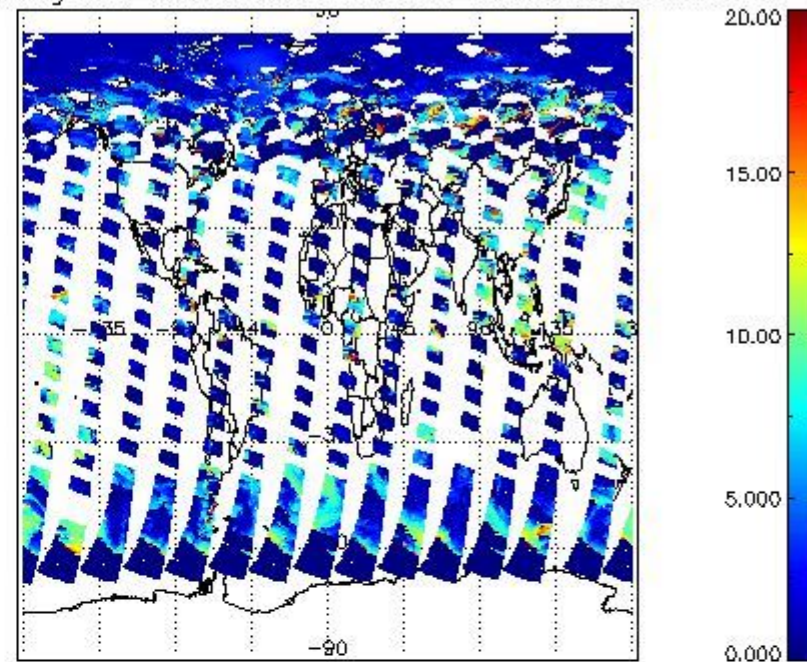
cL_top_height for 11JUN2011 00:00:00 to 12JUN2011 00:00:00
