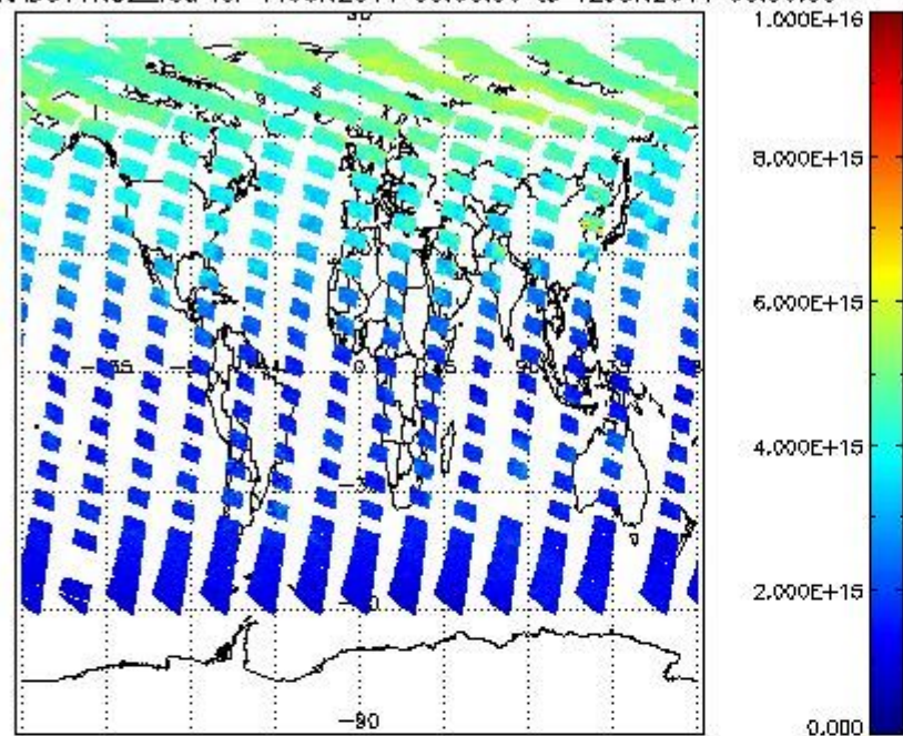
SCIOL2P_NADUV1NO2_vcd for 11JUN2011 00:00:00 to 12JUN2011 00:00:00
