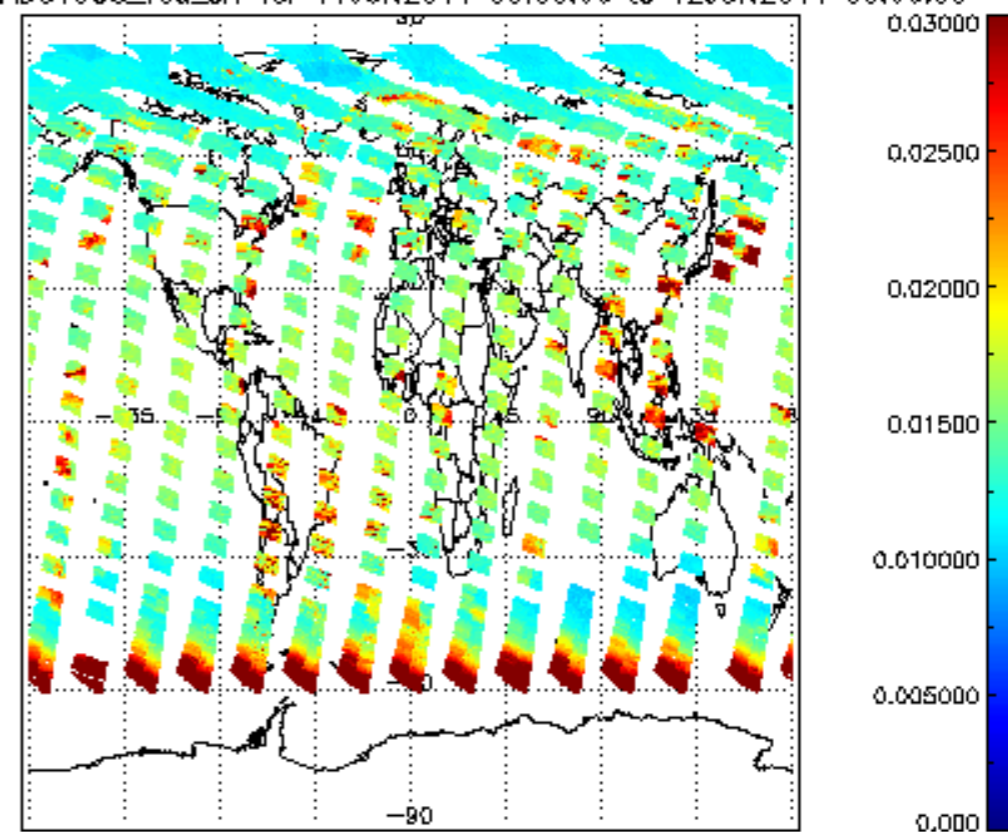
SCIOL2P_NADUV003_vcd_err for 11JUN2011 00:00:00 to 12JUN2011 00:00:00
