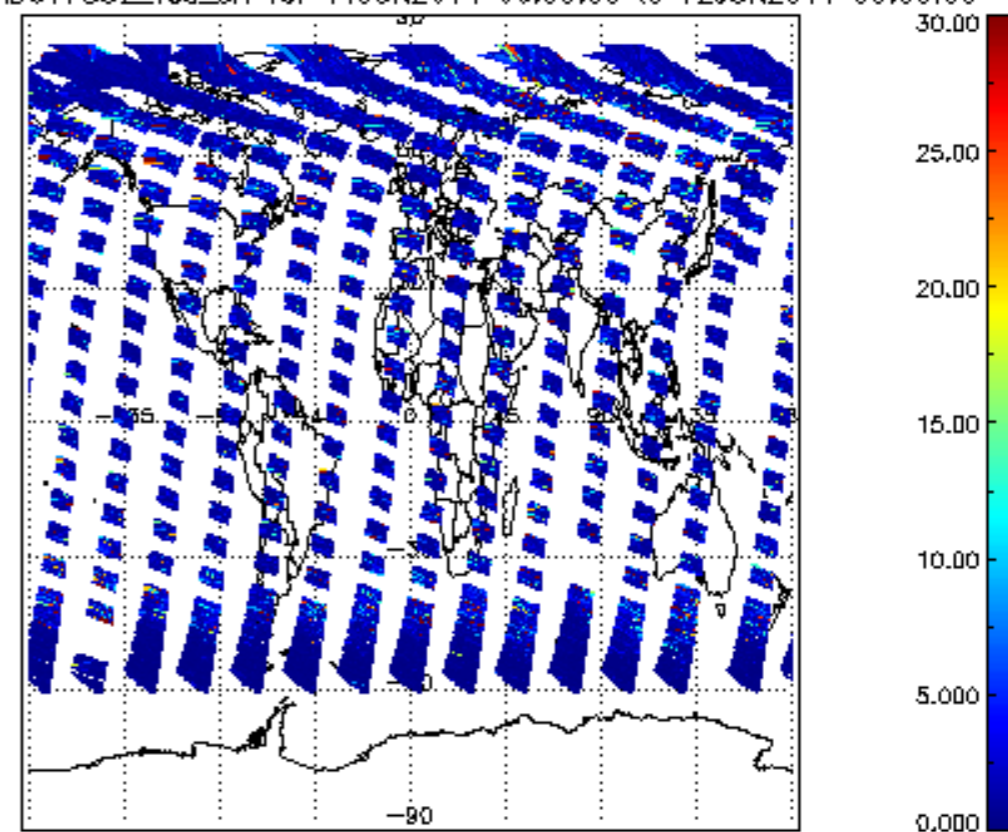
SCIOL2P_NADUV7S02_vcd_err for 11JUN2011 00:00:00 to 12JUN2011 00:00:00
