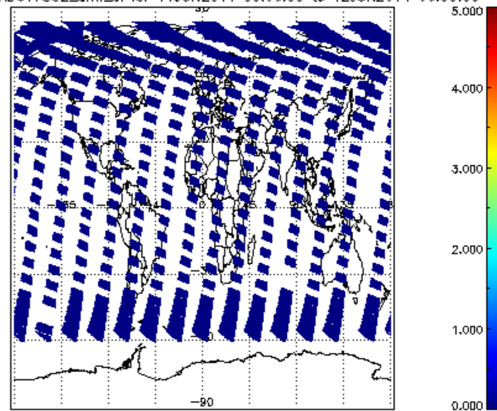
SCIOL2P_NADUV7S02_amf_cl for 11JUN2011 00:00:00 to 12JUN2011 00:00:00
