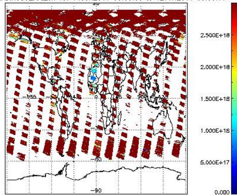
SCIO2P_NADIR3CO_vcd_err for 11JUN2011 00:00:00 to 12JUN2011 00:00:00
