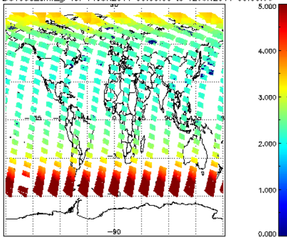
SCIOL2P_NADUV003_amf_gr for 11JUN2011 00:00:00 to 12JUN2011 00:00:00
