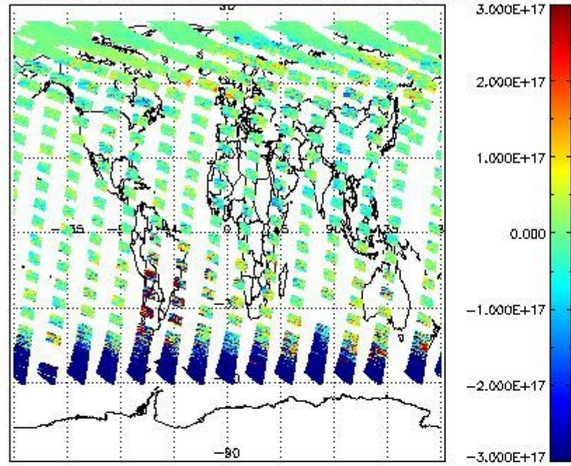
SCIOL2P_NADUV5S02_vcd for 11JUN2011 00:00:00 to 12JUN2011 00:00:00
