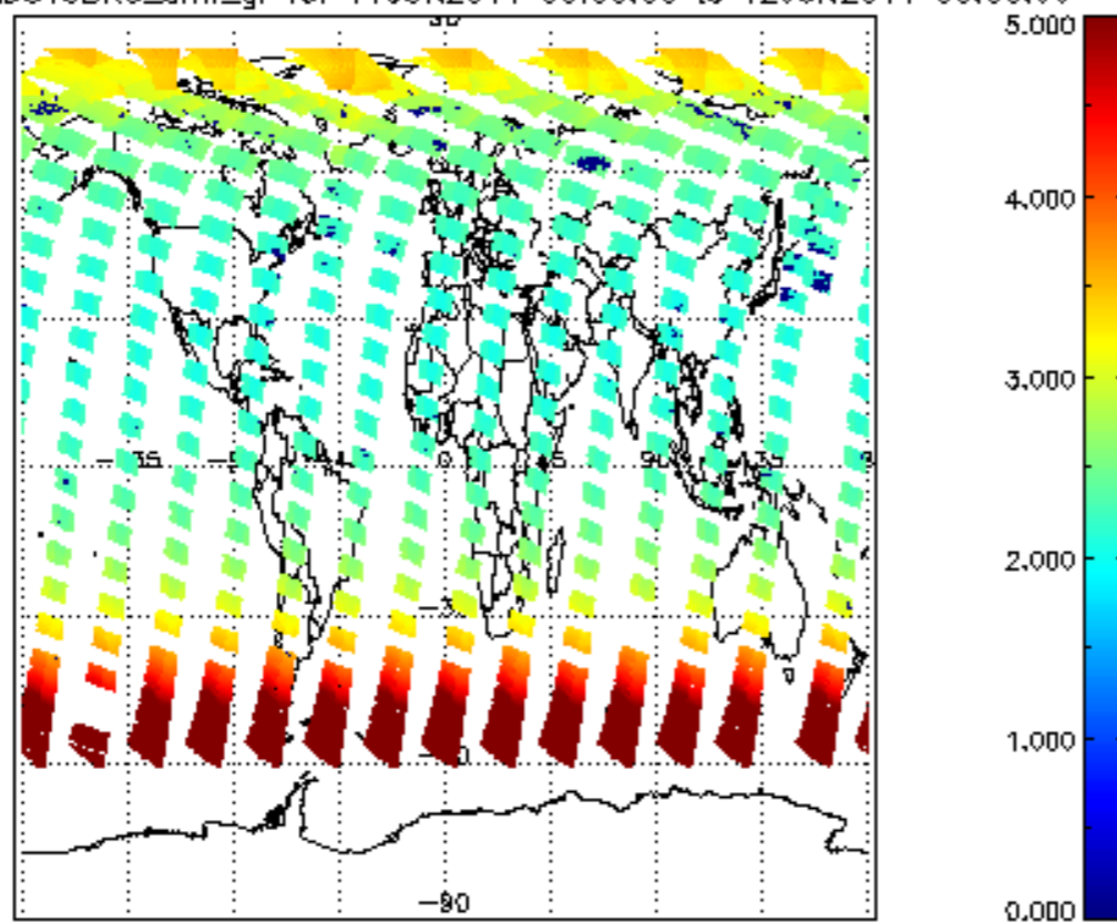
SCIOL2P_NADUV3BRO_amf_gr for 11JUN2011 00:00:00 to 12JUN2011 00:00:00
