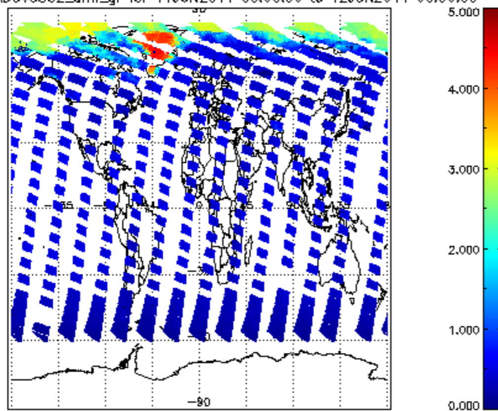
SCIOL2P_NADUV5S02_amf_gr for 11JUN2011 00:00:00 to 12JUN2011 00:00:00
