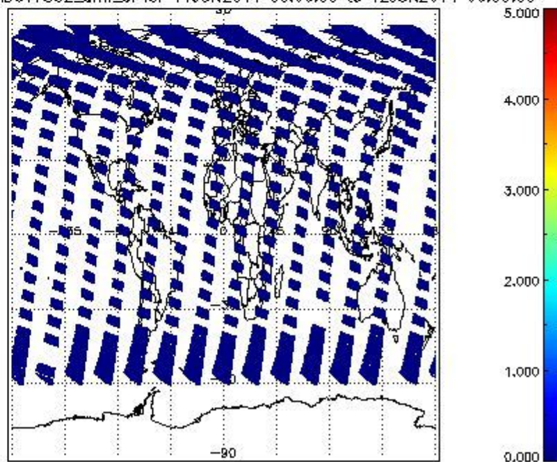
SCIOL2P_NADUV7S02_amf_cl for 11JUN2011 00:00:00 to 12JUN2011 00:00:00
