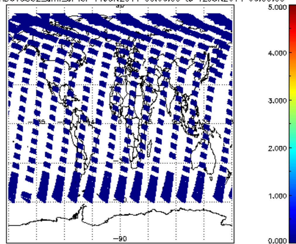
SCIOL2P_NADUV5S02_amf_cl for 11JUN2011 00:00:00 to 12JUN2011 00:00:00
