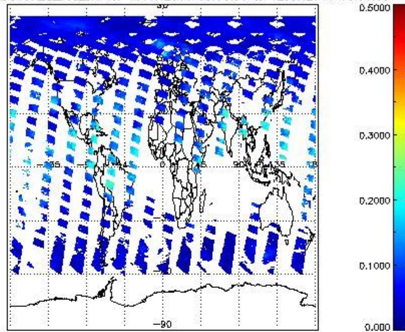
SCIOL2P_NADUV8H2O_vcd_err for 11JUN2011 00:00:00 to 12JUN2011 00:00:00
