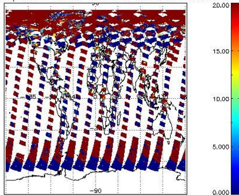
cL_opt_depth for 11JUN2011 00:00:00 to 12JUN2011 00:00:00
