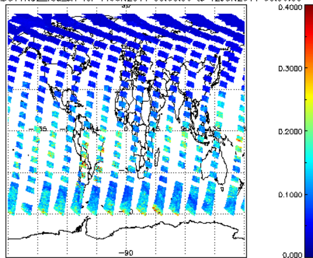
SCIOL2P_NADUV1NO2_vcd_err for 11JUN2011 00:00:00 to 12JUN2011 00:00:00
