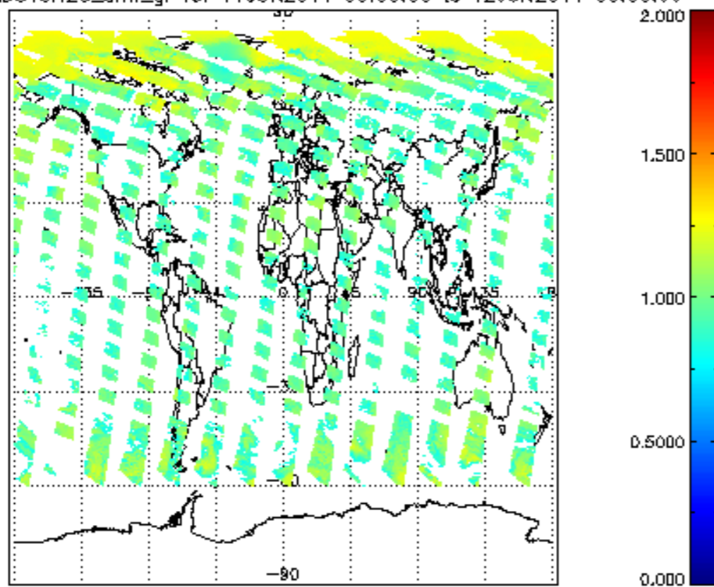
SCIOL2P_NADUV8H2O_amf_gr for 11JUN2011 00:00:00 to 12JUN2011 00:00:00
