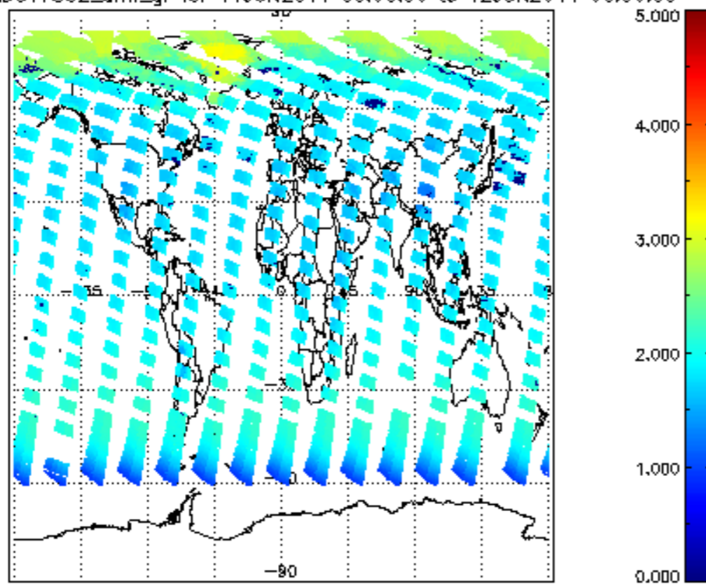
SCIOL2P_NADUV7S02_amf_gr for 11JUN2011 00:00:00 to 12JUN2011 00:00:00
