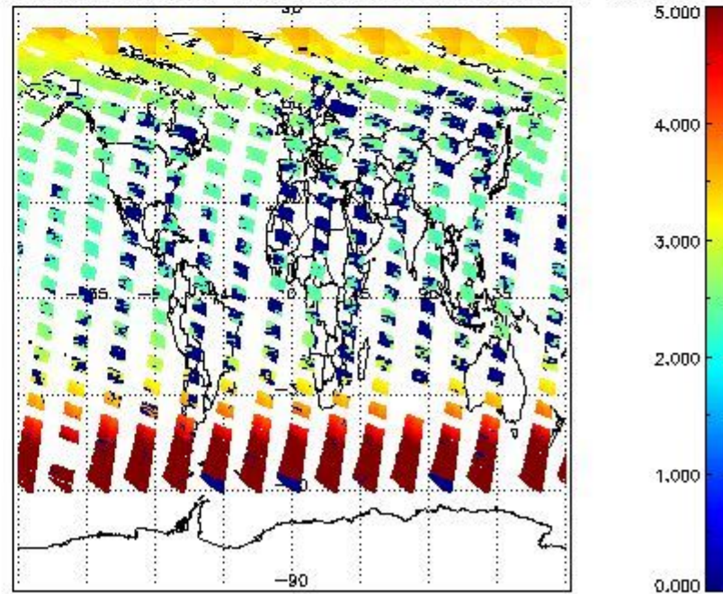
SCIOL2P_NADUV3BRO_amf_cl for 11JUN2011 00:00:00 to 12JUN2011 00:00:00
