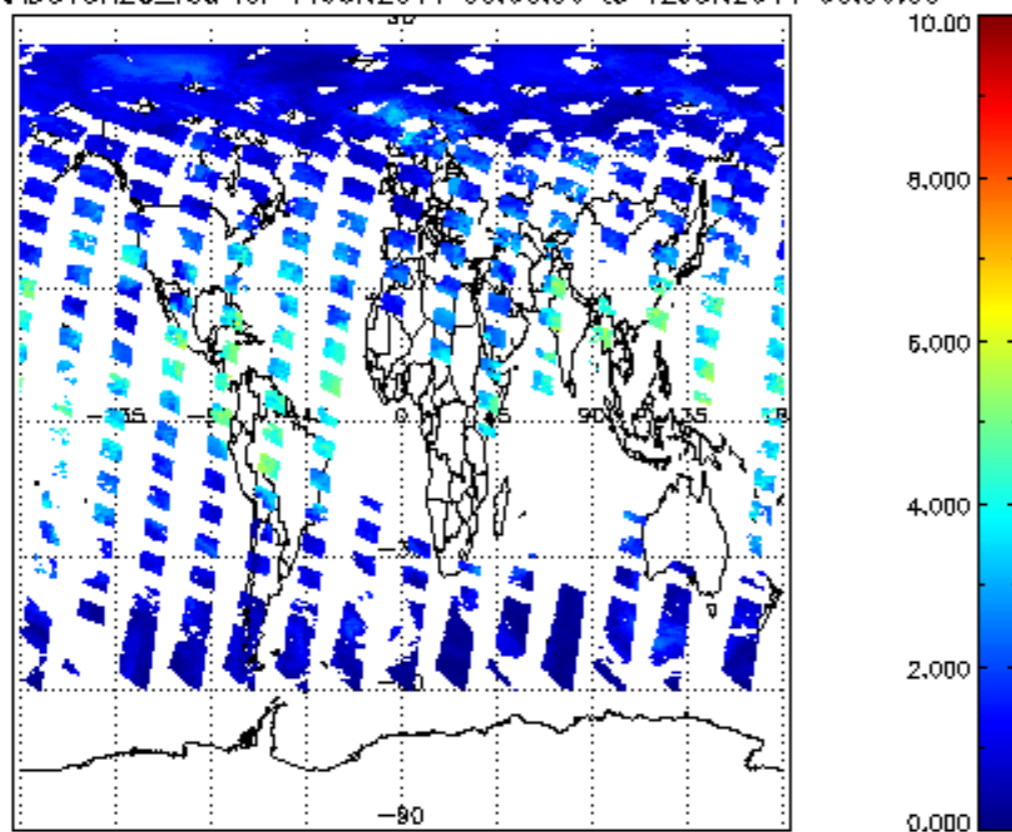
SCIOL2P_NADUV8H2O_vcd for 11JUN2011 00:00:00 to 12JUN2011 00:00:00
