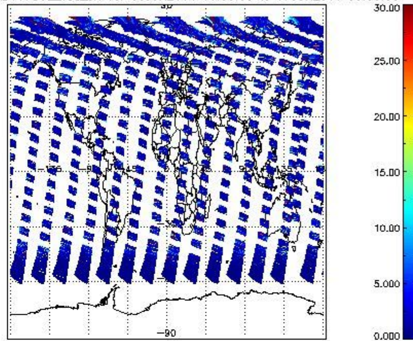
SCIOL2P_NADUV7S02_vcd_err for 06JUN2011 00:00:00 to 07JUN2011 00:00:00
