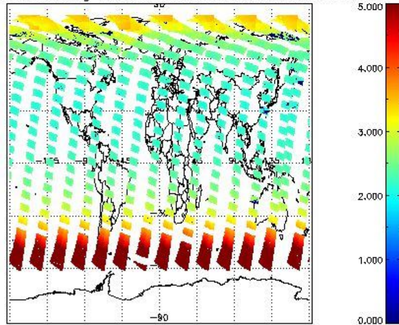
SCIOL2P_NADUV003_amf_gr for 06JUN2011 00:00:00 to 07JUN2011 00:00:00
