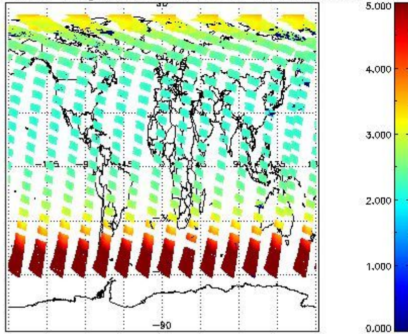
SCIOL2P_NADUV1NO2_amf_gr for 06JUN2011 00:00:00 to 07JUN2011 00:00:00
