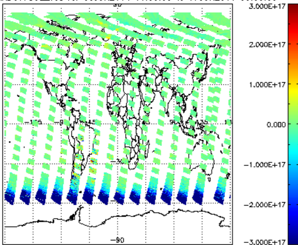
SCIOL2P_NADUV7S02_vcd for 06JUN2011 00:00:00 to 07JUN2011 00:00:00
