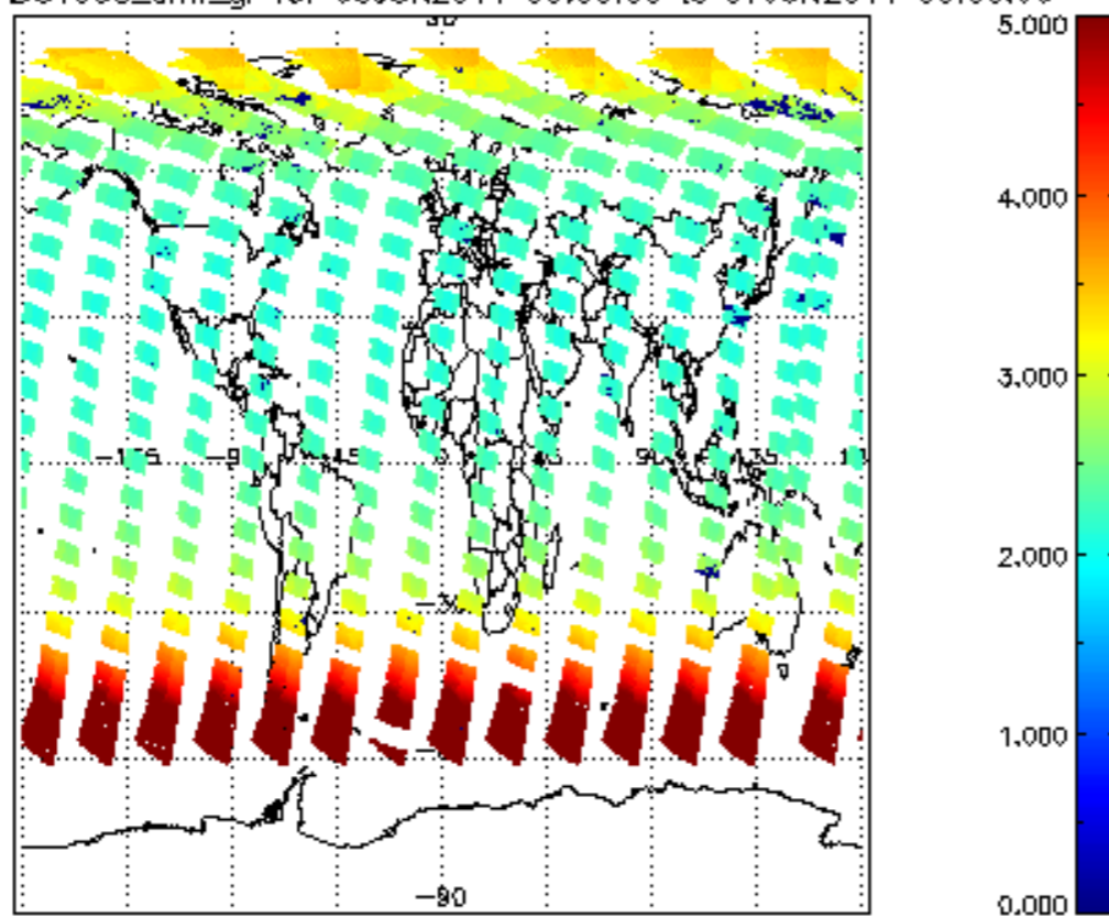
SCIOL2P_NADUV003_amf_gr for 06JUN2011 00:00:00 to 07JUN2011 00:00:00
