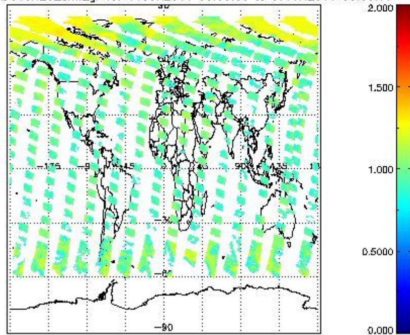
SCIOL2P_NADUV8H2O_amf_gr for 06JUN2011 00:00:00 to 07JUN2011 00:00:00
