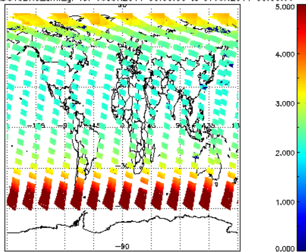
SCIOL2P_NADUV3BRO_amf_gr for 06JUN2011 00:00:00 to 07JUN2011 00:00:00
