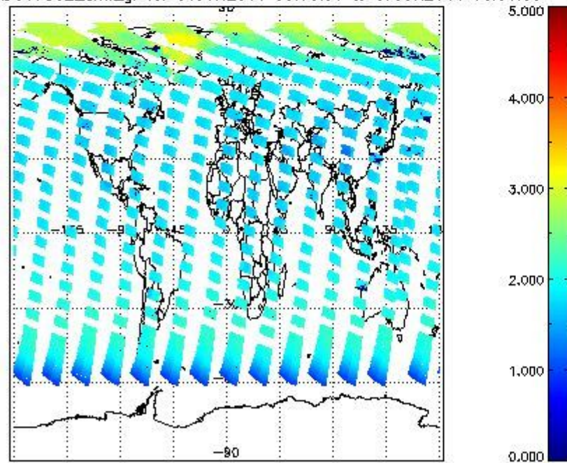
SCIOL2P_NADUV7S02_amf_gr for 06JUN2011 00:00:00 to 07JUN2011 00:00:00
