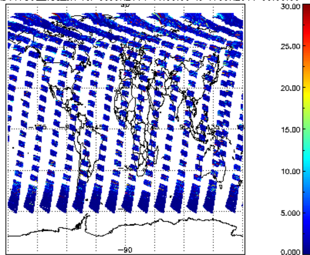
SCIOL2P_NADUV7S02_vcd_err for 06JUN2011 00:00:00 to 07JUN2011 00:00:00
