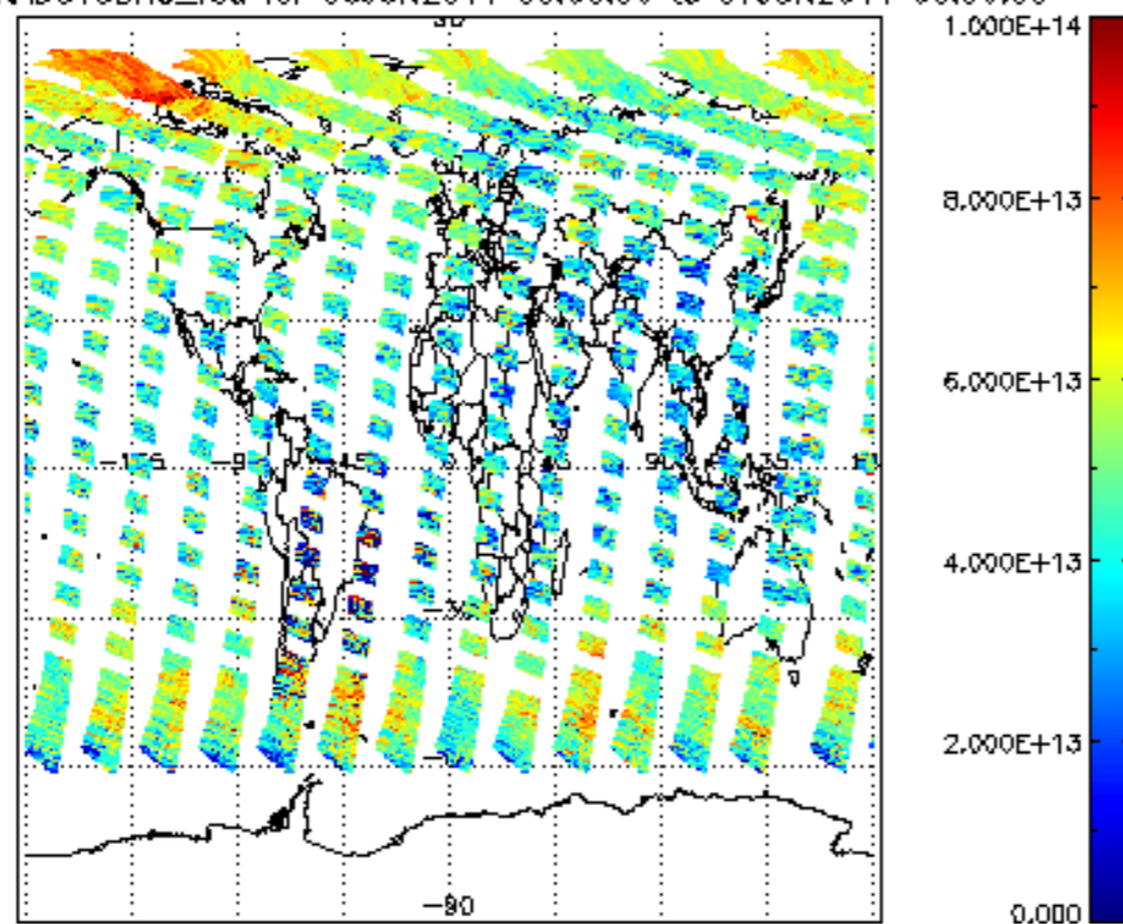
SCIOL2P_NADUV3BRO_vcd for 06JUN2011 00:00:00 to 07JUN2011 00:00:00
