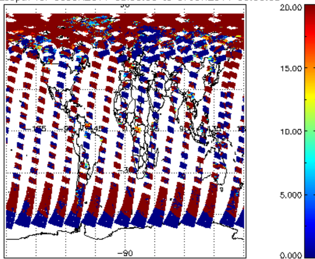
cl_opt_depth for 06JUN2011 00:00:00 to 07JUN2011 00:00:00
