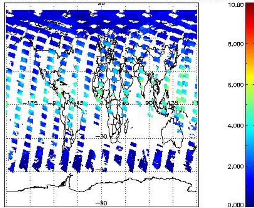
SCIOL2P_NADUV8H2O_vcd for 06JUN2011 00:00:00 to 07JUN2011 00:00:00
