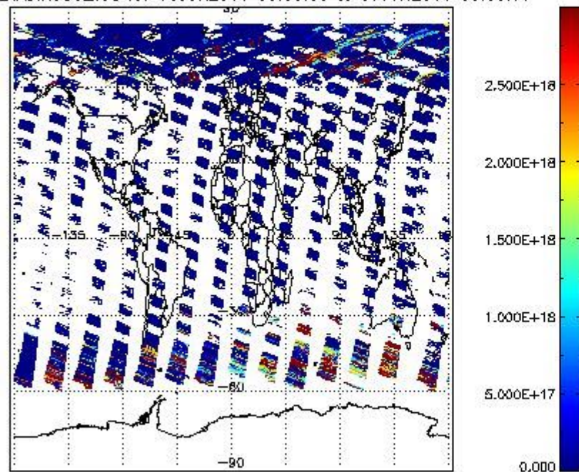
SCIOL2P_NADIR3CO_vcd for 06JUN2011 00:00:00 to 07JUN2011 00:00:00
