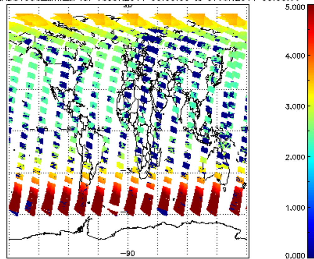
SCIOL2P_NADUV003_amf_cl for 06JUN2011 00:00:00 to 07JUN2011 00:00:00
