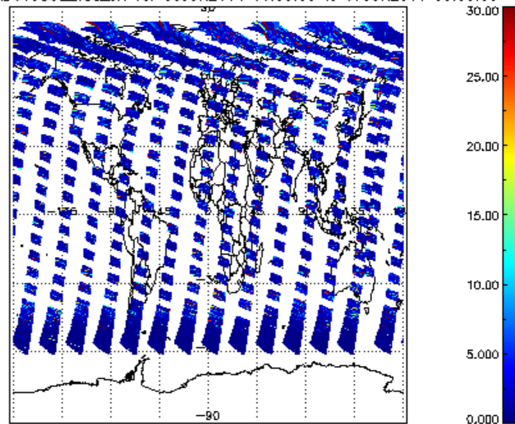
SCIOL2P_NADUV5S02_vcd_err for 06JUN2011 00:00:00 to 07JUN2011 00:00:00
