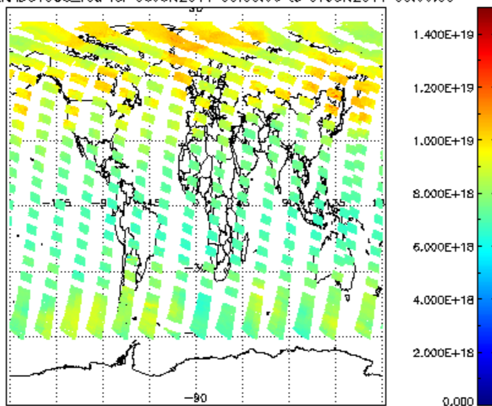
SCIOL2P_NADUV003_vcd for 06JUN2011 00:00:00 to 07JUN2011 00:00:00
