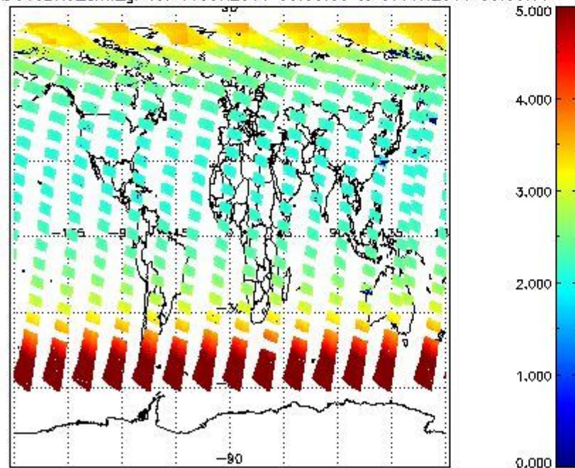
SCIOL2P_NADUV3BRO_amf_gr for 06JUN2011 00:00:00 to 07JUN2011 00:00:00
