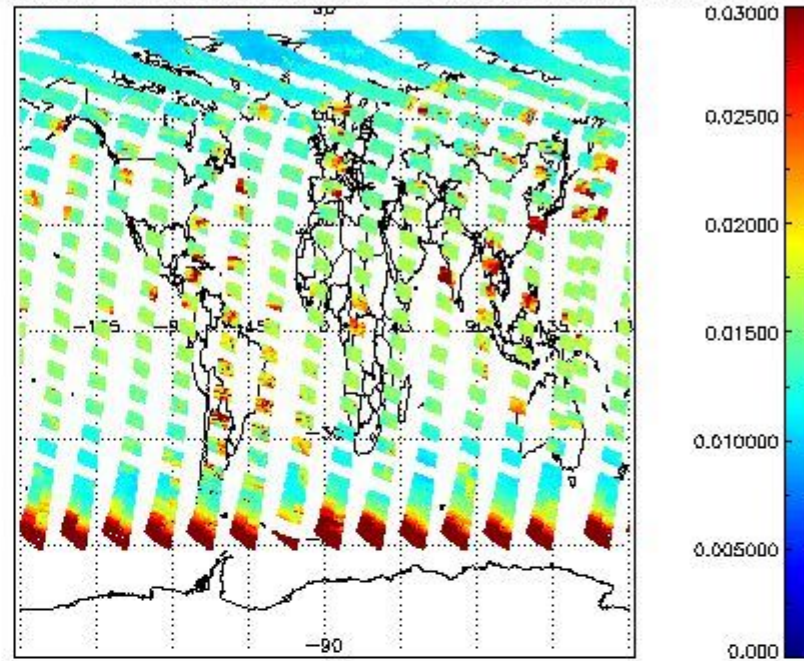
SCIOL2P_NADUV003_vcd_err for 06JUN2011 00:00:00 to 07JUN2011 00:00:00
