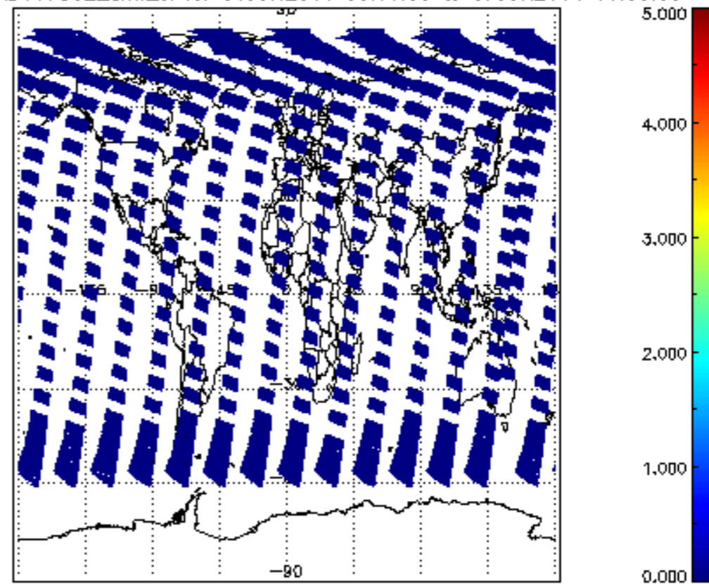
SCIOL2P_NADUV7S02_amf_cl for 06JUN2011 00:00:00 to 07JUN2011 00:00:00
