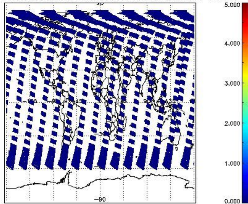
SCIOL2P_NADUV5S02_amf_cl for 06JUN2011 00:00:00 to 07JUN2011 00:00:00
