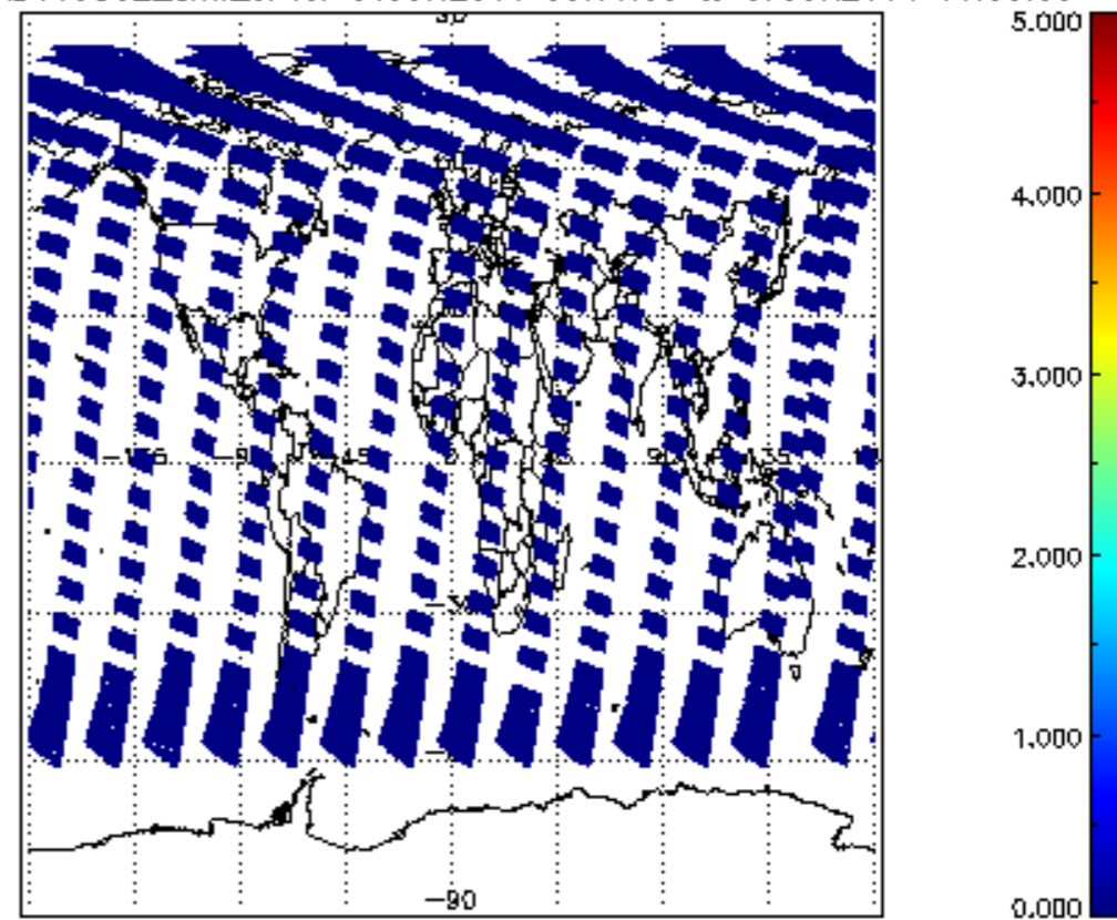
SCIOL2P_NADUV5S02_amf_cl for 06JUN2011 00:00:00 to 07JUN2011 00:00:00
