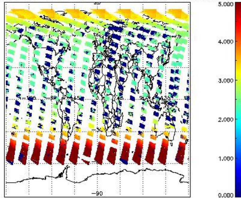
SCIOL2P_NADUV003_amf_cl for 06JUN2011 00:00:00 to 07JUN2011 00:00:00
