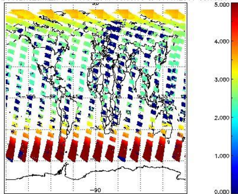
SCIOL2P_NADUV3BRO_amf_cl for 06JUN2011 00:00:00 to 07JUN2011 00:00:00
