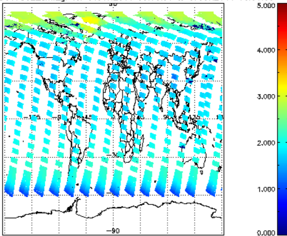
SCIOL2P_NADUV7S02_amf_gr for 06JUN2011 00:00:00 to 07JUN2011 00:00:00
