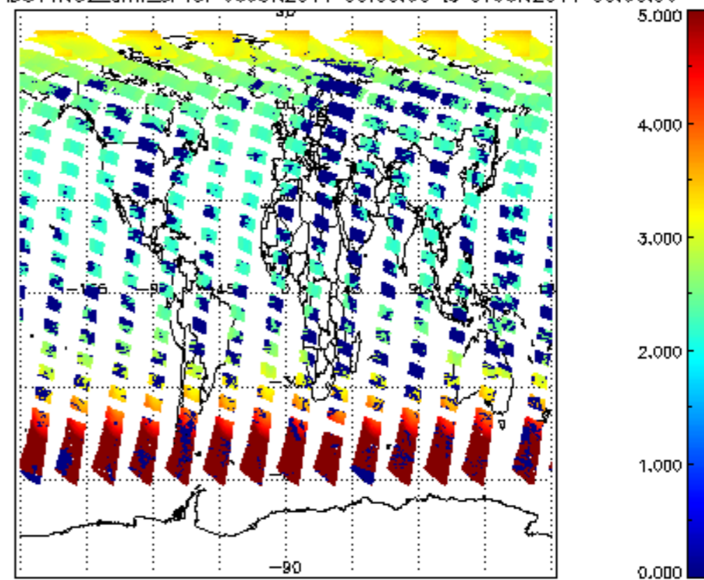
SCIOL2P_NADUV1NO2_amf_sl for 06JUN2011 00:00:00 to 07JUN2011 00:00:00
