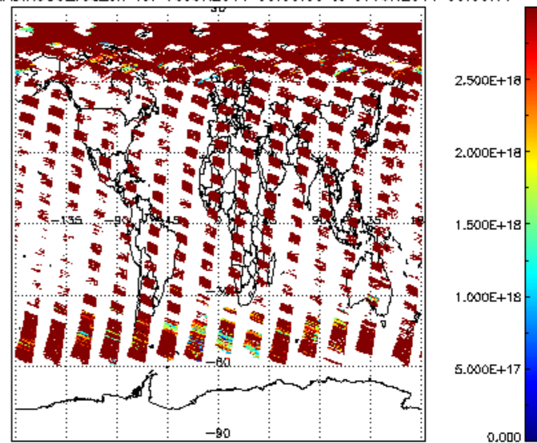
SCIOL2P_NADIR3CO_vcd_err for 06JUN2011 00:00:00 to 07JUN2011 00:00:00
