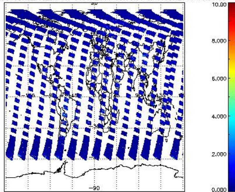
SCIOL2P_NADUV3BRO_vcd_err for 06JUN2011 00:00:00 to 07JUN2011 00:00:00
