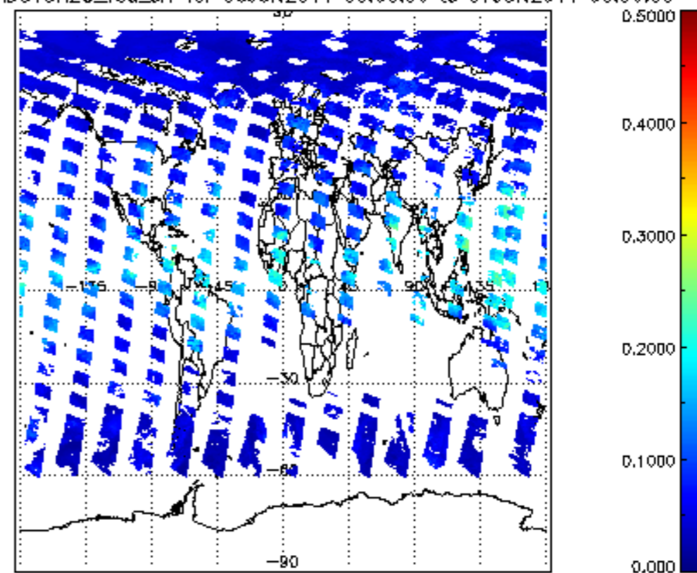
SCIOL2P_NADUV8H2O_vcd_err for 06JUN2011 00:00:00 to 07JUN2011 00:00:00
