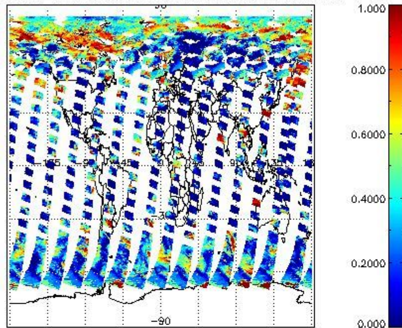
cL_frac for 06JUN2011 00:00:00 to 07JUN2011 00:00:00
