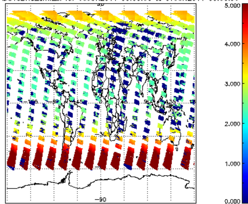
SCIOL2P_NADUV3BRO_amf_sl for 06JUN2011 00:00:00 to 07JUN2011 00:00:00
