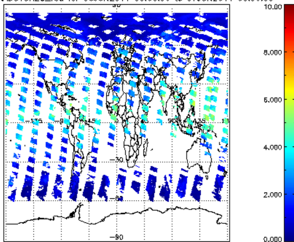
SCIOL2P_NADUV8H2O_vcd for 06JUN2011 00:00:00 to 07JUN2011 00:00:00
