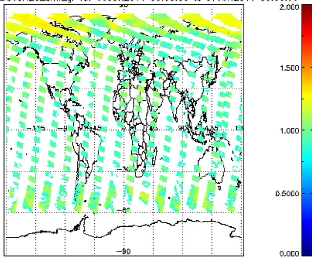
SCIOL2P_NADUV8H2O_amf_gr for 06JUN2011 00:00:00 to 07JUN2011 00:00:00
