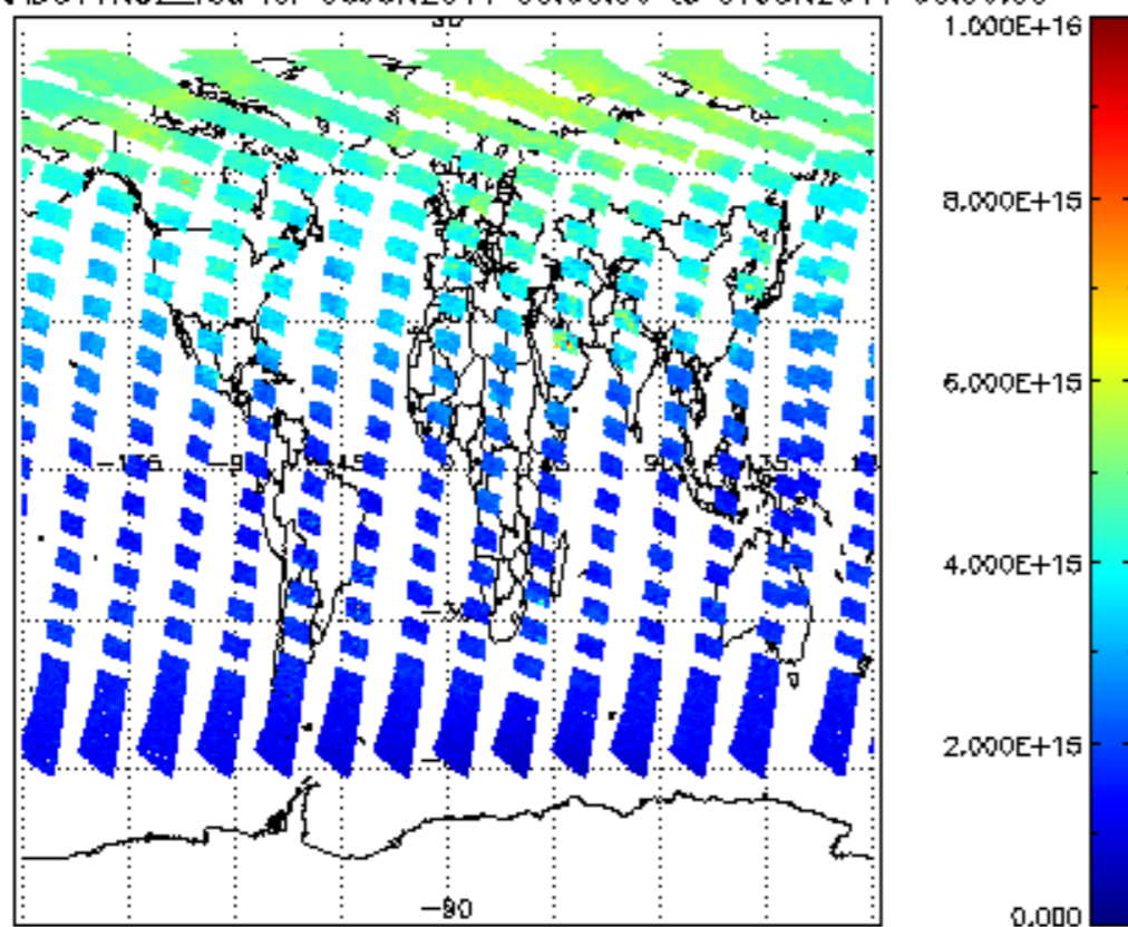
SCIOL2P_NADUV1NO2_vcd for 06JUN2011 00:00:00 to 07JUN2011 00:00:00
