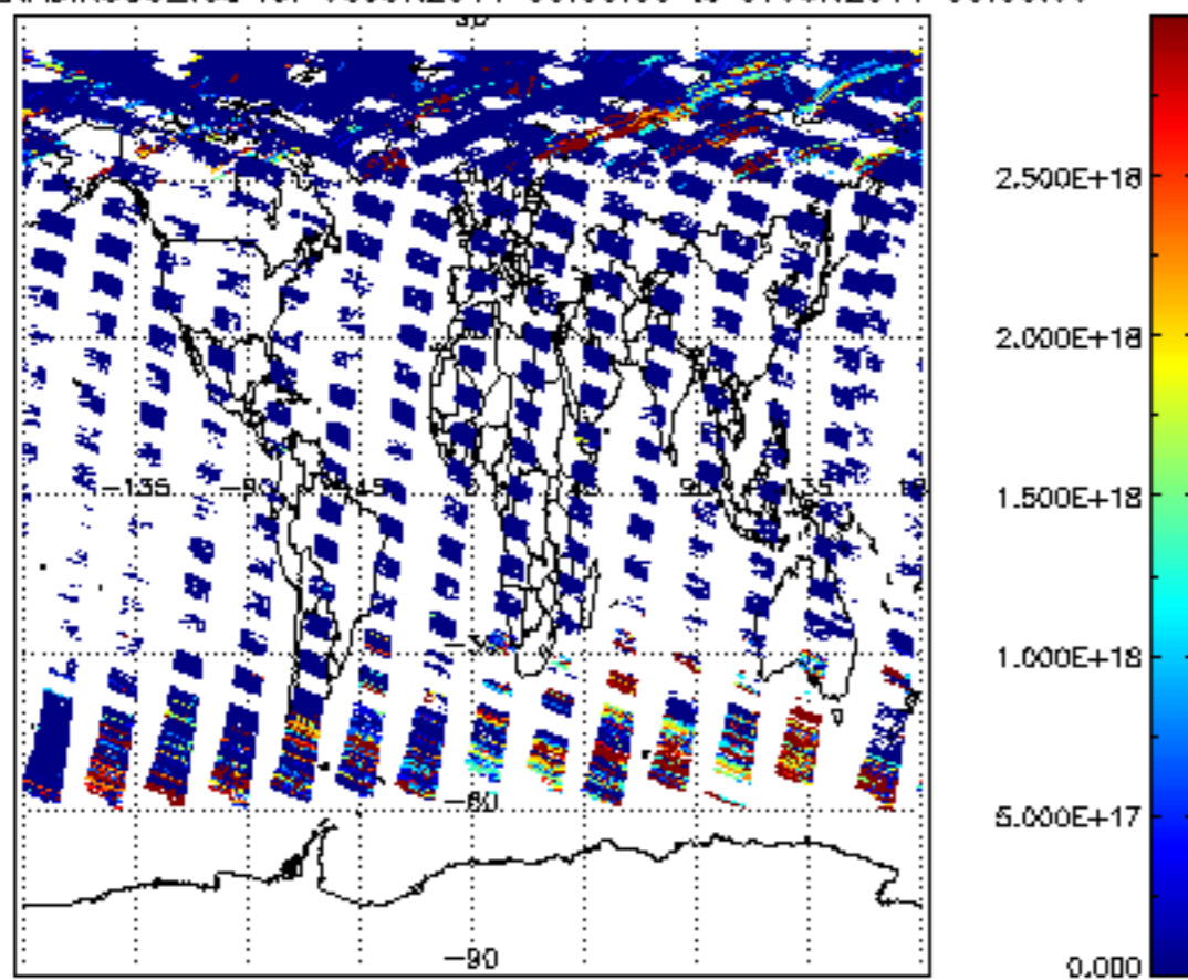
SCIOL2P_NADIR3CO_vcd for 06JUN2011 00:00:00 to 07JUN2011 00:00:00
