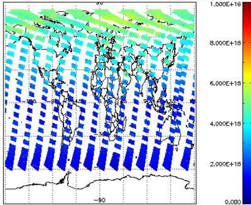
SCIOL2P_NADUV1NO2_vcd for 06JUN2011 00:00:00 to 07JUN2011 00:00:00
