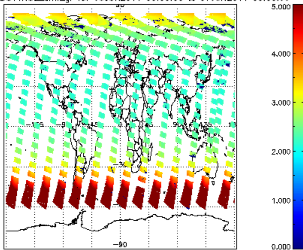
SCIOL2P_NADUV1NO2_amf_gr for 06JUN2011 00:00:00 to 07JUN2011 00:00:00
