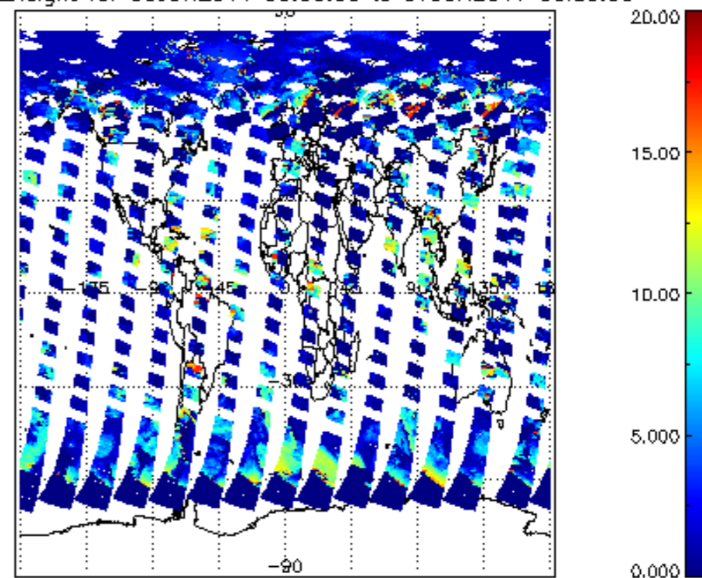
cl_top_height for 06JUN2011 00:00:00 to 07JUN2011 00:00:00
