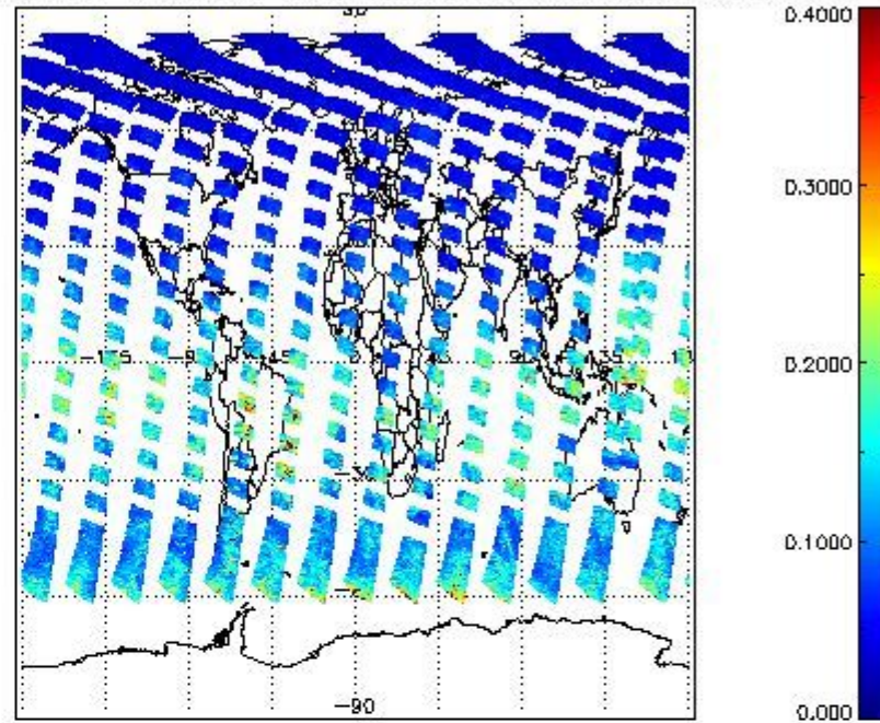
SCIOL2P_NADUV1NO2_vcd_err for 06JUN2011 00:00:00 to 07JUN2011 00:00:00
