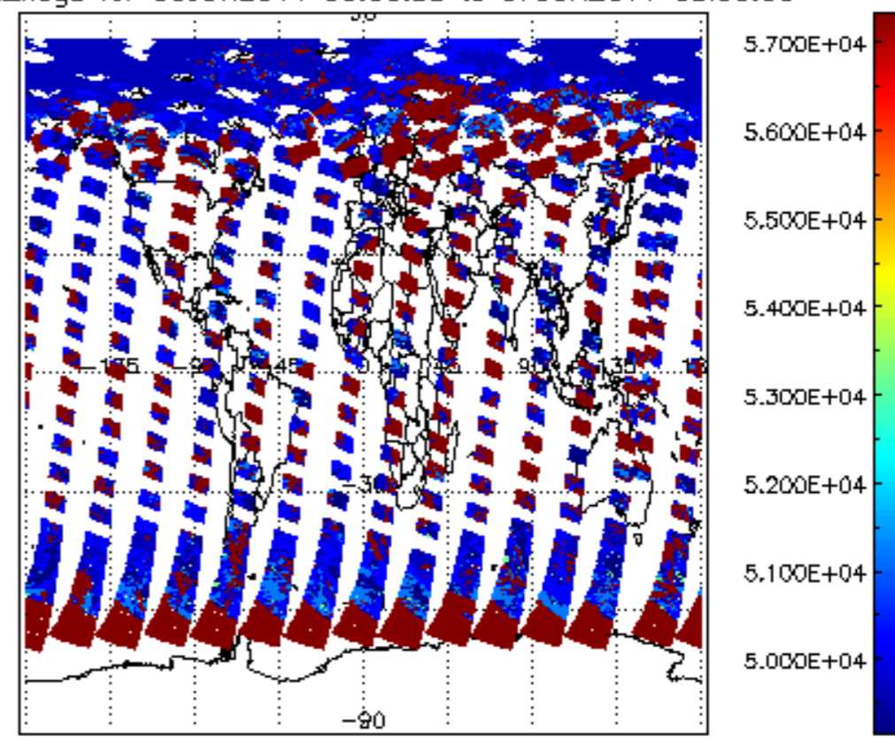
cloud_flags for 06JUN2011 00:00:00 to 07JUN2011 00:00:00
