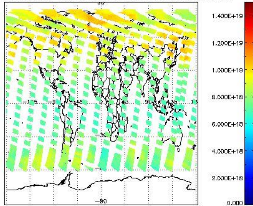
SCIOL2P_NADUV003_vcd for 06JUN2011 00:00:00 to 07JUN2011 00:00:00
