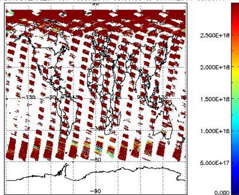
SCIOL2P_NADIR3CO_vcd_err for 06JUN2011 00:00:00 to 07JUN2011 00:00:00
