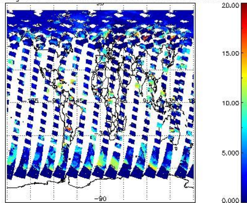
cL_top_height for 06JUN2011 00:00:00 to 07JUN2011 00:00:00
