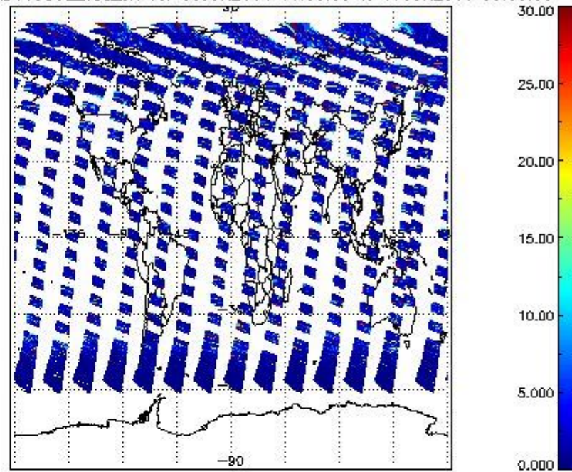
SCIOL2P_NADUV5S02_vcd_err for 06JUN2011 00:00:00 to 07JUN2011 00:00:00
