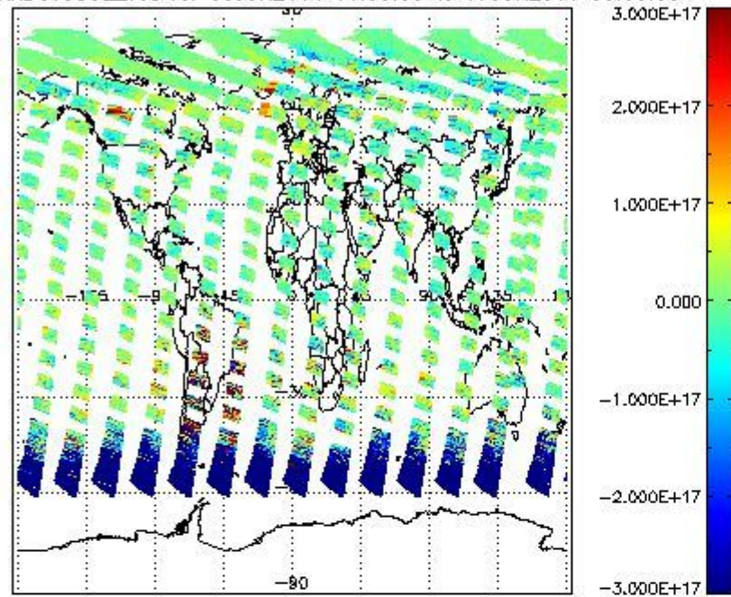
SCIOL2P_NADUV5S02_vcd for 06JUN2011 00:00:00 to 07JUN2011 00:00:00
