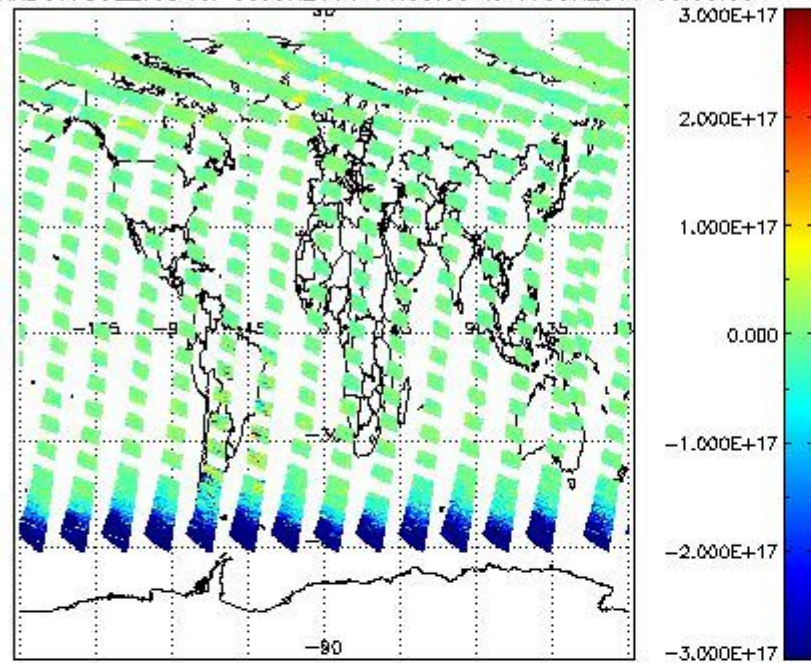
SCIOL2P_NADUV7S02_vcd for 06JUN2011 00:00:00 to 07JUN2011 00:00:00
