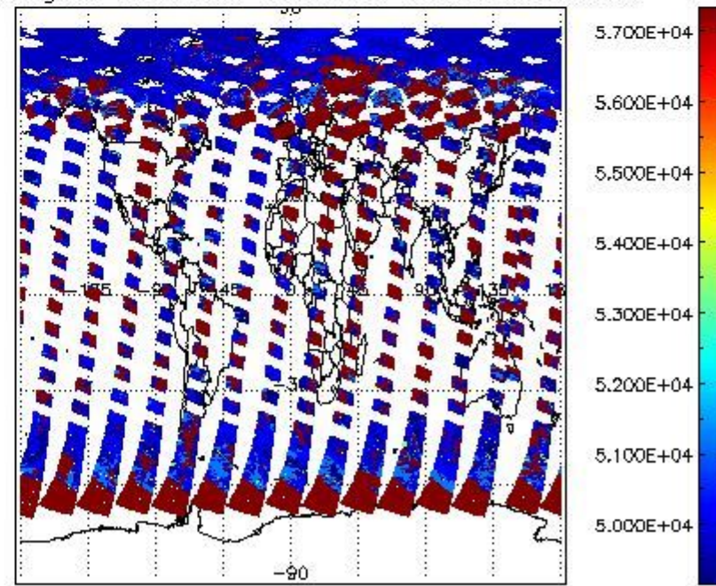
cloud_flags for 06JUN2011 00:00:00 to 07JUN2011 00:00:00
