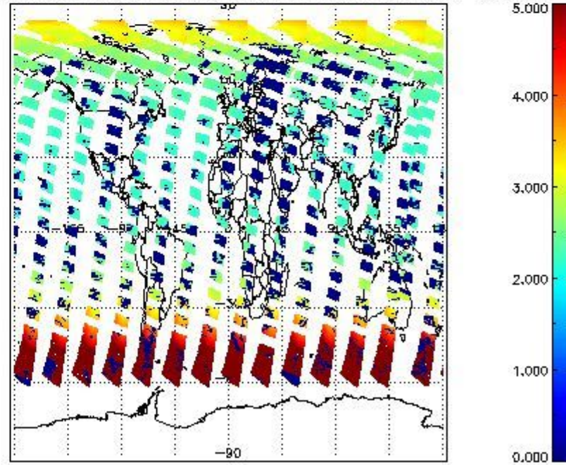
SCIOL2P_NADUV1NO2_amf_cl for 06JUN2011 00:00:00 to 07JUN2011 00:00:00
