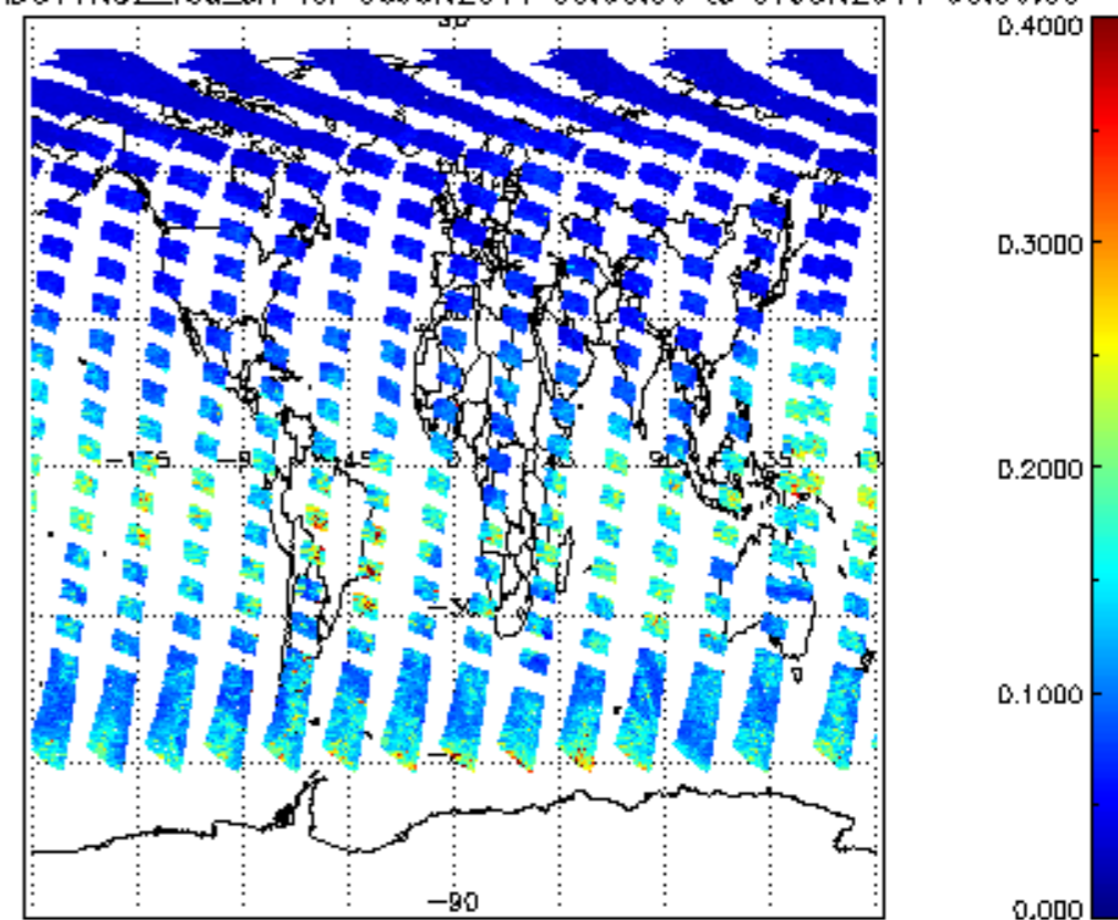
SCIOL2P_NADUV1NO2_vcd_err for 06JUN2011 00:00:00 to 07JUN2011 00:00:00
