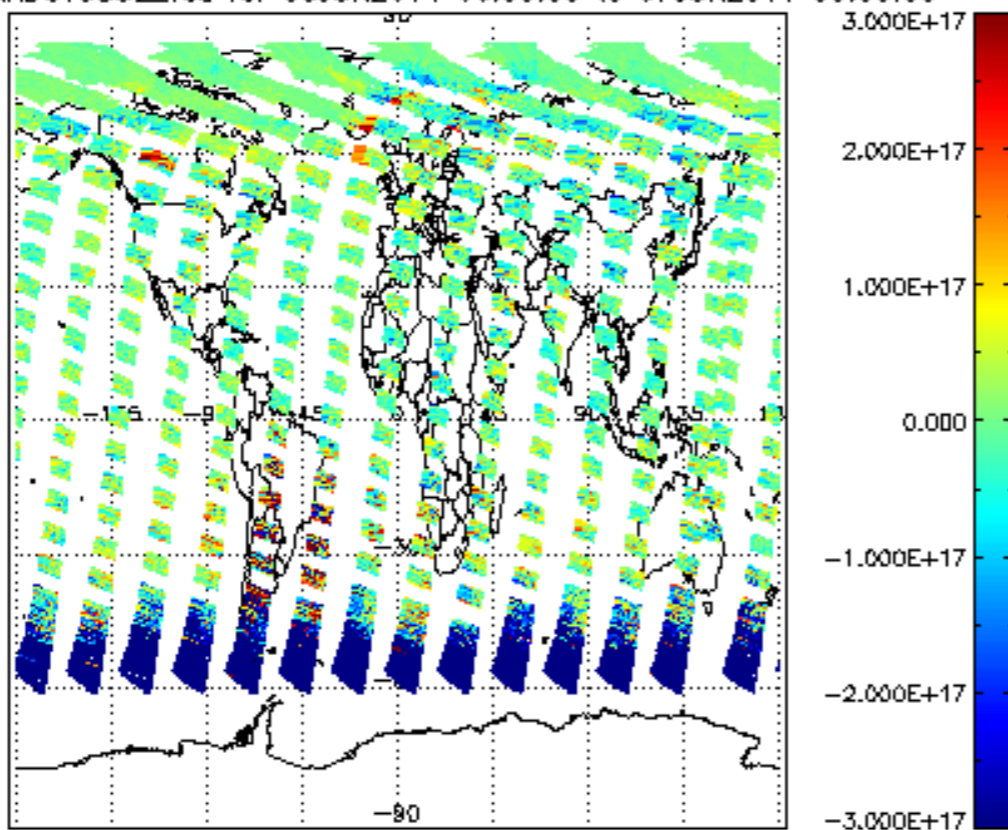
SCIOL2P_NADUV5S02_vcd for 06JUN2011 00:00:00 to 07JUN2011 00:00:00
