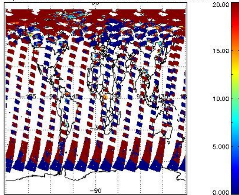
cL_opt_depth for 06JUN2011 00:00:00 to 07JUN2011 00:00:00
