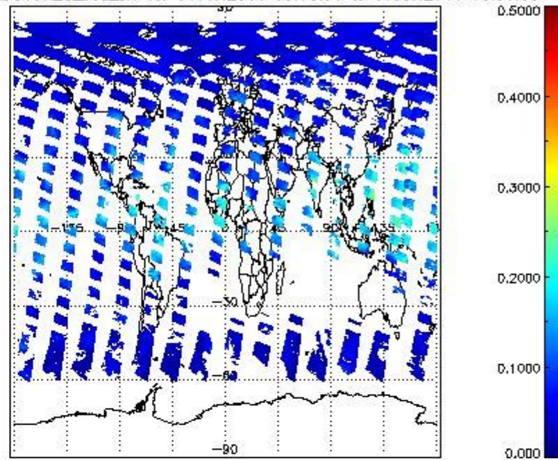
SCIOL2P_NADUV8H2O_vcd_err for 06JUN2011 00:00:00 to 07JUN2011 00:00:00
