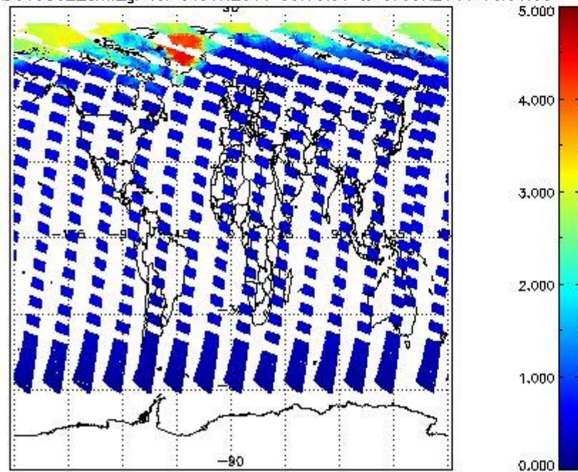
SCIOL2P_NADUV5S02_amf_gr for 06JUN2011 00:00:00 to 07JUN2011 00:00:00
