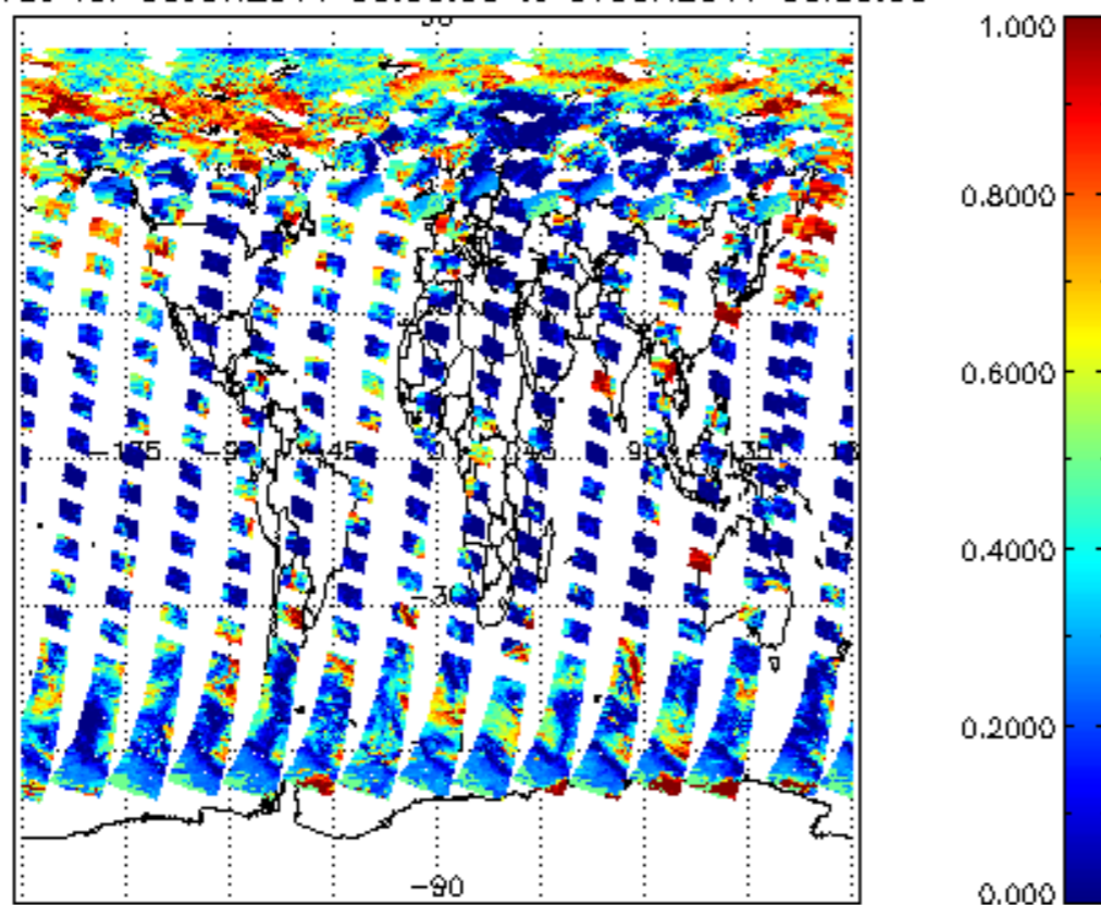
cl_frac for 06JUN2011 00:00:00 to 07JUN2011 00:00:00
