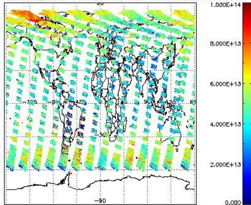
SCIOL2P_NADUV3BRO_vcd for 06JUN2011 00:00:00 to 07JUN2011 00:00:00
