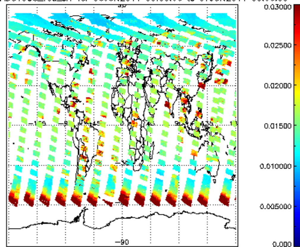
SCIOL2P_NADUV003_vcd_err for 06JUN2011 00:00:00 to 07JUN2011 00:00:00
