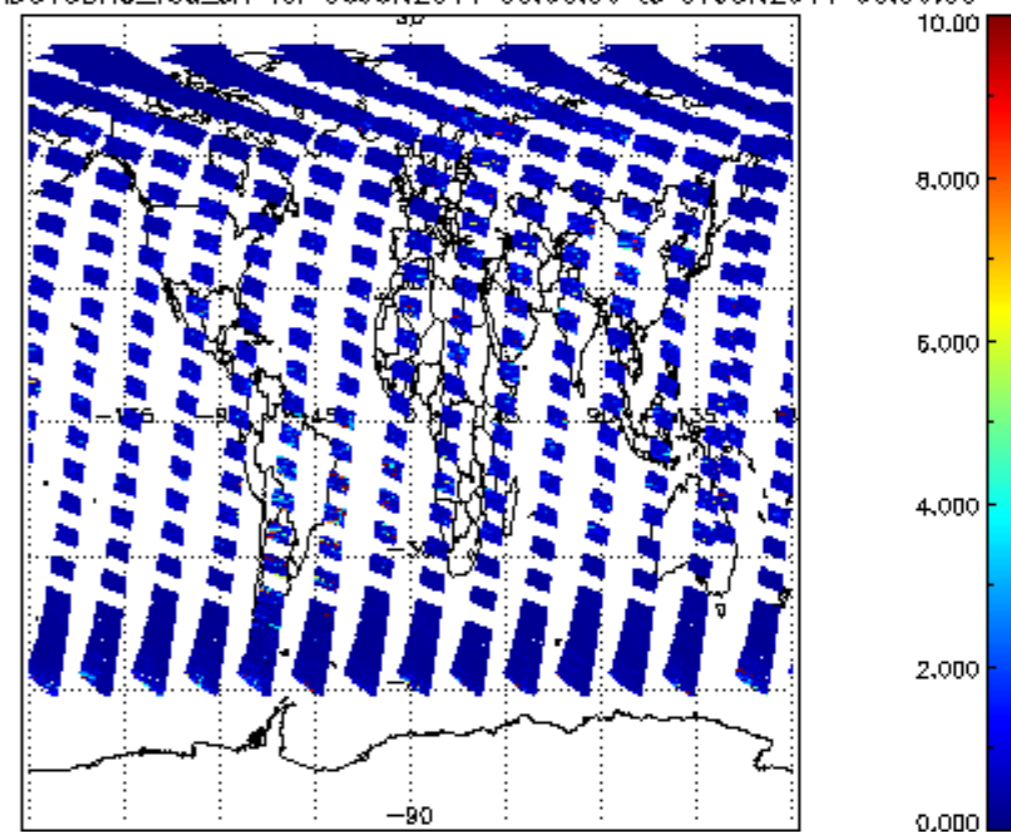
SCIOL2P_NADUV3BRO_vcd_err for 06JUN2011 00:00:00 to 07JUN2011 00:00:00
