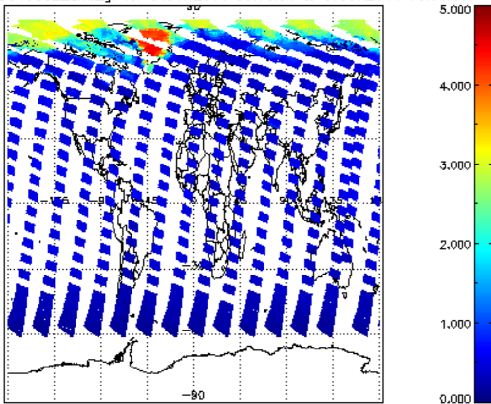
SCIOL2P_NADUV5S02_amf_gr for 06JUN2011 00:00:00 to 07JUN2011 00:00:00
