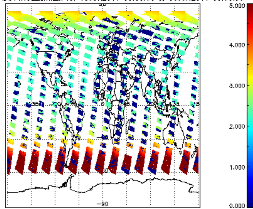
SCIOL2P_NADUV1NO2_amf_cl for 05JUN2011 00:00:00 to 06JUN2011 00:00:00
