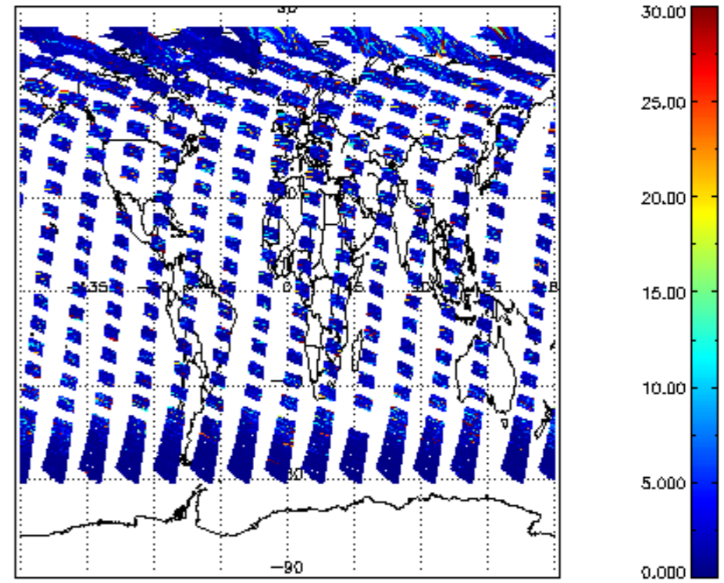
SCIOL2P_NADUV5S02_vcd_err for 05JUN2011 00:00:00 to 06JUN2011 00:00:00
