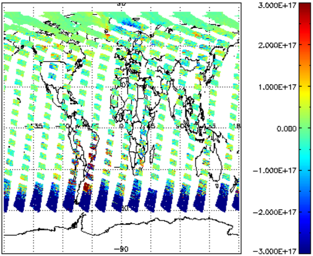
SCIOL2P_NADUV5S02_vcd for 05JUN2011 00:00:00 to 06JUN2011 00:00:00
