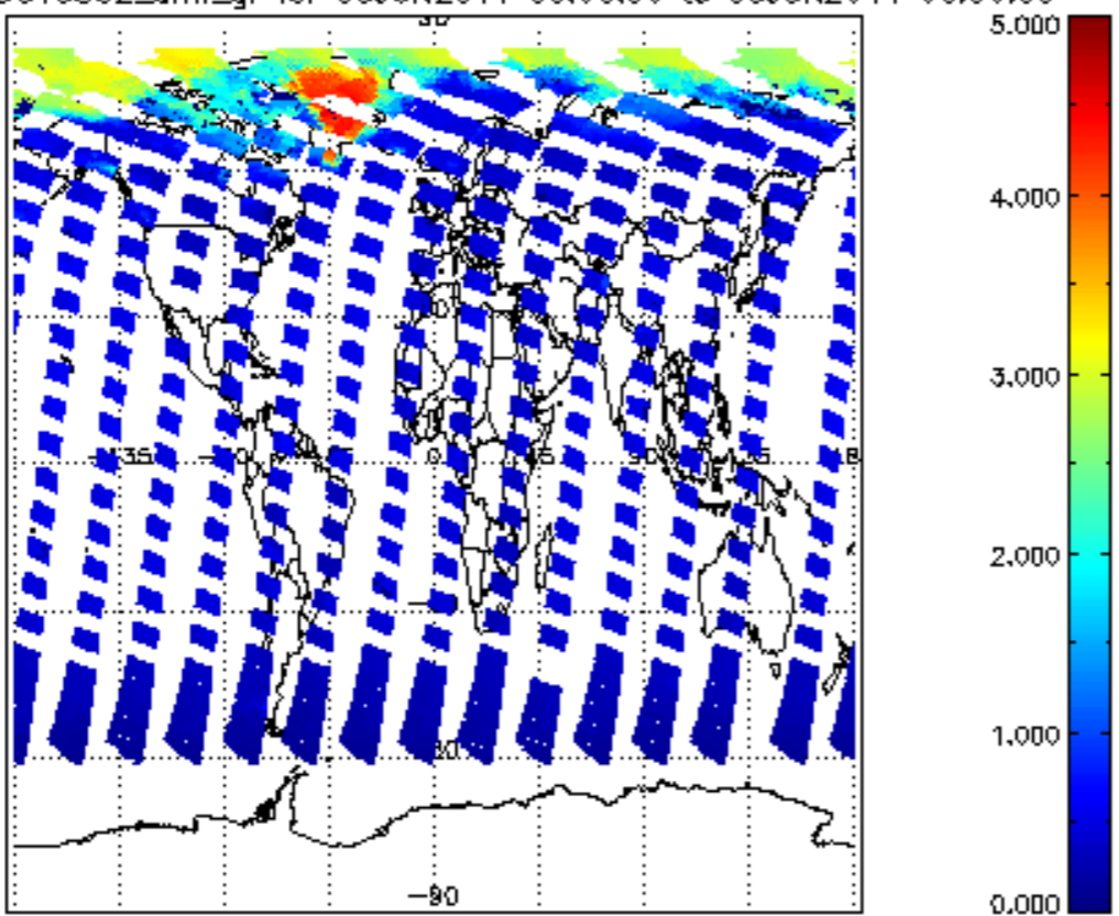
SCIOL2P_NADUV5S02_amf_gr for 05JUN2011 00:00:00 to 06JUN2011 00:00:00
