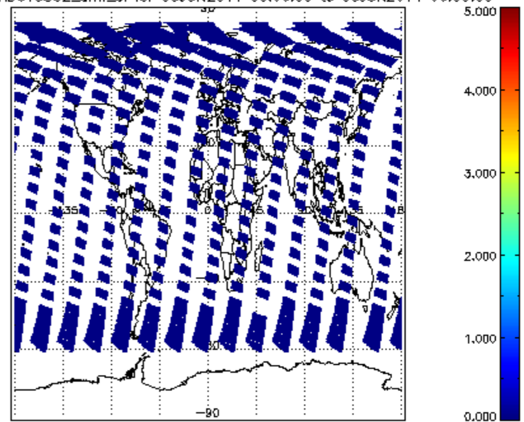
SCIOL2P_NADUV5S02_amf_cl for 05JUN2011 00:00:00 to 06JUN2011 00:00:00
