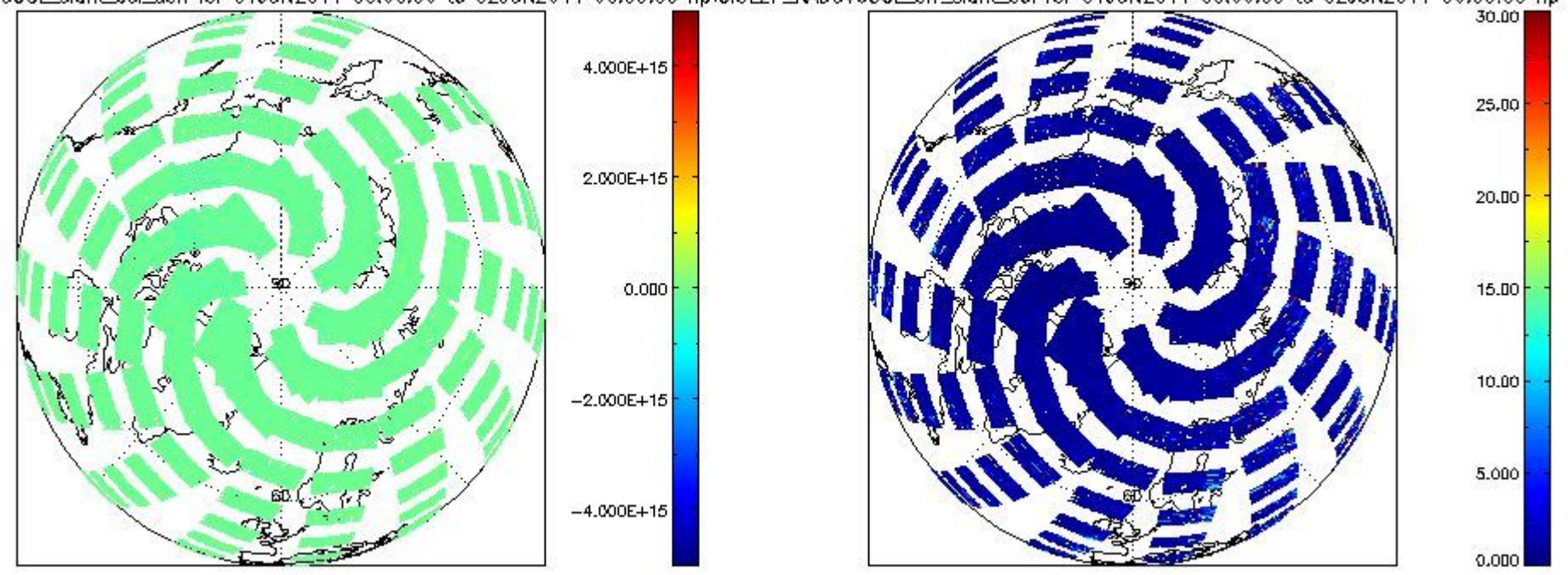
CIOL2P_NADUV60CL_slant_col_den for 01JUN2011 00:00:00 to 02JUN2011 00:00:00 np; CIOL2P_NADUV60CL_err_slant_col for 01JUN2011 00:00:00 to 02JUN2011 00:00:00 np
