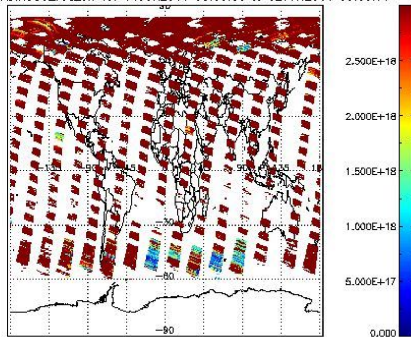
SCIO2P_NADIR3CO_vcd_err for 01JUN2011 00:00:00 to 02JUN2011 00:00:00
