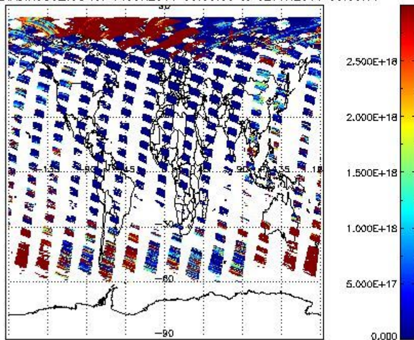
SCIO2P_NADIR3CO_vcd for 01JUN2011 00:00:00 to 02JUN2011 00:00:00
