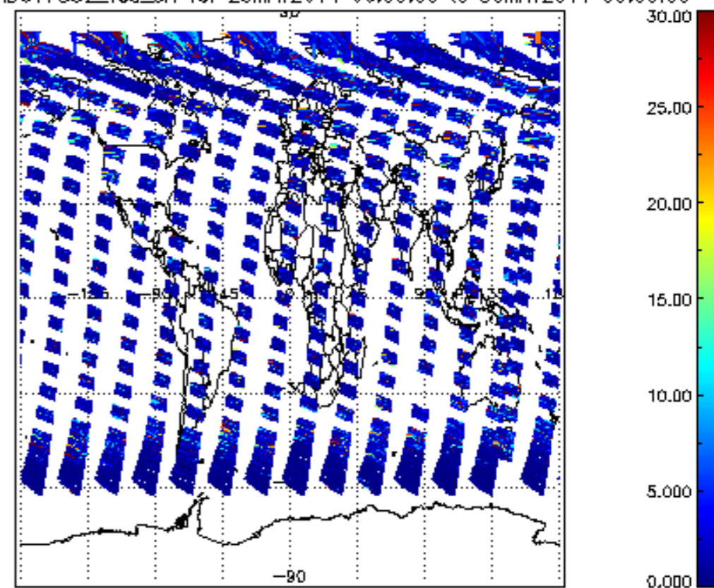
SCIOL2P_NADUV7S02_vcd_err for 29MAY2011 00:00:00 to 30MAY2011 00:00:00
