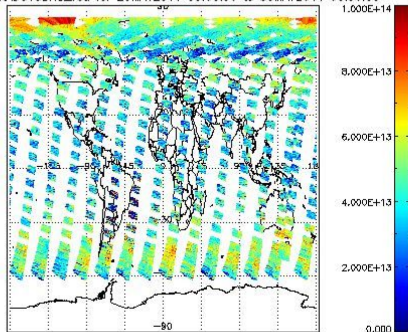
SCIOL2P_NADUV3BRO_vcd for 29MAY2011 00:00:00 to 30MAY2011 00:00:00
