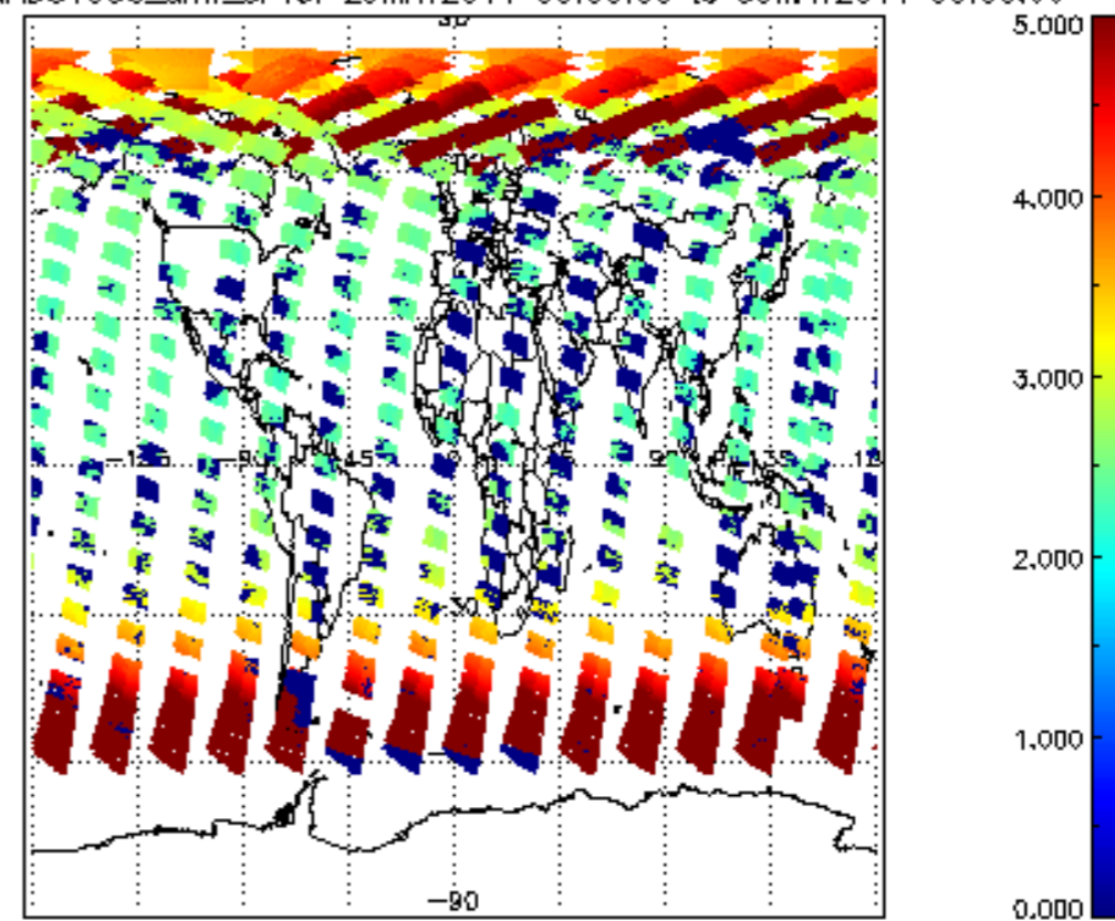
SCIOL2P_NADUV003_amf_cl for 29MAY2011 00:00:00 to 30MAY2011 00:00:00
