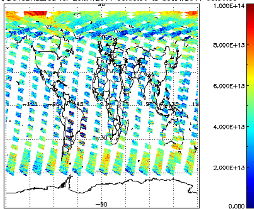
SCIOL2P_NADUV3BRO_vcd for 29MAY2011 00:00:00 to 30MAY2011 00:00:00
