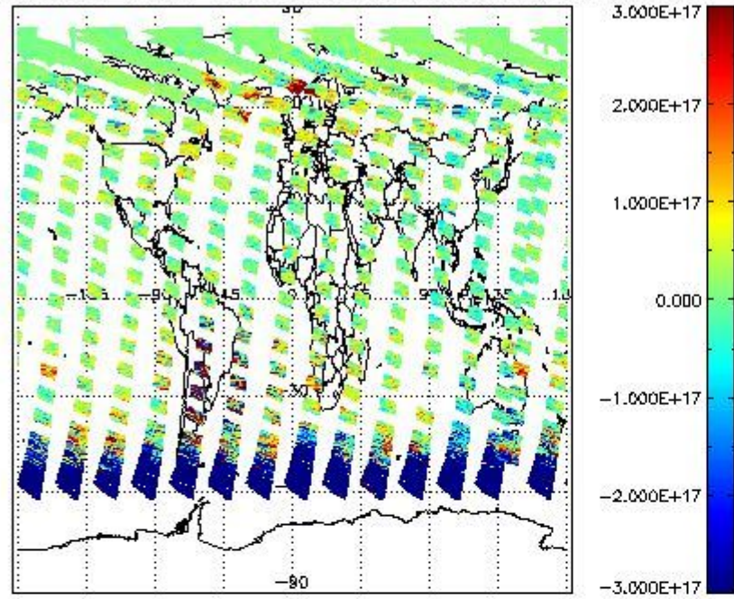
SCIOL2P_NADUV5S02_vcd for 29MAY2011 00:00:00 to 30MAY2011 00:00:00
