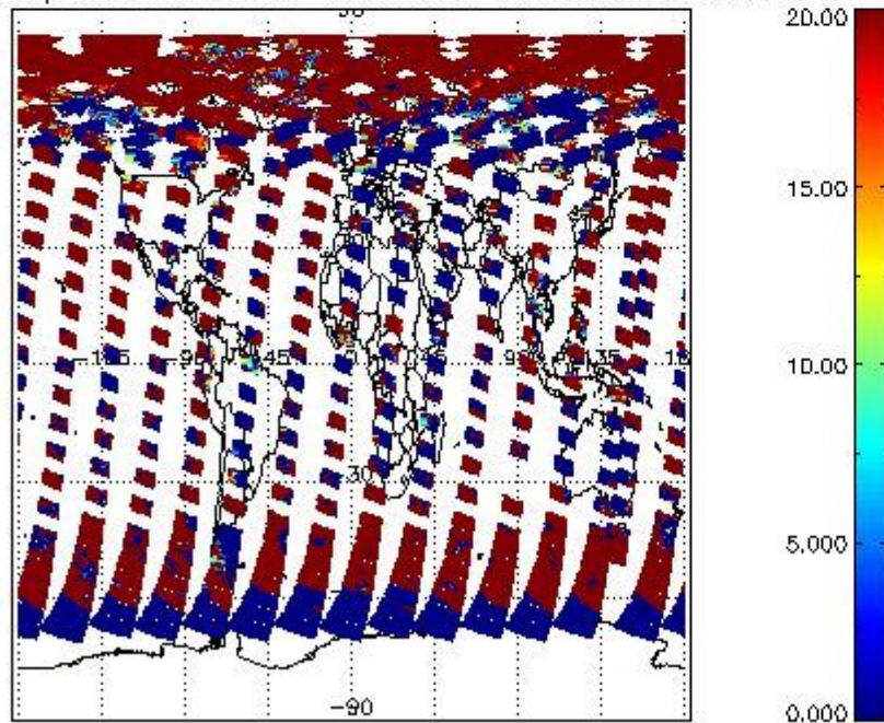
cL_opt_depth for 29MAY2011 00:00:00 to 30MAY2011 00:00:00
