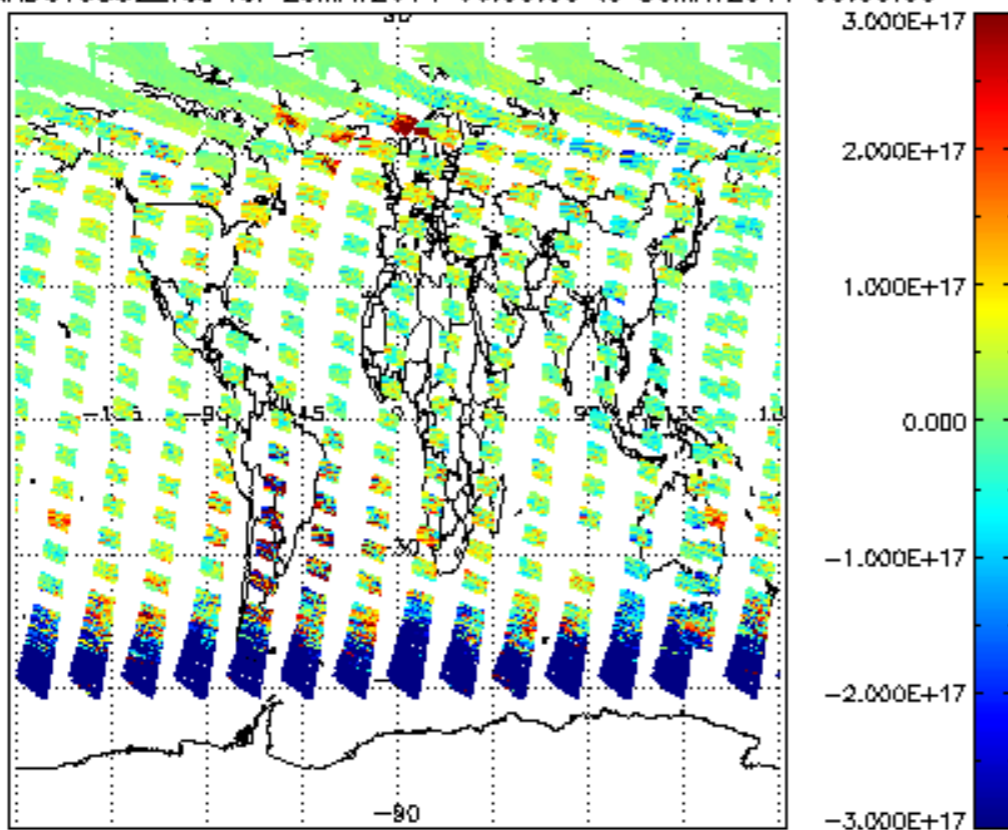
SCIOL2P_NADUV5S02_vcd for 29MAY2011 00:00:00 to 30MAY2011 00:00:00
