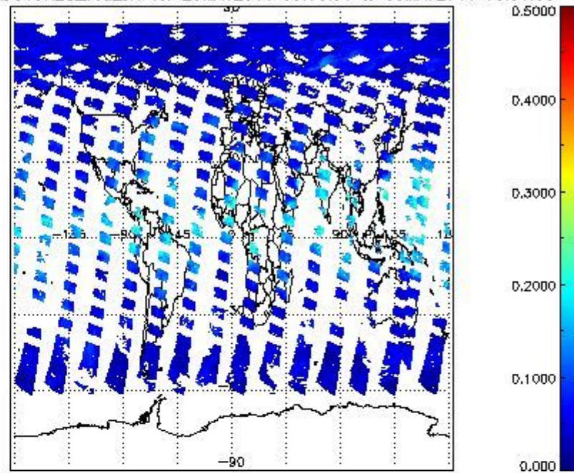
SCIOL2P_NADUV8H2O_vcd_err for 29MAY2011 00:00:00 to 30MAY2011 00:00:00
