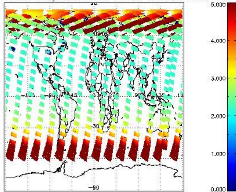
SCIOL2P_NADUV1NO2_amf_gr for 29MAY2011 00:00:00 to 30MAY2011 00:00:00
