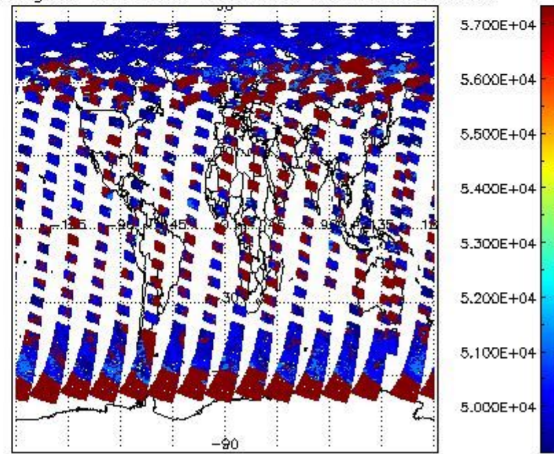
cloud_flags for 29MAY2011 00:00:00 to 30MAY2011 00:00:00
