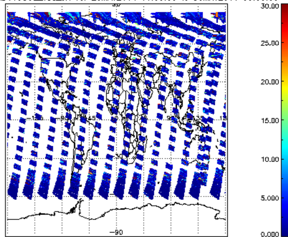
SCIOL2P_NADUV5S02_vcd_err for 29MAY2011 00:00:00 to 30MAY2011 00:00:00
