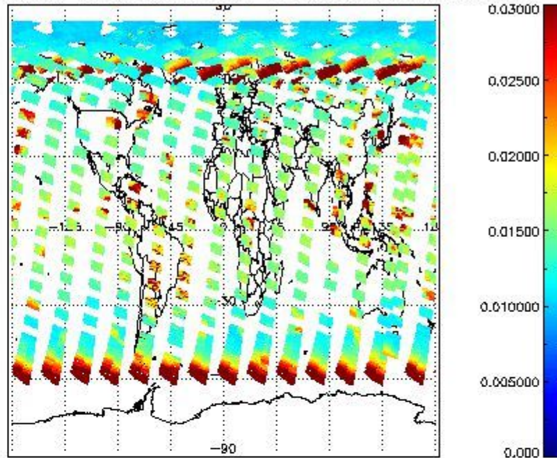
SCIOL2P_NADUV003_vcd_err for 29MAY2011 00:00:00 to 30MAY2011 00:00:00
