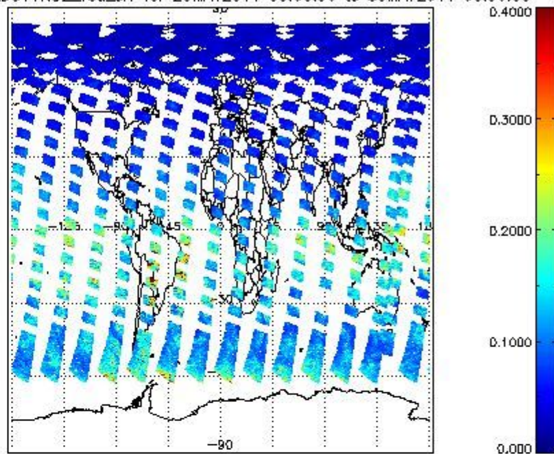
SCIOL2P_NADUV1NO2_vcd_err for 29MAY2011 00:00:00 to 30MAY2011 00:00:00
