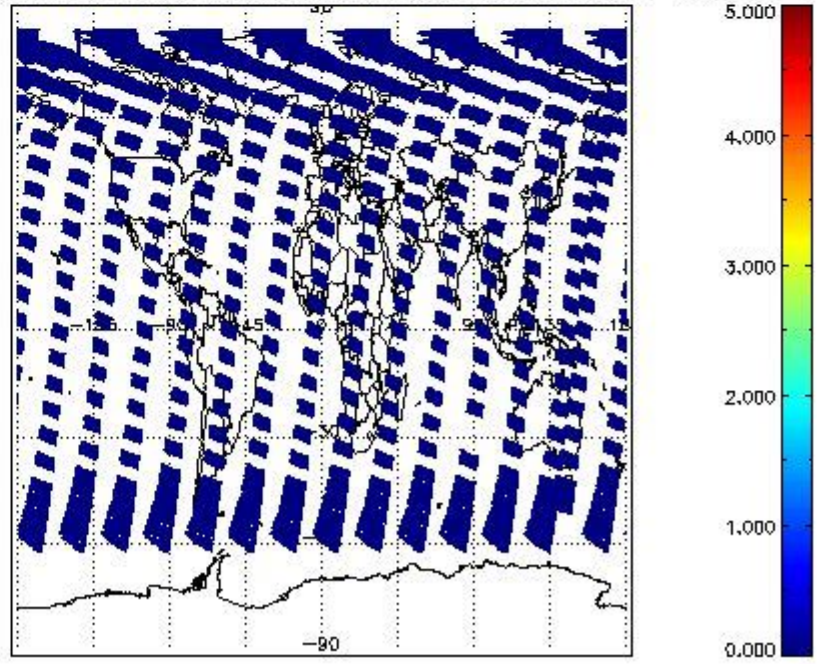
SCIOL2P_NADUV5S02_amf_cl for 29MAY2011 00:00:00 to 30MAY2011 00:00:00
