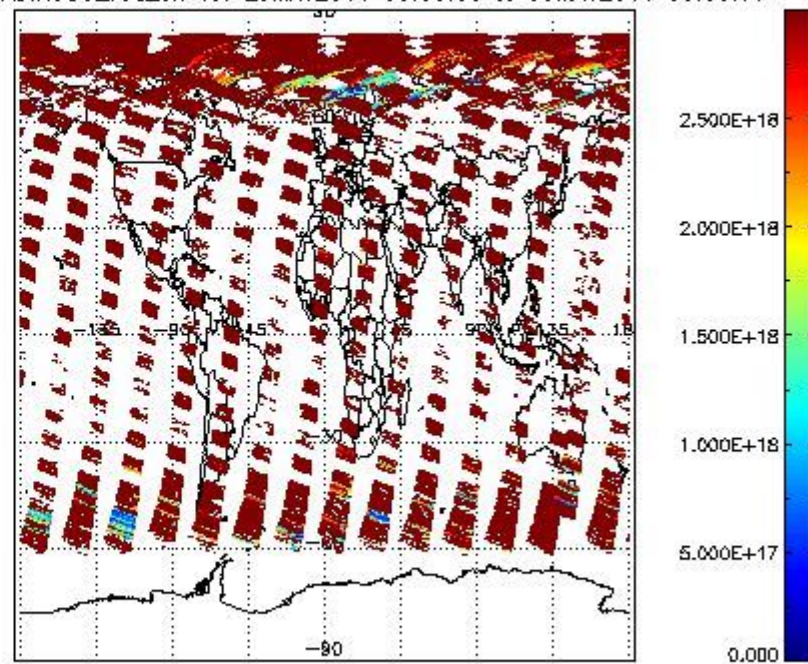
SCIDL2P_NADIR3CO_vcd_err for 29MAY2011 00:00:00 to 30MAY2011 00:00:00
