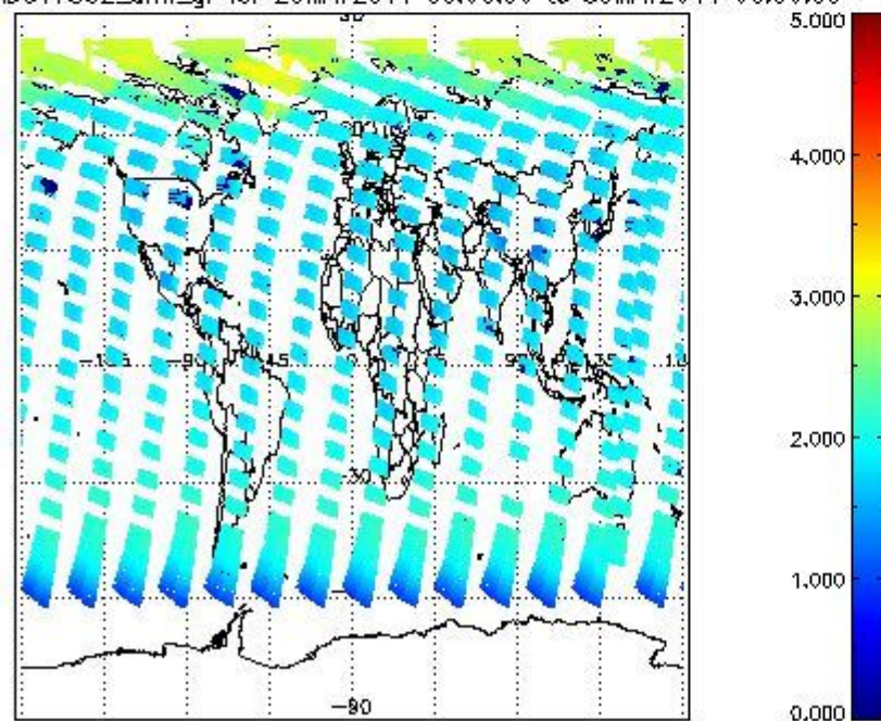
SCIOL2P_NADUV7S02_amf_gr for 29MAY2011 00:00:00 to 30MAY2011 00:00:00
