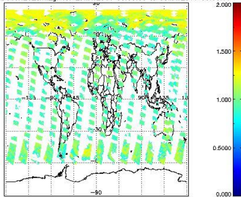
SCIOL2P_NADUV8H2O_arnf_gr for 29MAY2011 00:00:00 to 30MAY2011 00:00:00
