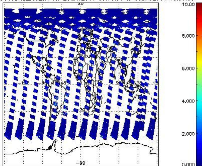
SCIOL2P_NADUV3BRO_vcd_err for 29MAY2011 00:00:00 to 30MAY2011 00:00:00
