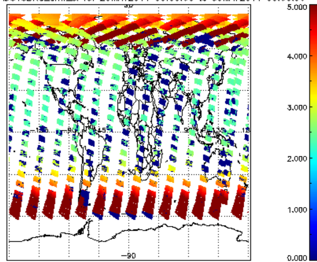
SCIOL2P_NADUV3BRO_amf_sl for 29MAY2011 00:00:00 to 30MAY2011 00:00:00
