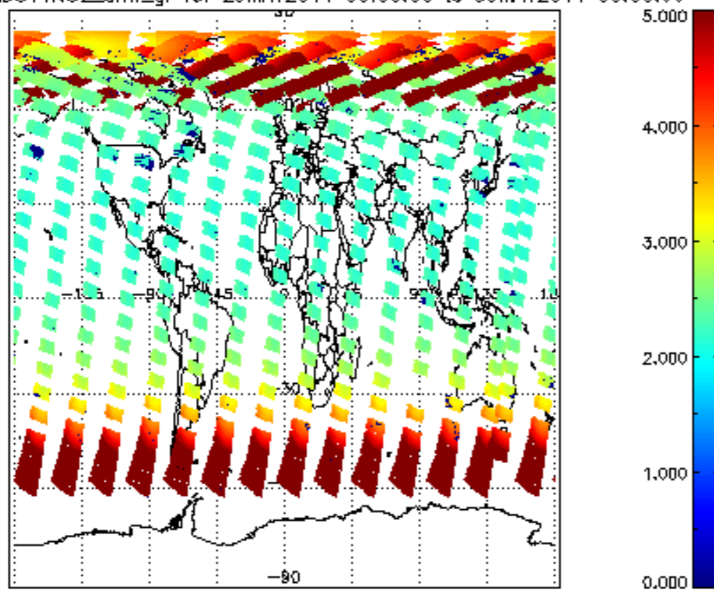
SCIOL2P_NADUV1NO2_amf_gr for 29MAY2011 00:00:00 to 30MAY2011 00:00:00
