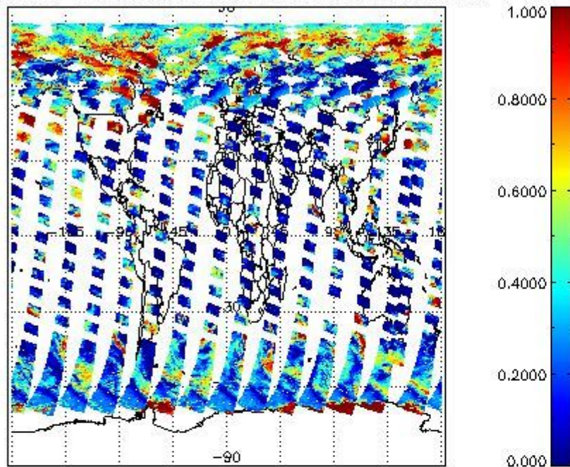
cL_frac for 29MAY2011 00:00:00 to 30MAY2011 00:00:00
