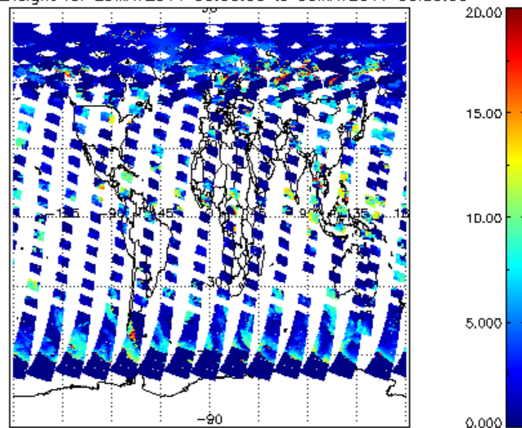
cL_top_height for 29MAY2011 00:00:00 to 30MAY2011 00:00:00
