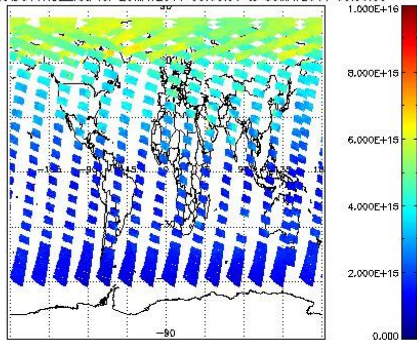
SCIOL2P_NADUV1NO2_vcd for 29MAY2011 00:00:00 to 30MAY2011 00:00:00
