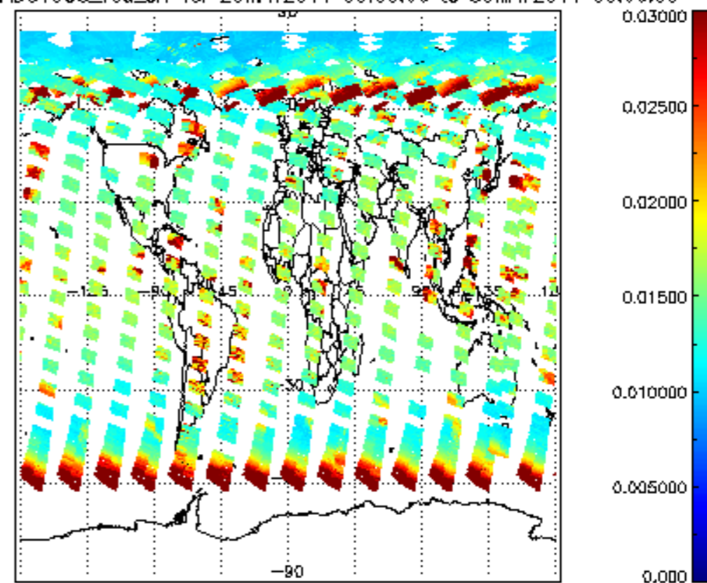
SCIOL2P_NADUV003_vcd_err for 29MAY2011 00:00:00 to 30MAY2011 00:00:00
