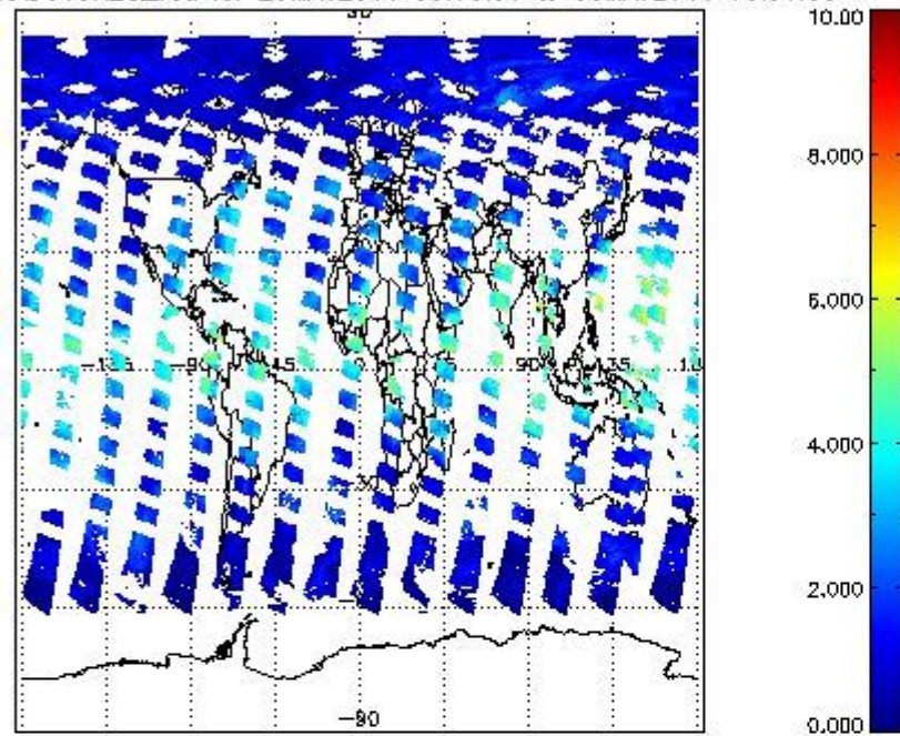
SCIOL2P_NADUV8H2O_vcd for 29MAY2011 00:00:00 to 30MAY2011 00:00:00
