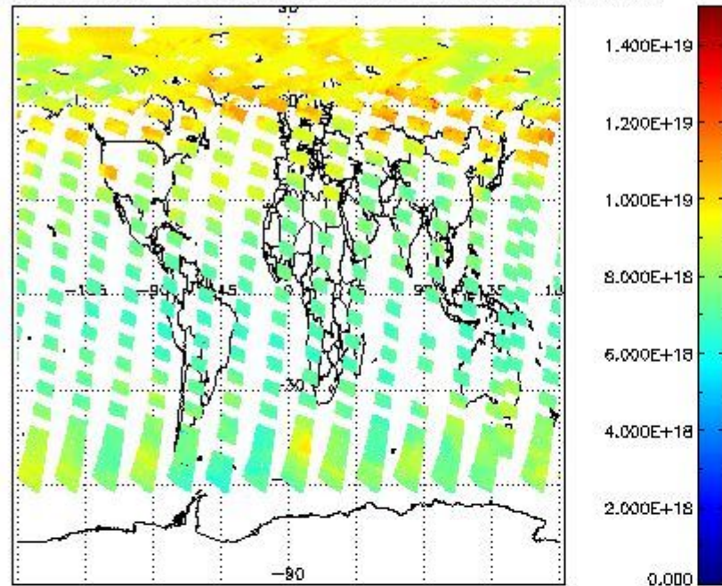
SCIOL2P_NADUV003_vcd for 29MAY2011 00:00:00 to 30MAY2011 00:00:00
