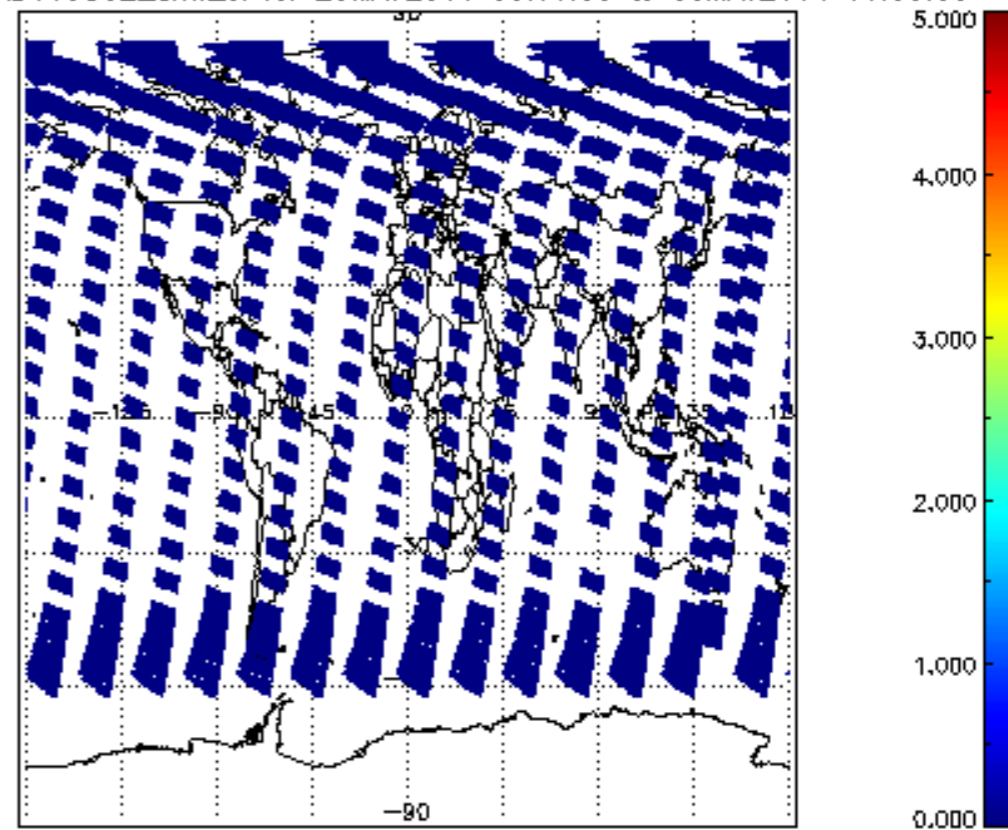
SCIOL2P_NADUV5S02_amf_cl for 29MAY2011 00:00:00 to 30MAY2011 00:00:00
