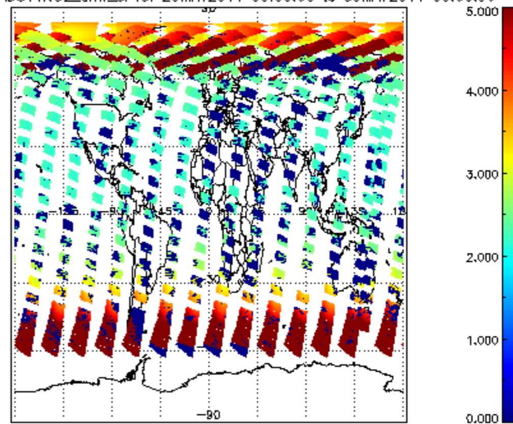
SCIOL2P_NADUV1NO2_amf_cl for 29MAY2011 00:00:00 to 30MAY2011 00:00:00
