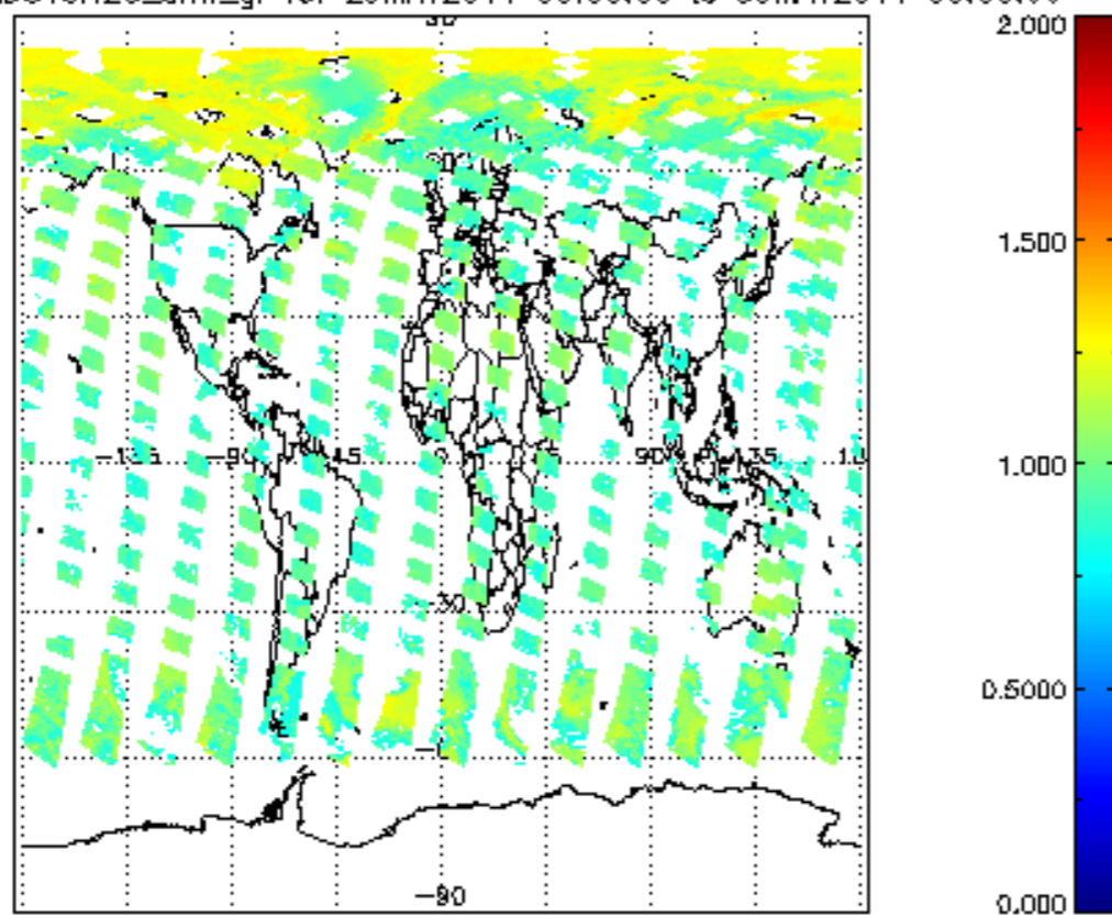
SCIOL2P_NADUV8H2O_amf_gr for 29MAY2011 00:00:00 to 30MAY2011 00:00:00
