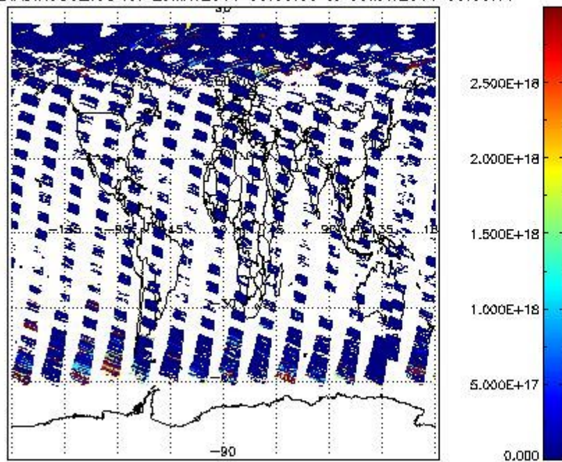
SCIDL2P_NADIR3CO_vcd for 29MAY2011 00:00:00 to 30MAY2011 00:00:00
