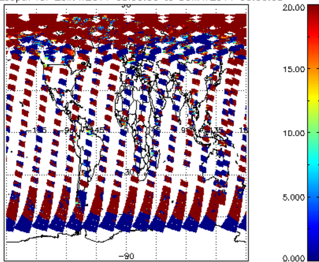
cL_opt_depth for 29MAY2011 00:00:00 to 30MAY2011 00:00:00
