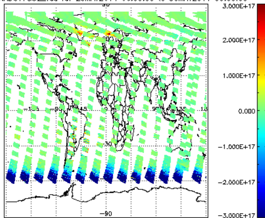
SCIOL2P_NADUV7S02_vcd for 29MAY2011 00:00:00 to 30MAY2011 00:00:00
