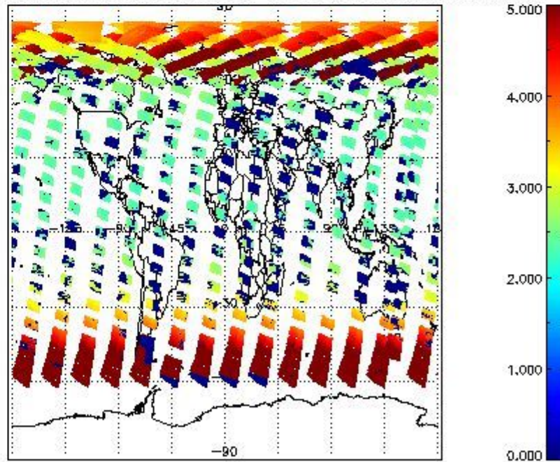
SCIOL2P_NADUV003_amf_cl for 29MAY2011 00:00:00 to 30MAY2011 00:00:00
