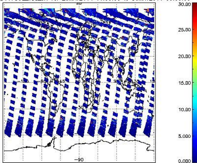
SCIOL2P_NADUV7S02_vcd_err for 29MAY2011 00:00:00 to 30MAY2011 00:00:00
