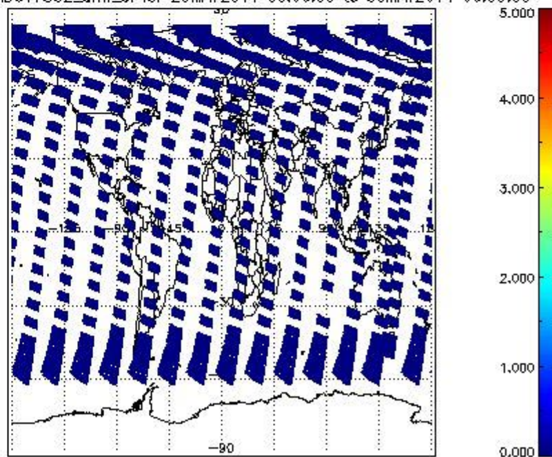
SCIOL2P_NADUV7S02_amf_cl for 29MAY2011 00:00:00 to 30MAY2011 00:00:00
