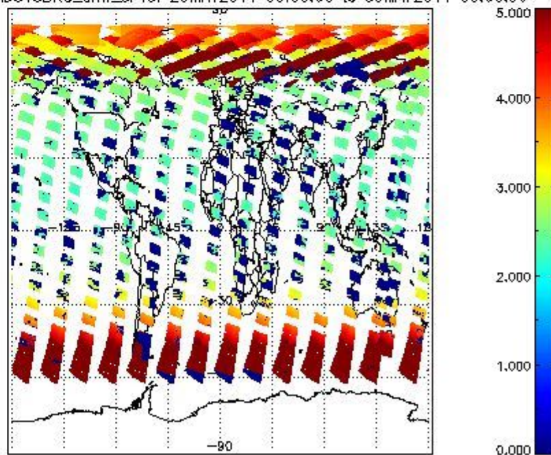
SCIOL2P_NADUV3BRO_amf_cl for 29MAY2011 00:00:00 to 30MAY2011 00:00:00
