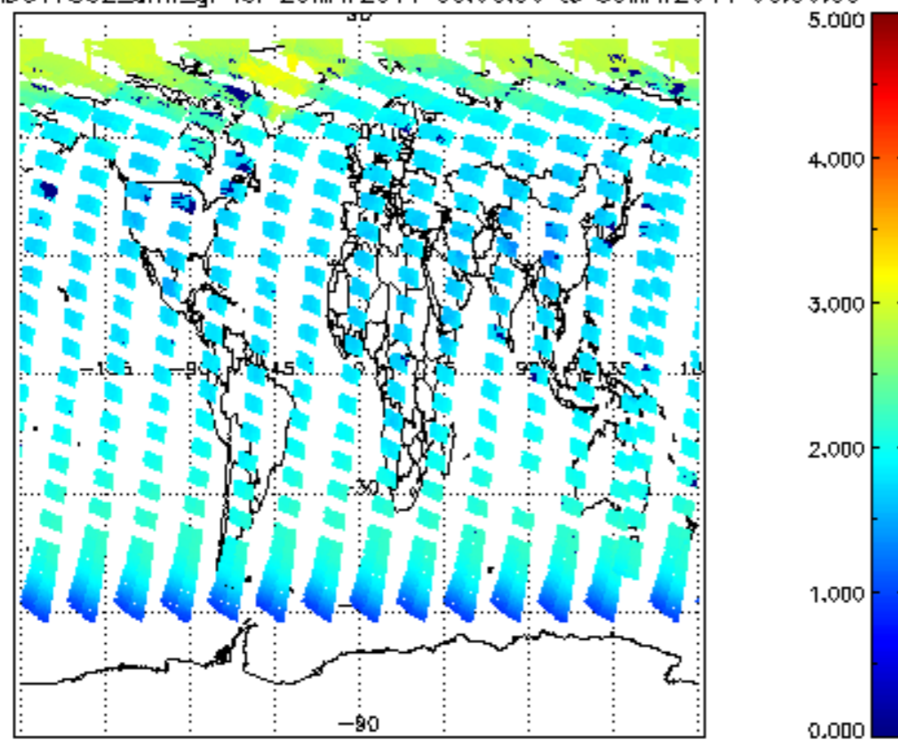
SCIOL2P_NADUV7S02_amf_gr for 29MAY2011 00:00:00 to 30MAY2011 00:00:00
