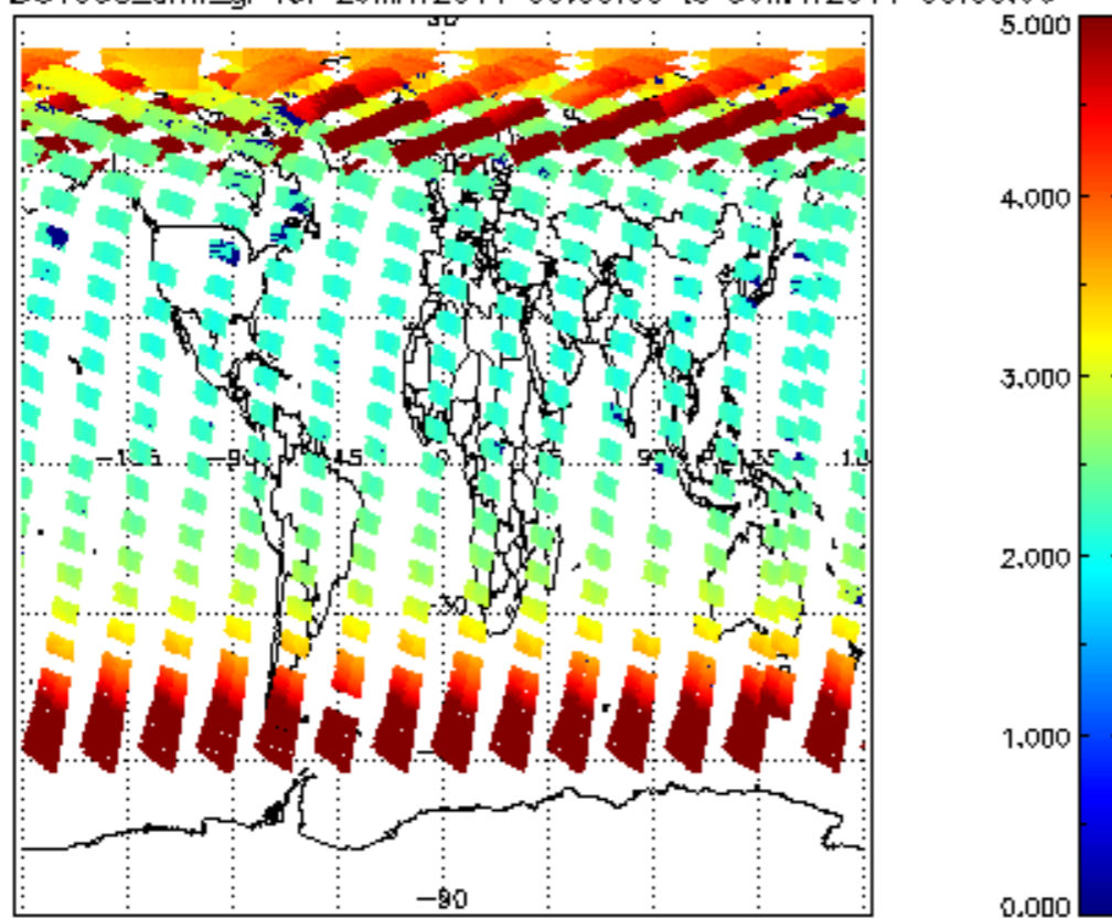
SCIOL2P_NADUV003_amf_gr for 29MAY2011 00:00:00 to 30MAY2011 00:00:00
