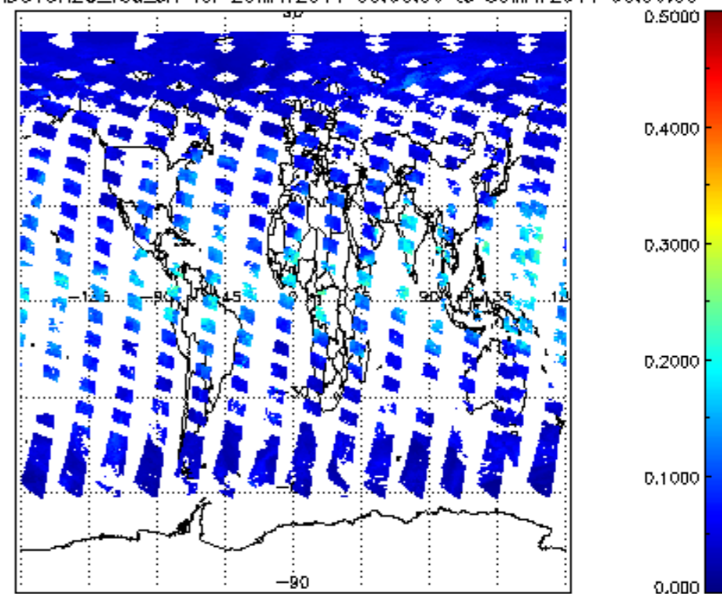
SCIOL2P_NADUV8H2O_vcd_err for 29MAY2011 00:00:00 to 30MAY2011 00:00:00
