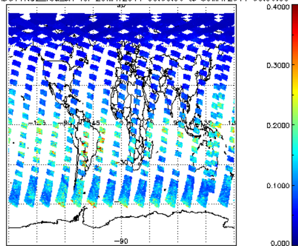
SCIOL2P_NADUV1NO2_vcd_err for 29MAY2011 00:00:00 to 30MAY2011 00:00:00
