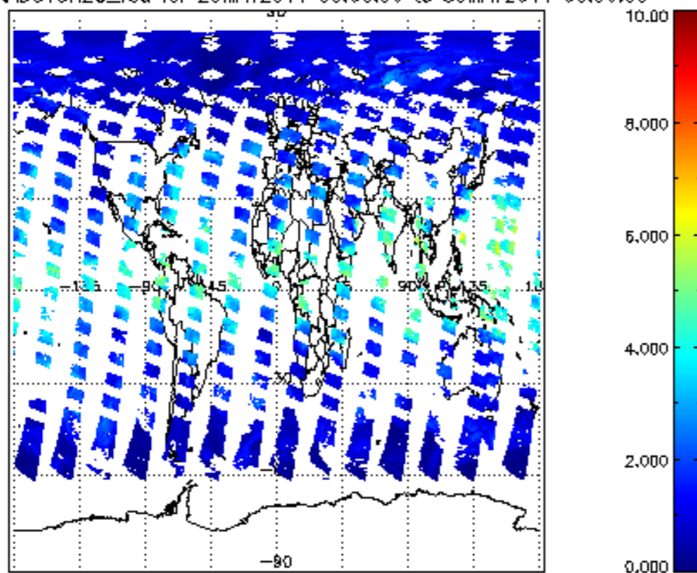
SCIOL2P_NADUV8H2O_vcd for 29MAY2011 00:00:00 to 30MAY2011 00:00:00
