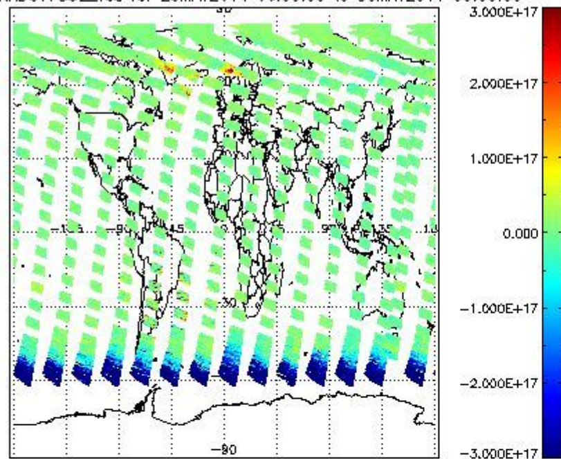
SCIOL2P_NADUV7S02_vcd for 29MAY2011 00:00:00 to 30MAY2011 00:00:00
