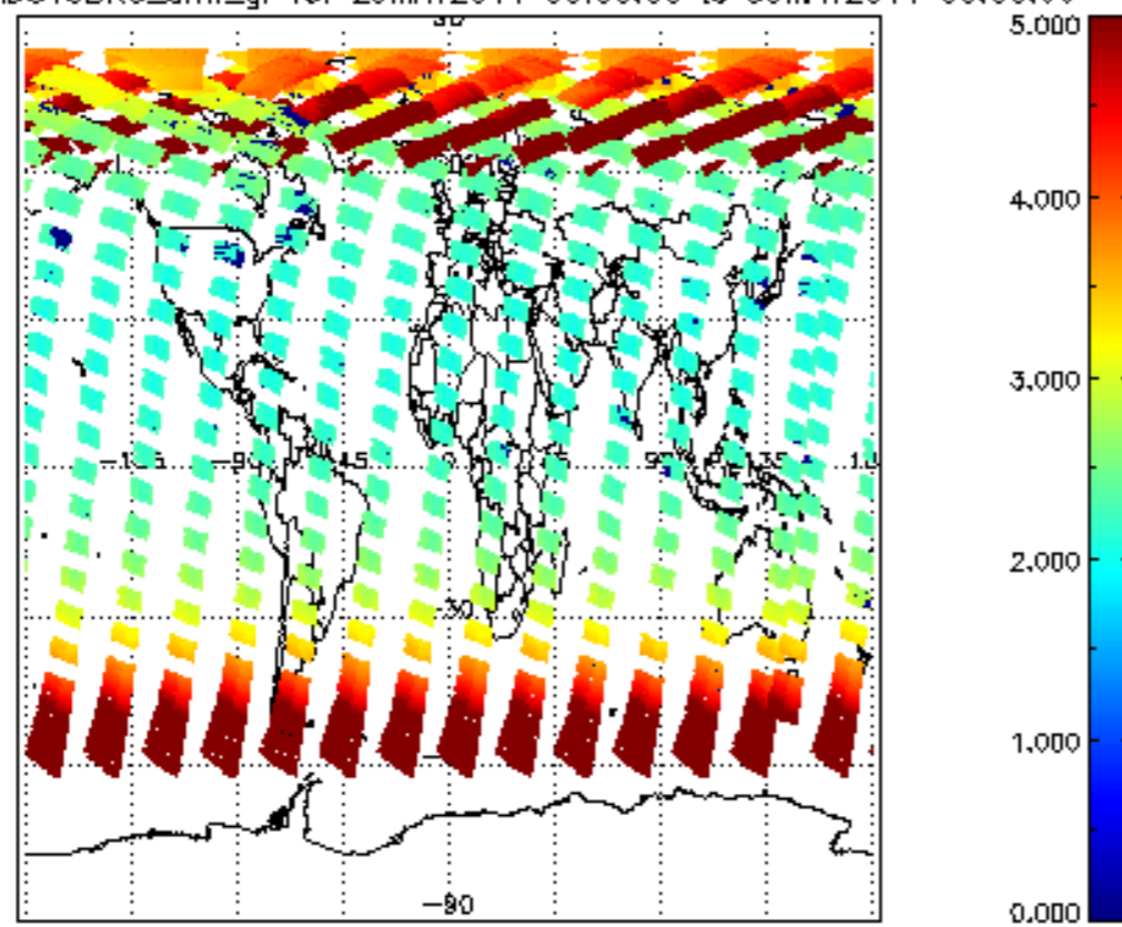
SCIOL2P_NADUV3BRO_amf_gr for 29MAY2011 00:00:00 to 30MAY2011 00:00:00
