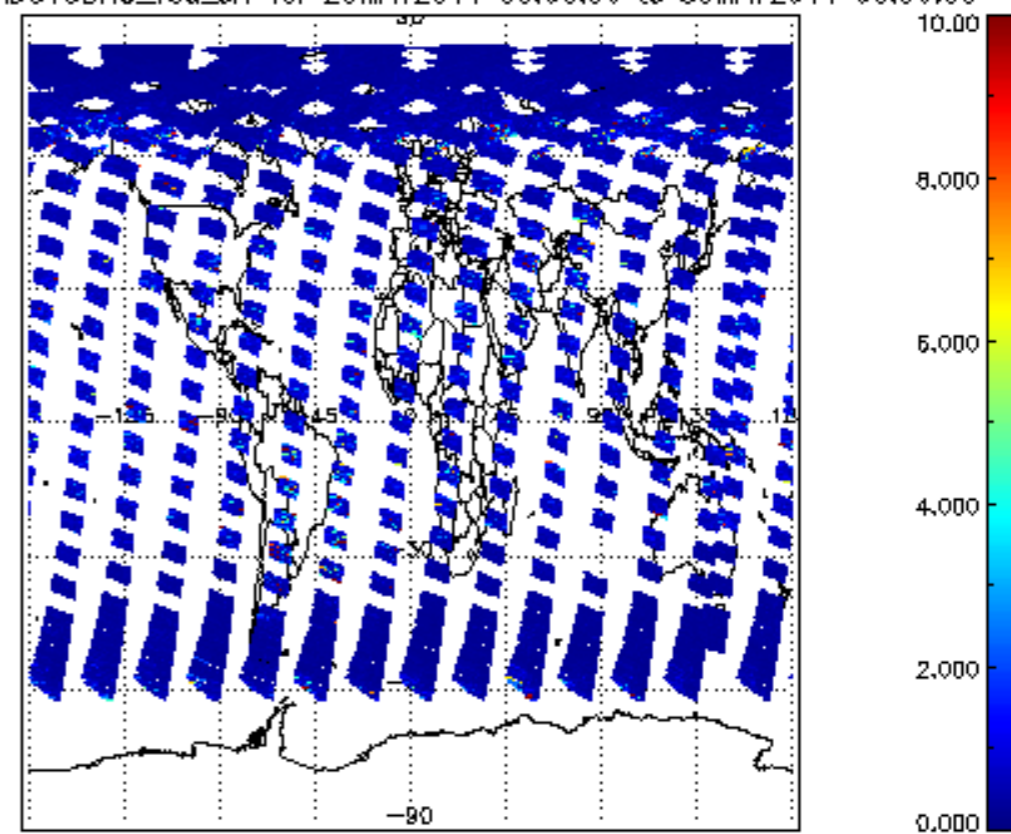
SCIOL2P_NADUV3BRO_vcd_err for 29MAY2011 00:00:00 to 30MAY2011 00:00:00
