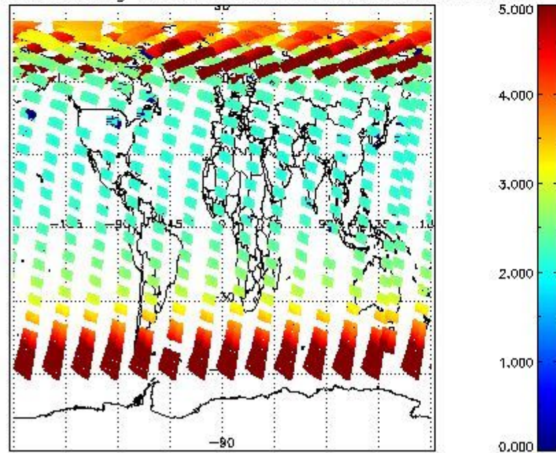
SCIOL2P_NADUV003_amf_gr for 29MAY2011 00:00:00 to 30MAY2011 00:00:00
