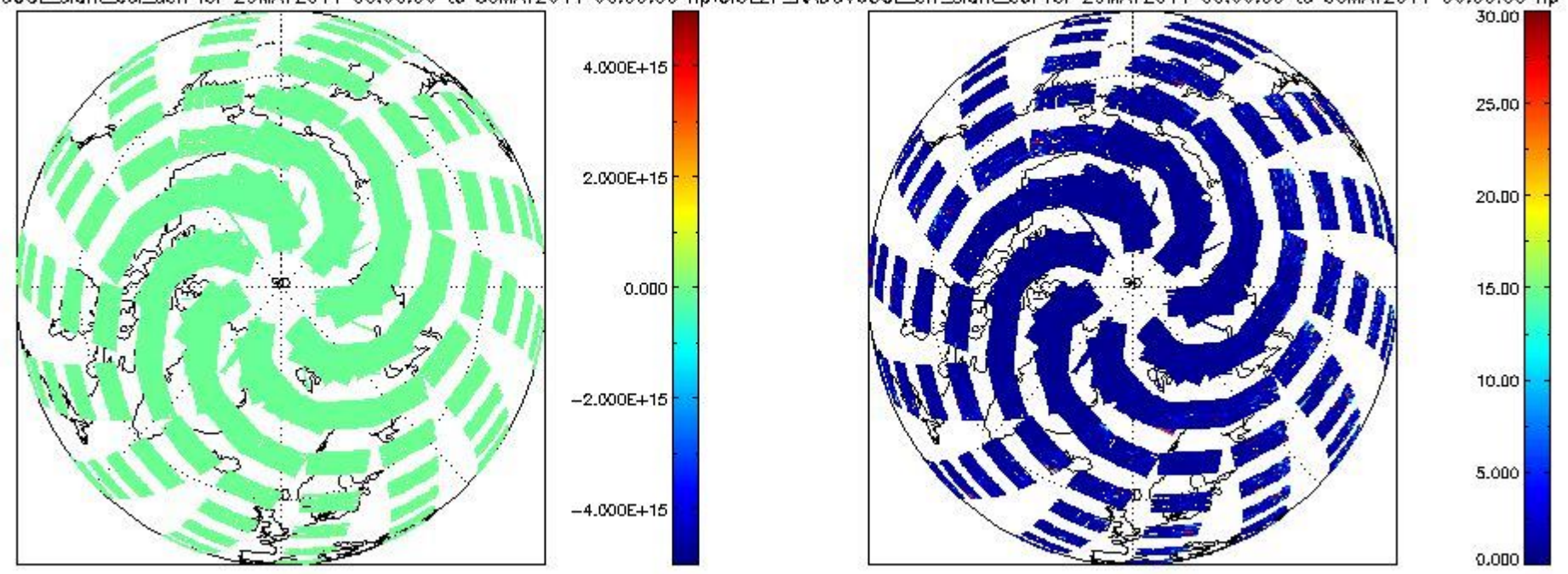
CIOL2P_NADUV6OCLslant_col_den for 29MAY2011 00:00:00 to 30MAY2011 00:00:00 np; CIOL2P_NADUV6OCLerr_slant_col for 29MAY2011 00:00:00 to 30MAY2011 00:00:00 np
