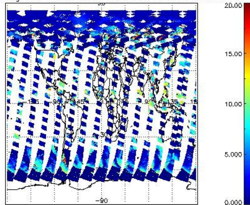
cL_top_height for 29MAY2011 00:00:00 to 30MAY2011 00:00:00
