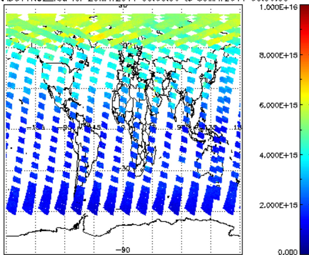
SCIOL2P_NADUV1NO2_vcd for 29MAY2011 00:00:00 to 30MAY2011 00:00:00
