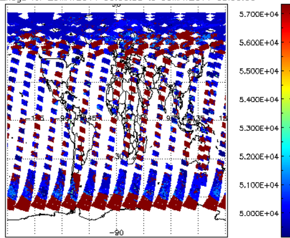
cloud_flags for 29MAY2011 00:00:00 to 30MAY2011 00:00:00
