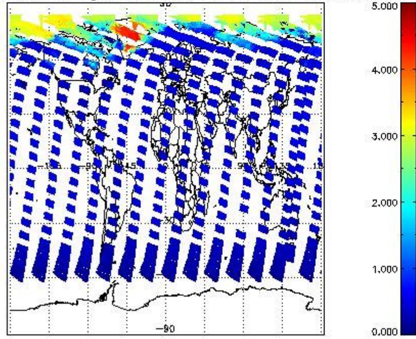
SCIOL2P_NADUV5S02_amf_gr for 29MAY2011 00:00:00 to 30MAY2011 00:00:00
