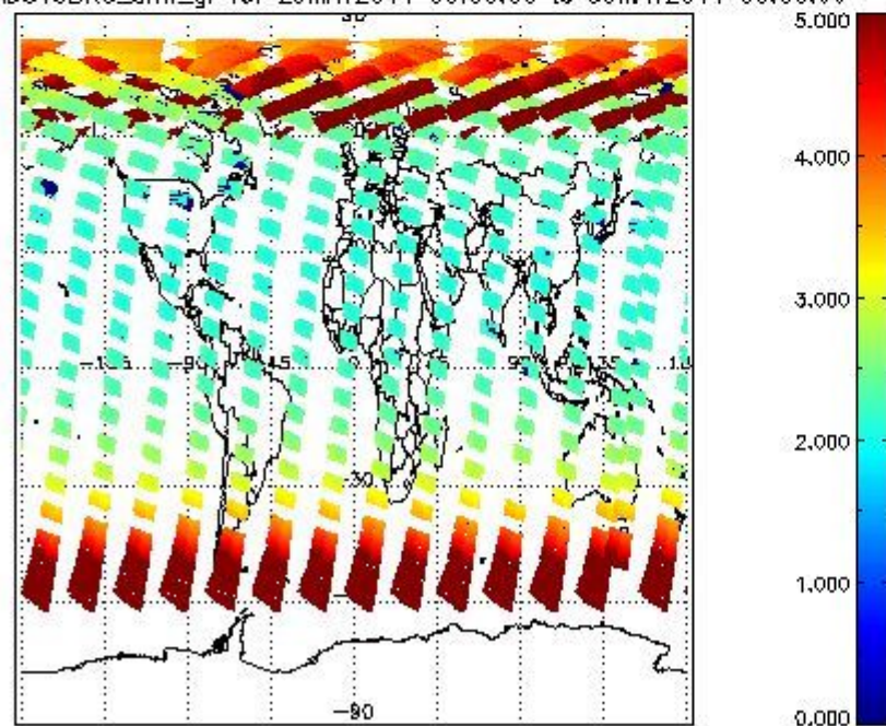
SCIOL2P_NADUV3BRO_amf_gr for 29MAY2011 00:00:00 to 30MAY2011 00:00:00
