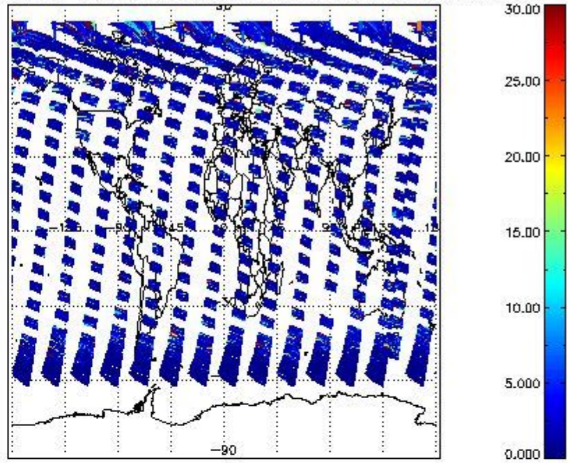
SCIOL2P_NADUV5S02_vcd_err for 29MAY2011 00:00:00 to 30MAY2011 00:00:00
