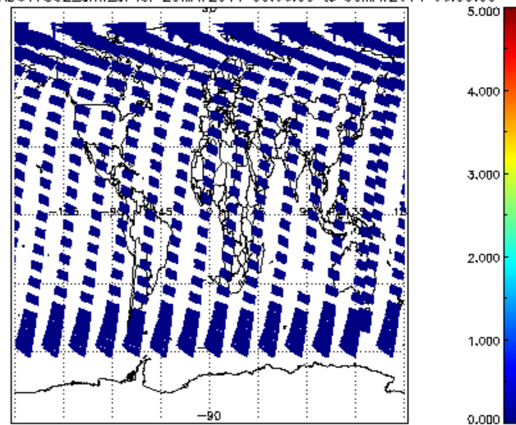
SCIOL2P_NADUV7S02_amf_cl for 29MAY2011 00:00:00 to 30MAY2011 00:00:00
