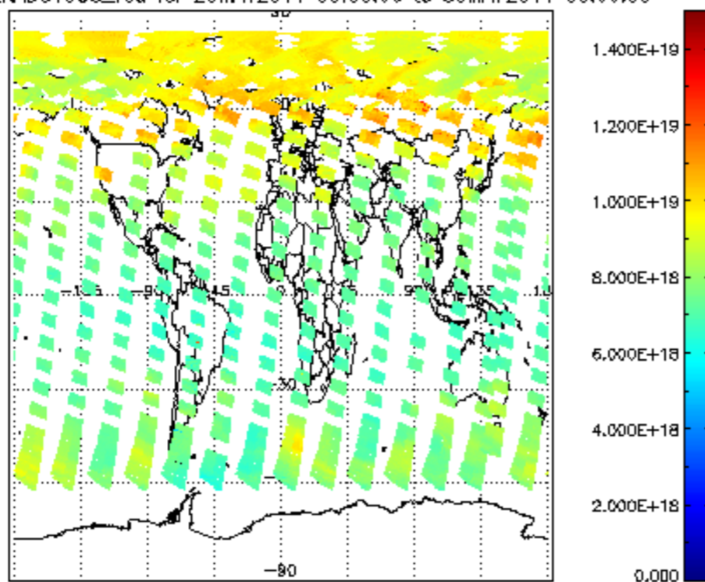
SCIOL2P_NADUV003_vcd for 29MAY2011 00:00:00 to 30MAY2011 00:00:00
