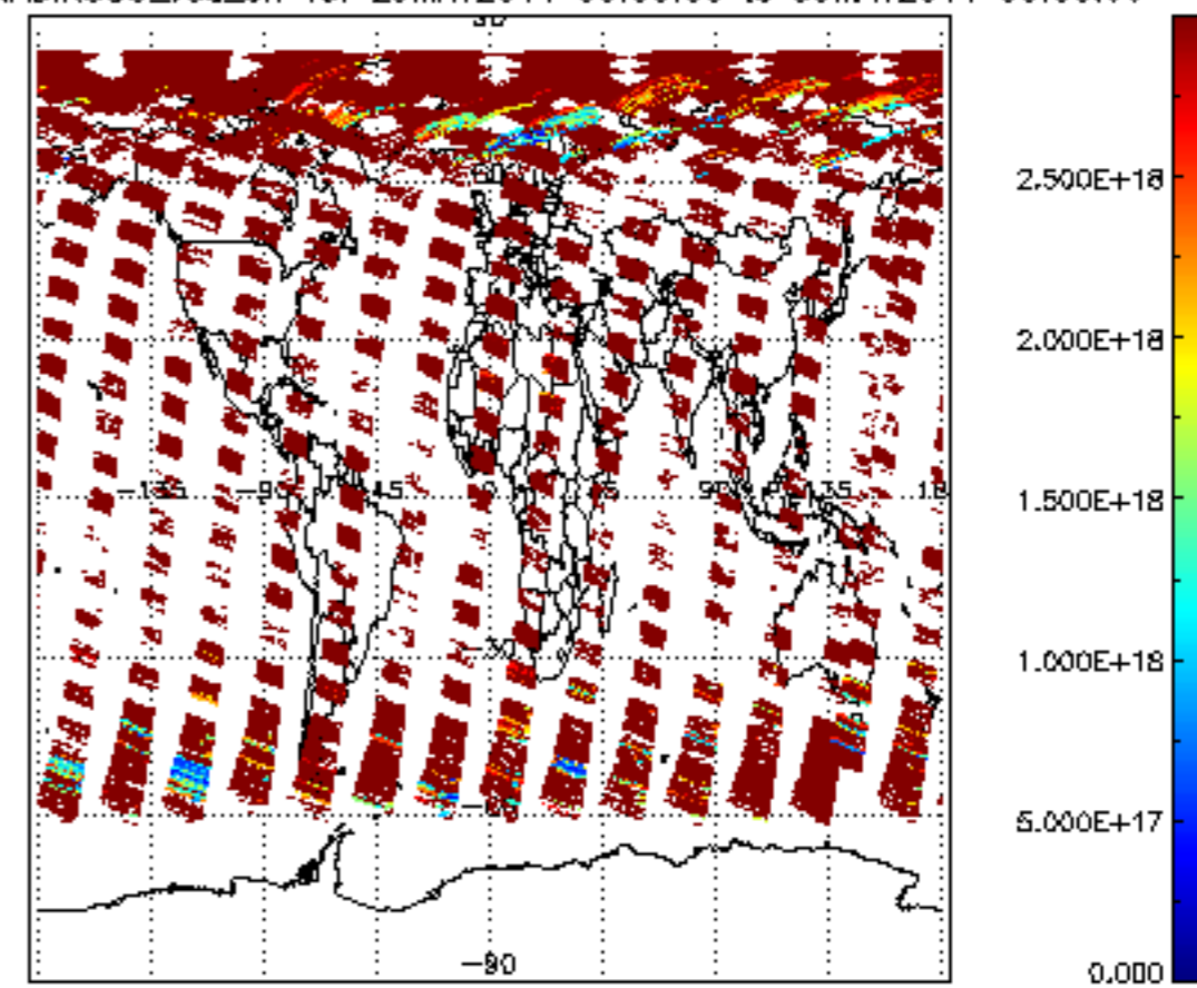
SCIOL2P_NADIR3CO_vcd_err for 29MAY2011 00:00:00 to 30MAY2011 00:00:00
