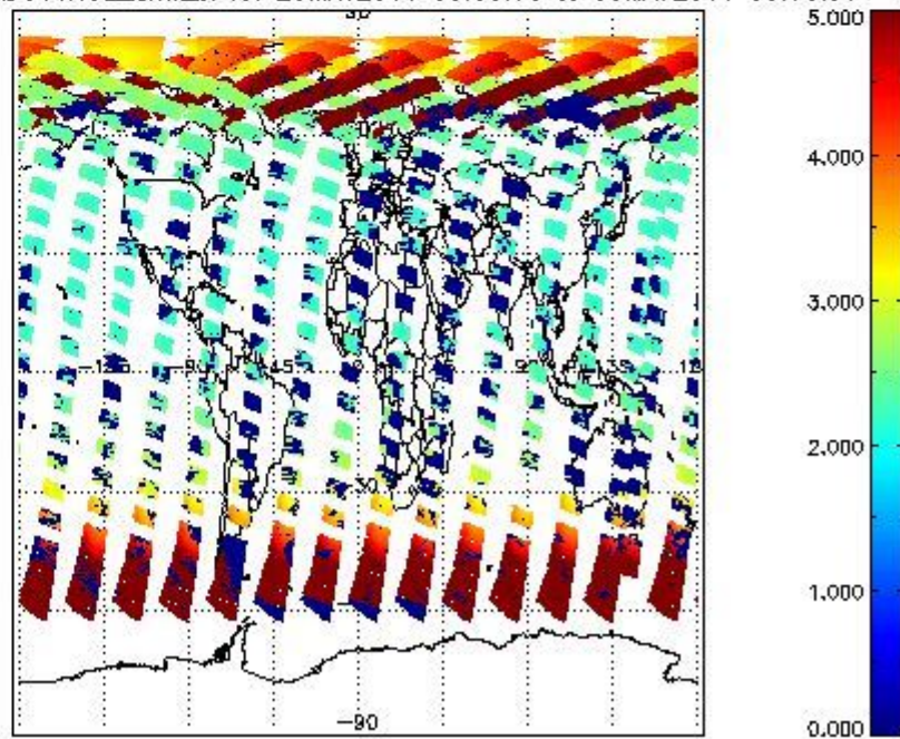
SCIOL2P_NADUV1NO2_amf_cl for 29MAY2011 00:00:00 to 30MAY2011 00:00:00
