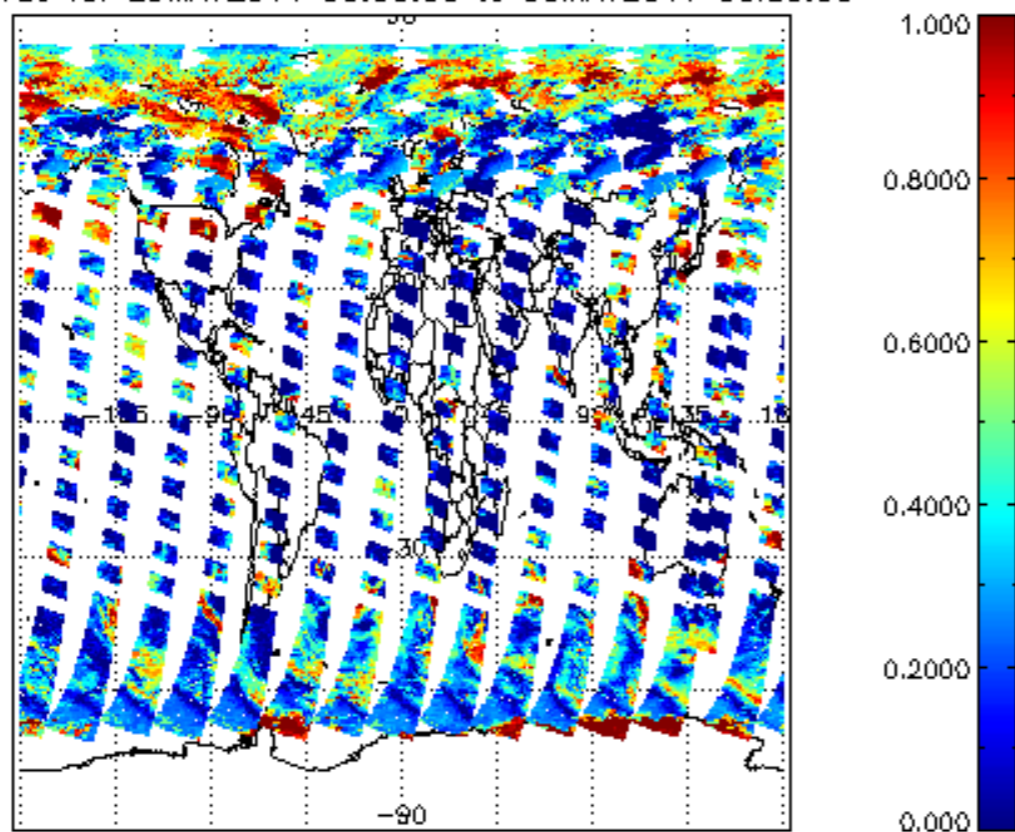
cL_frac for 29MAY2011 00:00:00 to 30MAY2011 00:00:00
