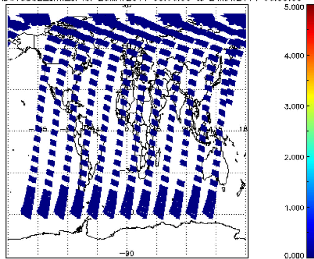
SCIOL2P_NADUV5S02_amf_cl for 23MAY2011 00:00:00 to 24MAY2011 00:00:00
