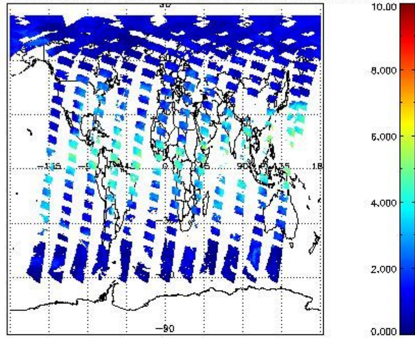
SCIOL2P_NADUV8H2O_vcd for 23MAY2011 00:00:00 to 24MAY2011 00:00:00
