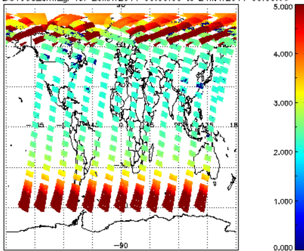
SCIOL2P_NADUV003_amf_gr for 23MAY2011 00:00:00 to 24MAY2011 00:00:00
