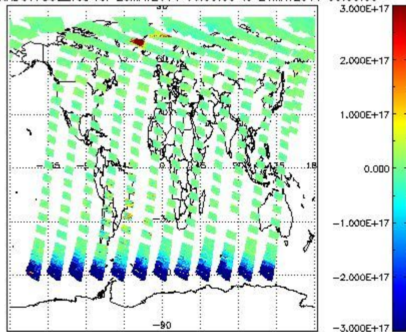
SCIOL2P_NADUV7S02_vcd for 23MAY2011 00:00:00 to 24MAY2011 00:00:00
