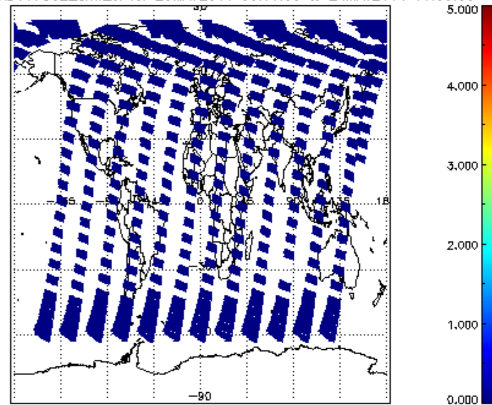
SCIOL2P_NADUV7S02_amf_cl for 23MAY2011 00:00:00 to 24MAY2011 00:00:00
