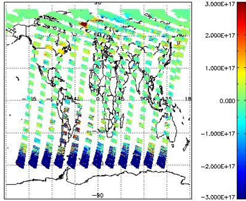
SCIOL2P_NADUV5S02_vcd for 23MAY2011 00:00:00 to 24MAY2011 00:00:00
