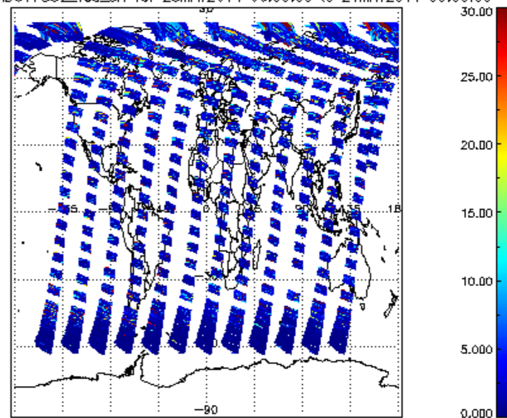
SCIOL2P_NADUV7S02_vcd_err for 23MAY2011 00:00:00 to 24MAY2011 00:00:00
