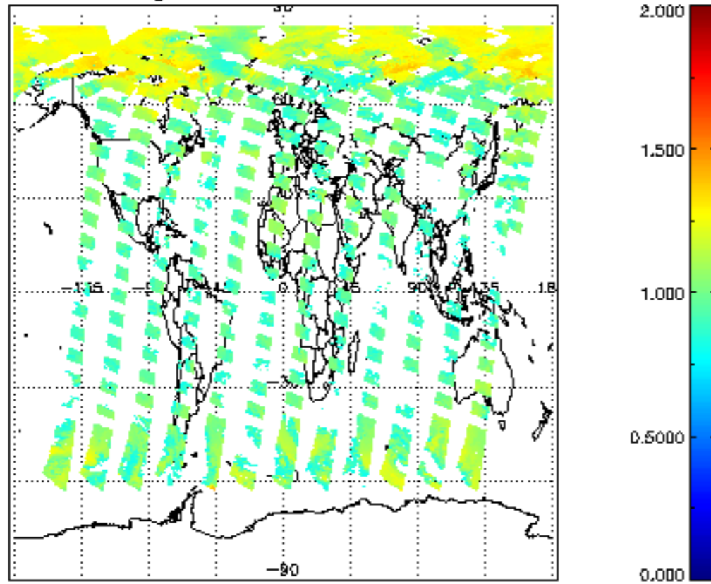
SCIOL2P_NADUV8H2O_amf_gr for 23MAY2011 00:00:00 to 24MAY2011 00:00:00
