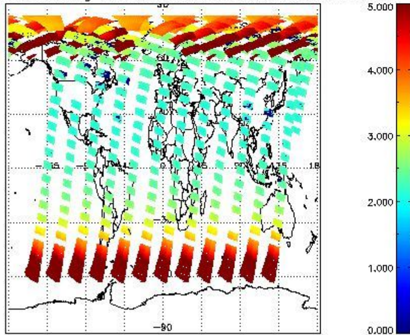
SCIOL2P_NADUV003_amf_gr for 23MAY2011 00:00:00 to 24MAY2011 00:00:00
