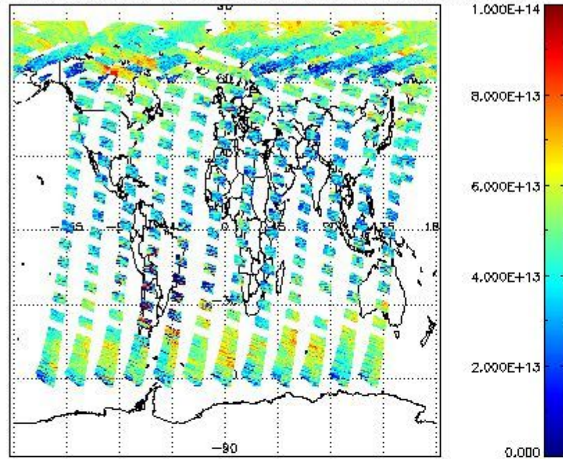
SCIOL2P_NADUV3BRO_vcd for 23MAY2011 00:00:00 to 24MAY2011 00:00:00
