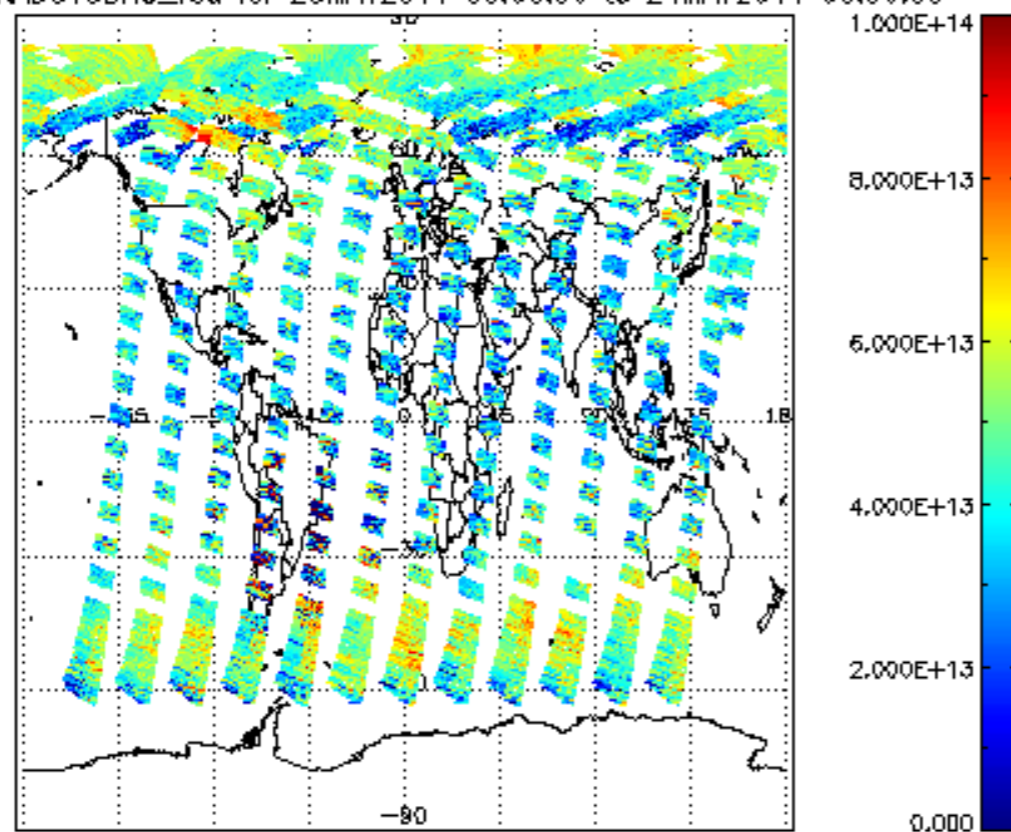
SCIOL2P_NADUV3BRO_vcd for 23MAY2011 00:00:00 to 24MAY2011 00:00:00
