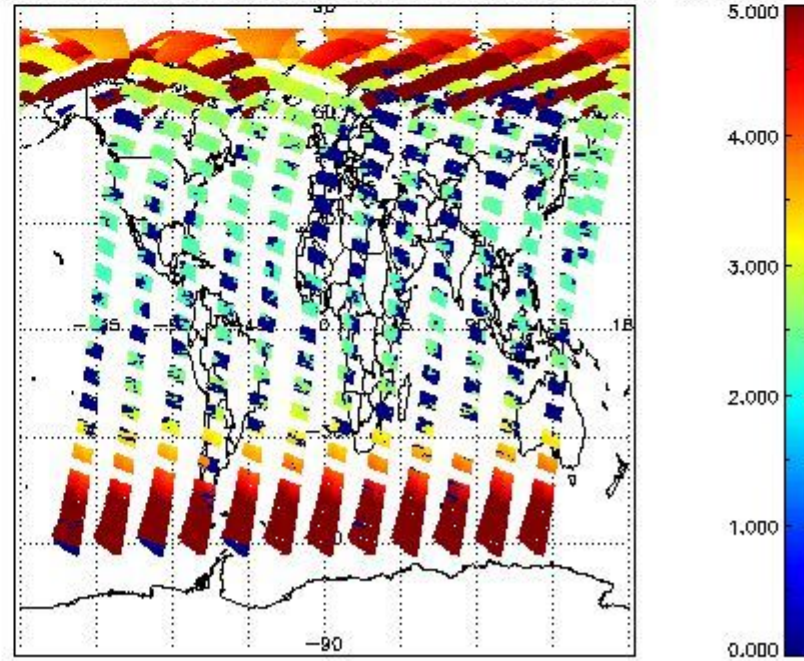
SCIOL2P_NADUV3BRO_amf_cl for 23MAY2011 00:00:00 to 24MAY2011 00:00:00
