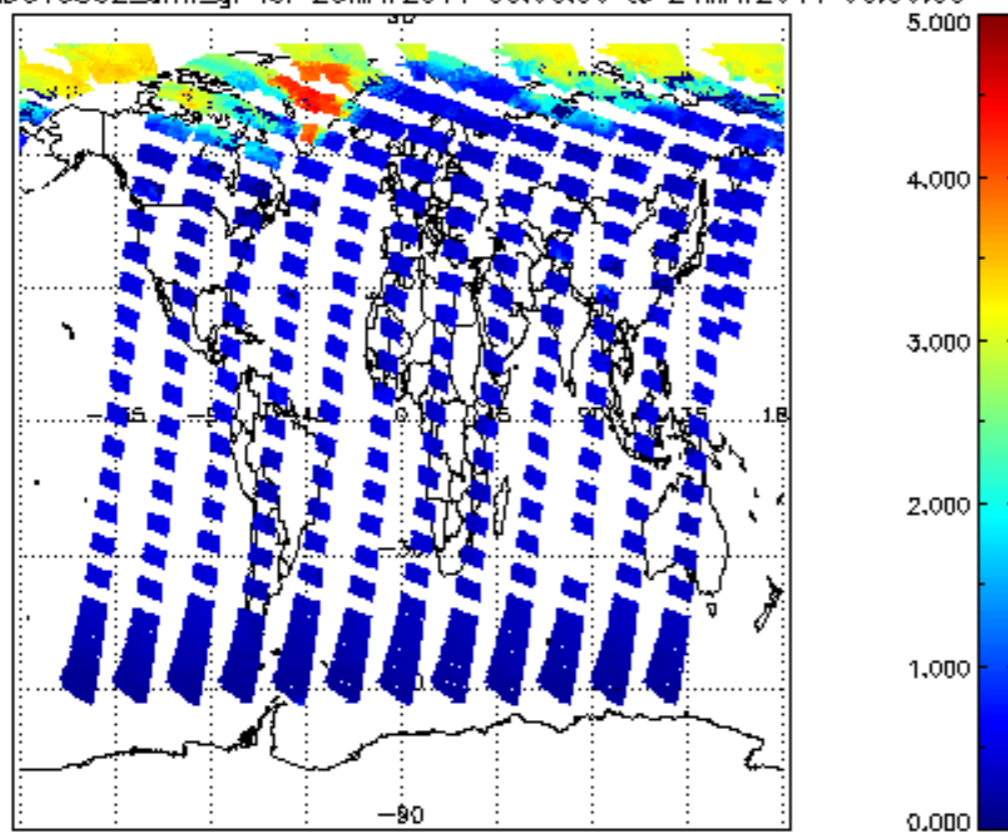
SCIOL2P_NADUV5S02_amf_gr for 23MAY2011 00:00:00 to 24MAY2011 00:00:00
