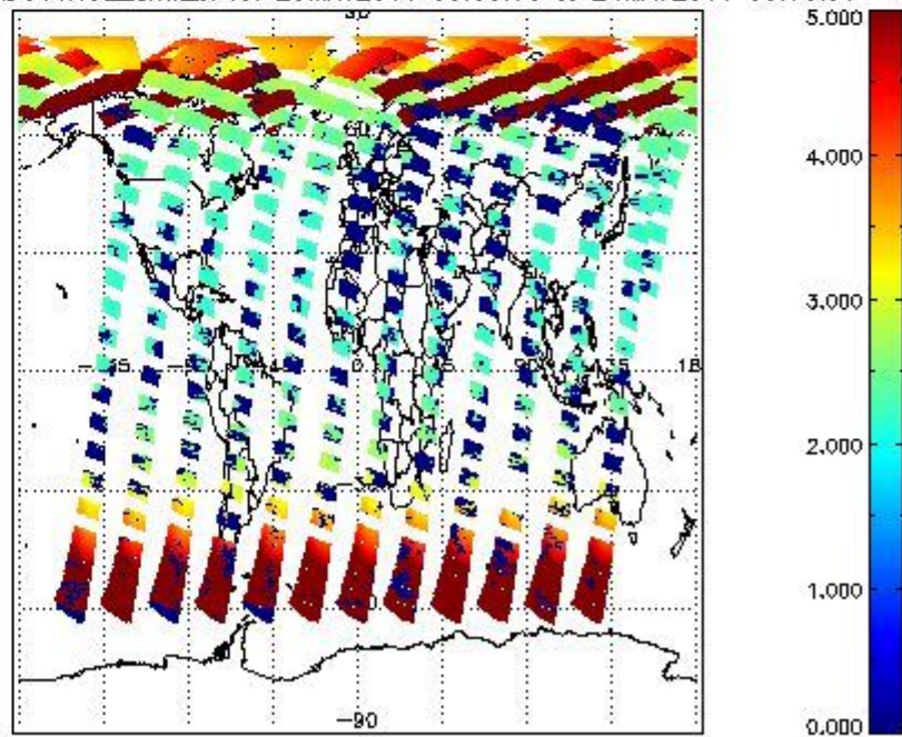
SCIOL2P_NADUV1NO2_amf_cl for 23MAY2011 00:00:00 to 24MAY2011 00:00:00
