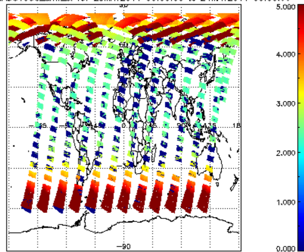
SCIOL2P_NADUV003_amf_cl for 23MAY2011 00:00:00 to 24MAY2011 00:00:00
