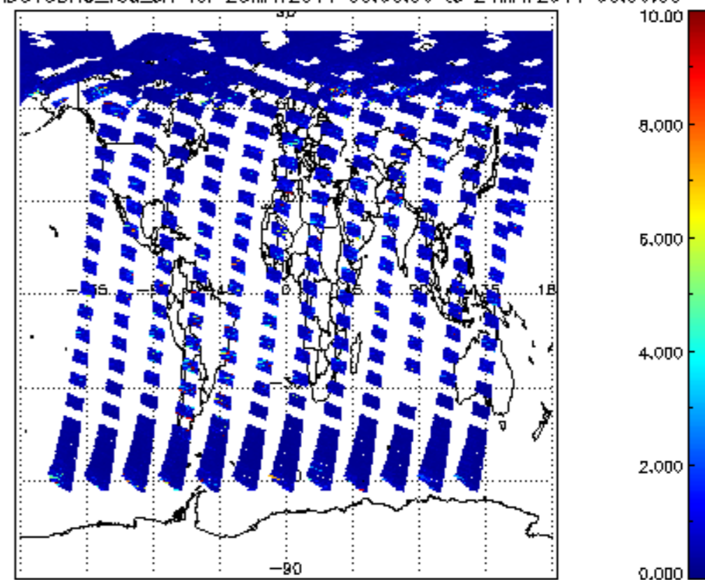
SCIOL2P_NADUV3BRO_vcd_err for 23MAY2011 00:00:00 to 24MAY2011 00:00:00
