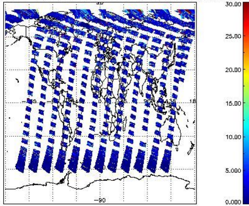
SCIOL2P_NADUV5S02_vcd_err for 23MAY2011 00:00:00 to 24MAY2011 00:00:00
