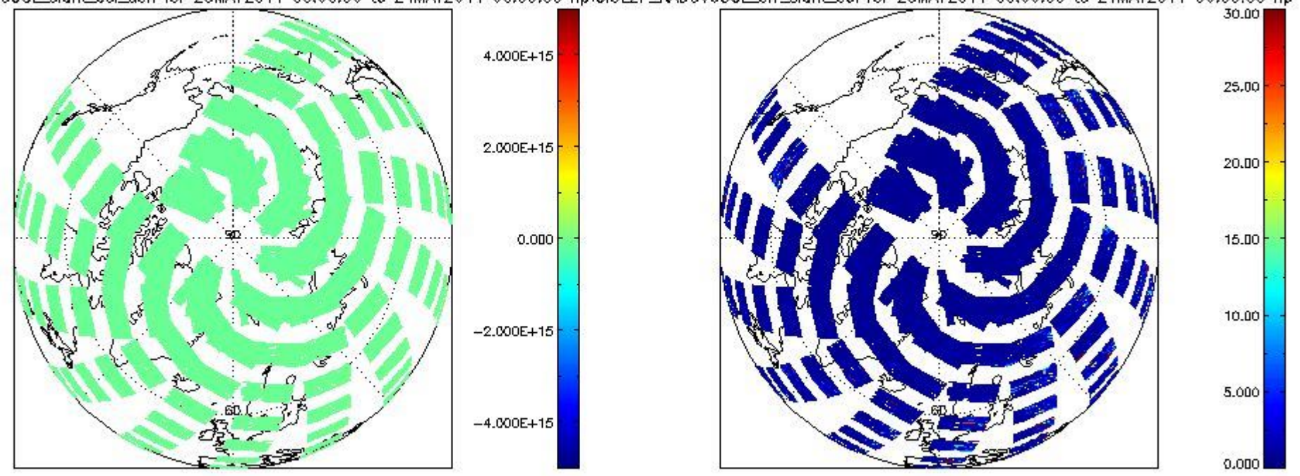
CIOL2P_NADUV60CLslant_col_den for 23MAY2011 00:00:00 to 24MAY2011 00:00:00 np; CIOL2P_NADUV60CLarr_slant_col for 23MAY2011 00:00:00 to 24MAY2011 00:00:00 np
