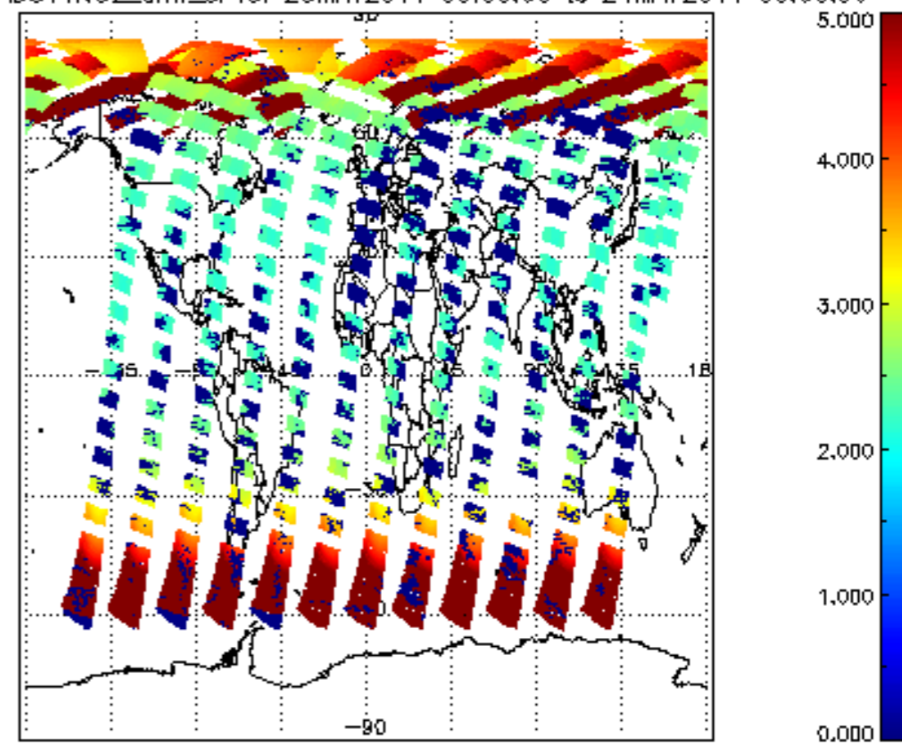
SCIOL2P_NADUV1NO2_amf_sl for 23MAY2011 00:00:00 to 24MAY2011 00:00:00
