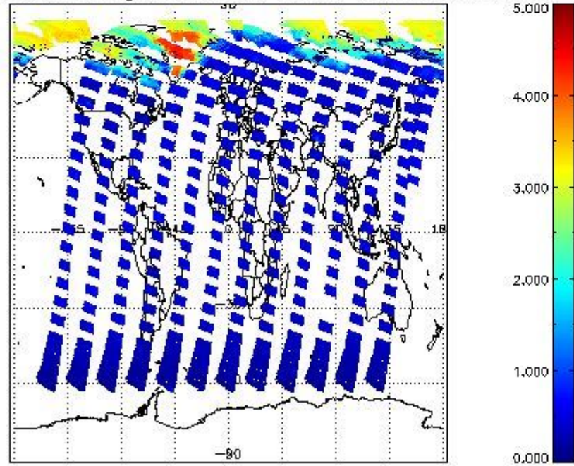
SCIOL2P_NADUV5S02_amf_gr for 23MAY2011 00:00:00 to 24MAY2011 00:00:00
