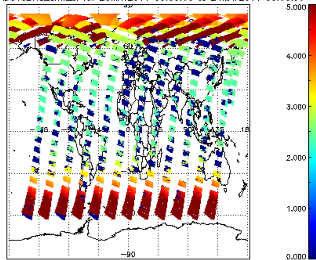
SCIOL2P_NADUV3BRO_amf_sl for 23MAY2011 00:00:00 to 24MAY2011 00:00:00
