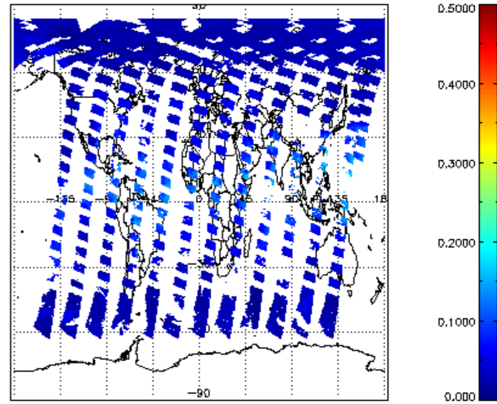
SCIOL2P_NADUV8H2O_vcd_err for 23MAY2011 00:00:00 to 24MAY2011 00:00:00
