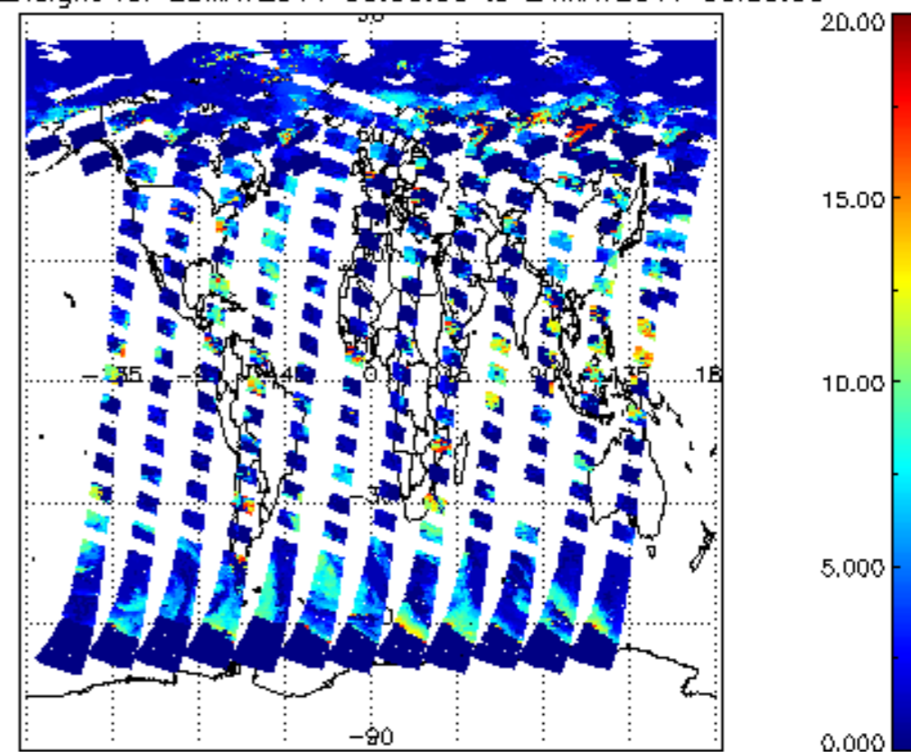
cL_top_height for 23MAY2011 00:00:00 to 24MAY2011 00:00:00
