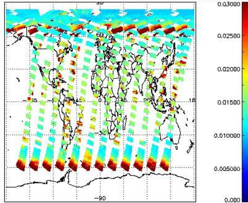
SCIOL2P_NADUV003_vcd_err for 23MAY2011 00:00:00 to 24MAY2011 00:00:00
