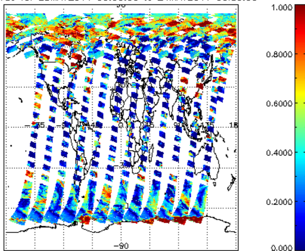
cL_frac for 23MAY2011 00:00:00 to 24MAY2011 00:00:00
