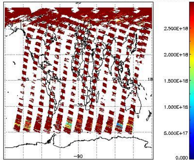
SCIDL2P_NADIR3CO_vcd_err for 23MAY2011 00:00:00 to 24MAY2011 00:00:00
