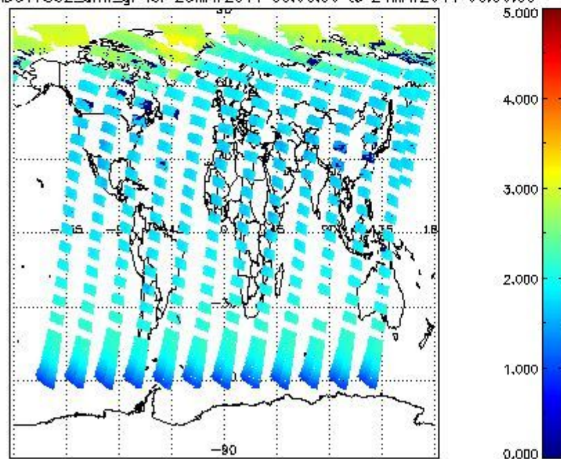
SCIOL2P_NADUV7S02_amf_gr for 23MAY2011 00:00:00 to 24MAY2011 00:00:00
