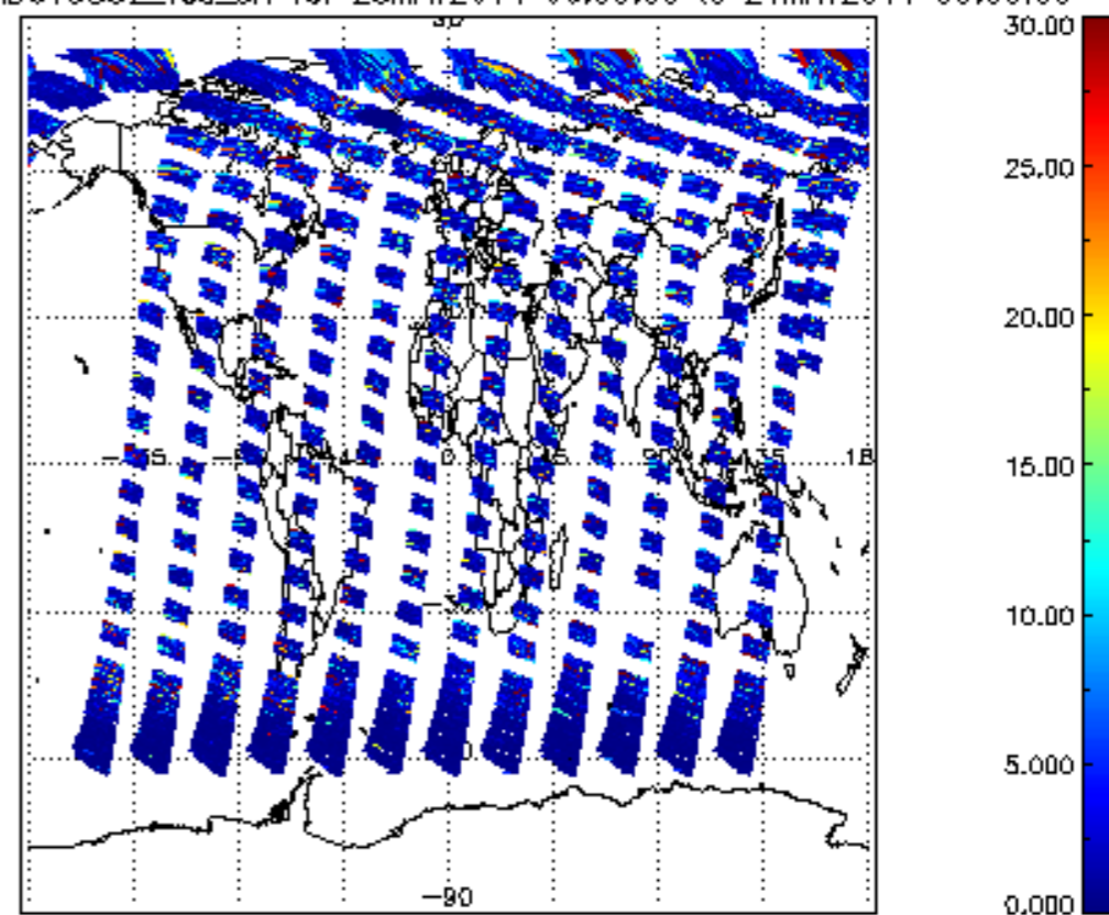
SCIOL2P_NADUV5S02_vcd_err for 23MAY2011 00:00:00 to 24MAY2011 00:00:00
