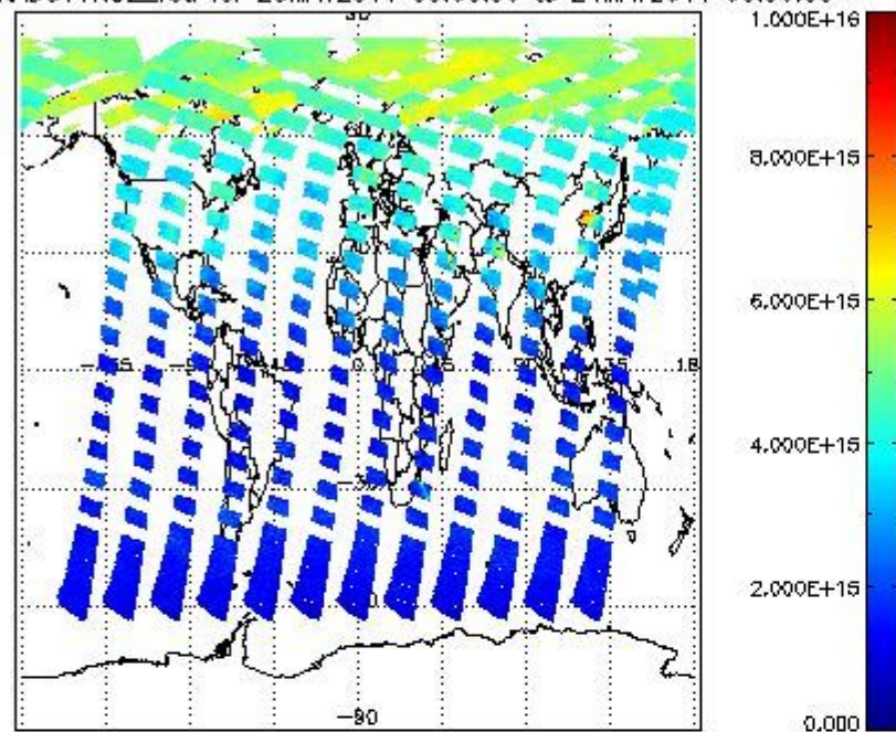
SCIOL2P_NADUV1NO2_vcd for 23MAY2011 00:00:00 to 24MAY2011 00:00:00
