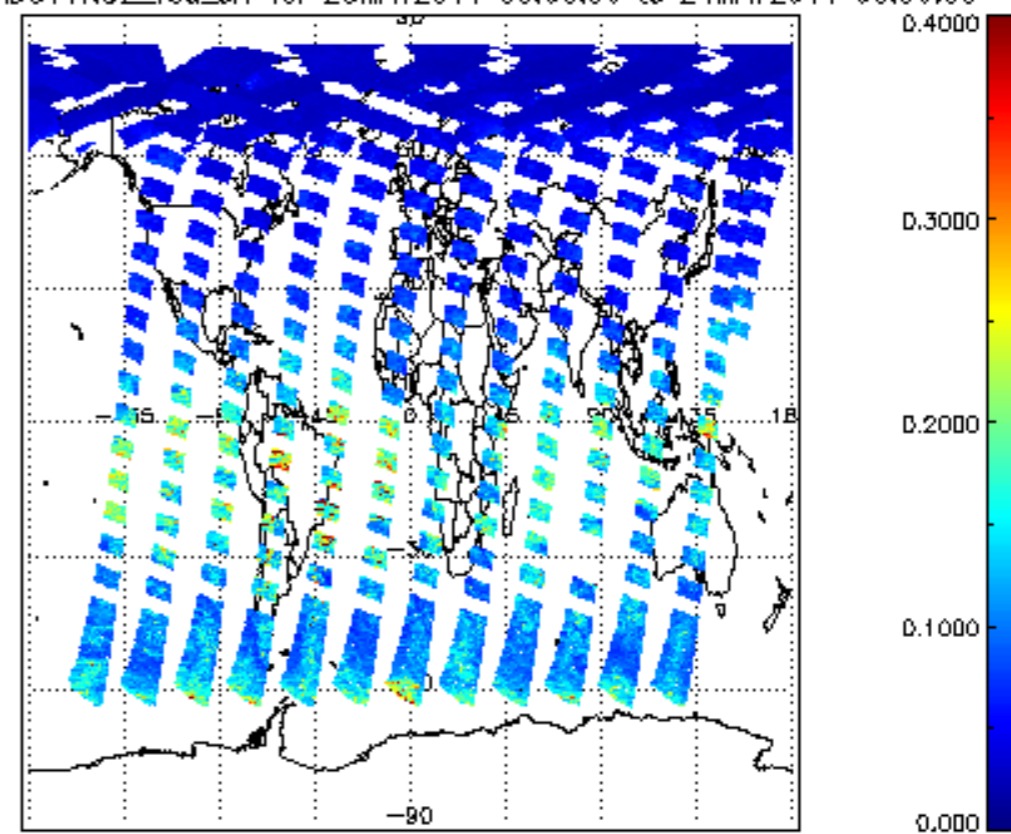
SCIOL2P_NADUV1NO2_vcd_err for 23MAY2011 00:00:00 to 24MAY2011 00:00:00
