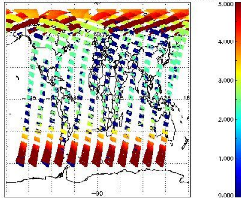
SCIOL2P_NADUV003_amf_cl for 23MAY2011 00:00:00 to 24MAY2011 00:00:00
