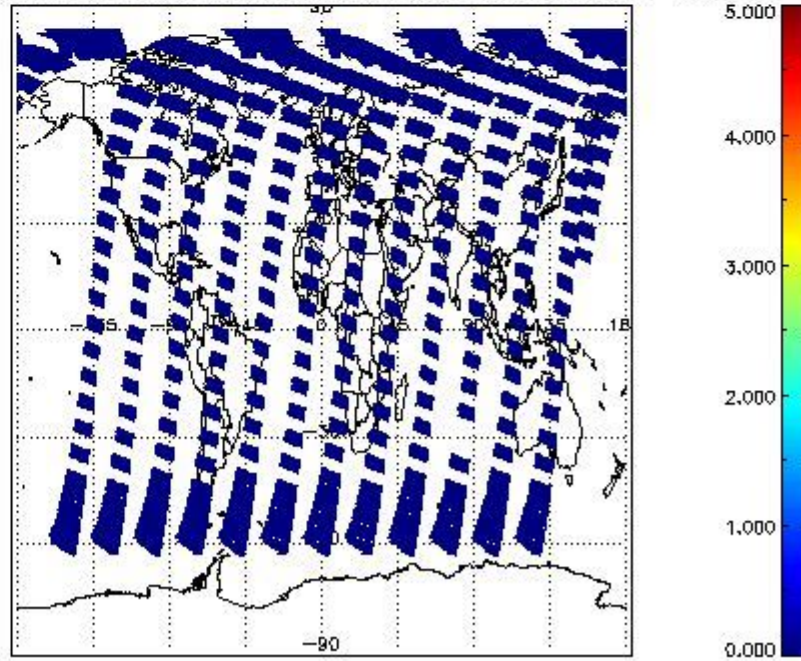
SCIOL2P_NADUV5S02_amf_cl for 23MAY2011 00:00:00 to 24MAY2011 00:00:00
