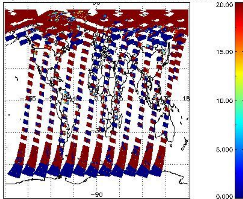
cL_opt_depth for 23MAY2011 00:00:00 to 24MAY2011 00:00:00
