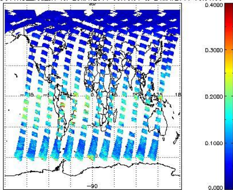
SCIOL2P_NADUV1NO2_vcd_err for 23MAY2011 00:00:00 to 24MAY2011 00:00:00
