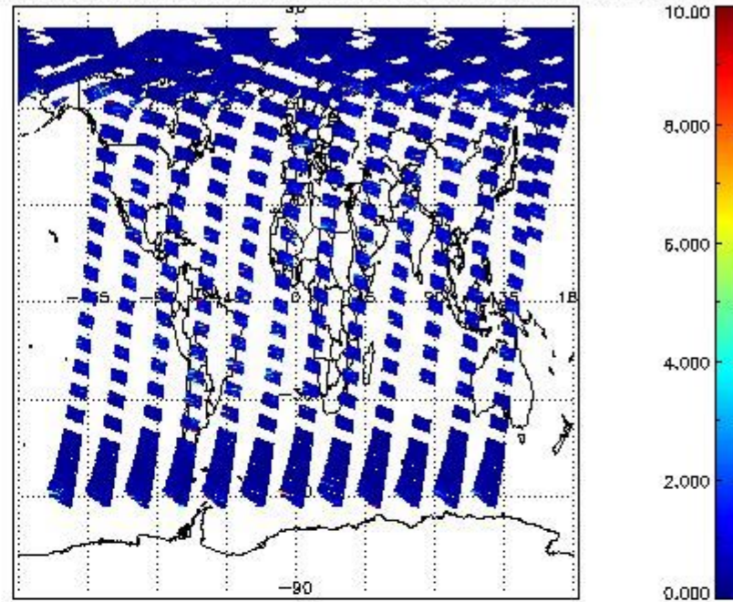
SCIOL2P_NADUV3BRO_vcd_err for 23MAY2011 00:00:00 to 24MAY2011 00:00:00
