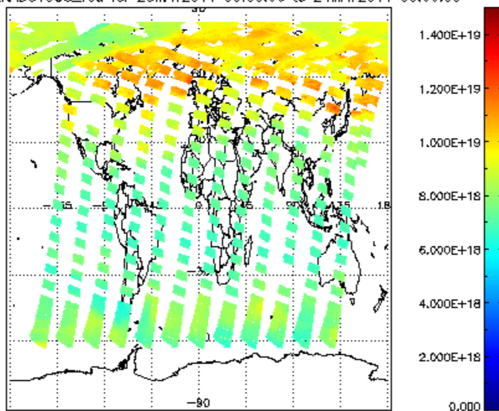
SCIOL2P_NADUV003_vcd for 23MAY2011 00:00:00 to 24MAY2011 00:00:00
