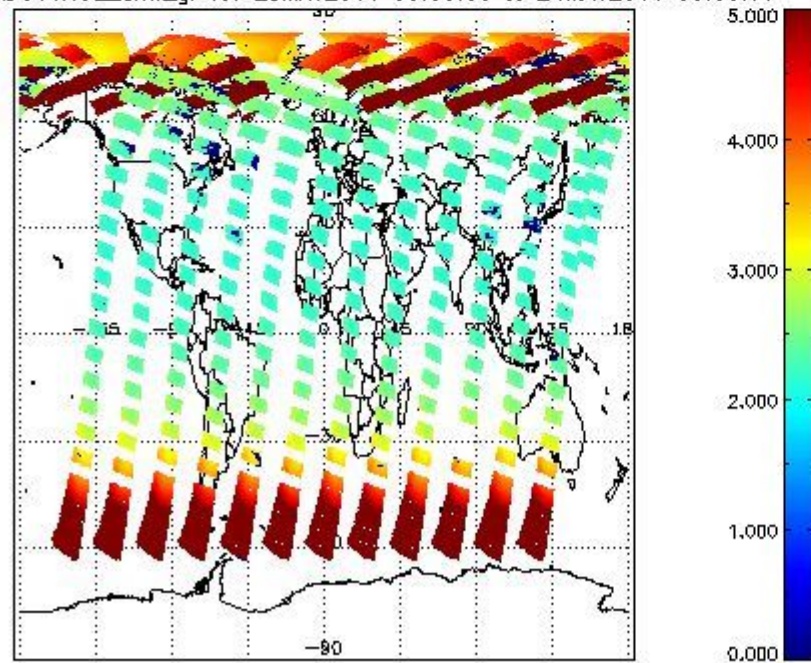
SCIOL2P_NADUV1NO2_amf_gr for 23MAY2011 00:00:00 to 24MAY2011 00:00:00
