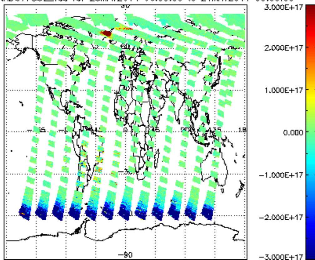
SCIOL2P_NADUV7S02_vcd for 23MAY2011 00:00:00 to 24MAY2011 00:00:00
