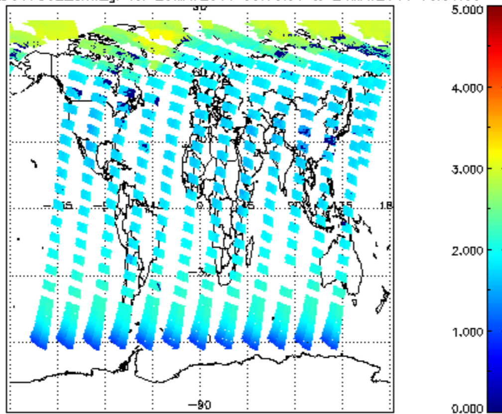
SCIOL2P_NADUV7S02_amf_gr for 23MAY2011 00:00:00 to 24MAY2011 00:00:00
