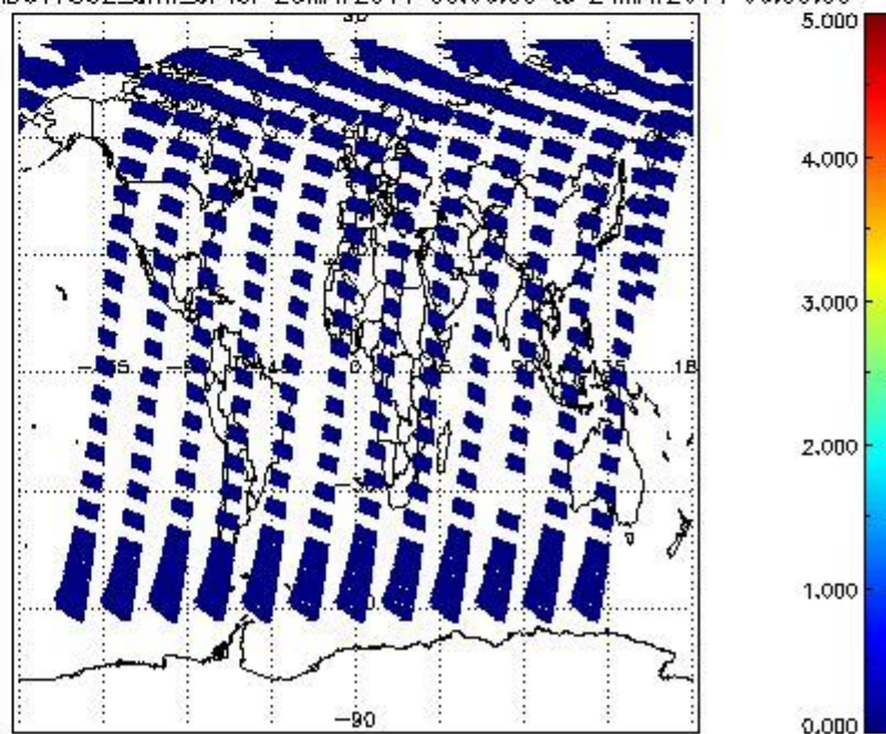
SCIOL2P_NADUV7S02_amf_cl for 23MAY2011 00:00:00 to 24MAY2011 00:00:00
