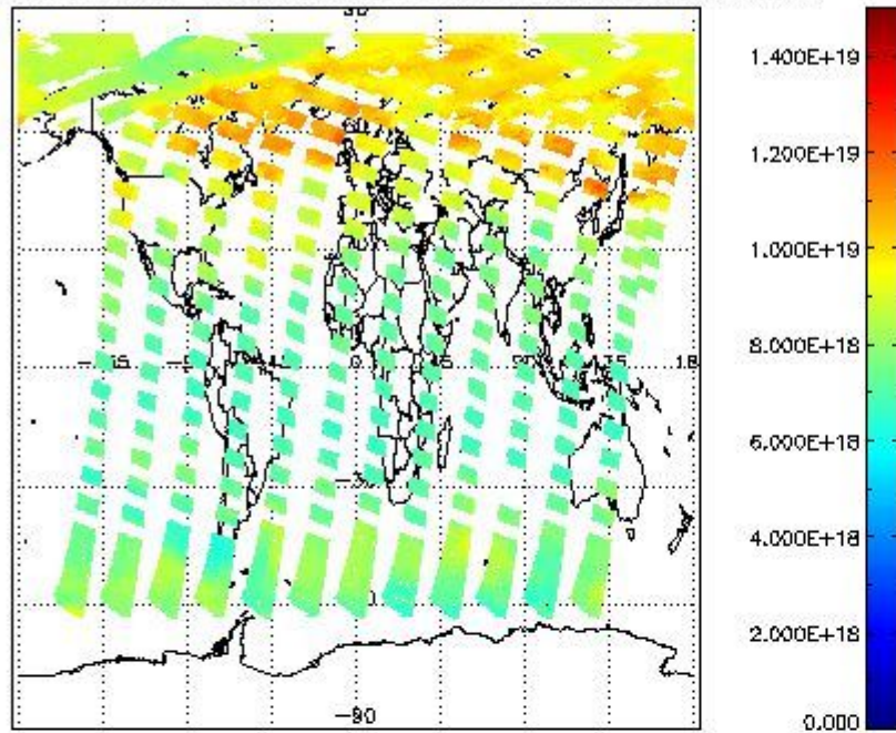
SCIOL2P_NADUV003_vcd for 23MAY2011 00:00:00 to 24MAY2011 00:00:00
