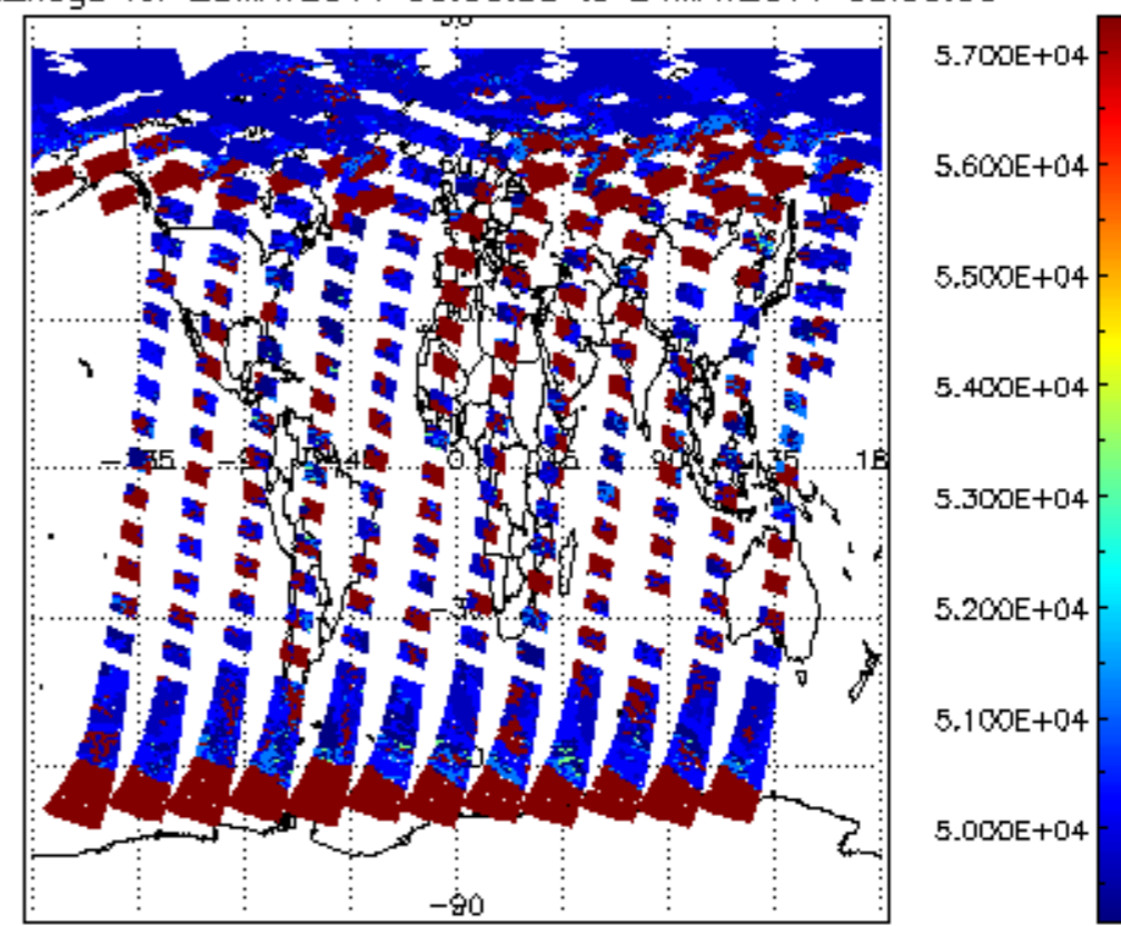
cloud_flags for 23MAY2011 00:00:00 to 24MAY2011 00:00:00
