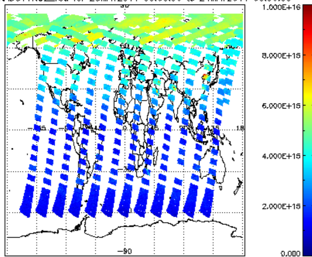
SCIOL2P_NADUV1NO2_vcd for 23MAY2011 00:00:00 to 24MAY2011 00:00:00
