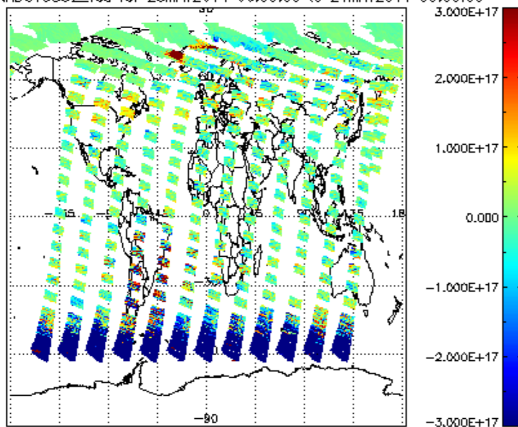
SCIOL2P_NADUV5S02_vcd for 23MAY2011 00:00:00 to 24MAY2011 00:00:00
