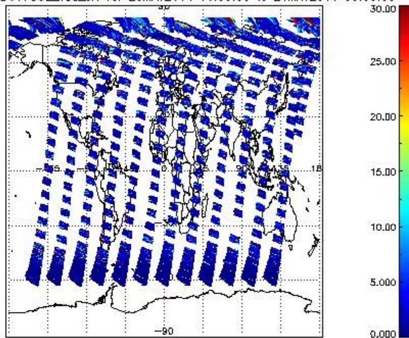
SCIOL2P_NADUV7S02_vcd_err for 23MAY2011 00:00:00 to 24MAY2011 00:00:00
