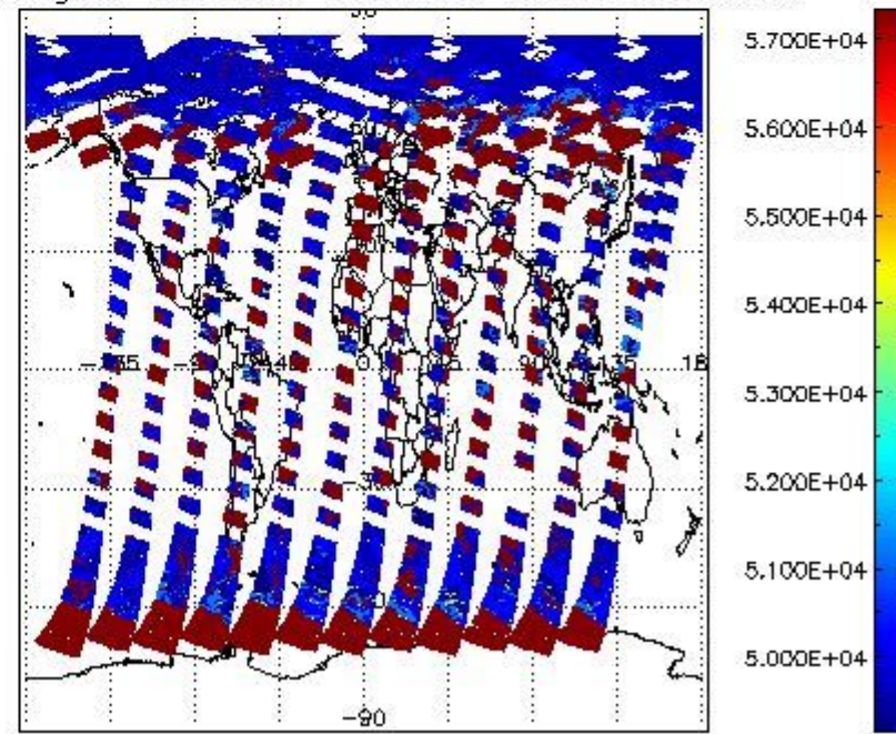
cloud_flags for 23MAY2011 00:00:00 to 24MAY2011 00:00:00
