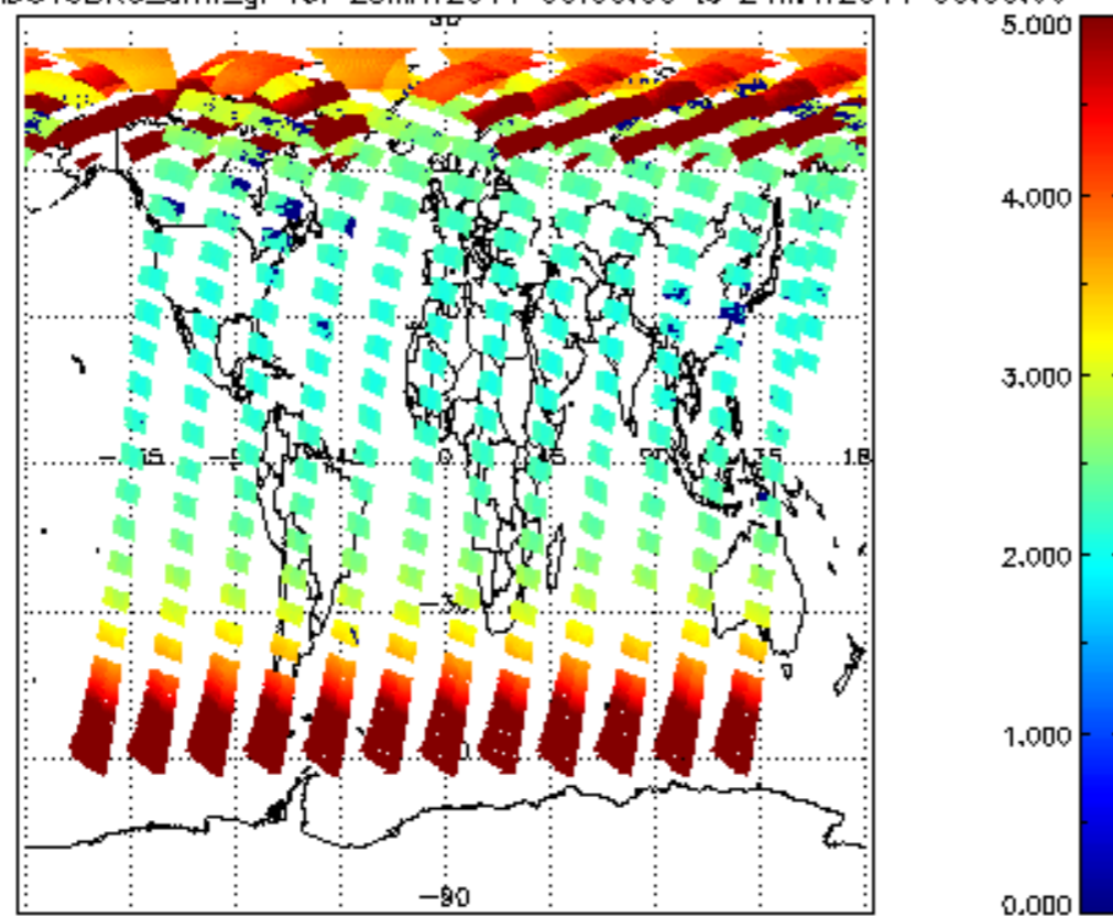
SCIOL2P_NADUV3BRO_amf_gr for 23MAY2011 00:00:00 to 24MAY2011 00:00:00
