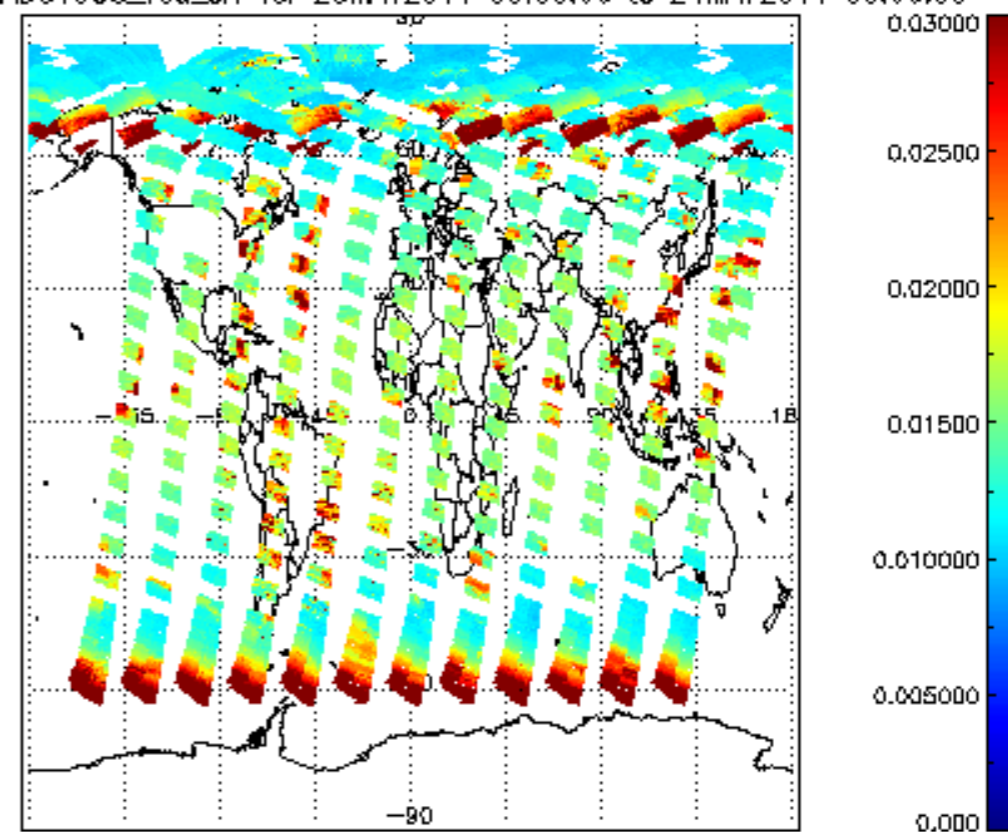
SCIOL2P_NADUV003_vcd_err for 23MAY2011 00:00:00 to 24MAY2011 00:00:00
