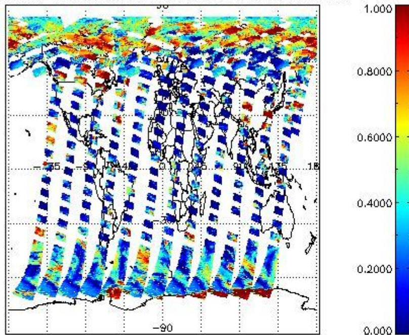
cL_frac for 23MAY2011 00:00:00 to 24MAY2011 00:00:00
