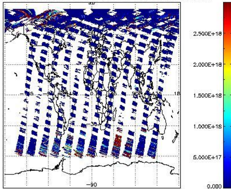
SCIDL2P_NADIR3CO_vcd for 23MAY2011 00:00:00 to 24MAY2011 00:00:00
