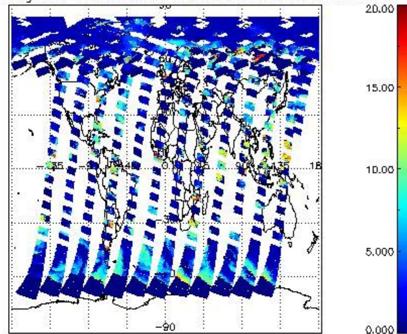
cL_top_height for 23MAY2011 00:00:00 to 24MAY2011 00:00:00
