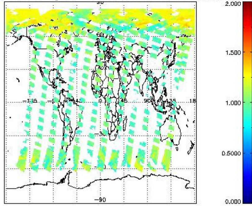
SCIOL2P_NADUV8H2O_arnf_gr for 23MAY2011 00:00:00 to 24MAY2011 00:00:00
