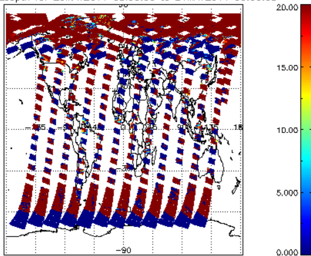
cL_opt_depth for 23MAY2011 00:00:00 to 24MAY2011 00:00:00
