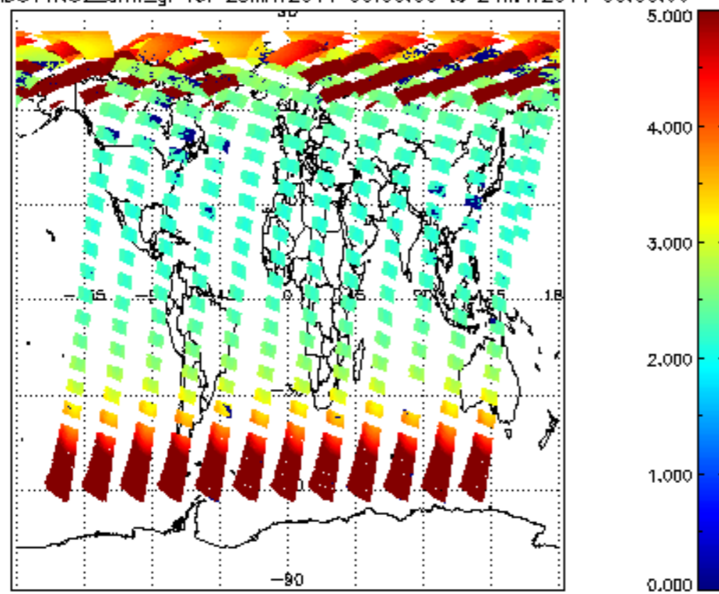
SCIOL2P_NADUV1NO2_amf_gr for 23MAY2011 00:00:00 to 24MAY2011 00:00:00
