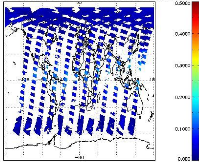
SCIOL2P_NADUV8H2O_vcd_err for 23MAY2011 00:00:00 to 24MAY2011 00:00:00
