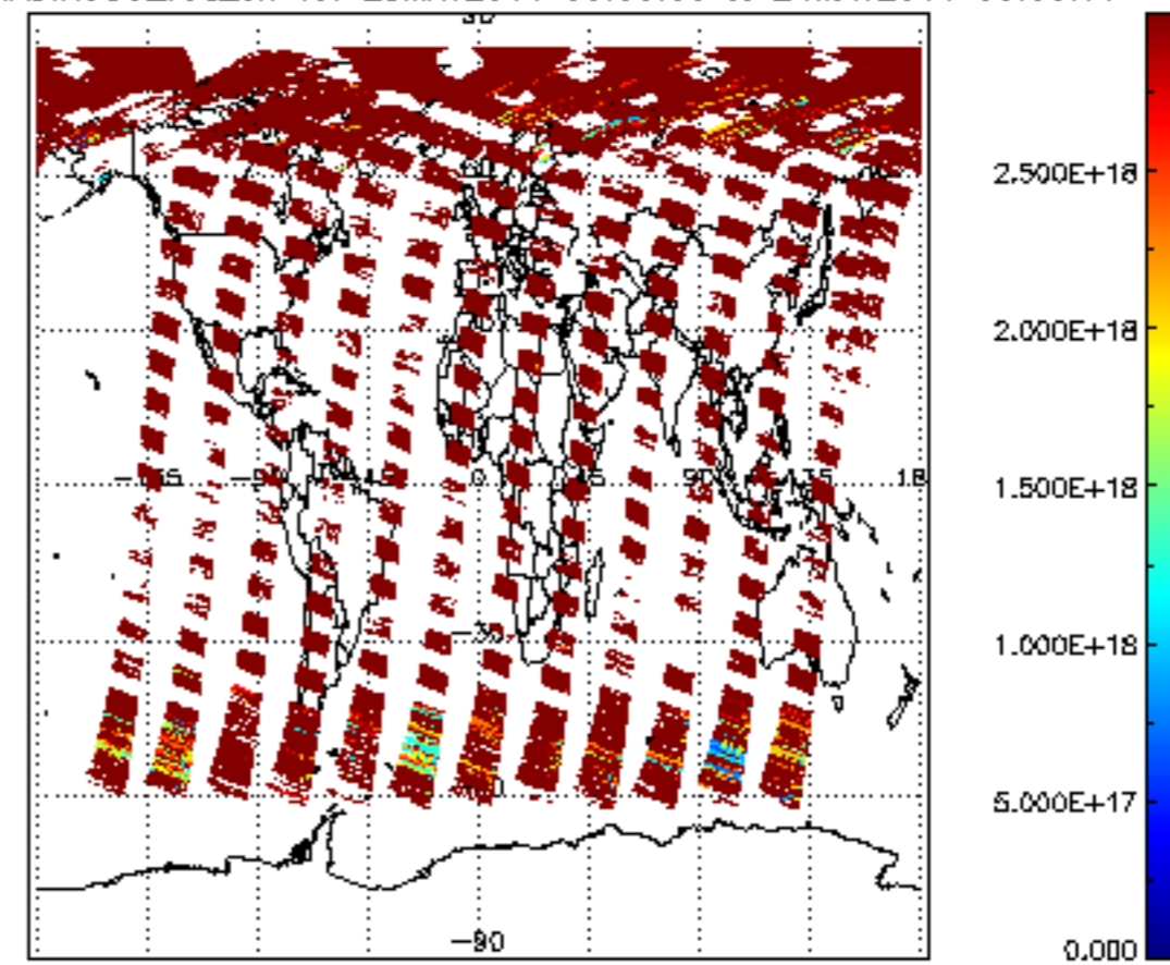
SCIOL2P_NADIR3CO_vcd_err for 23MAY2011 00:00:00 to 24MAY2011 00:00:00
