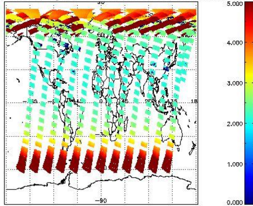
SCIOL2P_NADUV3BRO_amf_gr for 23MAY2011 00:00:00 to 24MAY2011 00:00:00
