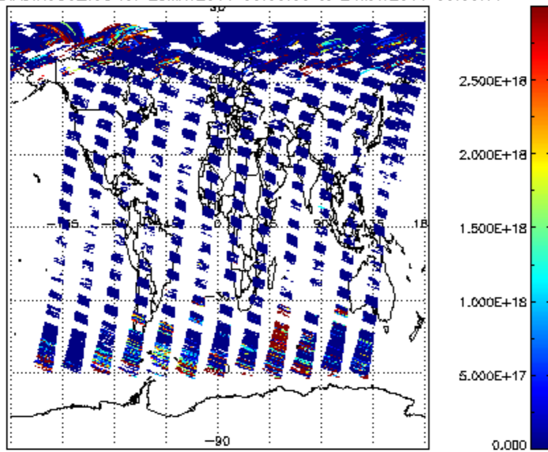
SCIOL2P_NADIR3CO_vcd for 23MAY2011 00:00:00 to 24MAY2011 00:00:00
