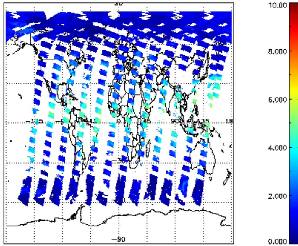
SCIOL2P_NADUV8H2O_vcd for 23MAY2011 00:00:00 to 24MAY2011 00:00:00
