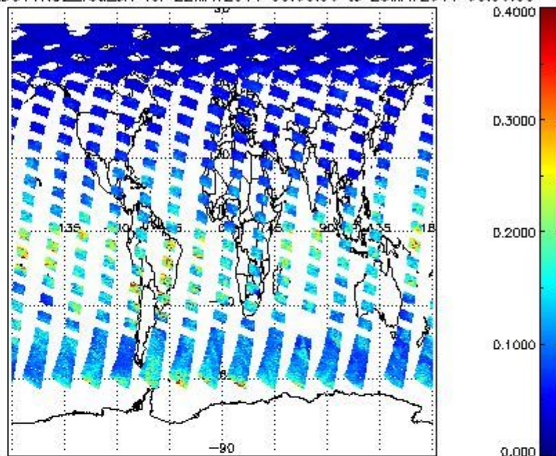
SCIOL2P_NADUV1NO2_vcd_err for 22MAY2011 00:00:00 to 23MAY2011 00:00:00
