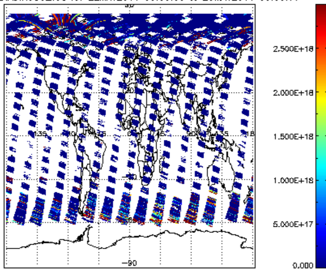
SCIOL2P_NADIR3CO_vcd for 22MAY2011 00:00:00 to 23MAY2011 00:00:00
