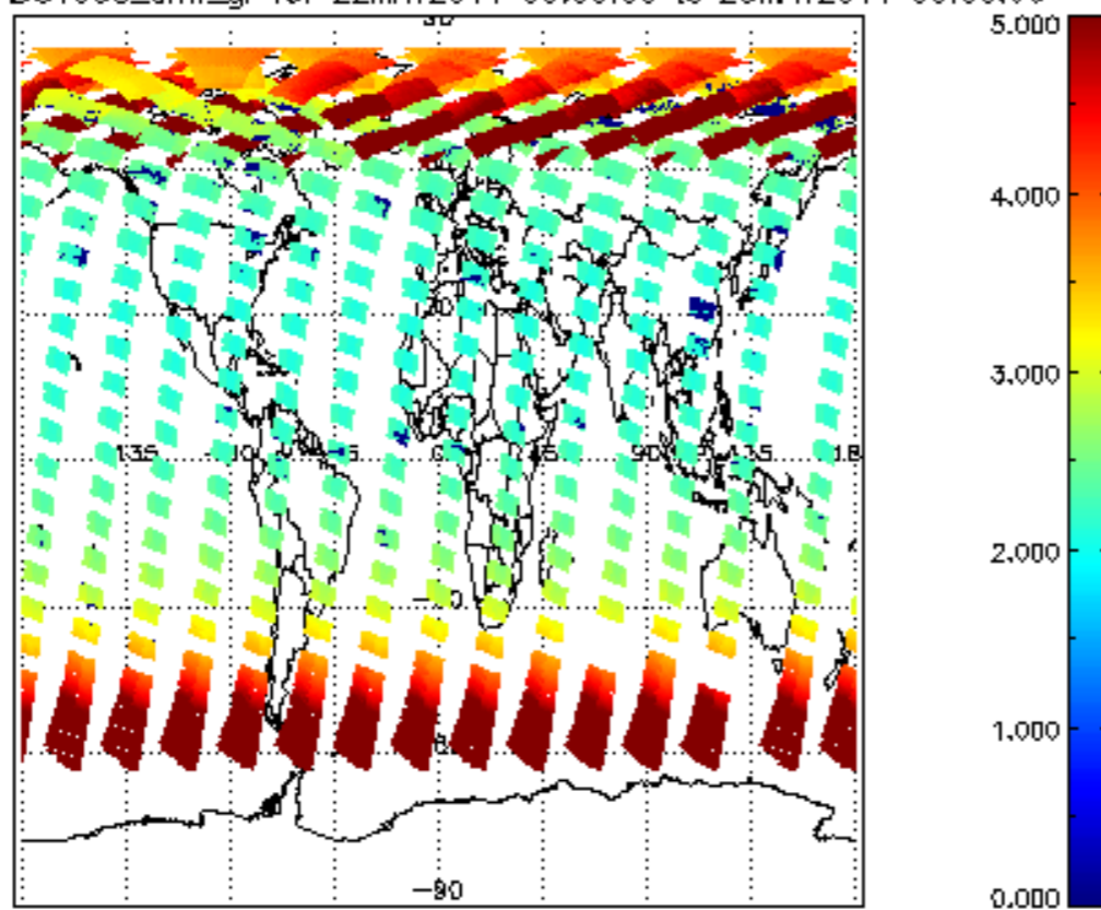
SCIOL2P_NADUV003_amf_gr for 22MAY2011 00:00:00 to 23MAY2011 00:00:00
