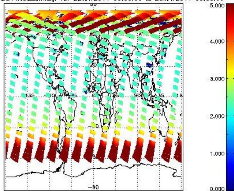
SCIOL2P_NADUV1NO2_amf_gr for 22MAY2011 00:00:00 to 23MAY2011 00:00:00
