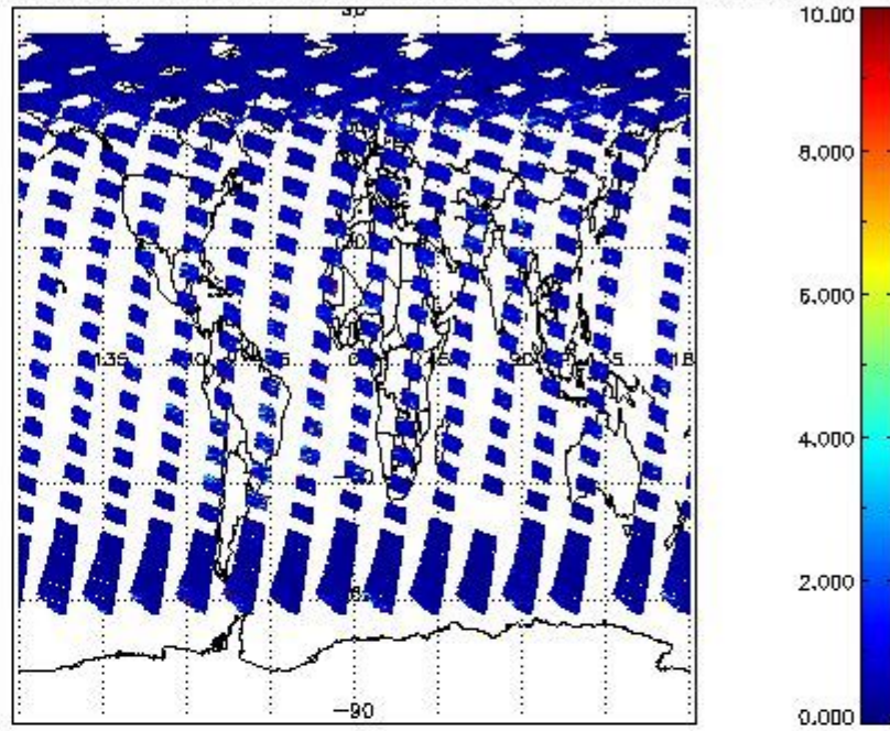
SCIOL2P_NADUV3BRO_vcd_err for 22MAY2011 00:00:00 to 23MAY2011 00:00:00
