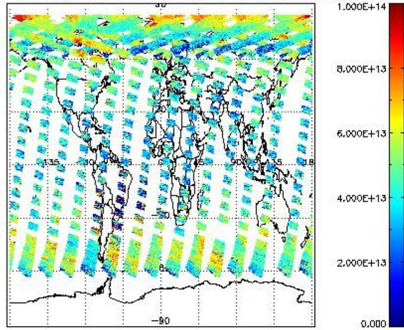
SCIOL2P_NADUV3BRO_vcd for 22MAY2011 00:00:00 to 23MAY2011 00:00:00
