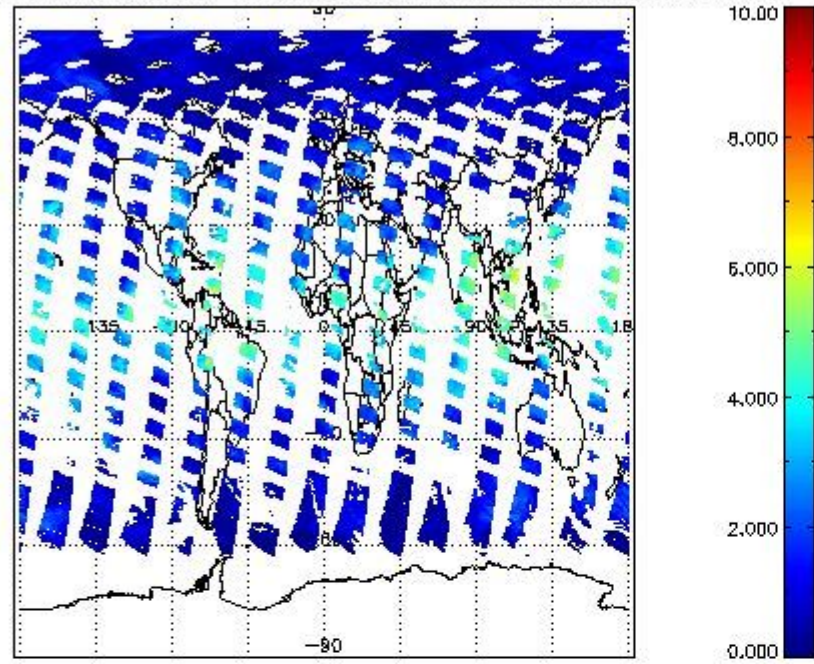
SCIOL2P_NADUV8H2O_vcd for 22MAY2011 00:00:00 to 23MAY2011 00:00:00
