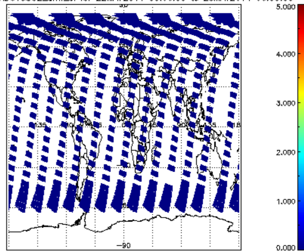
SCIOL2P_NADUV5S02_amf_cl for 22MAY2011 00:00:00 to 23MAY2011 00:00:00
