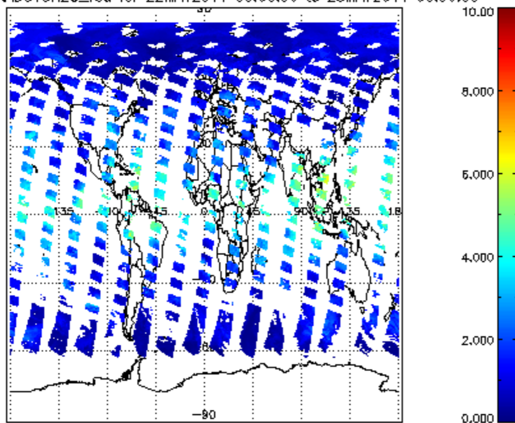
SCIOL2P_NADUV8H2O_vcd for 22MAY2011 00:00:00 to 23MAY2011 00:00:00
