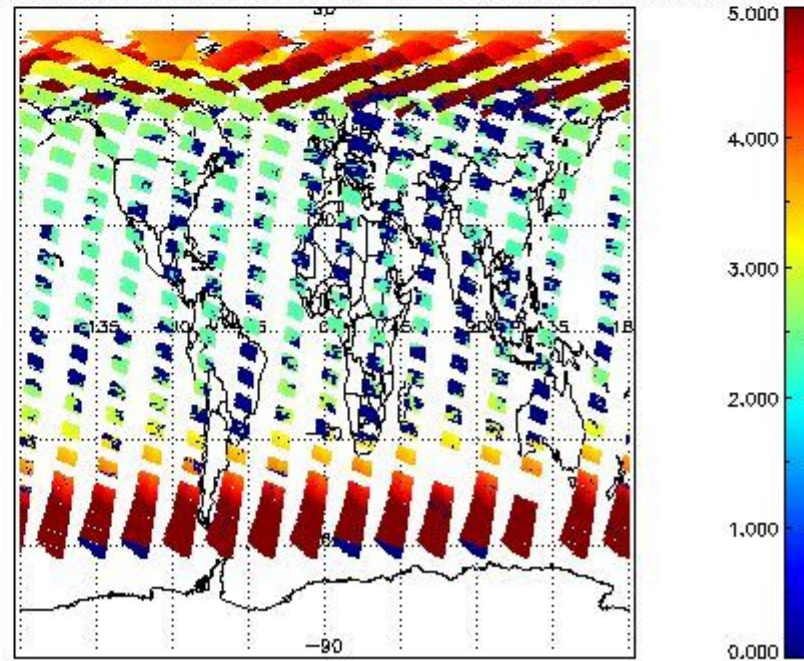
SCIOL2P_NADUV003_amf_cl for 22MAY2011 00:00:00 to 23MAY2011 00:00:00
