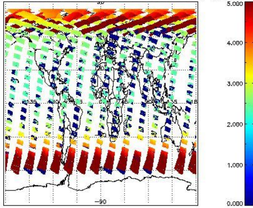
SCIOL2P_NADUV3BRO_amf_cl for 22MAY2011 00:00:00 to 23MAY2011 00:00:00
