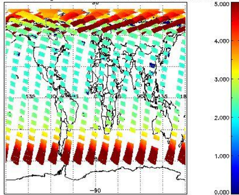
SCIOL2P_NADUV003_amf_gr for 22MAY2011 00:00:00 to 23MAY2011 00:00:00
