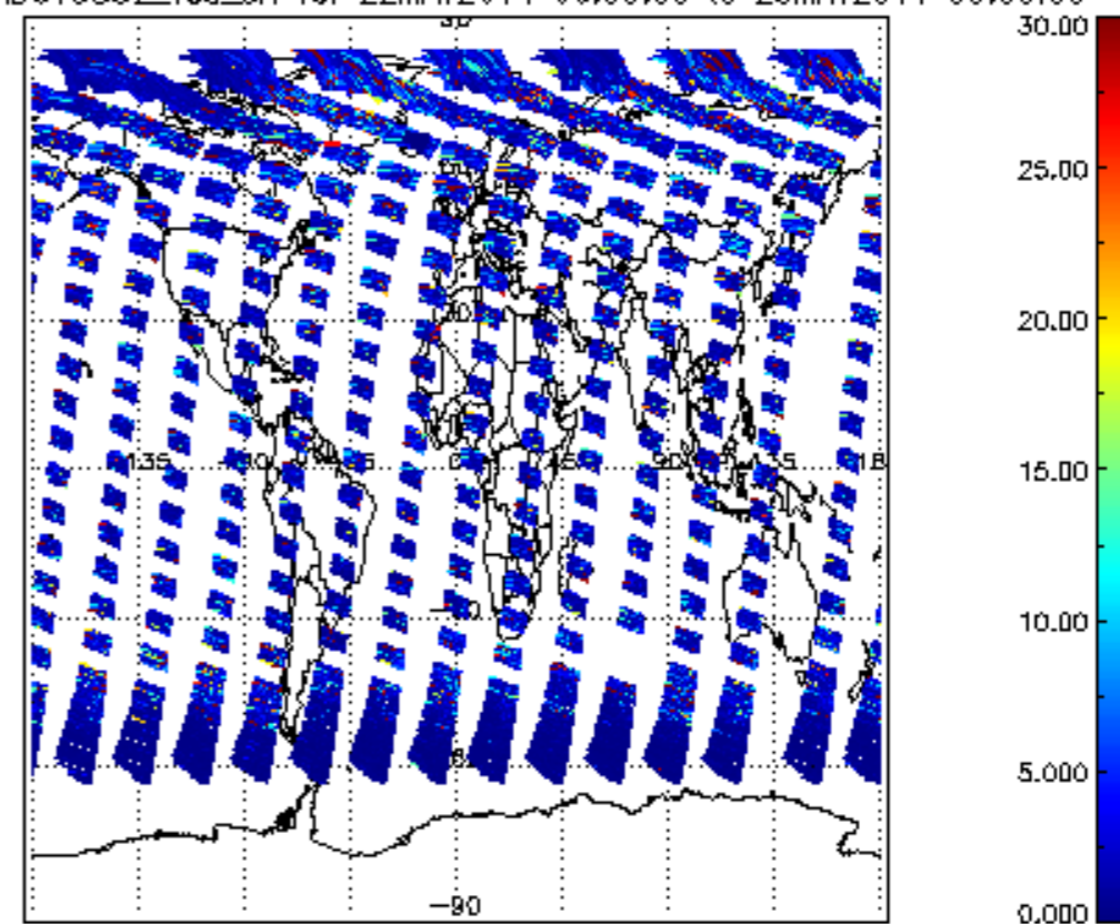
SCIOL2P_NADUV5S02_vcd_err for 22MAY2011 00:00:00 to 23MAY2011 00:00:00
