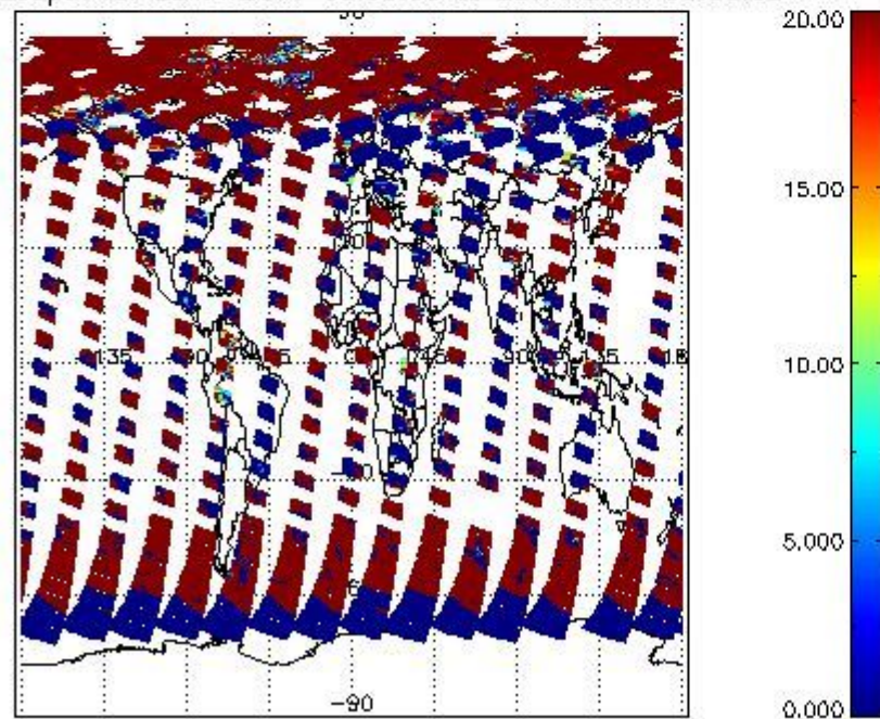
cL_opt_depth for 22MAY2011 00:00:00 to 23MAY2011 00:00:00
