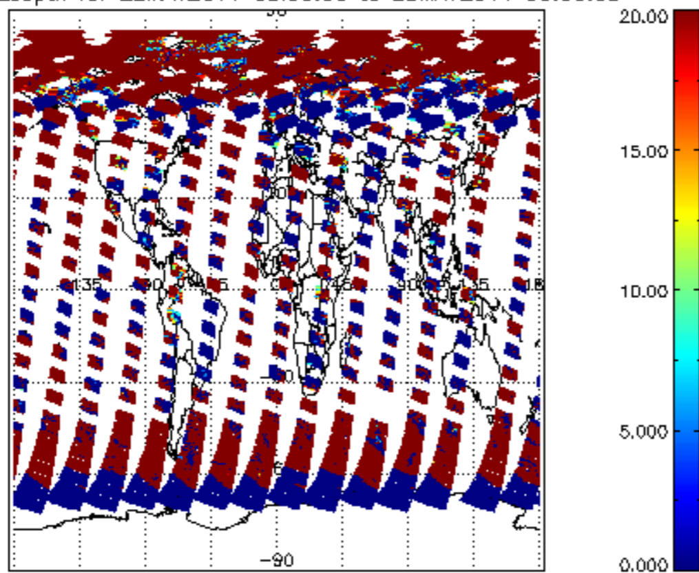
cl_opt_depth for 22MAY2011 00:00:00 to 23MAY2011 00:00:00
