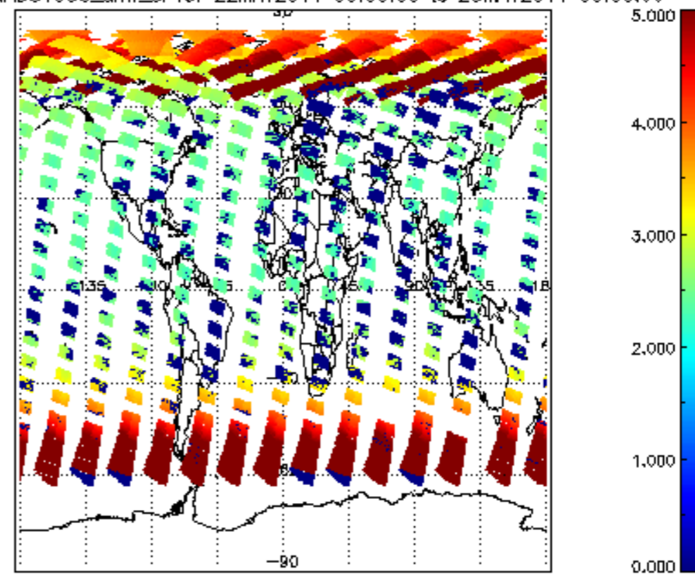
SCIOL2P_NADUV003_amf_cl for 22MAY2011 00:00:00 to 23MAY2011 00:00:00
