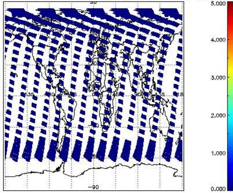
SCIOL2P_NADUV5S02_amf_cl for 22MAY2011 00:00:00 to 23MAY2011 00:00:00
