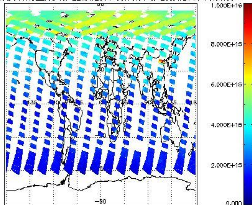
SCIOL2P_NADUV1NO2_vcd for 22MAY2011 00:00:00 to 23MAY2011 00:00:00
