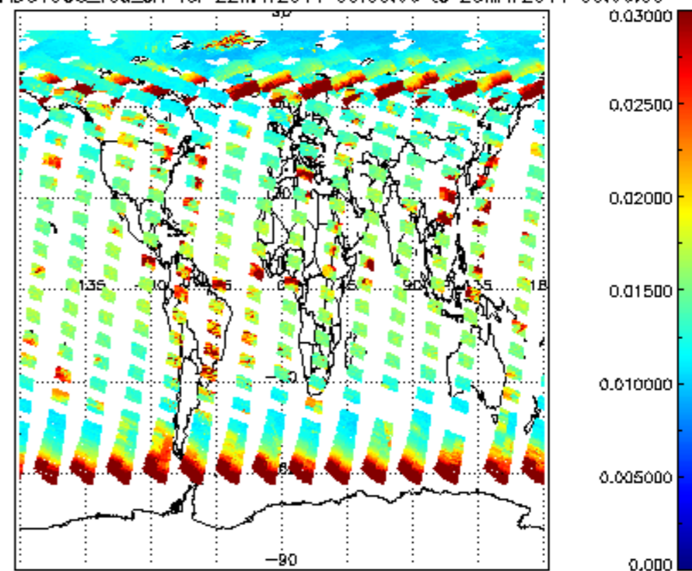
SCIOL2P_NADUV003_vcd_err for 22MAY2011 00:00:00 to 23MAY2011 00:00:00
