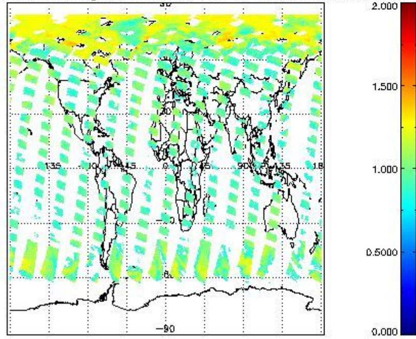
SCIOL2P_NADUV8H2O_arnf_gr for 22MAY2011 00:00:00 to 23MAY2011 00:00:00
