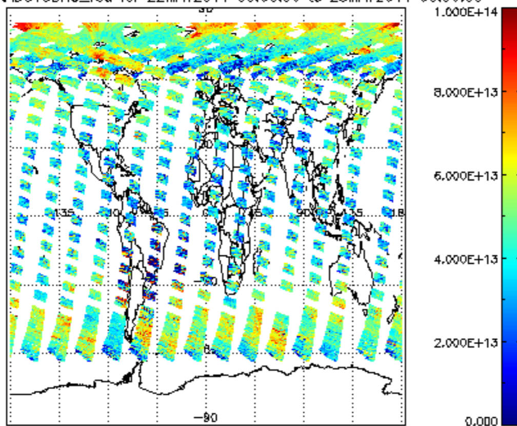
SCIOL2P_NADUV3BRO_vcd for 22MAY2011 00:00:00 to 23MAY2011 00:00:00
