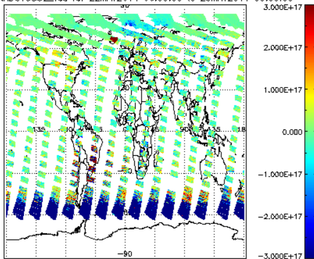
SCIOL2P_NADUV5S02_vcd for 22MAY2011 00:00:00 to 23MAY2011 00:00:00
