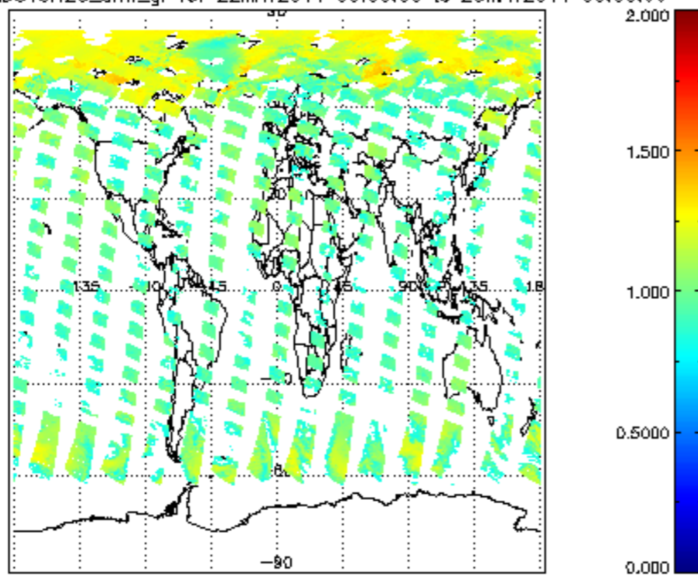
SCIOL2P_NADUV8H2O_amf_gr for 22MAY2011 00:00:00 to 23MAY2011 00:00:00
