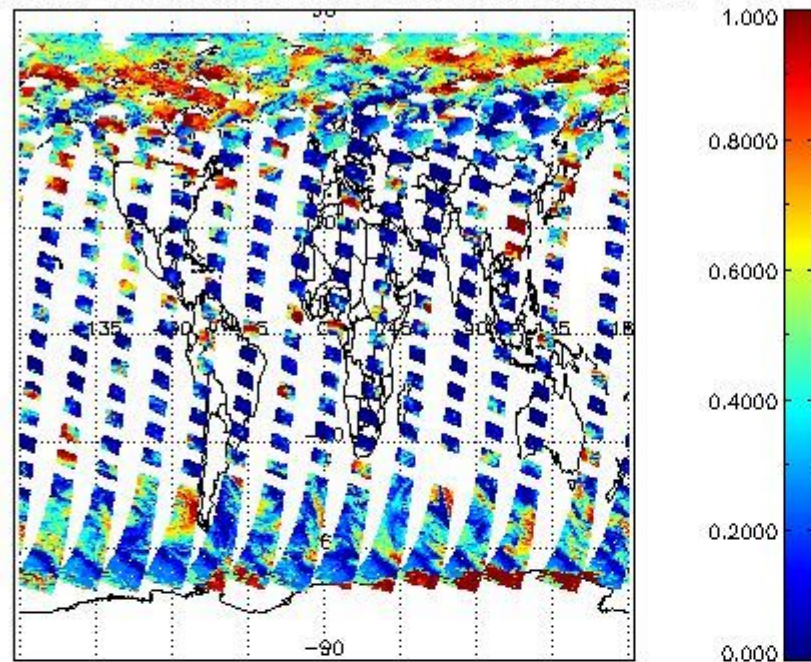
cL_frac for 22MAY2011 00:00:00 to 23MAY2011 00:00:00
