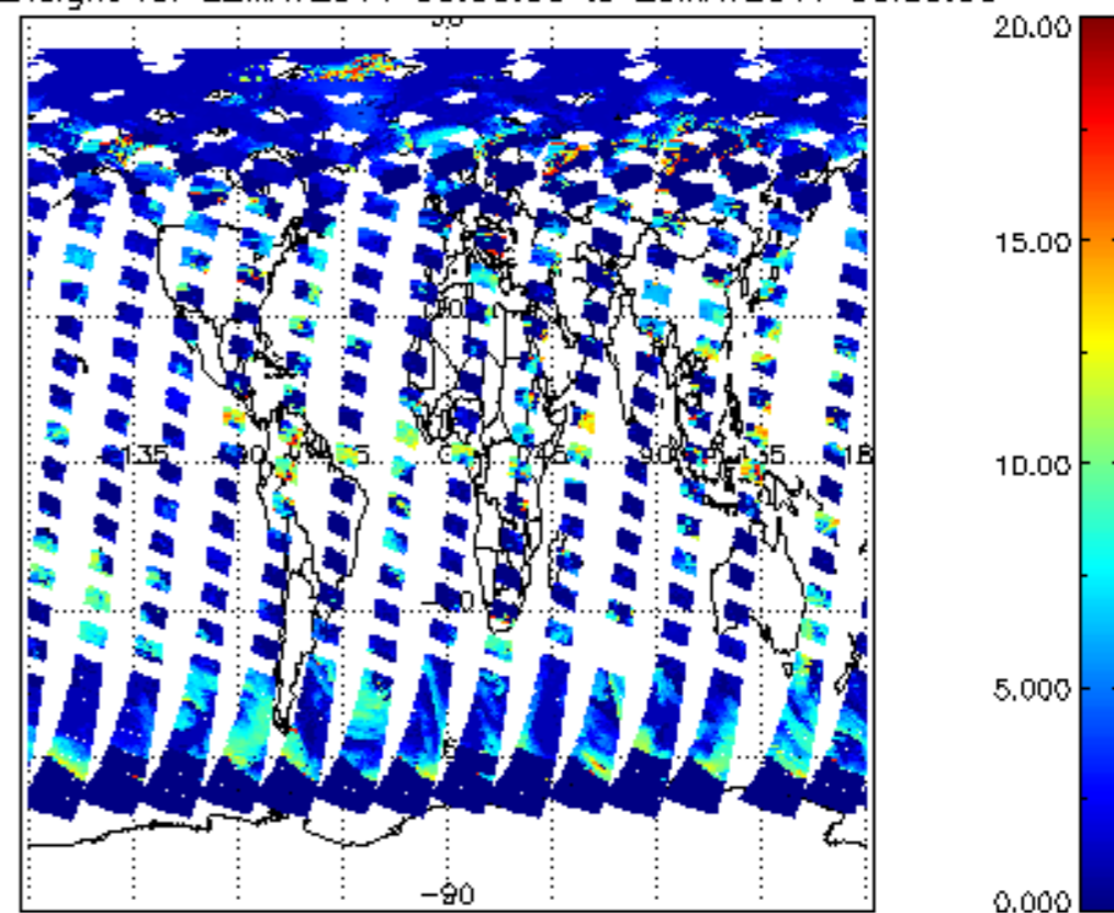
cl_top_height for 22MAY2011 00:00:00 to 23MAY2011 00:00:00
