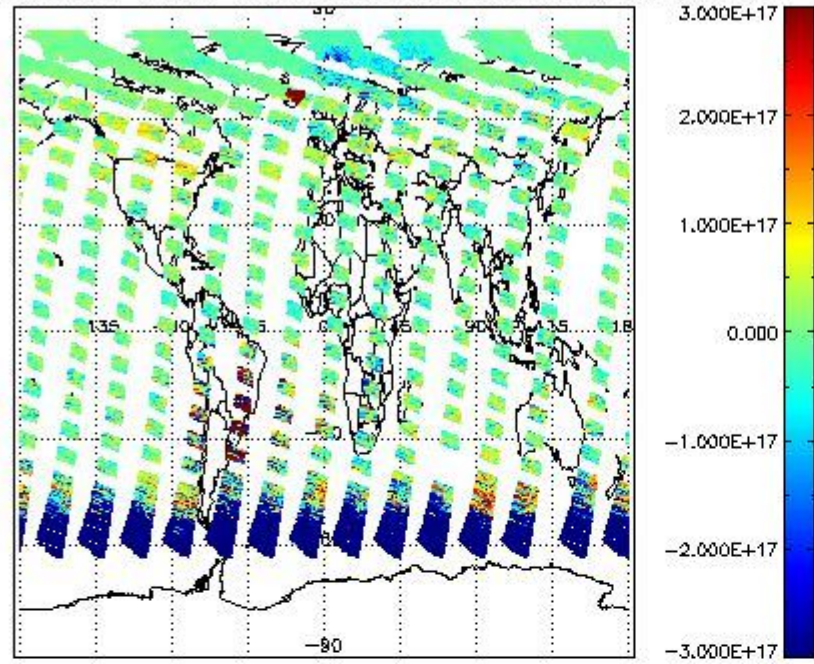
SCIOL2P_NADUV5S02_vcd for 22MAY2011 00:00:00 to 23MAY2011 00:00:00
