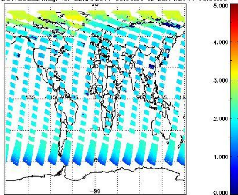
SCIOL2P_NADUV7S02_amf_gr for 22MAY2011 00:00:00 to 23MAY2011 00:00:00
