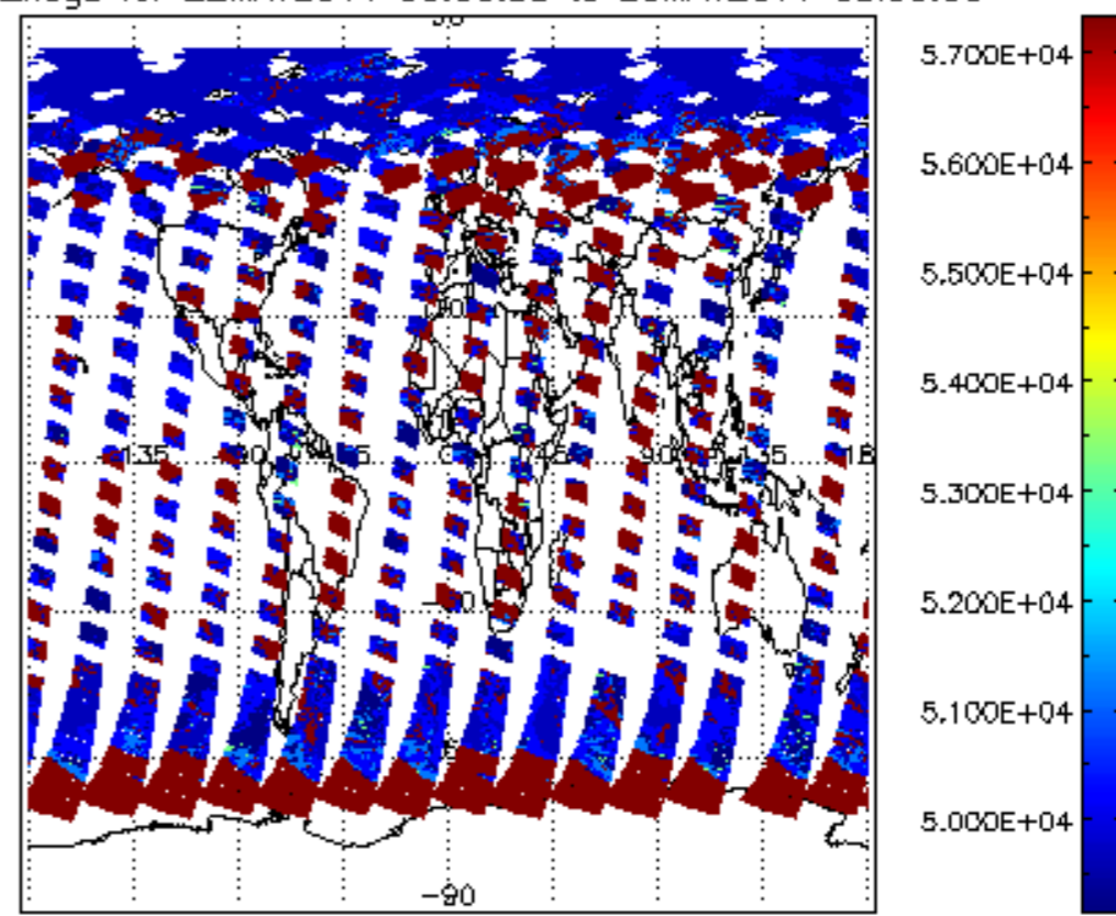
cloud_flags for 22MAY2011 00:00:00 to 23MAY2011 00:00:00
