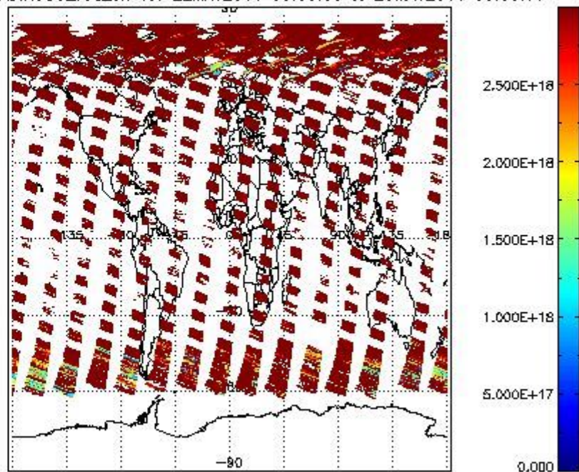
SCIDL2P_NADIR3CO_vcd_err for 22MAY2011 00:00:00 to 23MAY2011 00:00:00
