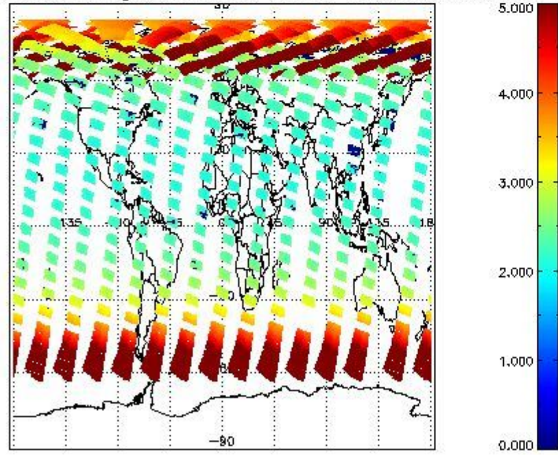
SCIOL2P_NADUV3BRO_amf_gr for 22MAY2011 00:00:00 to 23MAY2011 00:00:00
