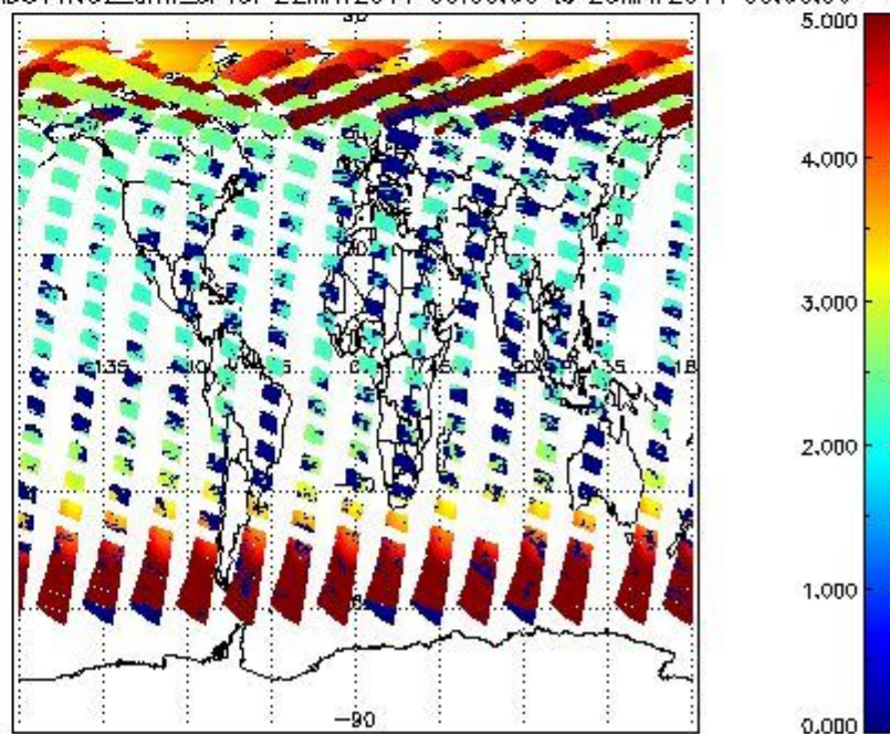
SCIOL2P_NADUV1NO2_amf_cl for 22MAY2011 00:00:00 to 23MAY2011 00:00:00
