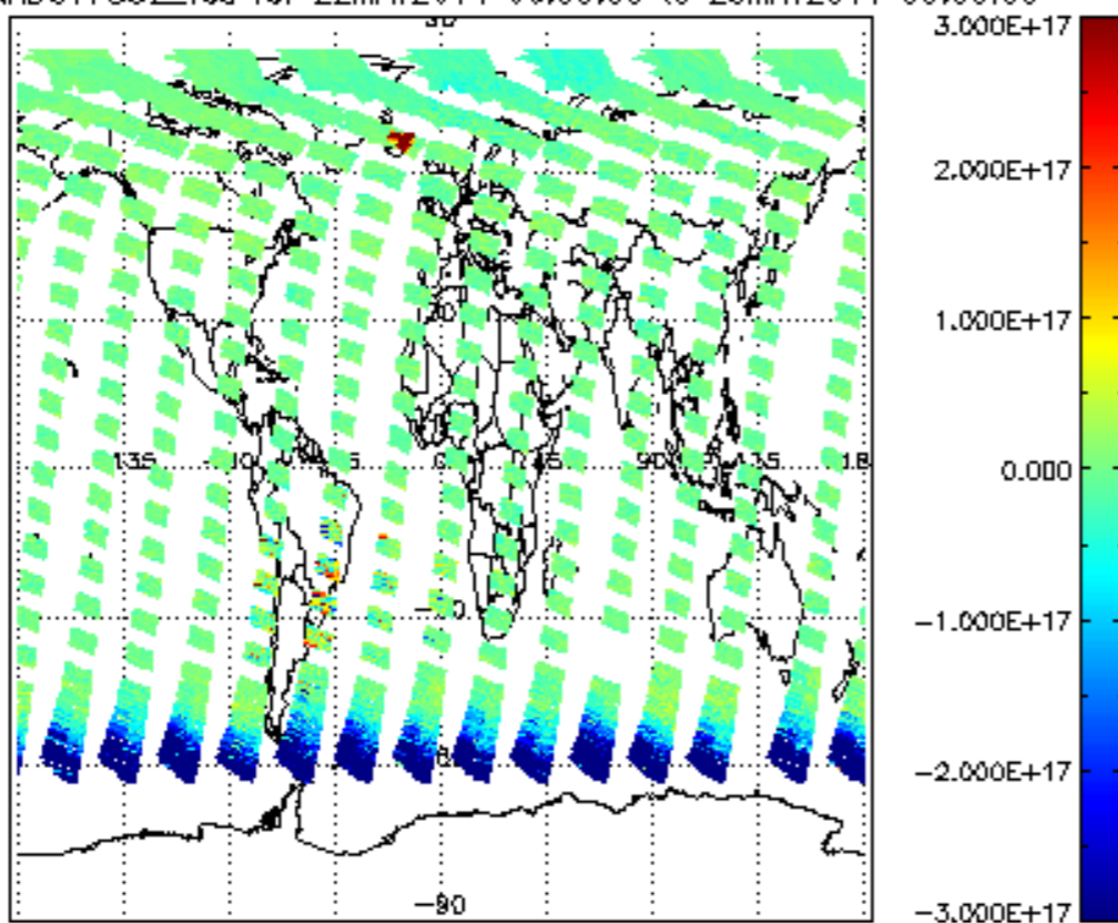
SCIOL2P_NADUV7S02_vcd for 22MAY2011 00:00:00 to 23MAY2011 00:00:00
