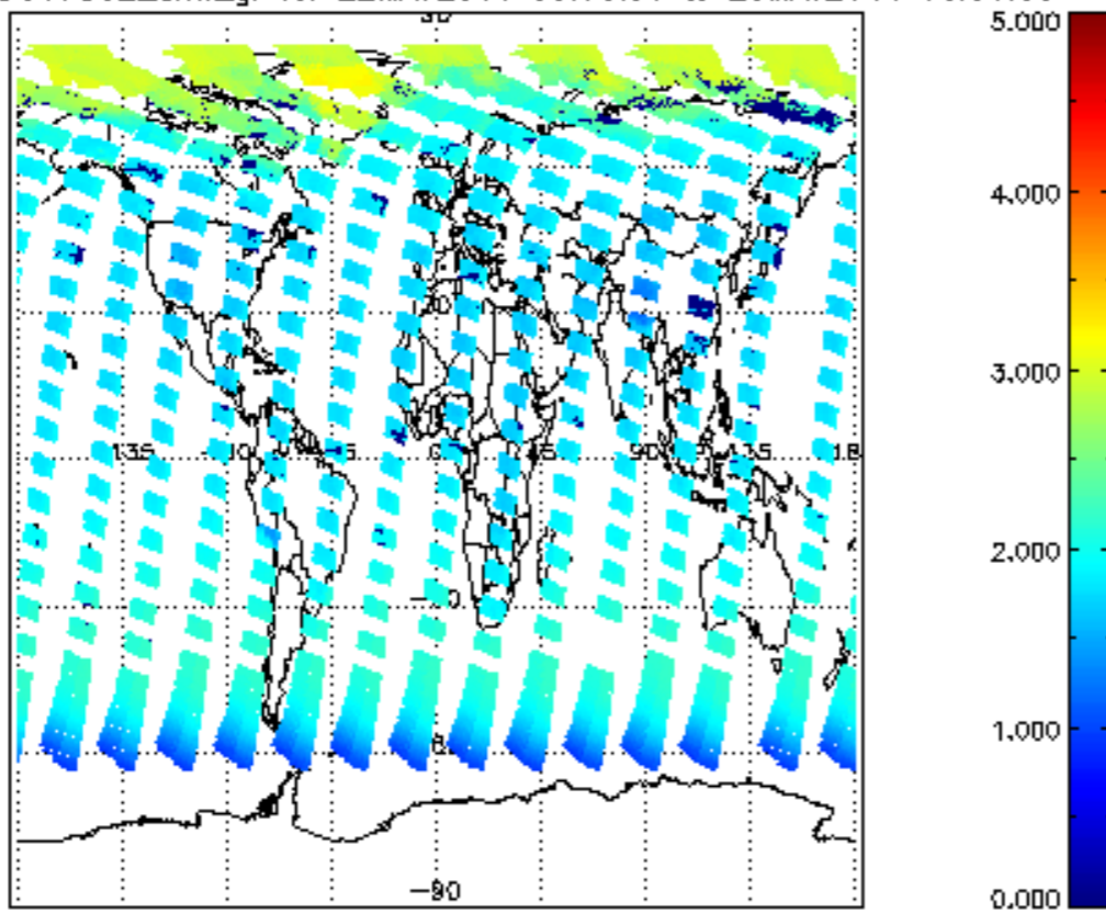
SCIOL2P_NADUV7S02_amf_gr for 22MAY2011 00:00:00 to 23MAY2011 00:00:00
