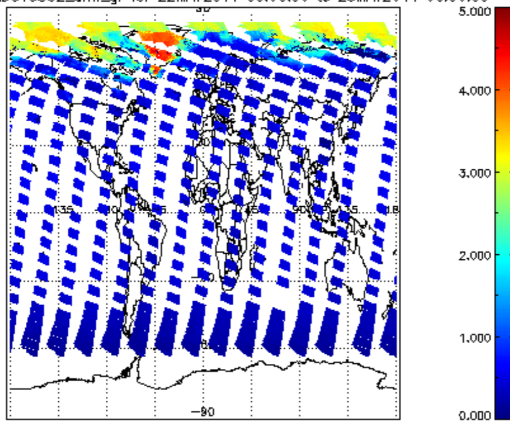
SCIOL2P_NADUV5S02_amf_gr for 22MAY2011 00:00:00 to 23MAY2011 00:00:00
