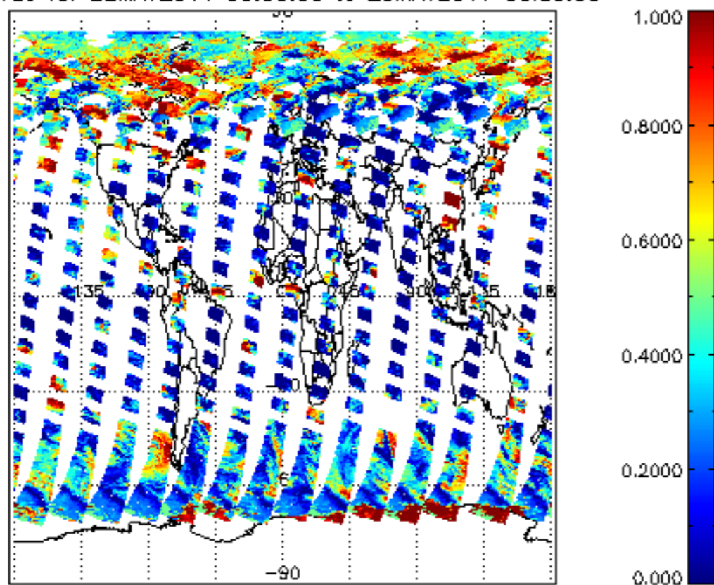
cl_frac for 22MAY2011 00:00:00 to 23MAY2011 00:00:00
