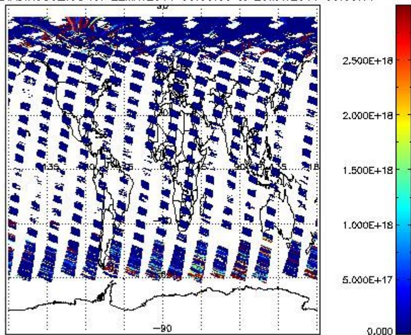
SCIDL2P_NADIR3CO_vcd for 22MAY2011 00:00:00 to 23MAY2011 00:00:00
