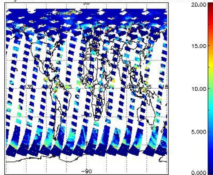
cL_top_height for 22MAY2011 00:00:00 to 23MAY2011 00:00:00
