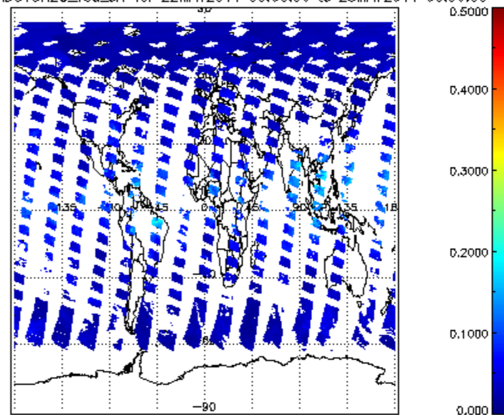
SCIOL2P_NADUV8H2O_vcd_err for 22MAY2011 00:00:00 to 23MAY2011 00:00:00
