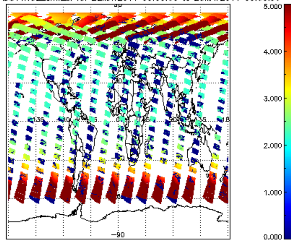
SCIOL2P_NADUV1NO2_amf_cl for 22MAY2011 00:00:00 to 23MAY2011 00:00:00
