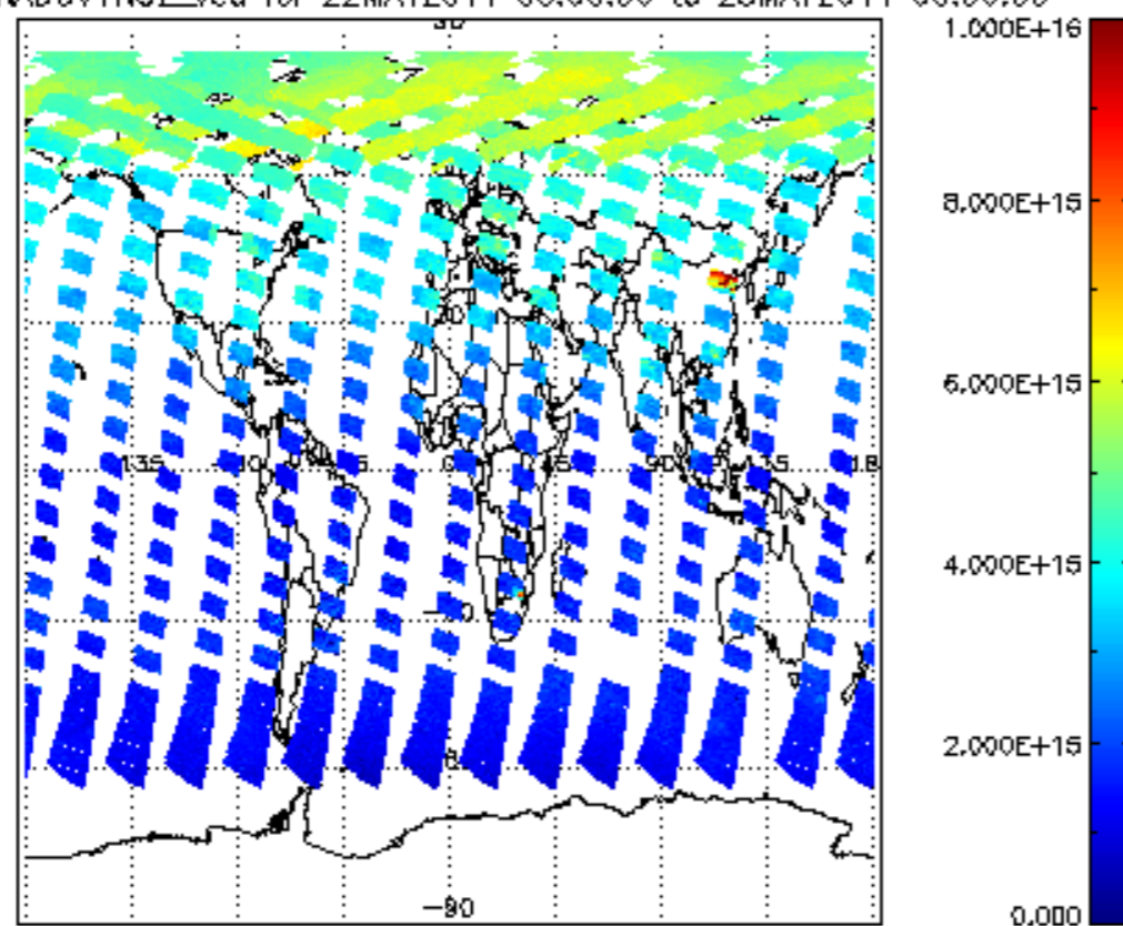
SCIOL2P_NADUV1NO2_vcd for 22MAY2011 00:00:00 to 23MAY2011 00:00:00
