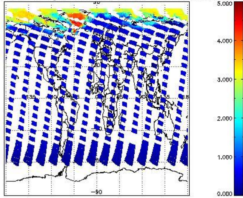
SCIOL2P_NADUV5S02_amf_gr for 22MAY2011 00:00:00 to 23MAY2011 00:00:00
