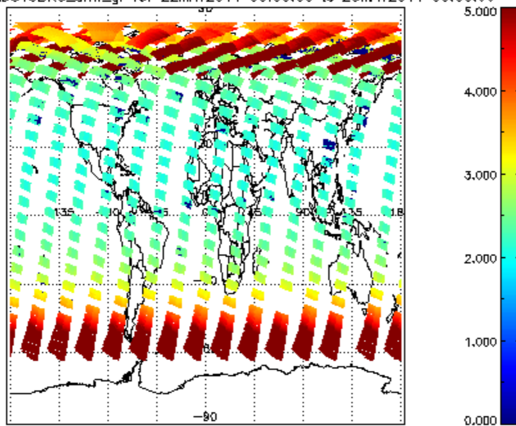
SCIOL2P_NADUV3BRO_amf_gr for 22MAY2011 00:00:00 to 23MAY2011 00:00:00
