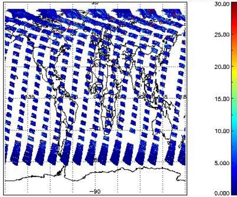
SCIOL2P_NADUV5S02_vcd_err for 22MAY2011 00:00:00 to 23MAY2011 00:00:00
