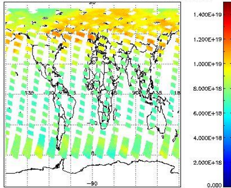
SCIOL2P_NADUV003_vcd for 22MAY2011 00:00:00 to 23MAY2011 00:00:00
