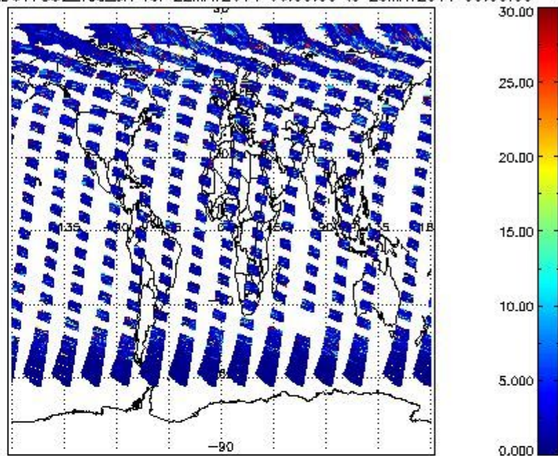
SCIOL2P_NADUV7S02_vcd_err for 22MAY2011 00:00:00 to 23MAY2011 00:00:00
