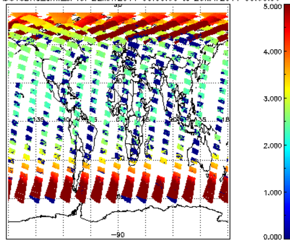
SCIOL2P_NADUV3BRO_amf_sl for 22MAY2011 00:00:00 to 23MAY2011 00:00:00
