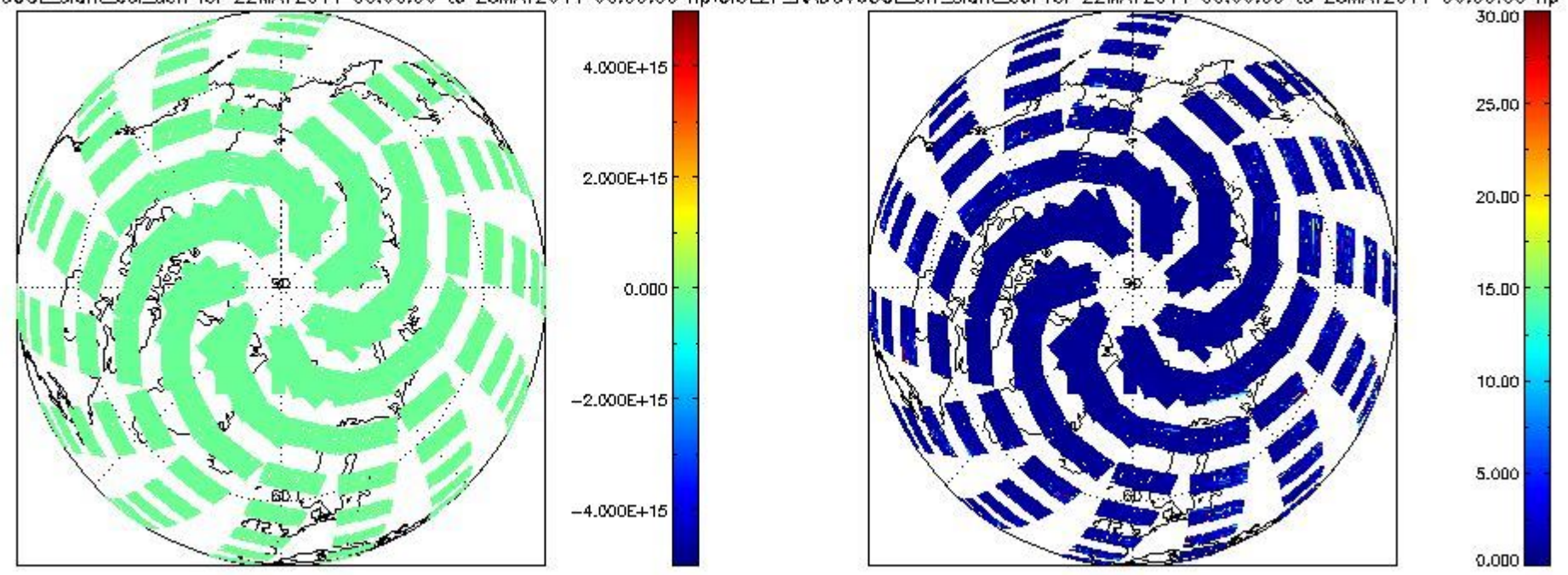
CIOL2P_NADUV60CL_slant_col_den for 22MAY2011 00:00:00 to 23MAY2011 00:00:00 np | CIOL2P_NADUV60CL_err_slant_col for 22MAY2011 00:00:00 to 23MAY2011 00:00:00 np
