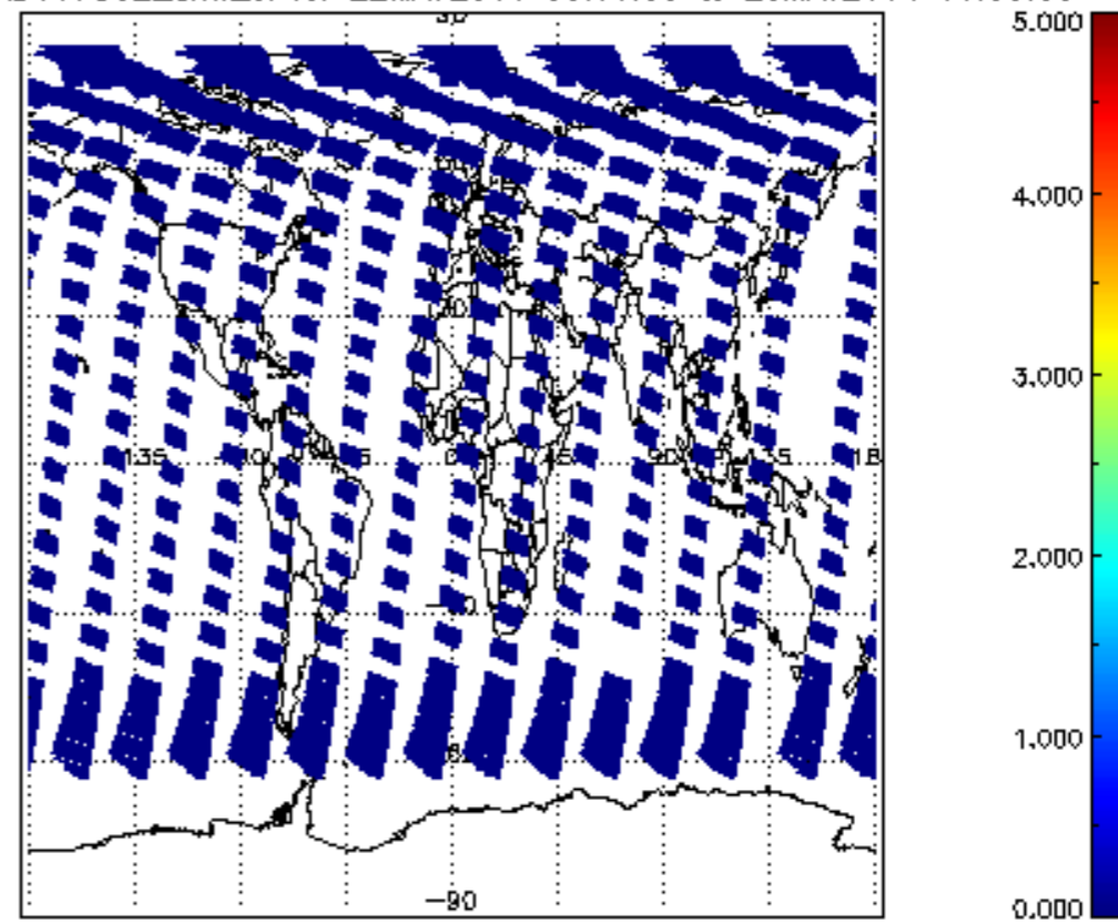
SCIOL2P_NADUV7S02_amf_cl for 22MAY2011 00:00:00 to 23MAY2011 00:00:00
