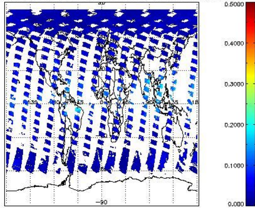
SCIOL2P_NADUV8H2O_vcd_err for 22MAY2011 00:00:00 to 23MAY2011 00:00:00
