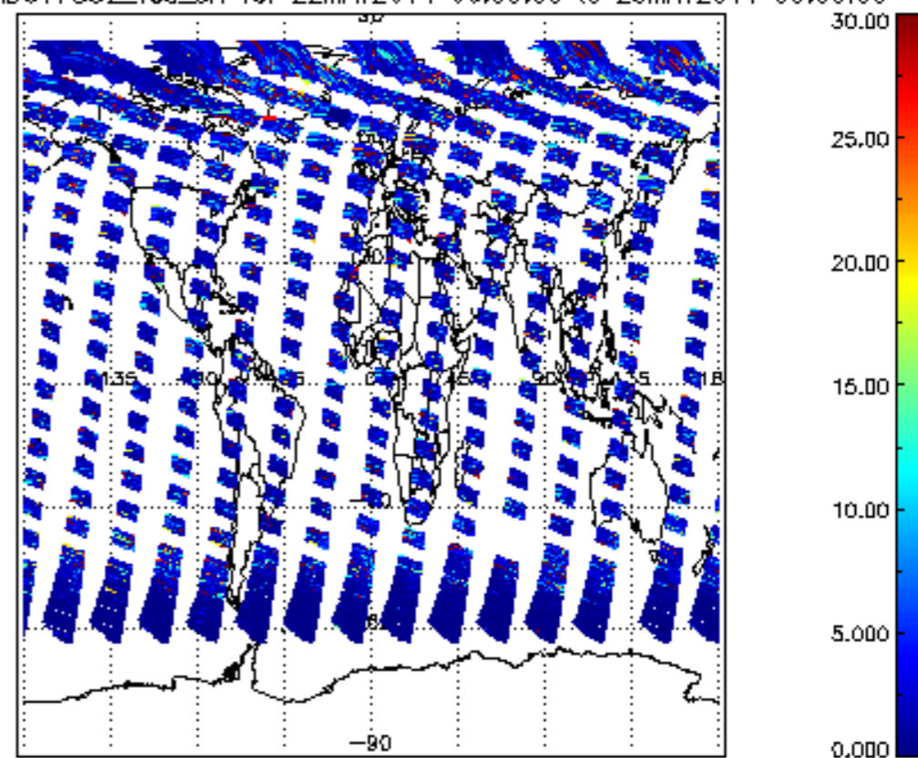
SCIOL2P_NADUV7S02_vcd_err for 22MAY2011 00:00:00 to 23MAY2011 00:00:00
