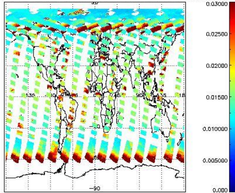
SCIOL2P_NADUV003_vcd_err for 22MAY2011 00:00:00 to 23MAY2011 00:00:00
