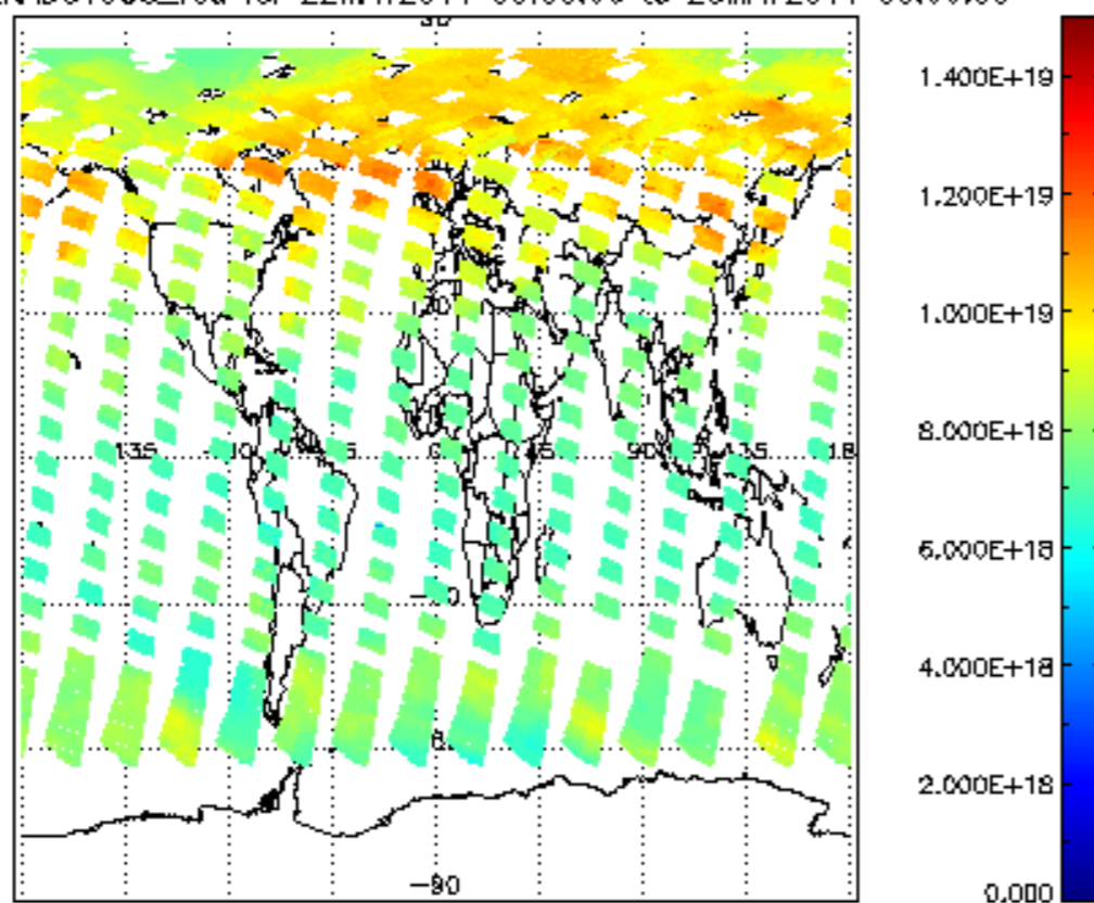
SCIOL2P_NADUV003_vcd for 22MAY2011 00:00:00 to 23MAY2011 00:00:00
