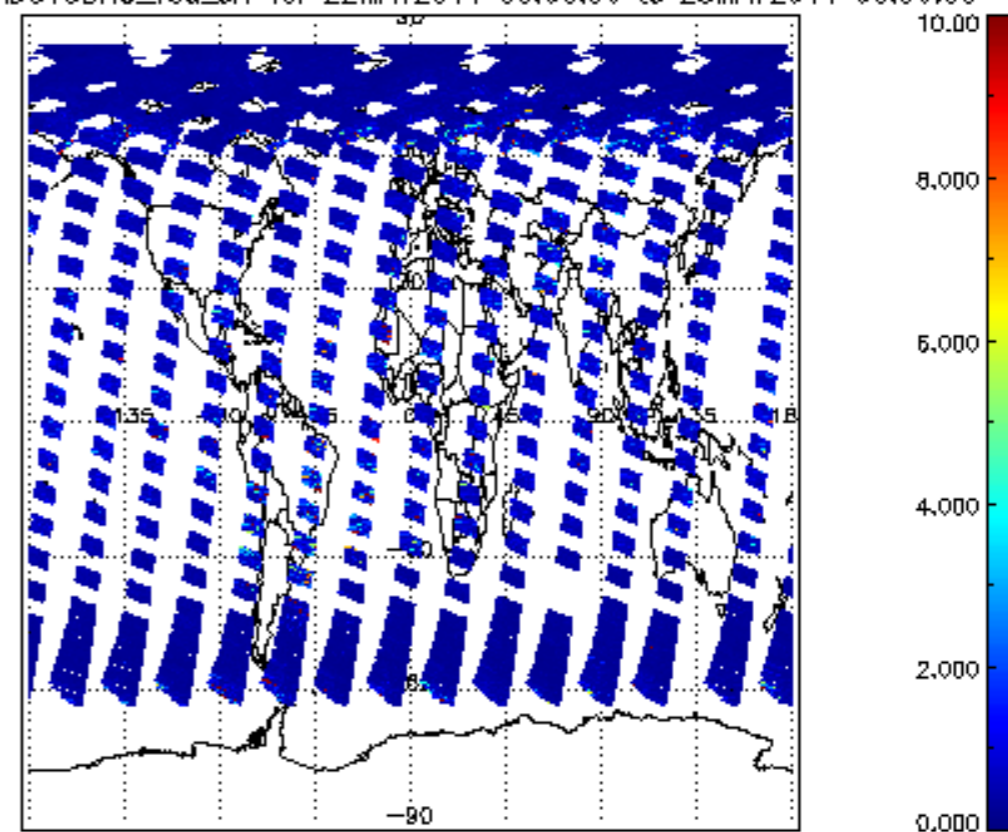
SCIOL2P_NADUV3BRO_vcd_err for 22MAY2011 00:00:00 to 23MAY2011 00:00:00
