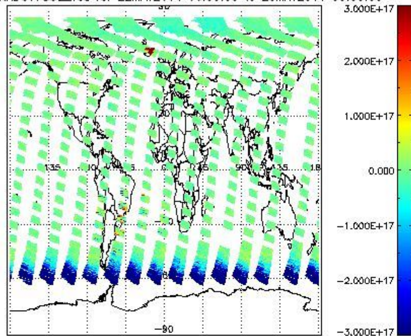
SCIOL2P_NADUV7S02_vcd for 22MAY2011 00:00:00 to 23MAY2011 00:00:00
