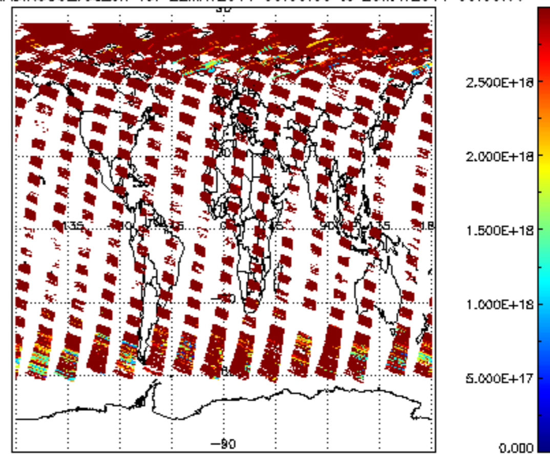
SCIOL2P_NADIR3CO_vcd_err for 22MAY2011 00:00:00 to 23MAY2011 00:00:00
