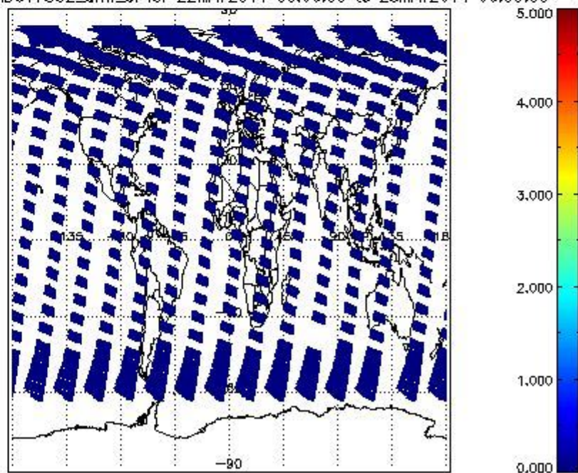
SCIOL2P_NADUV7S02_amf_cl for 22MAY2011 00:00:00 to 23MAY2011 00:00:00
