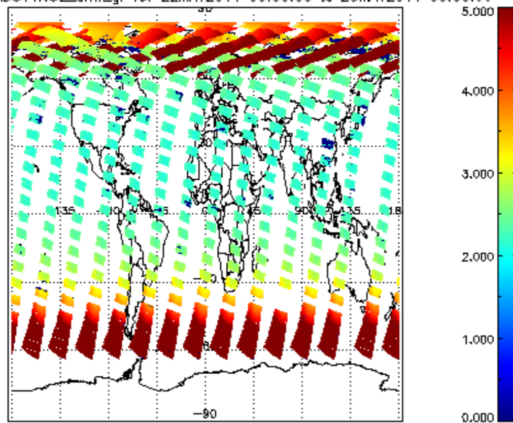
SCIOL2P_NADUV1NO2_amf_gr for 22MAY2011 00:00:00 to 23MAY2011 00:00:00
