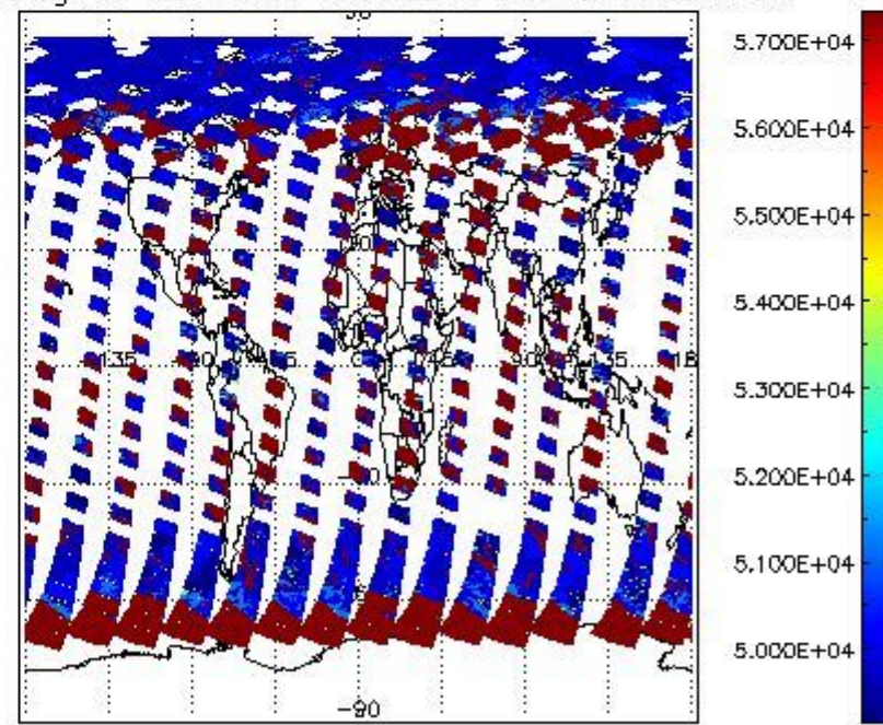
cloud_flags for 22MAY2011 00:00:00 to 23MAY2011 00:00:00
