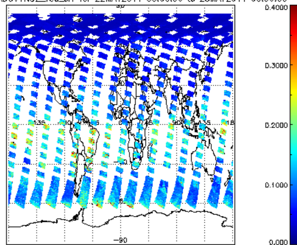
SCIOL2P_NADUV1NO2_vcd_err for 22MAY2011 00:00:00 to 23MAY2011 00:00:00
