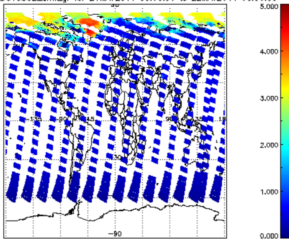
SCIOL2P_NADUV5S02_amf_gr for 21MAY2011 00:00:00 to 22MAY2011 00:00:00
