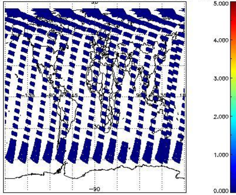
SCIOL2P_NADUV5S02_amf_cl for 21MAY2011 00:00:00 to 22MAY2011 00:00:00
