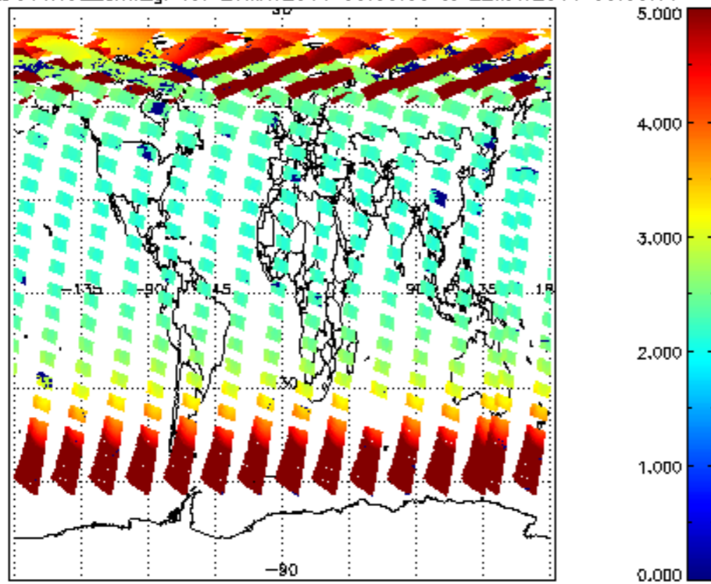
SCIOL2P_NADUV1NO2_amf_gr for 21MAY2011 00:00:00 to 22MAY2011 00:00:00
