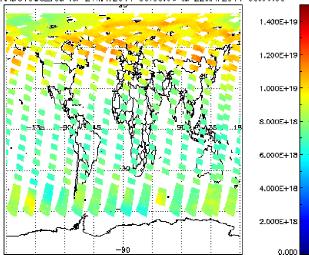
SCIOL2P_NADUV003_vcd for 21MAY2011 00:00:00 to 22MAY2011 00:00:00
