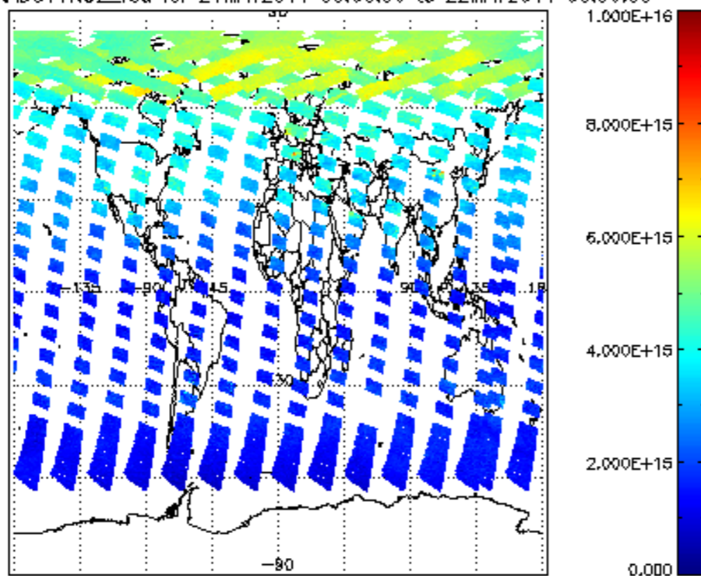
SCIOL2P_NADUV1NO2_vcd for 21MAY2011 00:00:00 to 22MAY2011 00:00:00
