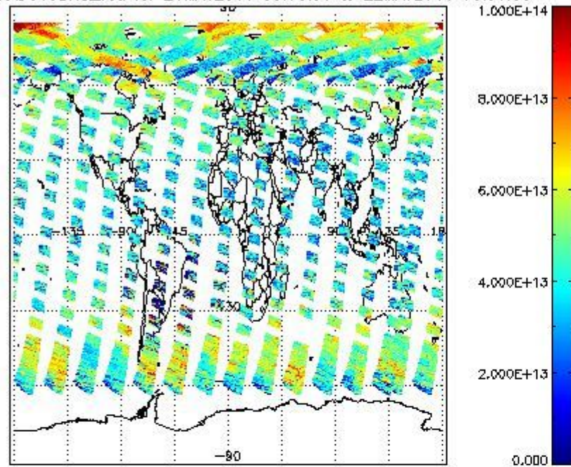
SCIOL2P_NADUV3BRO_vcd for 21MAY2011 00:00:00 to 22MAY2011 00:00:00
