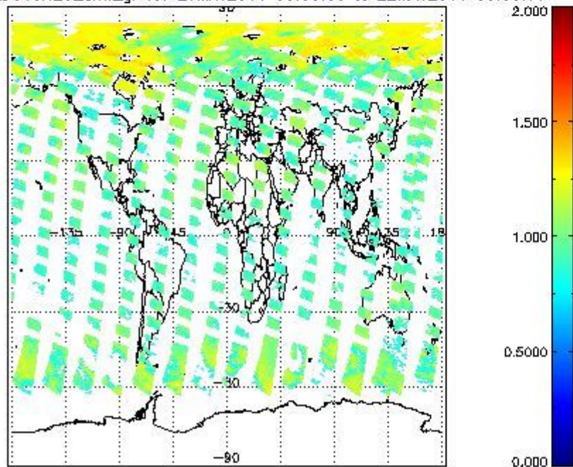
SCIOL2P_NADUV8H2O_arnf_gr for 21MAY2011 00:00:00 to 22MAY2011 00:00:00
