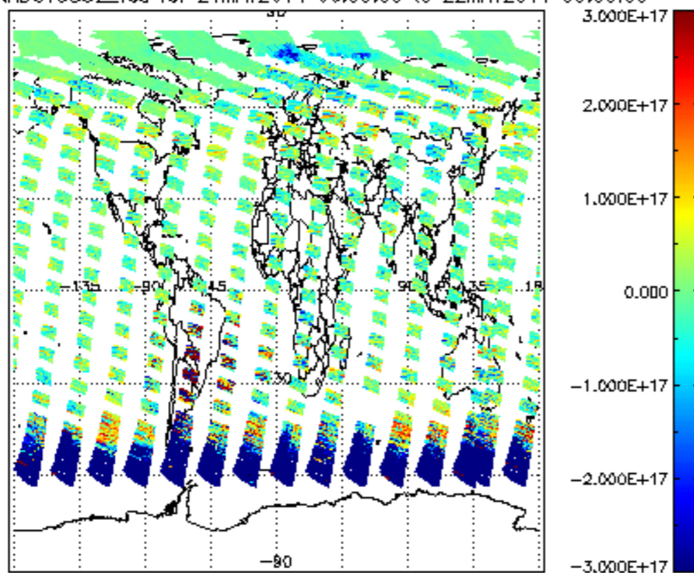
SCIOL2P_NADUV5S02_vcd for 21MAY2011 00:00:00 to 22MAY2011 00:00:00
