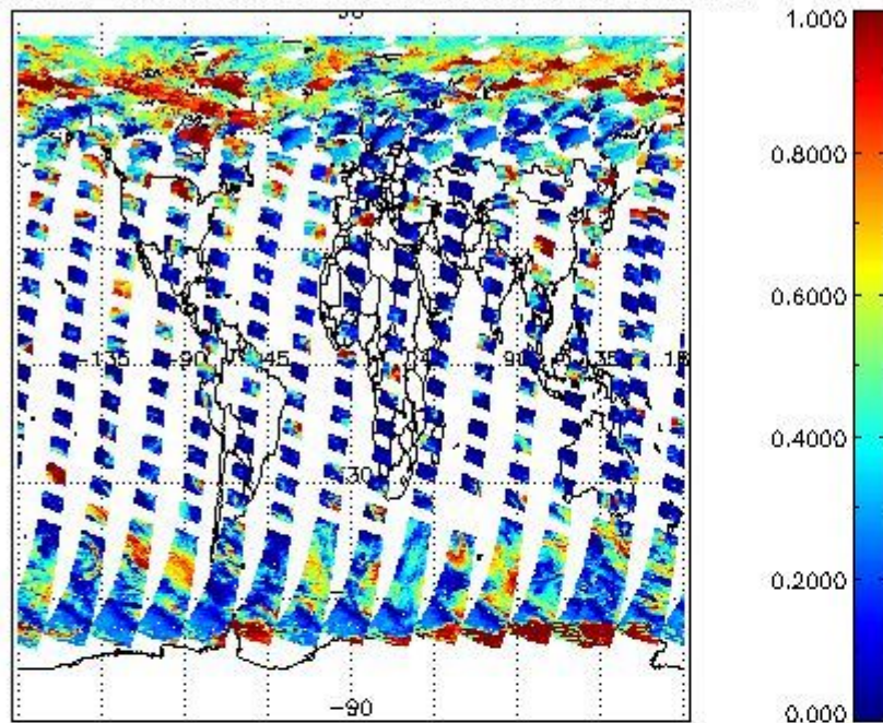
cL_frac for 21MAY2011 00:00:00 to 22MAY2011 00:00:00
