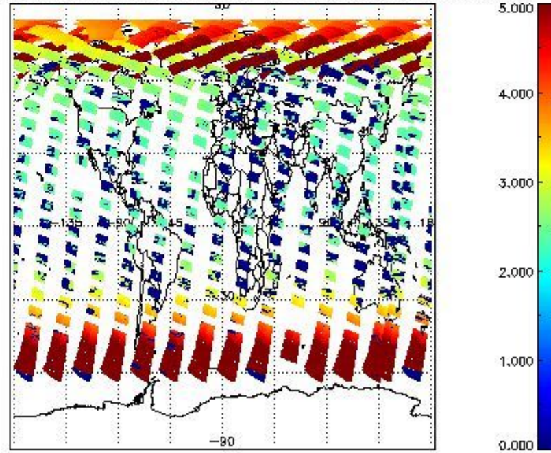
SCIOL2P_NADUV003_amf_cl for 21MAY2011 00:00:00 to 22MAY2011 00:00:00
