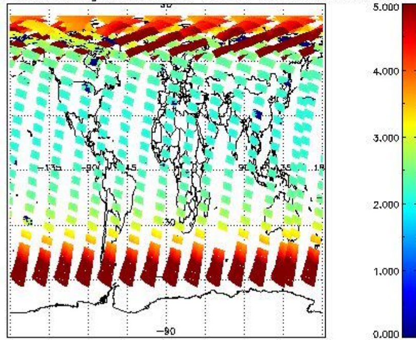
SCIOL2P_NADUV3BRO_amf_gr for 21MAY2011 00:00:00 to 22MAY2011 00:00:00
