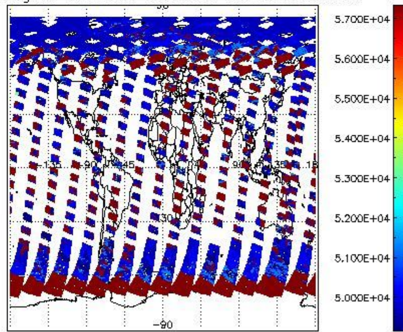
cloud_flags for 21MAY2011 00:00:00 to 22MAY2011 00:00:00
