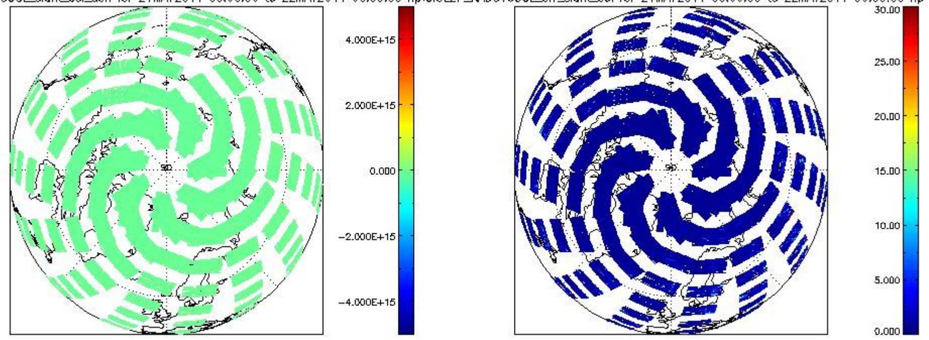
CIOL2P_NADUV6OCLslant_col_den for 21MAY2011 00:00:00 to 22MAY2011 00:00:00 np; CIOL2P_NADUV6OCLarr_slant_col for 21MAY2011 00:00:00 to 22MAY2011 00:00:00 np
