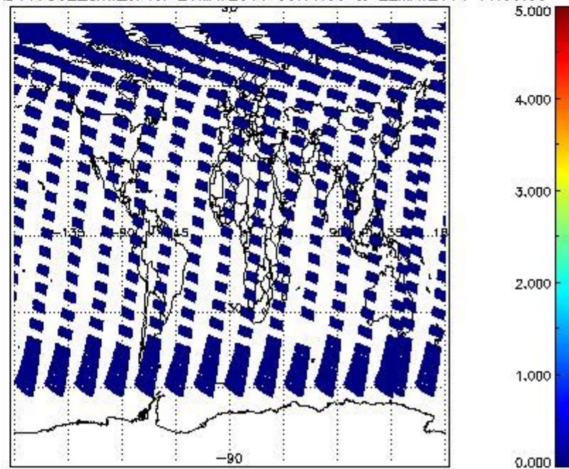
SCIOL2P_NADUV7S02_amf_cl for 21MAY2011 00:00:00 to 22MAY2011 00:00:00
