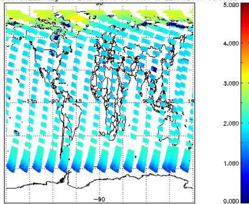
SCIOL2P_NADUV7S02_amf_gr for 21MAY2011 00:00:00 to 22MAY2011 00:00:00
