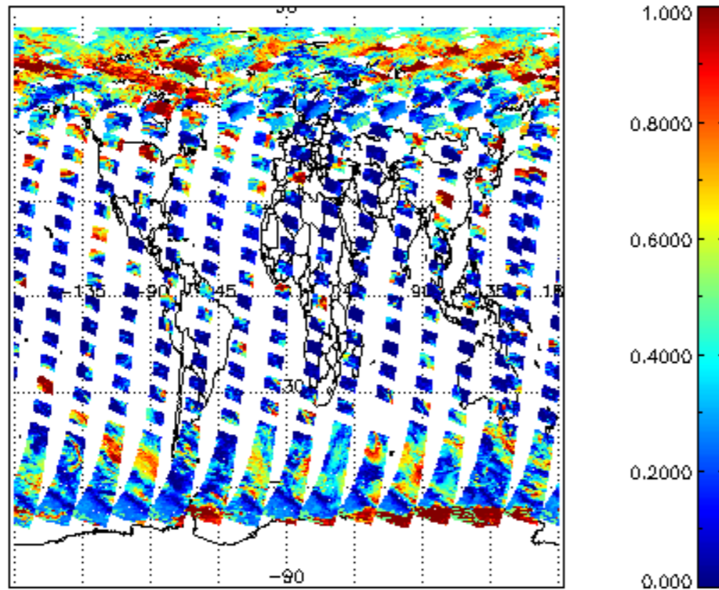
cl_frac for 21MAY2011 00:00:00 to 22MAY2011 00:00:00
