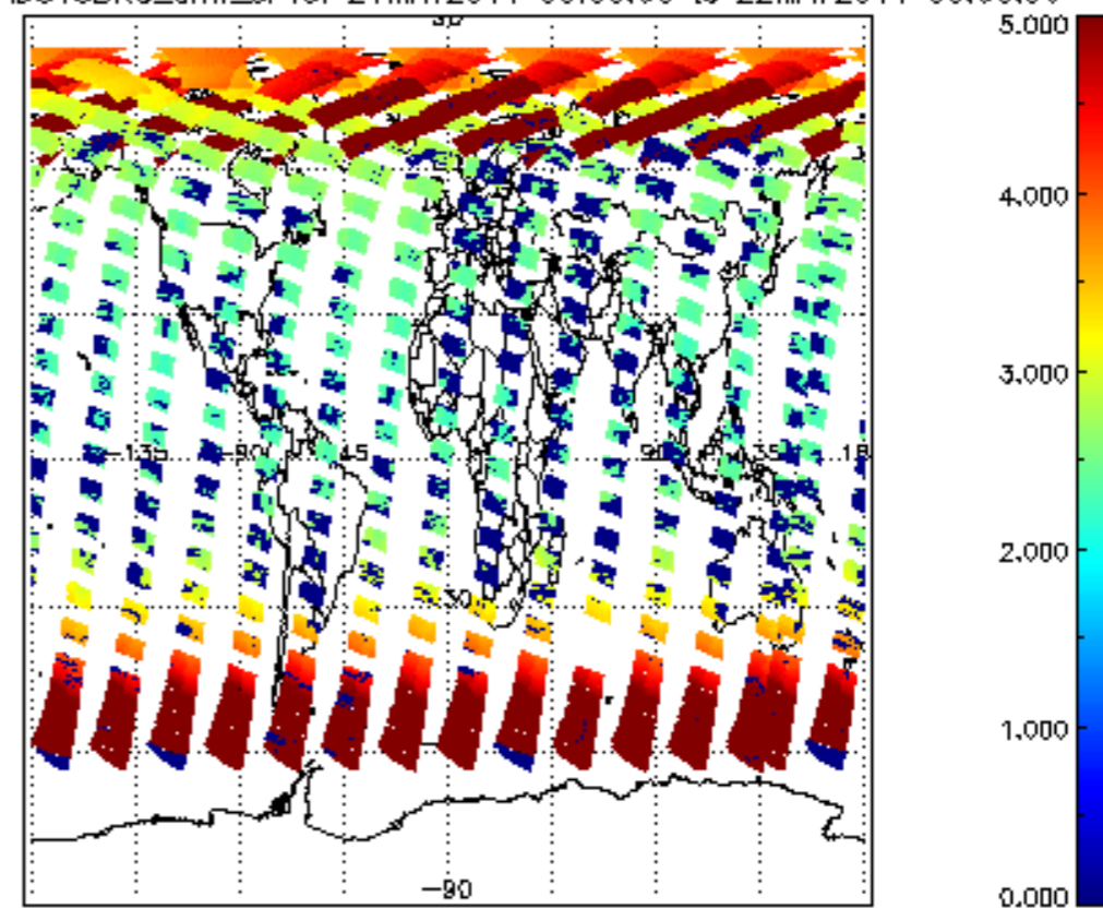
SCIOL2P_NADUV3BRO_amf_sl for 21MAY2011 00:00:00 to 22MAY2011 00:00:00
