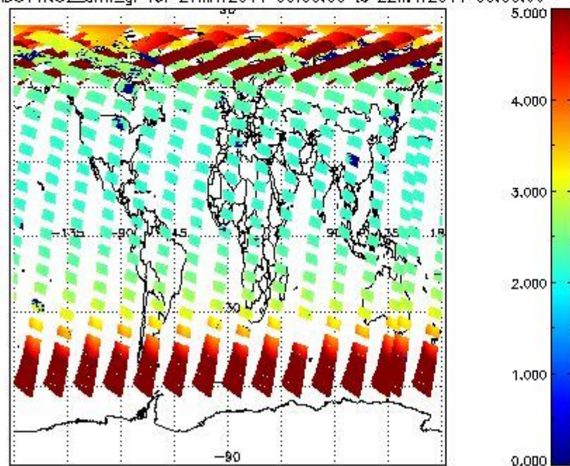
SCIOL2P_NADUV1NO2_amf_gr for 21MAY2011 00:00:00 to 22MAY2011 00:00:00
