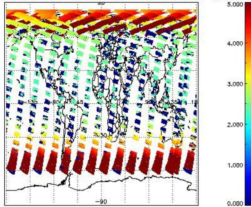
SCIOL2P_NADUV3BRO_amf_cl for 21MAY2011 00:00:00 to 22MAY2011 00:00:00
