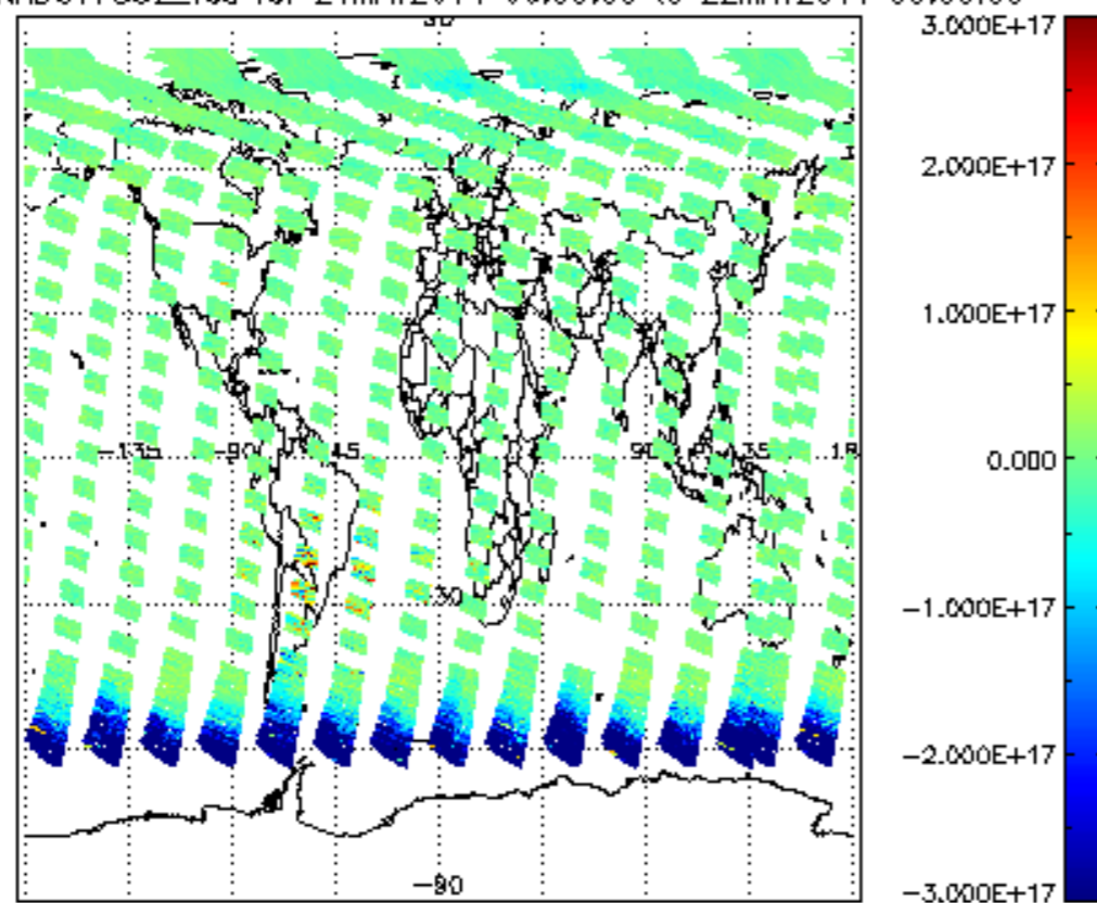
SCIOL2P_NADUV7S02_vcd for 21MAY2011 00:00:00 to 22MAY2011 00:00:00
