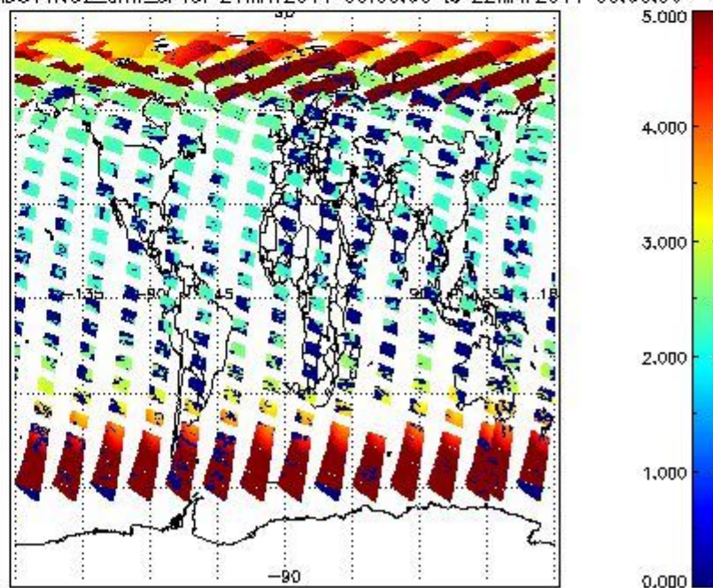
SCIOL2P_NADUV1NO2_amf_cl for 21MAY2011 00:00:00 to 22MAY2011 00:00:00
