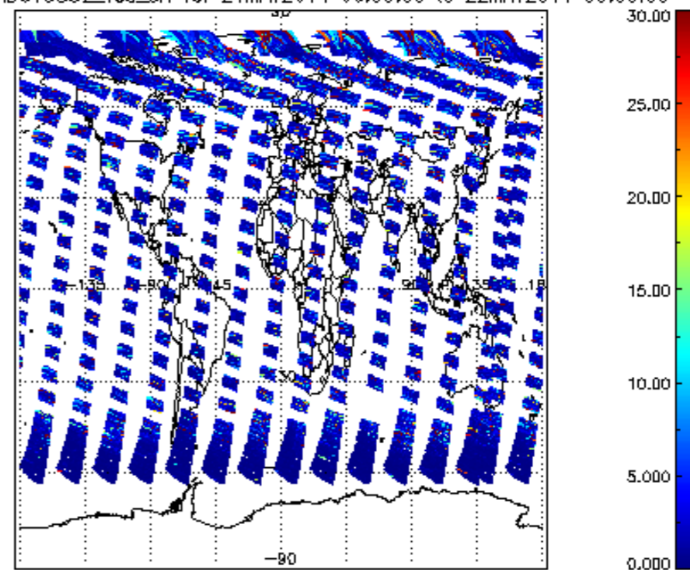
SCIOL2P_NADUV5S02_vcd_err for 21MAY2011 00:00:00 to 22MAY2011 00:00:00
