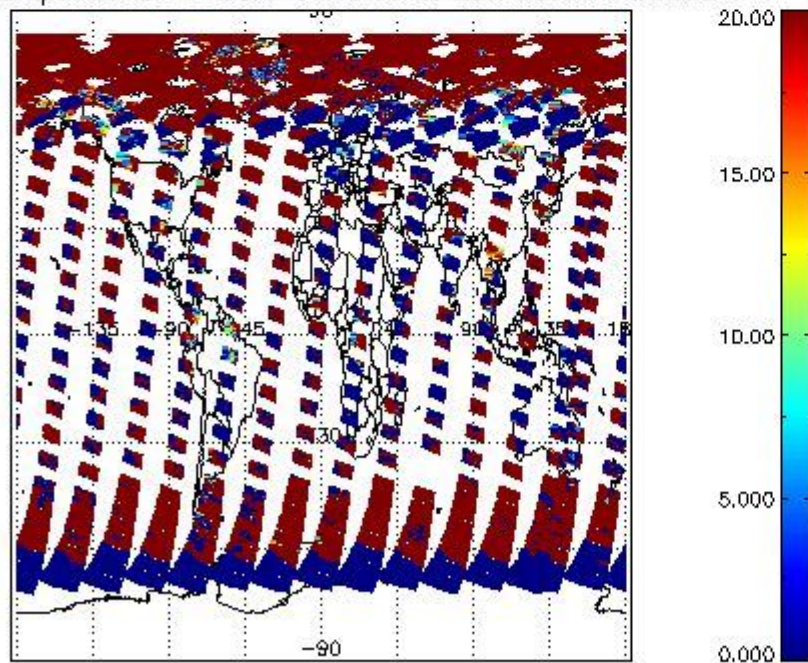
cL_opt_depth for 21MAY2011 00:00:00 to 22MAY2011 00:00:00
