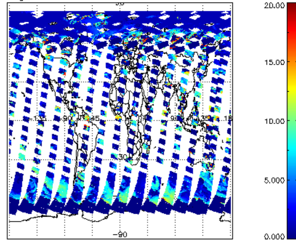
cl_top_height for 21MAY2011 00:00:00 to 22MAY2011 00:00:00
