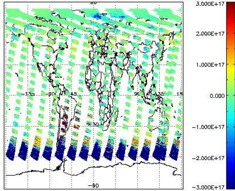
SCIOL2P_NADUV5S02_vcd for 21MAY2011 00:00:00 to 22MAY2011 00:00:00
