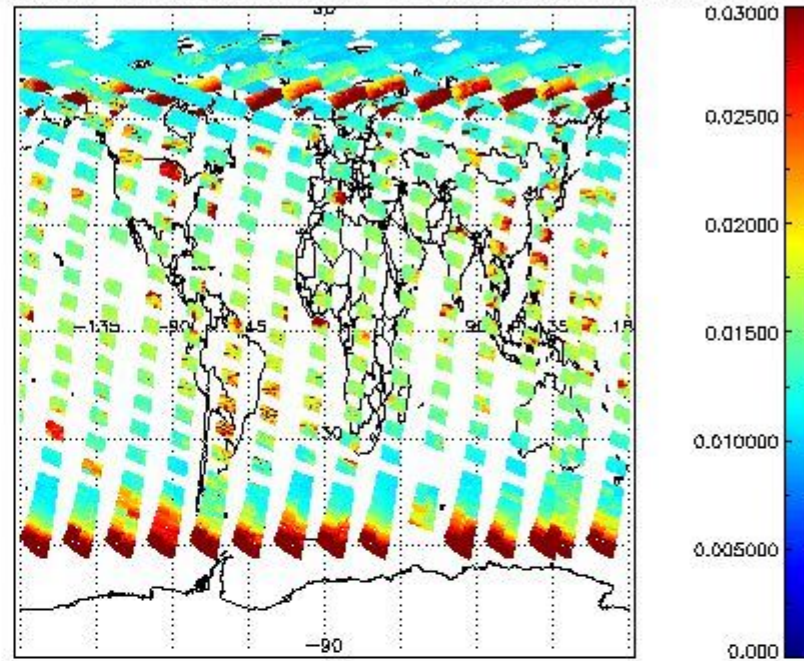
SCIOL2P_NADUV003_vcd_err for 21MAY2011 00:00:00 to 22MAY2011 00:00:00
