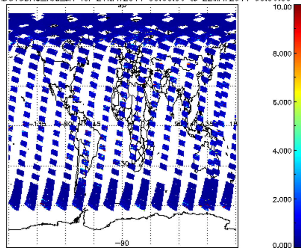
SCIOL2P_NADUV3BRO_vcd_err for 21MAY2011 00:00:00 to 22MAY2011 00:00:00
