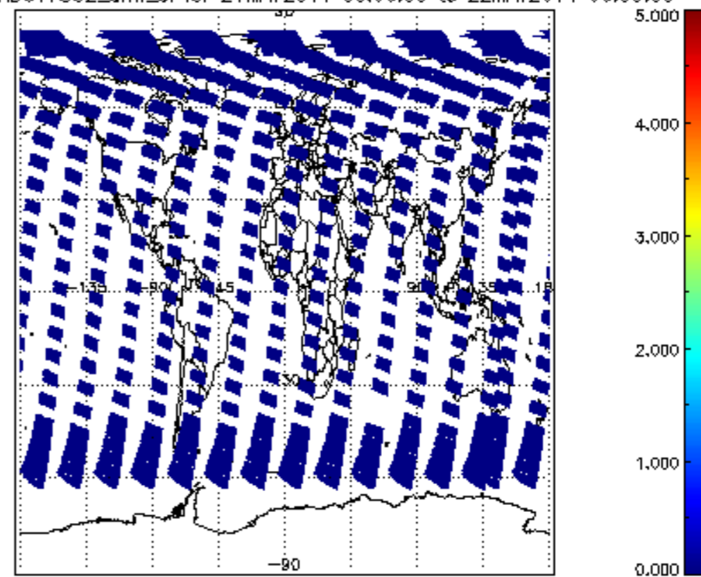
SCIOL2P_NADUV7S02_amf_cl for 21MAY2011 00:00:00 to 22MAY2011 00:00:00
