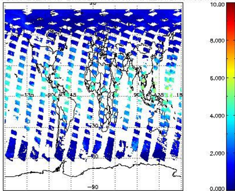
SCIOL2P_NADUV8H2O_vcd for 21MAY2011 00:00:00 to 22MAY2011 00:00:00
