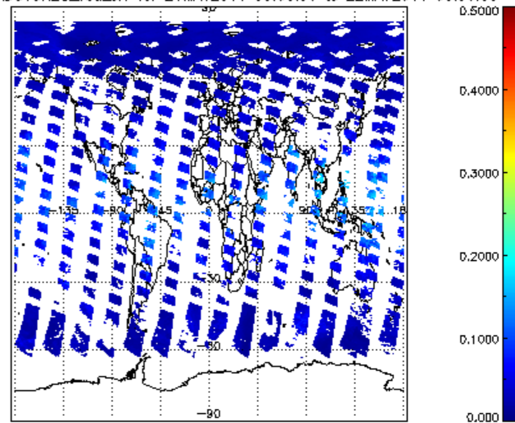
SCIOL2P_NADUV8H2O_vcd_err for 21MAY2011 00:00:00 to 22MAY2011 00:00:00
