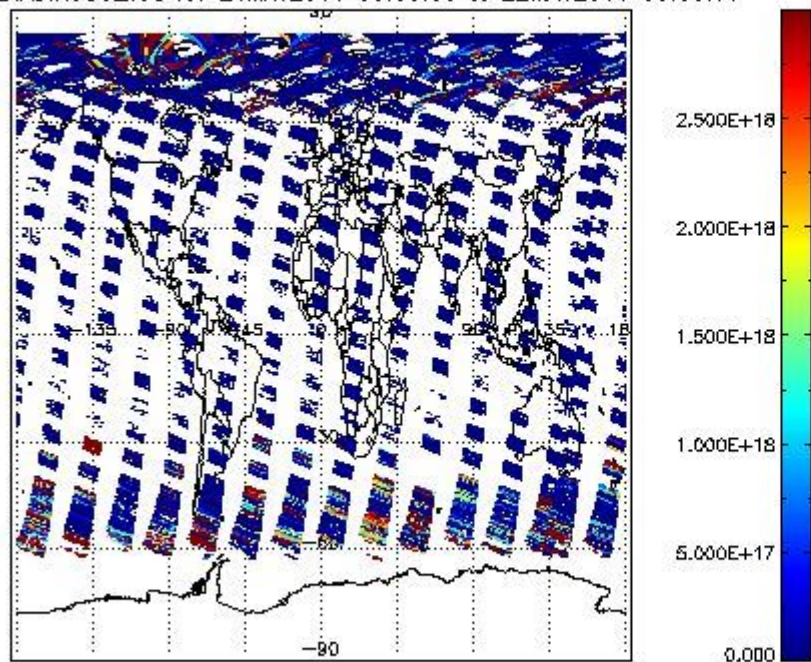
SCIDL2P_NADIR3CO_vcd for 21MAY2011 00:00:00 to 22MAY2011 00:00:00
