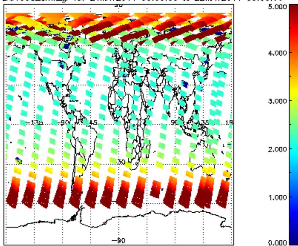
SCIOL2P_NADUV003_amf_gr for 21MAY2011 00:00:00 to 22MAY2011 00:00:00
