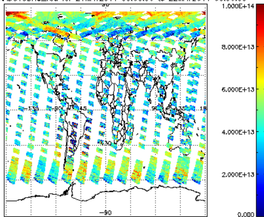
SCIOL2P_NADUV3BRO_vcd for 21MAY2011 00:00:00 to 22MAY2011 00:00:00
