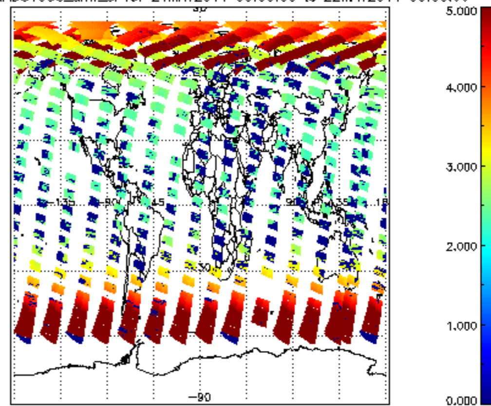
SCIOL2P_NADUV003_amf_cl for 21MAY2011 00:00:00 to 22MAY2011 00:00:00
