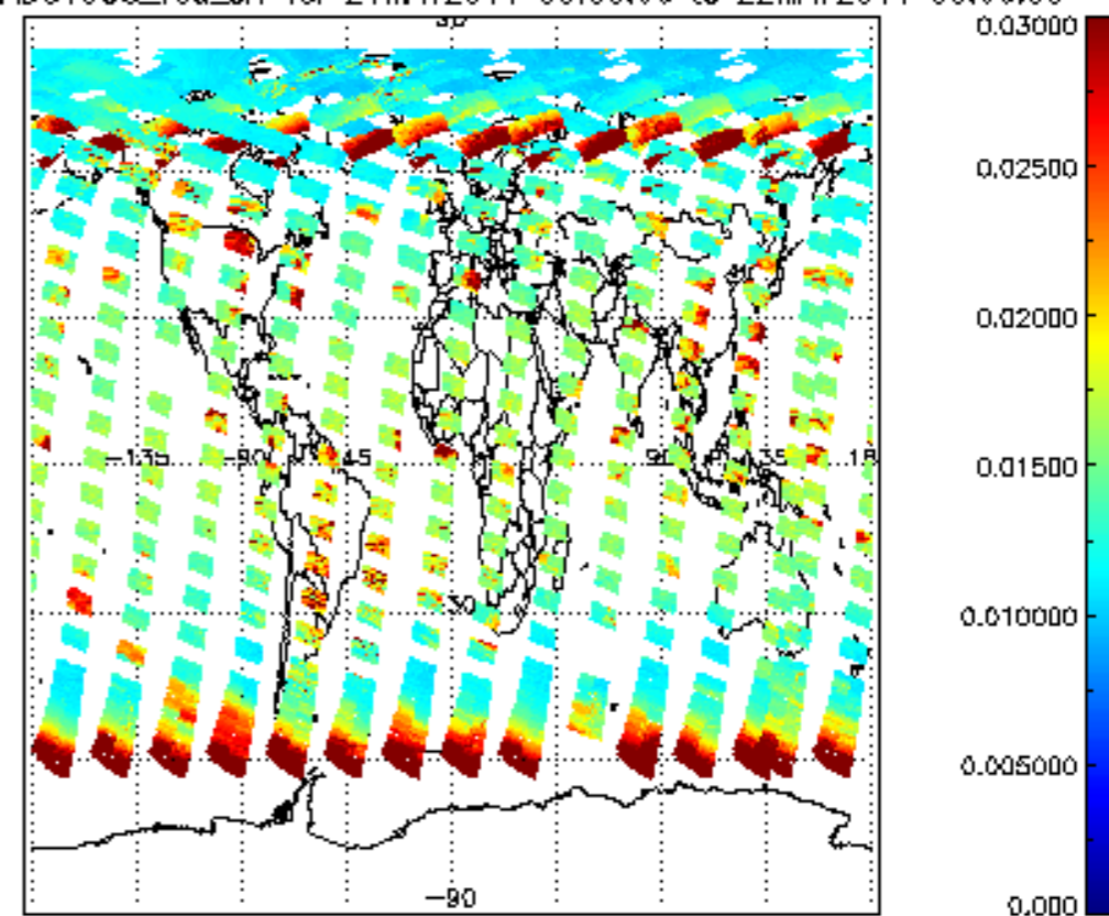
SCIOL2P_NADUV003_vcd_err for 21MAY2011 00:00:00 to 22MAY2011 00:00:00
