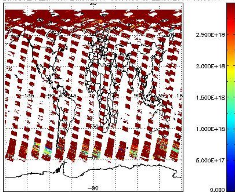
SCIDL2P_NADIR3CO_vcd_err for 21MAY2011 00:00:00 to 22MAY2011 00:00:00
