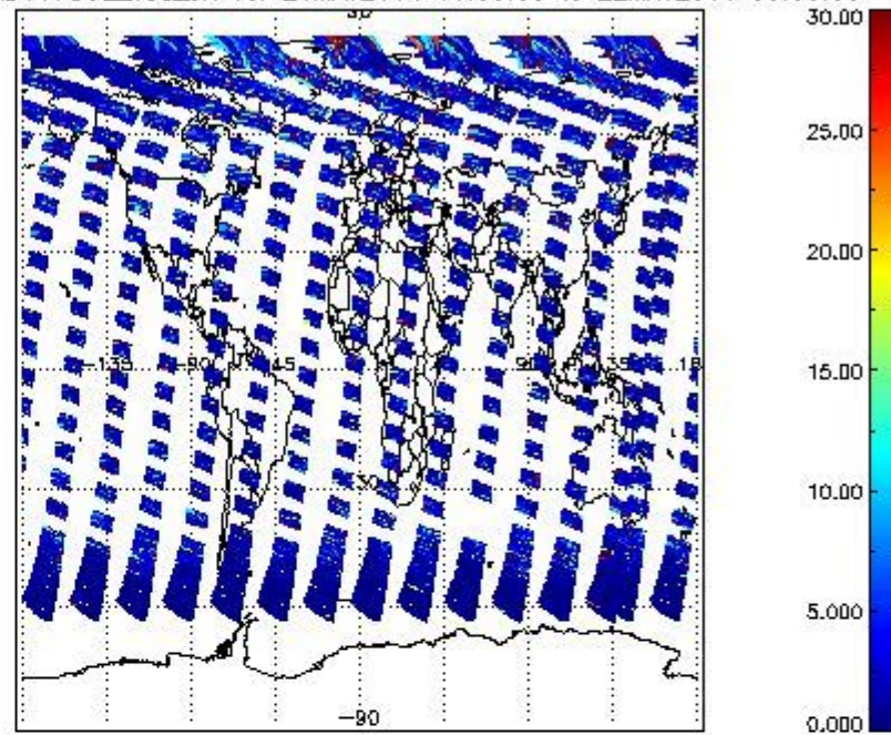
SCIOL2P_NADUV7S02_vcd_err for 21MAY2011 00:00:00 to 22MAY2011 00:00:00
