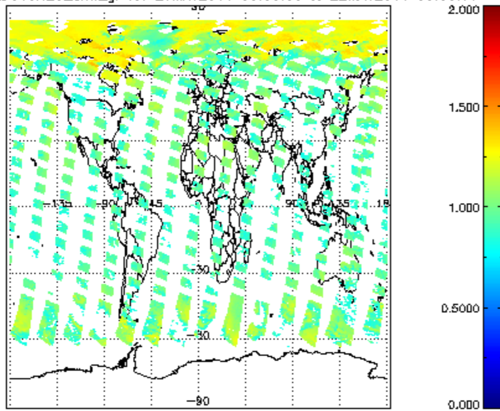
SCIOL2P_NADUV8H2O_amf_gr for 21MAY2011 00:00:00 to 22MAY2011 00:00:00
