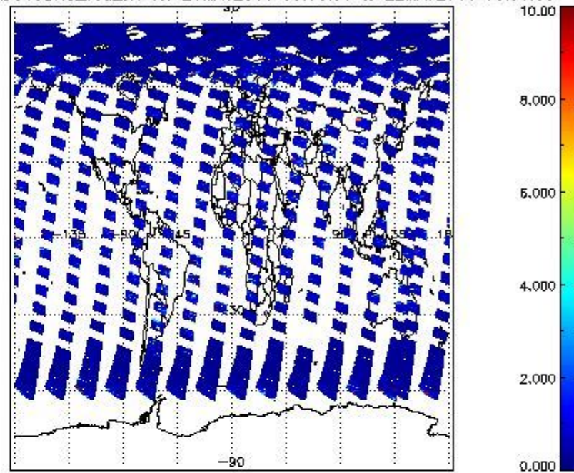
SCIOL2P_NADUV3BRO_vcd_err for 21MAY2011 00:00:00 to 22MAY2011 00:00:00
