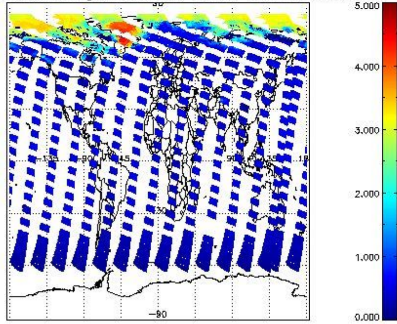
SCIOL2P_NADUV5S02_amf_gr for 21MAY2011 00:00:00 to 22MAY2011 00:00:00
