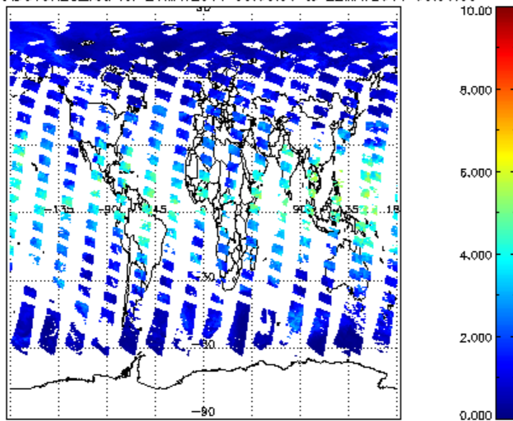
SCIOL2P_NADUV8H2O_vcd for 21MAY2011 00:00:00 to 22MAY2011 00:00:00
