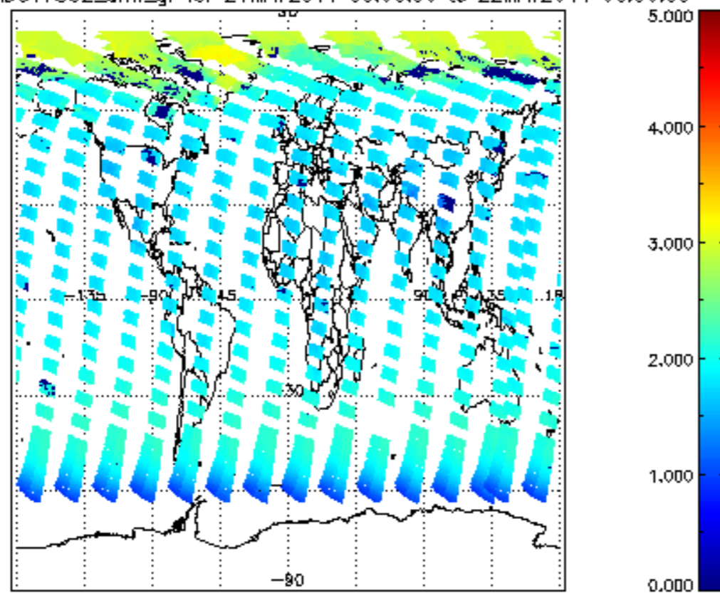
SCIOL2P_NADUV7S02_amf_gr for 21MAY2011 00:00:00 to 22MAY2011 00:00:00
