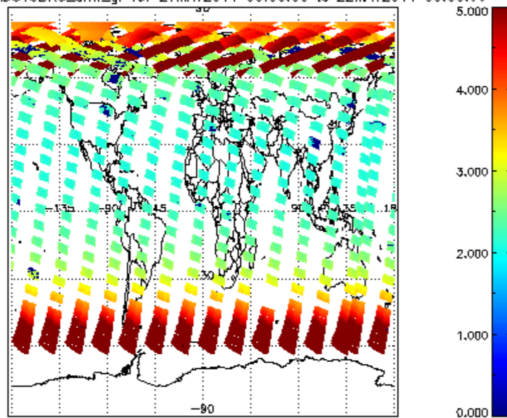
SCIOL2P_NADUV3BRO_amf_gr for 21MAY2011 00:00:00 to 22MAY2011 00:00:00
