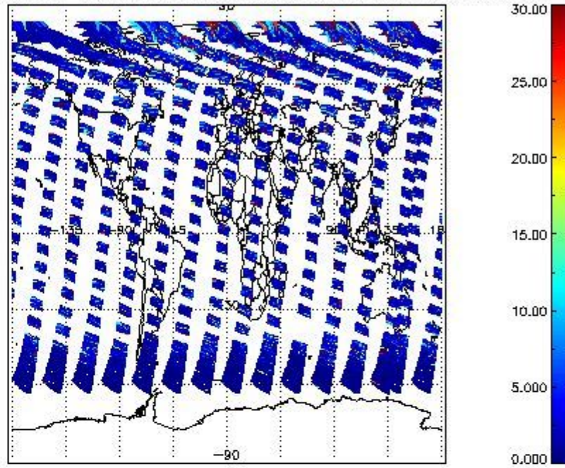
SCIOL2P_NADUV5S02_vcd_err for 21MAY2011 00:00:00 to 22MAY2011 00:00:00
