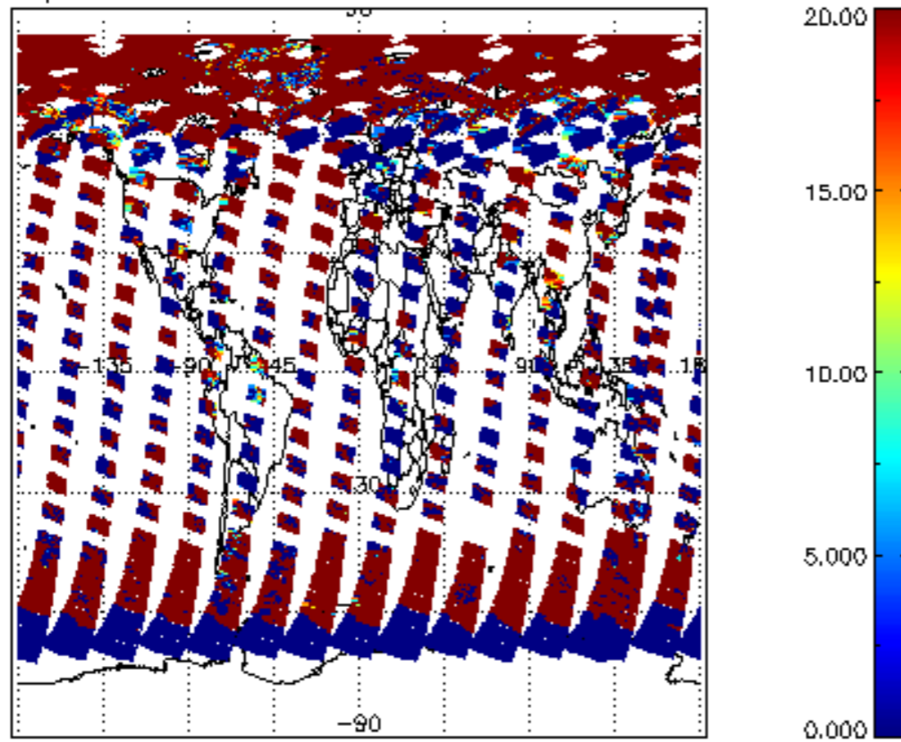
cl_opt_depth for 21MAY2011 00:00:00 to 22MAY2011 00:00:00
