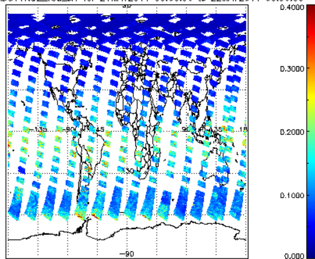
SCIOL2P_NADUV1NO2_vcd_err for 21MAY2011 00:00:00 to 22MAY2011 00:00:00
