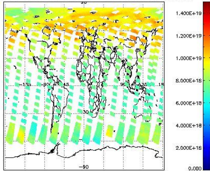
SCIOL2P_NADUV003_vcd for 21MAY2011 00:00:00 to 22MAY2011 00:00:00
