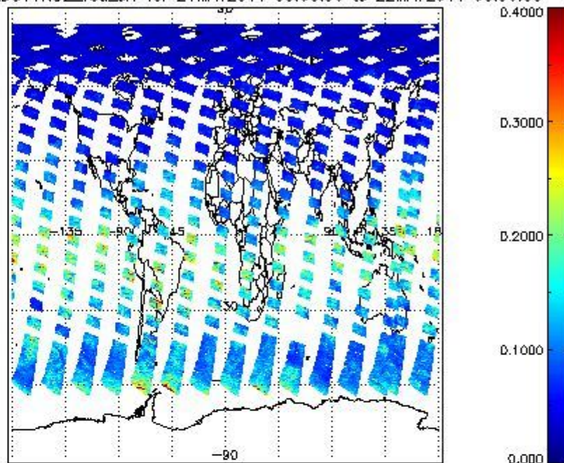
SCIOL2P_NADUV1NO2_vcd_err for 21MAY2011 00:00:00 to 22MAY2011 00:00:00
