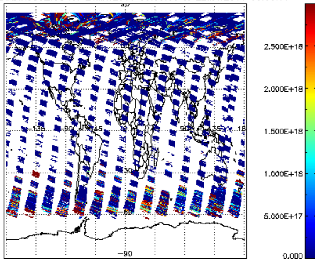
SCIOL2P_NADIR3CO_vcd for 21MAY2011 00:00:00 to 22MAY2011 00:00:00
