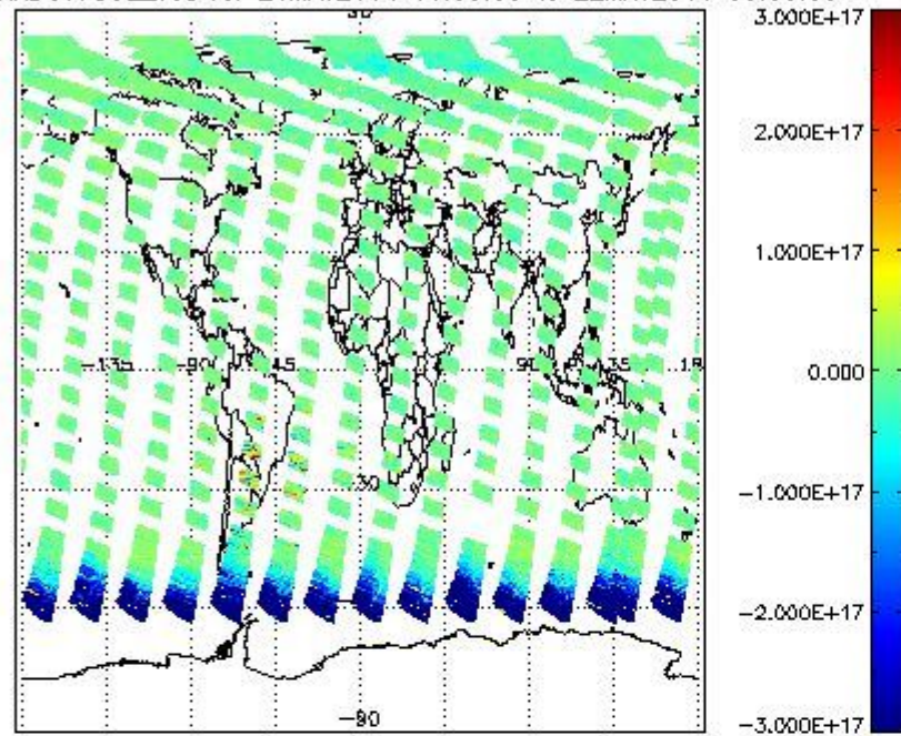
SCIOL2P_NADUV7S02_vcd for 21MAY2011 00:00:00 to 22MAY2011 00:00:00
