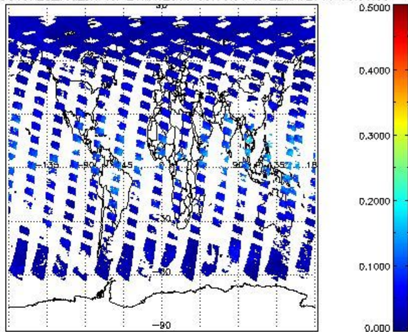
SCIOL2P_NADUV8H2O_vcd_err for 21MAY2011 00:00:00 to 22MAY2011 00:00:00
