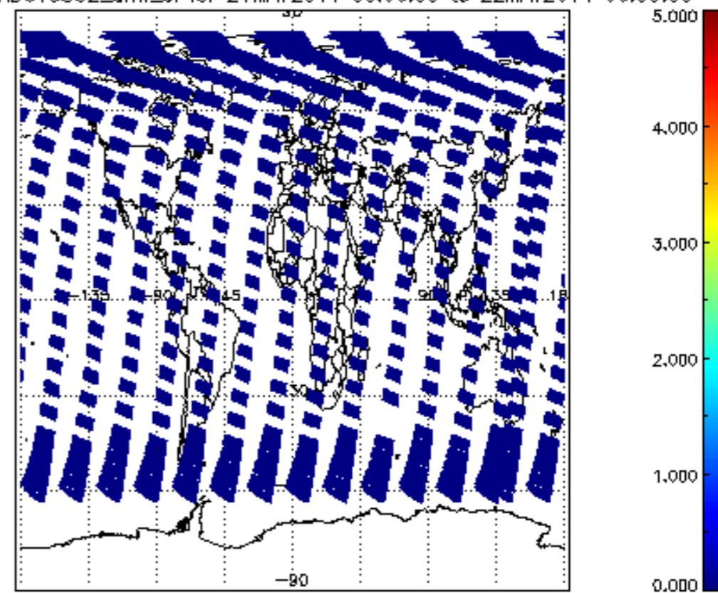
SCIOL2P_NADUV5S02_amf_cl for 21MAY2011 00:00:00 to 22MAY2011 00:00:00
