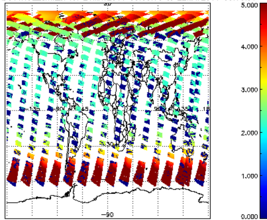
SCIOL2P_NADUV1NO2_amf_cl for 21MAY2011 00:00:00 to 22MAY2011 00:00:00
