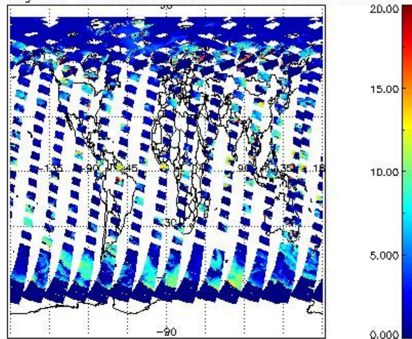
cL_top_height for 21MAY2011 00:00:00 to 22MAY2011 00:00:00
