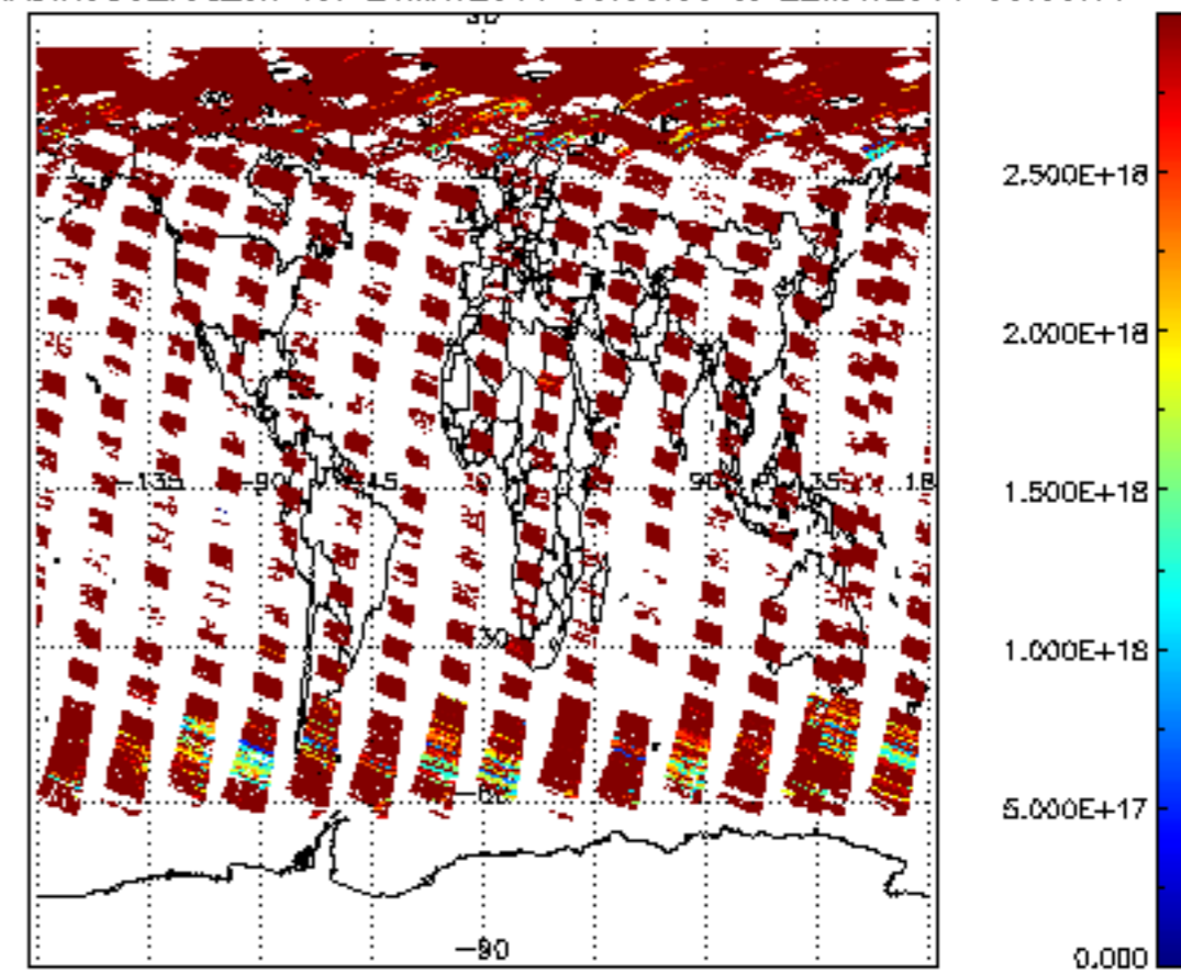
SCIOL2P_NADIR3CO_vcd_err for 21MAY2011 00:00:00 to 22MAY2011 00:00:00
