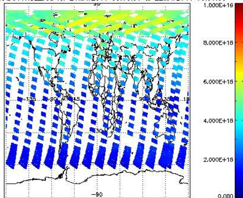
SCIOL2P_NADUV1NO2_vcd for 21MAY2011 00:00:00 to 22MAY2011 00:00:00
