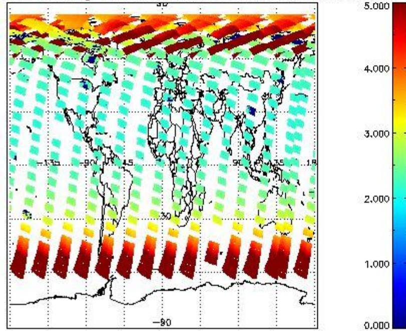
SCIOL2P_NADUV003_amf_gr for 21MAY2011 00:00:00 to 22MAY2011 00:00:00
