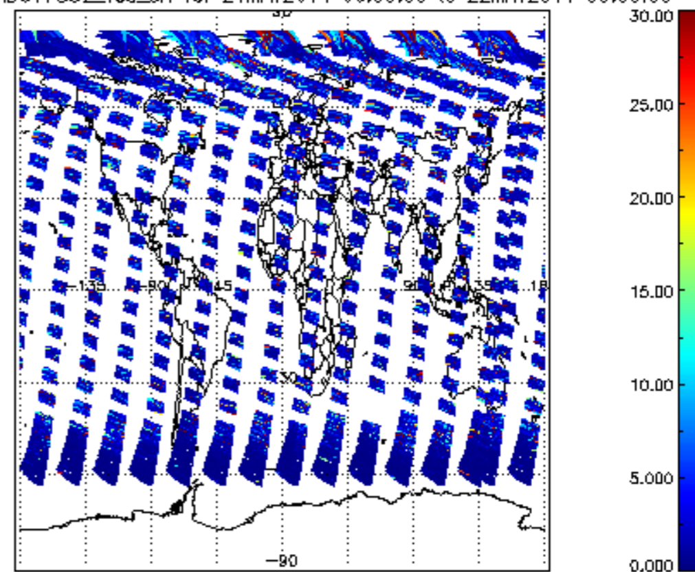
SCIOL2P_NADUV7S02_vcd_err for 21MAY2011 00:00:00 to 22MAY2011 00:00:00
