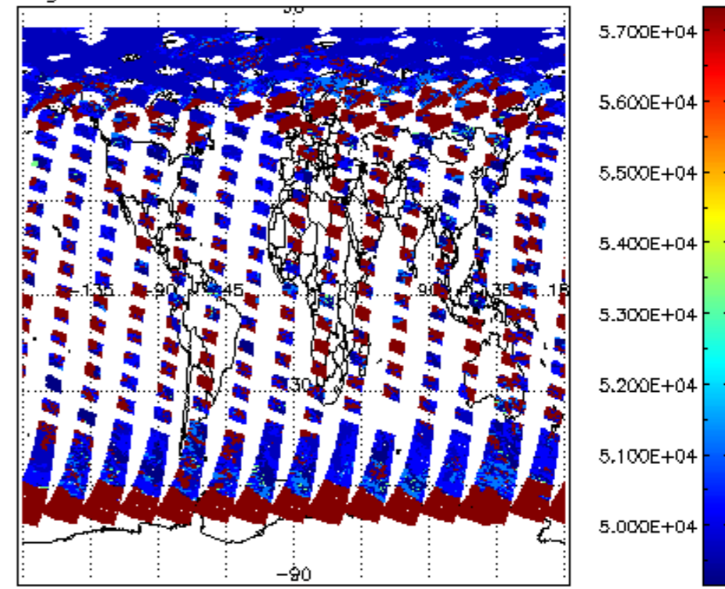
cloud_flags for 21MAY2011 00:00:00 to 22MAY2011 00:00:00
