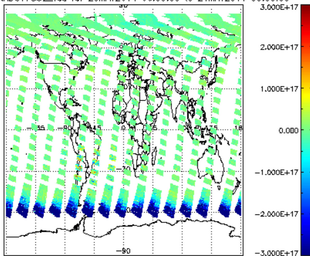
SCIOL2P_NADUV7S02_vcd for 20MAY2011 00:00:00 to 21MAY2011 00:00:00
