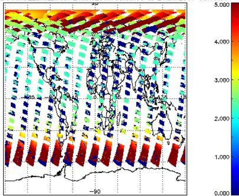
SCIOL2P_NADUV1NO2_amf_cl for 20MAY2011 00:00:00 to 21MAY2011 00:00:00
