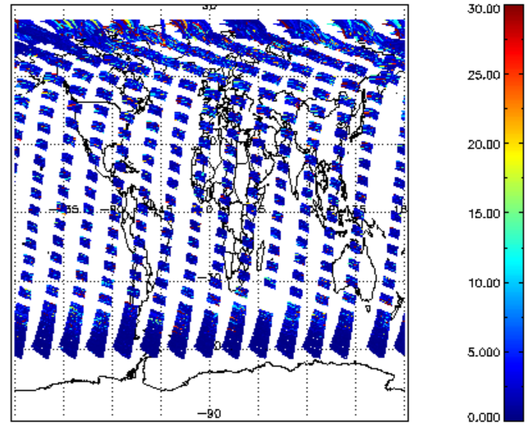
SCIOL2P_NADUV5S02_vcd_err for 20MAY2011 00:00:00 to 21MAY2011 00:00:00
