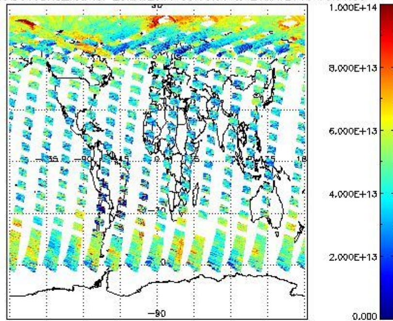
SCIOL2P_NADUV3BRO_vcd for 20MAY2011 00:00:00 to 21MAY2011 00:00:00
