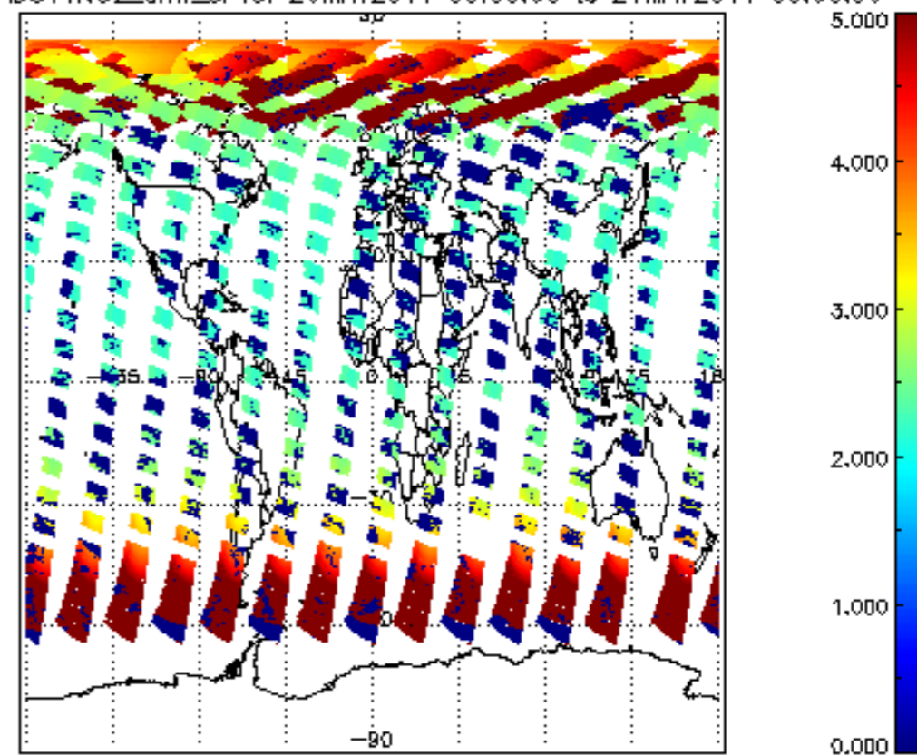
SCIOL2P_NADUV1NO2_amf_sl for 20MAY2011 00:00:00 to 21MAY2011 00:00:00
