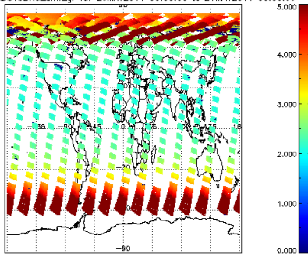
SCIOL2P_NADUV3BRO_amf_gr for 20MAY2011 00:00:00 to 21MAY2011 00:00:00
