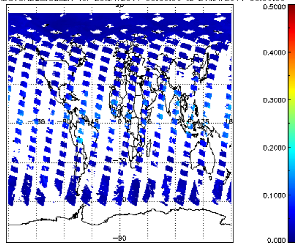
SCIOL2P_NADUV8H2O_vcd_err for 20MAY2011 00:00:00 to 21MAY2011 00:00:00
