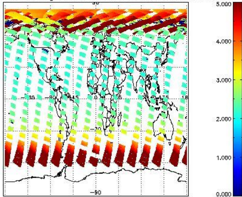
SCIOL2P_NADUV003_amf_gr for 20MAY2011 00:00:00 to 21MAY2011 00:00:00
