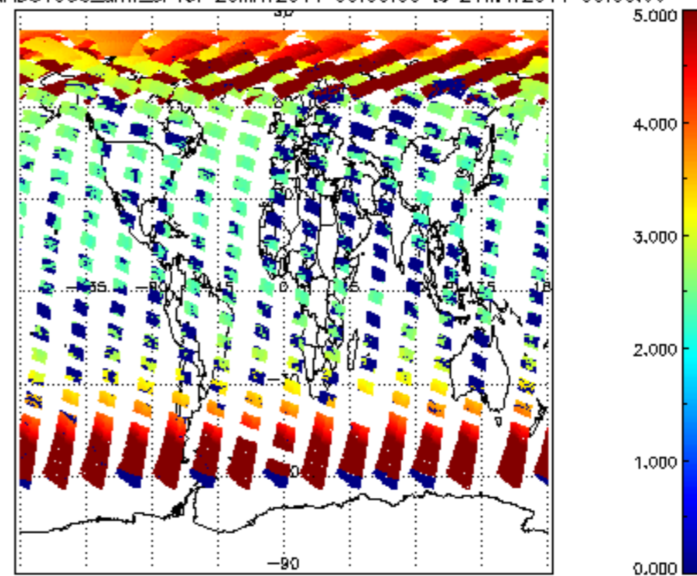
SCIOL2P_NADUV003_amf_cl for 20MAY2011 00:00:00 to 21MAY2011 00:00:00
