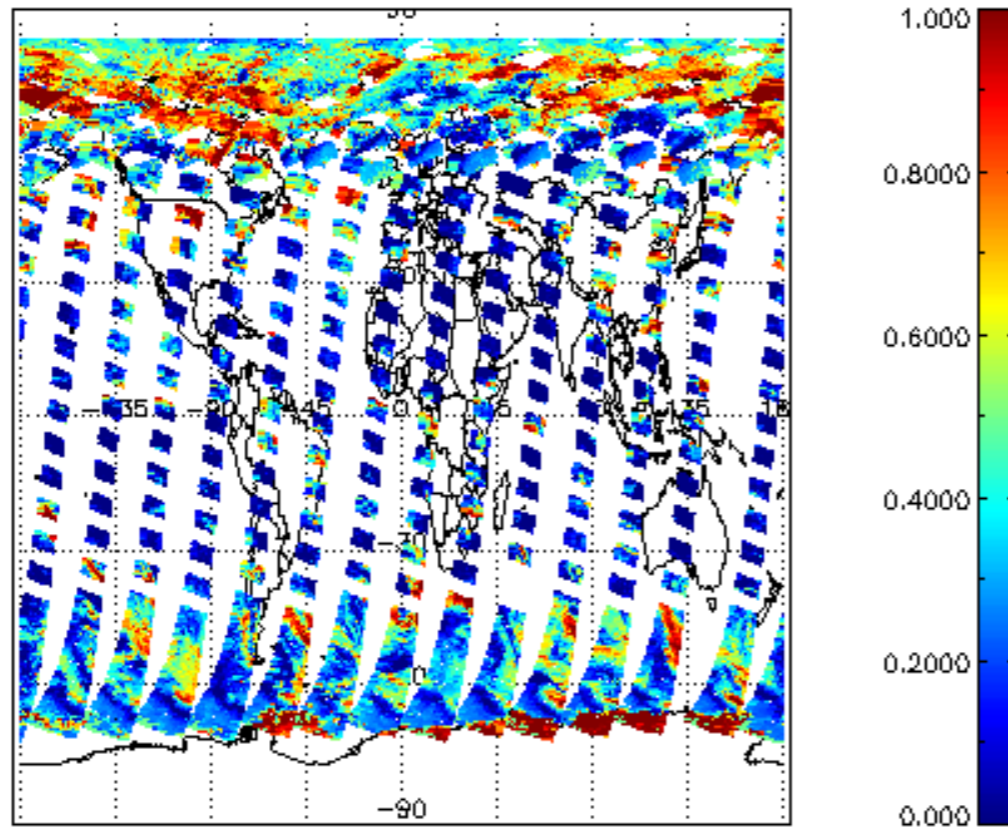
cl_frac for 20MAY2011 00:00:00 to 21MAY2011 00:00:00
