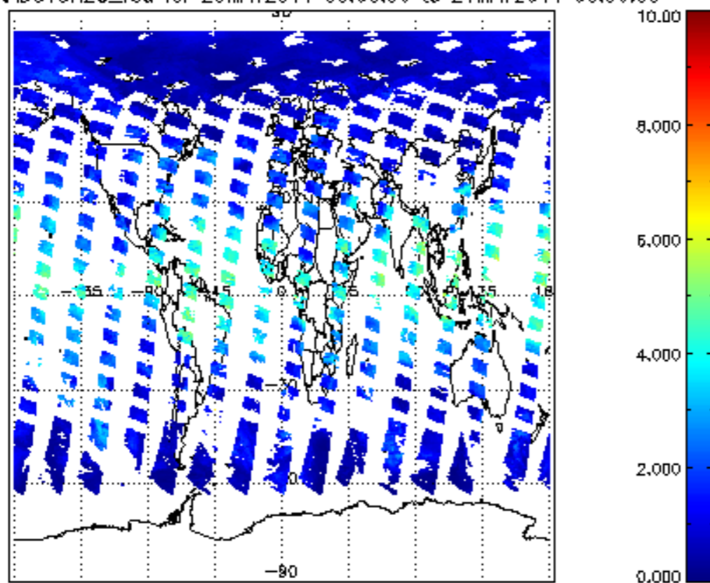
SCIOL2P_NADUV8H2O_vcd for 20MAY2011 00:00:00 to 21MAY2011 00:00:00
