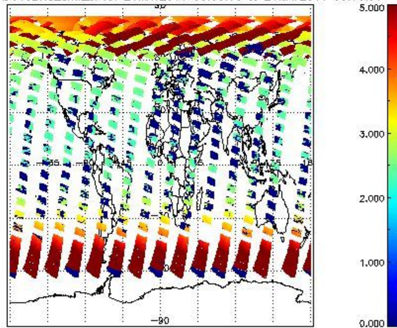
SCIOL2P_NADUV3BRO_amf_cl for 20MAY2011 00:00:00 to 21MAY2011 00:00:00
