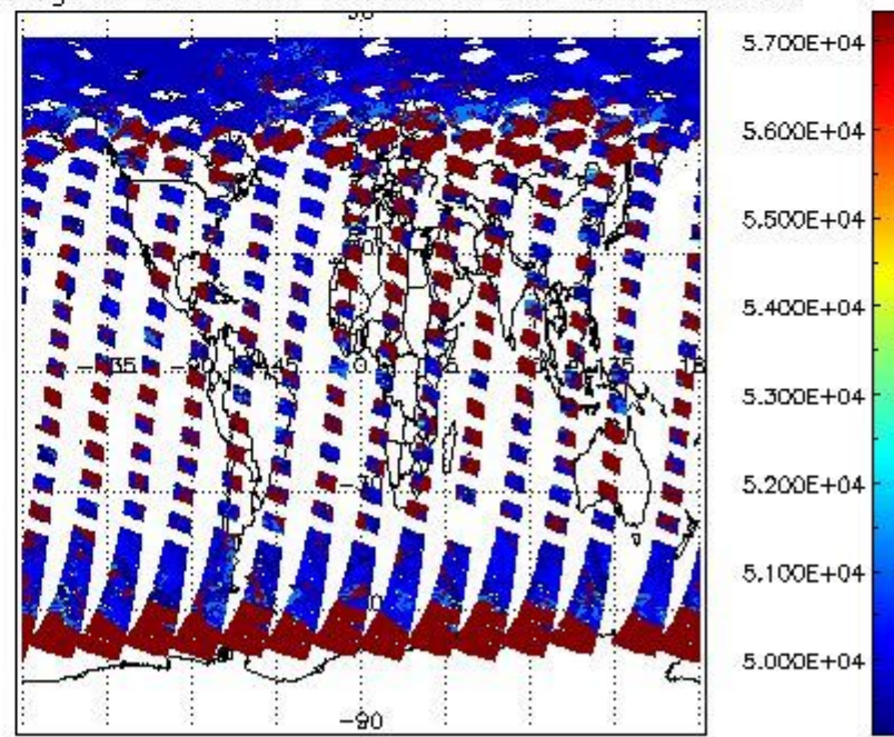
cloud_flags for 20MAY2011 00:00:00 to 21MAY2011 00:00:00
