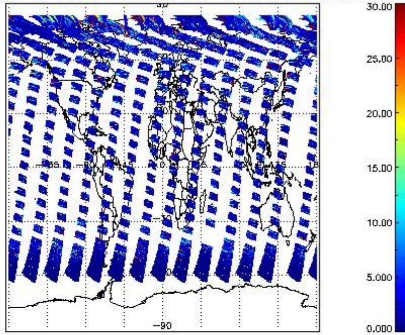
SCIOL2P_NADUV5S02_vcd_err for 20MAY2011 00:00:00 to 21MAY2011 00:00:00
