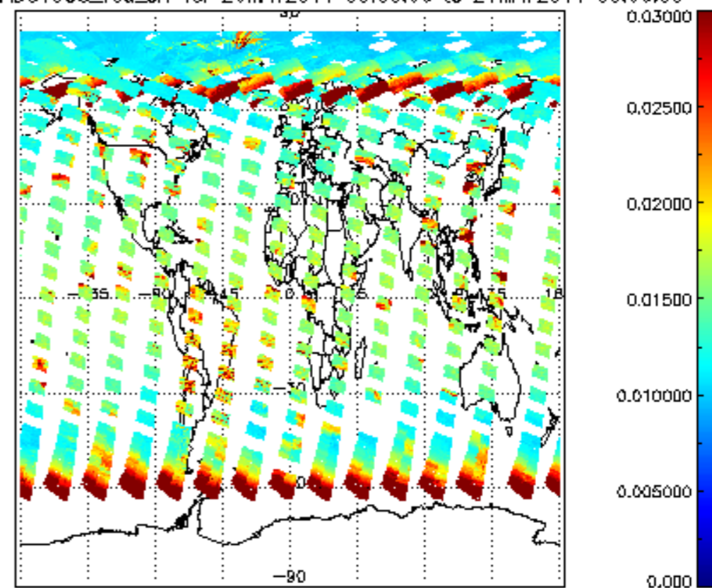
SCIOL2P_NADUV003_vcd_err for 20MAY2011 00:00:00 to 21MAY2011 00:00:00
