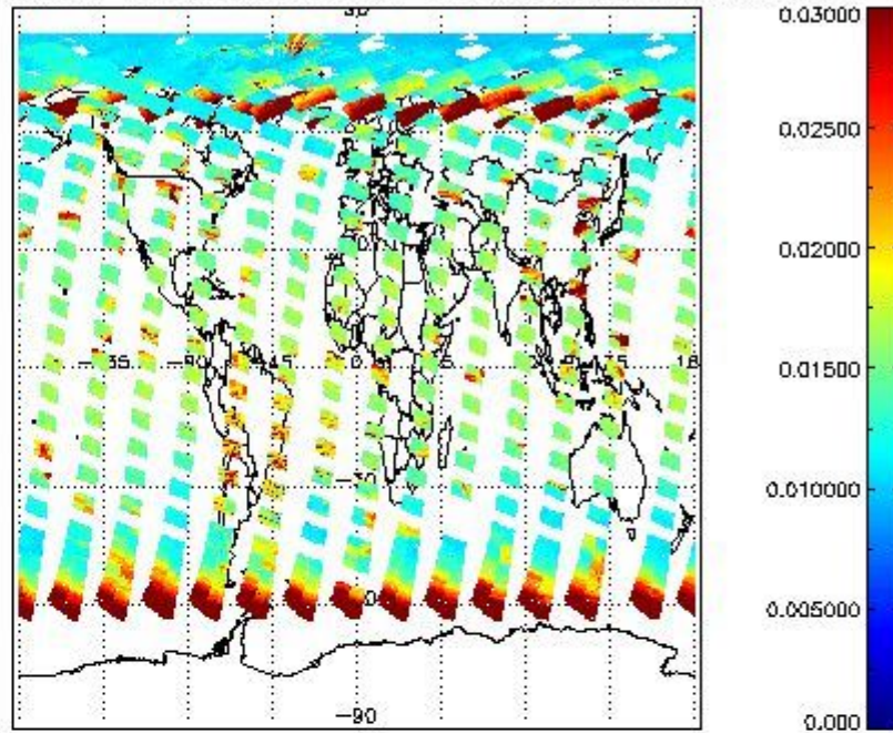
SCIOL2P_NADUV003_vcd_err for 20MAY2011 00:00:00 to 21MAY2011 00:00:00
