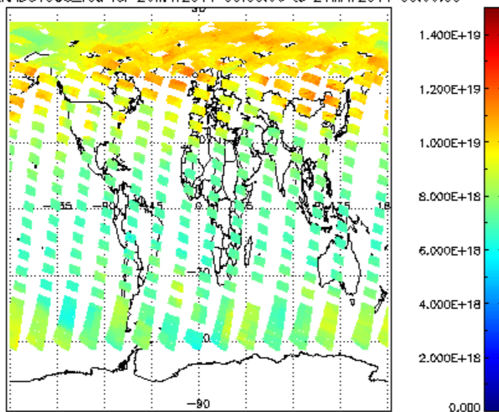
SCIOL2P_NADUV003_vcd for 20MAY2011 00:00:00 to 21MAY2011 00:00:00
