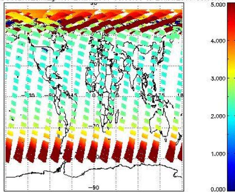
SCIOL2P_NADUV3BRO_amf_gr for 20MAY2011 00:00:00 to 21MAY2011 00:00:00
