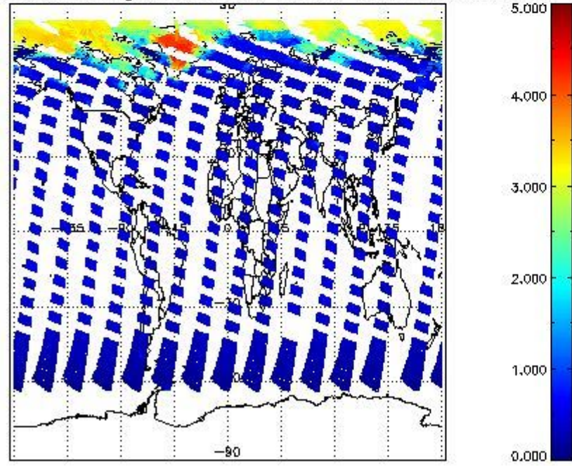
SCIOL2P_NADUV5S02_amf_gr for 20MAY2011 00:00:00 to 21MAY2011 00:00:00
