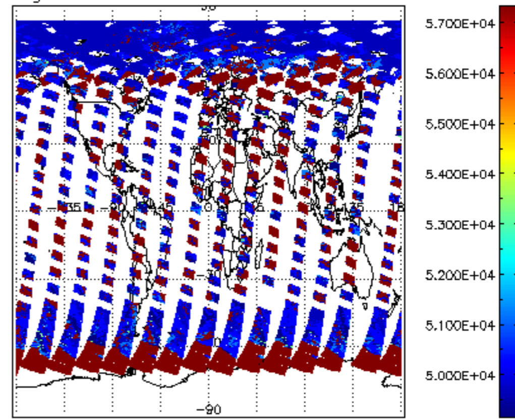
cloud_flags for 20MAY2011 00:00:00 to 21MAY2011 00:00:00
