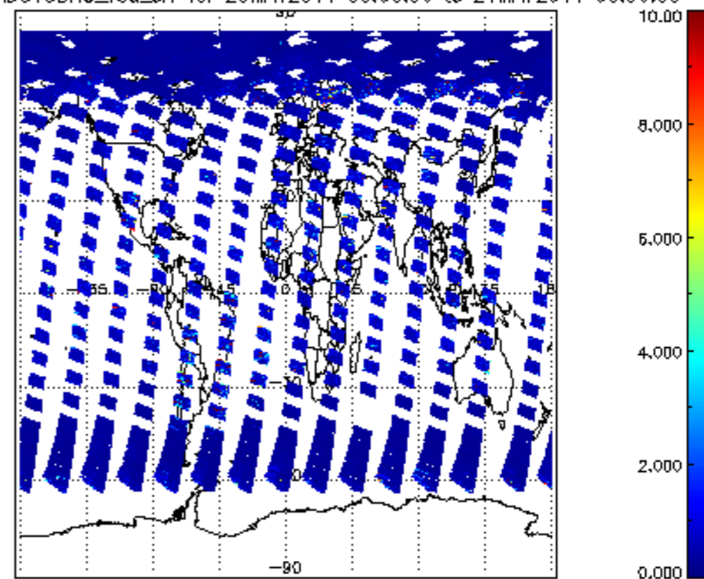
SCIOL2P_NADUV3BRO_vcd_err for 20MAY2011 00:00:00 to 21MAY2011 00:00:00
