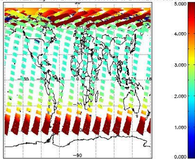
SCIOL2P_NADUV1NO2_amf_gr for 20MAY2011 00:00:00 to 21MAY2011 00:00:00
