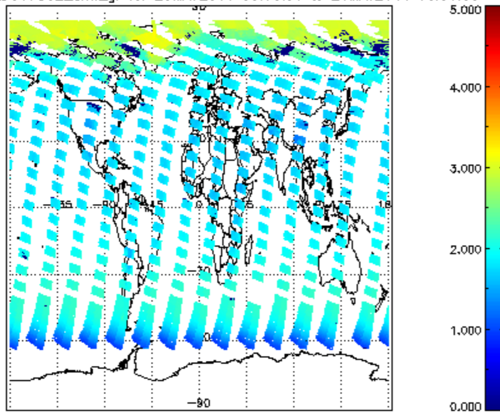
SCIOL2P_NADUV7S02_amf_gr for 20MAY2011 00:00:00 to 21MAY2011 00:00:00
