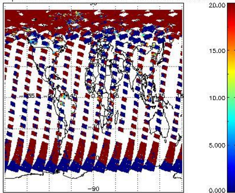
cL_opt_depth for 20MAY2011 00:00:00 to 21MAY2011 00:00:00
