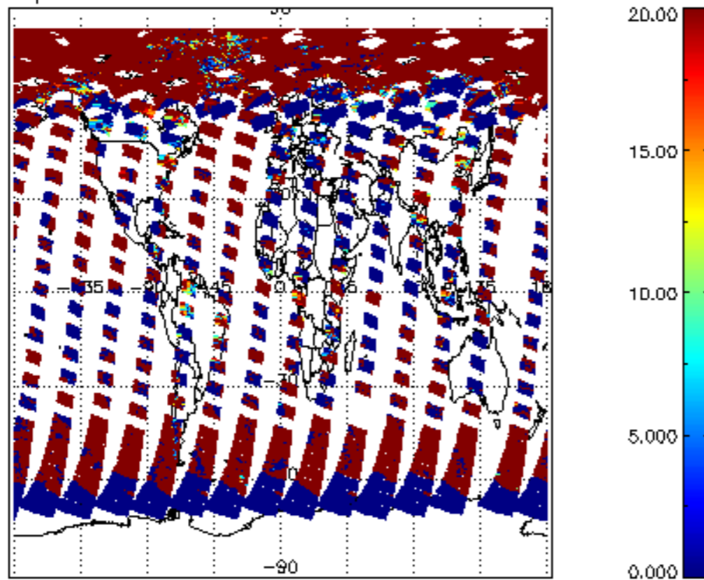
cl_opt_depth for 20MAY2011 00:00:00 to 21MAY2011 00:00:00
