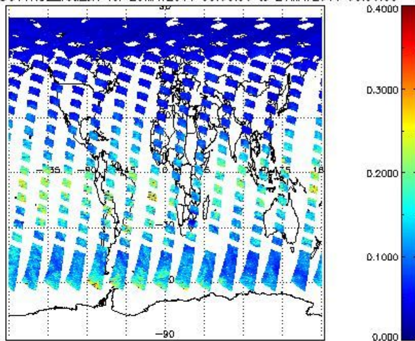
SCIOL2P_NADUV1NO2_vcd_err for 20MAY2011 00:00:00 to 21MAY2011 00:00:00
