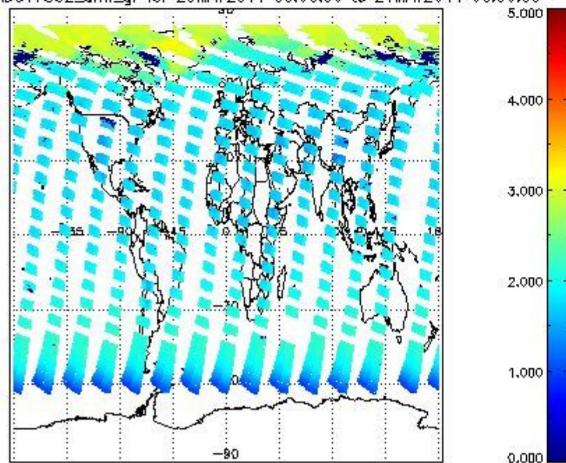
SCIOL2P_NADUV7S02_amf_gr for 20MAY2011 00:00:00 to 21MAY2011 00:00:00
