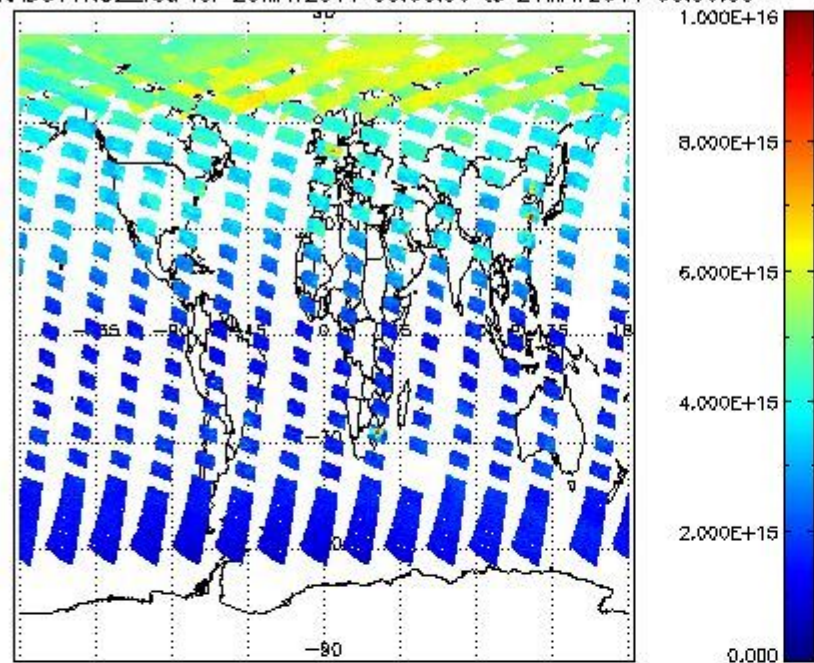
SCIOL2P_NADUV1NO2_vcd for 20MAY2011 00:00:00 to 21MAY2011 00:00:00
