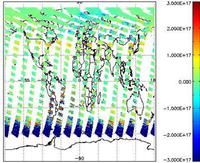
SCIOL2P_NADUV5S02_vcd for 20MAY2011 00:00:00 to 21MAY2011 00:00:00
