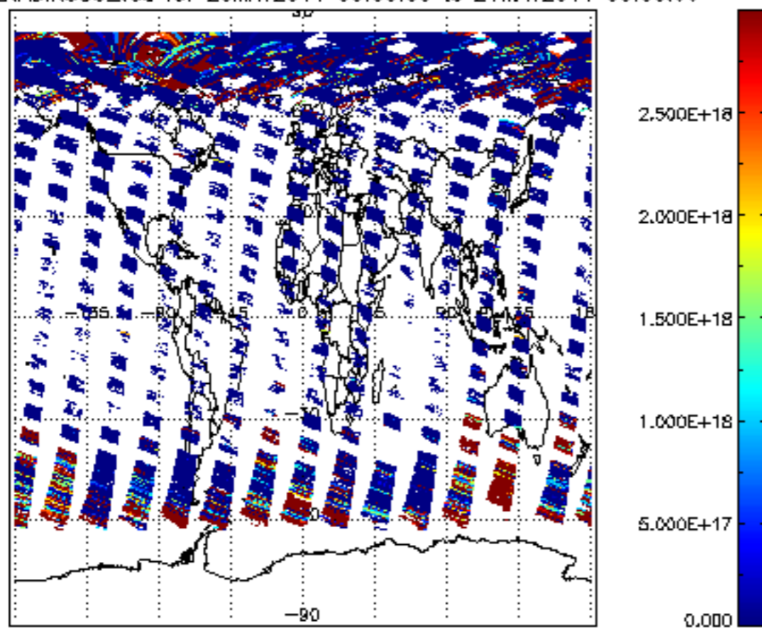
SCIOL2P_NADIR3CO_vcd for 20MAY2011 00:00:00 to 21MAY2011 00:00:00
