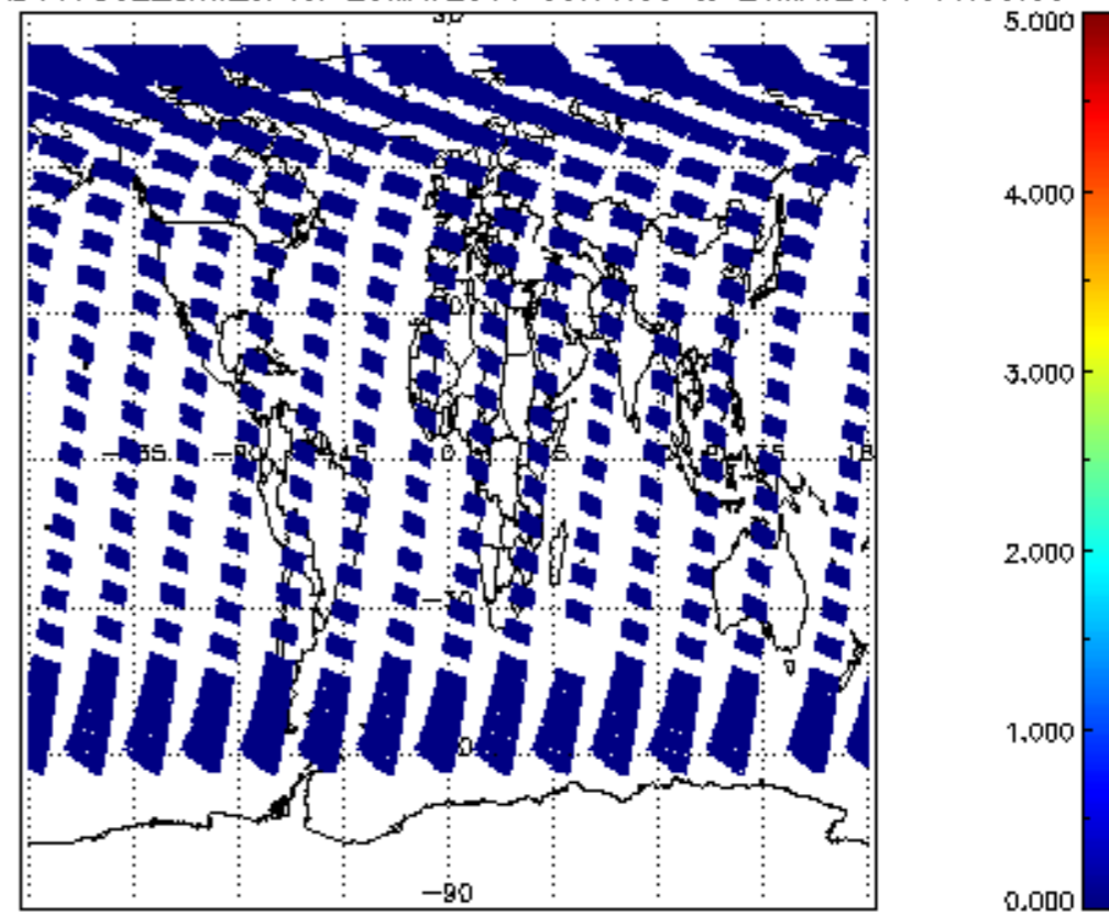
SCIOL2P_NADUV7S02_amf_cl for 20MAY2011 00:00:00 to 21MAY2011 00:00:00
