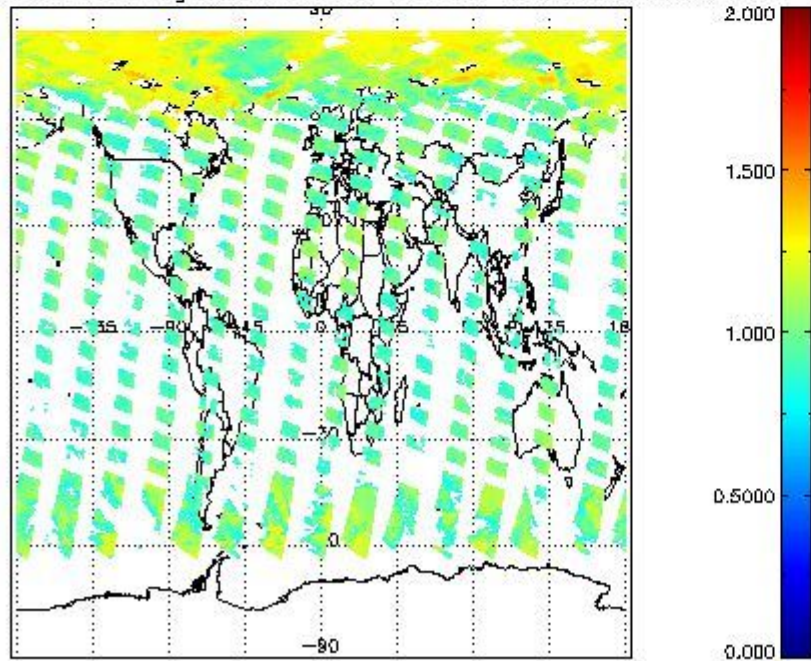
SCIOL2P_NADUV8H2O_arnf_gr for 20MAY2011 00:00:00 to 21MAY2011 00:00:00
