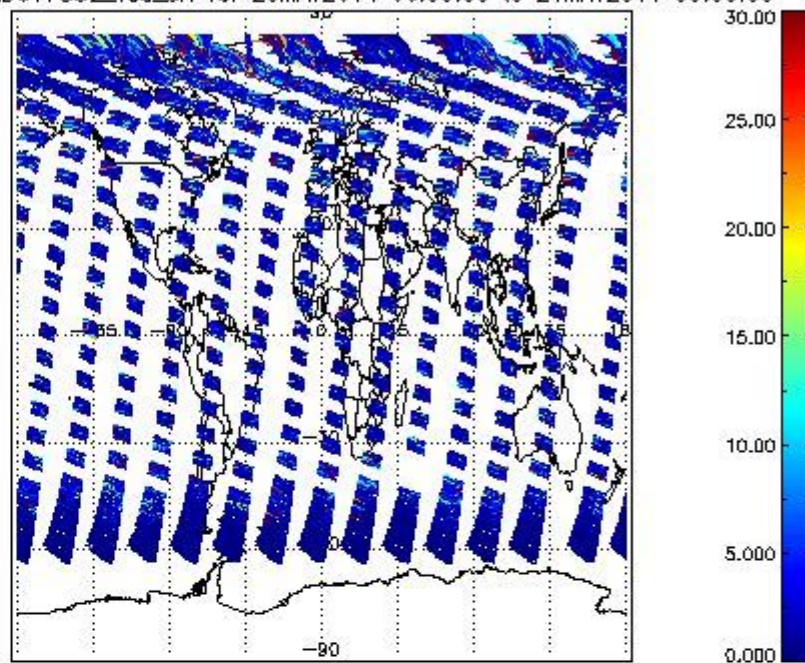
SCIOL2P_NADUV7S02_vcd_err for 20MAY2011 00:00:00 to 21MAY2011 00:00:00
