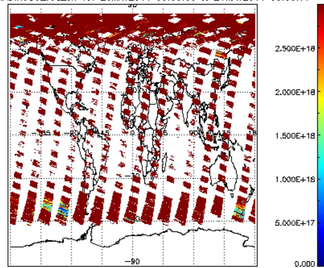
SCIOL2P_NADIR3CO_vcd_err for 20MAY2011 00:00:00 to 21MAY2011 00:00:00
