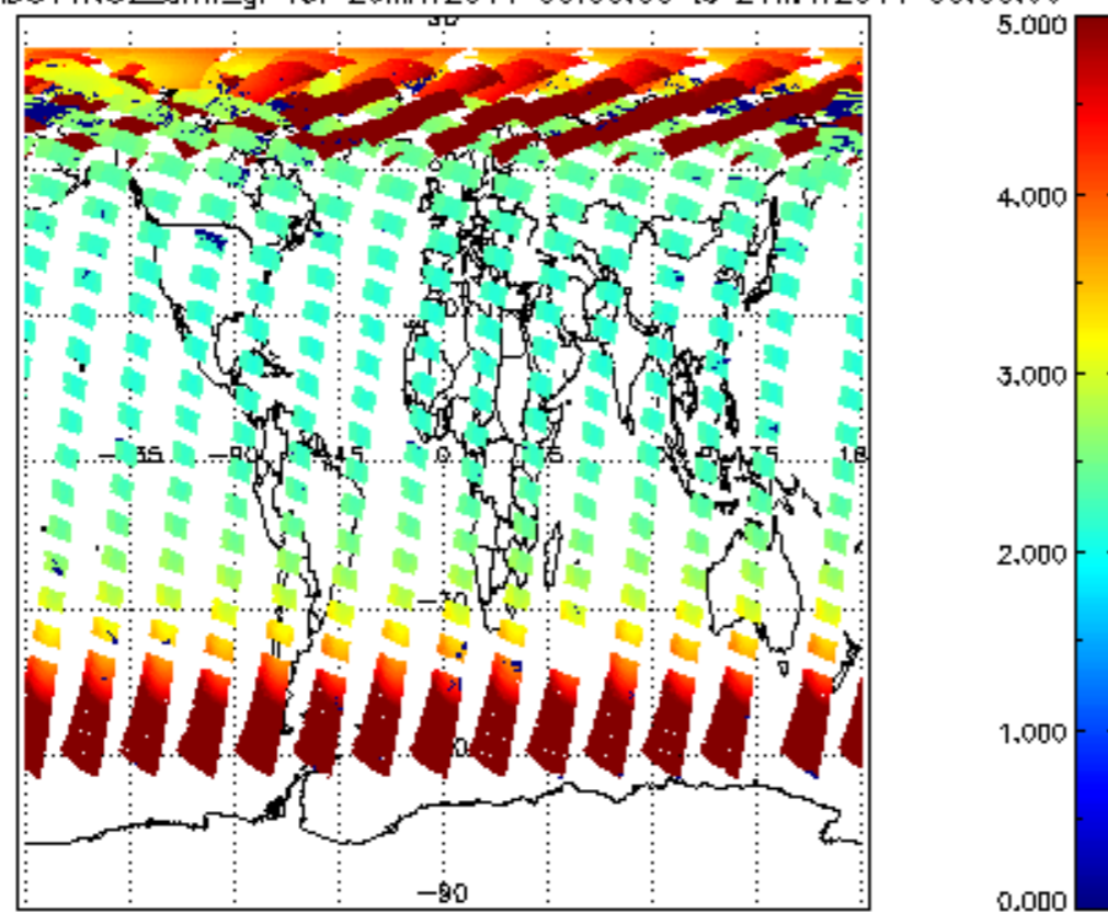
SCIOL2P_NADUV1NO2_amf_gr for 20MAY2011 00:00:00 to 21MAY2011 00:00:00
