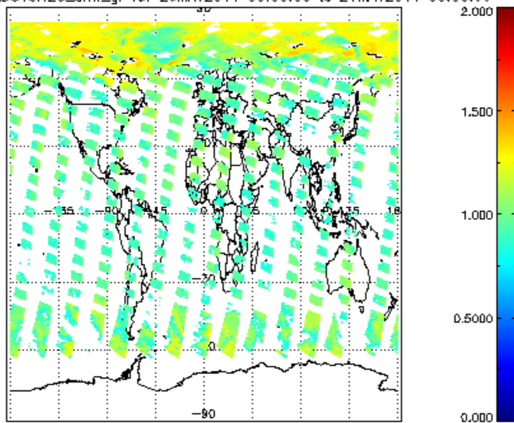
SCIOL2P_NADUV8H2O_amf_gr for 20MAY2011 00:00:00 to 21MAY2011 00:00:00
