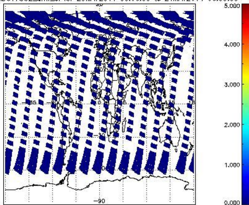
SCIOL2P_NADUV7S02_amf_cl for 20MAY2011 00:00:00 to 21MAY2011 00:00:00
