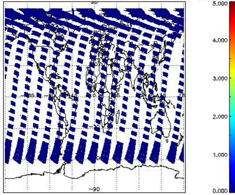
SCIOL2P_NADUV5S02_amf_cl for 20MAY2011 00:00:00 to 21MAY2011 00:00:00
