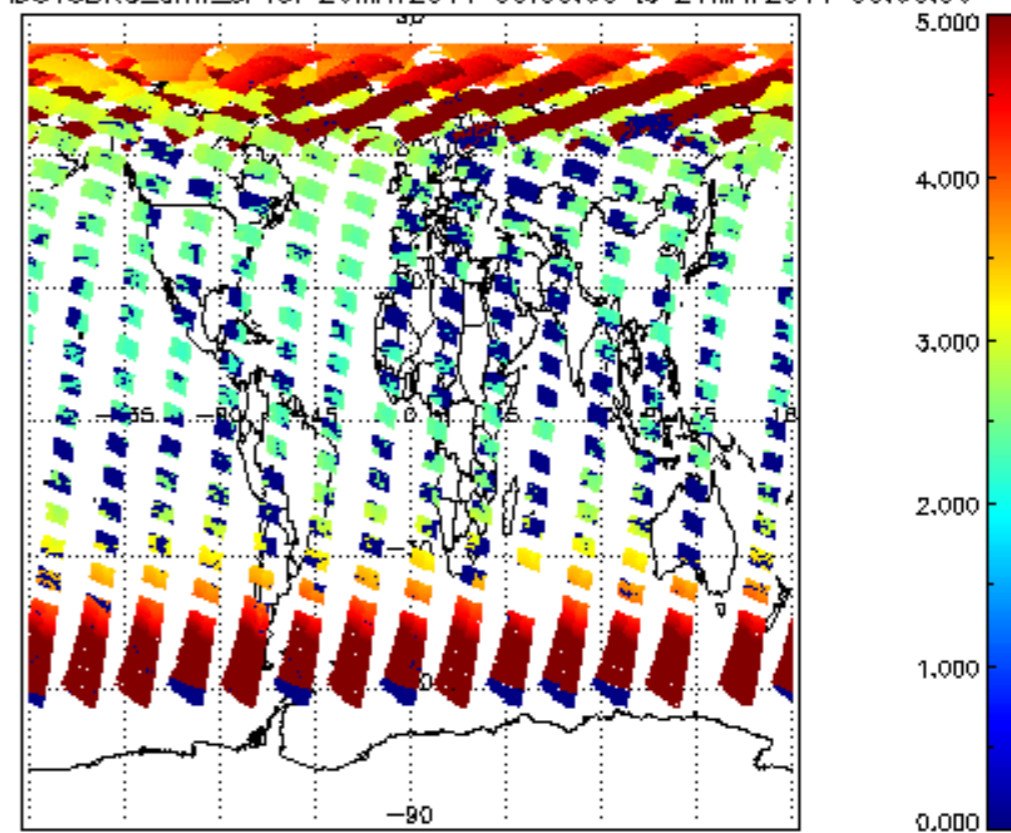
SCIOL2P_NADUV3BRO_amf_sl for 20MAY2011 00:00:00 to 21MAY2011 00:00:00
