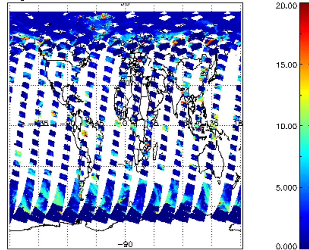
cl_top_height for 20MAY2011 00:00:00 to 21MAY2011 00:00:00
