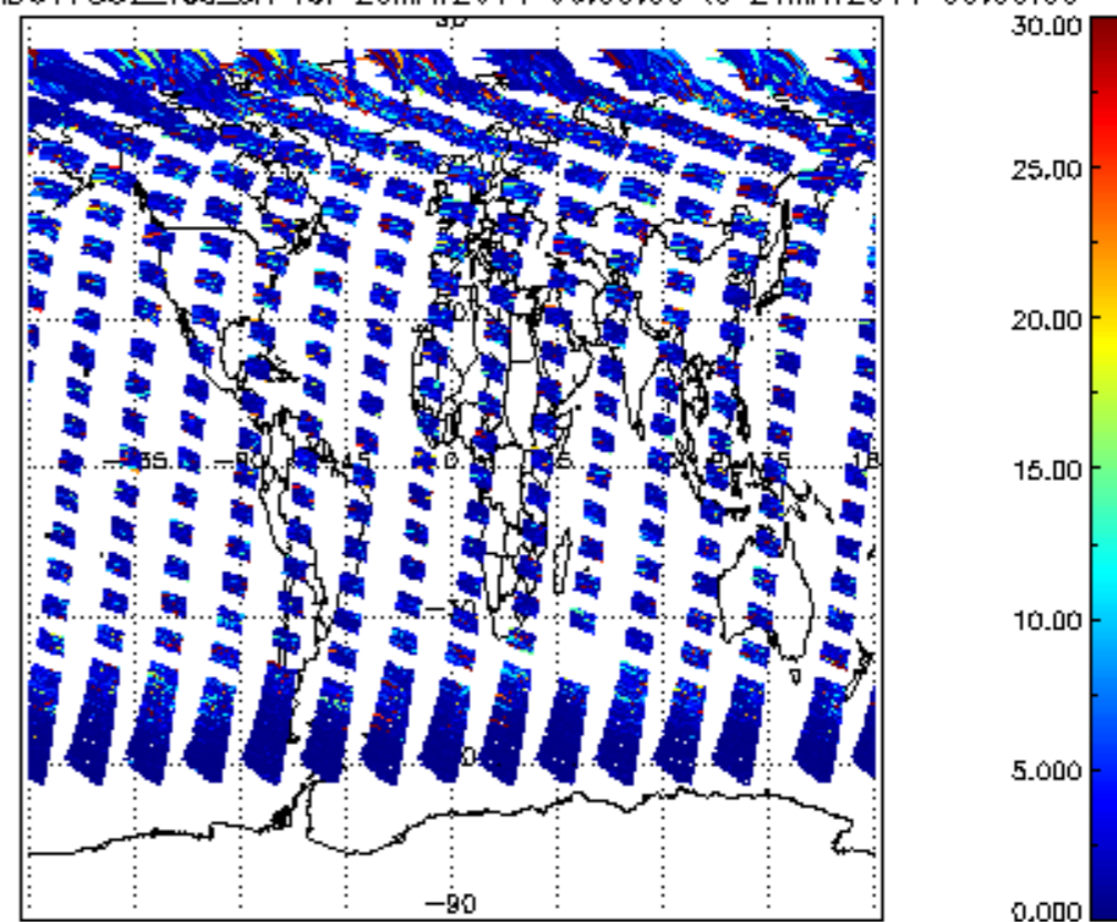
SCIOL2P_NADUV7S02_vcd_err for 20MAY2011 00:00:00 to 21MAY2011 00:00:00
