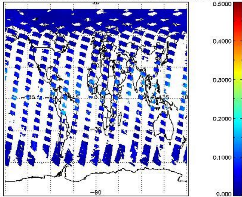
SCIOL2P_NADUV8H2O_vcd_err for 20MAY2011 00:00:00 to 21MAY2011 00:00:00
