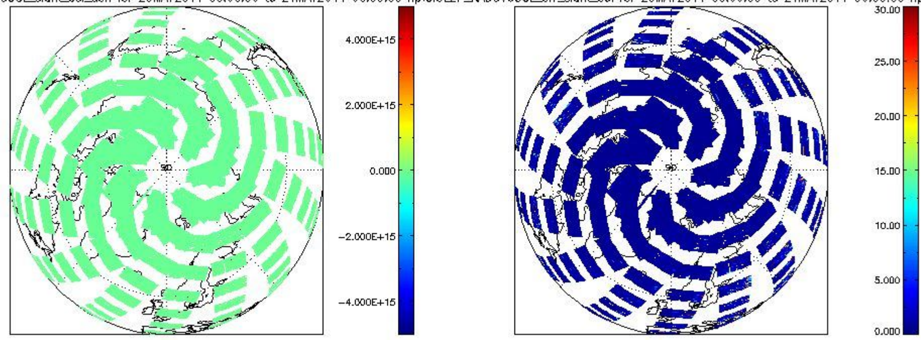
CIOL2P_NADUV60CLslant_col_den for 20MAY2011 00:00:00 to 21MAY2011 00:00:00 np; CIOL2P_NADUV60CLerr_slant_col for 20MAY2011 00:00:00 to 21MAY2011 00:00:00 np
