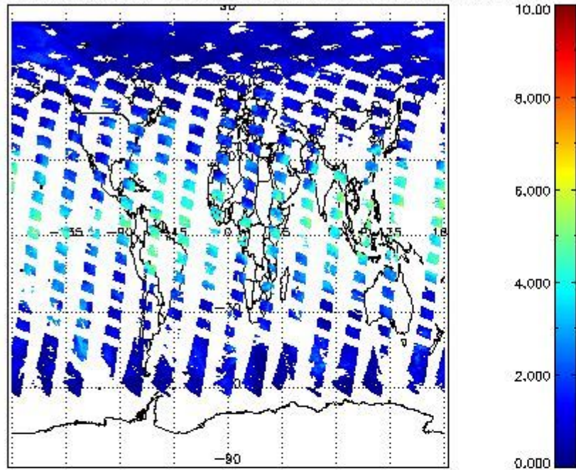
SCIOL2P_NADUV8H2O_vcd for 20MAY2011 00:00:00 to 21MAY2011 00:00:00
