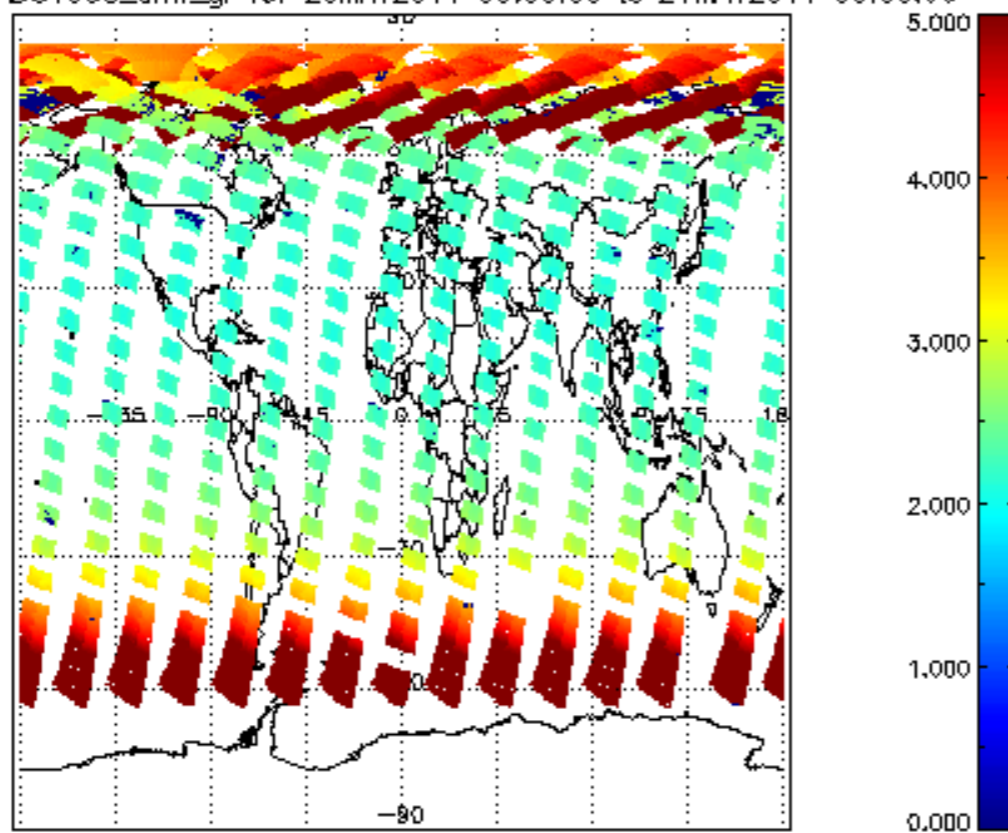
SCIOL2P_NADUV003_amf_gr for 20MAY2011 00:00:00 to 21MAY2011 00:00:00
