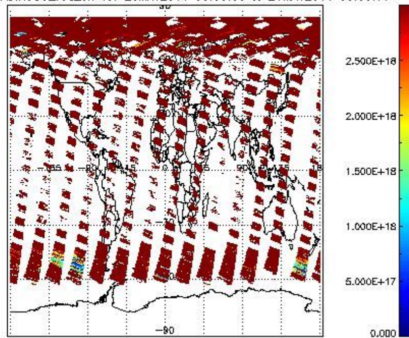
SCIDL2P_NADIR3CO_vcd_err for 20MAY2011 00:00:00 to 21MAY2011 00:00:00
