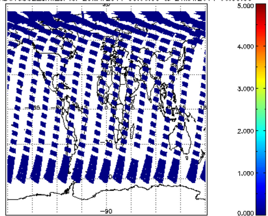
SCIOL2P_NADUV5S02_amf_cl for 20MAY2011 00:00:00 to 21MAY2011 00:00:00
