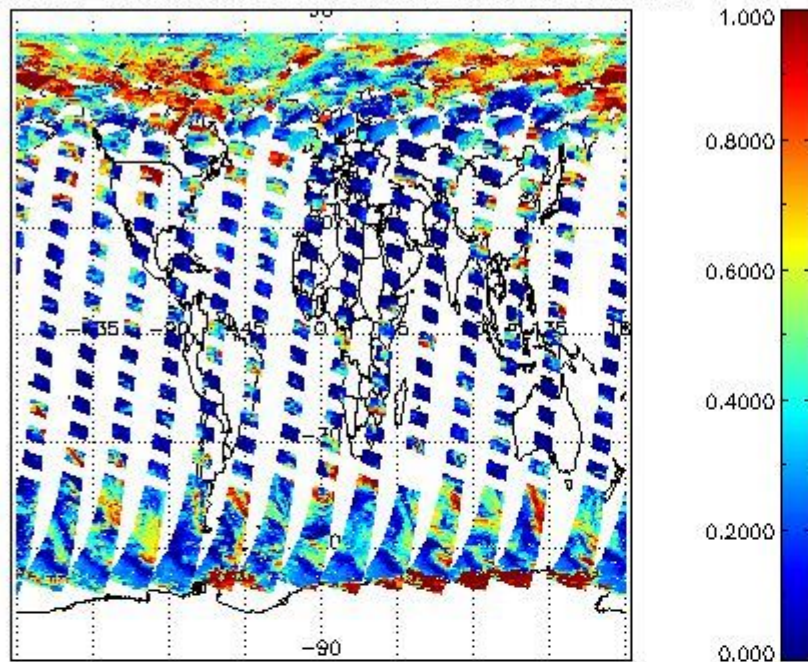
cL_frac for 20MAY2011 00:00:00 to 21MAY2011 00:00:00
