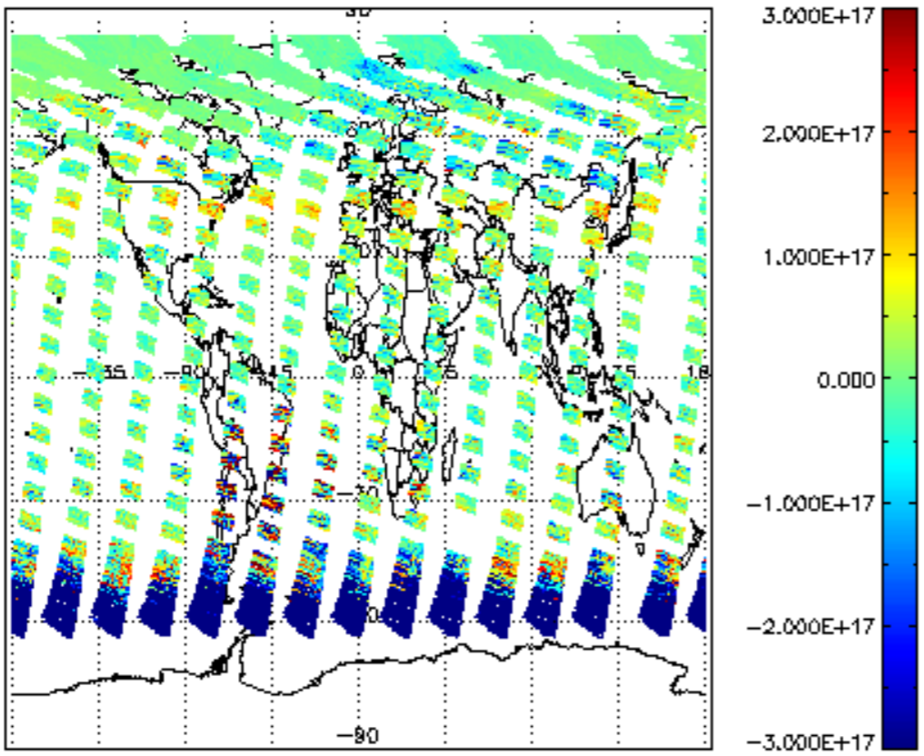
SCIOL2P_NADUV5S02_vcd for 20MAY2011 00:00:00 to 21MAY2011 00:00:00
