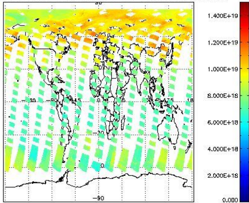
SCIOL2P_NADUV003_vcd for 20MAY2011 00:00:00 to 21MAY2011 00:00:00
