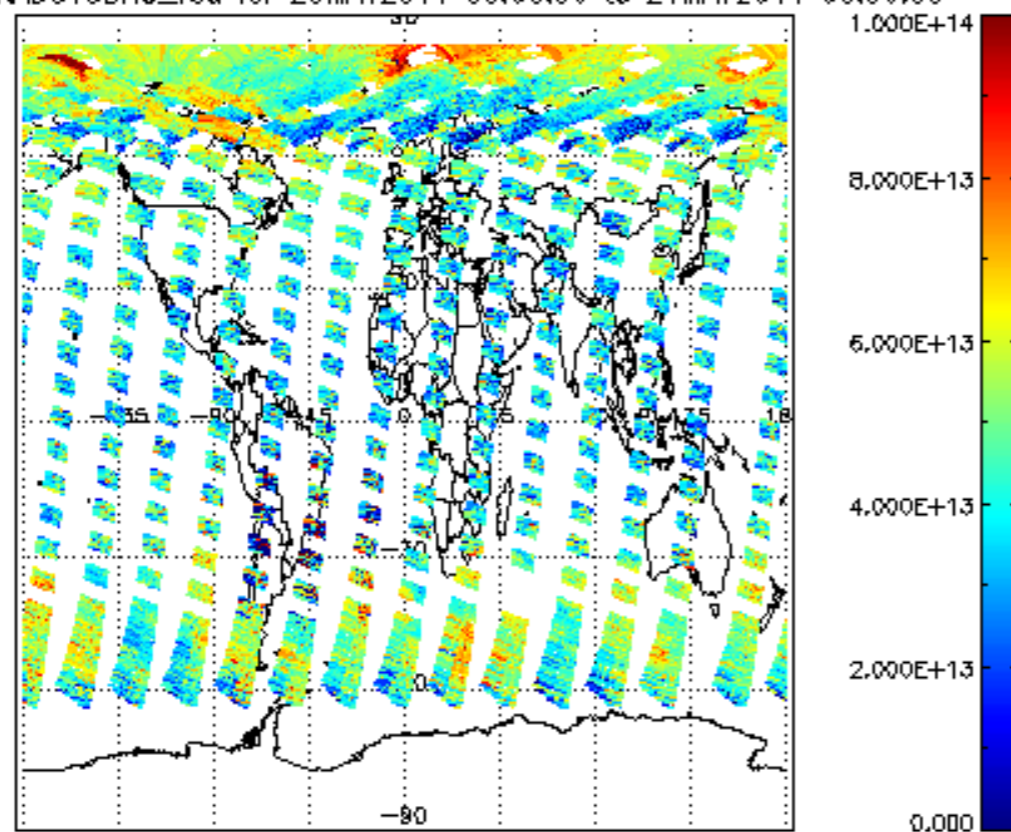
SCIOL2P_NADUV3BRO_vcd for 20MAY2011 00:00:00 to 21MAY2011 00:00:00
