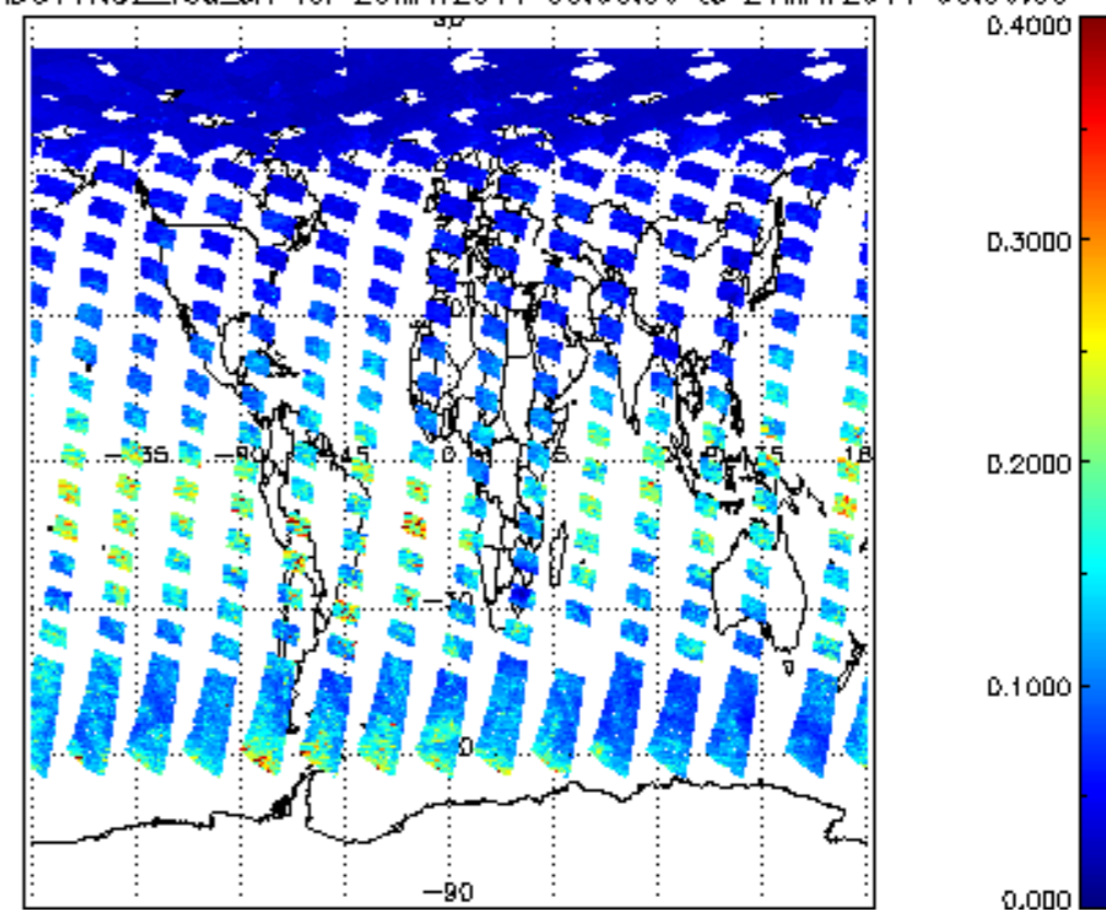
SCIOL2P_NADUV1NO2_vcd_err for 20MAY2011 00:00:00 to 21MAY2011 00:00:00
