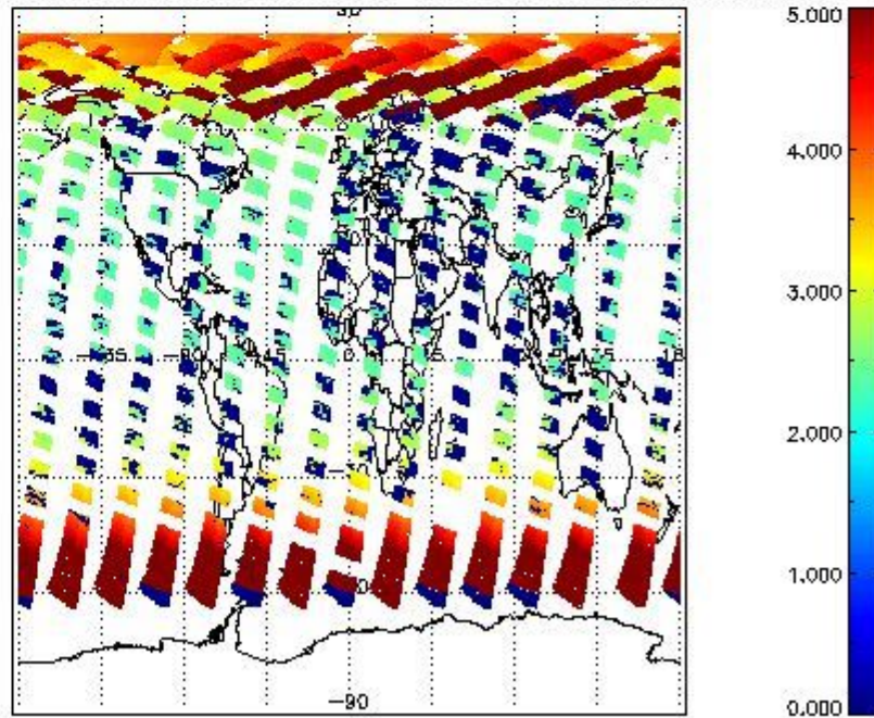
SCIOL2P_NADUV003_amf_cl for 20MAY2011 00:00:00 to 21MAY2011 00:00:00
