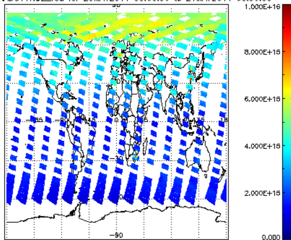
SCIOL2P_NADUV1NO2_vcd for 20MAY2011 00:00:00 to 21MAY2011 00:00:00
