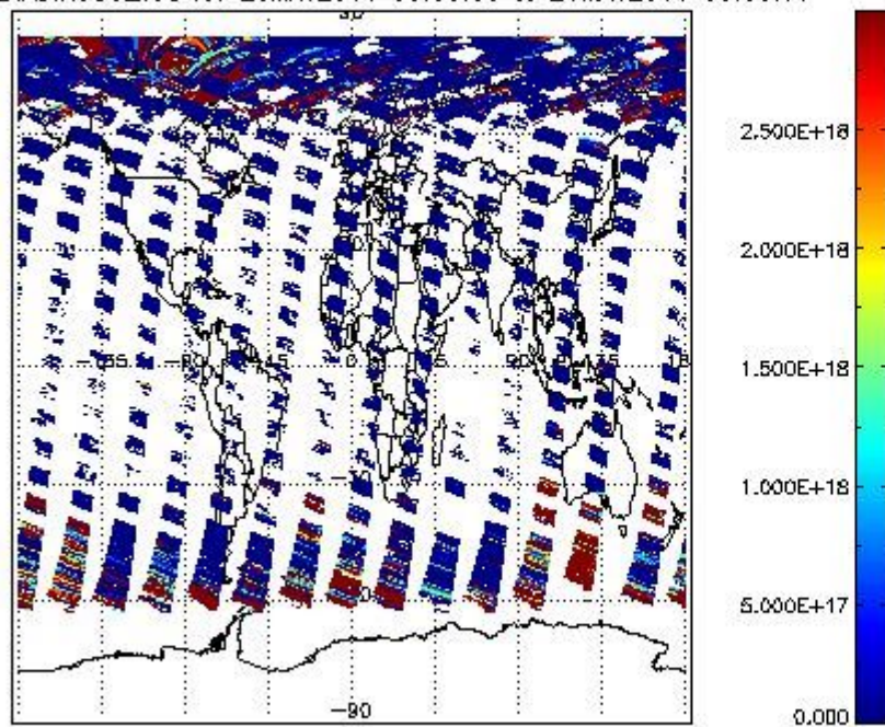
SCIDL2P_NADIR3CO_vcd for 20MAY2011 00:00:00 to 21MAY2011 00:00:00
