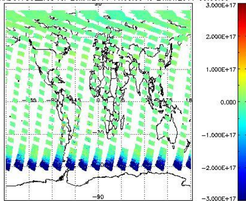
SCIOL2P_NADUV7S02_vcd for 20MAY2011 00:00:00 to 21MAY2011 00:00:00
