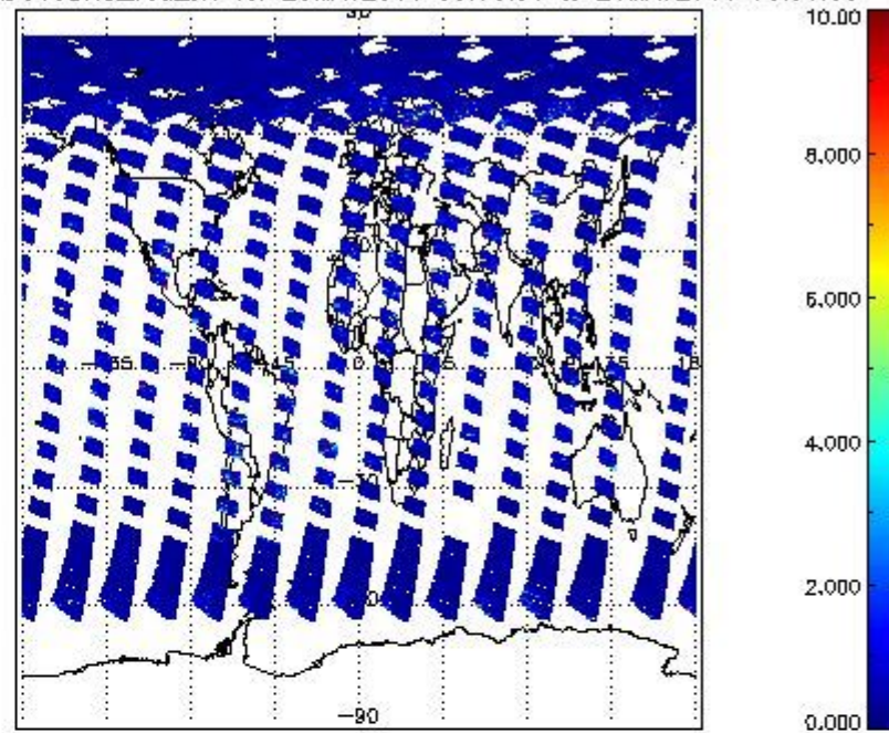
SCIOL2P_NADUV3BRO_vcd_err for 20MAY2011 00:00:00 to 21MAY2011 00:00:00
