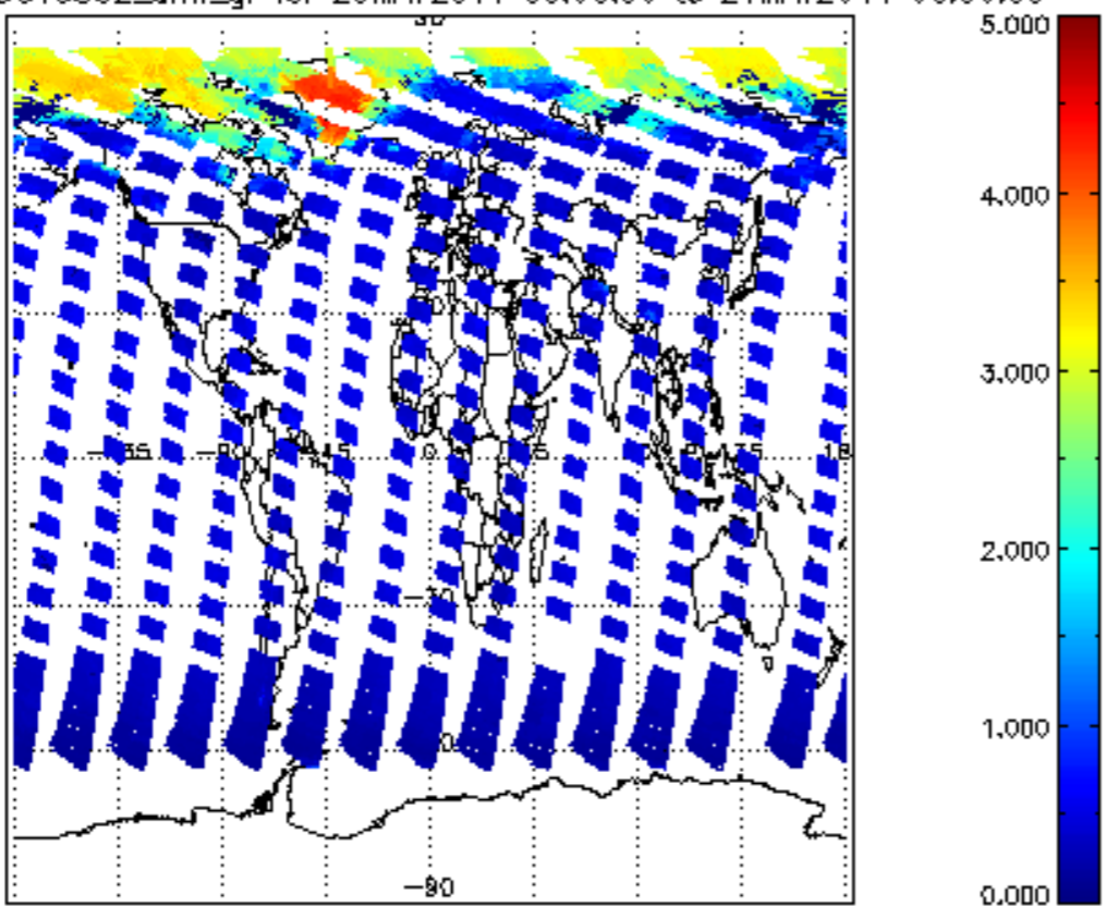
SCIOL2P_NADUV5S02_amf_gr for 20MAY2011 00:00:00 to 21MAY2011 00:00:00
