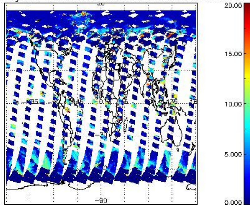
cL_top_height for 20MAY2011 00:00:00 to 21MAY2011 00:00:00
