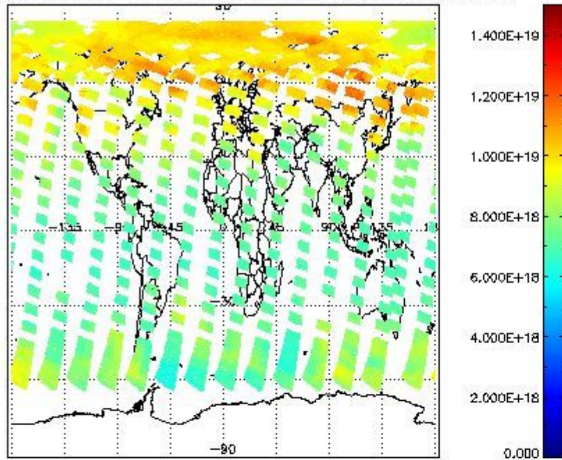
SCIOL2P_NADUV003_vcd for 18MAY2011 00:00:00 to 19MAY2011 00:00:00
