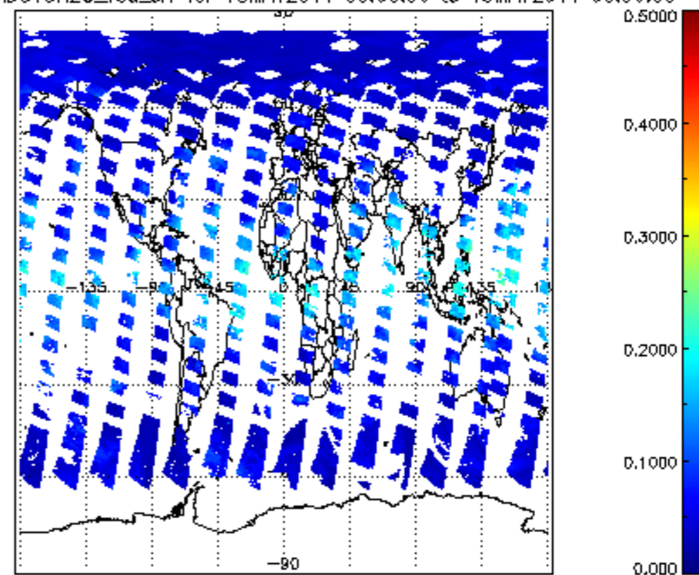
SCIOL2P_NADUV8H2O_vcd_err for 18MAY2011 00:00:00 to 19MAY2011 00:00:00
