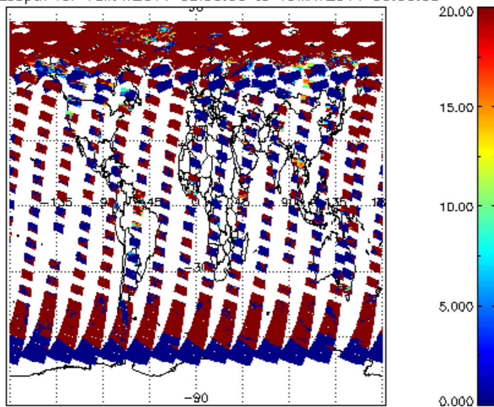
cL_opt_depth for 18MAY2011 00:00:00 to 19MAY2011 00:00:00
