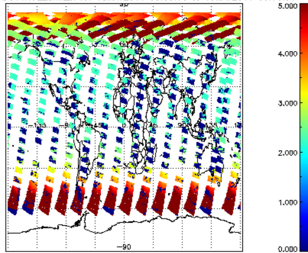
SCIOL2P_NADUV1NO2_amf_sl for 18MAY2011 00:00:00 to 19MAY2011 00:00:00
