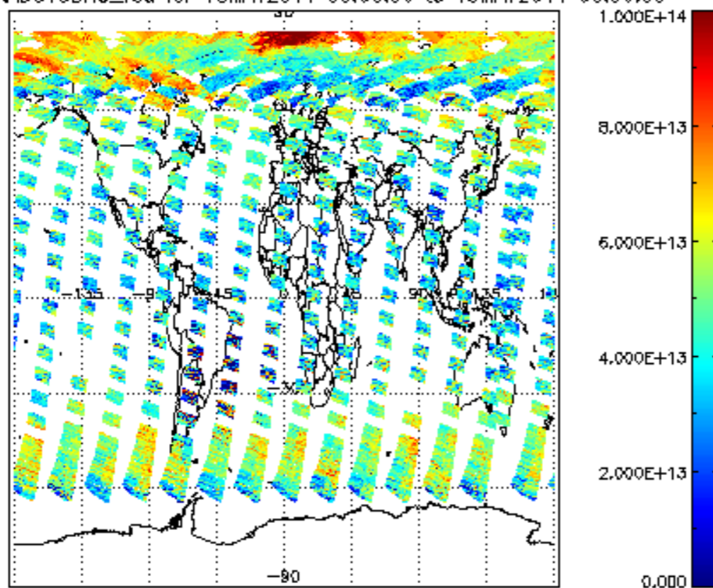
SCIOL2P_NADUV3BRO_vcd for 18MAY2011 00:00:00 to 19MAY2011 00:00:00
