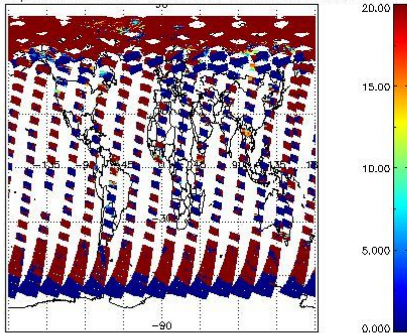
cL_opt_depth for 18MAY2011 00:00:00 to 19MAY2011 00:00:00
