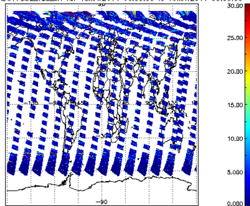
SCIOL2P_NADUV7S02_vcd_err for 18MAY2011 00:00:00 to 19MAY2011 00:00:00
