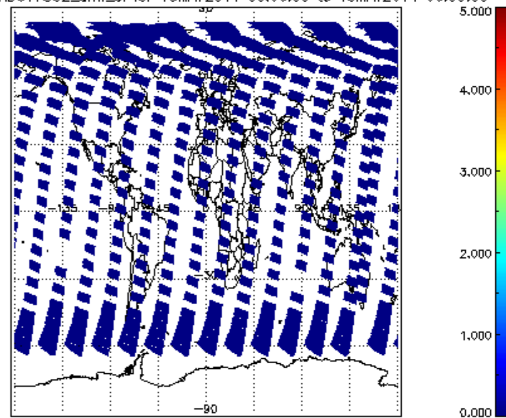
SCIOL2P_NADUV7S02_amf_cl for 18MAY2011 00:00:00 to 19MAY2011 00:00:00
