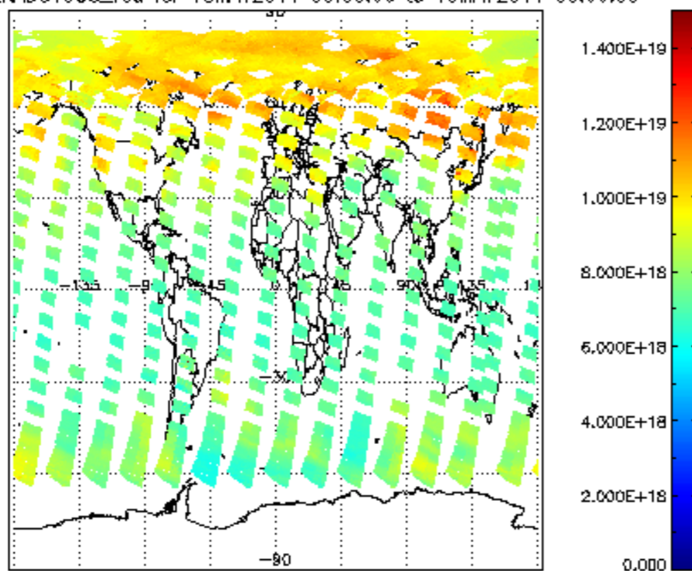
SCIOL2P_NADUV003_vcd for 18MAY2011 00:00:00 to 19MAY2011 00:00:00
