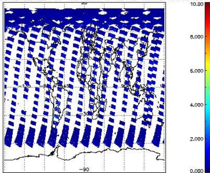
SCIOL2P_NADUV3BRO_vcd_err for 18MAY2011 00:00:00 to 19MAY2011 00:00:00
