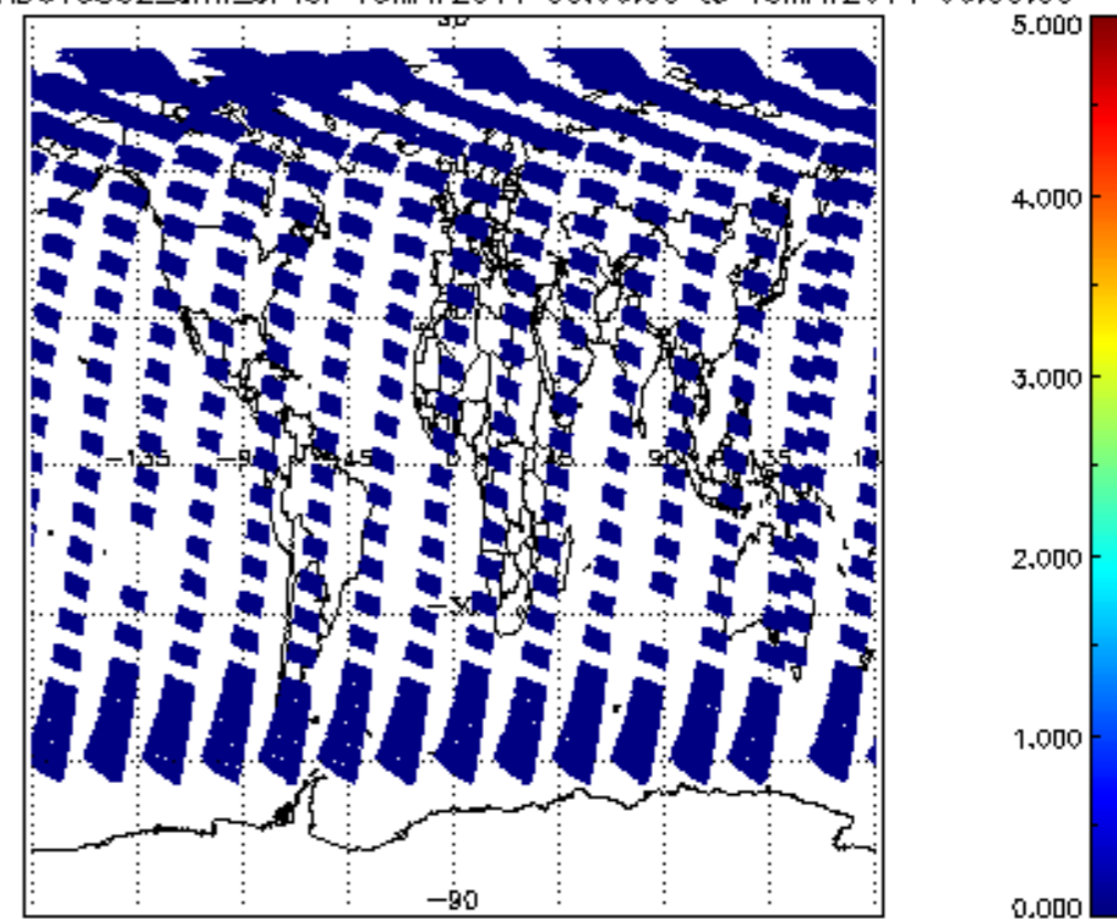
SCIOL2P_NADUV5S02_amf_cl for 18MAY2011 00:00:00 to 19MAY2011 00:00:00
