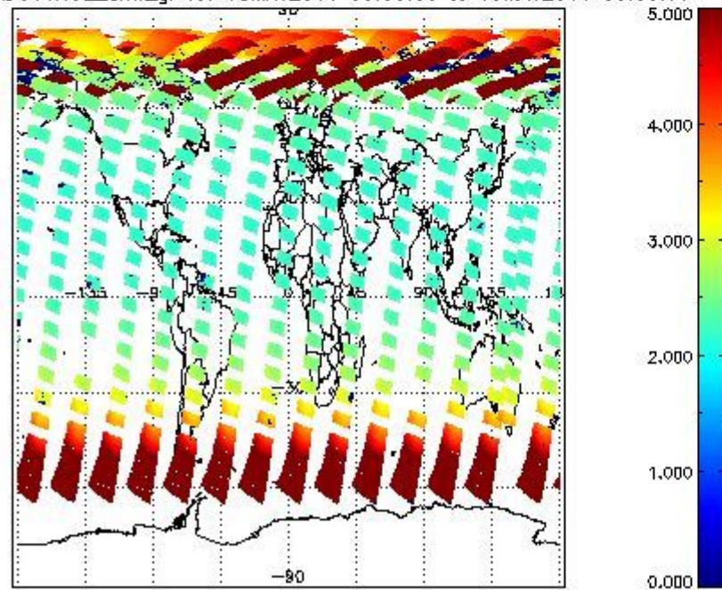
SCIOL2P_NADUV1NO2_amf_gr for 18MAY2011 00:00:00 to 19MAY2011 00:00:00
