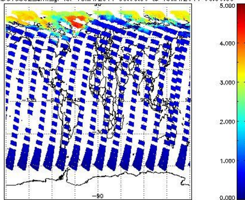
SCIOL2P_NADUV5S02_amf_gr for 18MAY2011 00:00:00 to 19MAY2011 00:00:00
