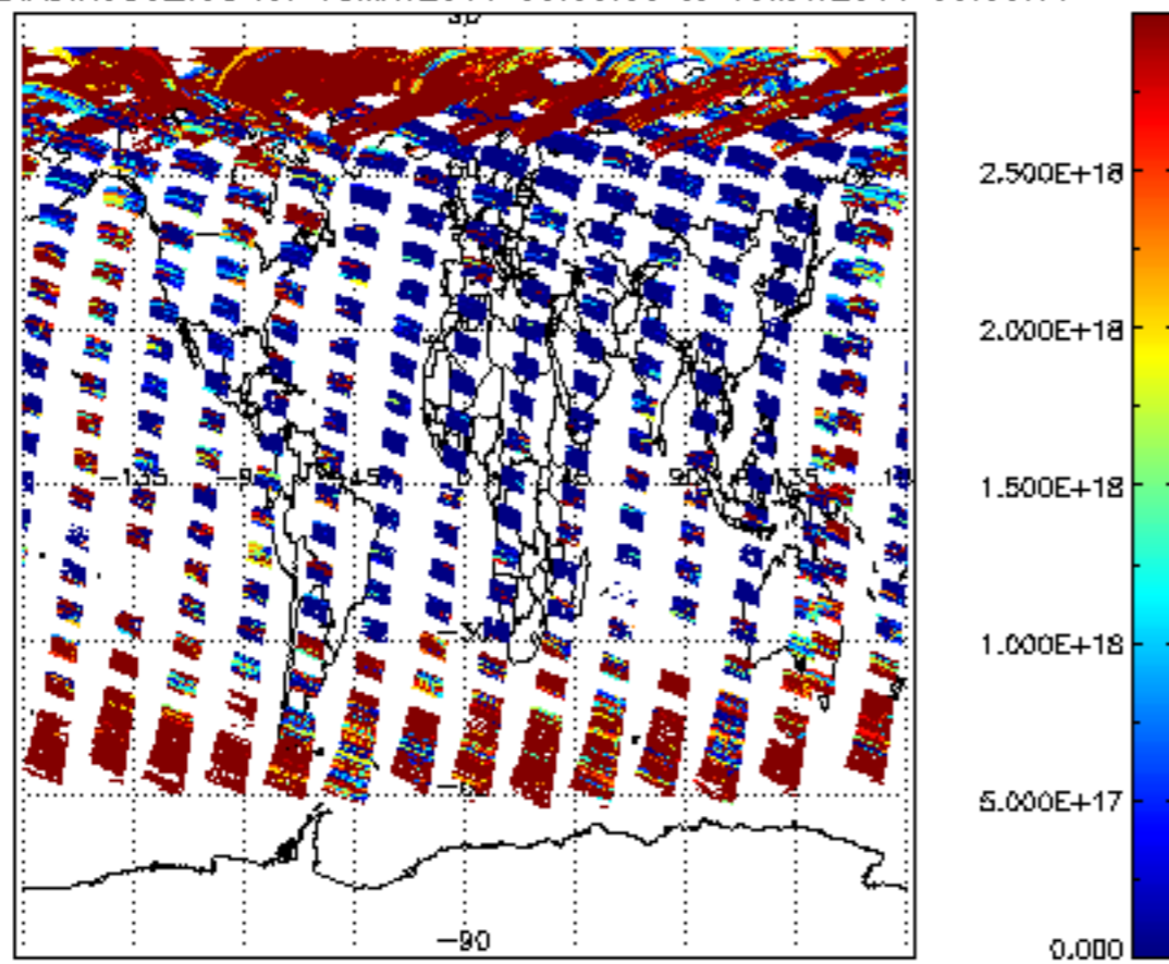
SCIOL2P_NADIR3CO_vcd for 18MAY2011 00:00:00 to 19MAY2011 00:00:00
