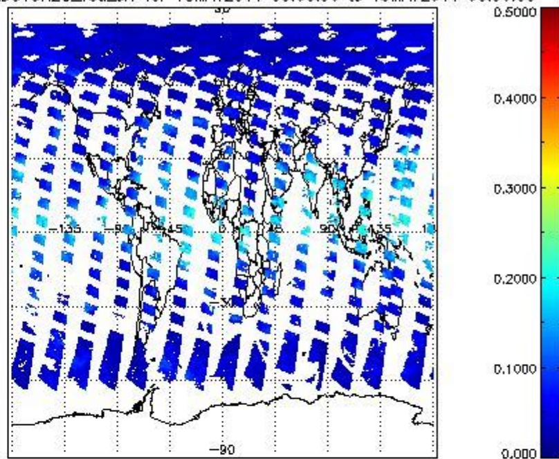
SCIOL2P_NADUV8H2O_vcd_err for 18MAY2011 00:00:00 to 19MAY2011 00:00:00
