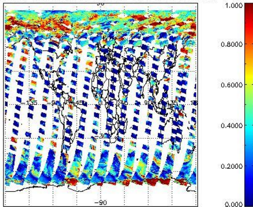
cL_frac for 18MAY2011 00:00:00 to 19MAY2011 00:00:00
