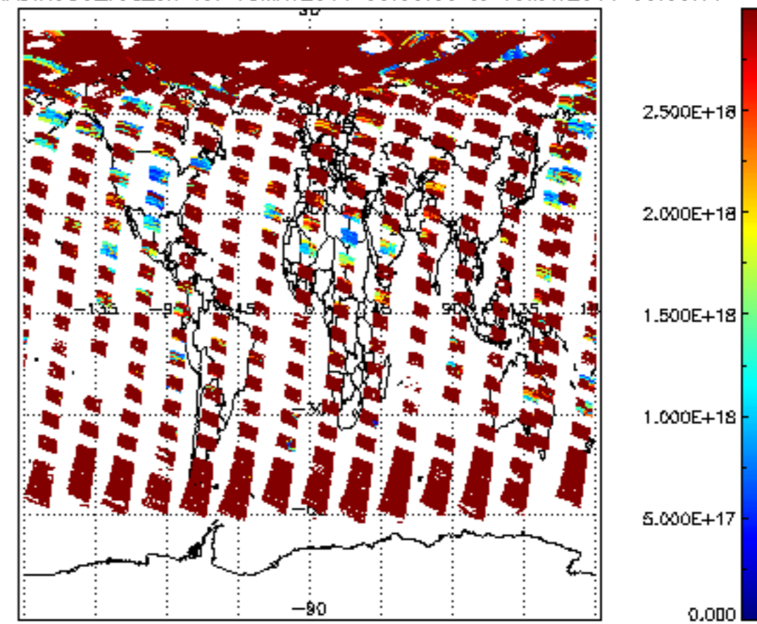
SCIOL2P_NADIR3CO_vcd_err for 18MAY2011 00:00:00 to 19MAY2011 00:00:00
