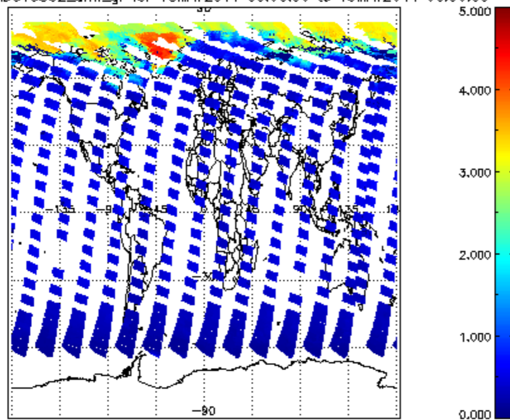
SCIOL2P_NADUV5S02_amf_gr for 18MAY2011 00:00:00 to 19MAY2011 00:00:00
