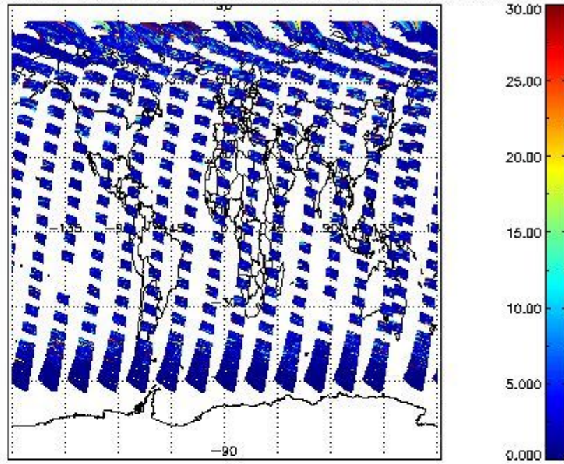
SCIOL2P_NADUV7S02_vcd_err for 18MAY2011 00:00:00 to 19MAY2011 00:00:00
