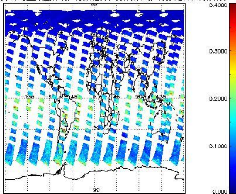
SCIOL2P_NADUV1NO2_vcd_err for 18MAY2011 00:00:00 to 19MAY2011 00:00:00
