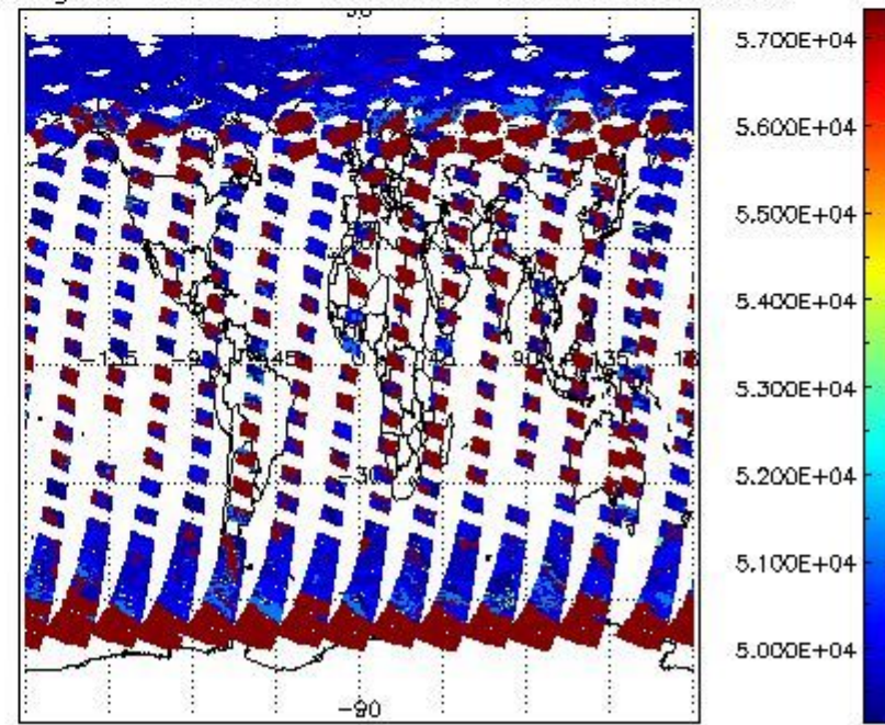
cloud_flags for 18MAY2011 00:00:00 to 19MAY2011 00:00:00
