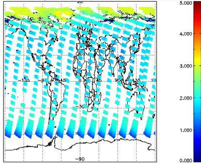
SCIOL2P_NADUV7S02_amf_gr for 18MAY2011 00:00:00 to 19MAY2011 00:00:00
