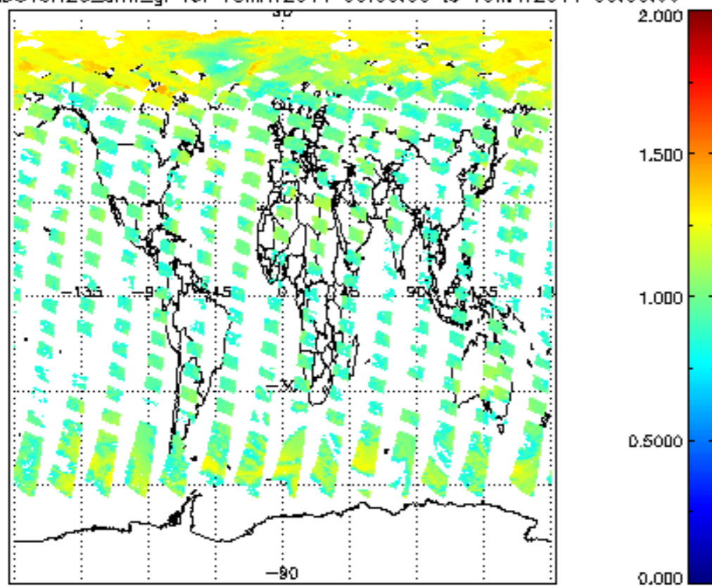
SCIOL2P_NADUV8H2O_amf_gr for 18MAY2011 00:00:00 to 19MAY2011 00:00:00
