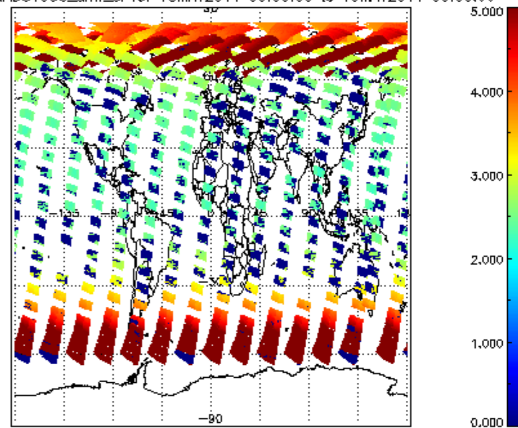
SCIOL2P_NADUV003_amf_cl for 18MAY2011 00:00:00 to 19MAY2011 00:00:00
