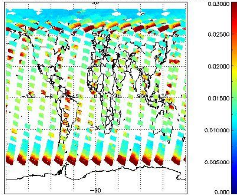
SCIOL2P_NADUV003_vcd_err for 18MAY2011 00:00:00 to 19MAY2011 00:00:00
