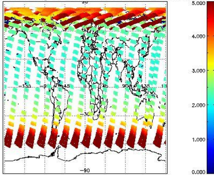
SCIOL2P_NADUV003_amf_gr for 18MAY2011 00:00:00 to 19MAY2011 00:00:00
