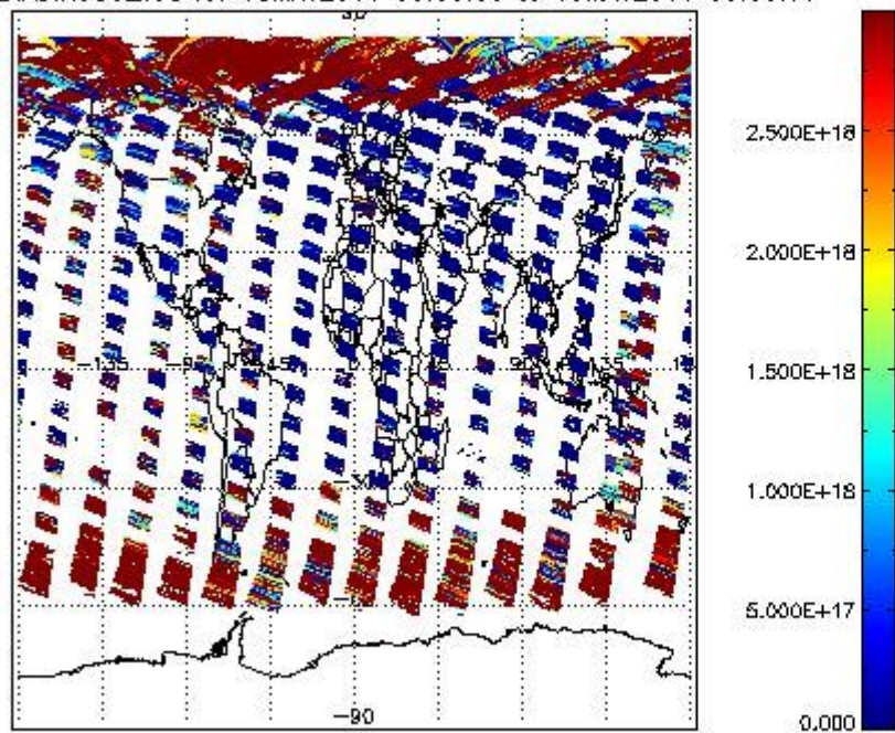
SCIO2P_NADIR3CO_vcd for 18MAY2011 00:00:00 to 19MAY2011 00:00:00
