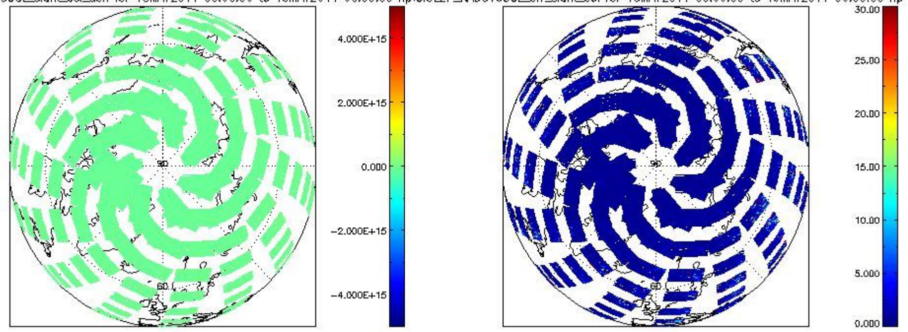
CIOL2P_NADUV6OCLslant_col_den for 18MAY2011 00:00:00 to 19MAY2011 00:00:00 np; CIOL2P_NADUV6OCLarr_slant_col for 18MAY2011 00:00:00 to 19MAY2011 00:00:00 np
