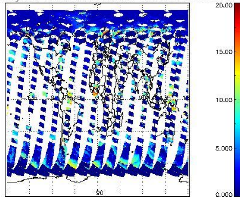
cL_top_height for 18MAY2011 00:00:00 to 19MAY2011 00:00:00
