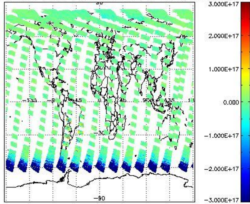
SCIOL2P_NADUV7S02_vcd for 18MAY2011 00:00:00 to 19MAY2011 00:00:00
