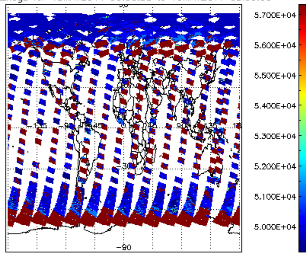
cloud_flags for 18MAY2011 00:00:00 to 19MAY2011 00:00:00
