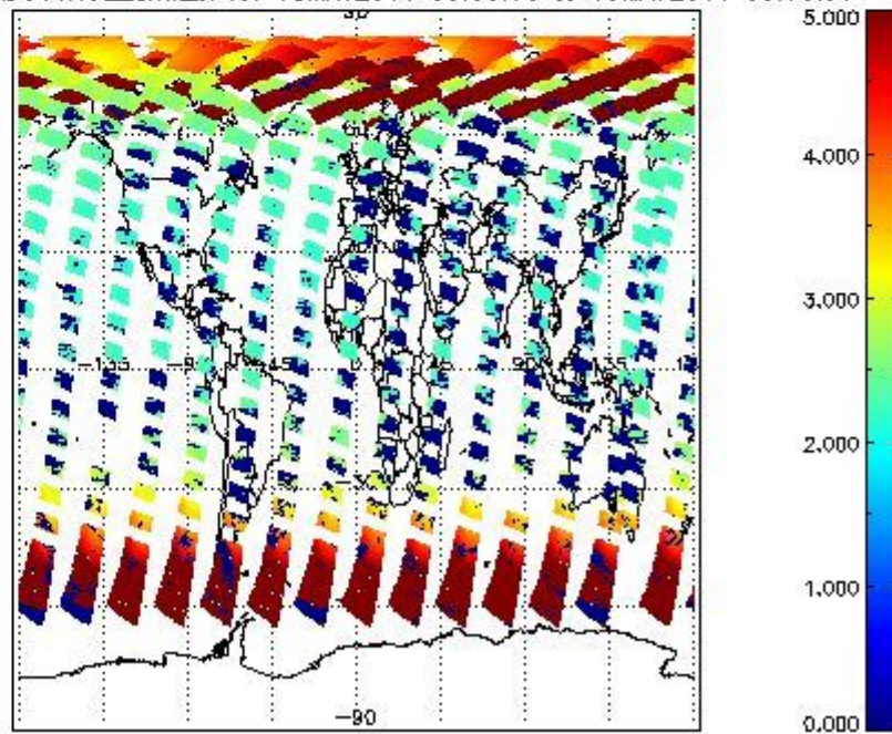
SCIOL2P_NADUV1NO2_amf_cl for 18MAY2011 00:00:00 to 19MAY2011 00:00:00
