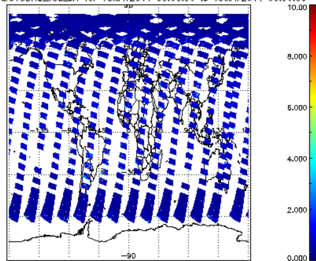
SCIOL2P_NADUV3BRO_vcd_err for 18MAY2011 00:00:00 to 19MAY2011 00:00:00
