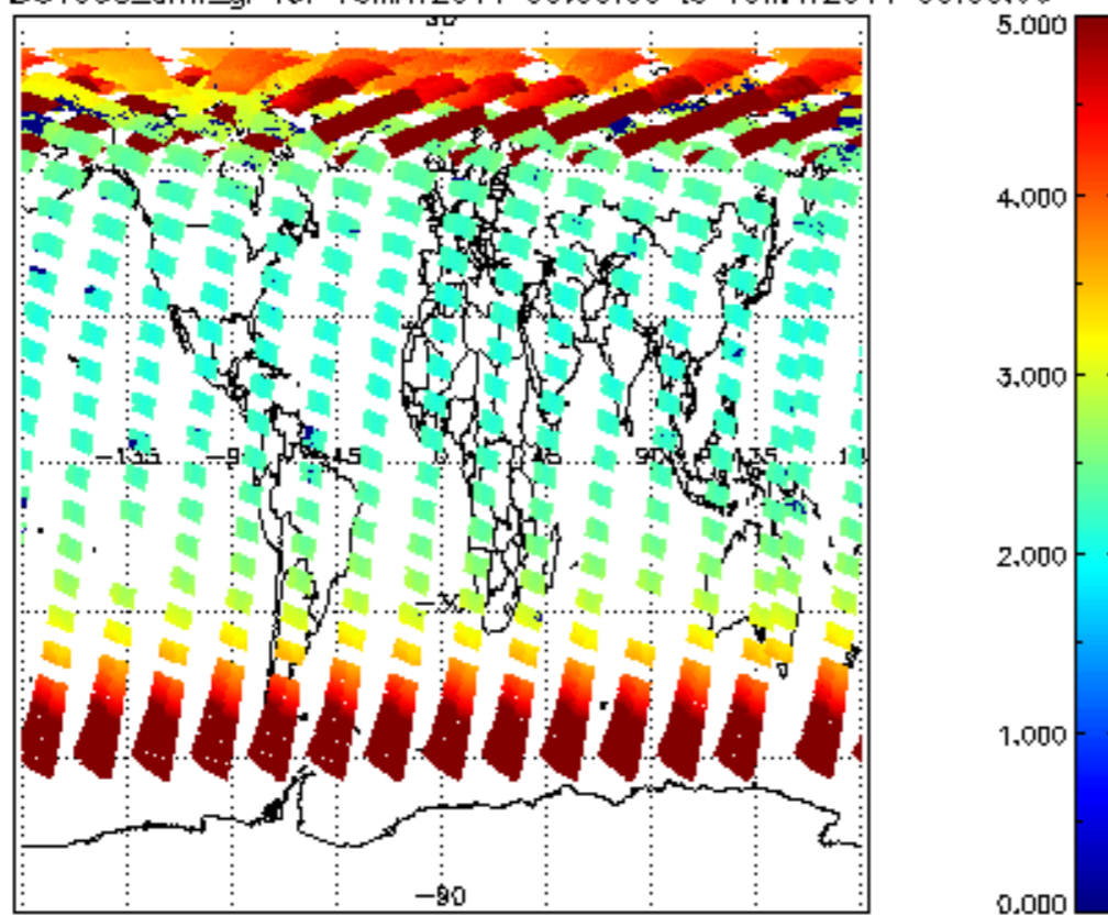
SCIOL2P_NADUV003_amf_gr for 18MAY2011 00:00:00 to 19MAY2011 00:00:00
