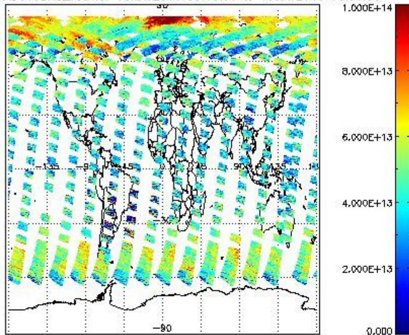
SCIOL2P_NADUV3BRO_vcd for 18MAY2011 00:00:00 to 19MAY2011 00:00:00
