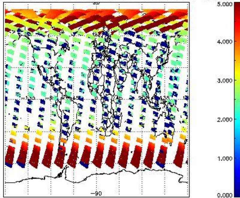
SCIOL2P_NADUV3BRO_amf_cl for 18MAY2011 00:00:00 to 19MAY2011 00:00:00
