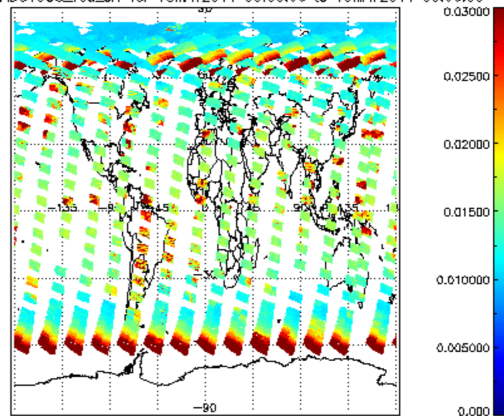
SCIOL2P_NADUV003_vcd_err for 18MAY2011 00:00:00 to 19MAY2011 00:00:00
