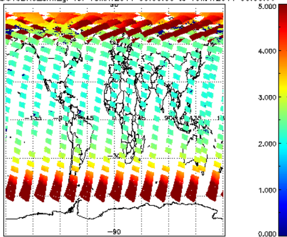
SCIOL2P_NADUV3BRO_amf_gr for 18MAY2011 00:00:00 to 19MAY2011 00:00:00
