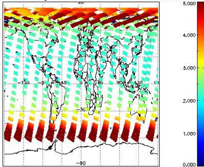
SCIOL2P_NADUV3BRO_amf_gr for 18MAY2011 00:00:00 to 19MAY2011 00:00:00
