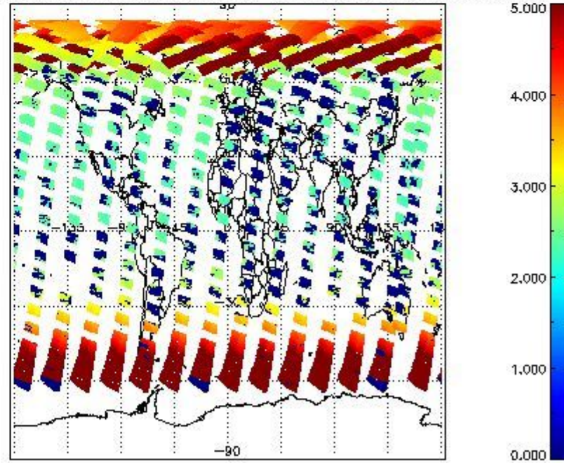
SCIOL2P_NADUV003_amf_cl for 18MAY2011 00:00:00 to 19MAY2011 00:00:00
