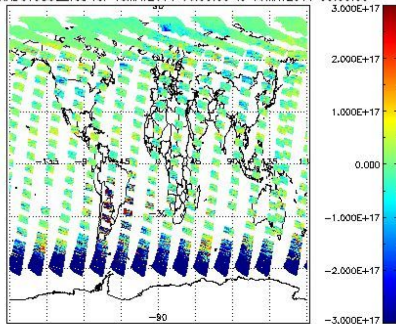
SCIOL2P_NADUV5S02_vcd for 18MAY2011 00:00:00 to 19MAY2011 00:00:00
