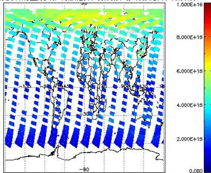
SCIOL2P_NADUV1NO2_vcd for 18MAY2011 00:00:00 to 19MAY2011 00:00:00
