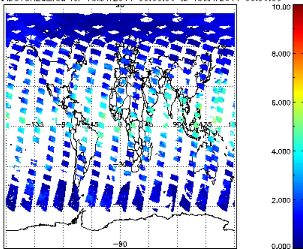
SCIOL2P_NADUV8H2O_vcd for 18MAY2011 00:00:00 to 19MAY2011 00:00:00
