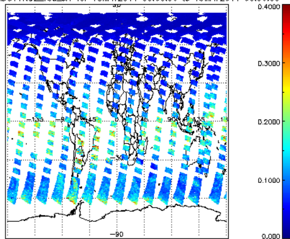
SCIOL2P_NADUV1NO2_vcd_err for 18MAY2011 00:00:00 to 19MAY2011 00:00:00
