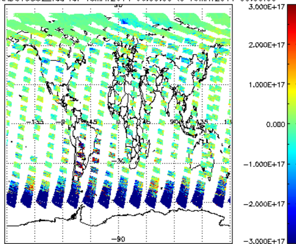
SCIOL2P_NADUV5S02_vcd for 18MAY2011 00:00:00 to 19MAY2011 00:00:00
