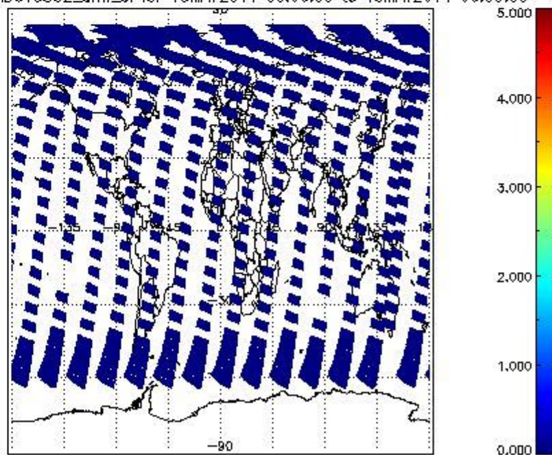
SCIOL2P_NADUV5S02_amf_cl for 18MAY2011 00:00:00 to 19MAY2011 00:00:00
