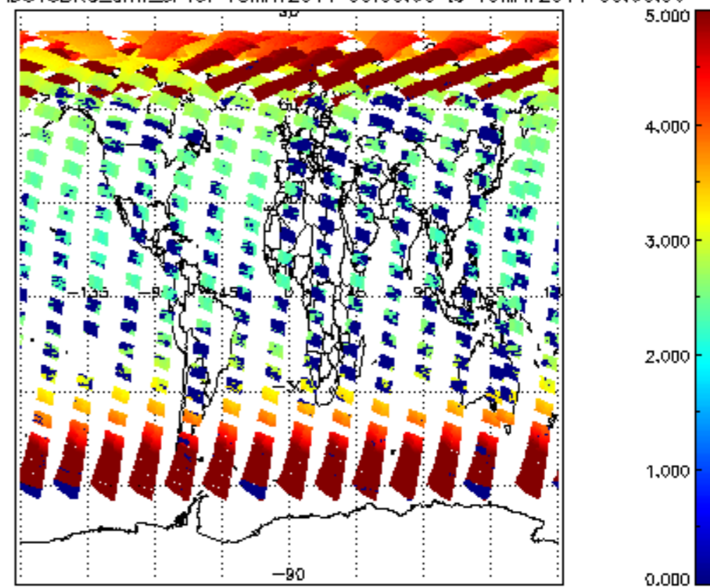
SCIOL2P_NADUV3BRO_amf_sl for 18MAY2011 00:00:00 to 19MAY2011 00:00:00
