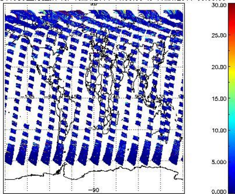
SCIOL2P_NADUV5S02_vcd_err for 18MAY2011 00:00:00 to 19MAY2011 00:00:00
