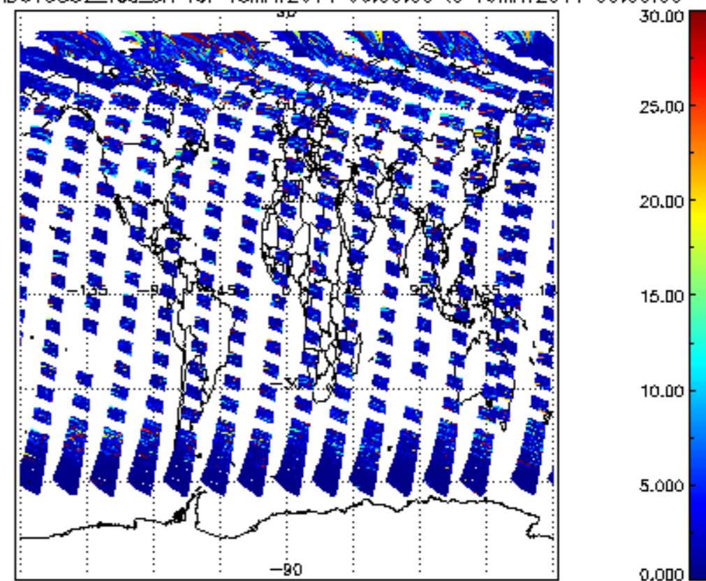
SCIOL2P_NADUV5S02_vcd_err for 18MAY2011 00:00:00 to 19MAY2011 00:00:00
