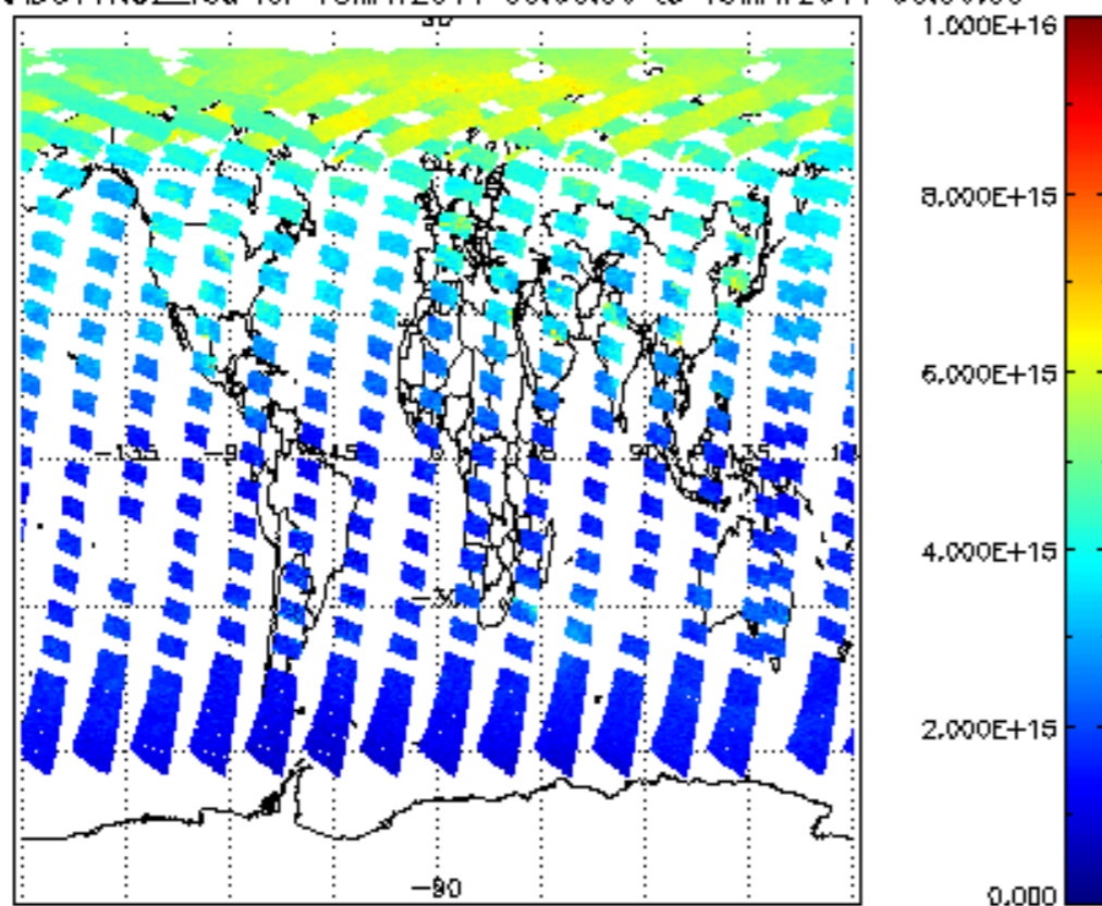
SCIOL2P_NADUV1NO2_vcd for 18MAY2011 00:00:00 to 19MAY2011 00:00:00
