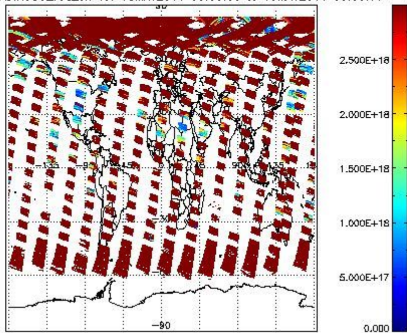
SCIO2P_NADIR3CO_vcd_err for 18MAY2011 00:00:00 to 19MAY2011 00:00:00
