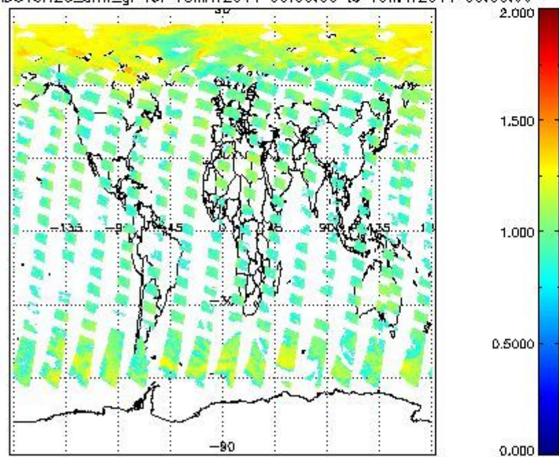
SCIOL2P_NADUV8H2O_arnf_gr for 18MAY2011 00:00:00 to 19MAY2011 00:00:00
