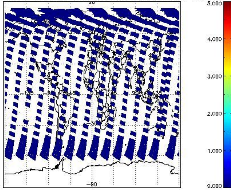
SCIOL2P_NADUV7S02_amf_cl for 18MAY2011 00:00:00 to 19MAY2011 00:00:00
