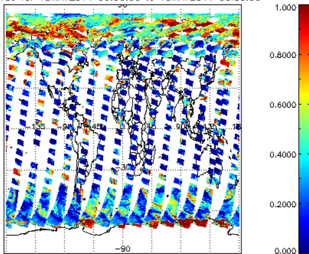
cL_frac for 18MAY2011 00:00:00 to 19MAY2011 00:00:00
