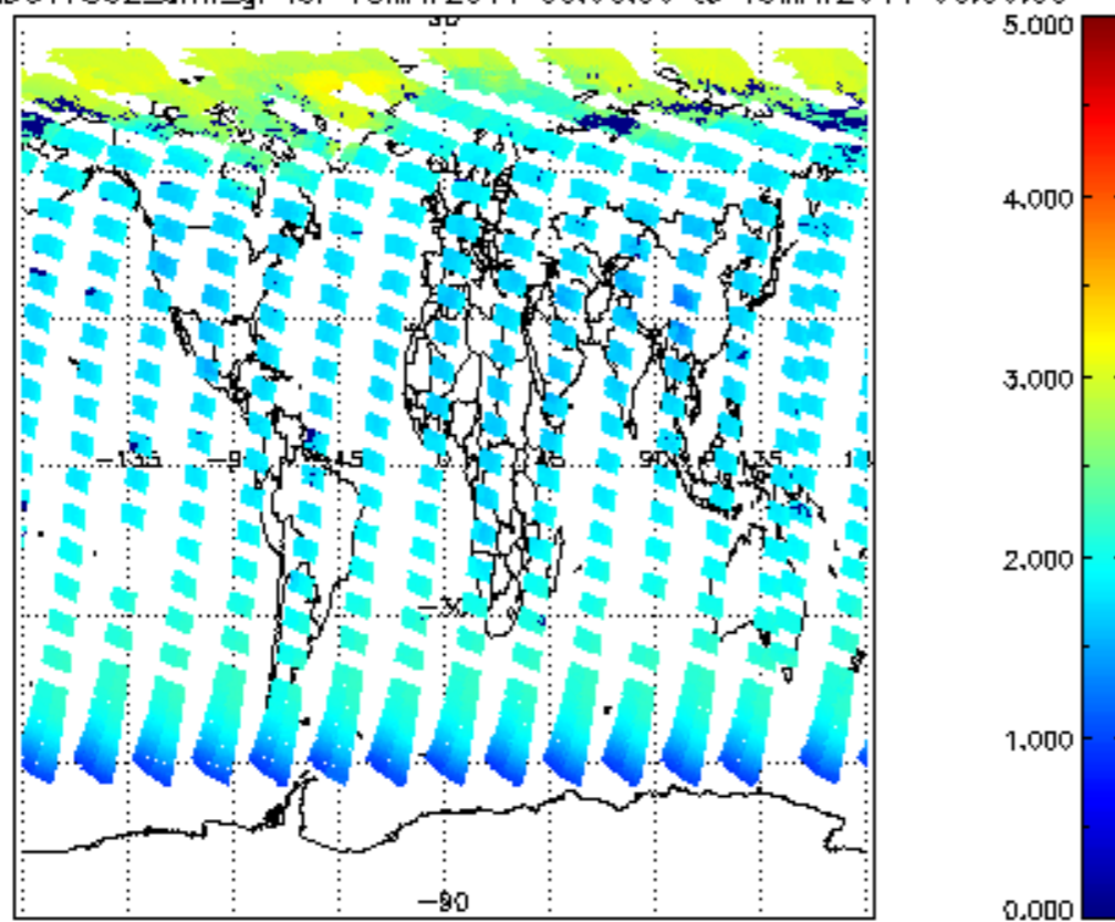
SCIOL2P_NADUV7S02_amf_gr for 18MAY2011 00:00:00 to 19MAY2011 00:00:00
