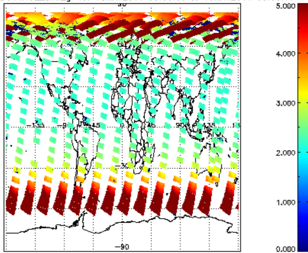
SCIOL2P_NADUV1NO2_amf_gr for 18MAY2011 00:00:00 to 19MAY2011 00:00:00
