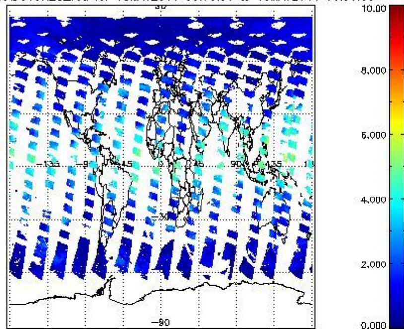
SCIOL2P_NADUV8H2O_vcd for 18MAY2011 00:00:00 to 19MAY2011 00:00:00
