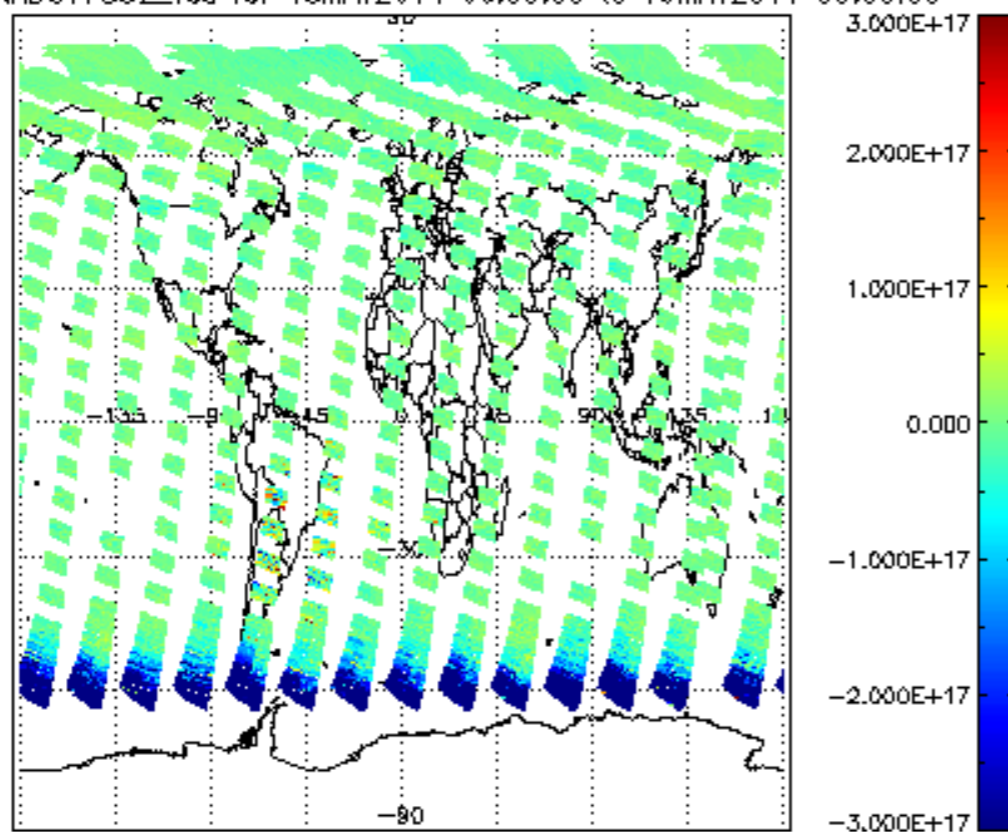
SCIOL2P_NADUV7S02_vcd for 18MAY2011 00:00:00 to 19MAY2011 00:00:00
