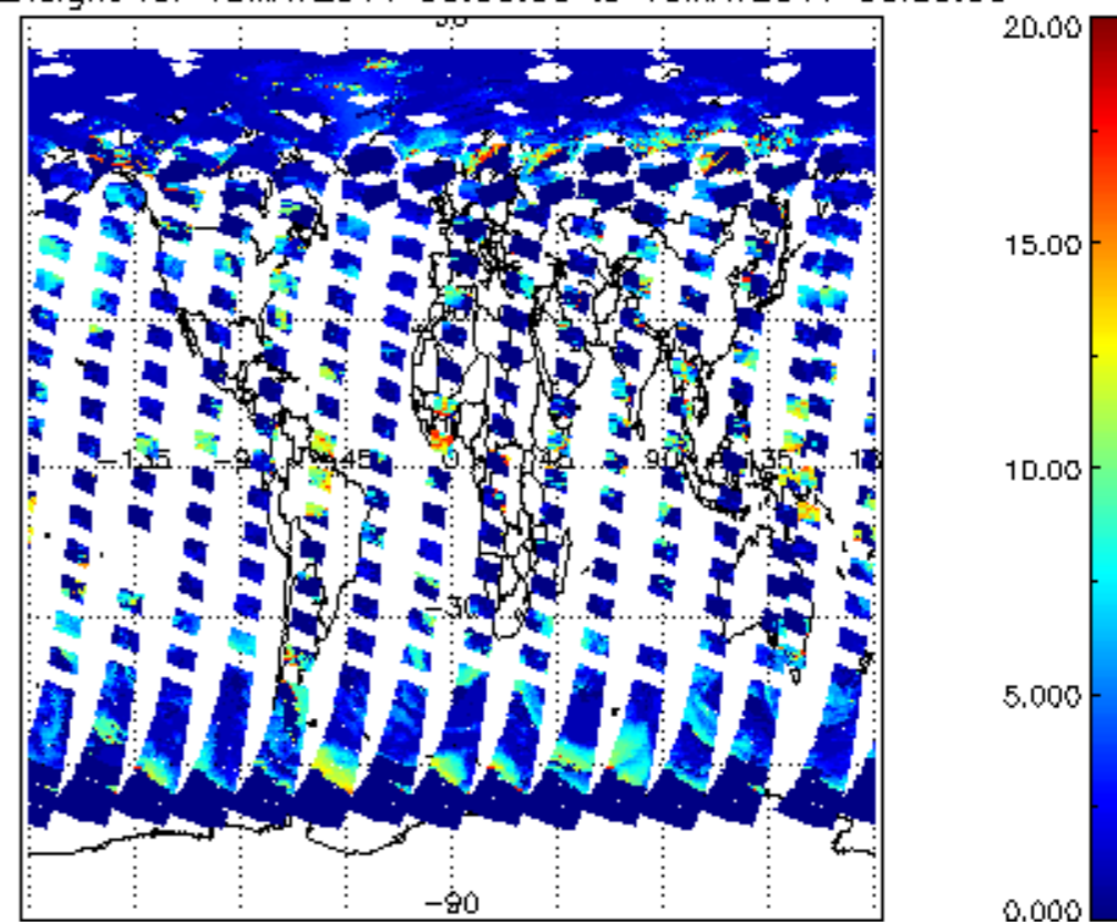
cL_top_height for 18MAY2011 00:00:00 to 19MAY2011 00:00:00
