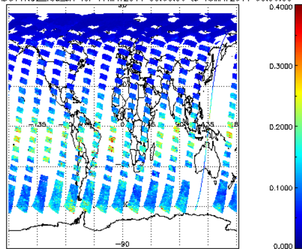
SCIOL2P_NADUV1NO2_vcd_err for 17MAY2011 00:00:00 to 18MAY2011 00:00:00
