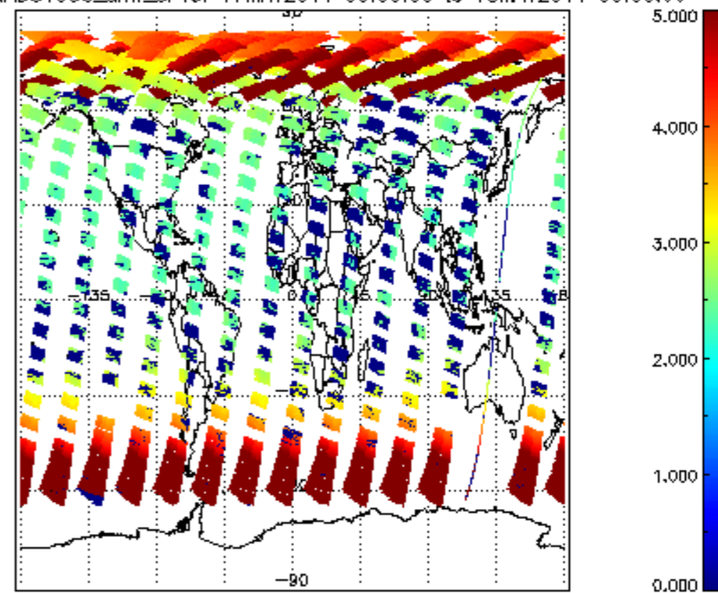
SCIOL2P_NADUV003_amf_cl for 17MAY2011 00:00:00 to 18MAY2011 00:00:00
