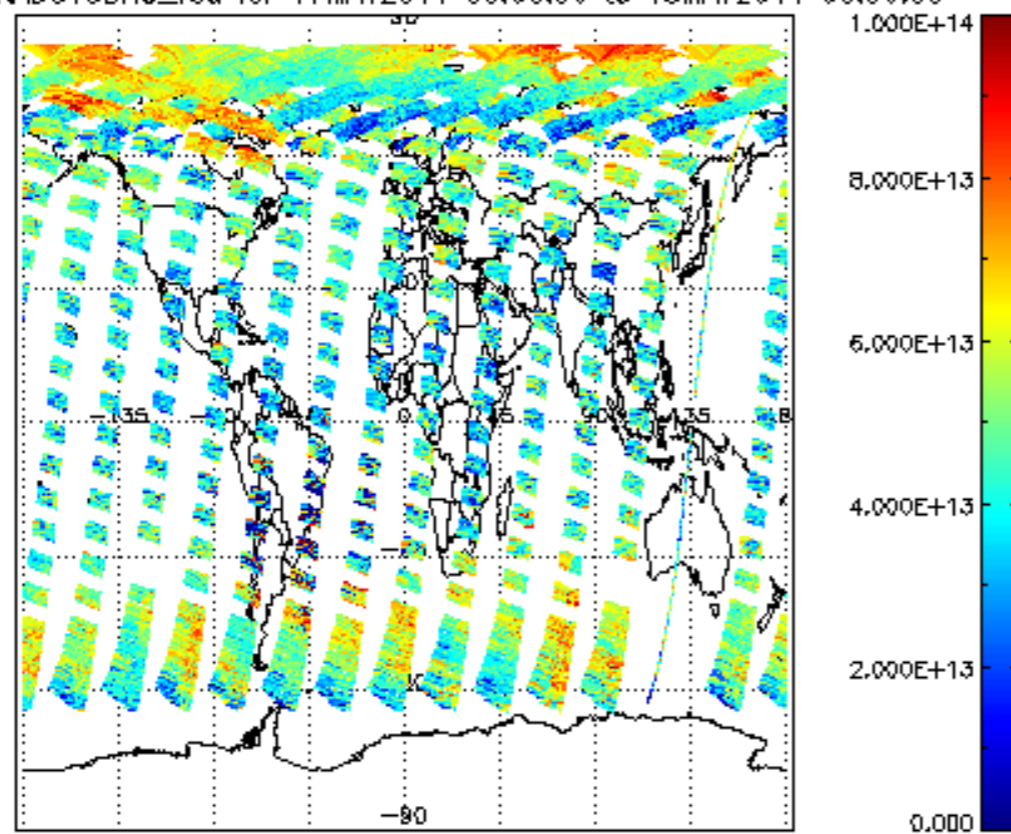
SCIOL2P_NADUV3BRO_vcd for 17MAY2011 00:00:00 to 18MAY2011 00:00:00
