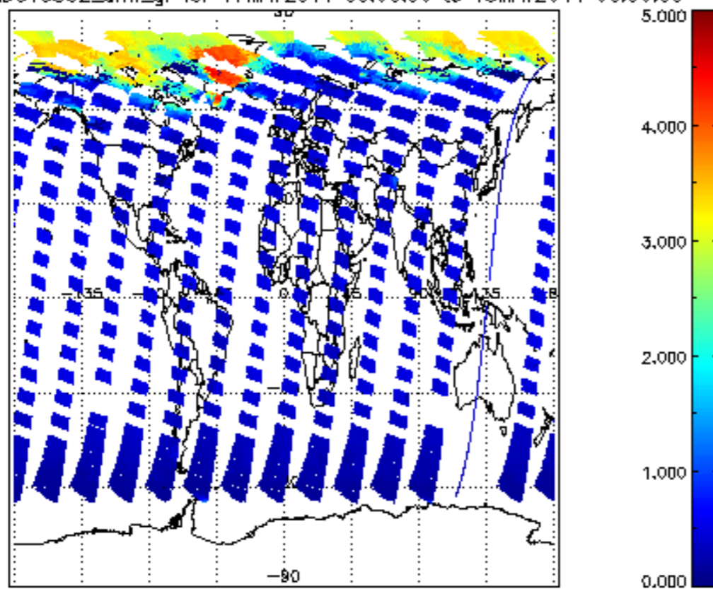
SCIOL2P_NADUV5S02_amf_gr for 17MAY2011 00:00:00 to 18MAY2011 00:00:00
