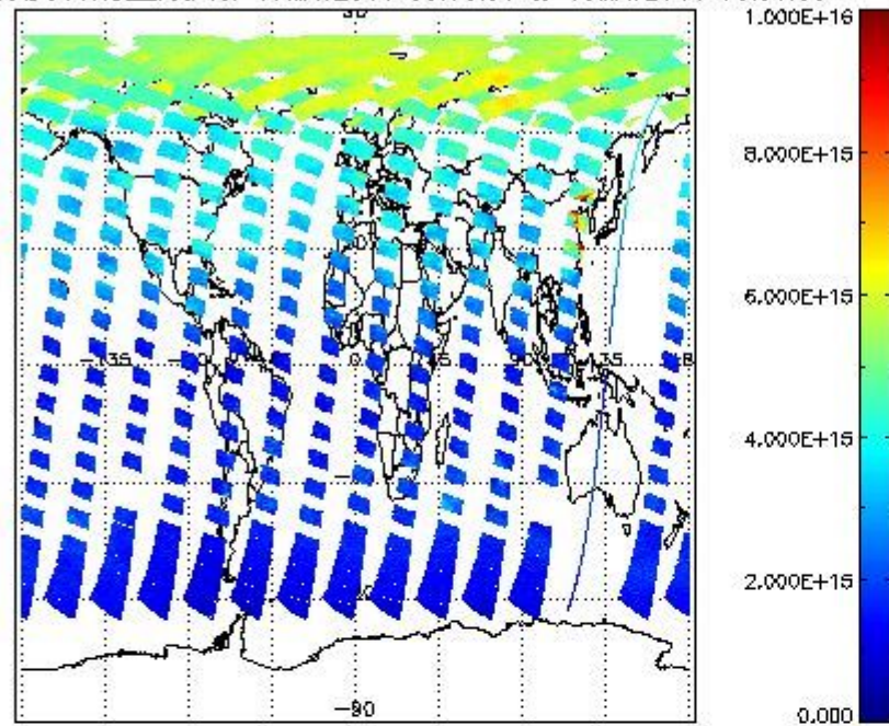
SCIOL2P_NADUV1NO2_vcd for 17MAY2011 00:00:00 to 18MAY2011 00:00:00
