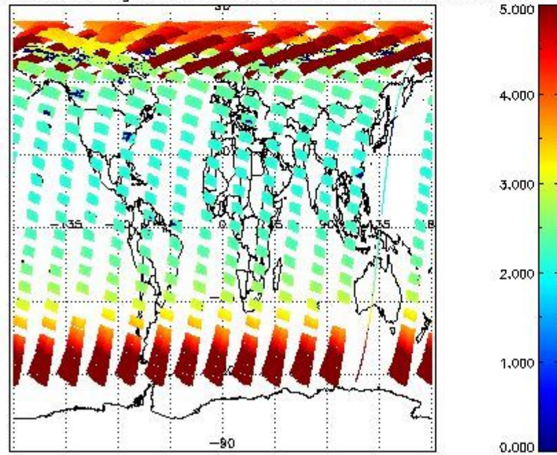
SCIOL2P_NADUV3BRO_amf_gr for 17MAY2011 00:00:00 to 18MAY2011 00:00:00
