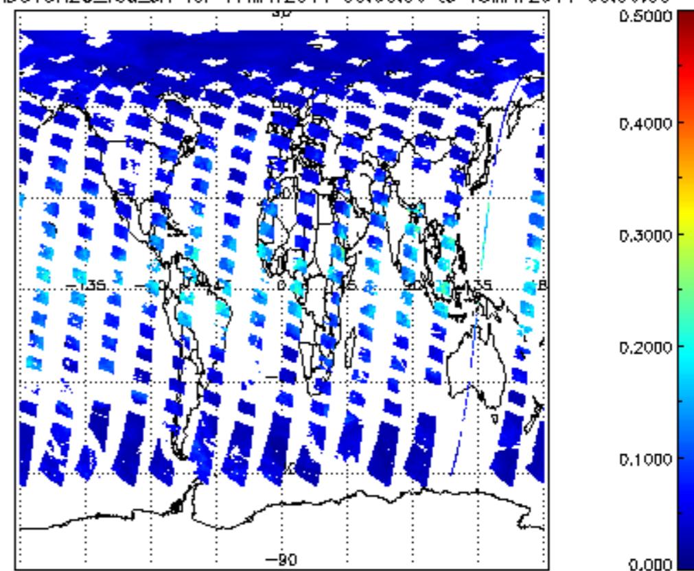
SCIOL2P_NADUV8H2O_vcd_err for 17MAY2011 00:00:00 to 18MAY2011 00:00:00
