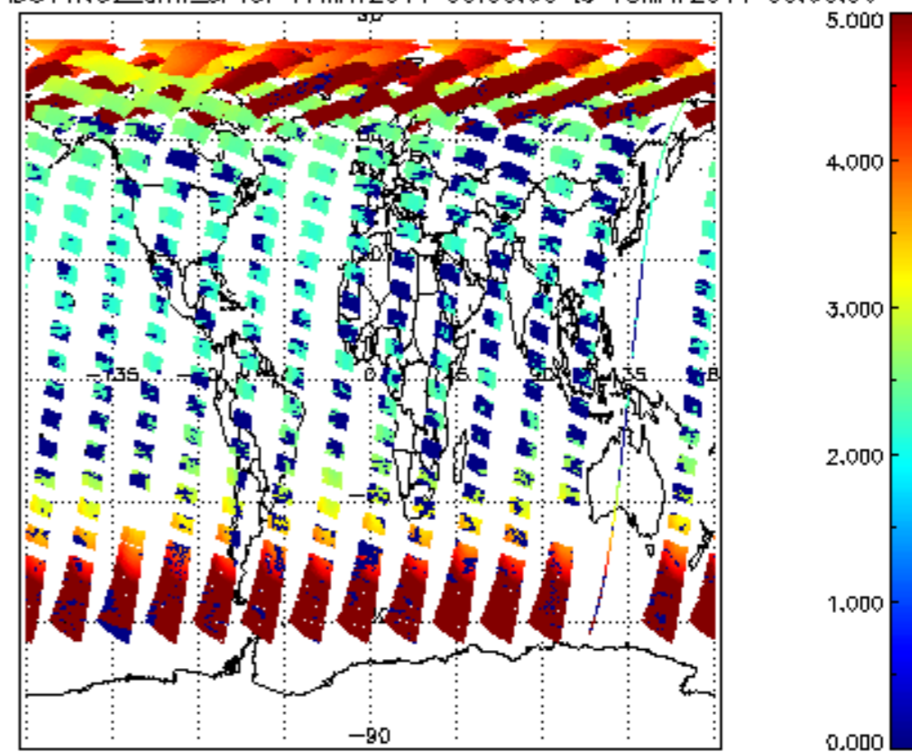
SCIOL2P_NADUV1NO2_amf_sl for 17MAY2011 00:00:00 to 18MAY2011 00:00:00
