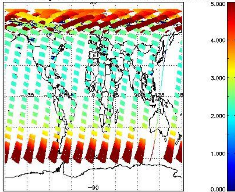
SCIOL2P_NADUV003_amf_gr for 17MAY2011 00:00:00 to 18MAY2011 00:00:00
