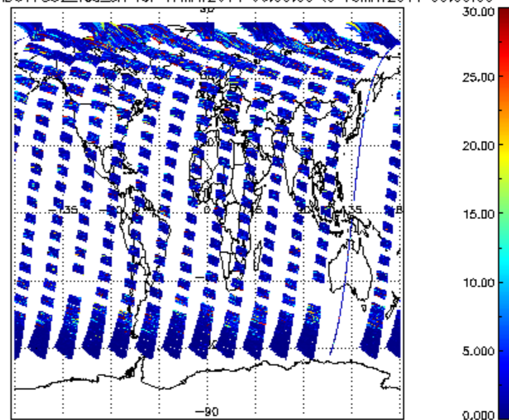
SCIOL2P_NADUV7S02_vcd_err for 17MAY2011 00:00:00 to 18MAY2011 00:00:00
