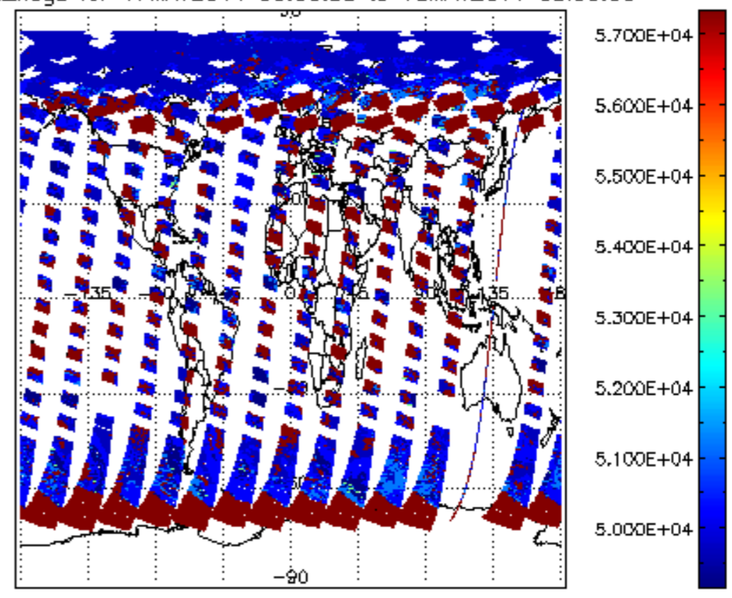
cloud_flags for 17MAY2011 00:00:00 to 18MAY2011 00:00:00
