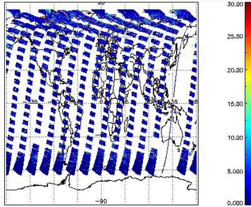
SCIOL2P_NADUV5S02_vcd_err for 17MAY2011 00:00:00 to 18MAY2011 00:00:00
