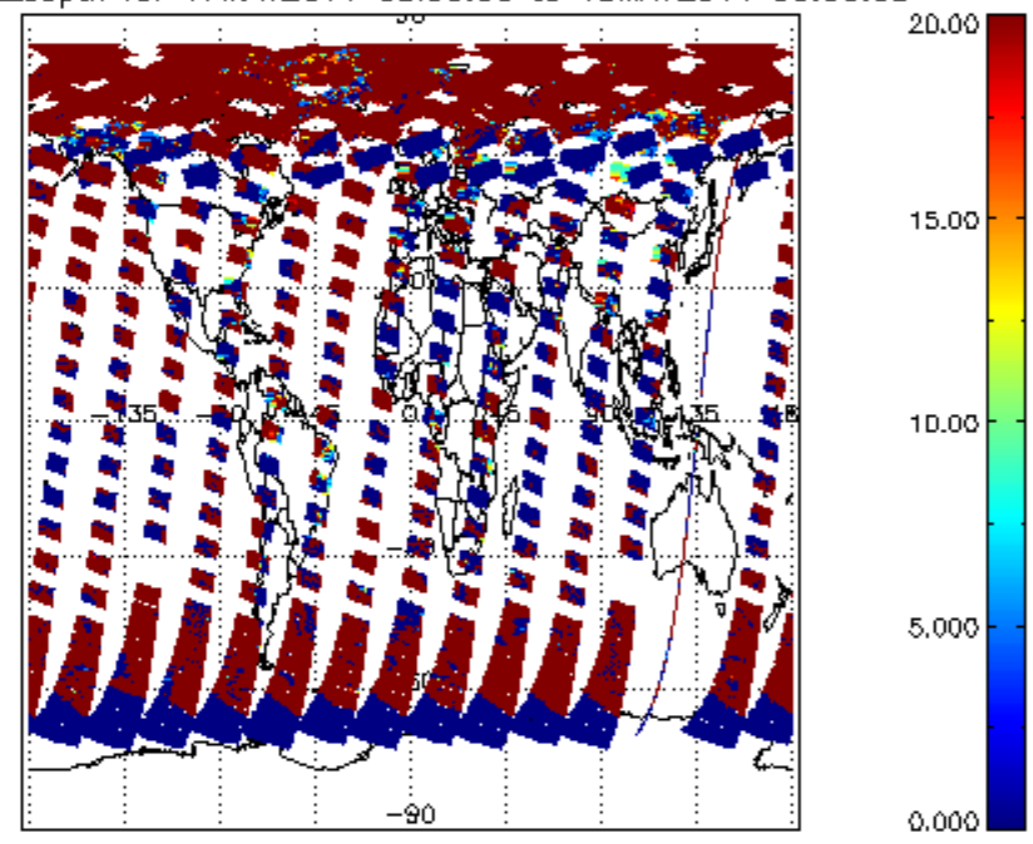
cl_opt_depth for 17MAY2011 00:00:00 to 18MAY2011 00:00:00
