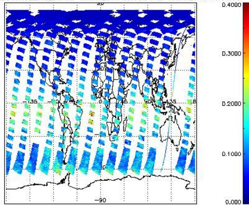
SCIOL2P_NADUV1NO2_vcd_err for 17MAY2011 00:00:00 to 18MAY2011 00:00:00
