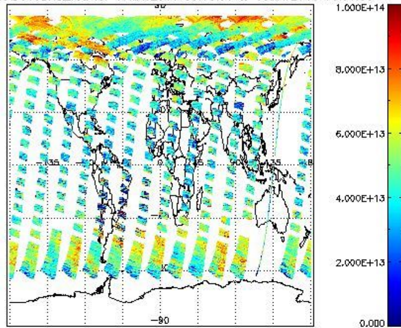
SCIOL2P_NADUV3BRO_vcd for 17MAY2011 00:00:00 to 18MAY2011 00:00:00
