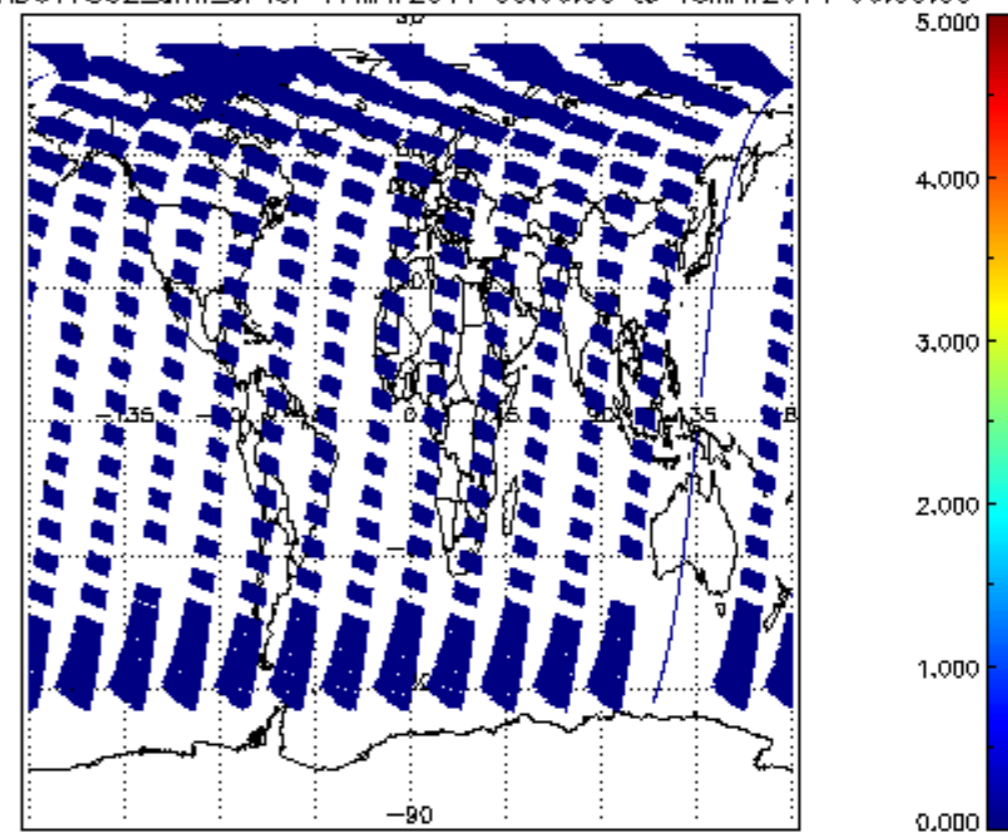
SCIOL2P_NADUV7S02_amf_cl for 17MAY2011 00:00:00 to 18MAY2011 00:00:00
