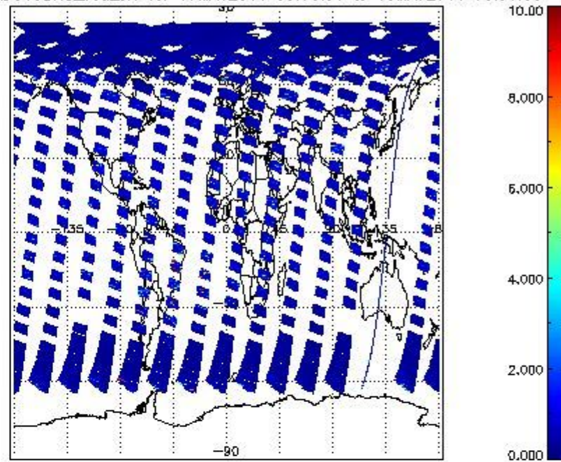
SCIOL2P_NADUV3BRO_vcd_err for 17MAY2011 00:00:00 to 18MAY2011 00:00:00
