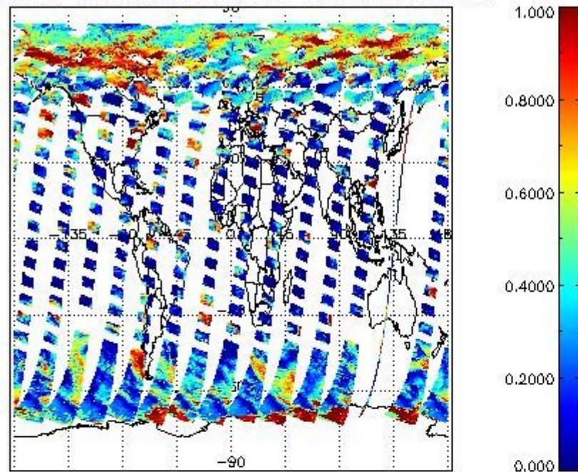
cL_frac for 17MAY2011 00:00:00 to 18MAY2011 00:00:00
