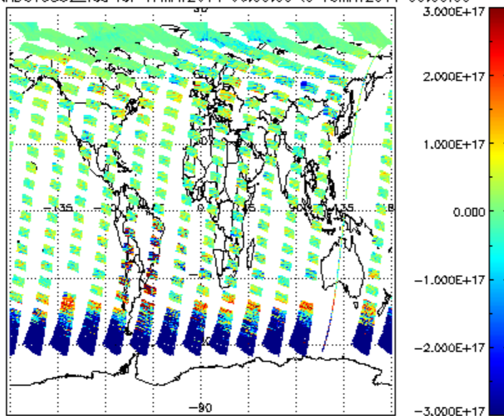
SCIOL2P_NADUV5S02_vcd for 17MAY2011 00:00:00 to 18MAY2011 00:00:00
