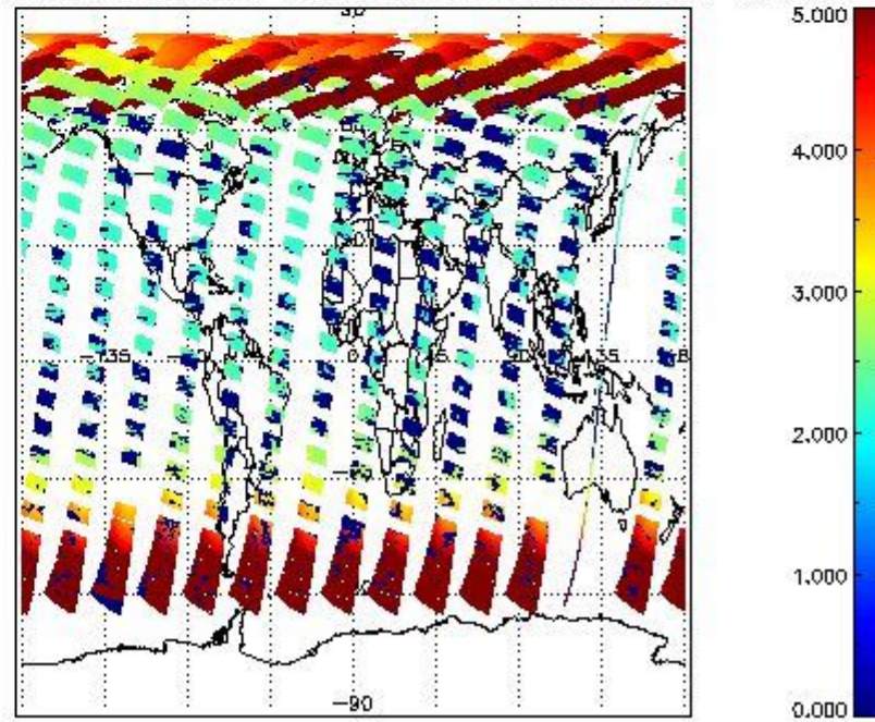
SCIOL2P_NADUV1NO2_amf_cl for 17MAY2011 00:00:00 to 18MAY2011 00:00:00
