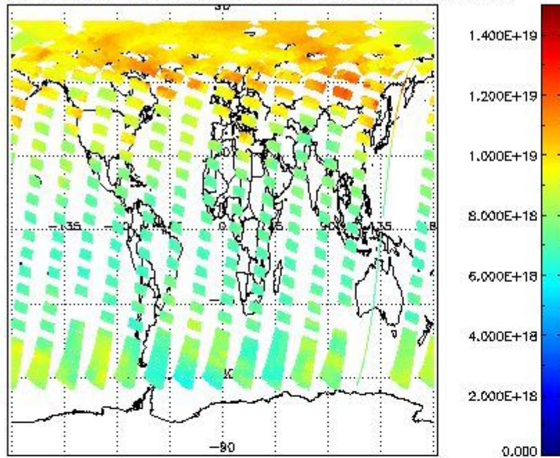
SCIOL2P_NADUV003_vcd for 17MAY2011 00:00:00 to 18MAY2011 00:00:00
