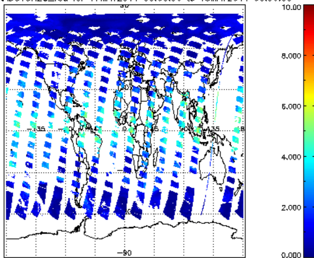
SCIOL2P_NADUV8H2O_vcd for 17MAY2011 00:00:00 to 18MAY2011 00:00:00
