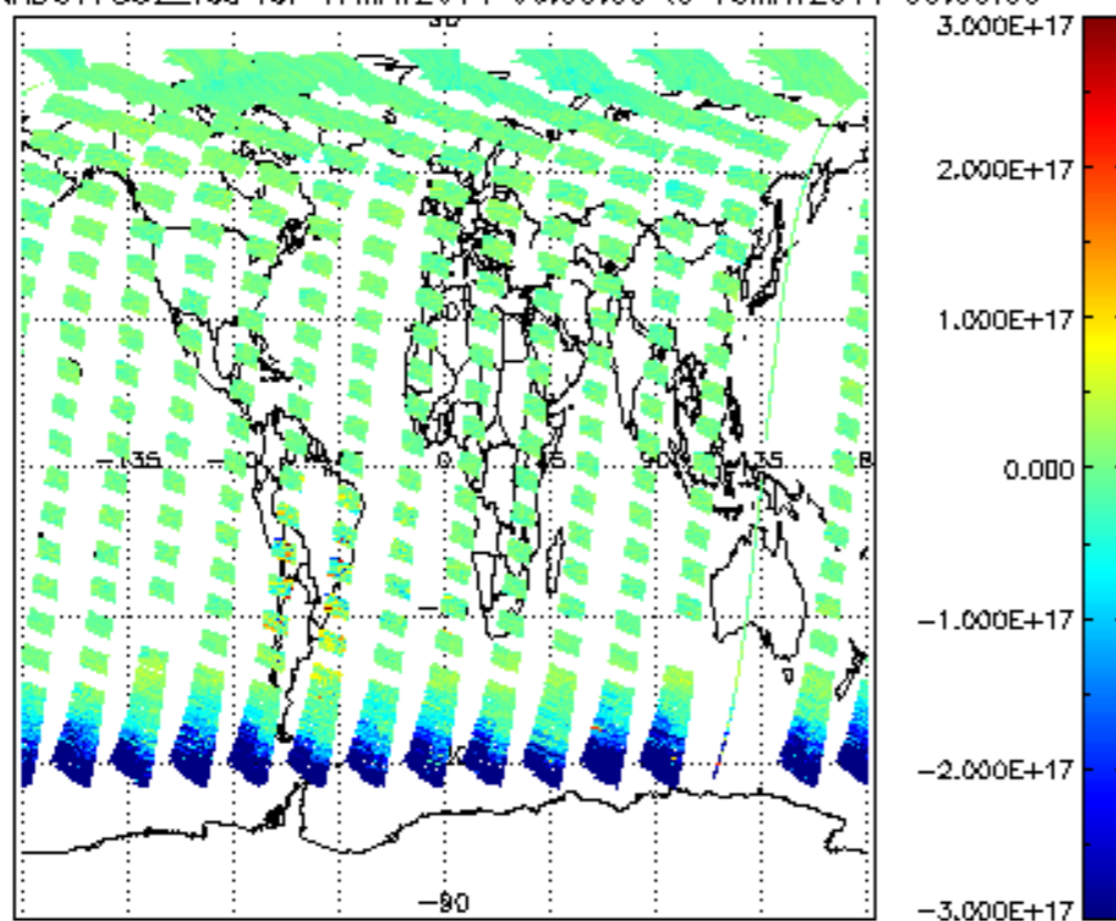
SCIOL2P_NADUV7S02_vcd for 17MAY2011 00:00:00 to 18MAY2011 00:00:00
