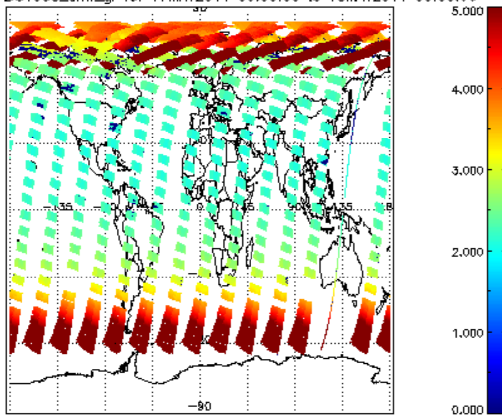
SCIOL2P_NADUV003_amf_gr for 17MAY2011 00:00:00 to 18MAY2011 00:00:00
