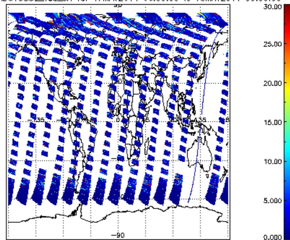
SCIOL2P_NADUV5S02_vcd_err for 17MAY2011 00:00:00 to 18MAY2011 00:00:00
