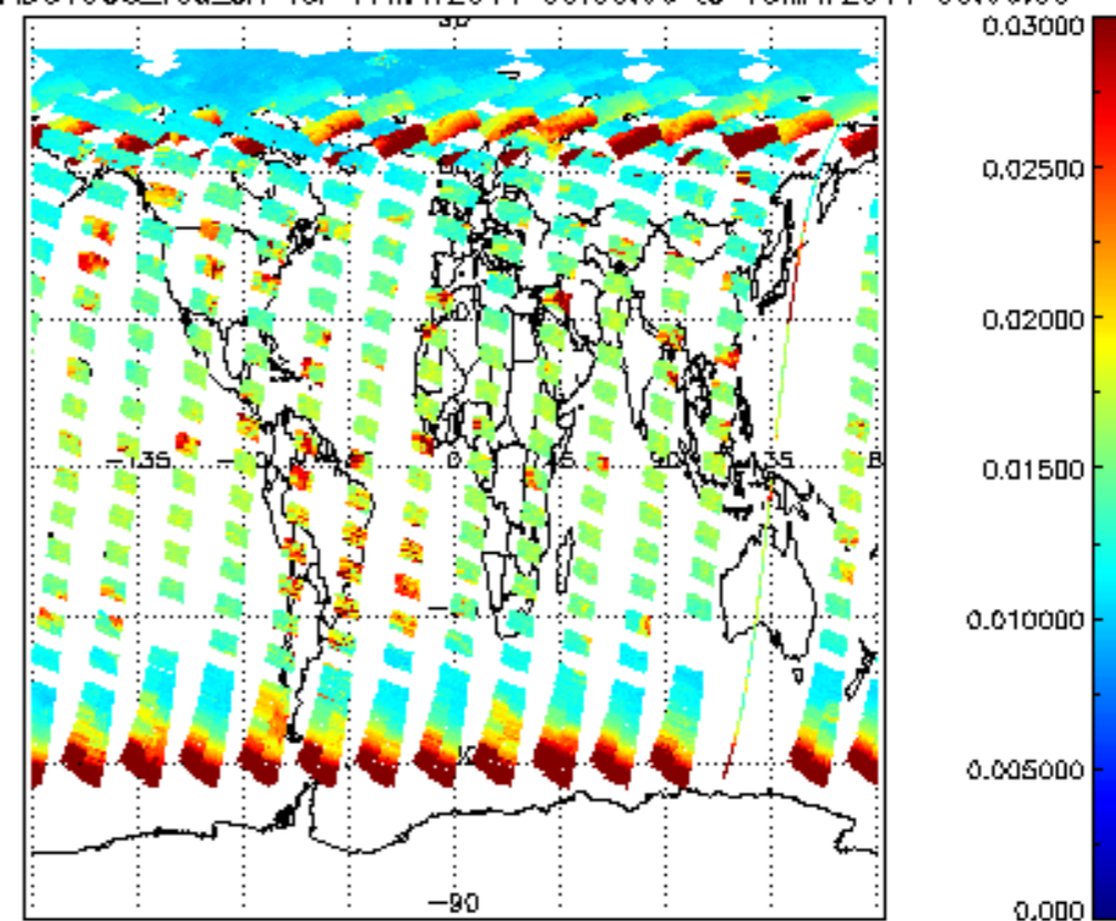
SCIOL2P_NADUV003_vcd_err for 17MAY2011 00:00:00 to 18MAY2011 00:00:00
