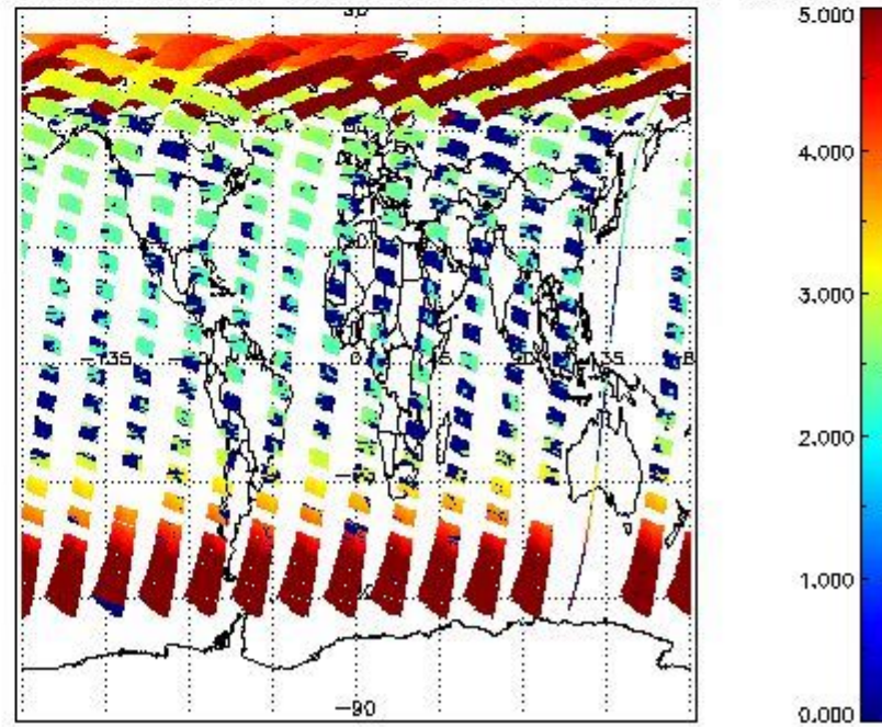
SCIOL2P_NADUV3BRO_amf_cl for 17MAY2011 00:00:00 to 18MAY2011 00:00:00
