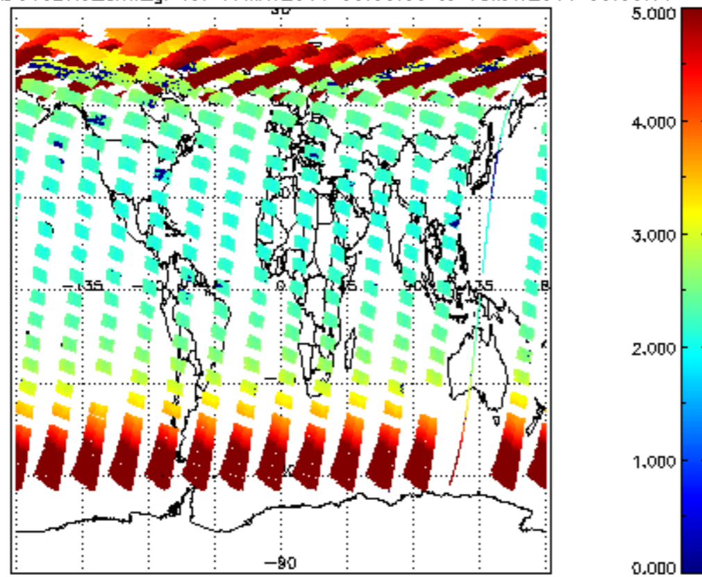
SCIOL2P_NADUV3BRO_amf_gr for 17MAY2011 00:00:00 to 18MAY2011 00:00:00
