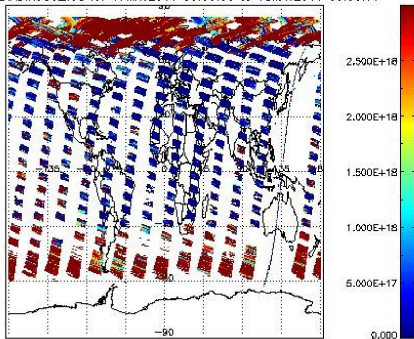
SCIDL2P_NADIR3CO_vcd for 17MAY2011 00:00:00 to 18MAY2011 00:00:00
