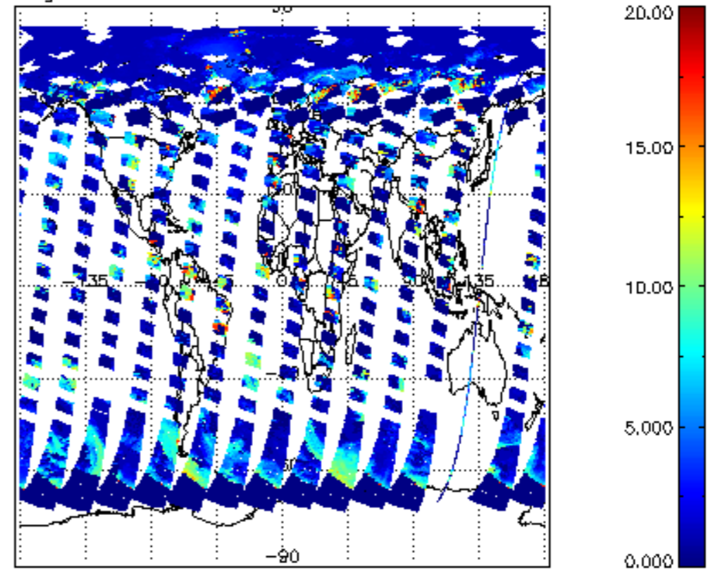
cl_top_height for 17MAY2011 00:00:00 to 18MAY2011 00:00:00
