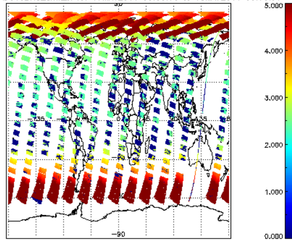
SCIOL2P_NADUV3BRO_amf_cl for 17MAY2011 00:00:00 to 18MAY2011 00:00:00
