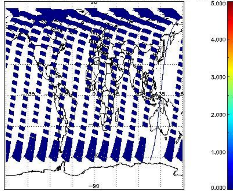
SCIOL2P_NADUV5S02_amf_cl for 17MAY2011 00:00:00 to 18MAY2011 00:00:00
