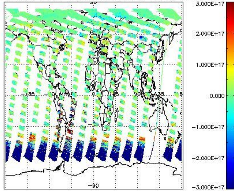
SCIOL2P_NADUV5S02_vcd for 17MAY2011 00:00:00 to 18MAY2011 00:00:00
