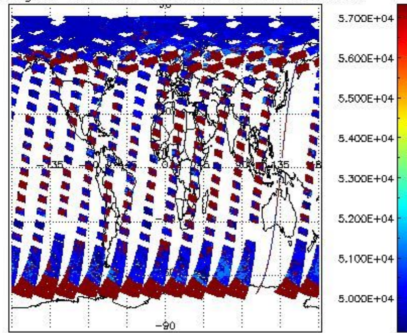
cloud_flags for 17MAY2011 00:00:00 to 18MAY2011 00:00:00
