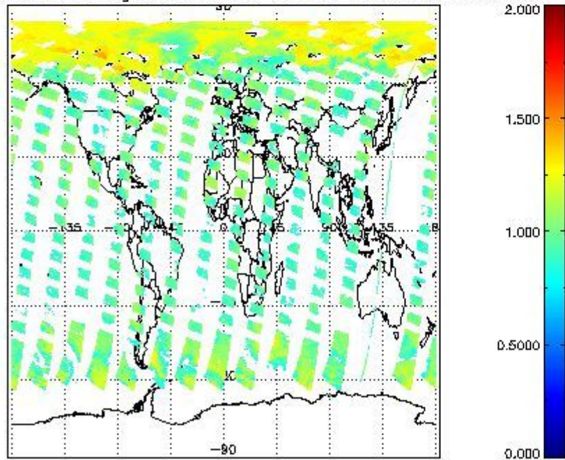
SCIOL2P_NADUV8H2O_arnf_gr for 17MAY2011 00:00:00 to 18MAY2011 00:00:00
