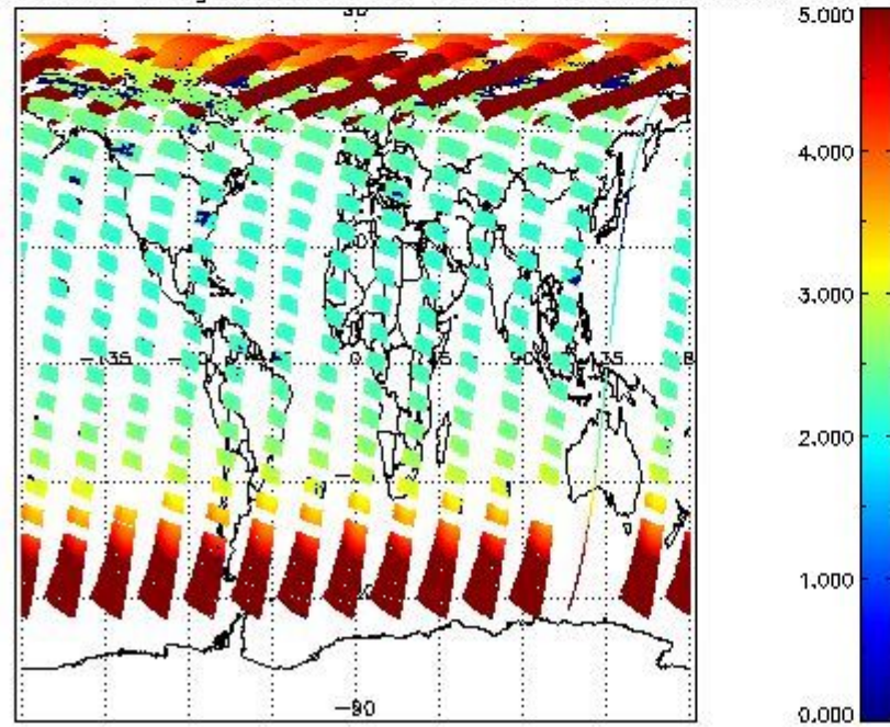
SCIOL2P_NADUV1NO2_amf_gr for 17MAY2011 00:00:00 to 18MAY2011 00:00:00
