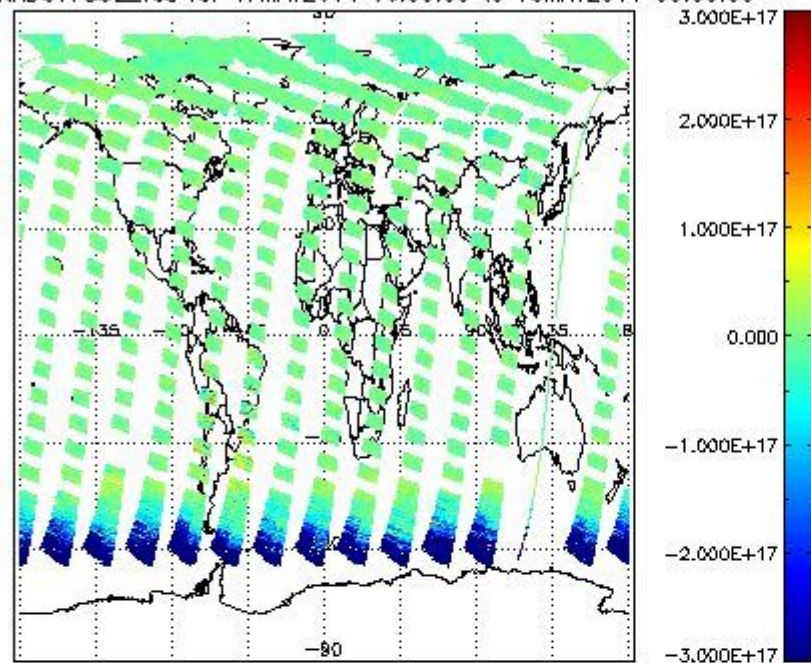
SCIOL2P_NADUV7S02_vcd for 17MAY2011 00:00:00 to 18MAY2011 00:00:00
