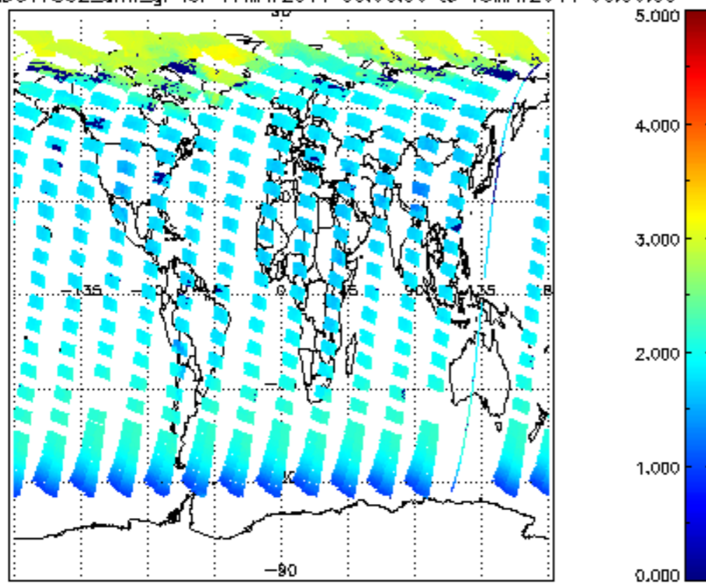
SCIOL2P_NADUV7S02_amf_gr for 17MAY2011 00:00:00 to 18MAY2011 00:00:00
