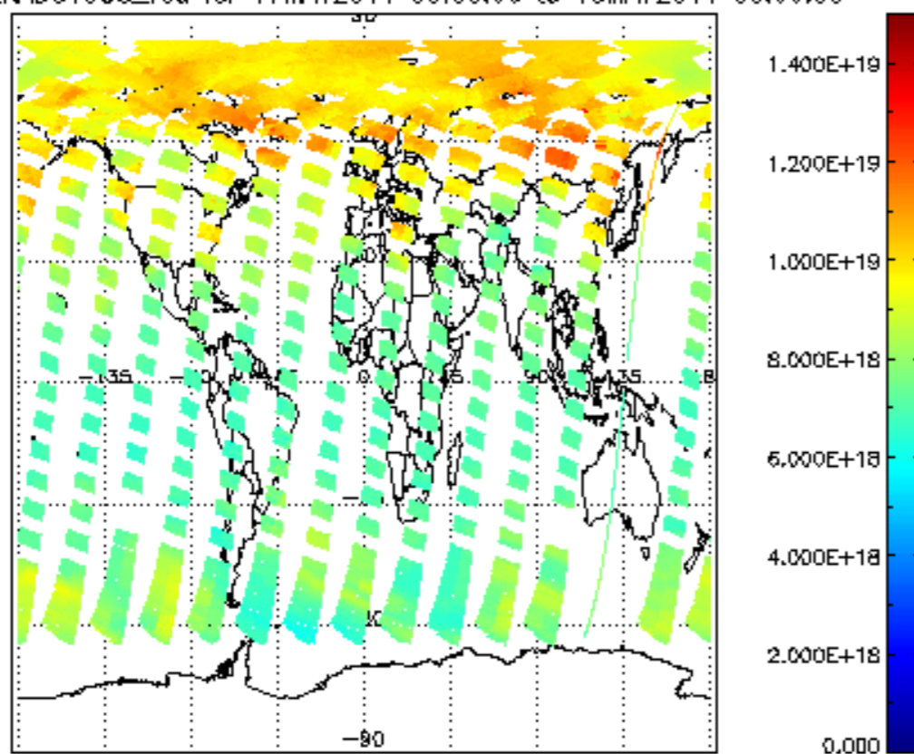
SCIOL2P_NADUV003_vcd for 17MAY2011 00:00:00 to 18MAY2011 00:00:00
