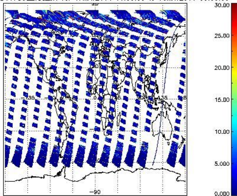
SCIOL2P_NADUV7S02_vcd_err for 17MAY2011 00:00:00 to 18MAY2011 00:00:00
