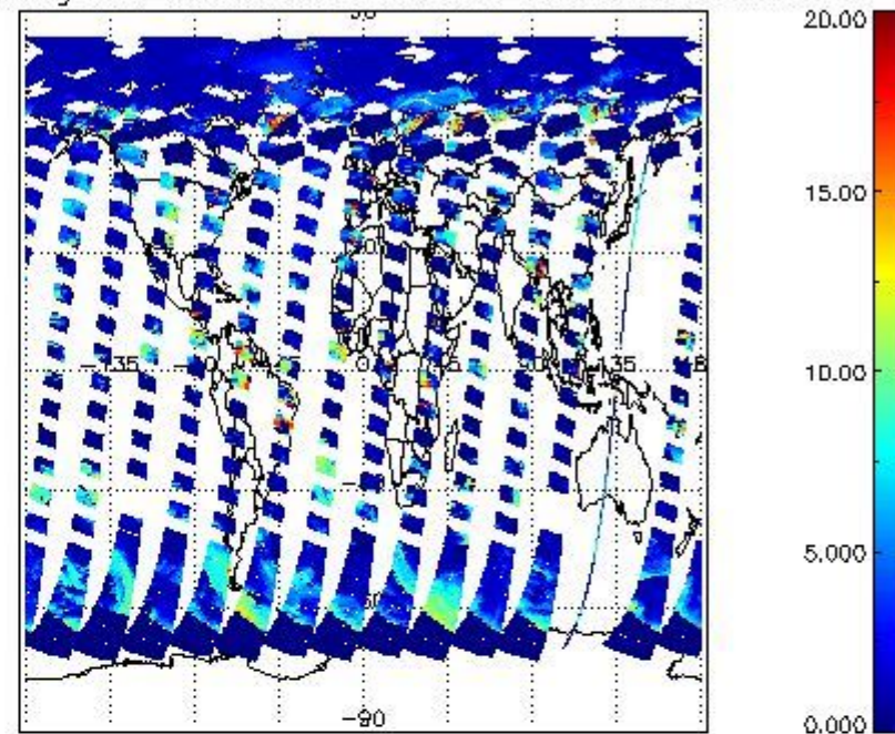
cL_top_height for 17MAY2011 00:00:00 to 18MAY2011 00:00:00
