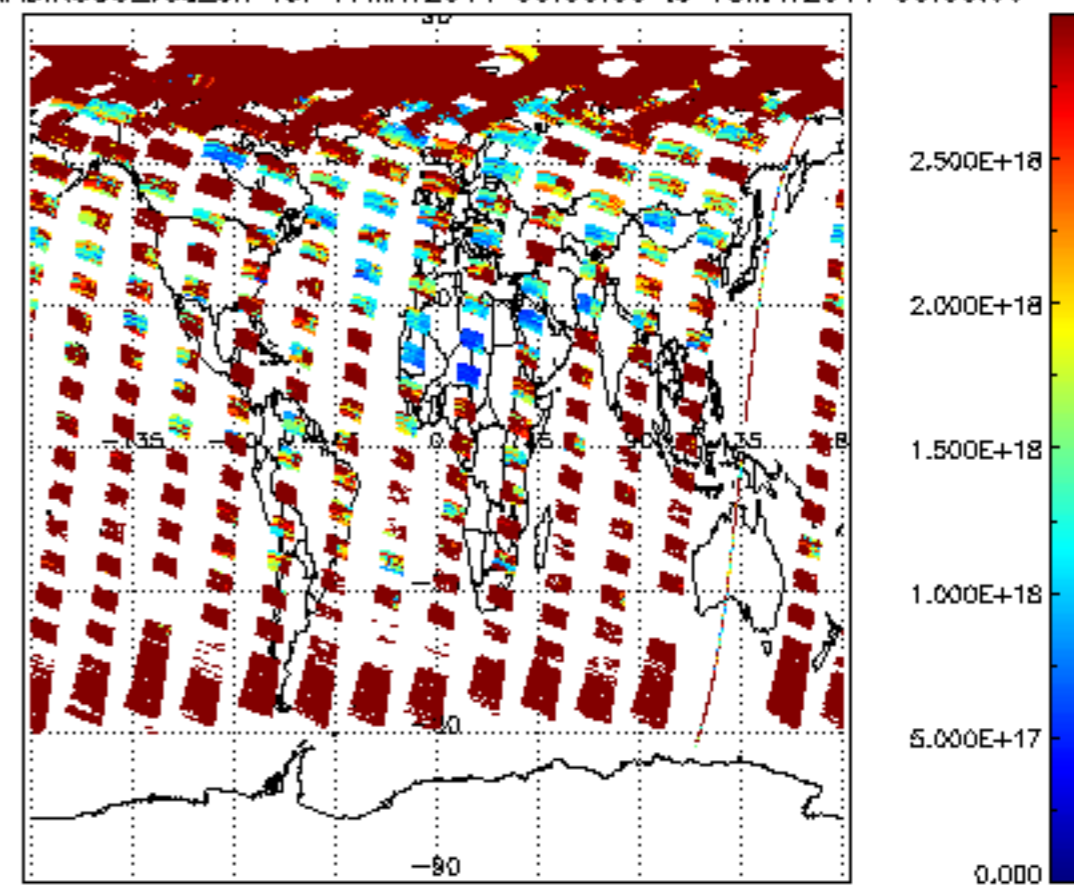
SCIOL2P_NADIR3CO_vcd_err for 17MAY2011 00:00:00 to 18MAY2011 00:00:00
