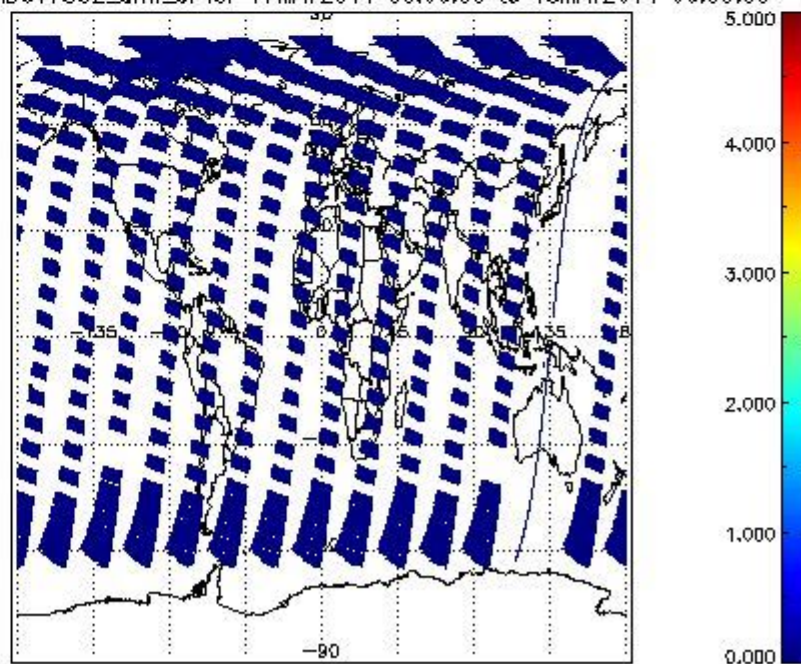
SCIOL2P_NADUV7S02_amf_cl for 17MAY2011 00:00:00 to 18MAY2011 00:00:00
