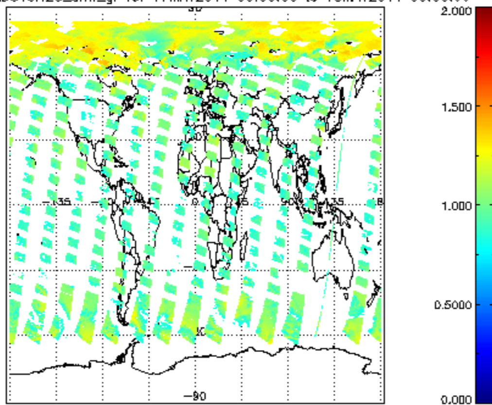
SCIOL2P_NADUV8H2O_amf_gr for 17MAY2011 00:00:00 to 18MAY2011 00:00:00
