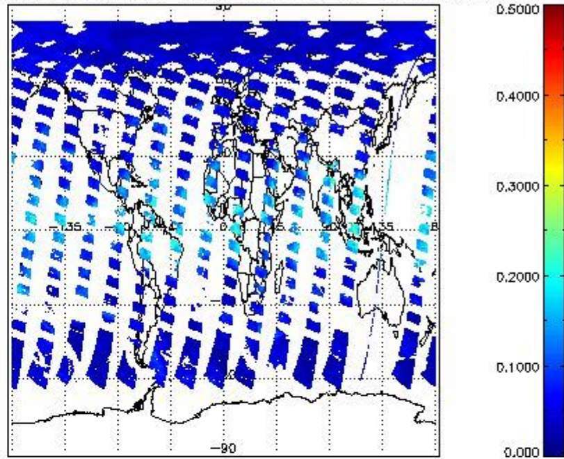
SCIOL2P_NADUV8H2O_vcd_err for 17MAY2011 00:00:00 to 18MAY2011 00:00:00
