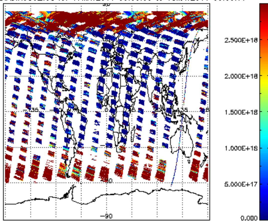
SCIOL2P_NADIR3CO_vcd for 17MAY2011 00:00:00 to 18MAY2011 00:00:00
