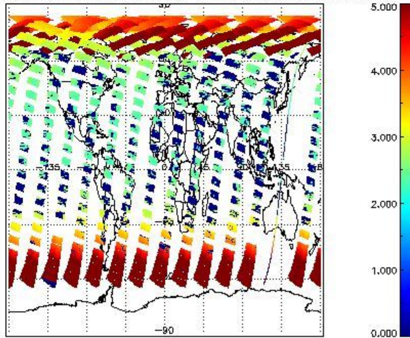
SCIOL2P_NADUV003_amf_cl for 17MAY2011 00:00:00 to 18MAY2011 00:00:00
