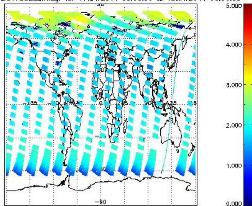
SCIOL2P_NADUV7S02_amf_gr for 17MAY2011 00:00:00 to 18MAY2011 00:00:00
