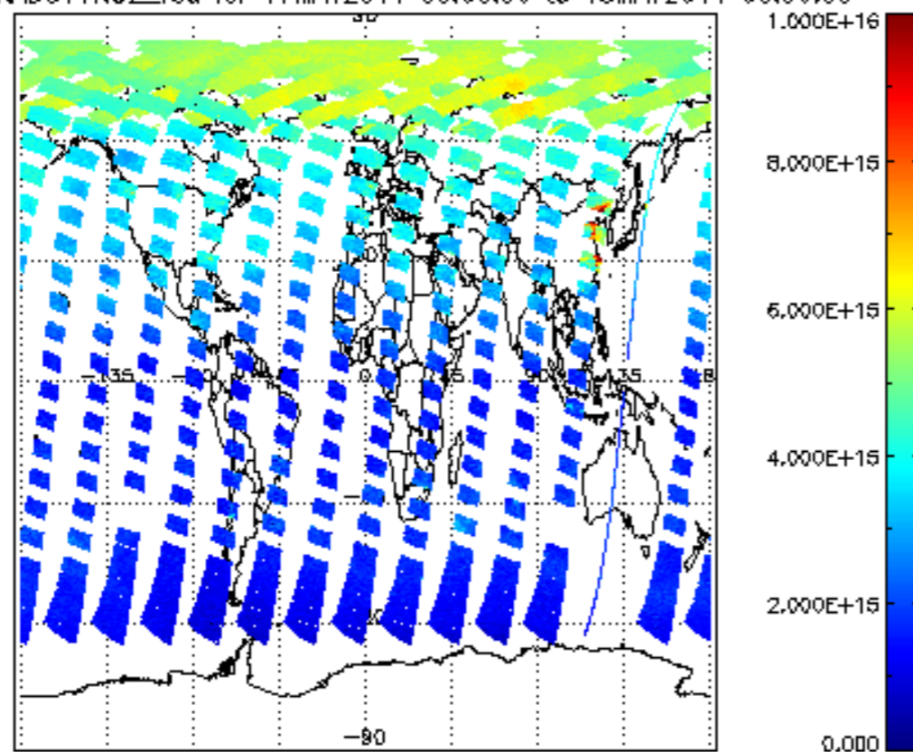
SCIOL2P_NADUV1NO2_vcd for 17MAY2011 00:00:00 to 18MAY2011 00:00:00
