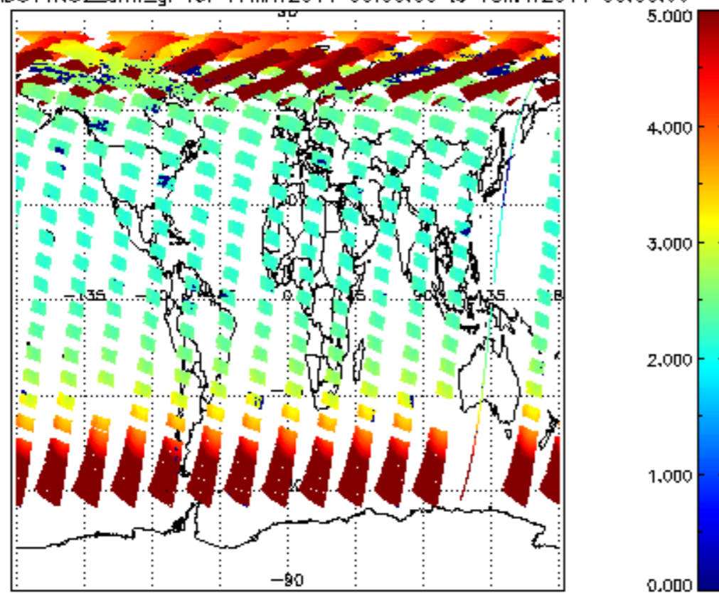
SCIOL2P_NADUV1NO2_amf_gr for 17MAY2011 00:00:00 to 18MAY2011 00:00:00
