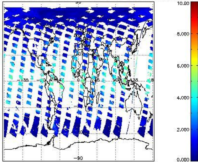
SCIOL2P_NADUV8H2O_vcd for 17MAY2011 00:00:00 to 18MAY2011 00:00:00
