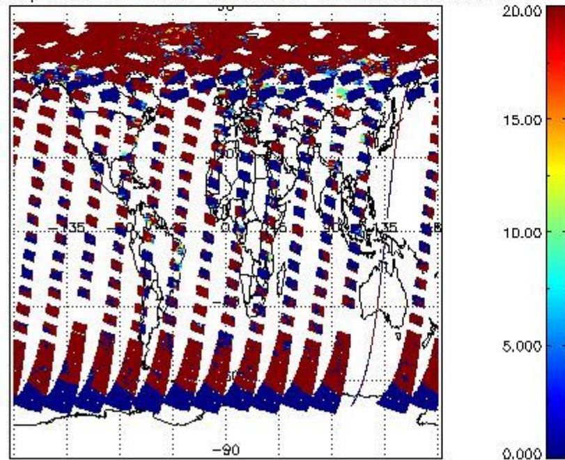
cL_opt_depth for 17MAY2011 00:00:00 to 18MAY2011 00:00:00
