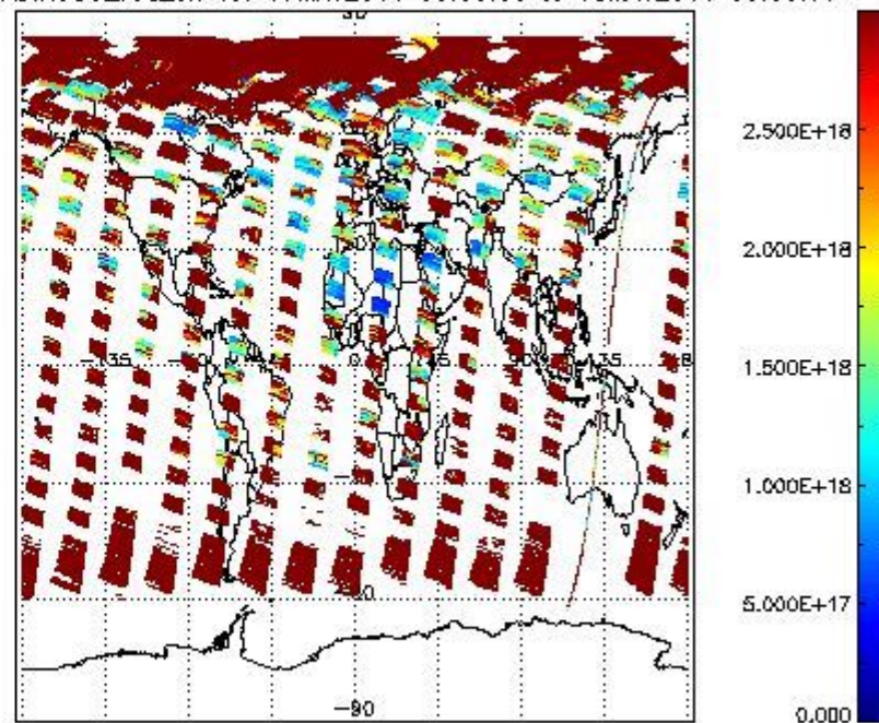
SCIDL2P_NADIR3CO_vcd_err for 17MAY2011 00:00:00 to 18MAY2011 00:00:00
