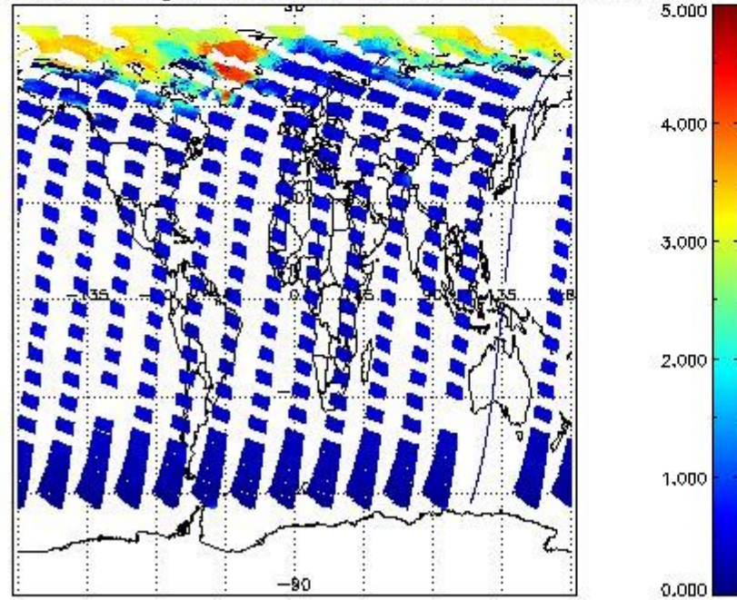
SCIOL2P_NADUV5S02_amf_gr for 17MAY2011 00:00:00 to 18MAY2011 00:00:00
