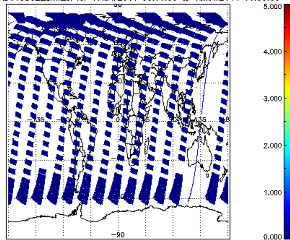
SCIOL2P_NADUV5S02_amf_cl for 17MAY2011 00:00:00 to 18MAY2011 00:00:00
