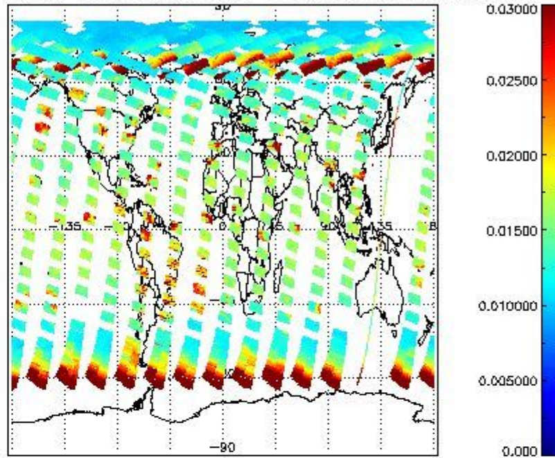
SCIOL2P_NADUV003_vcd_err for 17MAY2011 00:00:00 to 18MAY2011 00:00:00
