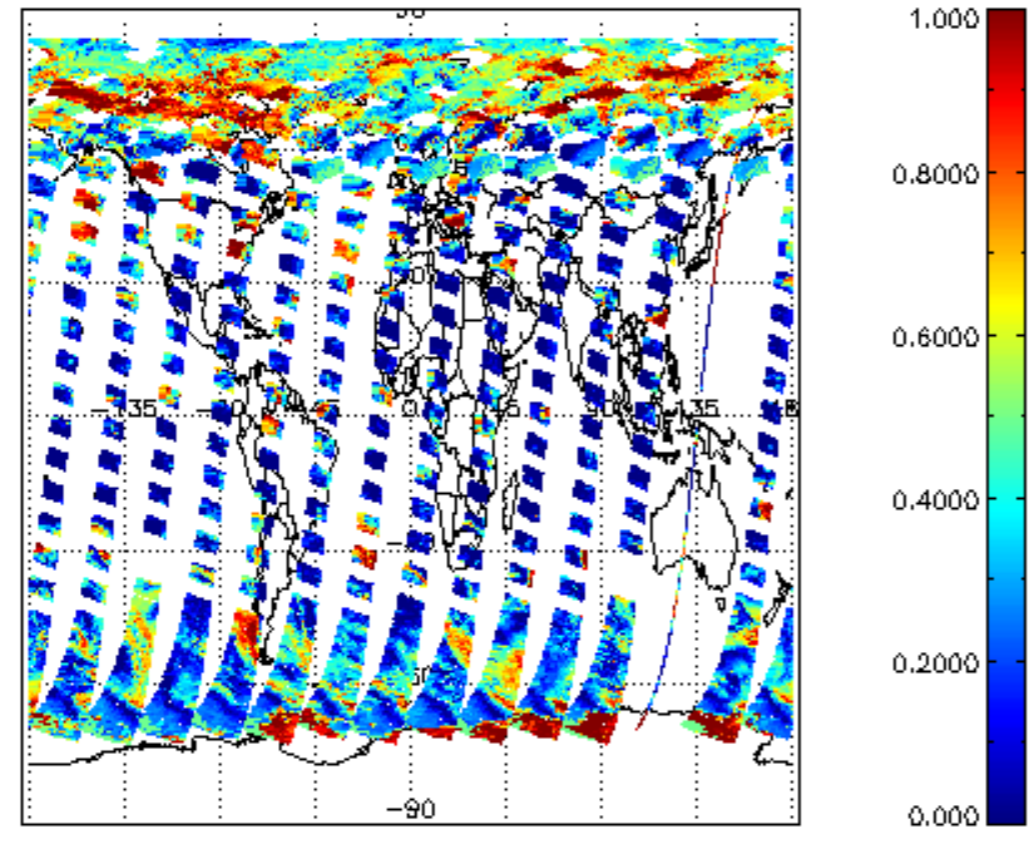
cl_frac for 17MAY2011 00:00:00 to 18MAY2011 00:00:00
