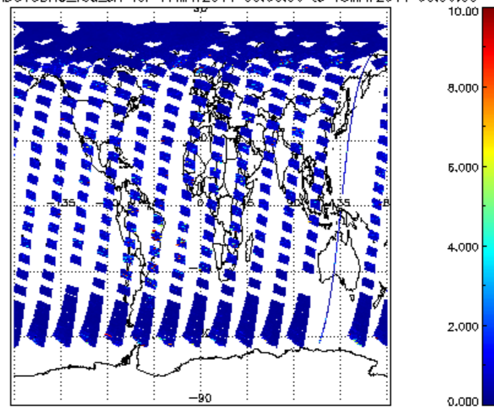
SCIOL2P_NADUV3BRO_vcd_err for 17MAY2011 00:00:00 to 18MAY2011 00:00:00
