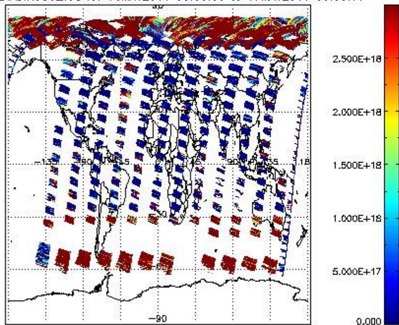
SCIDL2P_NADIR3CO_vcd for 16MAY2011 00:00:00 to 17MAY2011 00:00:00
