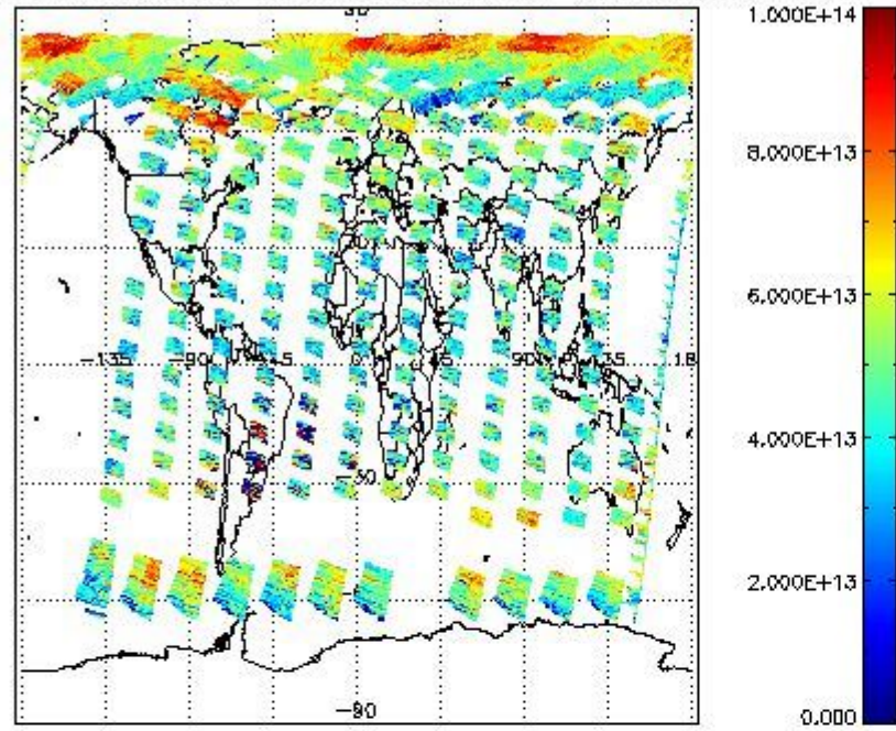
SCIOL2P_NADUV3BRO_vcd for 16MAY2011 00:00:00 to 17MAY2011 00:00:00
