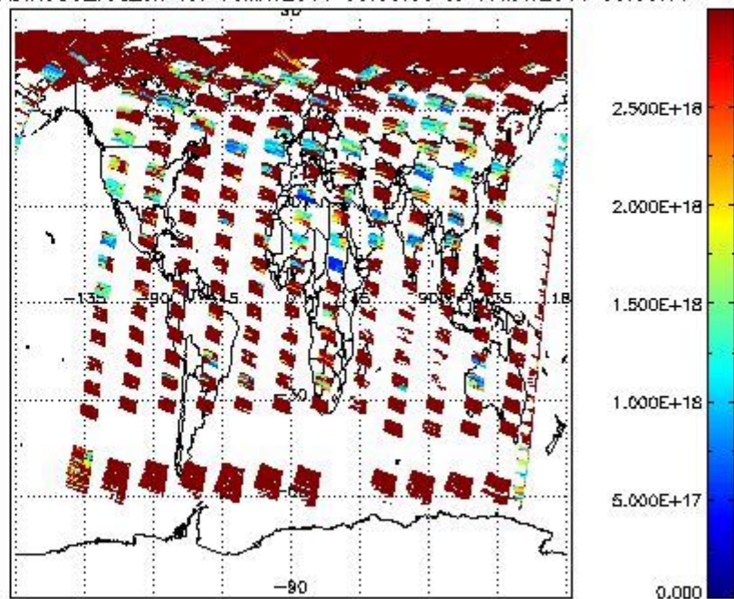
SCIDL2P_NADIR3CO_vcd_err for 16MAY2011 00:00:00 to 17MAY2011 00:00:00
