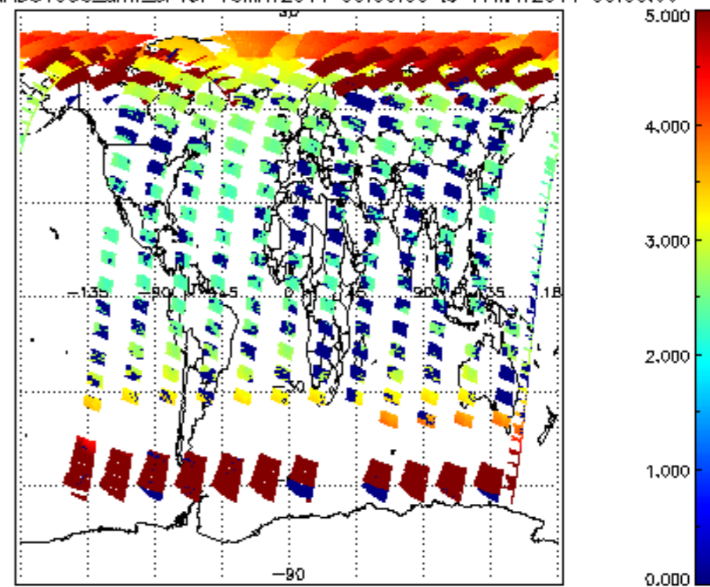
SCIOL2P_NADUV003_amf_cl for 16MAY2011 00:00:00 to 17MAY2011 00:00:00
