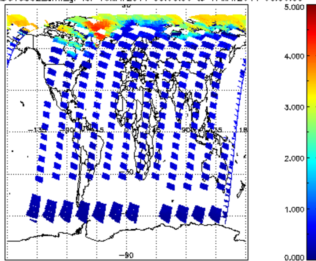
SCIOL2P_NADUV5S02_amf_gr for 16MAY2011 00:00:00 to 17MAY2011 00:00:00
