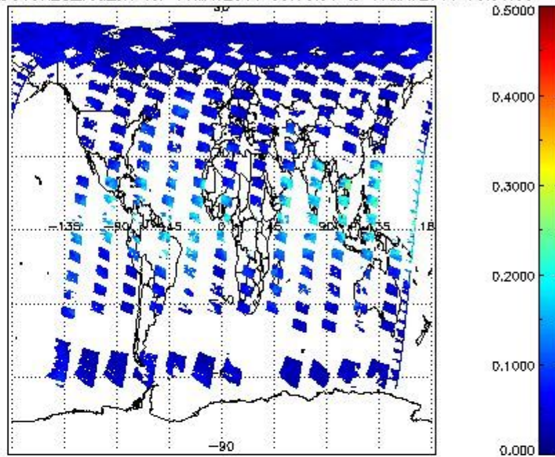
SCIOL2P_NADUV8H2O_vcd_err for 16MAY2011 00:00:00 to 17MAY2011 00:00:00
