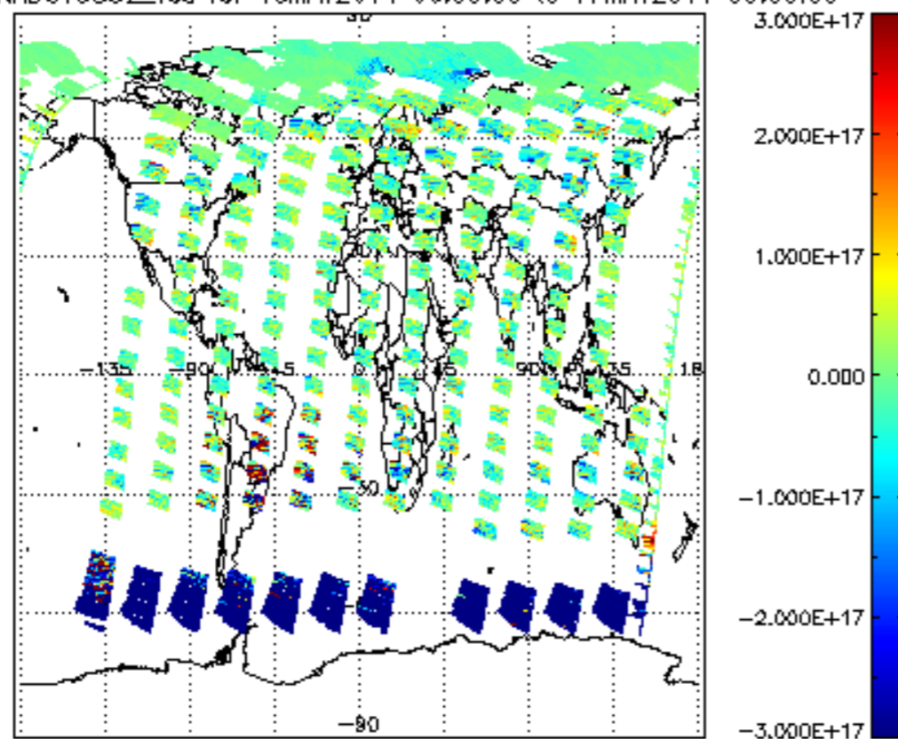
SCIOL2P_NADUV5S02_vcd for 16MAY2011 00:00:00 to 17MAY2011 00:00:00
