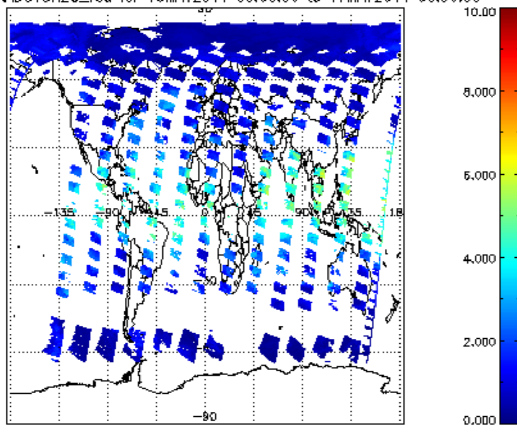
SCIOL2P_NADUV8H2O_vcd for 16MAY2011 00:00:00 to 17MAY2011 00:00:00
