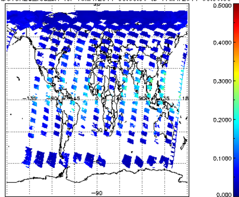
SCIOL2P_NADUV8H2O_vcd_err for 16MAY2011 00:00:00 to 17MAY2011 00:00:00
