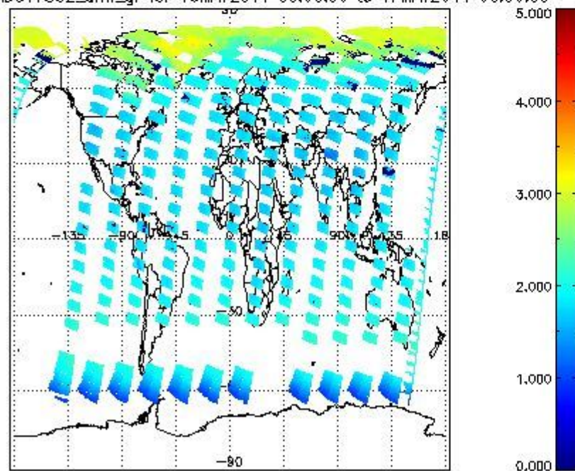
SCIOL2P_NADUV7S02_amf_gr for 16MAY2011 00:00:00 to 17MAY2011 00:00:00
