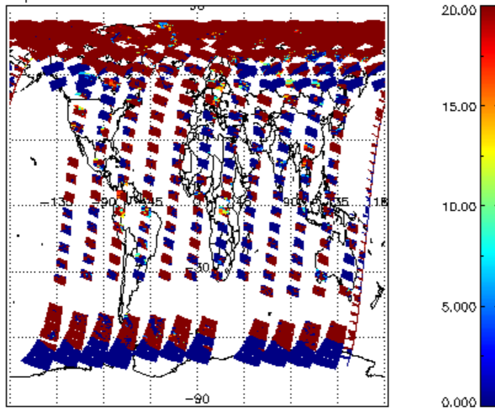
cl_opt_depth for 16MAY2011 00:00:00 to 17MAY2011 00:00:00
