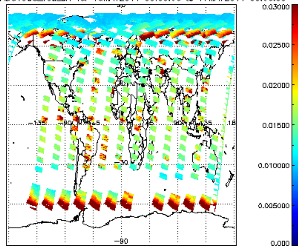
SCIOL2P_NADUV003_vcd_err for 16MAY2011 00:00:00 to 17MAY2011 00:00:00
