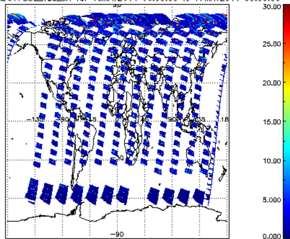
SCIOL2P_NADUV7S02_vcd_err for 16MAY2011 00:00:00 to 17MAY2011 00:00:00
