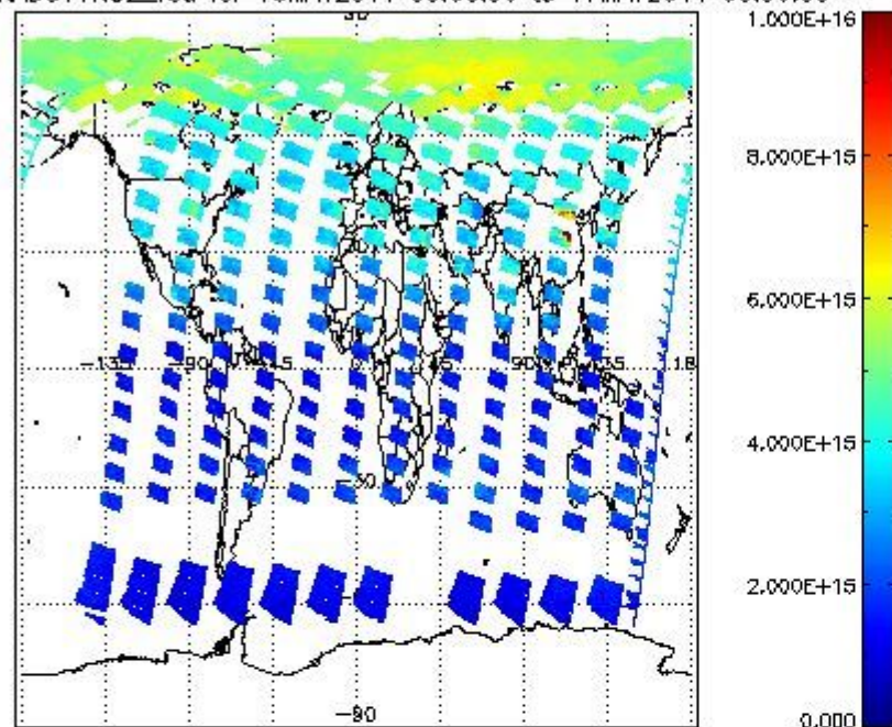
SCIOL2P_NADUV1NO2_vcd for 16MAY2011 00:00:00 to 17MAY2011 00:00:00
