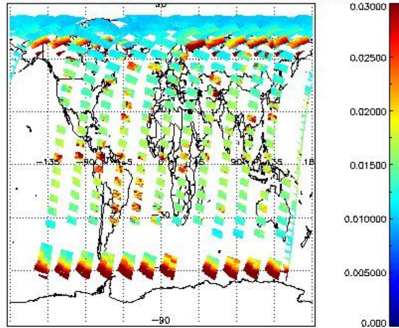
SCIOL2P_NADUV003_vcd_err for 16MAY2011 00:00:00 to 17MAY2011 00:00:00
