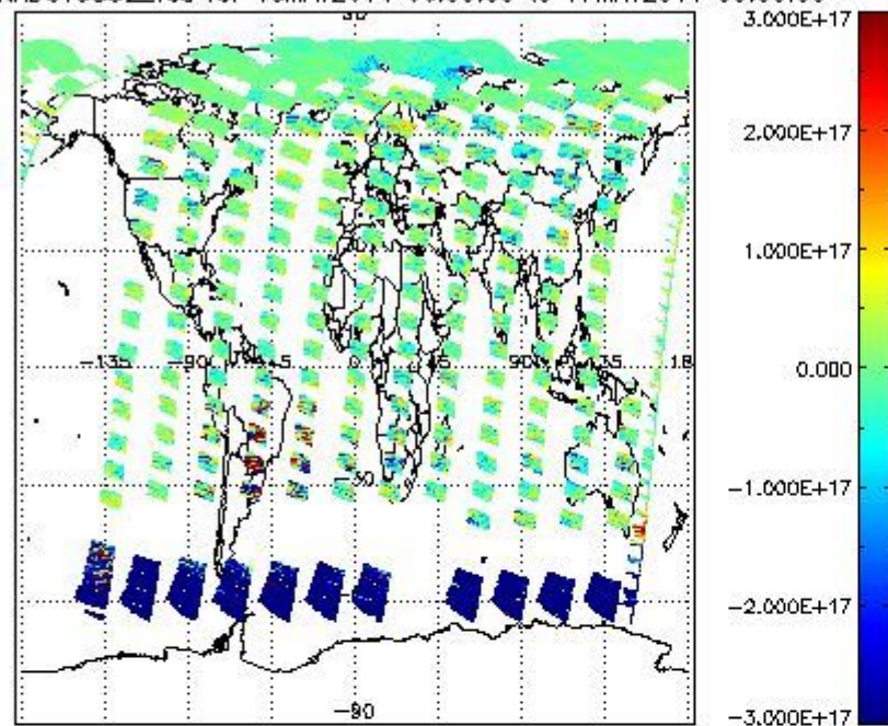
SCIOL2P_NADUV5S02_vcd for 16MAY2011 00:00:00 to 17MAY2011 00:00:00
