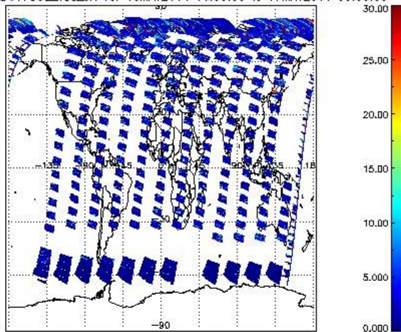
SCIOL2P_NADUV7S02_vcd_err for 16MAY2011 00:00:00 to 17MAY2011 00:00:00
