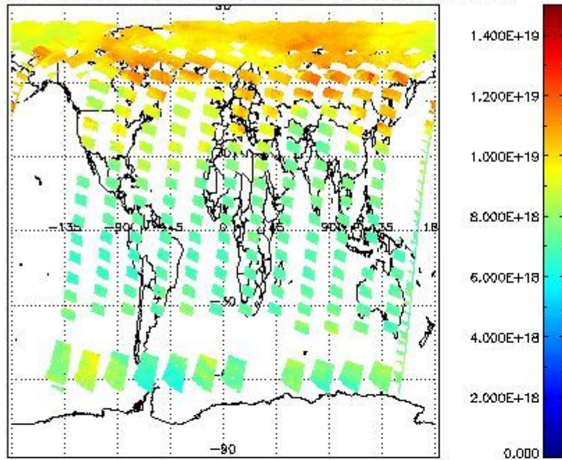
SCIOL2P_NADUV003_vcd for 16MAY2011 00:00:00 to 17MAY2011 00:00:00
