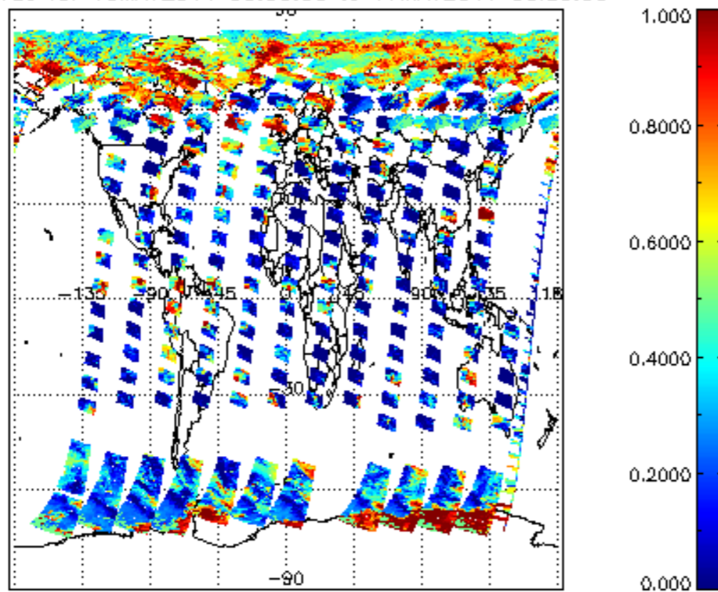
cl_frac for 16MAY2011 00:00:00 to 17MAY2011 00:00:00
