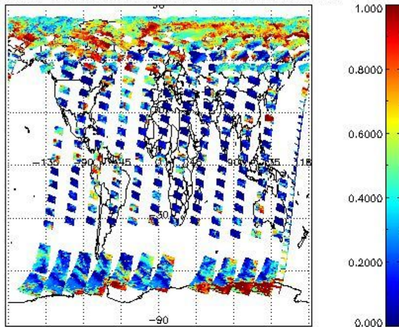
cL_frac for 16MAY2011 00:00:00 to 17MAY2011 00:00:00
