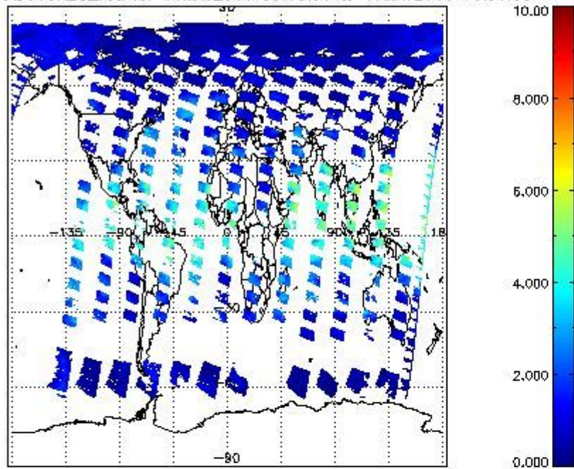
SCIOL2P_NADUV8H2O_vcd for 16MAY2011 00:00:00 to 17MAY2011 00:00:00
