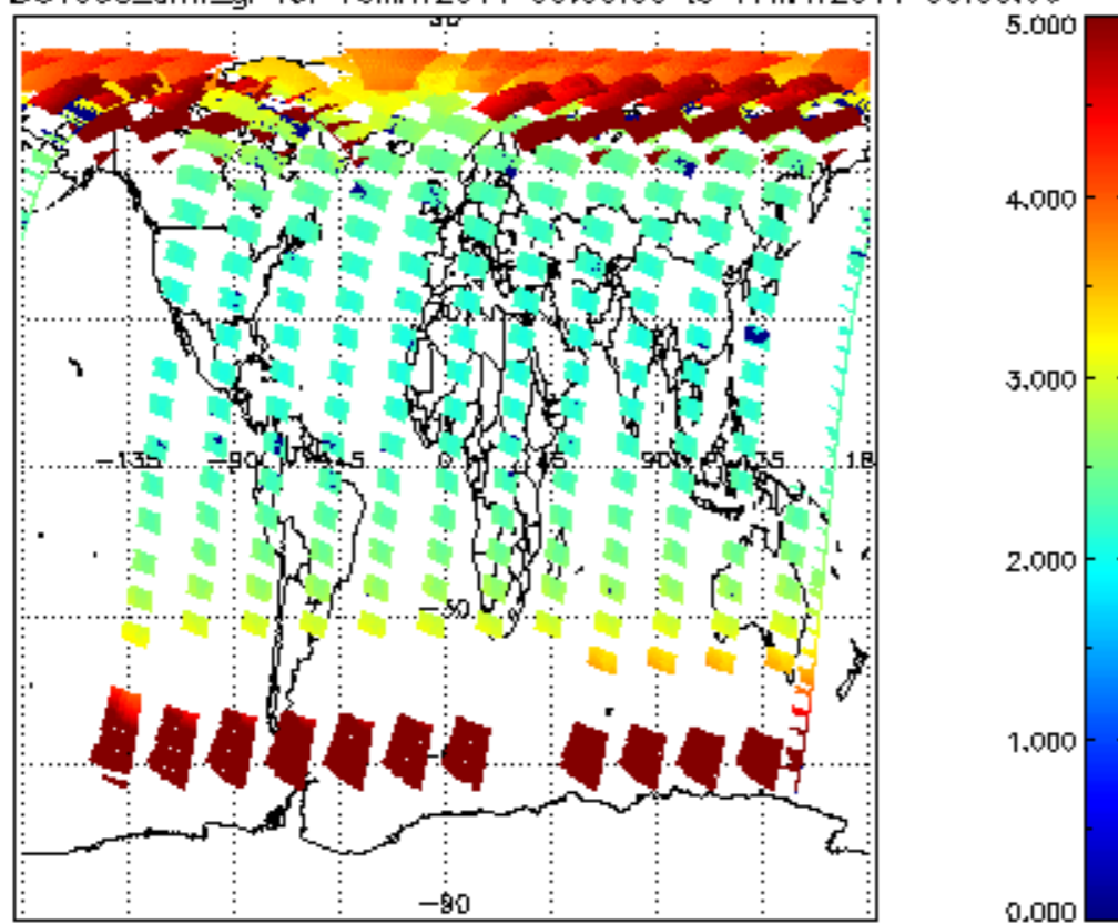
SCIOL2P_NADUV003_amf_gr for 16MAY2011 00:00:00 to 17MAY2011 00:00:00
