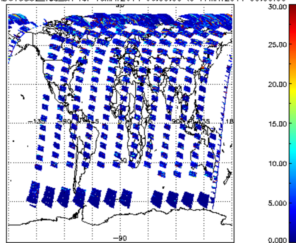
SCIOL2P_NADUV5S02_vcd_err for 16MAY2011 00:00:00 to 17MAY2011 00:00:00
