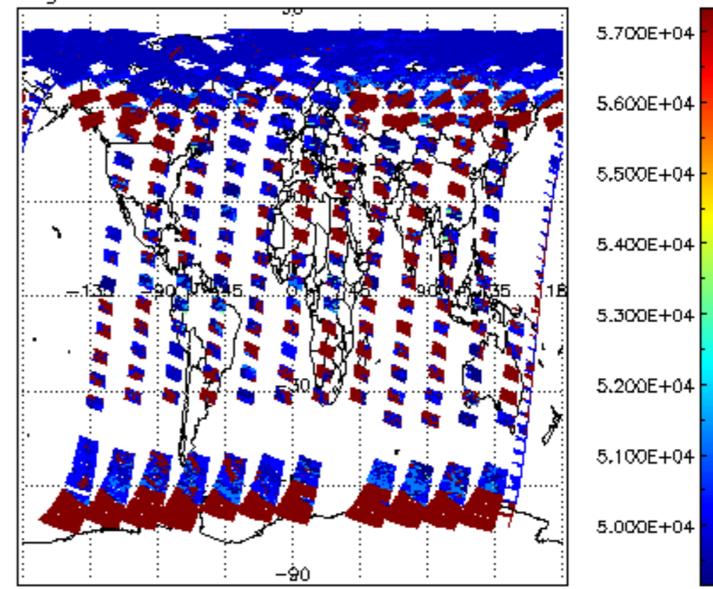
cloud_flags for 16MAY2011 00:00:00 to 17MAY2011 00:00:00
