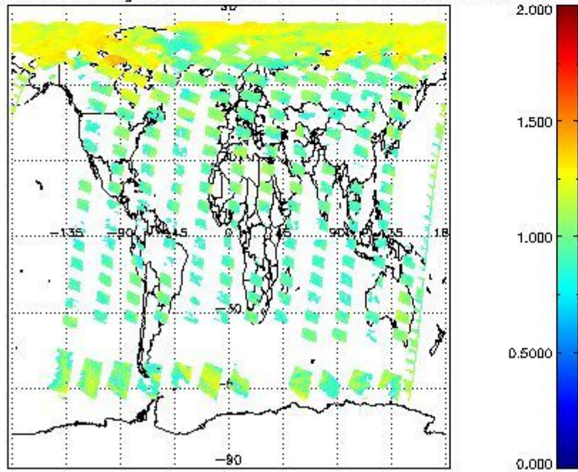
SCIOL2P_NADUV8H2O_arnf_gr for 16MAY2011 00:00:00 to 17MAY2011 00:00:00
