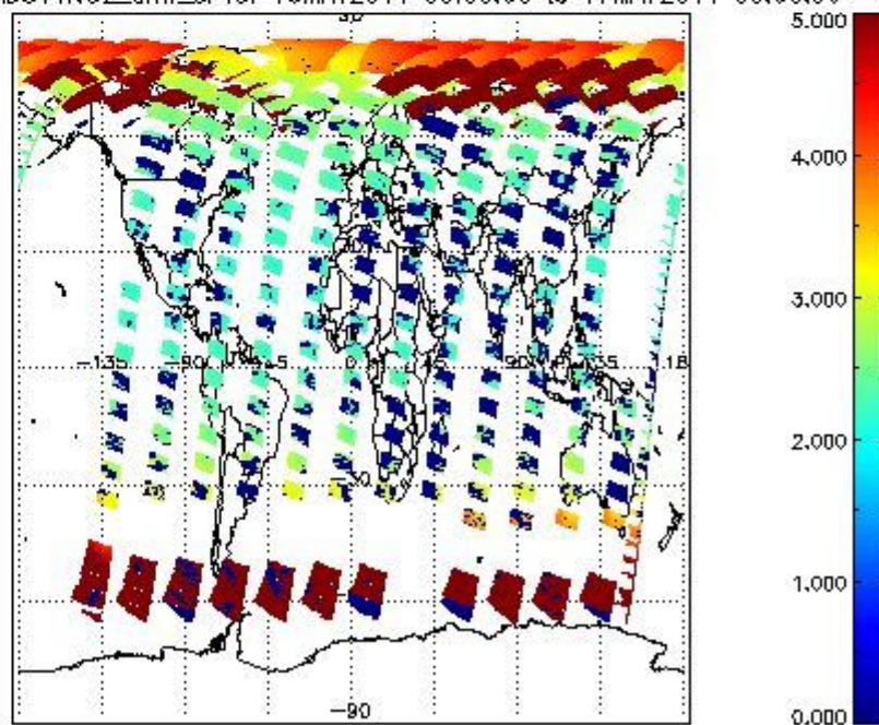
SCIOL2P_NADUV1NO2_amf_cl for 16MAY2011 00:00:00 to 17MAY2011 00:00:00
