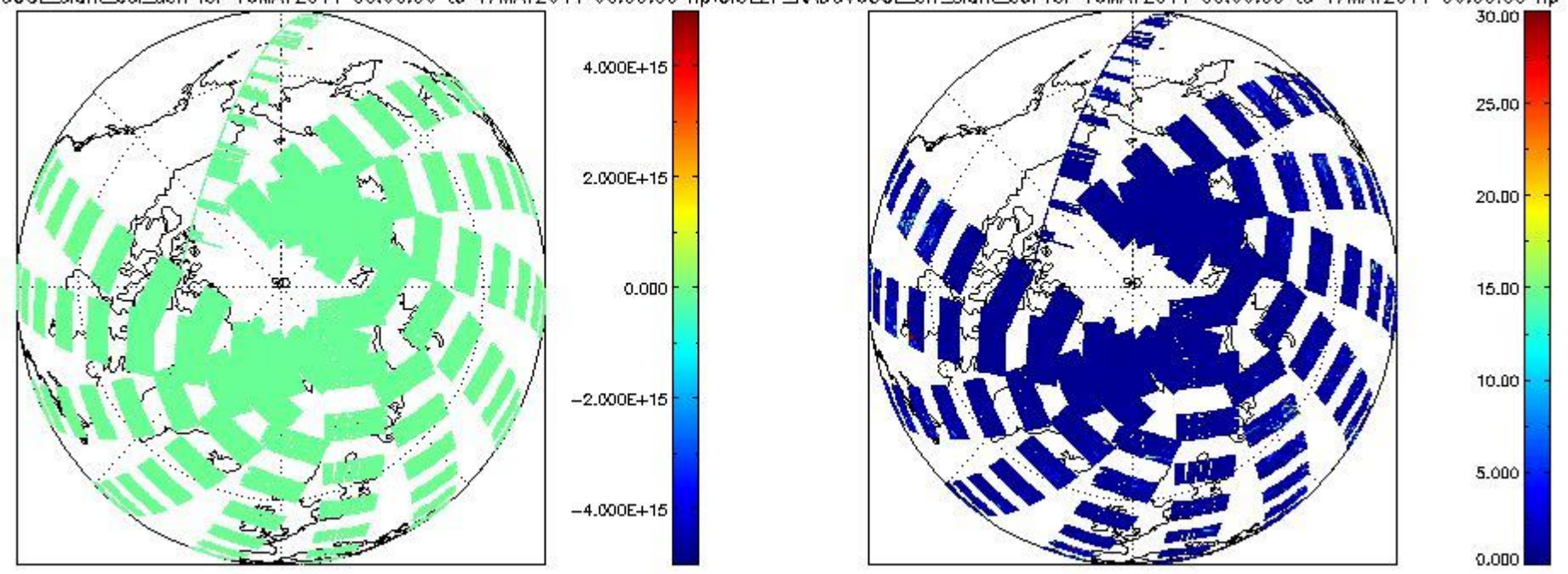
CIOL2P_NADUV60CLslant_col_den for 16MAY2011 00:00:00 to 17MAY2011 00:00:00 np CIOL2P_NADUV60CLerr_slant_col for 16MAY2011 00:00:00 to 17MAY2011 00:00:00 np
