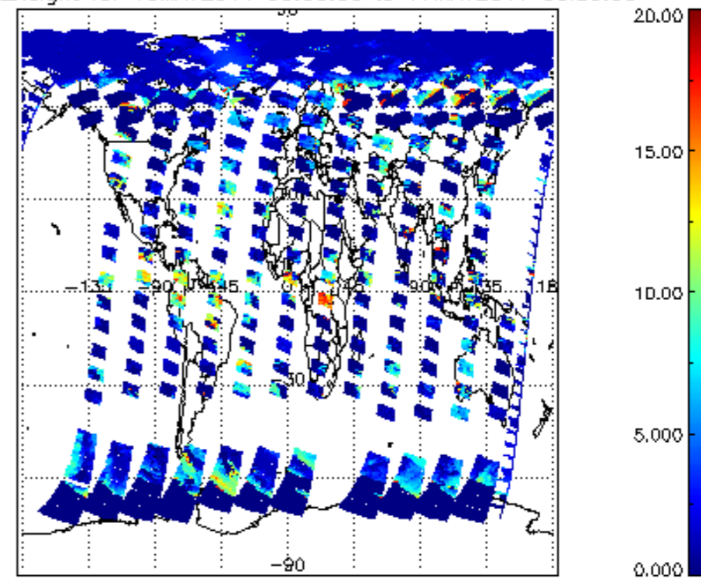
cl_top_height for 16MAY2011 00:00:00 to 17MAY2011 00:00:00
