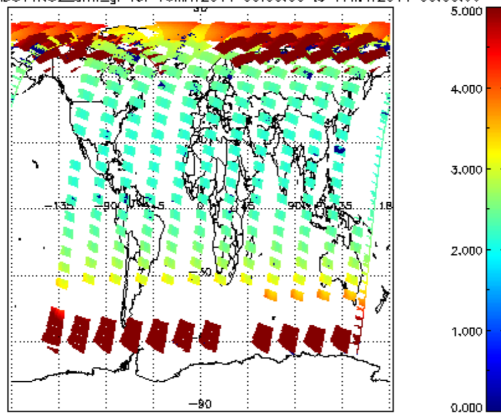
SCIOL2P_NADUV1NO2_amf_gr for 16MAY2011 00:00:00 to 17MAY2011 00:00:00
