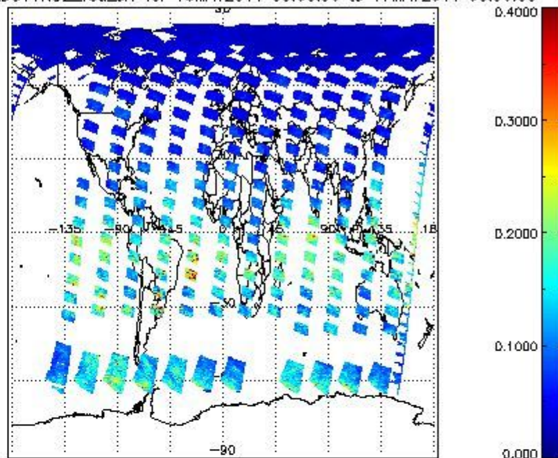
SCIOL2P_NADUV1NO2_vcd_err for 16MAY2011 00:00:00 to 17MAY2011 00:00:00
