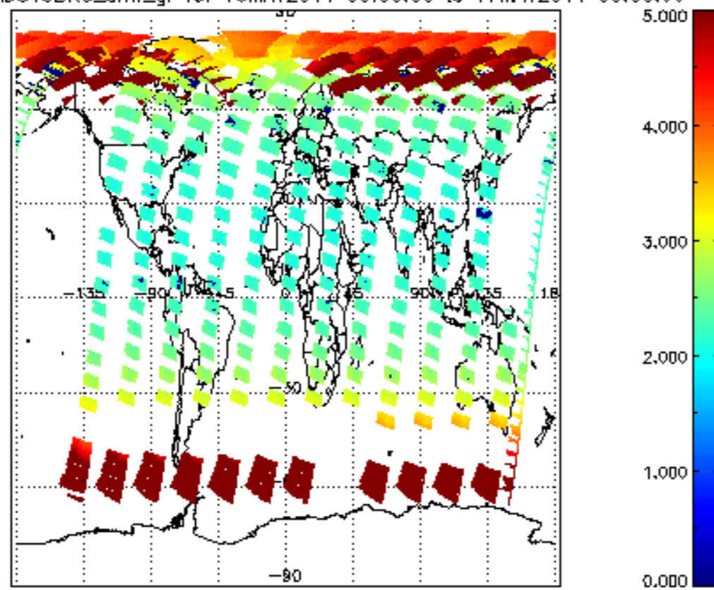
SCIOL2P_NADUV3BRO_amf_gr for 16MAY2011 00:00:00 to 17MAY2011 00:00:00
