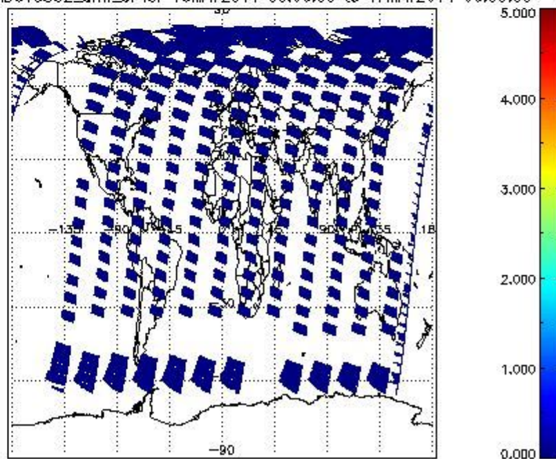
SCIOL2P_NADUV5S02_amf_cl for 16MAY2011 00:00:00 to 17MAY2011 00:00:00
