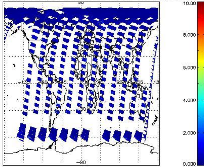
SCIOL2P_NADUV3BRO_vcd_err for 16MAY2011 00:00:00 to 17MAY2011 00:00:00
