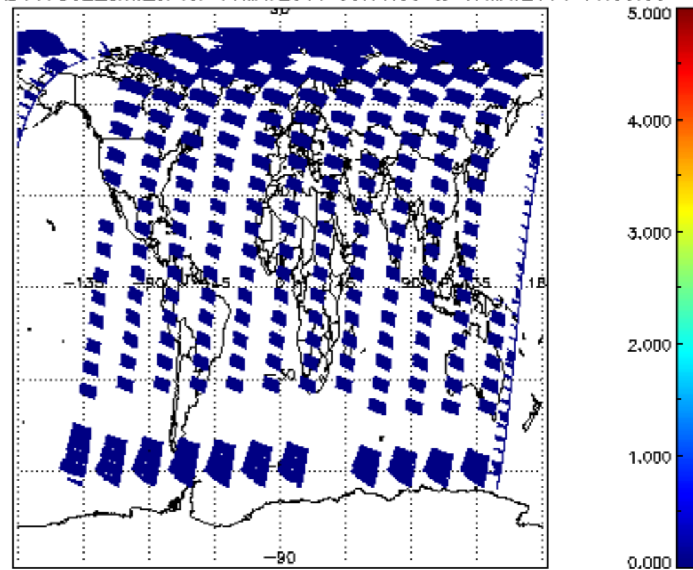
SCIOL2P_NADUV7S02_amf_cl for 16MAY2011 00:00:00 to 17MAY2011 00:00:00
