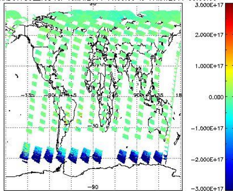
SCIOL2P_NADUV7S02_vcd for 16MAY2011 00:00:00 to 17MAY2011 00:00:00
