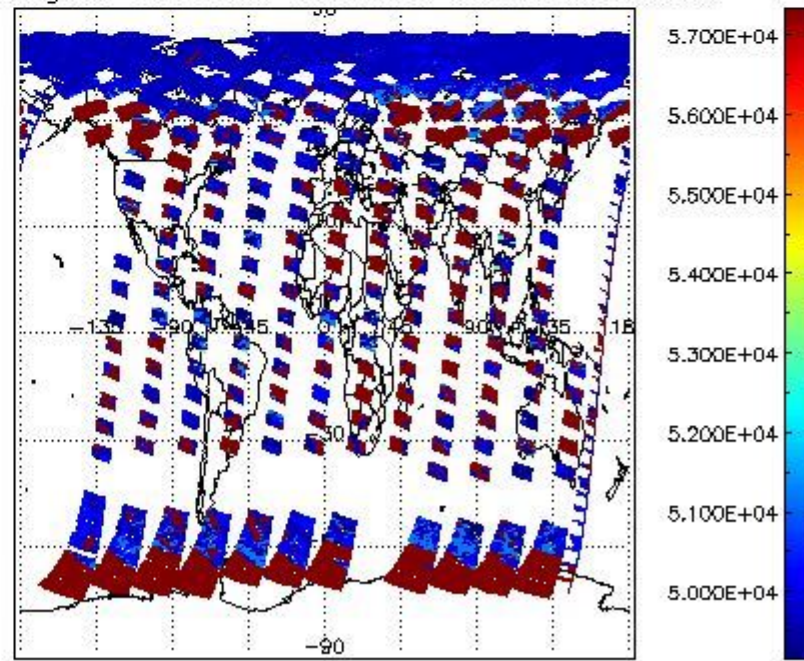
cloud_flags for 16MAY2011 00:00:00 to 17MAY2011 00:00:00
