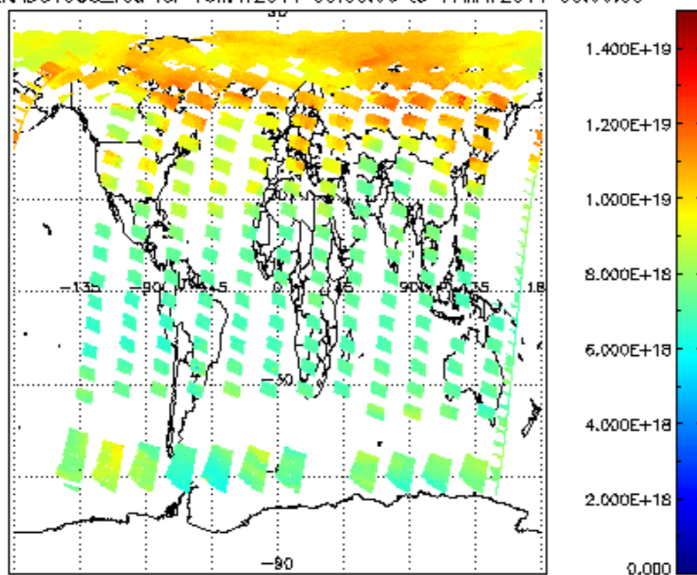
SCIOL2P_NADUV003_vcd for 16MAY2011 00:00:00 to 17MAY2011 00:00:00
