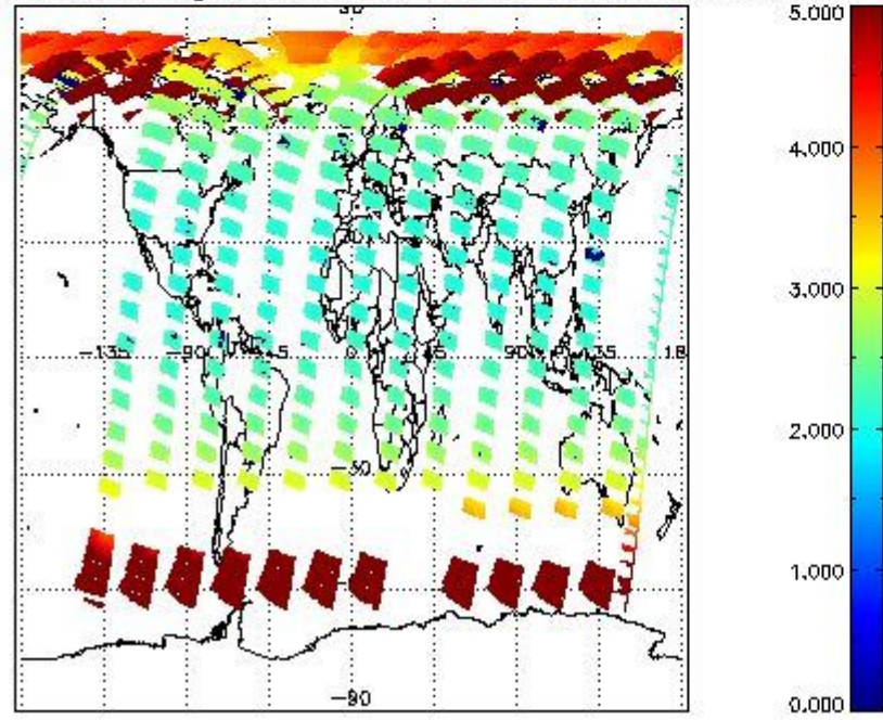
SCIOL2P_NADUV3BRO_amf_gr for 16MAY2011 00:00:00 to 17MAY2011 00:00:00
