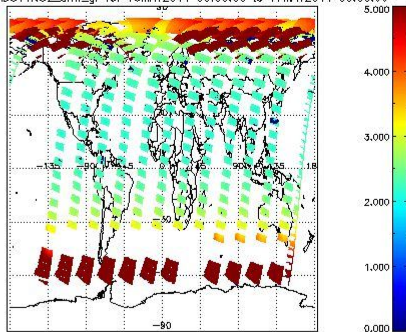
SCIOL2P_NADUV1NO2_amf_gr for 16MAY2011 00:00:00 to 17MAY2011 00:00:00
