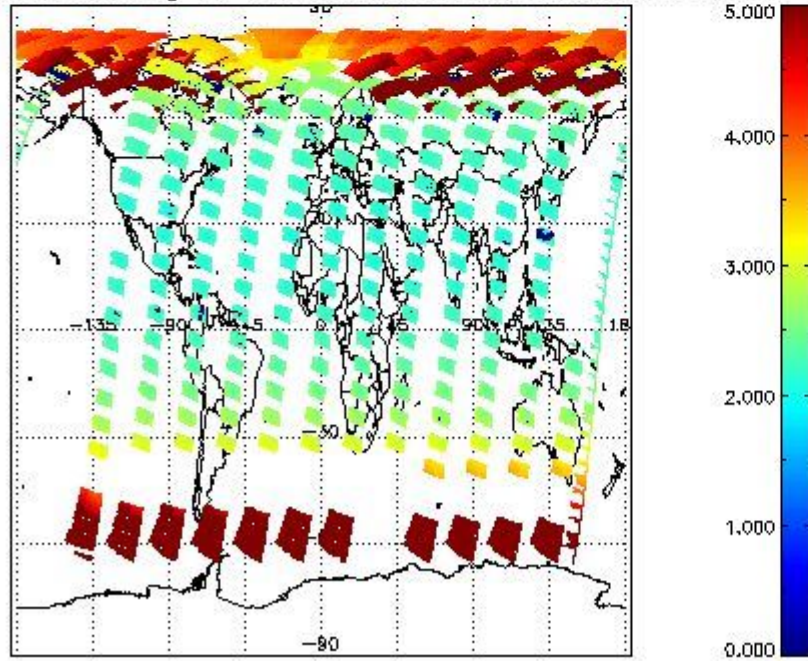
SCIOL2P_NADUV003_amf_gr for 16MAY2011 00:00:00 to 17MAY2011 00:00:00
