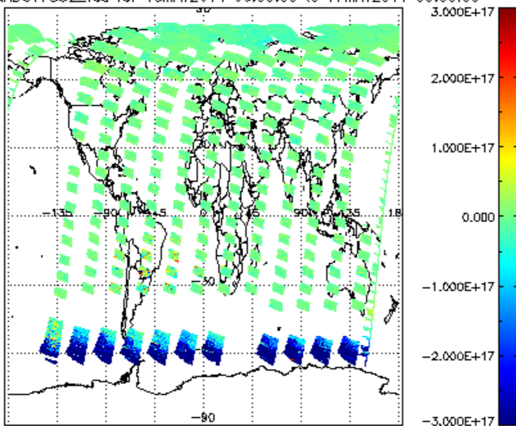
SCIOL2P_NADUV7S02_vcd for 16MAY2011 00:00:00 to 17MAY2011 00:00:00
