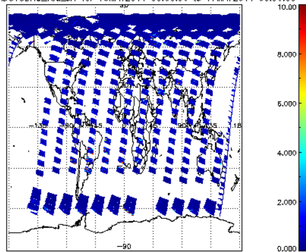
SCIOL2P_NADUV3BRO_vcd_err for 16MAY2011 00:00:00 to 17MAY2011 00:00:00
