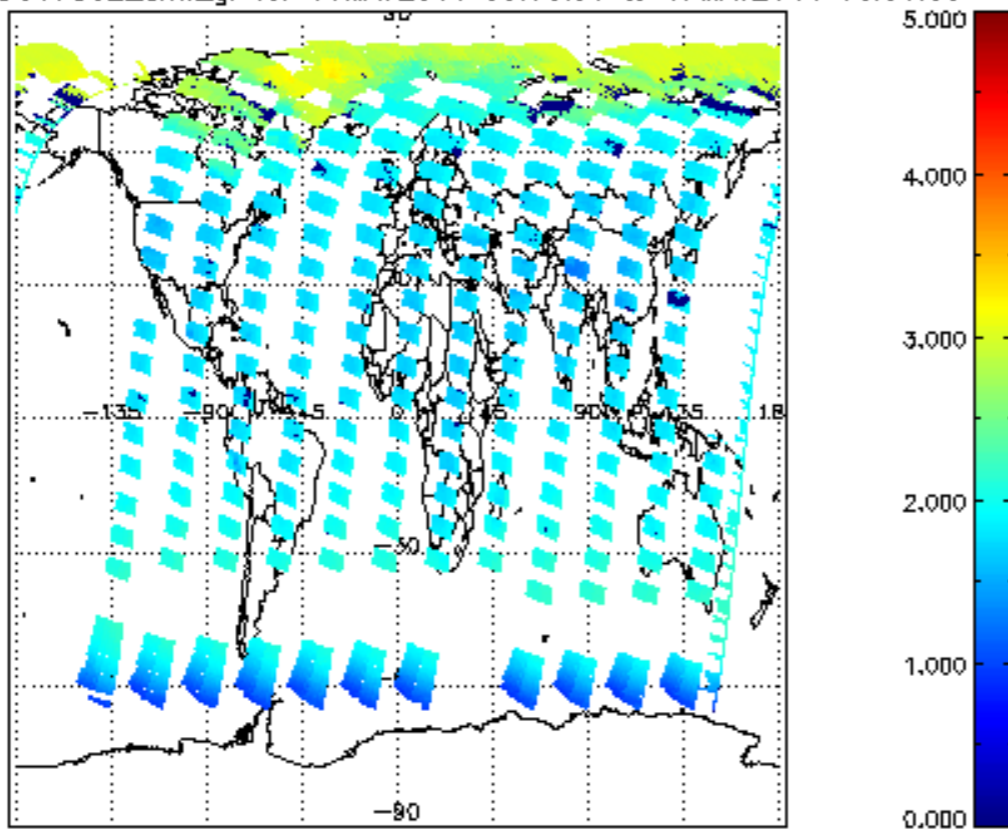
SCIOL2P_NADUV7S02_amf_gr for 16MAY2011 00:00:00 to 17MAY2011 00:00:00
