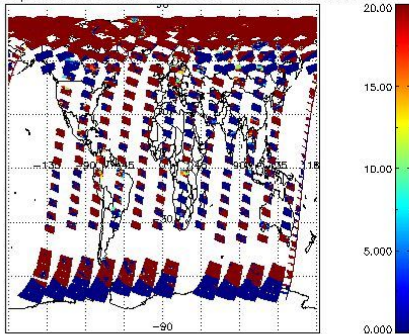
cL_opt_depth for 16MAY2011 00:00:00 to 17MAY2011 00:00:00
