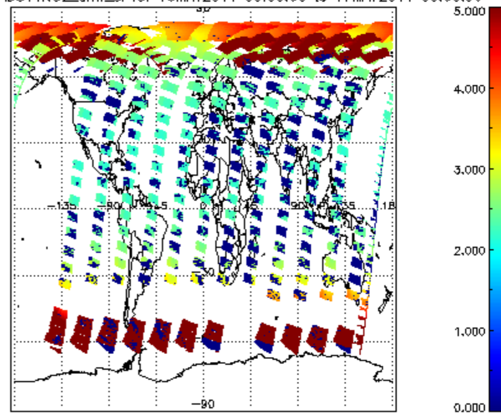
SCIOL2P_NADUV1NO2_amf_sl for 16MAY2011 00:00:00 to 17MAY2011 00:00:00
