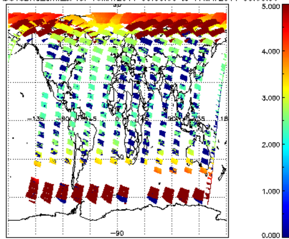
SCIOL2P_NADUV3BRO_amf_sl for 16MAY2011 00:00:00 to 17MAY2011 00:00:00
