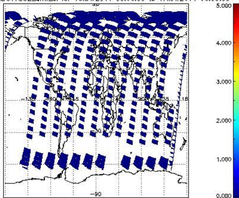
SCIOL2P_NADUV7S02_amf_cl for 16MAY2011 00:00:00 to 17MAY2011 00:00:00
