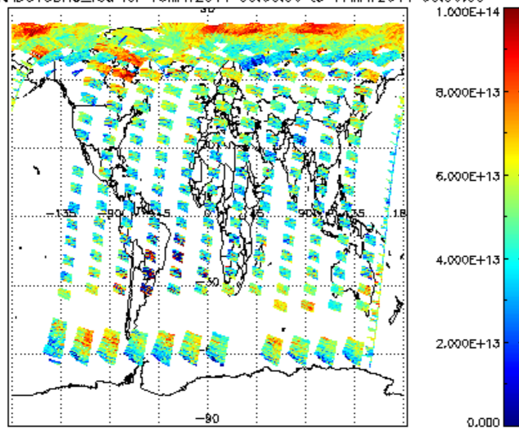
SCIOL2P_NADUV3BRO_vcd for 16MAY2011 00:00:00 to 17MAY2011 00:00:00
