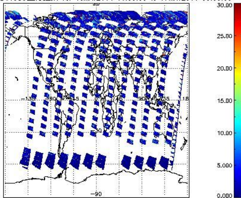
SCIOL2P_NADUV5S02_vcd_err for 16MAY2011 00:00:00 to 17MAY2011 00:00:00
