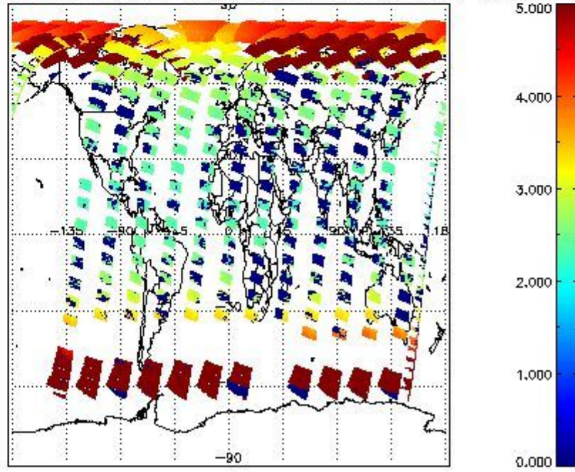
SCIOL2P_NADUV3BRO_amf_cl for 16MAY2011 00:00:00 to 17MAY2011 00:00:00
