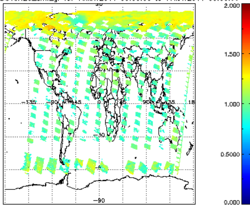
SCIOL2P_NADUV8H2O_amf_gr for 16MAY2011 00:00:00 to 17MAY2011 00:00:00
