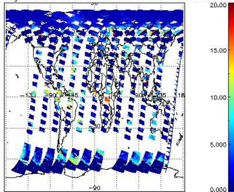
cL_top_height for 16MAY2011 00:00:00 to 17MAY2011 00:00:00
