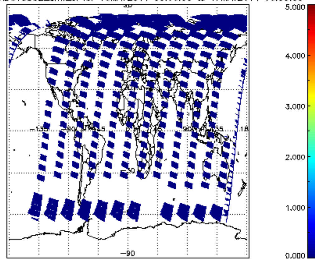
SCIOL2P_NADUV5S02_amf_cl for 16MAY2011 00:00:00 to 17MAY2011 00:00:00
