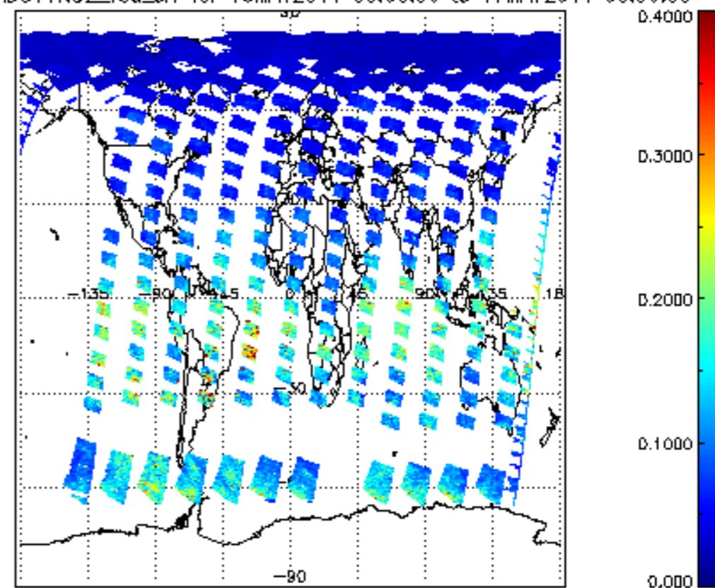
SCIOL2P_NADUV1NO2_vcd_err for 16MAY2011 00:00:00 to 17MAY2011 00:00:00
