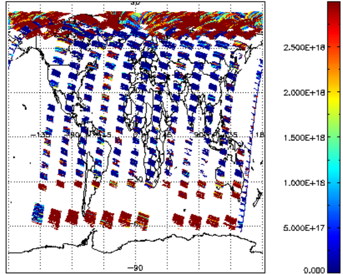
SCIOL2P_NADIR3CO_vcd for 16MAY2011 00:00:00 to 17MAY2011 00:00:00
