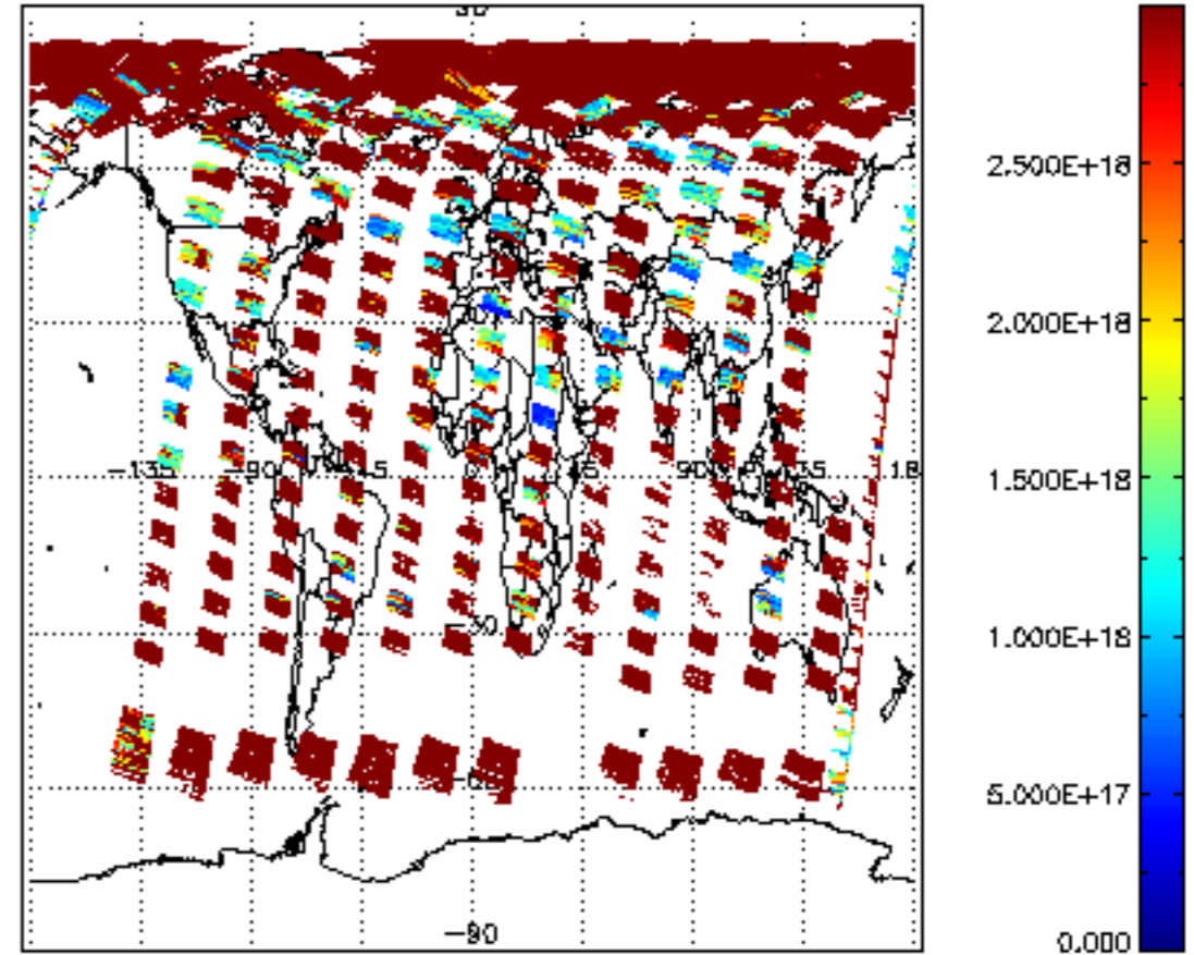
SCIOL2P_NADIR3CO_vcd_err for 16MAY2011 00:00:00 to 17MAY2011 00:00:00
