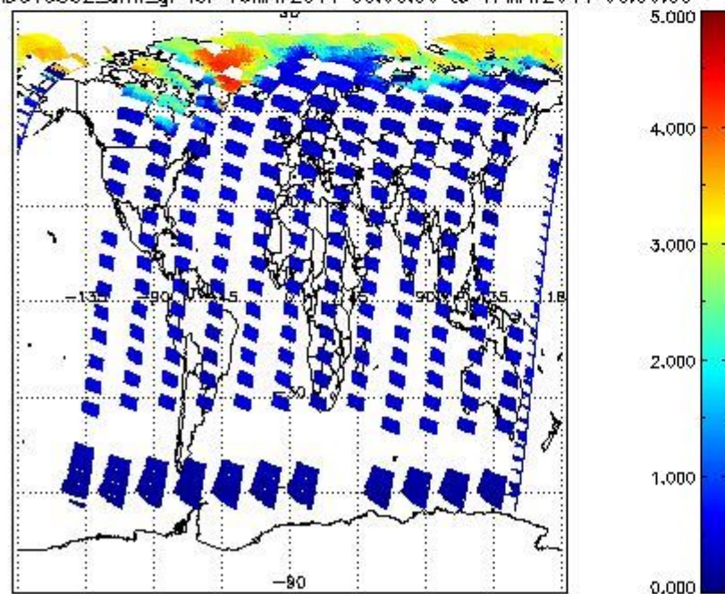
SCIOL2P_NADUV5S02_amf_gr for 16MAY2011 00:00:00 to 17MAY2011 00:00:00
