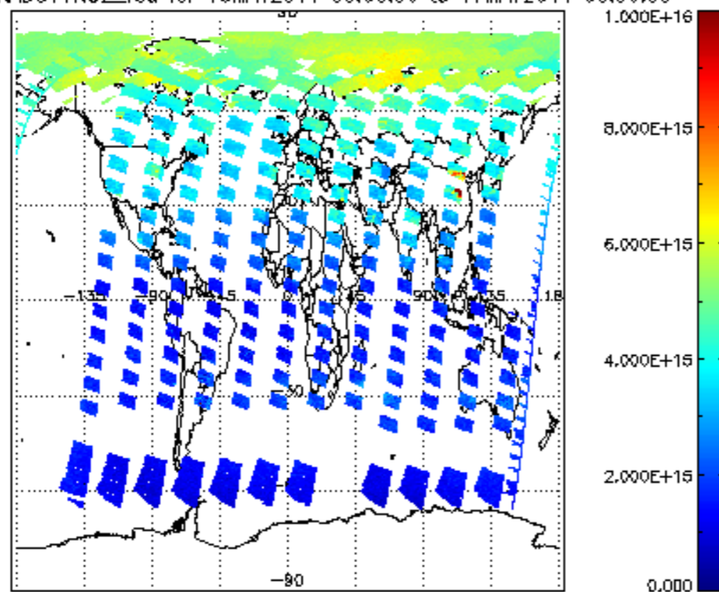
SCIOL2P_NADUV1NO2_vcd for 16MAY2011 00:00:00 to 17MAY2011 00:00:00
