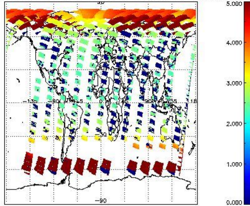
SCIOL2P_NADUV003_amf_cl for 16MAY2011 00:00:00 to 17MAY2011 00:00:00
