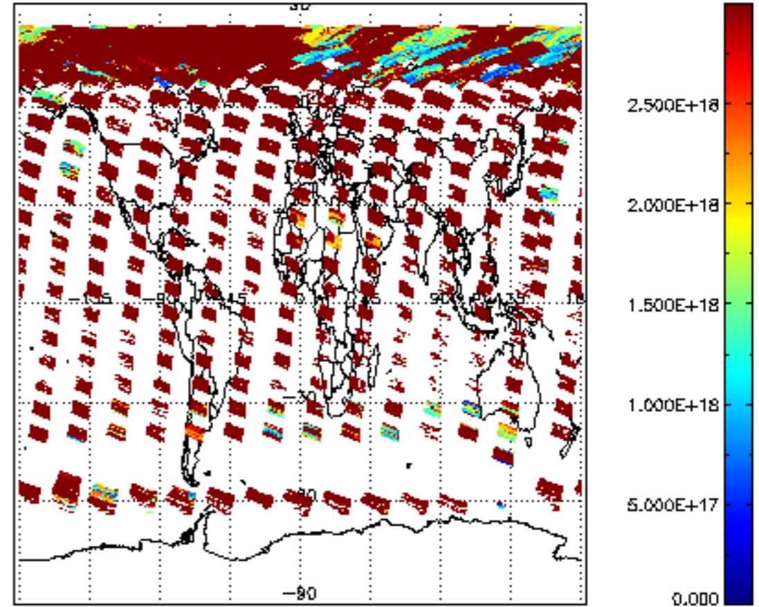
SCIOL2P_NADIR3CO_vcd_err for 15MAY2011 00:00:00 to 16MAY2011 00:00:00
