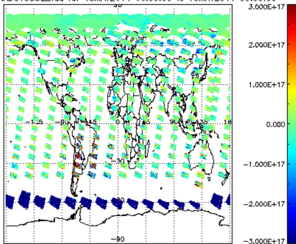
SCIOL2P_NADUV5S02_vcd for 15MAY2011 00:00:00 to 16MAY2011 00:00:00
