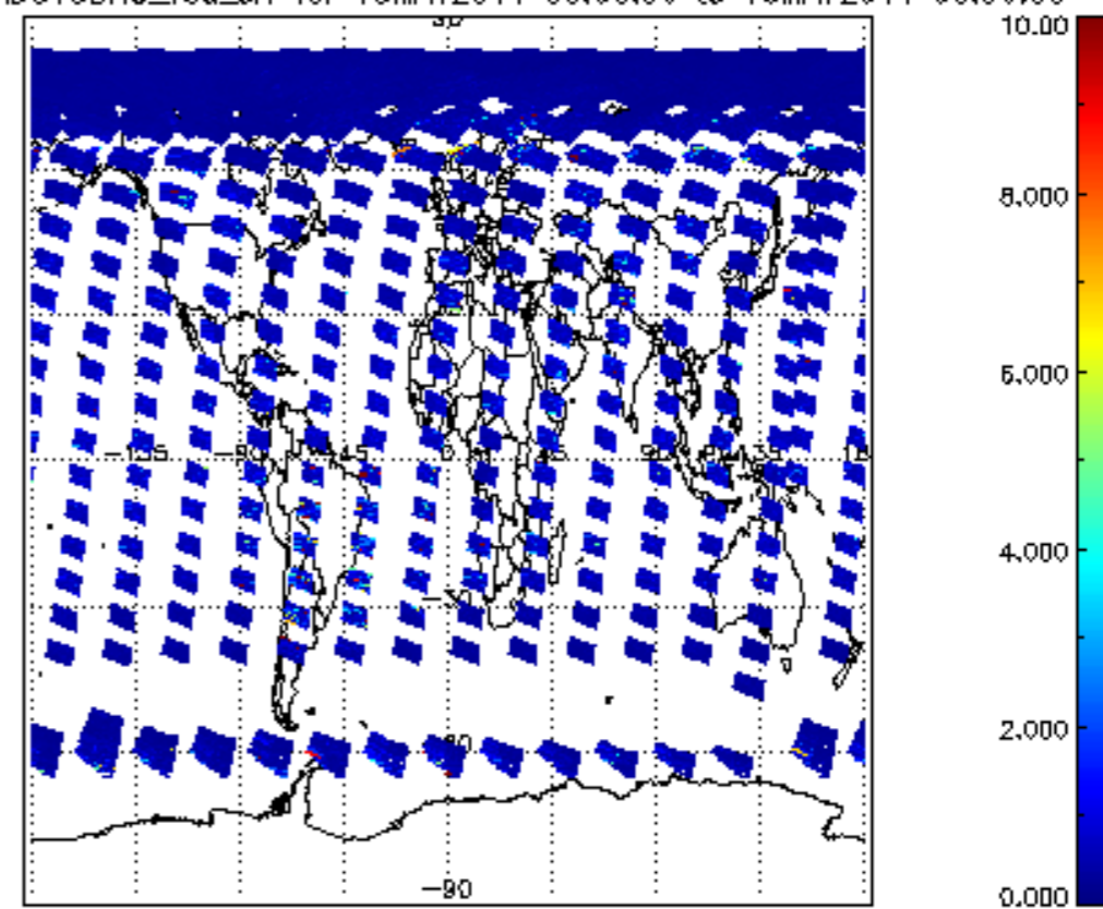
SCIOL2P_NADUV3BRO_vcd_err for 15MAY2011 00:00:00 to 16MAY2011 00:00:00
