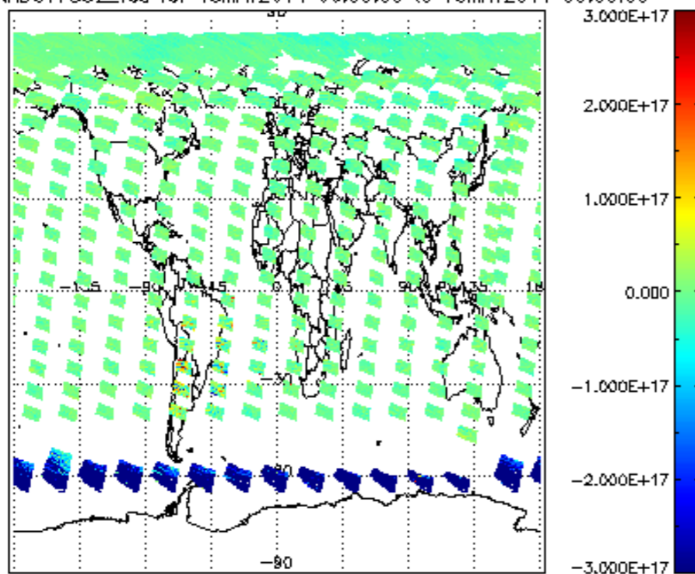
SCIOL2P_NADUV7S02_vcd for 15MAY2011 00:00:00 to 16MAY2011 00:00:00
