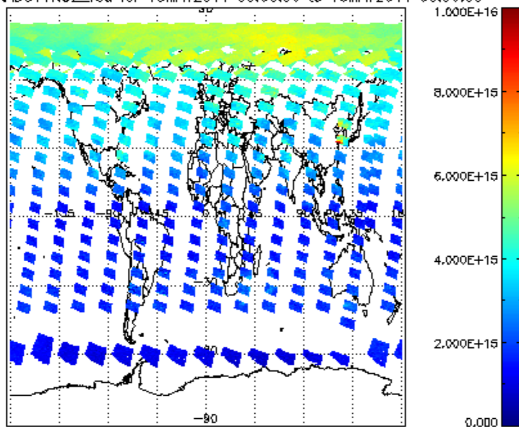
SCIOL2P_NADUV1NO2_vcd for 15MAY2011 00:00:00 to 16MAY2011 00:00:00
