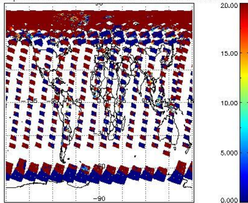
cL_opt_depth for 15MAY2011 00:00:00 to 16MAY2011 00:00:00
