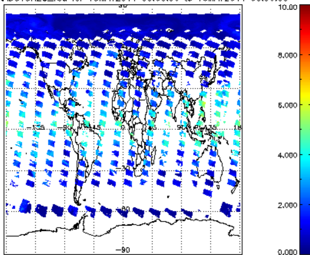
SCIOL2P_NADUV8H2O_vcd for 15MAY2011 00:00:00 to 16MAY2011 00:00:00
