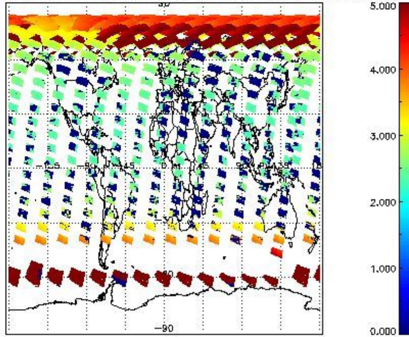
SCIOL2P_NADUV003_amf_cl for 15MAY2011 00:00:00 to 16MAY2011 00:00:00
