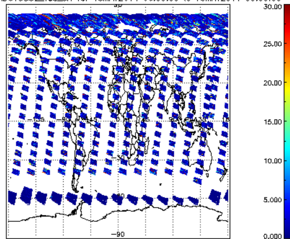
SCIOL2P_NADUV5S02_vcd_err for 15MAY2011 00:00:00 to 16MAY2011 00:00:00
