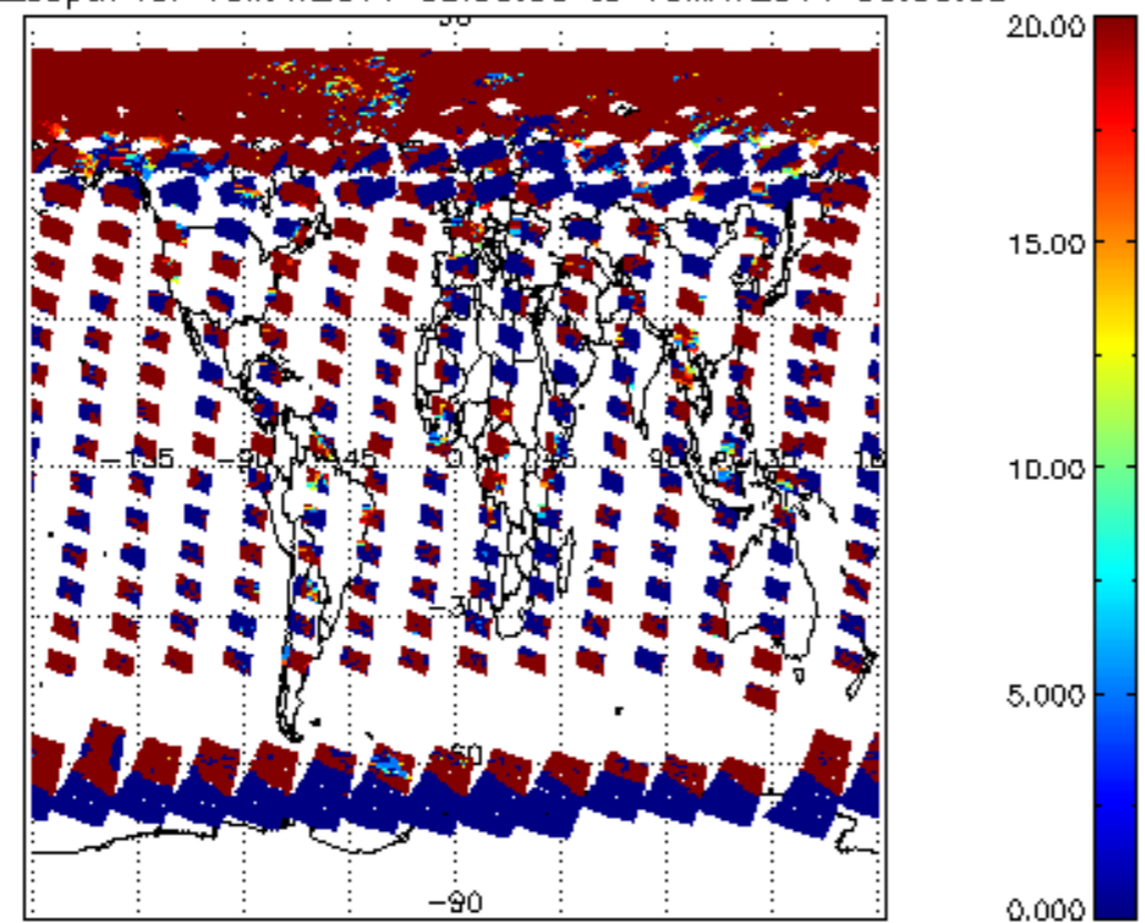
cl_opt_depth for 15MAY2011 00:00:00 to 16MAY2011 00:00:00
