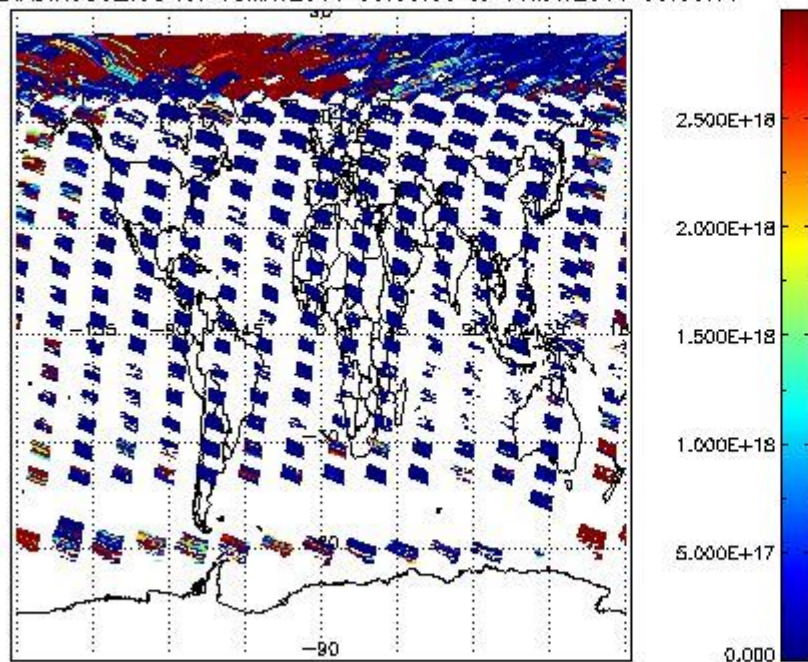
SCIDL2P_NADIR3CO_vcd for 15MAY2011 00:00:00 to 16MAY2011 00:00:00
