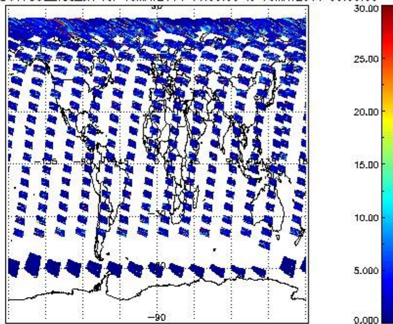
SCIOL2P_NADUV7S02_vcd_err for 15MAY2011 00:00:00 to 16MAY2011 00:00:00
