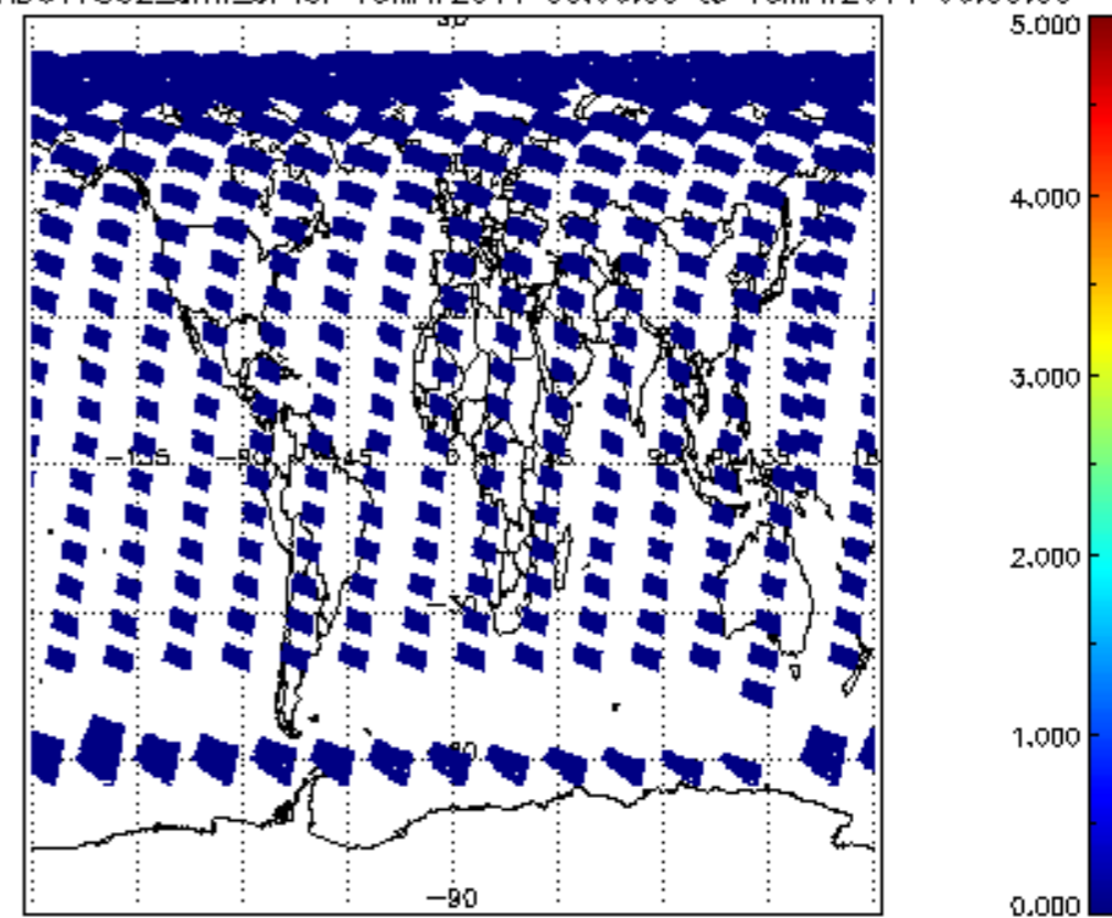
SCIOL2P_NADUV7S02_amf_cl for 15MAY2011 00:00:00 to 16MAY2011 00:00:00
