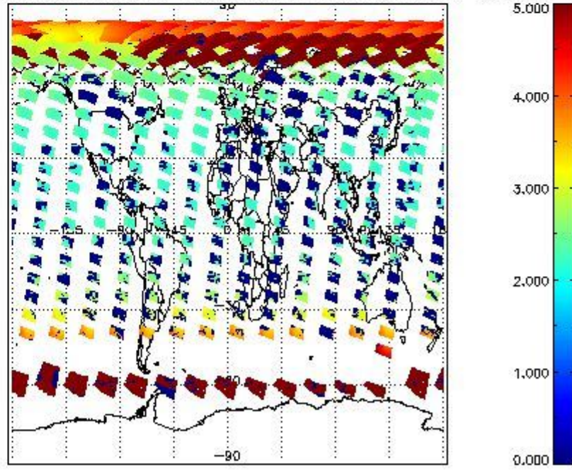
SCIOL2P_NADUV1NO2_amf_cl for 15MAY2011 00:00:00 to 16MAY2011 00:00:00
