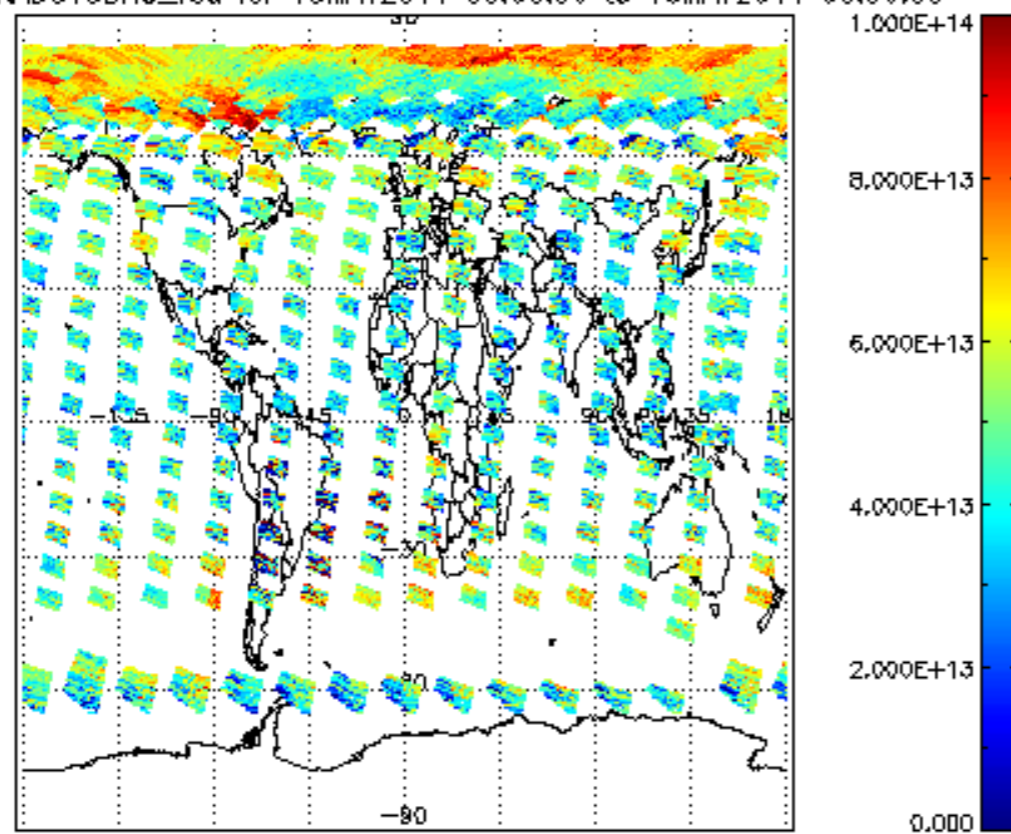
SCIOL2P_NADUV3BRO_vcd for 15MAY2011 00:00:00 to 16MAY2011 00:00:00
