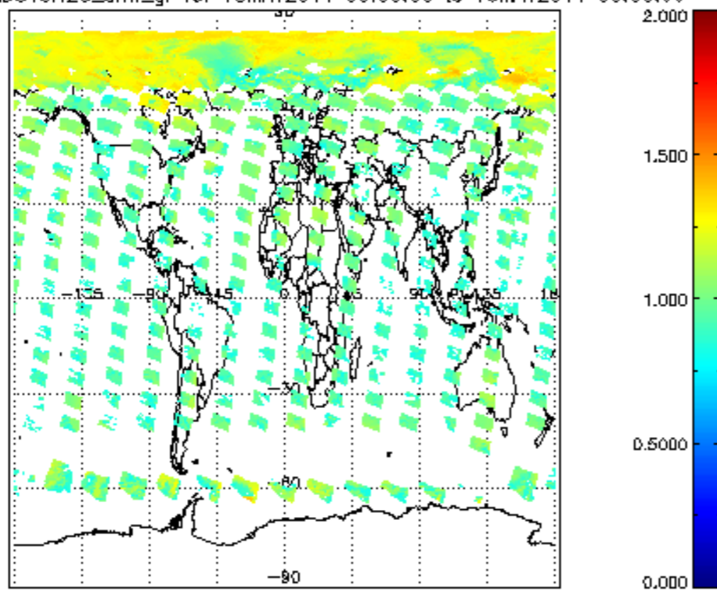
SCIOL2P_NADUV8H2O_amf_gr for 15MAY2011 00:00:00 to 16MAY2011 00:00:00
