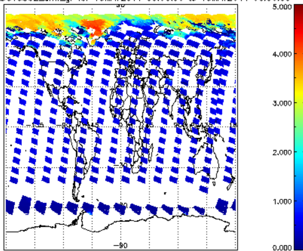
SCIOL2P_NADUV5S02_amf_gr for 15MAY2011 00:00:00 to 16MAY2011 00:00:00
