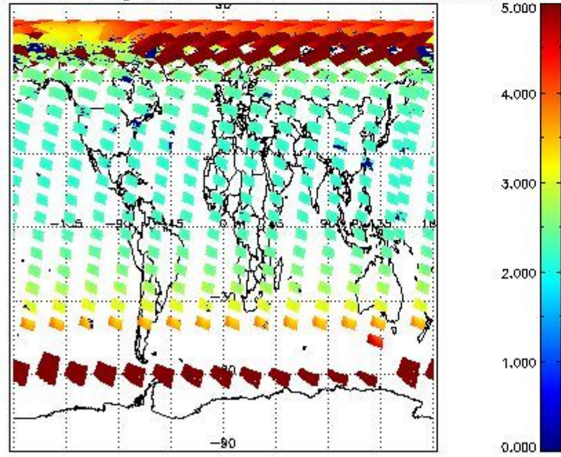
SCIOL2P_NADUV1NO2_amf_gr for 15MAY2011 00:00:00 to 16MAY2011 00:00:00
