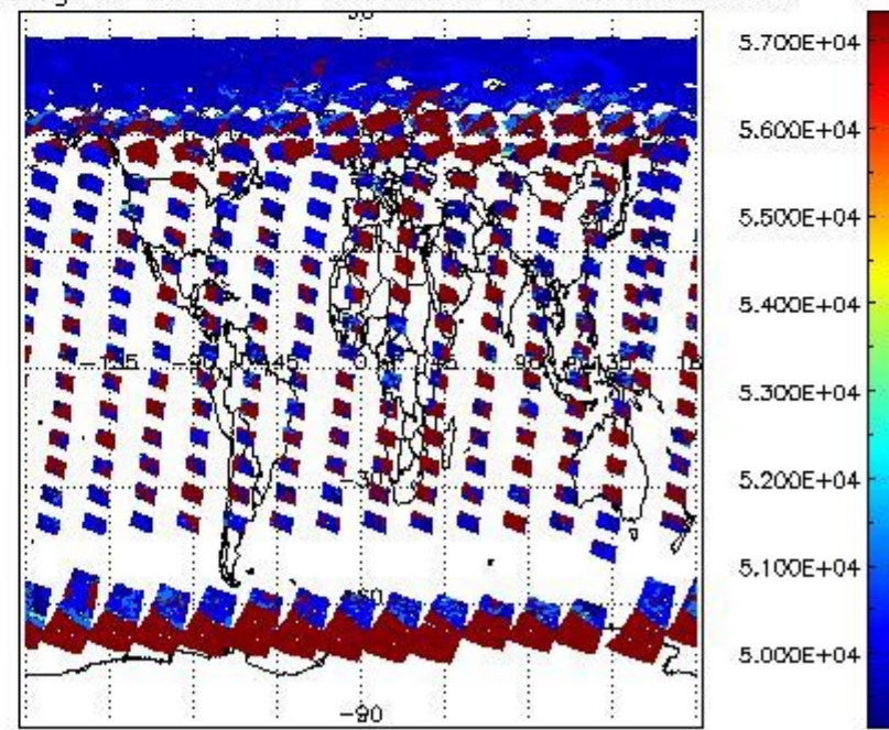
cloud_flags for 15MAY2011 00:00:00 to 16MAY2011 00:00:00
