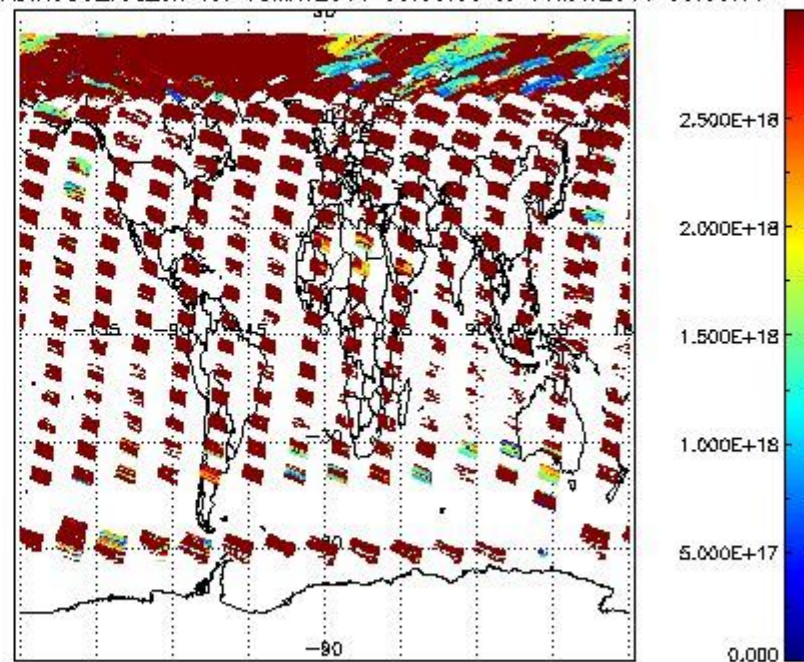
SCIDL2P_NADIR3CO_vcd_err for 15MAY2011 00:00:00 to 16MAY2011 00:00:00
