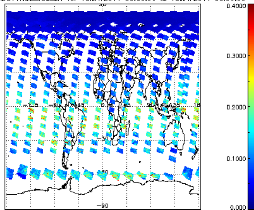
SCIOL2P_NADUV1NO2_vcd_err for 15MAY2011 00:00:00 to 16MAY2011 00:00:00
