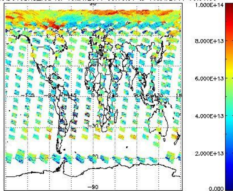
SCIOL2P_NADUV3BRO_vcd for 15MAY2011 00:00:00 to 16MAY2011 00:00:00
