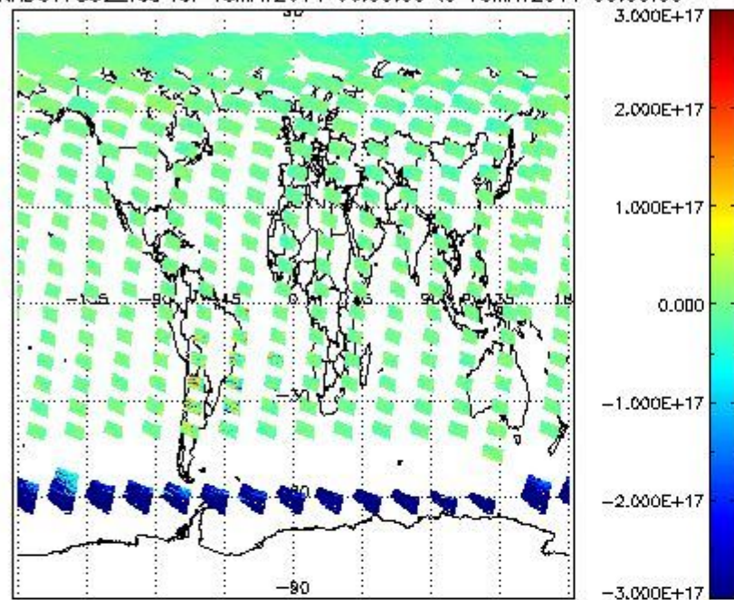
SCIOL2P_NADUV7S02_vcd for 15MAY2011 00:00:00 to 16MAY2011 00:00:00
