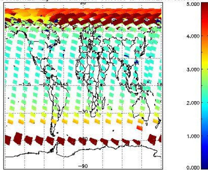
SCIOL2P_NADUV3BRO_amf_gr for 15MAY2011 00:00:00 to 16MAY2011 00:00:00
