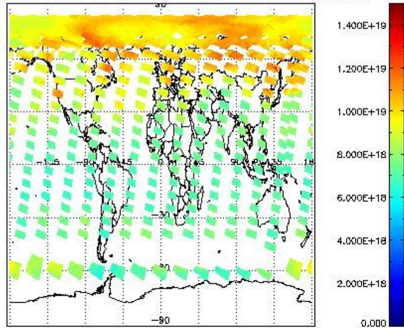
SCIOL2P_NADUV003_vcd for 15MAY2011 00:00:00 to 16MAY2011 00:00:00
