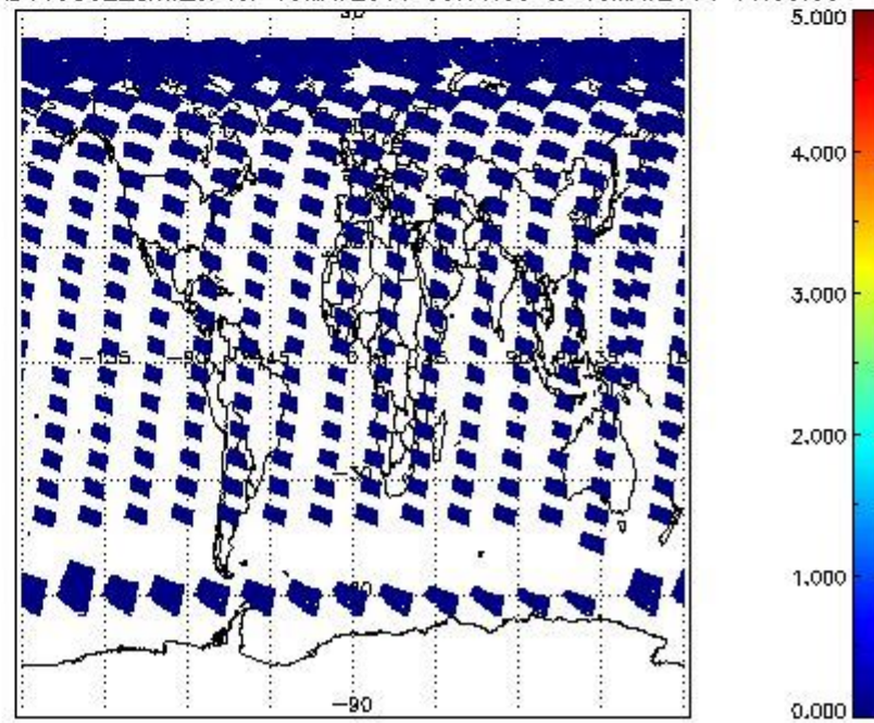
SCIOL2P_NADUV5S02_amf_cl for 15MAY2011 00:00:00 to 16MAY2011 00:00:00
