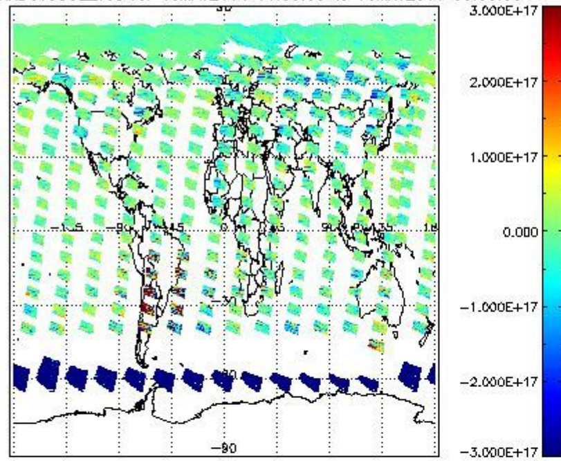
SCIOL2P_NADUV5S02_vcd for 15MAY2011 00:00:00 to 16MAY2011 00:00:00
