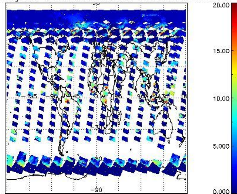
cL_top_height for 15MAY2011 00:00:00 to 16MAY2011 00:00:00
