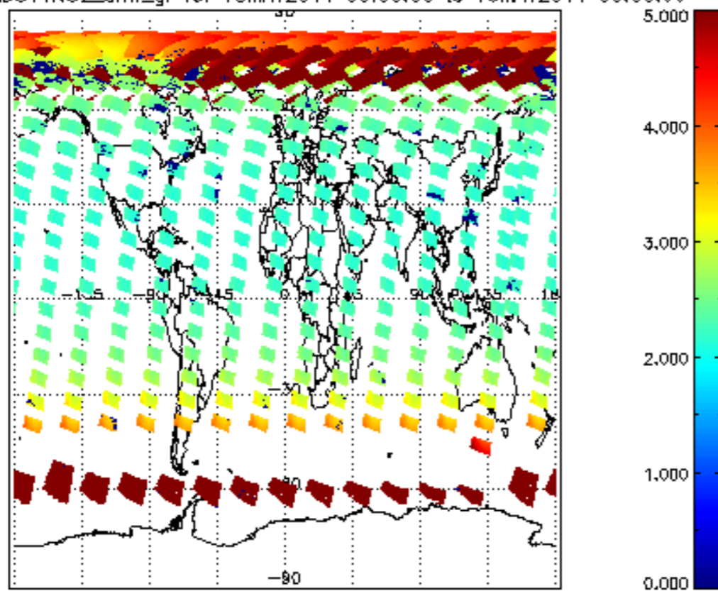
SCIOL2P_NADUV1NO2_amf_gr for 15MAY2011 00:00:00 to 16MAY2011 00:00:00
