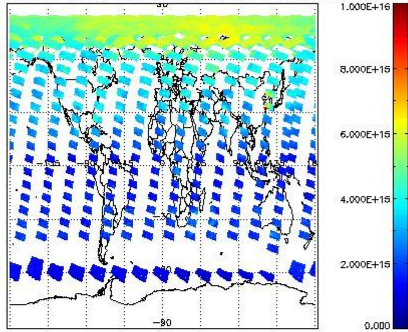
SCIOL2P_NADUV1NO2_vcd for 15MAY2011 00:00:00 to 16MAY2011 00:00:00
