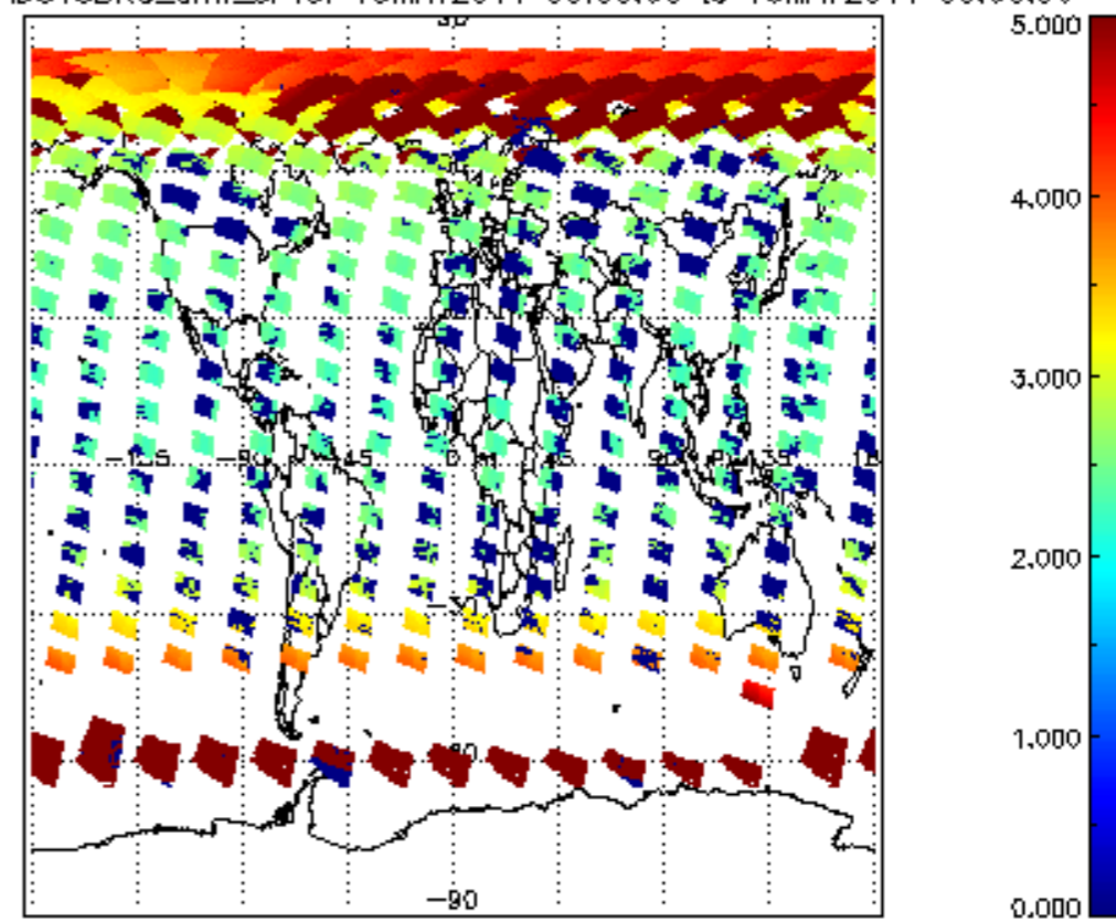
SCIOL2P_NADUV3BRO_amf_sl for 15MAY2011 00:00:00 to 16MAY2011 00:00:00
