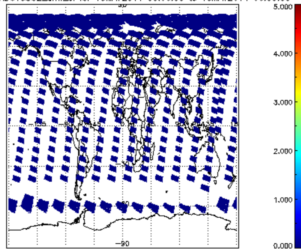
SCIOL2P_NADUV5S02_amf_cl for 15MAY2011 00:00:00 to 16MAY2011 00:00:00
