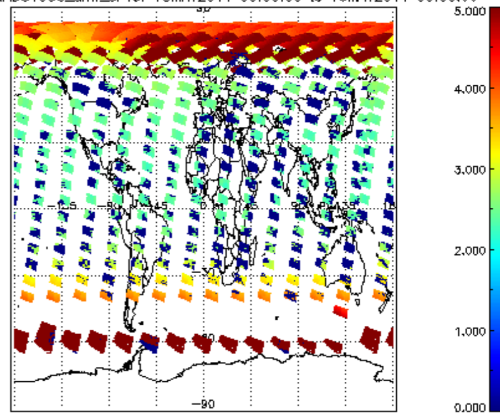
SCIOL2P_NADUV003_amf_cl for 15MAY2011 00:00:00 to 16MAY2011 00:00:00
