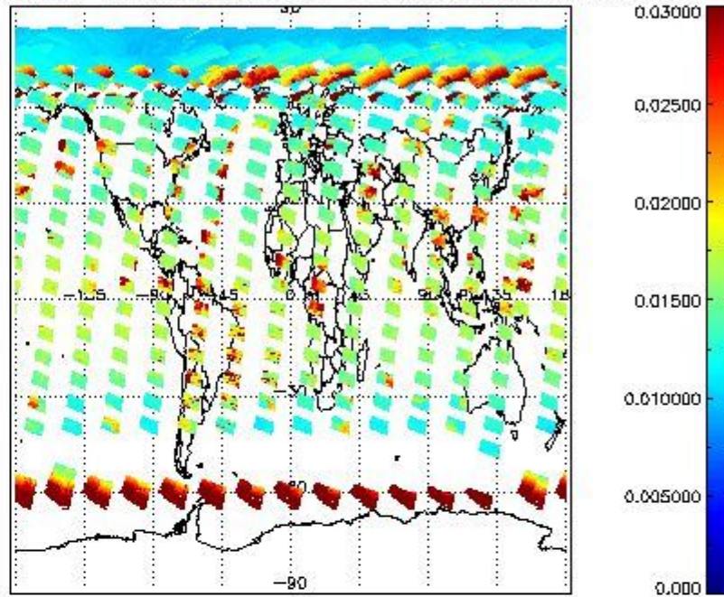
SCIOL2P_NADUV003_vcd_err for 15MAY2011 00:00:00 to 16MAY2011 00:00:00
