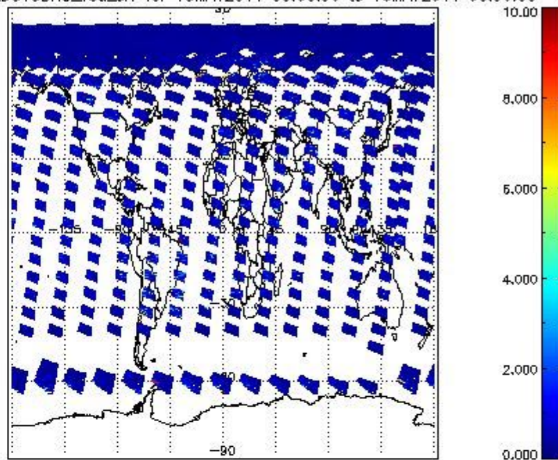
SCIOL2P_NADUV3BRO_vcd_err for 15MAY2011 00:00:00 to 16MAY2011 00:00:00
