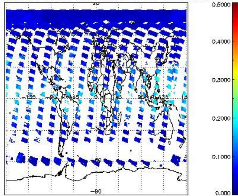
SCIOL2P_NADUV8H2O_vcd_err for 15MAY2011 00:00:00 to 16MAY2011 00:00:00
