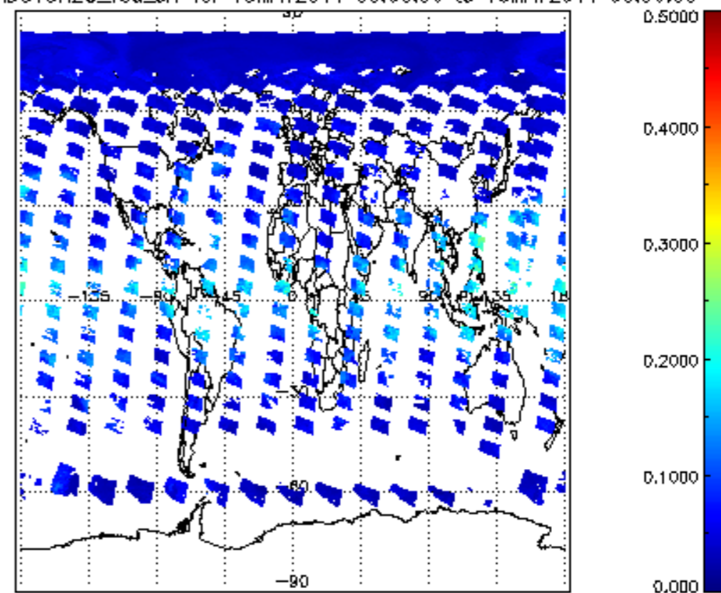
SCIOL2P_NADUV8H2O_vcd_err for 15MAY2011 00:00:00 to 16MAY2011 00:00:00
