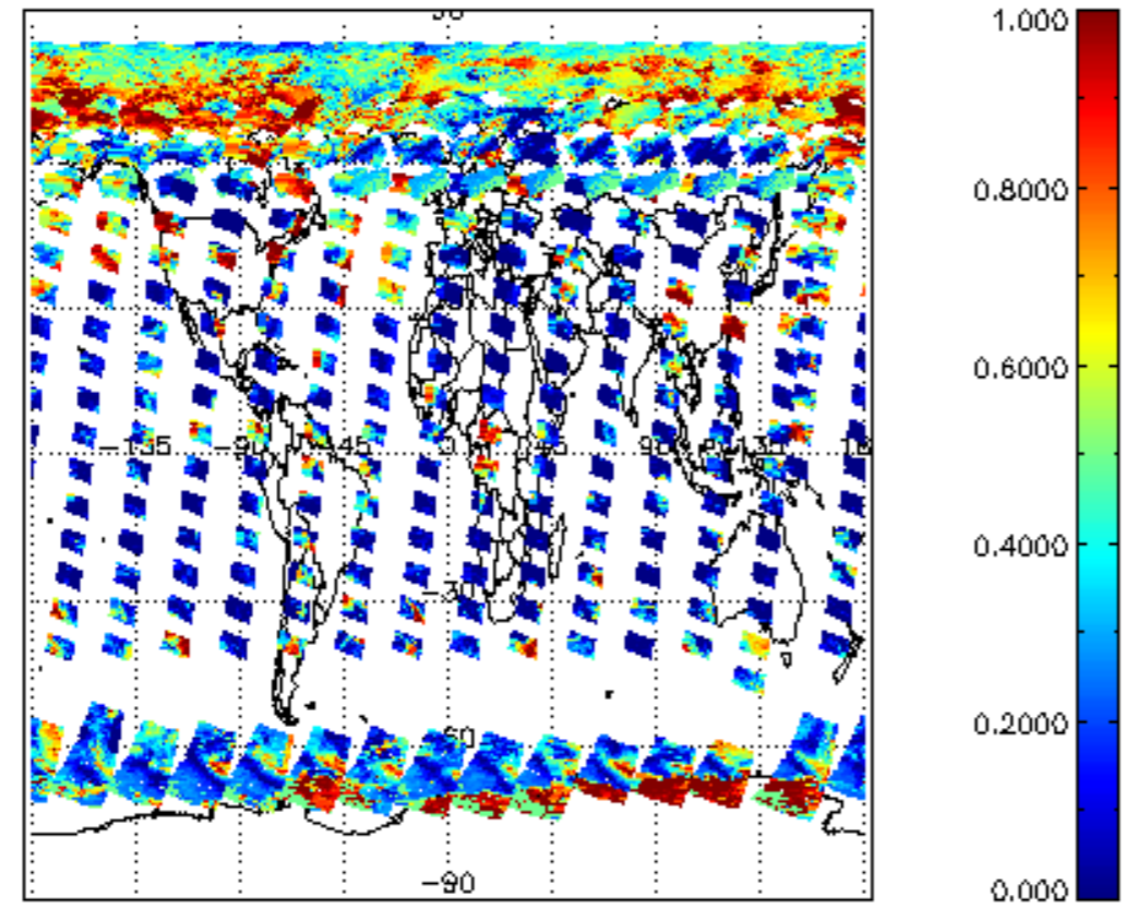
cl_frac for 15MAY2011 00:00:00 to 16MAY2011 00:00:00
