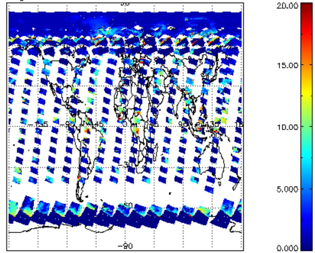
cl_top_height for 15MAY2011 00:00:00 to 16MAY2011 00:00:00
