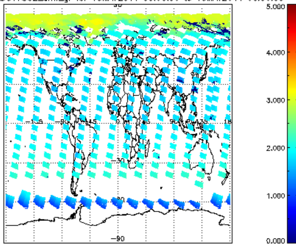
SCIOL2P_NADUV7S02_amf_gr for 15MAY2011 00:00:00 to 16MAY2011 00:00:00
