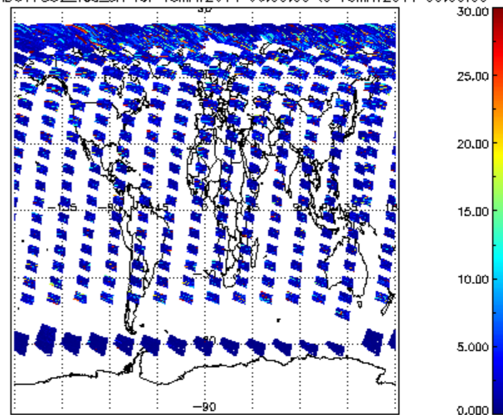
SCIOL2P_NADUV7S02_vcd_err for 15MAY2011 00:00:00 to 16MAY2011 00:00:00
