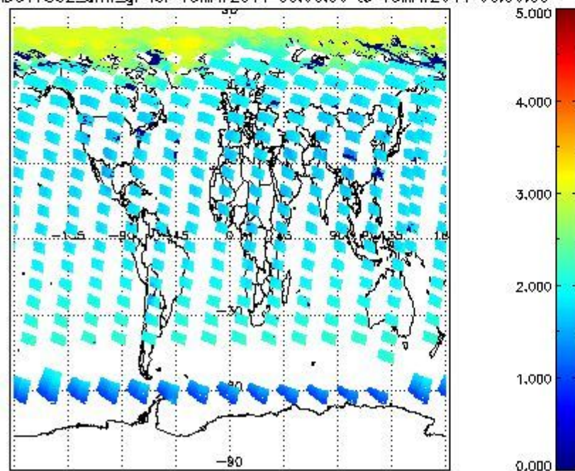
SCIOL2P_NADUV7S02_amf_gr for 15MAY2011 00:00:00 to 16MAY2011 00:00:00
