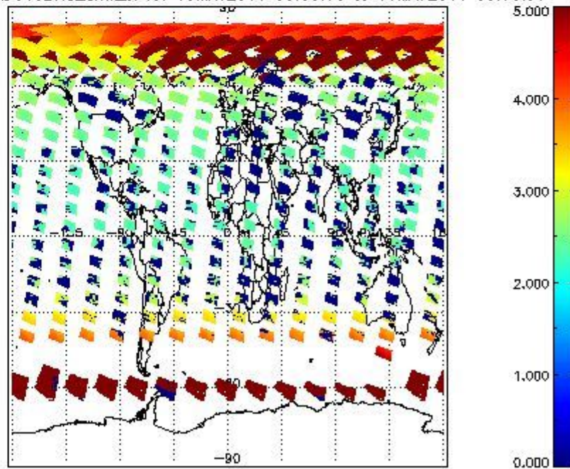
SCIOL2P_NADUV3BRO_amf_cl for 15MAY2011 00:00:00 to 16MAY2011 00:00:00
