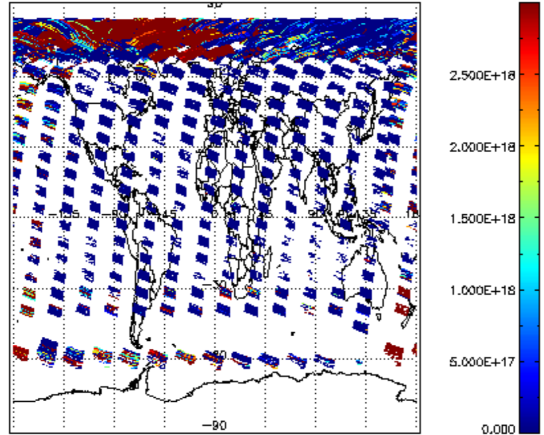
SCIOL2P_NADIR3CO_vcd for 15MAY2011 00:00:00 to 16MAY2011 00:00:00
