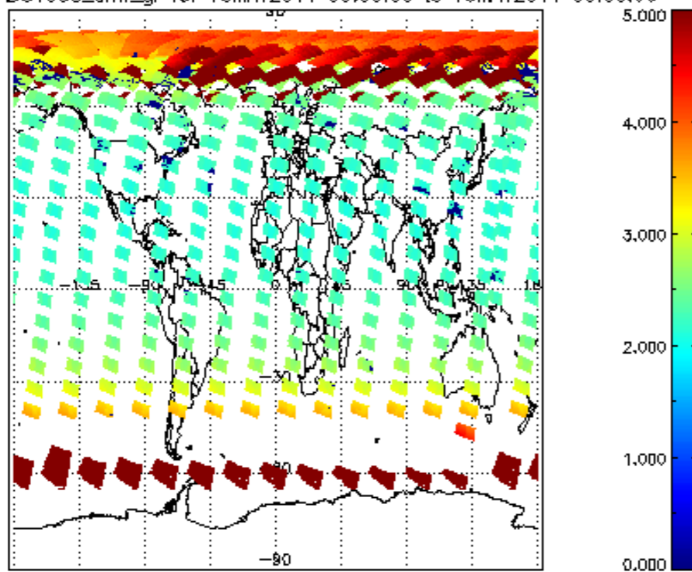
SCIOL2P_NADUV003_amf_gr for 15MAY2011 00:00:00 to 16MAY2011 00:00:00
