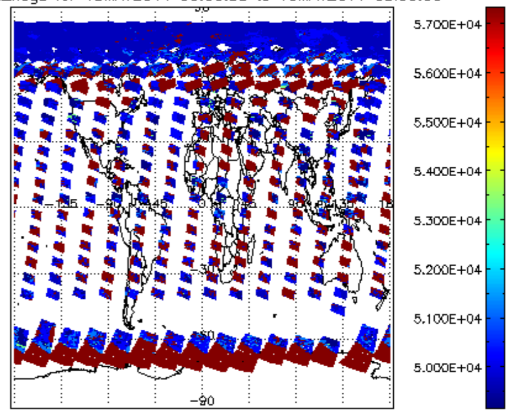
cloud_flags for 15MAY2011 00:00:00 to 16MAY2011 00:00:00
