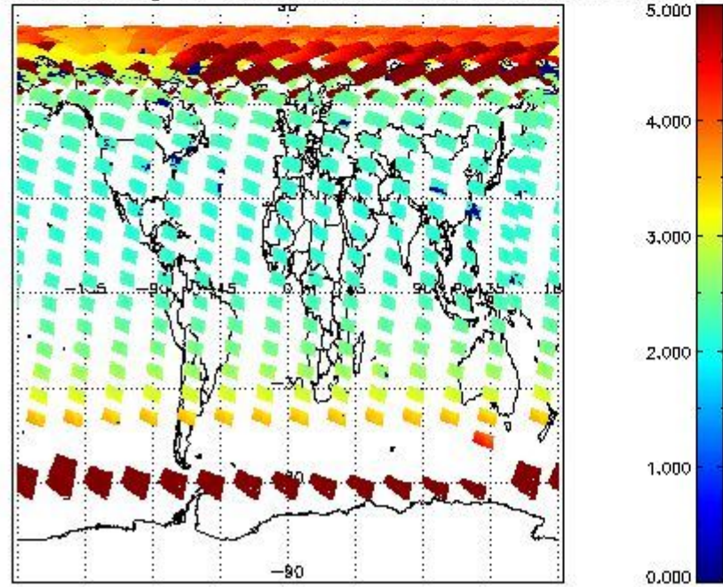
SCIOL2P_NADUV003_amf_gr for 15MAY2011 00:00:00 to 16MAY2011 00:00:00
