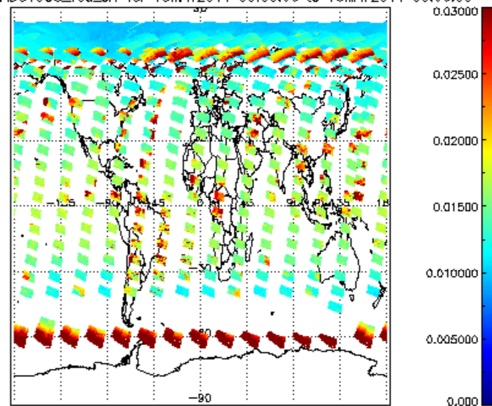
SCIOL2P_NADUV003_vcd_err for 15MAY2011 00:00:00 to 16MAY2011 00:00:00
