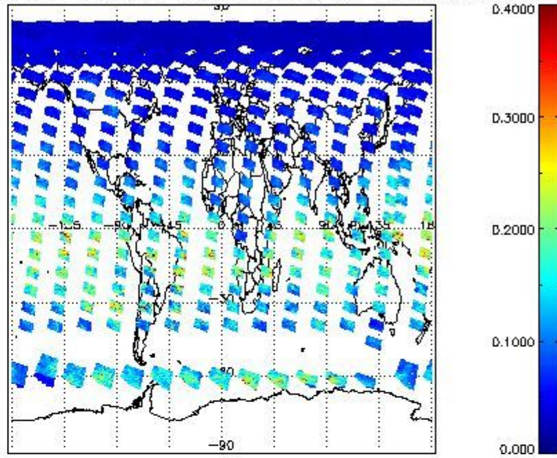
SCIOL2P_NADUV1NO2_vcd_err for 15MAY2011 00:00:00 to 16MAY2011 00:00:00
