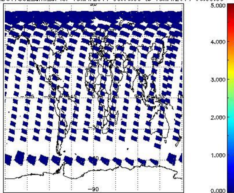
SCIOL2P_NADUV7S02_amf_cl for 15MAY2011 00:00:00 to 16MAY2011 00:00:00
