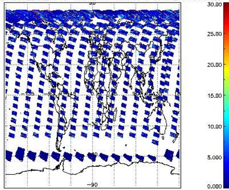
SCIOL2P_NADUV5S02_vcd_err for 15MAY2011 00:00:00 to 16MAY2011 00:00:00
