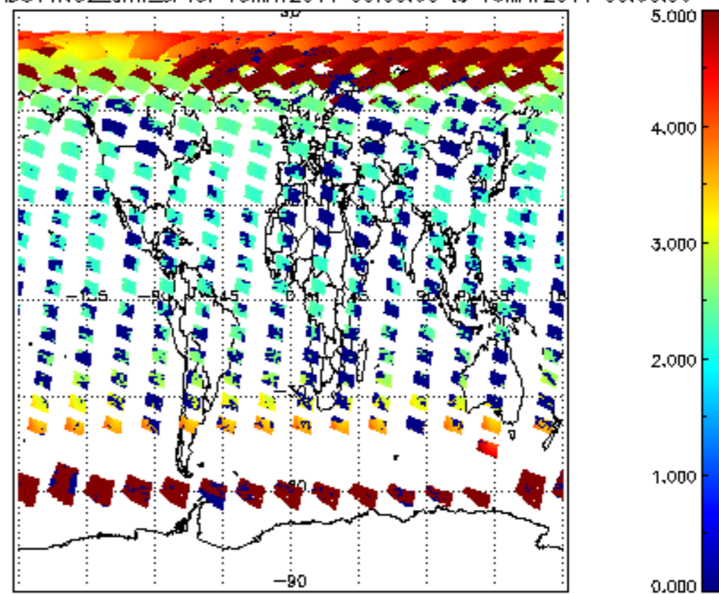
SCIOL2P_NADUV1NO2_amf_sl for 15MAY2011 00:00:00 to 16MAY2011 00:00:00
