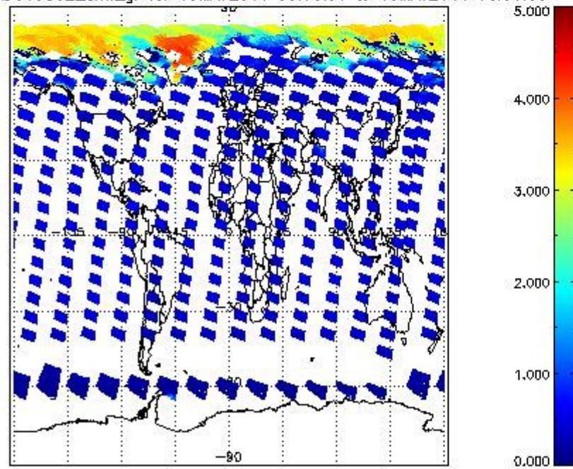
SCIOL2P_NADUV5S02_amf_gr for 15MAY2011 00:00:00 to 16MAY2011 00:00:00
