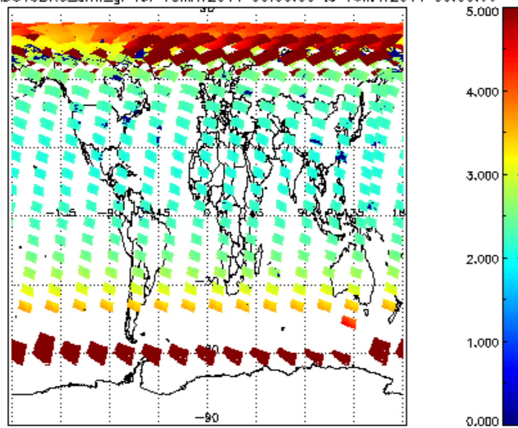
SCIOL2P_NADUV3BRO_amf_gr for 15MAY2011 00:00:00 to 16MAY2011 00:00:00
