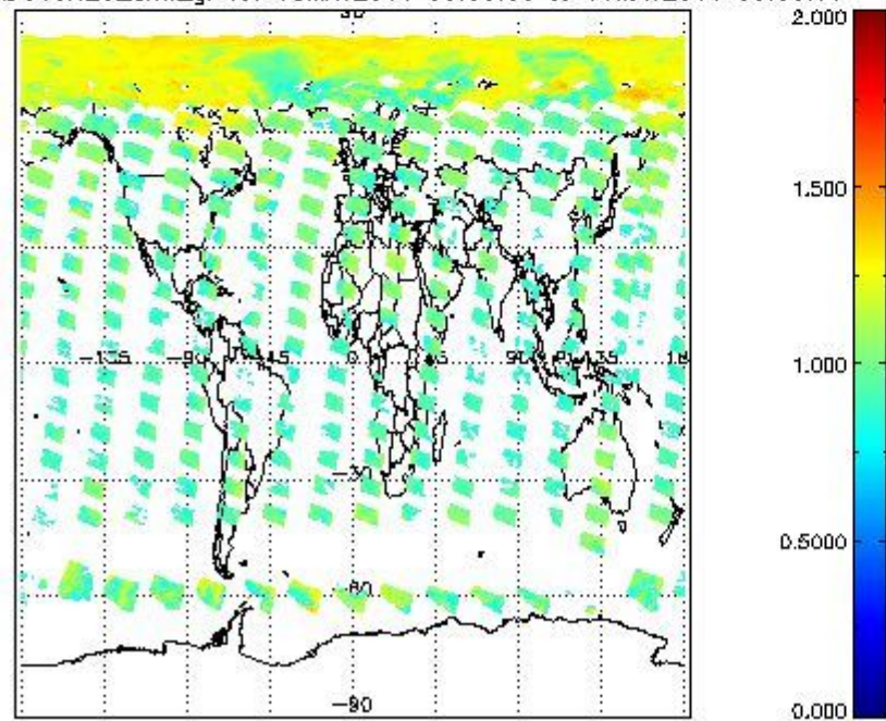
SCIOL2P_NADUV8H2O_arnf_gr for 15MAY2011 00:00:00 to 16MAY2011 00:00:00
