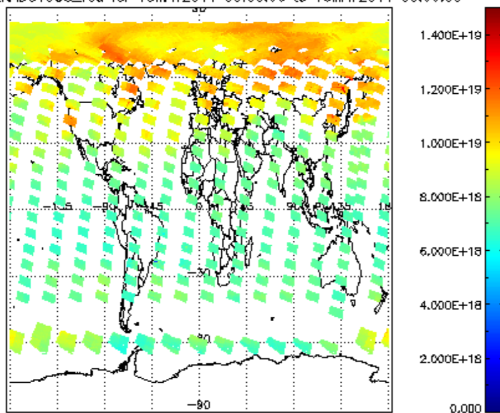
SCIOL2P_NADUV003_vcd for 15MAY2011 00:00:00 to 16MAY2011 00:00:00
