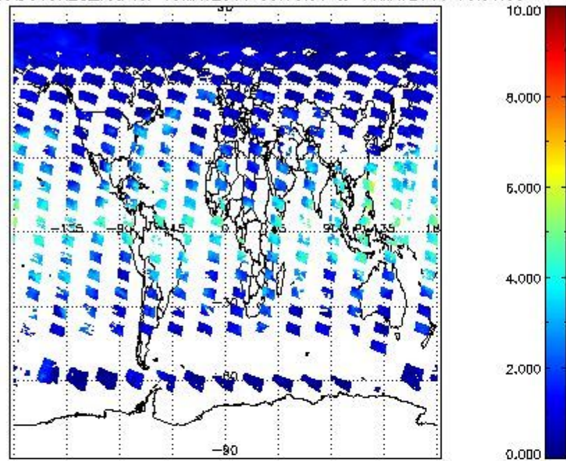
SCIOL2P_NADUV8H2O_vcd for 15MAY2011 00:00:00 to 16MAY2011 00:00:00
