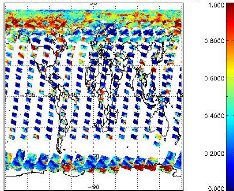
cL_frac for 15MAY2011 00:00:00 to 16MAY2011 00:00:00
