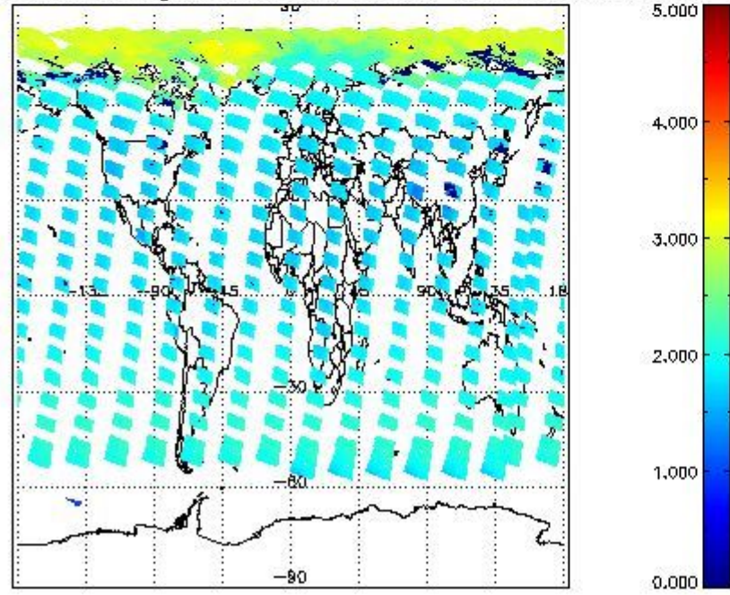
SCIOL2P_NADUV7S02_amf_gr for 13MAY2011 00:00:00 to 14MAY2011 00:00:00
