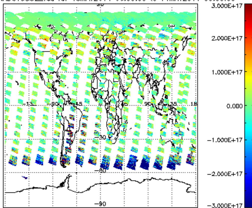
SCIOL2P_NADUV5S02_vcd for 13MAY2011 00:00:00 to 14MAY2011 00:00:00
