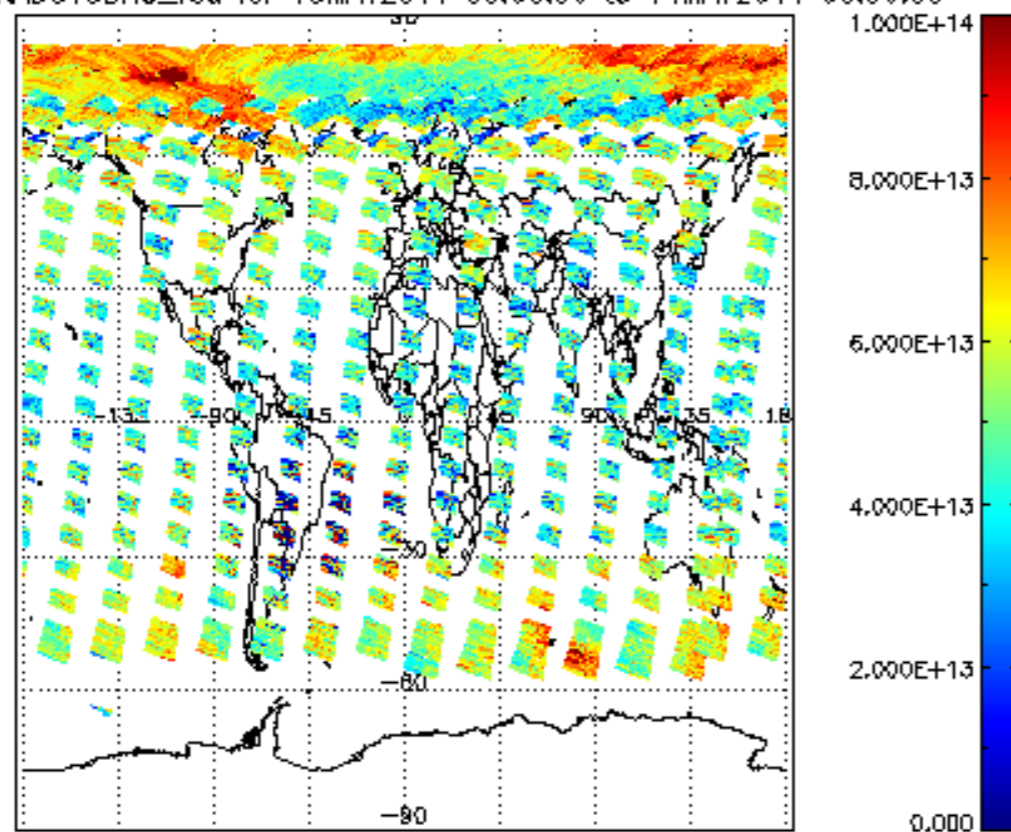
SCIOL2P_NADUV3BRO_vcd for 13MAY2011 00:00:00 to 14MAY2011 00:00:00
