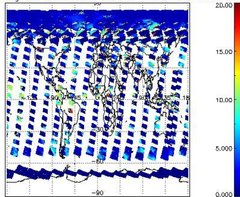
cL_top_height for 13MAY2011 00:00:00 to 14MAY2011 00:00:00
