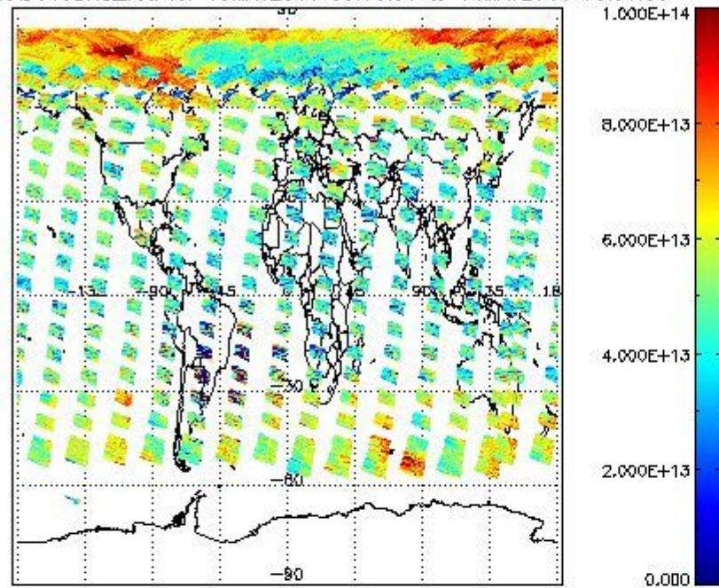
SCIOL2P_NADUV3BRO_vcd for 13MAY2011 00:00:00 to 14MAY2011 00:00:00
