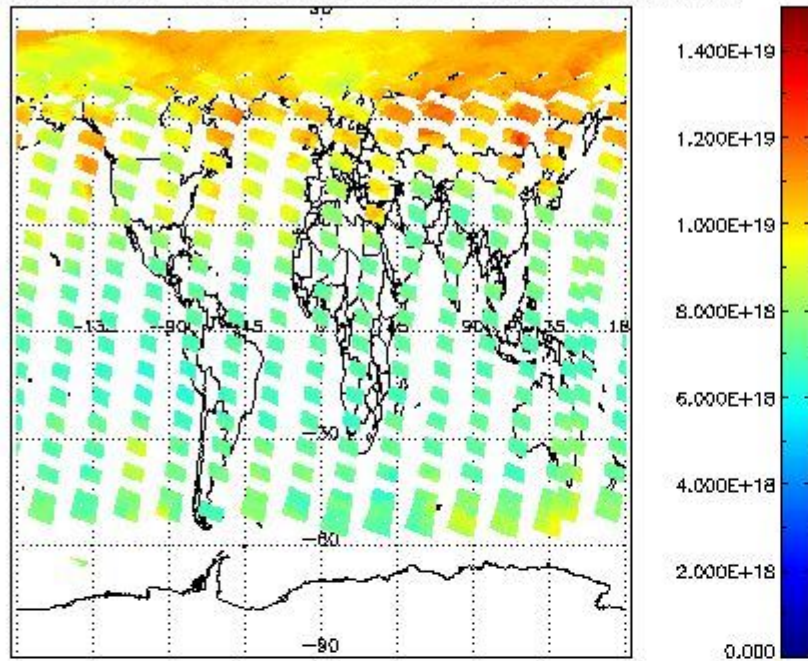
SCIOL2P_NADUV003_vcd for 13MAY2011 00:00:00 to 14MAY2011 00:00:00
