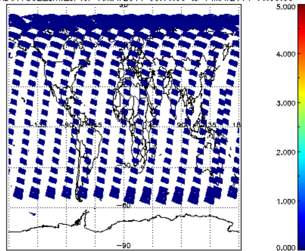
SCIOL2P_NADUV7S02_amf_cl for 13MAY2011 00:00:00 to 14MAY2011 00:00:00
