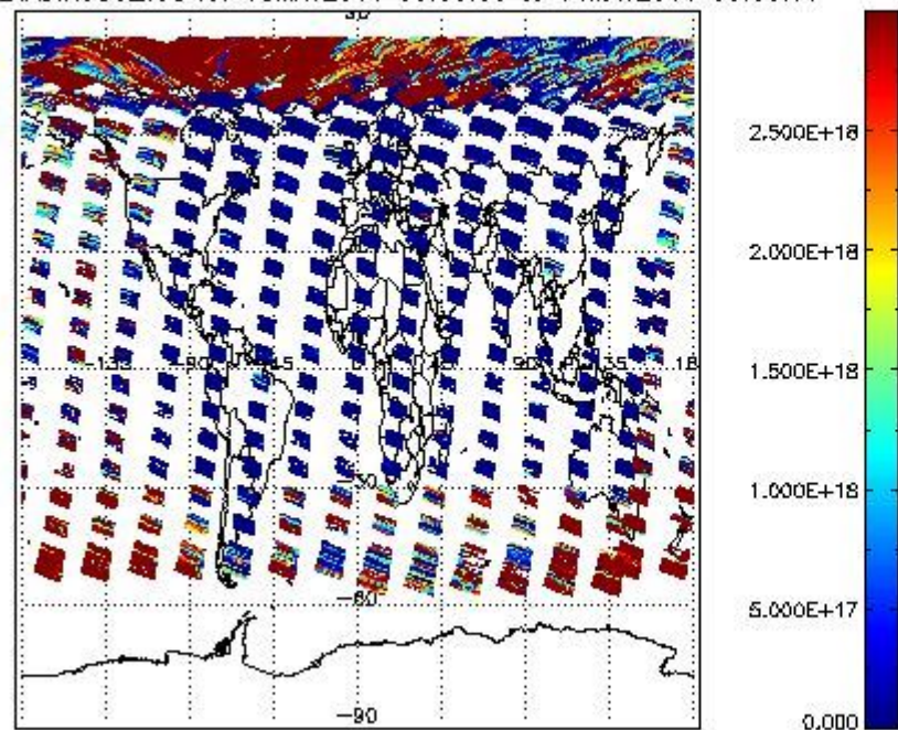
SCIO2P_NADIR3CO_vcd for 13MAY2011 00:00:00 to 14MAY2011 00:00:00
