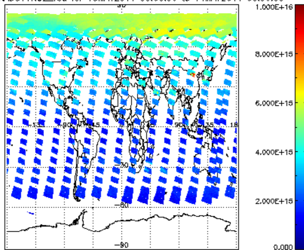
SCIOL2P_NADUV1NO2_vcd for 13MAY2011 00:00:00 to 14MAY2011 00:00:00
