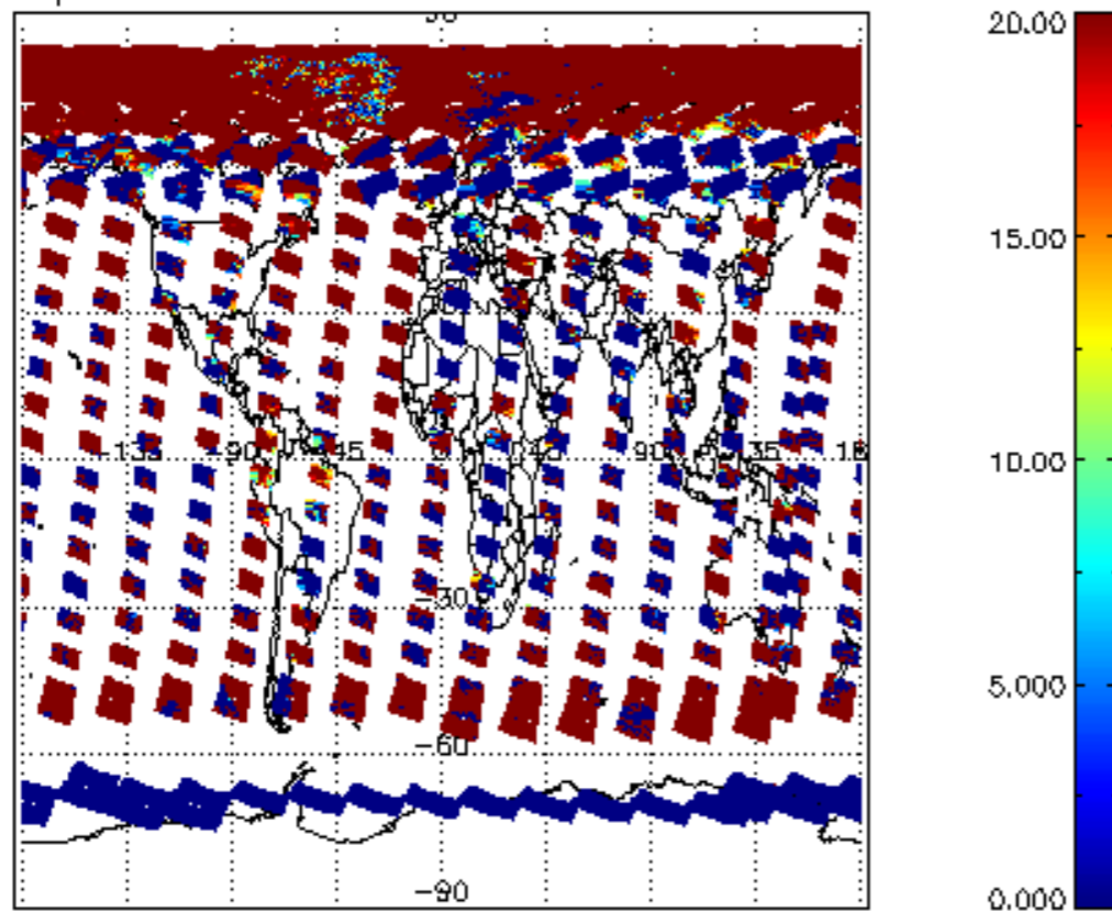
cL_opt_depth for 13MAY2011 00:00:00 to 14MAY2011 00:00:00
