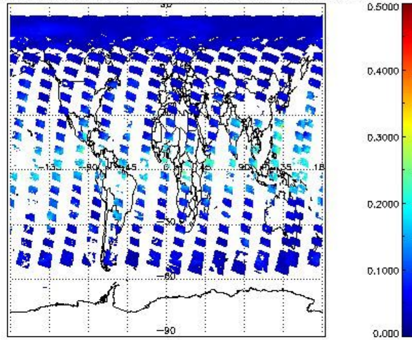
SCIOL2P_NADUV8H2O_vcd_err for 13MAY2011 00:00:00 to 14MAY2011 00:00:00
