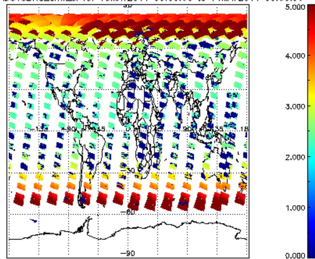
SCIOL2P_NADUV3BRO_amf_cl for 13MAY2011 00:00:00 to 14MAY2011 00:00:00
