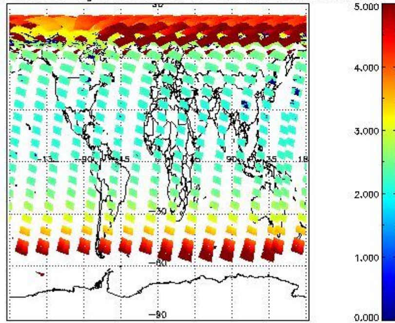
SCIOL2P_NADUV3BRO_amf_gr for 13MAY2011 00:00:00 to 14MAY2011 00:00:00
