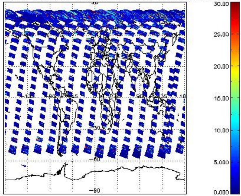
SCIOL2P_NADUV5S02_vcd_err for 13MAY2011 00:00:00 to 14MAY2011 00:00:00
