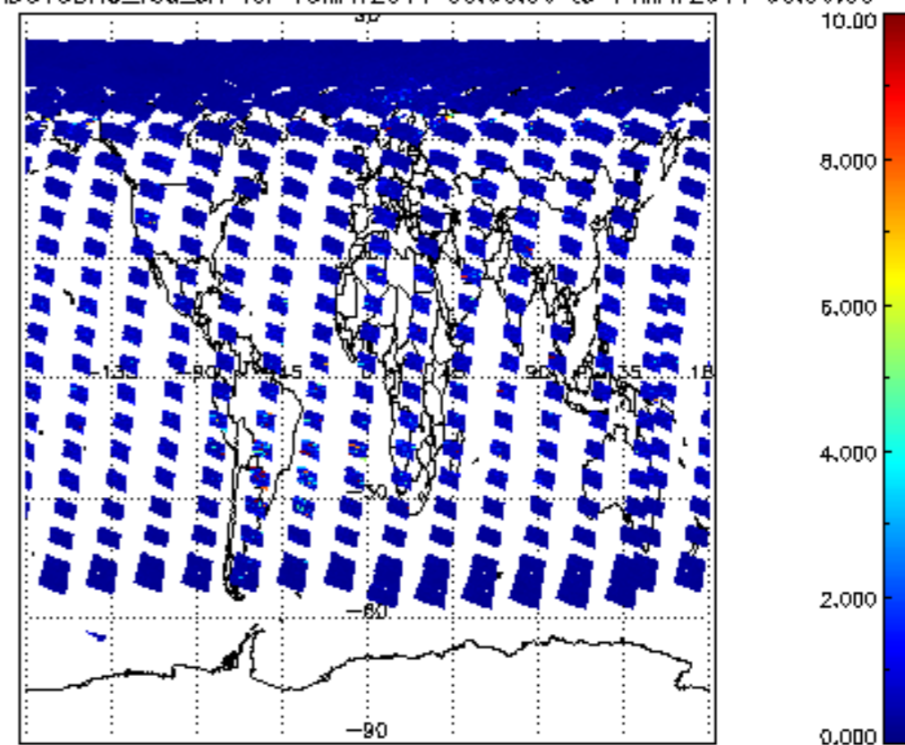
SCIOL2P_NADUV3BRO_vcd_err for 13MAY2011 00:00:00 to 14MAY2011 00:00:00
