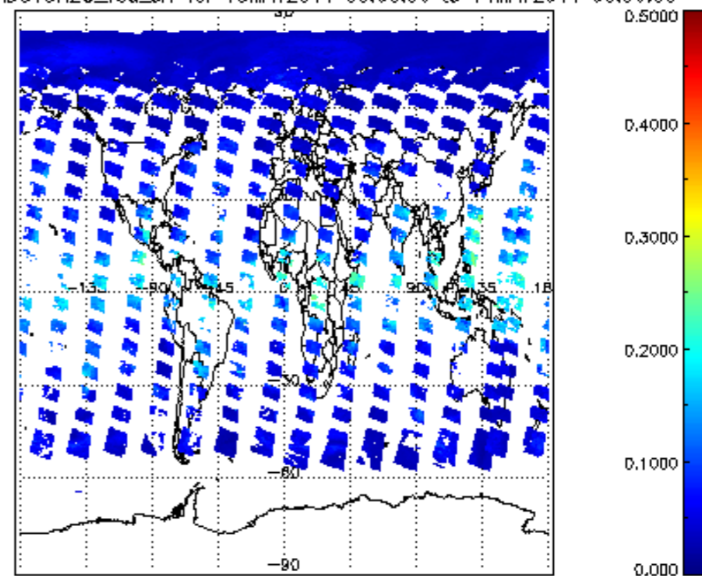
SCIOL2P_NADUV8H2O_vcd_err for 13MAY2011 00:00:00 to 14MAY2011 00:00:00
