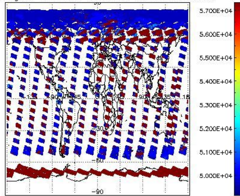
cloud_flags for 13MAY2011 00:00:00 to 14MAY2011 00:00:00
