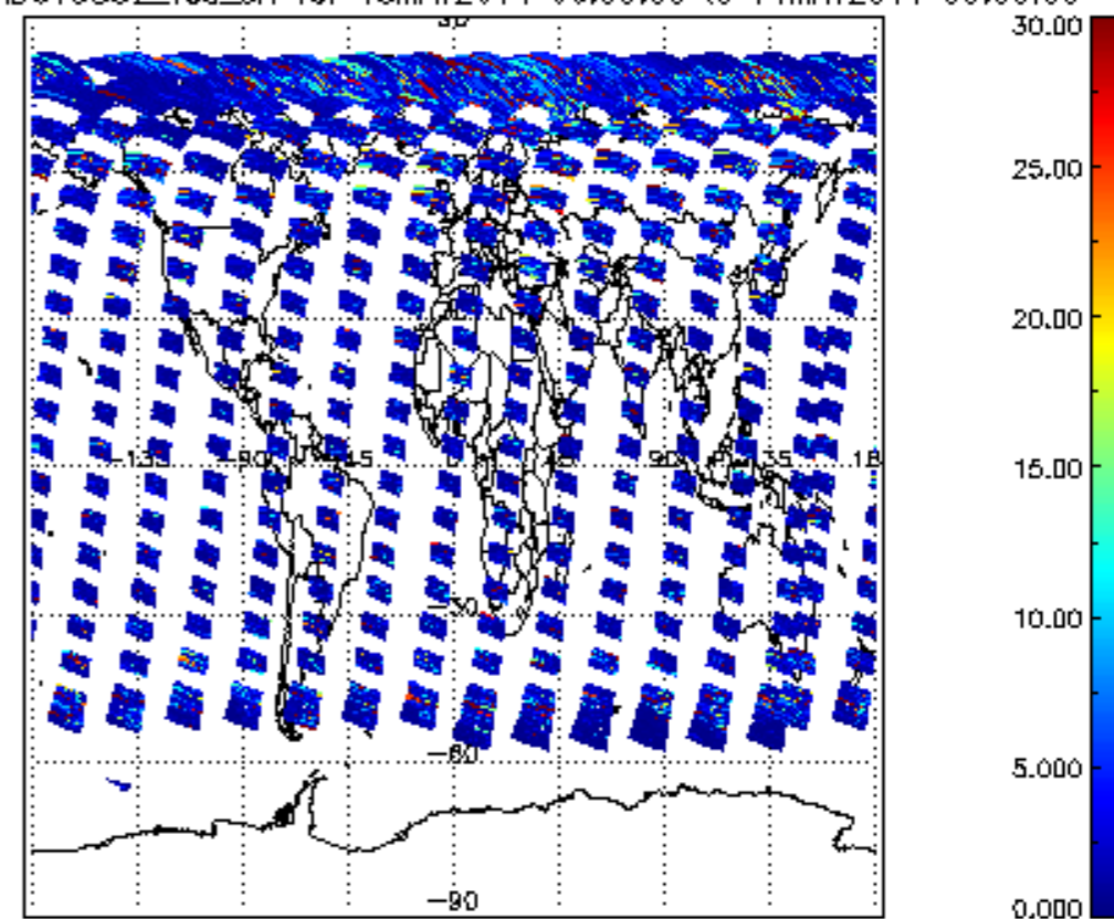
SCIOL2P_NADUV5S02_vcd_err for 13MAY2011 00:00:00 to 14MAY2011 00:00:00
