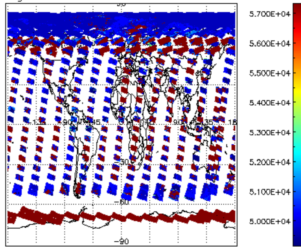
cloud_flags for 13MAY2011 00:00:00 to 14MAY2011 00:00:00
