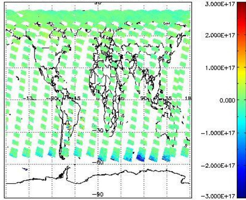
SCIOL2P_NADUV7S02_vcd for 13MAY2011 00:00:00 to 14MAY2011 00:00:00
