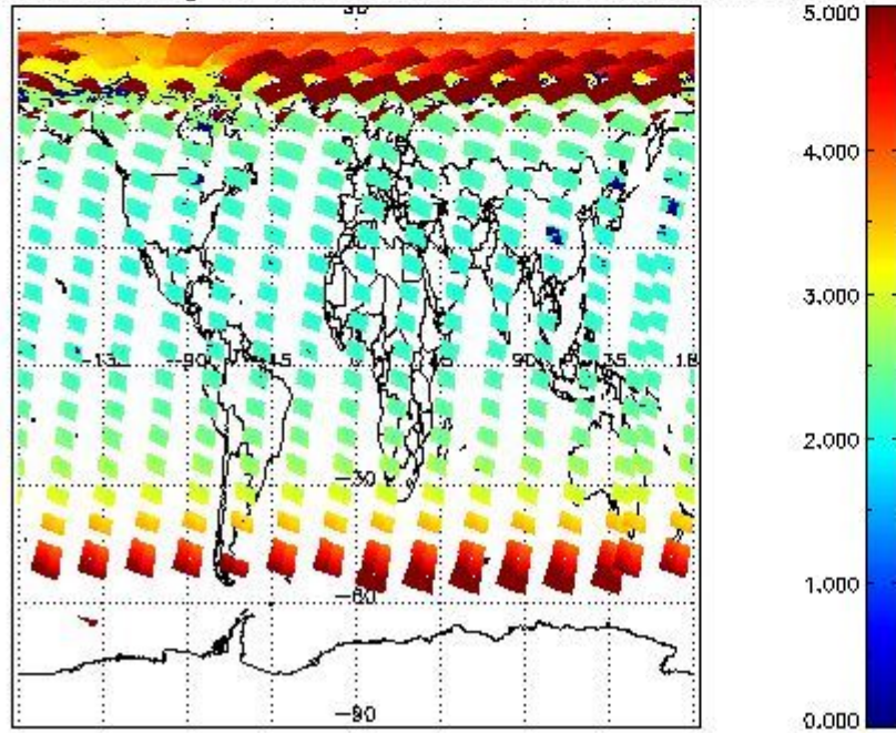
SCIOL2P_NADUV003_amf_gr for 13MAY2011 00:00:00 to 14MAY2011 00:00:00
