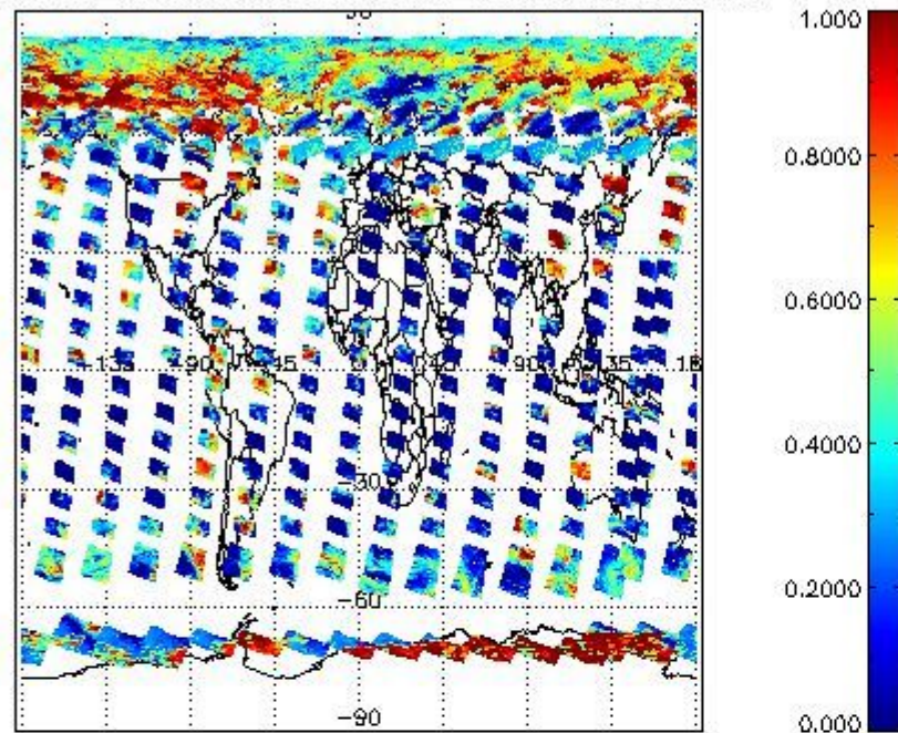
cL_frac for 13MAY2011 00:00:00 to 14MAY2011 00:00:00
