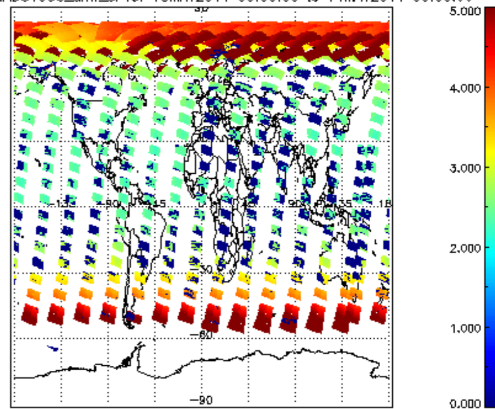
SCIOL2P_NADUV003_amf_cl for 13MAY2011 00:00:00 to 14MAY2011 00:00:00
