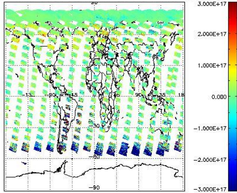
SCIOL2P_NADUV5S02_vcd for 13MAY2011 00:00:00 to 14MAY2011 00:00:00
