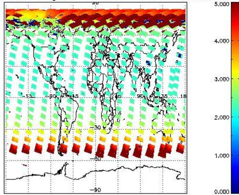
SCIOL2P_NADUV1NO2_amf_gr for 13MAY2011 00:00:00 to 14MAY2011 00:00:00
