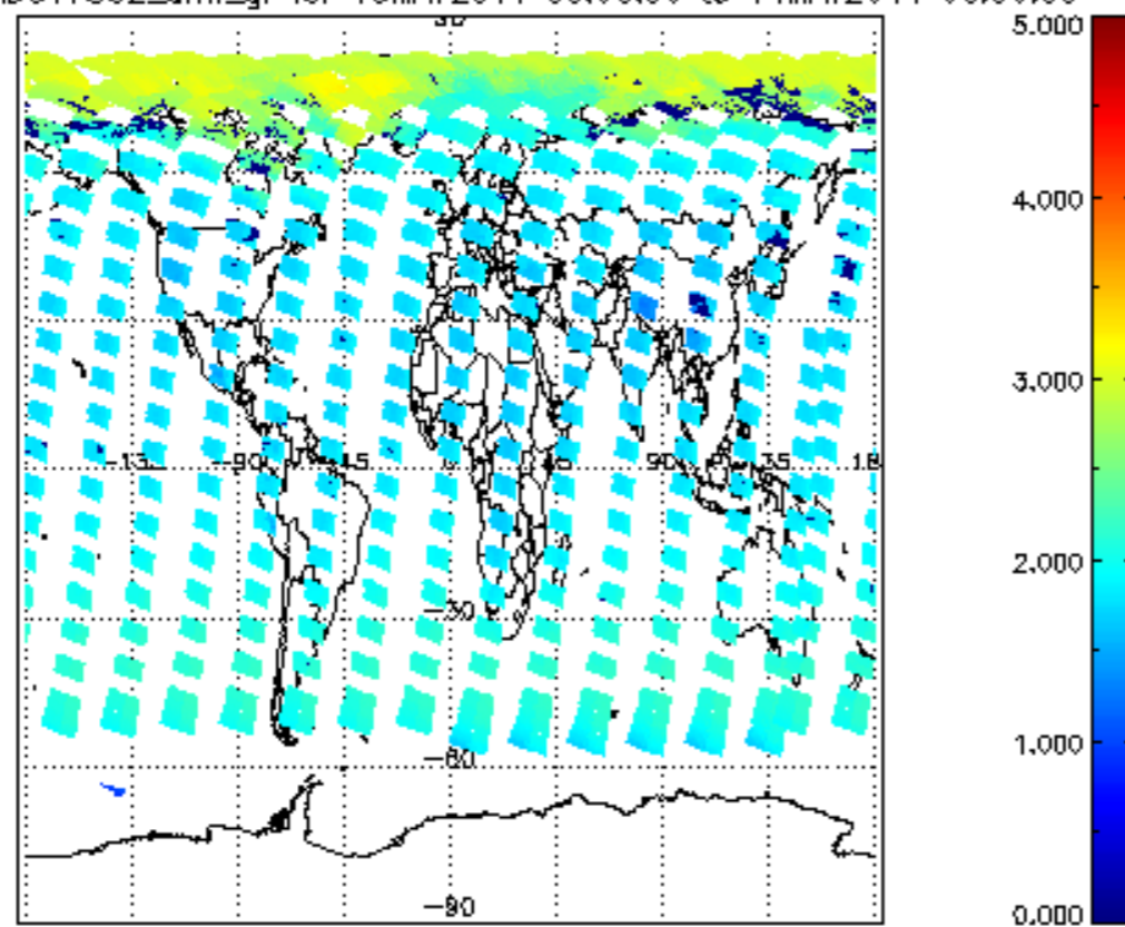
SCIOL2P_NADUV7S02_amf_gr for 13MAY2011 00:00:00 to 14MAY2011 00:00:00
