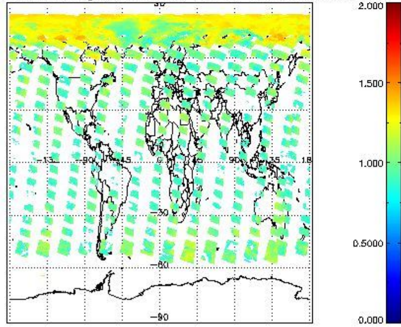
SCIOL2P_NADUV8H2O_arnf_gr for 13MAY2011 00:00:00 to 14MAY2011 00:00:00
