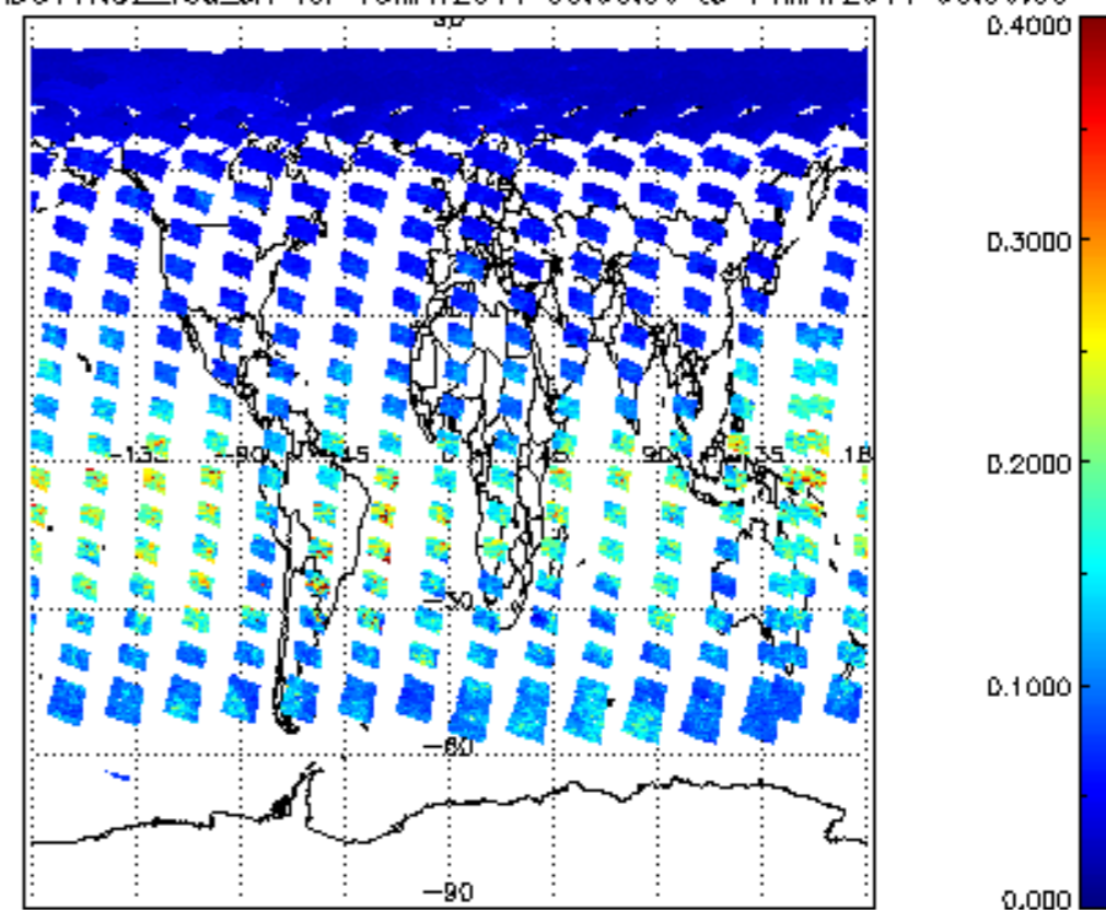
SCIOL2P_NADUV1NO2_vcd_err for 13MAY2011 00:00:00 to 14MAY2011 00:00:00
