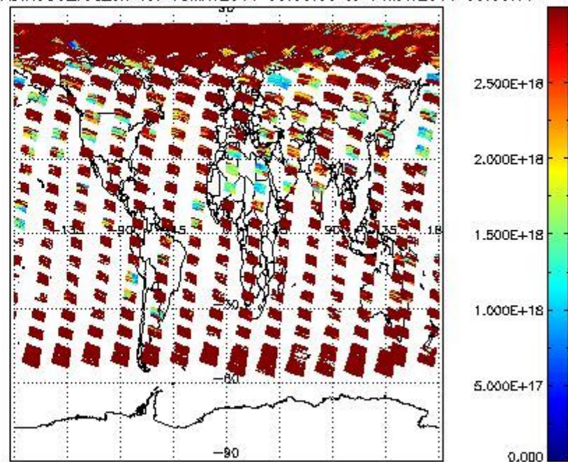
SCIO2P_NADIR3CO_vcd_err for 13MAY2011 00:00:00 to 14MAY2011 00:00:00
