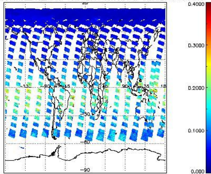
SCIOL2P_NADUV1NO2_vcd_err for 13MAY2011 00:00:00 to 14MAY2011 00:00:00
