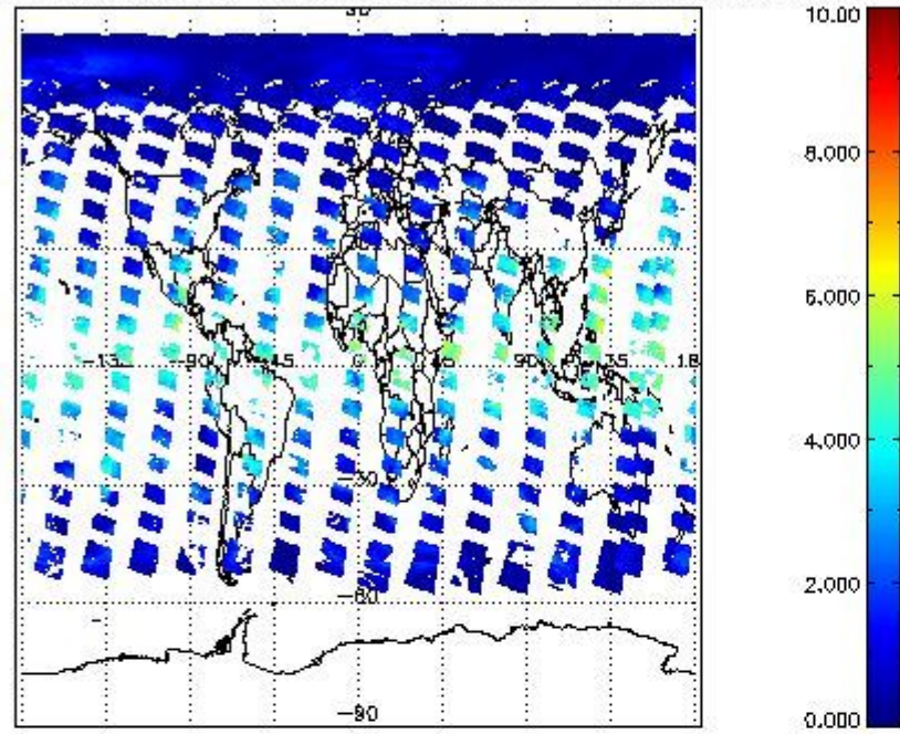
SCIOL2P_NADUV8H2O_vcd for 13MAY2011 00:00:00 to 14MAY2011 00:00:00
