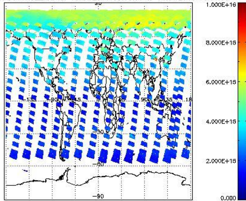
SCIOL2P_NADUV1NO2_vcd for 13MAY2011 00:00:00 to 14MAY2011 00:00:00
