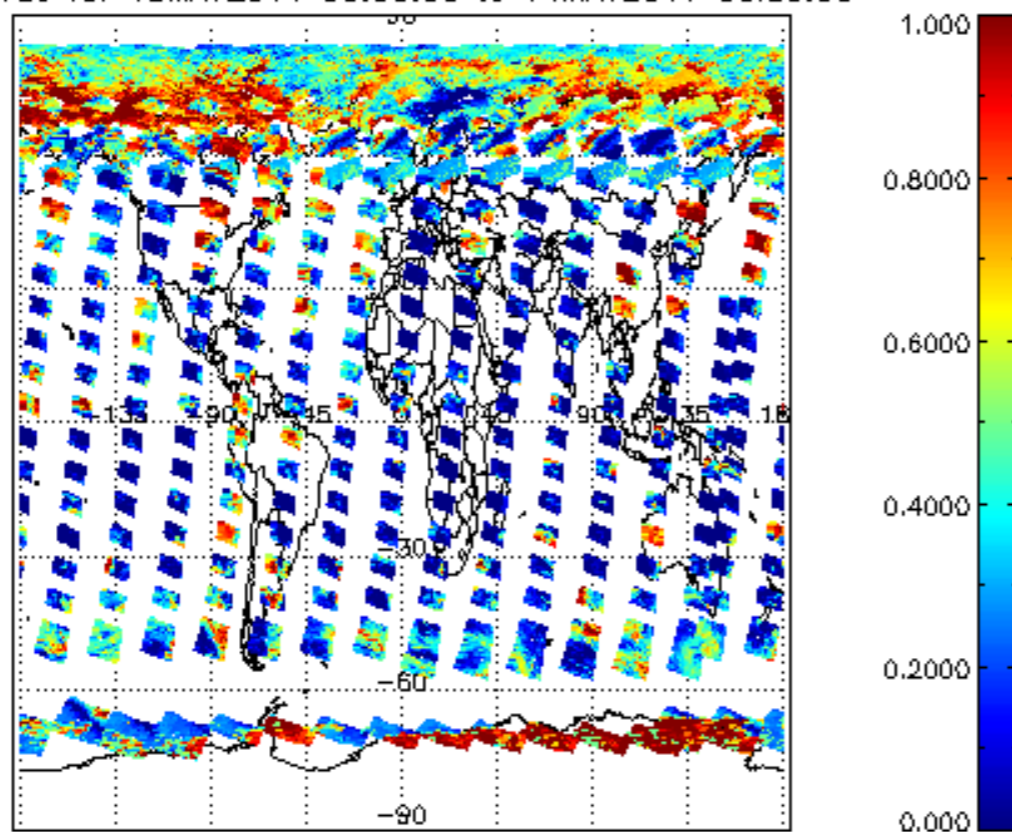
cL_frac for 13MAY2011 00:00:00 to 14MAY2011 00:00:00
