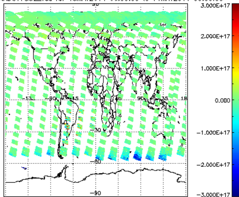
SCIOL2P_NADUV7S02_vcd for 13MAY2011 00:00:00 to 14MAY2011 00:00:00
