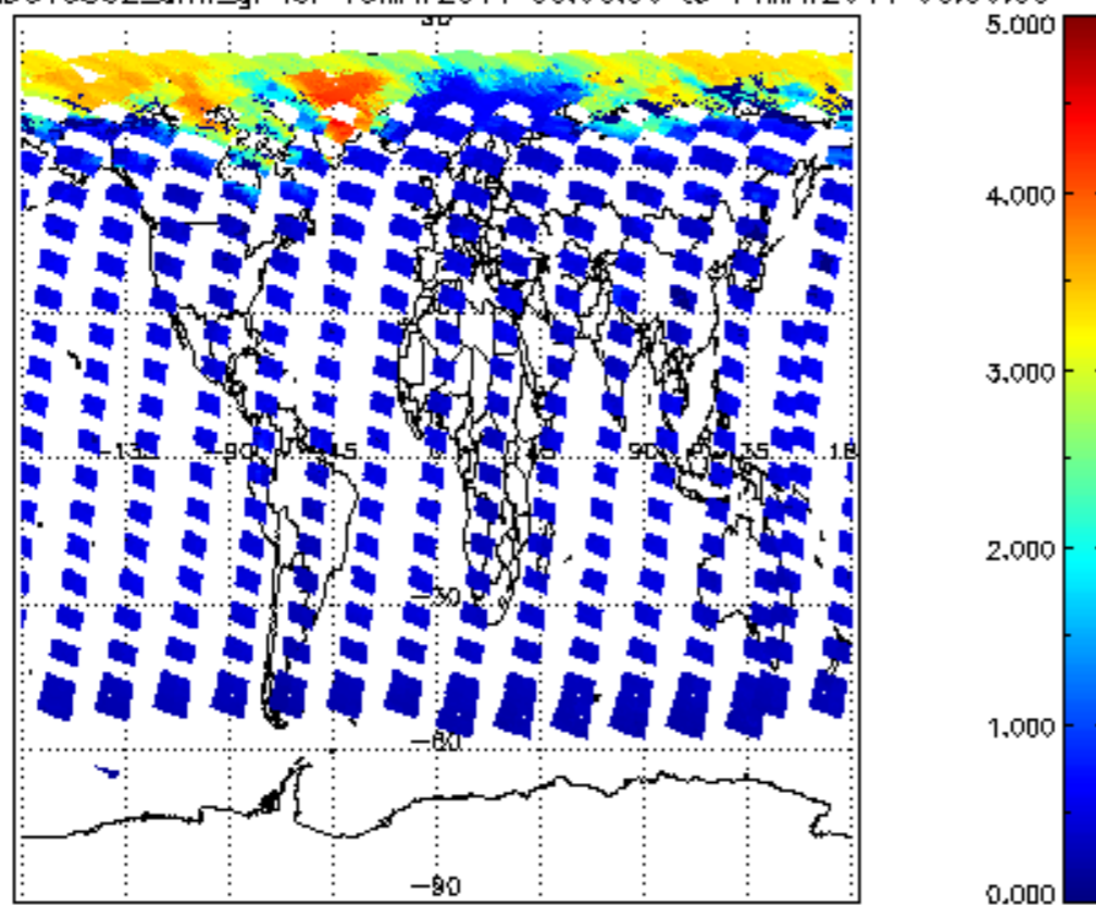
SCIOL2P_NADUV5S02_amf_gr for 13MAY2011 00:00:00 to 14MAY2011 00:00:00
