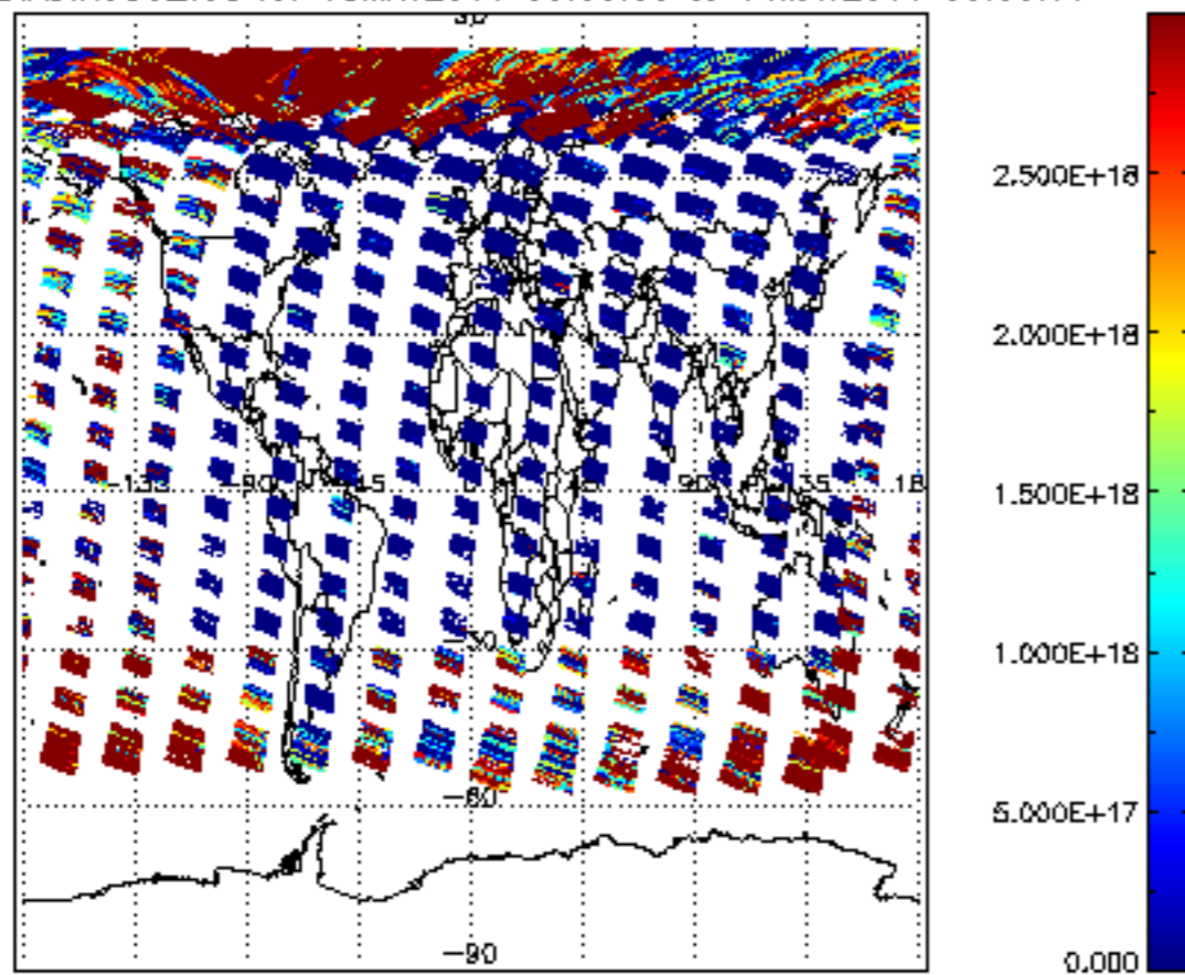
SCIOL2P_NADIR3CO_vcd for 13MAY2011 00:00:00 to 14MAY2011 00:00:00
