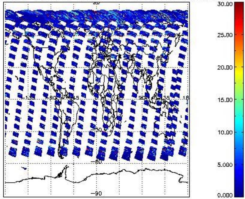
SCIOL2P_NADUV7S02_vcd_err for 13MAY2011 00:00:00 to 14MAY2011 00:00:00
