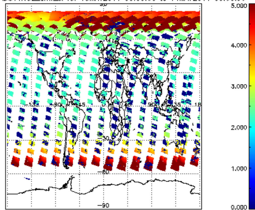
SCIOL2P_NADUV1NO2_amf_sl for 13MAY2011 00:00:00 to 14MAY2011 00:00:00
