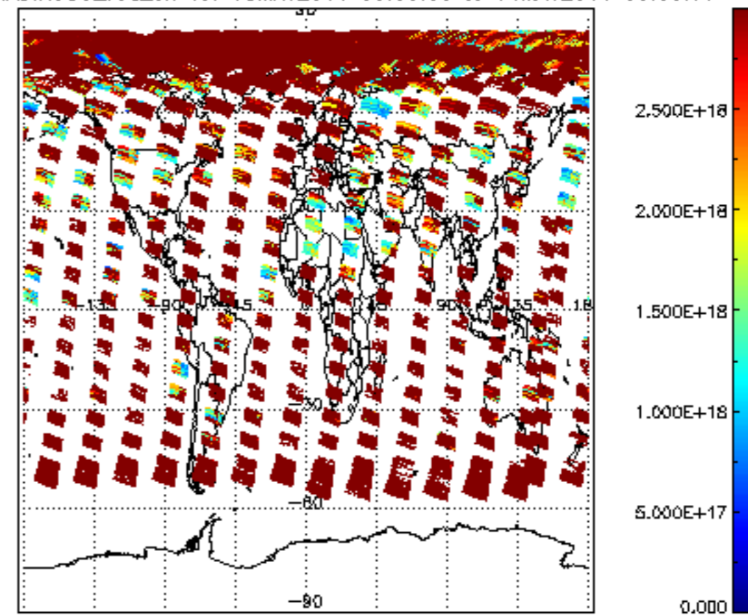
SCIOL2P_NADIR3CO_vcd_err for 13MAY2011 00:00:00 to 14MAY2011 00:00:00
