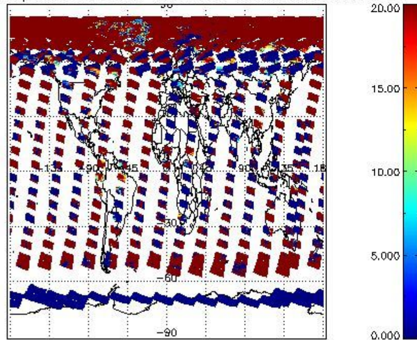
cL_opt_depth for 13MAY2011 00:00:00 to 14MAY2011 00:00:00
