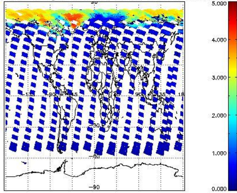
SCIOL2P_NADUV5S02_amf_gr for 13MAY2011 00:00:00 to 14MAY2011 00:00:00
