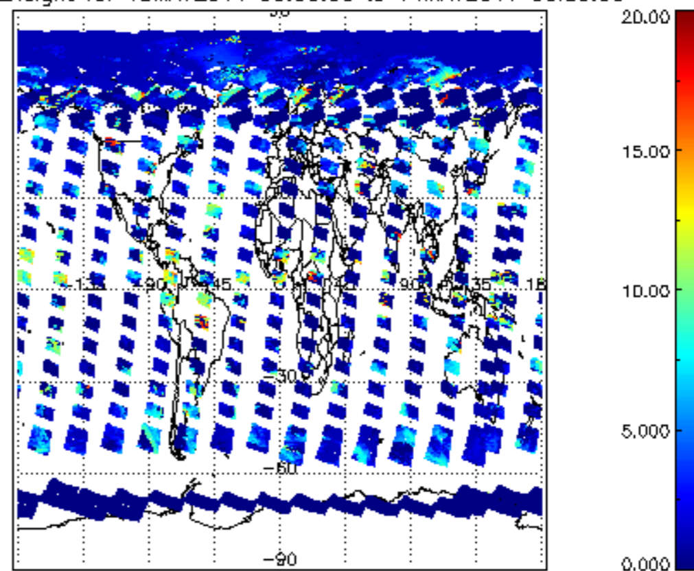
cL_top_height for 13MAY2011 00:00:00 to 14MAY2011 00:00:00
