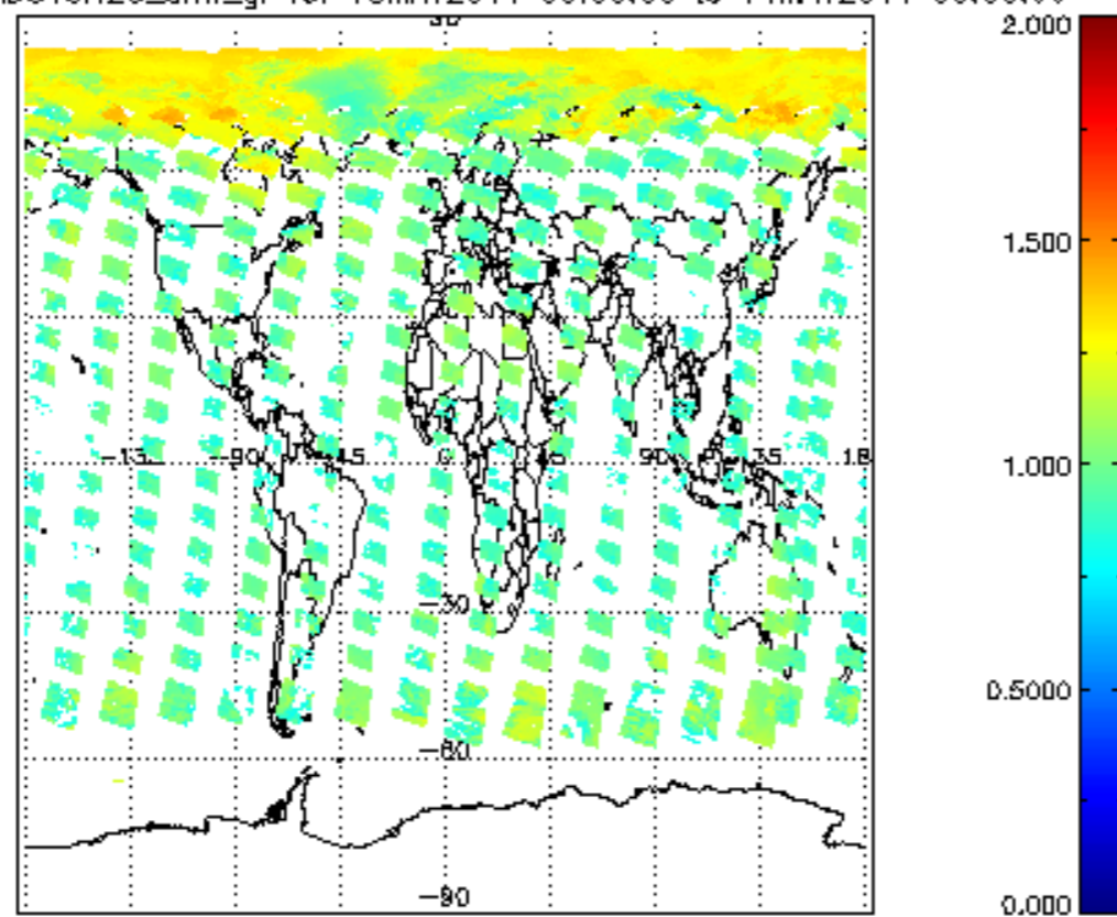
SCIOL2P_NADUV8H2O_amf_gr for 13MAY2011 00:00:00 to 14MAY2011 00:00:00
