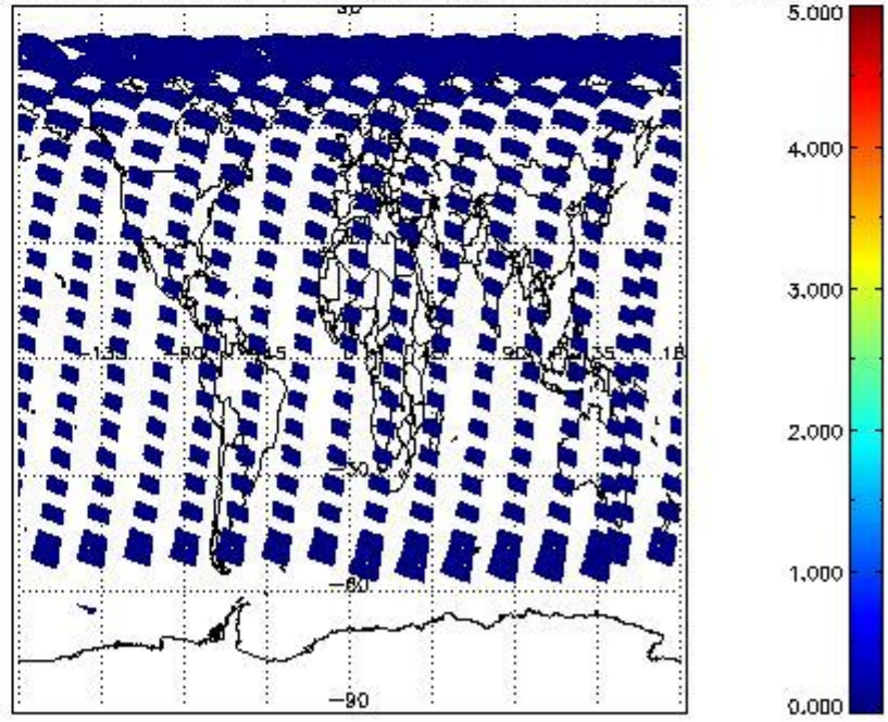
SCIOL2P_NADUV7S02_amf_cl for 13MAY2011 00:00:00 to 14MAY2011 00:00:00
