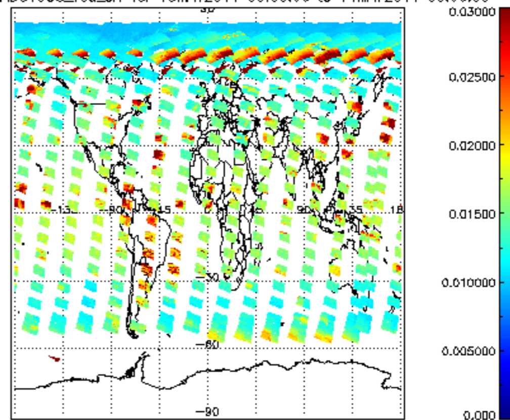
SCIOL2P_NADUV003_vcd_err for 13MAY2011 00:00:00 to 14MAY2011 00:00:00
