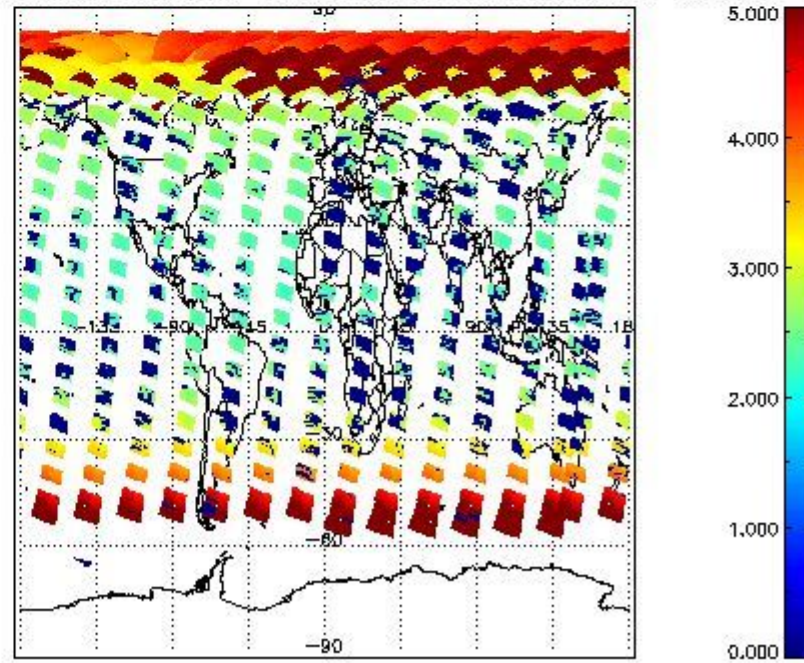
SCIOL2P_NADUV3BRO_amf_cl for 13MAY2011 00:00:00 to 14MAY2011 00:00:00
