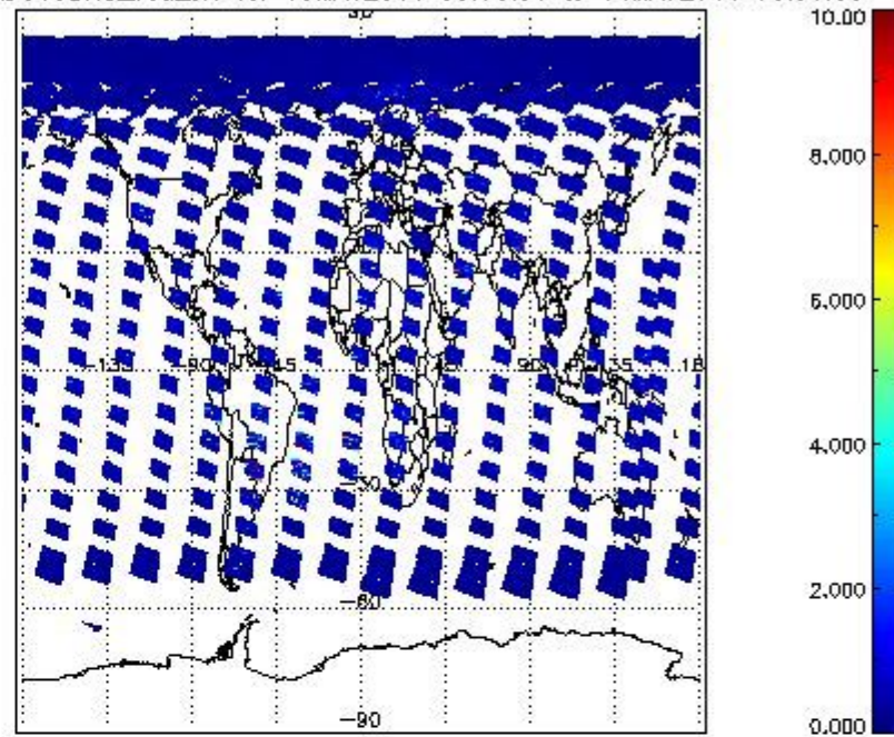
SCIOL2P_NADUV3BRO_vcd_err for 13MAY2011 00:00:00 to 14MAY2011 00:00:00
