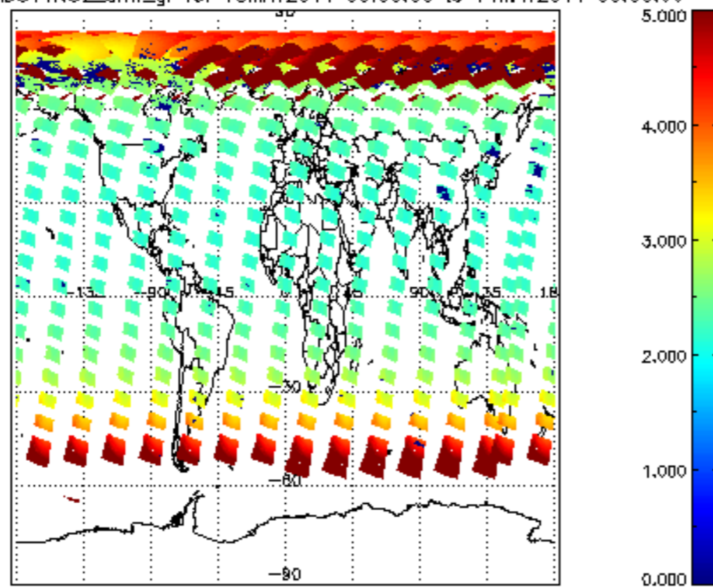
SCIOL2P_NADUV1NO2_amf_gr for 13MAY2011 00:00:00 to 14MAY2011 00:00:00
