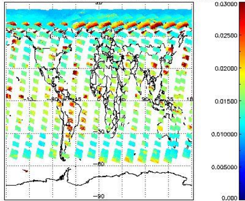
SCIOL2P_NADUV003_vcd_err for 13MAY2011 00:00:00 to 14MAY2011 00:00:00
