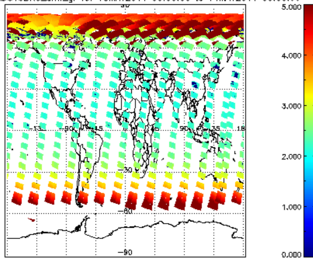
SCIOL2P_NADUV3BRO_amf_gr for 13MAY2011 00:00:00 to 14MAY2011 00:00:00
