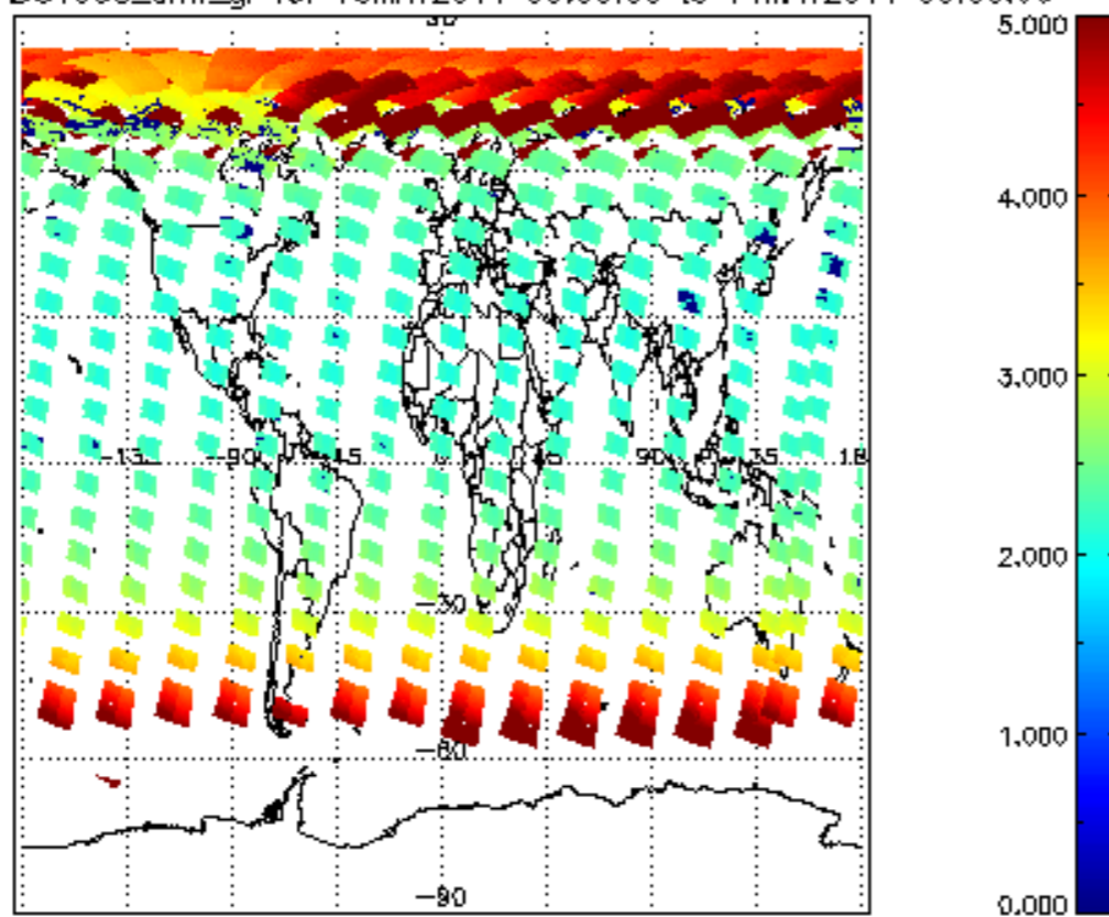
SCIOL2P_NADUV003_amf_gr for 13MAY2011 00:00:00 to 14MAY2011 00:00:00
