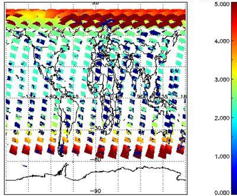
SCIOL2P_NADUV1NO2_amf_cl for 13MAY2011 00:00:00 to 14MAY2011 00:00:00
