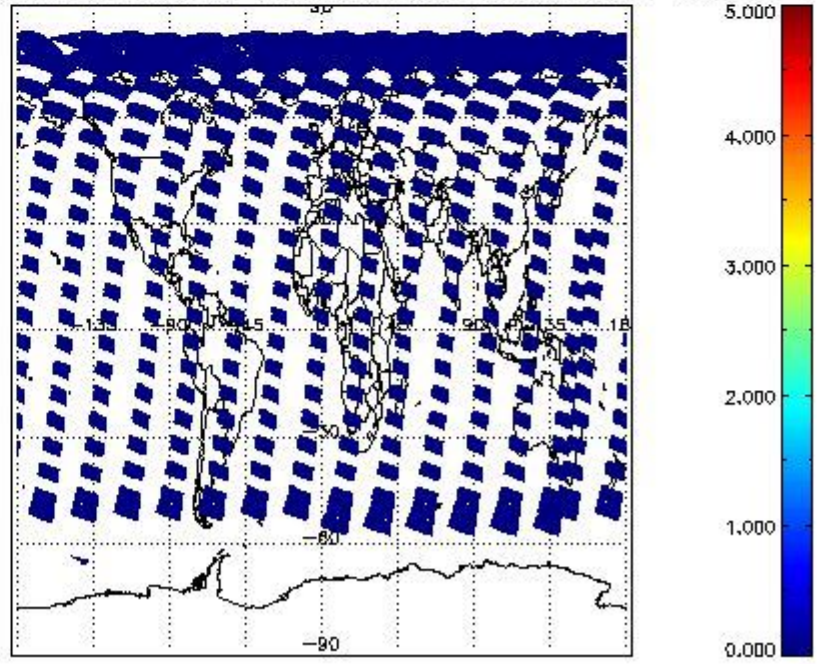
SCIOL2P_NADUV5S02_amf_cl for 13MAY2011 00:00:00 to 14MAY2011 00:00:00
