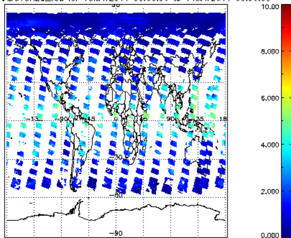
SCIOL2P_NADUV8H2O_vcd for 13MAY2011 00:00:00 to 14MAY2011 00:00:00
