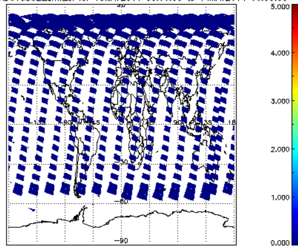
SCIOL2P_NADUV5S02_amf_cl for 13MAY2011 00:00:00 to 14MAY2011 00:00:00
