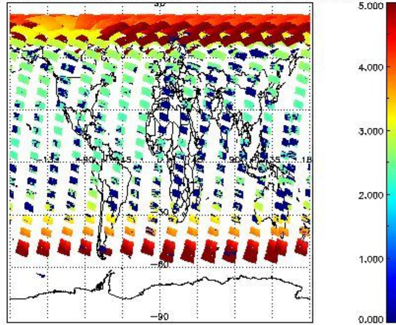
SCIOL2P_NADUV003_amf_cl for 13MAY2011 00:00:00 to 14MAY2011 00:00:00
