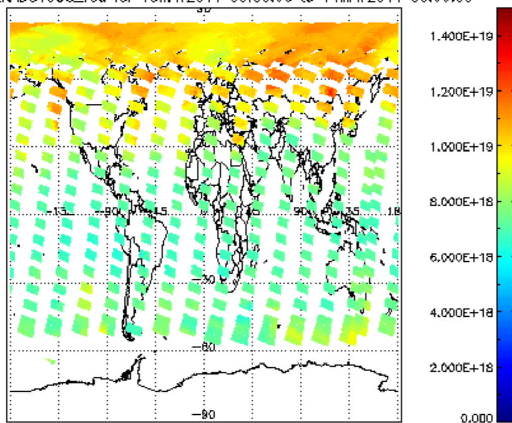
SCIOL2P_NADUV003_vcd for 13MAY2011 00:00:00 to 14MAY2011 00:00:00
