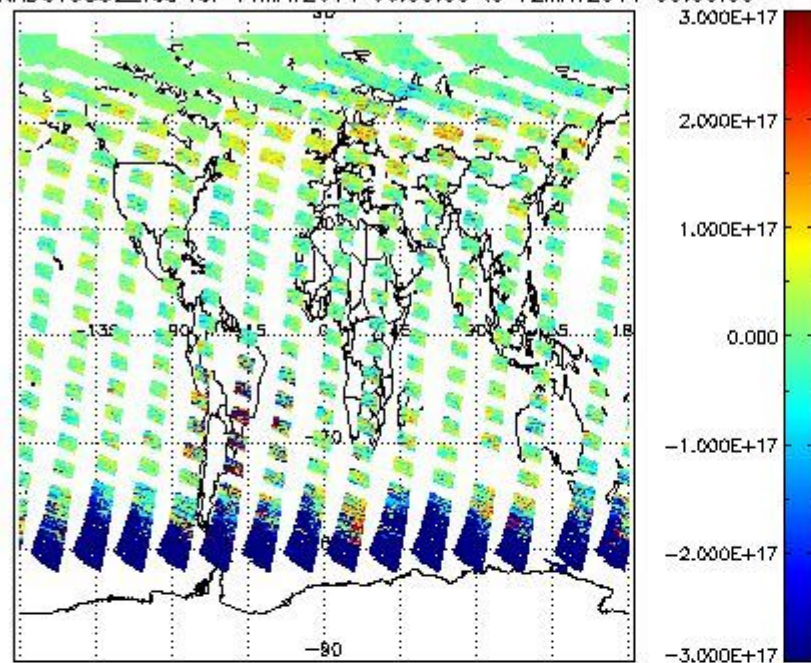
SCIOL2P_NADUV5S02_vcd for 11MAY2011 00:00:00 to 12MAY2011 00:00:00
