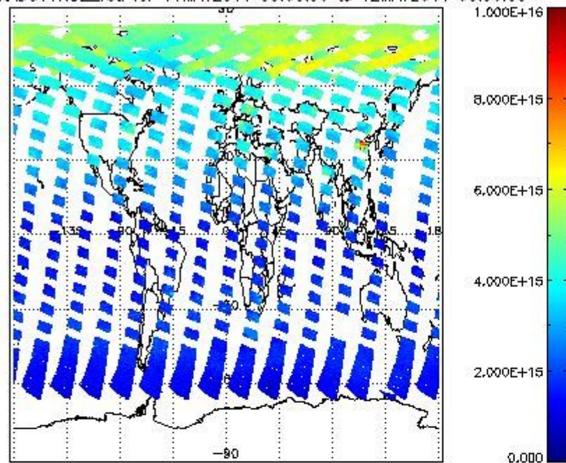
SCIOL2P_NADUV1NO2_vcd for 11MAY2011 00:00:00 to 12MAY2011 00:00:00
