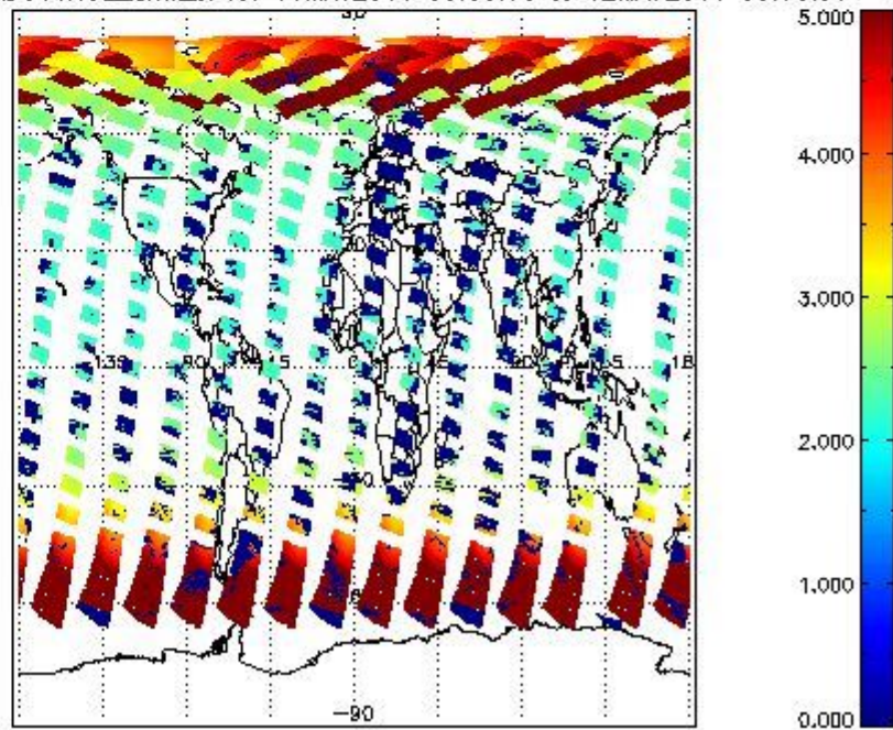
SCIOL2P_NADUV1NO2_amf_cl for 11MAY2011 00:00:00 to 12MAY2011 00:00:00
