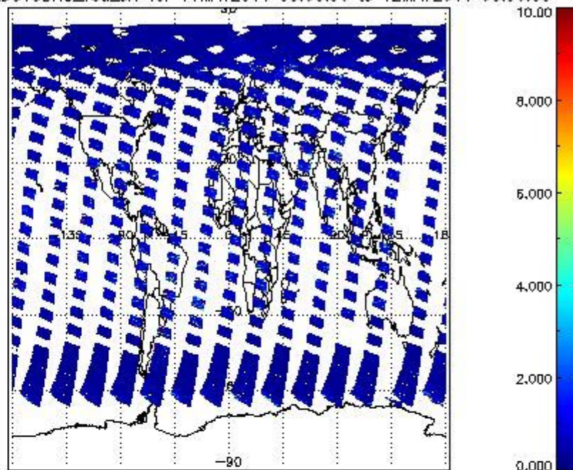
SCIOL2P_NADUV3BRO_vcd_err for 11MAY2011 00:00:00 to 12MAY2011 00:00:00
