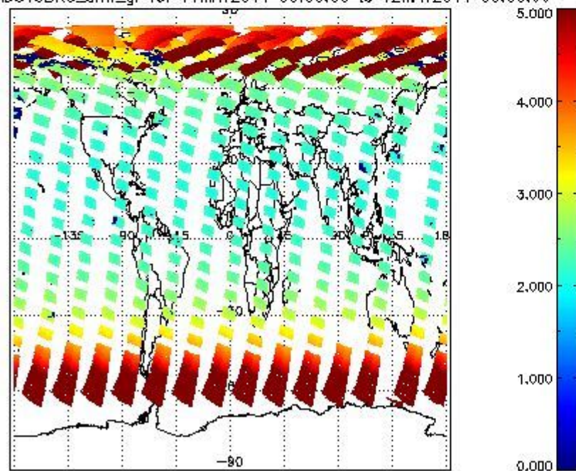
SCIOL2P_NADUV3BRO_amf_gr for 11MAY2011 00:00:00 to 12MAY2011 00:00:00
