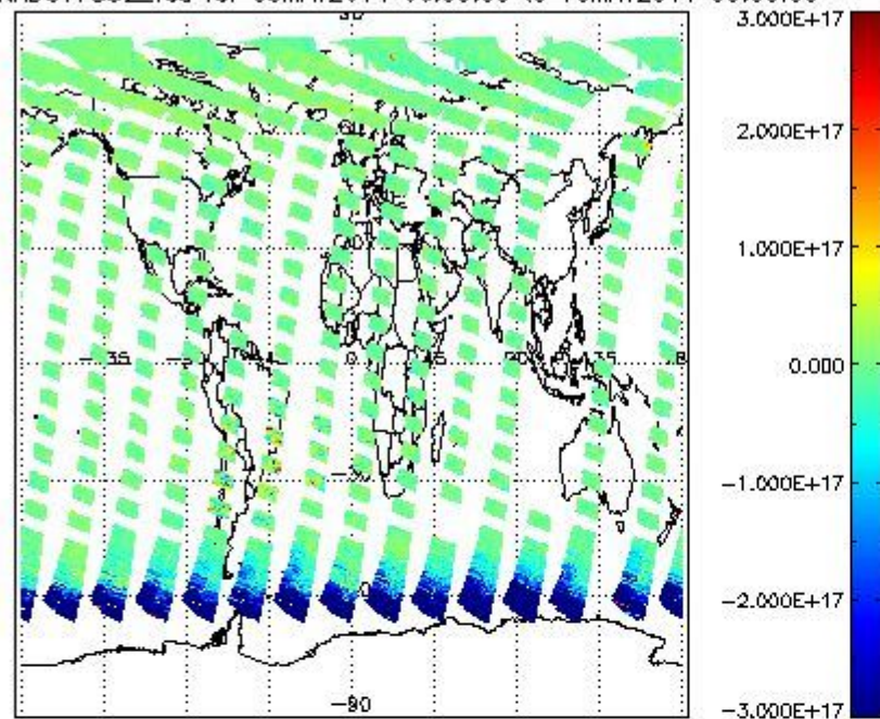
SCIOL2P_NADUV7S02_vcd for 09MAY2011 00:00:00 to 10MAY2011 00:00:00
