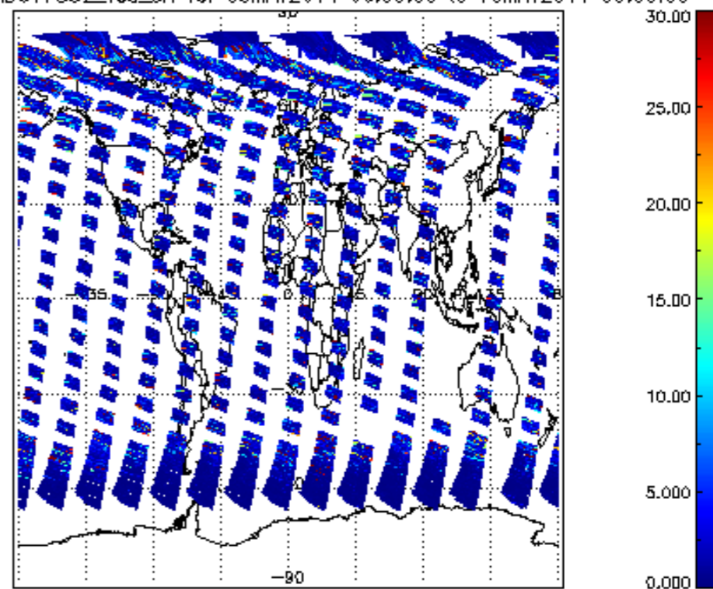
SCIOL2P_NADUV7S02_vcd_err for 09MAY2011 00:00:00 to 10MAY2011 00:00:00
