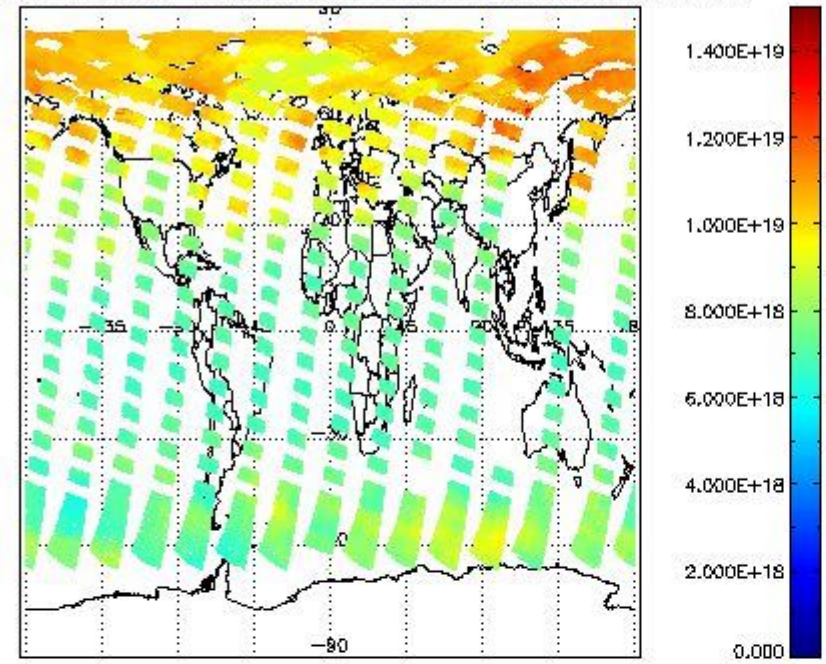
SCIOL2P_NADUV003_vcd for 09MAY2011 00:00:00 to 10MAY2011 00:00:00
