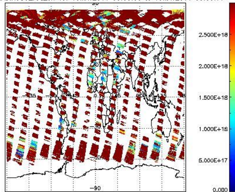
SCIDL2P_NADIR3CO_vcd_err for 09MAY2011 00:00:00 to 10MAY2011 00:00:00
