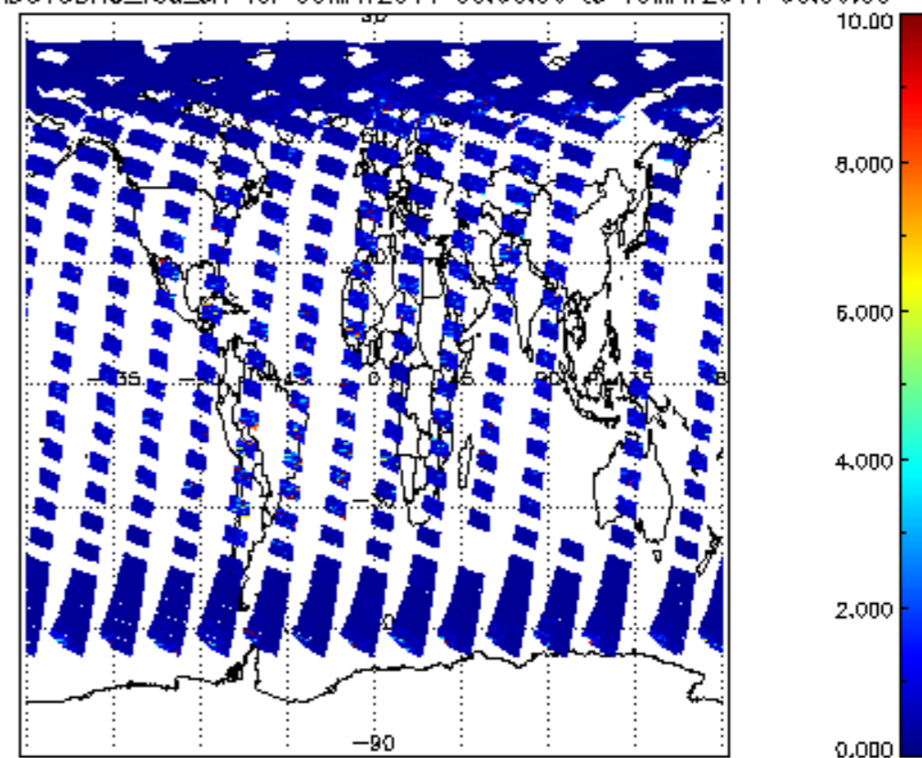
SCIOL2P_NADUV3BRO_vcd_err for 09MAY2011 00:00:00 to 10MAY2011 00:00:00
