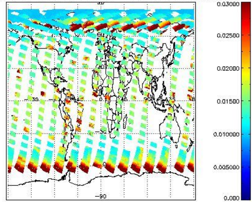
SCIOL2P_NADUV003_vcd_err for 09MAY2011 00:00:00 to 10MAY2011 00:00:00
