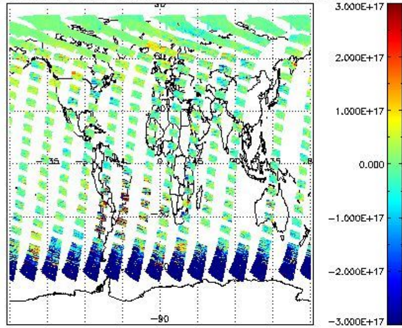
SCIOL2P_NADUV5S02_vcd for 09MAY2011 00:00:00 to 10MAY2011 00:00:00
