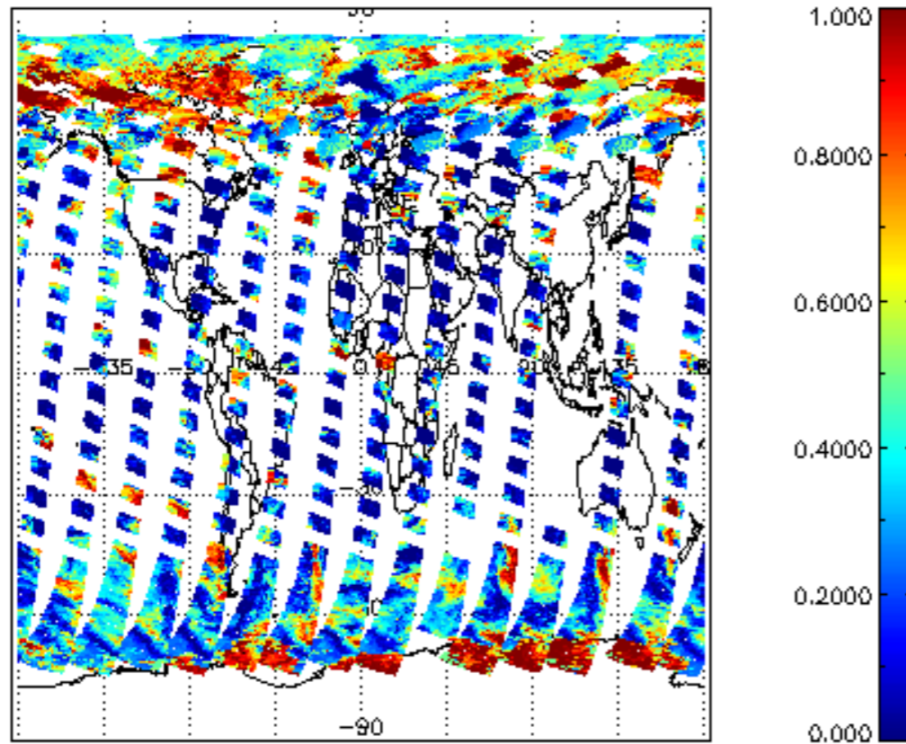
cL_frac for 09MAY2011 00:00:00 to 10MAY2011 00:00:00
