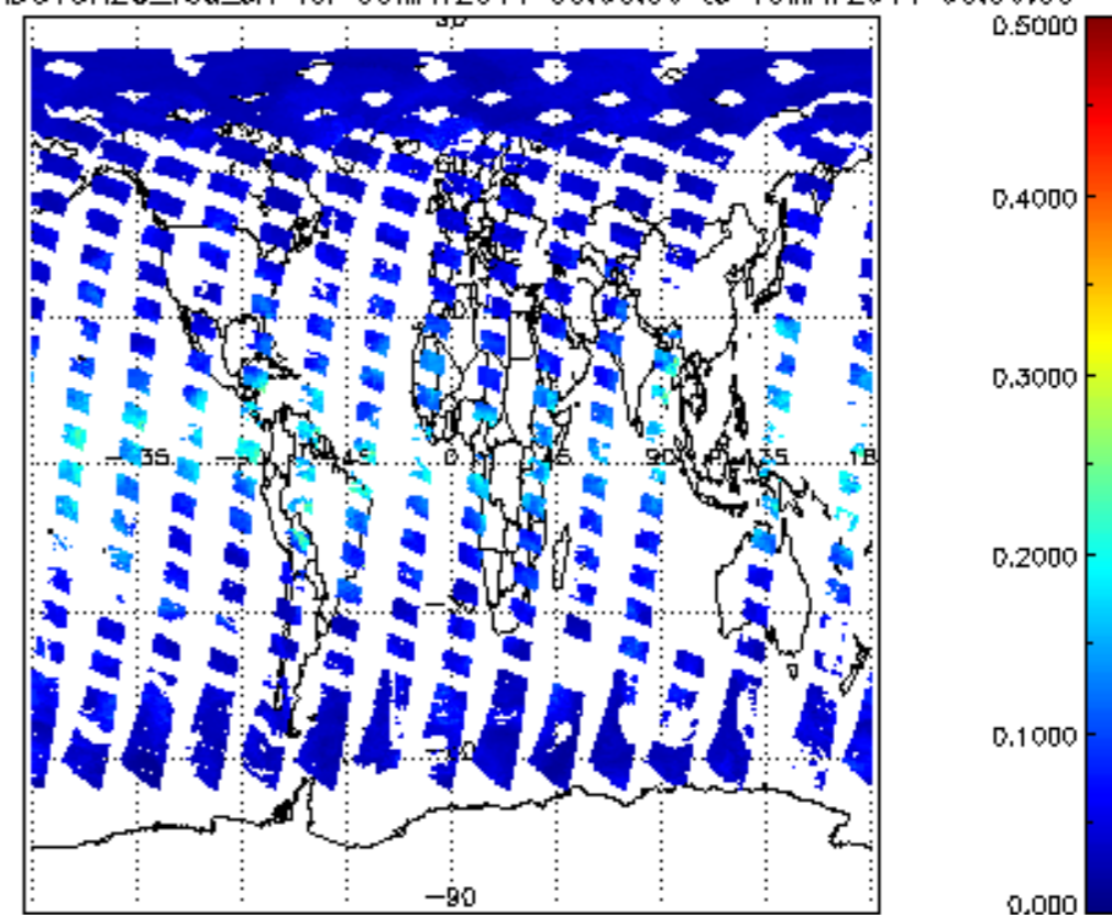
SCIOL2P_NADUV8H2O_vcd_err for 09MAY2011 00:00:00 to 10MAY2011 00:00:00
