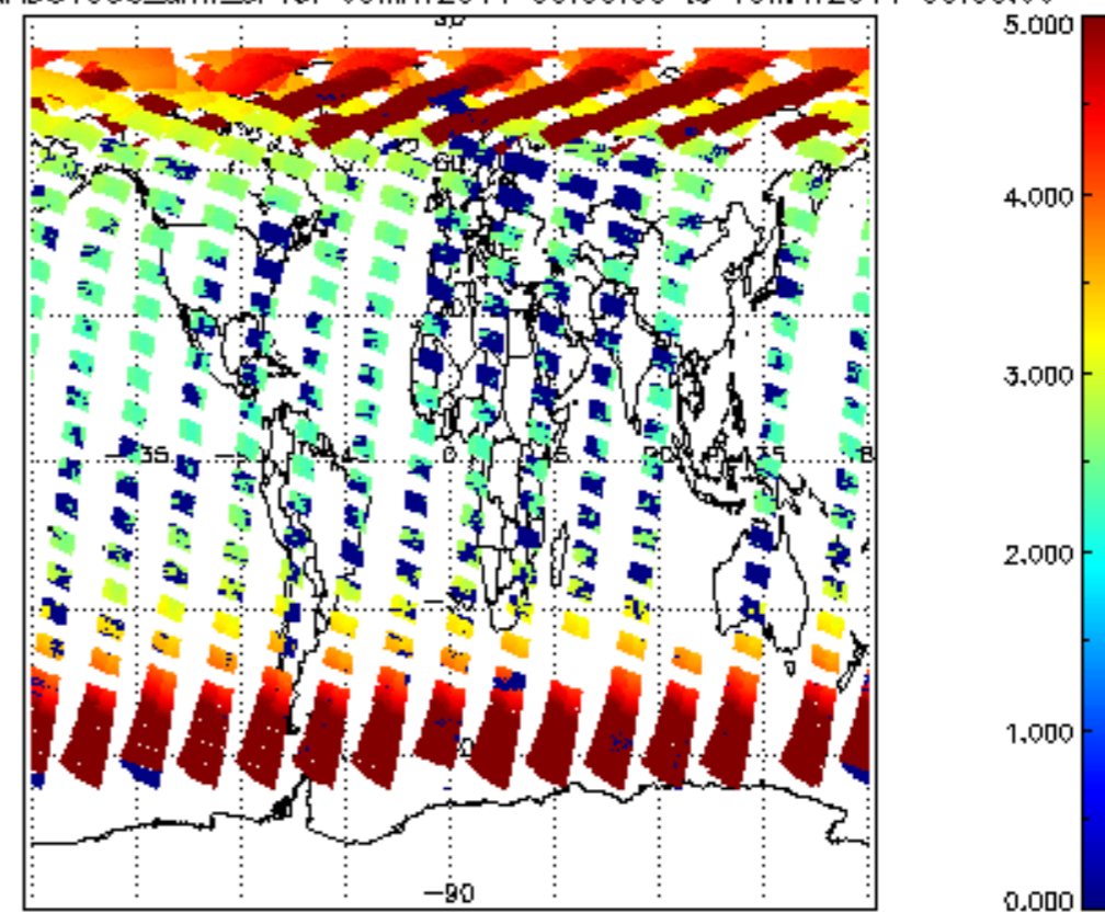
SCIOL2P_NADUV003_amf_cl for 09MAY2011 00:00:00 to 10MAY2011 00:00:00
