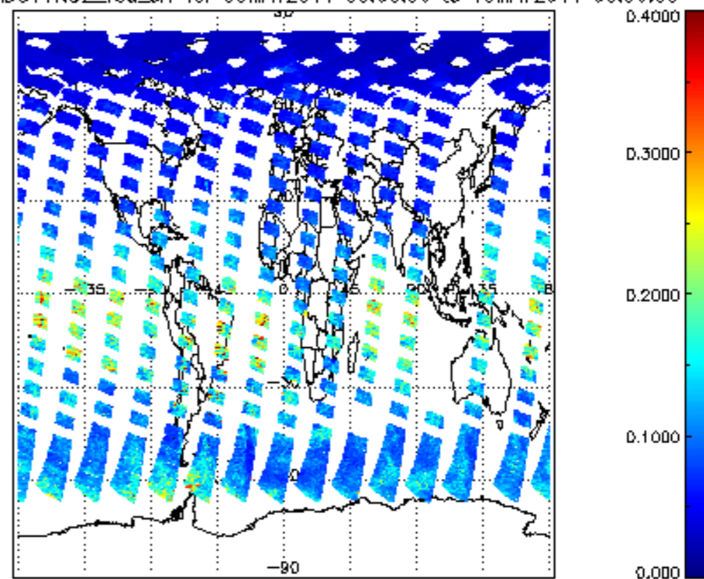
SCIOL2P_NADUV1NO2_vcd_err for 09MAY2011 00:00:00 to 10MAY2011 00:00:00
