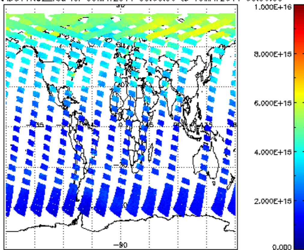
SCIOL2P_NADUV1NO2_vcd for 09MAY2011 00:00:00 to 10MAY2011 00:00:00
