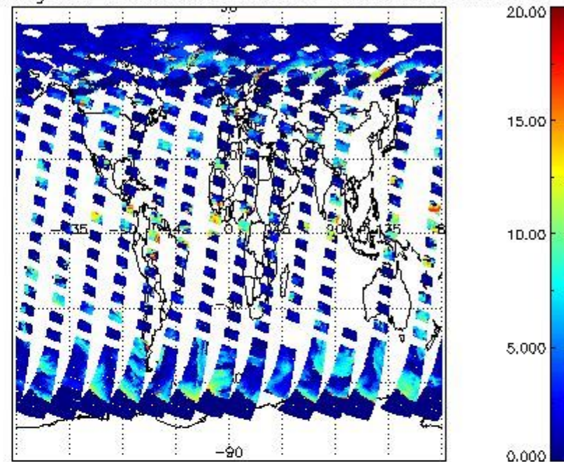
cL_top_height for 09MAY2011 00:00:00 to 10MAY2011 00:00:00
