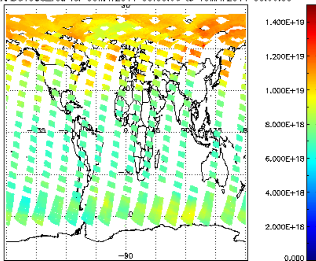
SCIOL2P_NADUV003_vcd for 09MAY2011 00:00:00 to 10MAY2011 00:00:00
