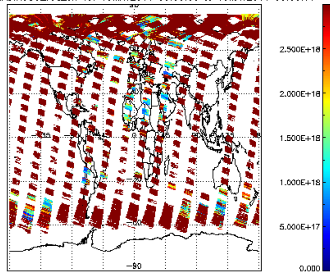
SCIOL2P_NADIR3CO_vcd_err for 09MAY2011 00:00:00 to 10MAY2011 00:00:00
