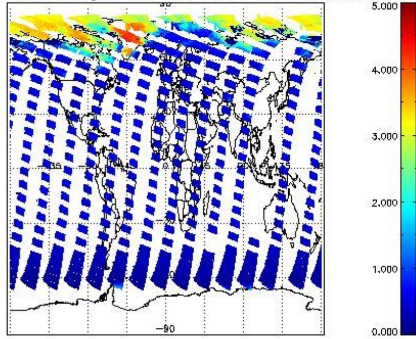
SCIOL2P_NADUV5S02_amf_gr for 09MAY2011 00:00:00 to 10MAY2011 00:00:00
