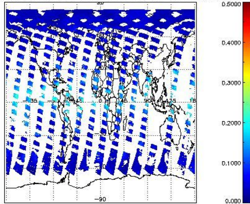
SCIOL2P_NADUV8H2O_vcd_err for 09MAY2011 00:00:00 to 10MAY2011 00:00:00
