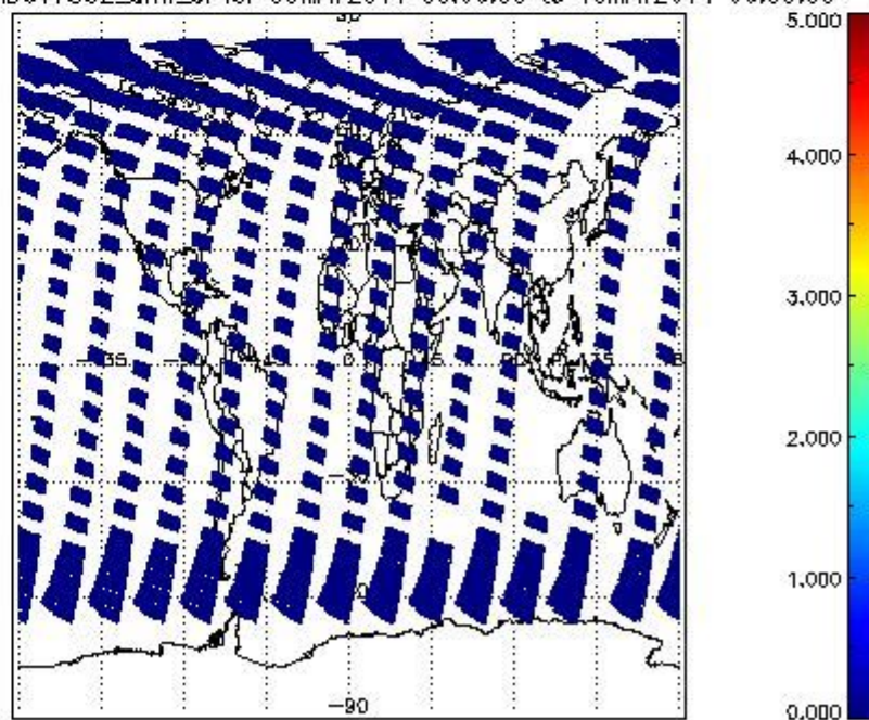
SCIOL2P_NADUV7S02_amf_cl for 09MAY2011 00:00:00 to 10MAY2011 00:00:00
