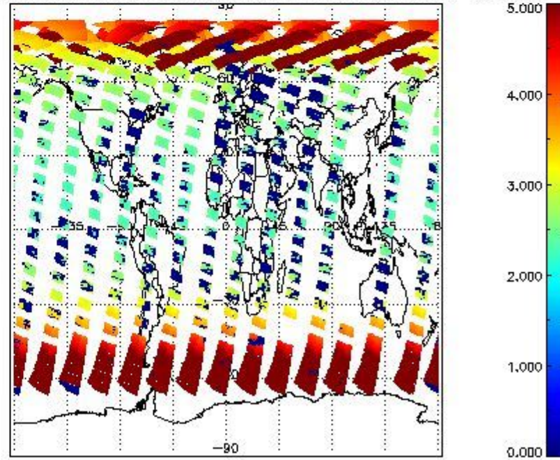
SCIOL2P_NADUV3BRO_amf_cl for 09MAY2011 00:00:00 to 10MAY2011 00:00:00
