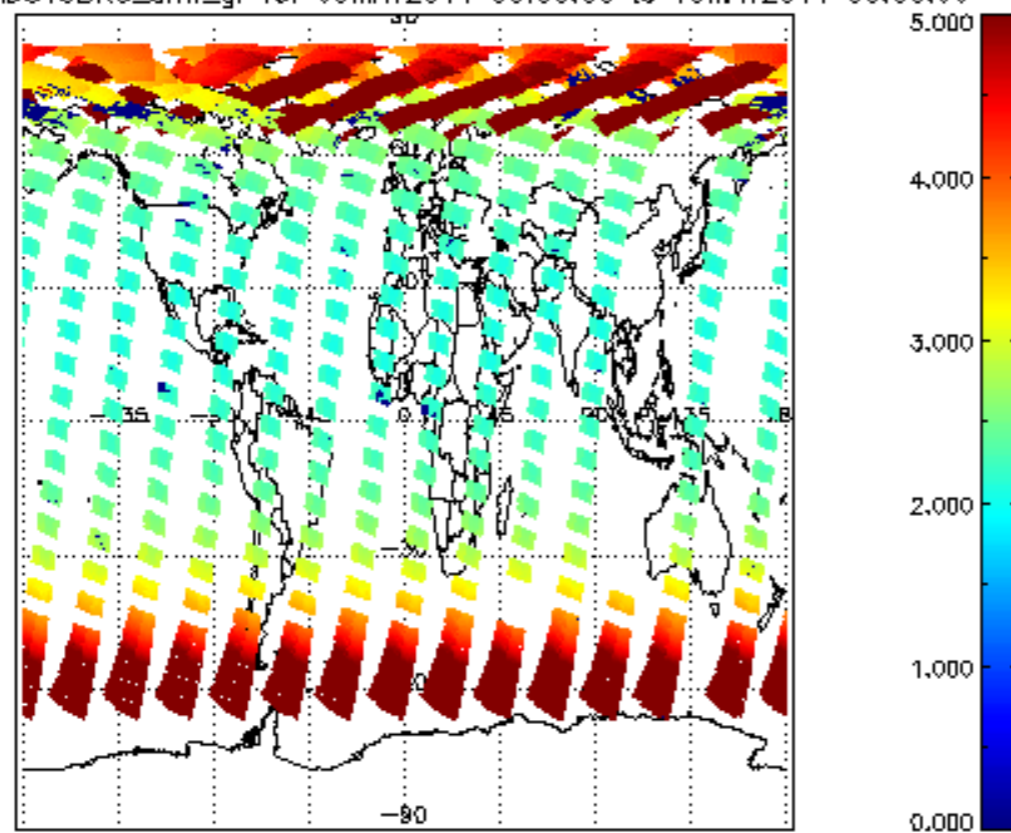
SCIOL2P_NADUV3BRO_amf_gr for 09MAY2011 00:00:00 to 10MAY2011 00:00:00
