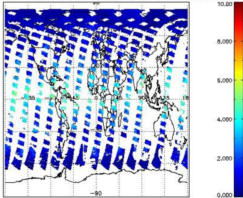
SCIOL2P_NADUV8H2O_vcd for 09MAY2011 00:00:00 to 10MAY2011 00:00:00
