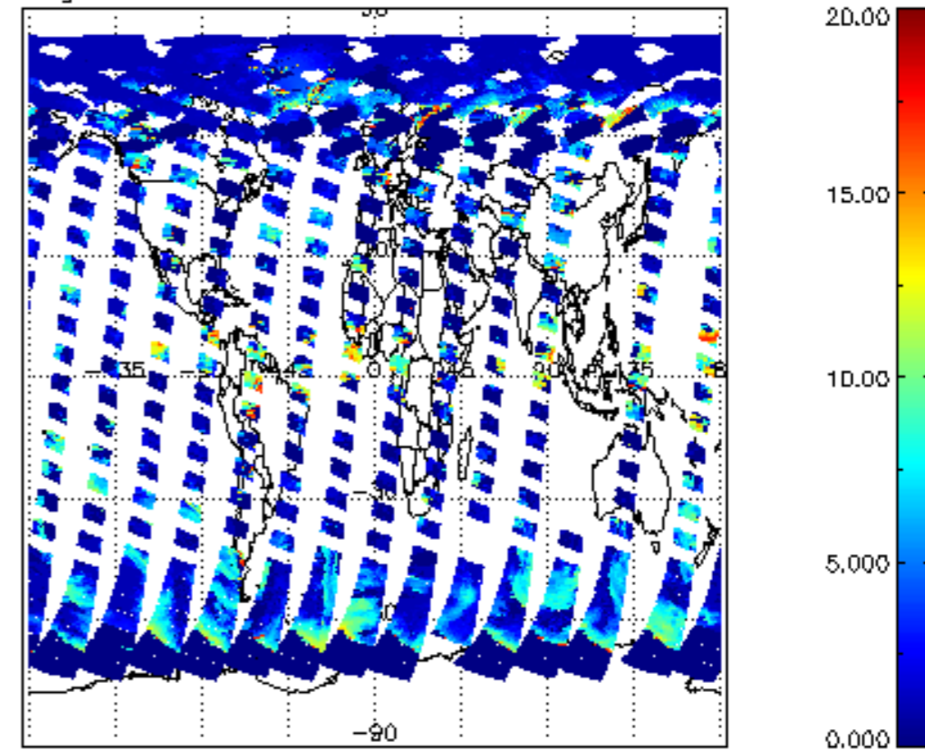
cL_top_height for 09MAY2011 00:00:00 to 10MAY2011 00:00:00
