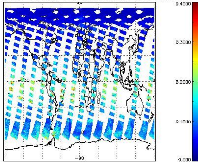
SCIOL2P_NADUV1NO2_vcd_err for 09MAY2011 00:00:00 to 10MAY2011 00:00:00
