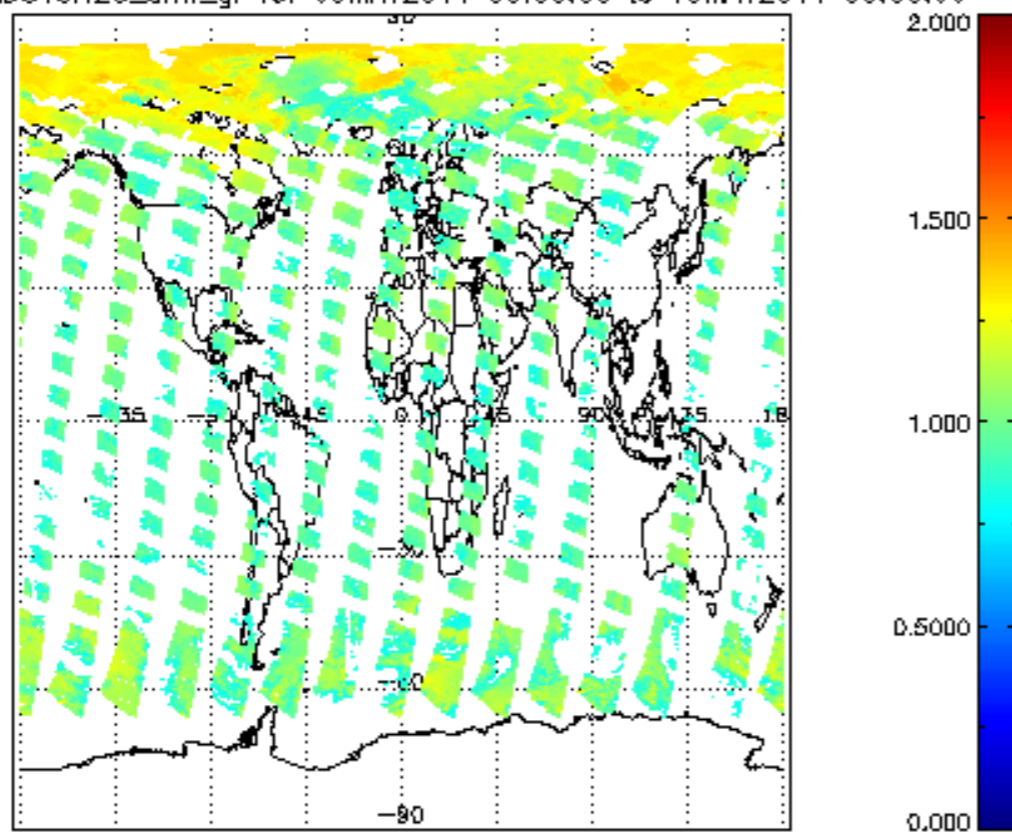
SCIOL2P_NADUV8H2O_amf_gr for 09MAY2011 00:00:00 to 10MAY2011 00:00:00
