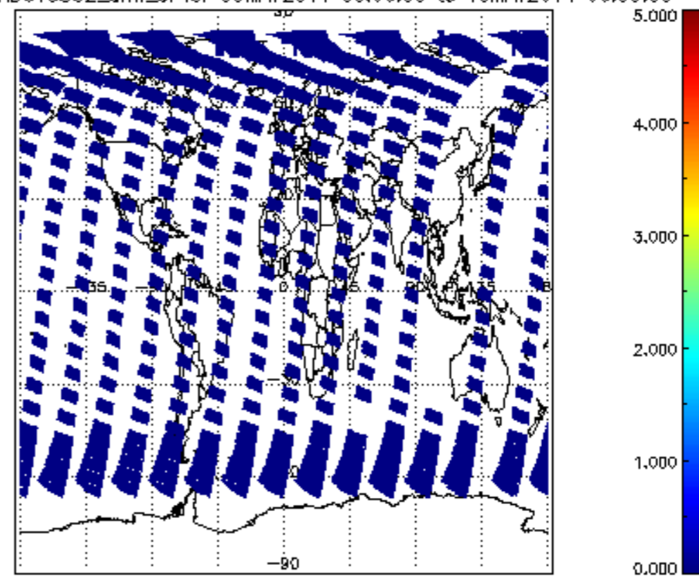
SCIOL2P_NADUV5S02_amf_cl for 09MAY2011 00:00:00 to 10MAY2011 00:00:00
