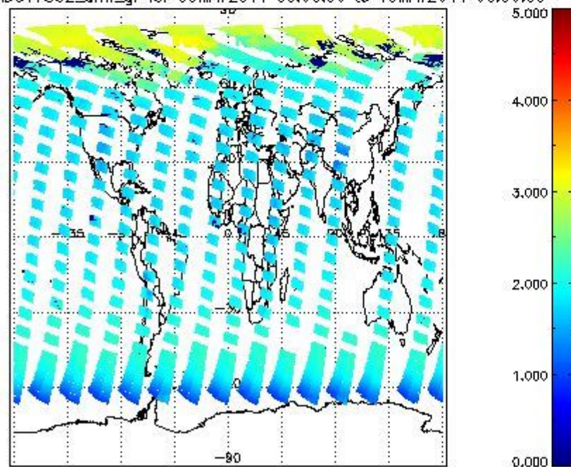
SCIOL2P_NADUV7S02_amf_gr for 09MAY2011 00:00:00 to 10MAY2011 00:00:00
