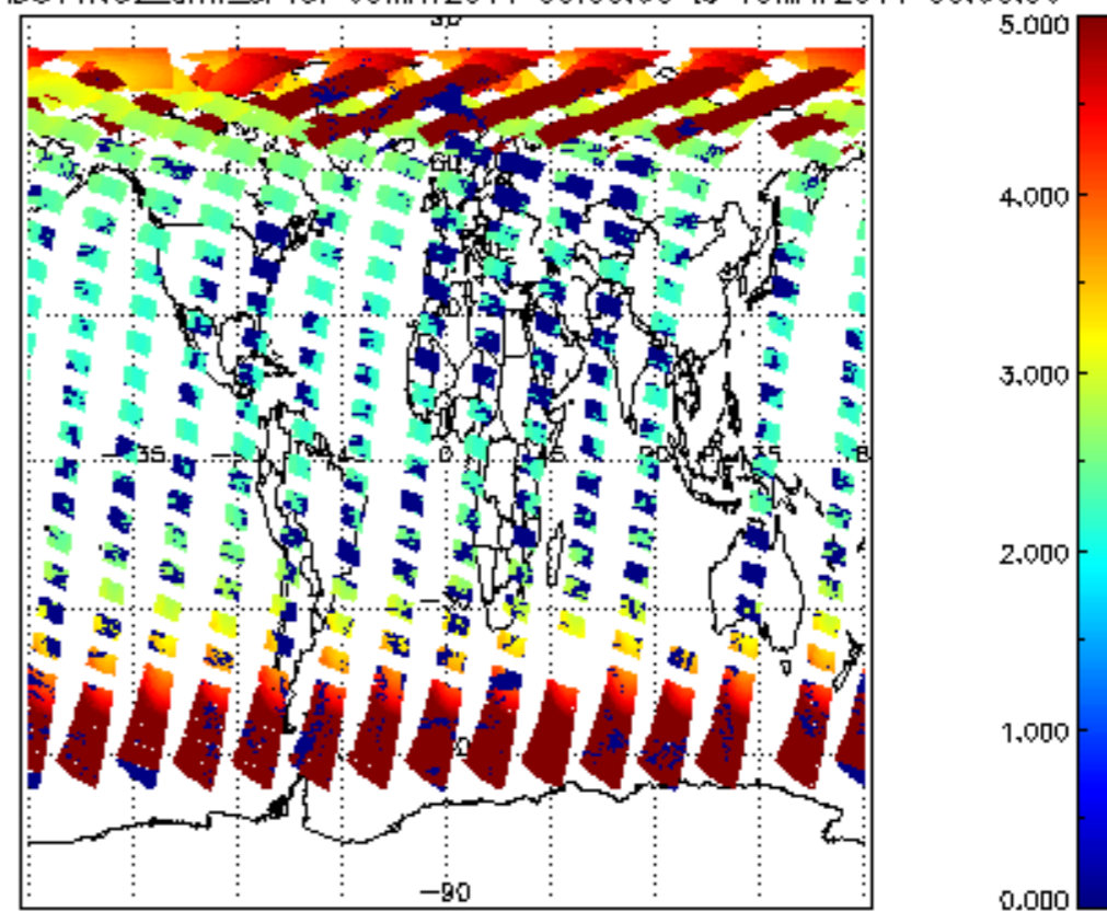
SCIOL2P_NADUV1NO2_amf_cl for 09MAY2011 00:00:00 to 10MAY2011 00:00:00
