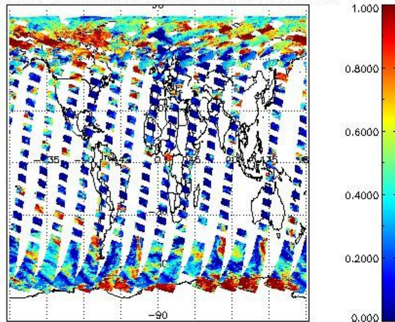
cL_frac for 09MAY2011 00:00:00 to 10MAY2011 00:00:00
