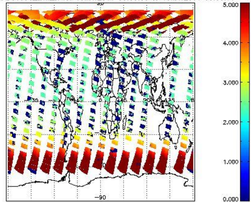
SCIOL2P_NADUV003_amf_cl for 09MAY2011 00:00:00 to 10MAY2011 00:00:00
