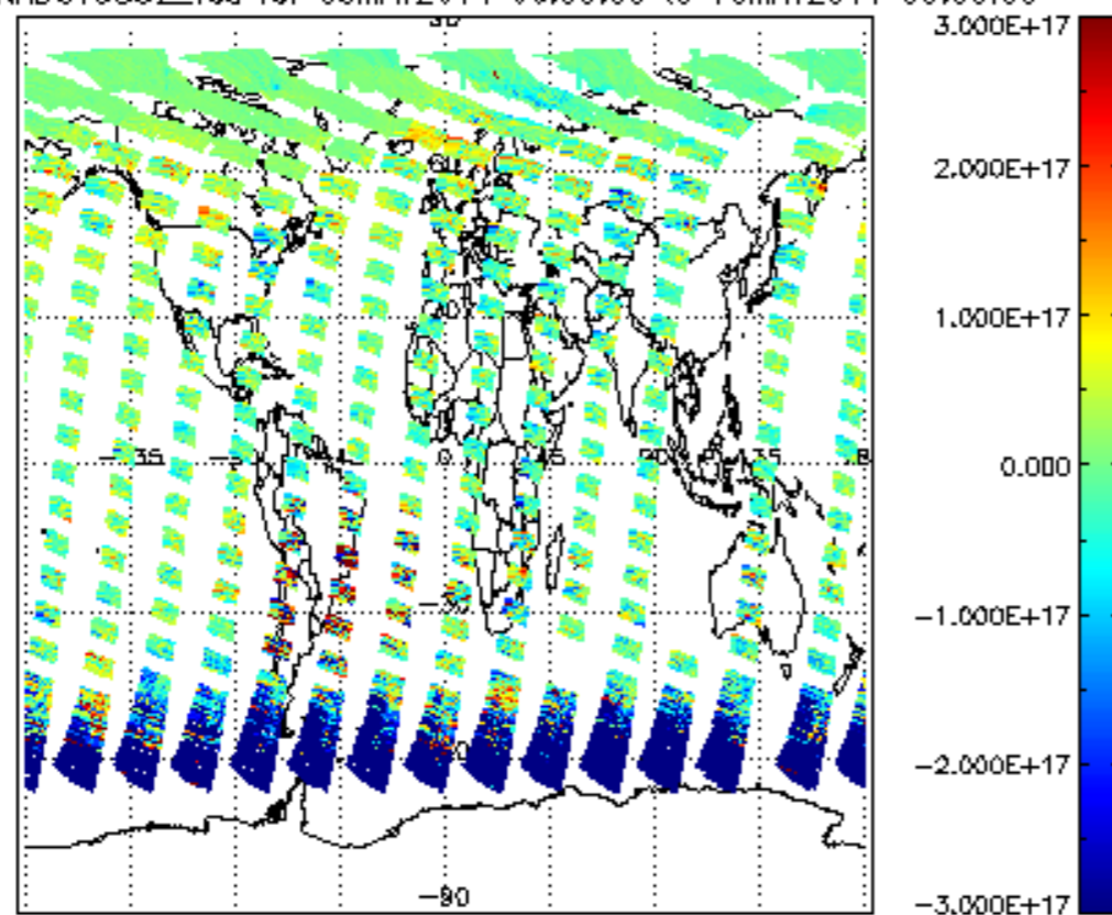
SCIOL2P_NADUV5S02_vcd for 09MAY2011 00:00:00 to 10MAY2011 00:00:00
