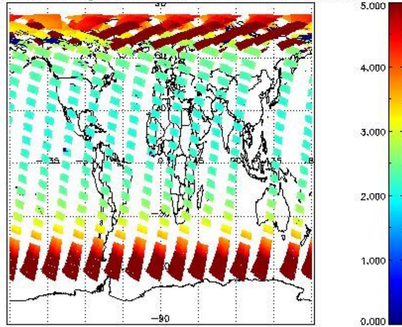
SCIOL2P_NADUV3BRO_amf_gr for 09MAY2011 00:00:00 to 10MAY2011 00:00:00
