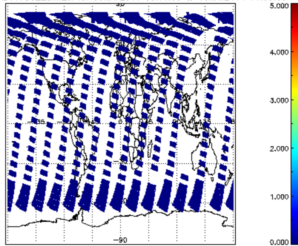
SCIOL2P_NADUV7S02_amf_cl for 09MAY2011 00:00:00 to 10MAY2011 00:00:00
