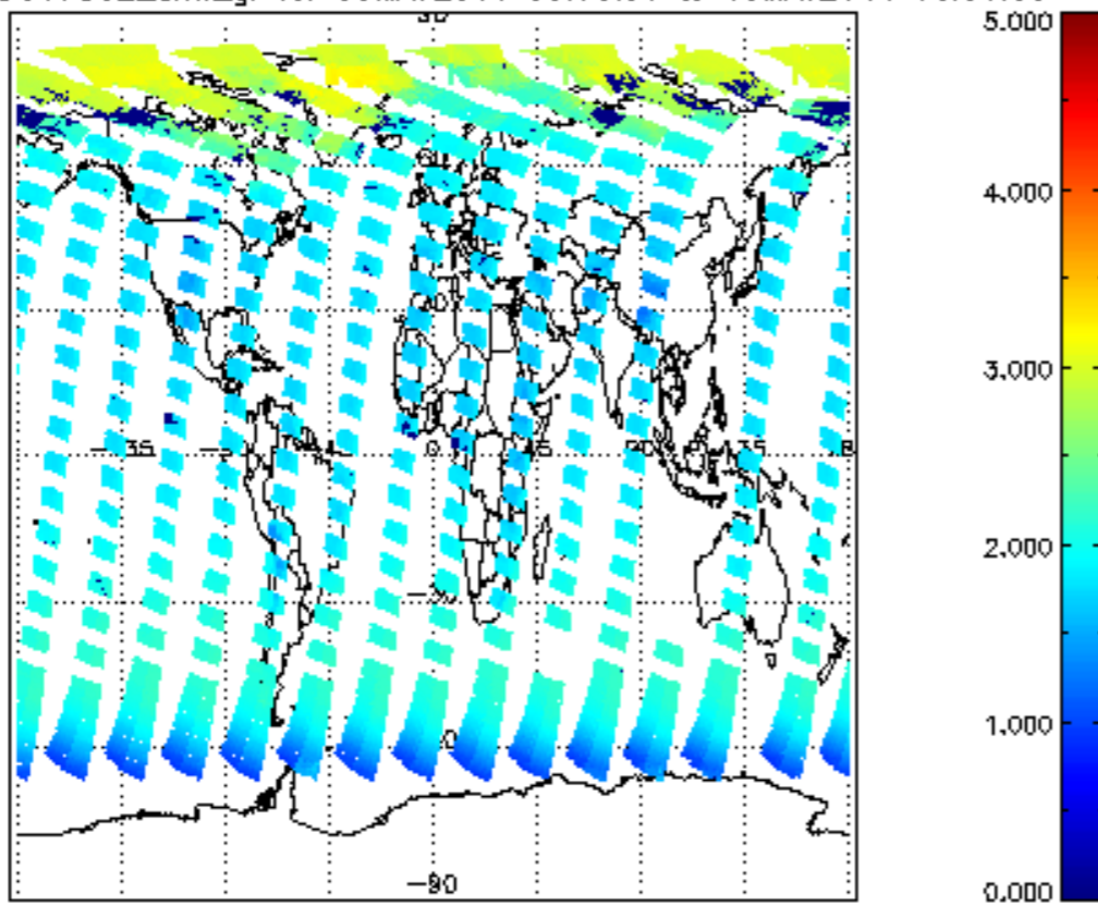
SCIOL2P_NADUV7S02_amf_gr for 09MAY2011 00:00:00 to 10MAY2011 00:00:00
