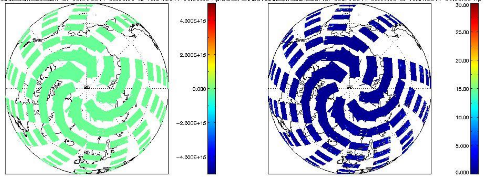
CIOL2P_NADUV60CLslant_col_den for 09MAY2011 00:00:00 to 10MAY2011 00:00:00 np; CIOL2P_NADUV60CLarr_slant_col for 09MAY2011 00:00:00 to 10MAY2011 00:00:00 np
