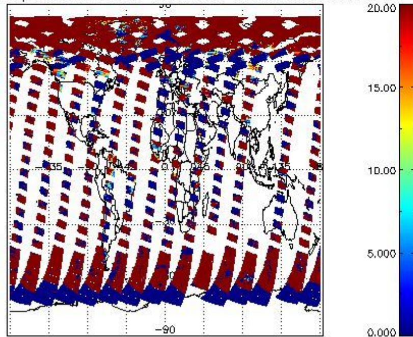
cL_opt_depth for 09MAY2011 00:00:00 to 10MAY2011 00:00:00
