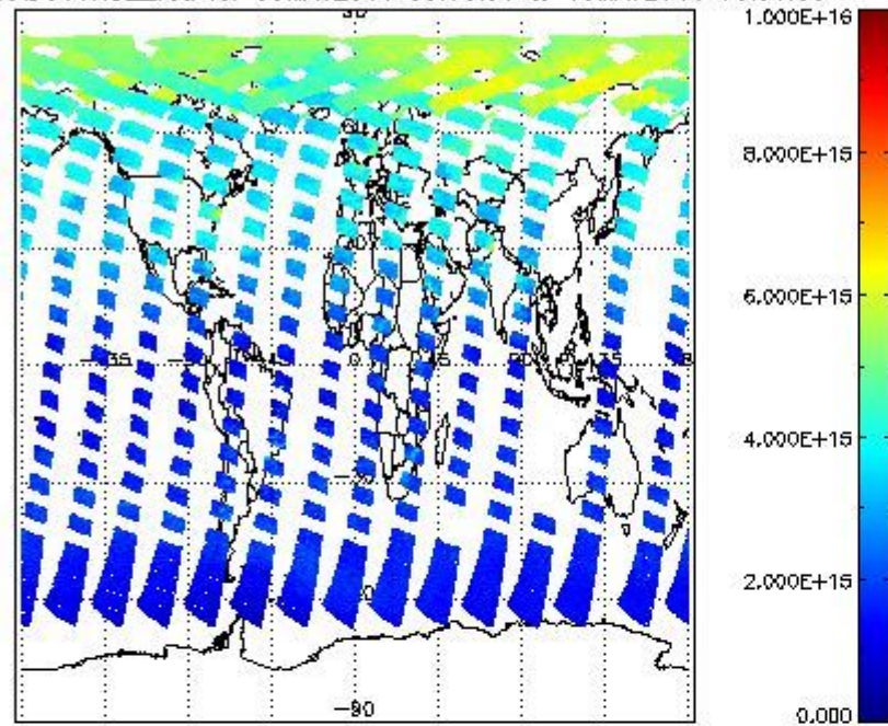
SCIOL2P_NADUV1NO2_vcd for 09MAY2011 00:00:00 to 10MAY2011 00:00:00
