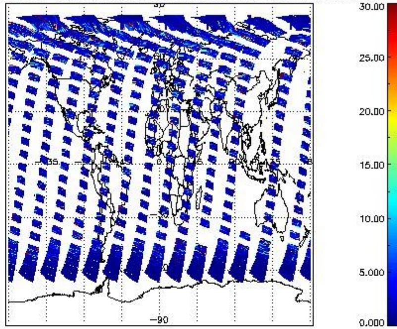
SCIOL2P_NADUV5S02_vcd_err for 09MAY2011 00:00:00 to 10MAY2011 00:00:00
