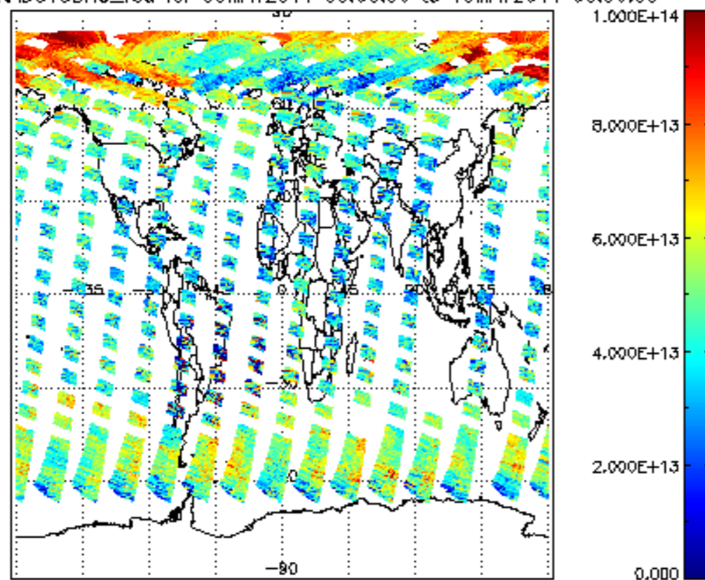
SCIOL2P_NADUV3BRO_vcd for 09MAY2011 00:00:00 to 10MAY2011 00:00:00
