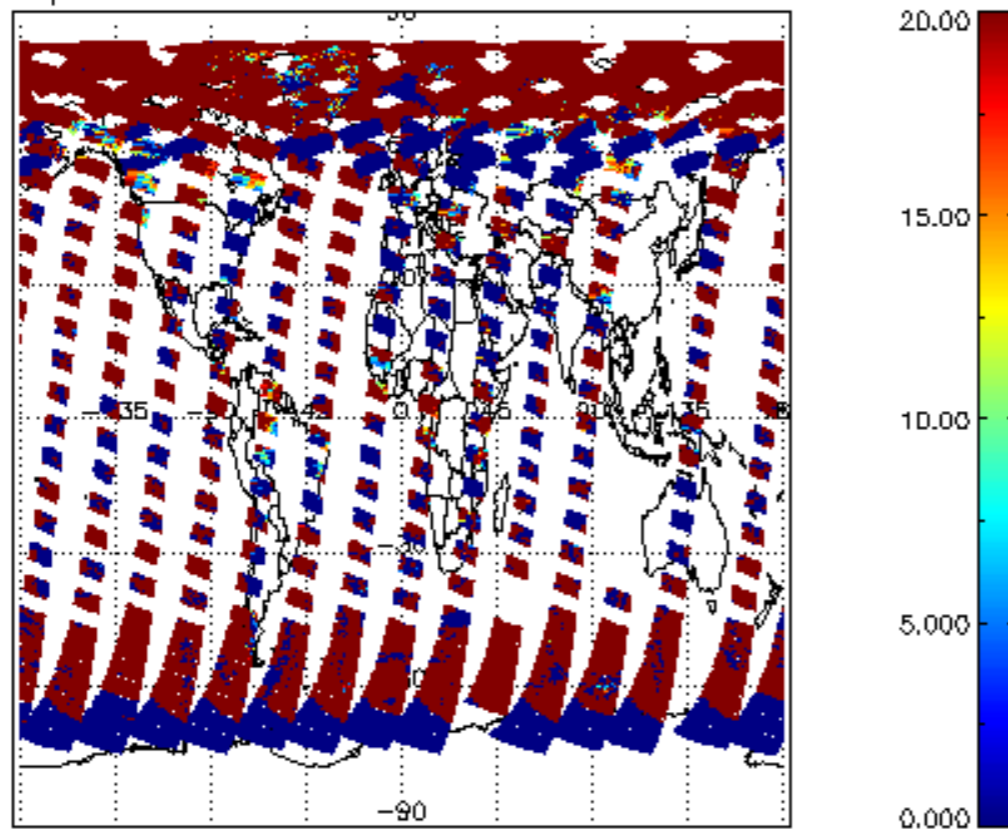
cL_opt_depth for 09MAY2011 00:00:00 to 10MAY2011 00:00:00
