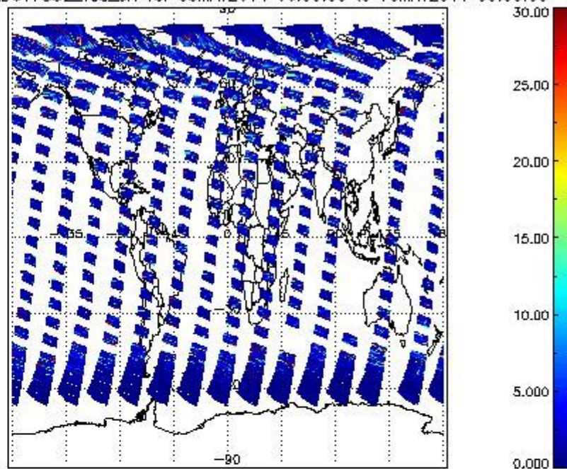
SCIOL2P_NADUV7S02_vcd_err for 09MAY2011 00:00:00 to 10MAY2011 00:00:00
