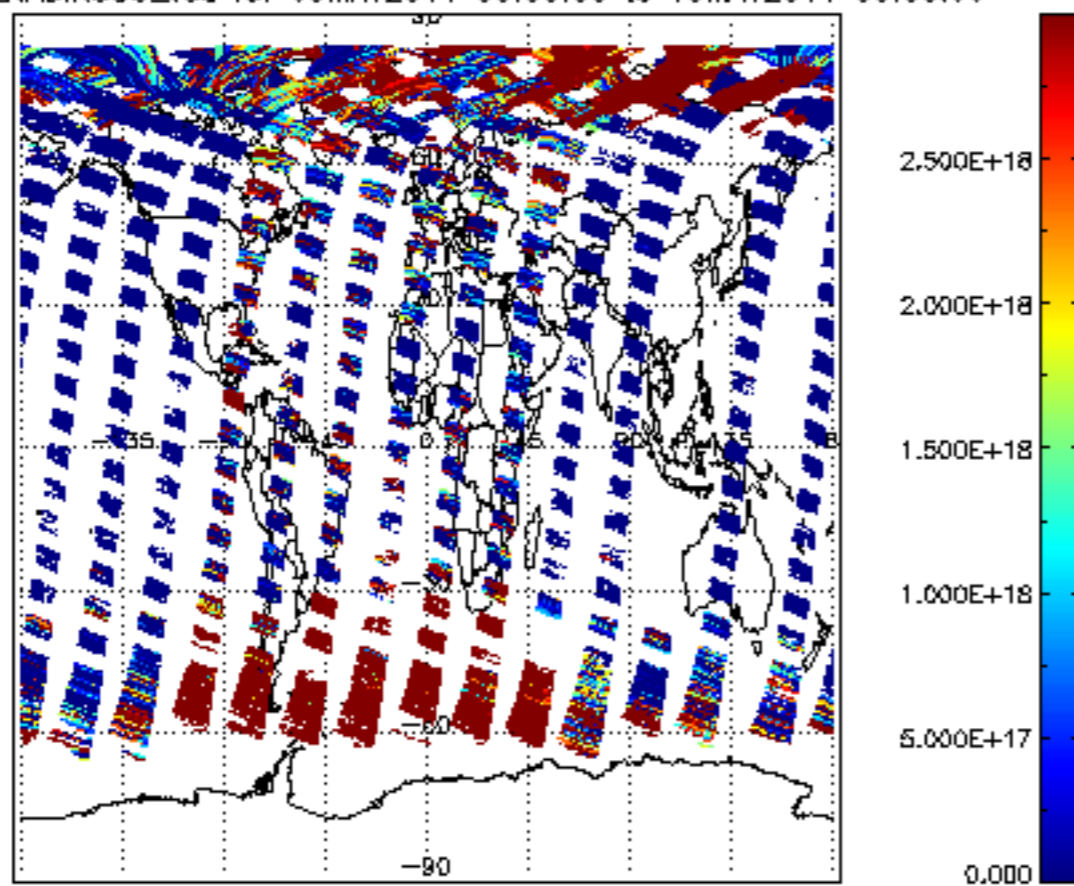
SCIOL2P_NADIR3CO_vcd for 09MAY2011 00:00:00 to 10MAY2011 00:00:00
