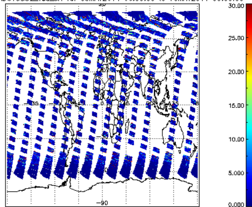
SCIOL2P_NADUV5S02_vcd_err for 09MAY2011 00:00:00 to 10MAY2011 00:00:00
