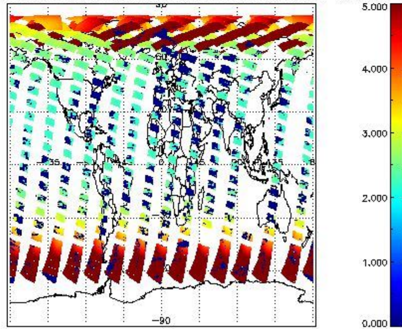
SCIOL2P_NADUV1NO2_amf_cl for 09MAY2011 00:00:00 to 10MAY2011 00:00:00
