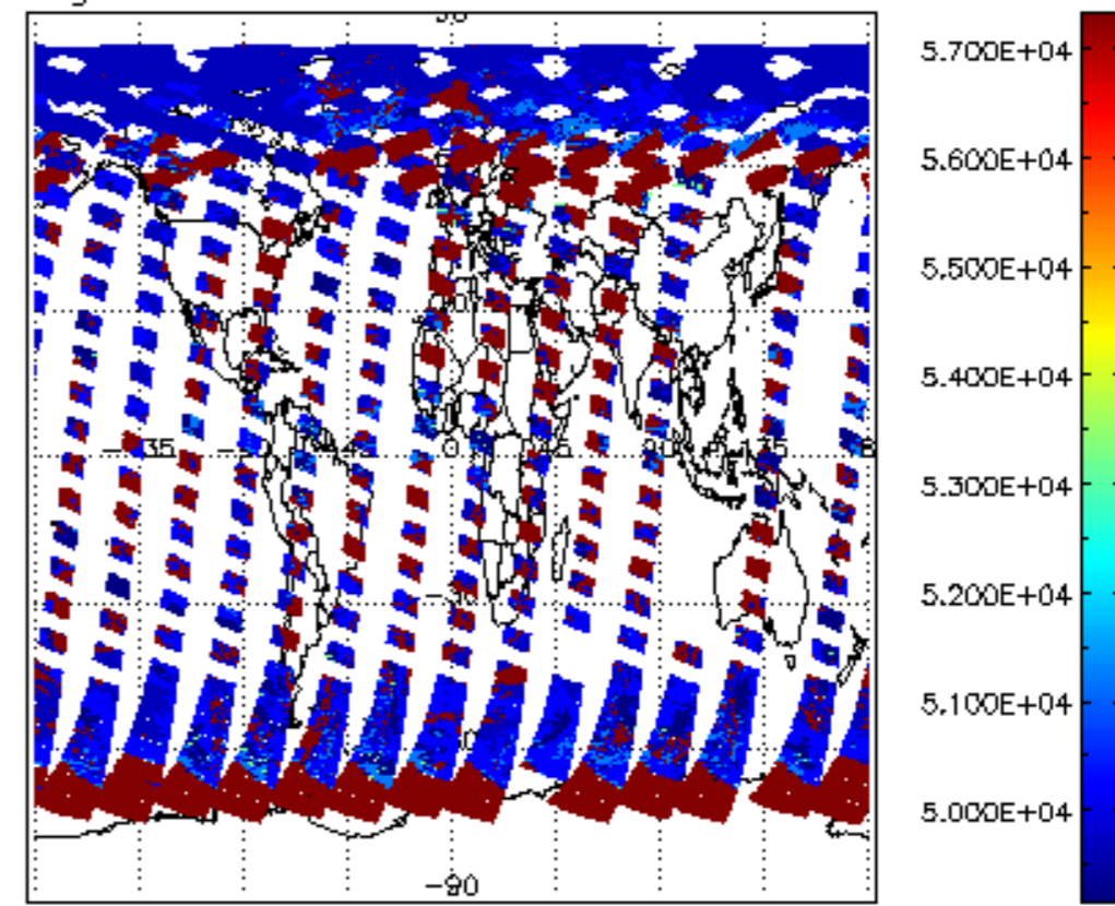
cloud_flags for 09MAY2011 00:00:00 to 10MAY2011 00:00:00
