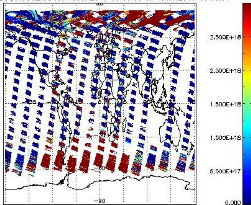
SCIDL2P_NADIR3CO_vcd for 09MAY2011 00:00:00 to 10MAY2011 00:00:00
