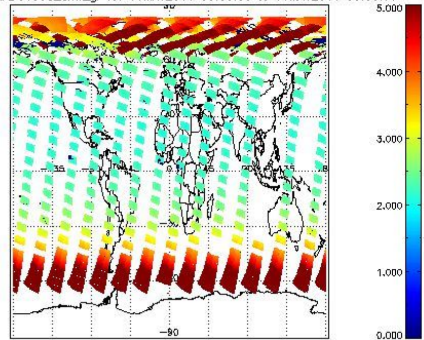
SCIOL2P_NADUV003_amf_gr for 09MAY2011 00:00:00 to 10MAY2011 00:00:00
