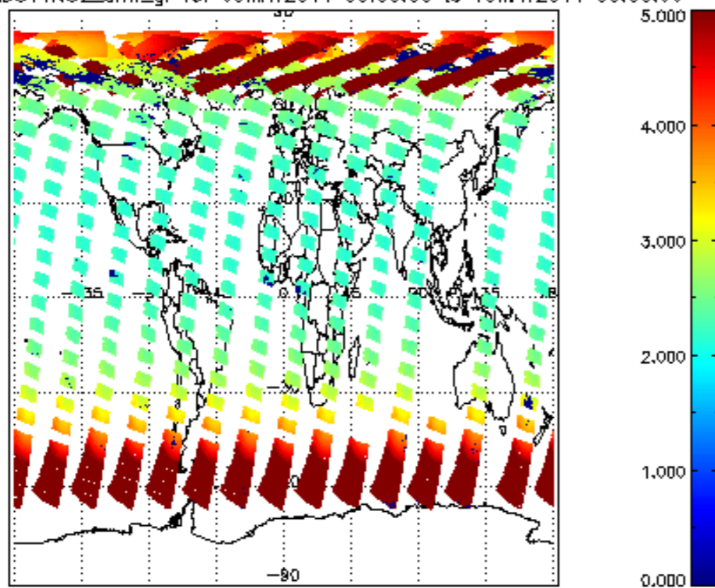
SCIOL2P_NADUV1NO2_amf_gr for 09MAY2011 00:00:00 to 10MAY2011 00:00:00
