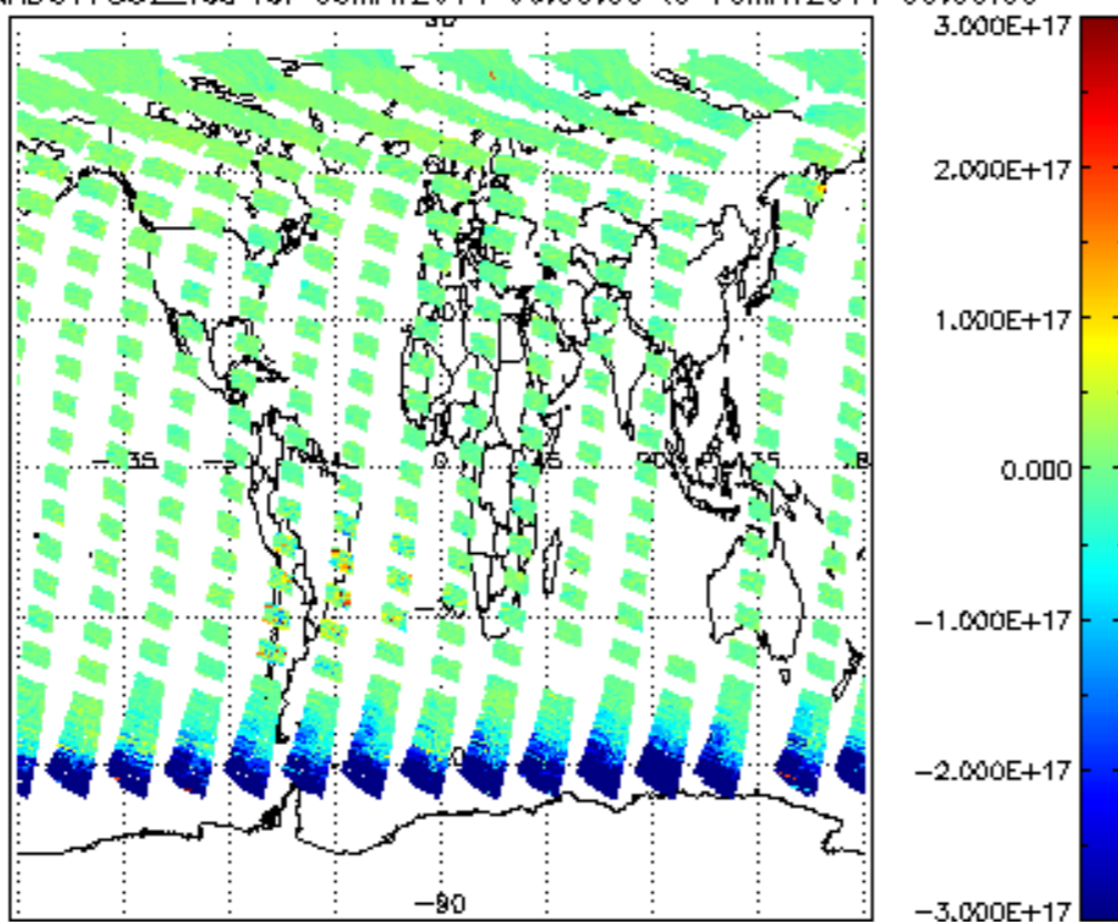
SCIOL2P_NADUV7S02_vcd for 09MAY2011 00:00:00 to 10MAY2011 00:00:00
