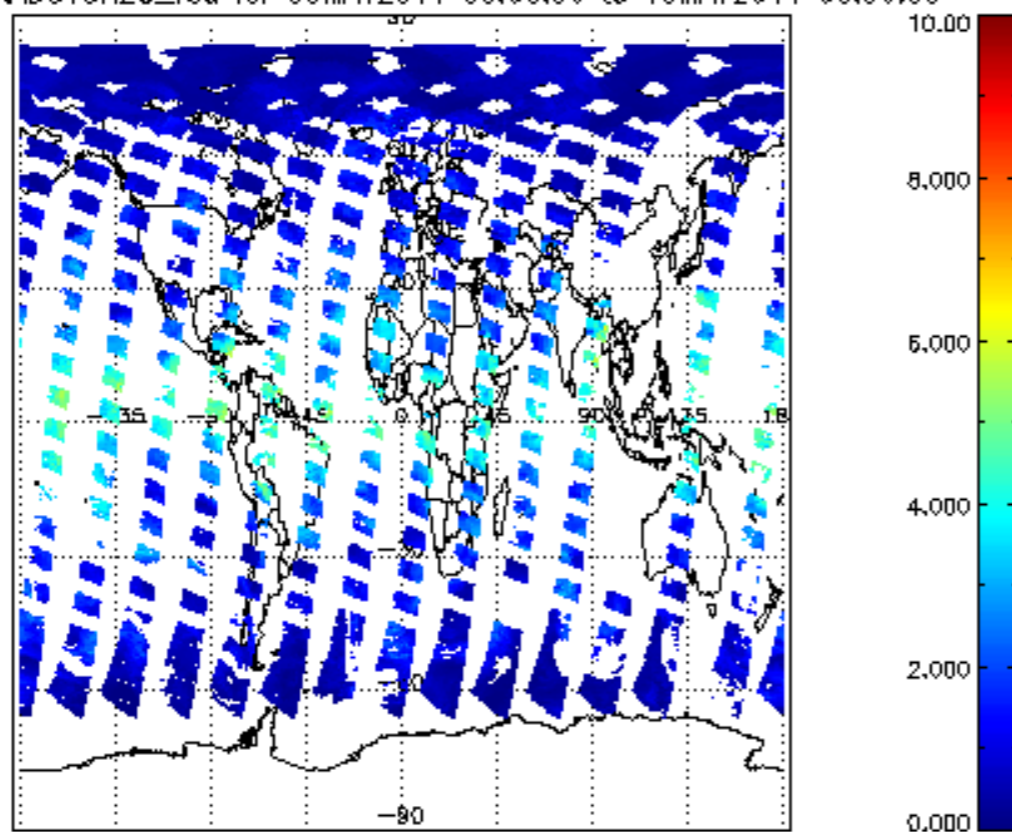
SCIOL2P_NADUV8H2O_vcd for 09MAY2011 00:00:00 to 10MAY2011 00:00:00
