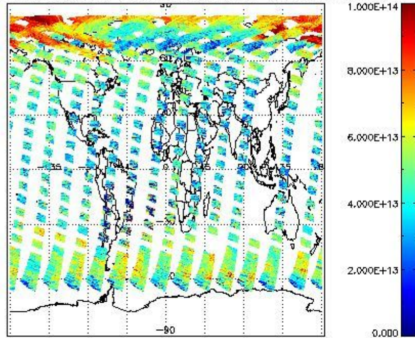
SCIOL2P_NADUV3BRO_vcd for 09MAY2011 00:00:00 to 10MAY2011 00:00:00
