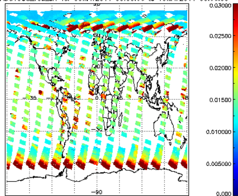
SCIOL2P_NADUV003_vcd_err for 09MAY2011 00:00:00 to 10MAY2011 00:00:00
