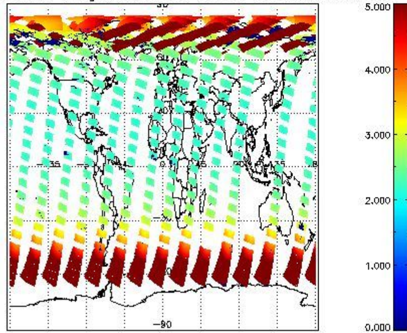
SCIOL2P_NADUV1NO2_amf_gr for 09MAY2011 00:00:00 to 10MAY2011 00:00:00
