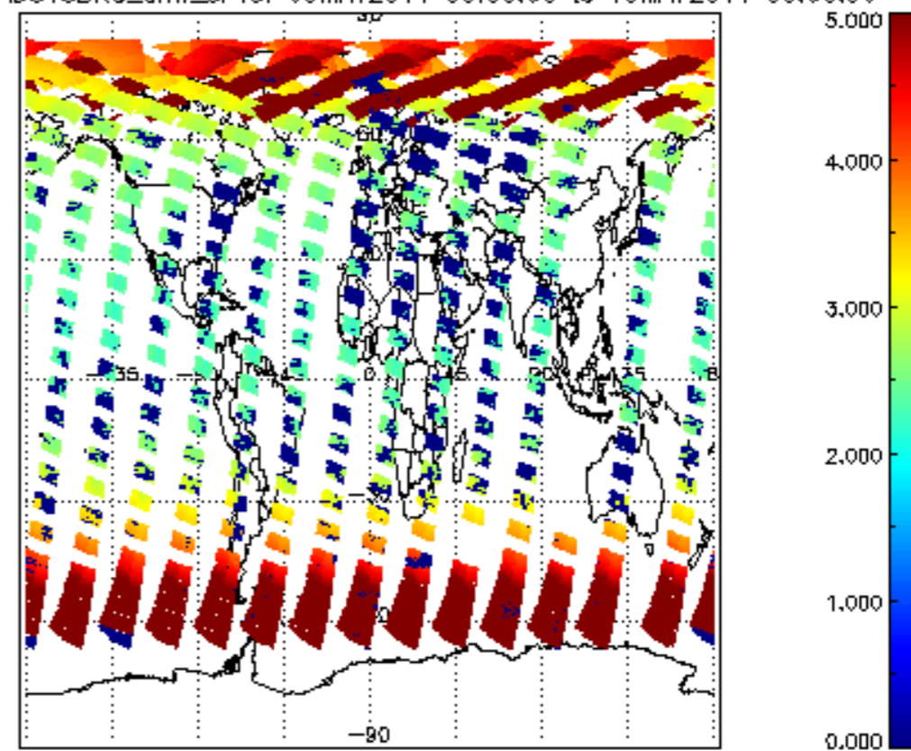
SCIOL2P_NADUV3BRO_amf_sl for 09MAY2011 00:00:00 to 10MAY2011 00:00:00
