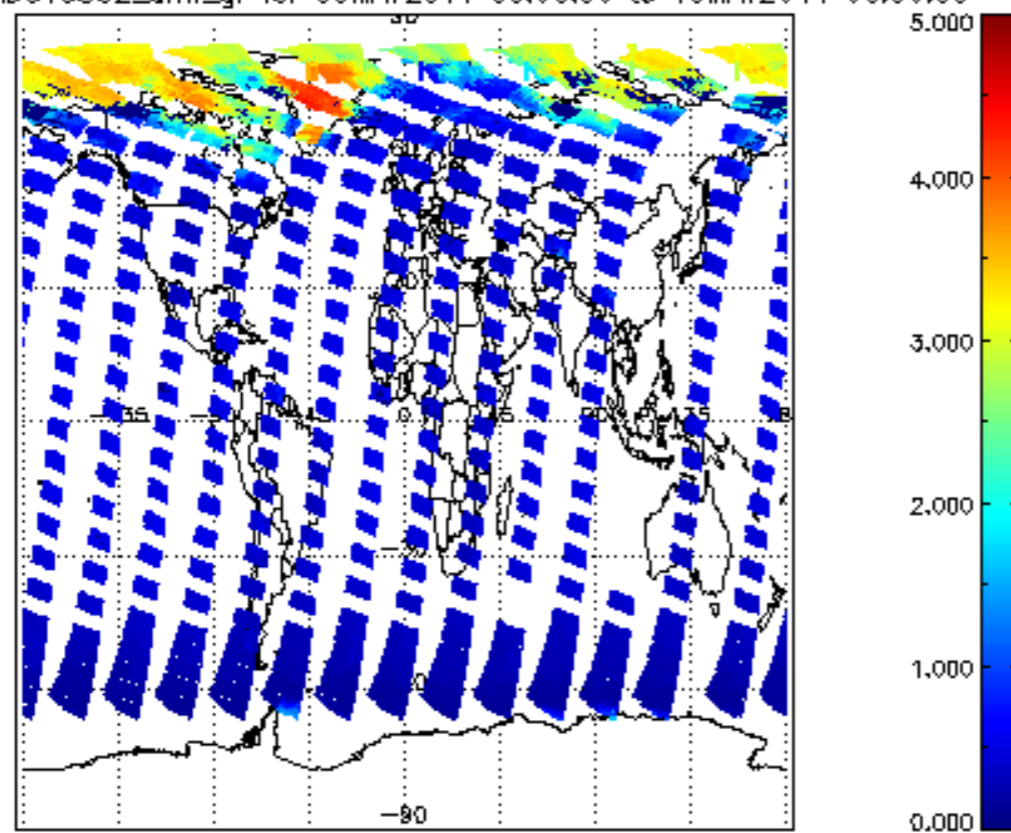
SCIOL2P_NADUV5S02_amf_gr for 09MAY2011 00:00:00 to 10MAY2011 00:00:00
