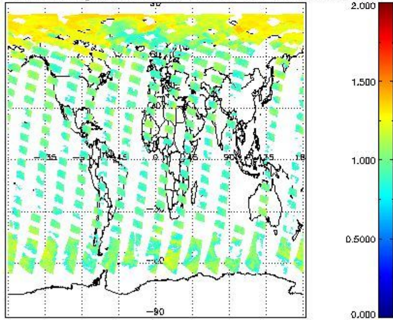
SCIOL2P_NADUV8H2O_arnf_gr for 09MAY2011 00:00:00 to 10MAY2011 00:00:00
