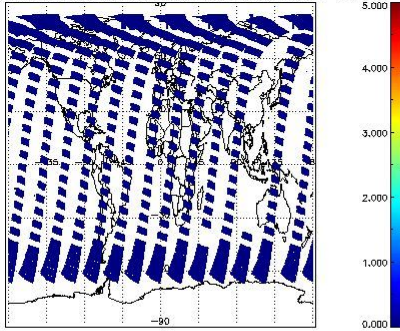
SCIOL2P_NADUV5S02_amf_cl for 09MAY2011 00:00:00 to 10MAY2011 00:00:00
