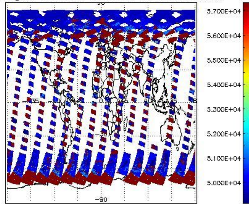
cloud_flags for 09MAY2011 00:00:00 to 10MAY2011 00:00:00
