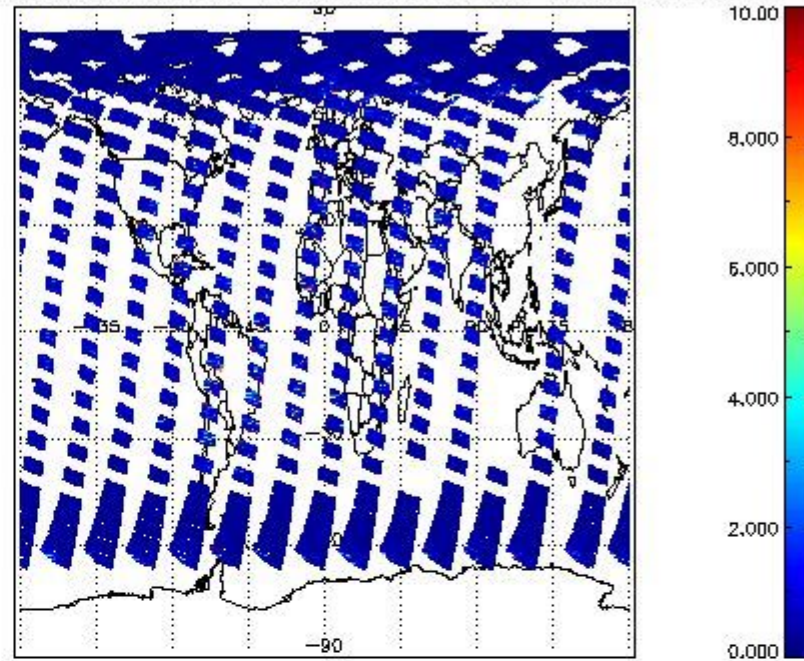
SCIOL2P_NADUV3BRO_vcd_err for 09MAY2011 00:00:00 to 10MAY2011 00:00:00
