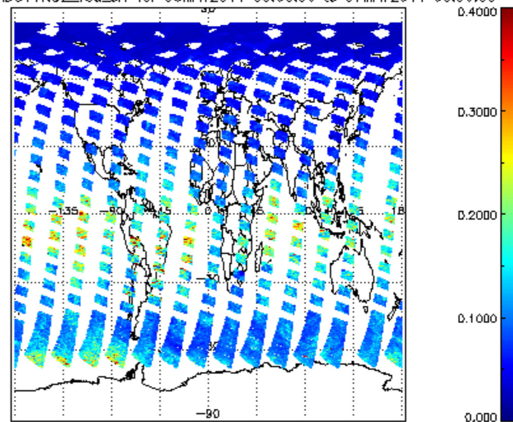
SCIOL2P_NADUV1NO2_vcd_err for 06MAY2011 00:00:00 to 07MAY2011 00:00:00
