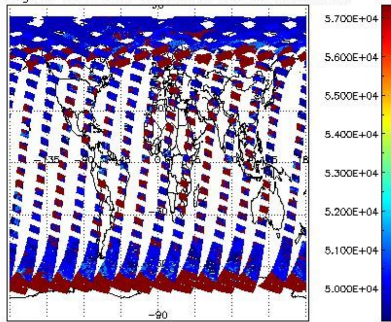
cloud_flags for 06MAY2011 00:00:00 to 07MAY2011 00:00:00
