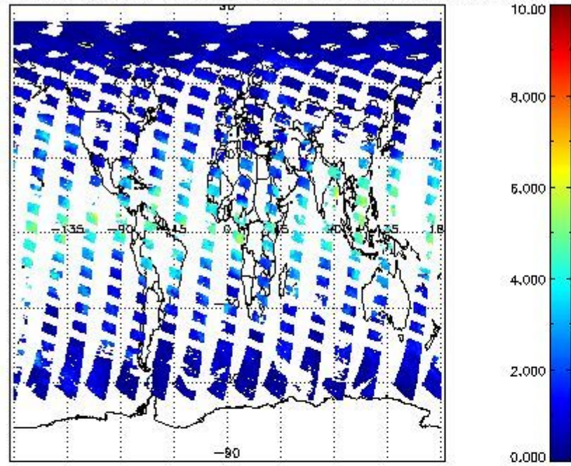
SCIOL2P_NADUV8H2O_vcd for 06MAY2011 00:00:00 to 07MAY2011 00:00:00
