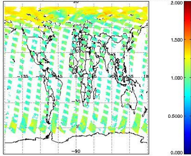
SCIOL2P_NADUV8H2O_arnf_gr for 06MAY2011 00:00:00 to 07MAY2011 00:00:00
