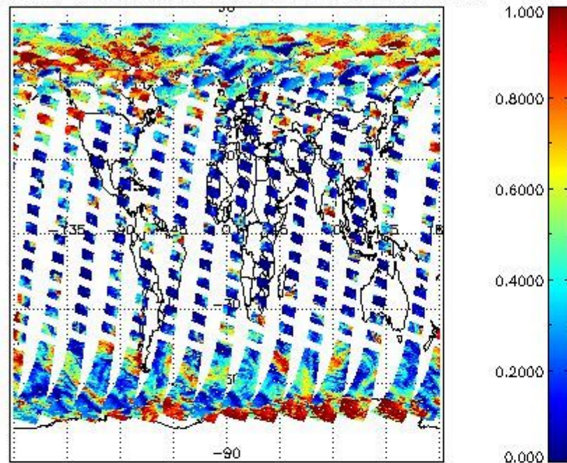
cL_frac for 06MAY2011 00:00:00 to 07MAY2011 00:00:00
