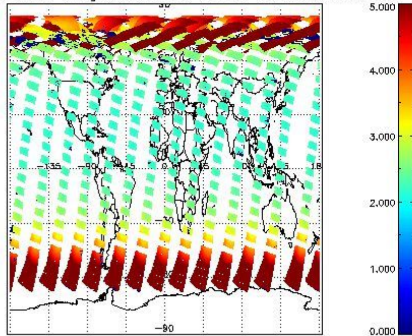
SCIOL2P_NADUV1NO2_amf_gr for 06MAY2011 00:00:00 to 07MAY2011 00:00:00
