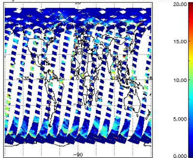
cL_top_height for 06MAY2011 00:00:00 to 07MAY2011 00:00:00
