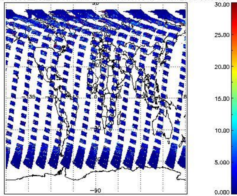
SCIOL2P_NADUV5S02_vcd_err for 06MAY2011 00:00:00 to 07MAY2011 00:00:00
