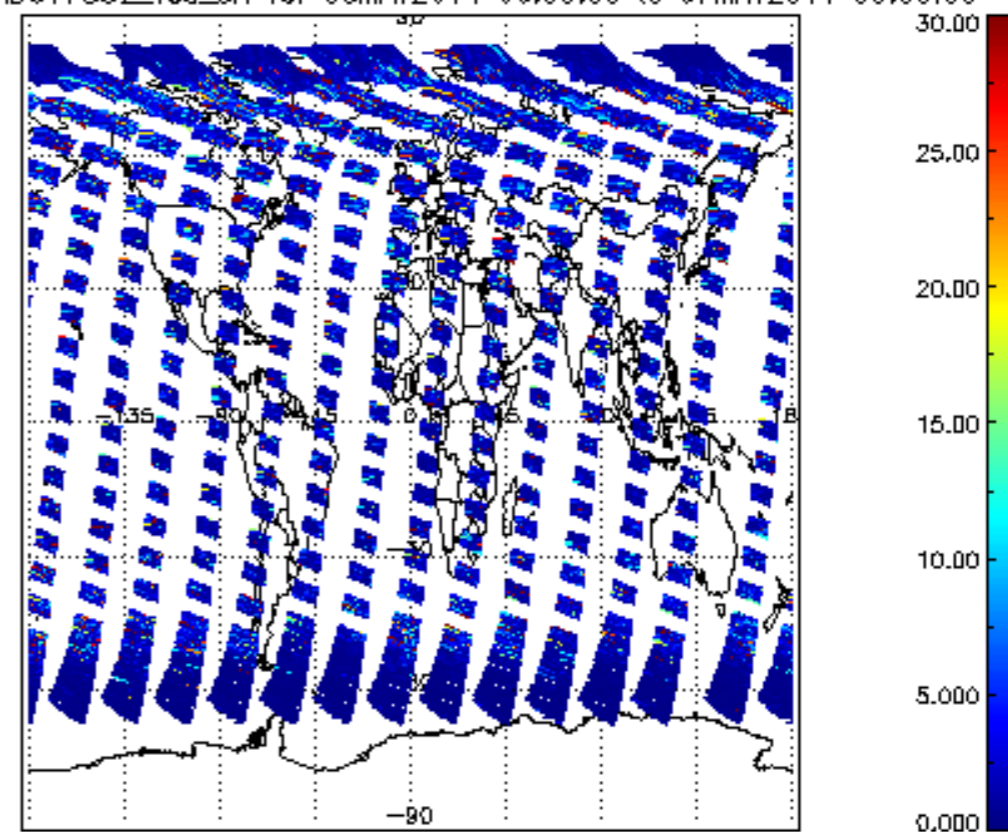
SCIOL2P_NADUV7S02_vcd_err for 06MAY2011 00:00:00 to 07MAY2011 00:00:00
