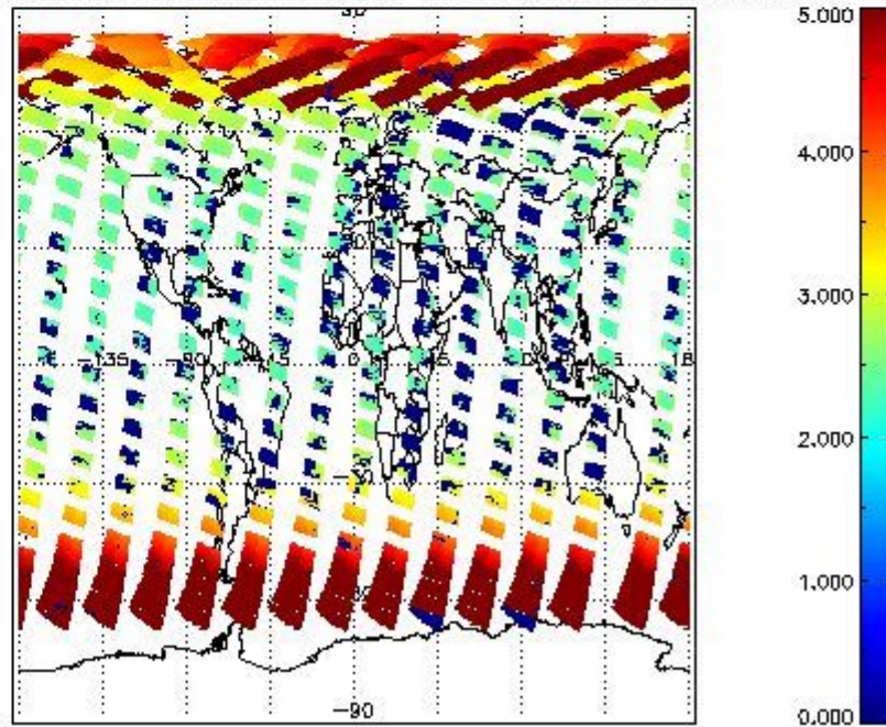
SCIOL2P_NADUV003_amf_cl for 06MAY2011 00:00:00 to 07MAY2011 00:00:00
