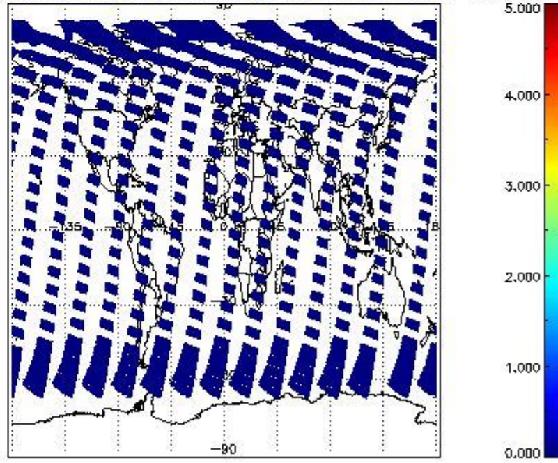
SCIOL2P_NADUV7S02_amf_cl for 06MAY2011 00:00:00 to 07MAY2011 00:00:00
