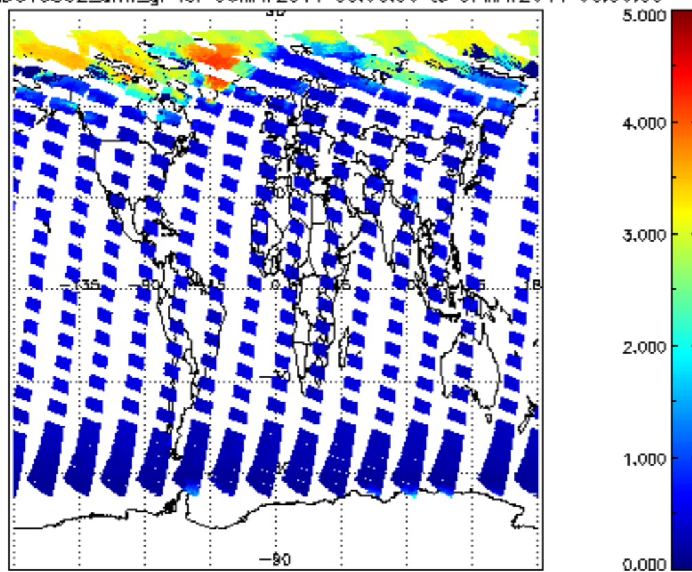
SCIOL2P_NADUV5S02_amf_gr for 06MAY2011 00:00:00 to 07MAY2011 00:00:00
