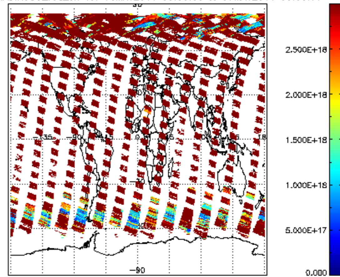
SCIOL2P_NADIR3CO_vcd_err for 06MAY2011 00:00:00 to 07MAY2011 00:00:00
