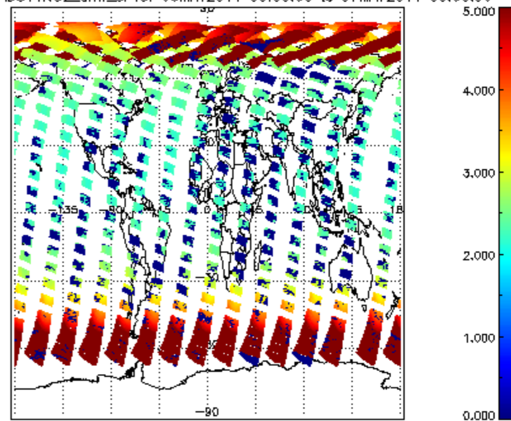
SCIOL2P_NADUV1NO2_amf_cl for 06MAY2011 00:00:00 to 07MAY2011 00:00:00
