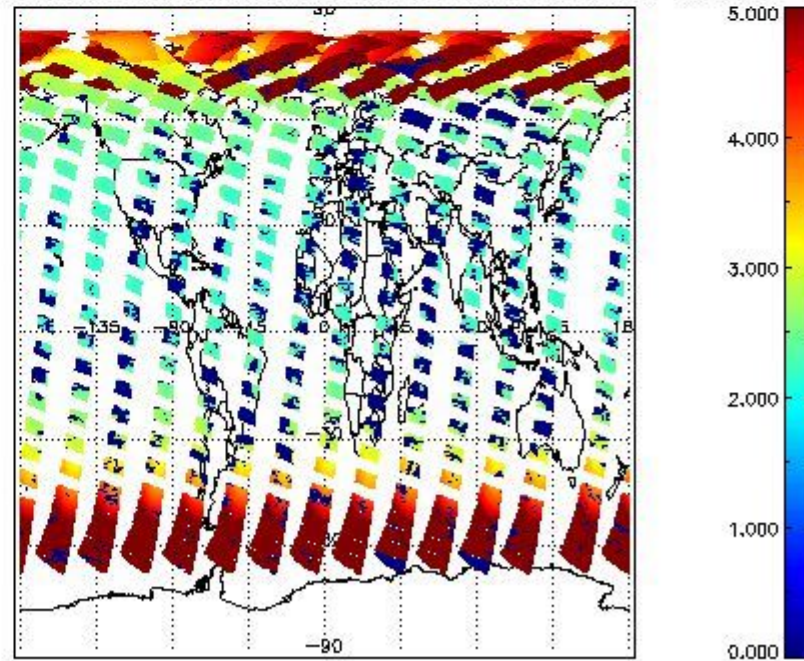
SCIOL2P_NADUV1NO2_amf_cl for 06MAY2011 00:00:00 to 07MAY2011 00:00:00
