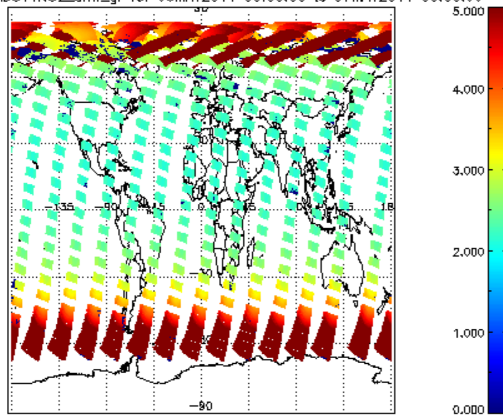
SCIOL2P_NADUV1NO2_amf_gr for 06MAY2011 00:00:00 to 07MAY2011 00:00:00
