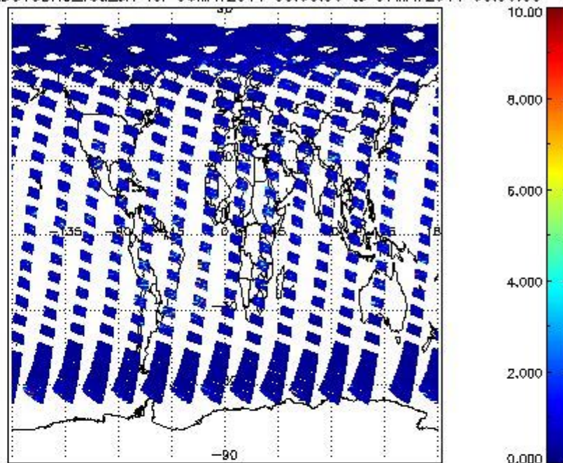
SCIOL2P_NADUV3BRO_vcd_err for 06MAY2011 00:00:00 to 07MAY2011 00:00:00
