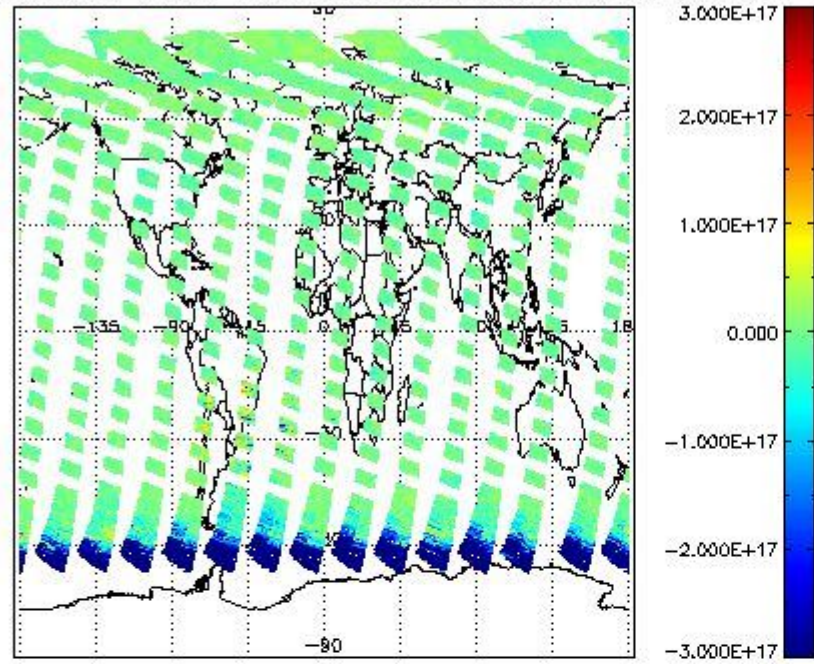
SCIOL2P_NADUV7S02_vcd for 06MAY2011 00:00:00 to 07MAY2011 00:00:00
