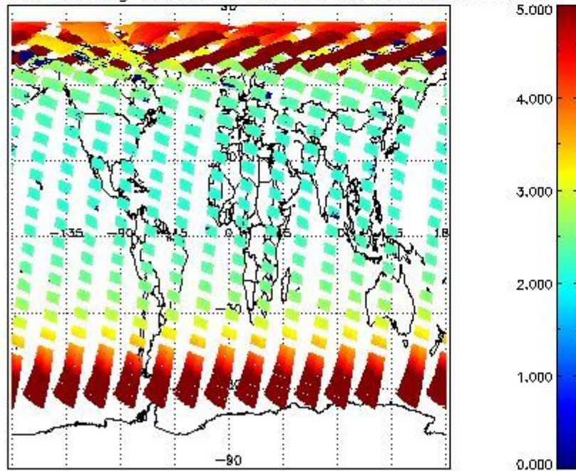
SCIOL2P_NADUV003_amf_gr for 06MAY2011 00:00:00 to 07MAY2011 00:00:00
