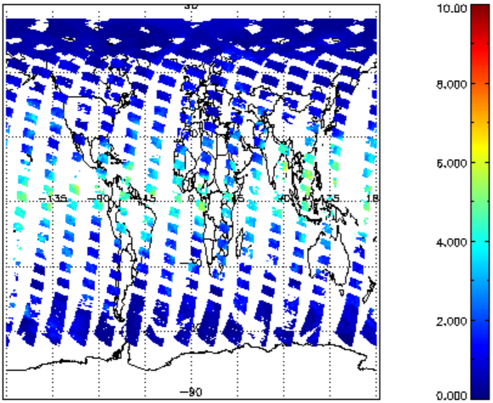
SCIOL2P_NADUV8H2O_vcd for 06MAY2011 00:00:00 to 07MAY2011 00:00:00
