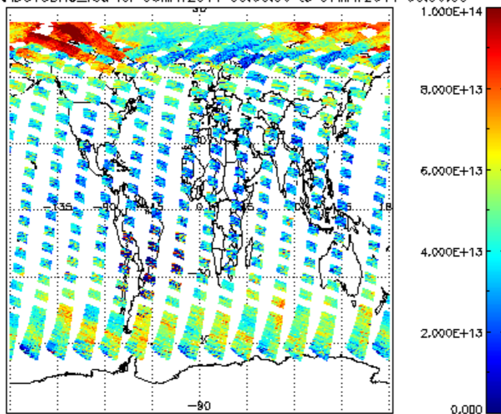
SCIOL2P_NADUV3BRO_vcd for 06MAY2011 00:00:00 to 07MAY2011 00:00:00
