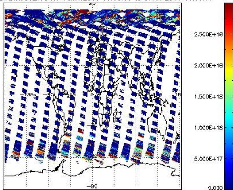
SCIDL2P_NADIR3CO_vcd for 06MAY2011 00:00:00 to 07MAY2011 00:00:00
