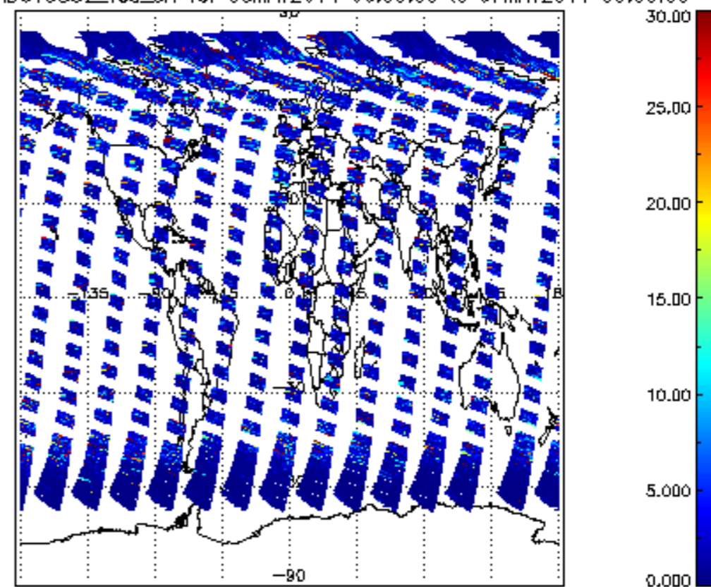
SCIOL2P_NADUV5S02_vcd_err for 06MAY2011 00:00:00 to 07MAY2011 00:00:00
