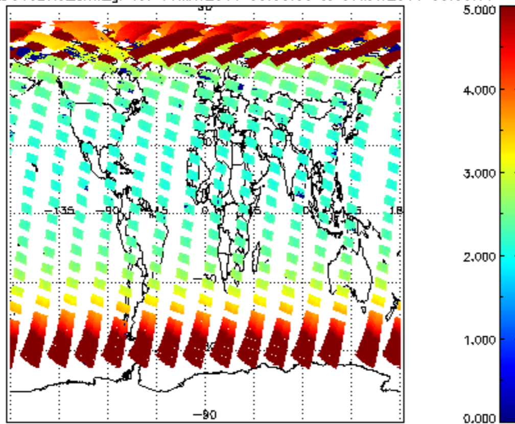
SCIOL2P_NADUV3BRO_amf_gr for 06MAY2011 00:00:00 to 07MAY2011 00:00:00
