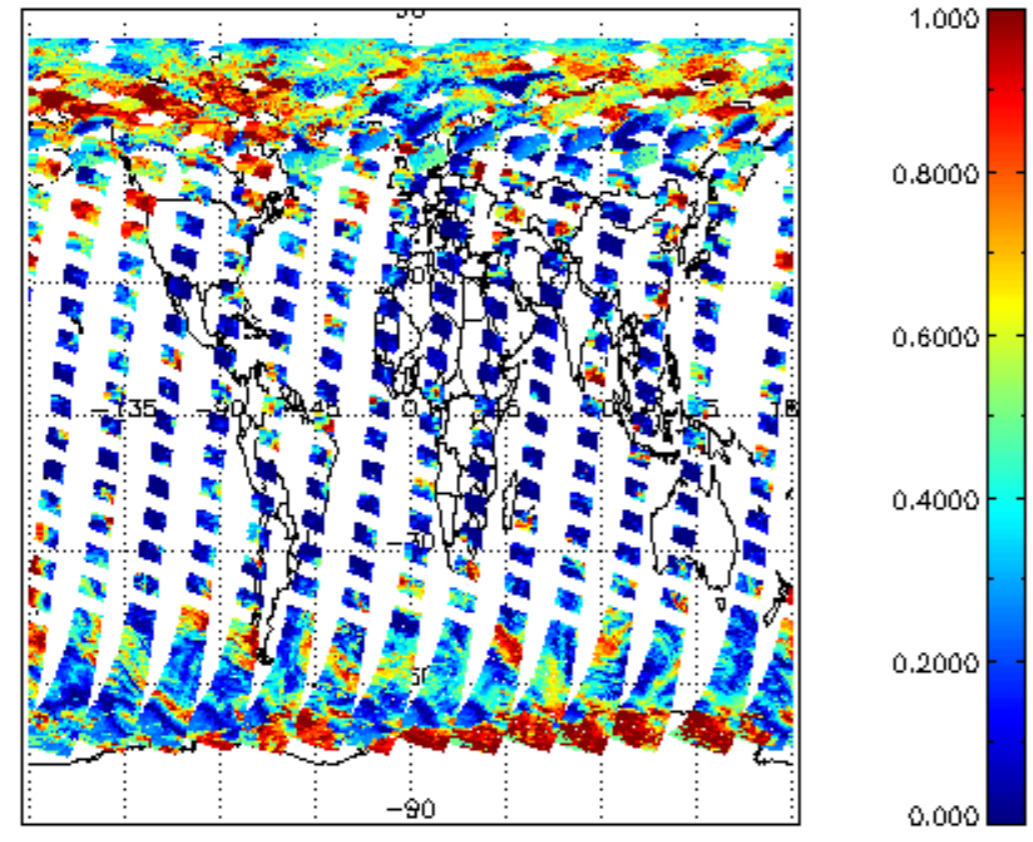
cl_frac for 06MAY2011 00:00:00 to 07MAY2011 00:00:00
