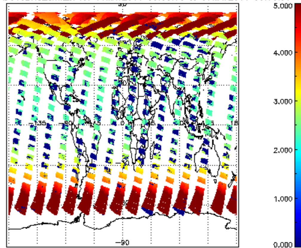
SCIOL2P_NADUV3BRO_amf_sl for 06MAY2011 00:00:00 to 07MAY2011 00:00:00
