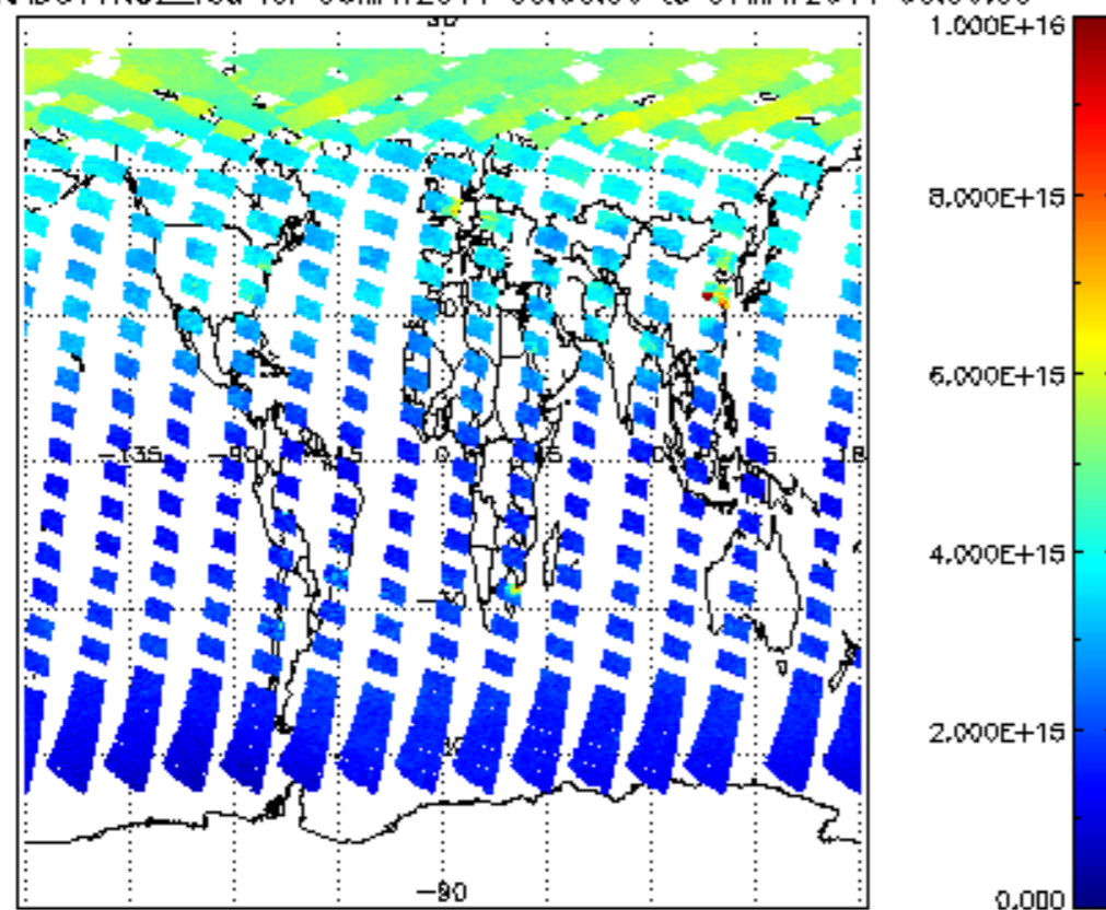
SCIOL2P_NADUV1NO2_vcd for 06MAY2011 00:00:00 to 07MAY2011 00:00:00
