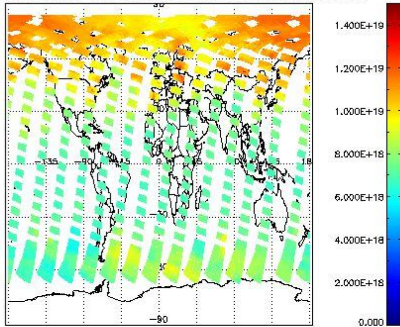
SCIOL2P_NADUV003_vcd for 06MAY2011 00:00:00 to 07MAY2011 00:00:00
