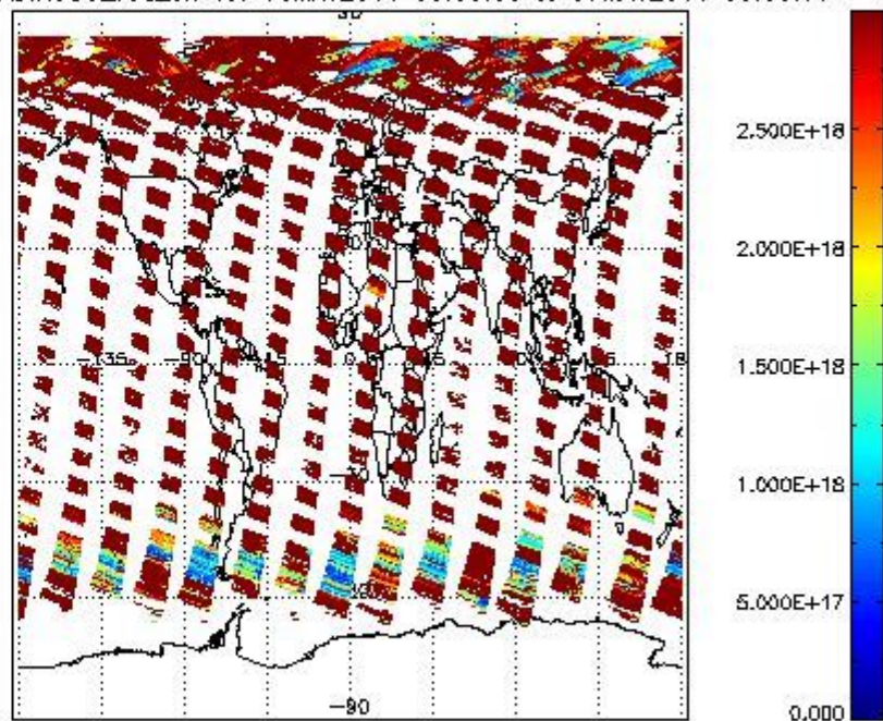
SCIDL2P_NADIR3CO_vcd_err for 06MAY2011 00:00:00 to 07MAY2011 00:00:00
