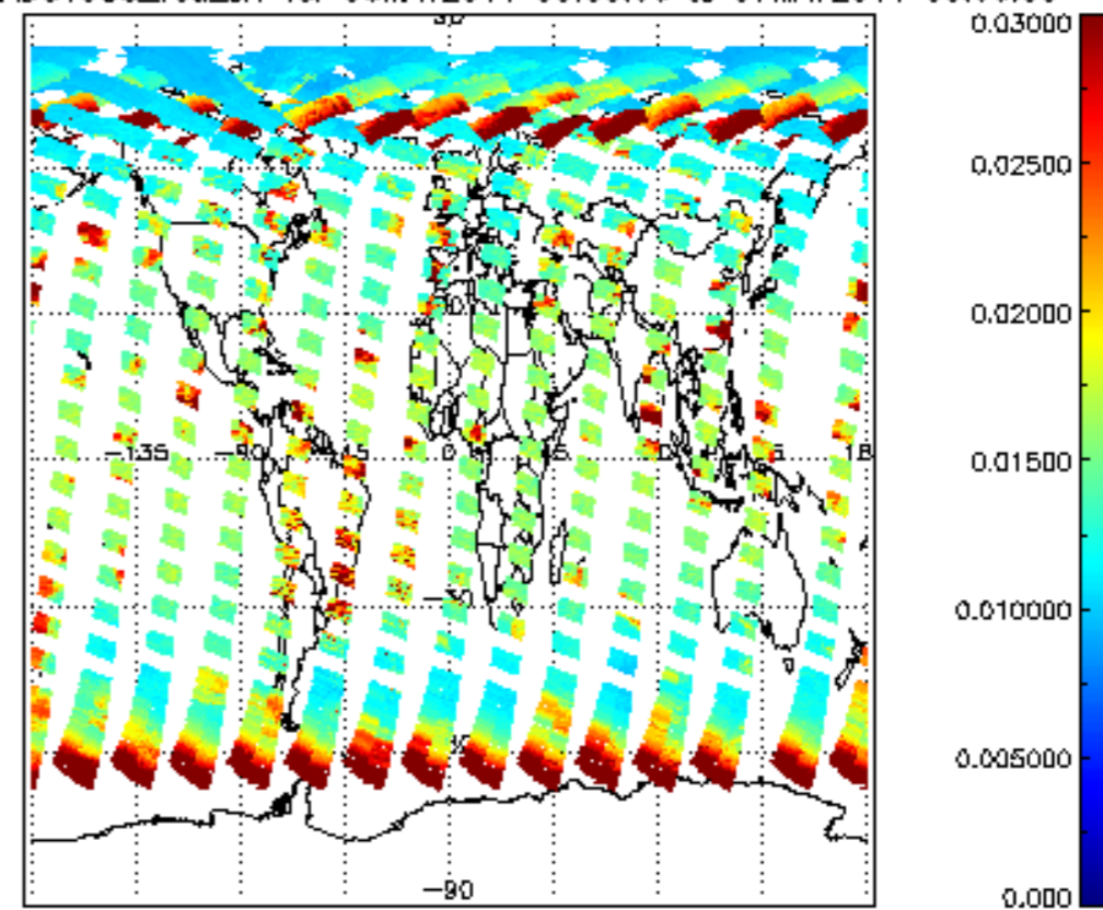
SCIOL2P_NADUV003_vcd_err for 06MAY2011 00:00:00 to 07MAY2011 00:00:00
