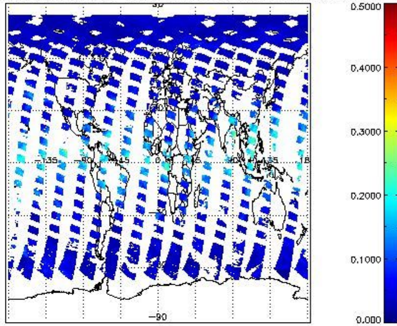
SCIOL2P_NADUV8H2O_vcd_err for 06MAY2011 00:00:00 to 07MAY2011 00:00:00
