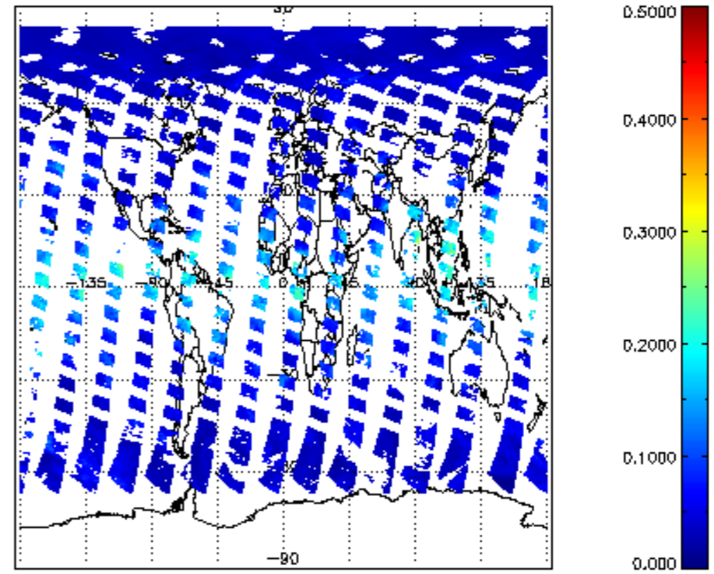
SCIOL2P_NADUV8H2O_vcd_err for 06MAY2011 00:00:00 to 07MAY2011 00:00:00
