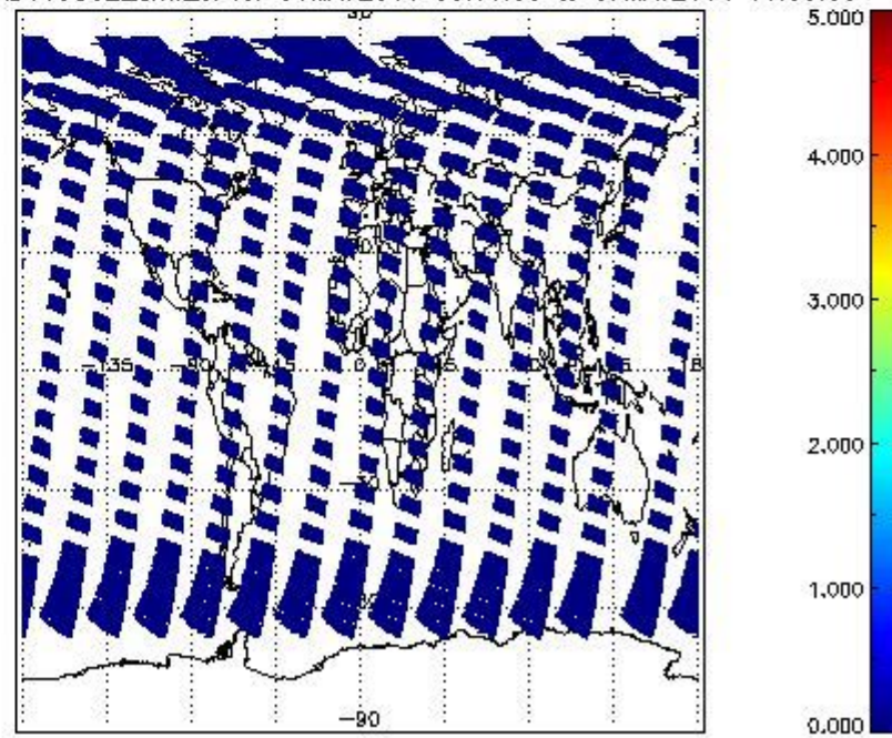
SCIOL2P_NADUV5S02_amf_cl for 06MAY2011 00:00:00 to 07MAY2011 00:00:00
