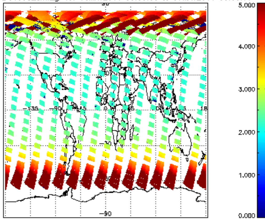
SCIOL2P_NADUV003_amf_gr for 06MAY2011 00:00:00 to 07MAY2011 00:00:00
