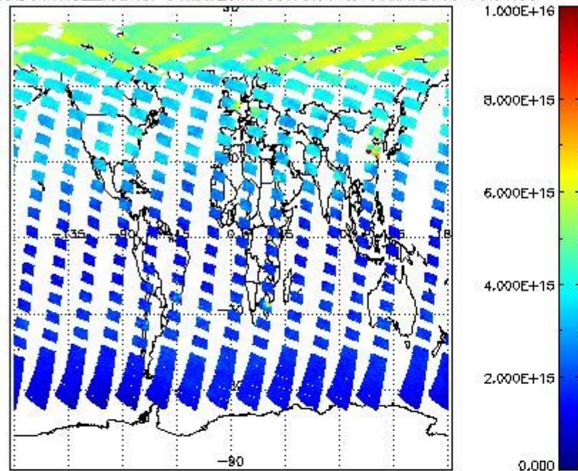
SCIOL2P_NADUV1NO2_vcd for 06MAY2011 00:00:00 to 07MAY2011 00:00:00
