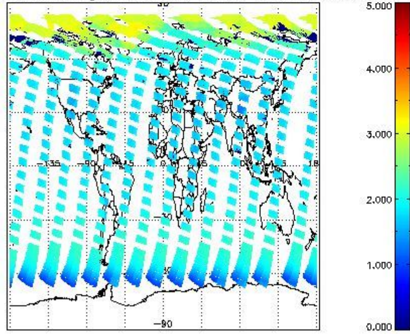
SCIOL2P_NADUV7S02_amf_gr for 06MAY2011 00:00:00 to 07MAY2011 00:00:00
