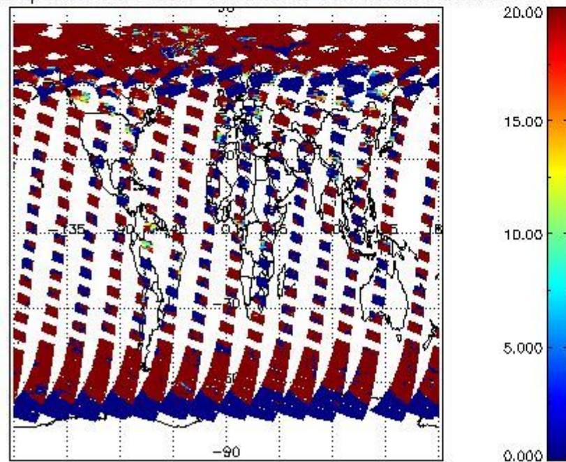
cL_opt_depth for 06MAY2011 00:00:00 to 07MAY2011 00:00:00
