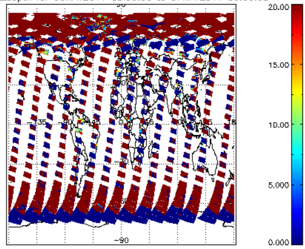
cl_opt_depth for 06MAY2011 00:00:00 to 07MAY2011 00:00:00
