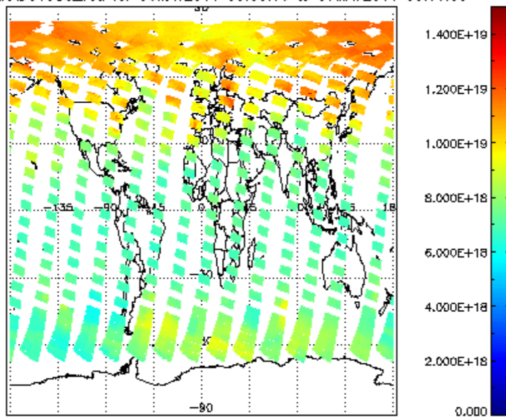
SCIOL2P_NADUV003_vcd for 06MAY2011 00:00:00 to 07MAY2011 00:00:00
