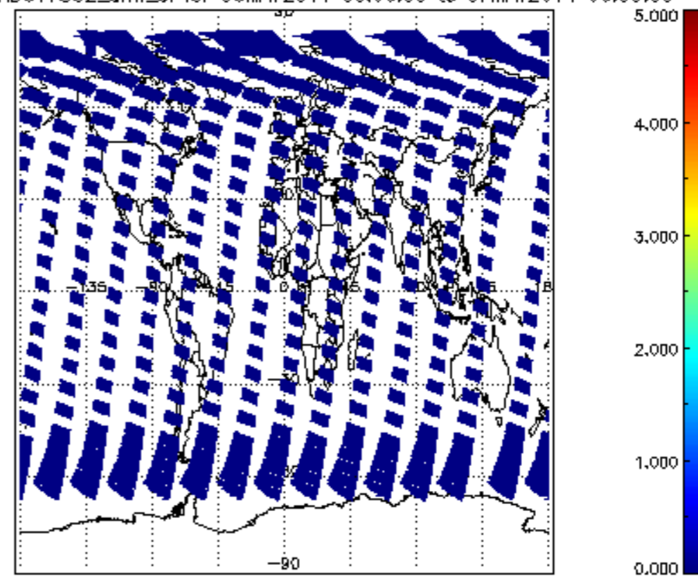
SCIOL2P_NADUV7S02_amf_cl for 06MAY2011 00:00:00 to 07MAY2011 00:00:00
