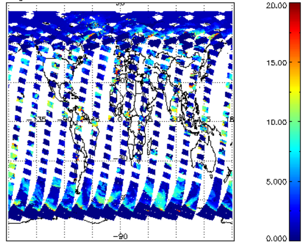
cl_top_height for 06MAY2011 00:00:00 to 07MAY2011 00:00:00
