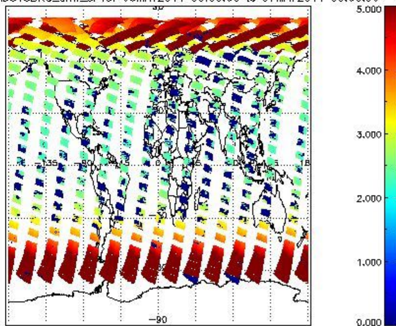
SCIOL2P_NADUV3BRO_amf_cl for 06MAY2011 00:00:00 to 07MAY2011 00:00:00
