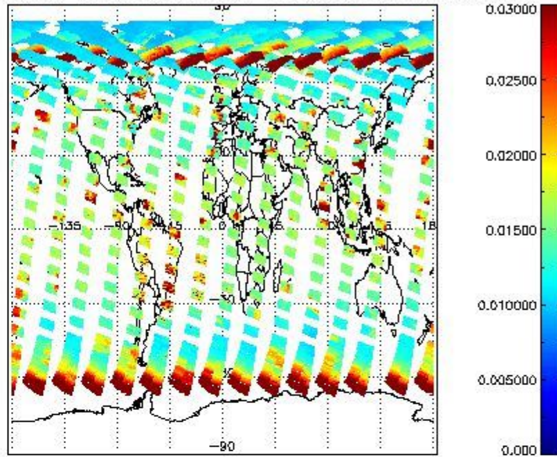
SCIOL2P_NADUV003_vcd_err for 06MAY2011 00:00:00 to 07MAY2011 00:00:00
