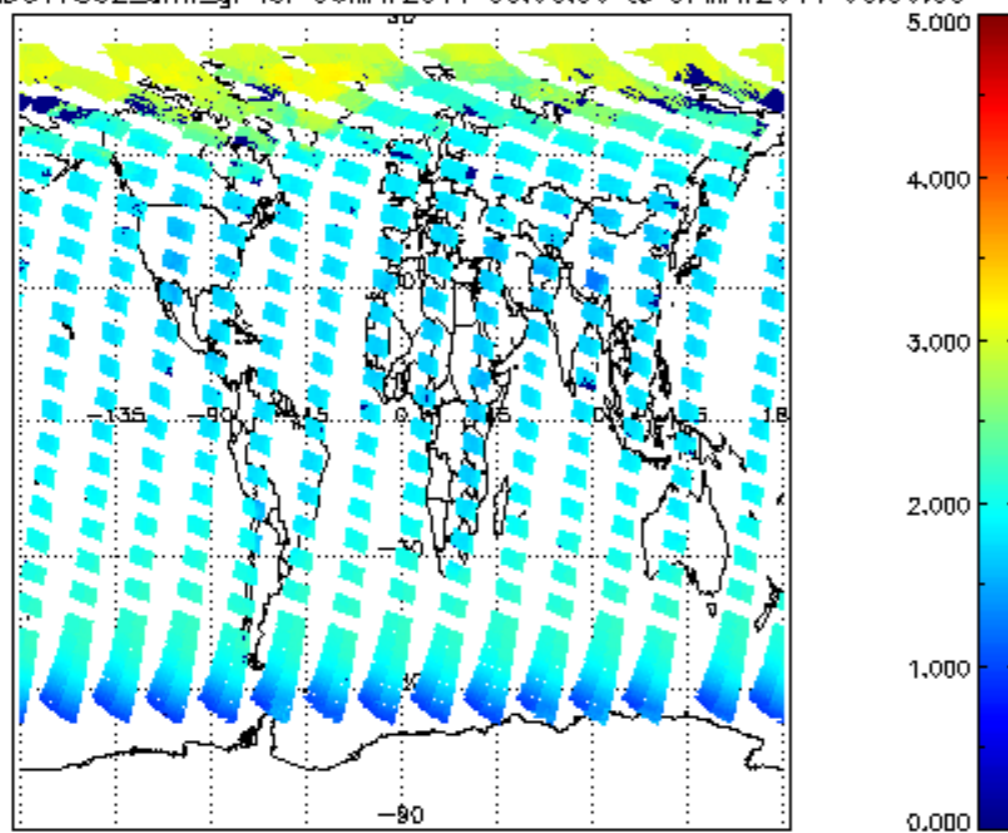
SCIOL2P_NADUV7S02_amf_gr for 06MAY2011 00:00:00 to 07MAY2011 00:00:00
