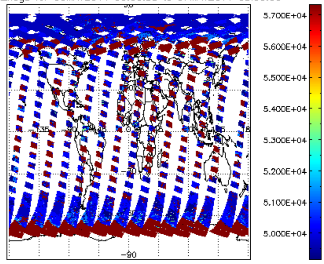
cloud_flags for 06MAY2011 00:00:00 to 07MAY2011 00:00:00
