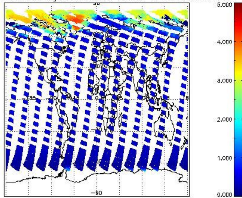
SCIOL2P_NADUV5S02_amf_gr for 06MAY2011 00:00:00 to 07MAY2011 00:00:00
