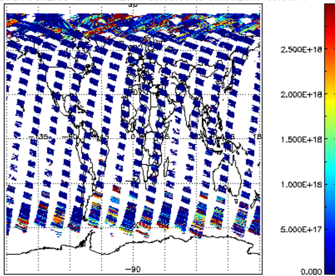
SCIOL2P_NADIR3CO_vcd for 06MAY2011 00:00:00 to 07MAY2011 00:00:00
