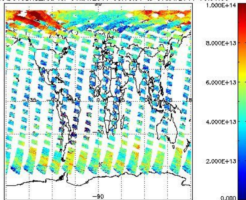
SCIOL2P_NADUV3BRO_vcd for 06MAY2011 00:00:00 to 07MAY2011 00:00:00
