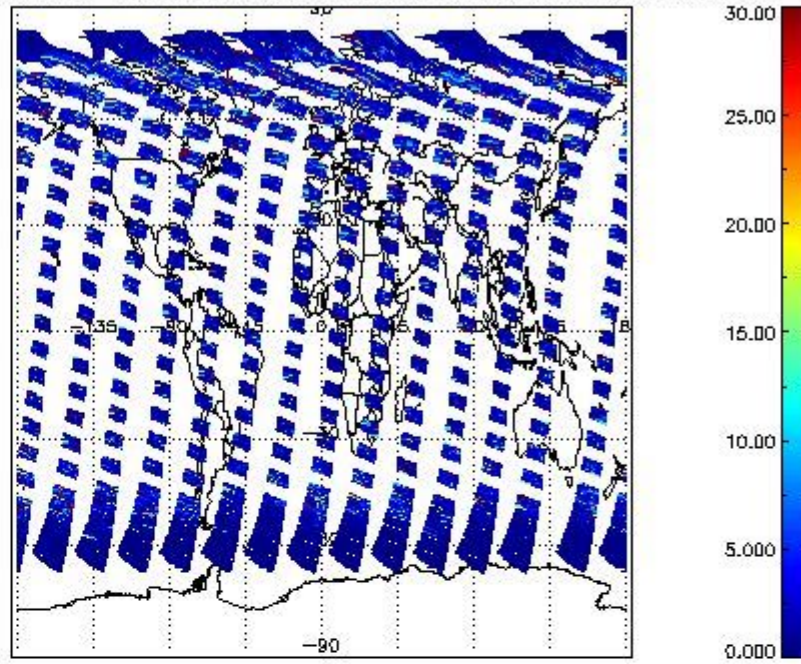
SCIOL2P_NADUV7S02_vcd_err for 06MAY2011 00:00:00 to 07MAY2011 00:00:00
