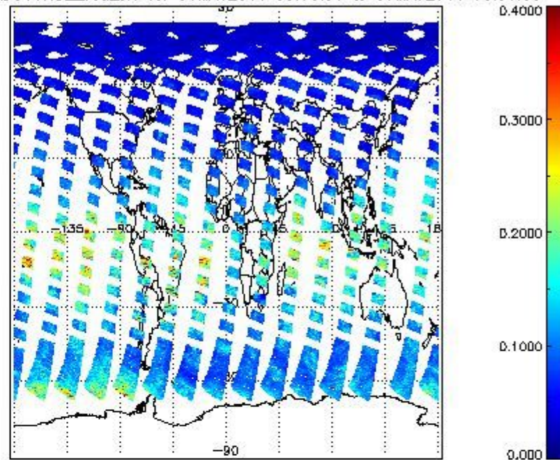
SCIOL2P_NADUV1NO2_vcd_err for 06MAY2011 00:00:00 to 07MAY2011 00:00:00
