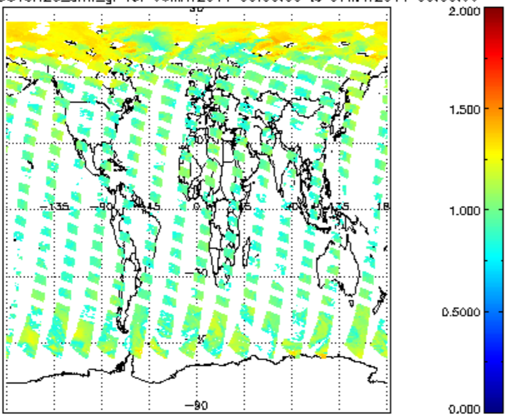
SCIOL2P_NADUV8H2O_amf_gr for 06MAY2011 00:00:00 to 07MAY2011 00:00:00
