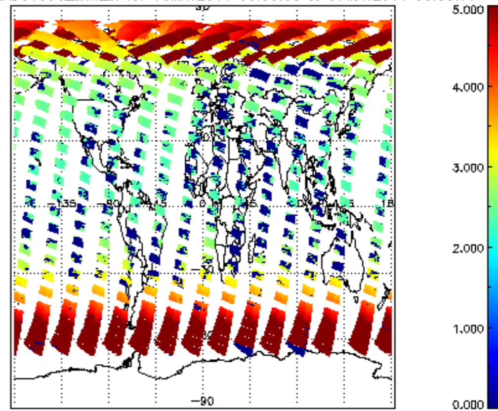
SCIOL2P_NADUV003_amf_cl for 06MAY2011 00:00:00 to 07MAY2011 00:00:00
