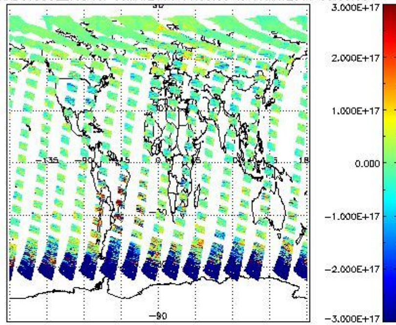
SCIOL2P_NADUV5S02_vcd for 06MAY2011 00:00:00 to 07MAY2011 00:00:00
