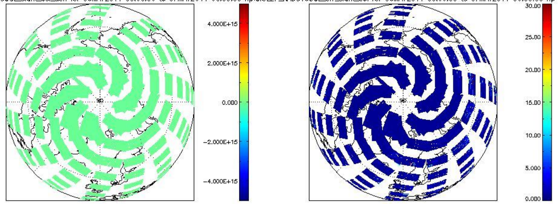
CIOL2P_NADUV6OCLslant_col_den for 06MAY2011 00:00:00 to 07MAY2011 00:00:00 np; CIOL2P_NADUV6OCLerr_slant_col for 06MAY2011 00:00:00 to 07MAY2011 00:00:00 np
