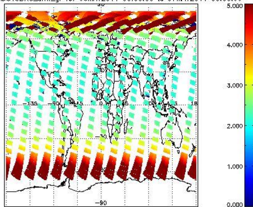
SCIOL2P_NADUV3BRO_amf_gr for 06MAY2011 00:00:00 to 07MAY2011 00:00:00
