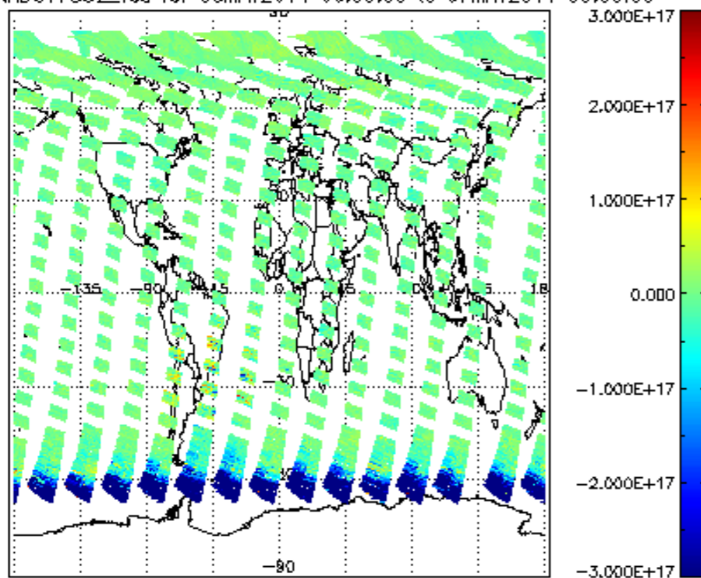
SCIOL2P_NADUV7S02_vcd for 06MAY2011 00:00:00 to 07MAY2011 00:00:00
