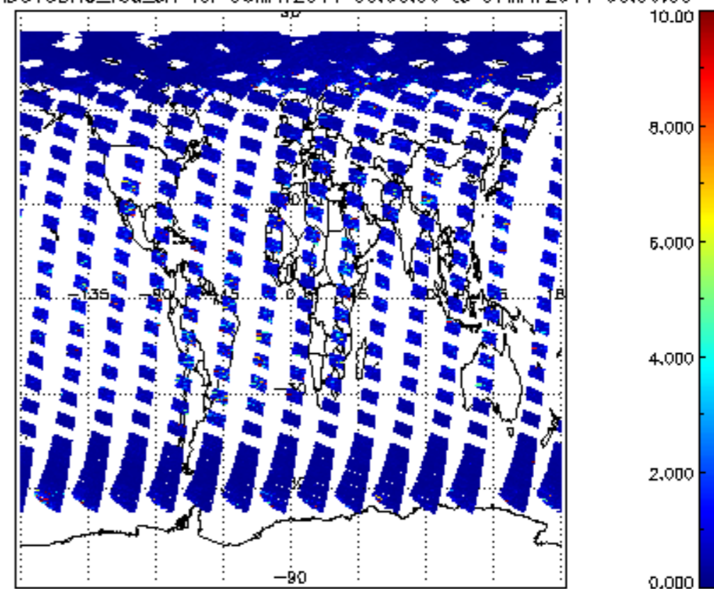
SCIOL2P_NADUV3BRO_vcd_err for 06MAY2011 00:00:00 to 07MAY2011 00:00:00
