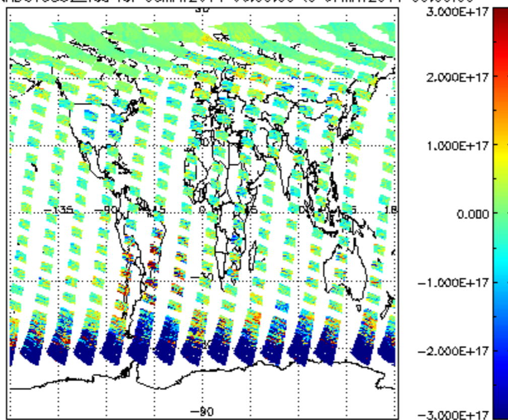
SCIOL2P_NADUV5S02_vcd for 06MAY2011 00:00:00 to 07MAY2011 00:00:00
