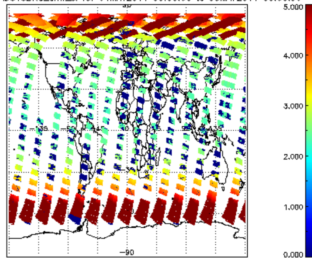
SCIOL2P_NADUV3BRO_amf_sl for 04MAY2011 00:00:00 to 05MAY2011 00:00:00
