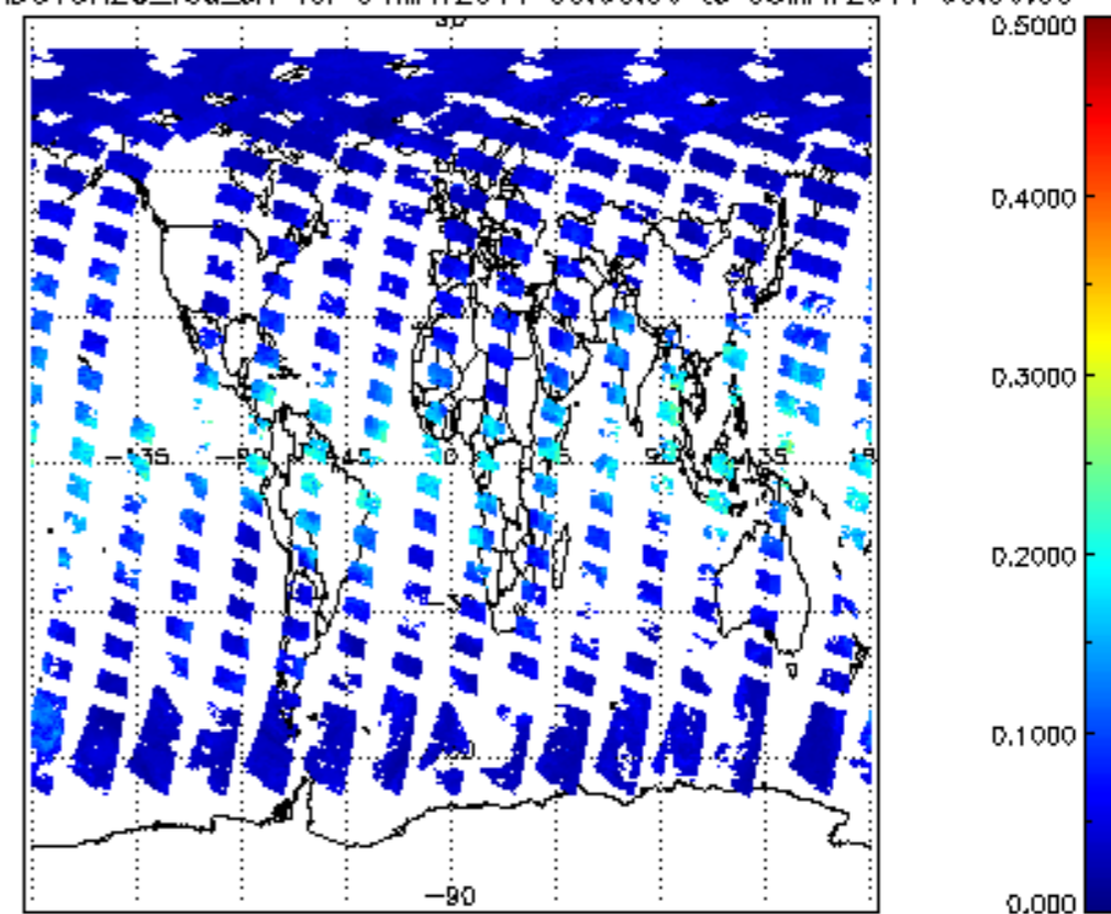
SCIOL2P_NADUV8H2O_vcd_err for 04MAY2011 00:00:00 to 05MAY2011 00:00:00
