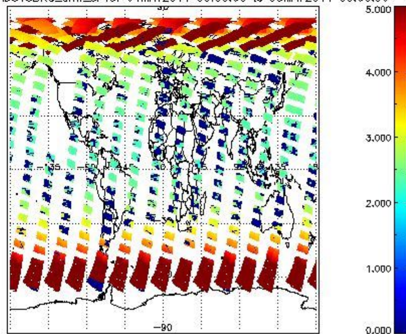
SCIOL2P_NADUV3BRO_amf_cl for 04MAY2011 00:00:00 to 05MAY2011 00:00:00
