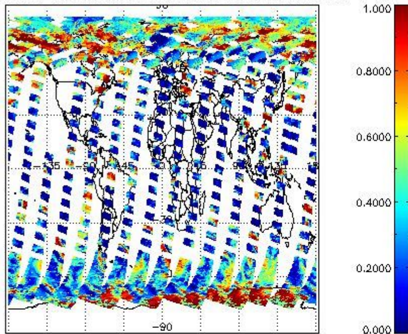
cL_frac for 04MAY2011 00:00:00 to 05MAY2011 00:00:00
