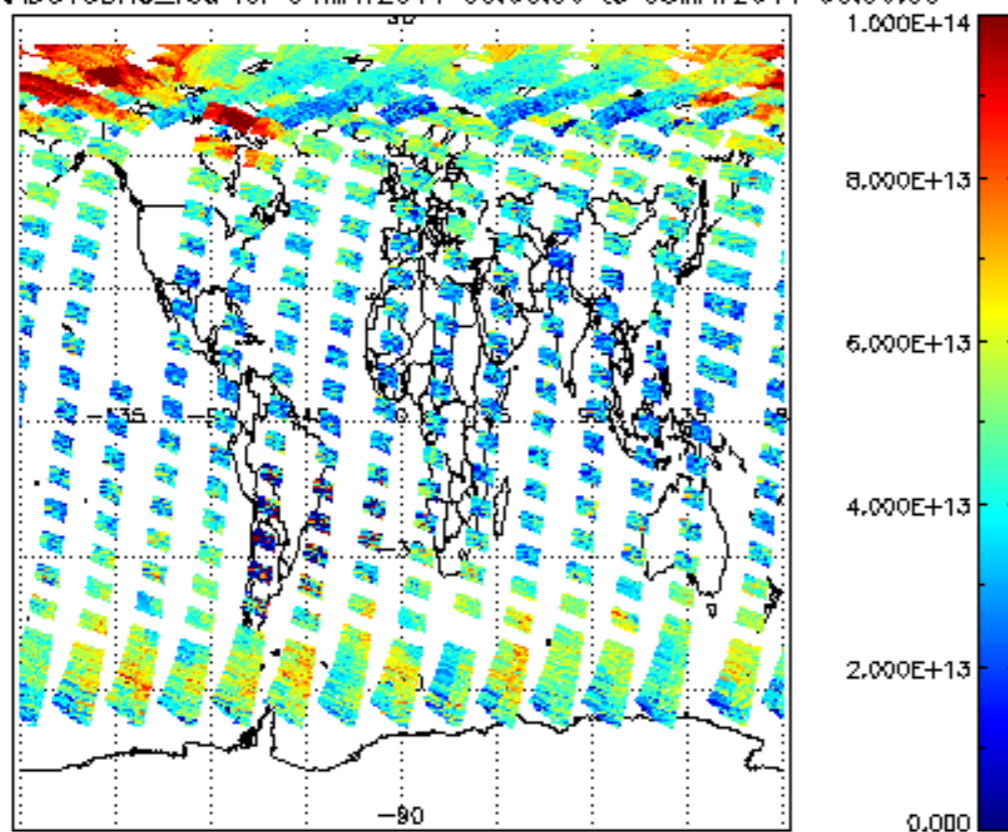
SCIOL2P_NADUV3BRO_vcd for 04MAY2011 00:00:00 to 05MAY2011 00:00:00
