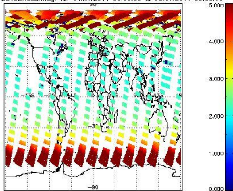
SCIOL2P_NADUV3BRO_amf_gr for 04MAY2011 00:00:00 to 05MAY2011 00:00:00
