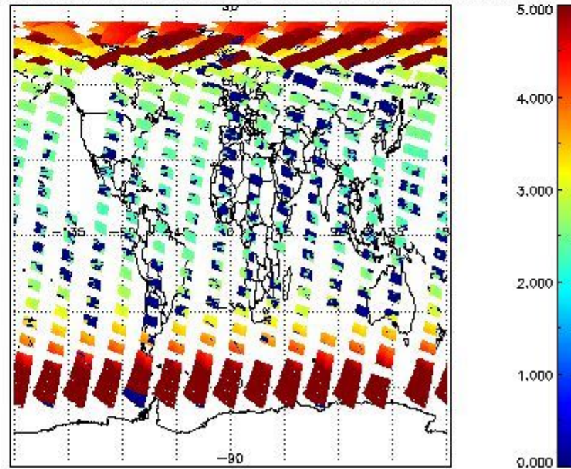
SCIOL2P_NADUV003_amf_cl for 04MAY2011 00:00:00 to 05MAY2011 00:00:00
