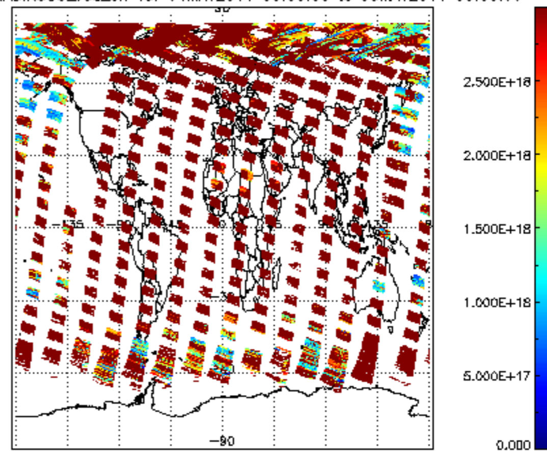
SCIOL2P_NADIR3CO_vcd_err for 04MAY2011 00:00:00 to 05MAY2011 00:00:00
