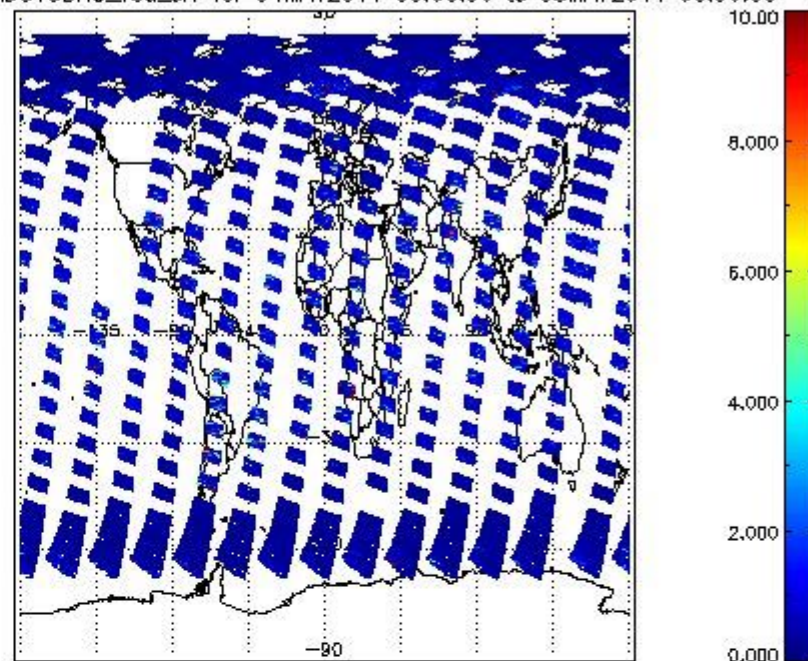
SCIOL2P_NADUV3BRO_vcd_err for 04MAY2011 00:00:00 to 05MAY2011 00:00:00
