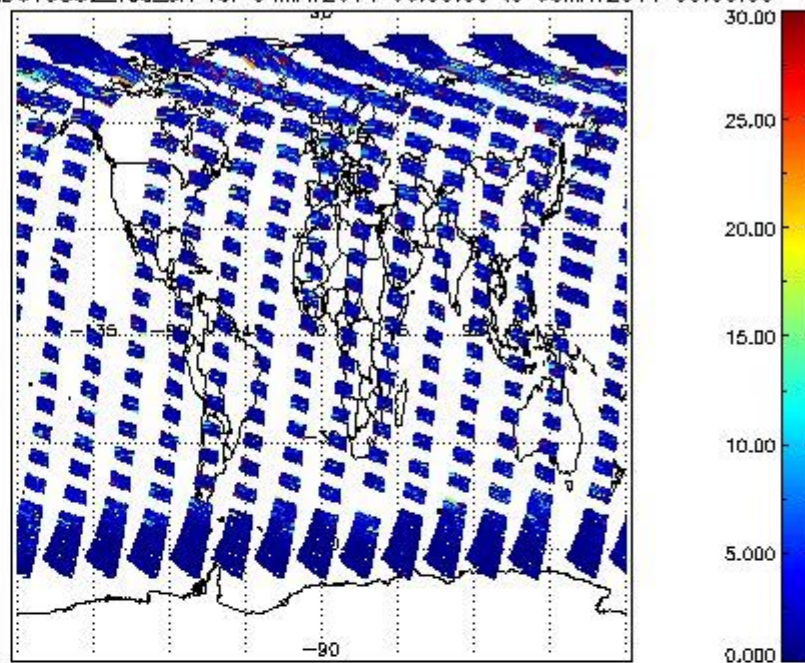
SCIOL2P_NADUV5S02_vcd_err for 04MAY2011 00:00:00 to 05MAY2011 00:00:00
