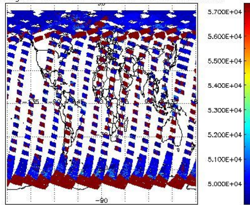
cloud_flags for 04MAY2011 00:00:00 to 05MAY2011 00:00:00
