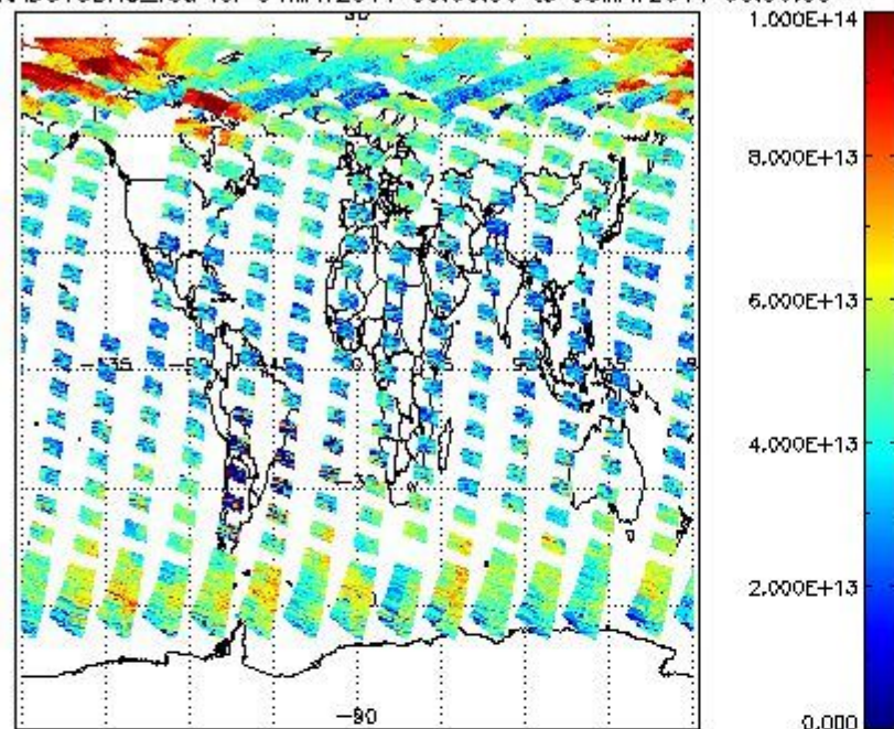
SCIOL2P_NADUV3BRO_vcd for 04MAY2011 00:00:00 to 05MAY2011 00:00:00
