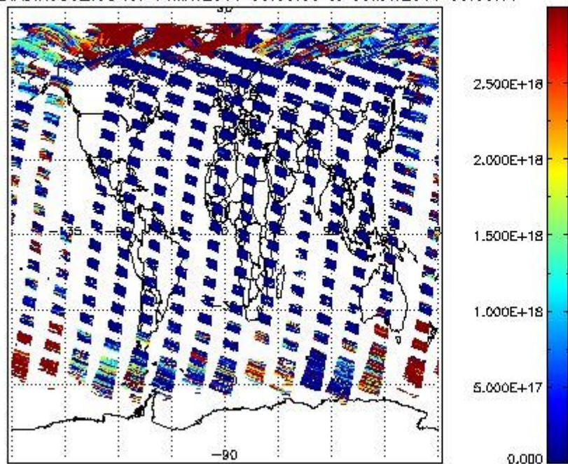
SCIO2P_NADIR3CO_vcd for 04MAY2011 00:00:00 to 05MAY2011 00:00:00
