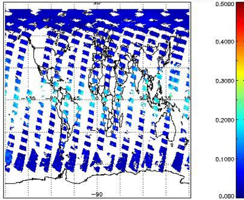
SCIOL2P_NADUV8H2O_vcd_err for 04MAY2011 00:00:00 to 05MAY2011 00:00:00
