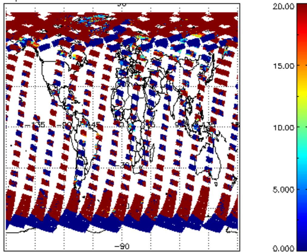
cL_opt_depth for 04MAY2011 00:00:00 to 05MAY2011 00:00:00
