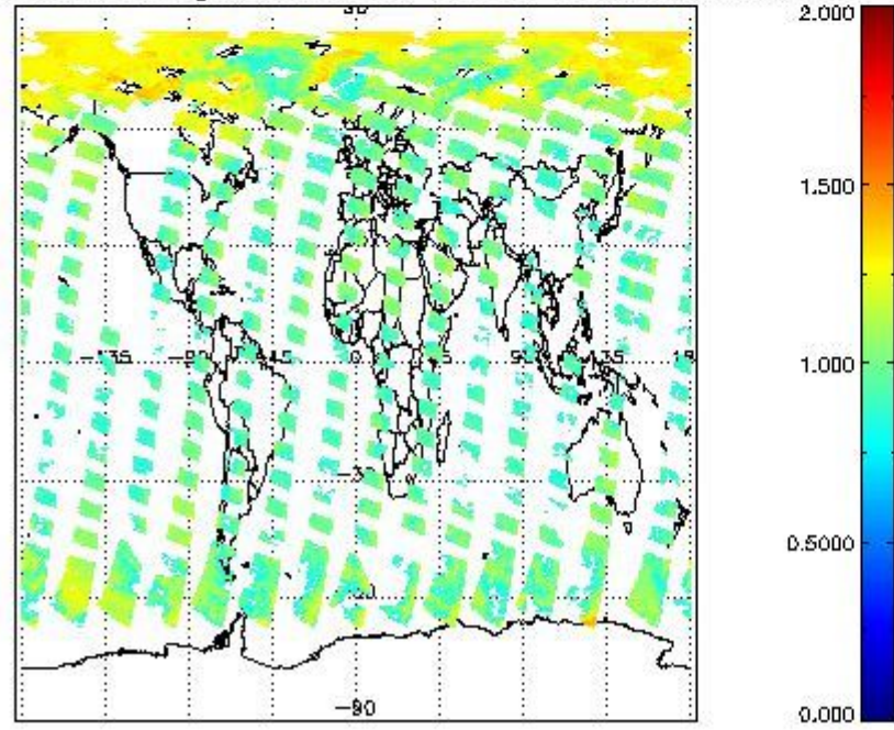
SCIOL2P_NADUV8H2O_arnf_gr for 04MAY2011 00:00:00 to 05MAY2011 00:00:00
