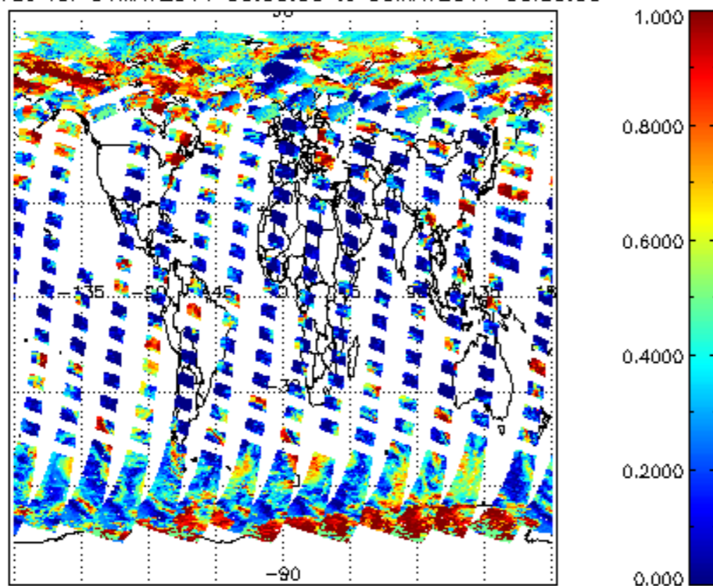
cL_frac for 04MAY2011 00:00:00 to 05MAY2011 00:00:00
