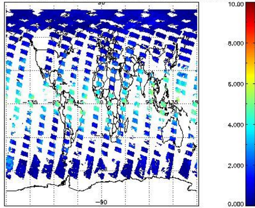
SCIOL2P_NADUV8H2O_vcd for 04MAY2011 00:00:00 to 05MAY2011 00:00:00
