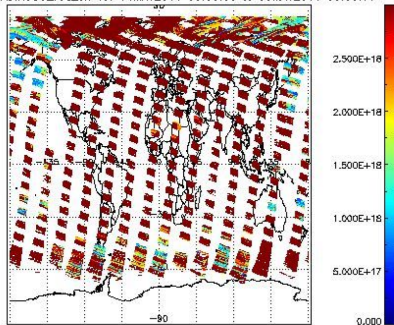
SCIO2P_NADIR3CO_vcd_err for 04MAY2011 00:00:00 to 05MAY2011 00:00:00
