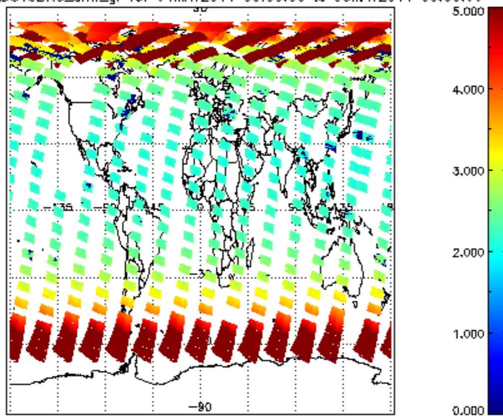
SCIOL2P_NADUV3BRO_amf_gr for 04MAY2011 00:00:00 to 05MAY2011 00:00:00
