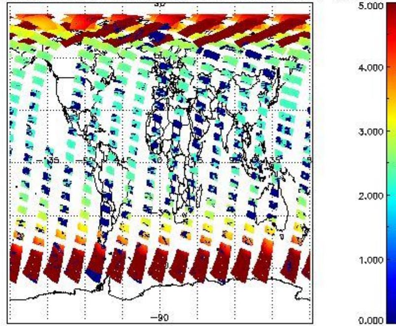
SCIOL2P_NADUV1NO2_amf_cl for 04MAY2011 00:00:00 to 05MAY2011 00:00:00
