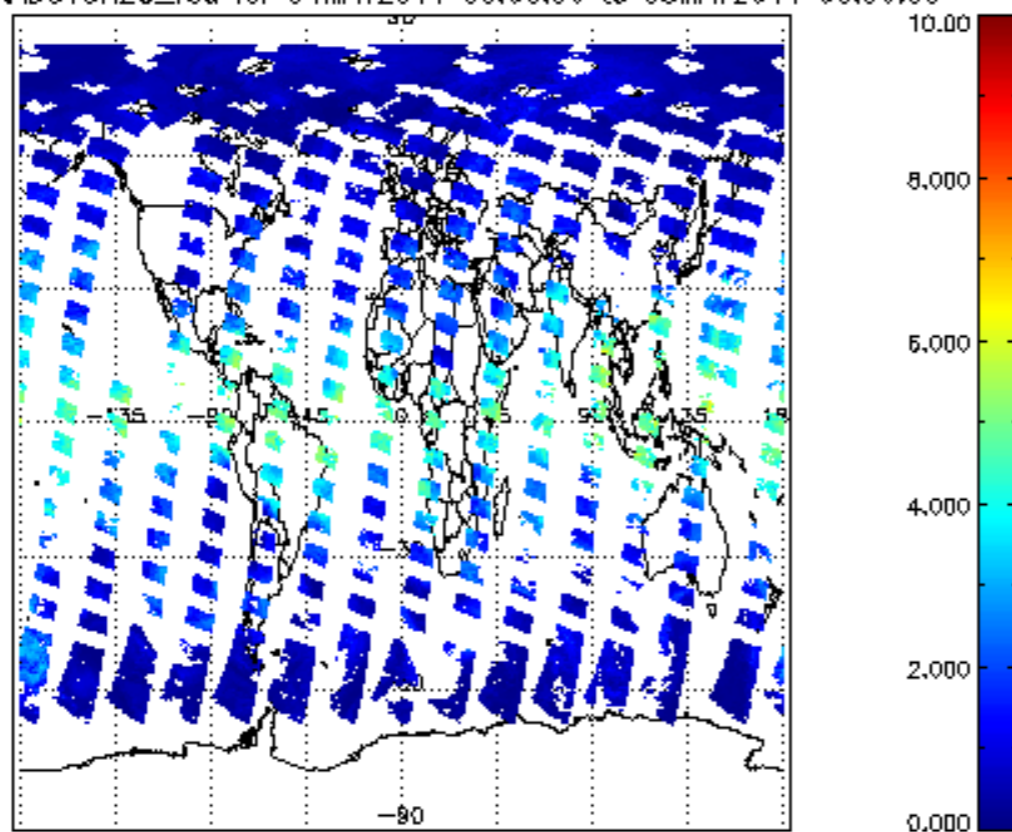
SCIOL2P_NADUV8H2O_vcd for 04MAY2011 00:00:00 to 05MAY2011 00:00:00
