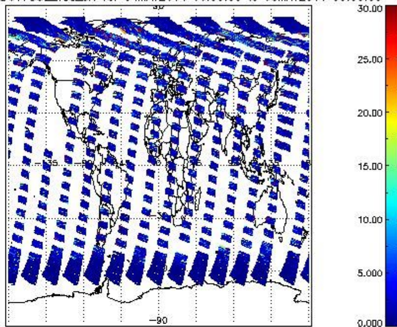
SCIOL2P_NADUV7S02_vcd_err for 04MAY2011 00:00:00 to 05MAY2011 00:00:00
