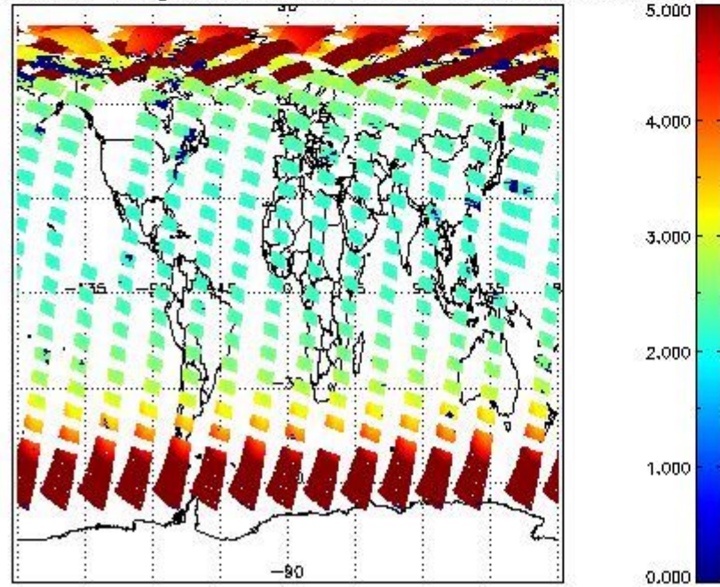
SCIOL2P_NADUV1NO2_amf_gr for 04MAY2011 00:00:00 to 05MAY2011 00:00:00
