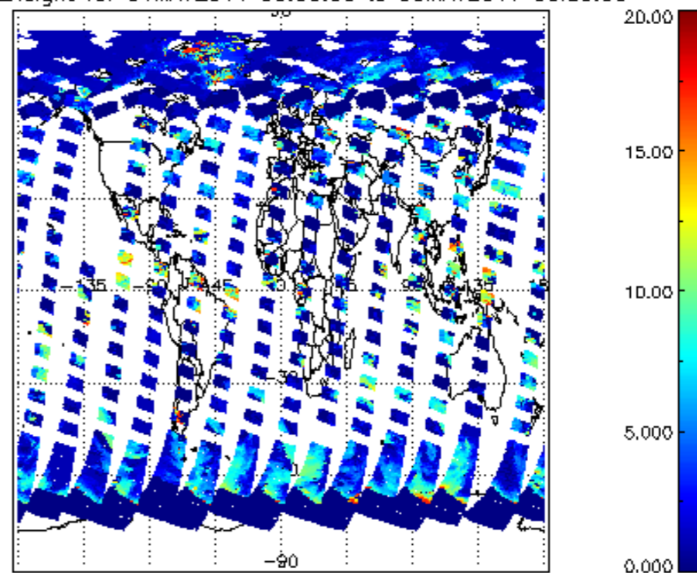
cL_top_height for 04MAY2011 00:00:00 to 05MAY2011 00:00:00
