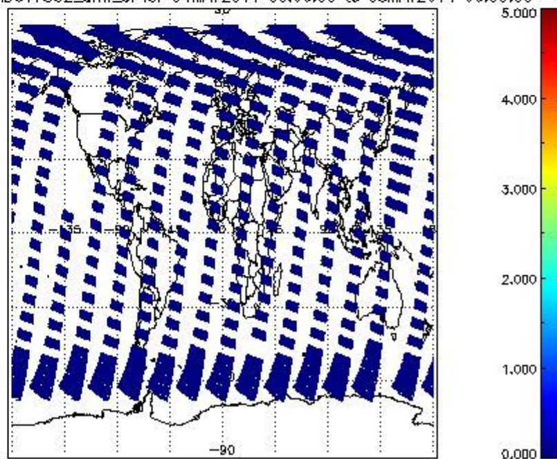
SCIOL2P_NADUV7S02_amf_cl for 04MAY2011 00:00:00 to 05MAY2011 00:00:00
