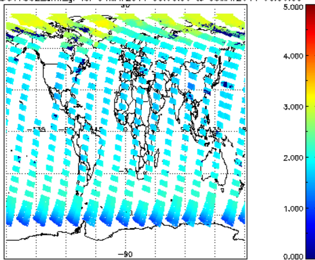
SCIOL2P_NADUV7S02_amf_gr for 04MAY2011 00:00:00 to 05MAY2011 00:00:00
