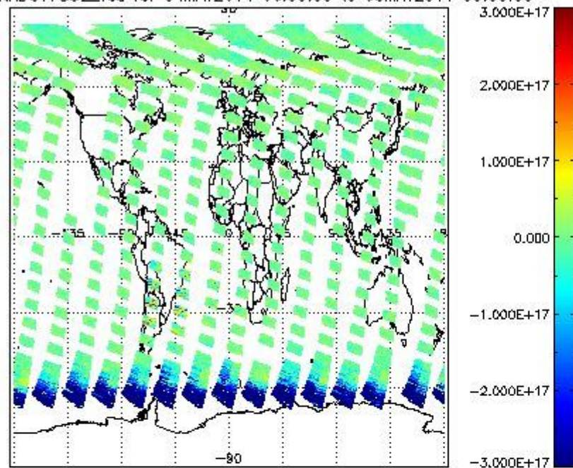
SCIOL2P_NADUV7S02_vcd for 04MAY2011 00:00:00 to 05MAY2011 00:00:00
