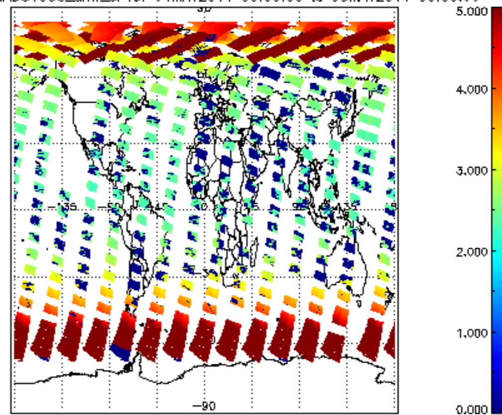
SCIOL2P_NADUV003_amf_cl for 04MAY2011 00:00:00 to 05MAY2011 00:00:00
