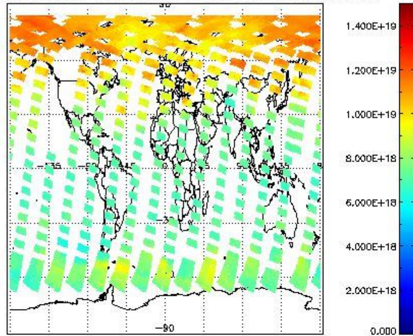
SCIOL2P_NADUV003_vcd for 04MAY2011 00:00:00 to 05MAY2011 00:00:00
