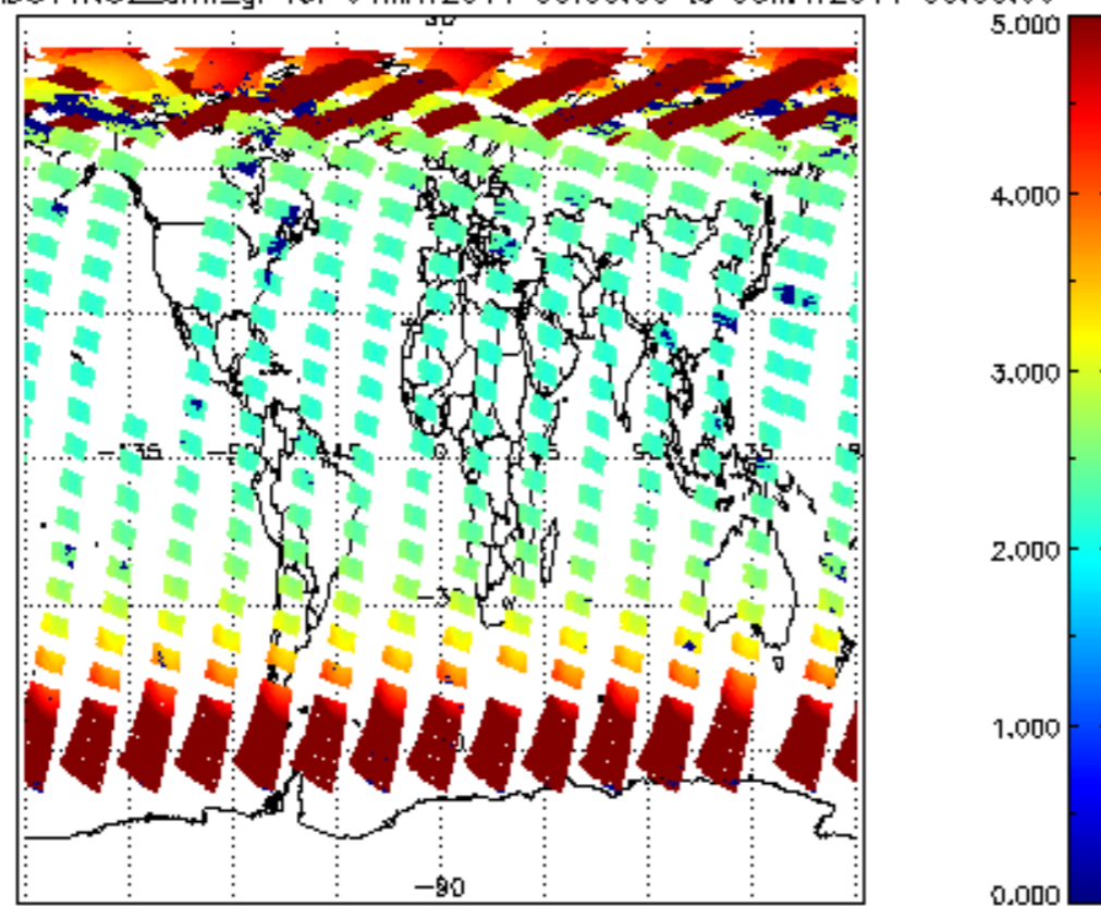
SCIOL2P_NADUV1NO2_amf_gr for 04MAY2011 00:00:00 to 05MAY2011 00:00:00
