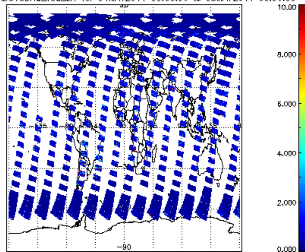
SCIOL2P_NADUV3BRO_vcd_err for 04MAY2011 00:00:00 to 05MAY2011 00:00:00
