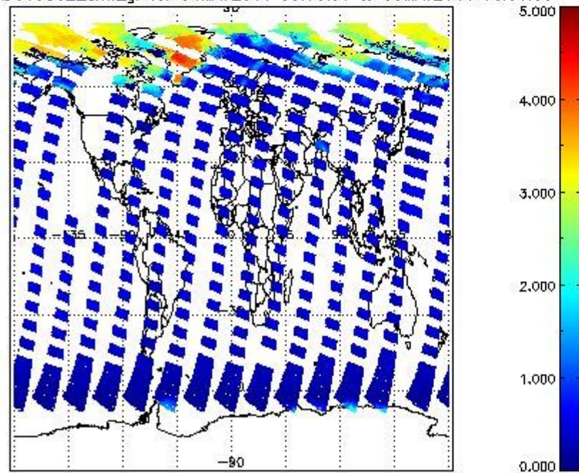
SCIOL2P_NADUV5S02_amf_gr for 04MAY2011 00:00:00 to 05MAY2011 00:00:00
