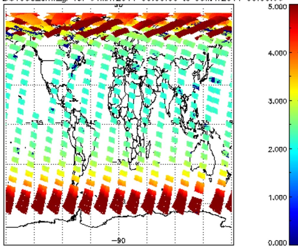
SCIOL2P_NADUV003_amf_gr for 04MAY2011 00:00:00 to 05MAY2011 00:00:00
