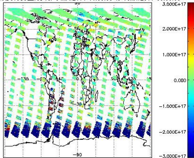
SCIOL2P_NADUV5S02_vcd for 04MAY2011 00:00:00 to 05MAY2011 00:00:00
