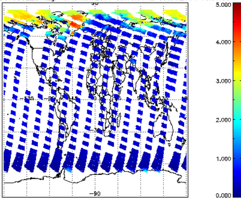
SCIOL2P_NADUV5S02_amf_gr for 04MAY2011 00:00:00 to 05MAY2011 00:00:00
