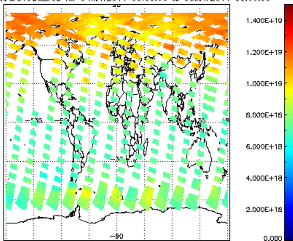
SCIOL2P_NADUV003_vcd for 04MAY2011 00:00:00 to 05MAY2011 00:00:00
