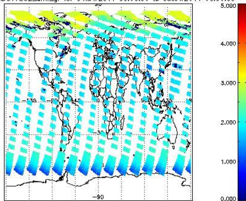
SCIOL2P_NADUV7S02_amf_gr for 04MAY2011 00:00:00 to 05MAY2011 00:00:00
