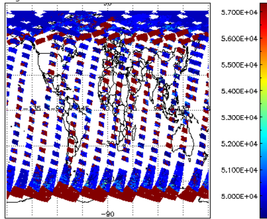
cloud_flags for 04MAY2011 00:00:00 to 05MAY2011 00:00:00
