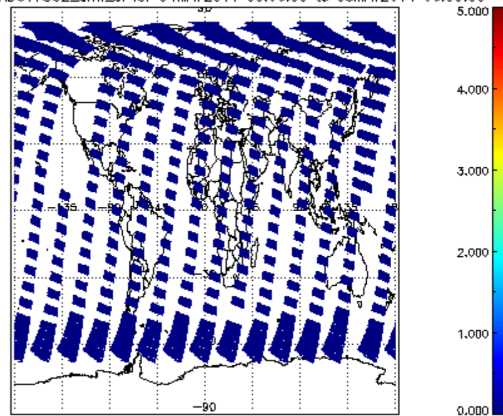
SCIOL2P_NADUV7S02_amf_cl for 04MAY2011 00:00:00 to 05MAY2011 00:00:00
