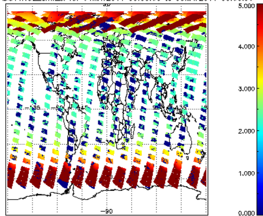
SCIOL2P_NADUV1NO2_amf_sl for 04MAY2011 00:00:00 to 05MAY2011 00:00:00
