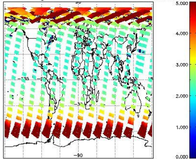
SCIOL2P_NADUV003_amf_gr for 04MAY2011 00:00:00 to 05MAY2011 00:00:00
