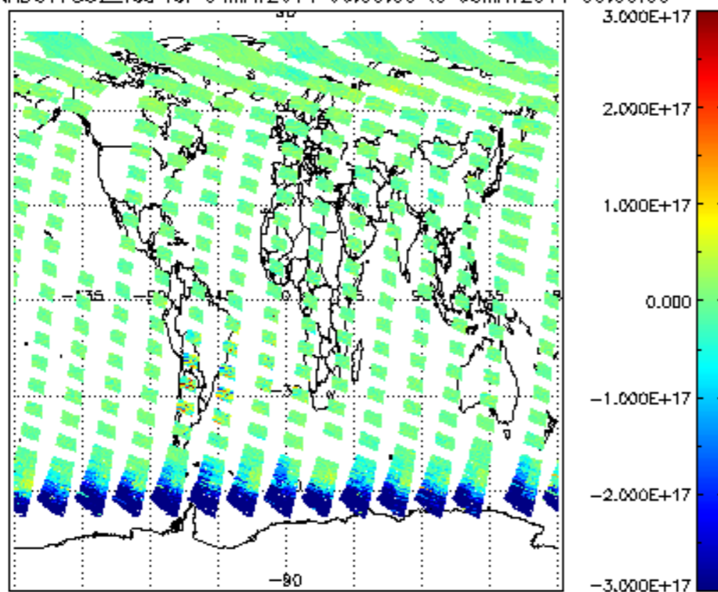
SCIOL2P_NADUV7S02_vcd for 04MAY2011 00:00:00 to 05MAY2011 00:00:00
