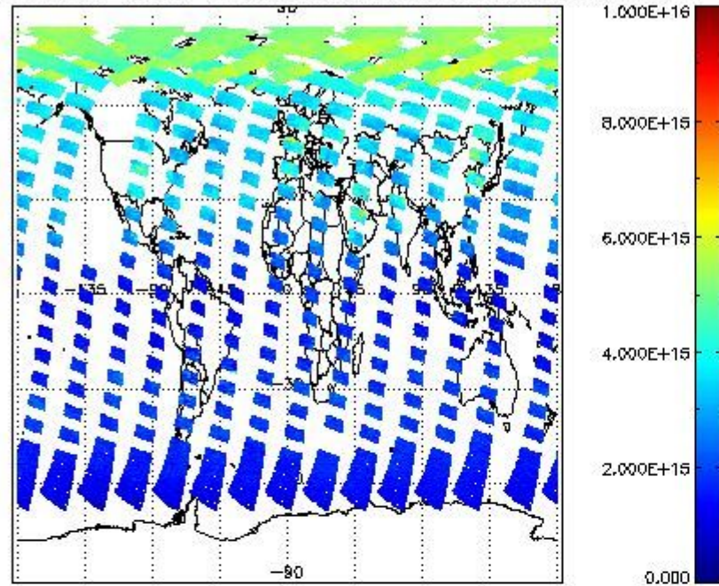
SCIOL2P_NADUV1NO2_vcd for 04MAY2011 00:00:00 to 05MAY2011 00:00:00
