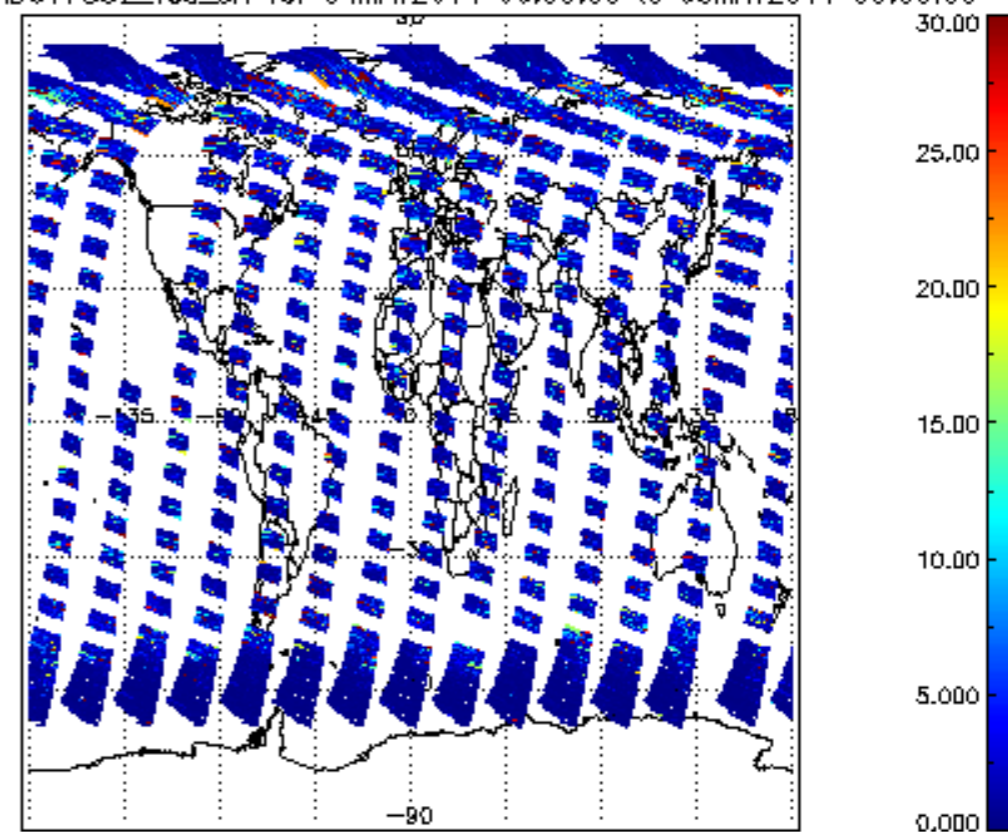
SCIOL2P_NADUV7S02_vcd_err for 04MAY2011 00:00:00 to 05MAY2011 00:00:00
