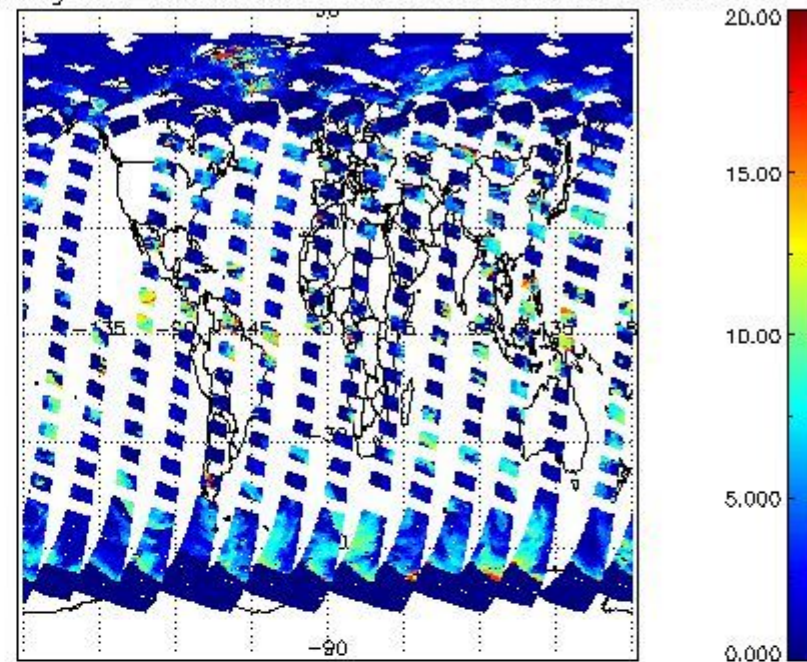
cL_top_height for 04MAY2011 00:00:00 to 05MAY2011 00:00:00
