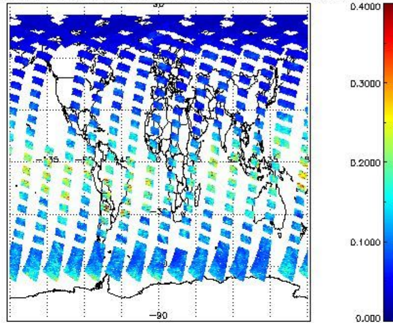
SCIOL2P_NADUV1NO2_vcd_err for 04MAY2011 00:00:00 to 05MAY2011 00:00:00
