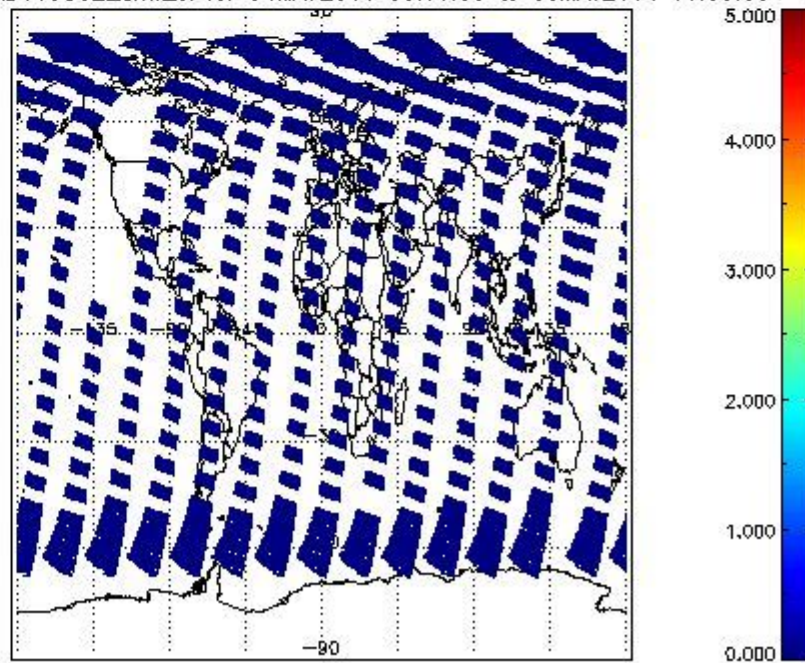
SCIOL2P_NADUV5S02_amf_cl for 04MAY2011 00:00:00 to 05MAY2011 00:00:00
