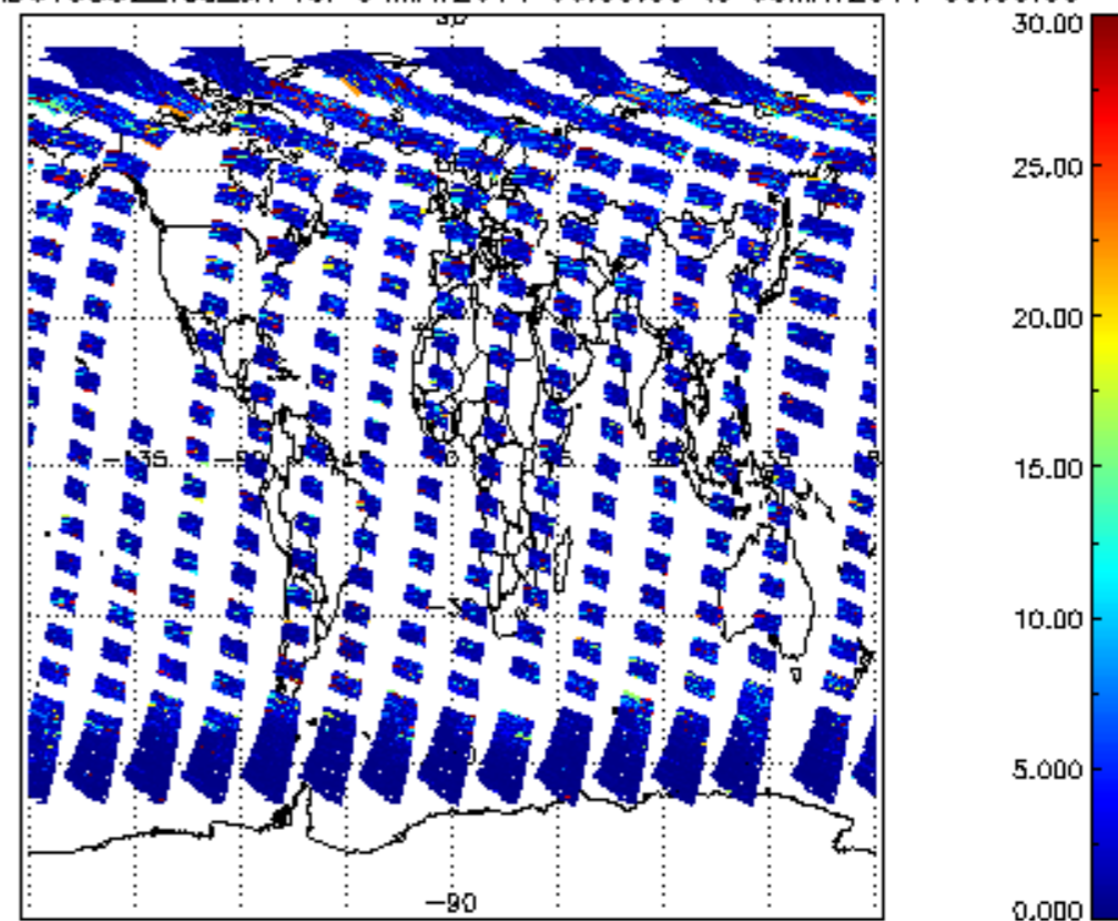
SCIOL2P_NADUV5S02_vcd_err for 04MAY2011 00:00:00 to 05MAY2011 00:00:00
