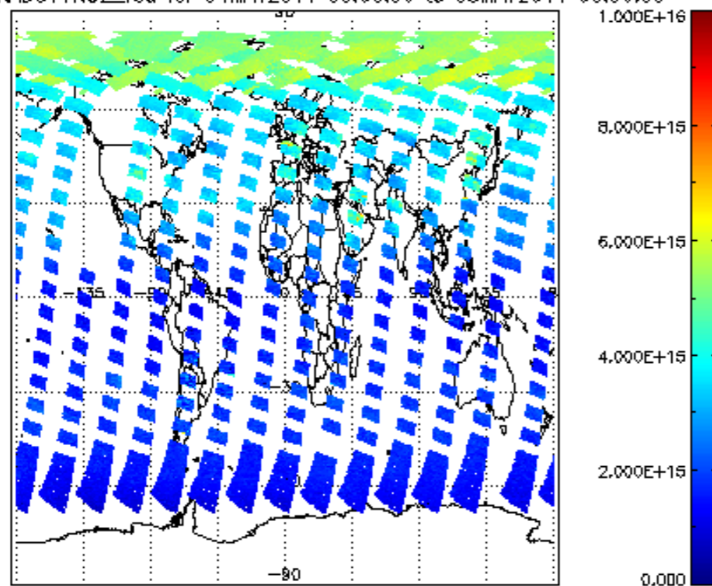
SCIOL2P_NADUV1NO2_vcd for 04MAY2011 00:00:00 to 05MAY2011 00:00:00
