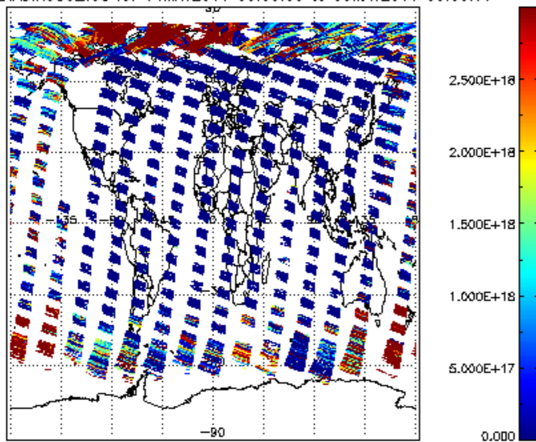
SCIOL2P_NADIR3CO_vcd for 04MAY2011 00:00:00 to 05MAY2011 00:00:00
