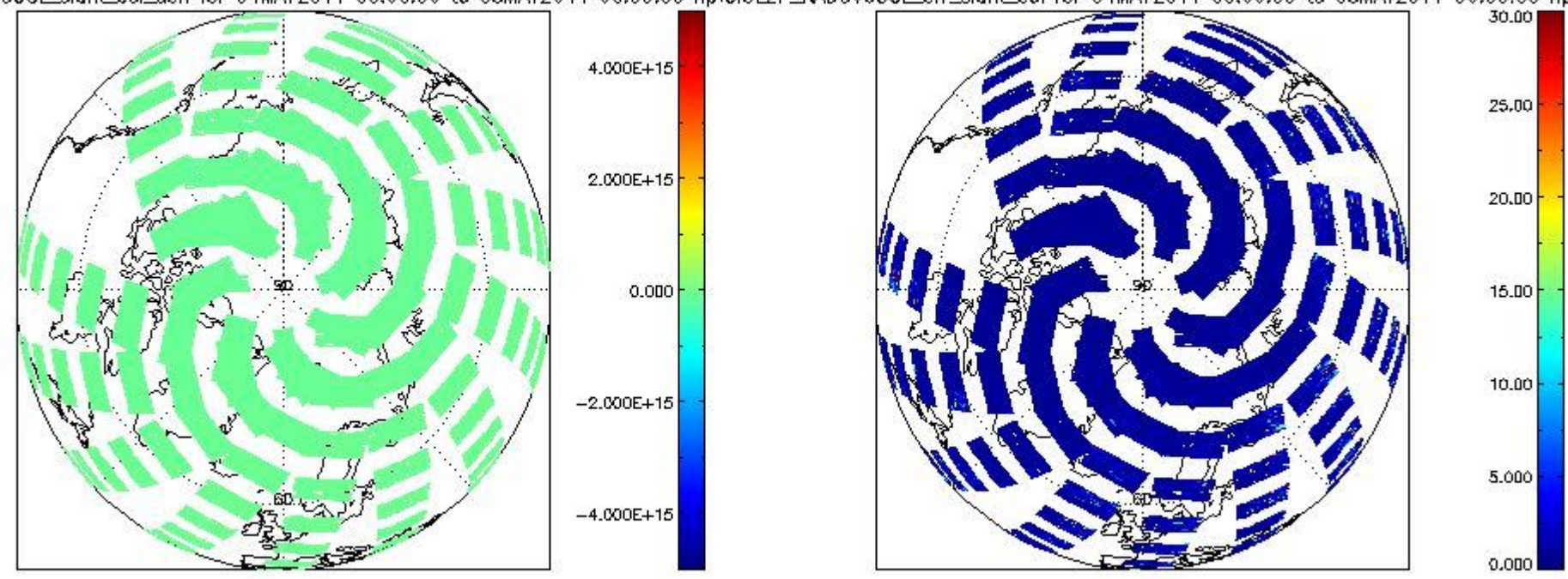
CIOL2P_NADUV60CLslant_col_den for 04MAY2011 00:00:00 to 05MAY2011 00:00:00 np; CIOL2P_NADUV60CLerr_slant_col for 04MAY2011 00:00:00 to 05MAY2011 00:00:00 np
