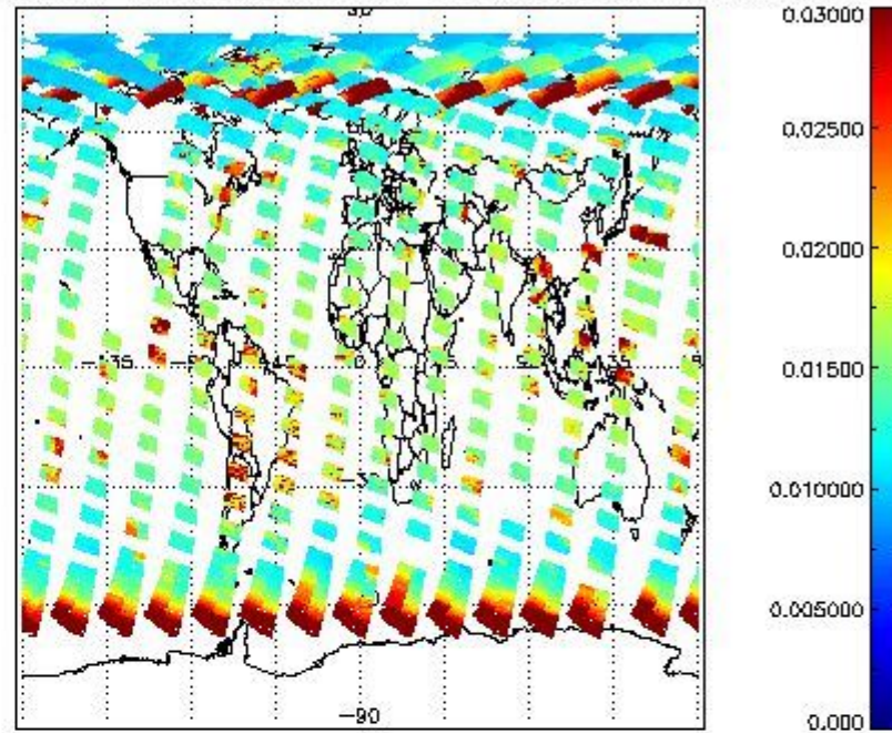
SCIOL2P_NADUV003_vcd_err for 04MAY2011 00:00:00 to 05MAY2011 00:00:00
