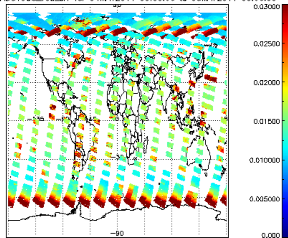
SCIOL2P_NADUV003_vcd_err for 04MAY2011 00:00:00 to 05MAY2011 00:00:00
