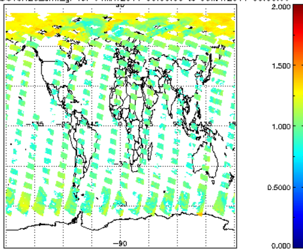
SCIOL2P_NADUV8H2O_amf_gr for 04MAY2011 00:00:00 to 05MAY2011 00:00:00
