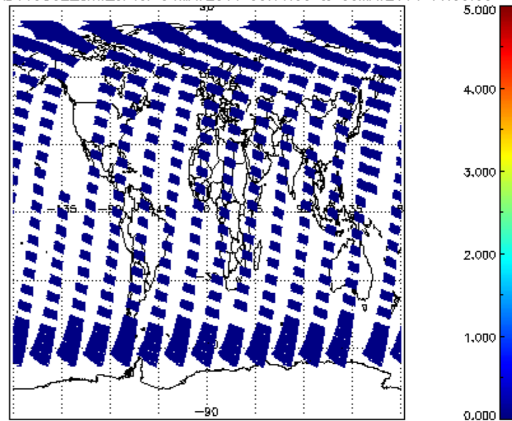
SCIOL2P_NADUV5S02_amf_cl for 04MAY2011 00:00:00 to 05MAY2011 00:00:00
