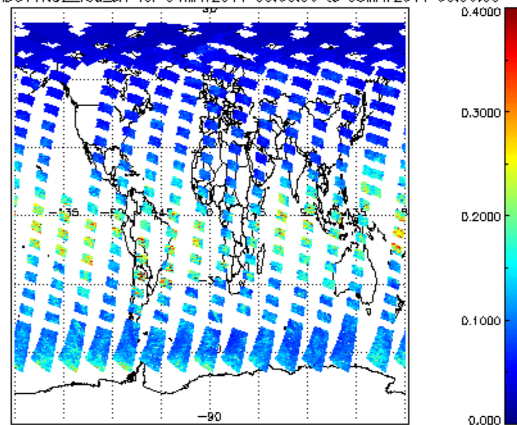
SCIOL2P_NADUV1NO2_vcd_err for 04MAY2011 00:00:00 to 05MAY2011 00:00:00
