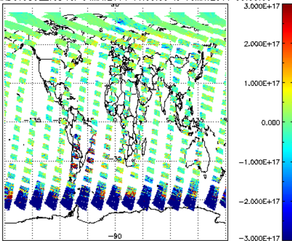
SCIOL2P_NADUV5S02_vcd for 04MAY2011 00:00:00 to 05MAY2011 00:00:00
