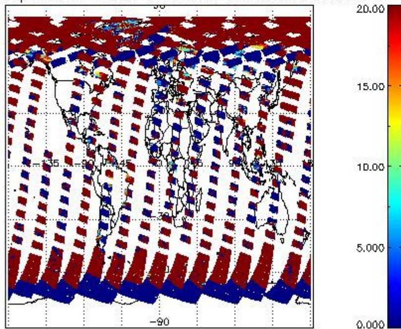
cL_opt_depth for 04MAY2011 00:00:00 to 05MAY2011 00:00:00
