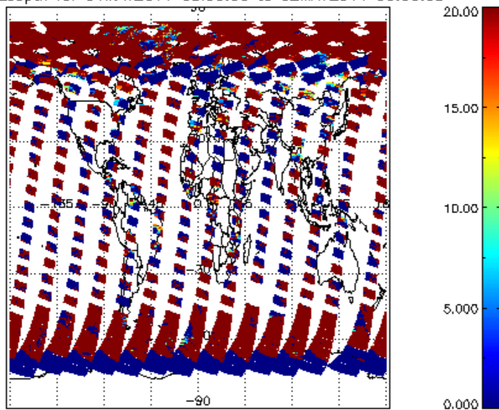
cl_opt_depth for 01MAY2011 00:00:00 to 02MAY2011 00:00:00
