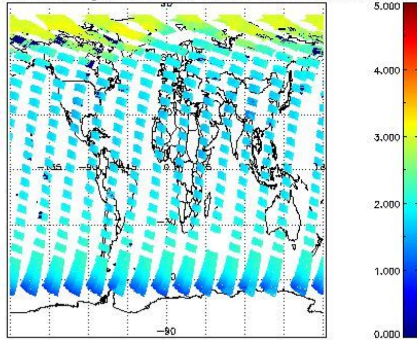
SCIOL2P_NADUV7S02_amf_gr for 01MAY2011 00:00:00 to 02MAY2011 00:00:00
