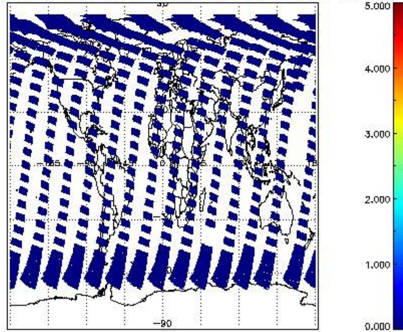
SCIOL2P_NADUV7S02_amf_cl for 01MAY2011 00:00:00 to 02MAY2011 00:00:00
