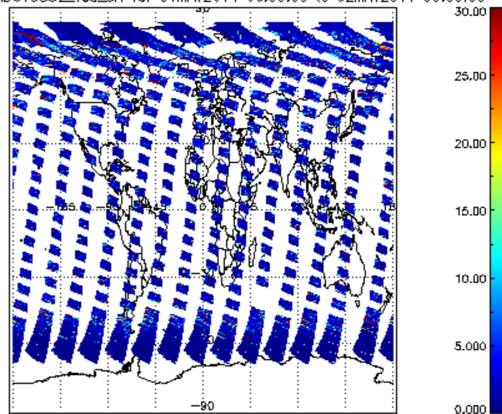
SCIOL2P_NADUV5S02_vcd_err for 01MAY2011 00:00:00 to 02MAY2011 00:00:00
