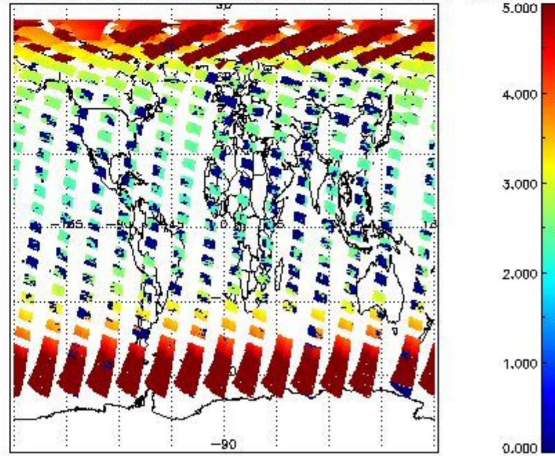
SCIOL2P_NADUV3BRO_amf_cl for 01MAY2011 00:00:00 to 02MAY2011 00:00:00
