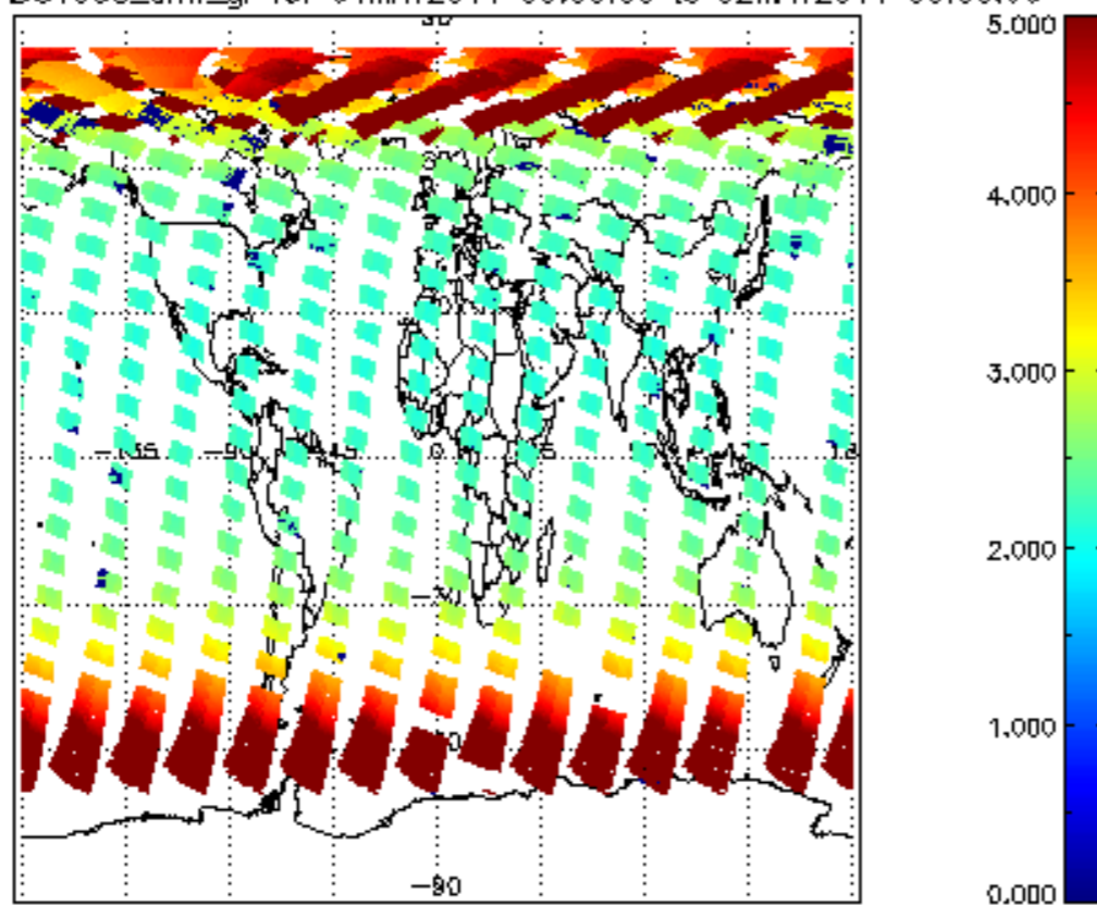
SCIOL2P_NADUV003_amf_gr for 01MAY2011 00:00:00 to 02MAY2011 00:00:00
