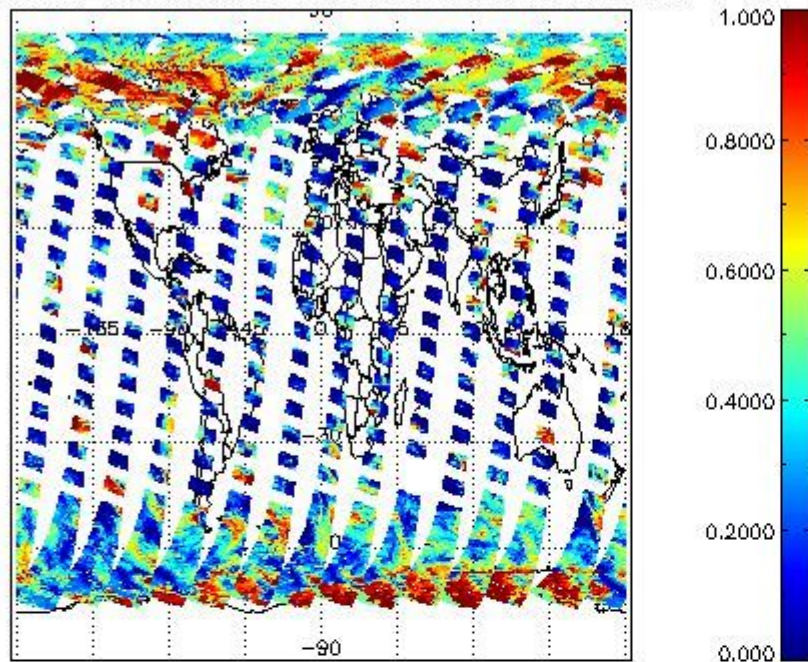
cL_frac for 01MAY2011 00:00:00 to 02MAY2011 00:00:00
