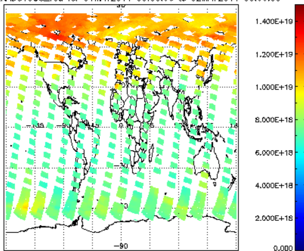
SCIOL2P_NADUV003_vcd for 01MAY2011 00:00:00 to 02MAY2011 00:00:00
