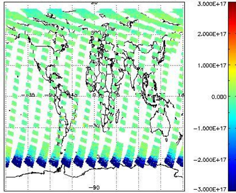
SCIOL2P_NADUV7S02_vcd for 01MAY2011 00:00:00 to 02MAY2011 00:00:00
