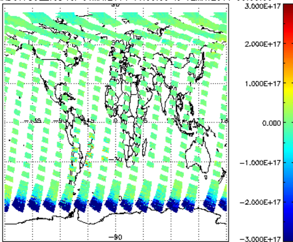
SCIOL2P_NADUV7S02_vcd for 01MAY2011 00:00:00 to 02MAY2011 00:00:00
