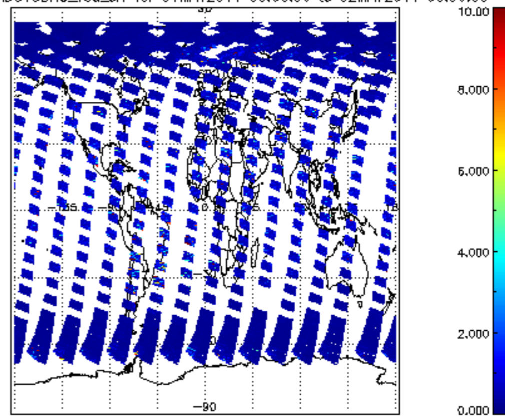
SCIOL2P_NADUV3BRO_vcd_err for 01MAY2011 00:00:00 to 02MAY2011 00:00:00
