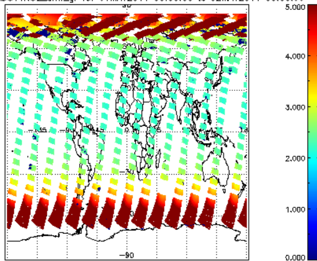
SCIOL2P_NADUV1NO2_amf_gr for 01MAY2011 00:00:00 to 02MAY2011 00:00:00
