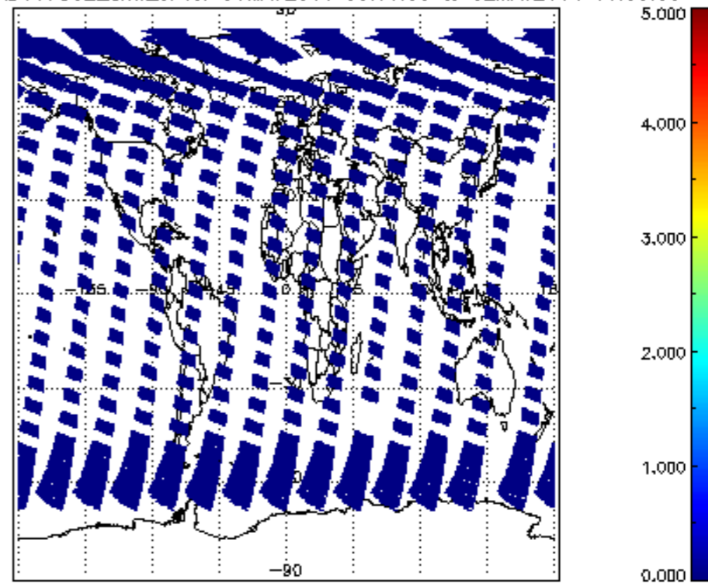
SCIOL2P_NADUV7S02_amf_cl for 01MAY2011 00:00:00 to 02MAY2011 00:00:00
