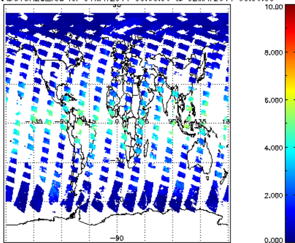
SCIOL2P_NADUV8H2O_vcd for 01MAY2011 00:00:00 to 02MAY2011 00:00:00
