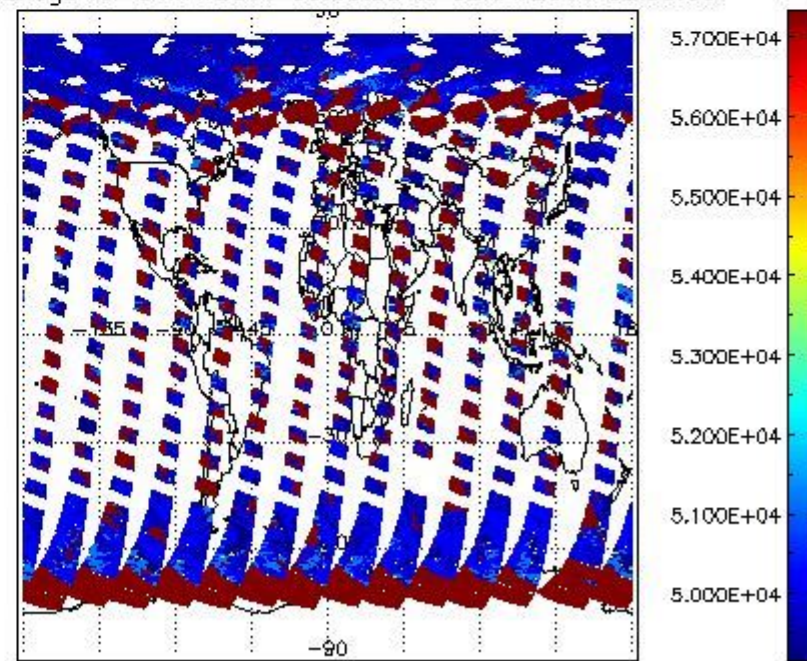
cloud_flags for 01MAY2011 00:00:00 to 02MAY2011 00:00:00
