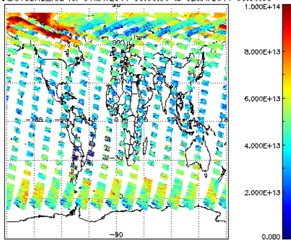
SCIOL2P_NADUV3BRO_vcd for 01MAY2011 00:00:00 to 02MAY2011 00:00:00
