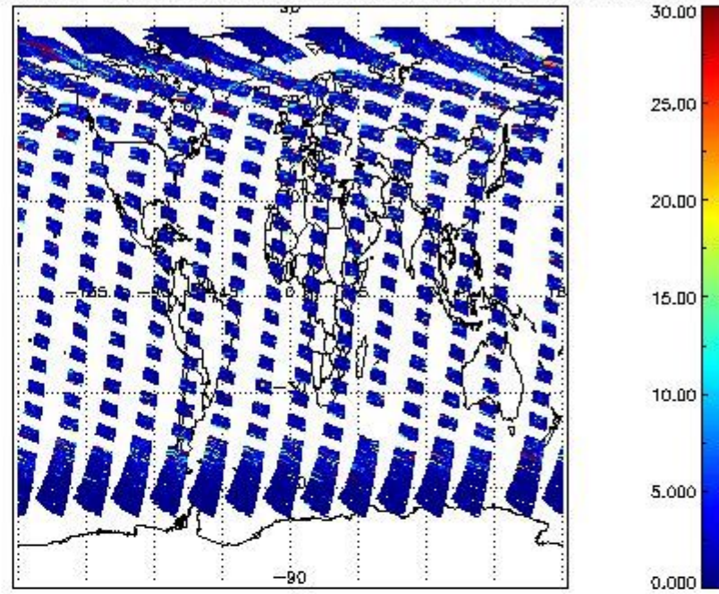
SCIOL2P_NADUV7S02_vcd_err for 01MAY2011 00:00:00 to 02MAY2011 00:00:00
