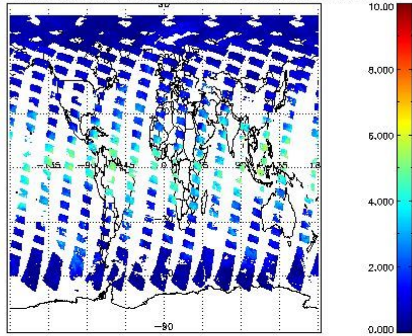
SCIOL2P_NADUV8H2O_vcd for 01MAY2011 00:00:00 to 02MAY2011 00:00:00
