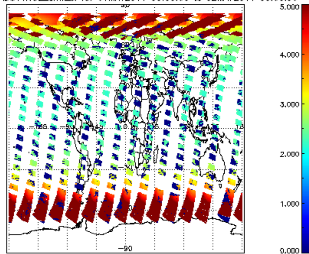
SCIOL2P_NADUV1NO2_amf_sl for 01MAY2011 00:00:00 to 02MAY2011 00:00:00
