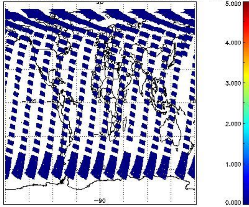
SCIOL2P_NADUV5S02_amf_cl for 01MAY2011 00:00:00 to 02MAY2011 00:00:00
