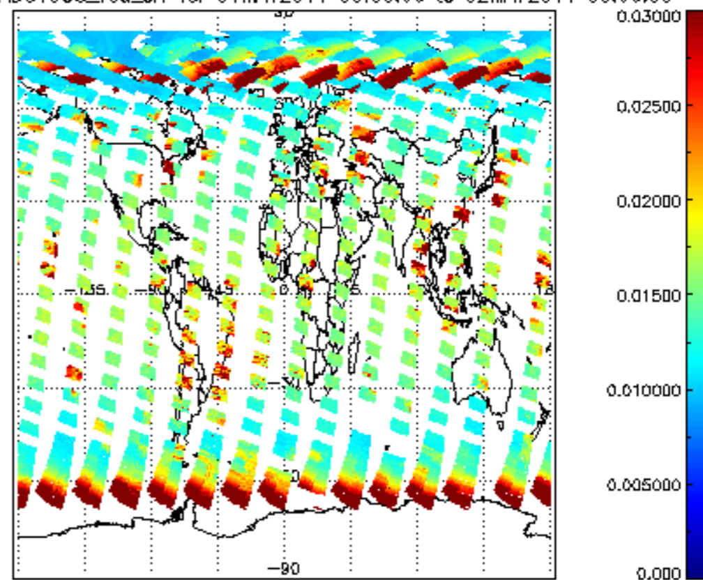
SCIOL2P_NADUV003_vcd_err for 01MAY2011 00:00:00 to 02MAY2011 00:00:00
