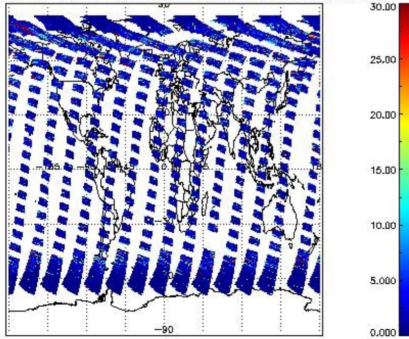
SCIOL2P_NADUV5S02_vcd_err for 01MAY2011 00:00:00 to 02MAY2011 00:00:00
