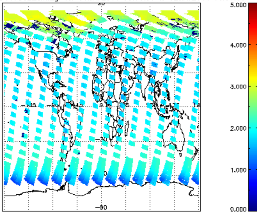
SCIOL2P_NADUV7S02_amf_gr for 01MAY2011 00:00:00 to 02MAY2011 00:00:00
