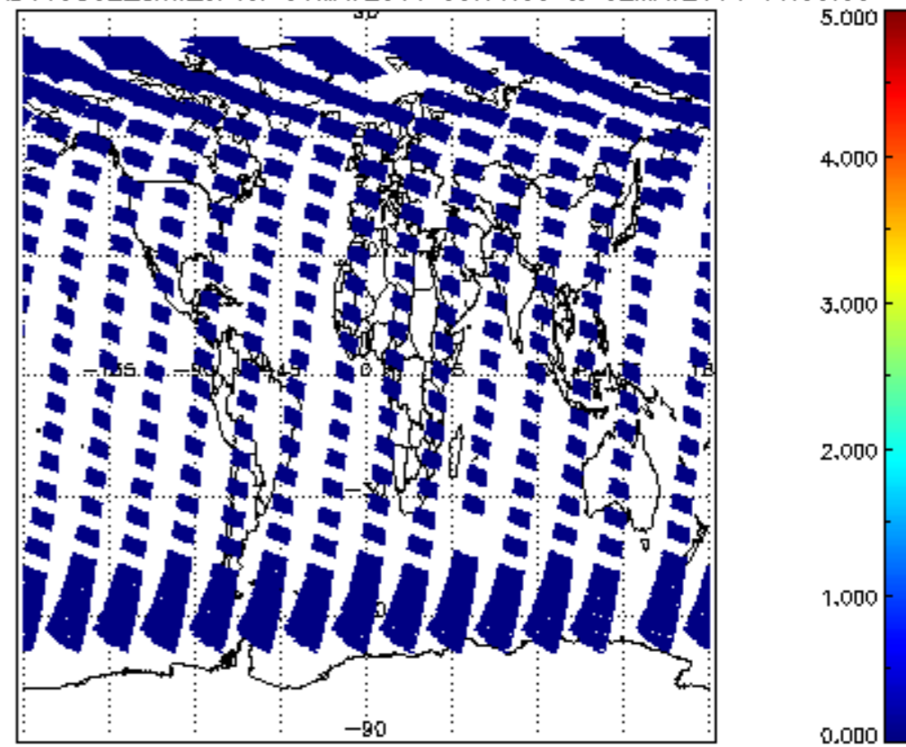
SCIOL2P_NADUV5S02_amf_cl for 01MAY2011 00:00:00 to 02MAY2011 00:00:00
