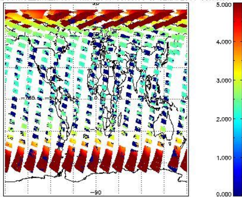
SCIOL2P_NADUV1NO2_amf_cl for 01MAY2011 00:00:00 to 02MAY2011 00:00:00
