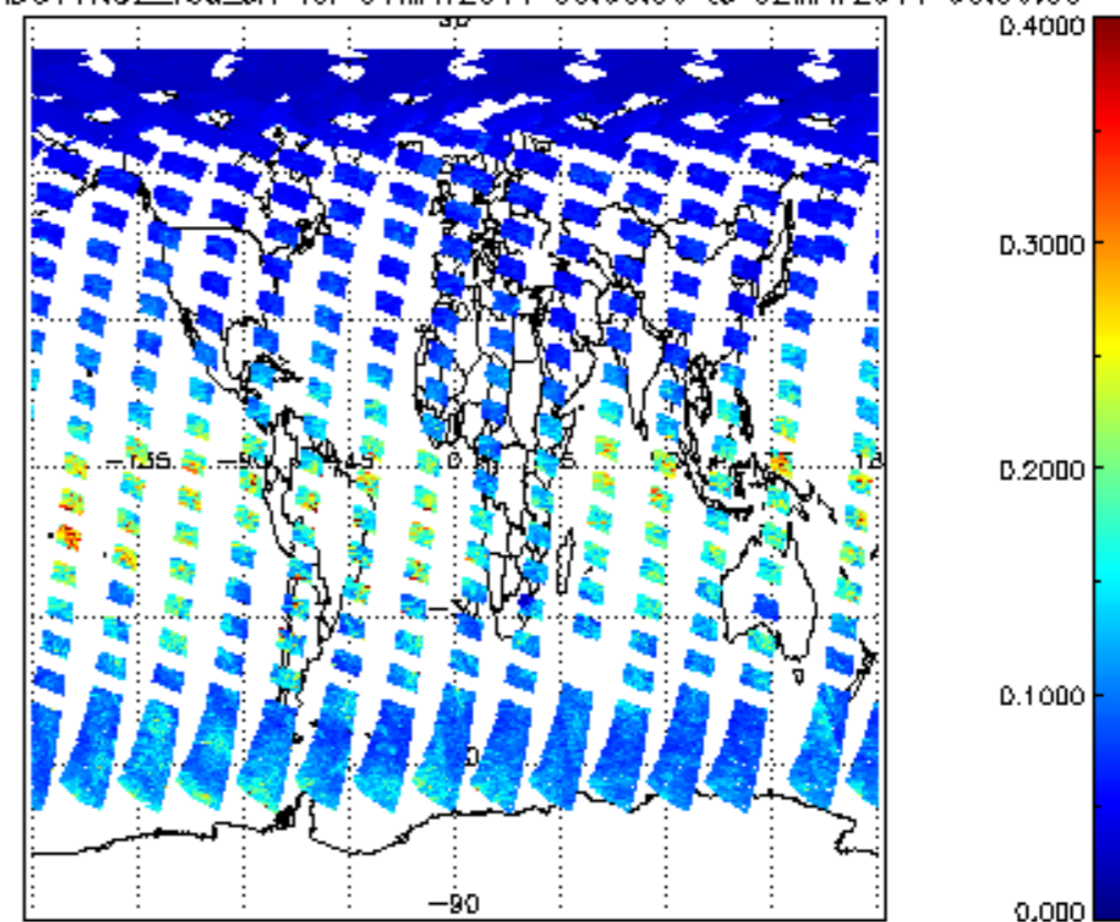
SCIOL2P_NADUV1NO2_vcd_err for 01MAY2011 00:00:00 to 02MAY2011 00:00:00
