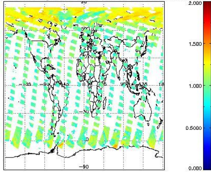
SCIOL2P_NADUV8H2O_arnf_gr for 01MAY2011 00:00:00 to 02MAY2011 00:00:00
