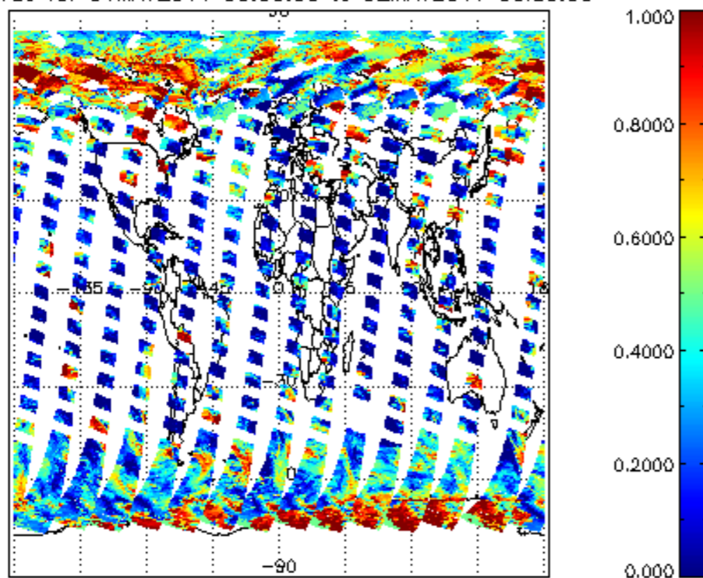
cl_frac for 01MAY2011 00:00:00 to 02MAY2011 00:00:00
