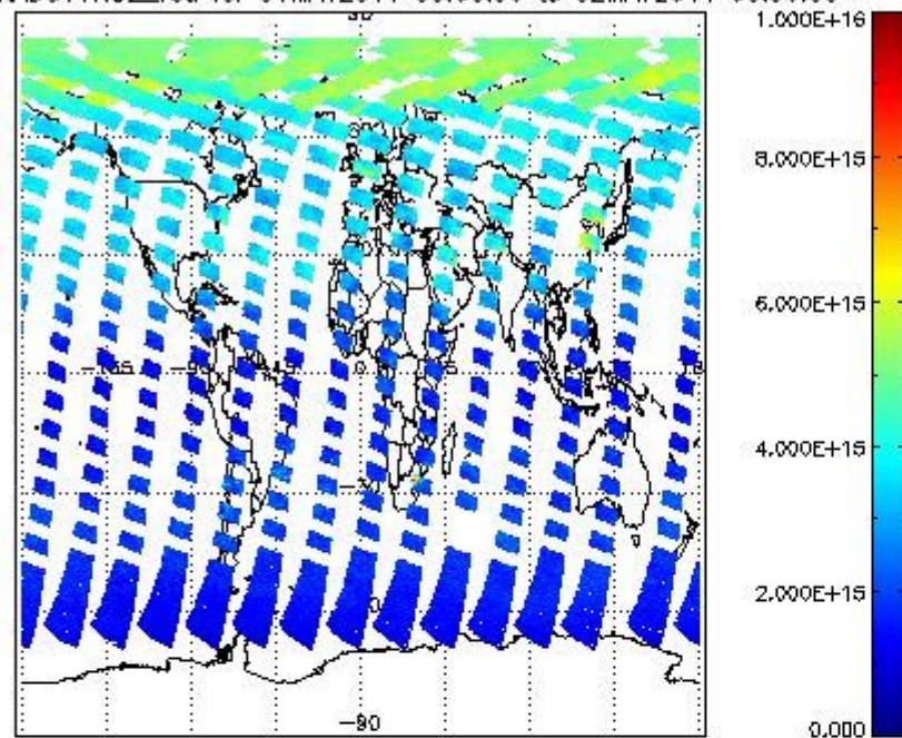
SCIOL2P_NADUV1NO2_vcd for 01MAY2011 00:00:00 to 02MAY2011 00:00:00
