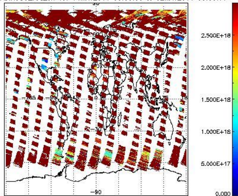
SCIDL2P_NADIR3CO_vcd_err for 01MAY2011 00:00:00 to 02MAY2011 00:00:00
