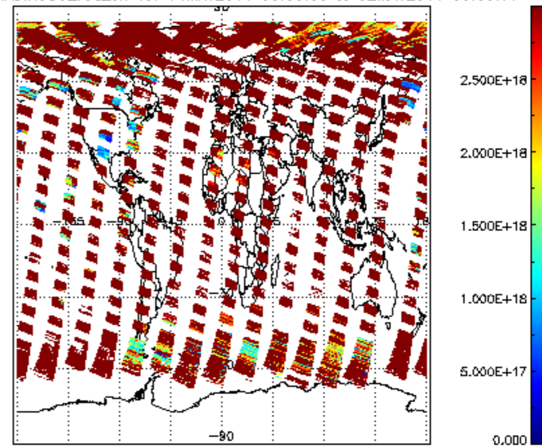
SCIOL2P_NADIR3CO_vcd_err for 01MAY2011 00:00:00 to 02MAY2011 00:00:00
