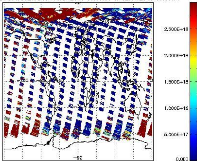
SCIDL2P_NADIR3CO_vcd for 01MAY2011 00:00:00 to 02MAY2011 00:00:00
