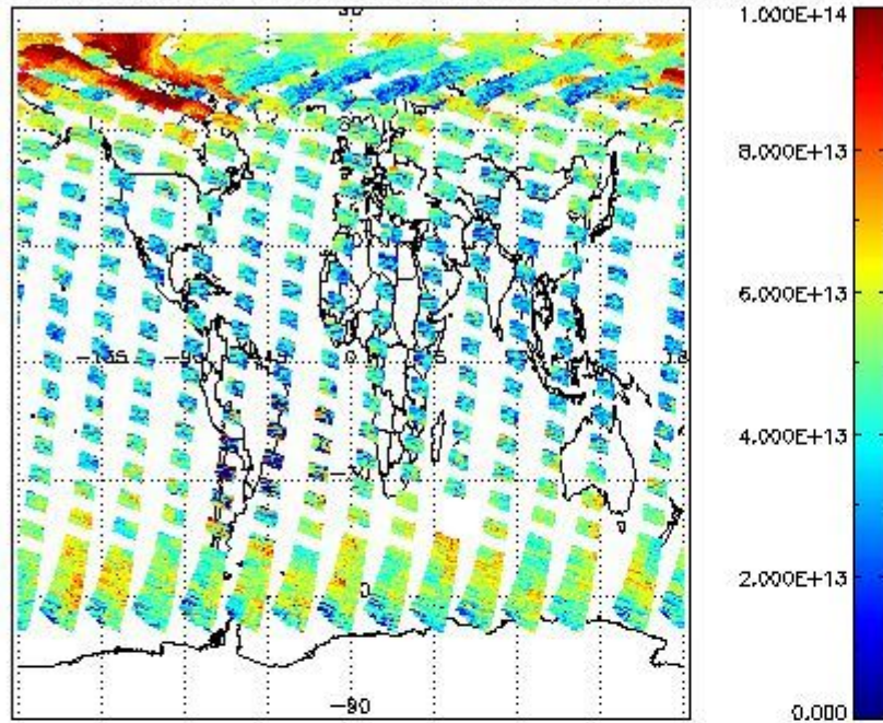
SCIOL2P_NADUV3BRO_vcd for 01MAY2011 00:00:00 to 02MAY2011 00:00:00
