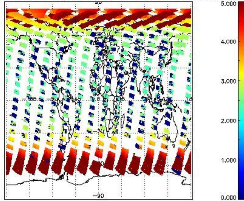
SCIOL2P_NADUV003_amf_cl for 01MAY2011 00:00:00 to 02MAY2011 00:00:00
