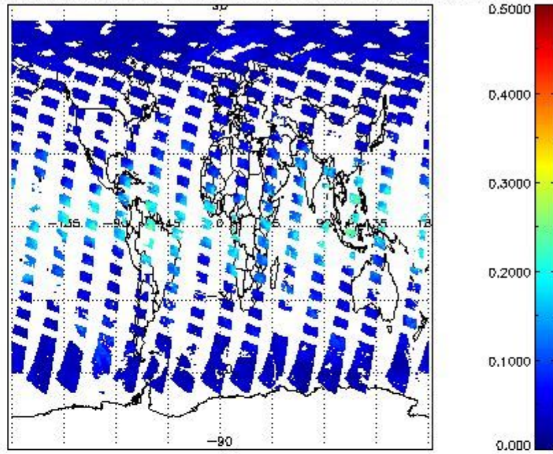
SCIOL2P_NADUV8H2O_vcd_err for 01MAY2011 00:00:00 to 02MAY2011 00:00:00
