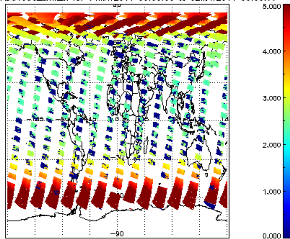
SCIOL2P_NADUV003_amf_cl for 01MAY2011 00:00:00 to 02MAY2011 00:00:00
