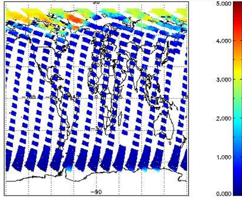
SCIOL2P_NADUV5S02_amf_gr for 01MAY2011 00:00:00 to 02MAY2011 00:00:00
