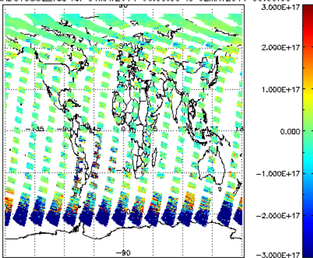
SCIOL2P_NADUV5S02_vcd for 01MAY2011 00:00:00 to 02MAY2011 00:00:00
