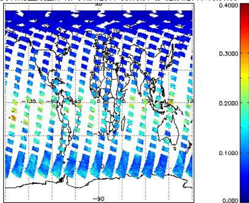
SCIOL2P_NADUV1NO2_vcd_err for 01MAY2011 00:00:00 to 02MAY2011 00:00:00
