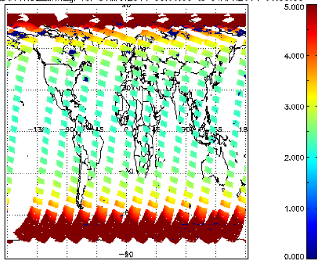
SCIOL2P_NADUV1NO2_amf_gr for 31MAR2011 00:00:00 to 01APR2011 00:00:00
