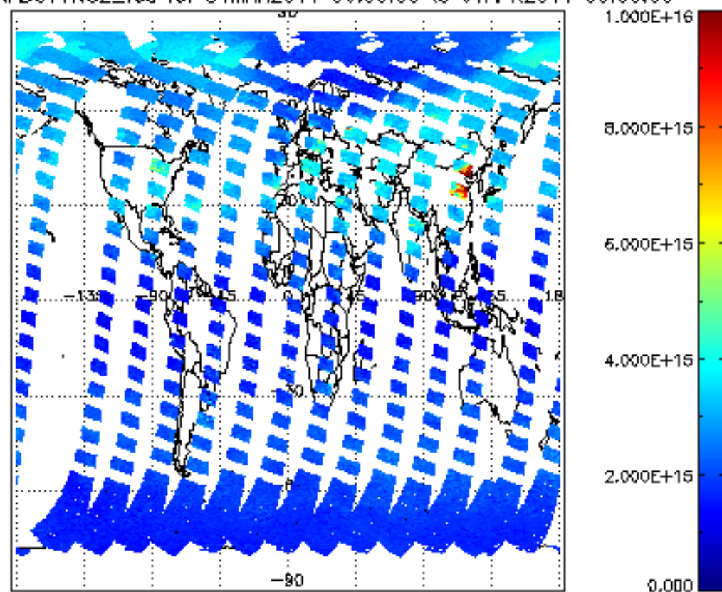
SCIOL2P_NADUV1NO2_vcd for 31MAR2011 00:00:00 to 01APR2011 00:00:00
