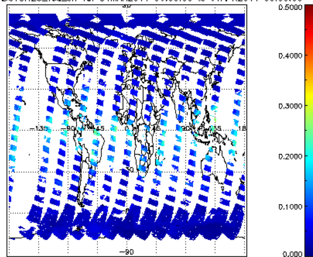
SCIOL2P_NADUV8H20_vcd_err for 31MAR2011 00:00:00 to 01APR2011 00:00:00
