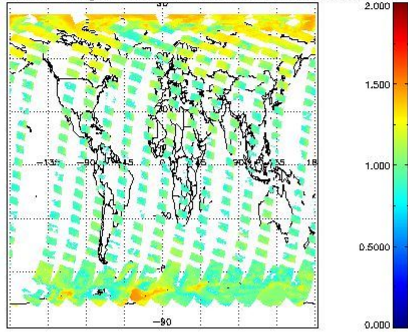
SCIOL2P_NADUV8H2O_amf_gr for 31MAR2011 00:00:00 to 01APR2011 00:00:00
