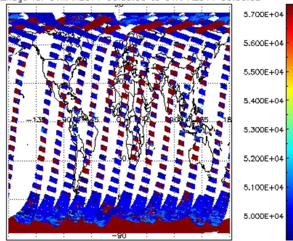
cloud_flags for 31MAR2011 00:00:00 to 01APR2011 00:00:00
