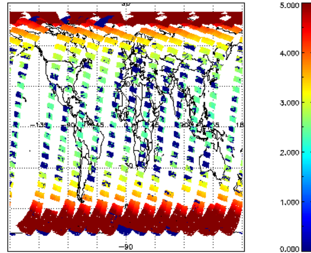
SCIOL2P_NADUV003_amf_cl for 31MAR2011 00:00:00 to 01APR2011 00:00:00
