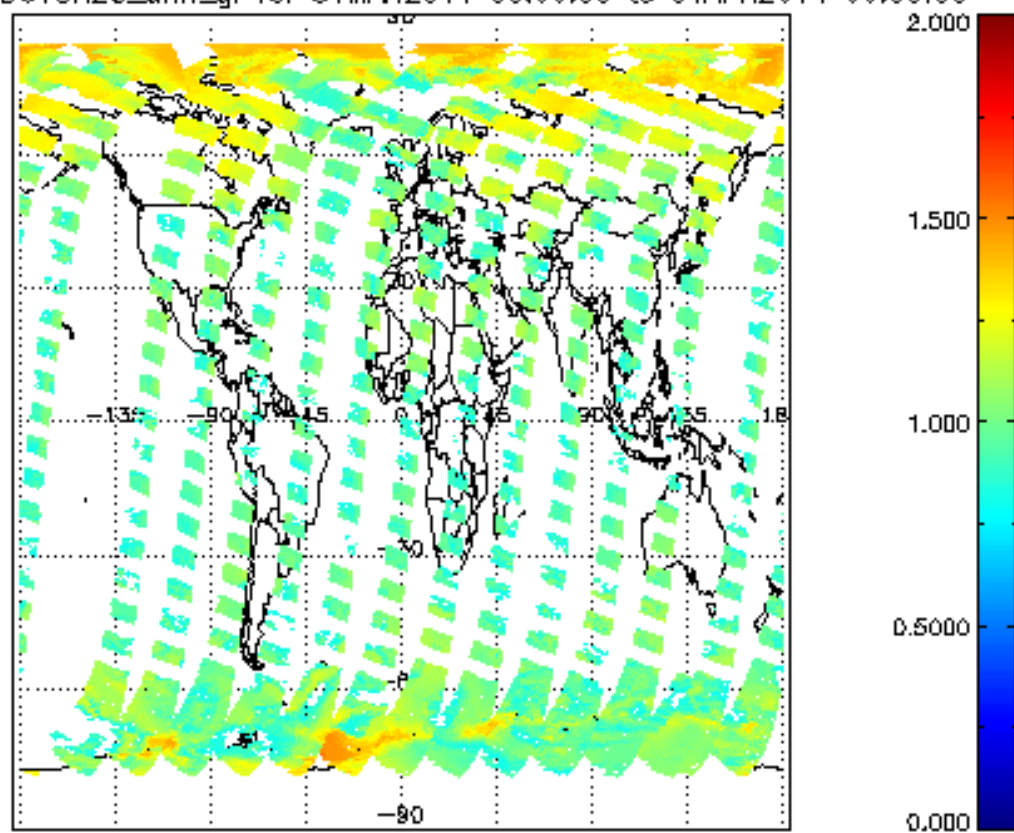
SCIOL2P_NADUV8H20_amf_gr for 31MAR2011 00:00:00 to 01APR2011 00:00:00
