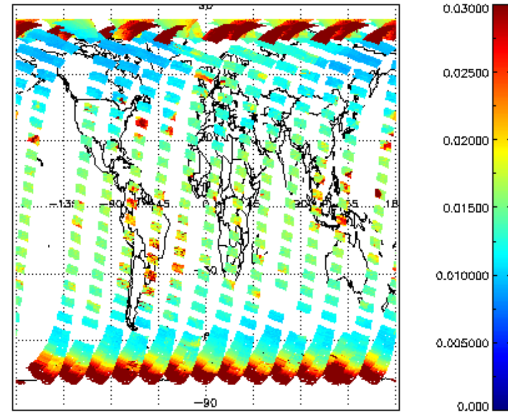
SCIOL2P_NADUV003_vcd_err for 31MAR2011 00:00:00 to 01APR2011 00:00:00
