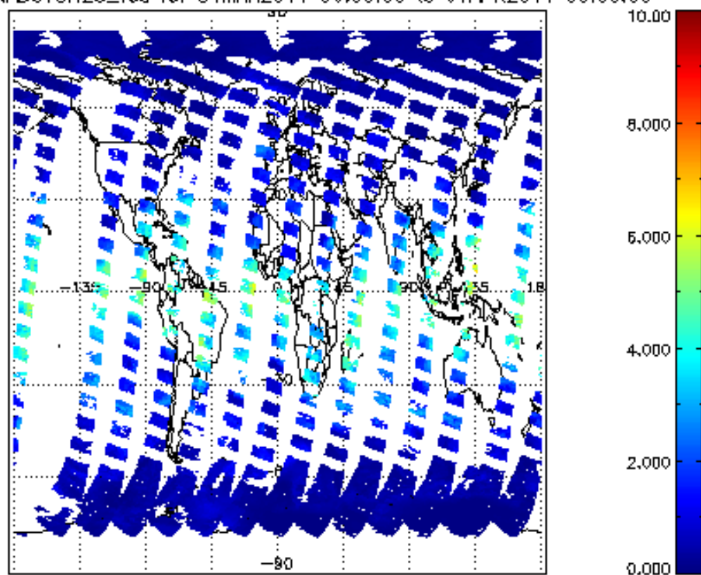
SCIOL2P_NADUV8H20_vcd for 31MAR2011 00:00:00 to 01APR2011 00:00:00
