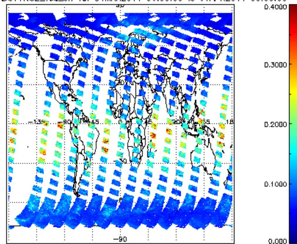
SCIOL2P_NADUV1NO2_vcd_err for 31MAR2011 00:00:00 to 01APR2011 00:00:00
