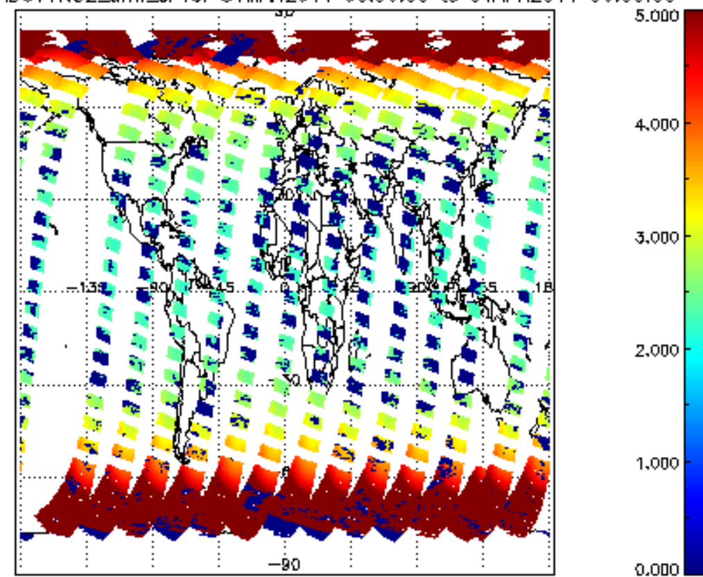
SCIOL2P_NADUV1NO2_amf_cl for 31MAR2011 00:00:00 to 01APR2011 00:00:00
