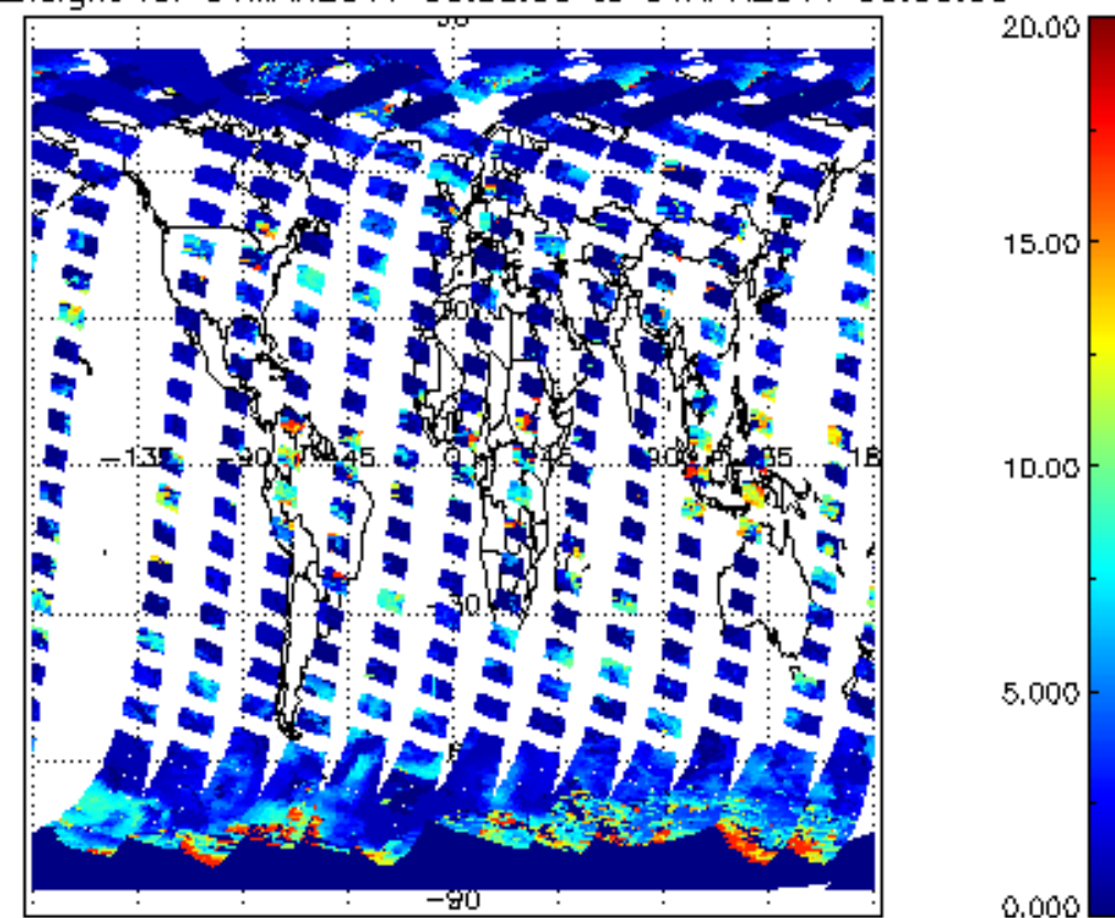
cL_top_height for 31MAR2011 00:00:00 to 01APR2011 00:00:00
