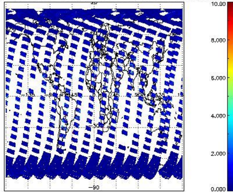
SCIOL2P_NADUV3BRO_vcd_err for 30MAR2011 00:00:00 to 31MAR2011 00:00:00
