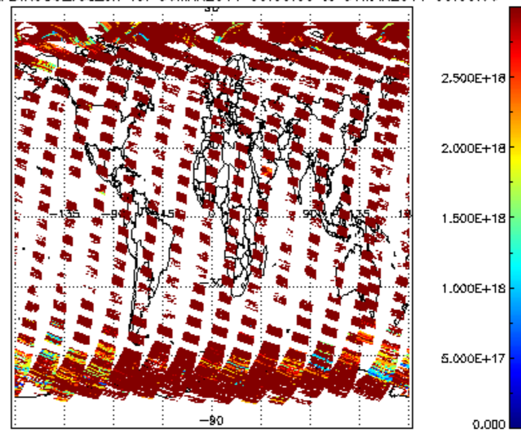
SCIOL2P_NADIR3CO_vcd_err for 30MAR2011 00:00:00 to 31MAR2011 00:00:00
