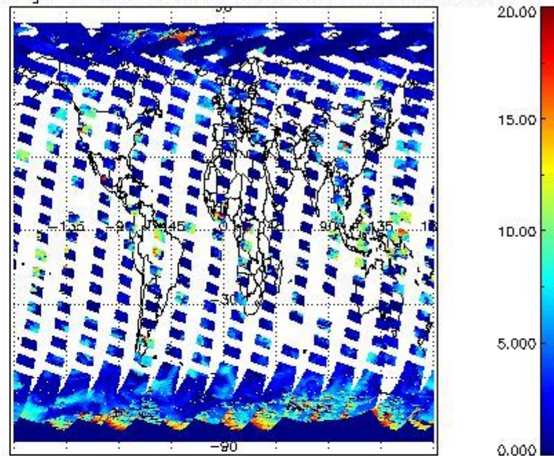
cL_top_height for 30MAR2011 00:00:00 to 31MAR2011 00:00:00
