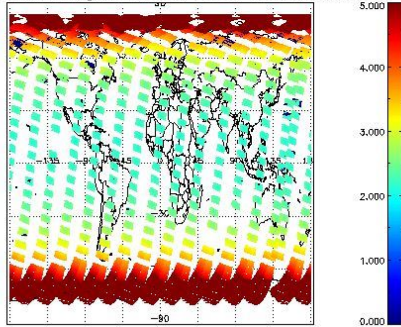
SCIOL2P_NADUV3BRO_amf_gr for 30MAR2011 00:00:00 to 31MAR2011 00:00:00
