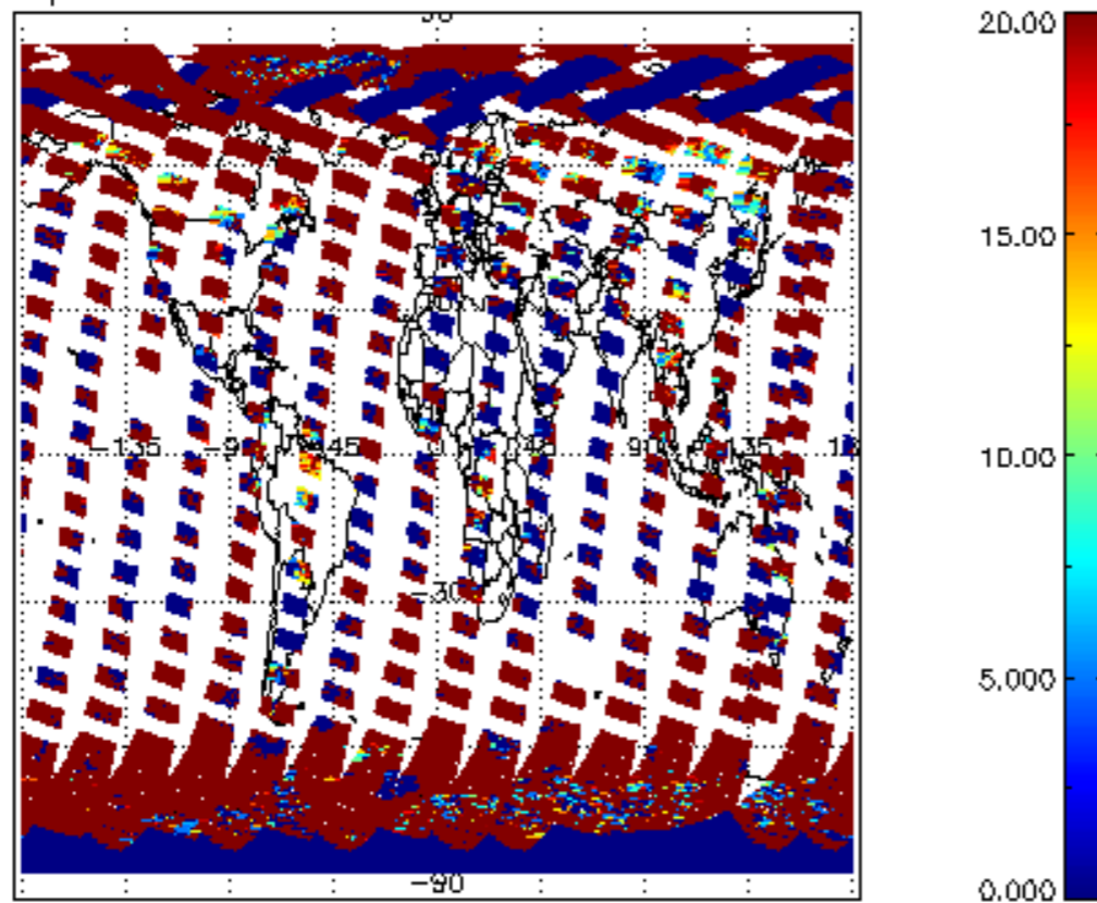
cL_opt_depth for 30MAR2011 00:00:00 to 31MAR2011 00:00:00
