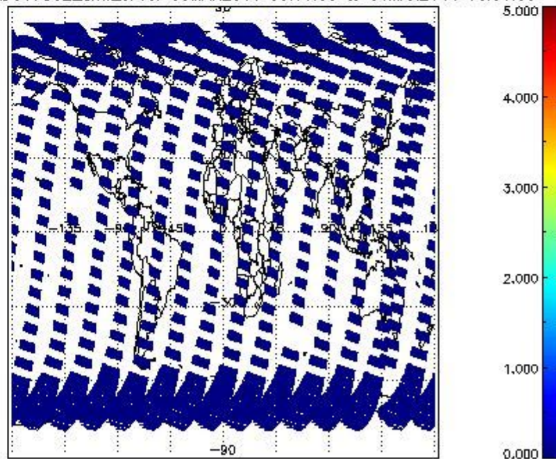
SCIOL2P_NADUV7S02_amf_cl for 30MAR2011 00:00:00 to 31MAR2011 00:00:00
