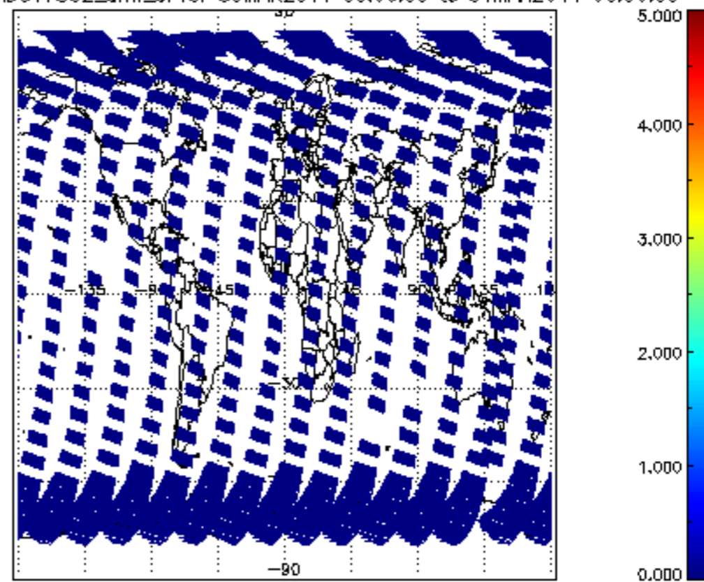
SCIOL2P_NADUV7S02_amf_cl for 30MAR2011 00:00:00 to 31MAR2011 00:00:00
