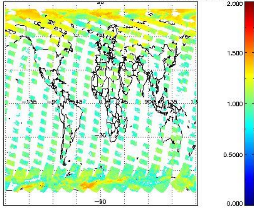
SCIOL2P_NADUV8H2O_arnf_gr for 30MAR2011 00:00:00 to 31MAR2011 00:00:00
