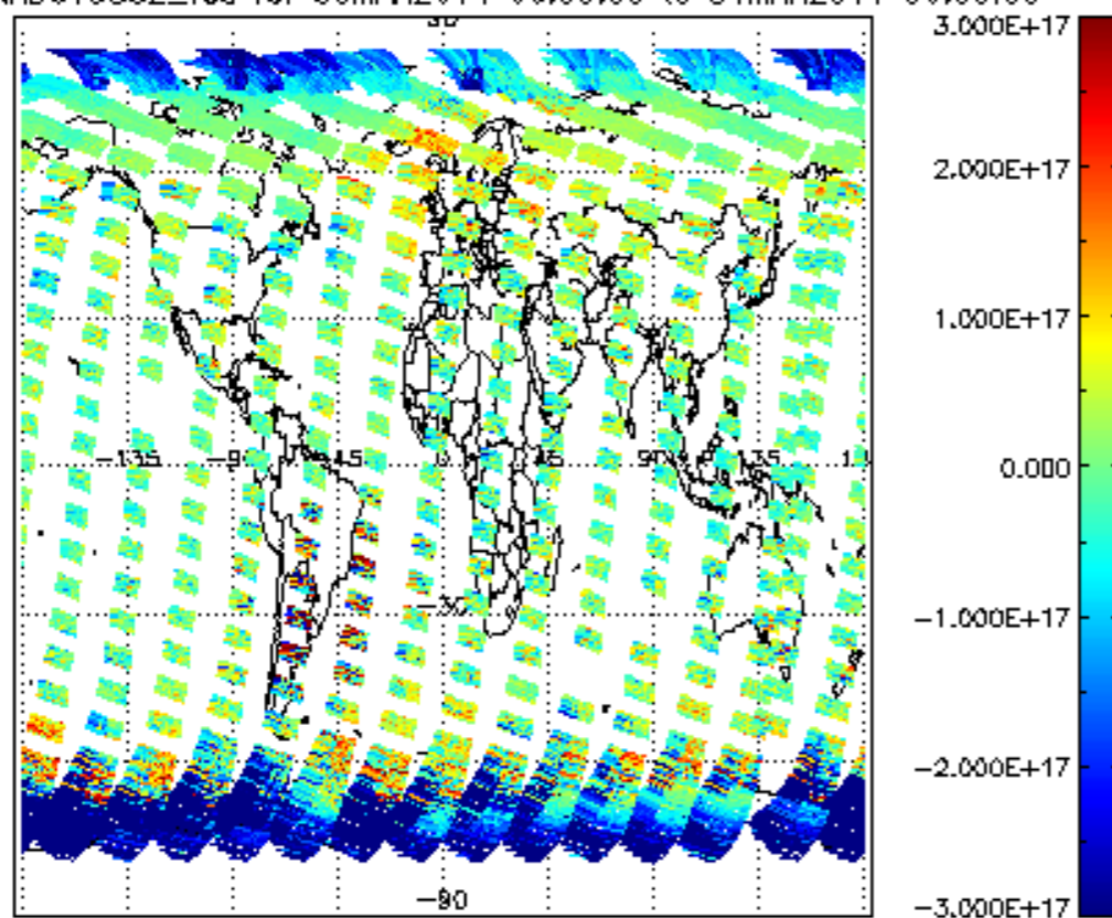
SCIOL2P_NADUV5S02_vcd for 30MAR2011 00:00:00 to 31MAR2011 00:00:00
