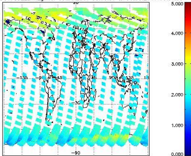
SCIOL2P_NADUV7S02_amf_gr for 30MAR2011 00:00:00 to 31MAR2011 00:00:00
