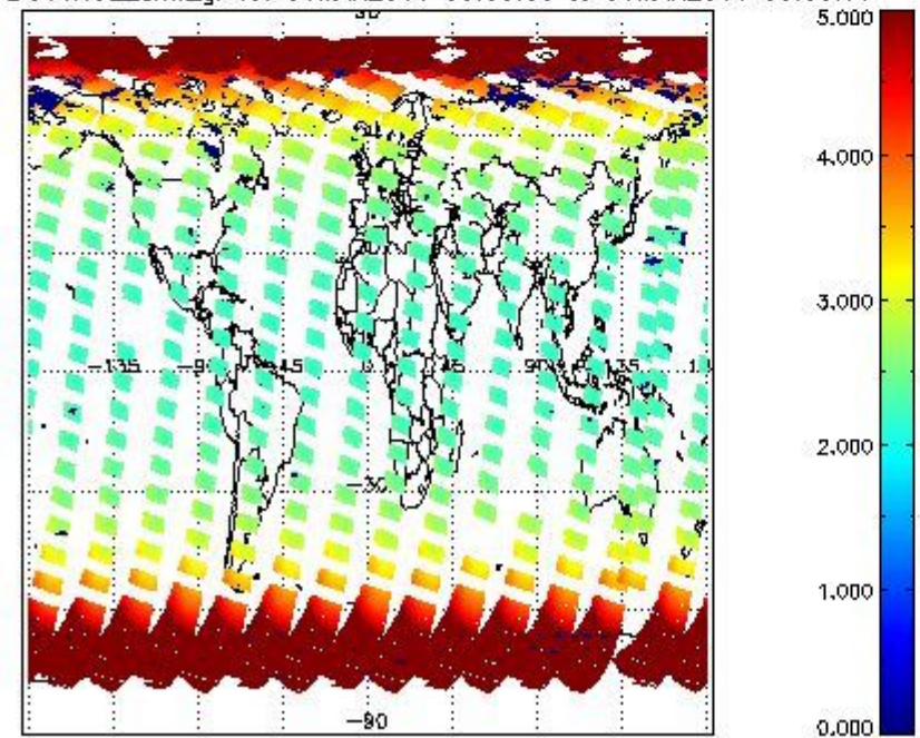
SCIOL2P_NADUV1NO2_amf_gr for 30MAR2011 00:00:00 to 31MAR2011 00:00:00
