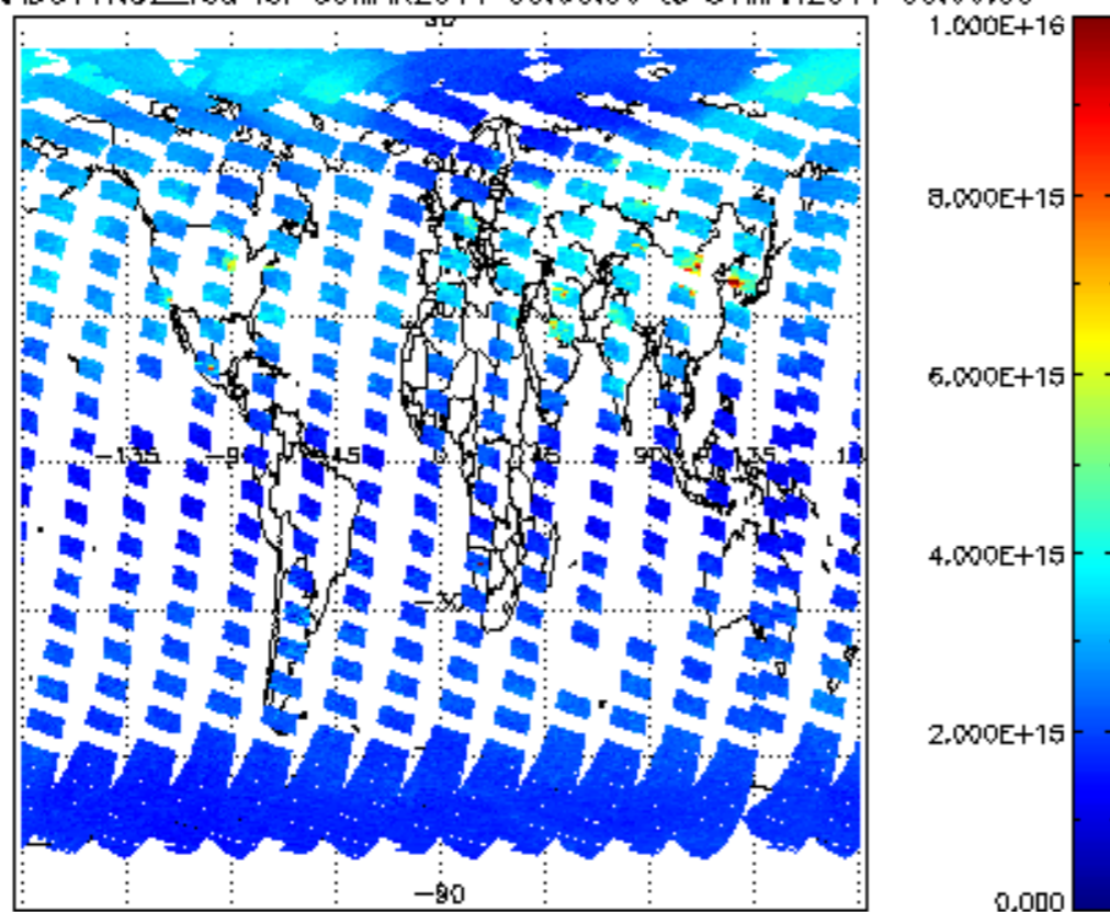
SCIOL2P_NADUV1NO2_vcd for 30MAR2011 00:00:00 to 31MAR2011 00:00:00
