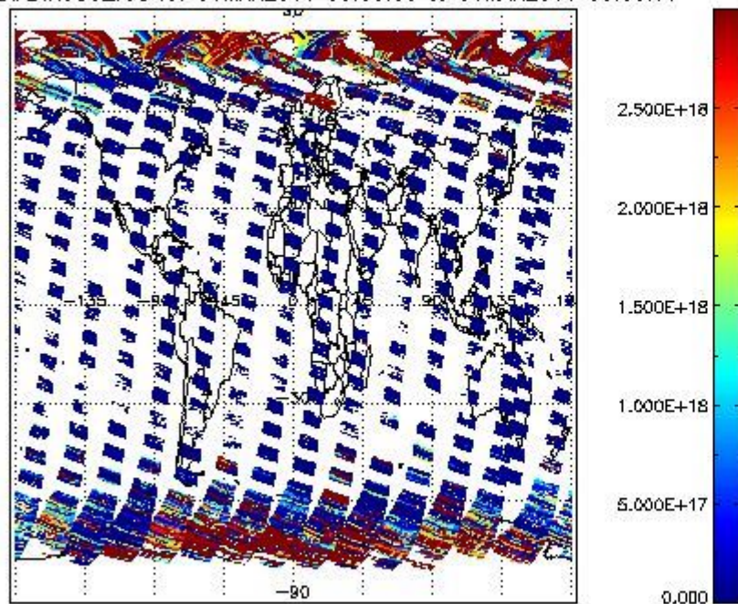
SCIOL2P_NADIR3CO_vcd for 30MAR2011 00:00:00 to 31MAR2011 00:00:00
