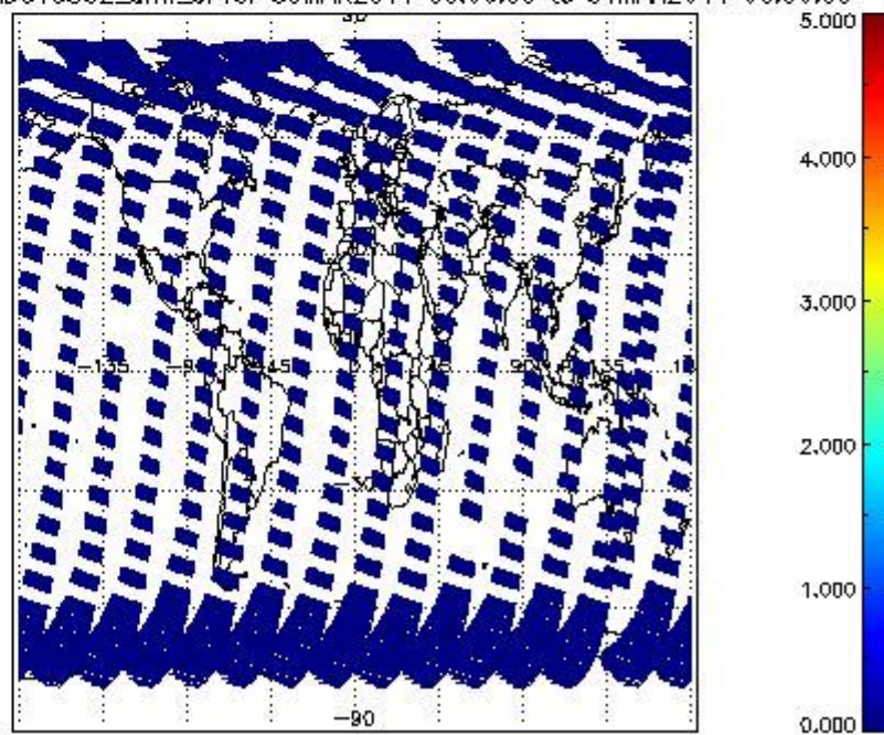
SCIOL2P_NADUV5SO2_amf_cl for 30MAR2011 00:00:00 to 31MAR2011 00:00:00
