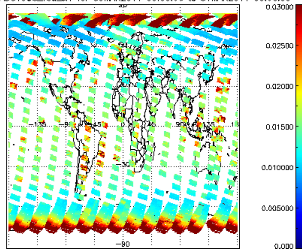
SCIOL2P_NADUV003_vcd_err for 30MAR2011 00:00:00 to 31MAR2011 00:00:00
