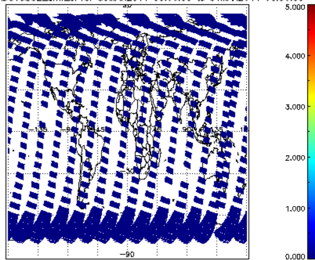
SCIOL2P_NADUV5S02_amf_cl for 30MAR2011 00:00:00 to 31MAR2011 00:00:00
