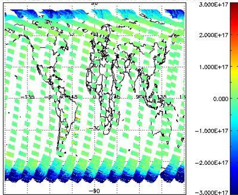
SCIOL2P_NADUV7S02_vcd for 30MAR2011 00:00:00 to 31MAR2011 00:00:00
