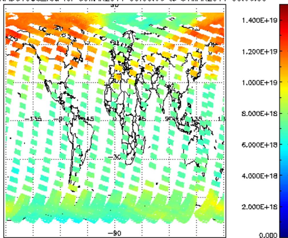
SCIOL2P_NADUV003_vcd for 30MAR2011 00:00:00 to 31MAR2011 00:00:00
