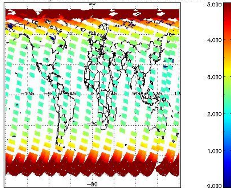
SCIOL2P_NADUV003_amf_gr for 30MAR2011 00:00:00 to 31MAR2011 00:00:00
