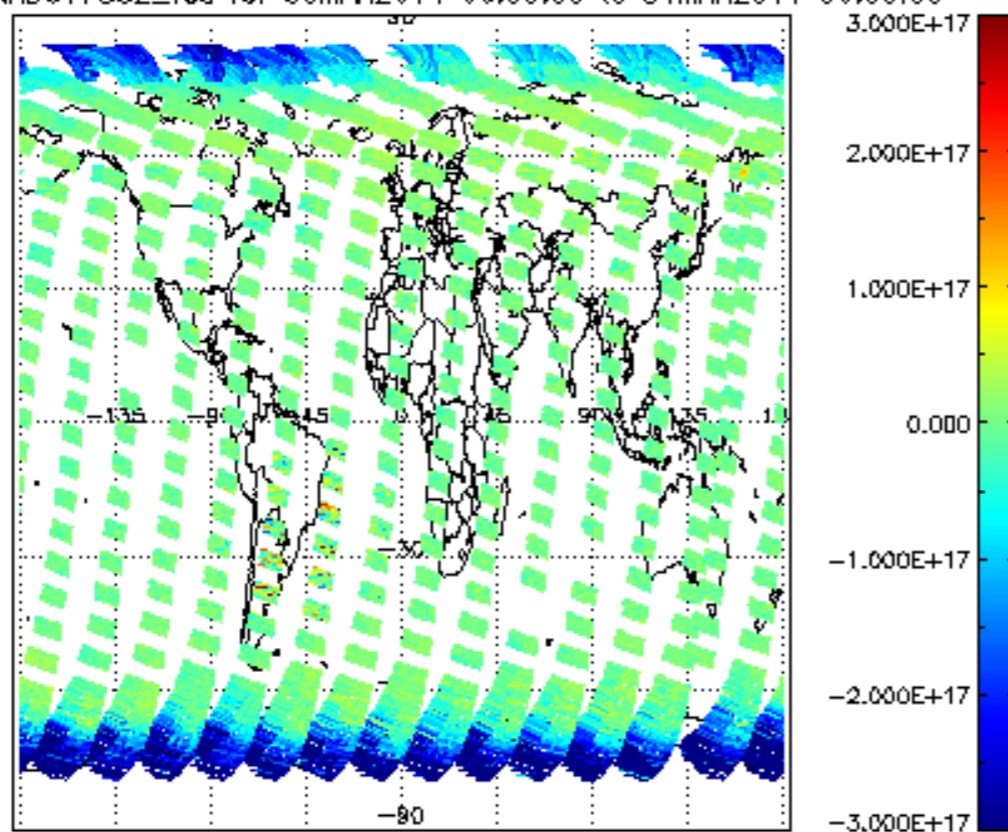
SCIOL2P_NADUV7S02_vcd for 30MAR2011 00:00:00 to 31MAR2011 00:00:00
