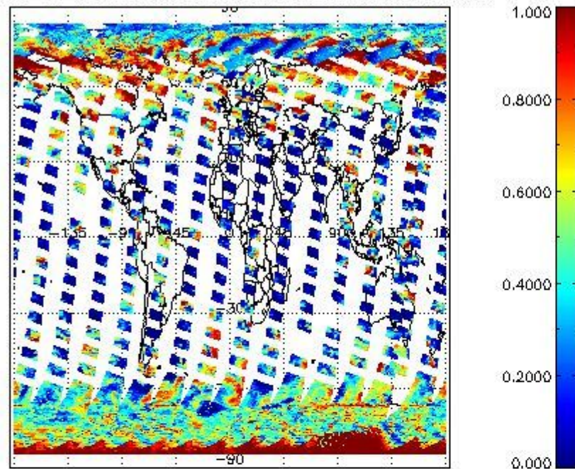
cL_frac for 30MAR2011 00:00:00 to 31MAR2011 00:00:00
