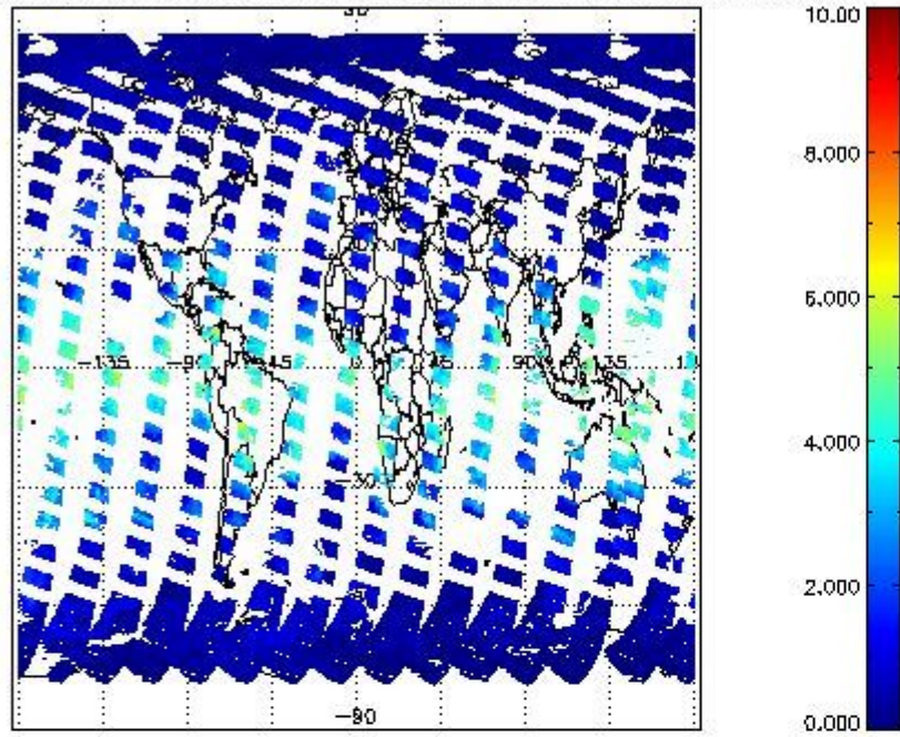
SCIOL2P_NADUV8H2O_vcd for 30MAR2011 00:00:00 to 31MAR2011 00:00:00
