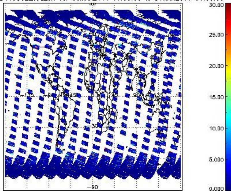
SCIOL2P_NADUV5SO2_vcd_err for 30MAR2011 00:00:00 to 31MAR2011 00:00:00
