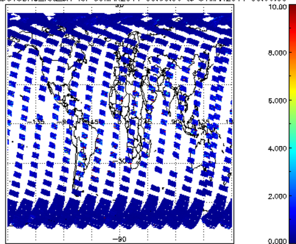
SCIOL2P_NADUV3BRO_vcd_err for 30MAR2011 00:00:00 to 31MAR2011 00:00:00
