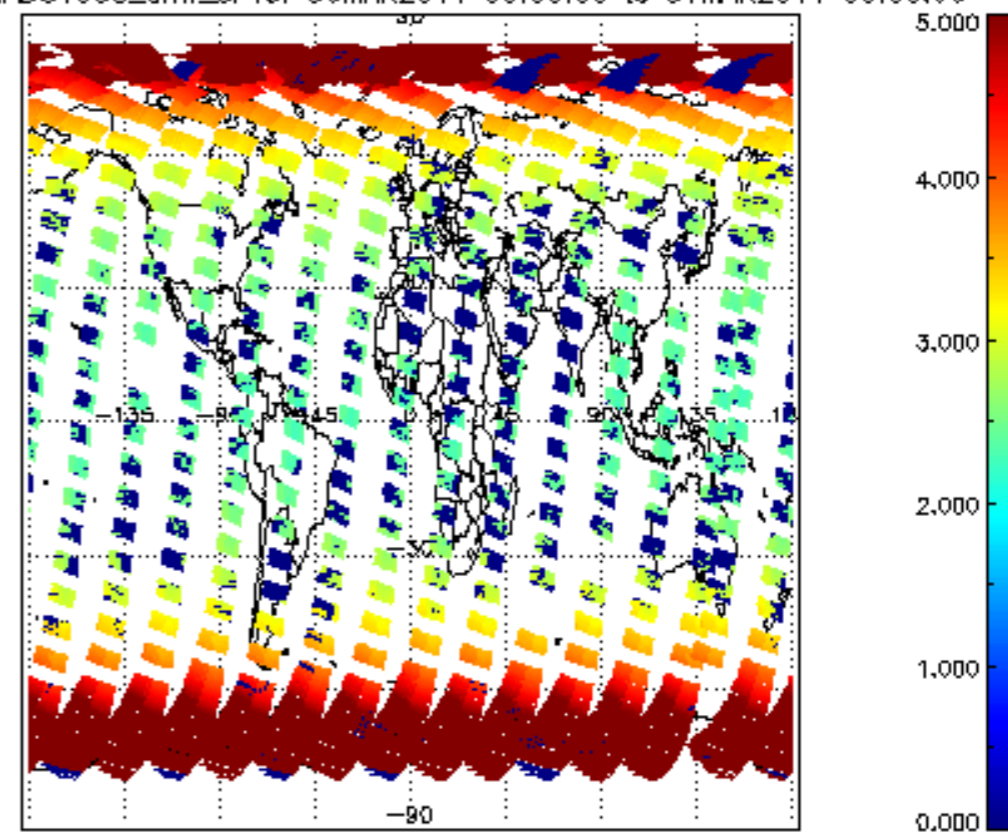
SCIOL2P_NADUV003_amf_cl for 30MAR2011 00:00:00 to 31MAR2011 00:00:00
