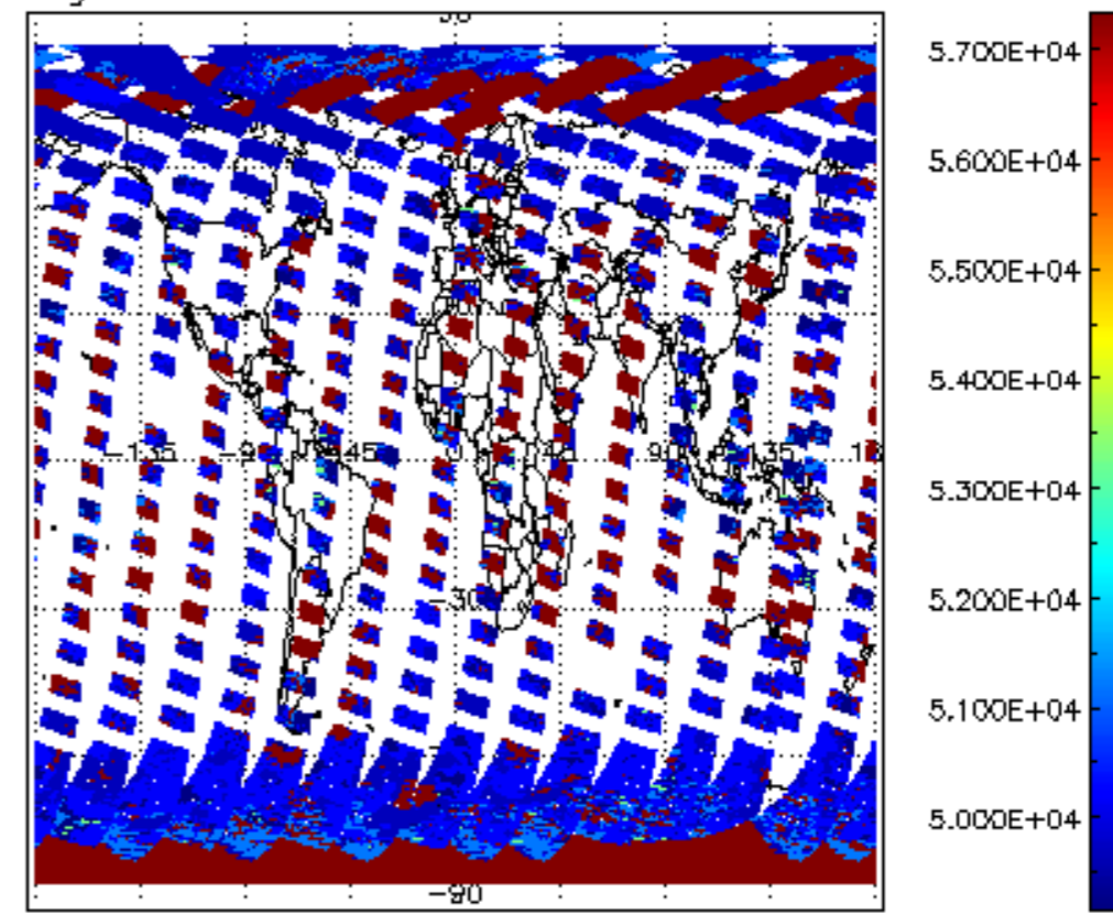
cloud_flags for 30MAR2011 00:00:00 to 31MAR2011 00:00:00
