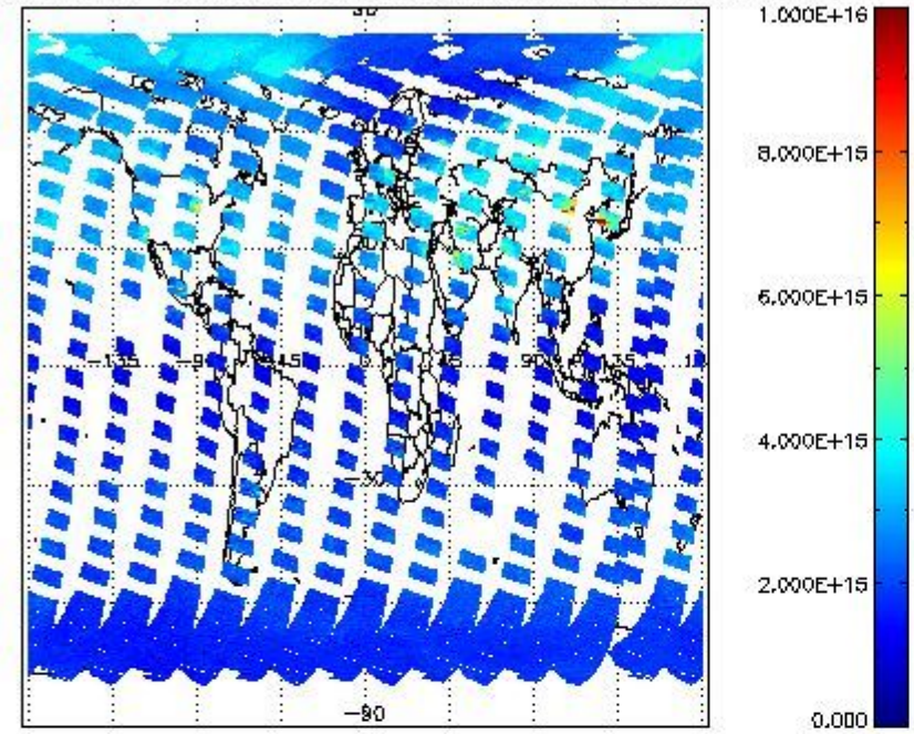
SCIOL2P_NADUV1NO2_vcd for 30MAR2011 00:00:00 to 31MAR2011 00:00:00
