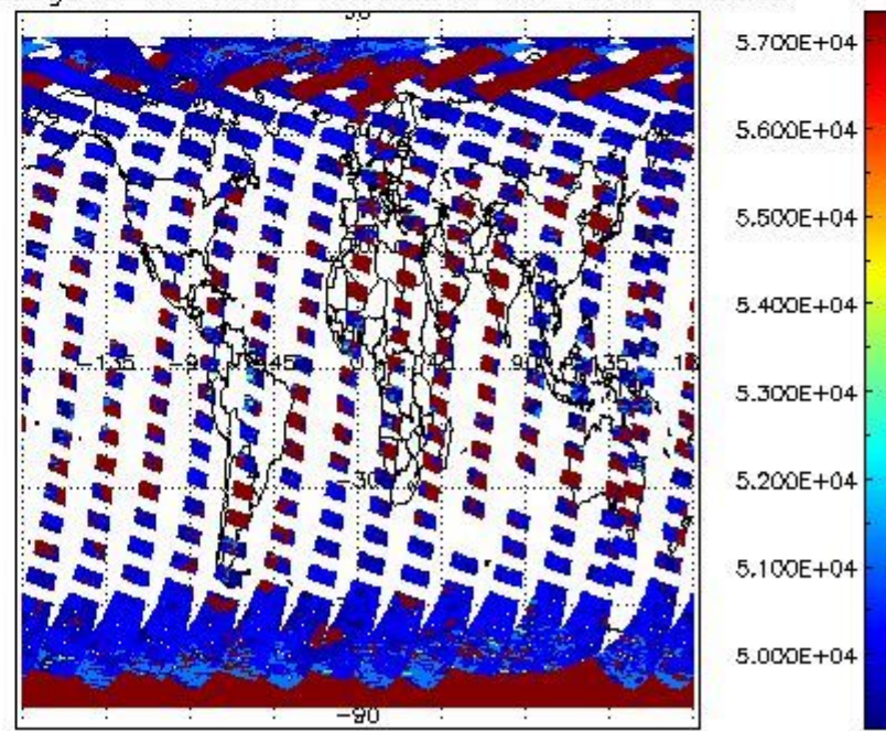
cloud_flags for 30MAR2011 00:00:00 to 31MAR2011 00:00:00
