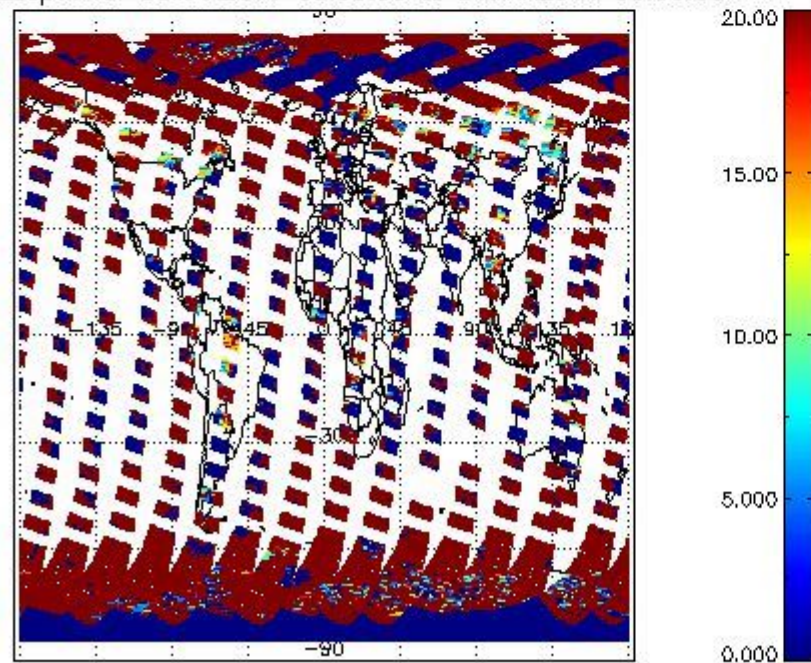
cL_opt_depth for 30MAR2011 00:00:00 to 31MAR2011 00:00:00
