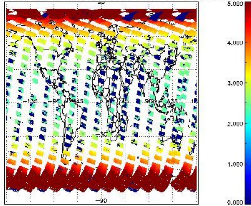
SCIOL2P_NADUV3BRO_amf_cl for 30MAR2011 00:00:00 to 31MAR2011 00:00:00
