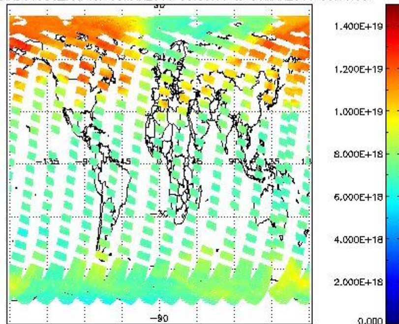
SCIOL2P_NADUV003_vcd for 30MAR2011 00:00:00 to 31MAR2011 00:00:00
