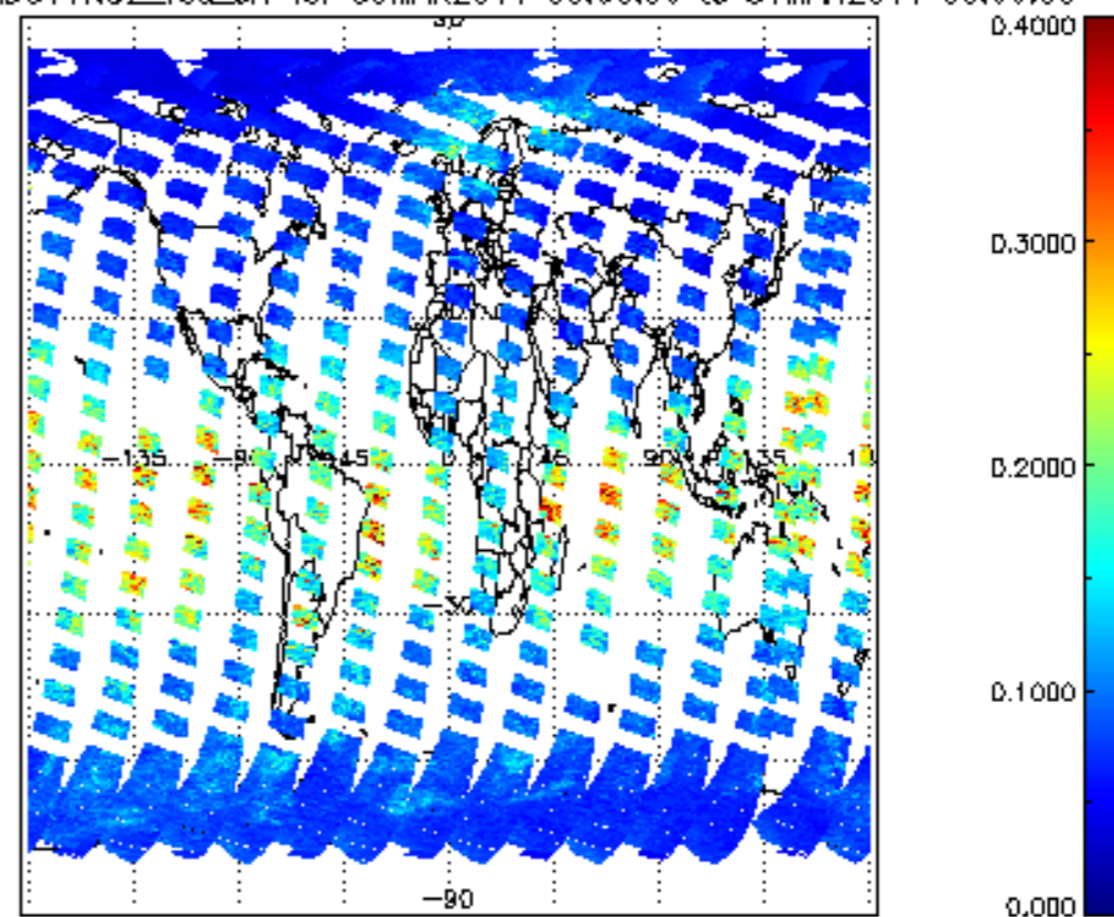
SCIOL2P_NADUV1NO2_vcd_err for 30MAR2011 00:00:00 to 31MAR2011 00:00:00
