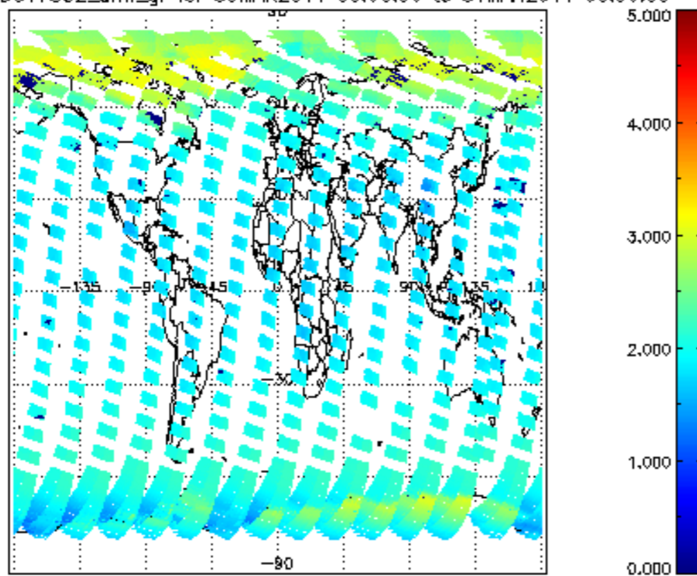
SCIOL2P_NADUV7S02_amf_gr for 30MAR2011 00:00:00 to 31MAR2011 00:00:00
