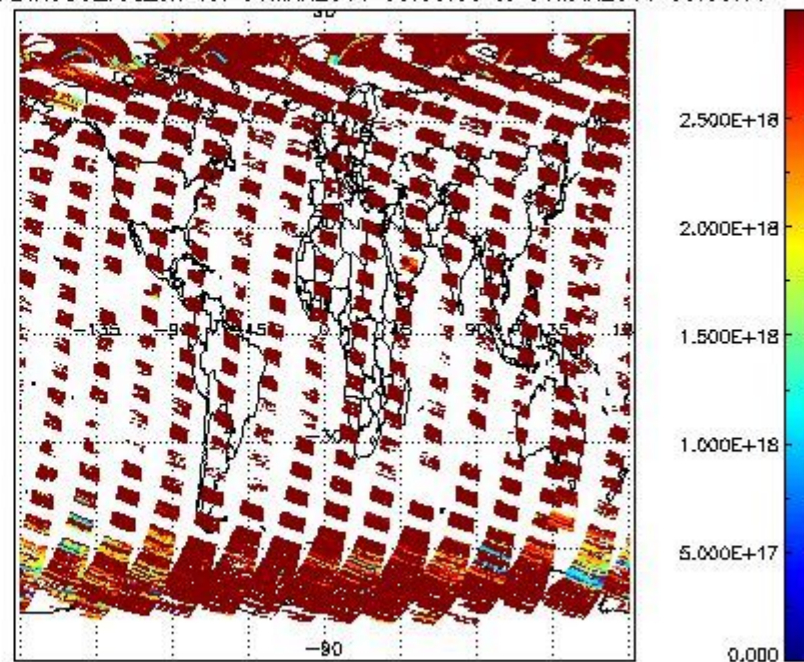
SCIOL2P_NADIR3CO_vcd_err for 30MAR2011 00:00:00 to 31MAR2011 00:00:00
