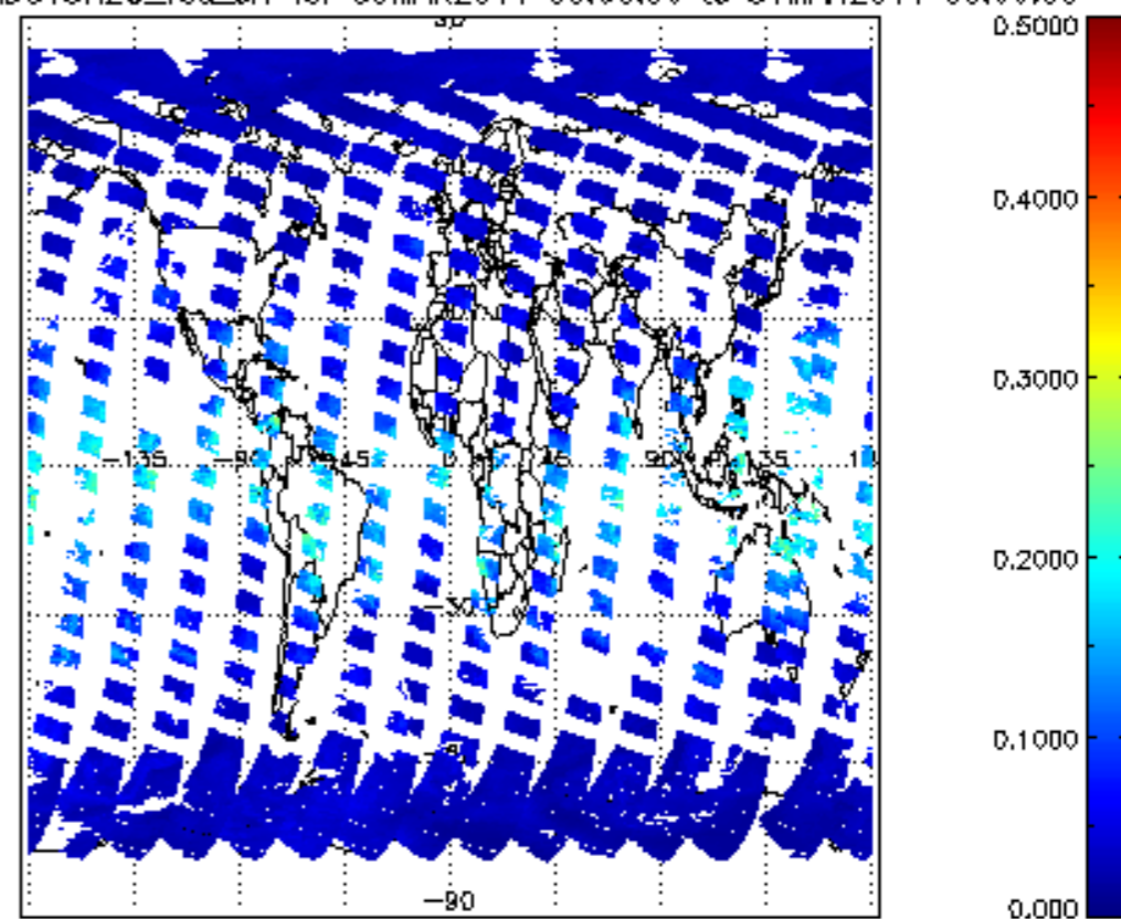
SCIOL2P_NADUV8H2O_vcd_err for 30MAR2011 00:00:00 to 31MAR2011 00:00:00
