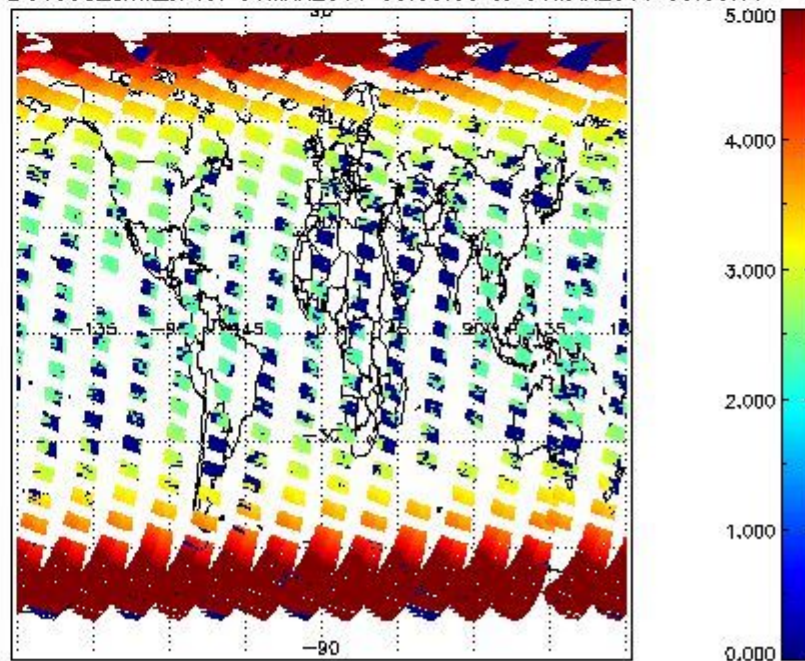
SCIOL2P_NADUV003_amf_cl for 30MAR2011 00:00:00 to 31MAR2011 00:00:00
