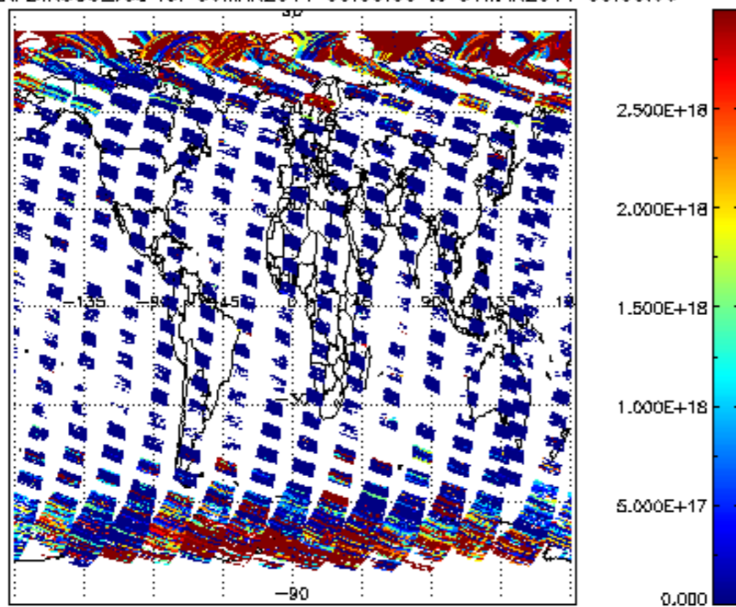
SCIOL2P_NADIR3CO_vcd for 30MAR2011 00:00:00 to 31MAR2011 00:00:00
