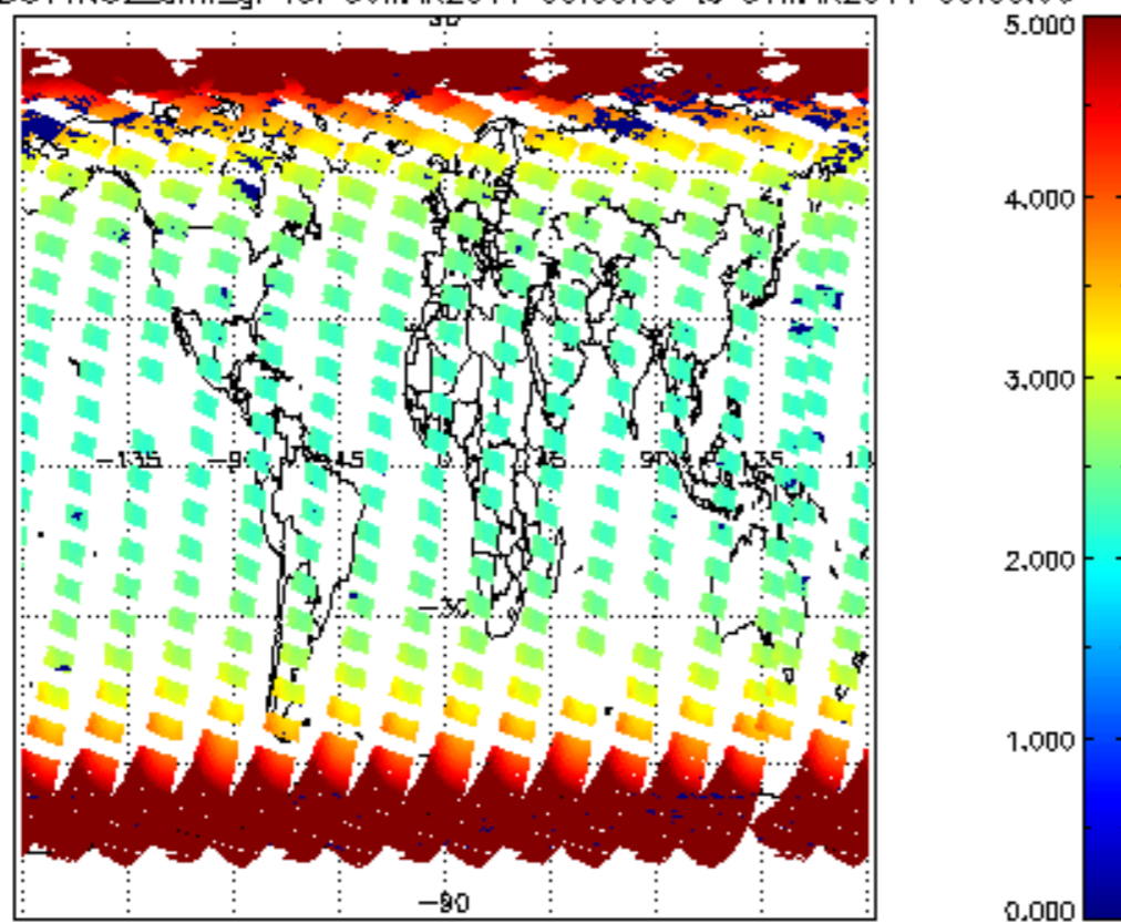
SCIOL2P_NADUV1NO2_amf_gr for 30MAR2011 00:00:00 to 31MAR2011 00:00:00
