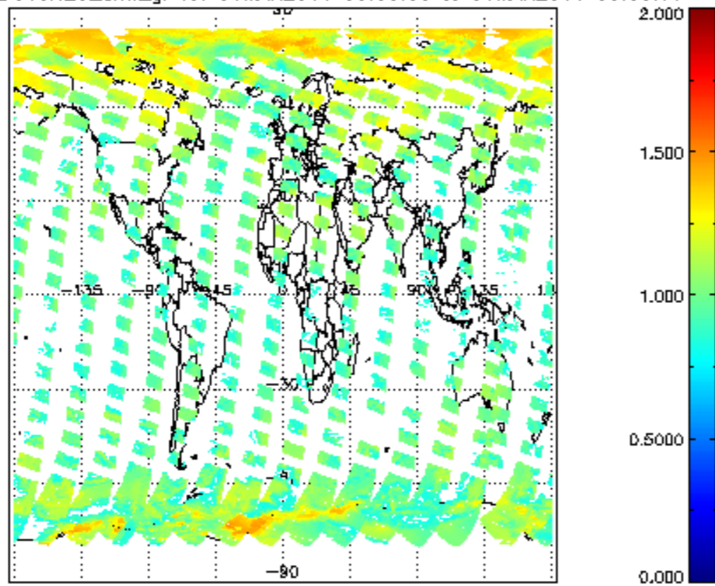
SCIOL2P_NADUV8H2O_arnf_gr for 30MAR2011 00:00:00 to 31MAR2011 00:00:00
