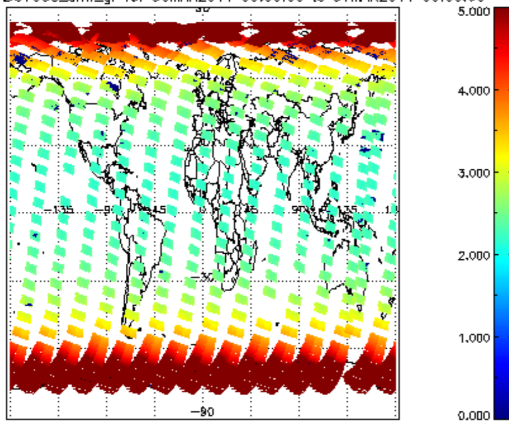
SCIOL2P_NADUV003_amf_gr for 30MAR2011 00:00:00 to 31MAR2011 00:00:00
