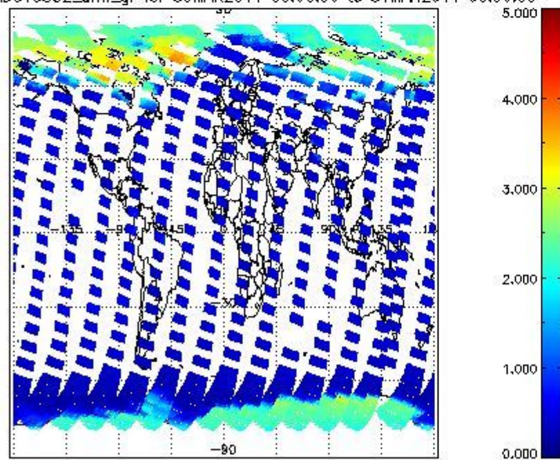
SCIOL2P_NADUV5SO2_amf_gr for 30MAR2011 00:00:00 to 31MAR2011 00:00:00
