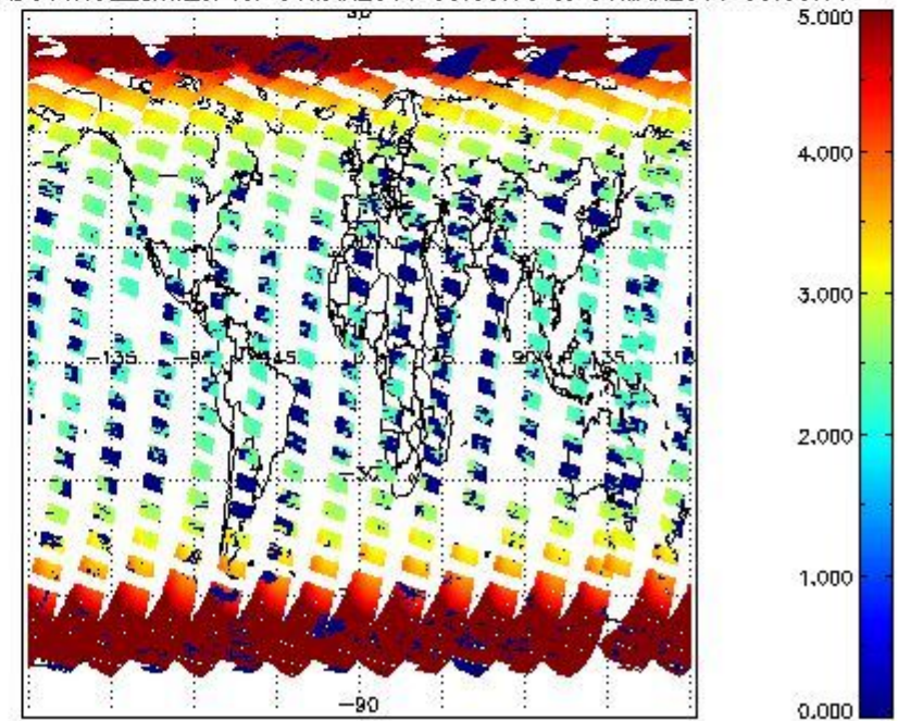
SCIOL2P_NADUV1NO2_amf_cl for 30MAR2011 00:00:00 to 31MAR2011 00:00:00
