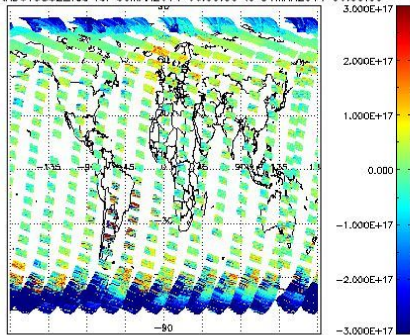
SCIOL2P_NADUV5SO2_vcd for 30MAR2011 00:00:00 to 31MAR2011 00:00:00
