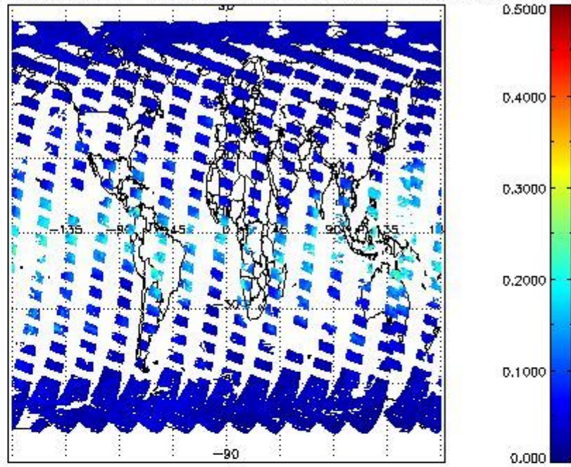
SCIOL2P_NADUV8H2O_vcd_err for 30MAR2011 00:00:00 to 31MAR2011 00:00:00
