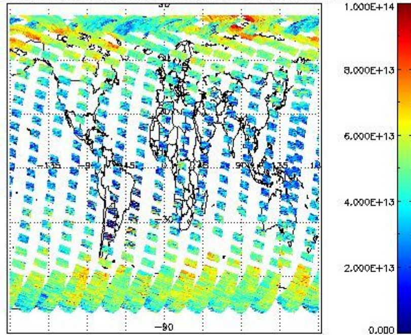
SCIOL2P_NADUV3BRO_vcd for 30MAR2011 00:00:00 to 31MAR2011 00:00:00
