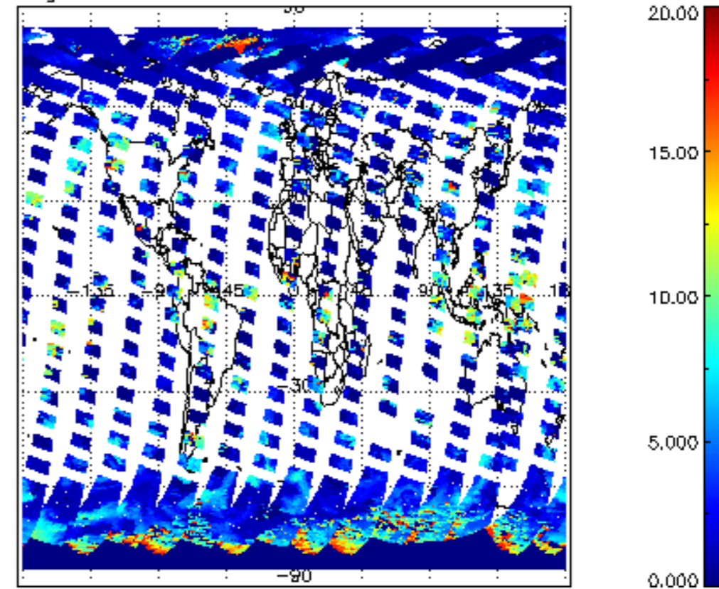
cL_top_height for 30MAR2011 00:00:00 to 31MAR2011 00:00:00
