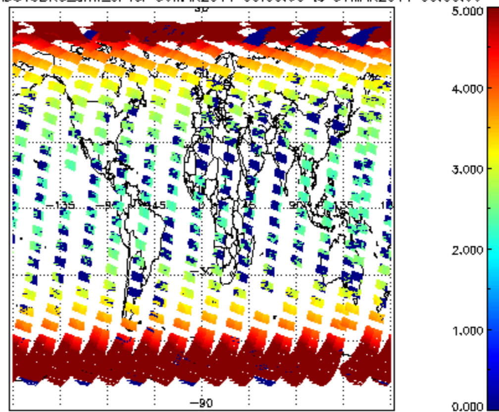
SCIOL2P_NADUV3BRO_amf_cl for 30MAR2011 00:00:00 to 31MAR2011 00:00:00
