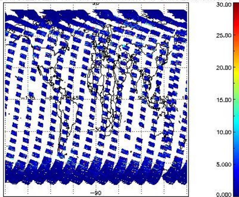
SCIOL2P_NADUV7S02_vcd_err for 30MAR2011 00:00:00 to 31MAR2011 00:00:00
