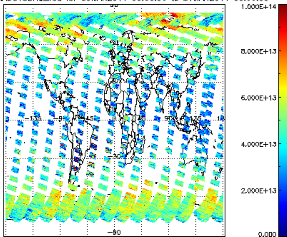
SCIOL2P_NADUV3BRO_vcd for 30MAR2011 00:00:00 to 31MAR2011 00:00:00
