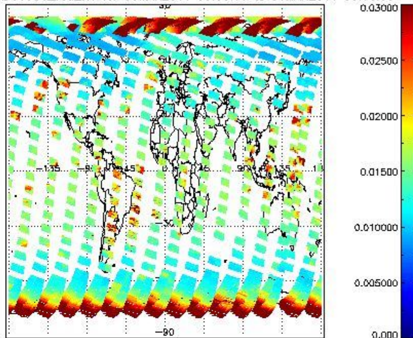
SCIOL2P_NADUV003_vcd_err for 30MAR2011 00:00:00 to 31MAR2011 00:00:00
