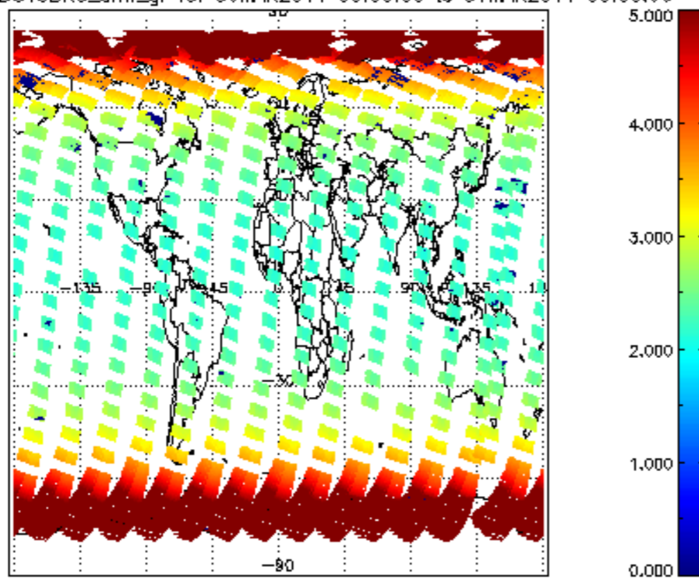
SCIOL2P_NADUV3BRO_amf_gr for 30MAR2011 00:00:00 to 31MAR2011 00:00:00
