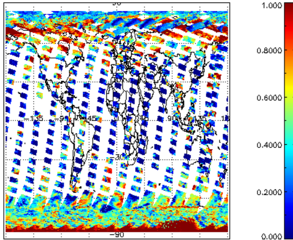
cL_frac for 30MAR2011 00:00:00 to 31MAR2011 00:00:00
