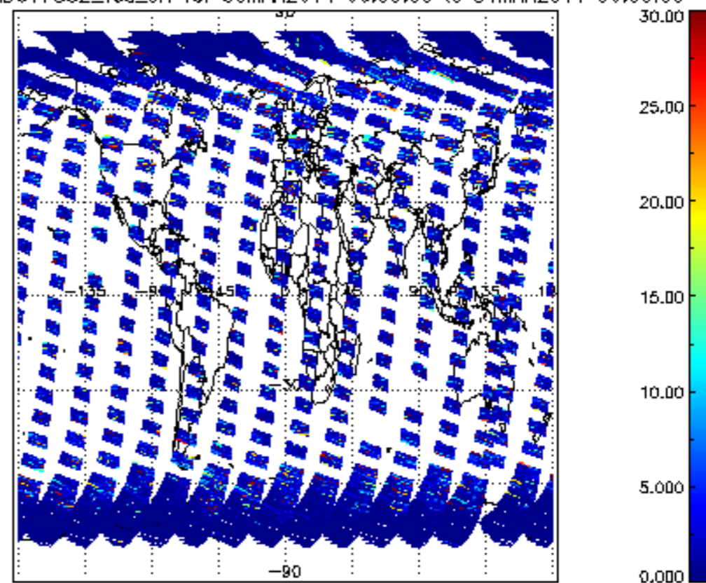
SCIOL2P_NADUV7S02_vcd_err for 30MAR2011 00:00:00 to 31MAR2011 00:00:00
