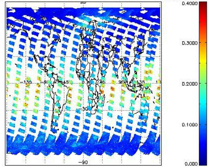
SCIOL2P_NADUV1NO2_vcd_err for 30MAR2011 00:00:00 to 31MAR2011 00:00:00
