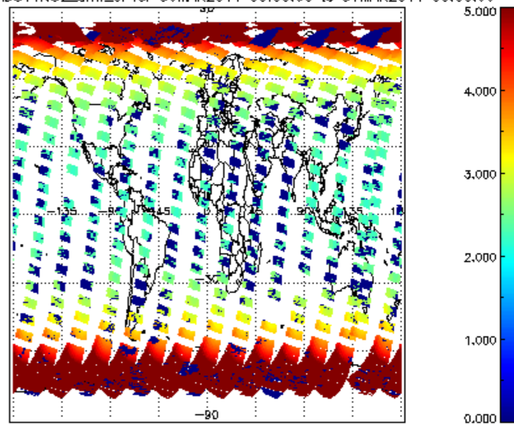
SCIOL2P_NADUV1NO2_amf_cl for 30MAR2011 00:00:00 to 31MAR2011 00:00:00
