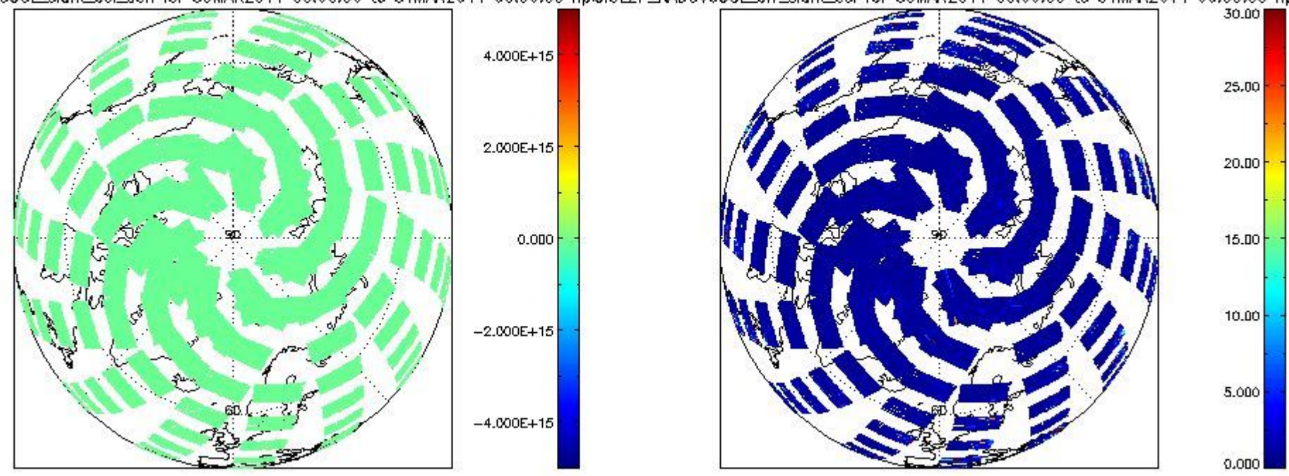
CIOL2P_NADUV6OCL_slant_col_den for 30MAR2011 00:00:00 to 31MAR2011 00:00:00 npCIOL2P_NADUV6OCL_err_slant_col for 30MAR2011 00:00:00 to 31MAR2011 00:00:00 np
