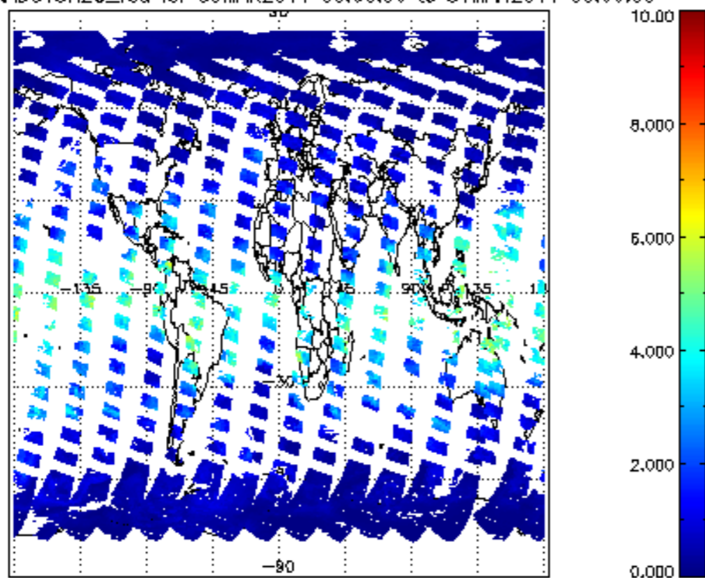
SCIOL2P_NADUV8H2O_vcd for 30MAR2011 00:00:00 to 31MAR2011 00:00:00
