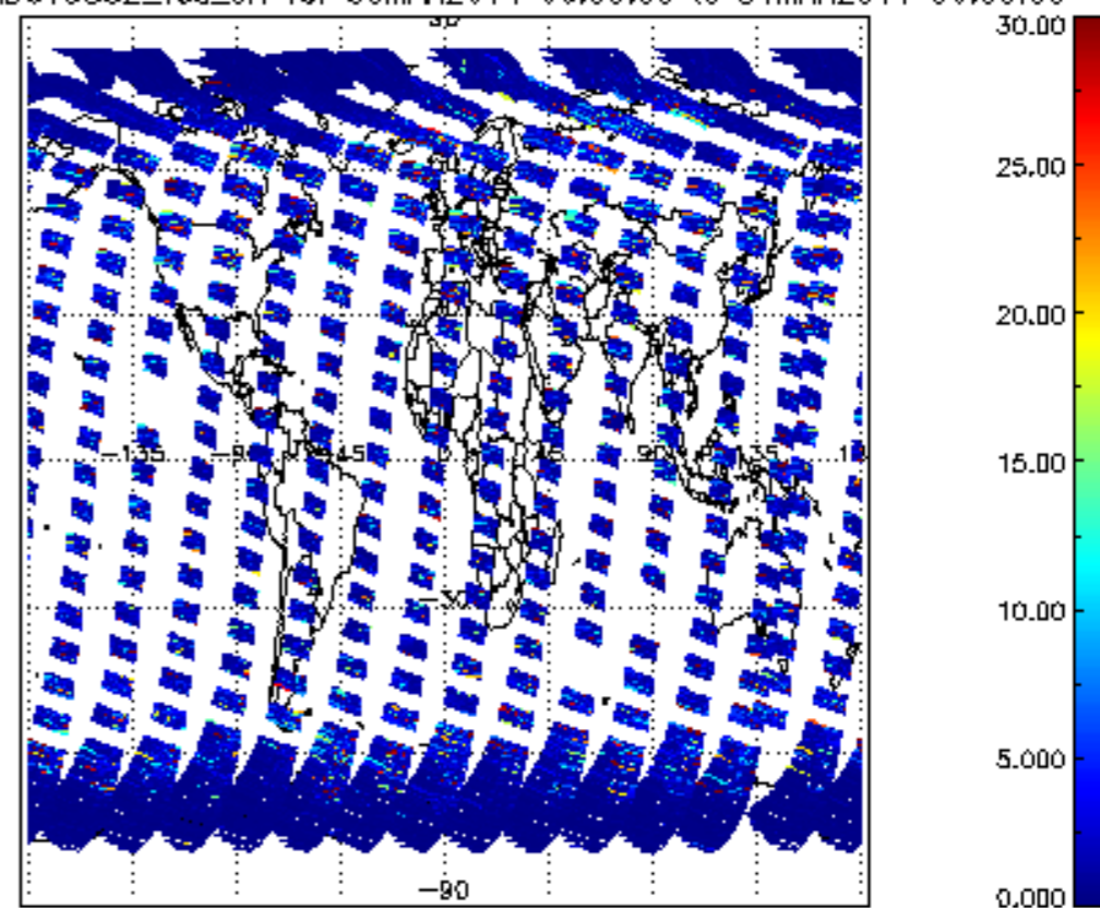
SCIOL2P_NADUV5S02_vcd_err for 30MAR2011 00:00:00 to 31MAR2011 00:00:00
