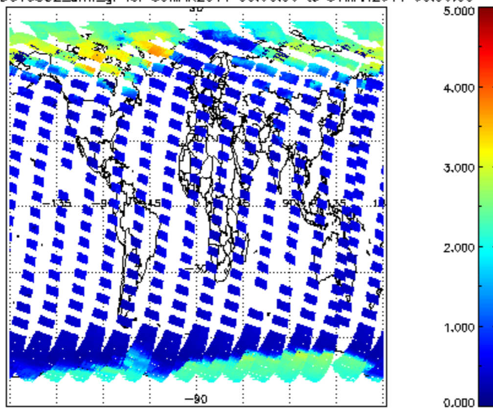
SCIOL2P_NADUV5S02_amf_gr for 30MAR2011 00:00:00 to 31MAR2011 00:00:00
