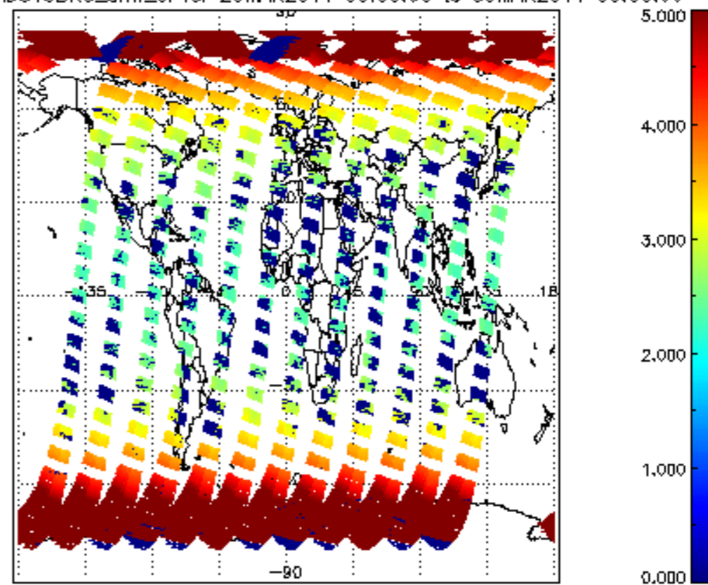
SCIOL2P_NADUV3BRO_arnf_cl for 29MAR2011 00:00:00 to 30MAR2011 00:00:00
