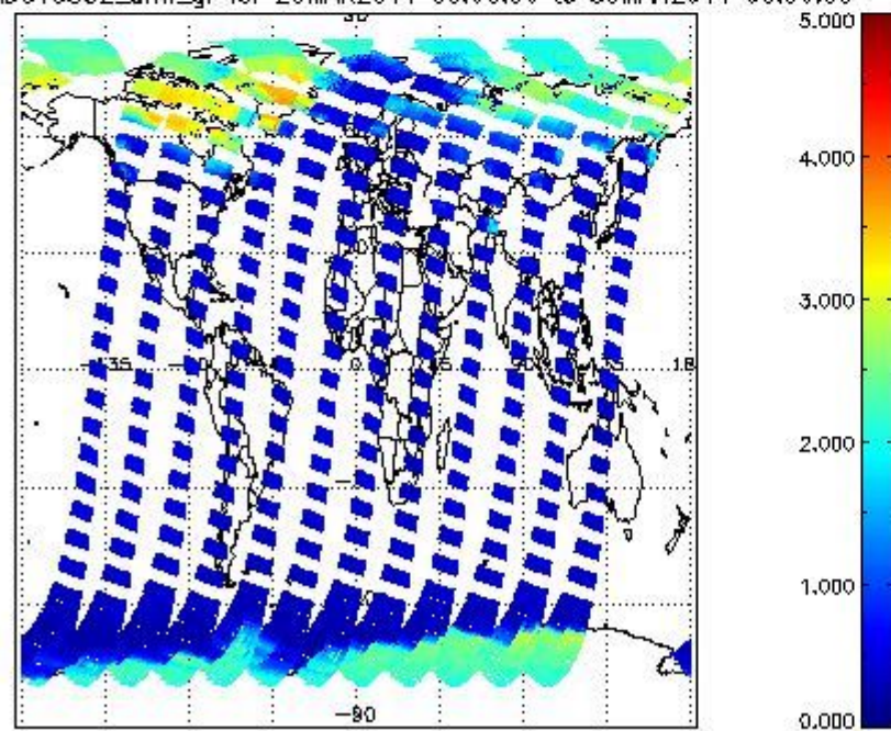
SCIOL2P_NADUV5S02_amf_gr for 29MAR2011 00:00:00 to 30MAR2011 00:00:00
