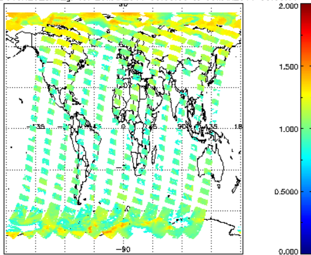
SCIOL2P_NADUV8H20_arnf_gr for 29MAR2011 00:00:00 to 30MAR2011 00:00:00
