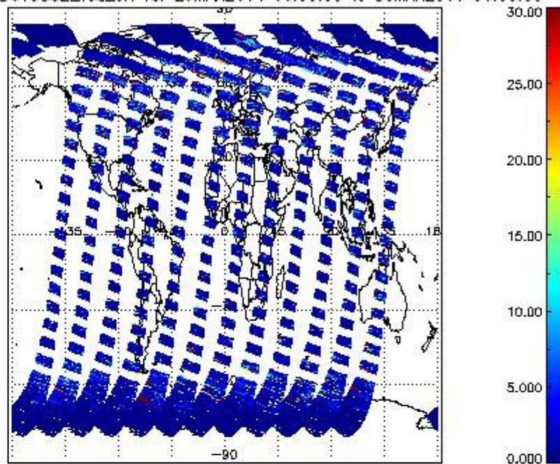
SCIOL2P_NADUV5S02_vcd_err for 29MAR2011 00:00:00 to 30MAR2011 00:00:00
