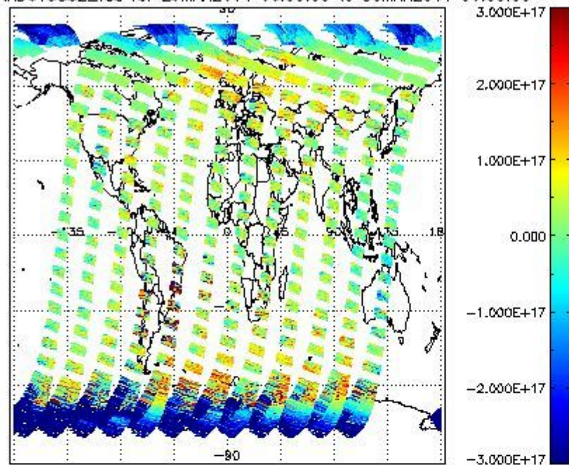
SCIOL2P_NADUV5S02_vcd for 29MAR2011 00:00:00 to 30MAR2011 00:00:00
