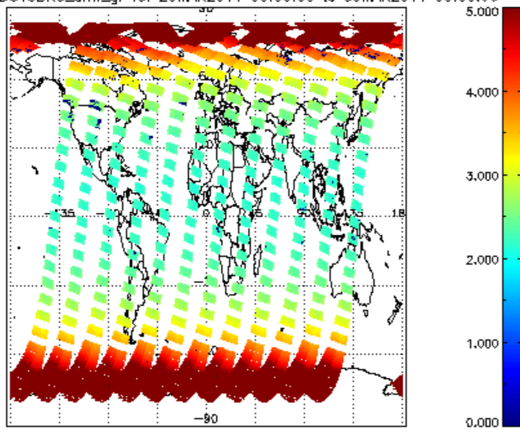
SCIOL2P_NADUV3BRO_arnf_gr for 29MAR2011 00:00:00 to 30MAR2011 00:00:00
