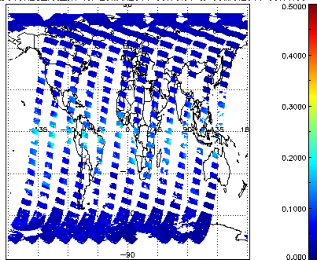
SCIOL2P_NADUV8H20_vcd_err for 29MAR2011 00:00:00 to 30MAR2011 00:00:00
