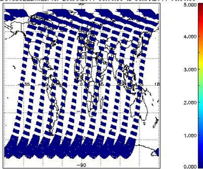
SCIOL2P_NADUV5S02_amf_cl for 29MAR2011 00:00:00 to 30MAR2011 00:00:00
