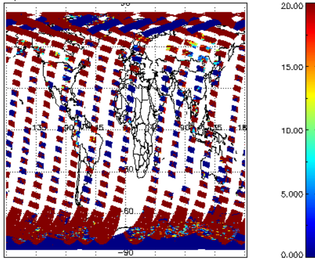
cL_opt_depth for 28MAR2011 00:00:00 to 29MAR2011 00:00:00
