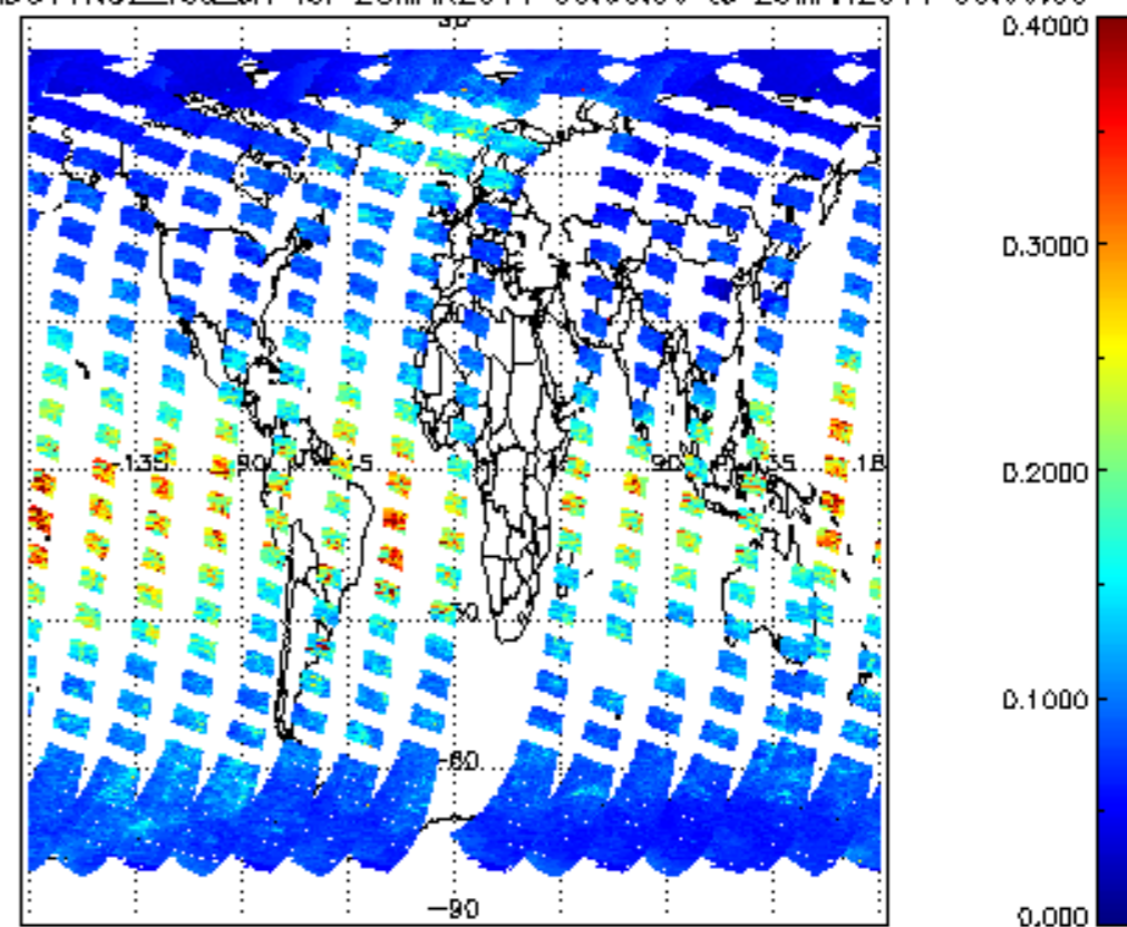
SCIOL2P_NADUV1NO2_vcd_Lerr for 28MAR2011 00:00:00 to 29MAR2011 00:00:00
