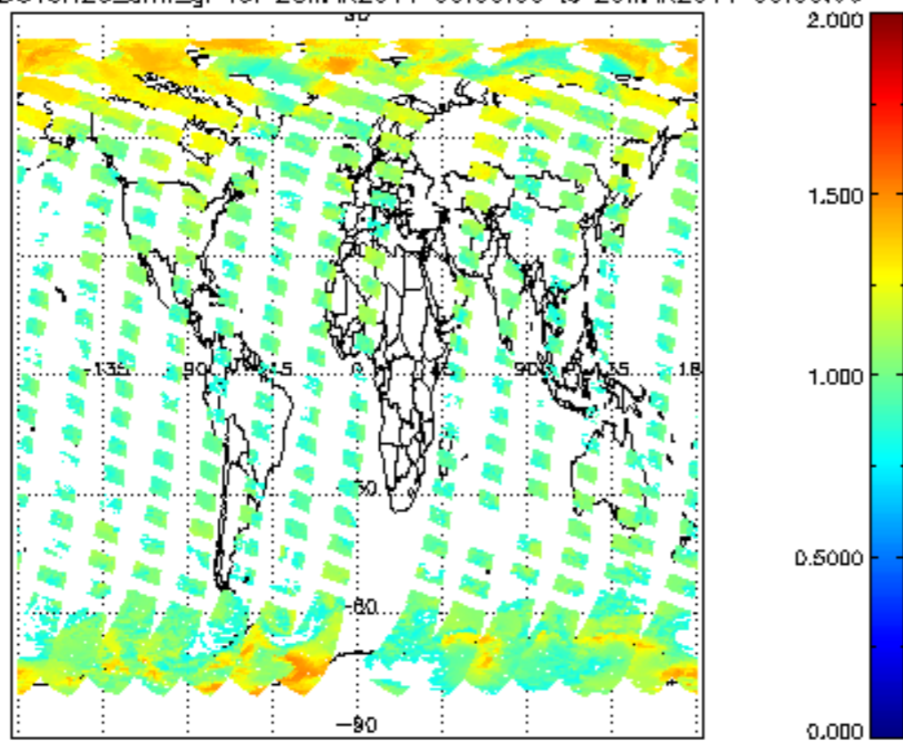
SCIOL2P_NADUV8H20_arnf_gr for 28MAR2011 00:00:00 to 29MAR2011 00:00:00
