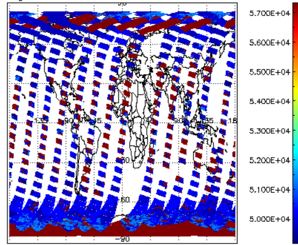
cloud_flags for 28MAR2011 00:00:00 to 29MAR2011 00:00:00
