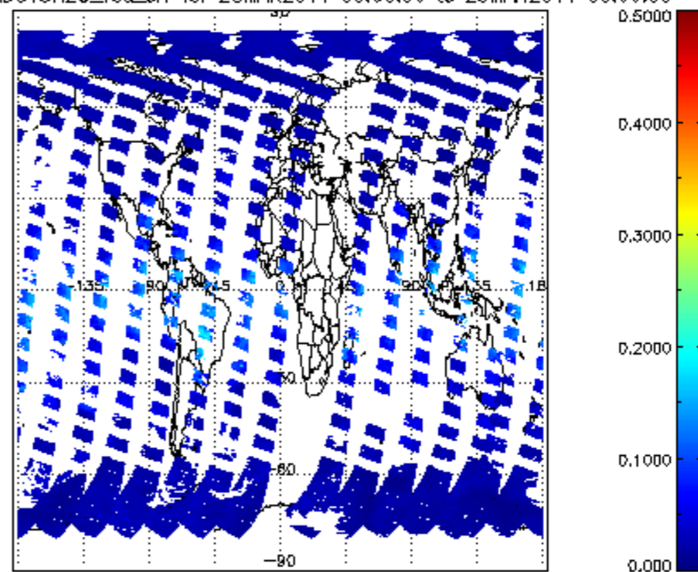
SCIOL2P_NADUV8H20_vcd_err for 28MAR2011 00:00:00 to 29MAR2011 00:00:00
