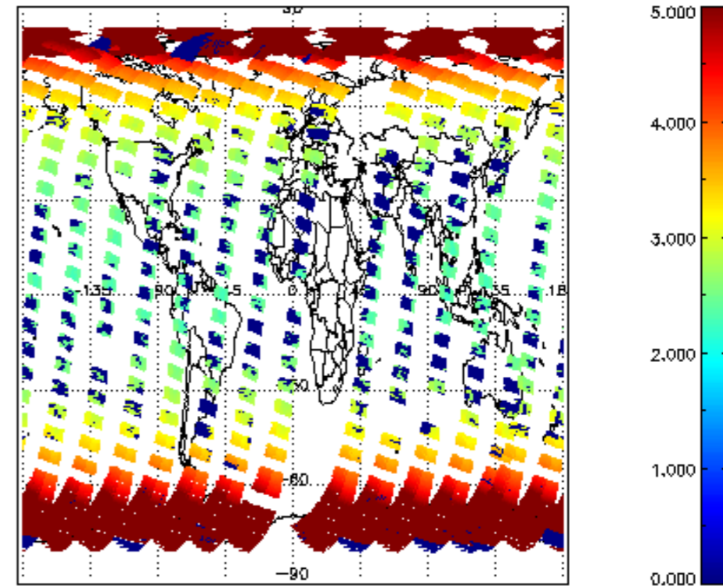
SCIOL2P_NADUV003_arnf_cl for 28MAR2011 00:00:00 to 29MAR2011 00:00:00
