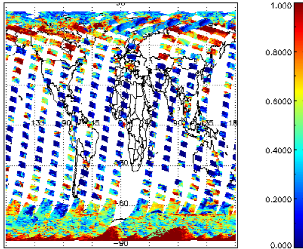
cL_frac for 28MAR2011 00:00:00 to 29MAR2011 00:00:00
