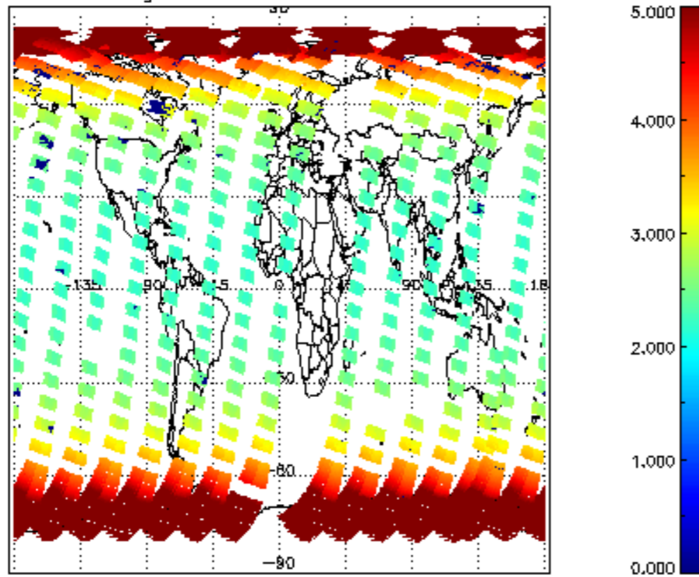
SCIOL2P_NADUV003_arnf_gr for 28MAR2011 00:00:00 to 29MAR2011 00:00:00
