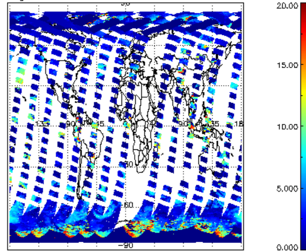
cL_top_height for 28MAR2011 00:00:00 to 29MAR2011 00:00:00
