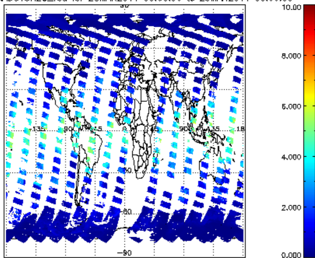
SCIOL2P_NADUV8H20_vcd for 28MAR2011 00:00:00 to 29MAR2011 00:00:00
