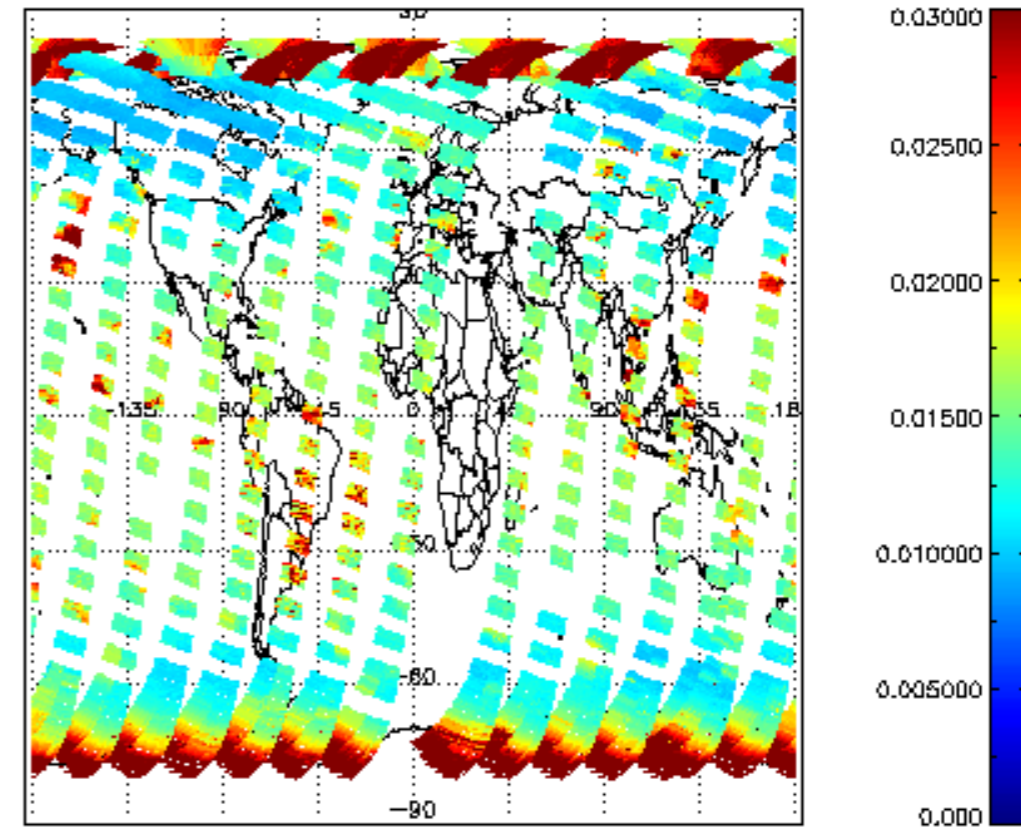
SCIOL2P_NADUV003_vcd_err for 28MAR2011 00:00:00 to 29MAR2011 00:00:00
