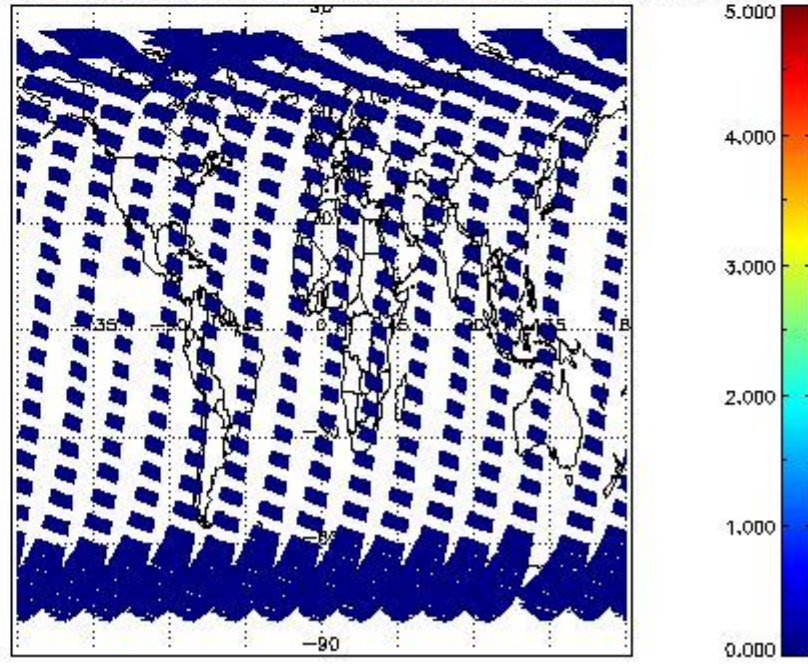
SCIOL2P_NADUV5SO2_amf_cl for 26MAR2011 00:00:00 to 27MAR2011 00:00:00
