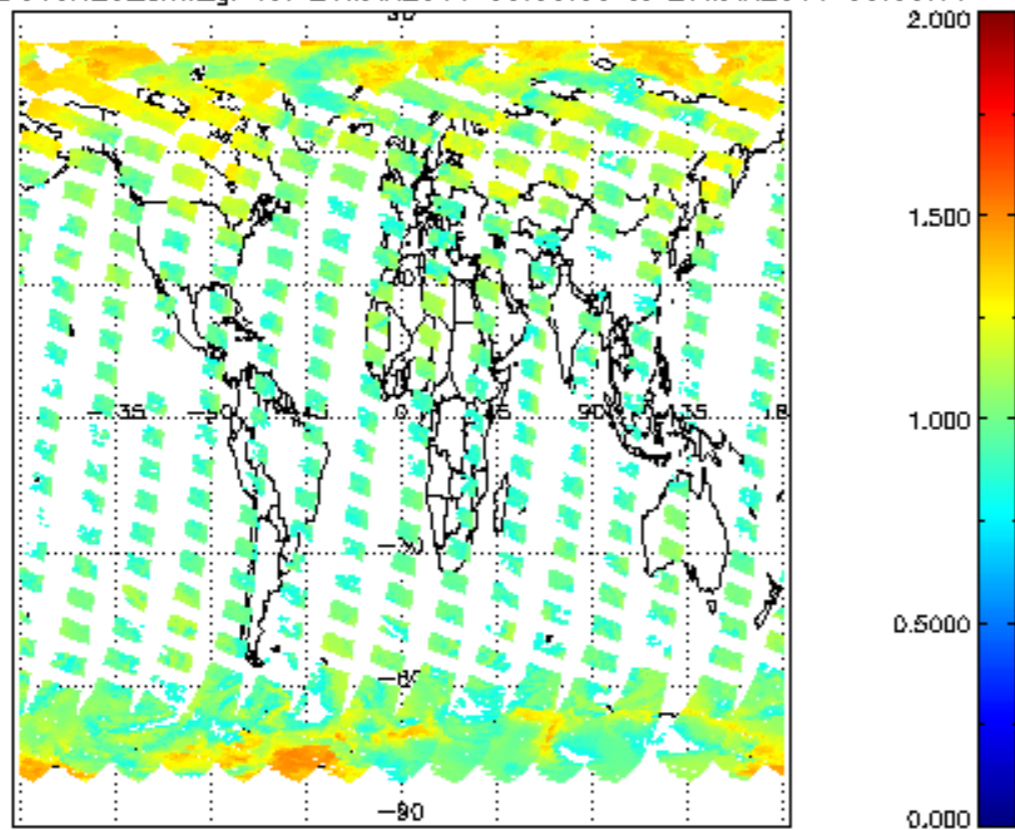
SCIOL2P_NADUV8H20_arnf_gr for 26MAR2011 00:00:00 to 27MAR2011 00:00:00
