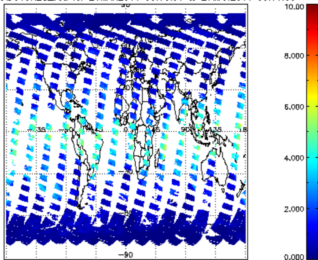
SCIOL2P_NADUV8H20_vcd for 26MAR2011 00:00:00 to 27MAR2011 00:00:00
