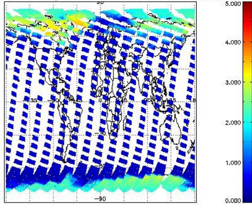
SCIOL2P_NADUV5SO2_amf_gr for 26MAR2011 00:00:00 to 27MAR2011 00:00:00
