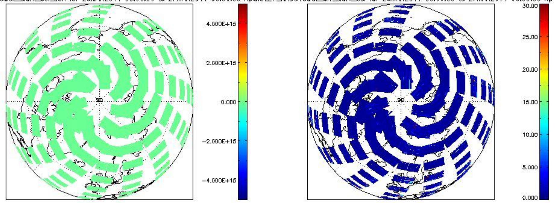
CIOL2P_NADUV6OCL_slant_col_den for 26MAR2011 00:00:00 to 27MAR2011 00:00:00 np CIOL2P_NADUV6OCL_err_slant_col for 26MAR2011 00:00:00 to 27MAR2011 00:00:00 np
