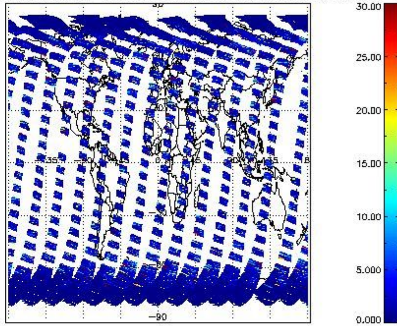
SCIOL2P_NADUV5SO2_vcd_err for 26MAR2011 00:00:00 to 27MAR2011 00:00:00
