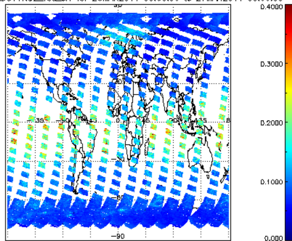
SCIOL2P_NADUV1NO2_vcd_err for 26MAR2011 00:00:00 to 27MAR2011 00:00:00
