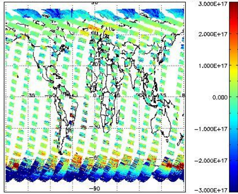
SCIOL2P_NADUV5SO2_vcd for 26MAR2011 00:00:00 to 27MAR2011 00:00:00
