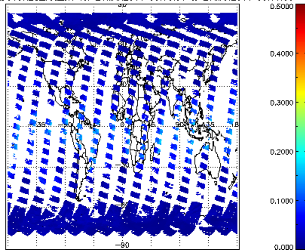
SCIOL2P_NADUV8H20_vcd_err for 26MAR2011 00:00:00 to 27MAR2011 00:00:00
