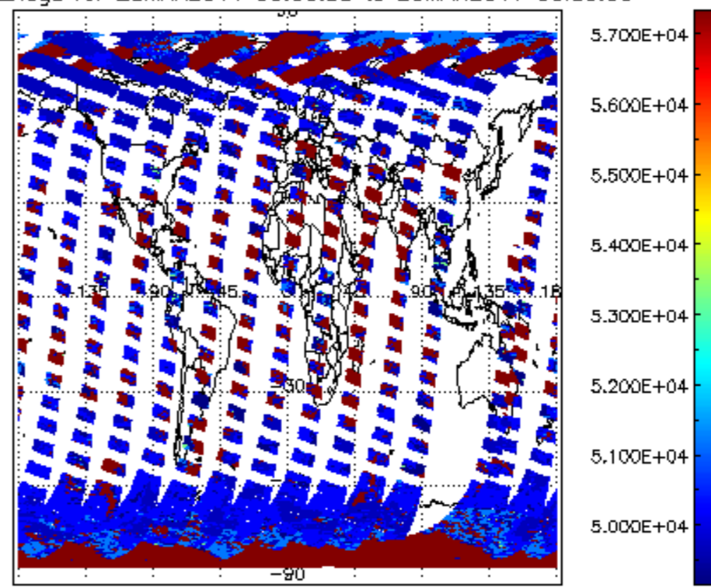
cloud_flags for 25MAR2011 00:00:00 to 26MAR2011 00:00:00
