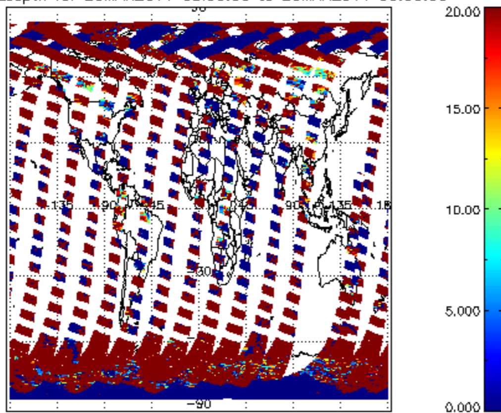
cL_opt_depth for 25MAR2011 00:00:00 to 26MAR2011 00:00:00
