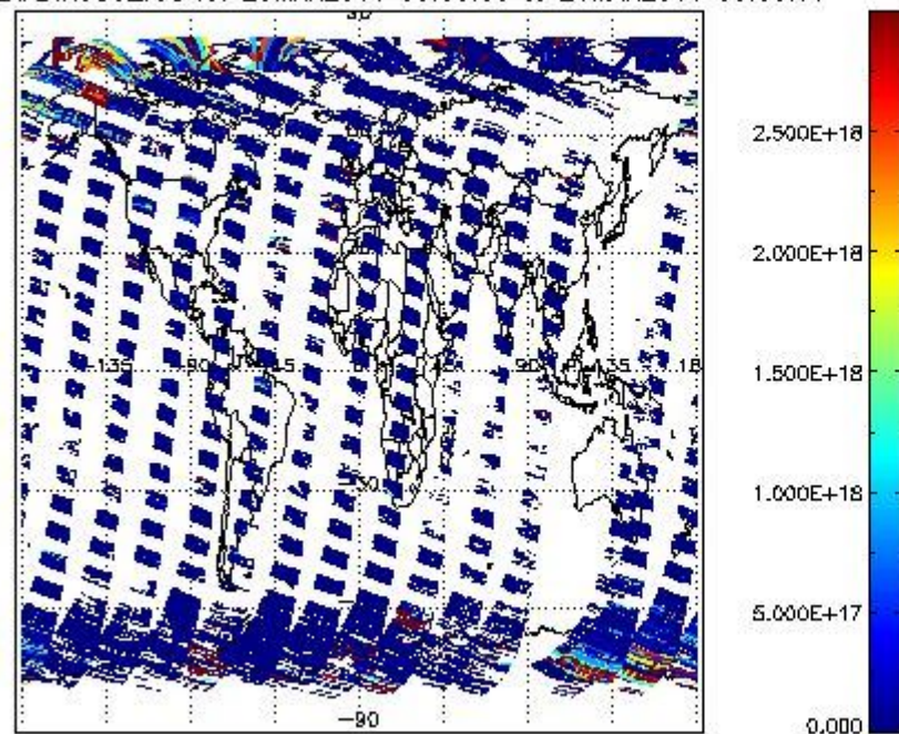
SCIDL2P_NADIR3CO_vcd for 25MAR2011 00:00:00 to 26MAR2011 00:00:00
