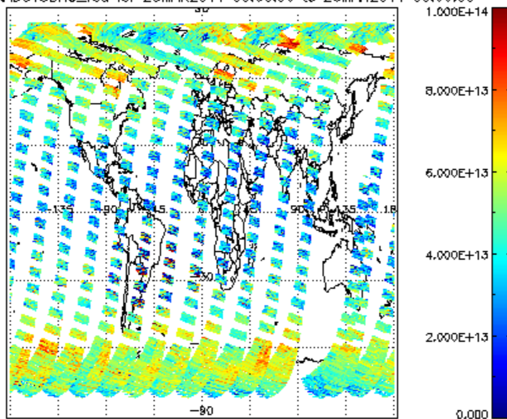
SCIOL2P_NADUV3BRO_vcd for 25MAR2011 00:00:00 to 26MAR2011 00:00:00
