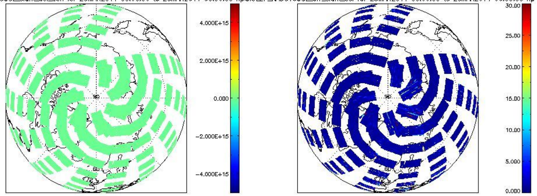
CIOL2P_NADUV6OCLslant_col_den for 25MAR2011 00:00:00 to 26MAR2011 00:00:00 npCIOL2P_NADUV6OCLarr_slant_col for 25MAR2011 00:00:00 to 26MAR2011 00:00:00 np
