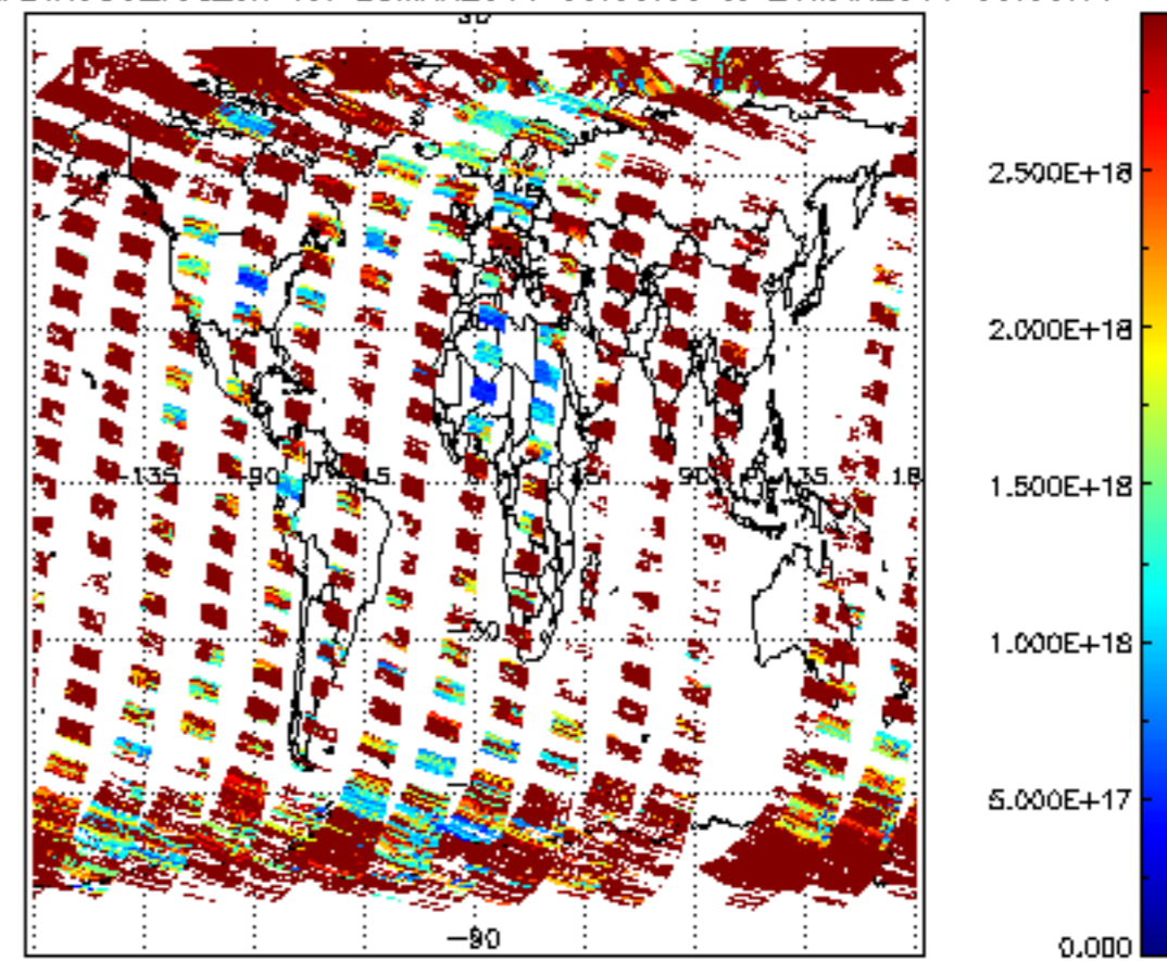
SCIOL2P_NADIR3CO_vcd_err for 25MAR2011 00:00:00 to 26MAR2011 00:00:00
