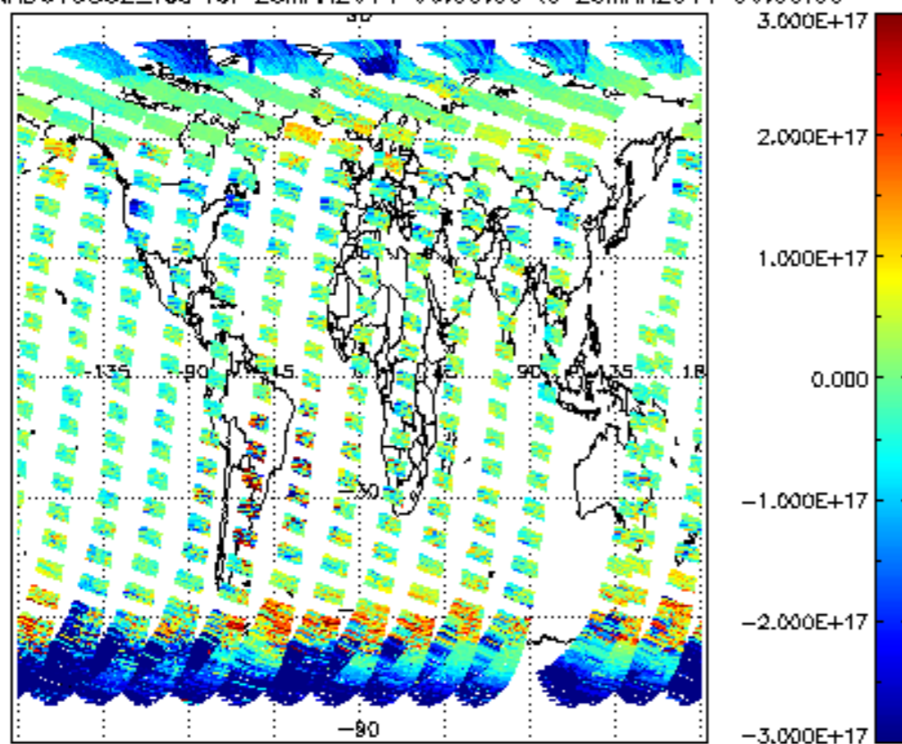
SCIOL2P_NADUV5S02_vcd for 25MAR2011 00:00:00 to 26MAR2011 00:00:00
