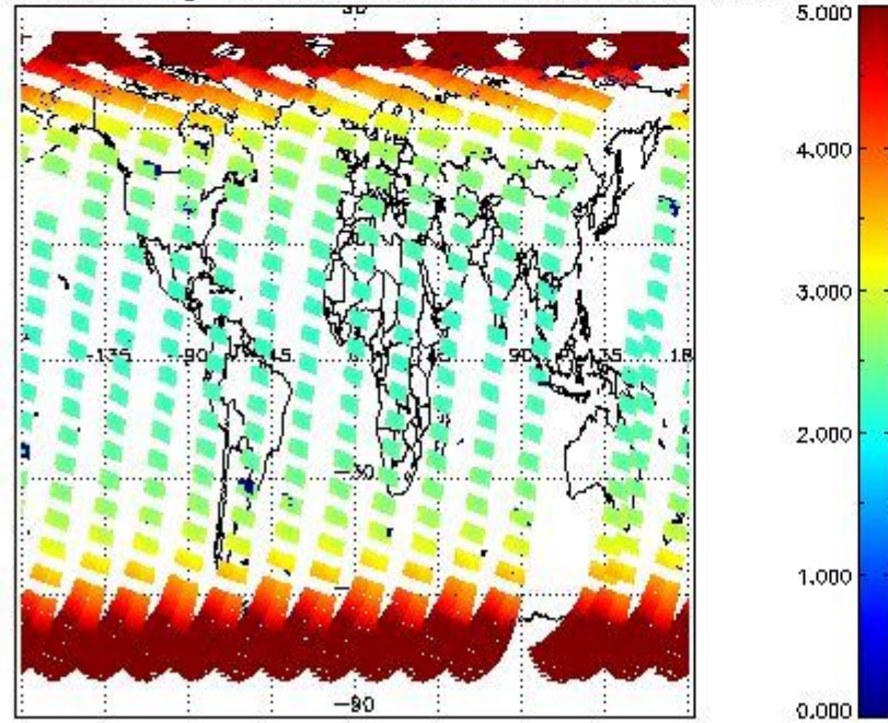
SCIOL2P_NADUV003_amf_gr for 25MAR2011 00:00:00 to 26MAR2011 00:00:00
