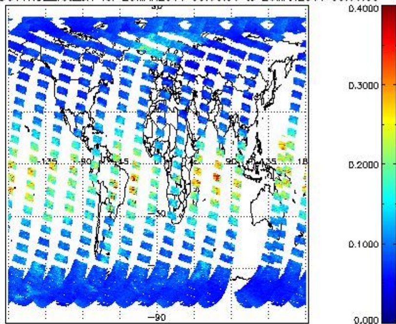
SCIOL2P_NADUV1NO2_vcd_err for 25MAR2011 00:00:00 to 26MAR2011 00:00:00
