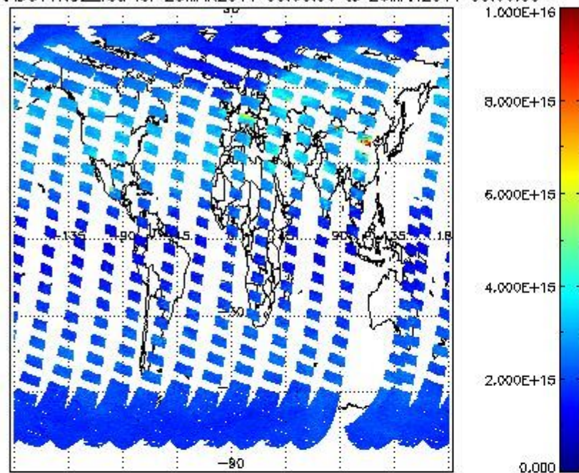
SCIOL2P_NADUV1NO2_vcd for 25MAR2011 00:00:00 to 26MAR2011 00:00:00
