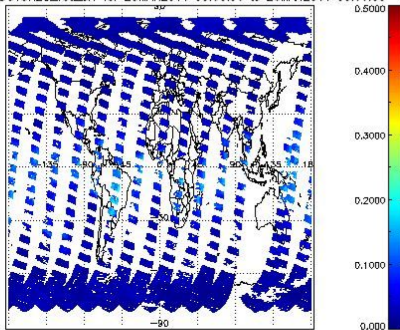
SCIOL2P_NADUV8H2O_vcd_err for 25MAR2011 00:00:00 to 26MAR2011 00:00:00
