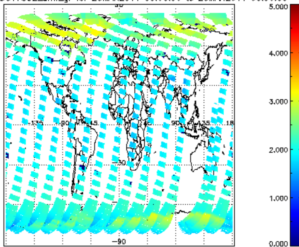
SCIOL2P_NADUV7S02_amf_gr for 25MAR2011 00:00:00 to 26MAR2011 00:00:00
