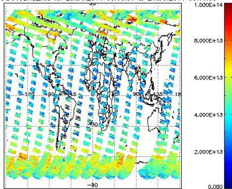
SCIOL2P_NADUV3BRO_vcd for 25MAR2011 00:00:00 to 26MAR2011 00:00:00
