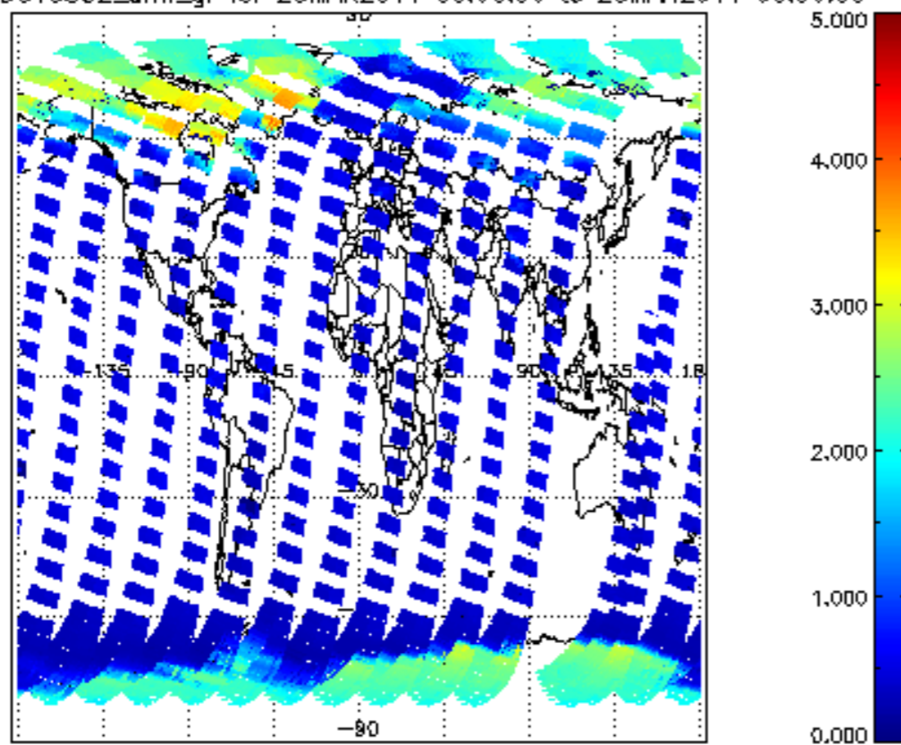
SCIOL2P_NADUV5S02_amf_gr for 25MAR2011 00:00:00 to 26MAR2011 00:00:00
