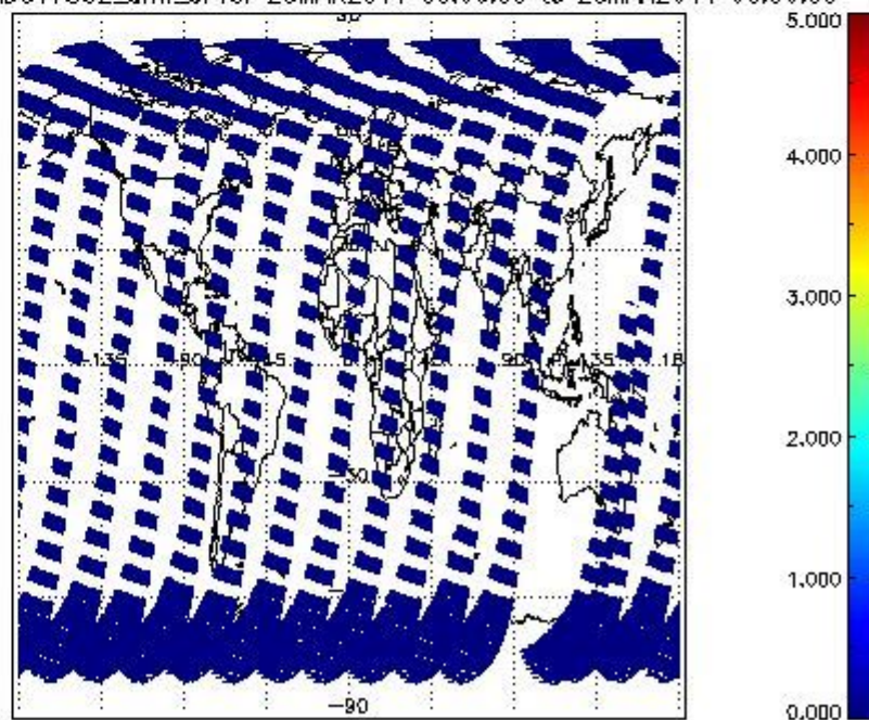
SCIOL2P_NADUV7S02_amf_cl for 25MAR2011 00:00:00 to 26MAR2011 00:00:00
