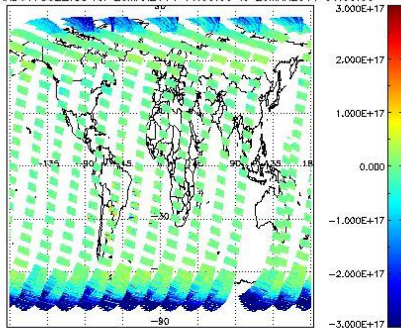
SCIOL2P_NADUV7S02_vcd for 25MAR2011 00:00:00 to 26MAR2011 00:00:00
