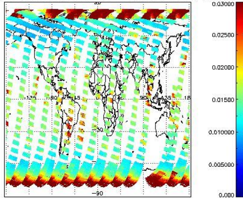
SCIOL2P_NADUV003_vcd_err for 25MAR2011 00:00:00 to 26MAR2011 00:00:00
