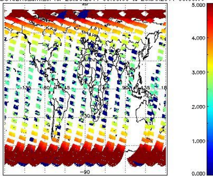
SCIOL2P_NADUV3BRO_amf_cl for 25MAR2011 00:00:00 to 26MAR2011 00:00:00
