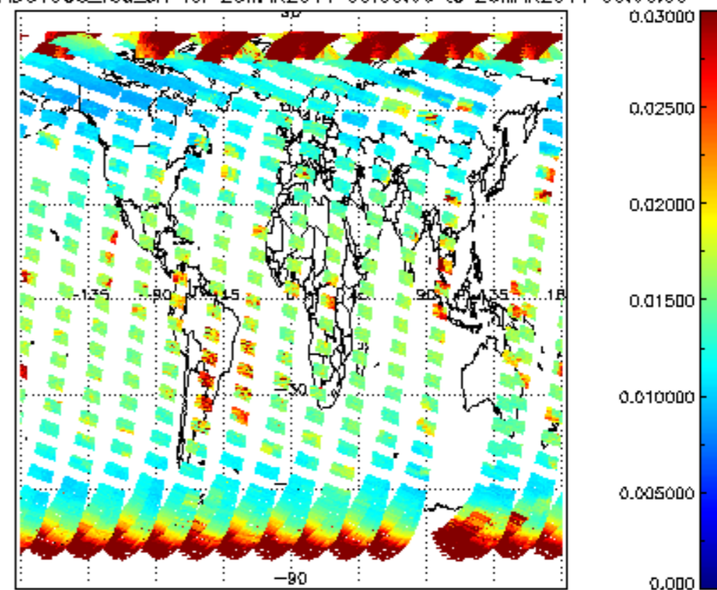
SCIOL2P_NADUV003_vcd_err for 25MAR2011 00:00:00 to 26MAR2011 00:00:00
