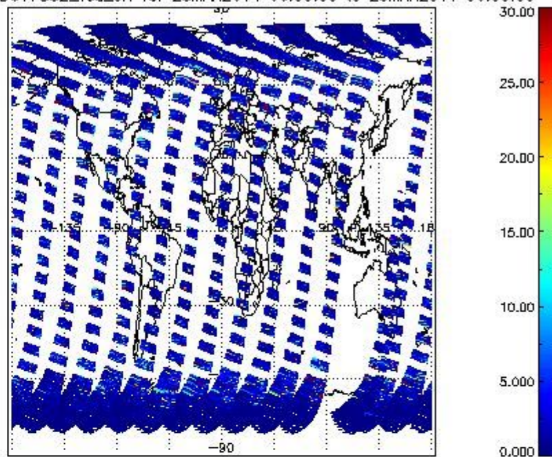
SCIOL2P_NADUV7S02_vcd_err for 25MAR2011 00:00:00 to 26MAR2011 00:00:00
