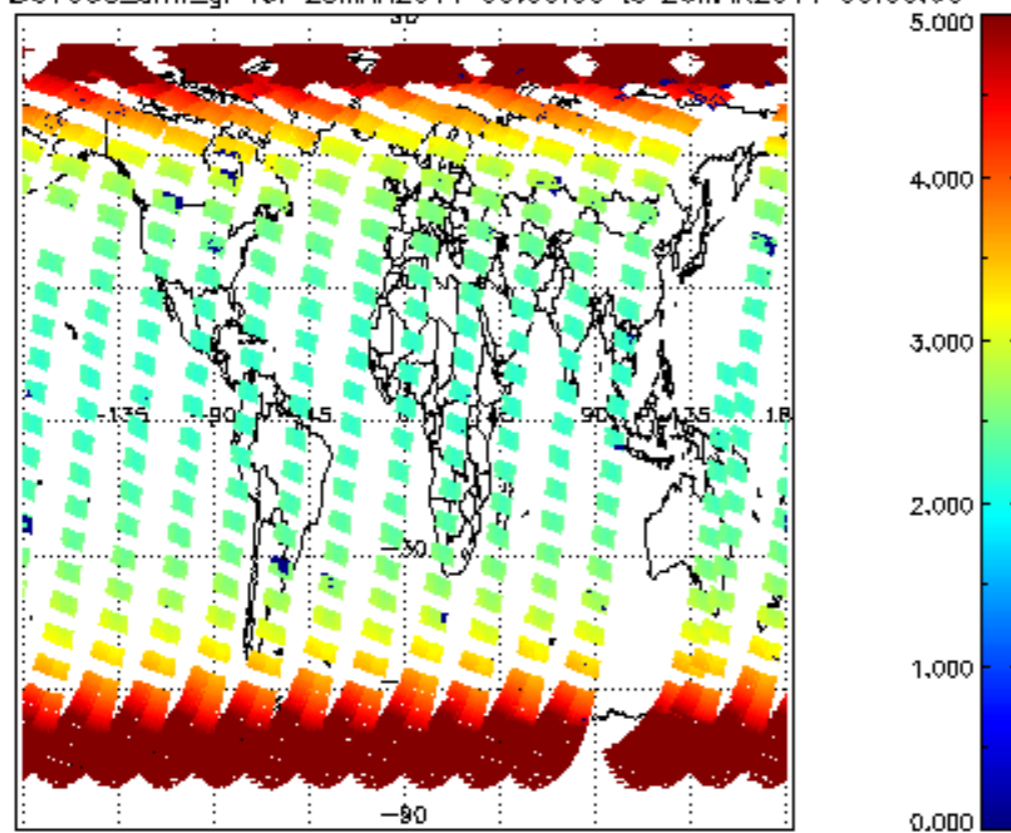
SCIOL2P_NADUV003_arnf_gr for 25MAR2011 00:00:00 to 26MAR2011 00:00:00
