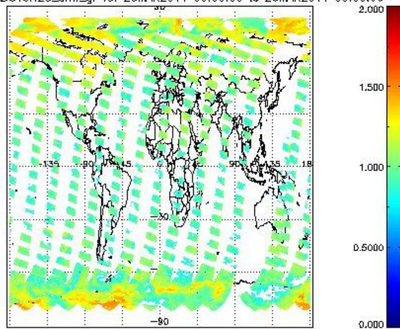
SCIOL2P_NADUV8H2O_arnf_gr for 25MAR2011 00:00:00 to 26MAR2011 00:00:00
