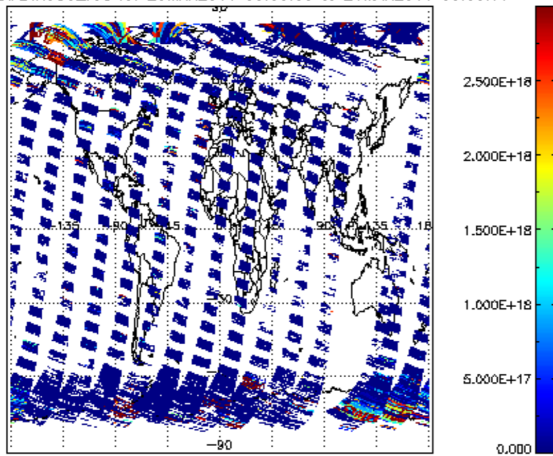
SCIOL2P_NADIR3CO_vcd for 25MAR2011 00:00:00 to 26MAR2011 00:00:00
