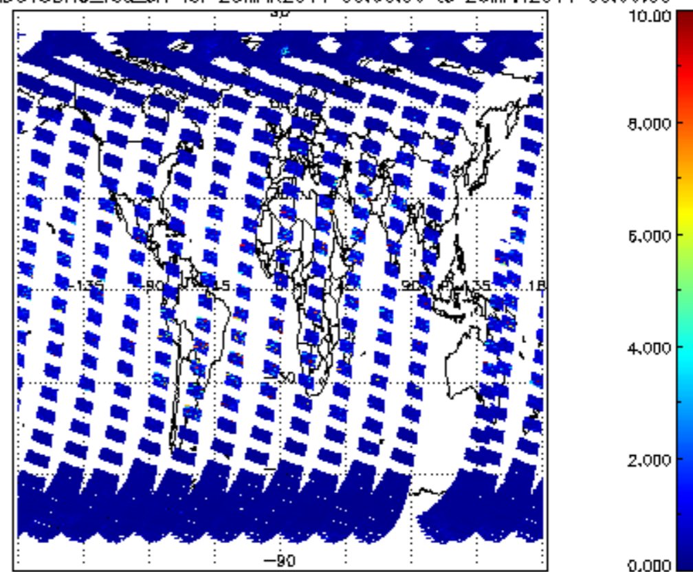
SCIOL2P_NADUV3BRO_vcd_err for 25MAR2011 00:00:00 to 26MAR2011 00:00:00
