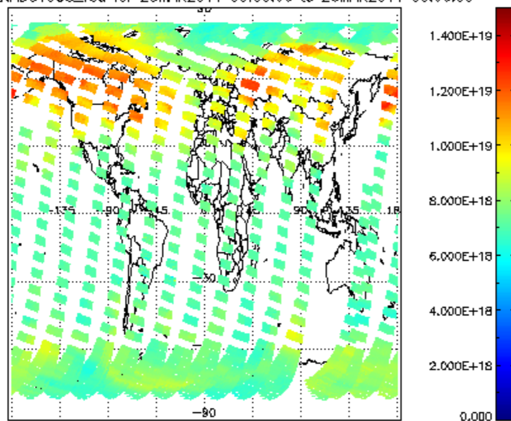
SCIOL2P_NADUV003_vcd for 25MAR2011 00:00:00 to 26MAR2011 00:00:00
