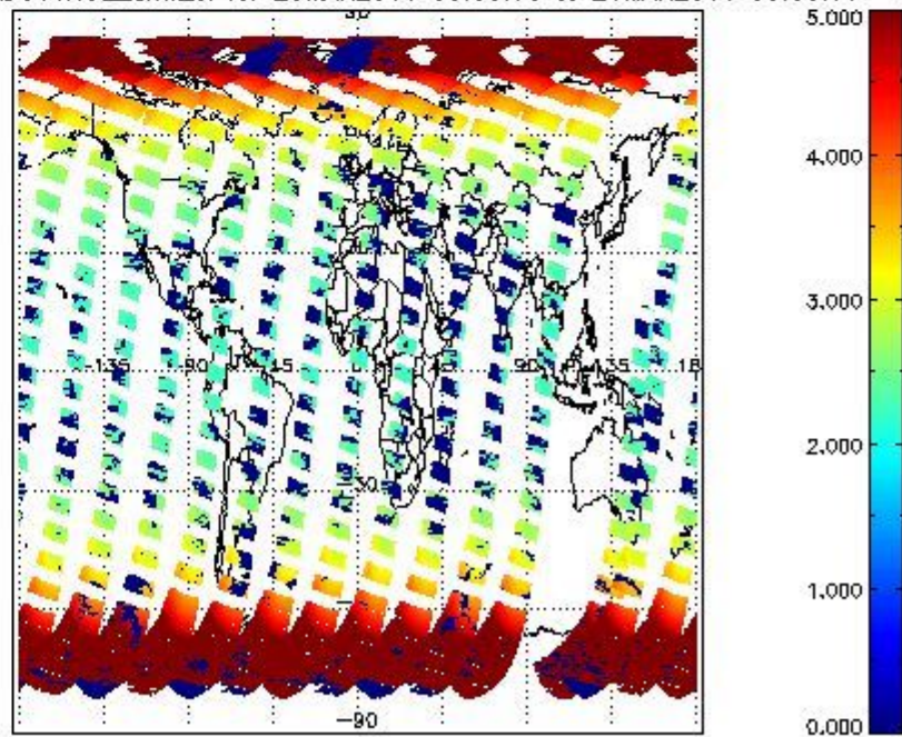
SCIOL2P_NADUV1NO2_amf_cl for 25MAR2011 00:00:00 to 26MAR2011 00:00:00
