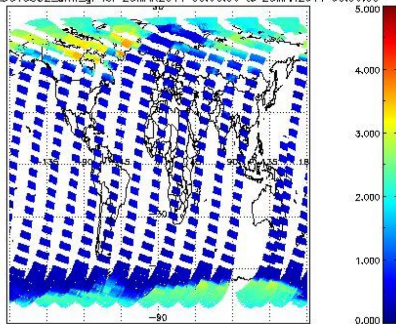
SCIOL2P_NADUV5SO2_amf_gr for 25MAR2011 00:00:00 to 26MAR2011 00:00:00
