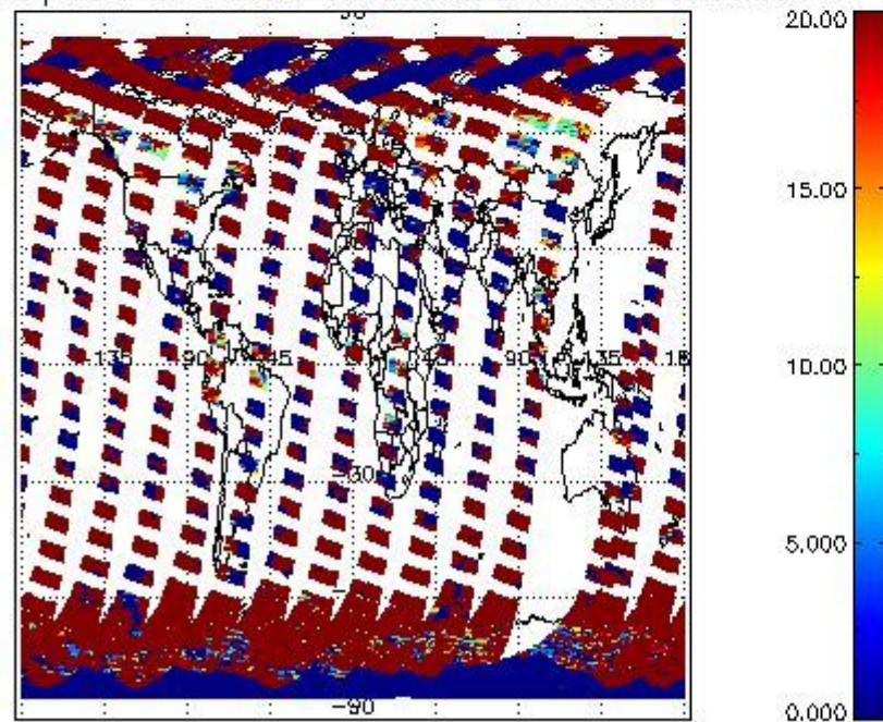
cL_opt_depth for 25MAR2011 00:00:00 to 26MAR2011 00:00:00
