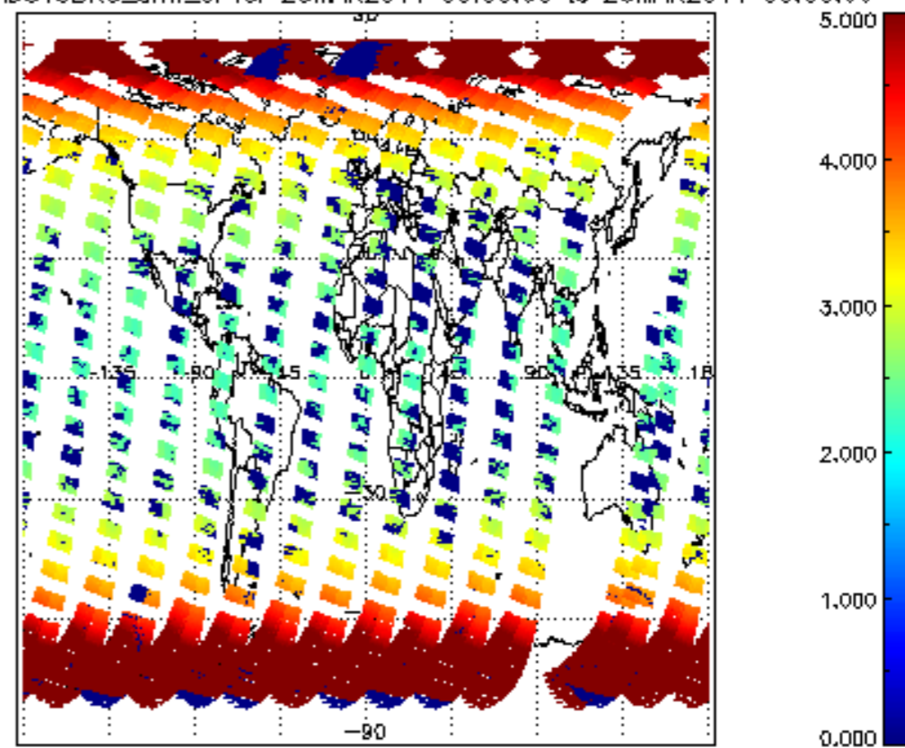
SCIOL2P_NADUV3BRO_amf_cl for 25MAR2011 00:00:00 to 26MAR2011 00:00:00
