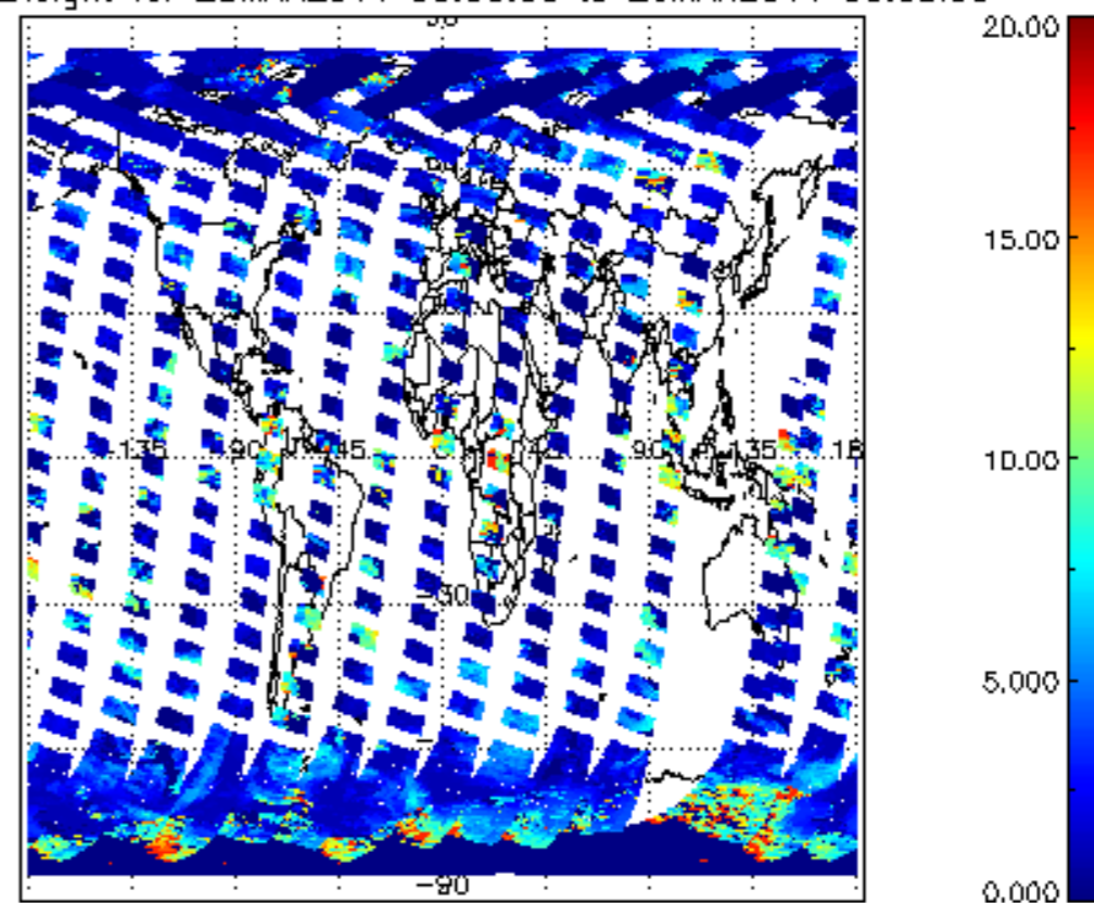
cL_top_height for 25MAR2011 00:00:00 to 26MAR2011 00:00:00
