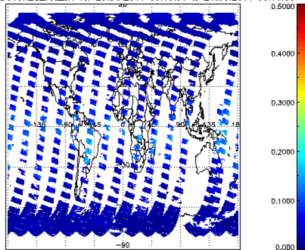
SCIOL2P_NADUV8H2O_vcd_err for 25MAR2011 00:00:00 to 26MAR2011 00:00:00
