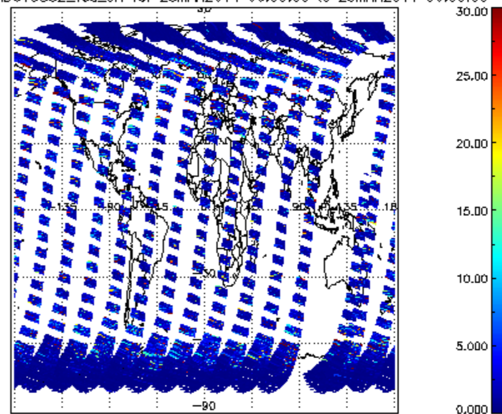
SCIOL2P_NADUV5S02_vcd_err for 25MAR2011 00:00:00 to 26MAR2011 00:00:00
