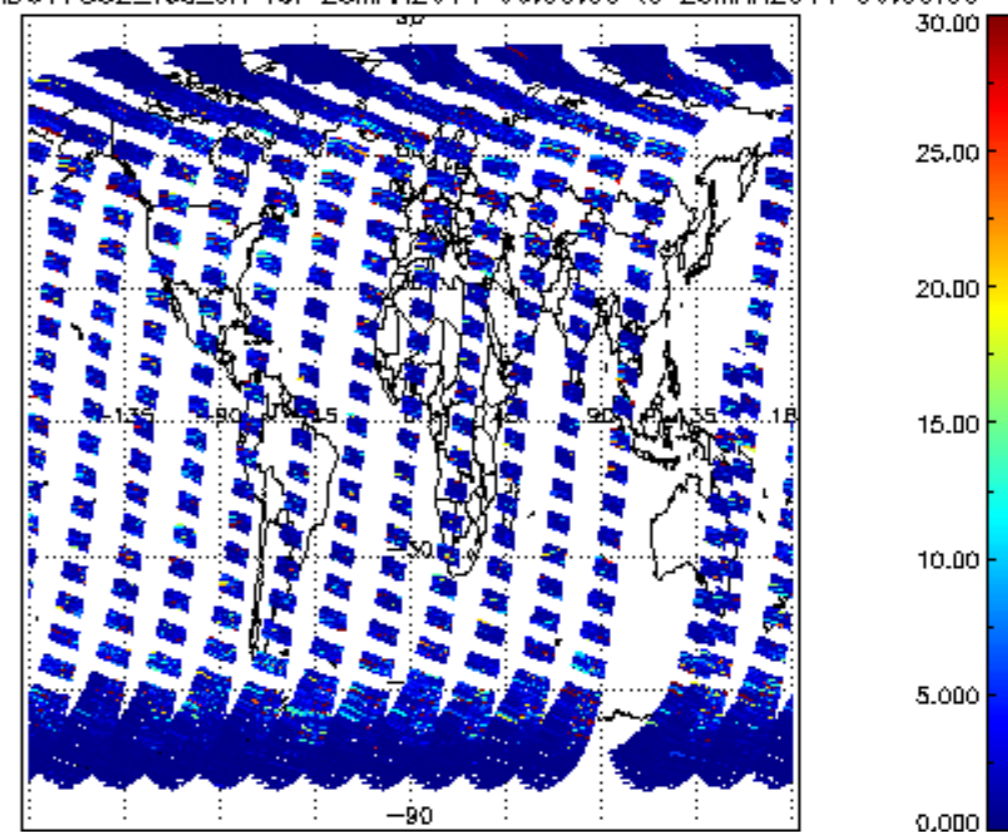
SCIOL2P_NADUV7S02_vcd_err for 25MAR2011 00:00:00 to 26MAR2011 00:00:00
