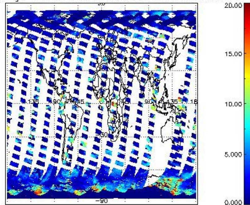
cL_top_height for 25MAR2011 00:00:00 to 26MAR2011 00:00:00
