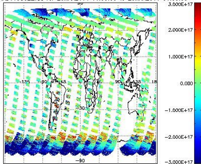
SCIOL2P_NADUV5SO2_vcd for 25MAR2011 00:00:00 to 26MAR2011 00:00:00
