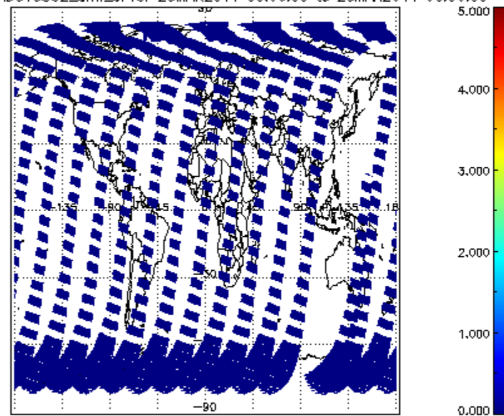
SCIOL2P_NADUV5S02_amf_cl for 25MAR2011 00:00:00 to 26MAR2011 00:00:00
