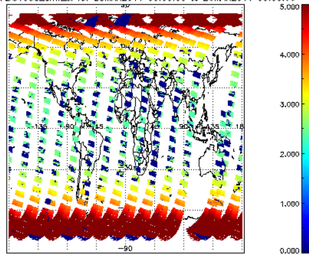
SCIOL2P_NADUV003_arnf_cl for 25MAR2011 00:00:00 to 26MAR2011 00:00:00
