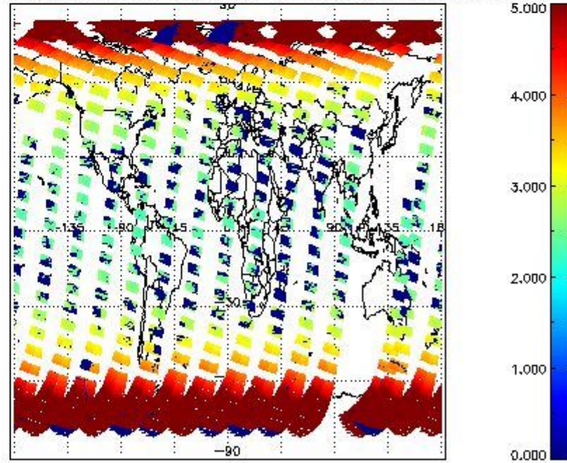
SCIOL2P_NADUV003_amf_cl for 25MAR2011 00:00:00 to 26MAR2011 00:00:00
