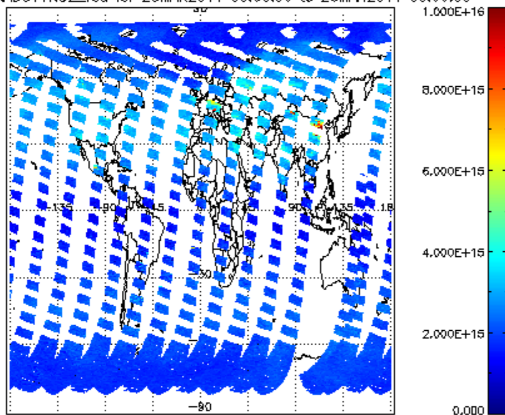
SCIOL2P_NADUV1NO2_vcd for 25MAR2011 00:00:00 to 26MAR2011 00:00:00
