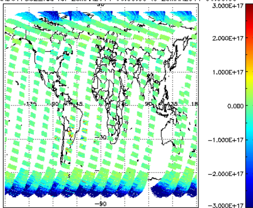
SCIOL2P_NADUV7S02_vcd for 25MAR2011 00:00:00 to 26MAR2011 00:00:00
