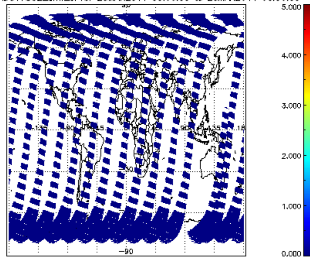
SCIOL2P_NADUV7S02_amf_cl for 25MAR2011 00:00:00 to 26MAR2011 00:00:00
