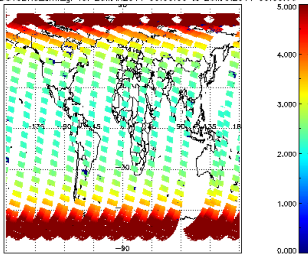
SCIOL2P_NADUV3BRO_amf_gr for 25MAR2011 00:00:00 to 26MAR2011 00:00:00
