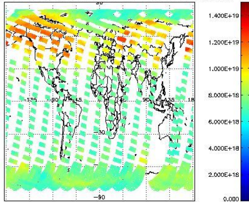
SCIOL2P_NADUV003_vcd for 25MAR2011 00:00:00 to 26MAR2011 00:00:00
