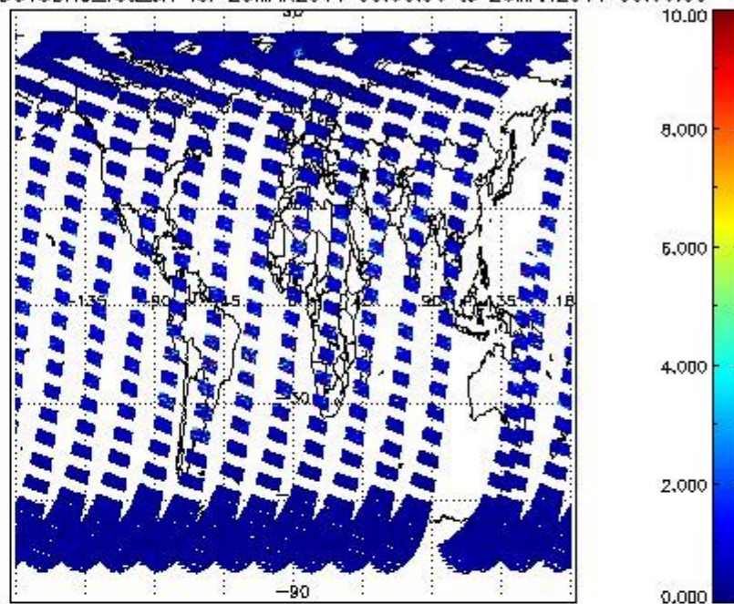
SCIOL2P_NADUV3BRO_vcd_err for 25MAR2011 00:00:00 to 26MAR2011 00:00:00
