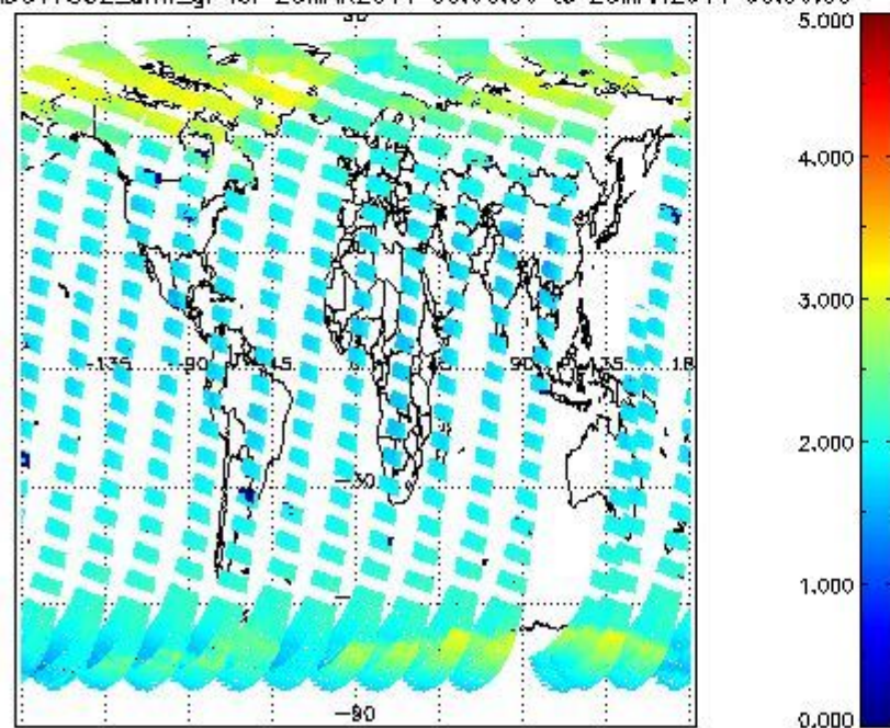
SCIOL2P_NADUV7S02_amf_gr for 25MAR2011 00:00:00 to 26MAR2011 00:00:00
