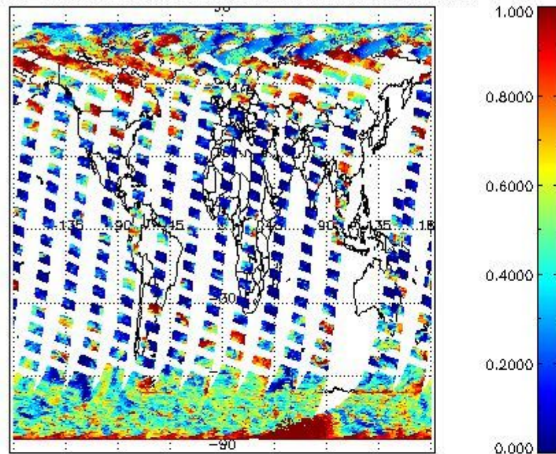
cL_frac for 25MAR2011 00:00:00 to 26MAR2011 00:00:00
