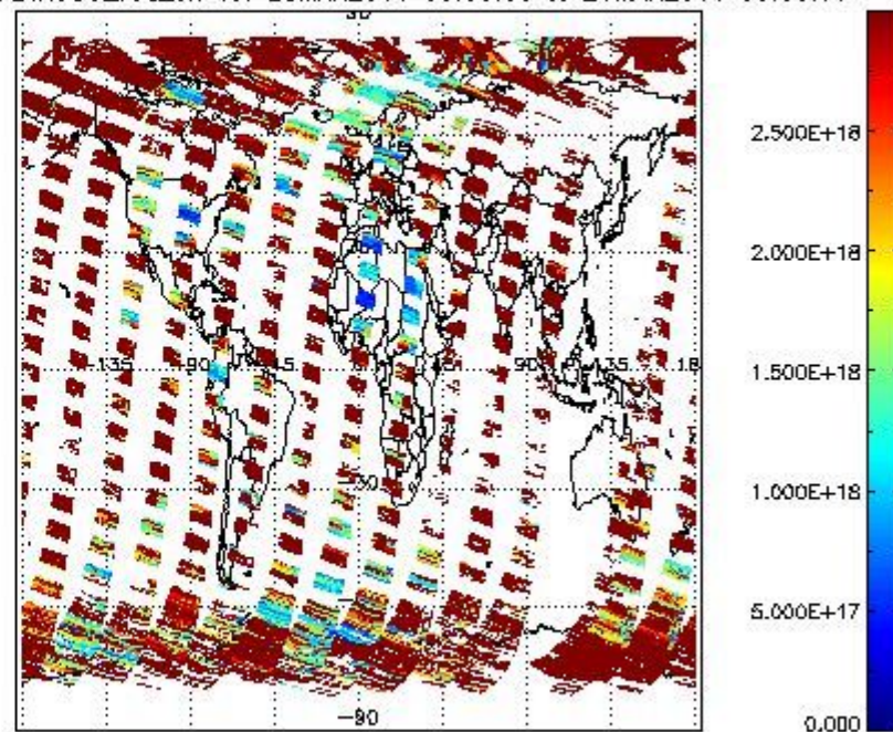
SCIDL2P_NADIR3CO_vcd_err for 25MAR2011 00:00:00 to 26MAR2011 00:00:00
