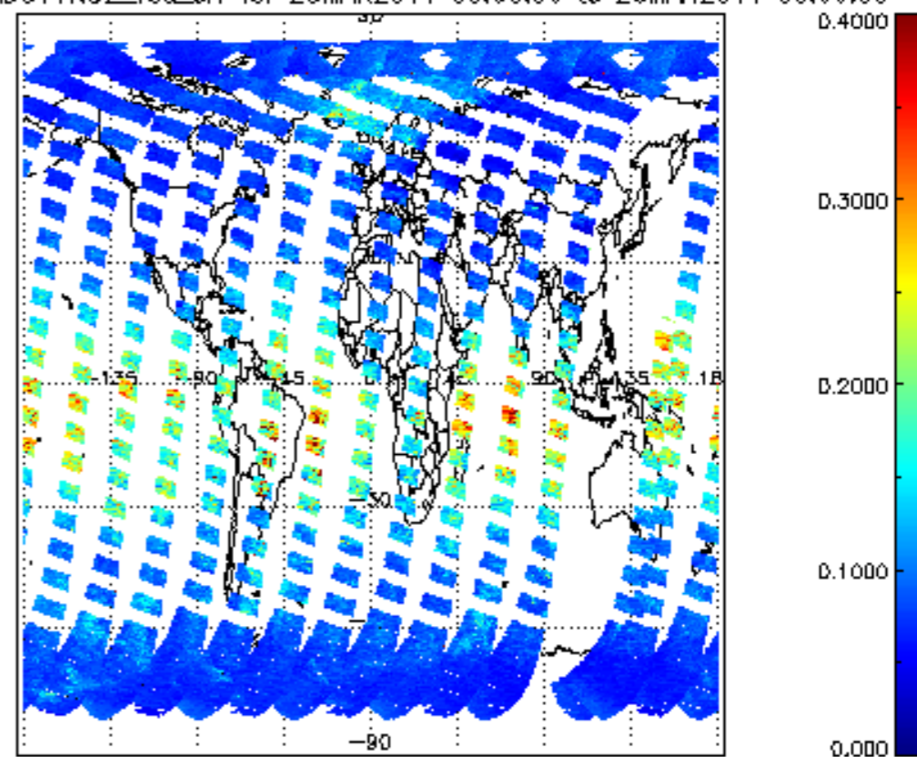
SCIOL2P_NADUV1NO2_vcd_err for 25MAR2011 00:00:00 to 26MAR2011 00:00:00
