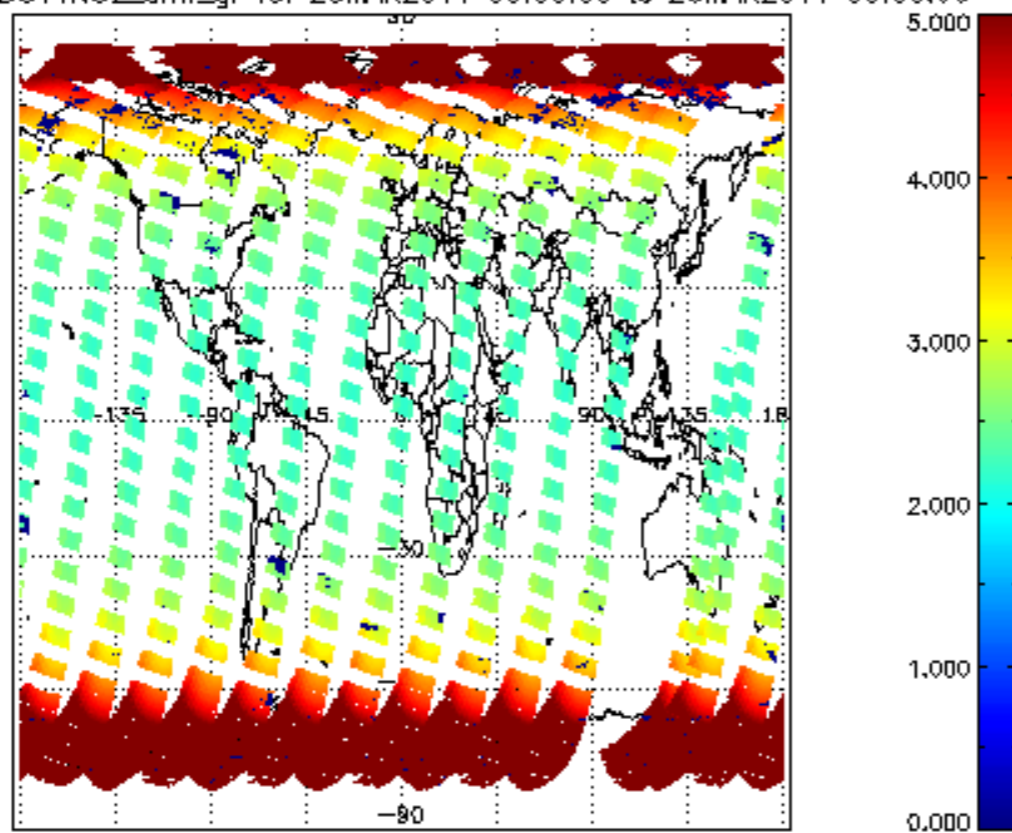
SCIOL2P_NADUV1NO2_amf_gr for 25MAR2011 00:00:00 to 26MAR2011 00:00:00
