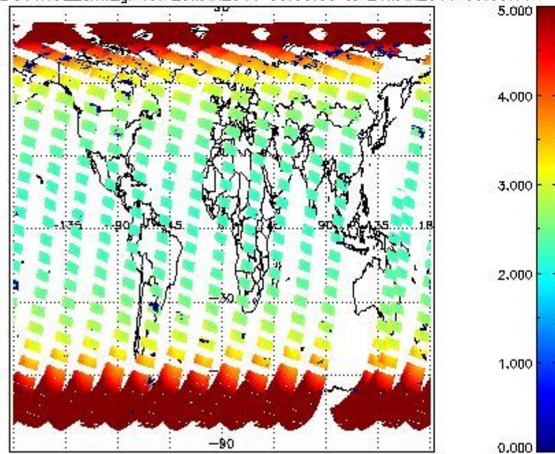
SCIOL2P_NADUV1NO2_amf_gr for 25MAR2011 00:00:00 to 26MAR2011 00:00:00
