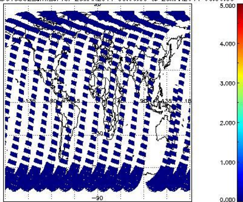
SCIOL2P_NADUV5SO2_amf_cl for 25MAR2011 00:00:00 to 26MAR2011 00:00:00
