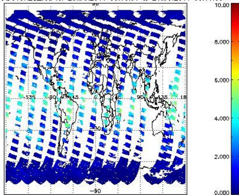
SCIOL2P_NADUV8H2O_vcd for 25MAR2011 00:00:00 to 26MAR2011 00:00:00
