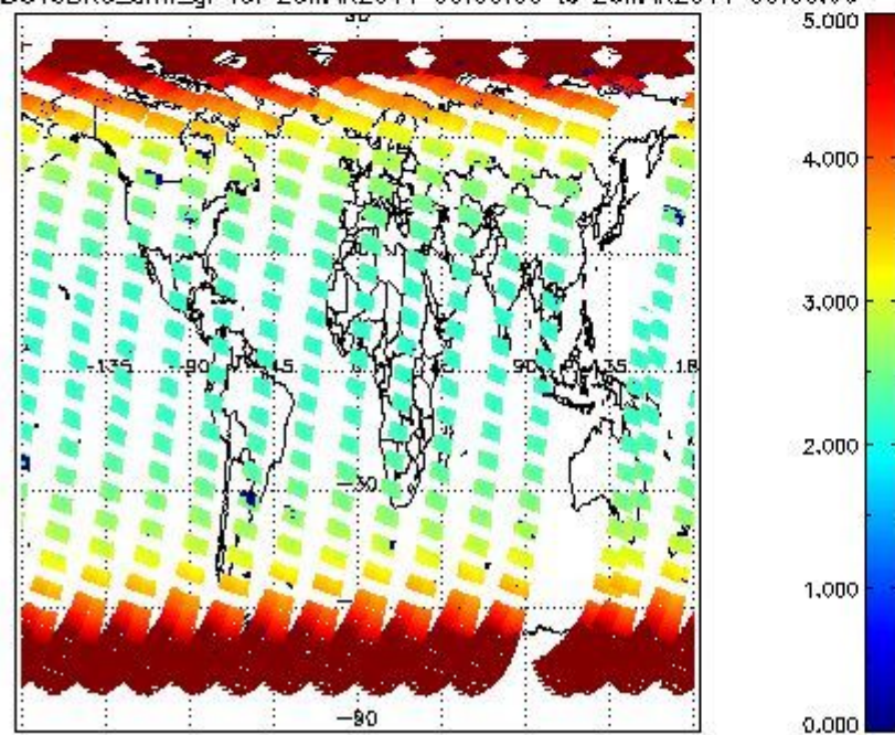
SCIOL2P_NADUV3BRO_amf_gr for 25MAR2011 00:00:00 to 26MAR2011 00:00:00
