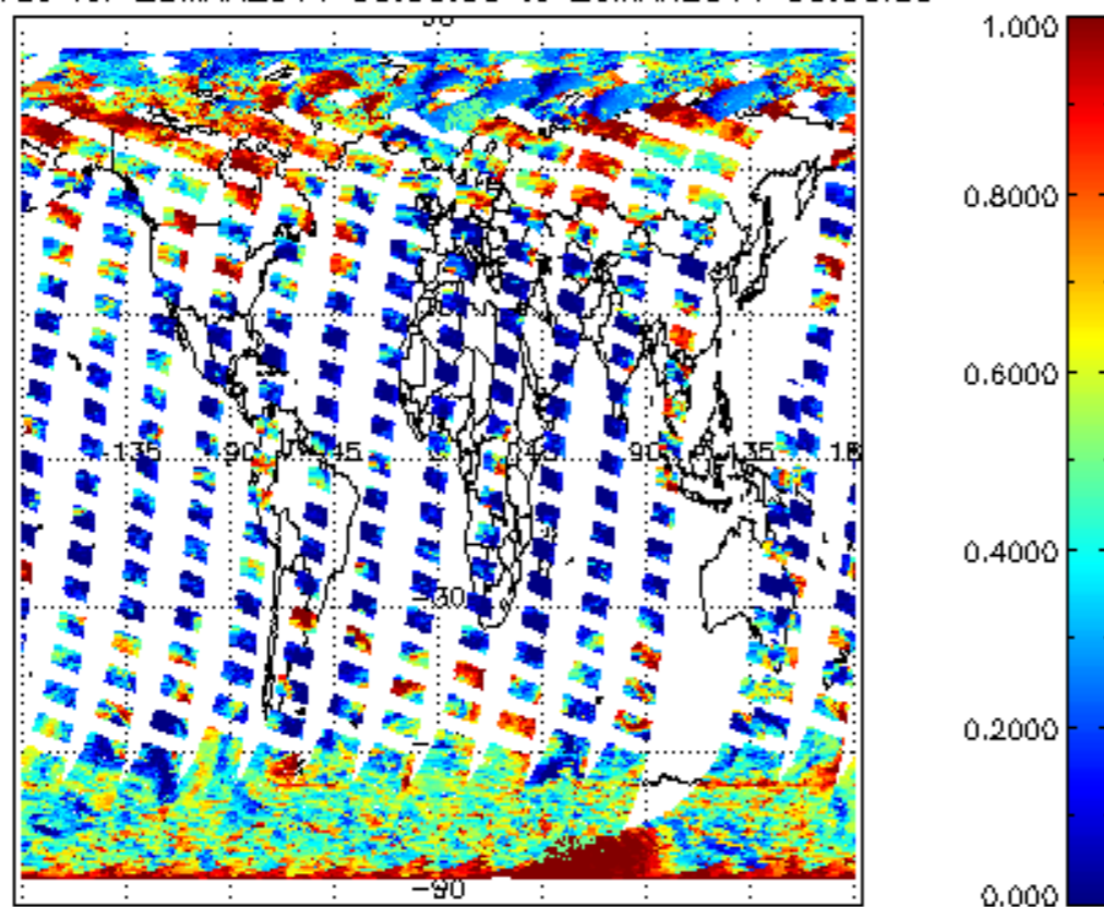
cL_frac for 25MAR2011 00:00:00 to 26MAR2011 00:00:00
