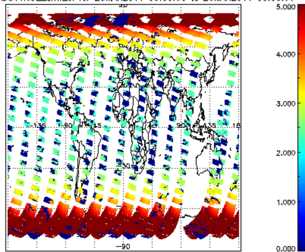
SCIOL2P_NADUV1NO2_amf_cl for 25MAR2011 00:00:00 to 26MAR2011 00:00:00
