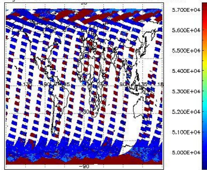
cloud_flags for 25MAR2011 00:00:00 to 26MAR2011 00:00:00
