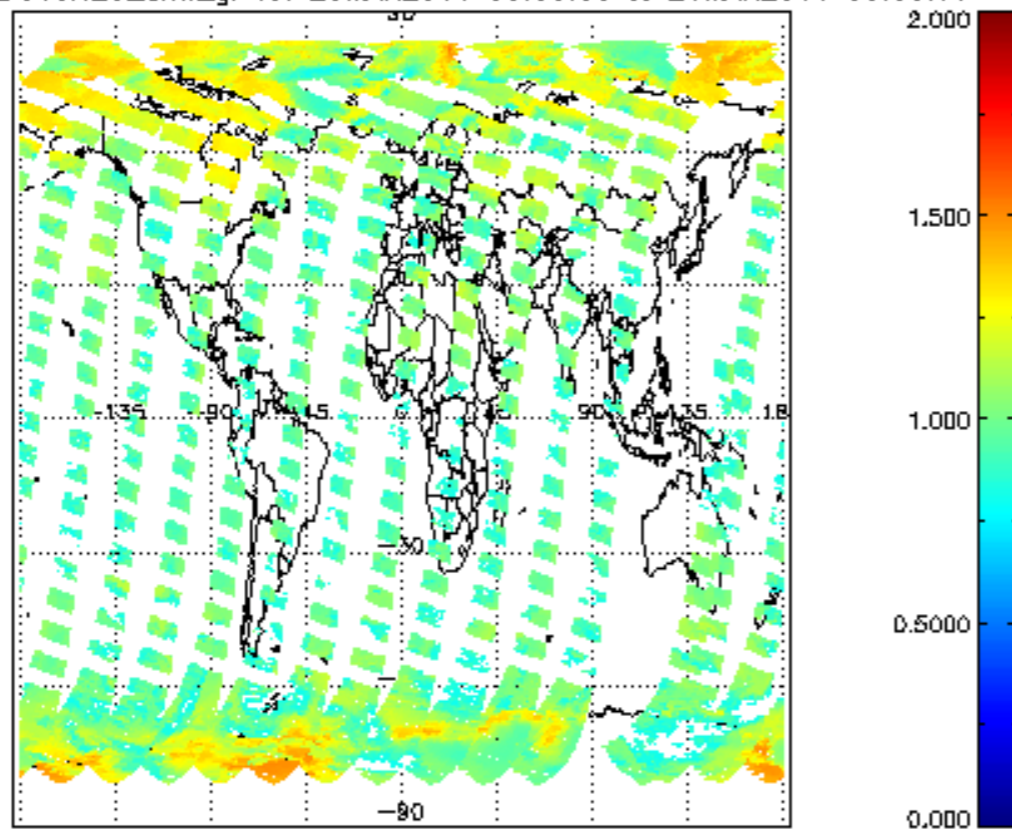
SCIOL2P_NADUV8H2O_arnf_gr for 25MAR2011 00:00:00 to 26MAR2011 00:00:00
