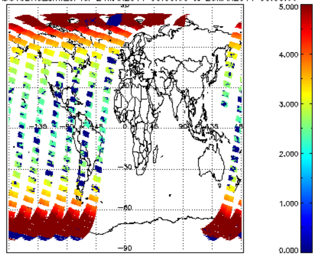
SCIOL2P_NADUV3BRO_arnf_cl for 24MAR2011 00:00:00 to 25MAR2011 00:00:00
