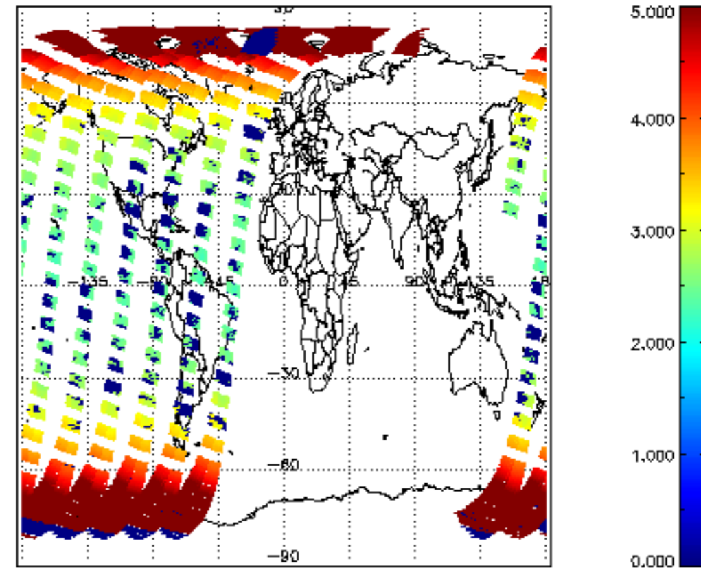
SCIOL2P_NADUV003_arnf_cl for 24MAR2011 00:00:00 to 25MAR2011 00:00:00
