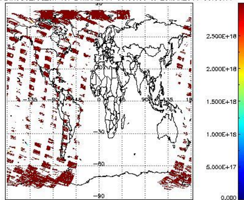
SCIOL2P_NADIR3CO_vcd_err for 24MAR2011 00:00:00 to 25MAR2011 00:00:00
