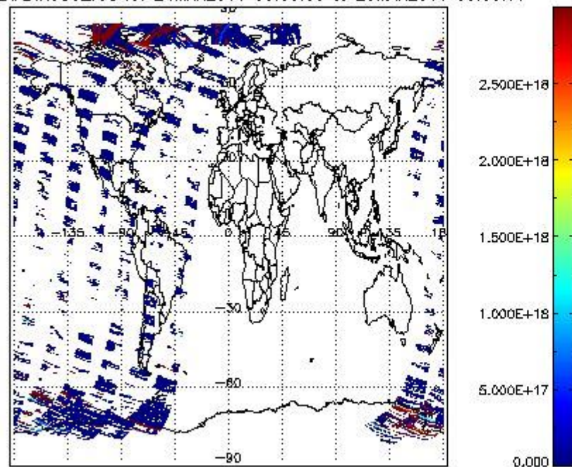
SCIOL2P_NADIR3CO_vcd for 24MAR2011 00:00:00 to 25MAR2011 00:00:00
