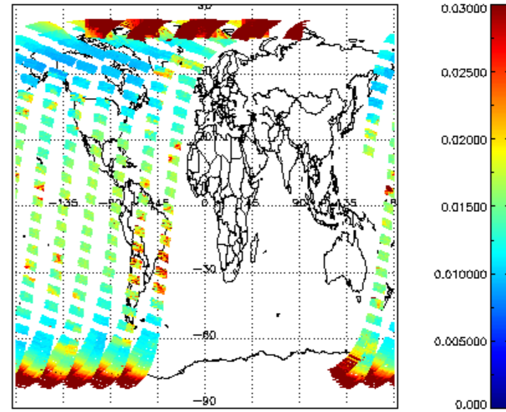
SCIOL2P_NADUV003_vcd_err for 24MAR2011 00:00:00 to 25MAR2011 00:00:00
