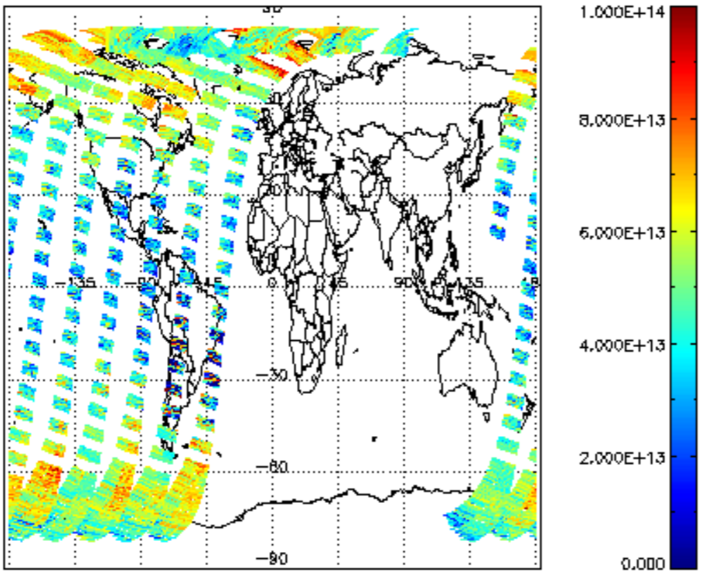
SCIOL2P_NADUV3BRO_vcd for 24MAR2011 00:00:00 to 25MAR2011 00:00:00
