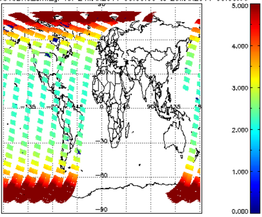
SCIOL2P_NADUV3BRO_arnf_gr for 24MAR2011 00:00:00 to 25MAR2011 00:00:00
