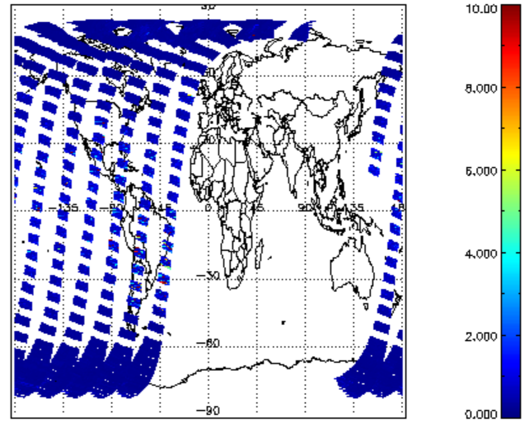
SCIOL2P_NADUV3BRO_vcd_err for 24MAR2011 00:00:00 to 25MAR2011 00:00:00
