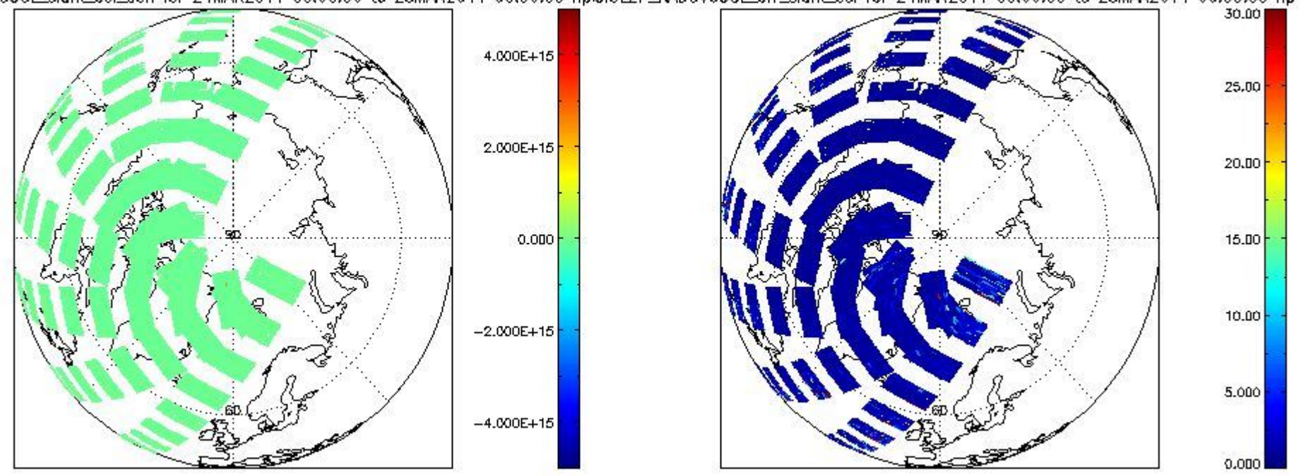
CIOL2P_NADUV6OCL_slant_col_den for 24MAR2011 00:00:00 to 25MAR2011 00:00:00 np CIOL2P_NADUV6OCL_err_slant_col for 24MAR2011 00:00:00 to 25MAR2011 00:00:00 np
