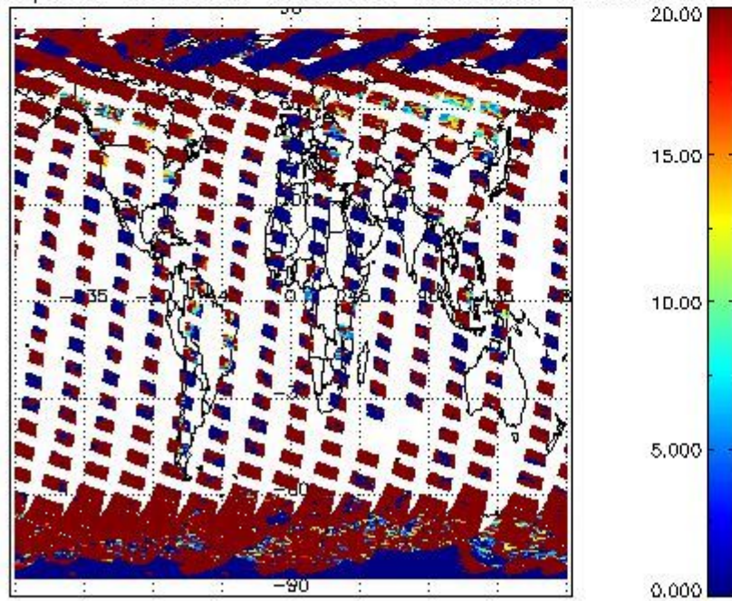
cL_opt_depth for 21MAR2011 00:00:00 to 22MAR2011 00:00:00
