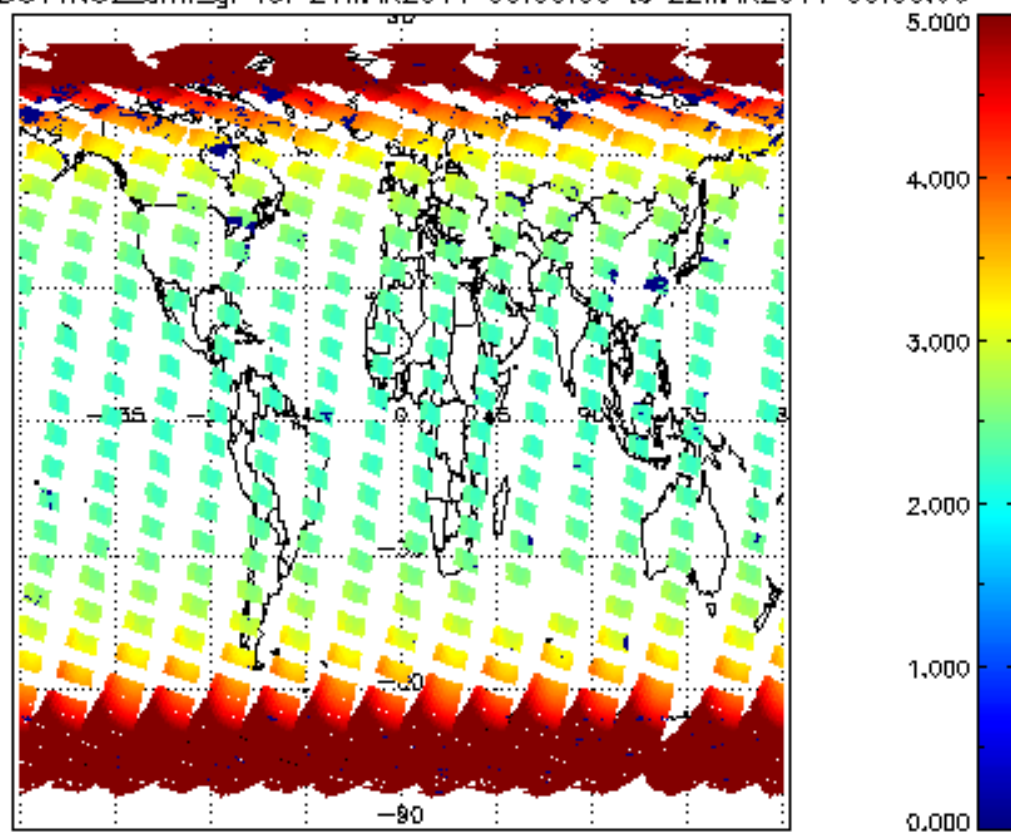
SCIOL2P_NADUV1NO2_amf_gr for 21MAR2011 00:00:00 to 22MAR2011 00:00:00
