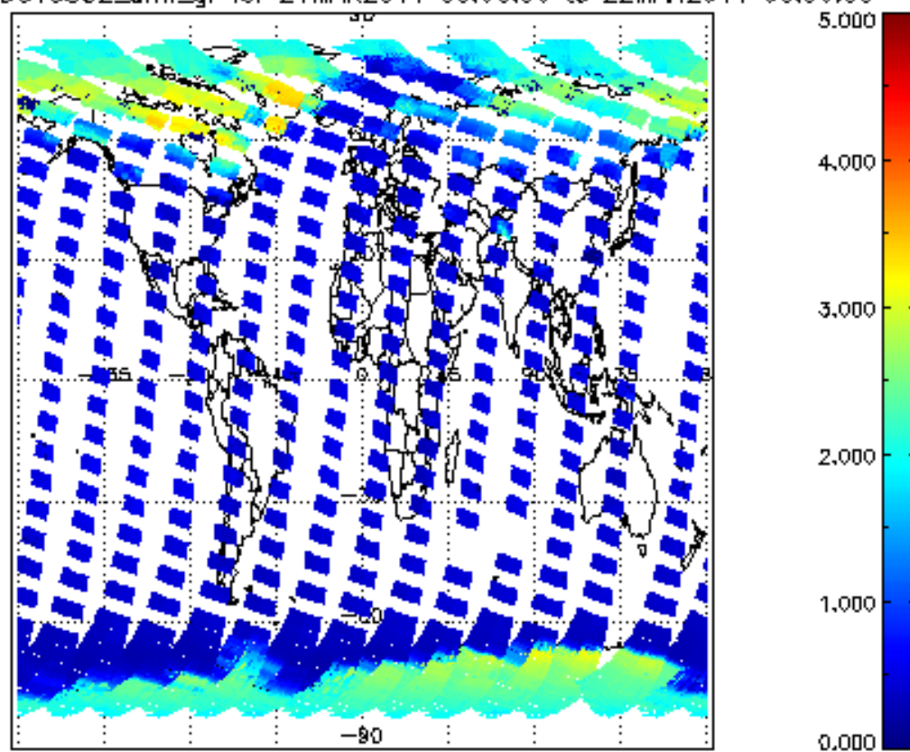
SCIOL2P_NADUV5S02_amf_gr for 21MAR2011 00:00:00 to 22MAR2011 00:00:00
