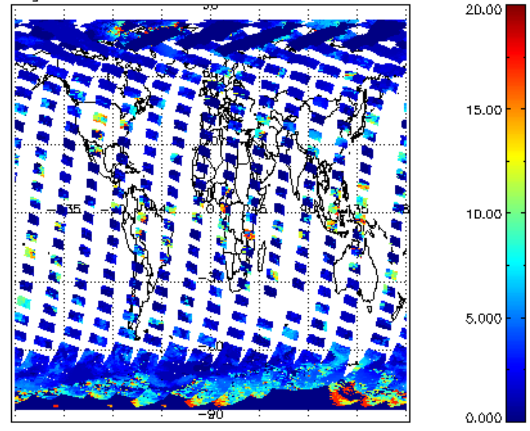
cL_top_height for 21MAR2011 00:00:00 to 22MAR2011 00:00:00
