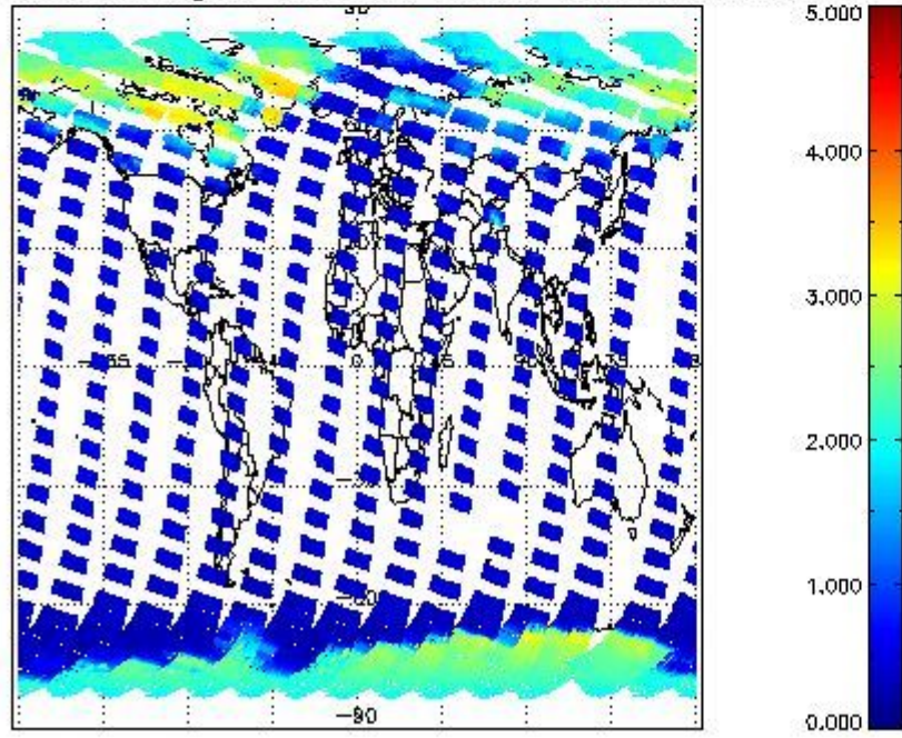
SCIOL2P_NADUV5S02_amf_gr for 21MAR2011 00:00:00 to 22MAR2011 00:00:00
