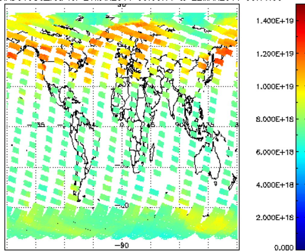
SCIOL2P_NADUV003_vcd for 21MAR2011 00:00:00 to 22MAR2011 00:00:00
