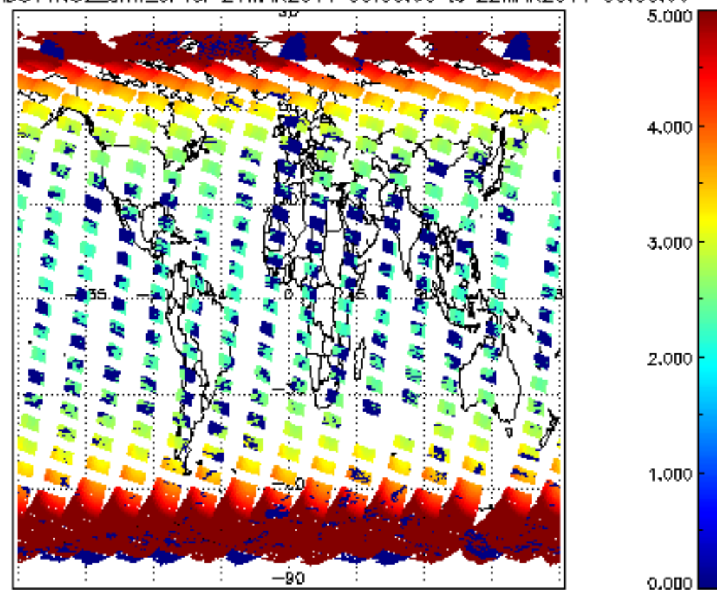
SCIOL2P_NADUV1NO2_amf_cl for 21MAR2011 00:00:00 to 22MAR2011 00:00:00
