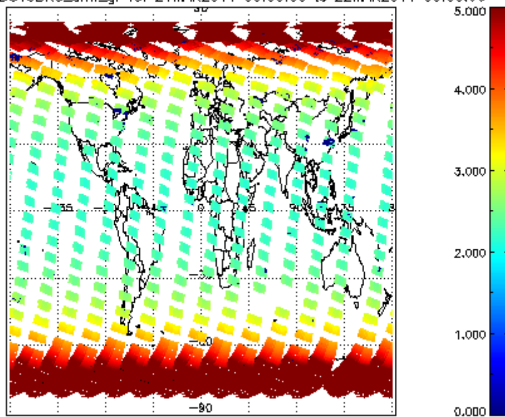
SCIOL2P_NADUV3BRO_amf_gr for 21MAR2011 00:00:00 to 22MAR2011 00:00:00
