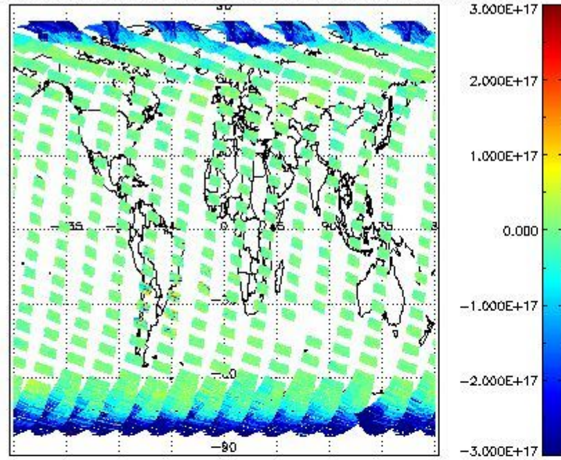
SCIOL2P_NADUV7S02_vcd for 21MAR2011 00:00:00 to 22MAR2011 00:00:00
