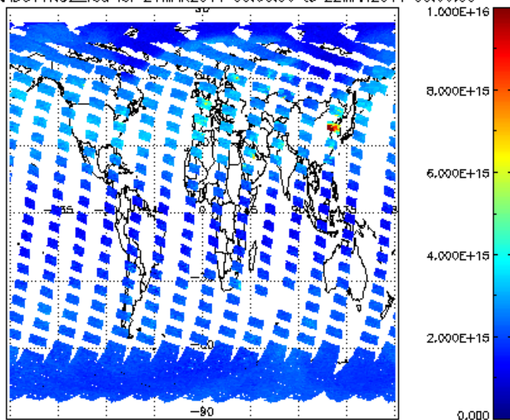
SCIOL2P_NADUV1NO2_vcd for 21MAR2011 00:00:00 to 22MAR2011 00:00:00
