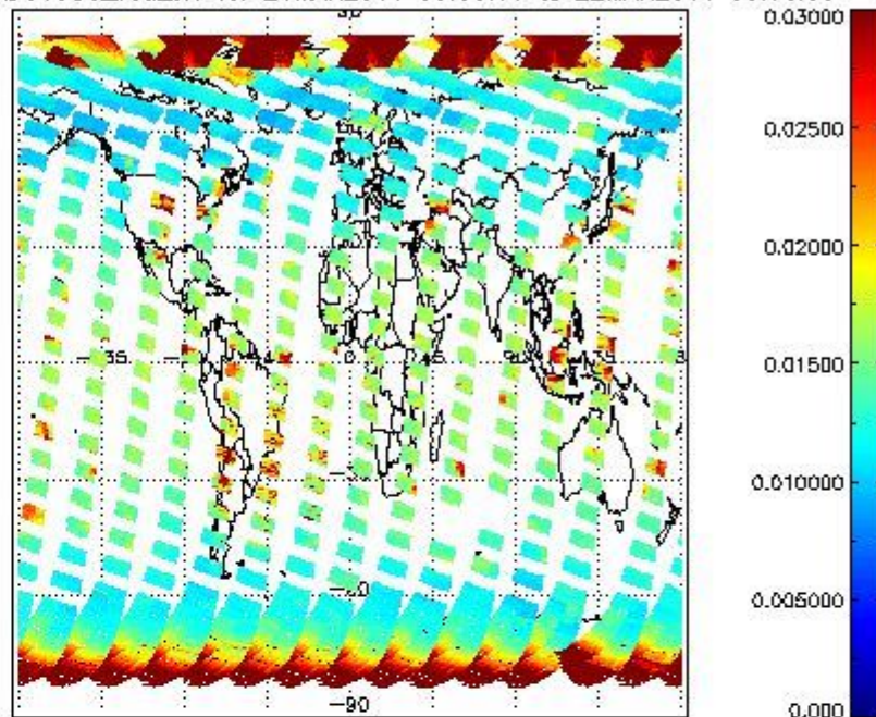
SCIOL2P_NADUV003_vcd_err for 21MAR2011 00:00:00 to 22MAR2011 00:00:00
