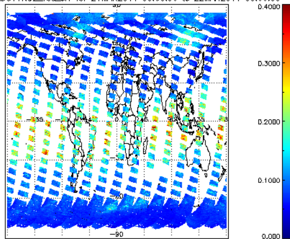
SCIOL2P_NADUV1NO2_vcd_err for 21MAR2011 00:00:00 to 22MAR2011 00:00:00
