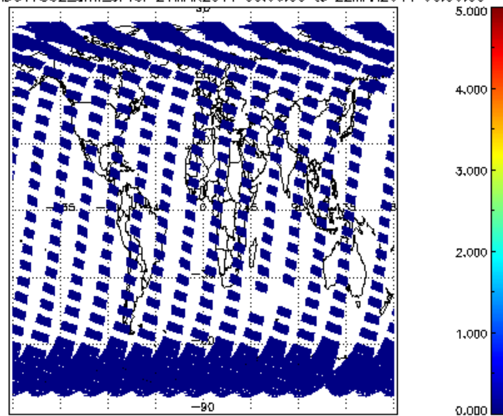
SCIOL2P_NADUV7S02_amf_cl for 21MAR2011 00:00:00 to 22MAR2011 00:00:00
