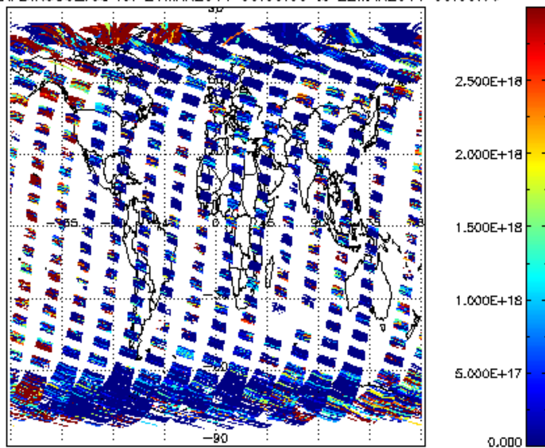
SCIOL2P_NADIR3CO_vcd for 21MAR2011 00:00:00 to 22MAR2011 00:00:00
