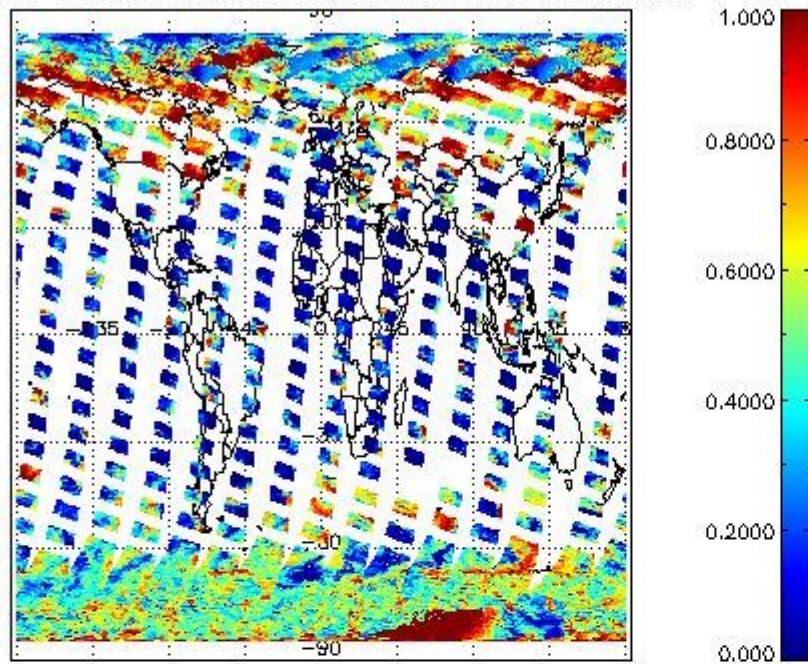
cL_frac for 21MAR2011 00:00:00 to 22MAR2011 00:00:00
