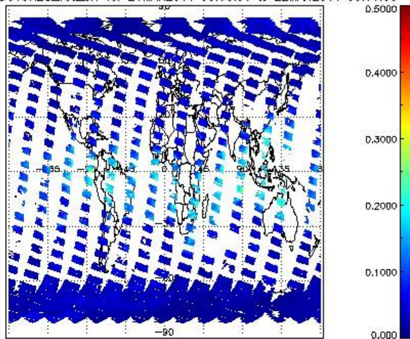
SCIOL2P_NADUV8H2O_vcd_err for 21MAR2011 00:00:00 to 22MAR2011 00:00:00
