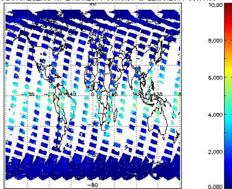
SCIOL2P_NADUV8H2O_vcd for 21MAR2011 00:00:00 to 22MAR2011 00:00:00
