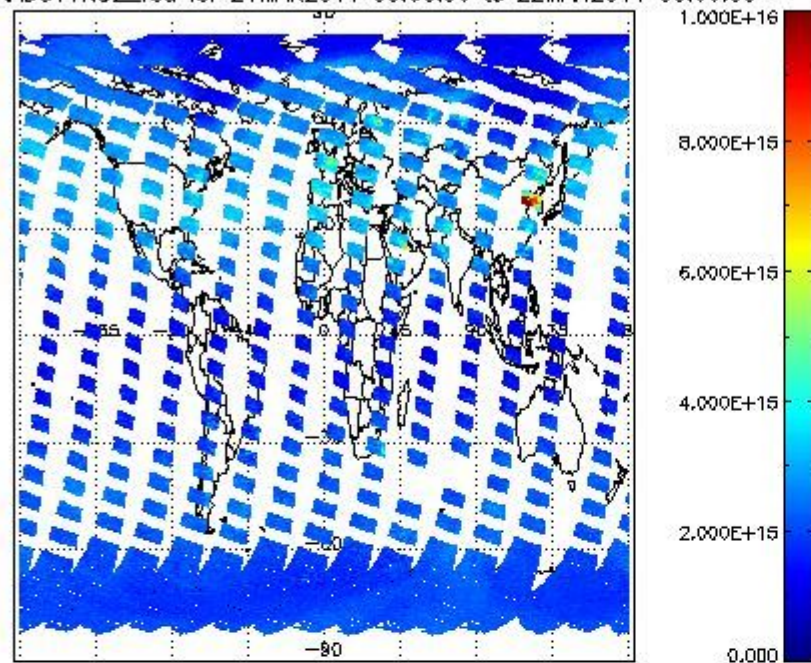
SCIOL2P_NADUV1NO2_vcd for 21MAR2011 00:00:00 to 22MAR2011 00:00:00
