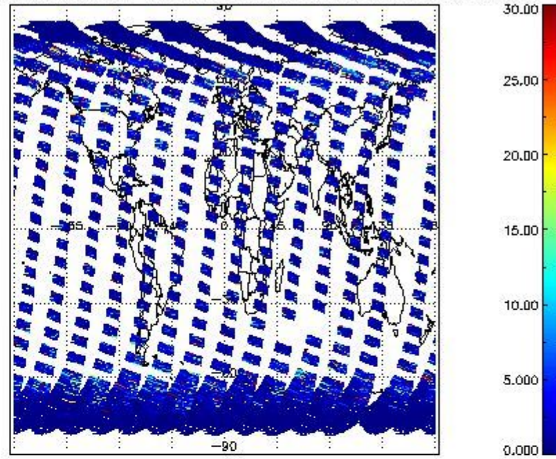
SCIOL2P_NADUV7S02_vcd_err for 21MAR2011 00:00:00 to 22MAR2011 00:00:00
