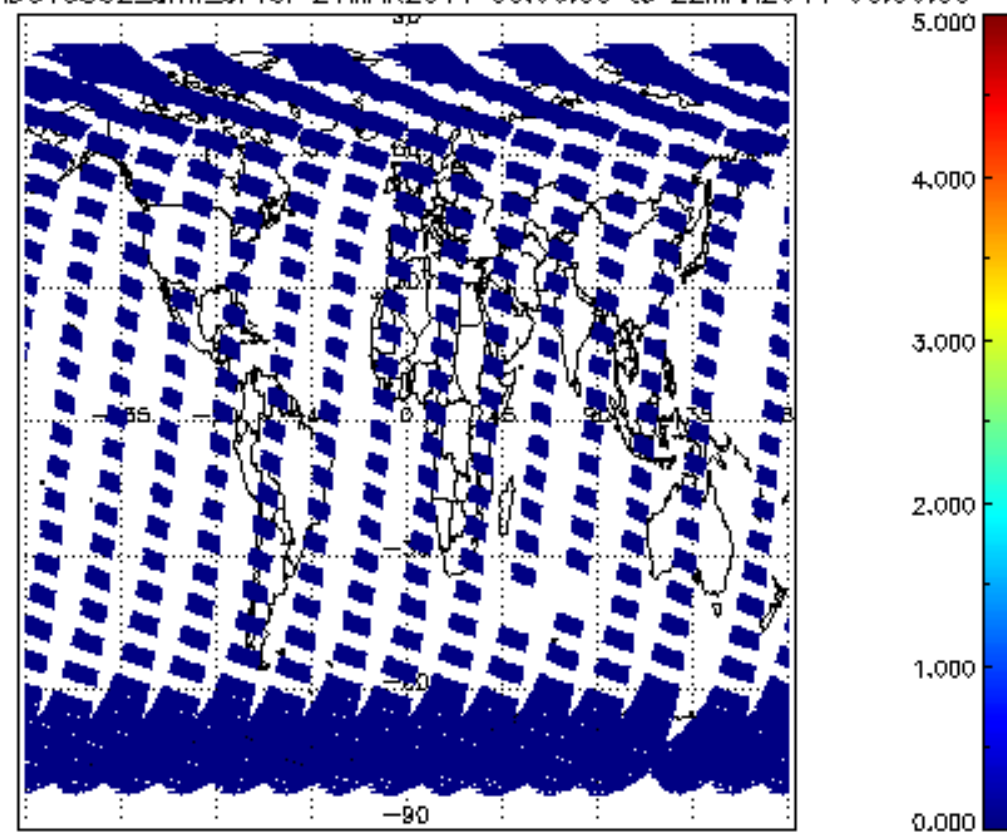
SCIOL2P_NADUV5S02_amf_cl for 21MAR2011 00:00:00 to 22MAR2011 00:00:00
