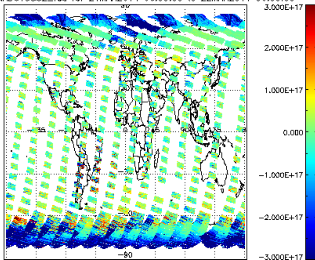
SCIOL2P_NADUV5S02_vcd for 21MAR2011 00:00:00 to 22MAR2011 00:00:00
