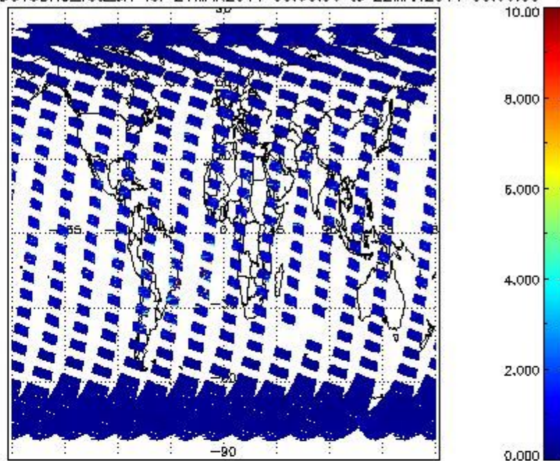
SCIOL2P_NADUV3BRO_vcd_err for 21MAR2011 00:00:00 to 22MAR2011 00:00:00
