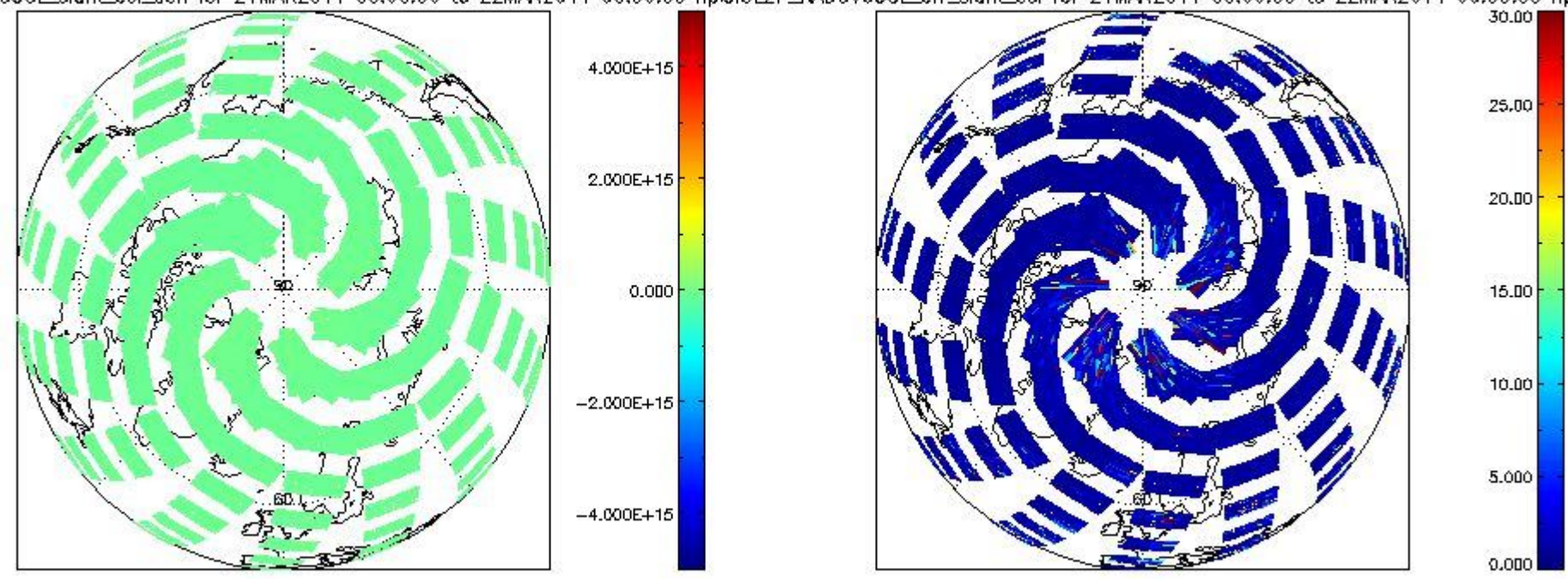
CIOL2P_NADUV6OCLslant_col_den for 21MAR2011 00:00:00 to 22MAR2011 00:00:00 npCIOL2P_NADUV6OCLerr_slant_col for 21MAR2011 00:00:00 to 22MAR2011 00:00:00 np
