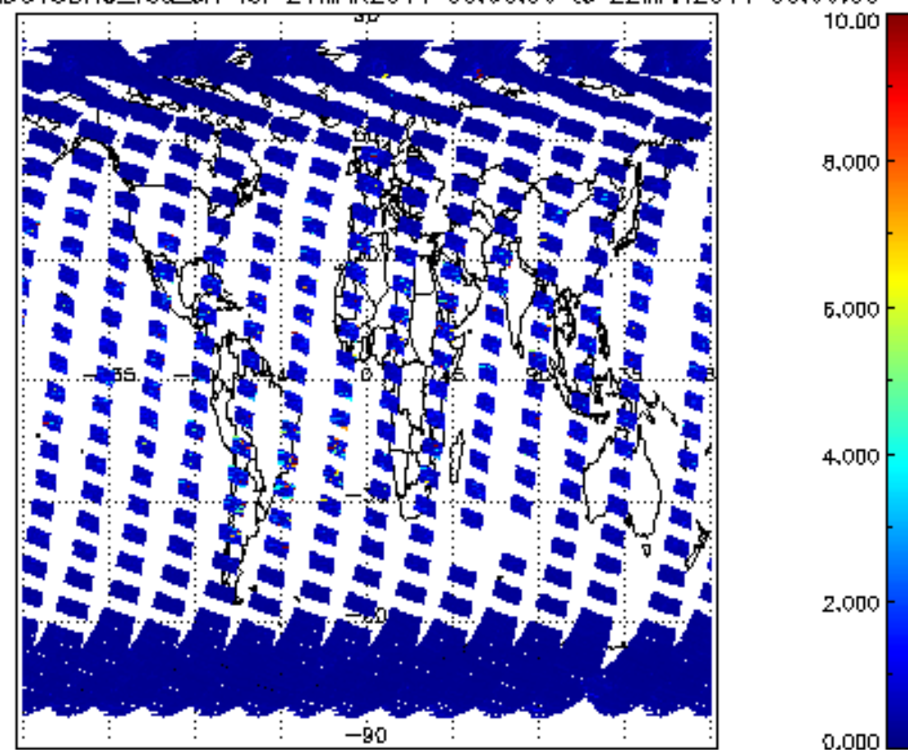
SCIOL2P_NADUV3BRO_vcd_err for 21MAR2011 00:00:00 to 22MAR2011 00:00:00
