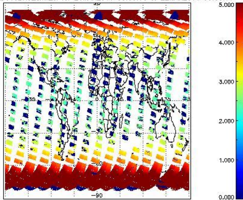
SCIOL2P_NADUV3BRO_amf_cl for 21MAR2011 00:00:00 to 22MAR2011 00:00:00
