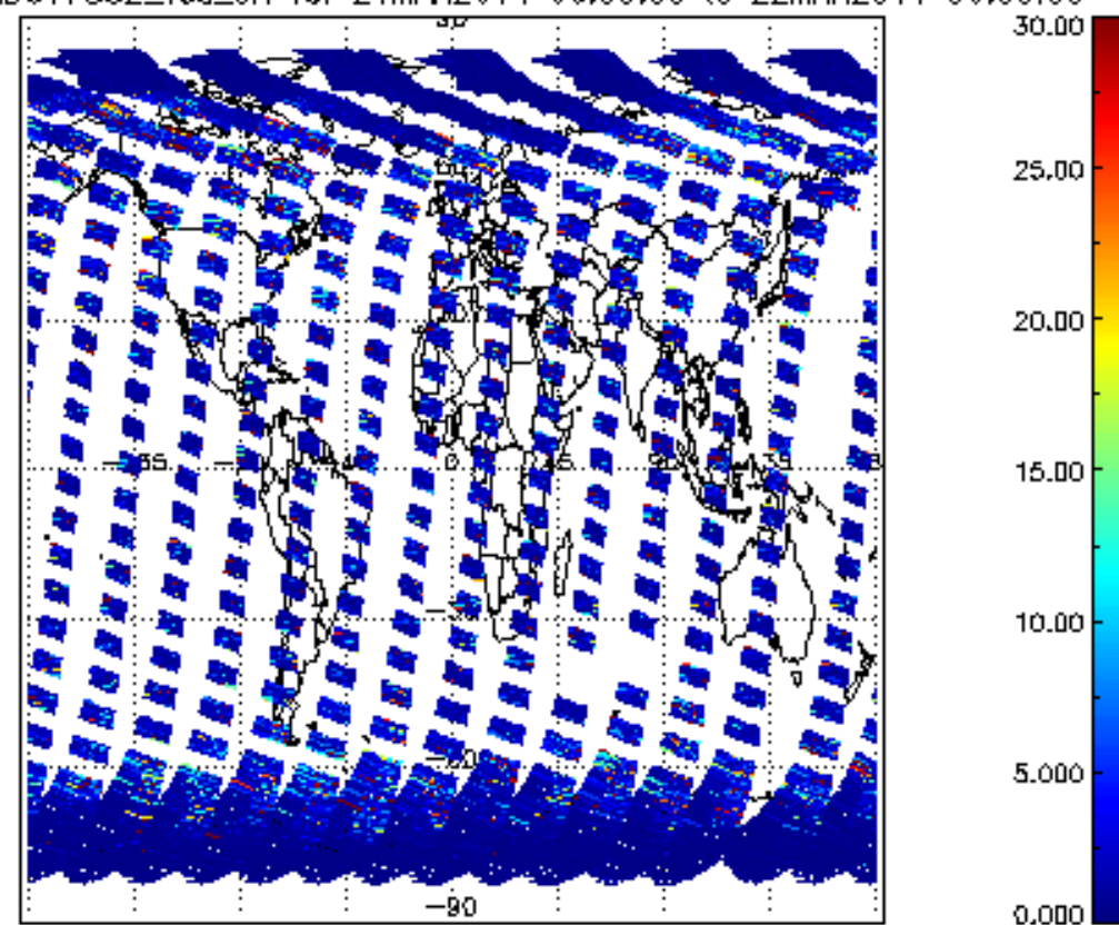
SCIOL2P_NADUV7S02_vcd_err for 21MAR2011 00:00:00 to 22MAR2011 00:00:00
