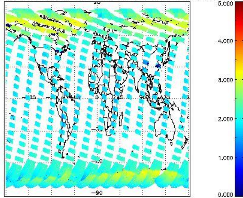
SCIOL2P_NADUV7S02_amf_gr for 21MAR2011 00:00:00 to 22MAR2011 00:00:00
