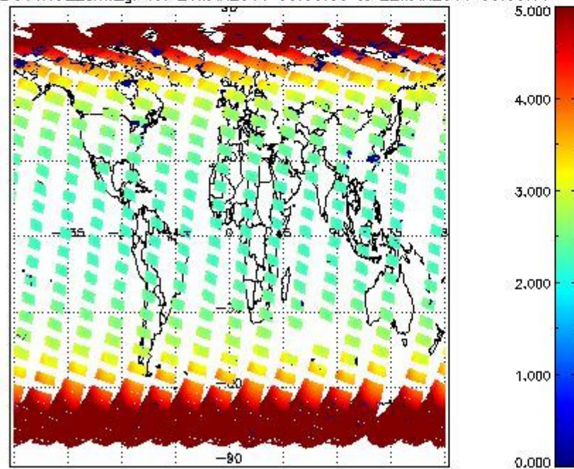
SCIOL2P_NADUV1NO2_amf_gr for 21MAR2011 00:00:00 to 22MAR2011 00:00:00
