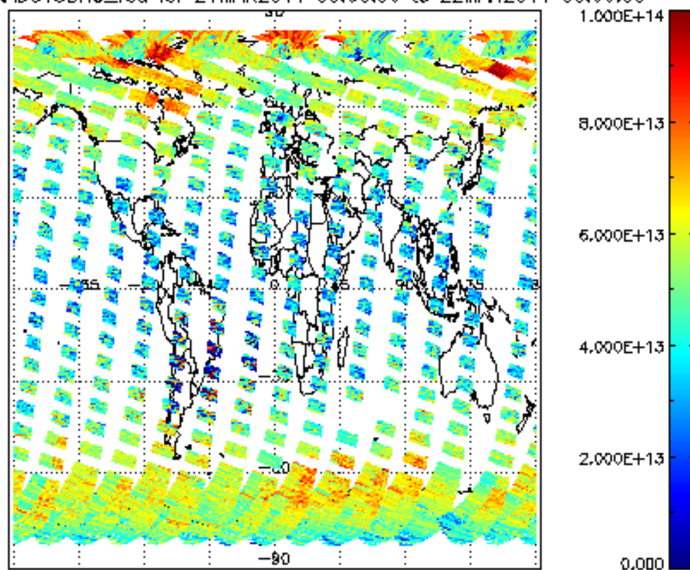
SCIOL2P_NADUV3BRO_vcd for 21MAR2011 00:00:00 to 22MAR2011 00:00:00
