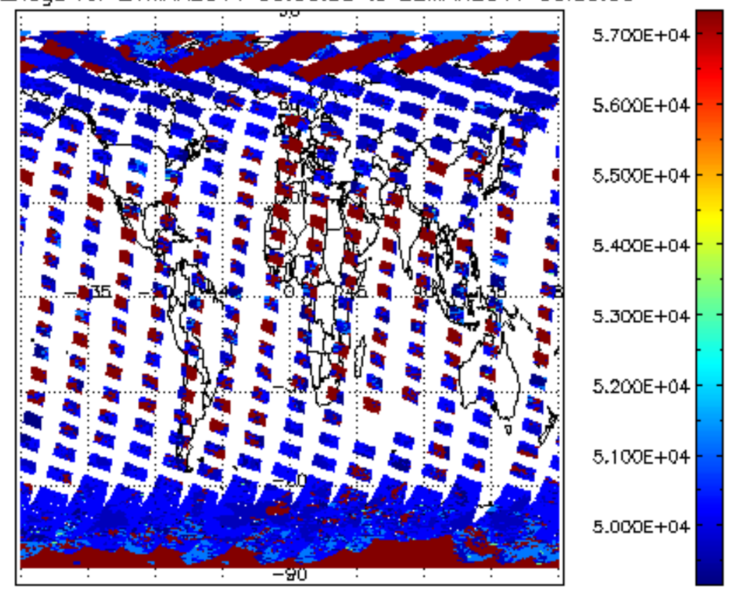
cloud_flags for 21MAR2011 00:00:00 to 22MAR2011 00:00:00
