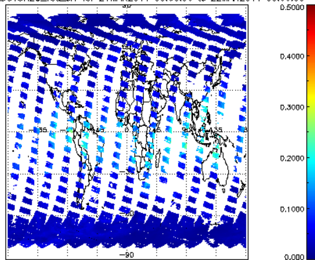
SCIOL2P_NADUV8H20_vcd_err for 21MAR2011 00:00:00 to 22MAR2011 00:00:00
