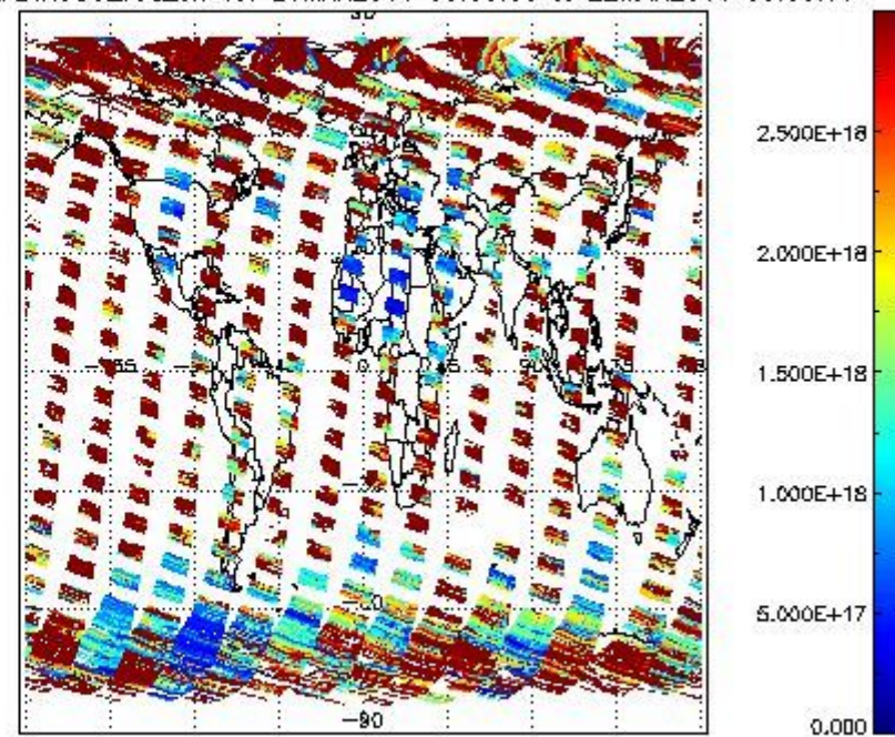
SCIDL2P_NADIR3CO_vcd_err for 21MAR2011 00:00:00 to 22MAR2011 00:00:00
