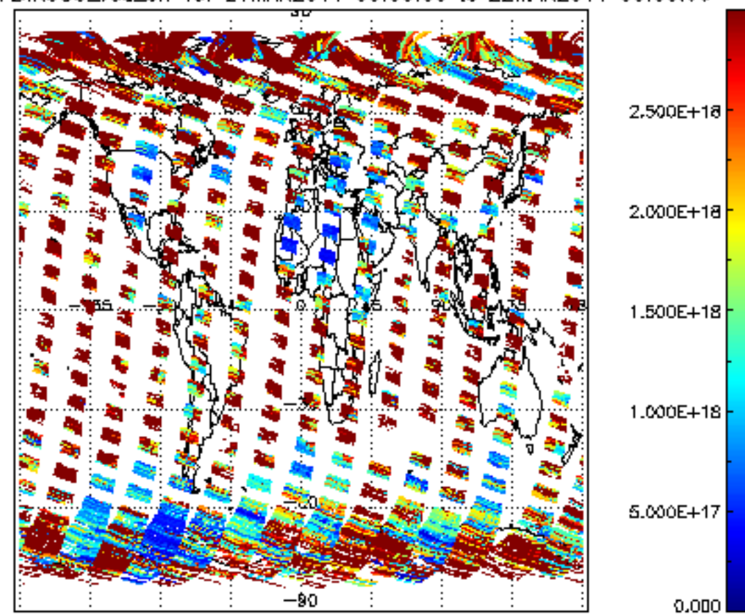
SCIOL2P_NADIR3CO_vcd_err for 21MAR2011 00:00:00 to 22MAR2011 00:00:00
