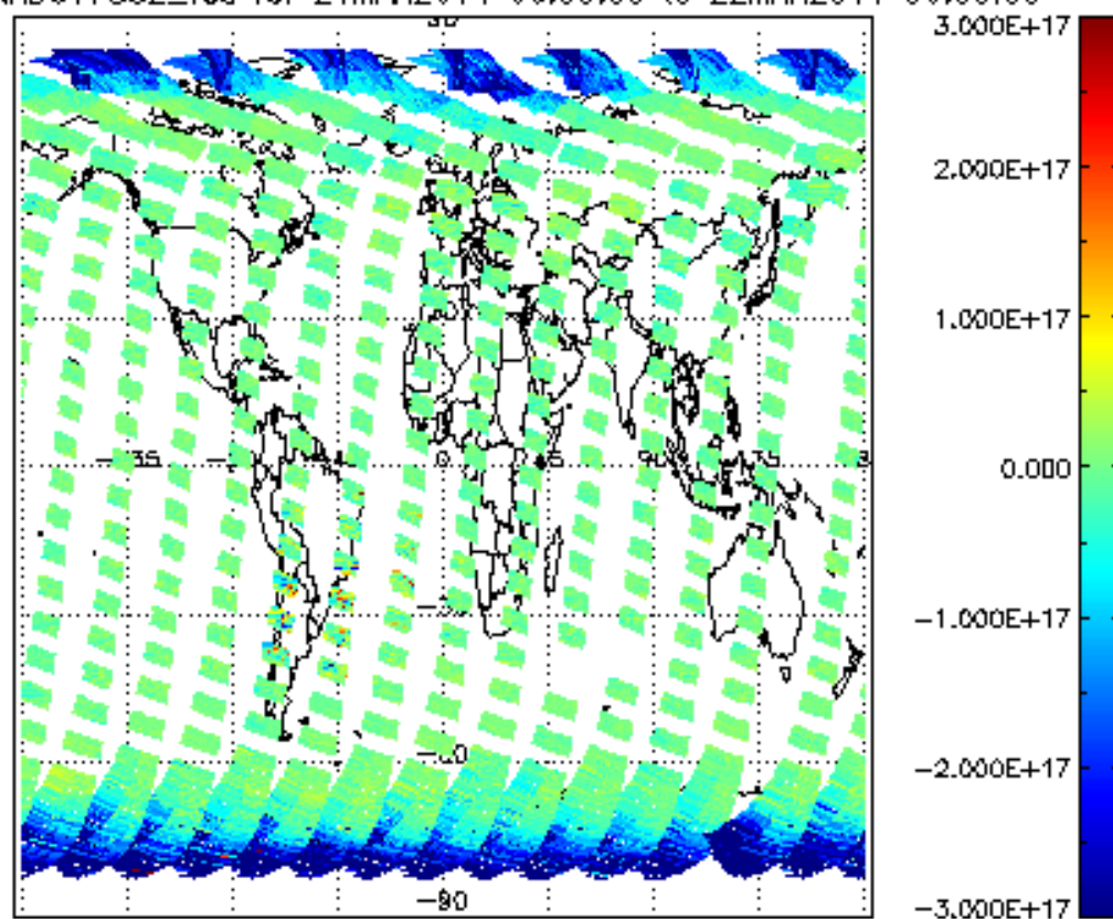
SCIOL2P_NADUV7S02_vcd for 21MAR2011 00:00:00 to 22MAR2011 00:00:00
