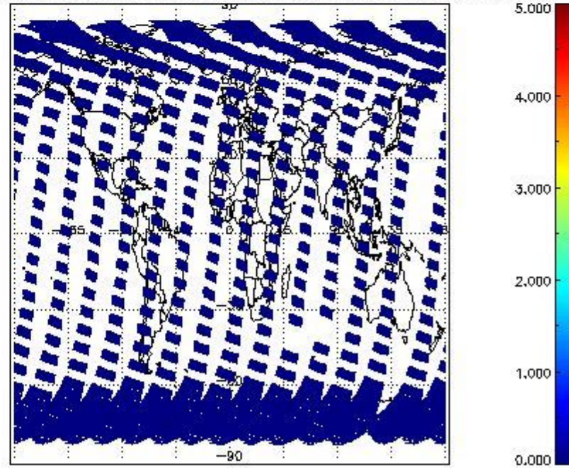
SCIOL2P_NADUV7S02_amf_cl for 21MAR2011 00:00:00 to 22MAR2011 00:00:00
