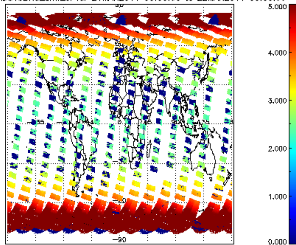
SCIOL2P_NADUV3BRO_amf_cl for 21MAR2011 00:00:00 to 22MAR2011 00:00:00
