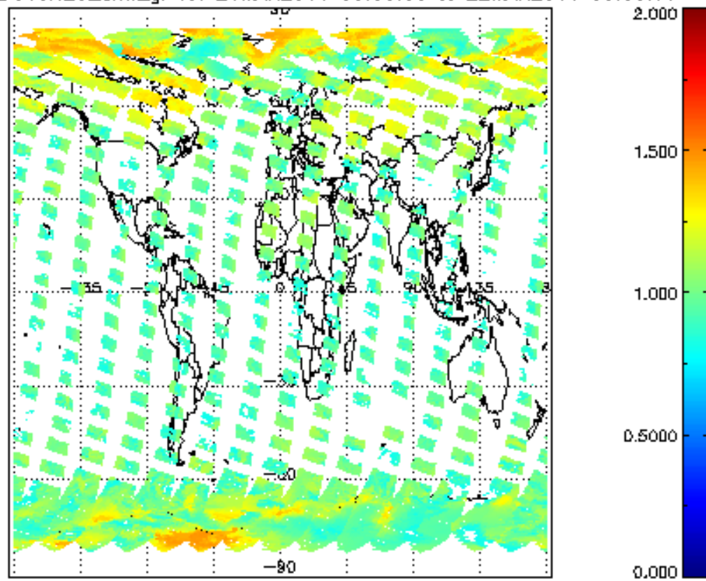
SCIOL2P_NADUV8H20_arnf_gr for 21MAR2011 00:00:00 to 22MAR2011 00:00:00
