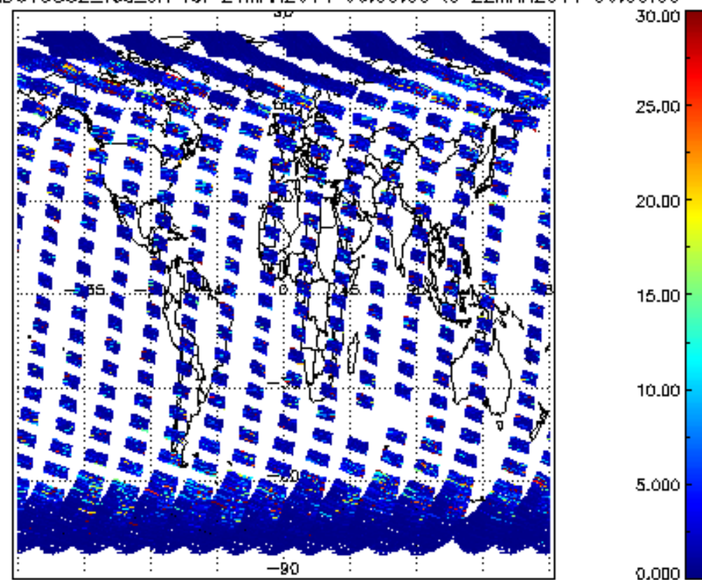
SCIOL2P_NADUV5S02_vcd_err for 21MAR2011 00:00:00 to 22MAR2011 00:00:00
