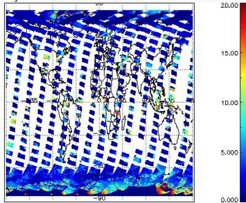
cL_top_height for 21MAR2011 00:00:00 to 22MAR2011 00:00:00
