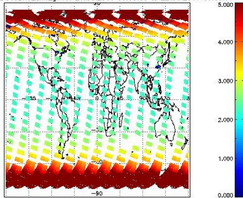
SCIOL2P_NADUV3BRO_amf_gr for 21MAR2011 00:00:00 to 22MAR2011 00:00:00
