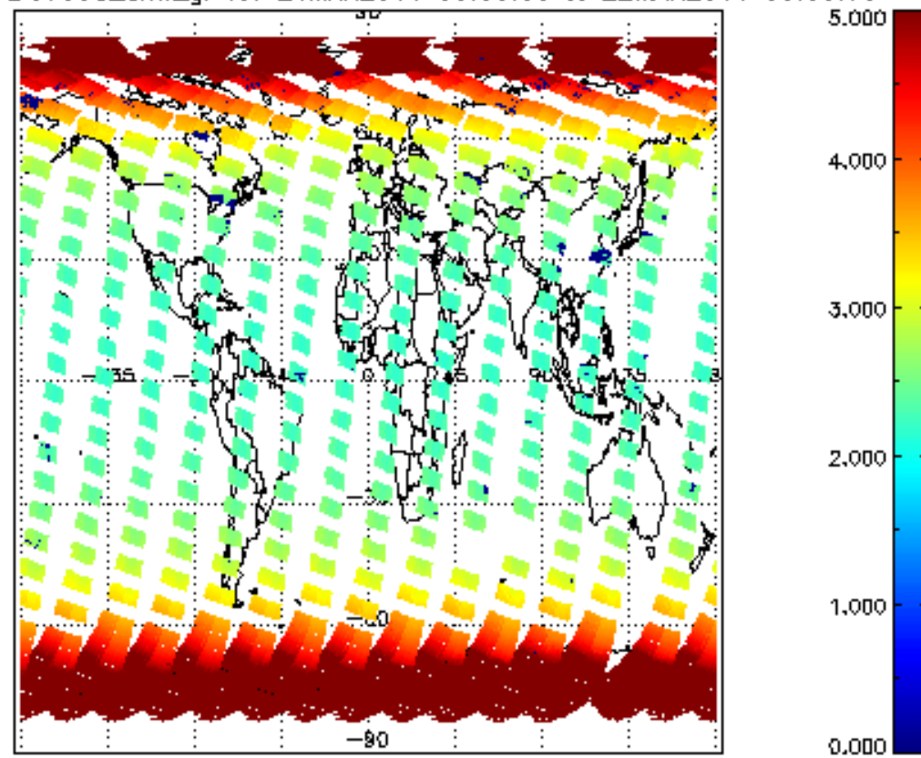
SCIOL2P_NADUV003_amf_gr for 21MAR2011 00:00:00 to 22MAR2011 00:00:00
