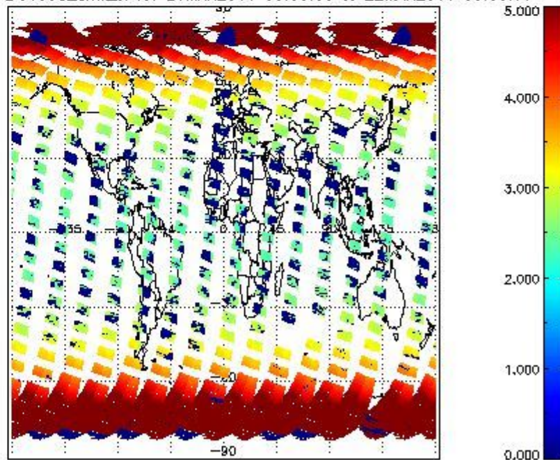
SCIOL2P_NADUV003_amf_cl for 21MAR2011 00:00:00 to 22MAR2011 00:00:00
