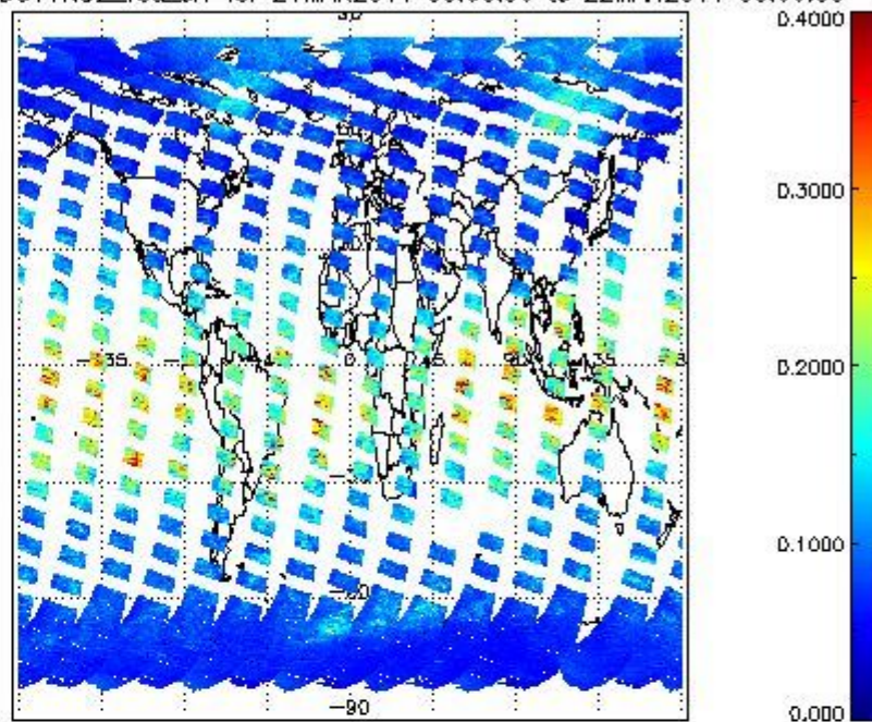
SCIOL2P_NADUV1NO2_vcd_err for 21MAR2011 00:00:00 to 22MAR2011 00:00:00
