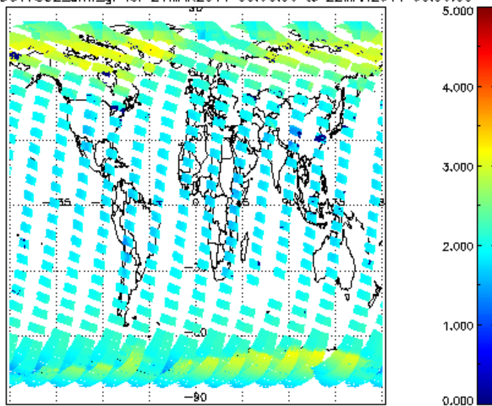
SCIOL2P_NADUV7S02_amf_gr for 21MAR2011 00:00:00 to 22MAR2011 00:00:00
