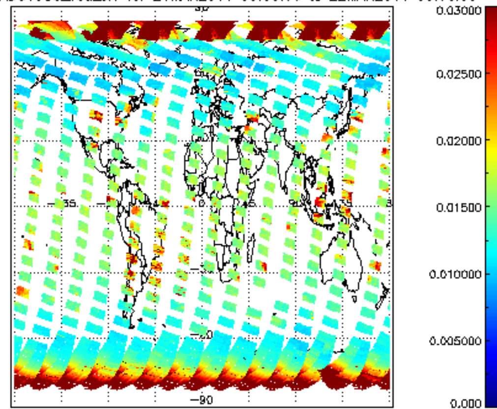
SCIOL2P_NADUV003_vcd_err for 21MAR2011 00:00:00 to 22MAR2011 00:00:00
