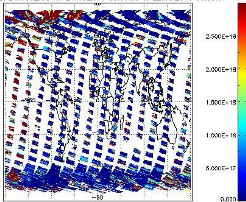
SCIDL2P_NADIR3CO_vcd for 21MAR2011 00:00:00 to 22MAR2011 00:00:00
