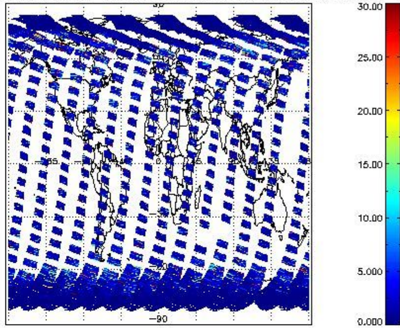
SCIOL2P_NADUV5S02_vcd_err for 21MAR2011 00:00:00 to 22MAR2011 00:00:00
