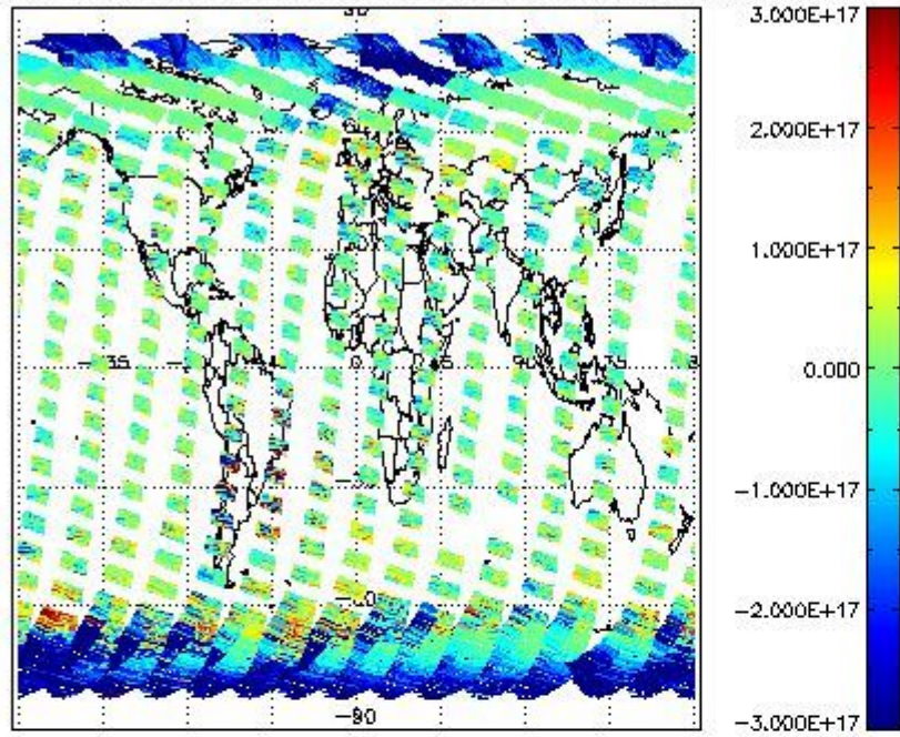
SCIOL2P_NADUV5S02_vcd for 21MAR2011 00:00:00 to 22MAR2011 00:00:00
