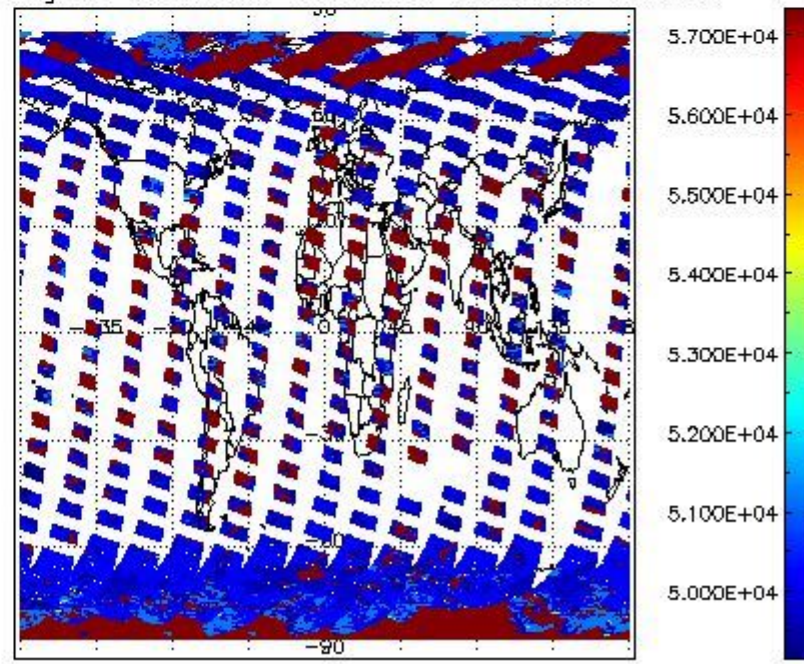
cloud_flags for 21MAR2011 00:00:00 to 22MAR2011 00:00:00
