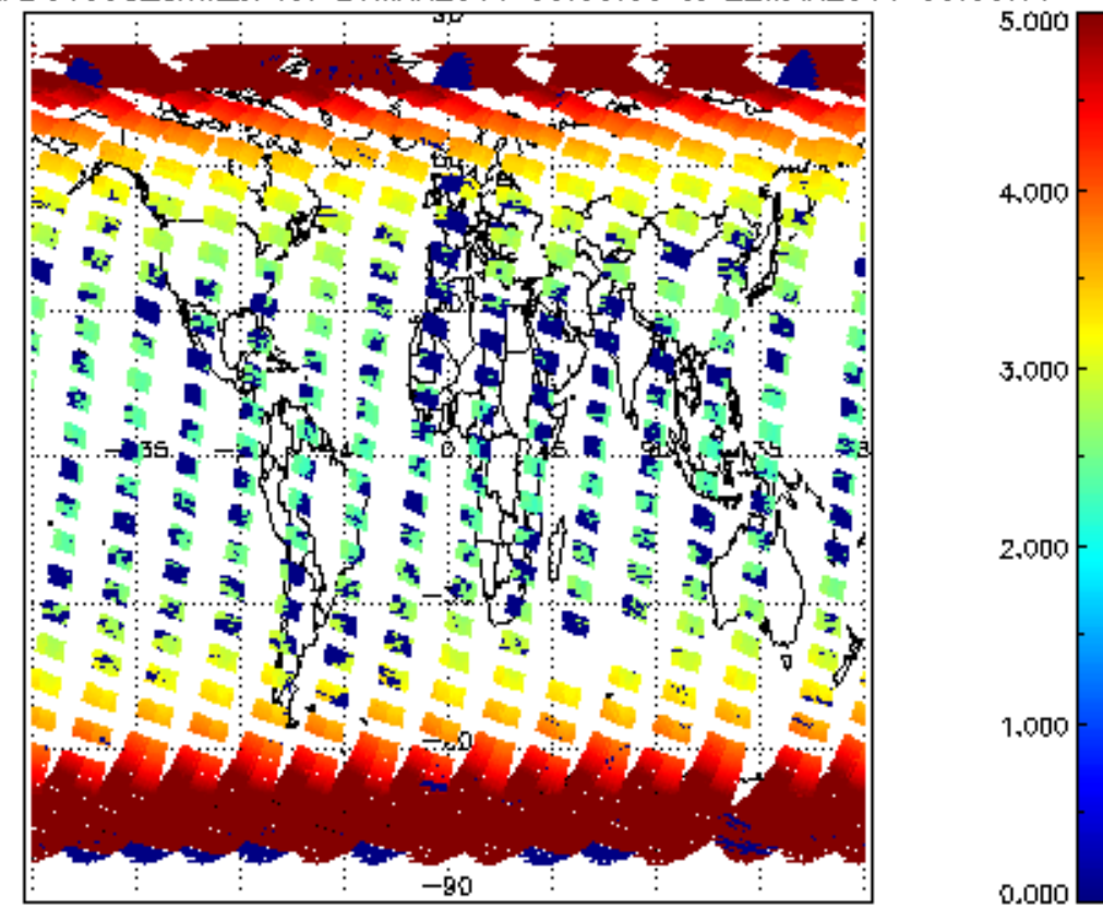
SCIOL2P_NADUV003_amf_cl for 21MAR2011 00:00:00 to 22MAR2011 00:00:00
