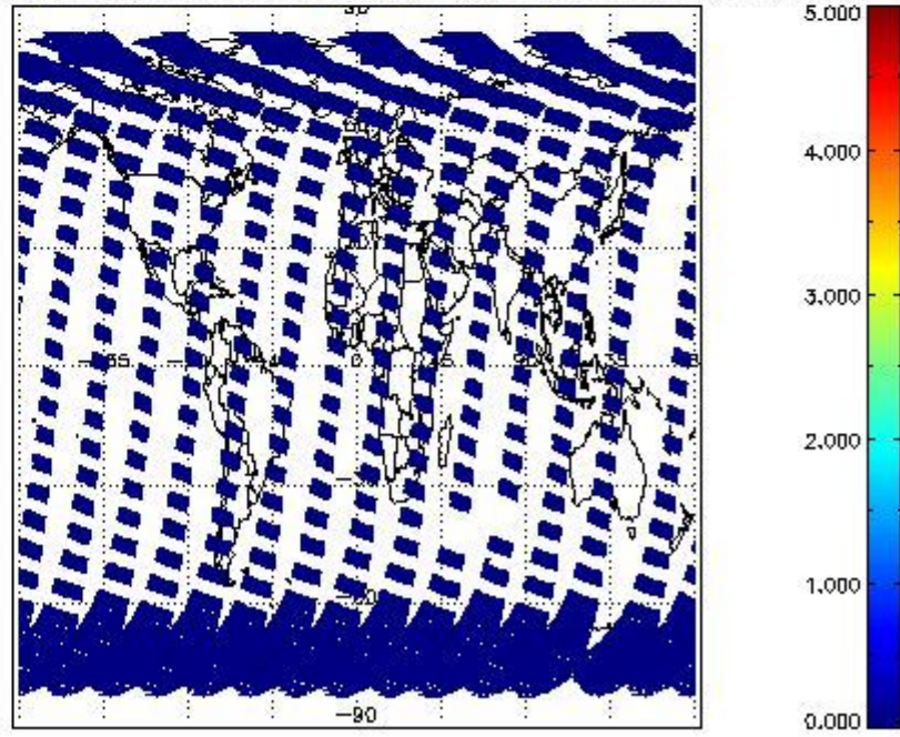
SCIOL2P_NADUV5S02_amf_cl for 21MAR2011 00:00:00 to 22MAR2011 00:00:00
