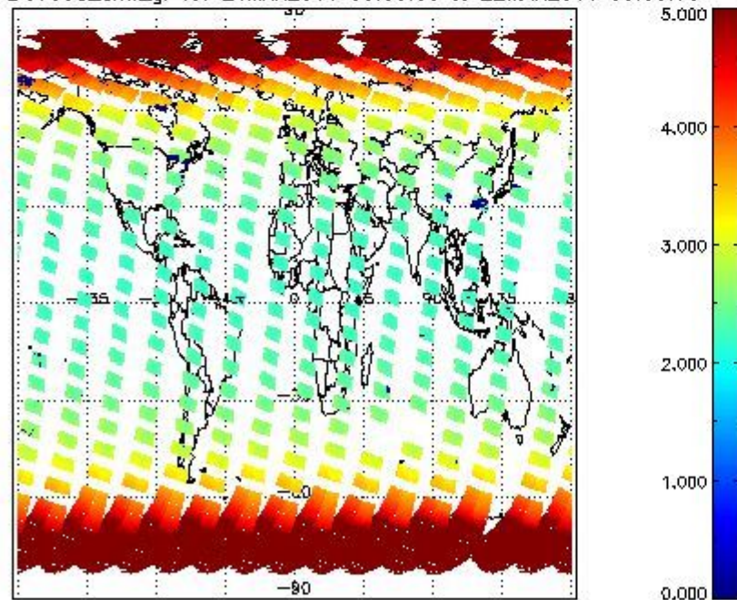
SCIOL2P_NADUV003_amf_gr for 21MAR2011 00:00:00 to 22MAR2011 00:00:00
