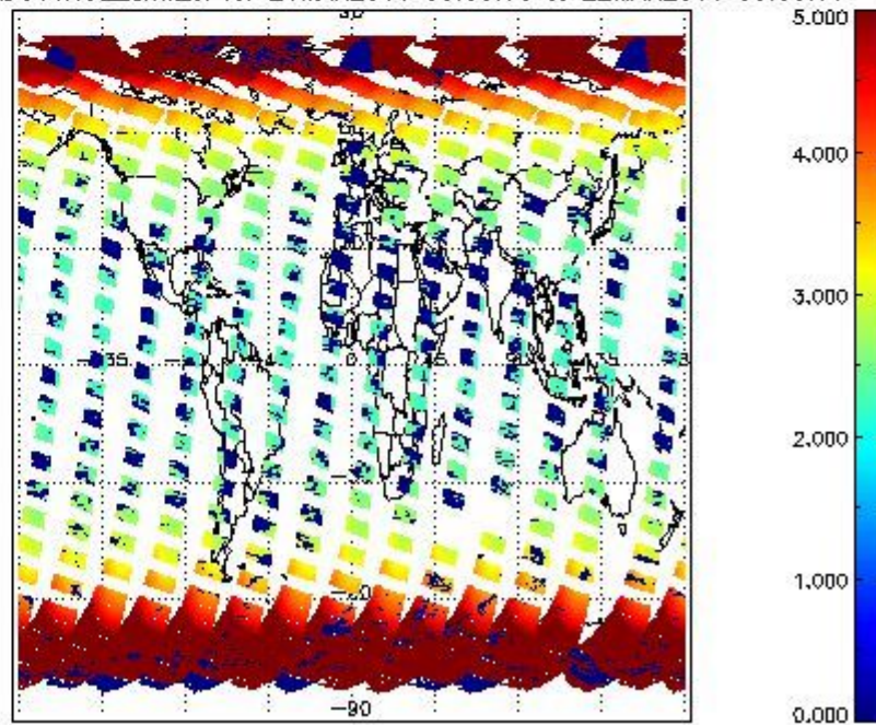
SCIOL2P_NADUV1NO2_amf_cl for 21MAR2011 00:00:00 to 22MAR2011 00:00:00
