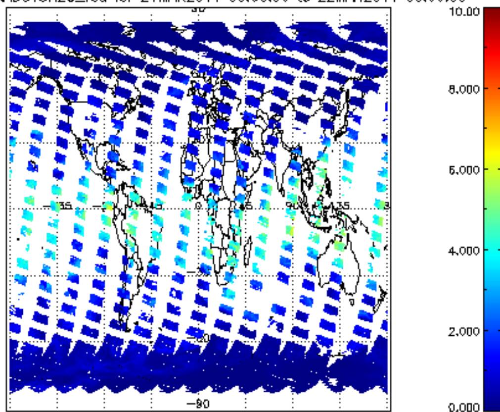
SCIOL2P_NADUV8H20_vcd for 21MAR2011 00:00:00 to 22MAR2011 00:00:00
