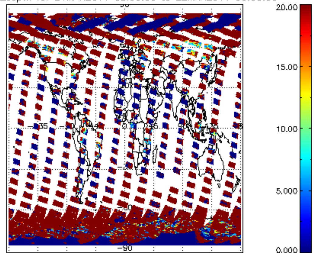
cL_opt_depth for 21MAR2011 00:00:00 to 22MAR2011 00:00:00
