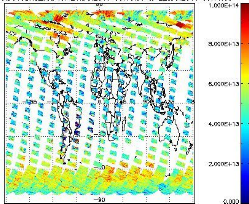
SCIOL2P_NADUV3BRO_vcd for 21MAR2011 00:00:00 to 22MAR2011 00:00:00
