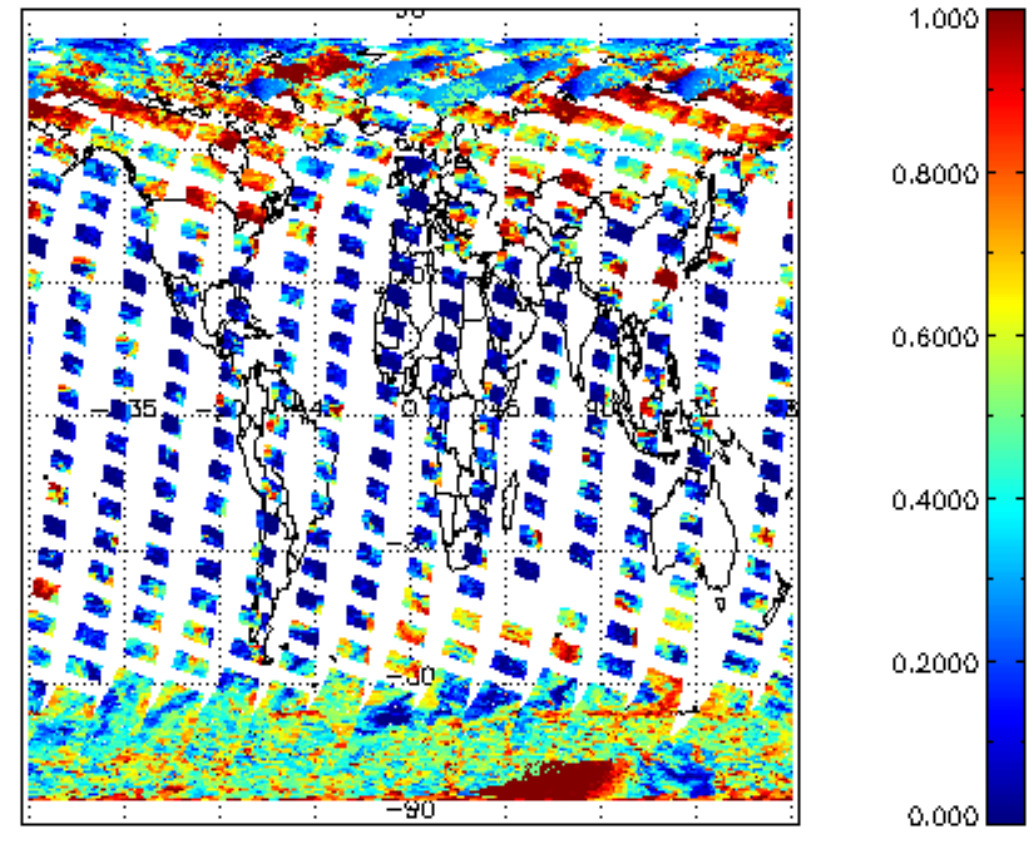
cL_frac for 21MAR2011 00:00:00 to 22MAR2011 00:00:00
