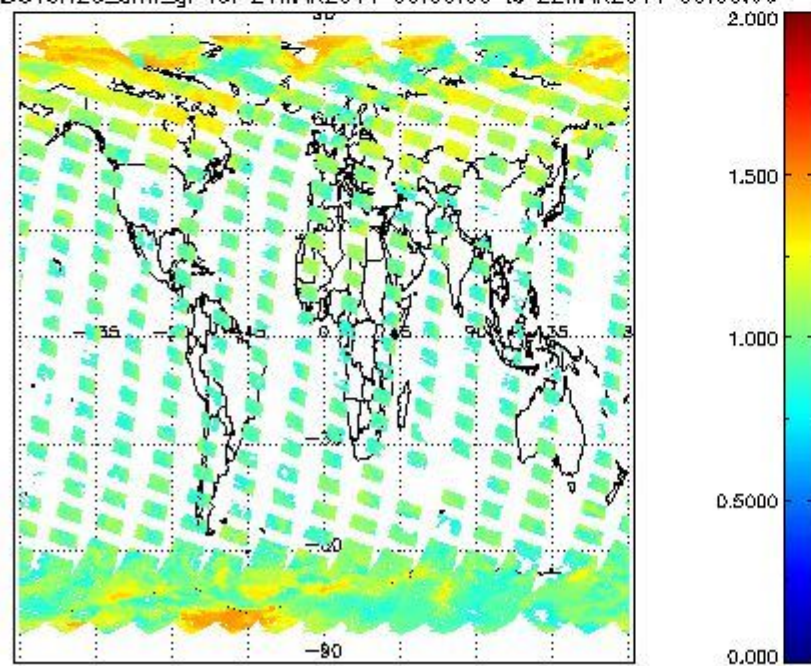
SCIOL2P_NADUV8H2O_amb_gr for 21MAR2011 00:00:00 to 22MAR2011 00:00:00
