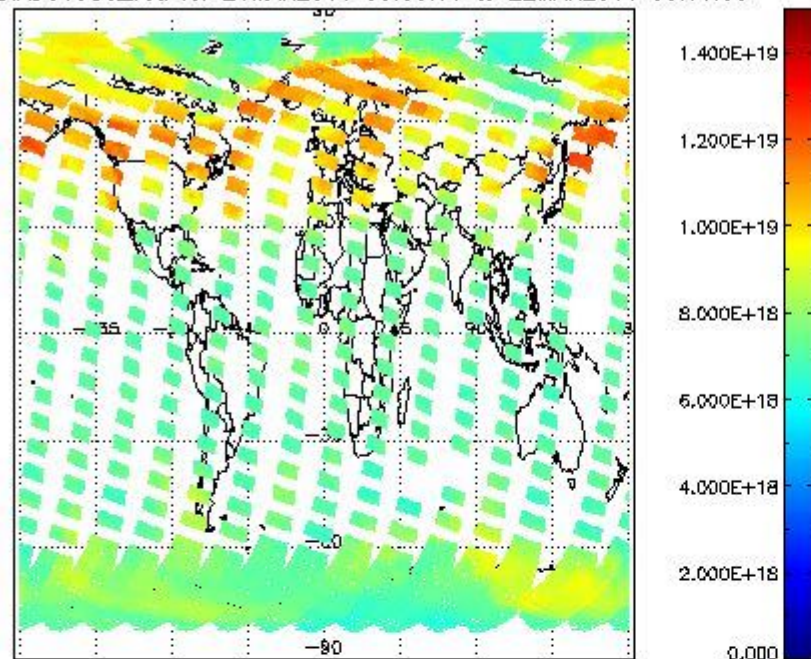
SCIOL2P_NADUV003_vcd for 21MAR2011 00:00:00 to 22MAR2011 00:00:00
