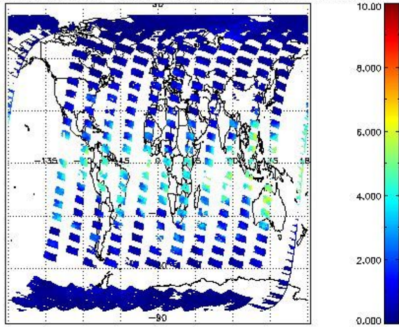
SCIOL2P_NADUV8H2O_vcd for 18MAR2011 00:00:00 to 19MAR2011 00:00:00
