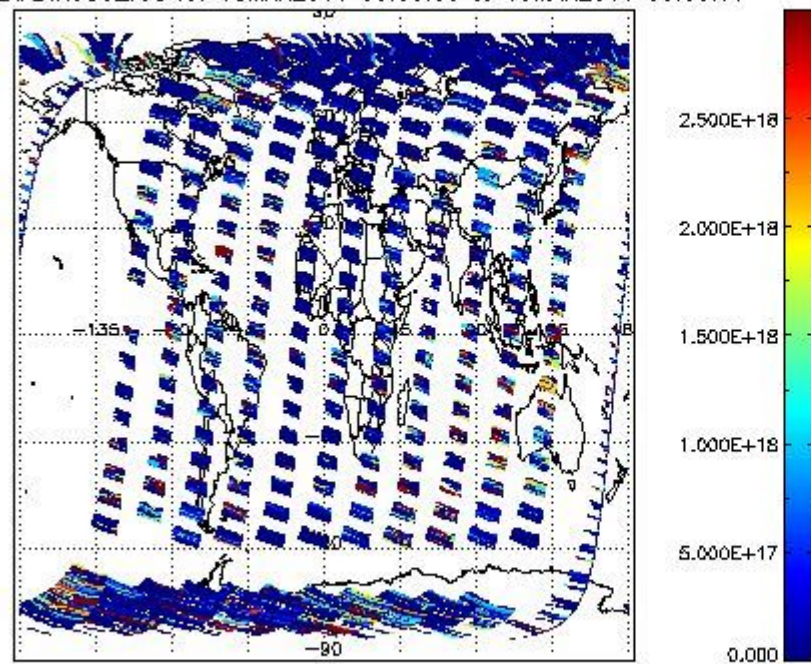
SCIOL2P_NADIR3CO_vcd for 18MAR2011 00:00:00 to 19MAR2011 00:00:00
