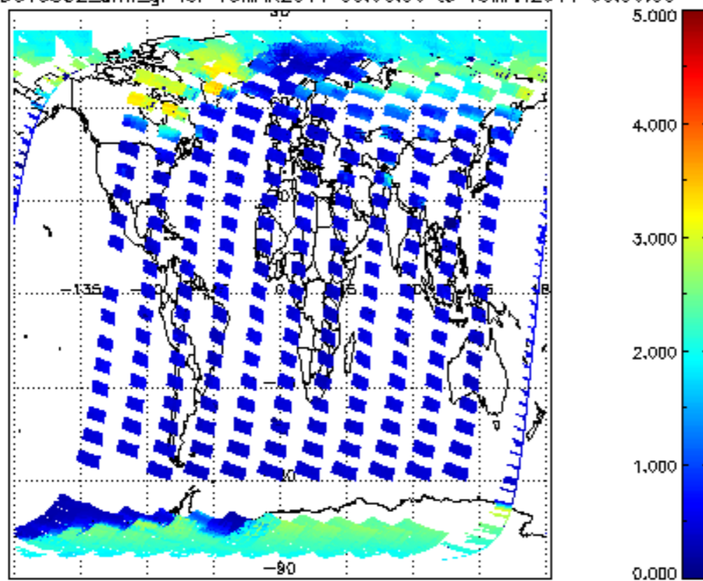
SCIOL2P_NADUV5S02_amf_gr for 18MAR2011 00:00:00 to 19MAR2011 00:00:00
