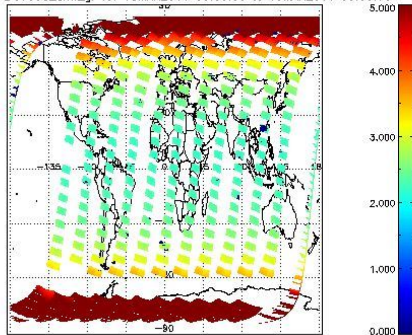
SCIOL2P_NADUV003_amf_gr for 18MAR2011 00:00:00 to 19MAR2011 00:00:00
