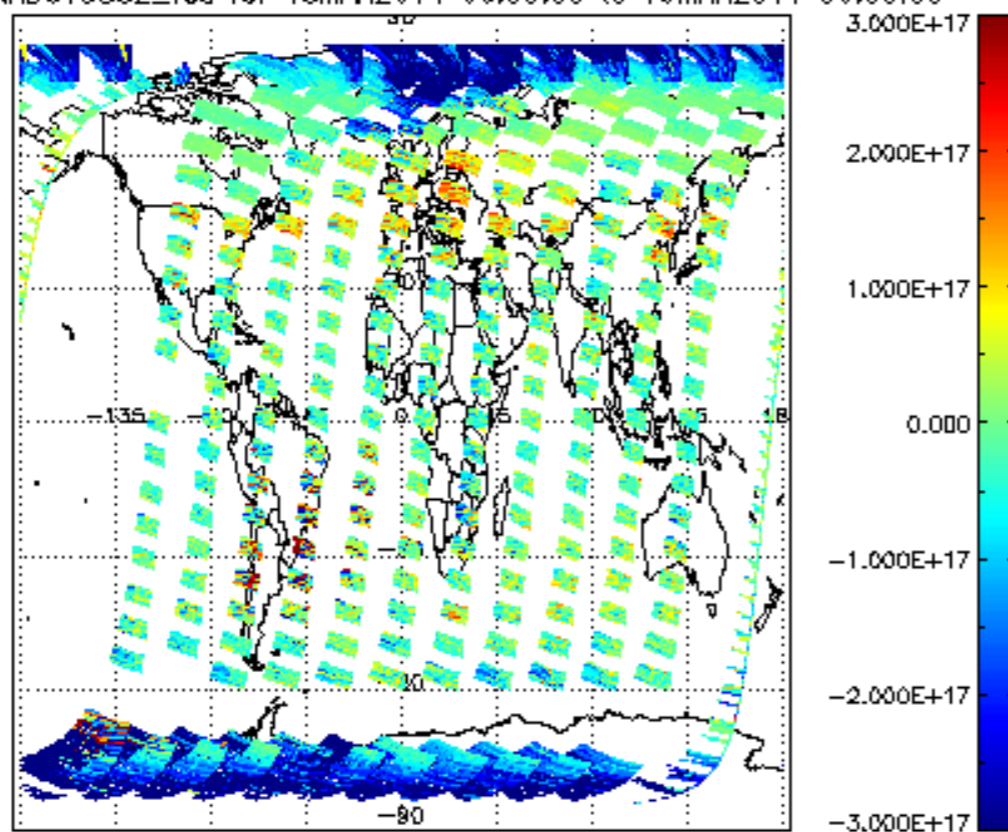
SCIOL2P_NADUV5S02_vcd for 18MAR2011 00:00:00 to 19MAR2011 00:00:00
