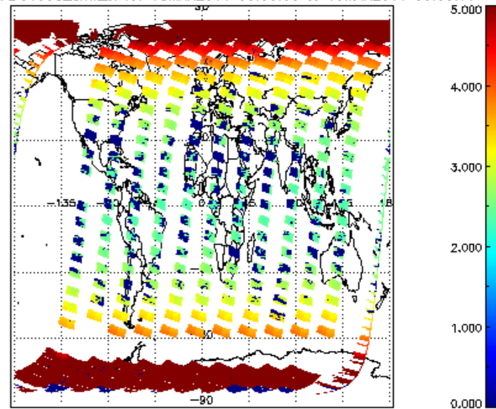
SCIOL2P_NADUV003_amf_cl for 18MAR2011 00:00:00 to 19MAR2011 00:00:00
