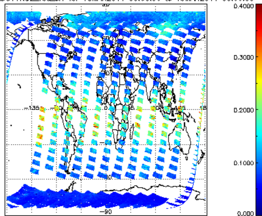
SCIOL2P_NADUV1NO2_vcd_err for 18MAR2011 00:00:00 to 19MAR2011 00:00:00
