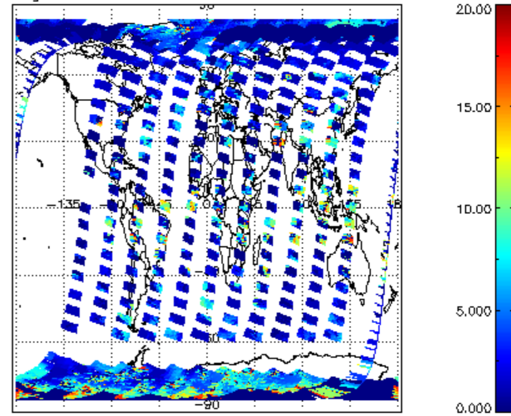
cL_top_height for 18MAR2011 00:00:00 to 19MAR2011 00:00:00
