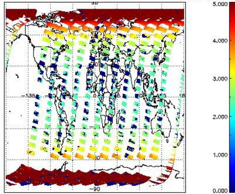
SCIOL2P_NADUV1NO2_amf_cl for 18MAR2011 00:00:00 to 19MAR2011 00:00:00
