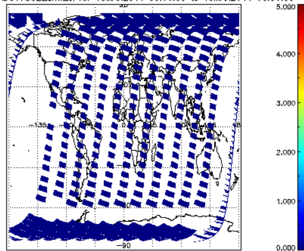
SCIOL2P_NADUV7S02_amf_cl for 18MAR2011 00:00:00 to 19MAR2011 00:00:00
