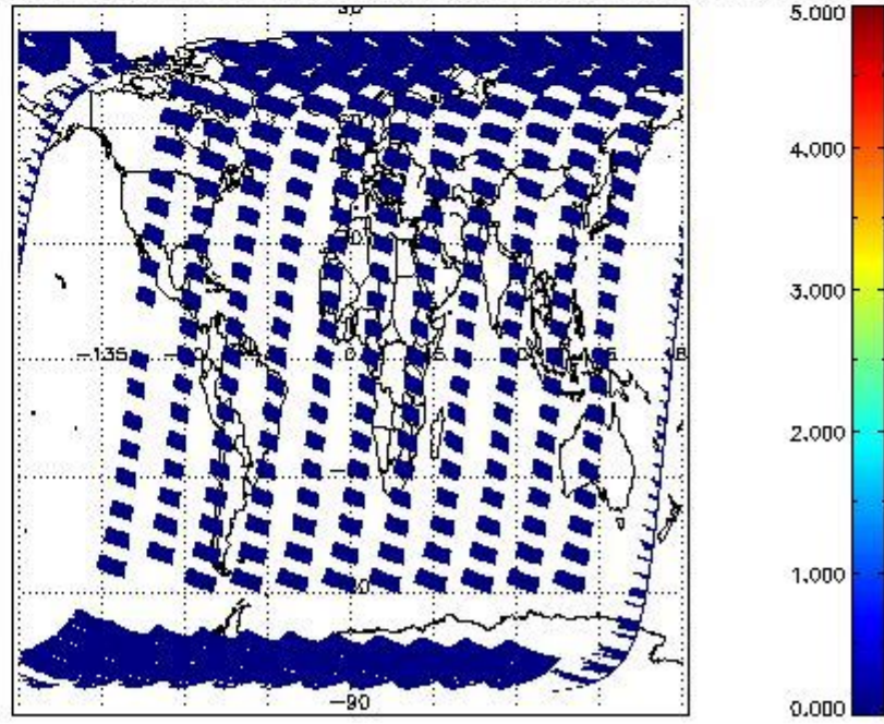
SCIOL2P_NADUV5SO2_amf_cl for 18MAR2011 00:00:00 to 19MAR2011 00:00:00
