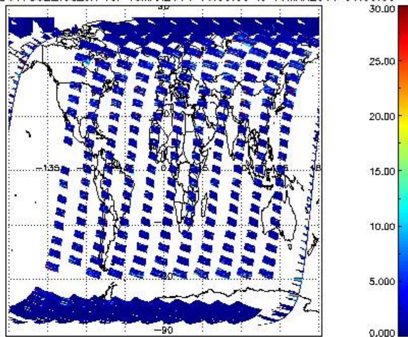
SCIOL2P_NADUV7S02_vcd_err for 18MAR2011 00:00:00 to 19MAR2011 00:00:00
