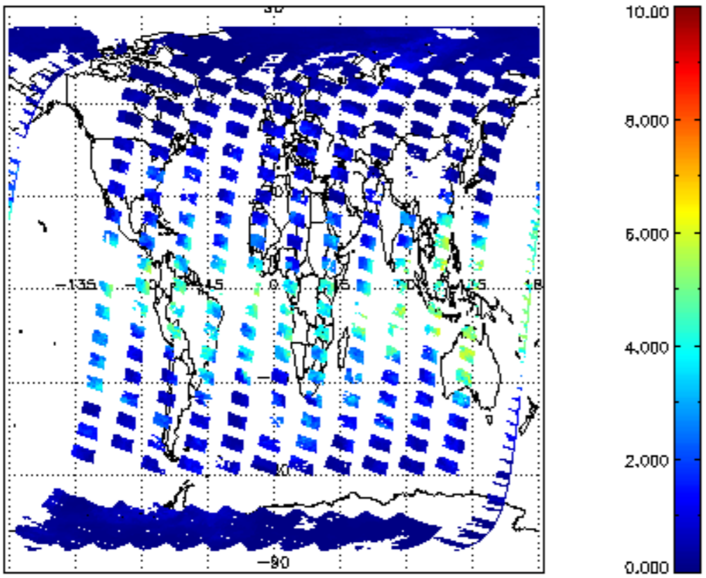
SCIOL2P_NADUV8H20_vcd for 18MAR2011 00:00:00 to 19MAR2011 00:00:00
