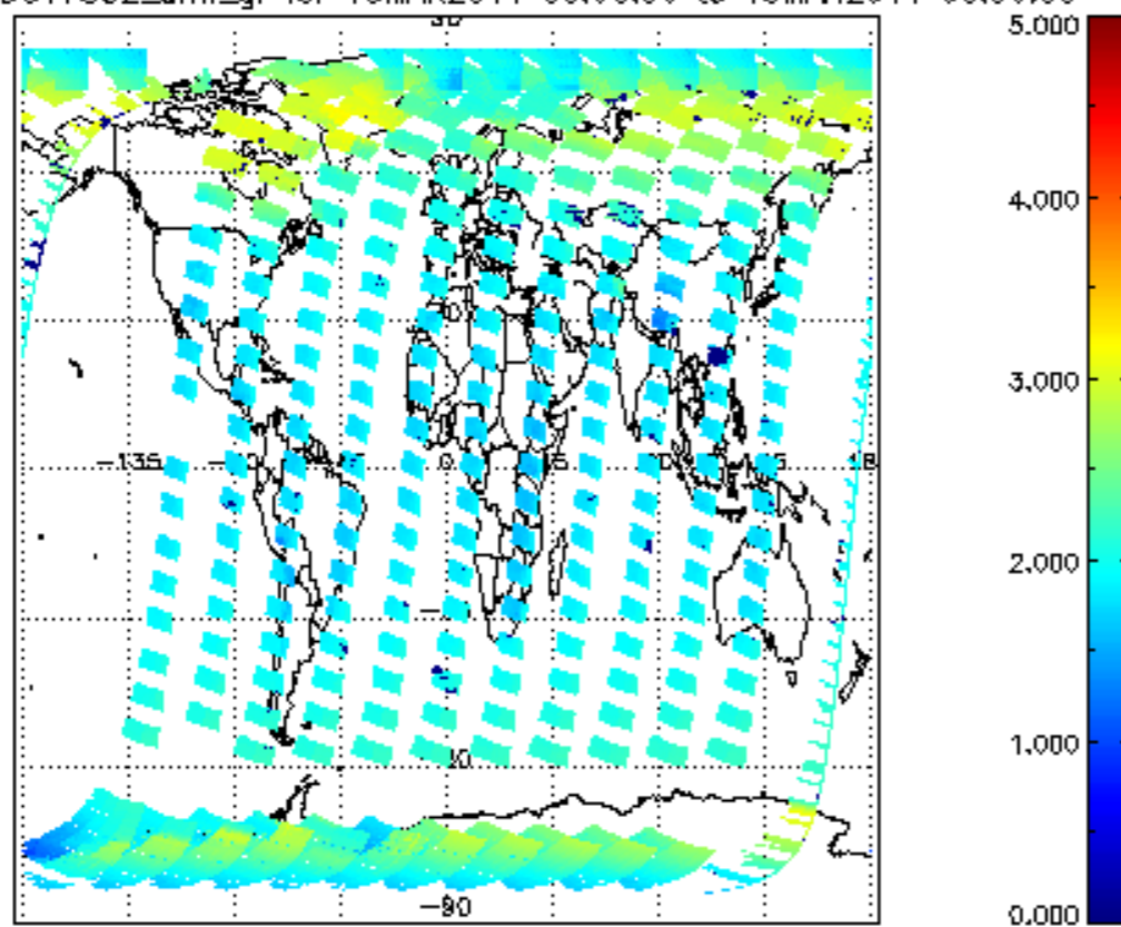
SCIOL2P_NADUV7S02_amf_gr for 18MAR2011 00:00:00 to 19MAR2011 00:00:00
