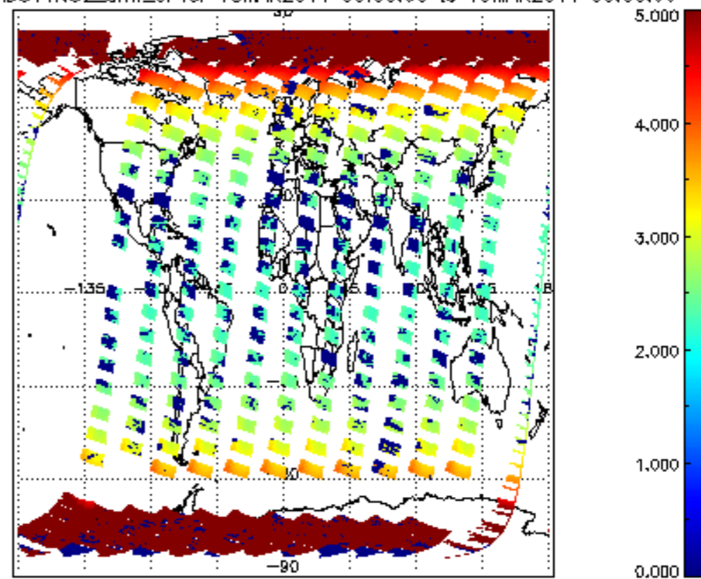
SCIOL2P_NADUV1NO2_amf_cl for 18MAR2011 00:00:00 to 19MAR2011 00:00:00
