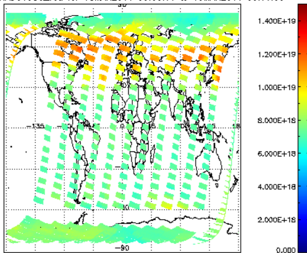
SCIOL2P_NADUV003_vcd for 18MAR2011 00:00:00 to 19MAR2011 00:00:00
