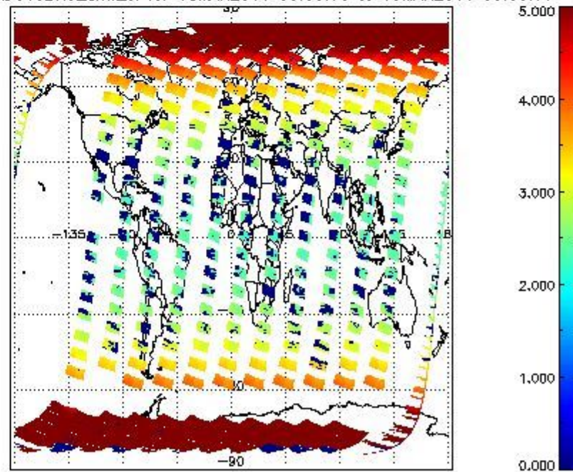
SCIOL2P_NADUV3BRO_amf_cl for 18MAR2011 00:00:00 to 19MAR2011 00:00:00
