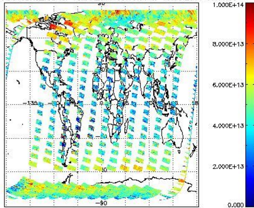
SCIOL2P_NADUV3BRO_vcd for 18MAR2011 00:00:00 to 19MAR2011 00:00:00
