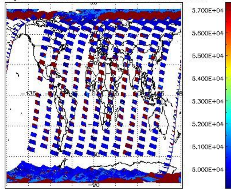
cloud_flags for 18MAR2011 00:00:00 to 19MAR2011 00:00:00
