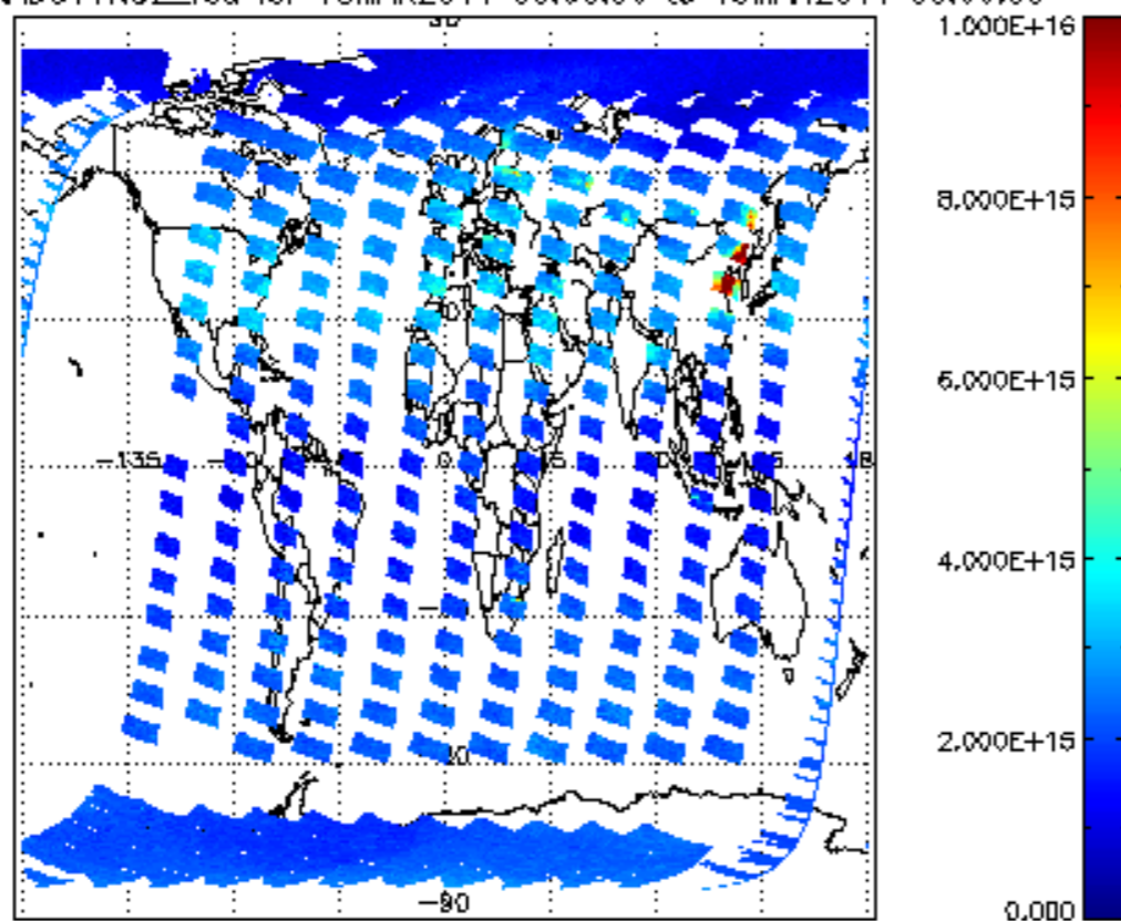
SCIOL2P_NADUV1NO2_vcd for 18MAR2011 00:00:00 to 19MAR2011 00:00:00
