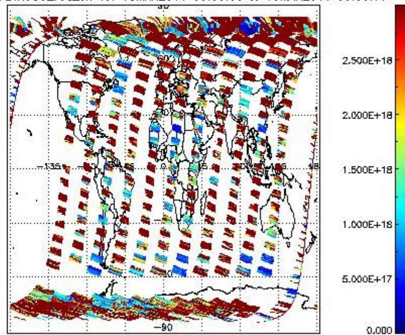
SCIOL2P_NADIR3CO_vcd_err for 18MAR2011 00:00:00 to 19MAR2011 00:00:00
