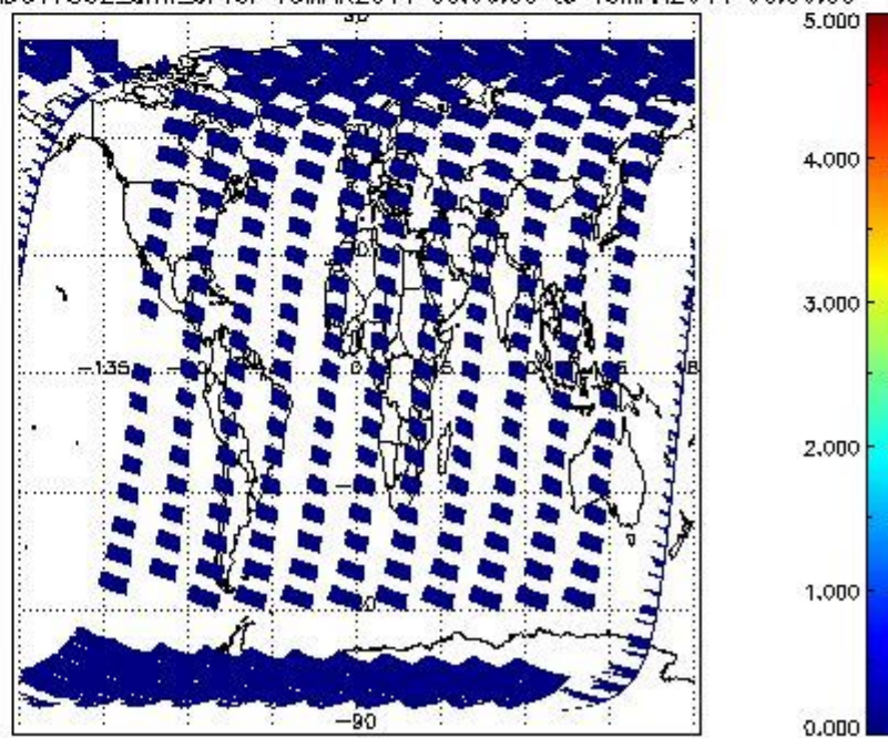
SCIOL2P_NADUV7S02_amf_cl for 18MAR2011 00:00:00 to 19MAR2011 00:00:00
