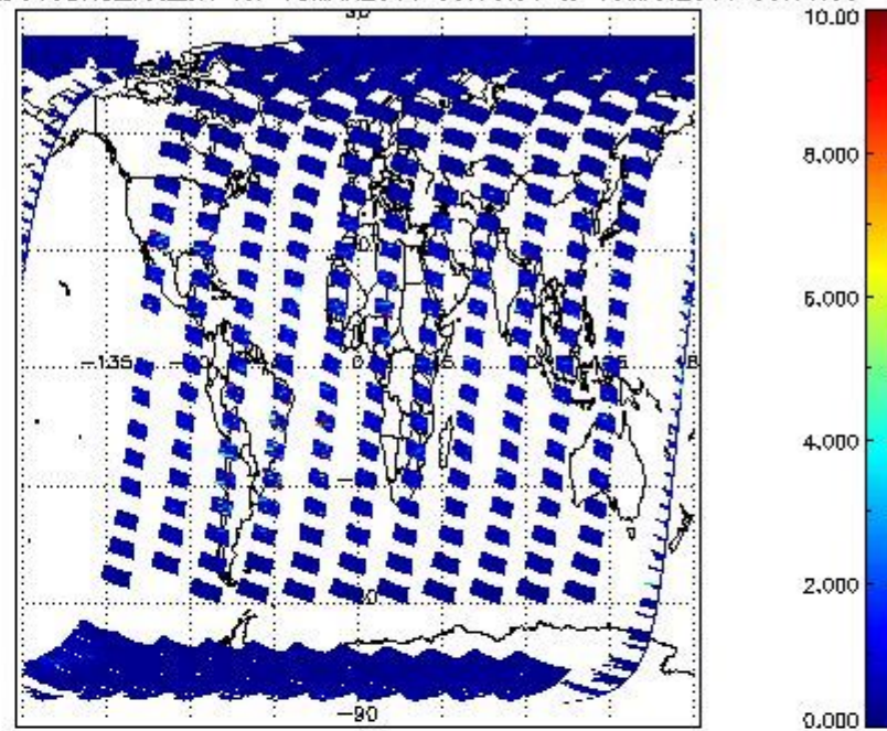
SCIOL2P_NADUV3BRO_vcd_err for 18MAR2011 00:00:00 to 19MAR2011 00:00:00
