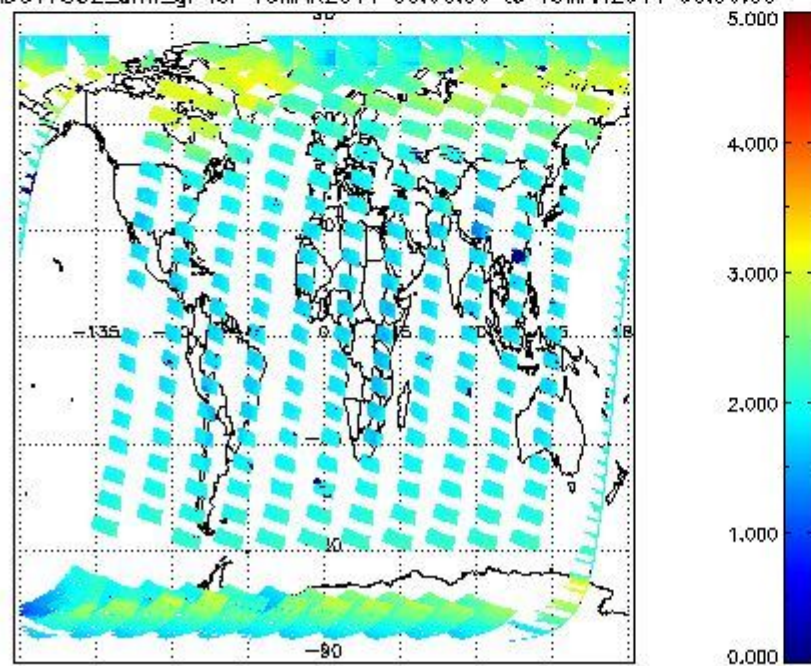
SCIOL2P_NADUV7S02_amf_gr for 18MAR2011 00:00:00 to 19MAR2011 00:00:00
