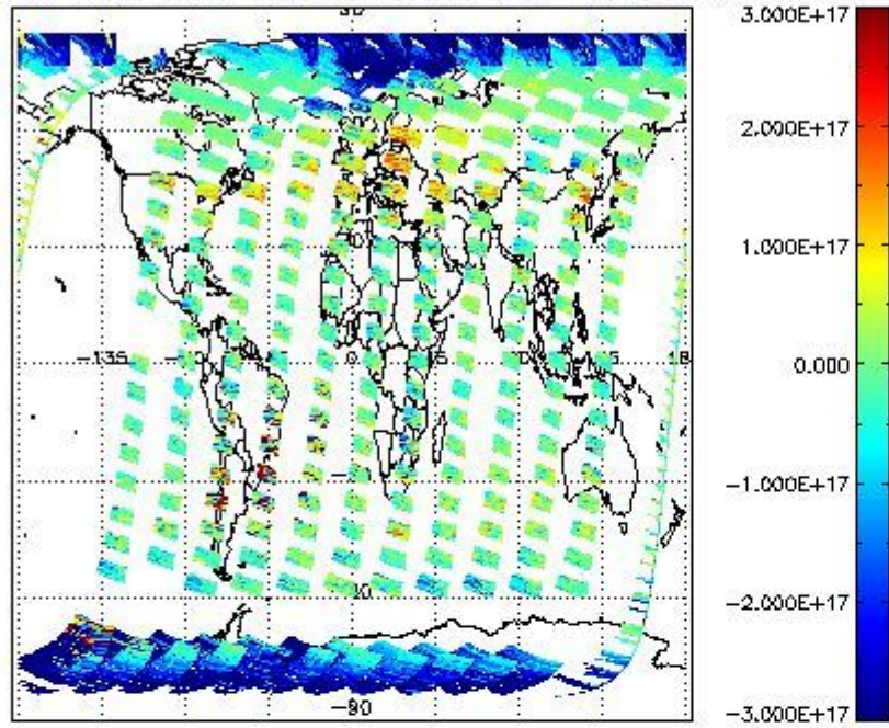
SCIOL2P_NADUV5SO2_vcd for 18MAR2011 00:00:00 to 19MAR2011 00:00:00
