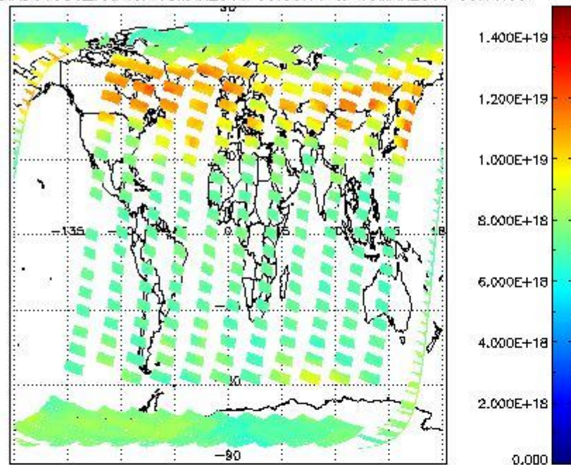
SCIOL2P_NADUV003_vcd for 18MAR2011 00:00:00 to 19MAR2011 00:00:00
