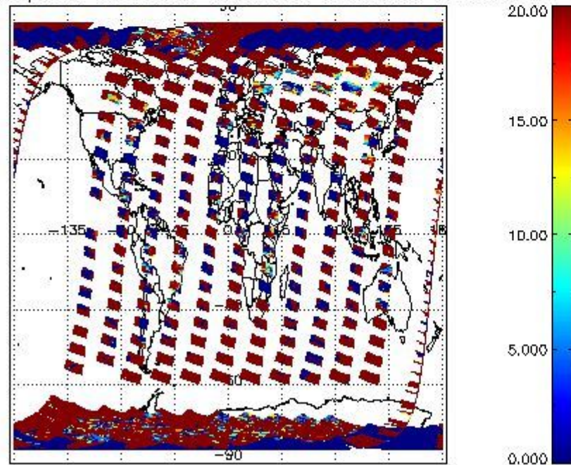
cL_opt_depth for 18MAR2011 00:00:00 to 19MAR2011 00:00:00
