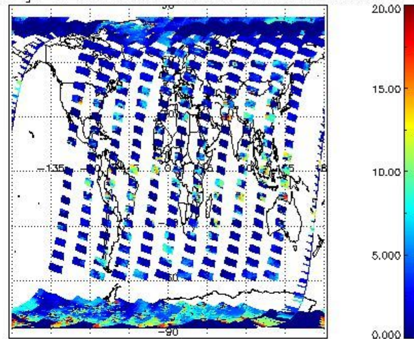
cL_top_height for 18MAR2011 00:00:00 to 19MAR2011 00:00:00
