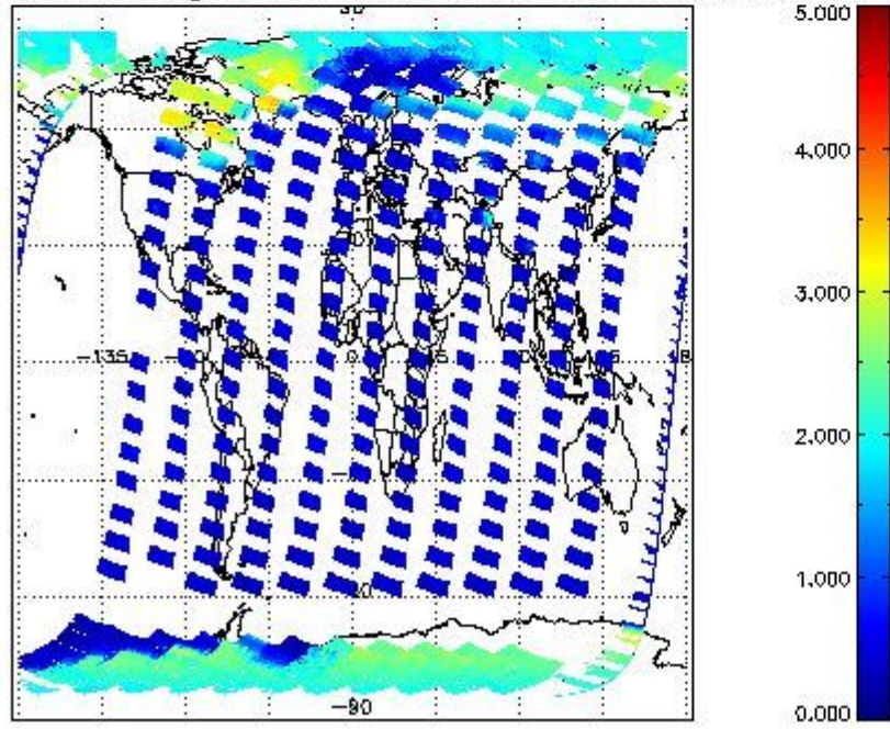
SCIOL2P_NADUV5SO2_amf_gr for 18MAR2011 00:00:00 to 19MAR2011 00:00:00
