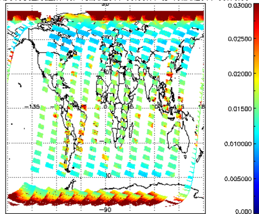
SCIOL2P_NADUV003_vcd_err for 18MAR2011 00:00:00 to 19MAR2011 00:00:00
