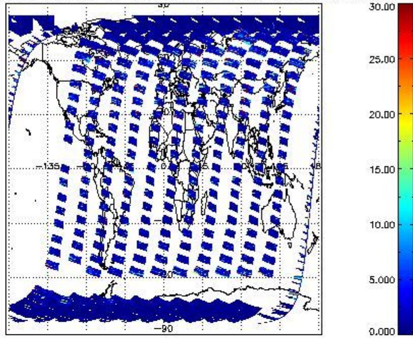
SCIOL2P_NADUV5SO2_vcd_err for 18MAR2011 00:00:00 to 19MAR2011 00:00:00
