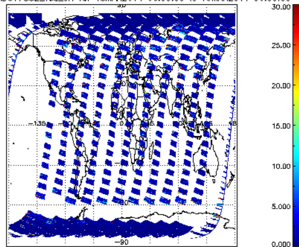
SCIOL2P_NADUV7S02_vcd_err for 18MAR2011 00:00:00 to 19MAR2011 00:00:00
