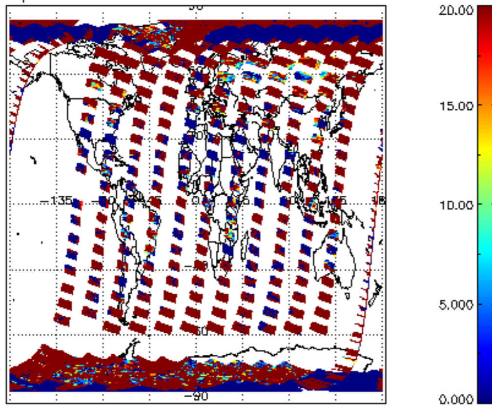
cL_opt_depth for 18MAR2011 00:00:00 to 19MAR2011 00:00:00
