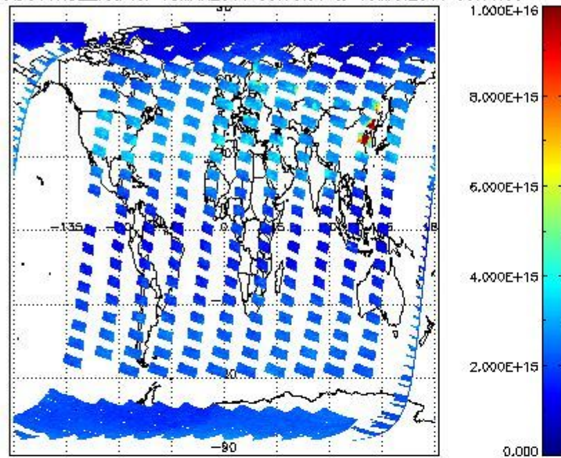
SCIOL2P_NADUV1NO2_vcd for 18MAR2011 00:00:00 to 19MAR2011 00:00:00
