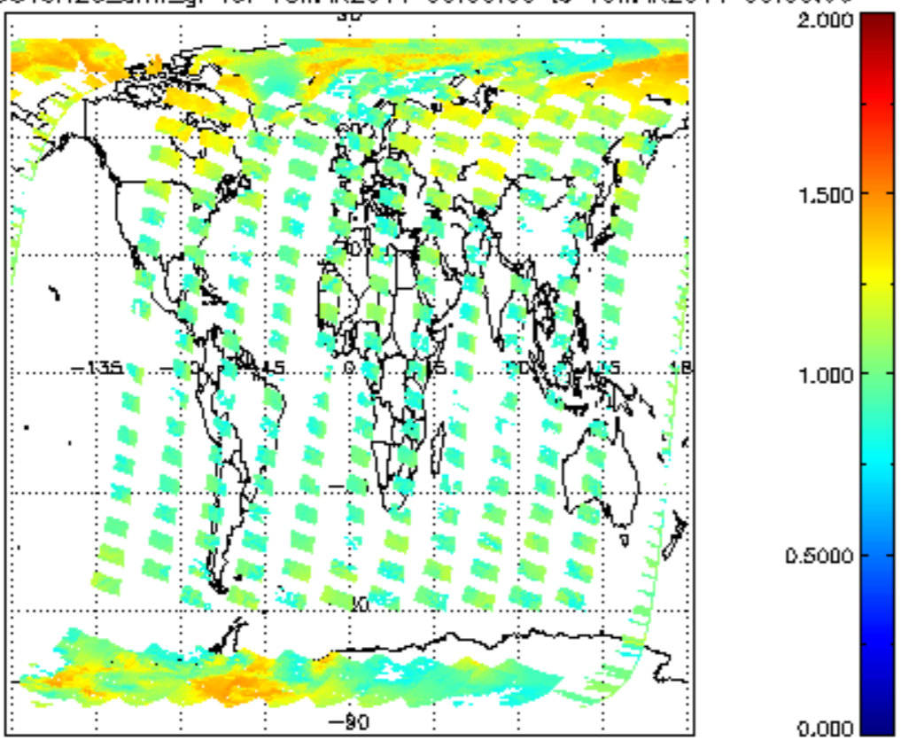
SCIOL2P_NADUV8H20_arnf_gr for 18MAR2011 00:00:00 to 19MAR2011 00:00:00
