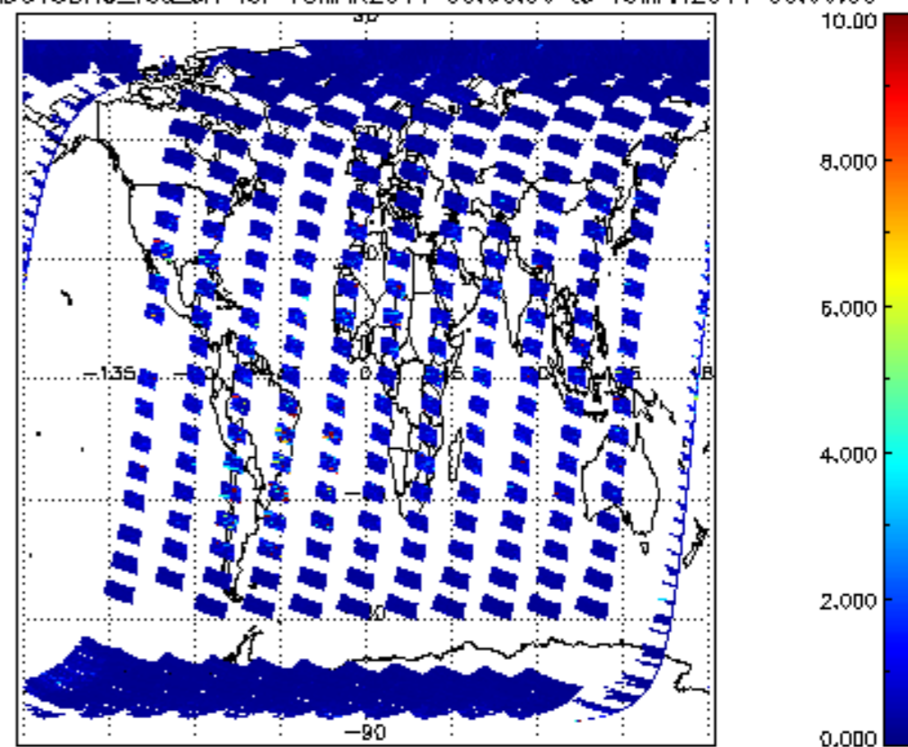
SCIOL2P_NADUV3BRO_vcd_err for 18MAR2011 00:00:00 to 19MAR2011 00:00:00
