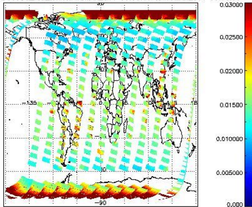
SCIOL2P_NADUV003_vcd_err for 18MAR2011 00:00:00 to 19MAR2011 00:00:00
