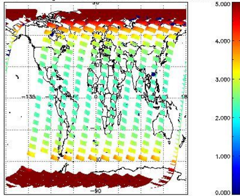
SCIOL2P_NADUV1NO2_amf_gr for 18MAR2011 00:00:00 to 19MAR2011 00:00:00
