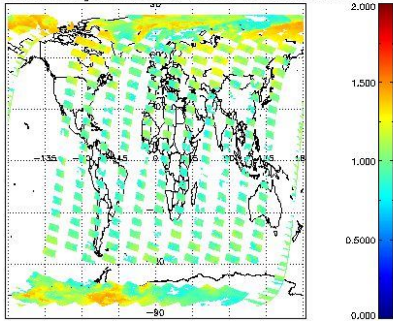
SCIOL2P_NADUV8H2O_arnf_gr for 18MAR2011 00:00:00 to 19MAR2011 00:00:00
