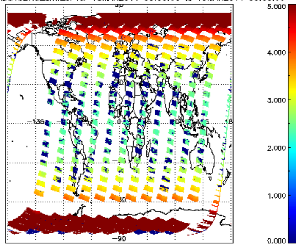
SCIOL2P_NADUV3BRO_amf_cl for 18MAR2011 00:00:00 to 19MAR2011 00:00:00
