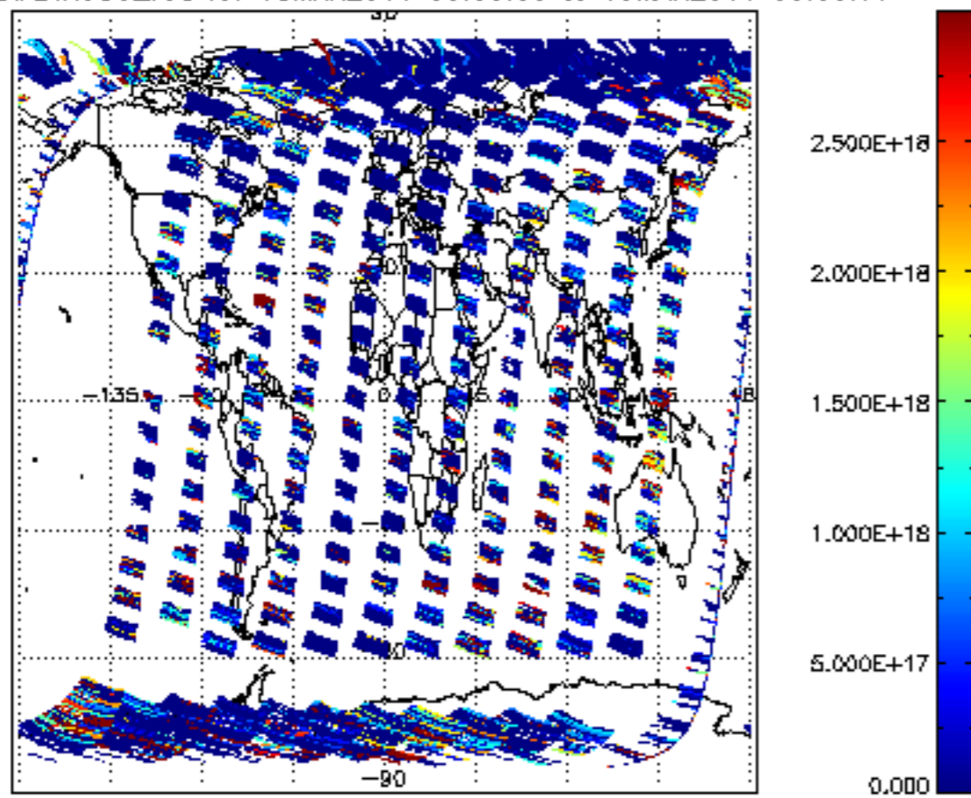
SCIOL2P_NADIR3CO_vcd for 18MAR2011 00:00:00 to 19MAR2011 00:00:00
