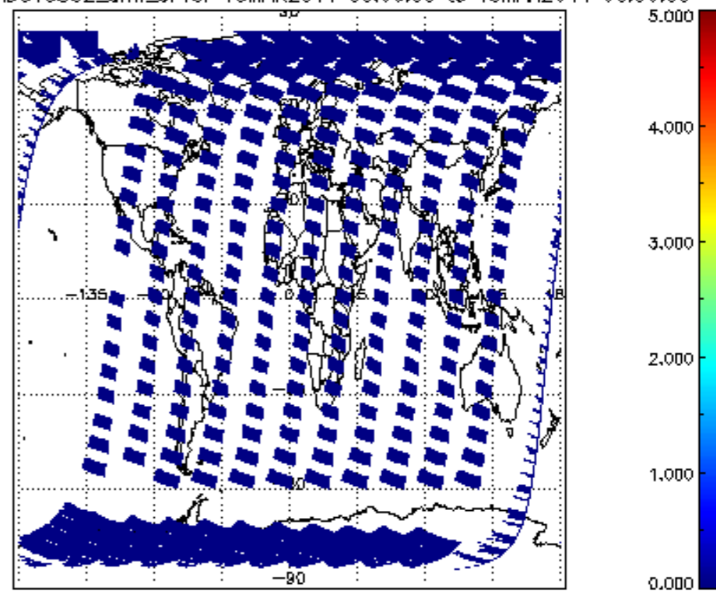
SCIOL2P_NADUV5S02_amf_cl for 18MAR2011 00:00:00 to 19MAR2011 00:00:00
