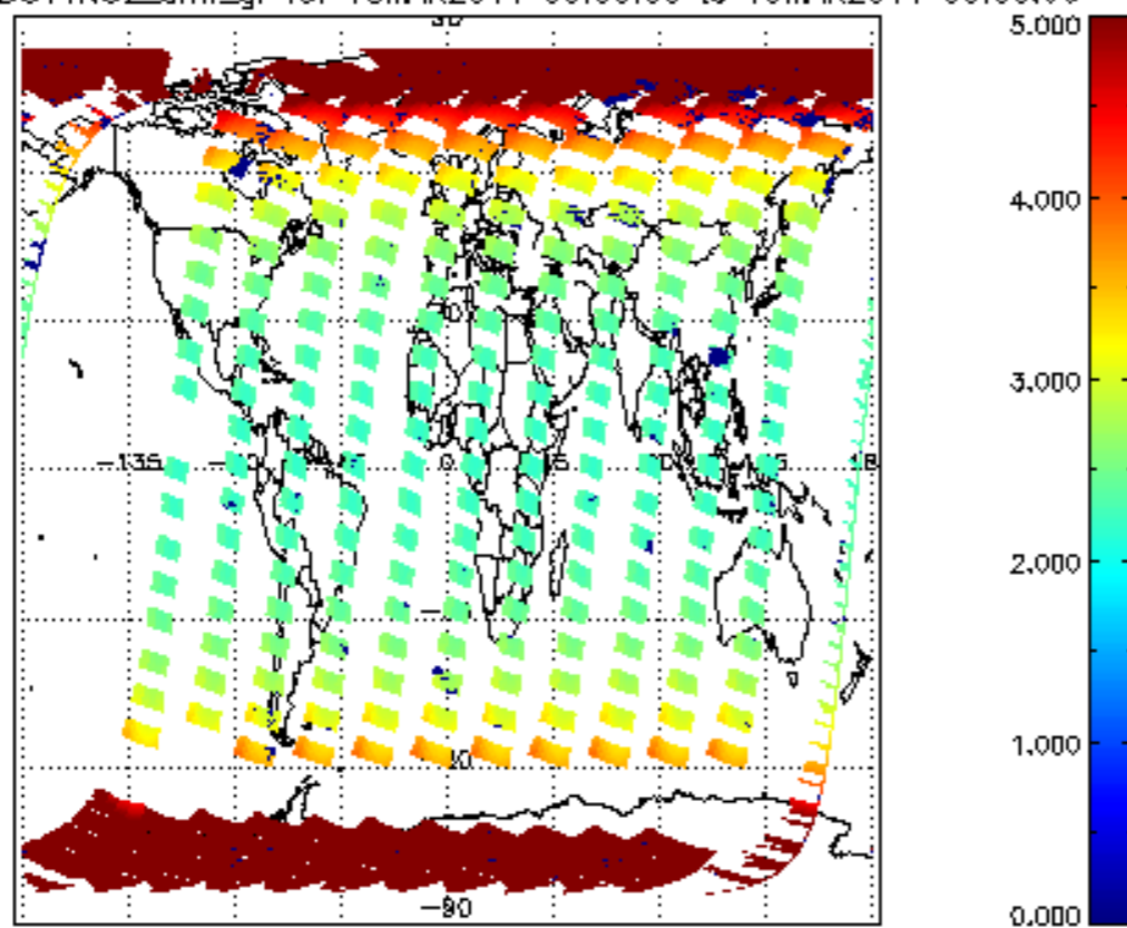
SCIOL2P_NADUV1NO2_amf_gr for 18MAR2011 00:00:00 to 19MAR2011 00:00:00
