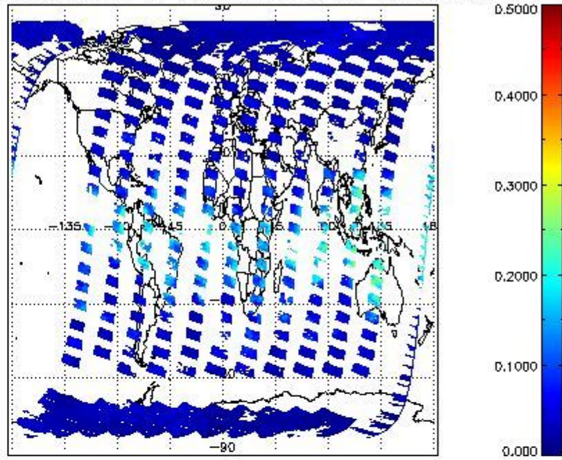
SCIOL2P_NADUV8H2O_vcd_err for 18MAR2011 00:00:00 to 19MAR2011 00:00:00
