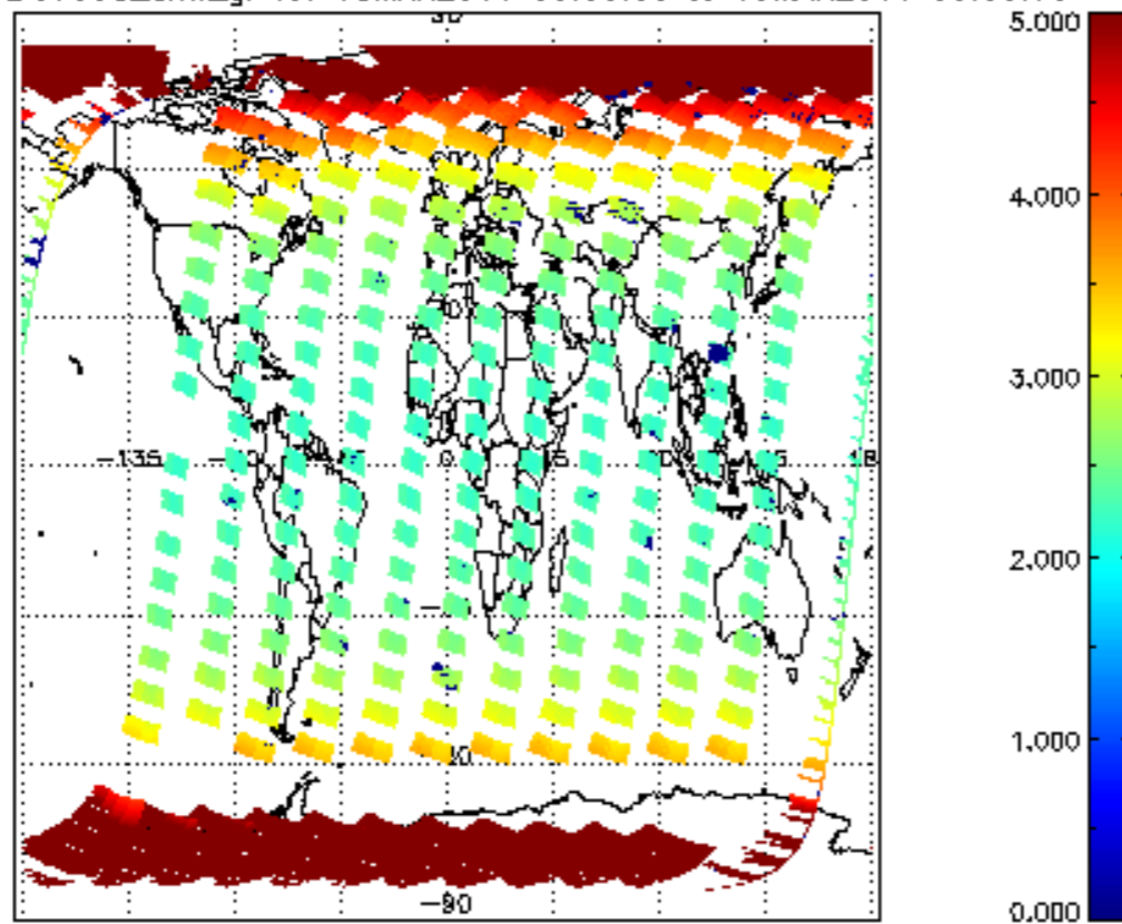
SCIOL2P_NADUV003_amf_gr for 18MAR2011 00:00:00 to 19MAR2011 00:00:00
