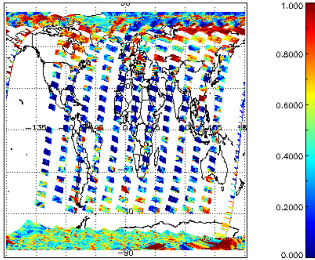
cL_frac for 18MAR2011 00:00:00 to 19MAR2011 00:00:00
