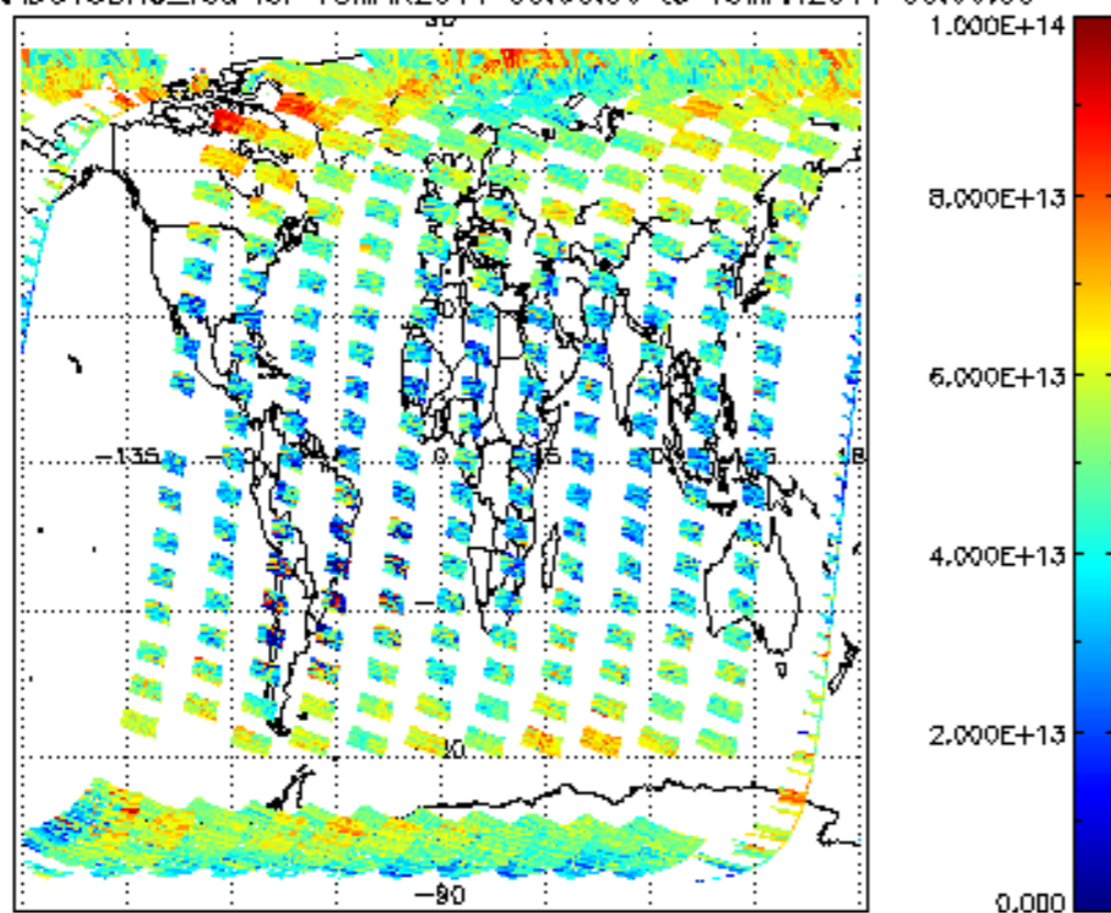
SCIOL2P_NADUV3BRO_vcd for 18MAR2011 00:00:00 to 19MAR2011 00:00:00
