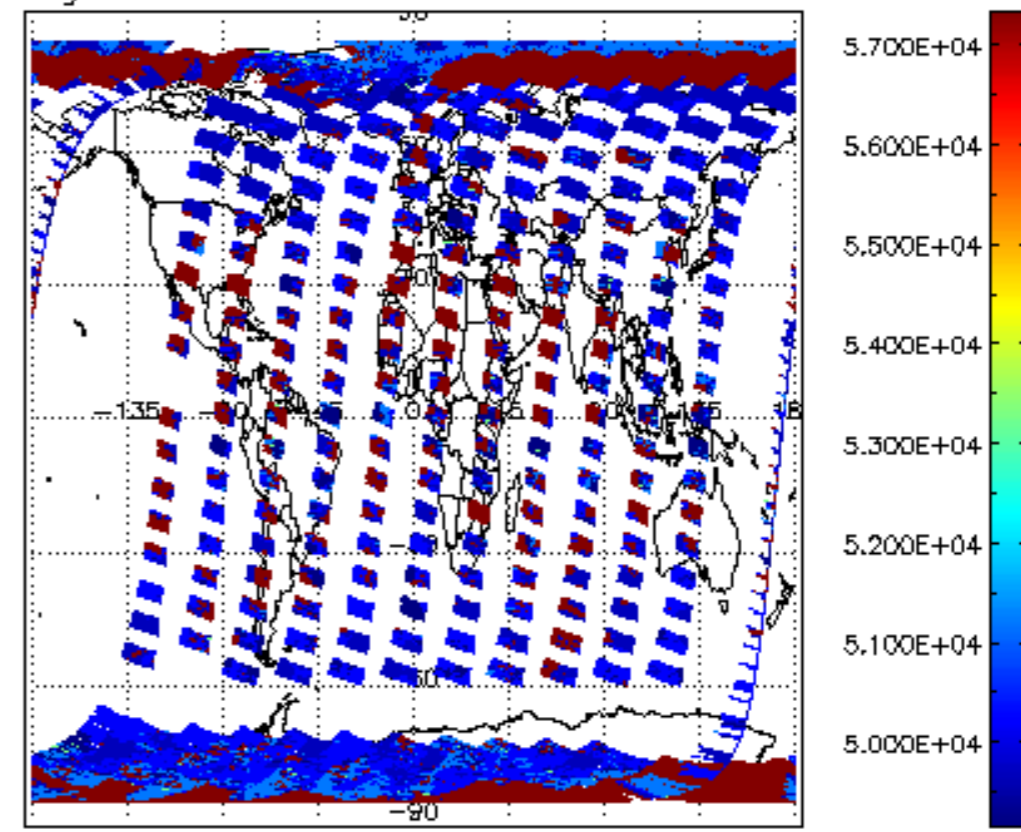
cloud_flags for 18MAR2011 00:00:00 to 19MAR2011 00:00:00
