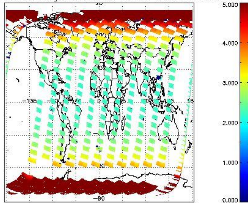
SCIOL2P_NADUV3BRO_amf_gr for 18MAR2011 00:00:00 to 19MAR2011 00:00:00
