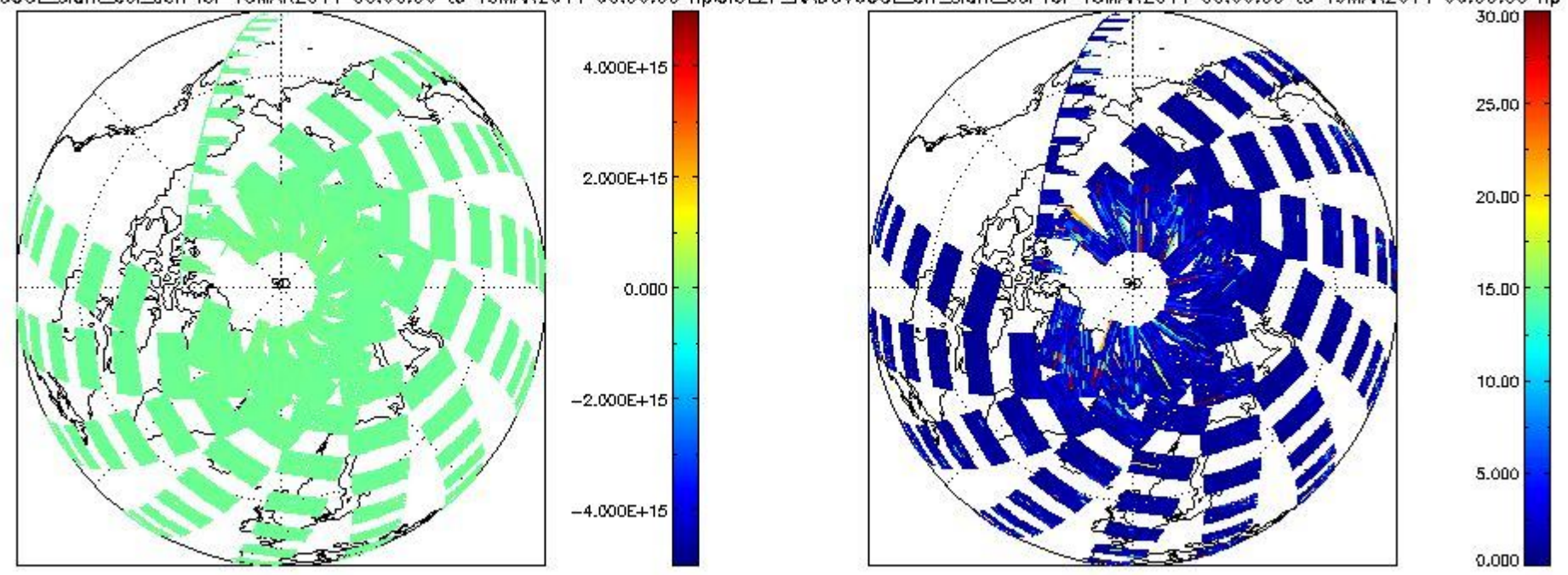
CIOL2P_NADUV6OCL_slant_col_den for 18MAR2011 00:00:00 to 19MAR2011 00:00:00 npCIOL2P_NADUV6OCL_err_slant_col for 18MAR2011 00:00:00 to 19MAR2011 00:00:00 np
