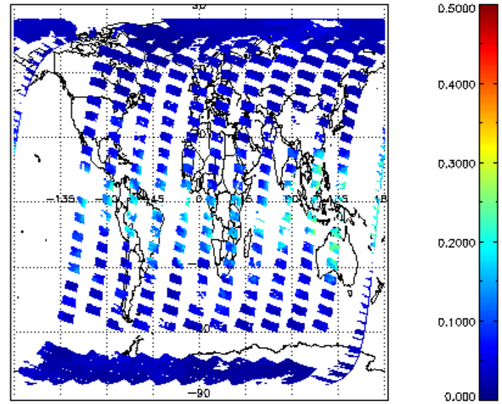
SCIOL2P_NADUV8H20_vcd_err for 18MAR2011 00:00:00 to 19MAR2011 00:00:00
