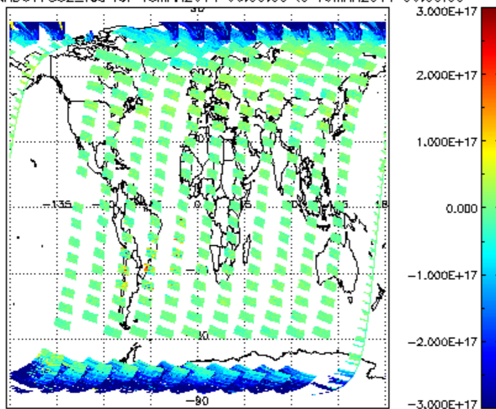
SCIOL2P_NADUV7S02_vcd for 18MAR2011 00:00:00 to 19MAR2011 00:00:00
