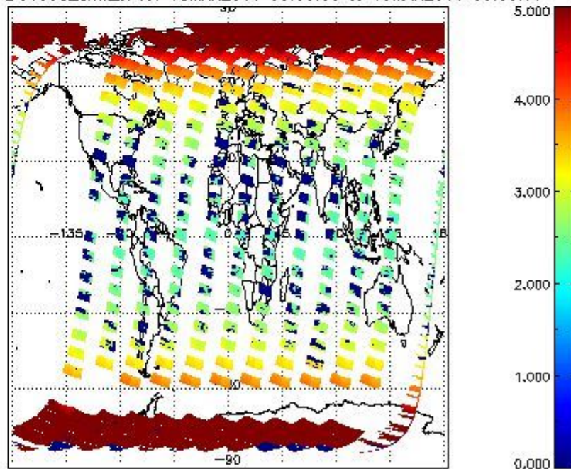
SCIOL2P_NADUV003_amf_cl for 18MAR2011 00:00:00 to 19MAR2011 00:00:00
