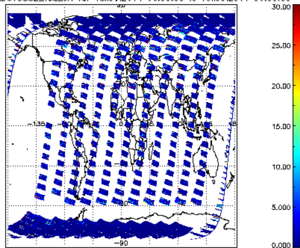
SCIOL2P_NADUV5S02_vcd_err for 18MAR2011 00:00:00 to 19MAR2011 00:00:00
