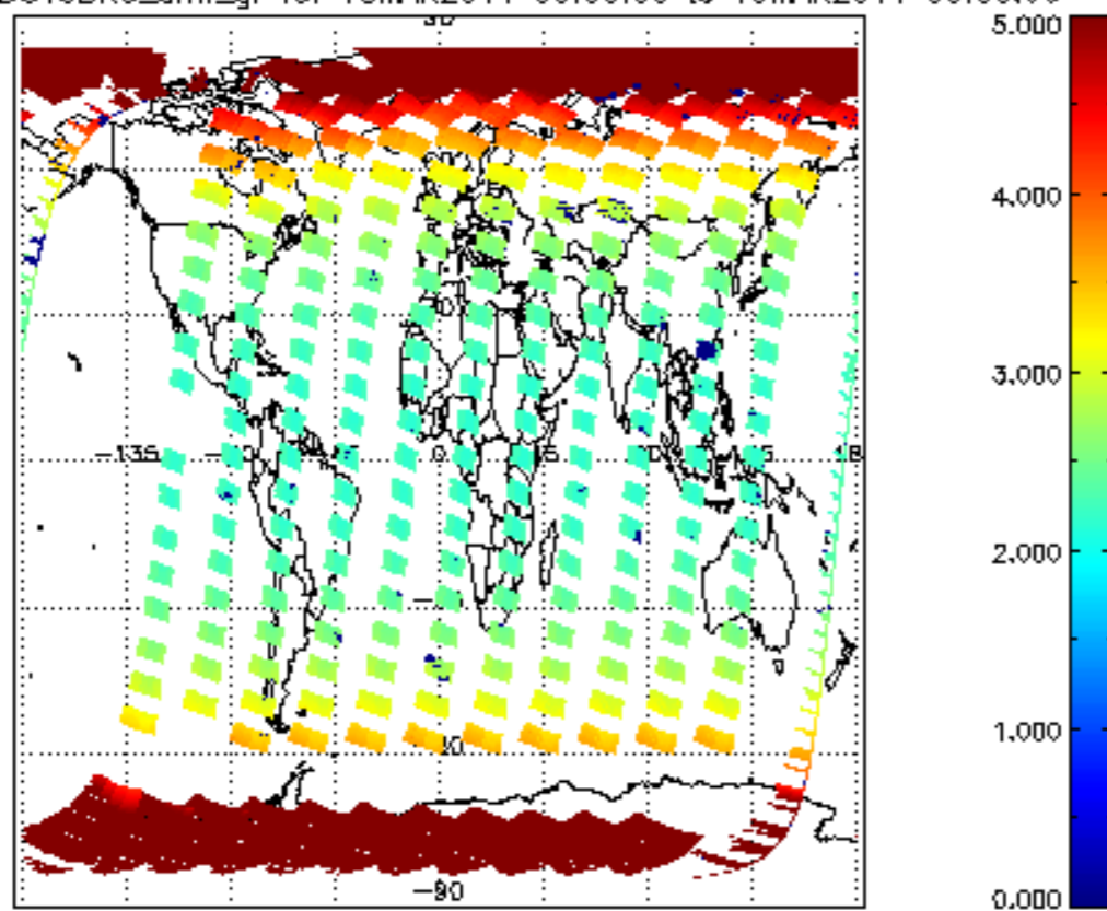
SCIOL2P_NADUV3BRO_amf_gr for 18MAR2011 00:00:00 to 19MAR2011 00:00:00
