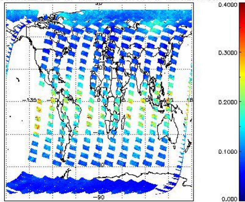
SCIOL2P_NADUV1NO2_vcd_err for 18MAR2011 00:00:00 to 19MAR2011 00:00:00
