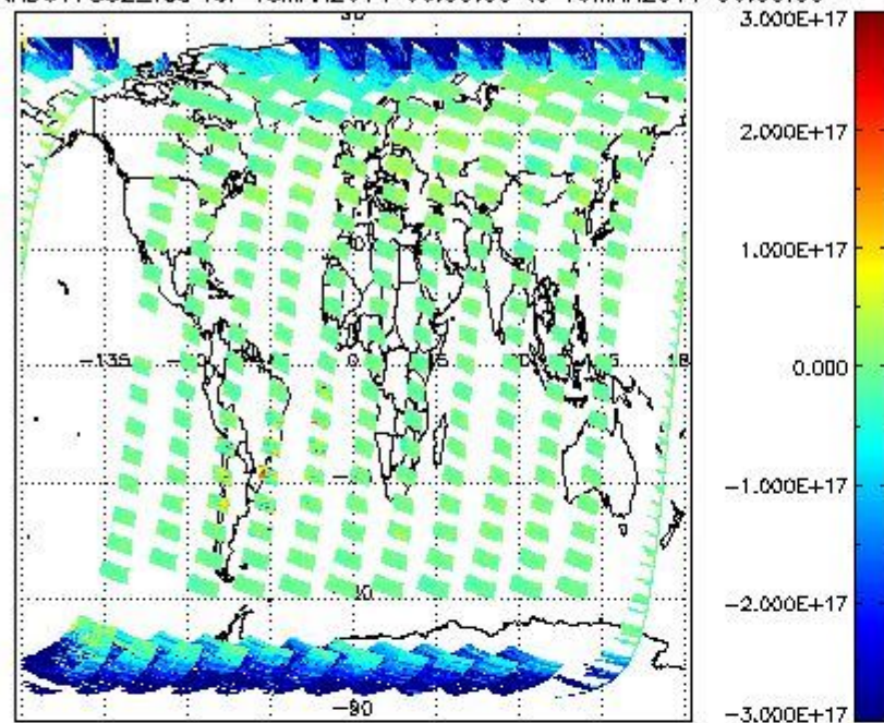
SCIOL2P_NADUV7S02_vcd for 18MAR2011 00:00:00 to 19MAR2011 00:00:00
