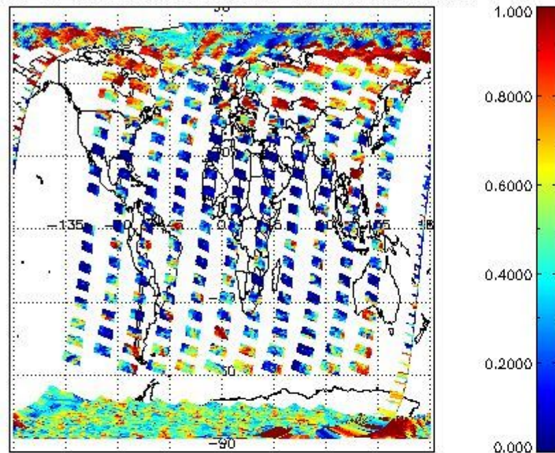
cL_frac for 18MAR2011 00:00:00 to 19MAR2011 00:00:00
