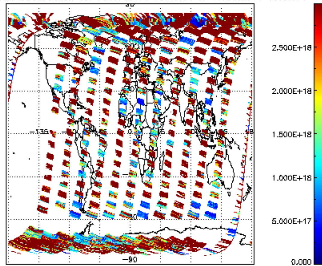
SCIOL2P_NADIR3CO_vcd_err for 18MAR2011 00:00:00 to 19MAR2011 00:00:00
