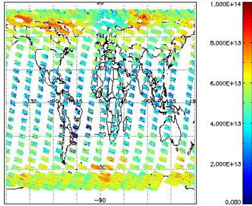
SCIOL2P_NADUV3BRO_vcd for 15MAR2011 00:00:00 to 16MAR2011 00:00:00
