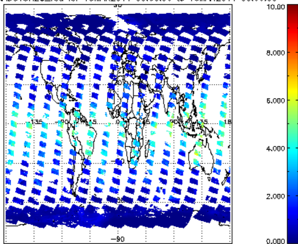
SCIOL2P_NADUV8H20_vcd for 15MAR2011 00:00:00 to 16MAR2011 00:00:00
