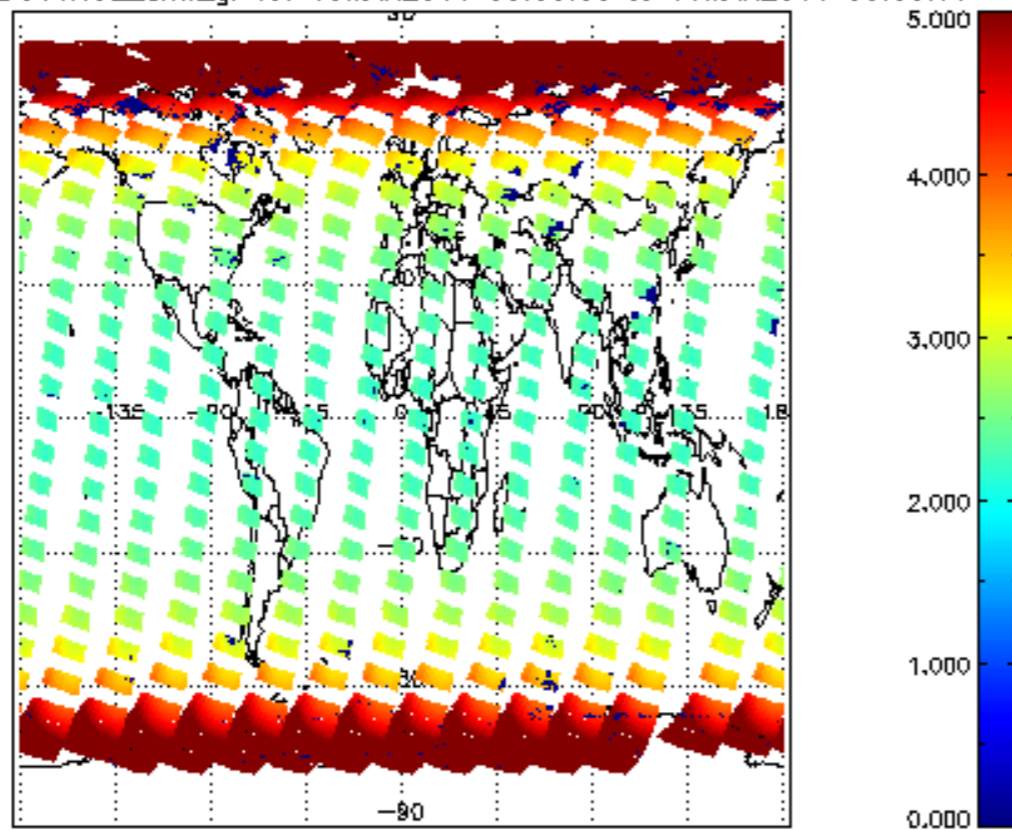
SCIOL2P_NADUV1NO2_amf_gr for 15MAR2011 00:00:00 to 16MAR2011 00:00:00
