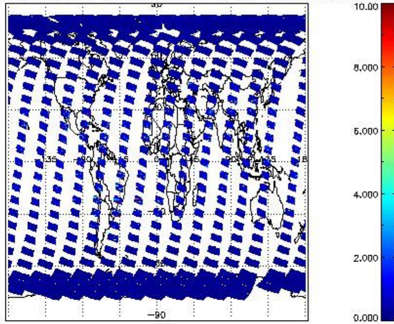
SCIOL2P_NADUV3BRO_vcd_err for 15MAR2011 00:00:00 to 16MAR2011 00:00:00
