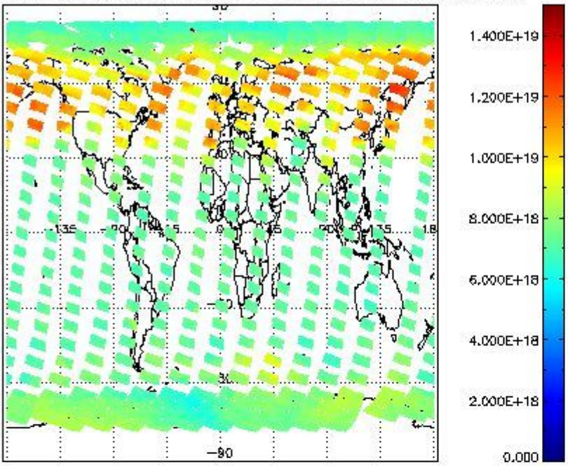
SCIOL2P_NADUV003_vcd for 15MAR2011 00:00:00 to 16MAR2011 00:00:00
