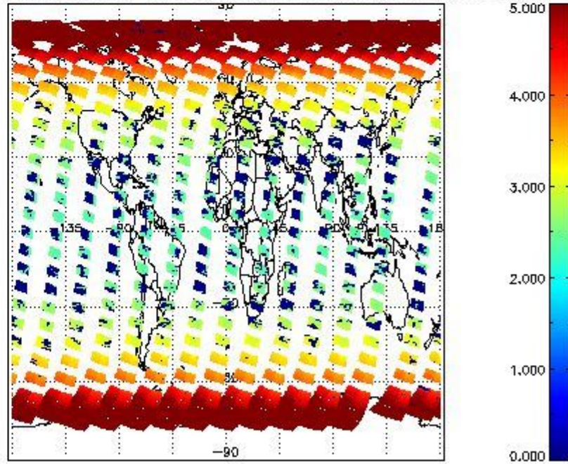
SCIOL2P_NADUV3BRO_amf_cl for 15MAR2011 00:00:00 to 16MAR2011 00:00:00
