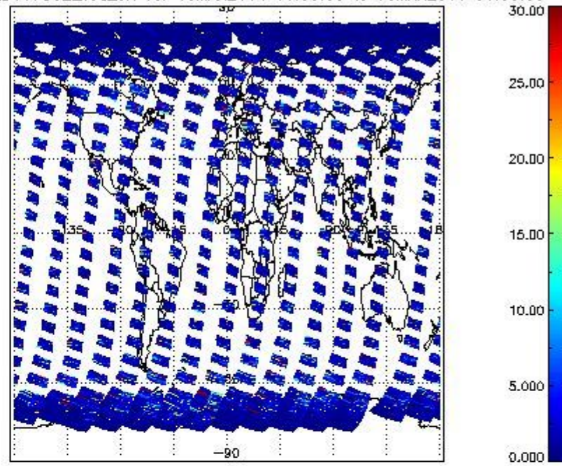
SCIOL2P_NADUV7S02_vcd_err for 15MAR2011 00:00:00 to 16MAR2011 00:00:00
