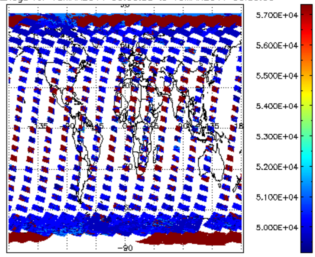
cloud_flags for 15MAR2011 00:00:00 to 16MAR2011 00:00:00
