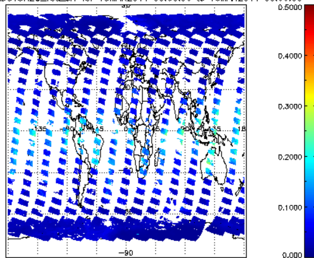
SCIOL2P_NADUV8H20_vcd_err for 15MAR2011 00:00:00 to 16MAR2011 00:00:00
