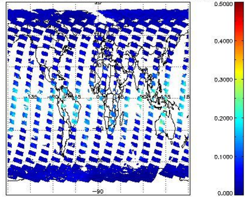
SCIOL2P_NADUV8H2O_vcd_err for 15MAR2011 00:00:00 to 16MAR2011 00:00:00
