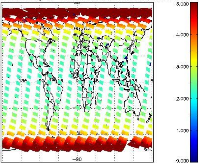
SCIOL2P_NADUV003_amf_gr for 15MAR2011 00:00:00 to 16MAR2011 00:00:00
