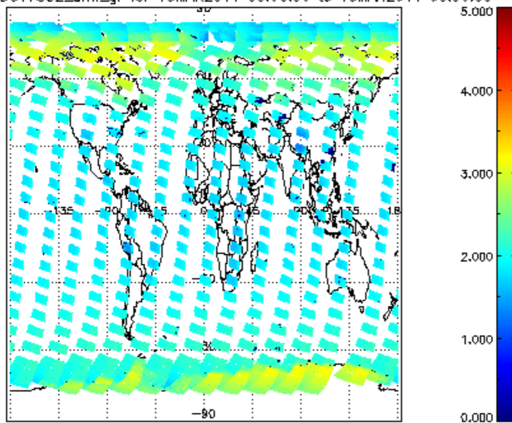
SCIOL2P_NADUV7S02_amf_gr for 15MAR2011 00:00:00 to 16MAR2011 00:00:00
