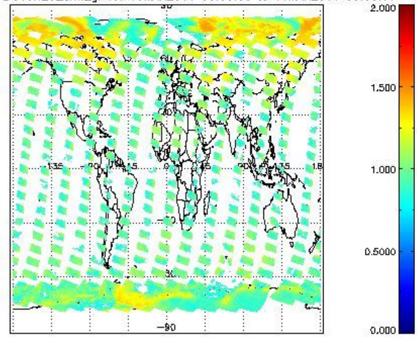
SCIOL2P_NADUV8H2O_arnf_gr for 15MAR2011 00:00:00 to 16MAR2011 00:00:00
