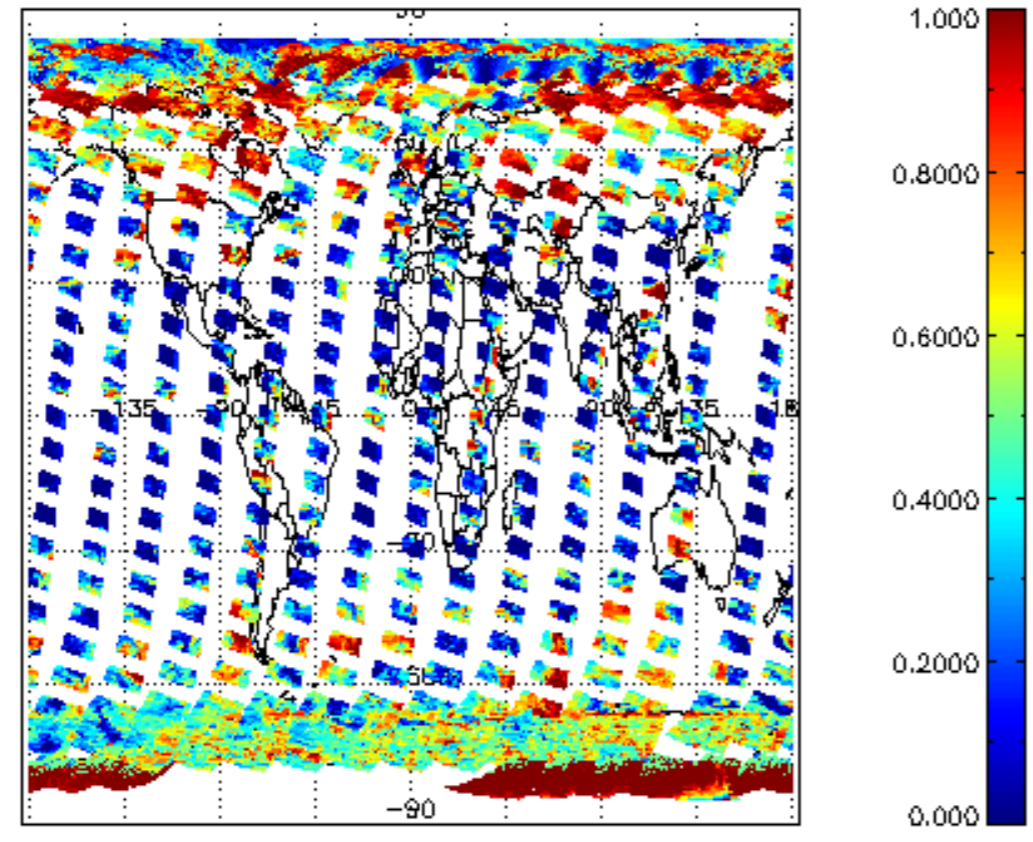
cLfrac for 15MAR2011 00:00:00 to 16MAR2011 00:00:00
