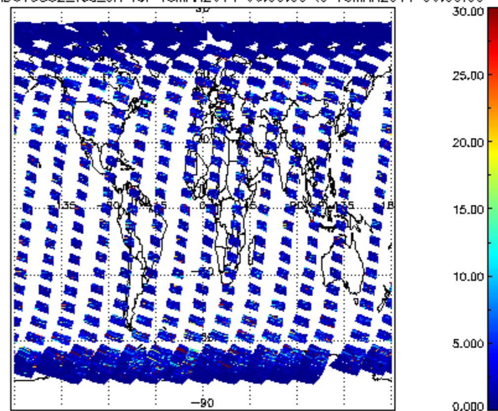
SCIOL2P_NADUV5S02_vcd_err for 15MAR2011 00:00:00 to 16MAR2011 00:00:00
