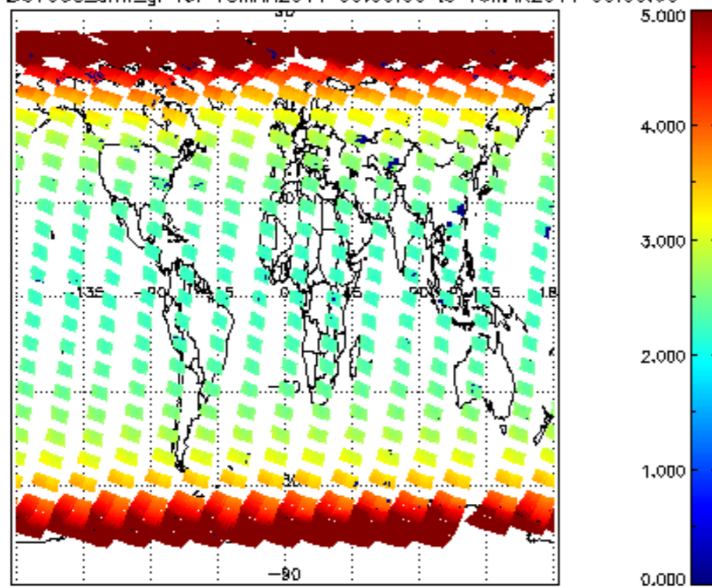
SCIOL2P_NADUV003_arnf_gr for 15MAR2011 00:00:00 to 16MAR2011 00:00:00
