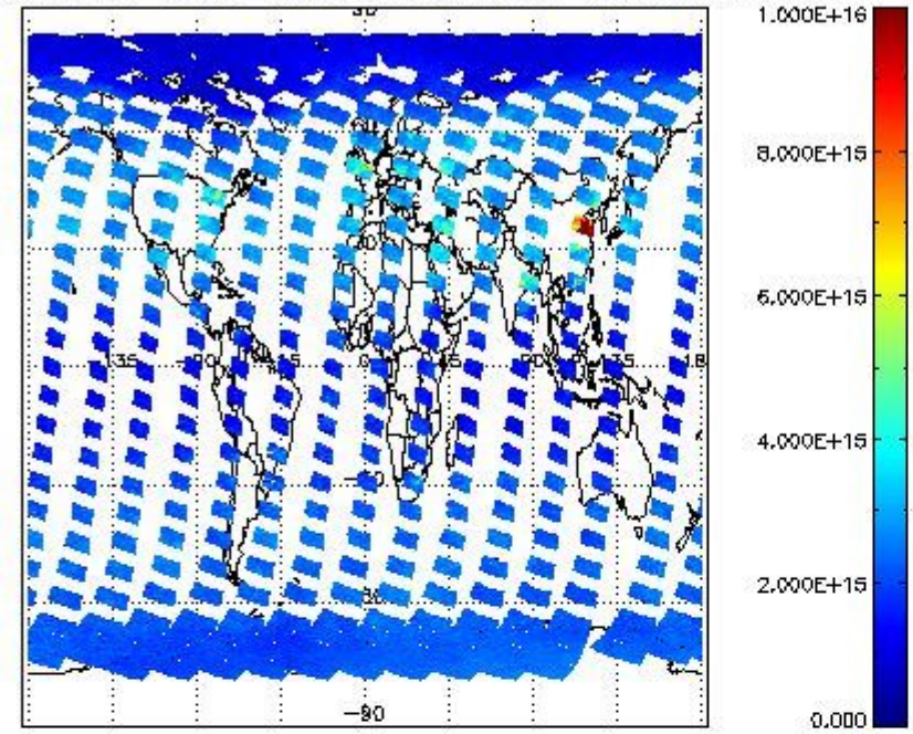
SCIOL2P_NADUV1NO2_vcd for 15MAR2011 00:00:00 to 16MAR2011 00:00:00
