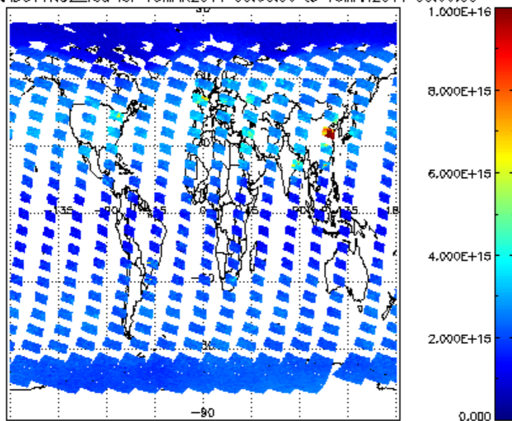
SCIOL2P_NADUV1NO2_vcd for 15MAR2011 00:00:00 to 16MAR2011 00:00:00
