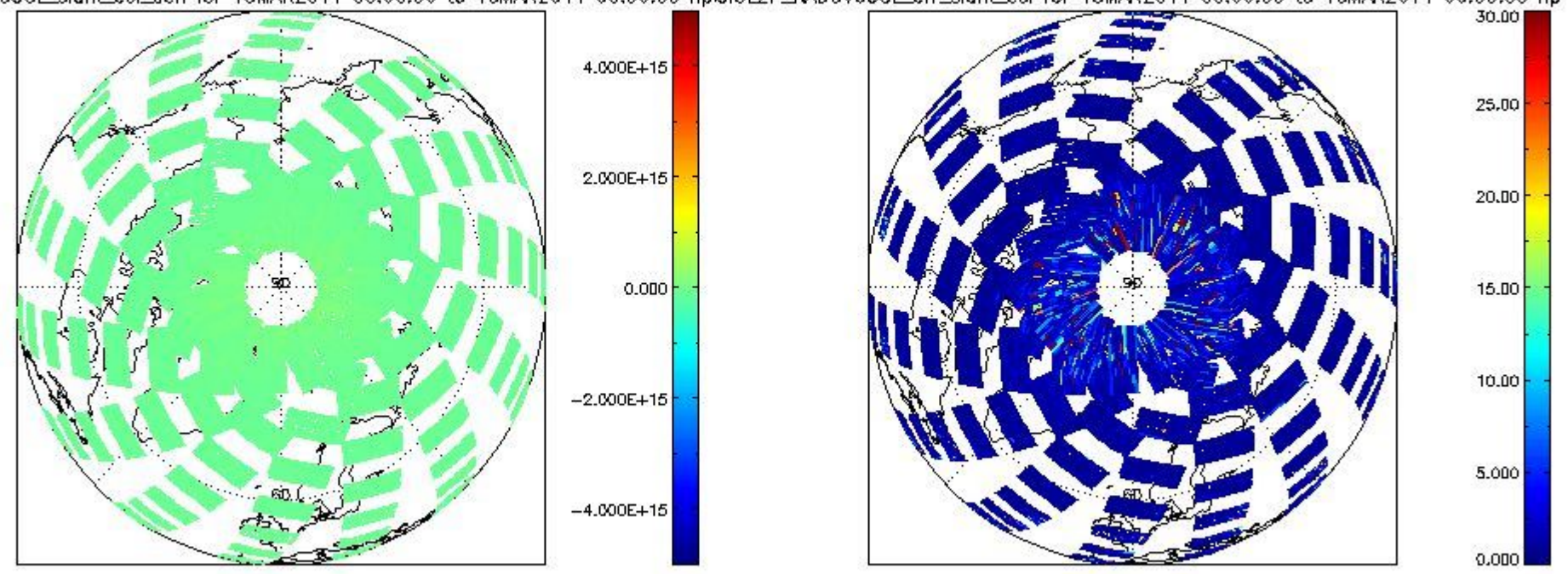
CIOL2P_NADUV6OCL_slant_col_den for 15MAR2011 00:00:00 to 16MAR2011 00:00:00 np CIOL2P_NADUV6OCL_err_slant_col for 15MAR2011 00:00:00 to 16MAR2011 00:00:00 np
