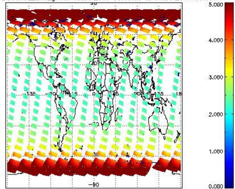
SCIOL2P_NADUV1NO2_amf_gr for 15MAR2011 00:00:00 to 16MAR2011 00:00:00
