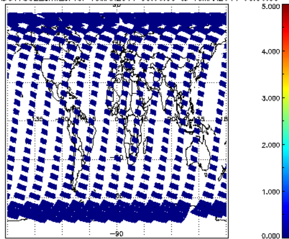
SCIOL2P_NADUV7S02_amf_cl for 15MAR2011 00:00:00 to 16MAR2011 00:00:00
