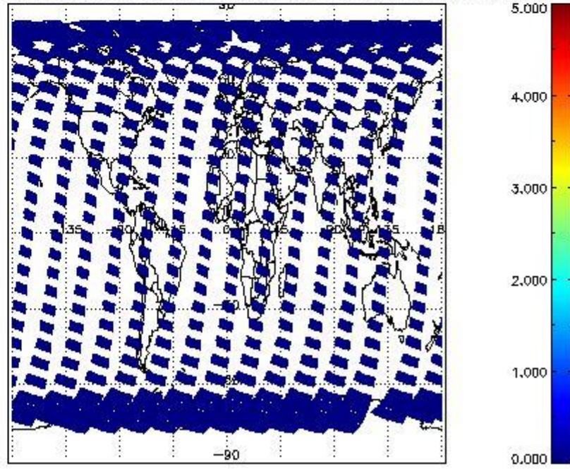
SCIOL2P_NADUV5S02_amf_cl for 15MAR2011 00:00:00 to 16MAR2011 00:00:00
