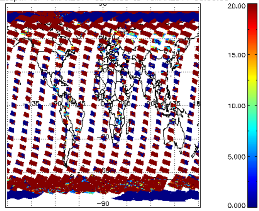
cL_opt_depth for 15MAR2011 00:00:00 to 16MAR2011 00:00:00
