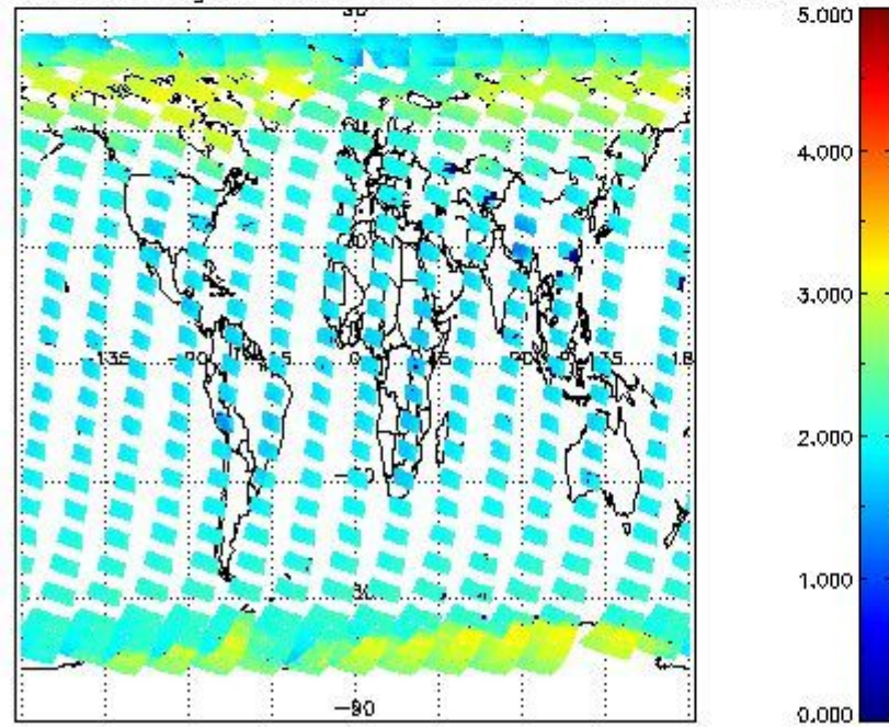
SCIOL2P_NADUV7S02_amf_gr for 15MAR2011 00:00:00 to 16MAR2011 00:00:00
