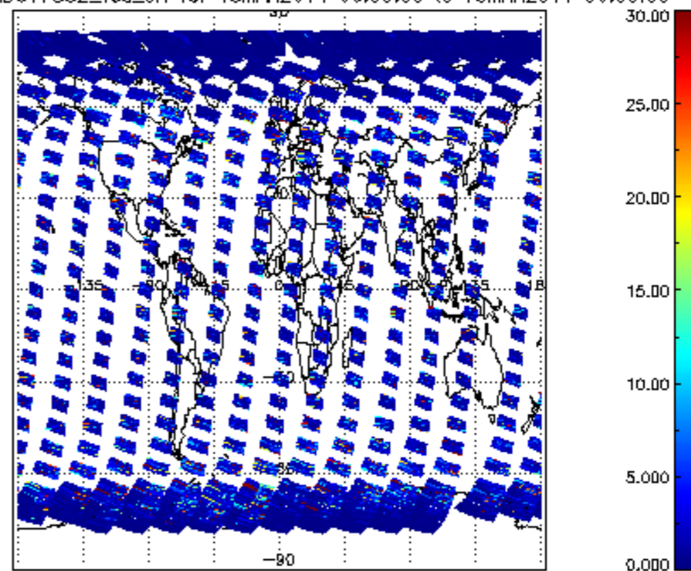
SCIOL2P_NADUV7S02_vcd_err for 15MAR2011 00:00:00 to 16MAR2011 00:00:00
