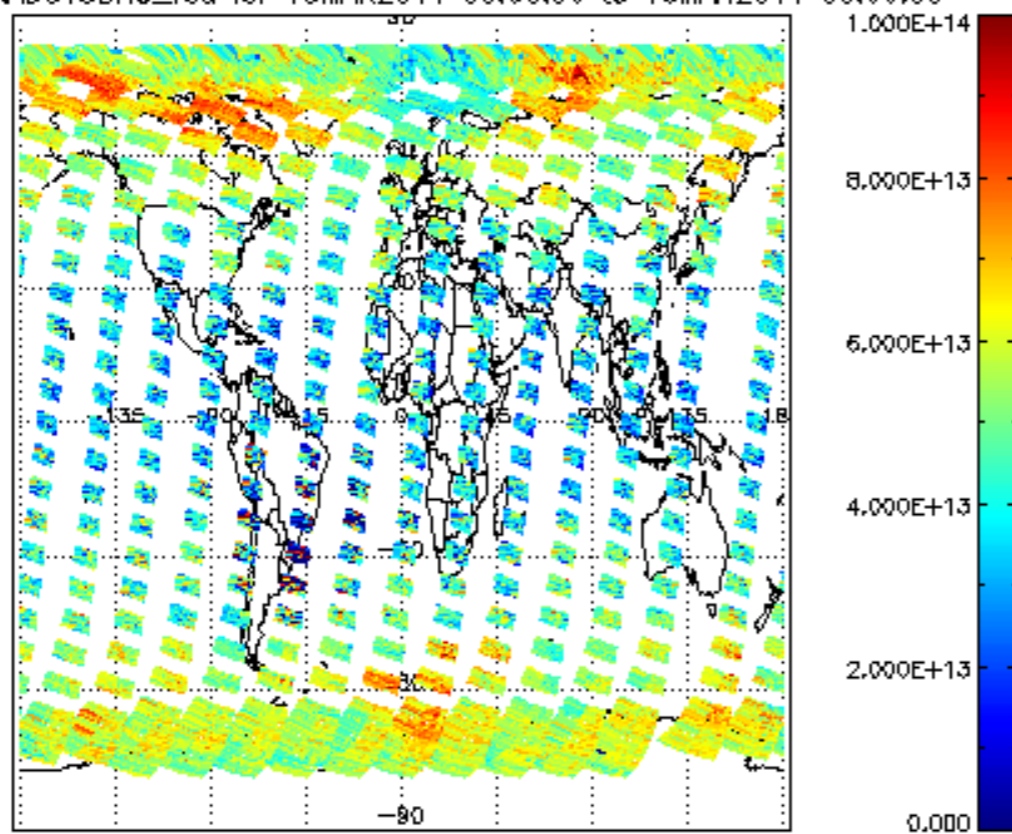
SCIOL2P_NADUV3BRO_vcd for 15MAR2011 00:00:00 to 16MAR2011 00:00:00
