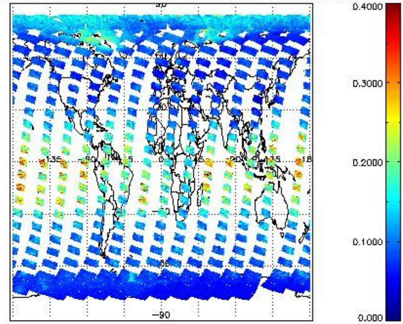
SCIOL2P_NADUV1NO2_vcd_err for 15MAR2011 00:00:00 to 16MAR2011 00:00:00
