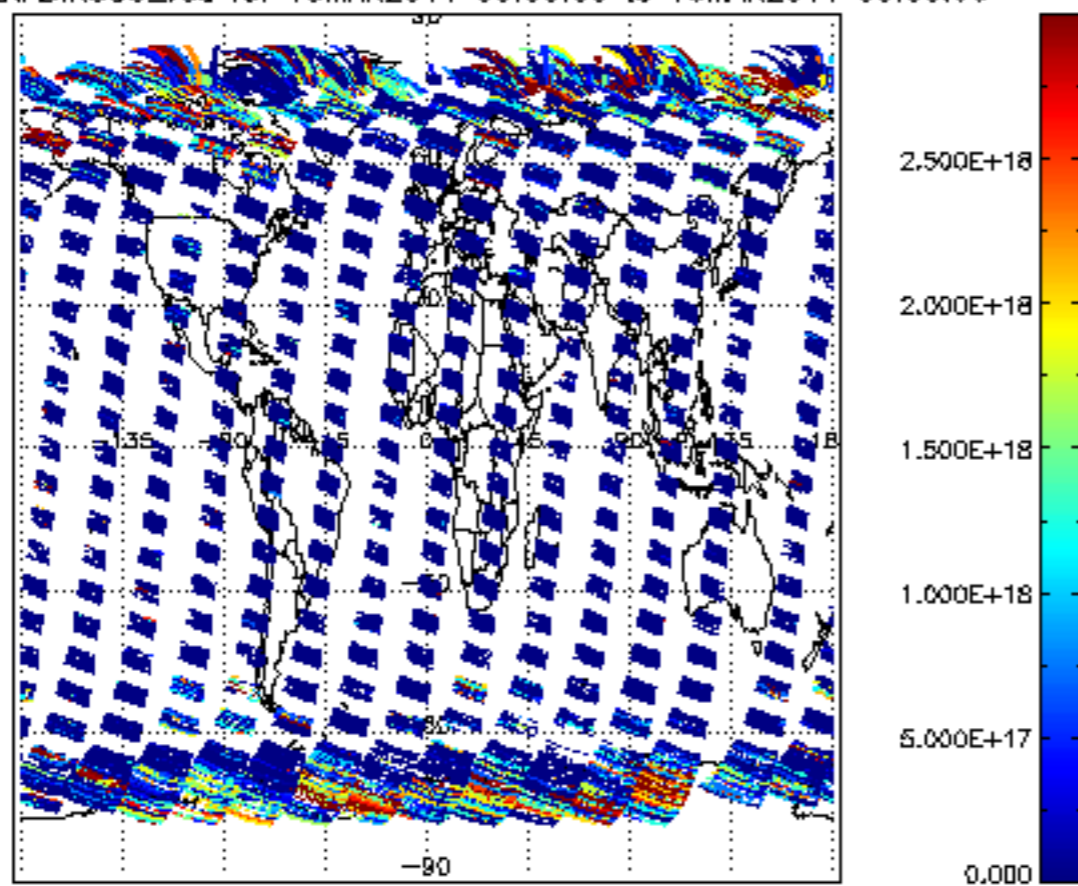
SCIOL2P_NADIR3CO_vcd for 15MAR2011 00:00:00 to 16MAR2011 00:00:00
