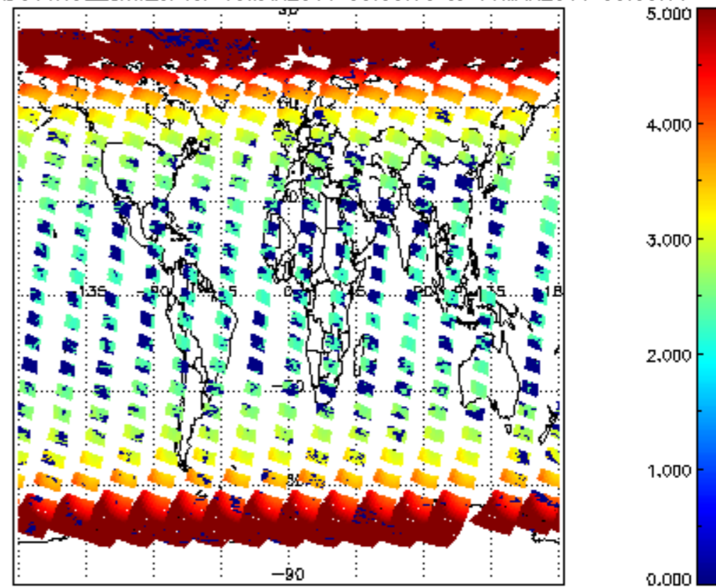
SCIOL2P_NADUV1NO2_amf_cl for 15MAR2011 00:00:00 to 16MAR2011 00:00:00
