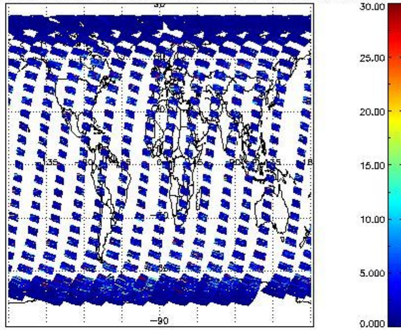
SCIOL2P_NADUV5S02_vcd_err for 15MAR2011 00:00:00 to 16MAR2011 00:00:00
