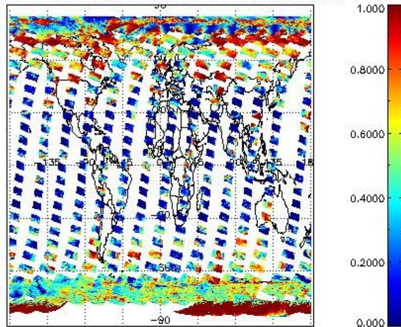
cL_frac for 15MAR2011 00:00:00 to 16MAR2011 00:00:00
