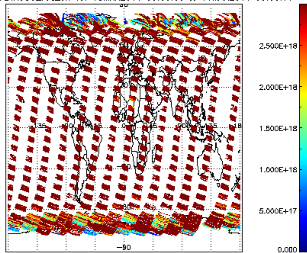
SCIOL2P_NADIR3CO_vcd_err for 15MAR2011 00:00:00 to 16MAR2011 00:00:00
