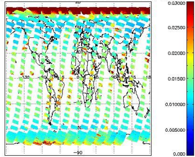
SCIOL2P_NADUV003_vcd_err for 15MAR2011 00:00:00 to 16MAR2011 00:00:00
