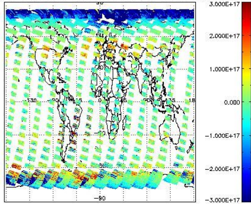
SCIOL2P_NADUV5S02_vcd for 15MAR2011 00:00:00 to 16MAR2011 00:00:00
