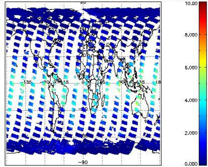
SCIOL2P_NADUV8H2O_vcd for 15MAR2011 00:00:00 to 16MAR2011 00:00:00
