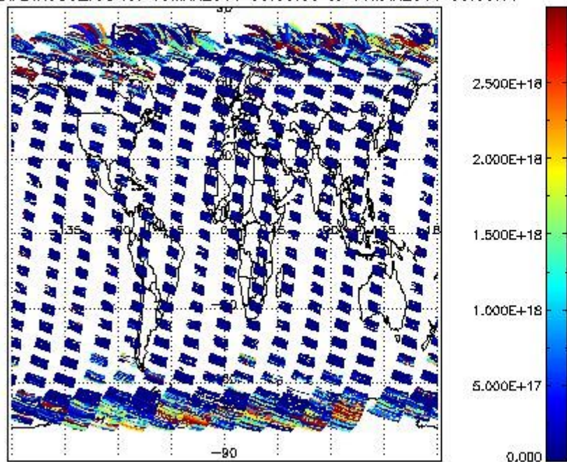
SCIDL2P_NADIR3CO_vcd for 15MAR2011 00:00:00 to 16MAR2011 00:00:00
