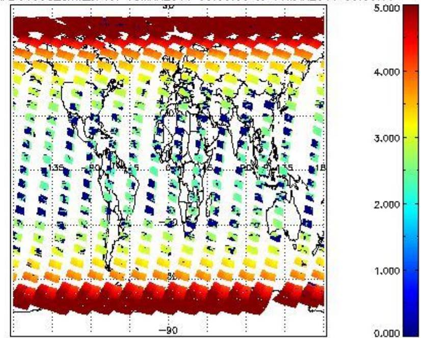
SCIOL2P_NADUV003_amf_cl for 15MAR2011 00:00:00 to 16MAR2011 00:00:00
