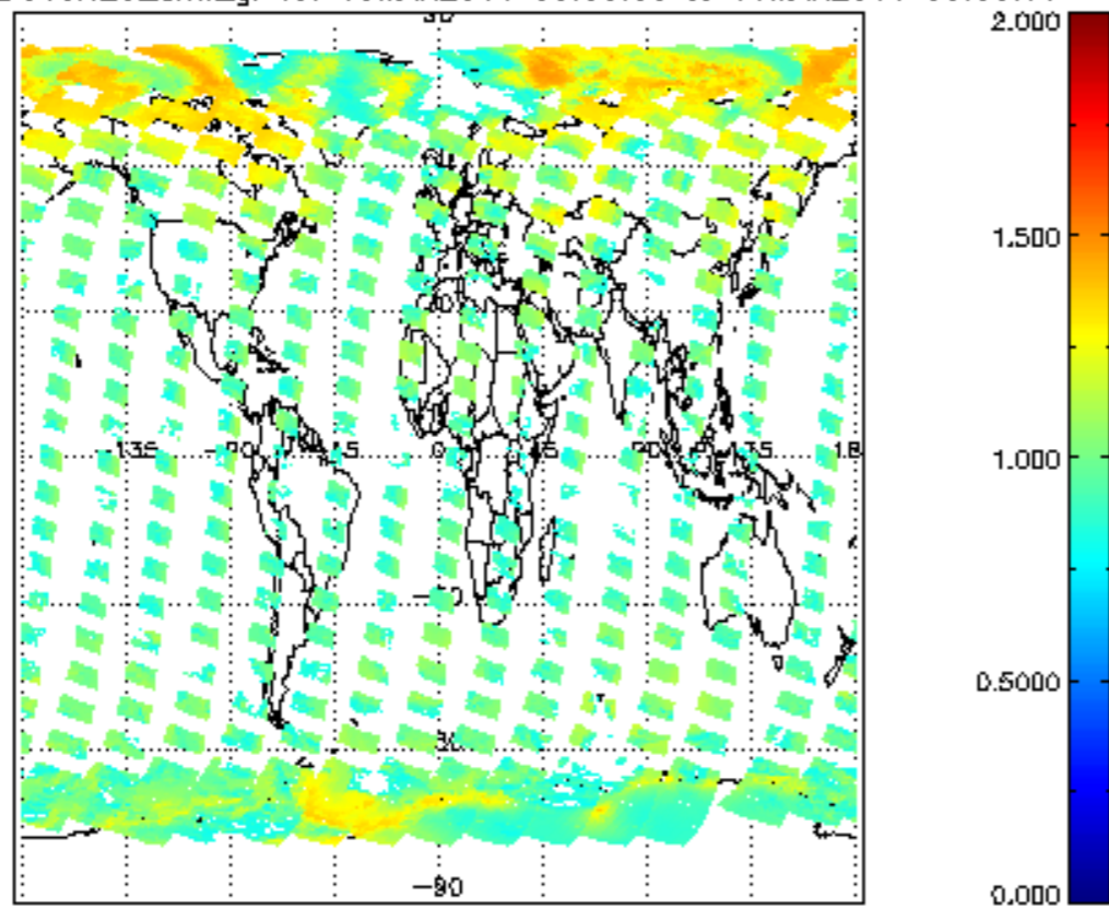
SCIOL2P_NADUV8H20_arnf_gr for 15MAR2011 00:00:00 to 16MAR2011 00:00:00
