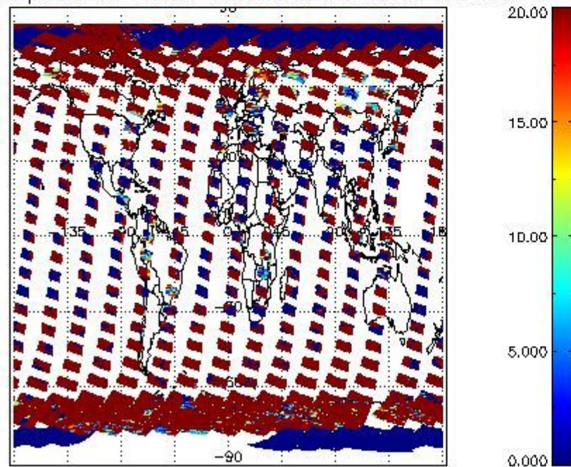
cL_opt_depth for 15MAR2011 00:00:00 to 16MAR2011 00:00:00
