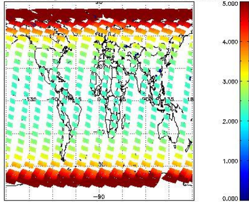
SCIOL2P_NADUV3BRO_amf_gr for 15MAR2011 00:00:00 to 16MAR2011 00:00:00
