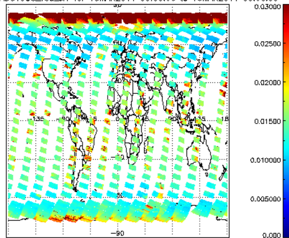
SCIOL2P_NADUV003_vcd_err for 15MAR2011 00:00:00 to 16MAR2011 00:00:00
