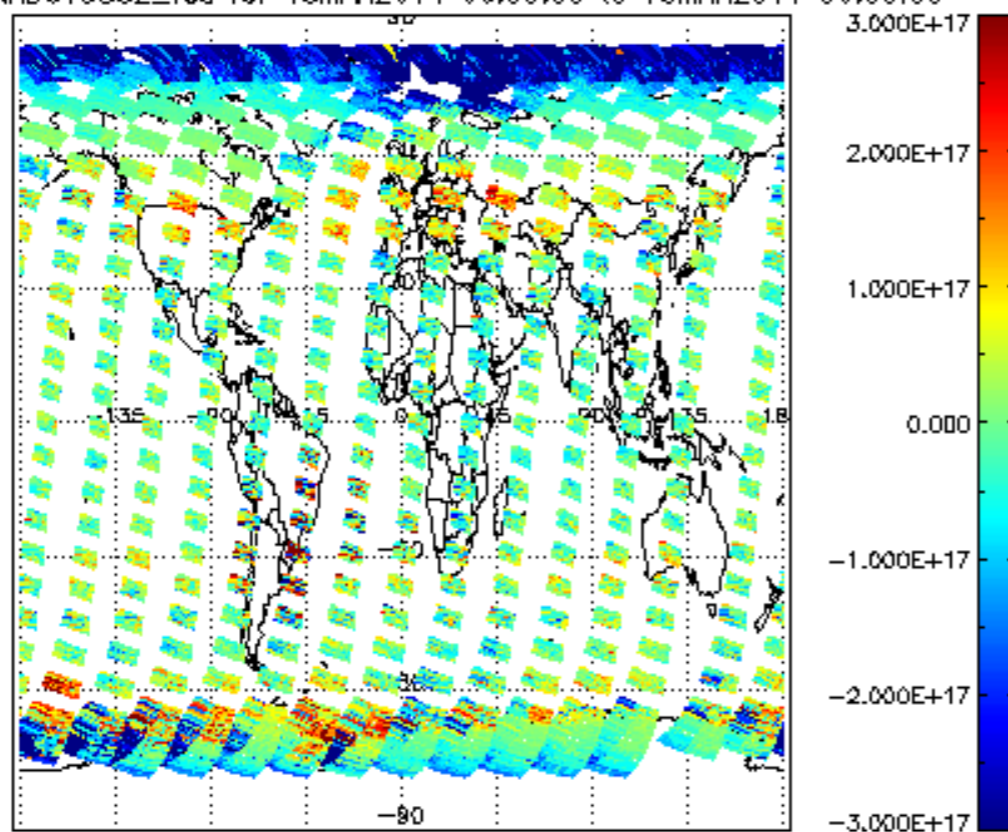
SCIOL2P_NADUV5S02_vcd for 15MAR2011 00:00:00 to 16MAR2011 00:00:00
