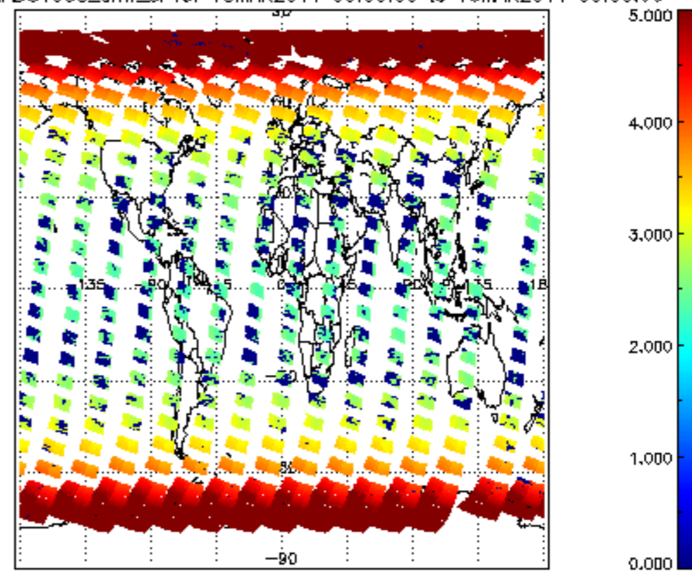
SCIOL2P_NADUV003_arnf_cl for 15MAR2011 00:00:00 to 16MAR2011 00:00:00
