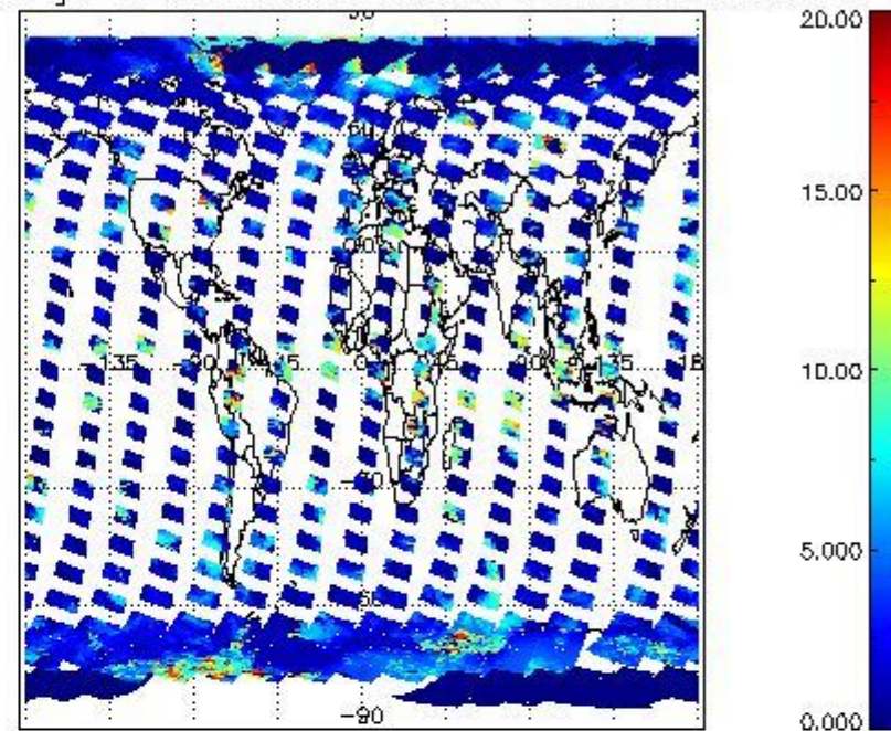
cL_top_height for 15MAR2011 00:00:00 to 16MAR2011 00:00:00
