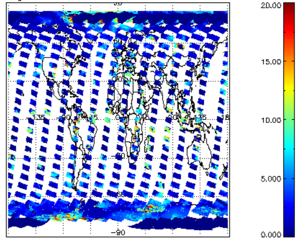
cL_top_height for 15MAR2011 00:00:00 to 16MAR2011 00:00:00
