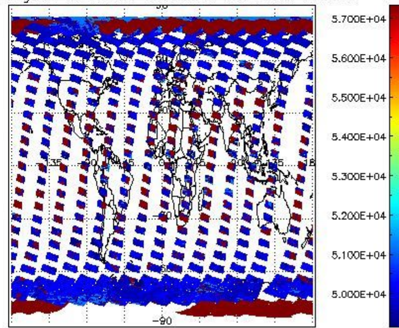
cloud_flags for 15MAR2011 00:00:00 to 16MAR2011 00:00:00
