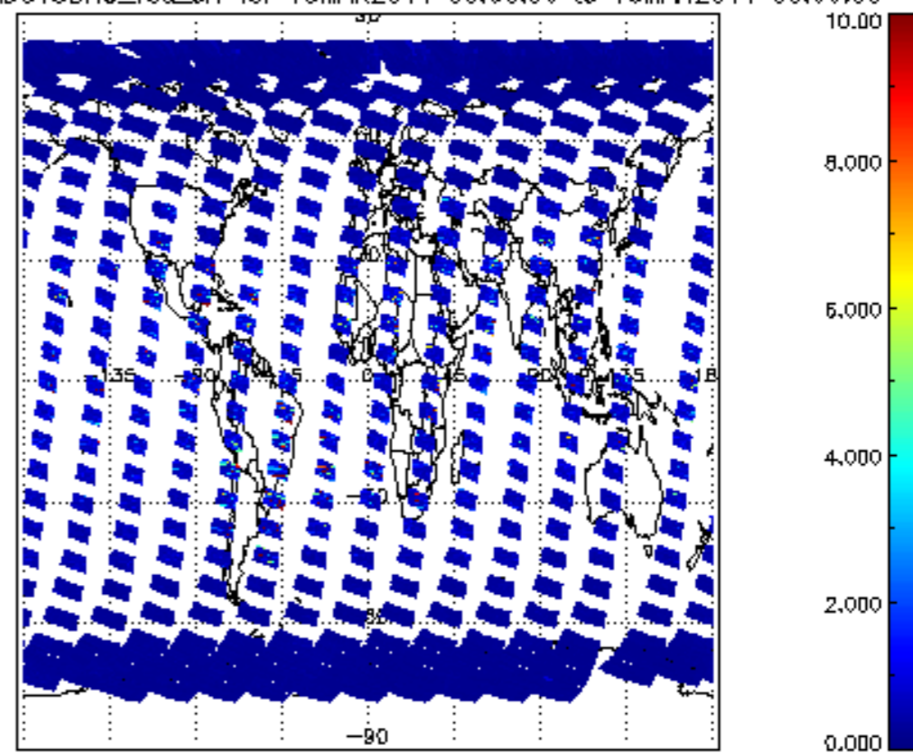
SCIOL2P_NADUV3BRO_vcd_err for 15MAR2011 00:00:00 to 16MAR2011 00:00:00
