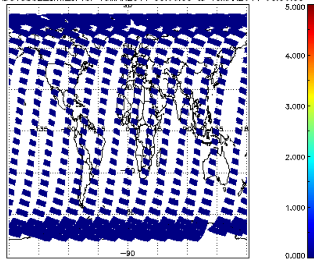
SCIOL2P_NADUV5S02_amf_cl for 15MAR2011 00:00:00 to 16MAR2011 00:00:00
