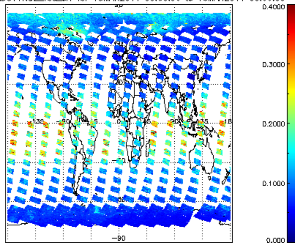
SCIOL2P_NADUV1NO2_vcd_err for 15MAR2011 00:00:00 to 16MAR2011 00:00:00
