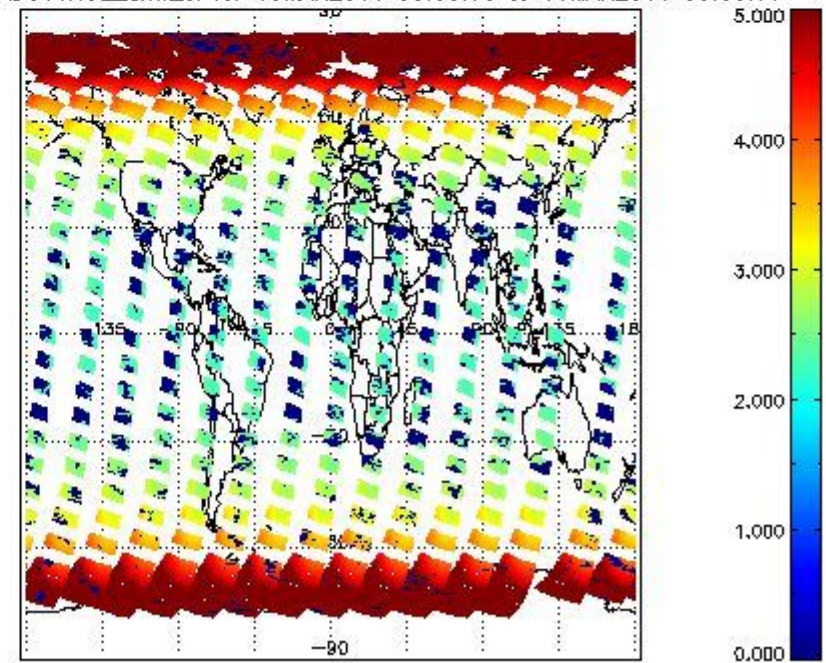
SCIOL2P_NADUV1NO2_amf_cl for 15MAR2011 00:00:00 to 16MAR2011 00:00:00
