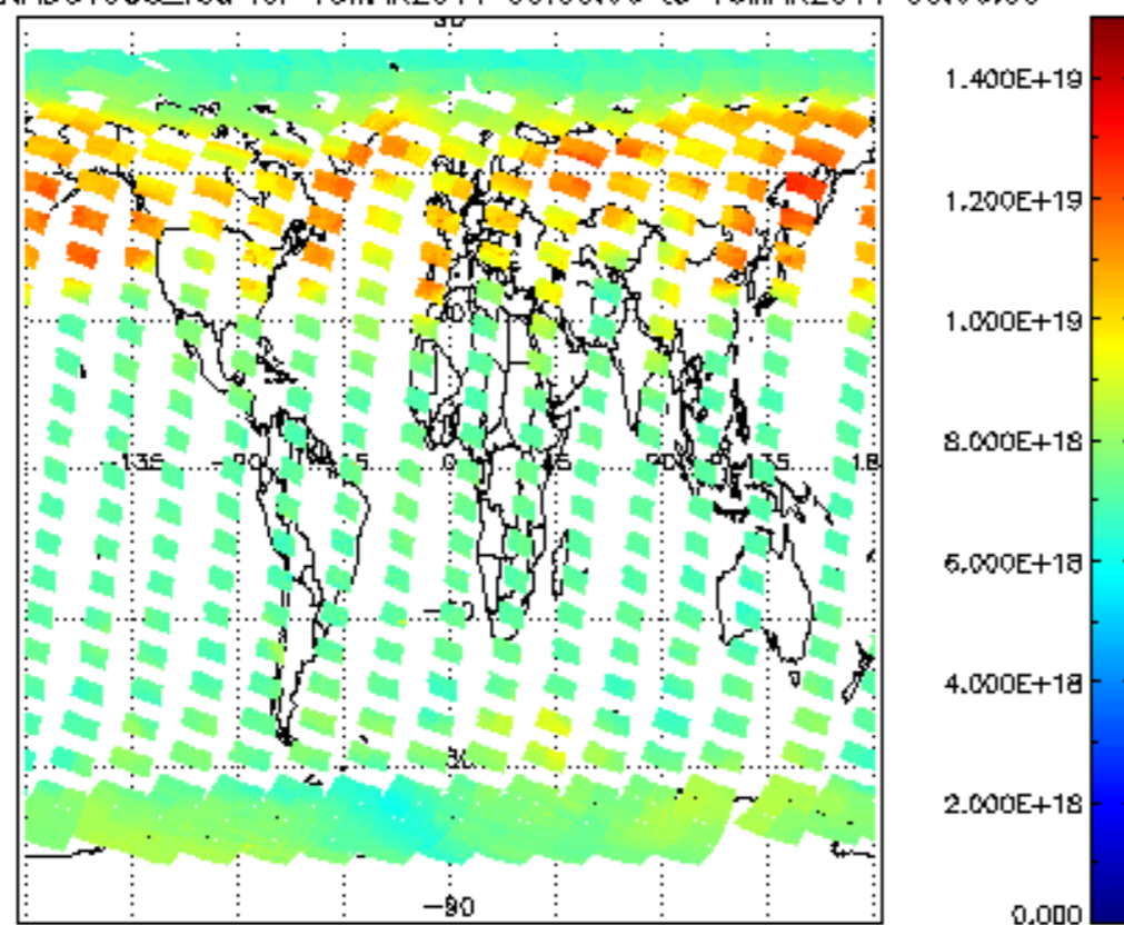
SCIOL2P_NADUV003_vcd for 15MAR2011 00:00:00 to 16MAR2011 00:00:00
