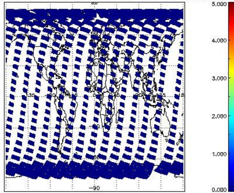
SCIOL2P_NADUV7S02_amf_cl for 15MAR2011 00:00:00 to 16MAR2011 00:00:00
