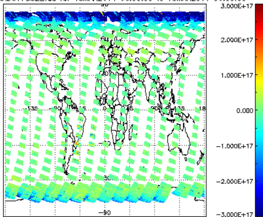
SCIOL2P_NADUV7S02_vcd for 15MAR2011 00:00:00 to 16MAR2011 00:00:00
