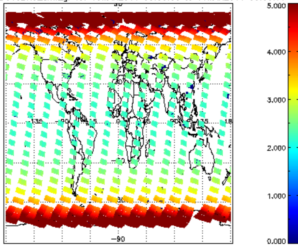
SCIOL2P_NADUV3BRO_amf_gr for 15MAR2011 00:00:00 to 16MAR2011 00:00:00
