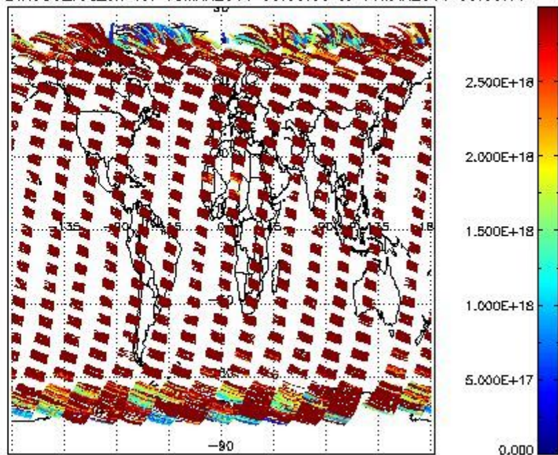
SCIDL2P_NADIR3CO_vcd_err for 15MAR2011 00:00:00 to 16MAR2011 00:00:00
