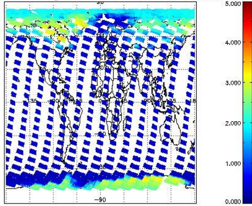
SCIOL2P_NADUV5S02_amf_gr for 15MAR2011 00:00:00 to 16MAR2011 00:00:00
