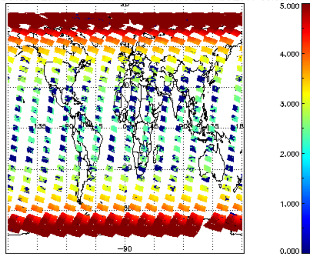
SCIOL2P_NADUV3BRO_amf_cl for 15MAR2011 00:00:00 to 16MAR2011 00:00:00
