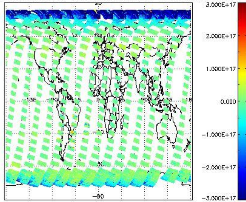
SCIOL2P_NADUV7S02_vcd for 15MAR2011 00:00:00 to 16MAR2011 00:00:00
