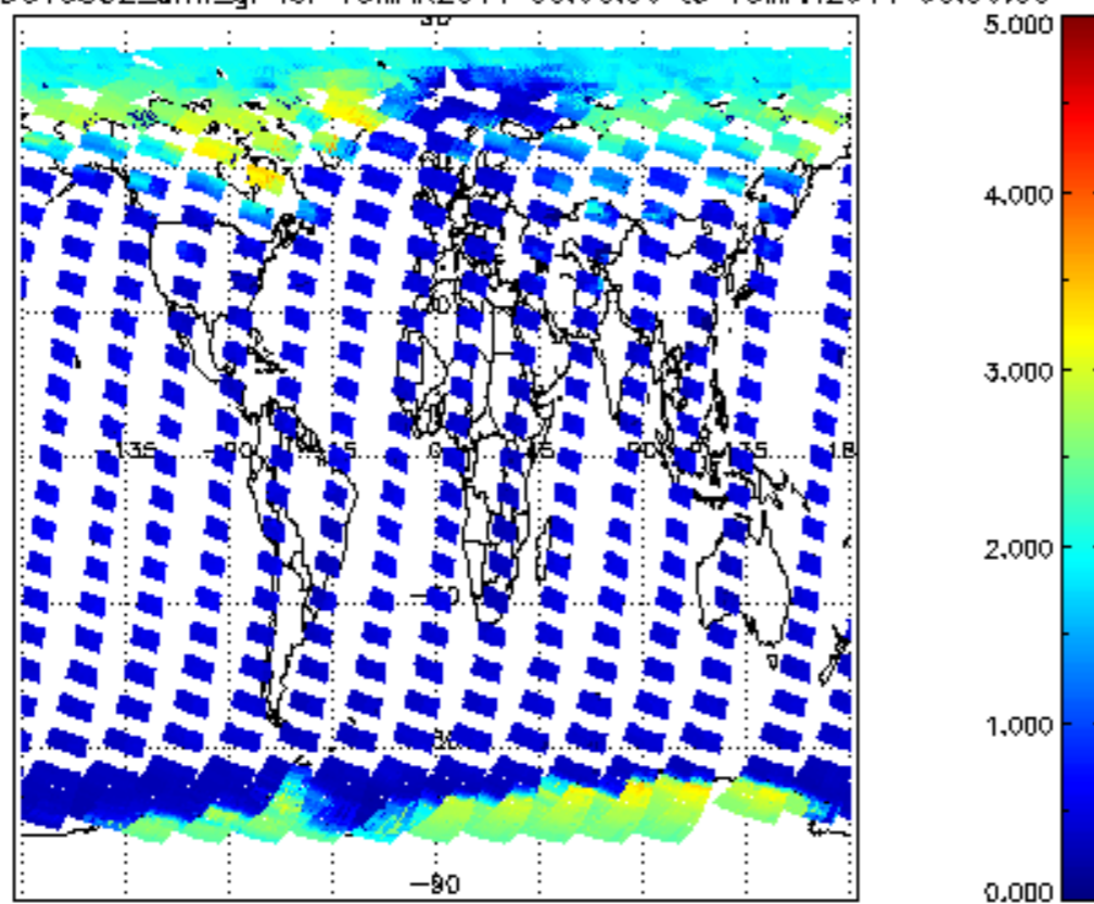
SCIOL2P_NADUV5S02_amf_gr for 15MAR2011 00:00:00 to 16MAR2011 00:00:00
