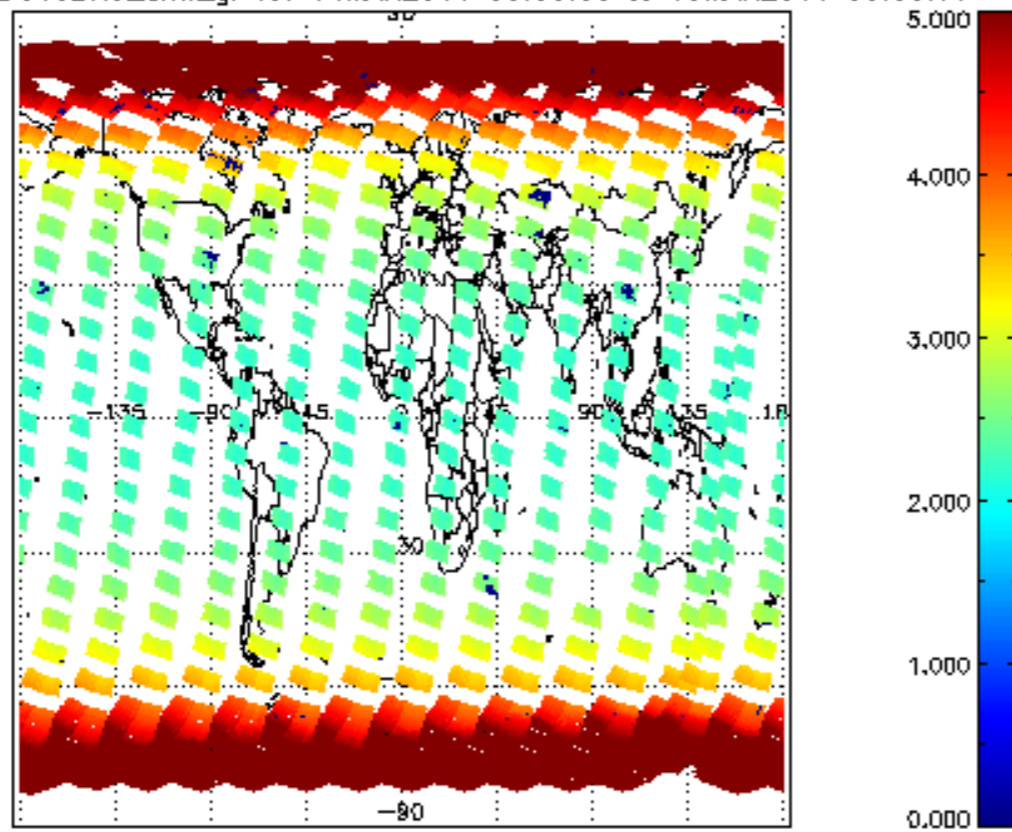
SCIOL2P_NADUV3BRO_amf_gr for 14MAR2011 00:00:00 to 15MAR2011 00:00:00
