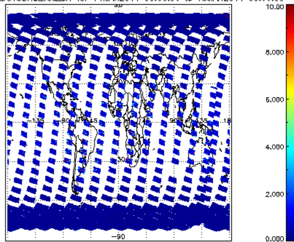
SCIOL2P_NADUV3BRO_vcd_err for 14MAR2011 00:00:00 to 15MAR2011 00:00:00
