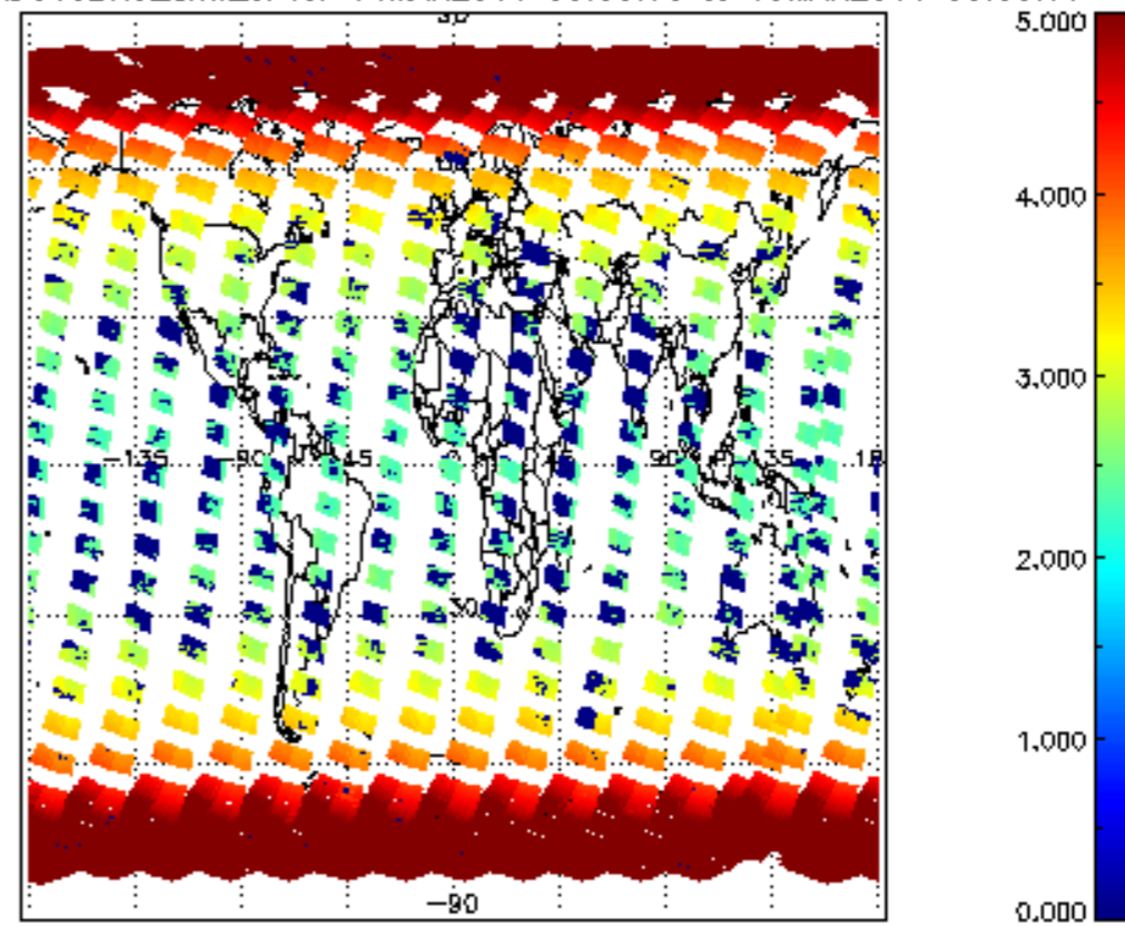
SCIOL2P_NADUV3BRO_amf_cl for 14MAR2011 00:00:00 to 15MAR2011 00:00:00
