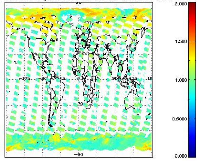
SCIOL2P_NADUV8H2O_amf_gr for 14MAR2011 00:00:00 to 15MAR2011 00:00:00
