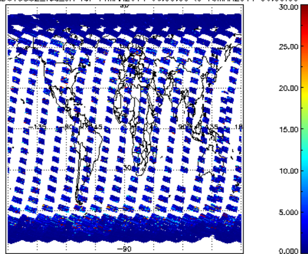
SCIOL2P_NADUV5S02_vcd_err for 14MAR2011 00:00:00 to 15MAR2011 00:00:00
