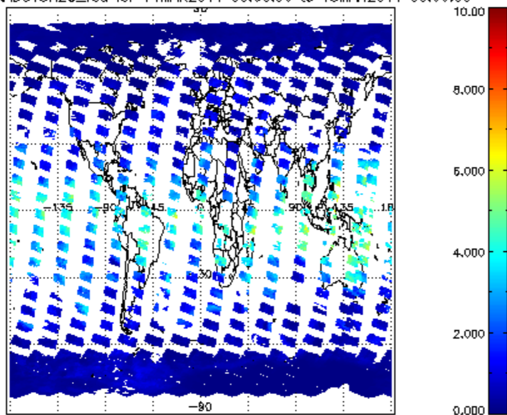
SCIOL2P_NADUV8H2O_vcd for 14MAR2011 00:00:00 to 15MAR2011 00:00:00
