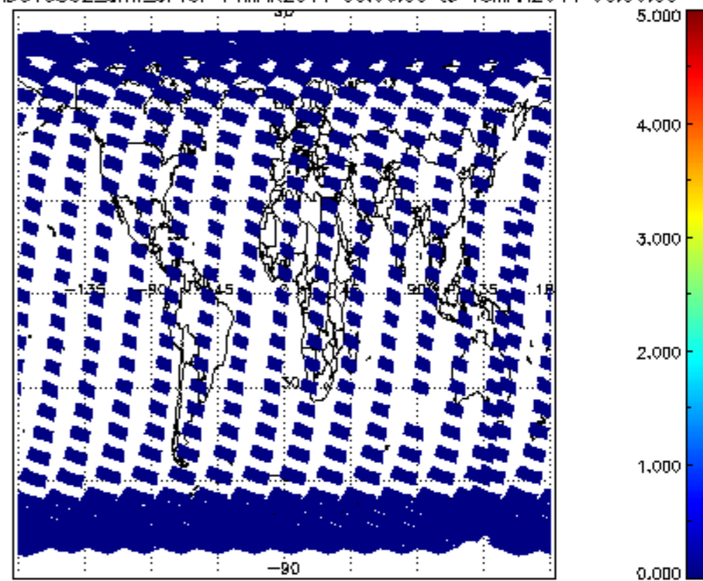
SCIOL2P_NADUV5S02_amf_cl for 14MAR2011 00:00:00 to 15MAR2011 00:00:00
