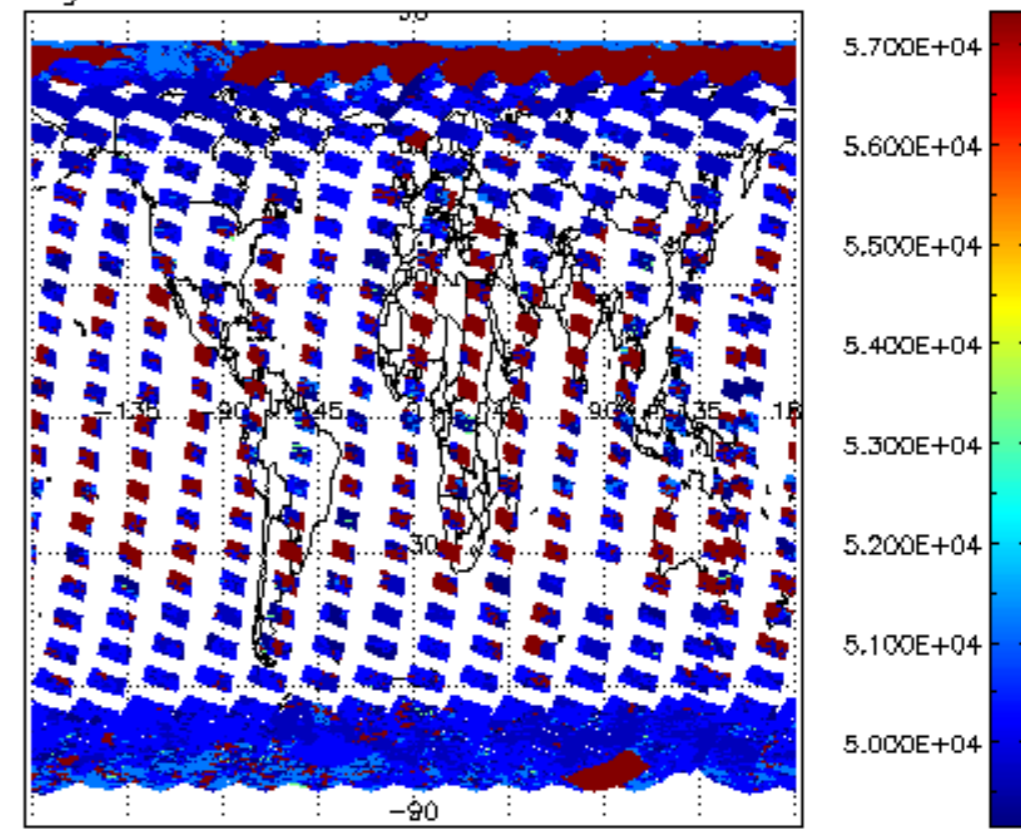
cloud_flags for 14MAR2011 00:00:00 to 15MAR2011 00:00:00
