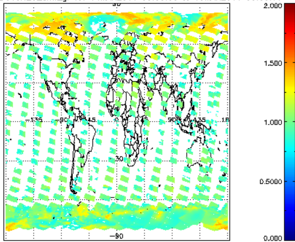
SCIOL2P_NADUV8H2O_arnf_gr for 14MAR2011 00:00:00 to 15MAR2011 00:00:00
