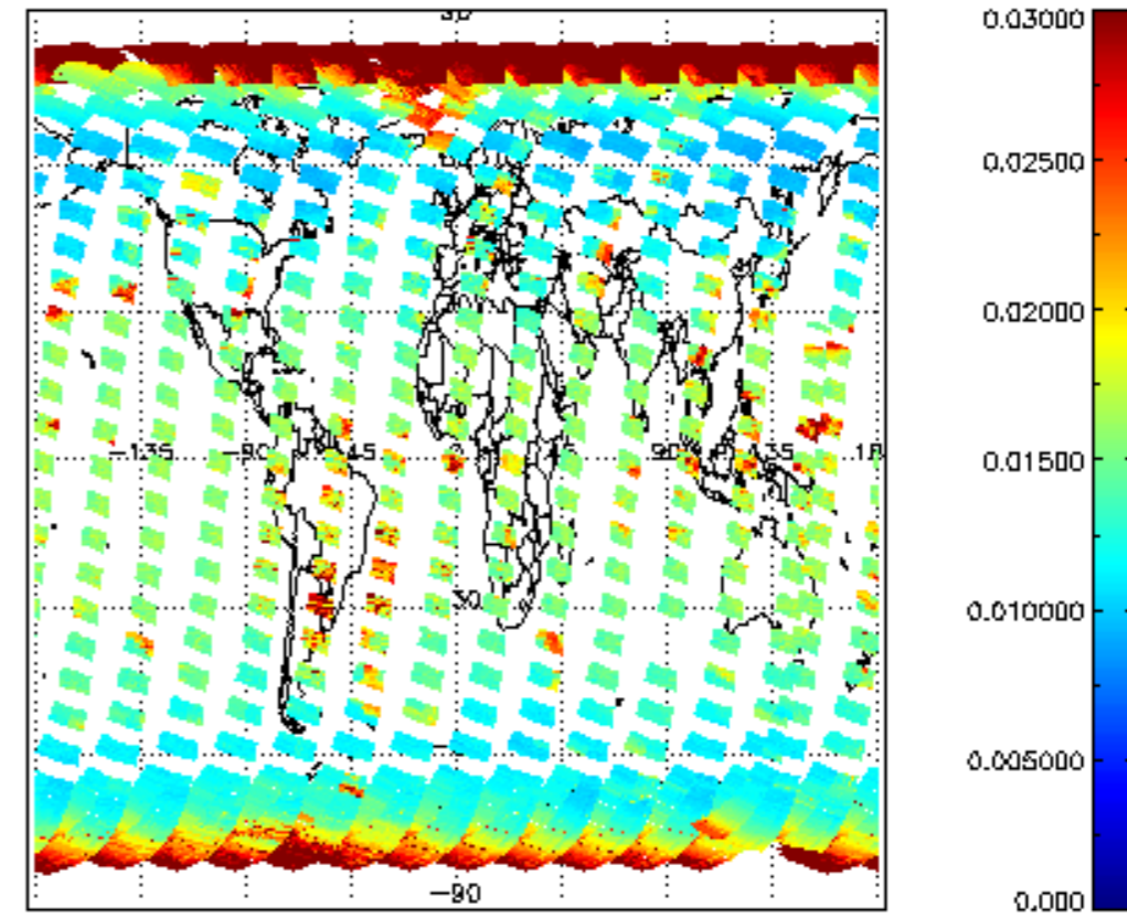
SCIOL2P_NADUV003_vcd_err for 14MAR2011 00:00:00 to 15MAR2011 00:00:00
