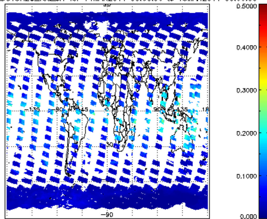
SCIOL2P_NADUV8H2O_vcd_Lerr for 14MAR2011 00:00:00 to 15MAR2011 00:00:00
