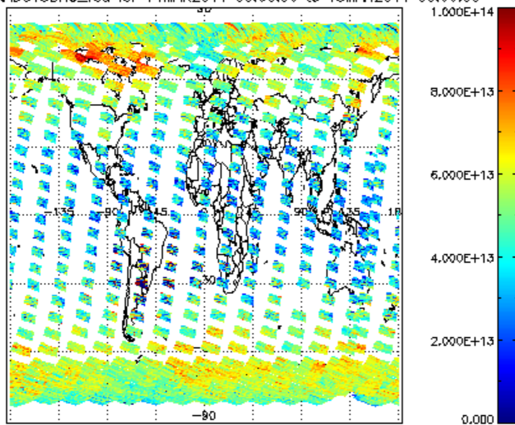
SCIOL2P_NADUV3BRO_vcd for 14MAR2011 00:00:00 to 15MAR2011 00:00:00
