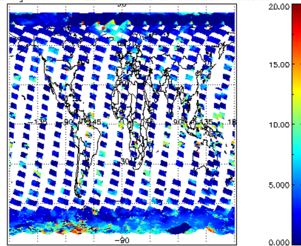
cL_top_height for 14MAR2011 00:00:00 to 15MAR2011 00:00:00
