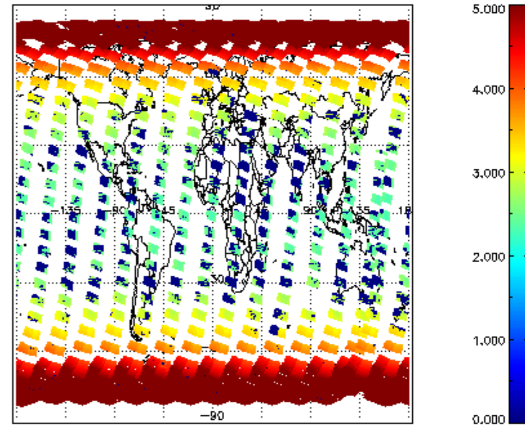
SCIOL2P_NADUV003_amf_cl for 14MAR2011 00:00:00 to 15MAR2011 00:00:00
